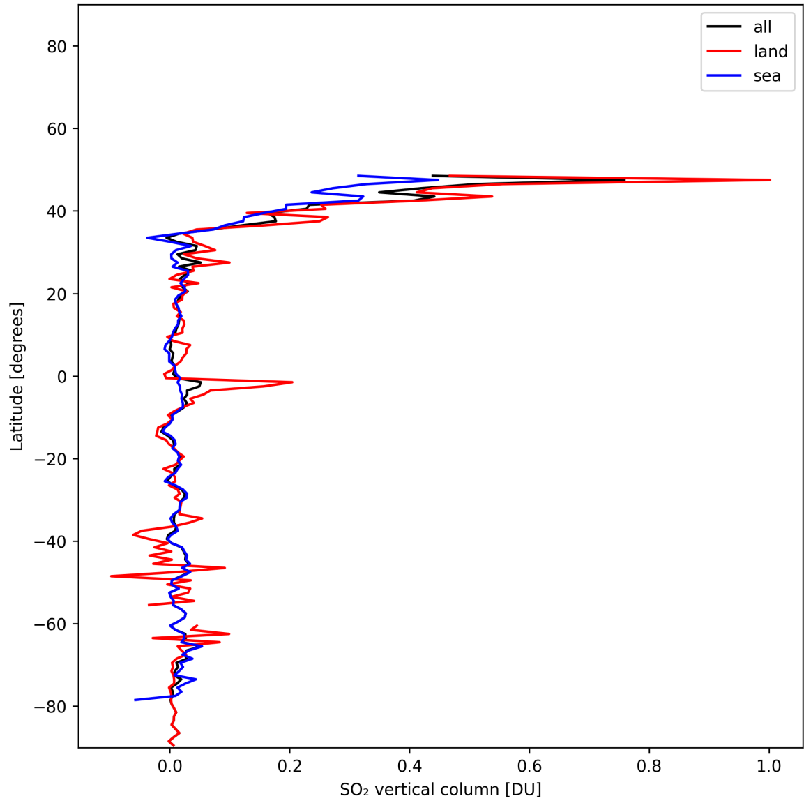
Figure 31: Zonal average of “SO 2 vertical column” for 2025-01-12 to 2025-01-13.
