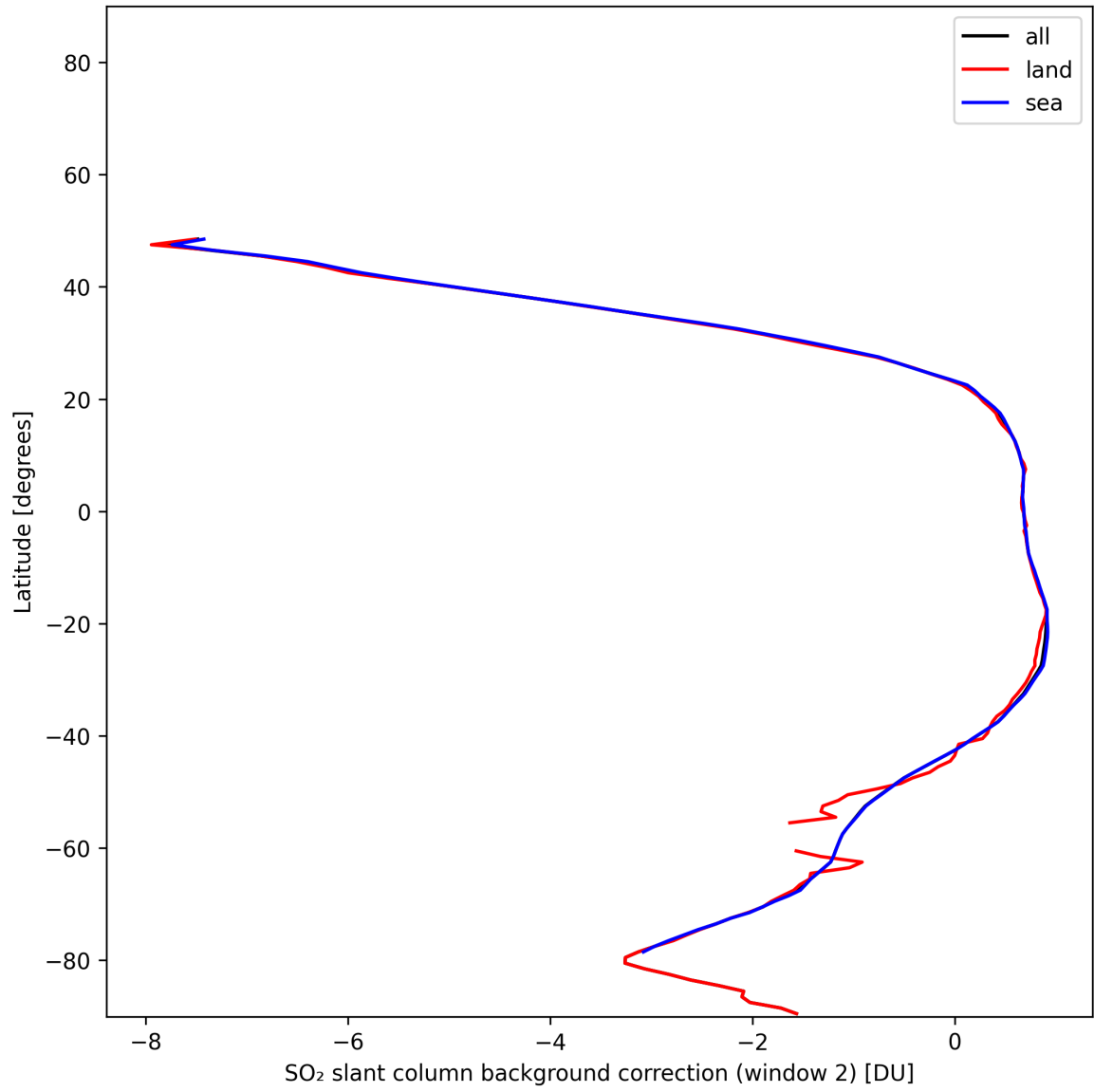
Figure 43: Zonal average of “SO 2 slant column background correction (window 2)” for 2025-01-12 to 2025-01-13.
