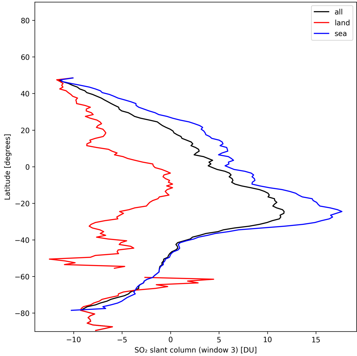
Figure 44: Zonal average of “SO 2 slant column (window 3)” for 2025-01-12 to 2025-01-13.
