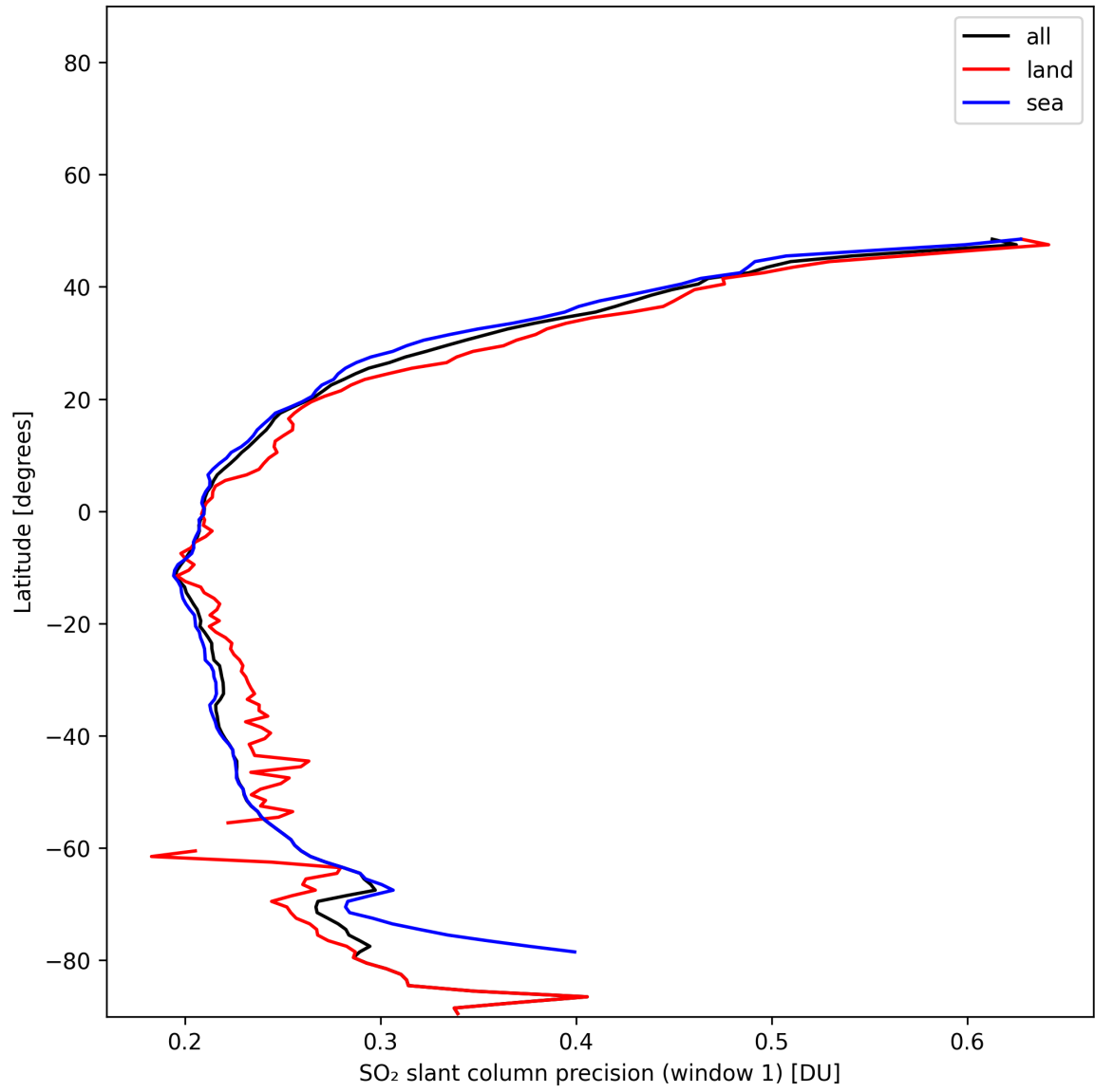
Figure 37: Zonal average of “SO 2 slant column precision (window 1)” for 2025-01-12 to 2025-01-13.
