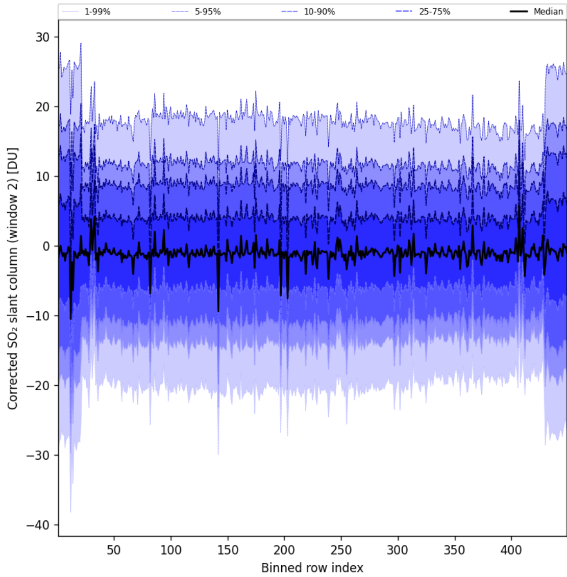
Figure 96: Along track statistics of “Corrected SO 2 slant column (window 2)” for 2025-01-12 to 2025-01-13
