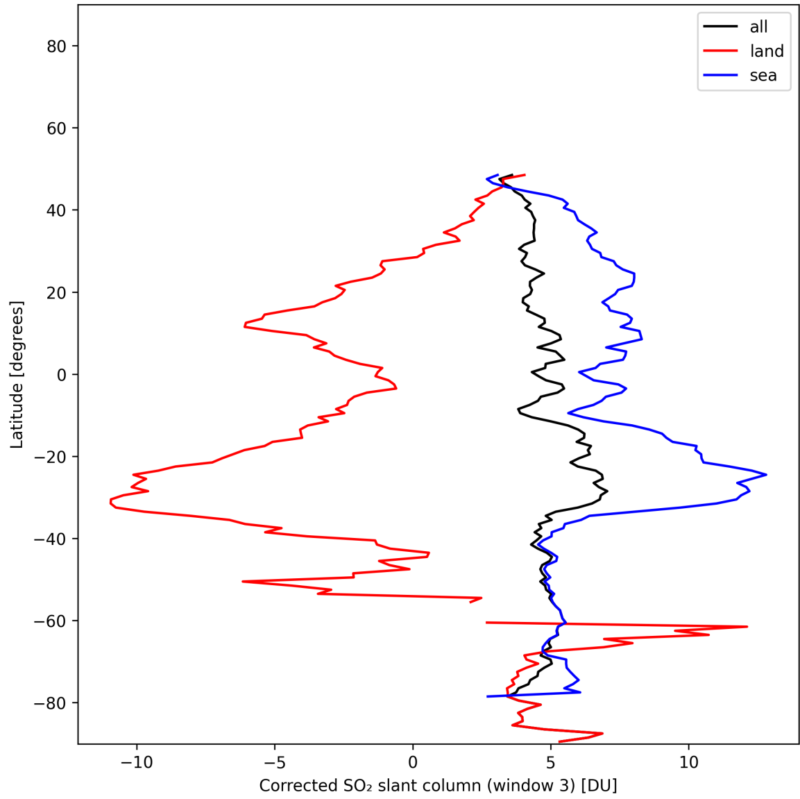
Figure 46: Zonal average of “Corrected SO 2 slant column (window 3)” for 2025-01-12 to 2025-01-13.
