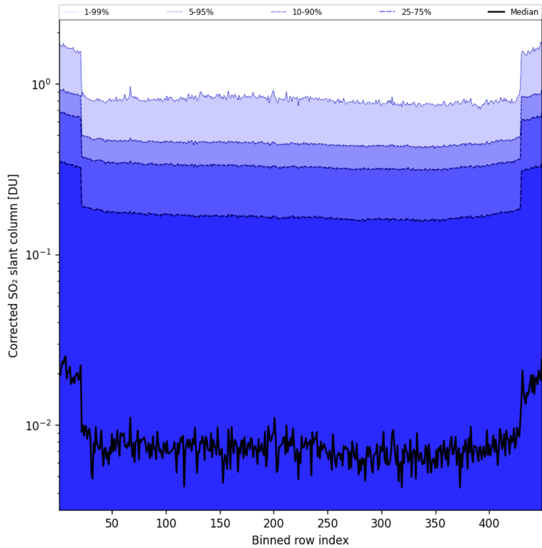
Figure 87: Along track statistics of "Corrected SO 2 slant column" for 2025-01-12 to 2025-01-13
