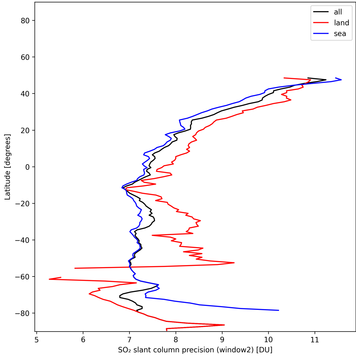
Figure 41: Zonal average of “SO 2 slant column precision (window2)” for 2025-01-12 to 2025-01-13.
