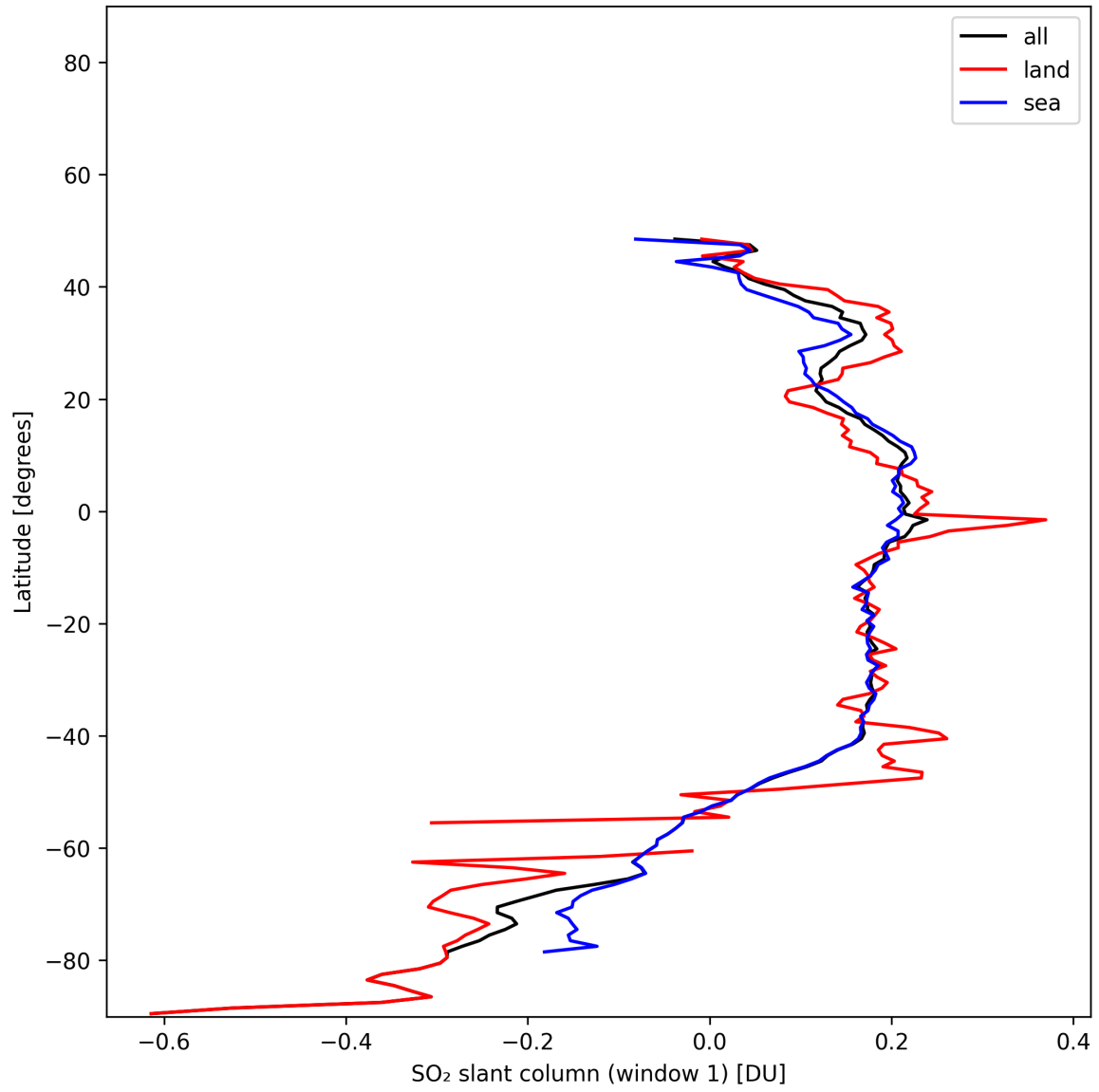
Figure 36: Zonal average of “SO 2 slant column (window 1)” for 2025-01-12 to 2025-01-13.
