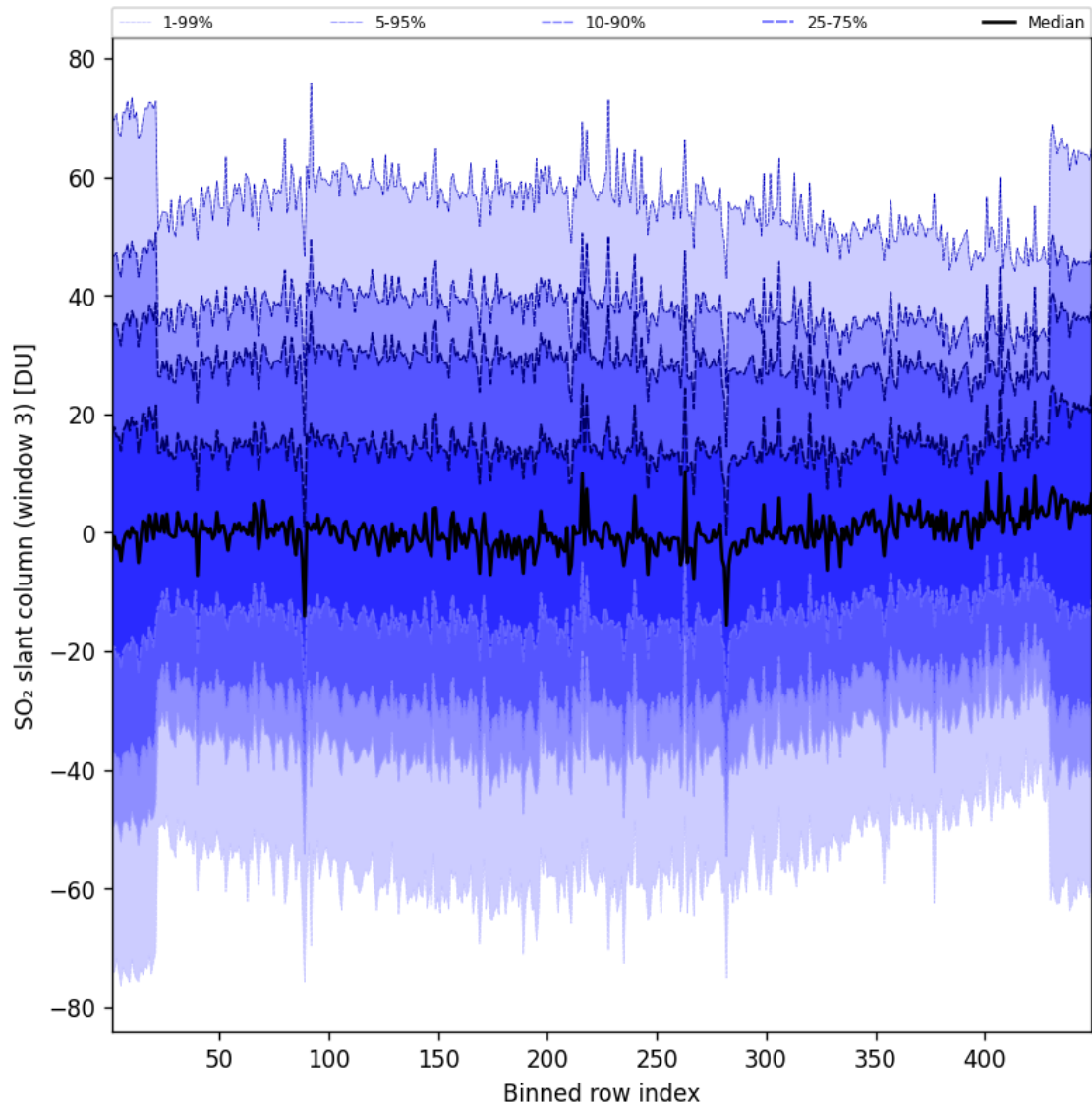
Figure 98: Along track statistics of “SO 2 slant column (window 3)” for 2025-01-12 to 2025-01-13
