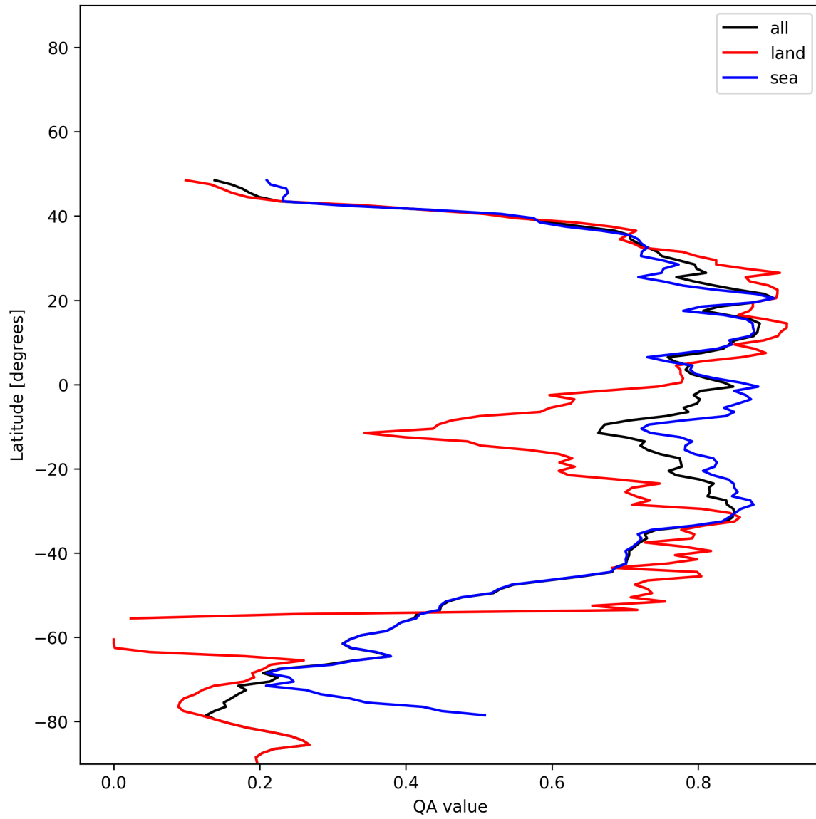
Figure 30: Zonal average of “QA value” for 2025-01-12 to 2025-01-13.
