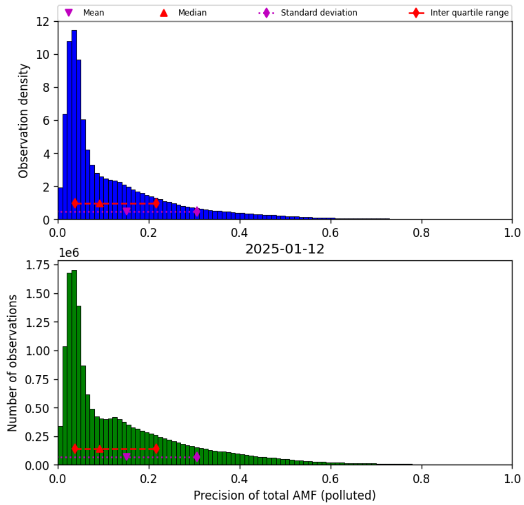
Figure 81: Histogram of “Precision of total AMF (polluted)” for 2025-01-12 to 2025-01-13
