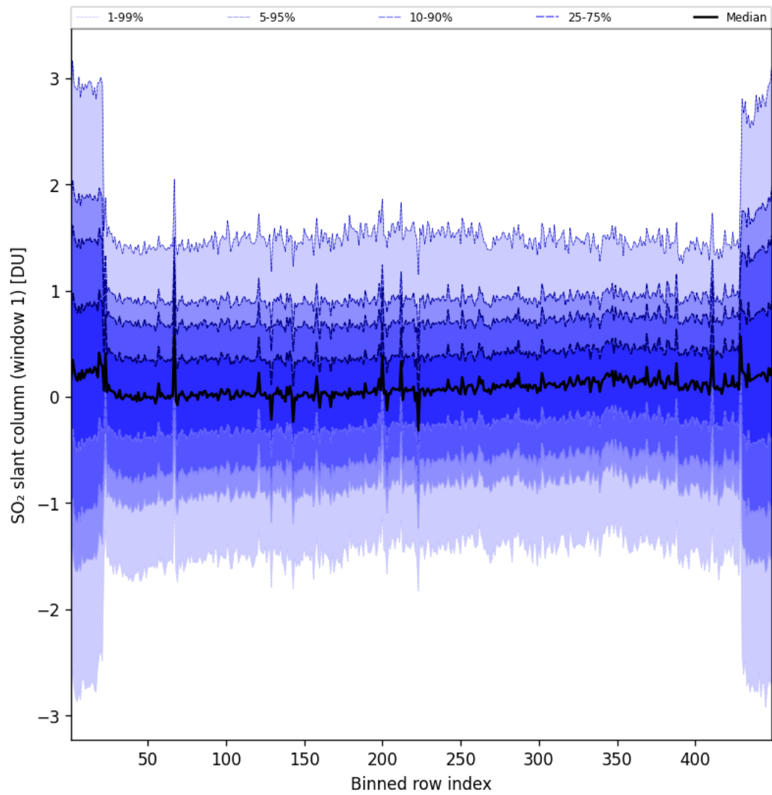
Figure 90: Along track statistics of “SO 2 slant column (window 1)” for 2025-01-12 to 2025-01-13
