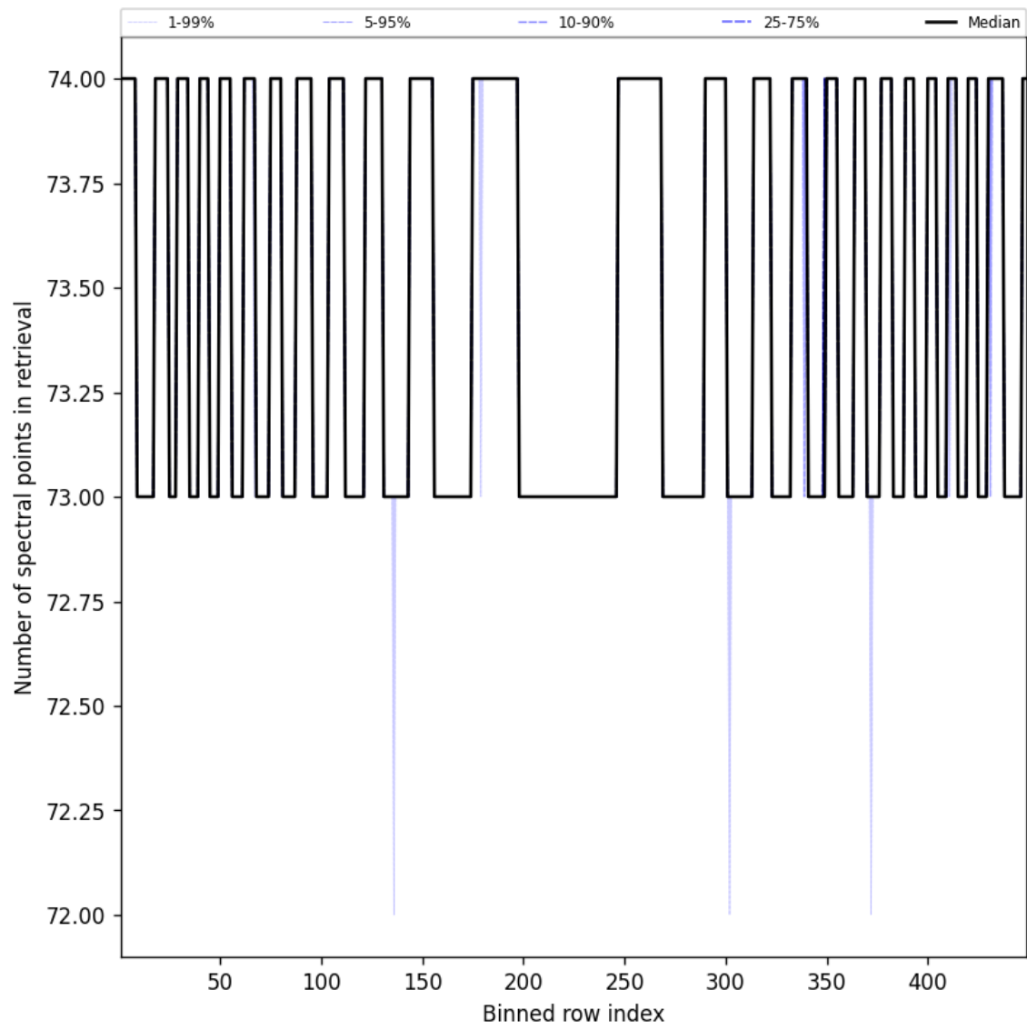
Figure 110: Along track statistics of “Number of spectral points in retrieval” for 2025-01-12 to 2025-01-13
