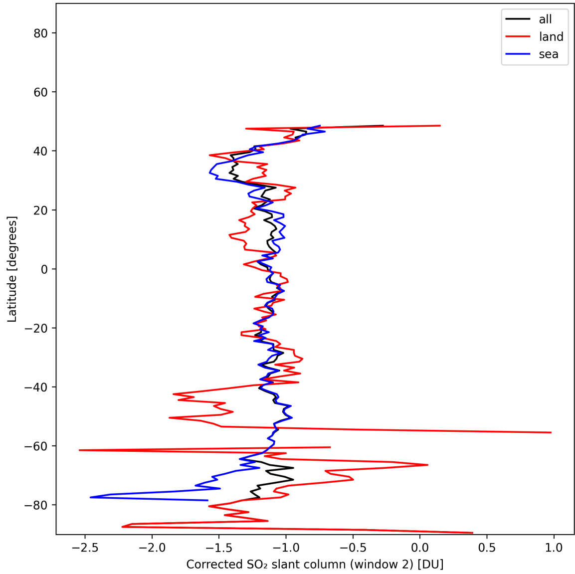
Figure 42: Zonal average of “Corrected SO 2 slant column (window 2)” for 2025-01-12 to 2025-01-13.
