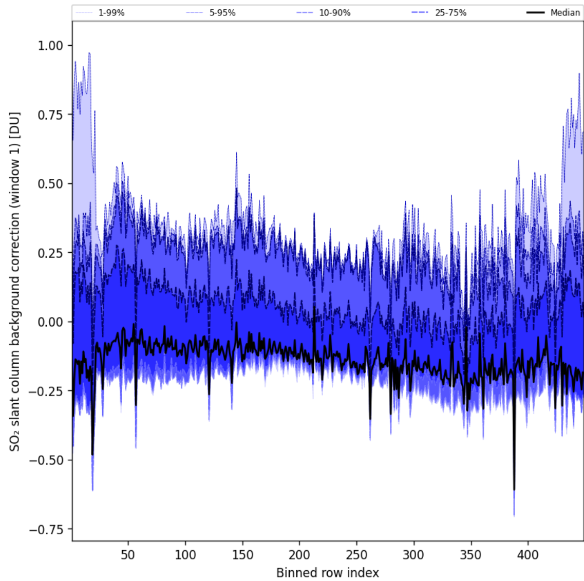
Figure 93: Along track statistics of “SO 2 slant column background correction (window 1)” for 2025-01-12 to 2025-01-13
