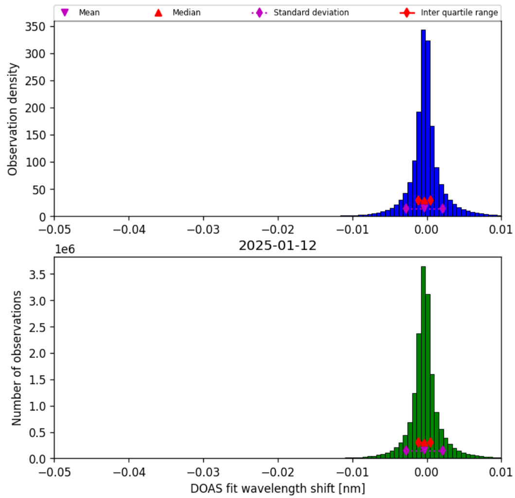
Figure 77: Histogram of “DOAS fit wavelength shift” for 2025-01-12 to 2025-01-13
