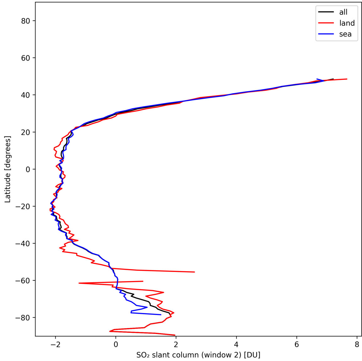
Figure 40: Zonal average of “SO 2 slant column (window 2)” for 2025-01-12 to 2025-01-13.
