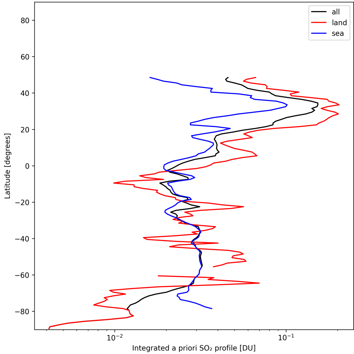
Figure 49: Zonal average of “Integrated a priori SO 2 profile” for 2025-01-12 to 2025-01-13.
