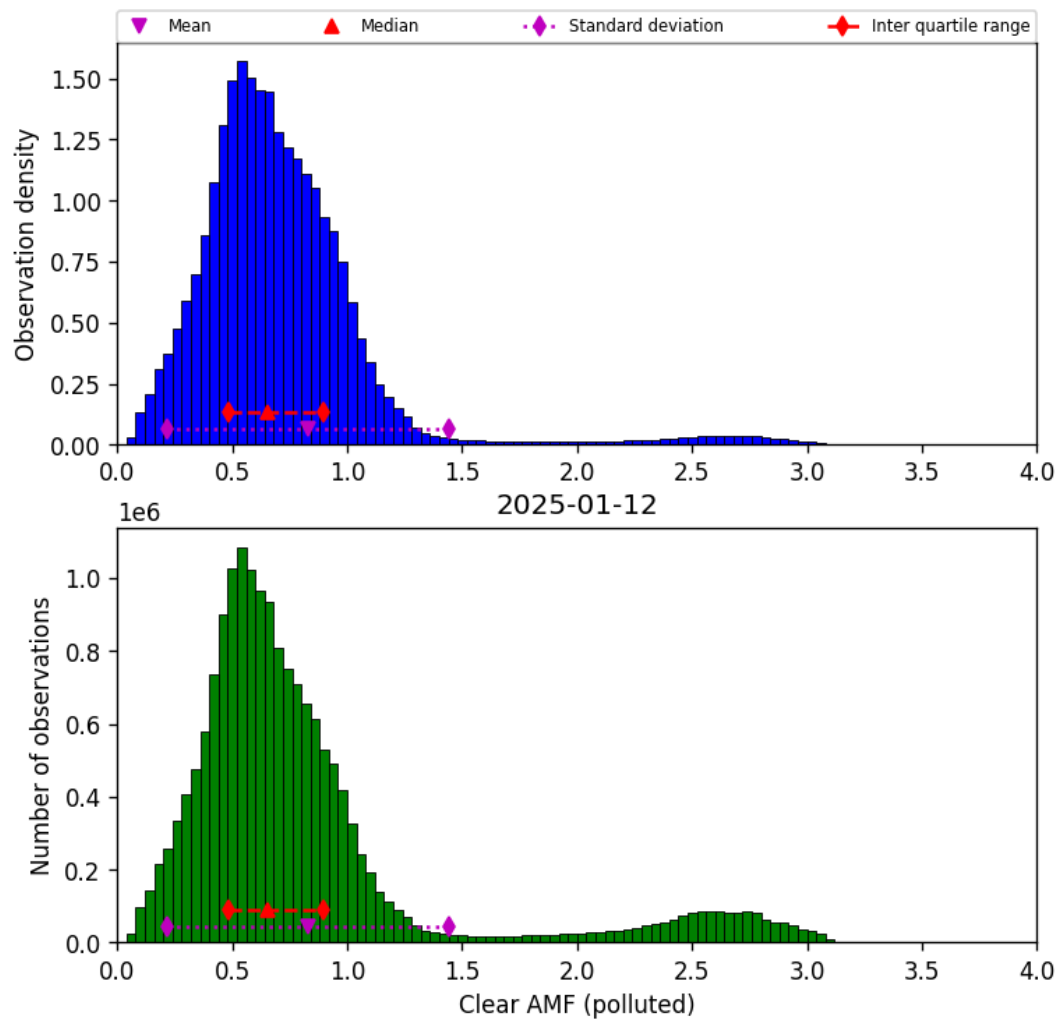
Figure 82: Histogram of “Clear AMF (polluted)” for 2025-01-12 to 2025-01-13
