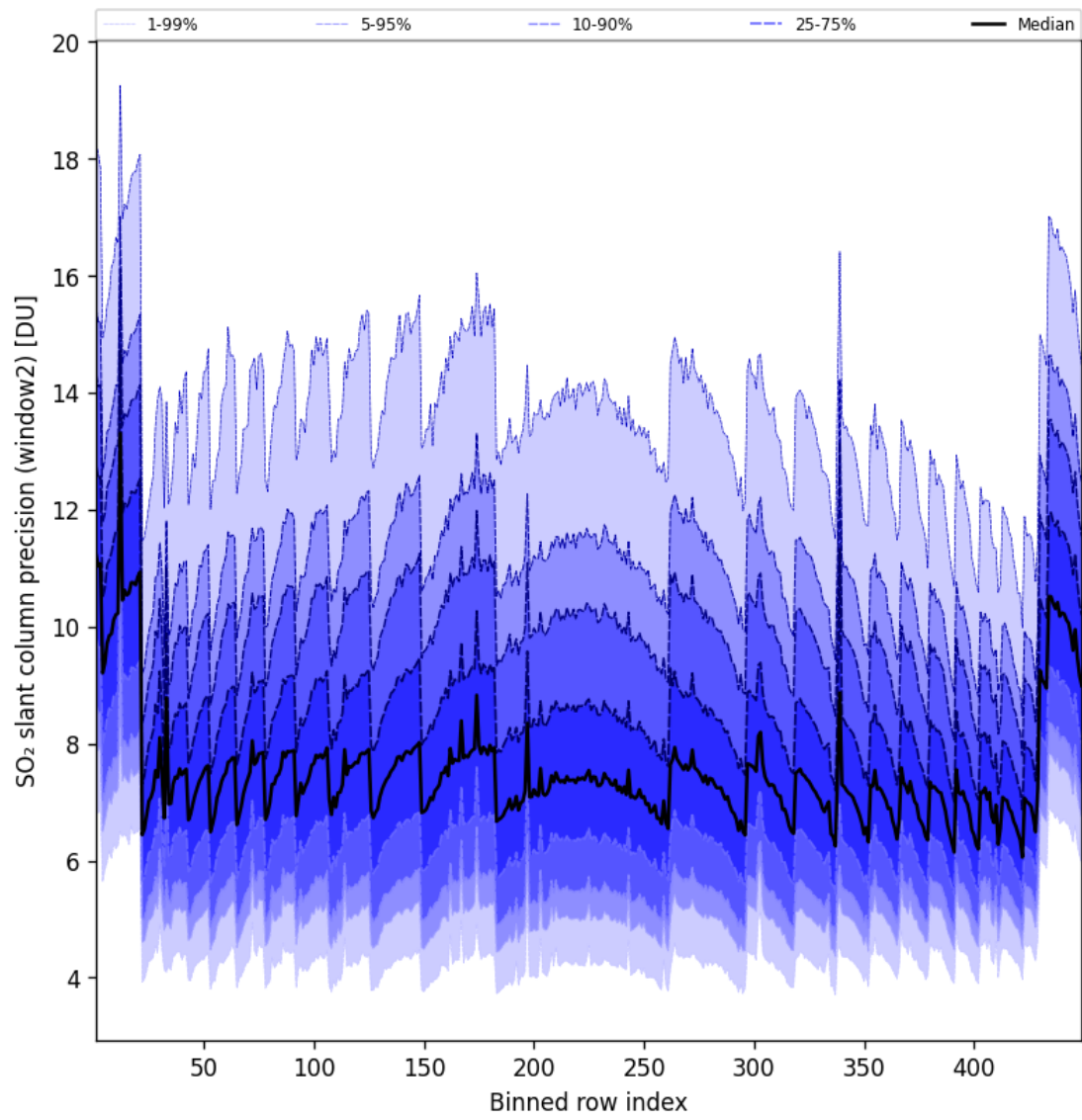
Figure 95: Along track statistics of “SO 2 slant column precision (window2)” for 2025-01-12 to 2025-01-13
