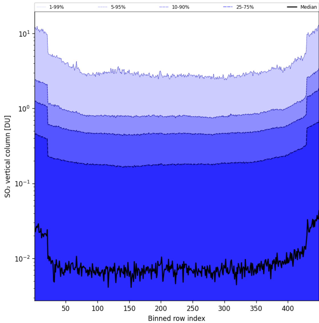
Figure 85: Along track statistics of “SO 2 vertical column” for 2025-01-12 to 2025-01-13
