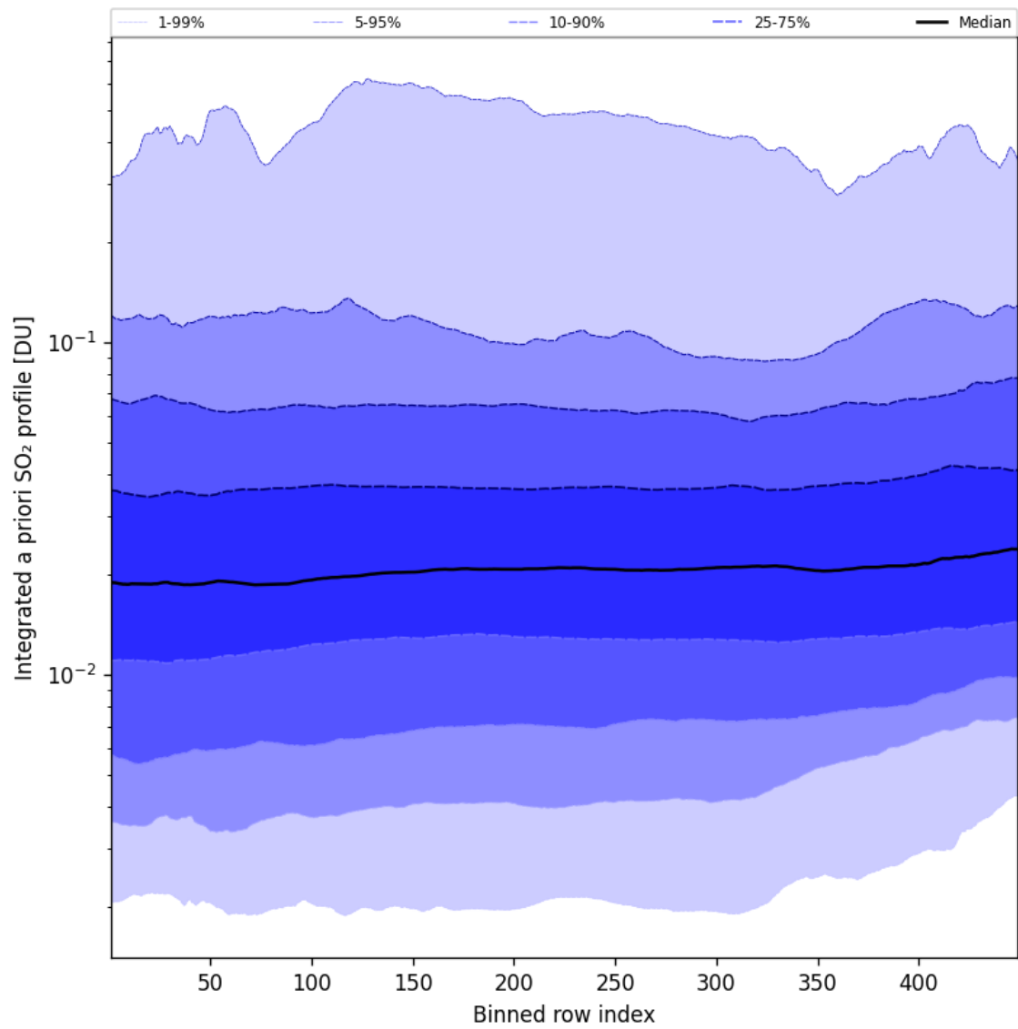
Figure 103: Along track statistics of “Integrated a priori SO 2 profile” for 2025-01-12 to 2025-01-13
