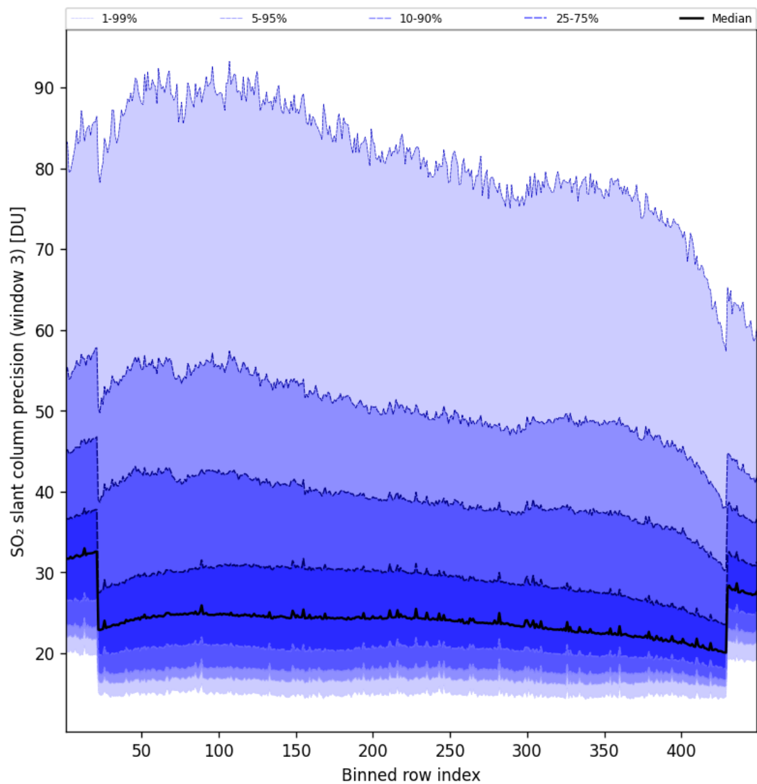
Figure 99: Along track statistics of “SO 2 slant column precision (window 3)” for 2025-01-12 to 2025-01-13
