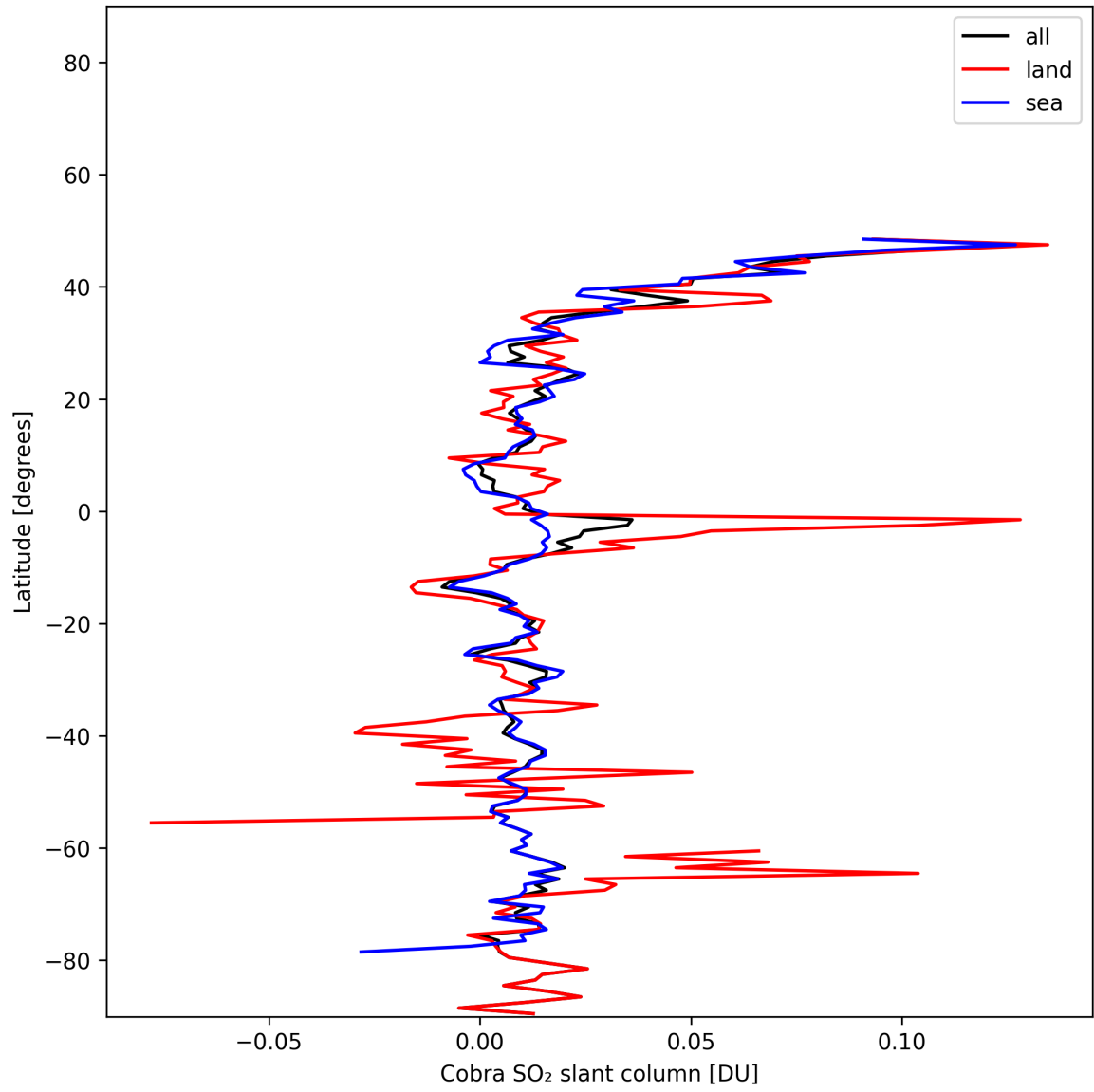
Figure 34: Zonal average of “Cobra SO 2 slant column” for 2025-01-12 to 2025-01-13.
