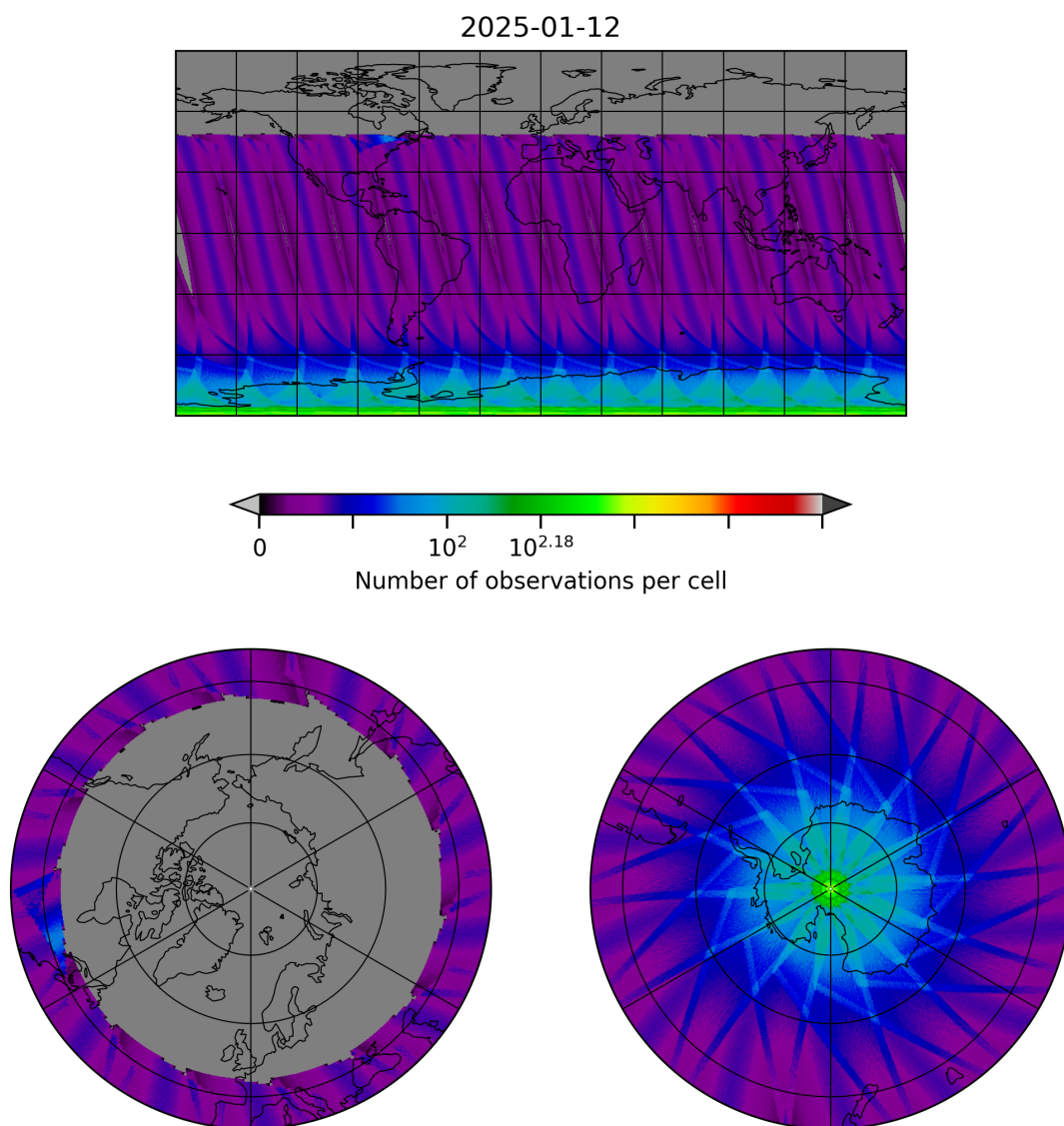
Figure 29: Map of the number of observations for 2025-01-12 to 2025-01-13
