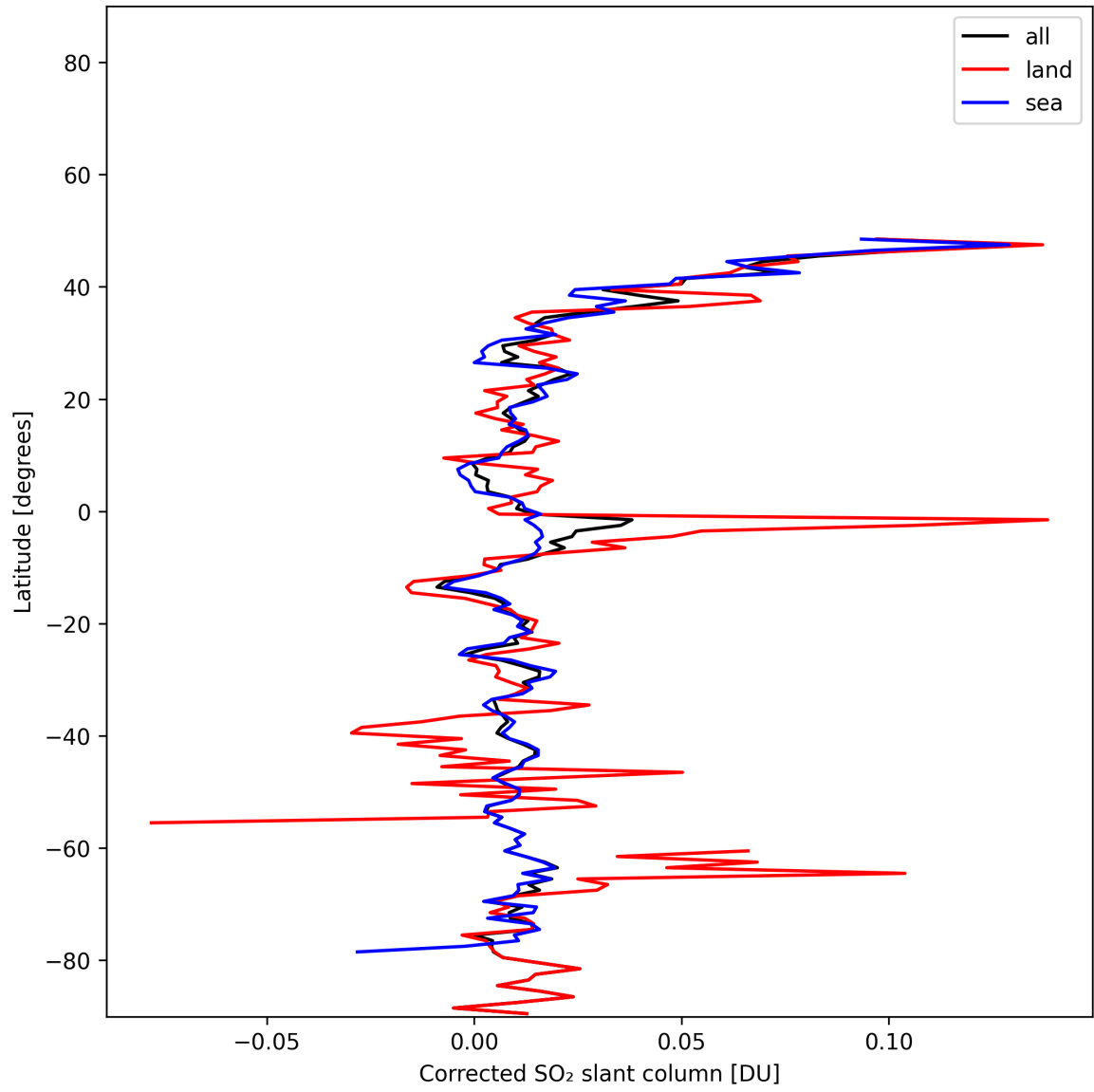
Figure 33: Zonal average of "Corrected SO 2 slant column" for 2025-01-12 to 2025-01-13.
