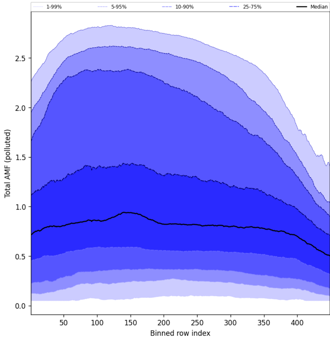
Figure 107: Along track statistics of “Total AMF (polluted)” for 2025-01-12 to 2025-01-13
