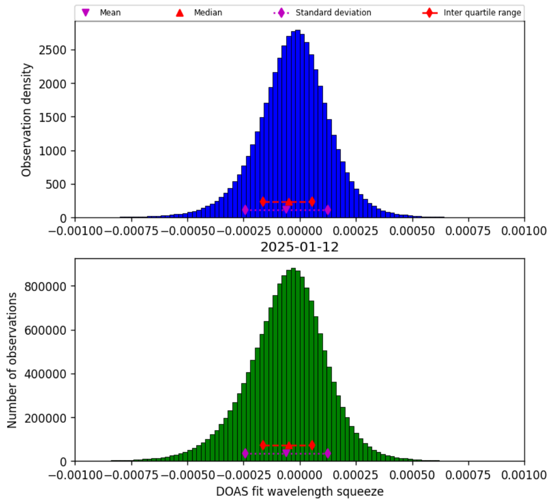
Figure 78: Histogram of “DOAS fit wavelength squeeze” for 2025-01-12 to 2025-01-13
