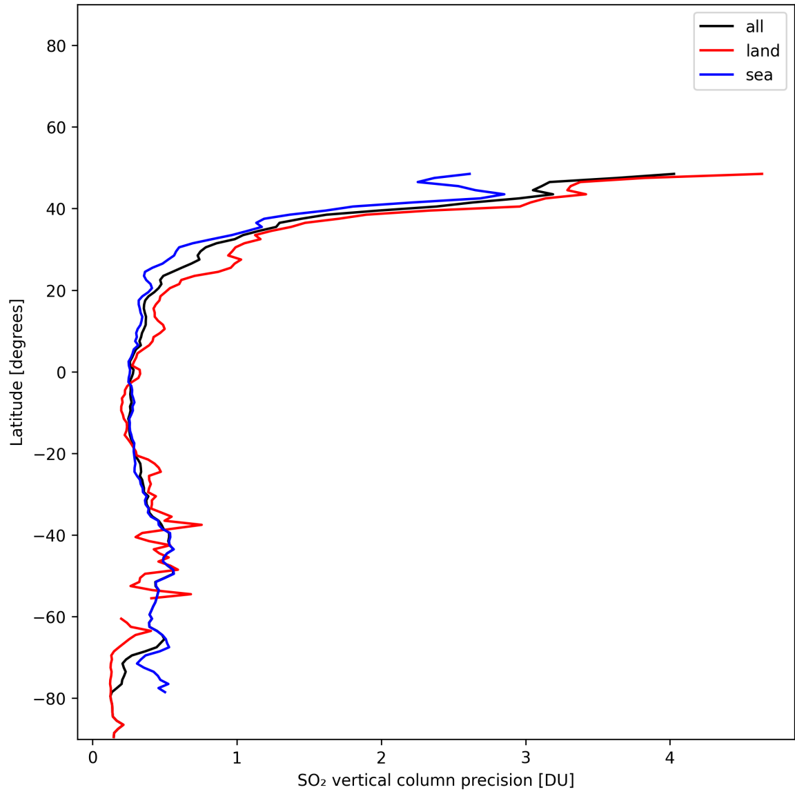
Figure 32: Zonal average of “SO 2 vertical column precision” for 2025-01-12 to 2025-01-13.
