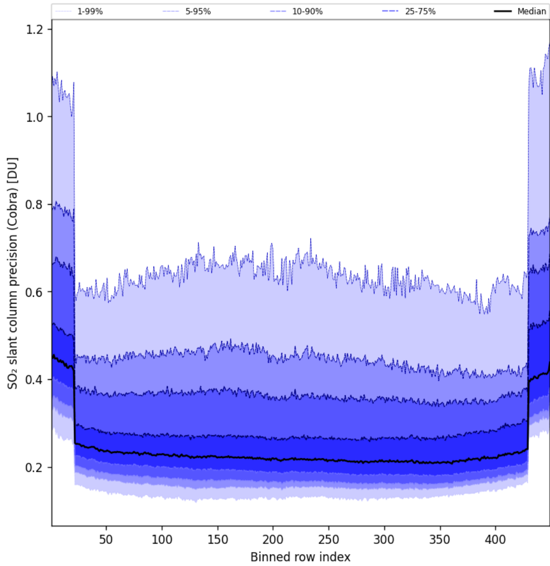
Figure 89: Along track statistics of “SO 2 slant column precision (Cobra)” for 2025-01-12 to 2025-01-13
