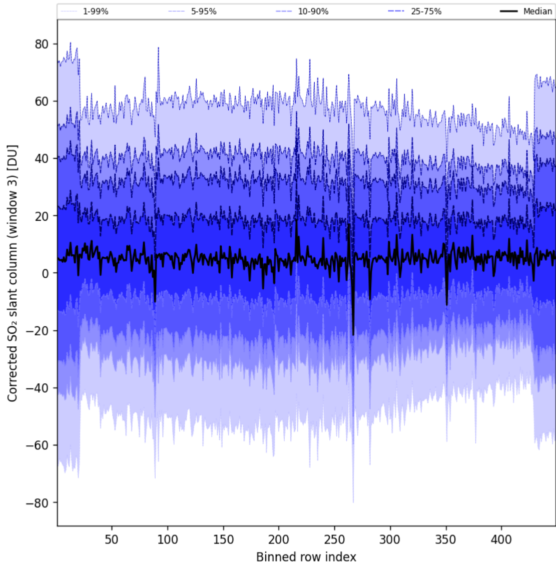
Figure 100: Along track statistics of “Corrected SO 2 slant column (window 3)” for 2025-01-12 to 2025-01-13
