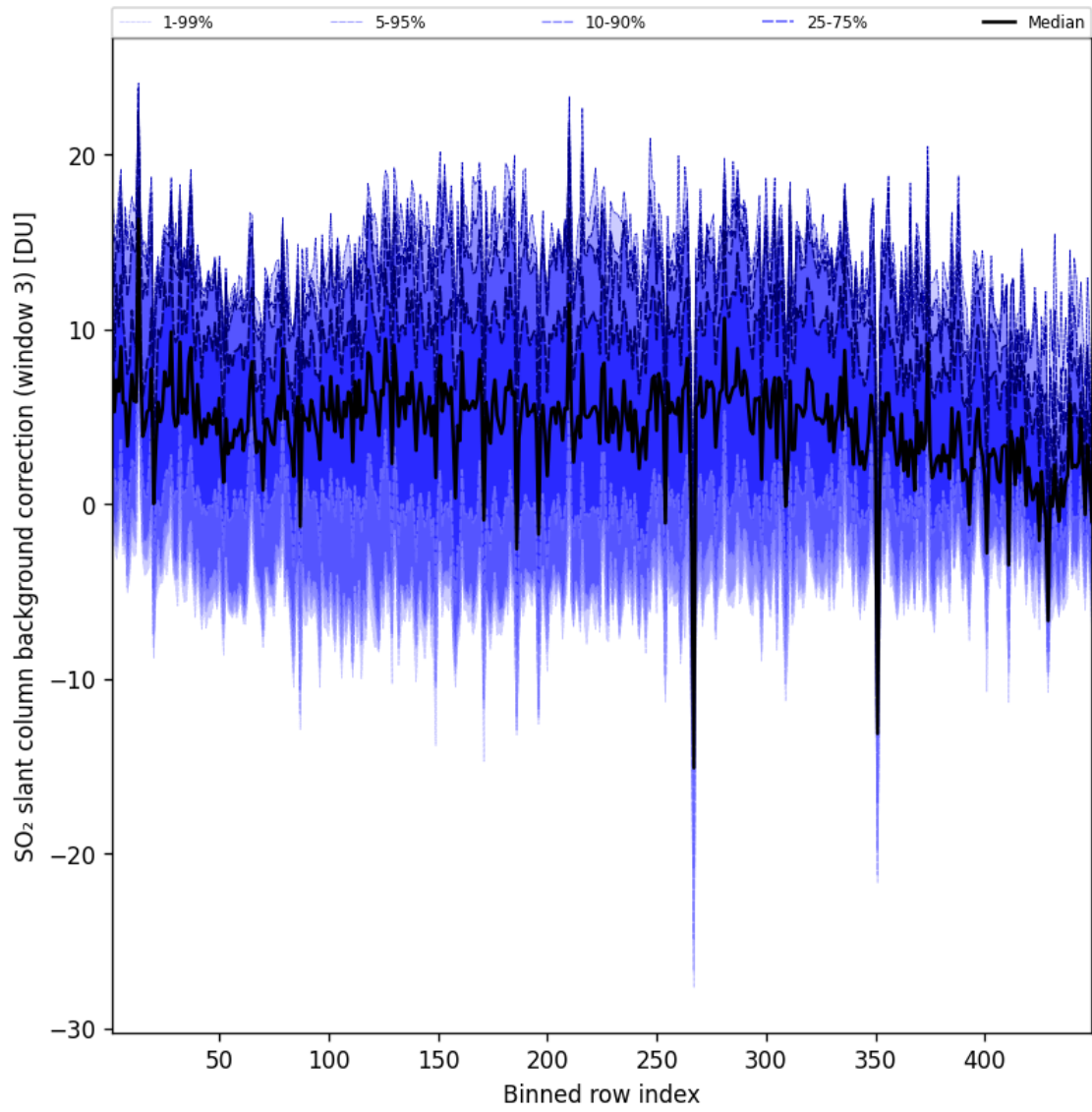
Figure 101: Along track statistics of “SO 2 slant column background correction (window 3)” for 2025-01-12 to 2025-01-13
