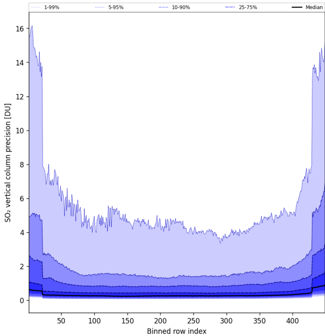
Figure 86: Along track statistics of “SO 2 vertical column precision” for 2025-01-12 to 2025-01-13
