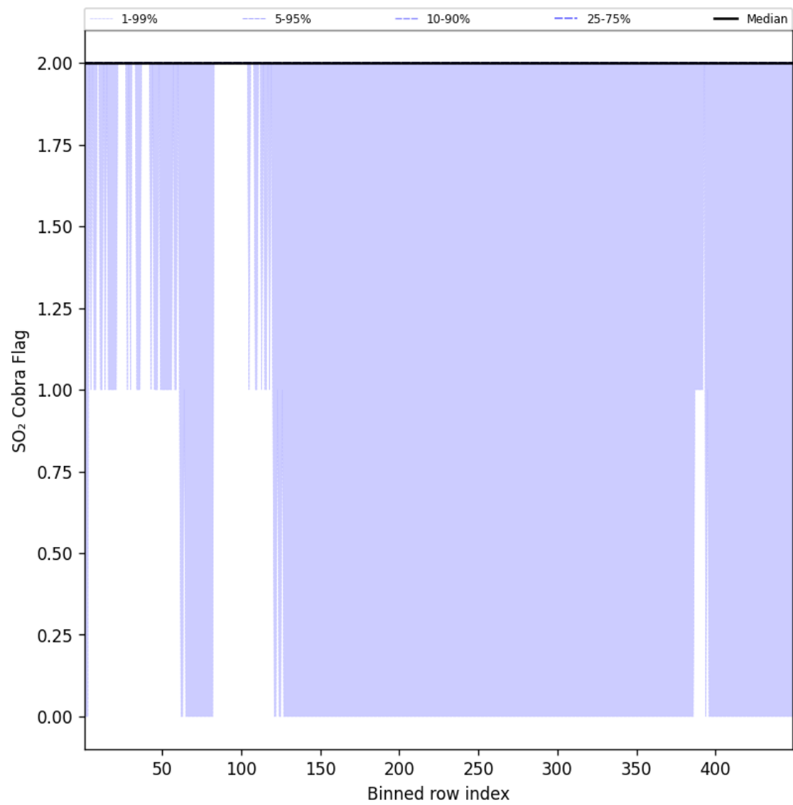
Figure 102: Along track statistics of “SO 2 Cobra Flag” for 2025-01-12 to 2025-01-13
