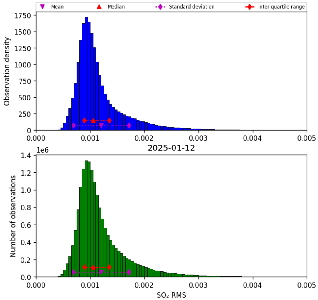
Figure 79: Histogram of “SO 2 RMS” for 2025-01-12 to 2025-01-13
