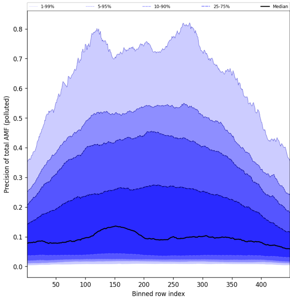
Figure 108: Along track statistics of “Precision of total AMF (polluted)” for 2025-01-12 to 2025-01-13
