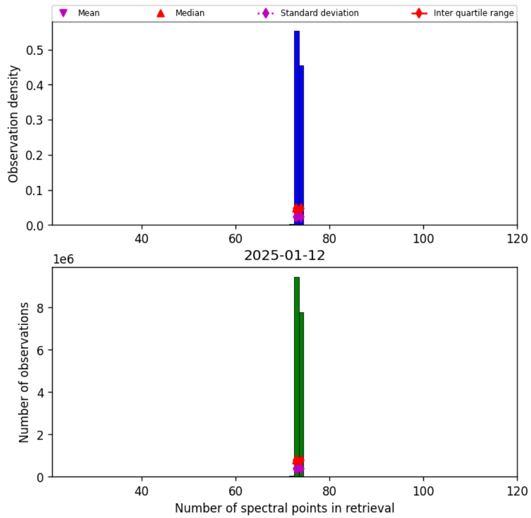
Figure 83: Histogram of “Number of spectral points in retrieval” for 2025-01-12 to 2025-01-13
