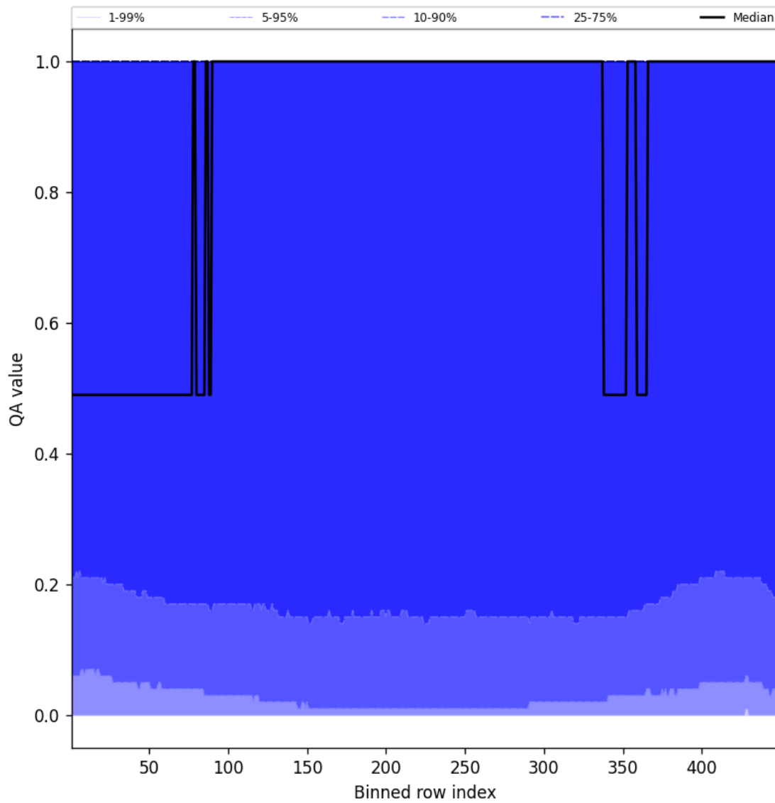
Figure 84: Along track statistics of “QA value” for 2025-01-12 to 2025-01-13
