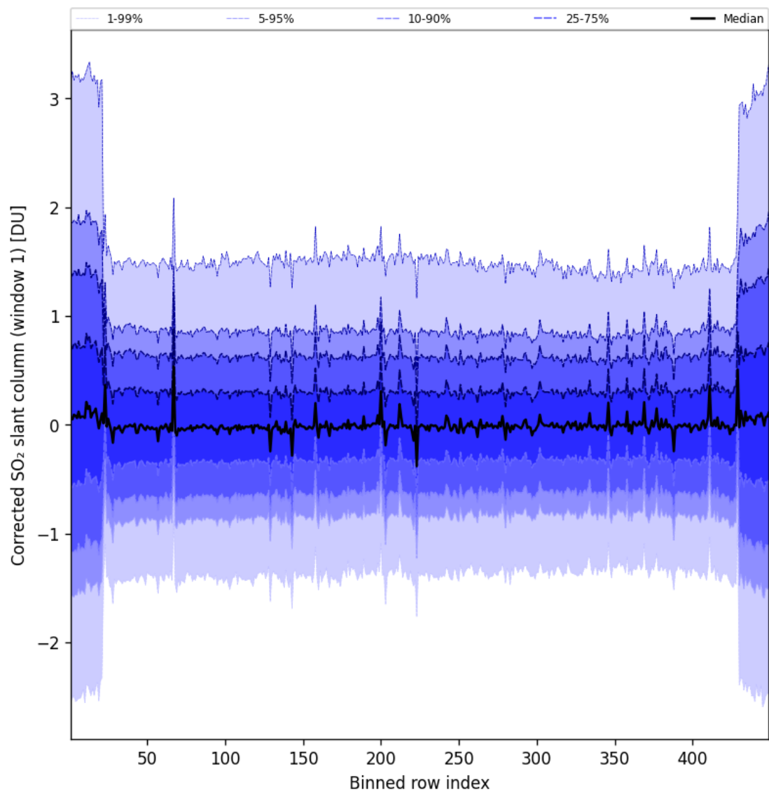
Figure 92: Along track statistics of “Corrected SO 2 slant column (window 1)” for 2025-01-12 to 2025-01-13
