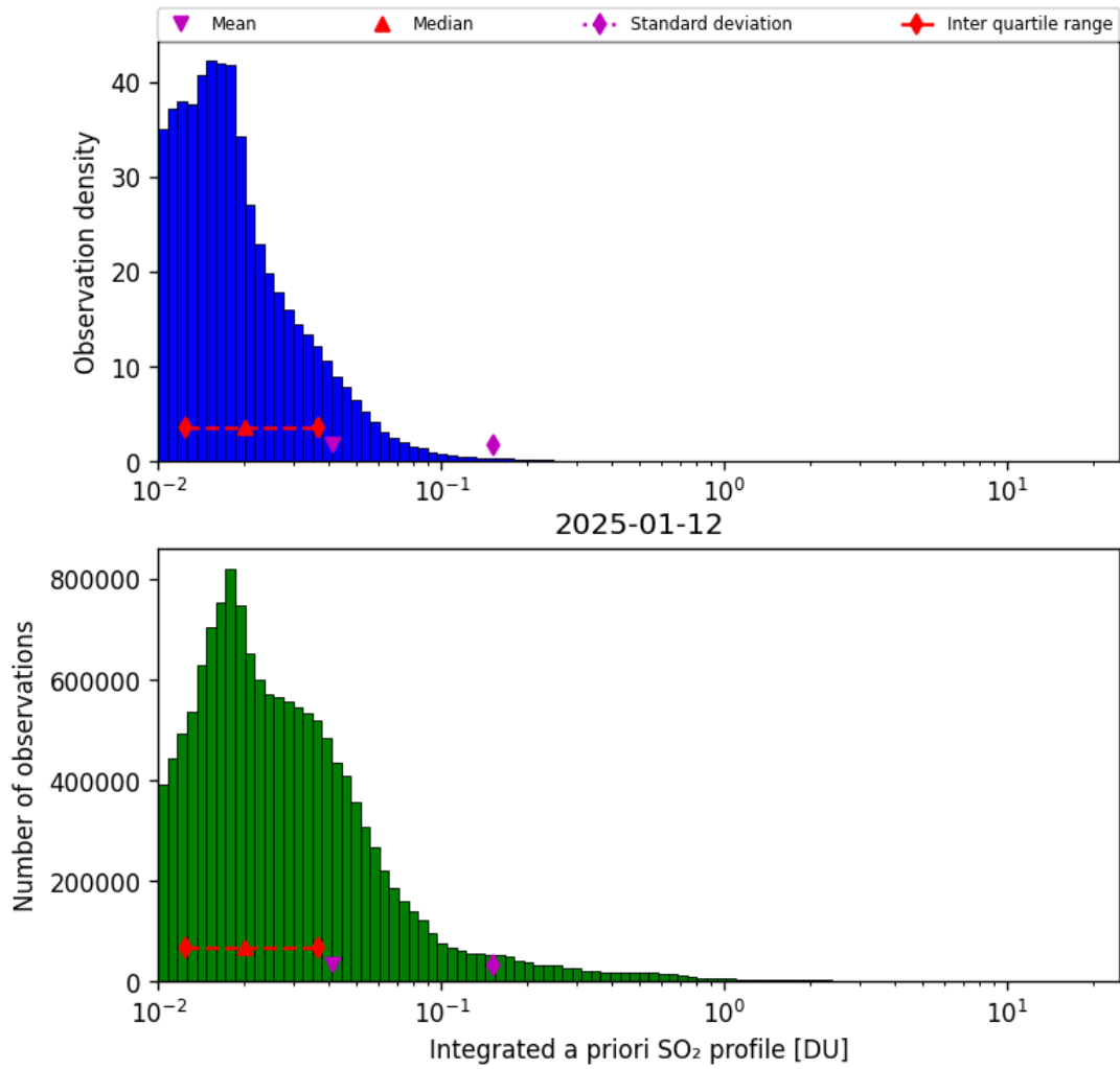
Figure 76: Histogram of “Integrated a priori SO 2 profile” for 2025-01-12 to 2025-01-13
