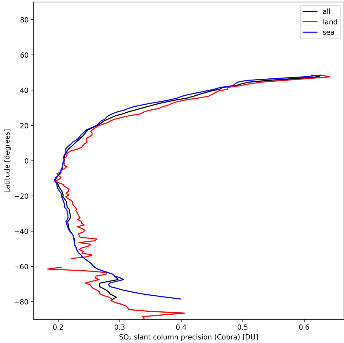
Figure 35: Zonal average of “SO 2 slant column precision (Cobra)” for 2025-01-12 to 2025-01-13.
