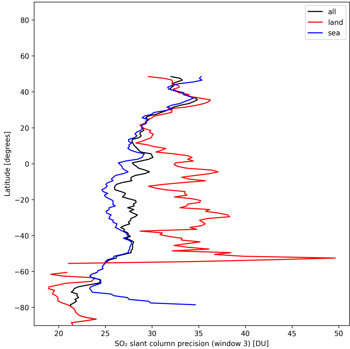
Figure 45: Zonal average of “SO 2 slant column precision (window 3)” for 2025-01-12 to 2025-01-13.
