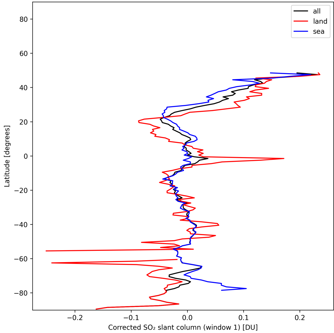
Figure 38: Zonal average of “Corrected SO 2 slant column (window 1)” for 2025-01-12 to 2025-01-13.
