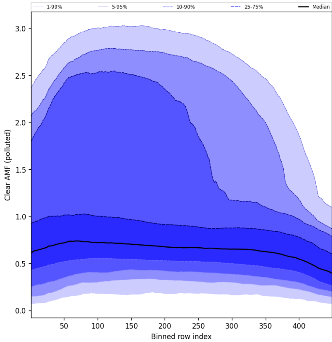
Figure 109: Along track statistics of “Clear AMF (polluted)” for 2025-01-12 to 2025-01-13
