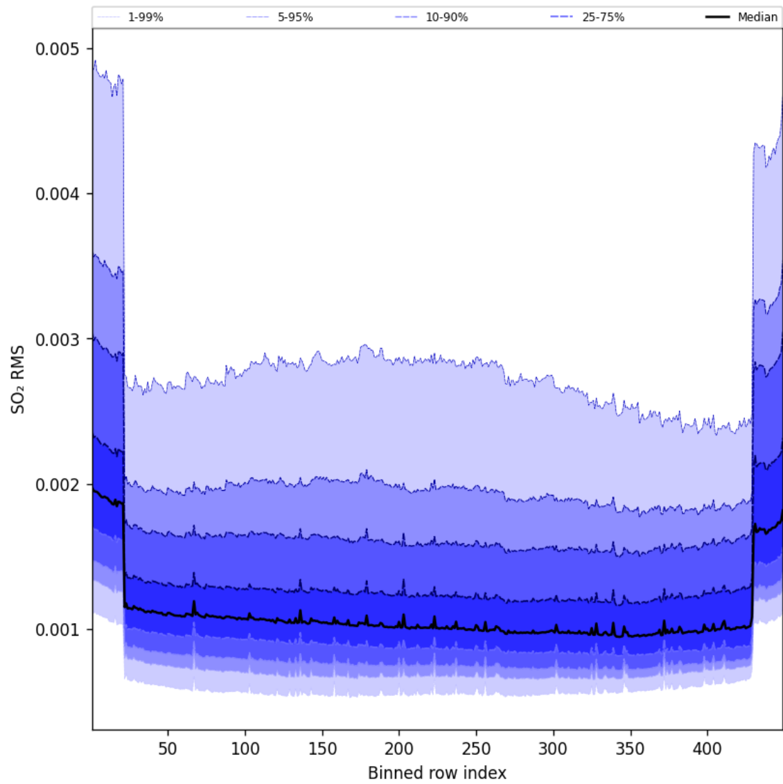
Figure 106: Along track statistics of “SO 2 RMS” for 2025-01-12 to 2025-01-13
