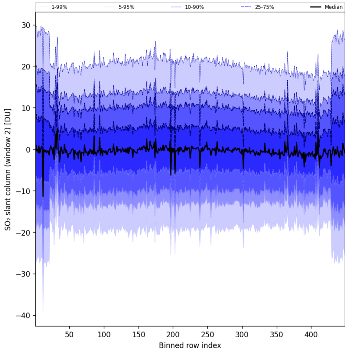
Figure 94: Along track statistics of "SO 2 slant column (window 2)" for 2025-01-12 to 2025-01-13
