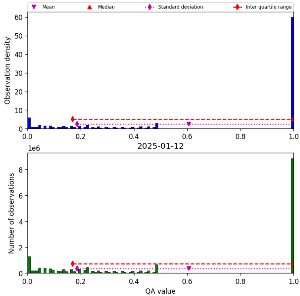
Figure 57: Histogram of “QA value” for 2025-01-12 to 2025-01-13
