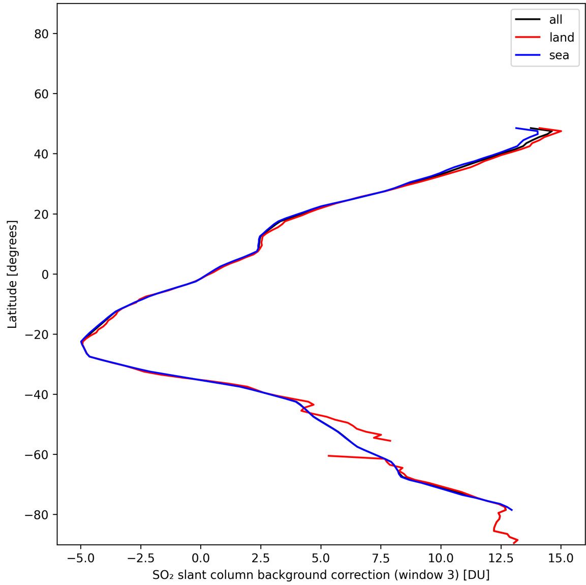
Figure 47: Zonal average of “SO 2 slant column background correction (window 3)” for 2025-01-12 to 2025-01-13.
