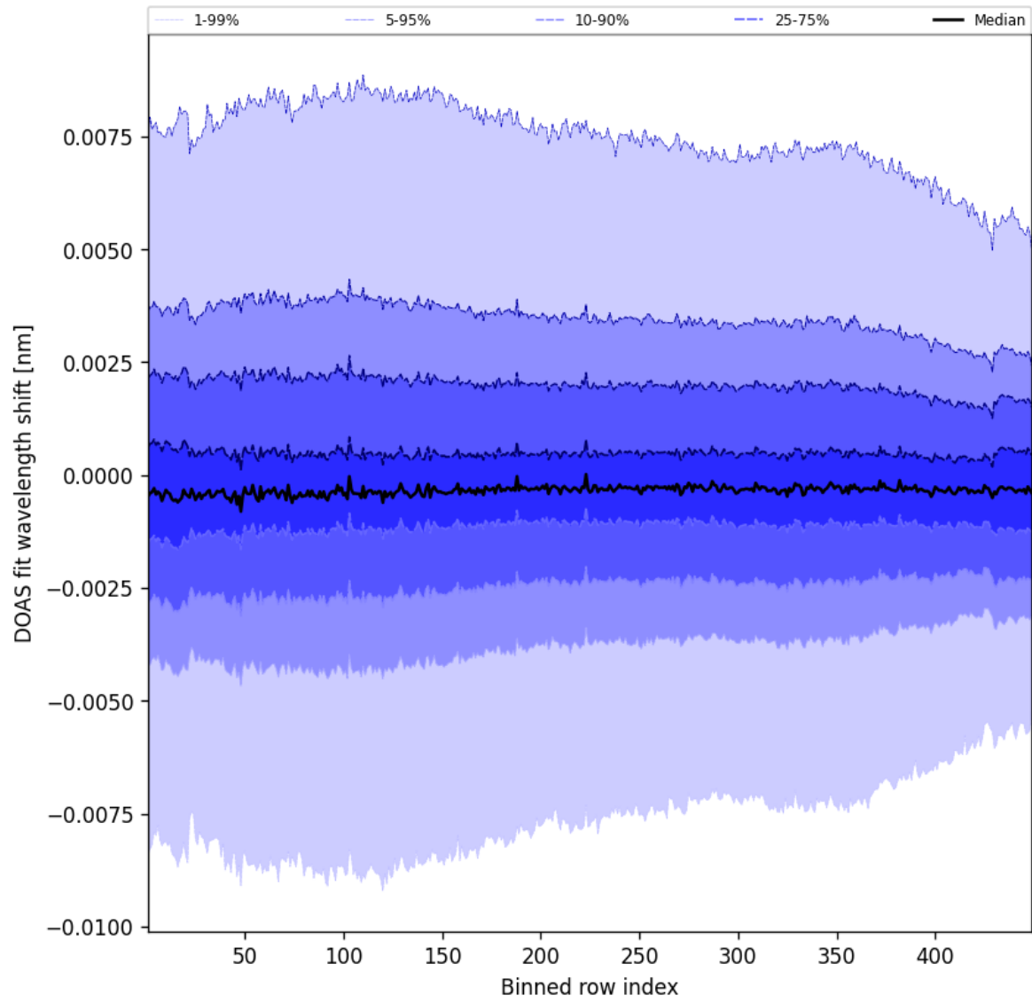
Figure 104: Along track statistics of “DOAS fit wavelength shift” for 2025-01-12 to 2025-01-13
