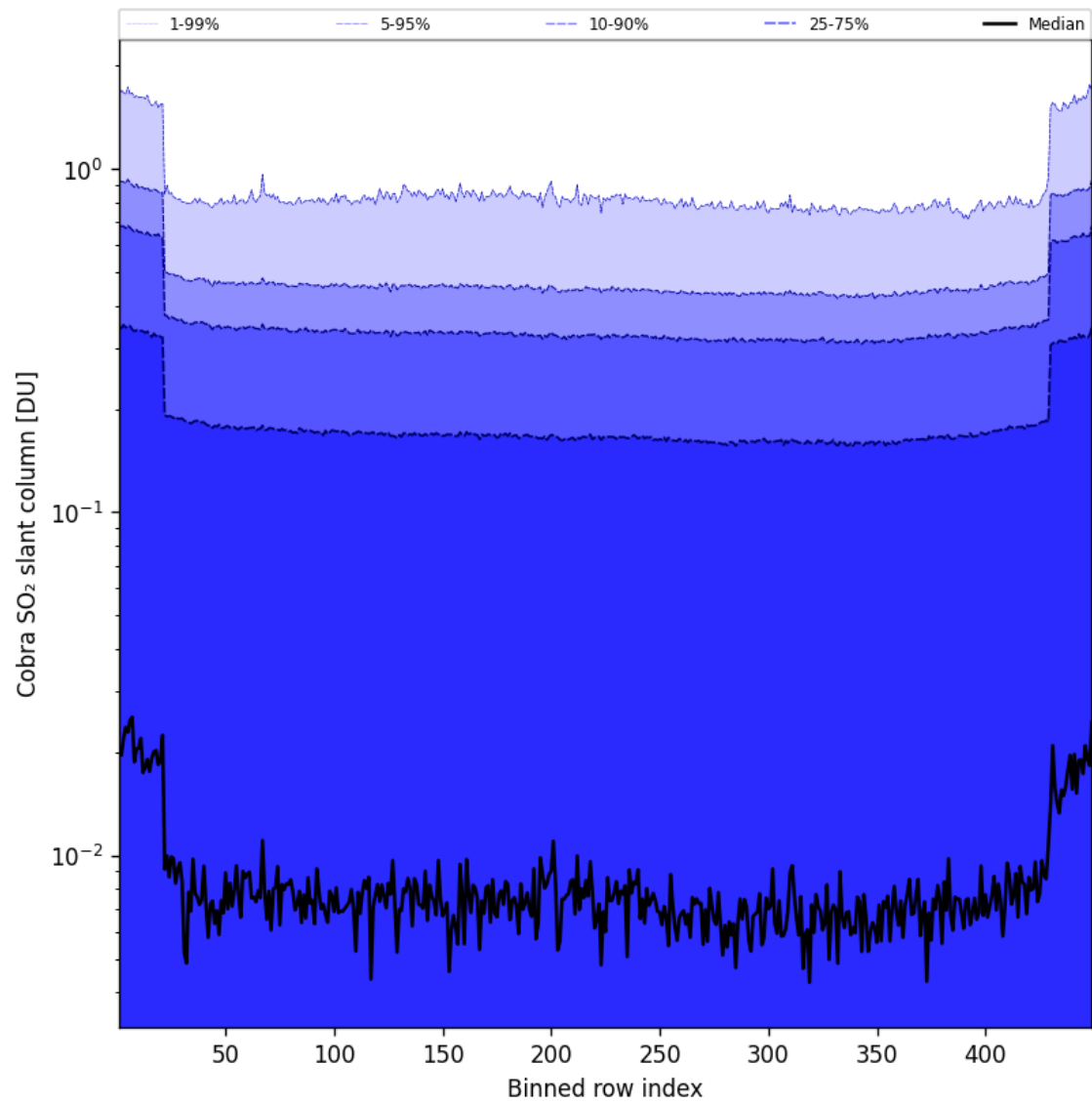
Figure 88: Along track statistics of “Cobra SO 2 slant column” for 2025-01-12 to 2025-01-13
