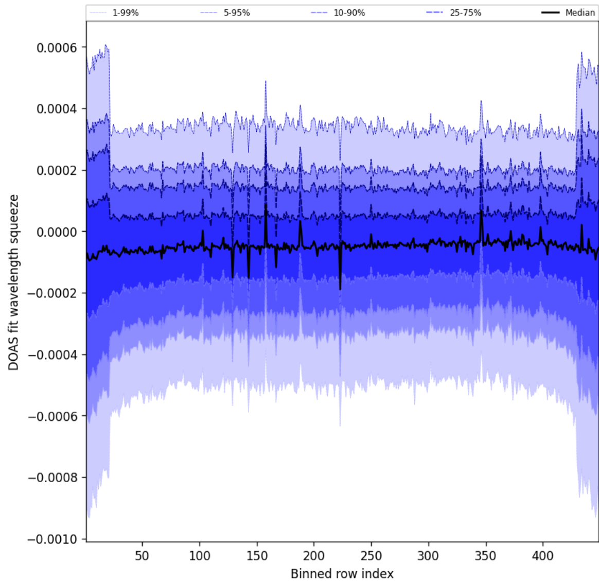
Figure 105: Along track statistics of “DOAS fit wavelength squeeze” for 2025-01-12 to 2025-01-13
