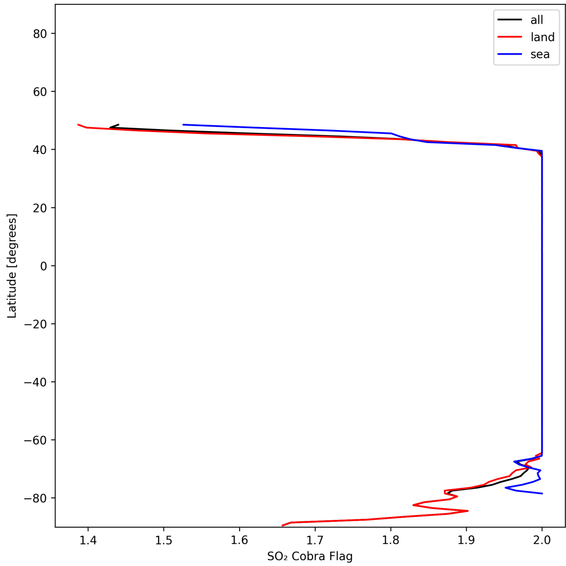
Figure 48: Zonal average of "SO 2 Cobra Flag" for 2025-01-12 to 2025-01-13.
