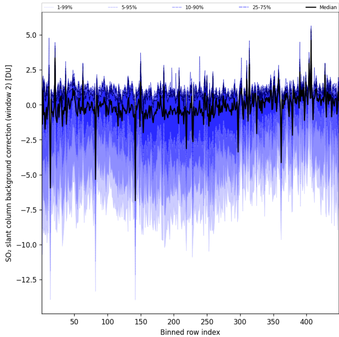
Figure 97: Along track statistics of “SO 2 slant column background correction (window 2)” for 2025-01-12 to 2025-01-13
