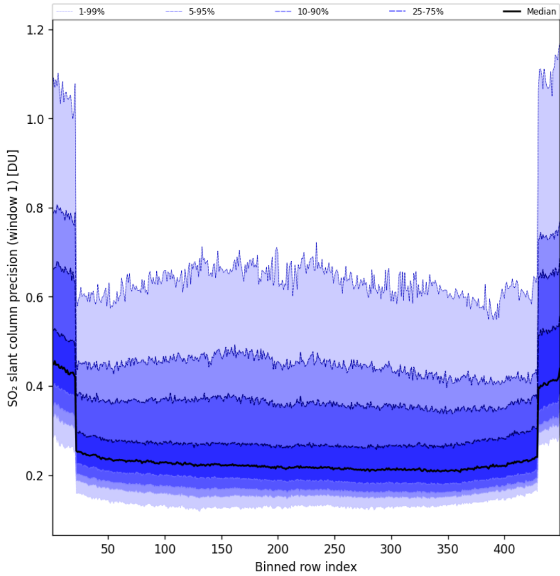
Figure 91: Along track statistics of “SO 2 slant column precision (window 1)” for 2025-01-12 to 2025-01-13
