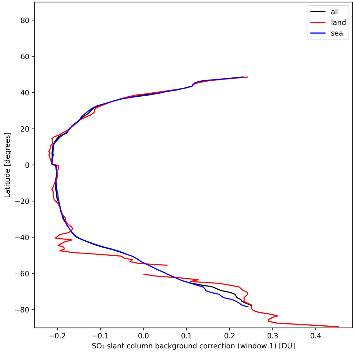
Figure 39: Zonal average of “SO 2 slant column background correction (window 1)” for 2025-01-12 to 2025-01-13.
