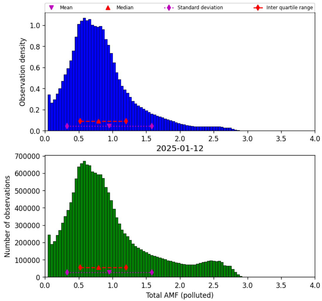
Figure 80: Histogram of “Total AMF (polluted)” for 2025-01-12 to 2025-01-13
