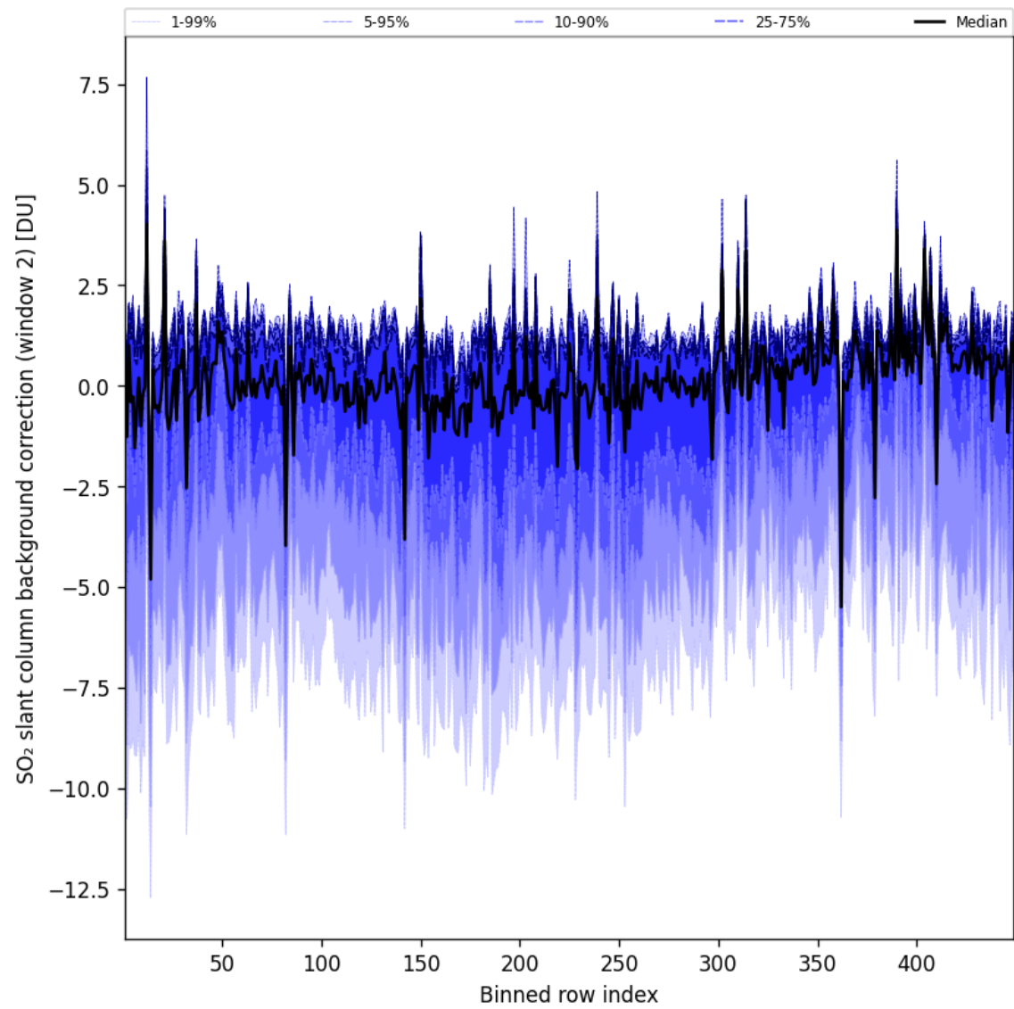
Figure 97: Along track statistics of “SO 2 slant column background correction (window 2)” for 2025-01-13 to 2025-01-14
