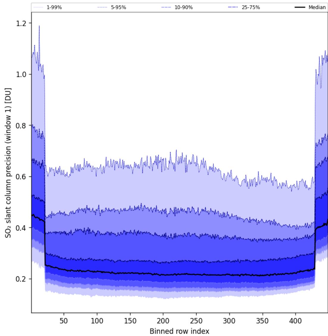
Figure 91: Along track statistics of “SO 2 slant column precision (window 1)” for 2025-01-13 to 2025-01-14
