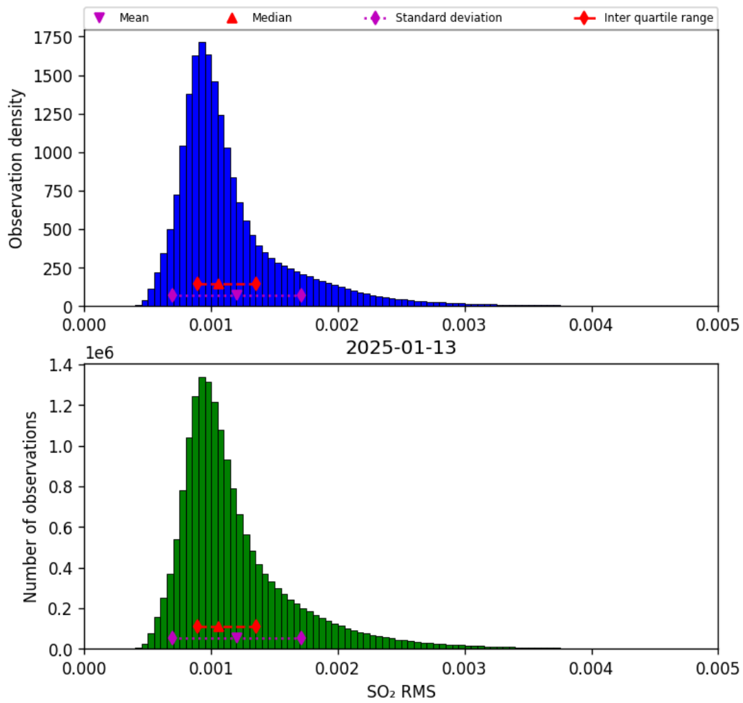
Figure 79: Histogram of “SO 2 RMS” for 2025-01-13 to 2025-01-14
