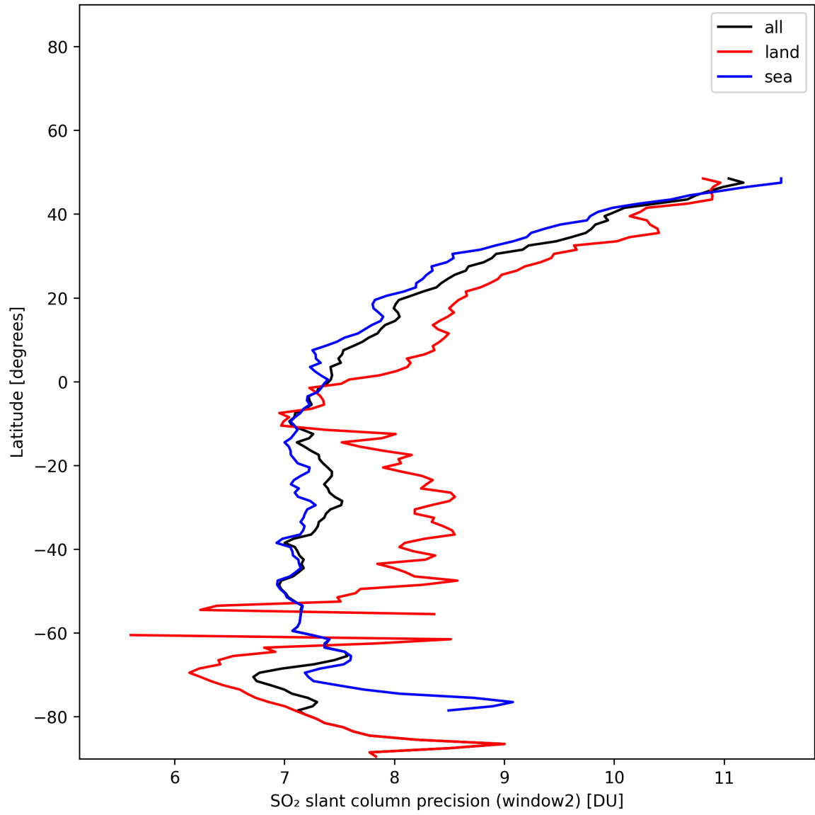
Figure 41: Zonal average of “SO 2 slant column precision (window2)” for 2025-01-13 to 2025-01-14.
