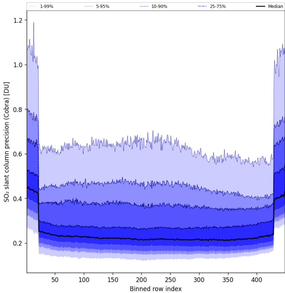
Figure 89: Along track statistics of “SO 2 slant column precision (Cobra)” for 2025-01-13 to 2025-01-14
