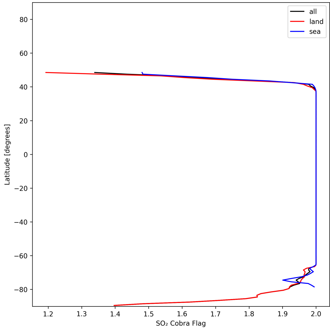
Figure 48: Zonal average of "SO 2 Cobra Flag" for 2025-01-13 to 2025-01-14.
