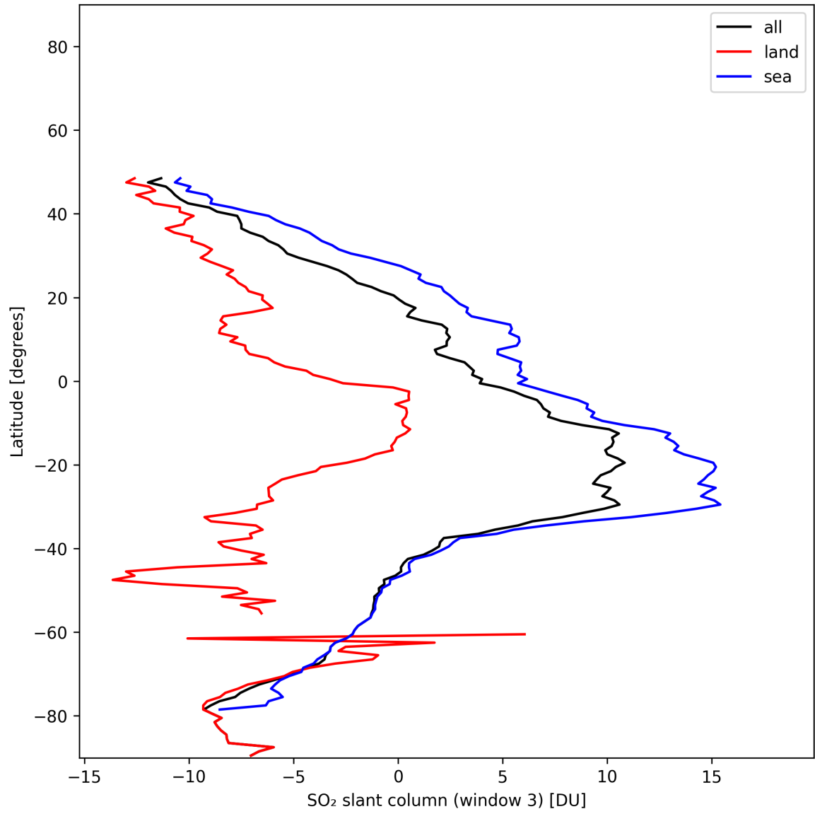
Figure 44: Zonal average of “SO 2 slant column (window 3)” for 2025-01-13 to 2025-01-14.
