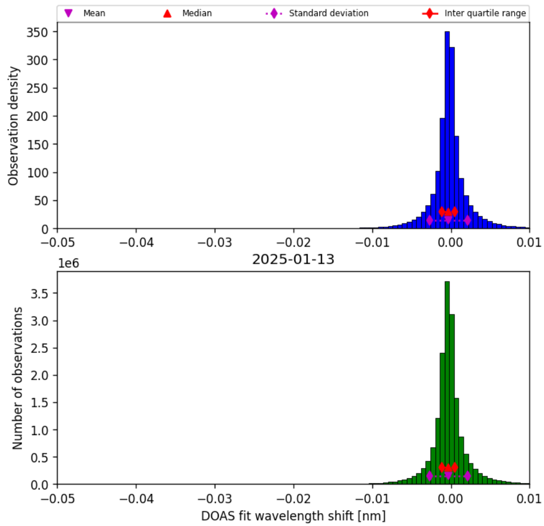
Figure 77: Histogram of “DOAS fit wavelength shift” for 2025-01-13 to 2025-01-14
