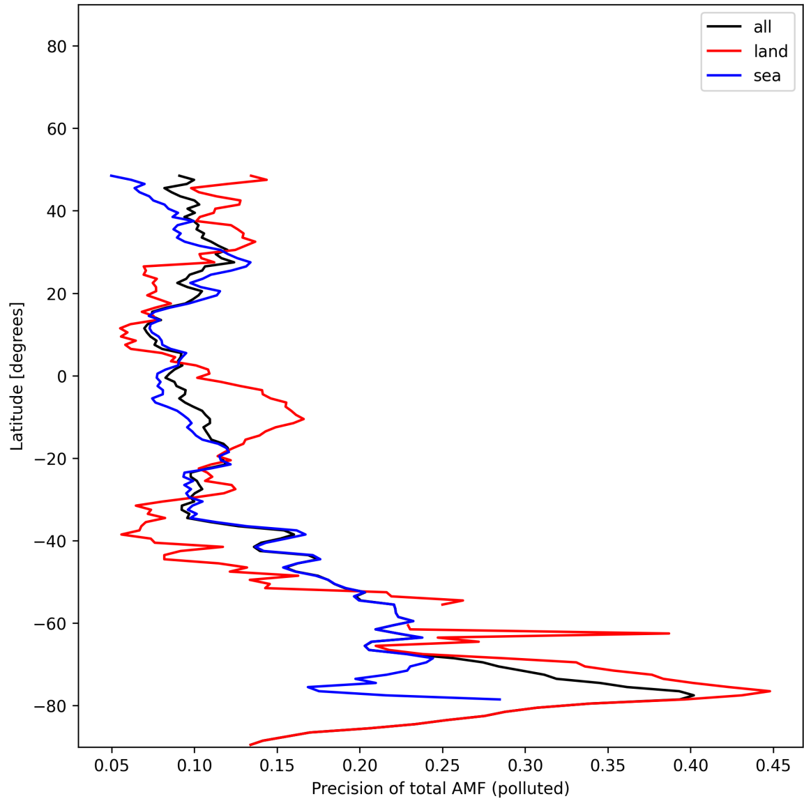
Figure 54: Zonal average of “Precision of total AMF (polluted)” for 2025-01-13 to 2025-01-14.
