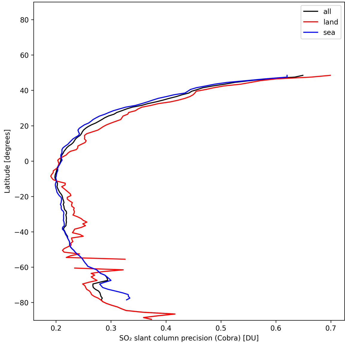
Figure 35: Zonal average of “SO 2 slant column precision (Cobra)” for 2025-01-13 to 2025-01-14.
