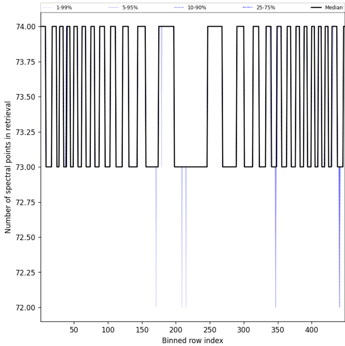
Figure 110: Along track statistics of “Number of spectral points in retrieval” for 2025-01-13 to 2025-01-14
