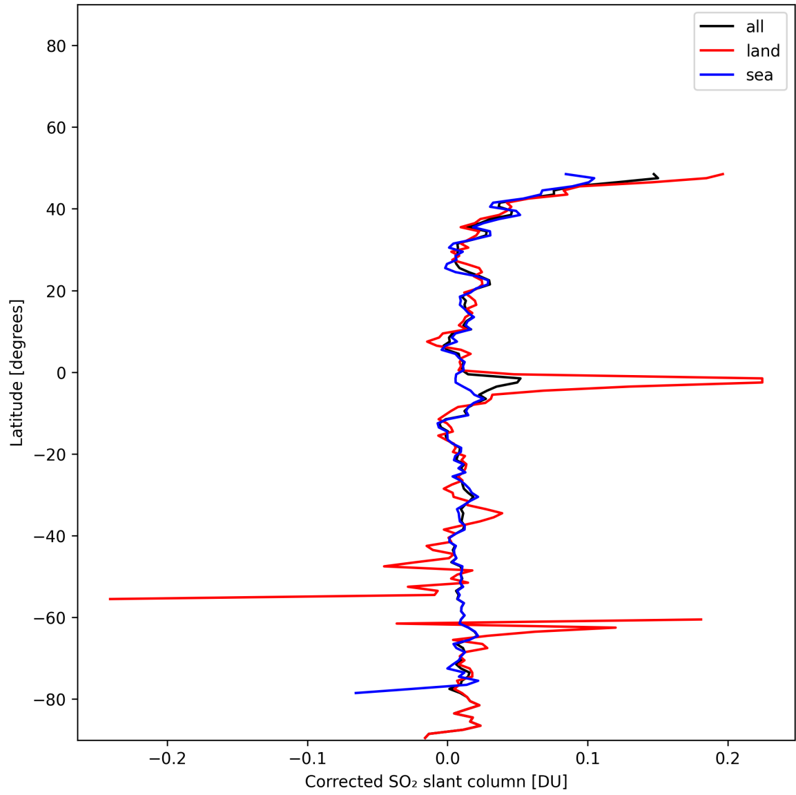
Figure 33: Zonal average of “Corrected SO 2 slant column” for 2025-01-13 to 2025-01-14.
