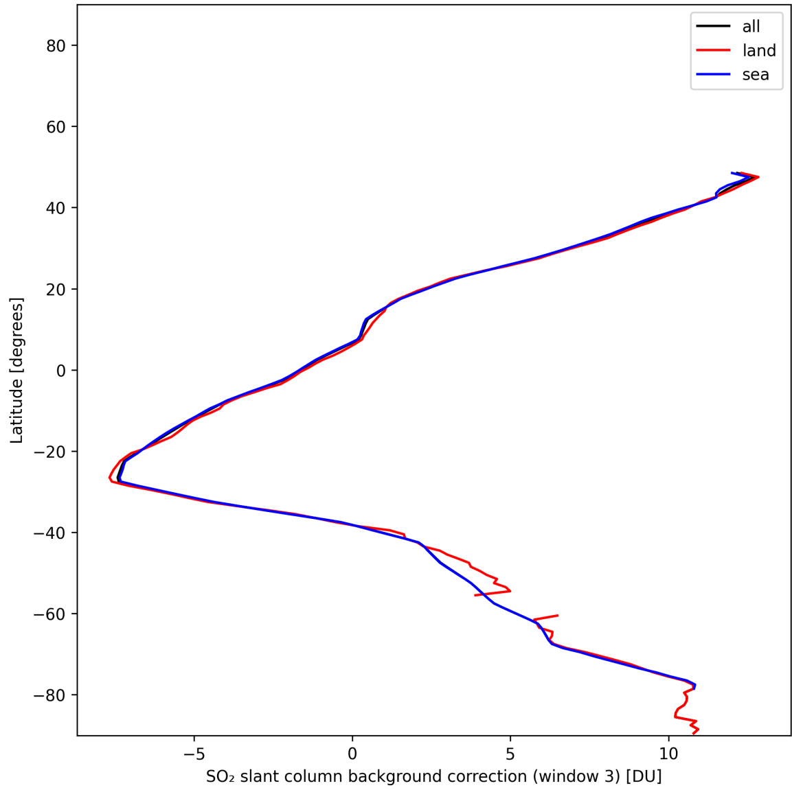
Figure 47: Zonal average of “SO 2 slant column background correction (window 3)” for 2025-01-13 to 2025-01-14.
