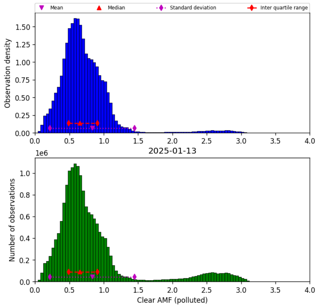
Figure 82: Histogram of “Clear AMF (polluted)” for 2025-01-13 to 2025-01-14
