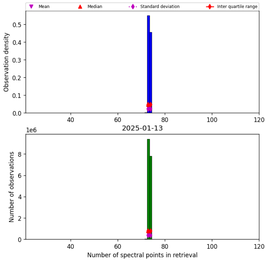
Figure 83: Histogram of “Number of spectral points in retrieval” for 2025-01-13 to 2025-01-14
