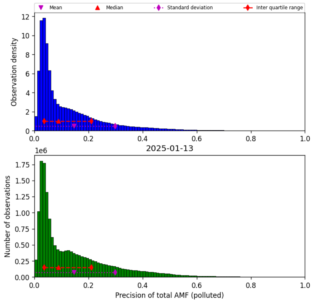
Figure 81: Histogram of “Precision of total AMF (polluted)” for 2025-01-13 to 2025-01-14
