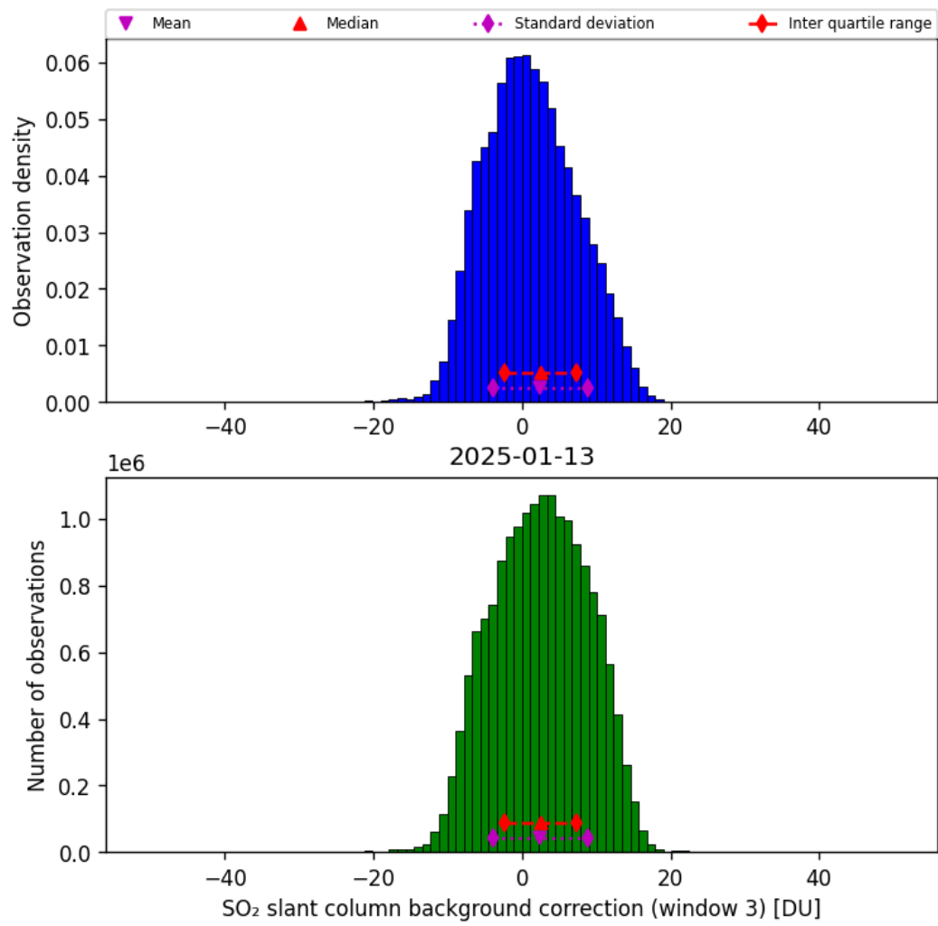
Figure 74: Histogram of “SO 2 slant column background correction (window 3)” for 2025-01-13 to 2025-01-14
