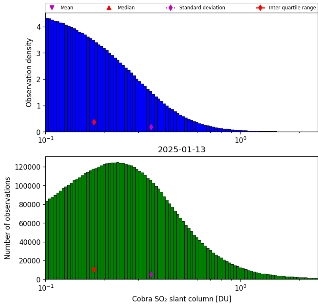
Figure 61: Histogram of “Cobra SO 2 slant column” for 2025-01-13 to 2025-01-14
