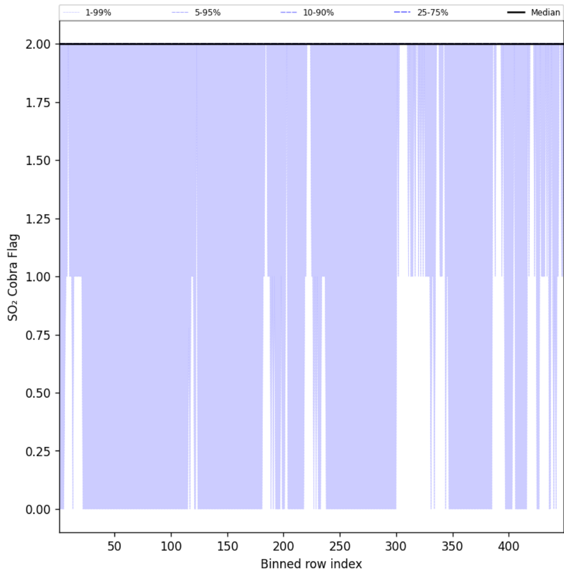
Figure 102: Along track statistics of “SO 2 Cobra Flag” for 2025-01-13 to 2025-01-14
