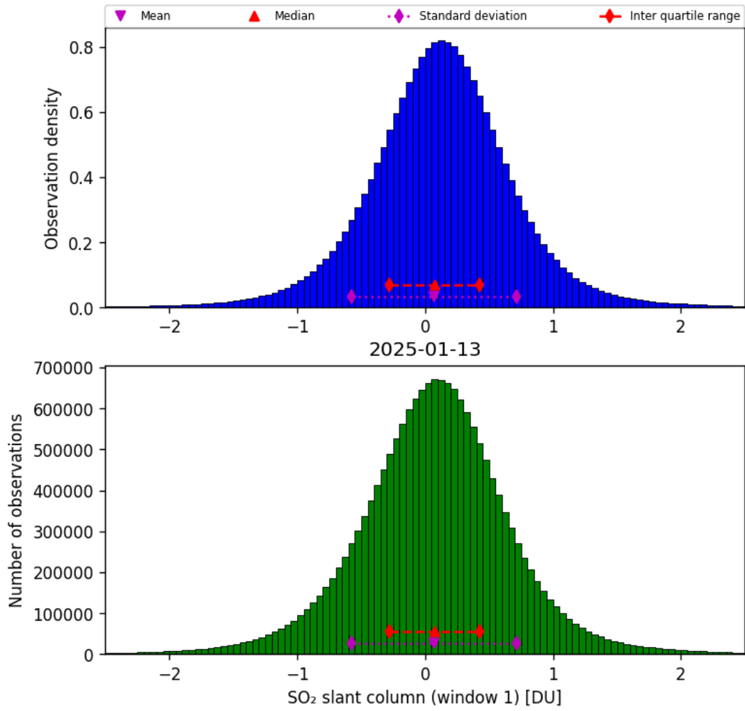
Figure 63: Histogram of “SO 2 slant column (window 1)” for 2025-01-13 to 2025-01-14
