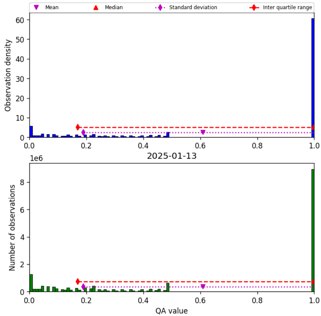
Figure 57: Histogram of “QA value” for 2025-01-13 to 2025-01-14
