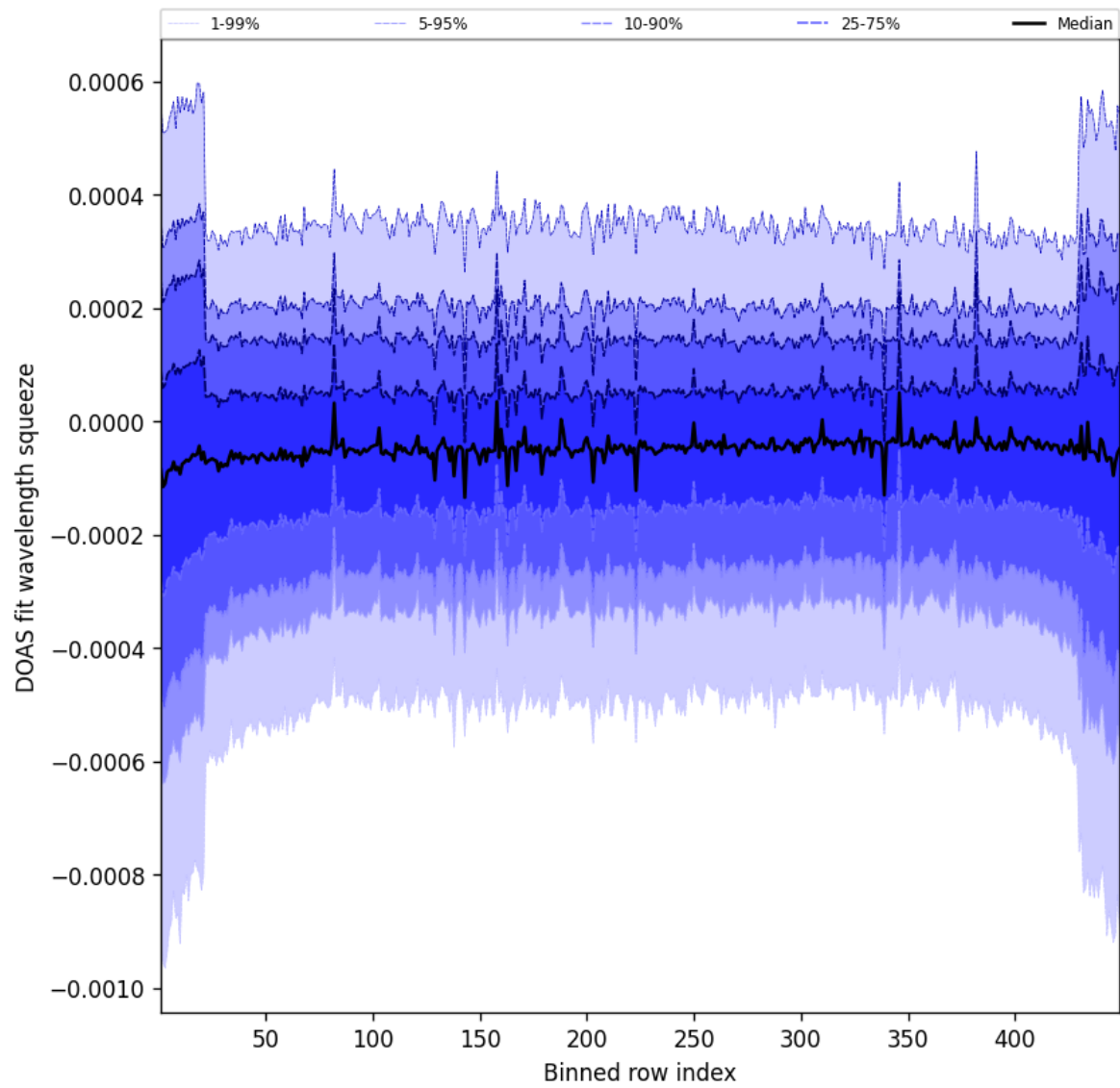
Figure 105: Along track statistics of “DOAS fit wavelength squeeze” for 2025-01-13 to 2025-01-14
