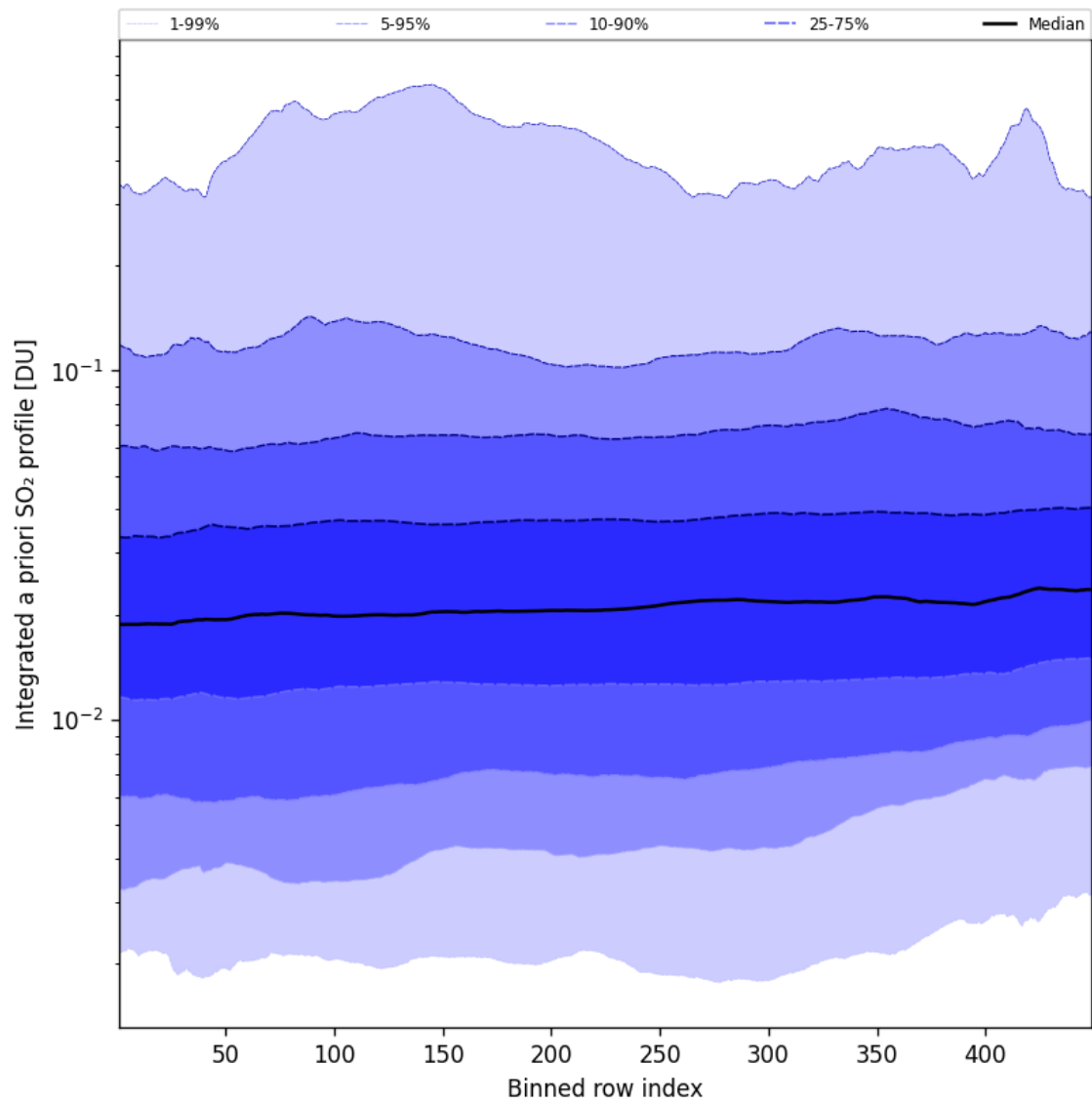
Figure 103: Along track statistics of “Integrated a priori SO 2 profile” for 2025-01-13 to 2025-01-14
