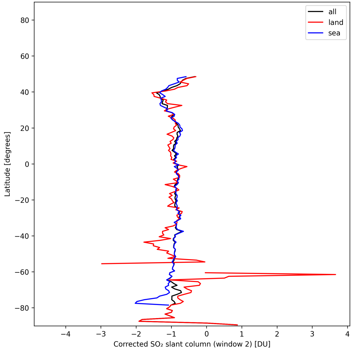
Figure 42: Zonal average of “Corrected SO 2 slant column (window 2)” for 2025-01-13 to 2025-01-14.
