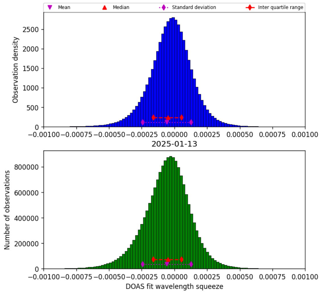
Figure 78: Histogram of “DOAS fit wavelength squeeze” for 2025-01-13 to 2025-01-14
