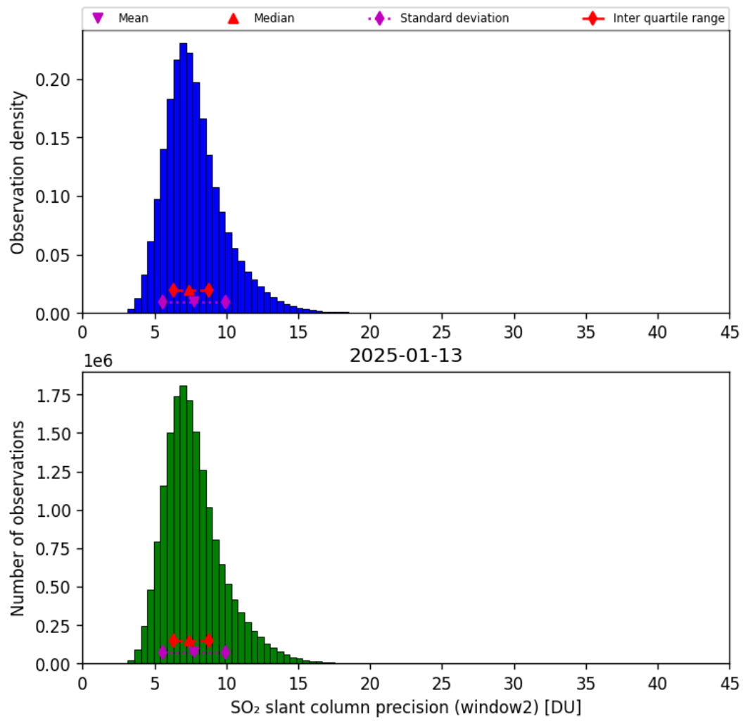
Figure 68: Histogram of “SO 2 slant column precision (window2)” for 2025-01-13 to 2025-01-14
