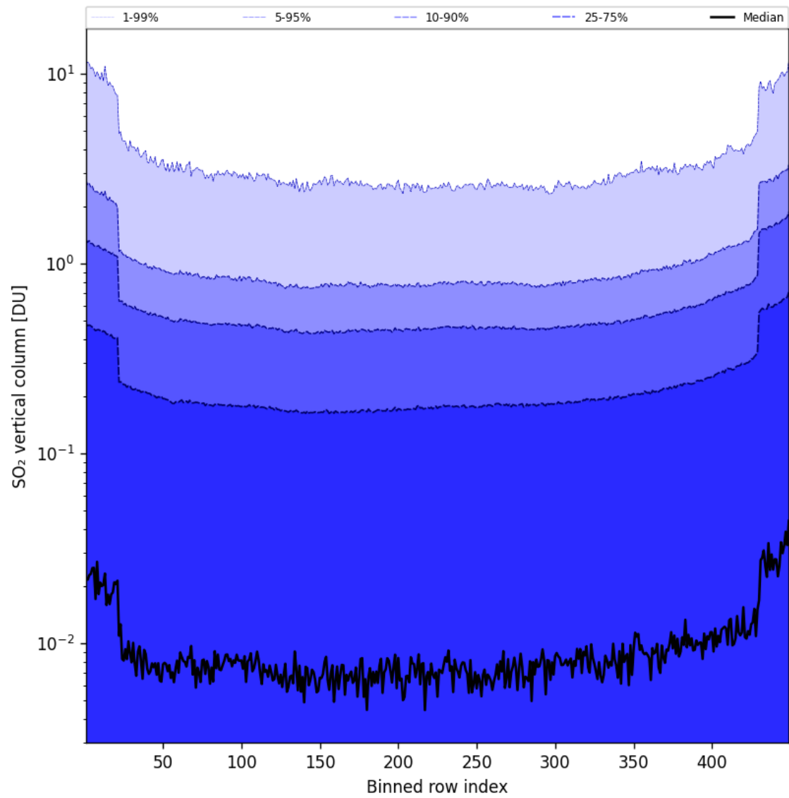
Figure 85: Along track statistics of “SO 2 vertical column” for 2025-01-13 to 2025-01-14
