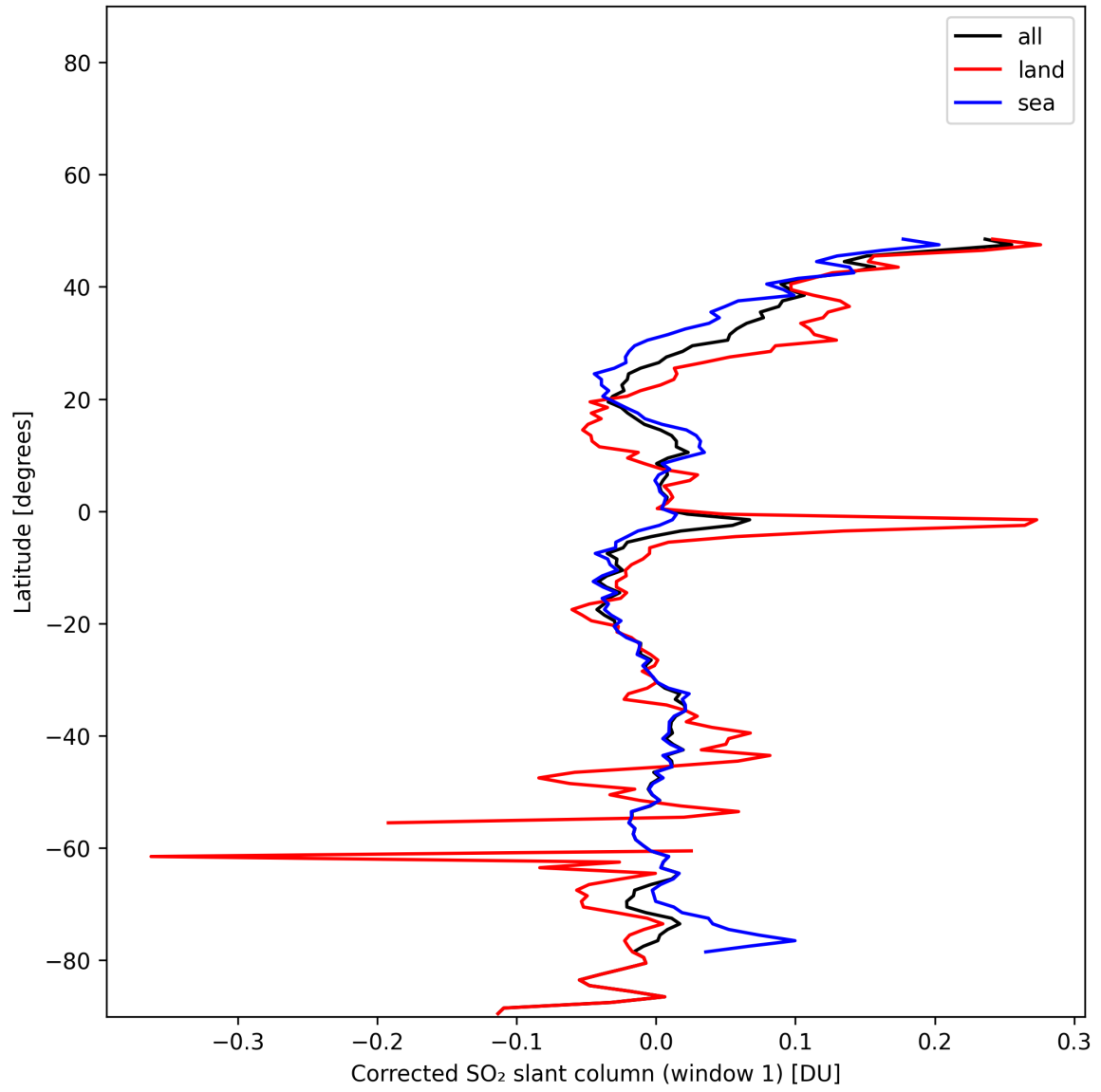
Figure 38: Zonal average of “Corrected SO 2 slant column (window 1)” for 2025-01-13 to 2025-01-14.
