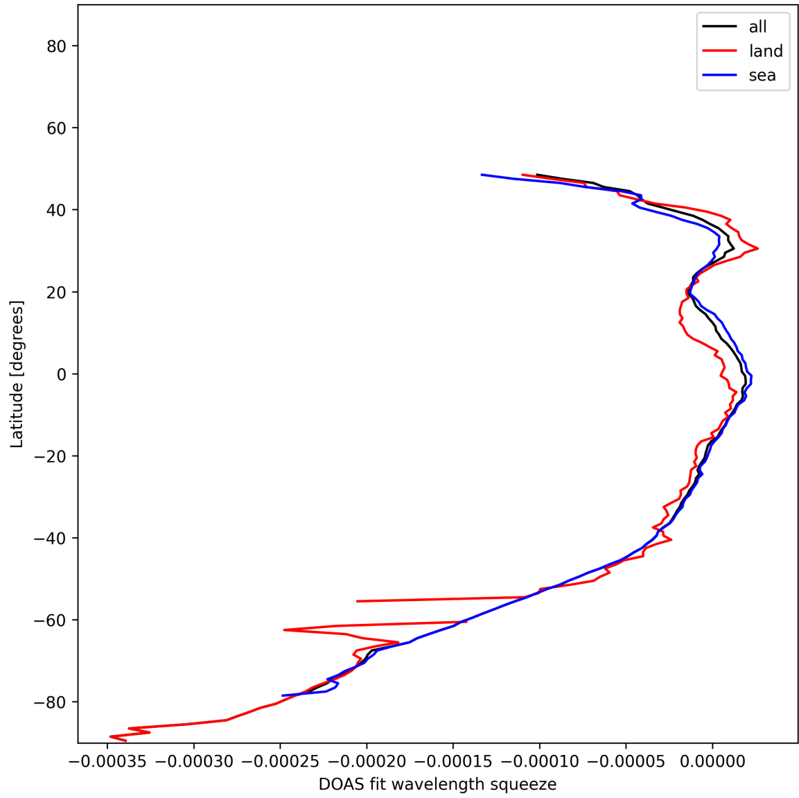
Figure 51: Zonal average of “DOAS fit wavelength squeeze” for 2025-01-13 to 2025-01-14.
