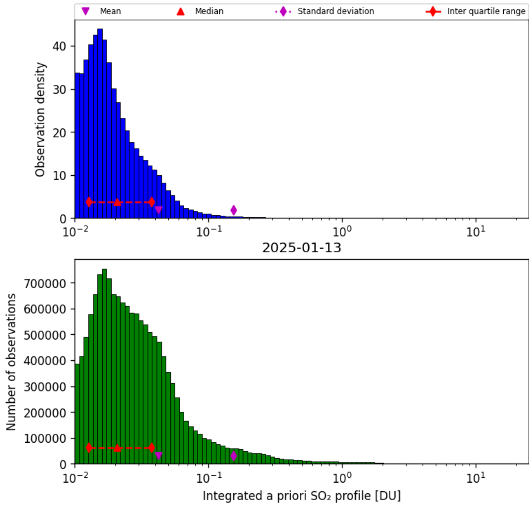
Figure 76: Histogram of “Integrated a priori SO 2 profile” for 2025-01-13 to 2025-01-14
