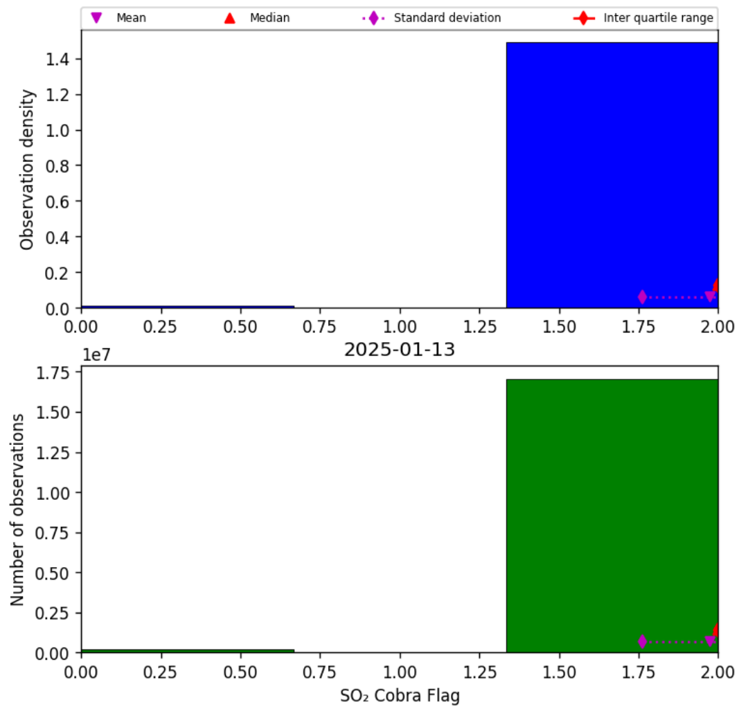
Figure 75: Histogram of “SO 2 Cobra Flag” for 2025-01-13 to 2025-01-14
