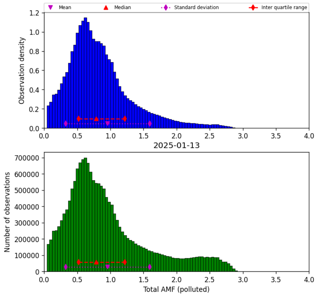
Figure 80: Histogram of “Total AMF (polluted)” for 2025-01-13 to 2025-01-14
