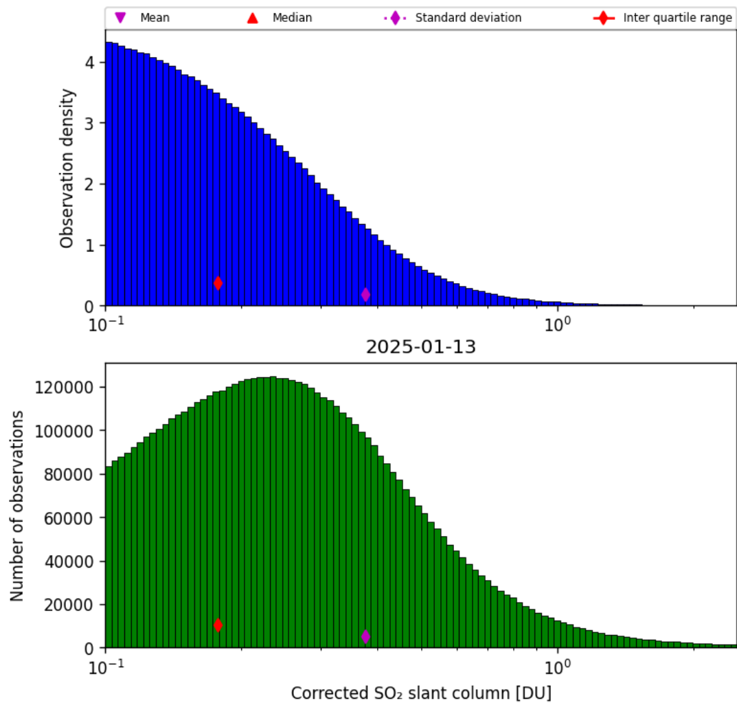
Figure 60: Histogram of “Corrected SO 2 slant column” for 2025-01-13 to 2025-01-14
