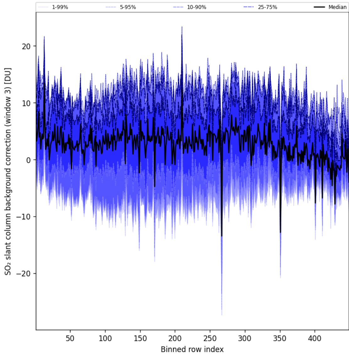
Figure 101: Along track statistics of “SO 2 slant column background correction (window 3)” for 2025-01-13 to 2025-01-14
