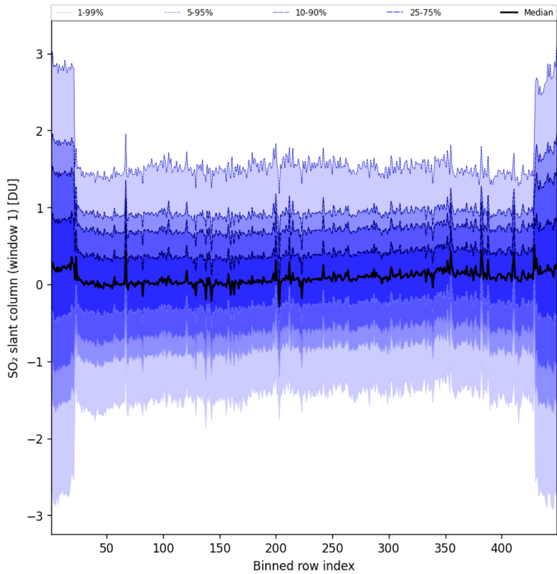
Figure 90: Along track statistics of “SO 2 slant column (window 1)” for 2025-01-13 to 2025-01-14
