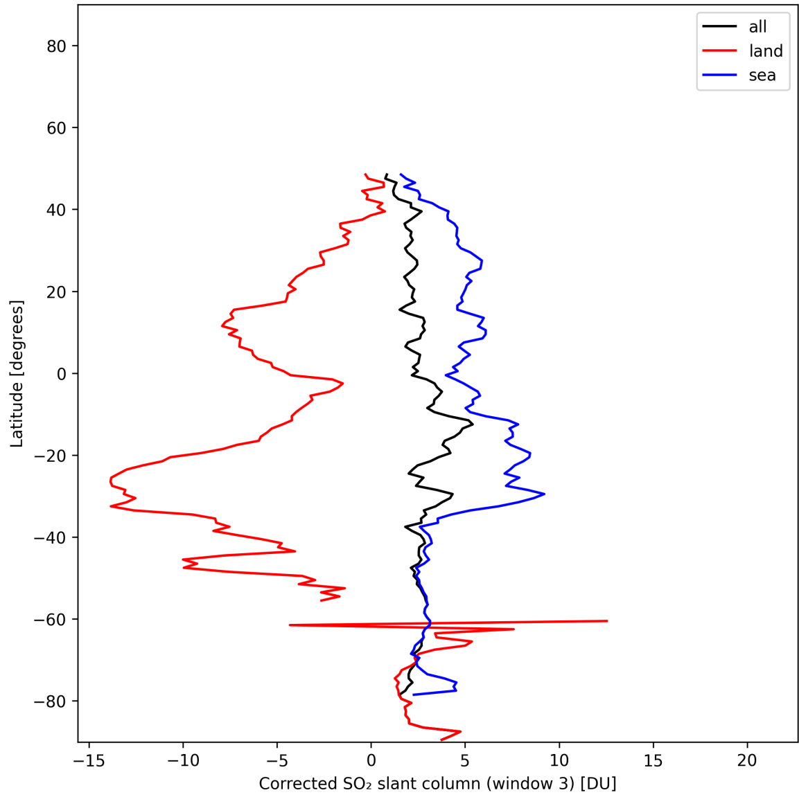
Figure 46: Zonal average of “Corrected SO 2 slant column (window 3)” for 2025-01-13 to 2025-01-14.
