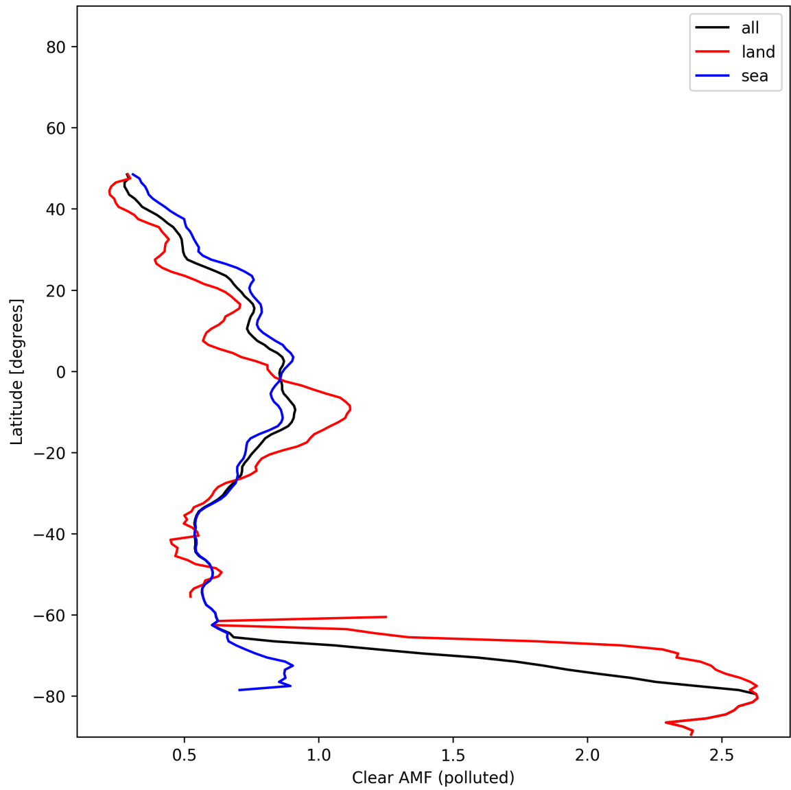
Figure 55: Zonal average of “Clear AMF (polluted)” for 2025-01-13 to 2025-01-14.
