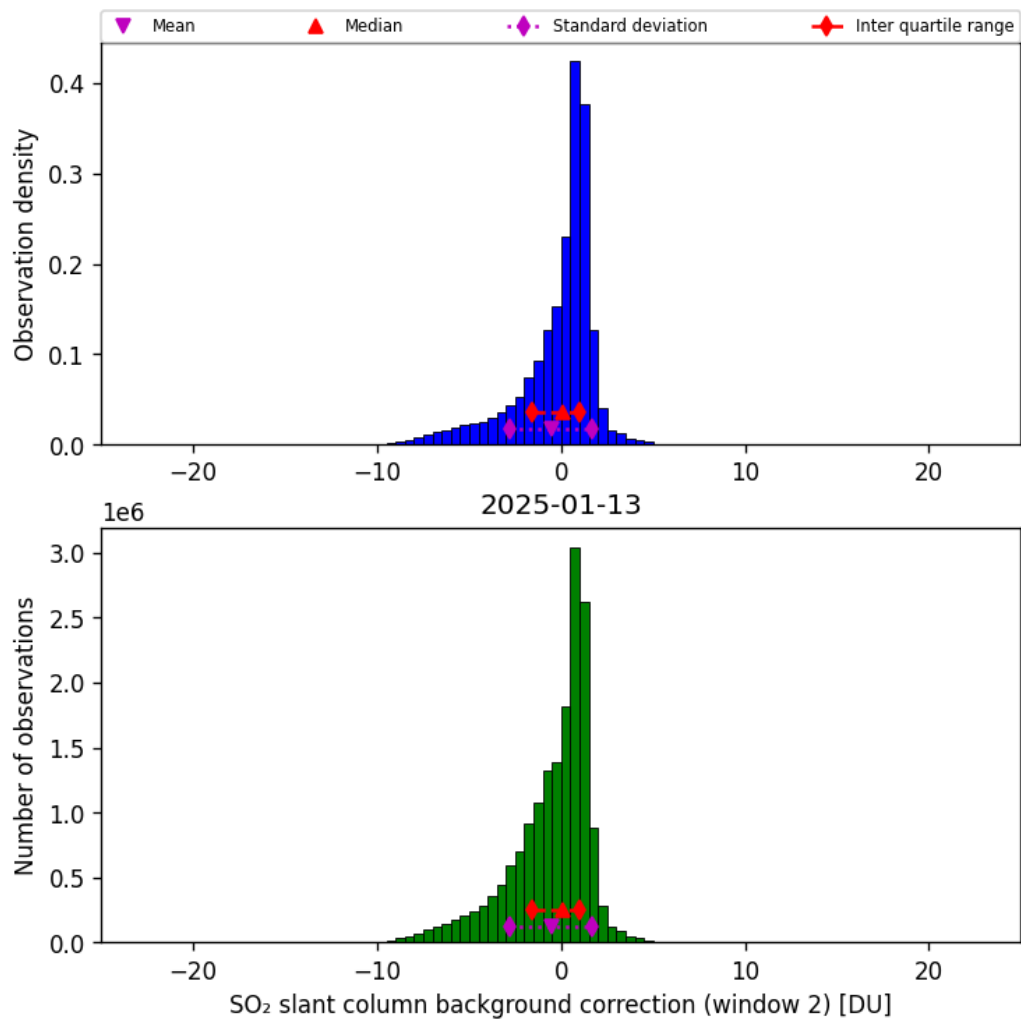
Figure 70: Histogram of “SO 2 slant column background correction (window 2)” for 2025-01-13 to 2025-01-14
