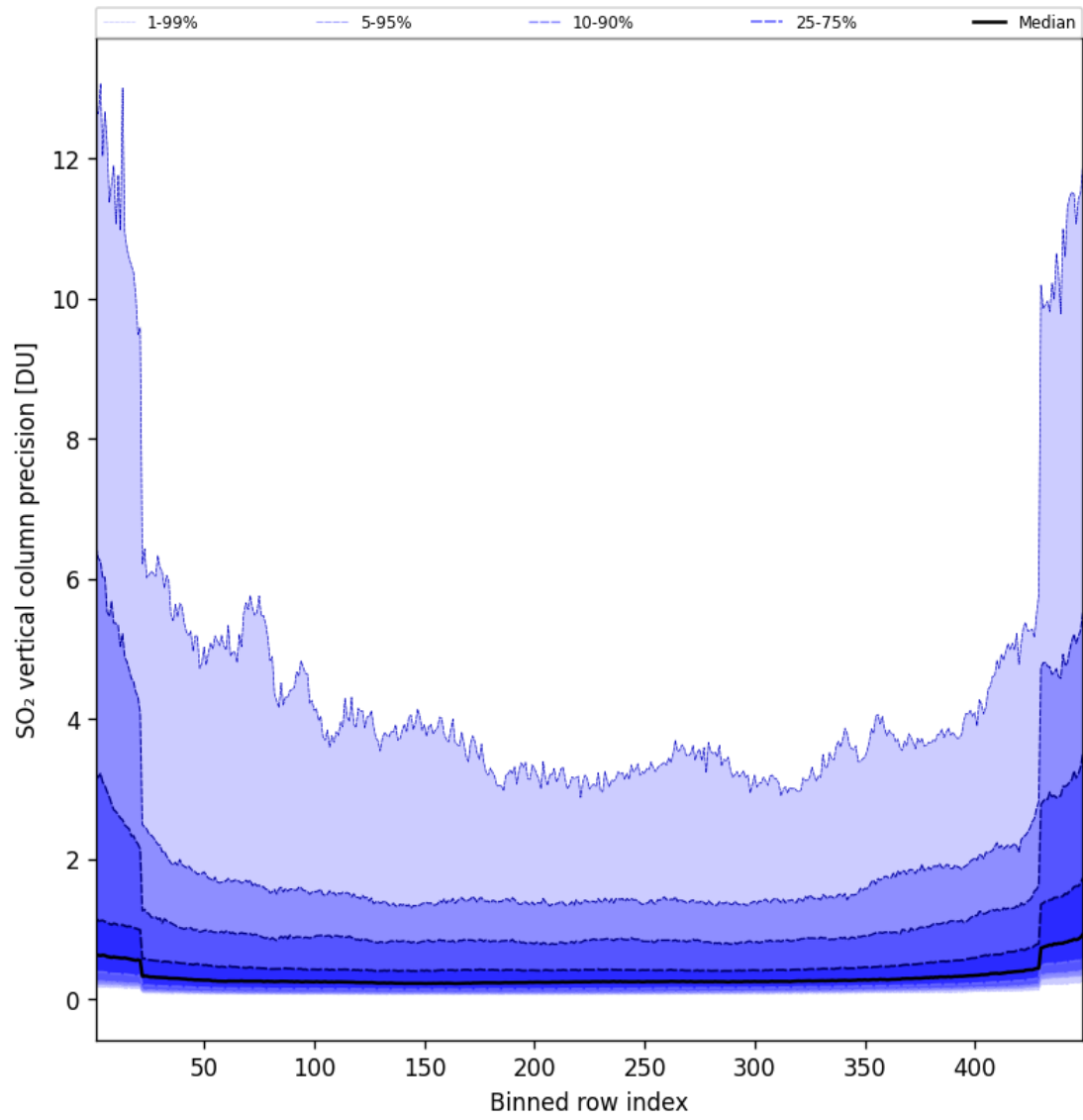
Figure 86: Along track statistics of “SO 2 vertical column precision” for 2025-01-13 to 2025-01-14
