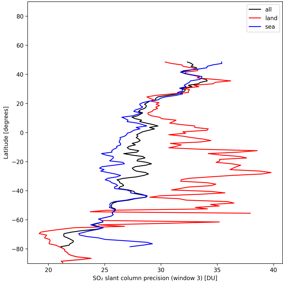
Figure 45: Zonal average of “SO 2 slant column precision (window 3)” for 2025-01-13 to 2025-01-14.
