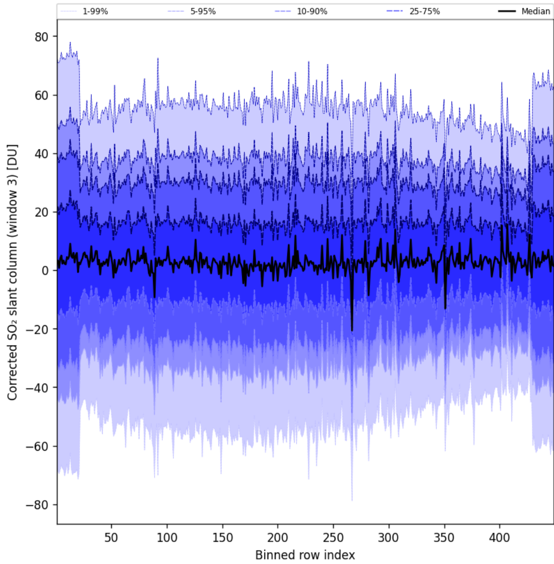
Figure 100: Along track statistics of “Corrected SO 2 slant column (window 3)” for 2025-01-13 to 2025-01-14
