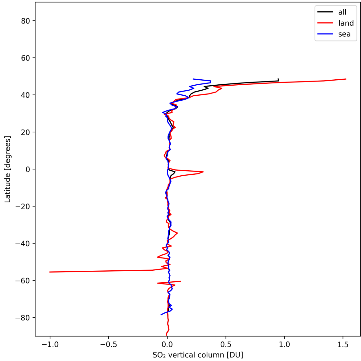
Figure 31: Zonal average of “SO 2 vertical column” for 2025-01-13 to 2025-01-14.
