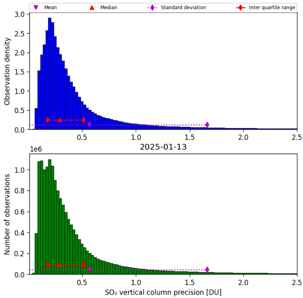
Figure 59: Histogram of “SO 2 vertical column precision” for 2025-01-13 to 2025-01-14
