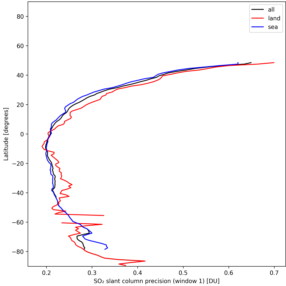
Figure 37: Zonal average of “SO 2 slant column precision (window 1)” for 2025-01-13 to 2025-01-14.
