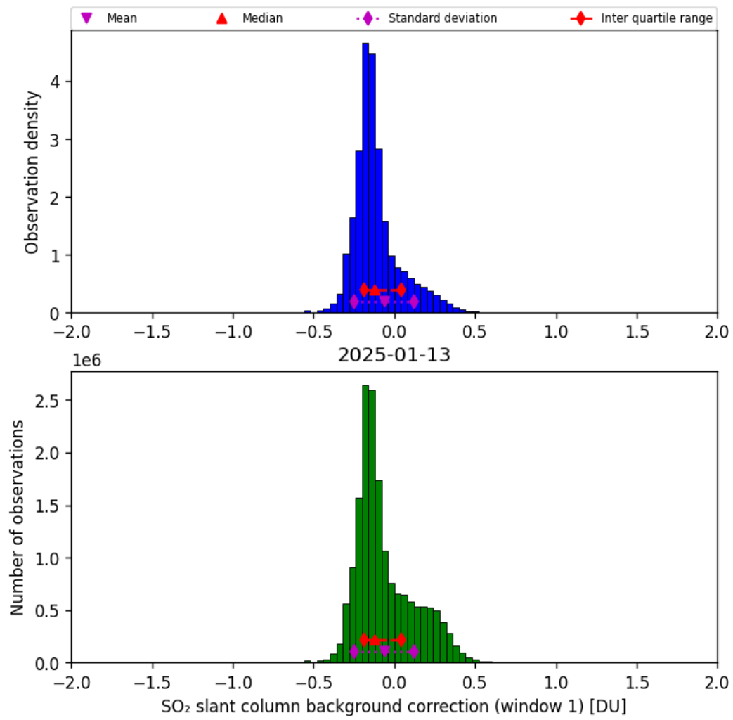
Figure 66: Histogram of “SO 2 slant column background correction (window 1)” for 2025-01-13 to 2025-01-14
