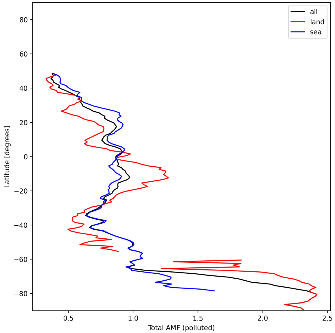
Figure 53: Zonal average of “Total AMF (polluted)” for 2025-01-13 to 2025-01-14.
