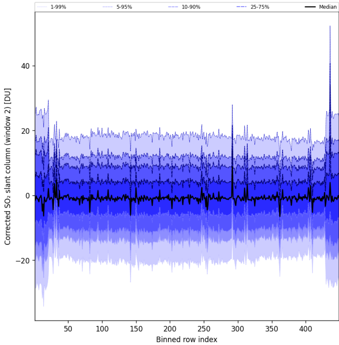
Figure 96: Along track statistics of “Corrected SO 2 slant column (window 2)” for 2025-01-13 to 2025-01-14
