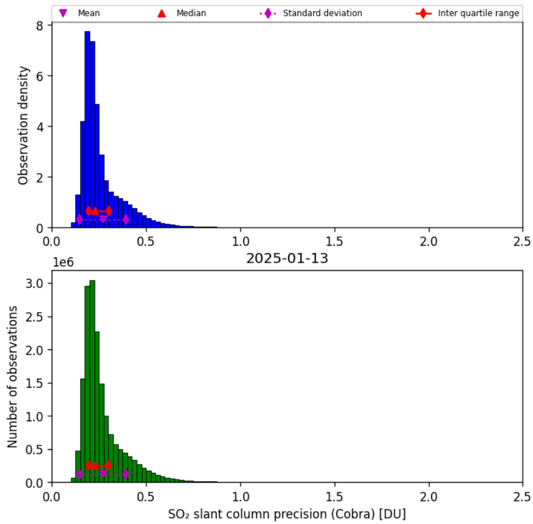
Figure 62: Histogram of “SO 2 slant column precision (Cobra)” for 2025-01-13 to 2025-01-14
