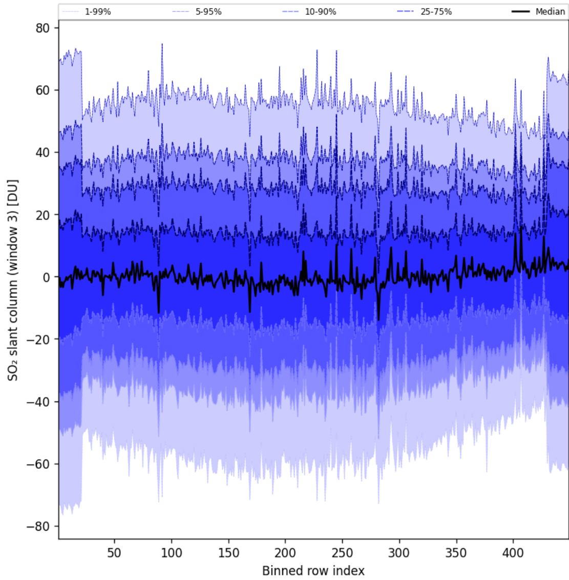
Figure 98: Along track statistics of “SO 2 slant column (window 3)” for 2025-01-13 to 2025-01-14
