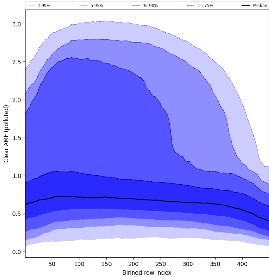
Figure 109: Along track statistics of “Clear AMF (polluted)” for 2025-01-13 to 2025-01-14
