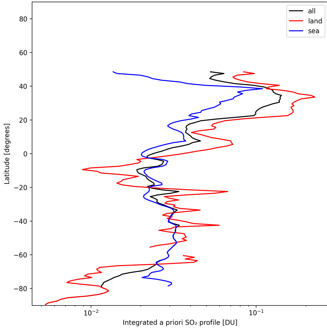
Figure 49: Zonal average of “Integrated a priori SO 2 profile” for 2025-01-13 to 2025-01-14.
