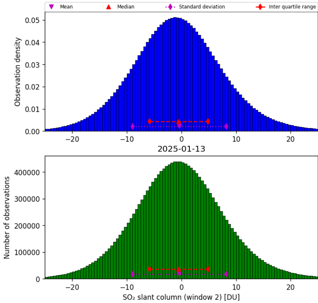
Figure 67: Histogram of “SO 2 slant column (window 2)” for 2025-01-13 to 2025-01-14
