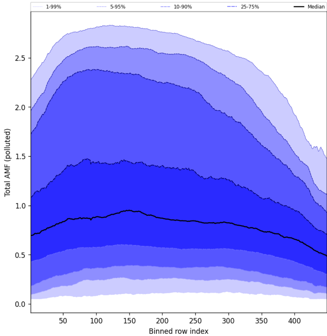
Figure 107: Along track statistics of “Total AMF (polluted)” for 2025-01-13 to 2025-01-14
