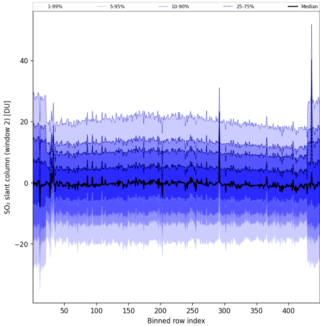
Figure 94: Along track statistics of “SO 2 slant column (window 2)” for 2025-01-13 to 2025-01-14
