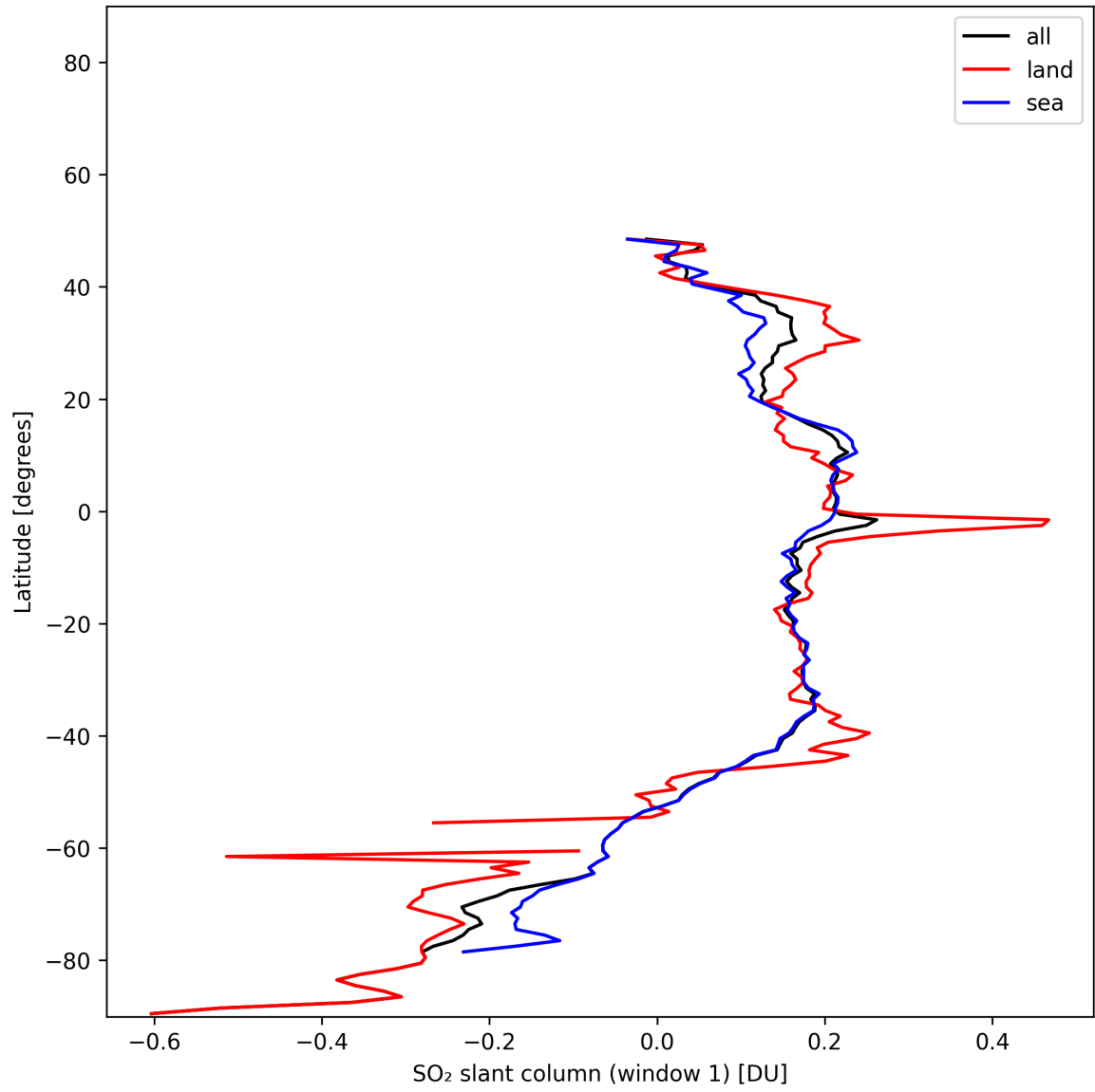
Figure 36: Zonal average of “SO 2 slant column (window 1)” for 2025-01-13 to 2025-01-14.
