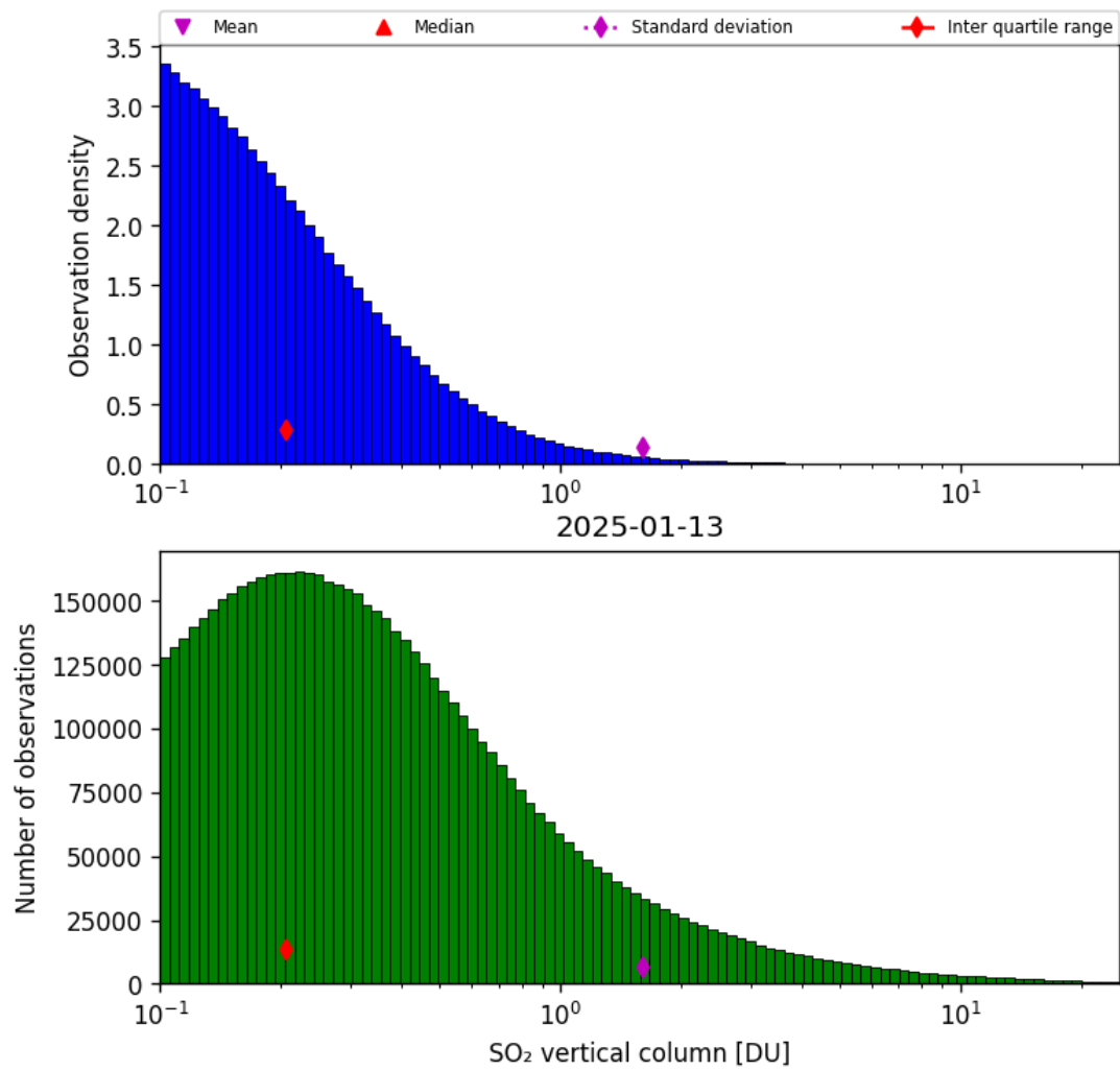
Figure 58: Histogram of “SO 2 vertical column” for 2025-01-13 to 2025-01-14
