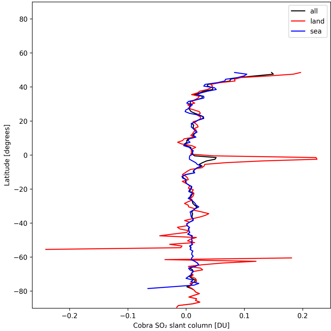
Figure 34: Zonal average of “Cobra SO 2 slant column” for 2025-01-13 to 2025-01-14.
