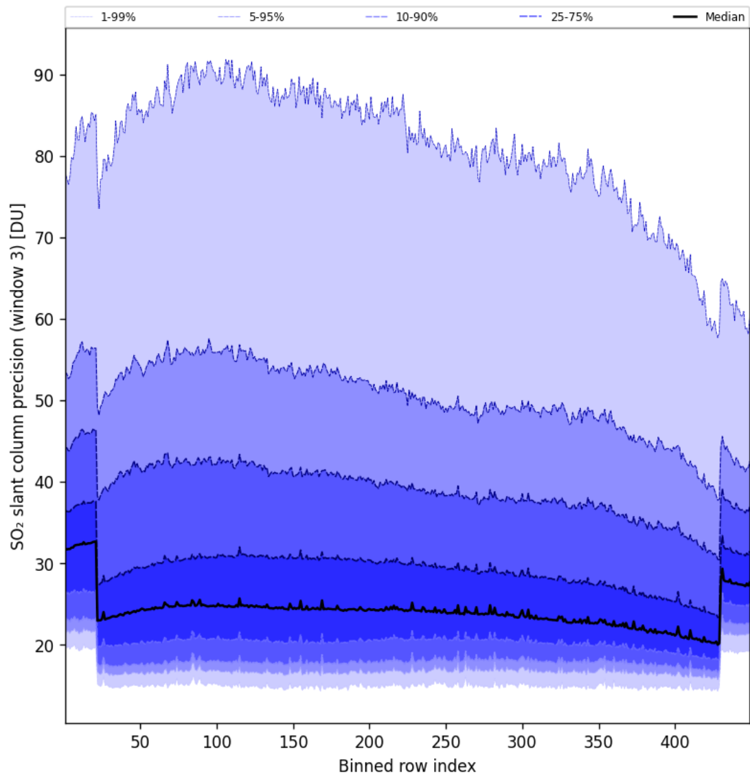
Figure 99: Along track statistics of “SO 2 slant column precision (window 3)” for 2025-01-13 to 2025-01-14
