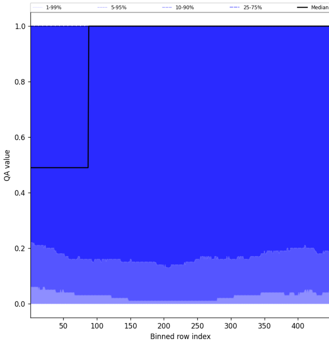
Figure 84: Along track statistics of “QA value” for 2025-01-13 to 2025-01-14
