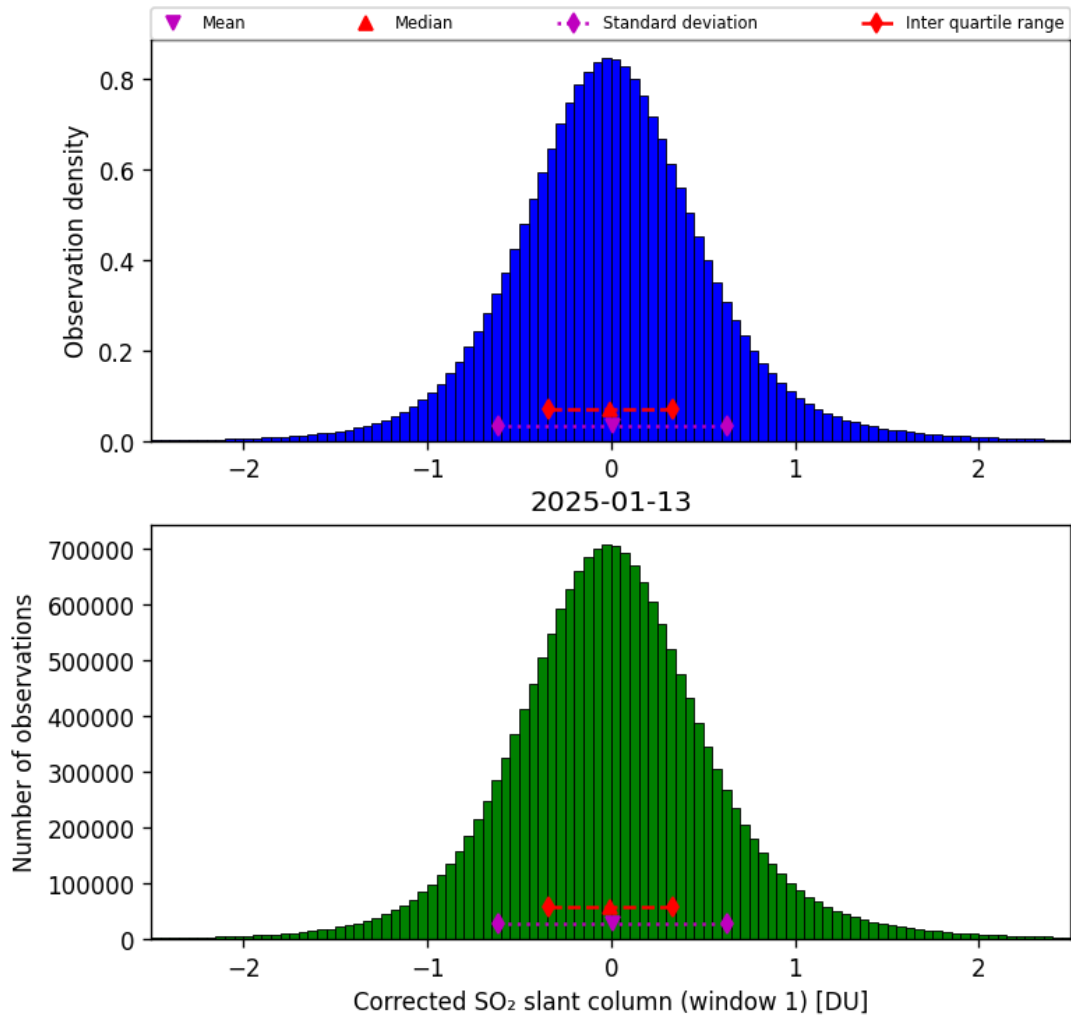
Figure 65: Histogram of “Corrected SO 2 slant column (window 1)” for 2025-01-13 to 2025-01-14
