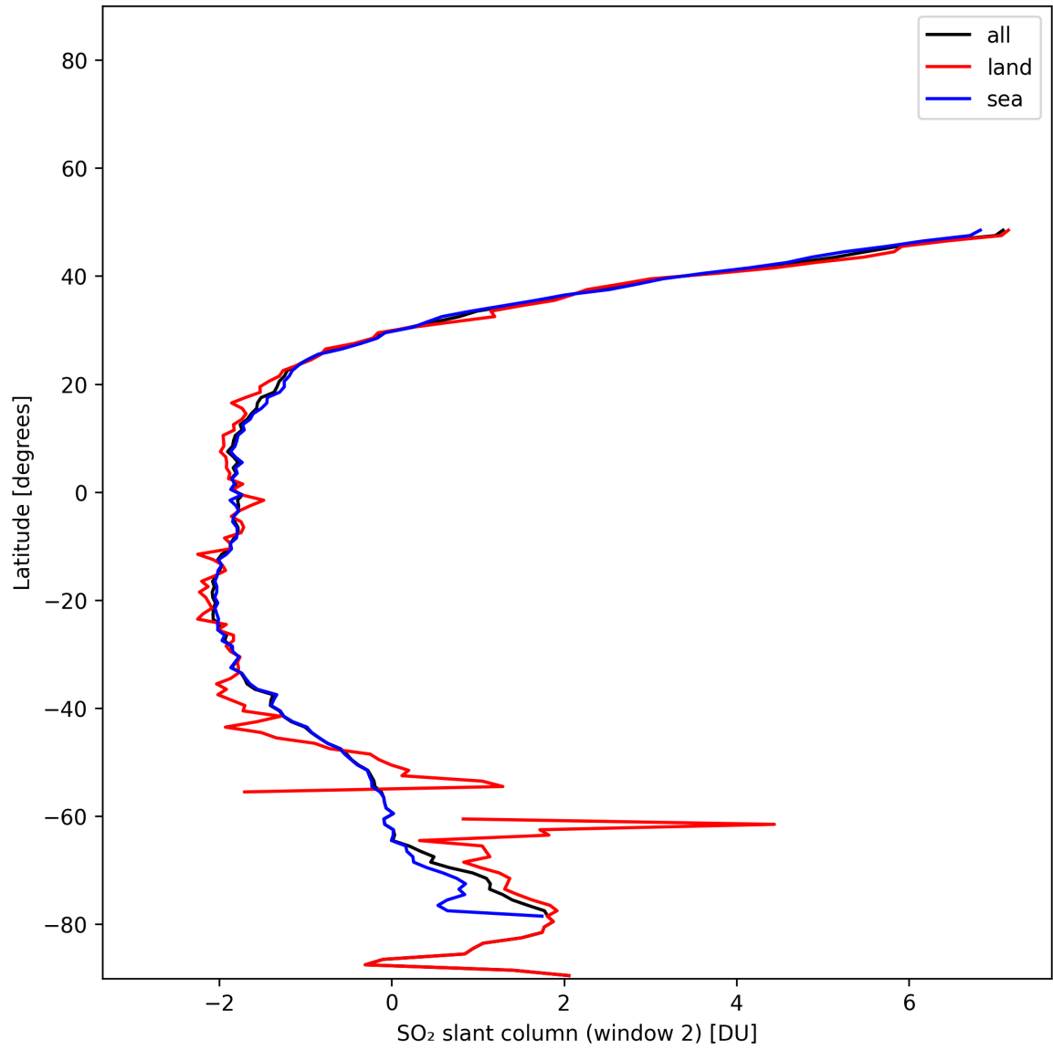
Figure 40: Zonal average of “SO 2 slant column (window 2)” for 2025-01-13 to 2025-01-14.
