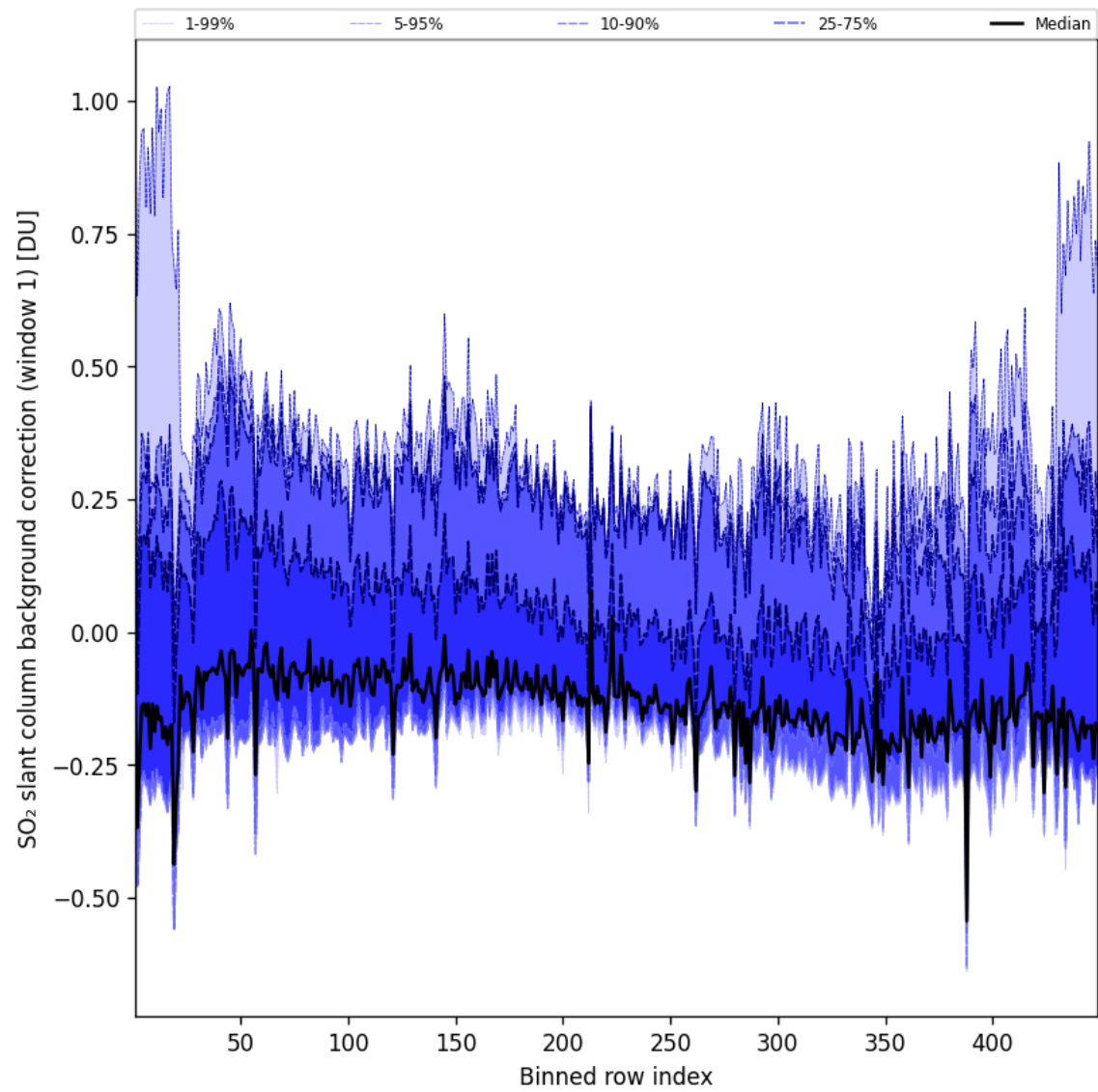
Figure 93: Along track statistics of “SO 2 slant column background correction (window 1)” for 2025-01-13 to 2025-01-14
