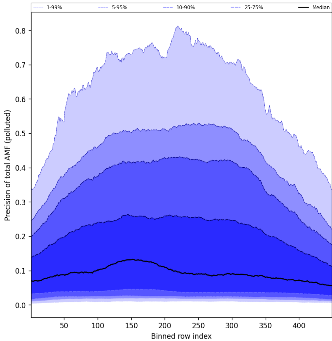
Figure 108: Along track statistics of “Precision of total AMF (polluted)” for 2025-01-13 to 2025-01-14
