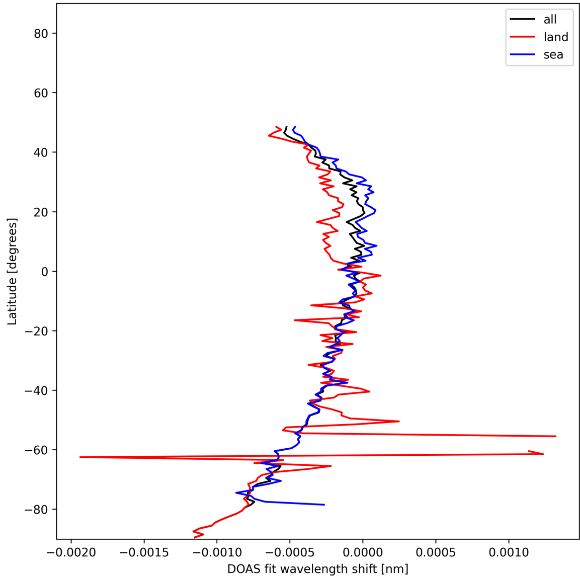
Figure 50: Zonal average of "DOAS fit wavelength shift" for 2025-01-13 to 2025-01-14.
