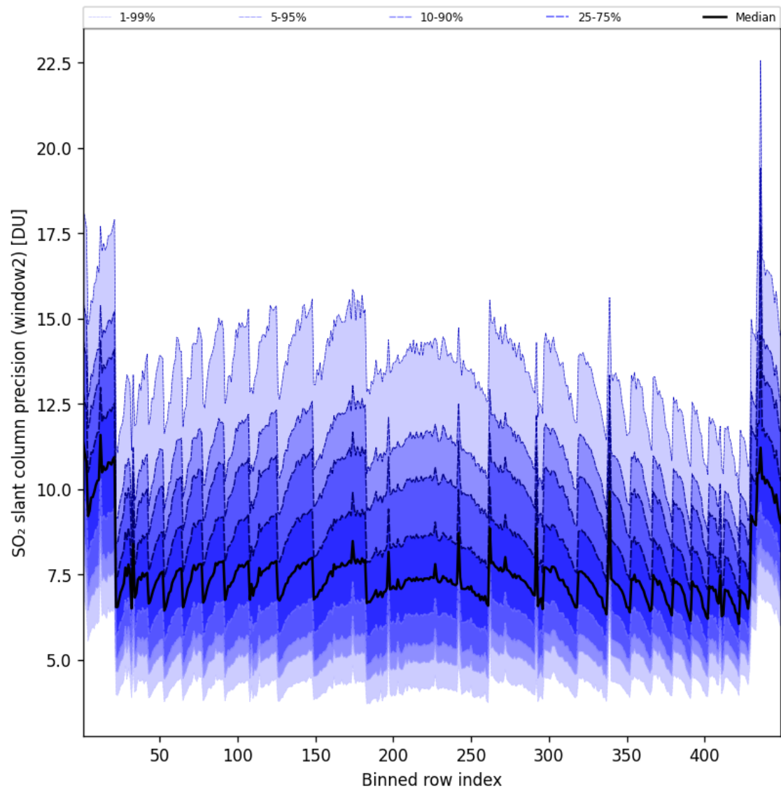
Figure 95: Along track statistics of “SO 2 slant column precision (window2)” for 2025-01-13 to 2025-01-14
