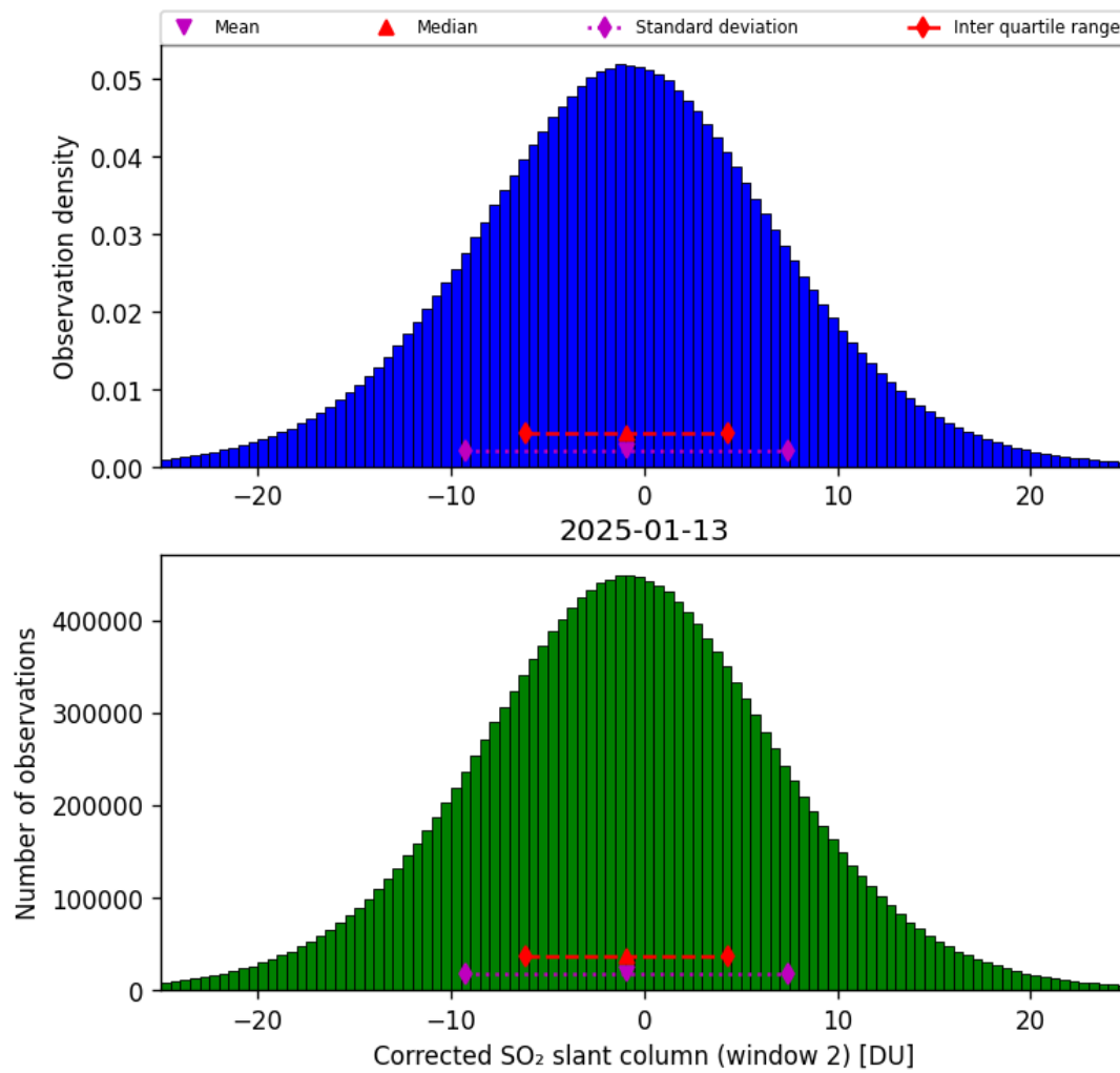
Figure 69: Histogram of “Corrected SO 2 slant column (window 2)” for 2025-01-13 to 2025-01-14
