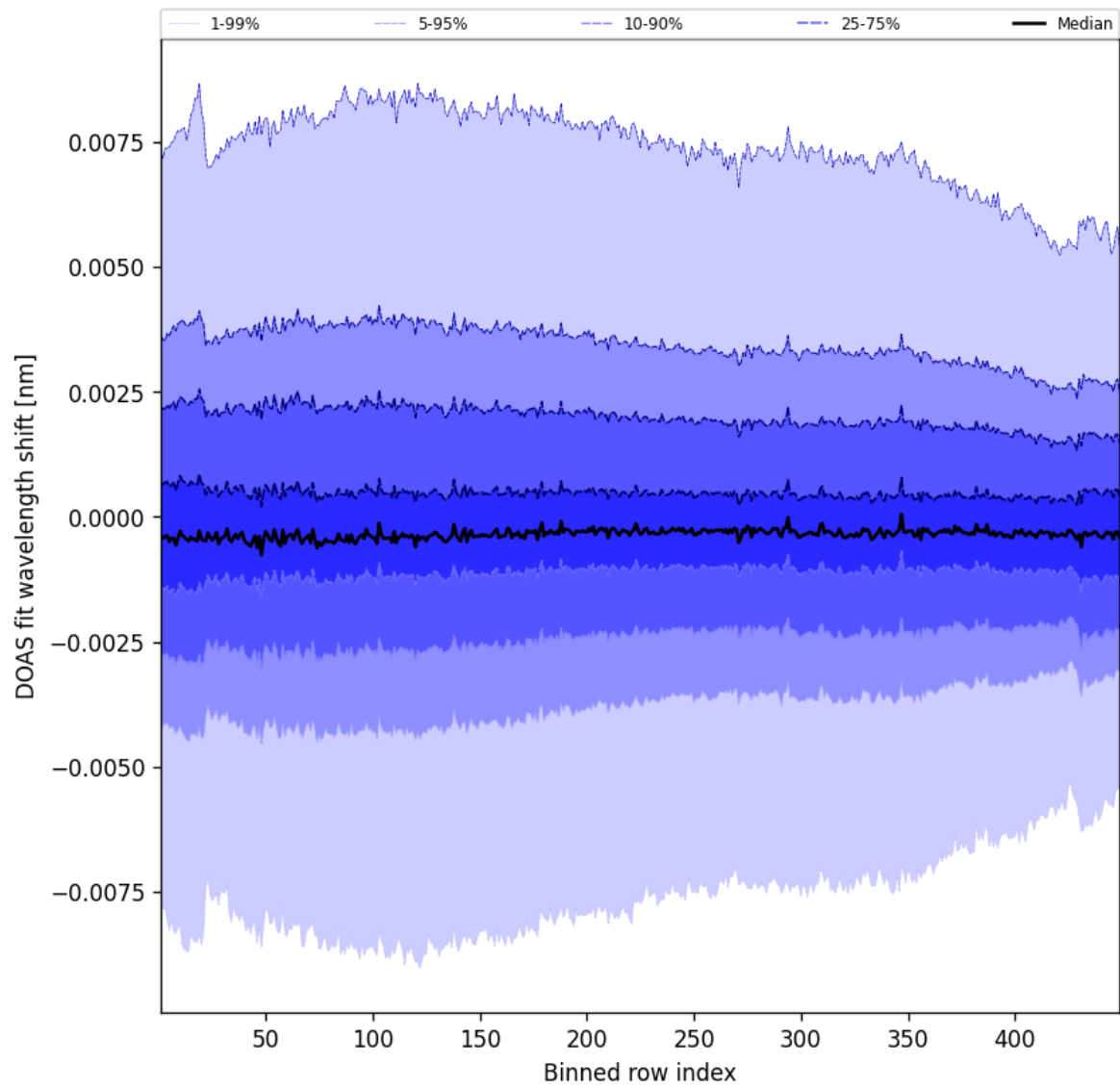
Figure 104: Along track statistics of “DOAS fit wavelength shift” for 2025-01-13 to 2025-01-14
