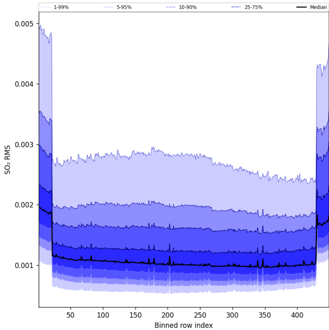
Figure 106: Along track statistics of “SO 2 RMS” for 2025-01-13 to 2025-01-14
