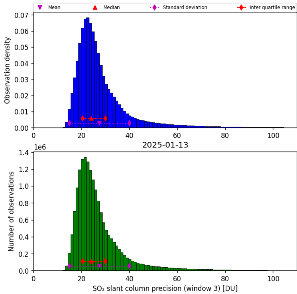
Figure 72: Histogram of “SO 2 slant column precision (window 3)” for 2025-01-13 to 2025-01-14
