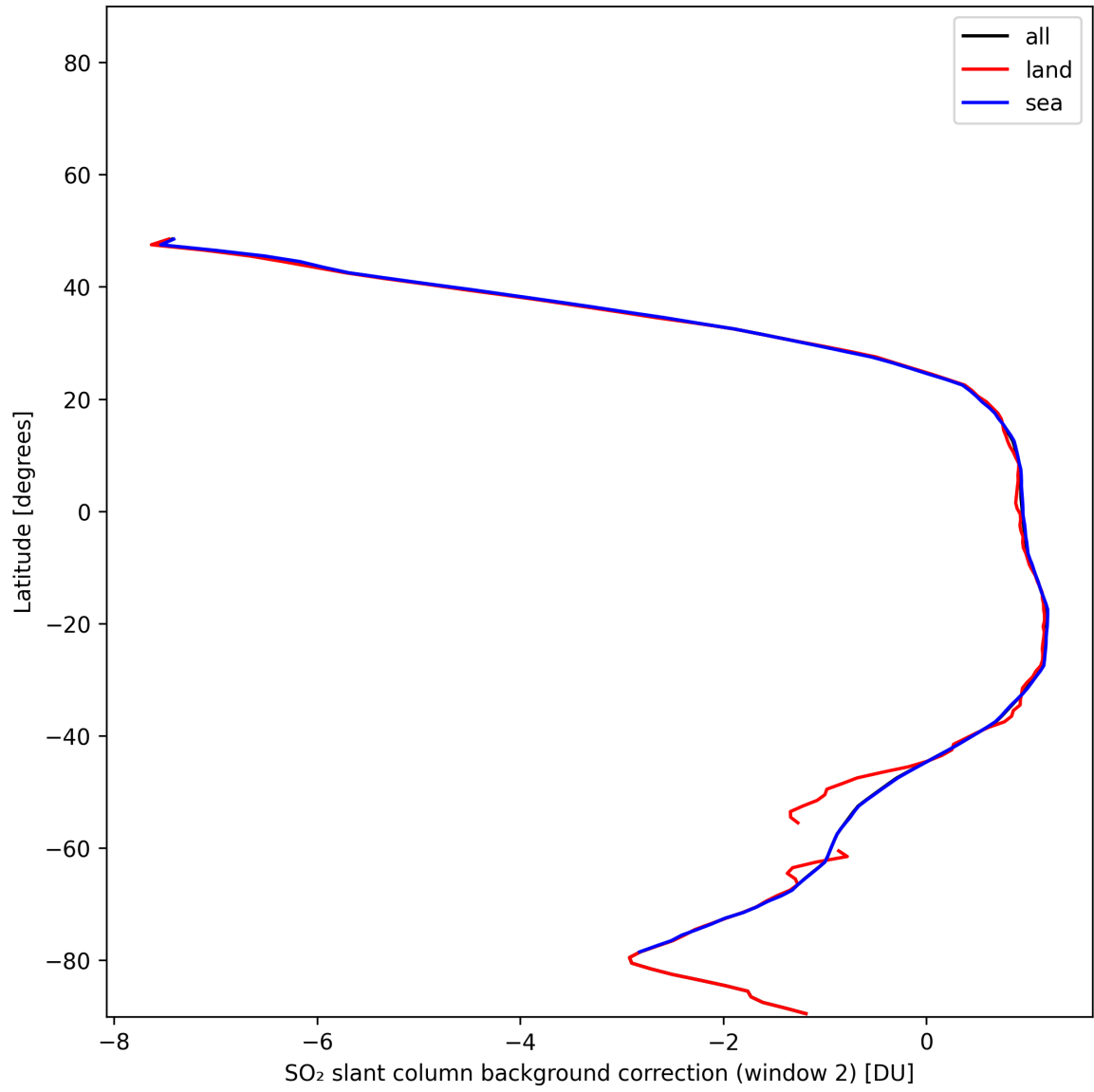
Figure 43: Zonal average of “SO 2 slant column background correction (window 2)” for 2025-01-13 to 2025-01-14.
