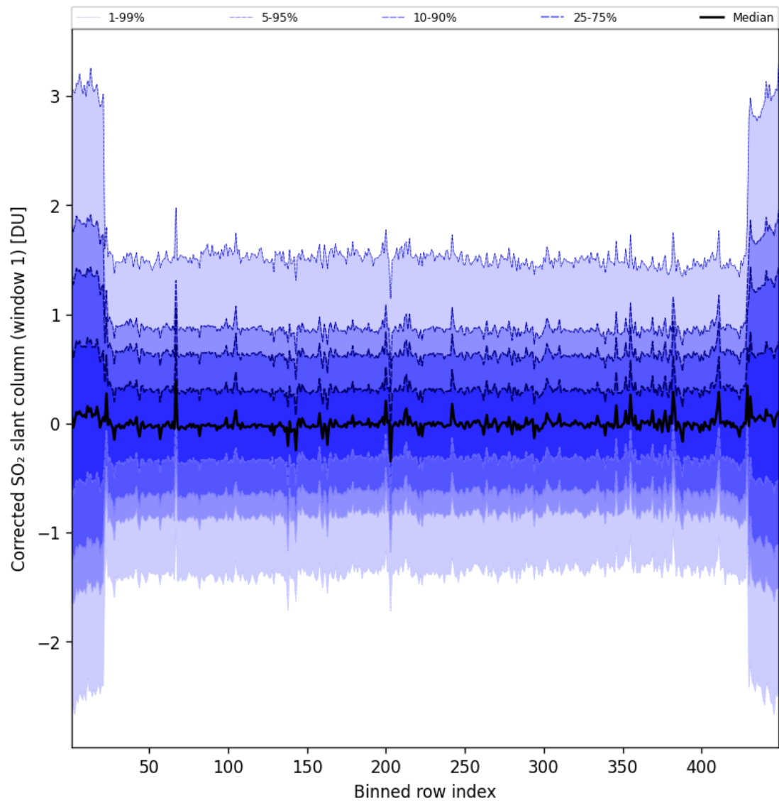
Figure 92: Along track statistics of “Corrected SO 2 slant column (window 1)” for 2025-01-13 to 2025-01-14
