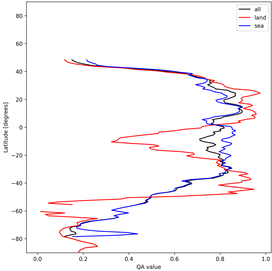
Figure 30: Zonal average of “QA value” for 2025-01-13 to 2025-01-14.
