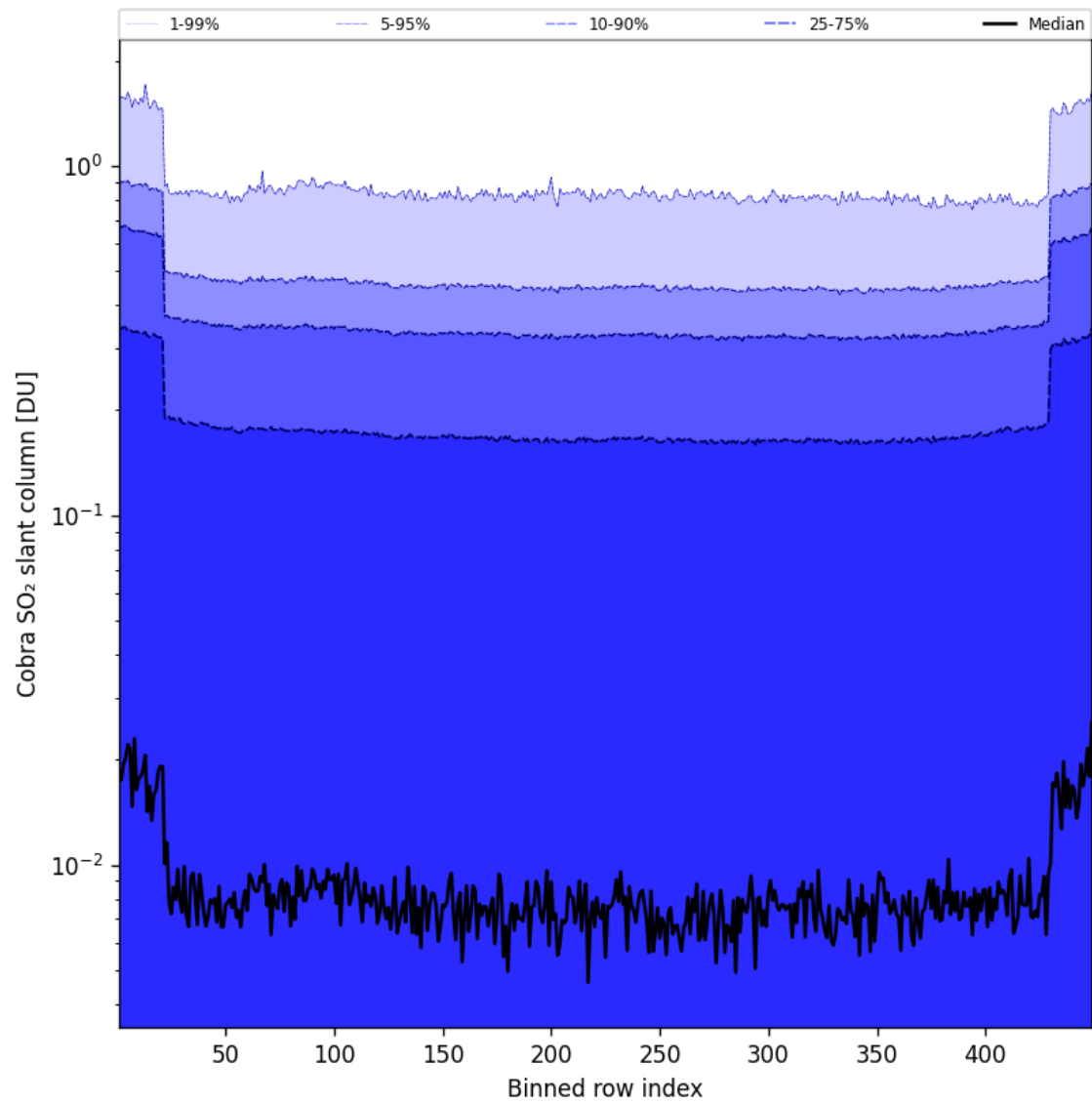
Figure 88: Along track statistics of “Cobra SO 2 slant column” for 2025-01-13 to 2025-01-14
