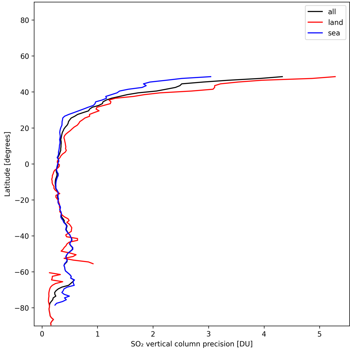
Figure 32: Zonal average of “SO 2 vertical column precision” for 2025-01-13 to 2025-01-14.
