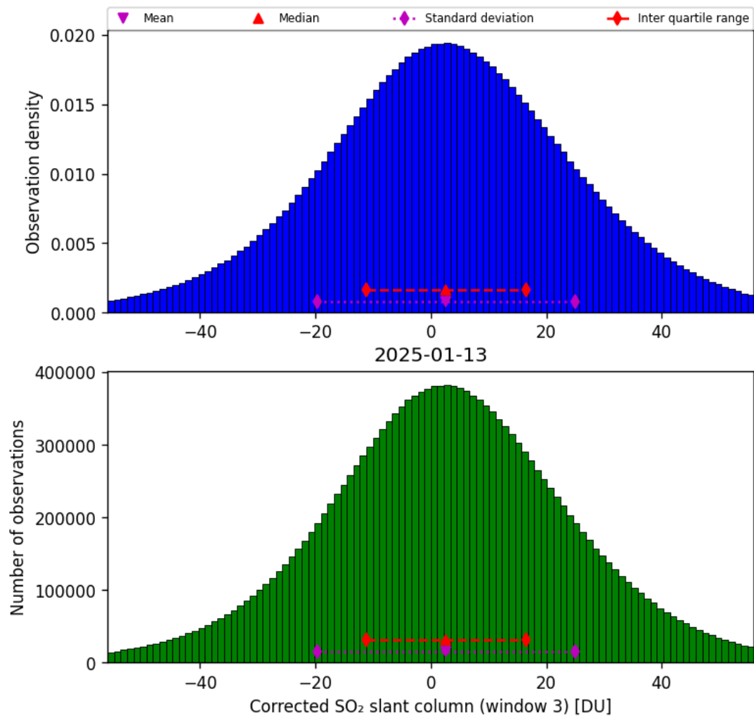
Figure 73: Histogram of “Corrected SO 2 slant column (window 3)” for 2025-01-13 to 2025-01-14
