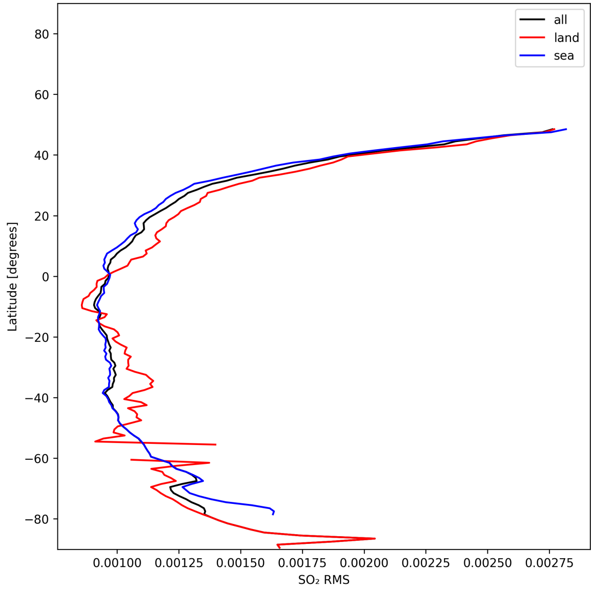
Figure 52: Zonal average of “SO 2 RMS” for 2025-01-13 to 2025-01-14.
