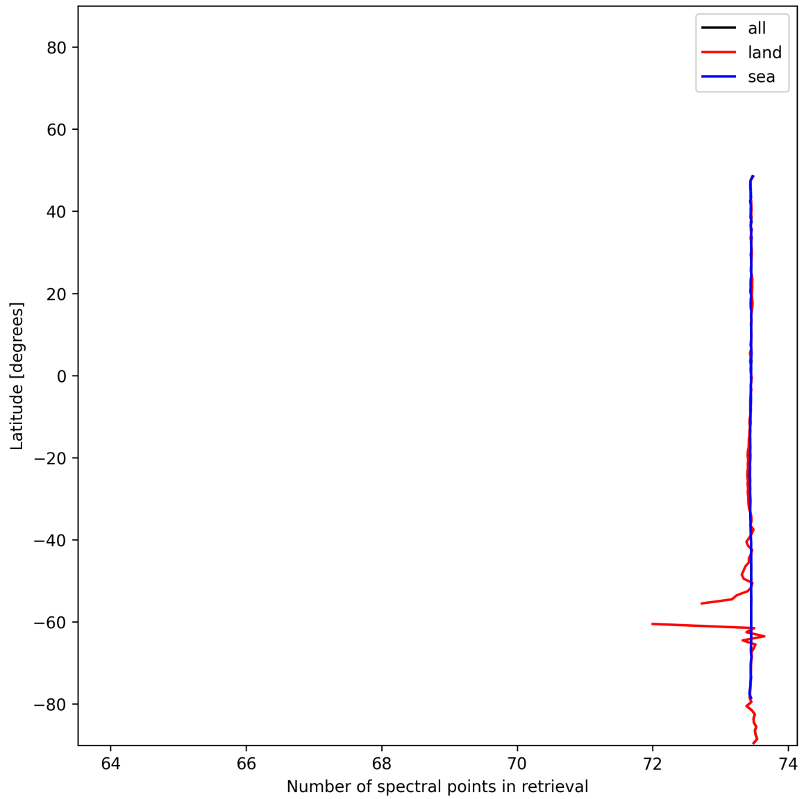
Figure 56: Zonal average of “Number of spectral points in retrieval” for 2025-01-13 to 2025-01-14.
