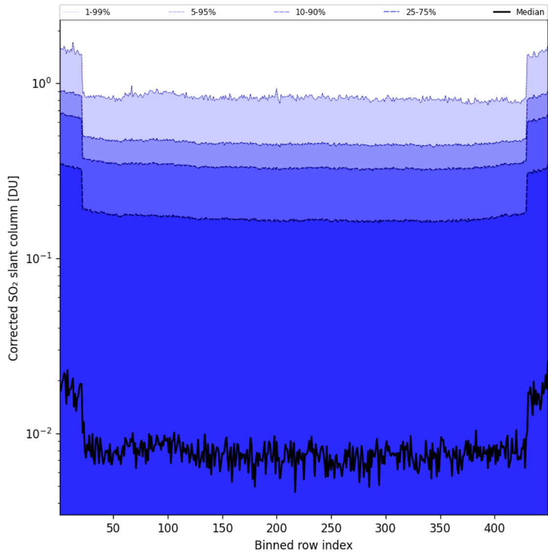
Figure 87: Along track statistics of "Corrected SO 2 slant column" for 2025-01-13 to 2025-01-14
