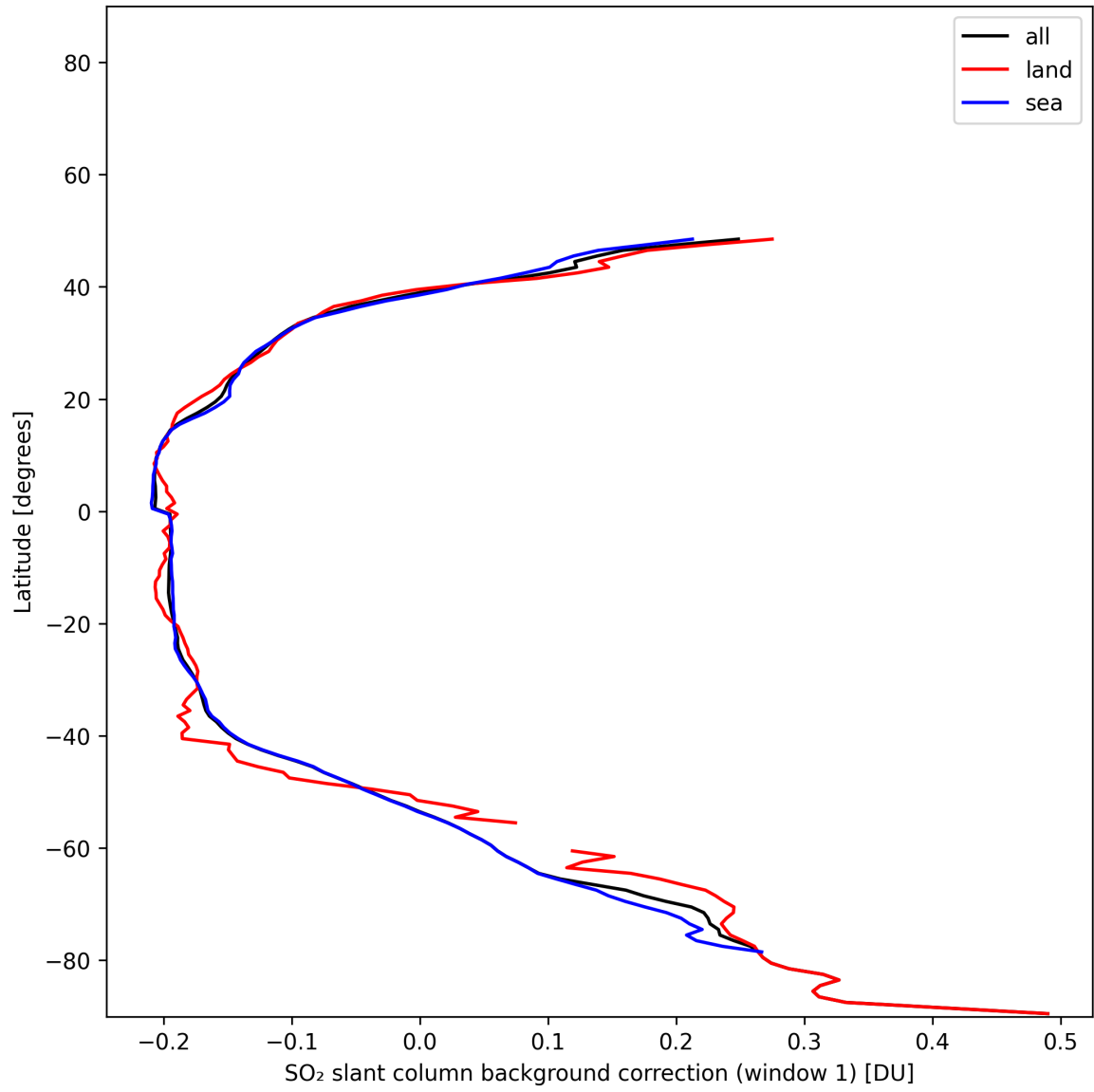
Figure 39: Zonal average of "SO 2 slant column background correction (window 1)" for 2025-01-13 to 2025-01-14.
