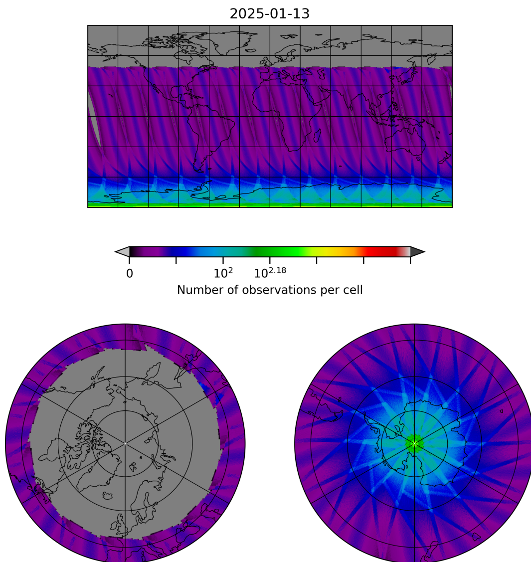
Figure 29: Map of the number of observations for 2025-01-13 to 2025-01-14
