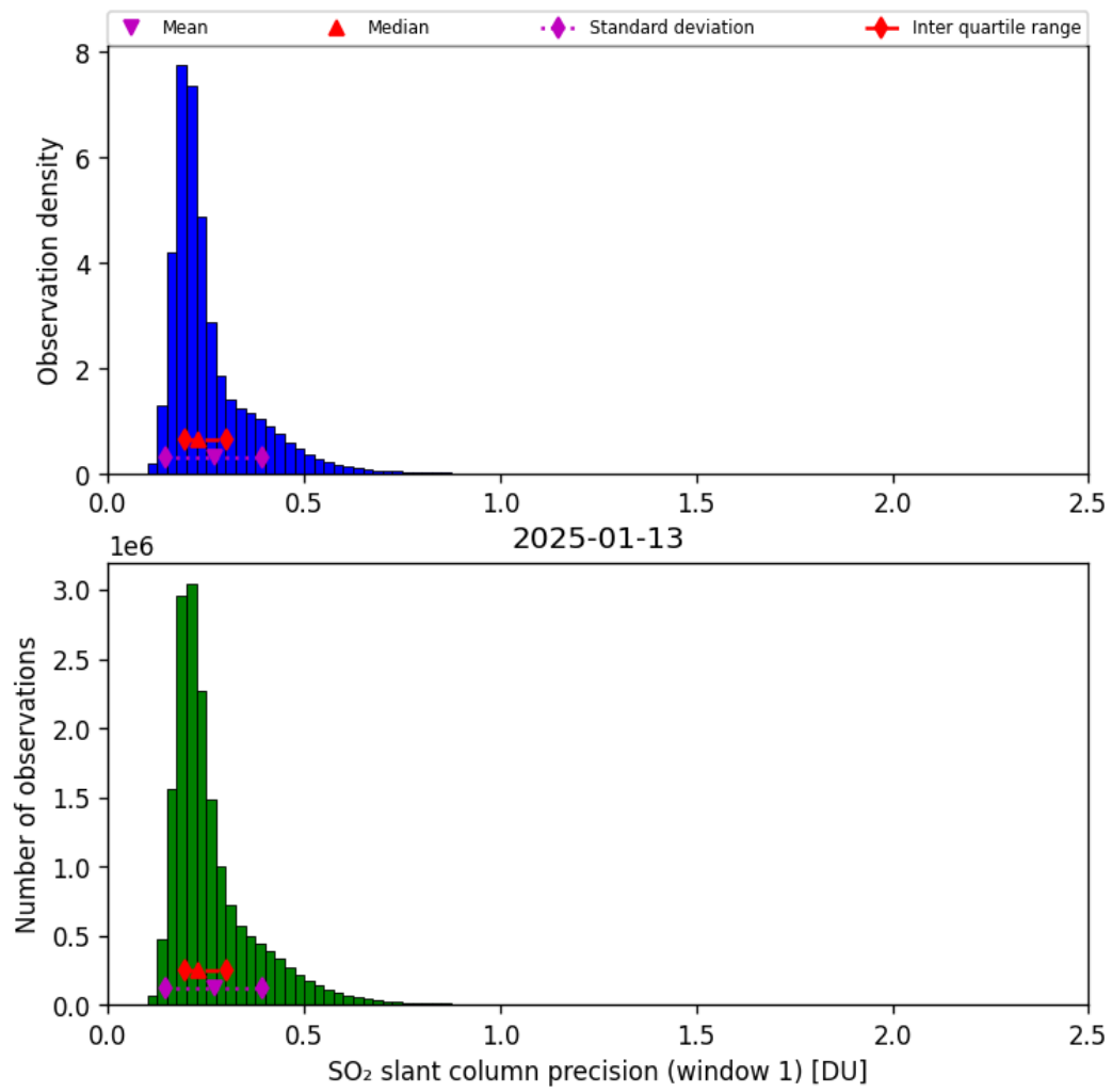
Figure 64: Histogram of “SO 2 slant column precision (window 1)” for 2025-01-13 to 2025-01-14
