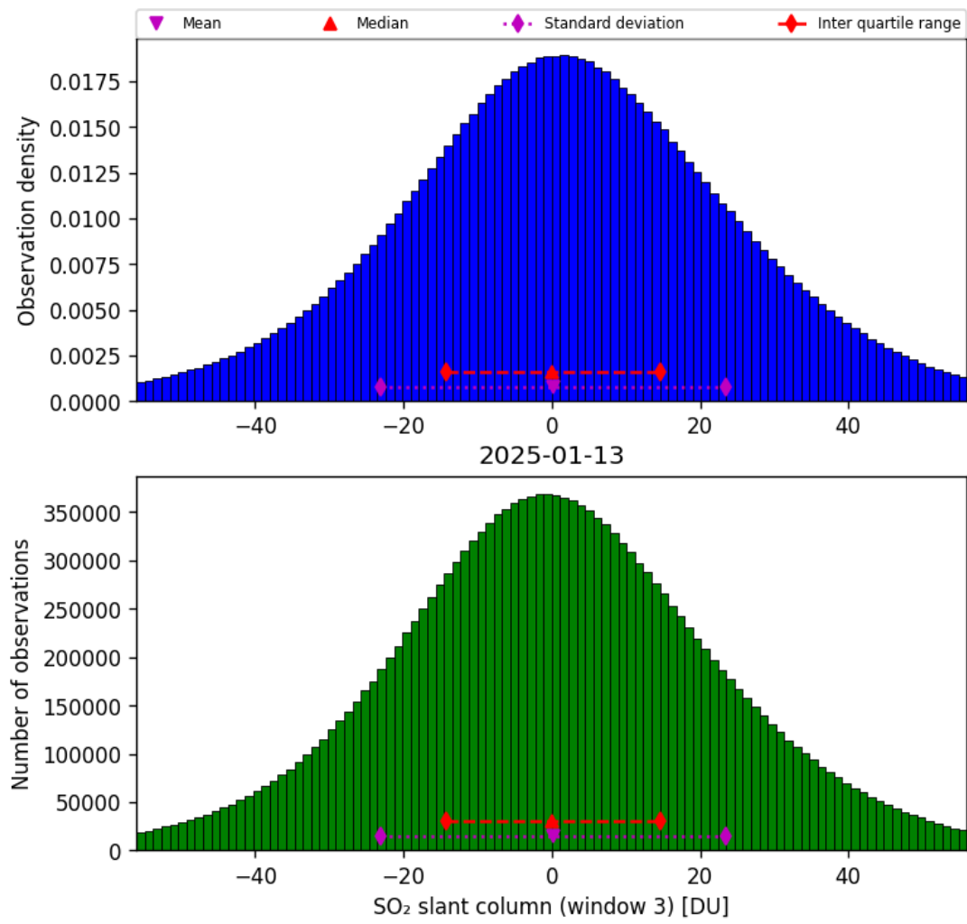
Figure 71: Histogram of “SO 2 slant column (window 3)” for 2025-01-13 to 2025-01-14
