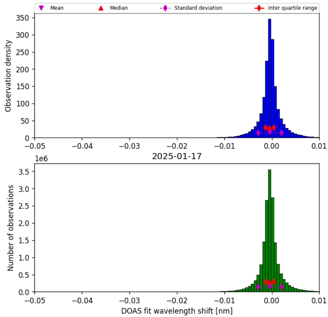
Figure 77: Histogram of “DOAS fit wavelength shift” for 2025-01-17 to 2025-01-18
