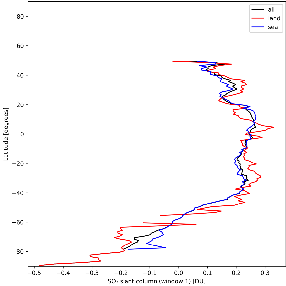
Figure 36: Zonal average of “SO 2 slant column (window 1)” for 2025-01-17 to 2025-01-18.
