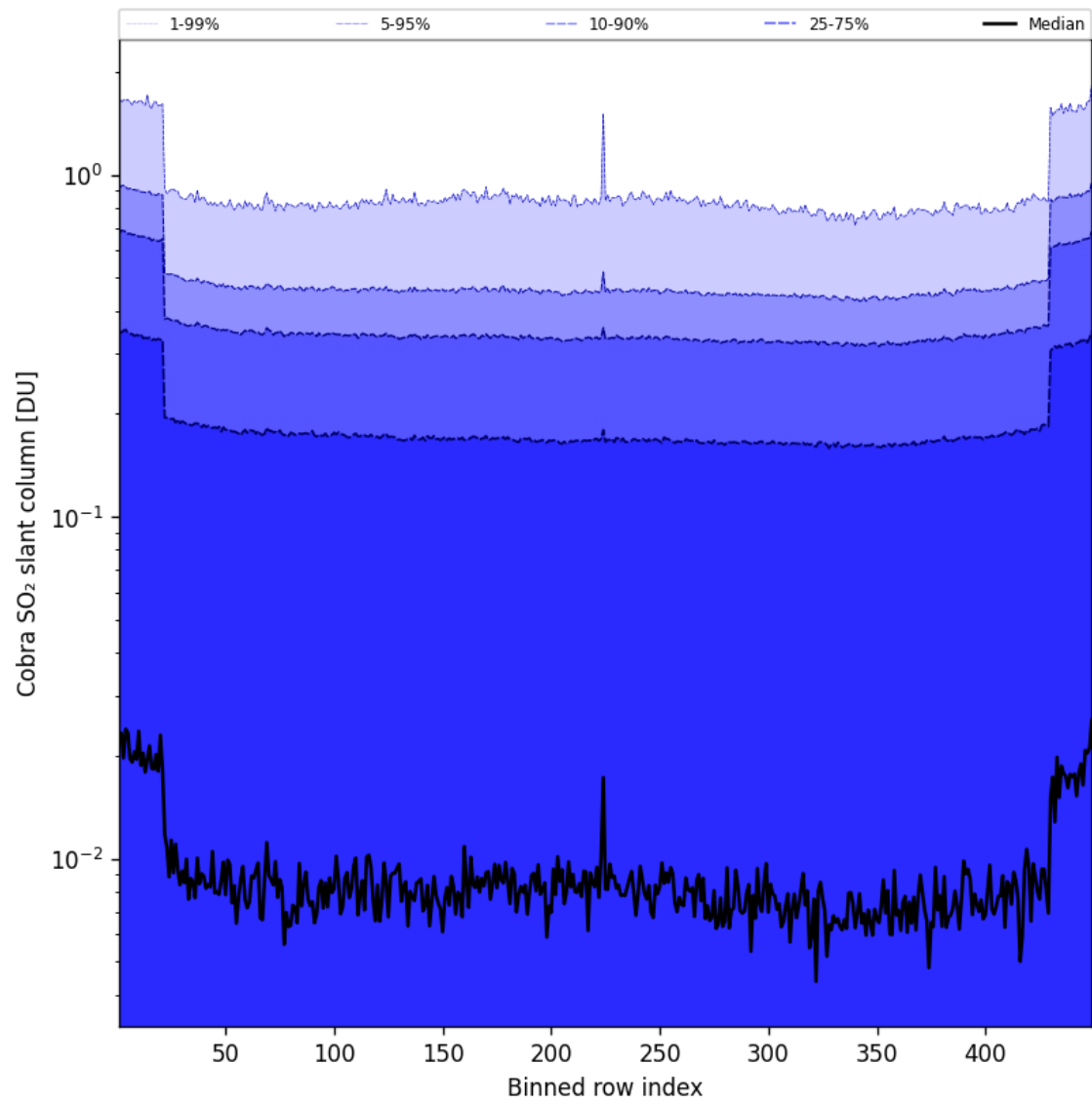
Figure 88: Along track statistics of “Cobra SO 2 slant column” for 2025-01-17 to 2025-01-18
