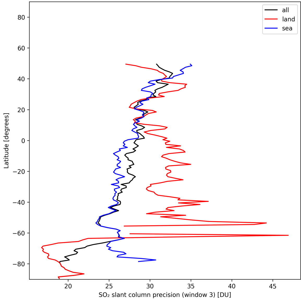
Figure 45: Zonal average of “SO 2 slant column precision (window 3)” for 2025-01-17 to 2025-01-18.
