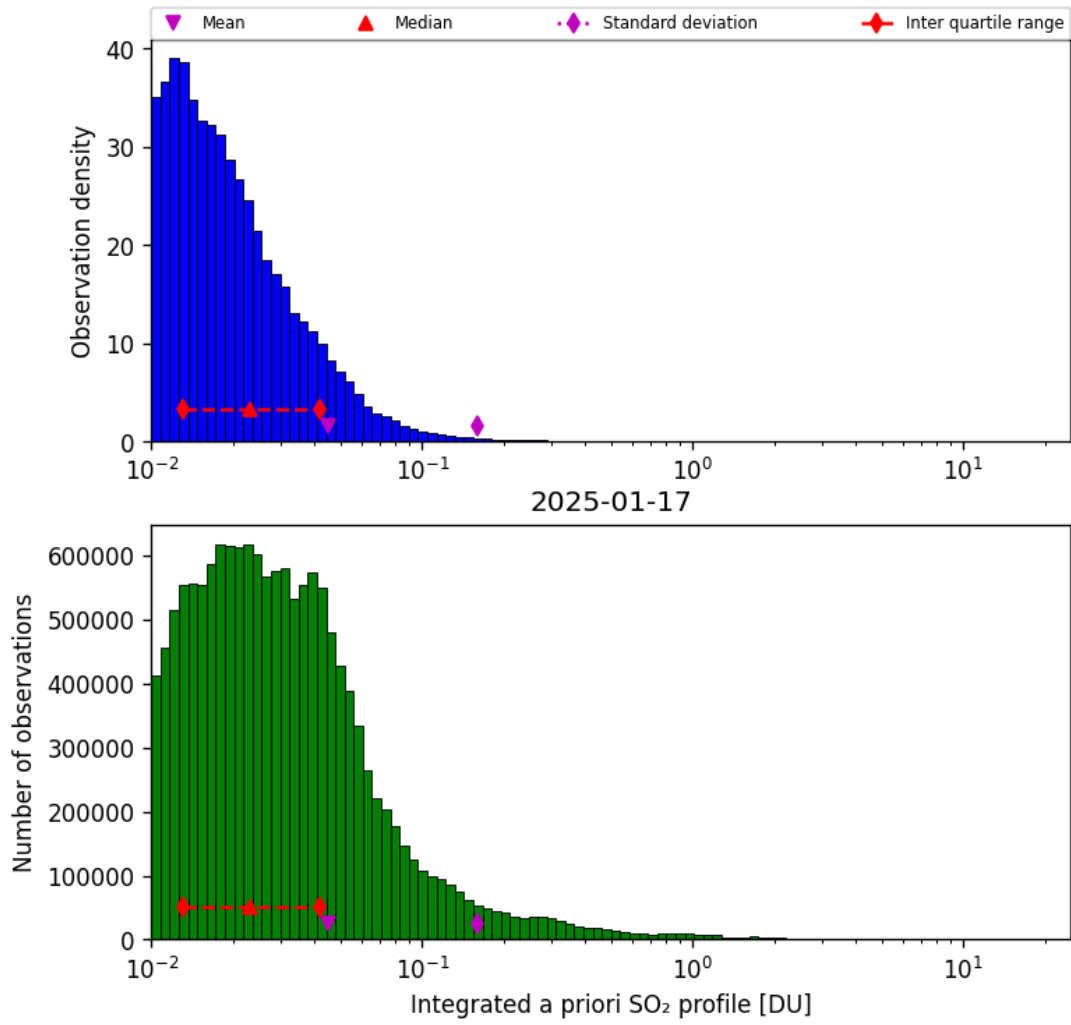
Figure 76: Histogram of “Integrated a priori SO 2 profile” for 2025-01-17 to 2025-01-18
