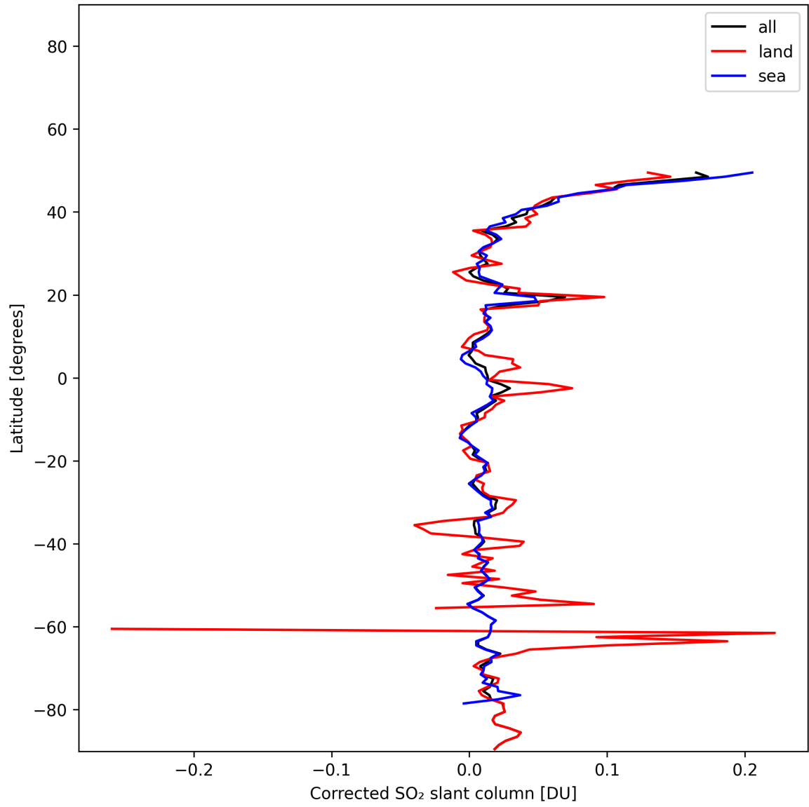
Figure 33: Zonal average of “Corrected SO 2 slant column” for 2025-01-17 to 2025-01-18.
