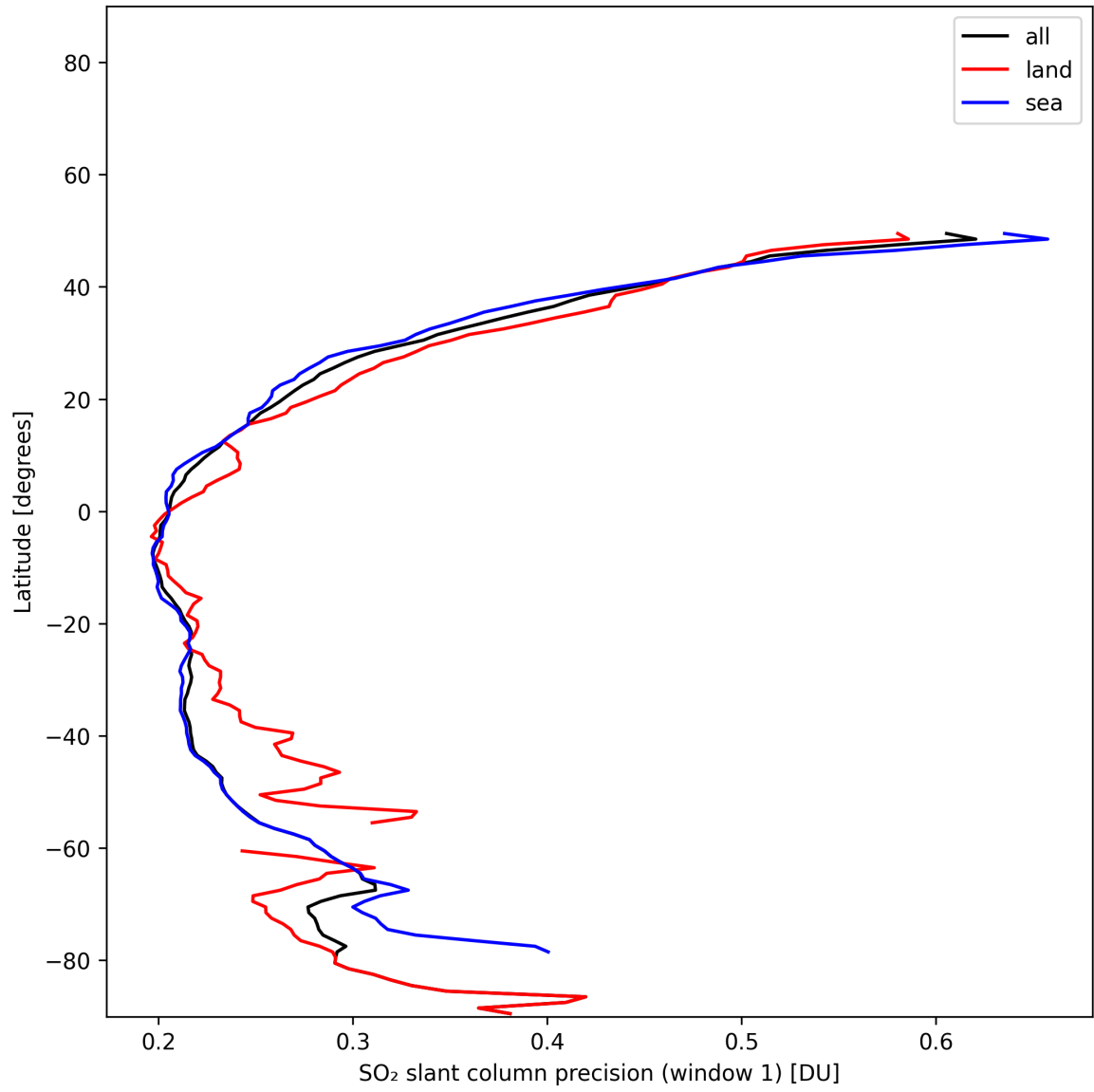
Figure 37: Zonal average of “SO 2 slant column precision (window 1)” for 2025-01-17 to 2025-01-18.
