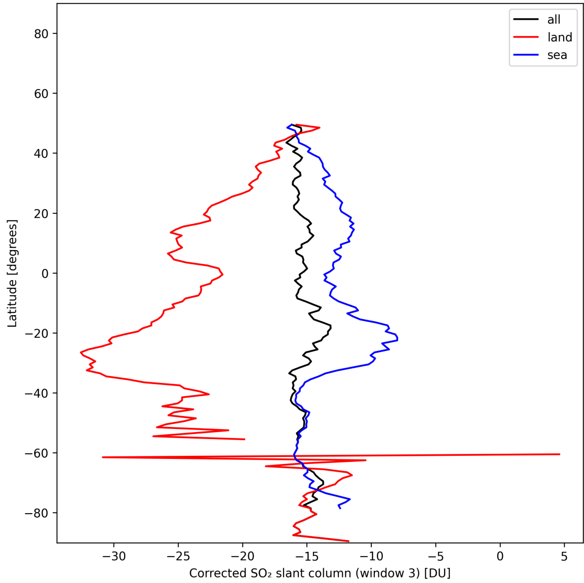
Figure 46: Zonal average of “Corrected SO 2 slant column (window 3)” for 2025-01-17 to 2025-01-18.
