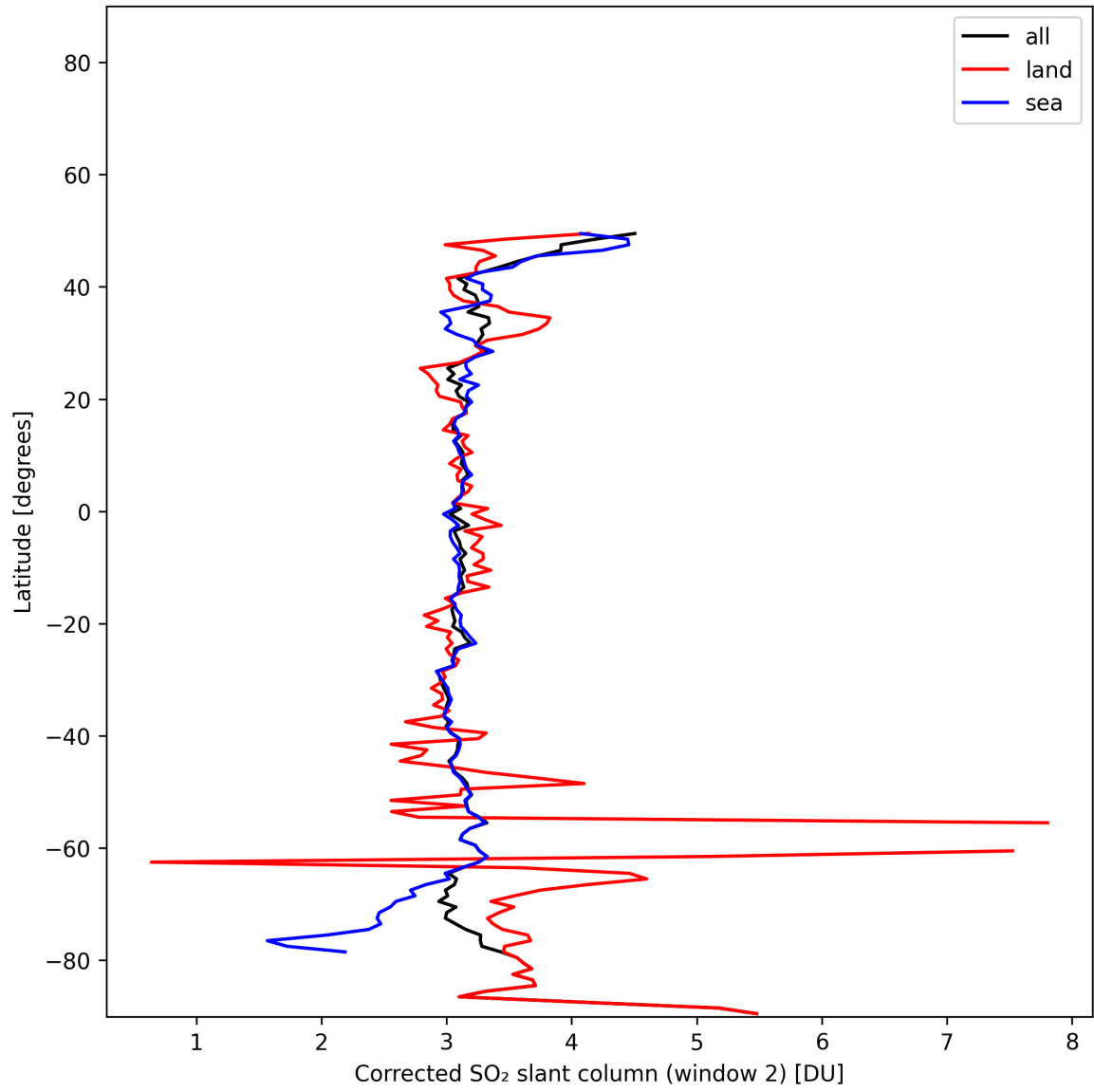
Figure 42: Zonal average of “Corrected SO 2 slant column (window 2)” for 2025-01-17 to 2025-01-18.
