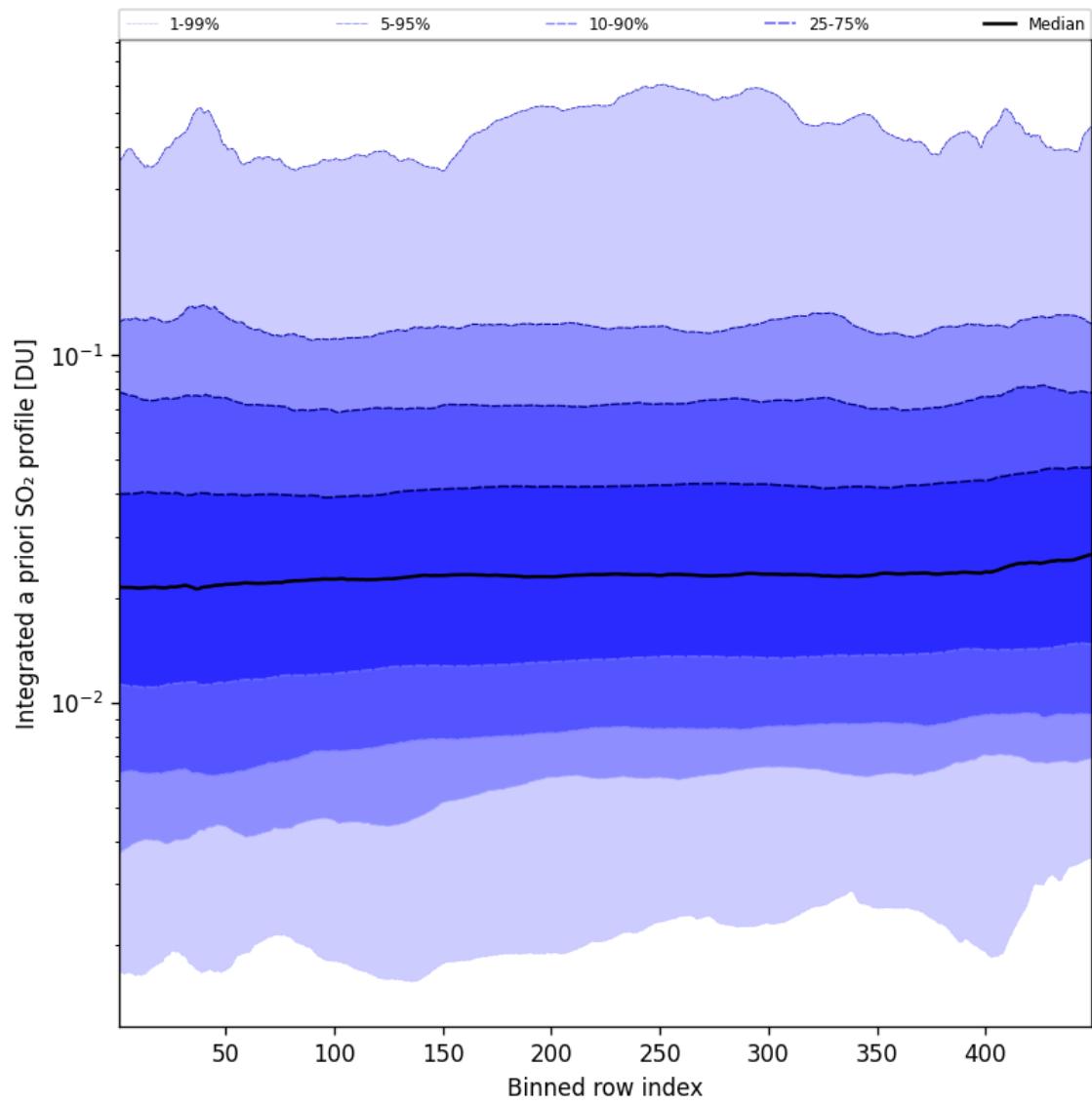
Figure 103: Along track statistics of “Integrated a priori SO 2 profile” for 2025-01-17 to 2025-01-18
