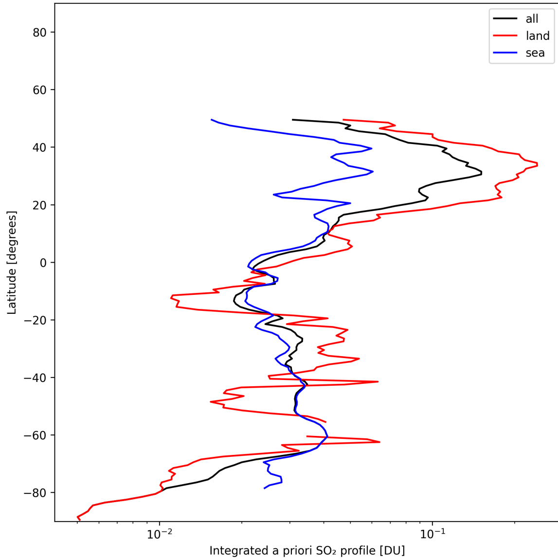
Figure 49: Zonal average of “Integrated a priori SO 2 profile” for 2025-01-17 to 2025-01-18.
