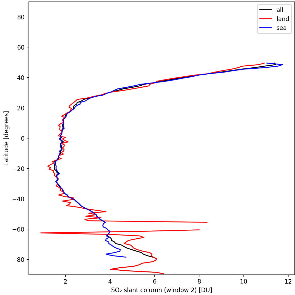
Figure 40: Zonal average of “SO 2 slant column (window 2)” for 2025-01-17 to 2025-01-18.
