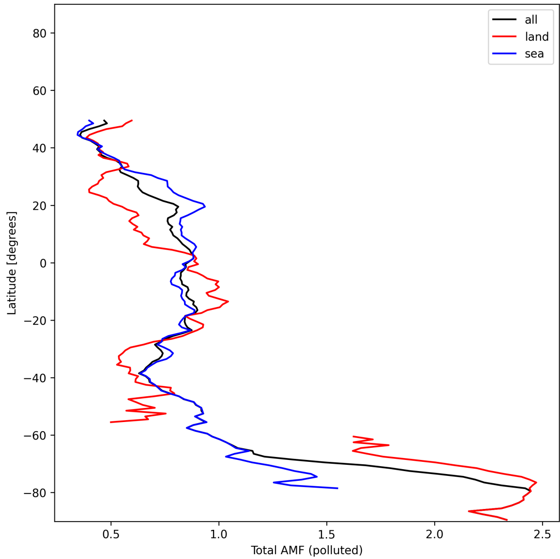
Figure 53: Zonal average of “Total AMF (polluted)” for 2025-01-17 to 2025-01-18.
