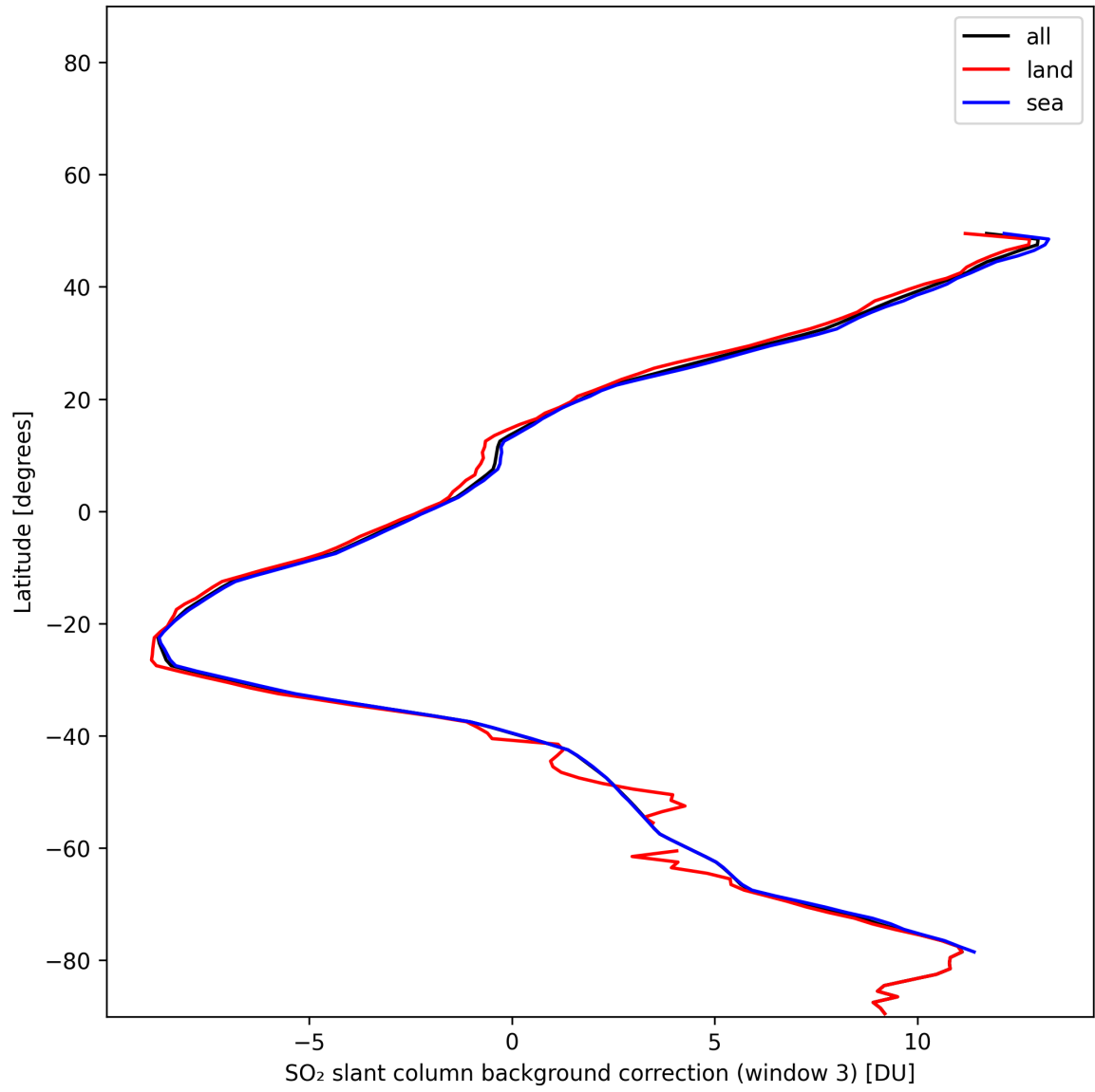
Figure 47: Zonal average of “SO 2 slant column background correction (window 3)” for 2025-01-17 to 2025-01-18.
