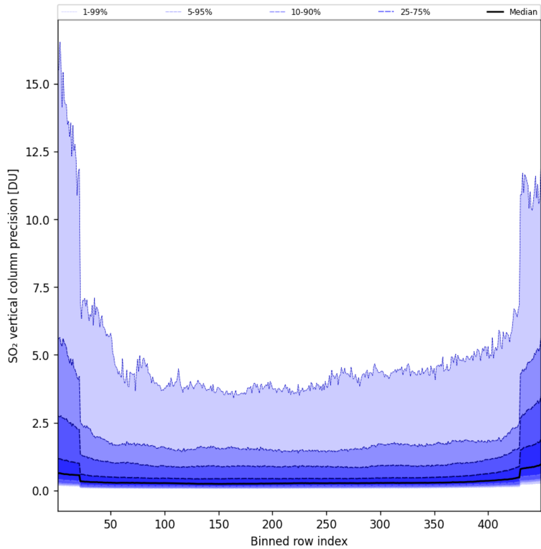
Figure 86: Along track statistics of “SO 2 vertical column precision” for 2025-01-17 to 2025-01-18
