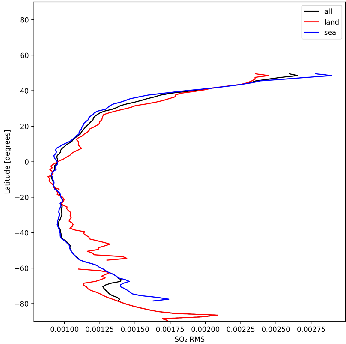
Figure 52: Zonal average of “SO 2 RMS” for 2025-01-17 to 2025-01-18.
