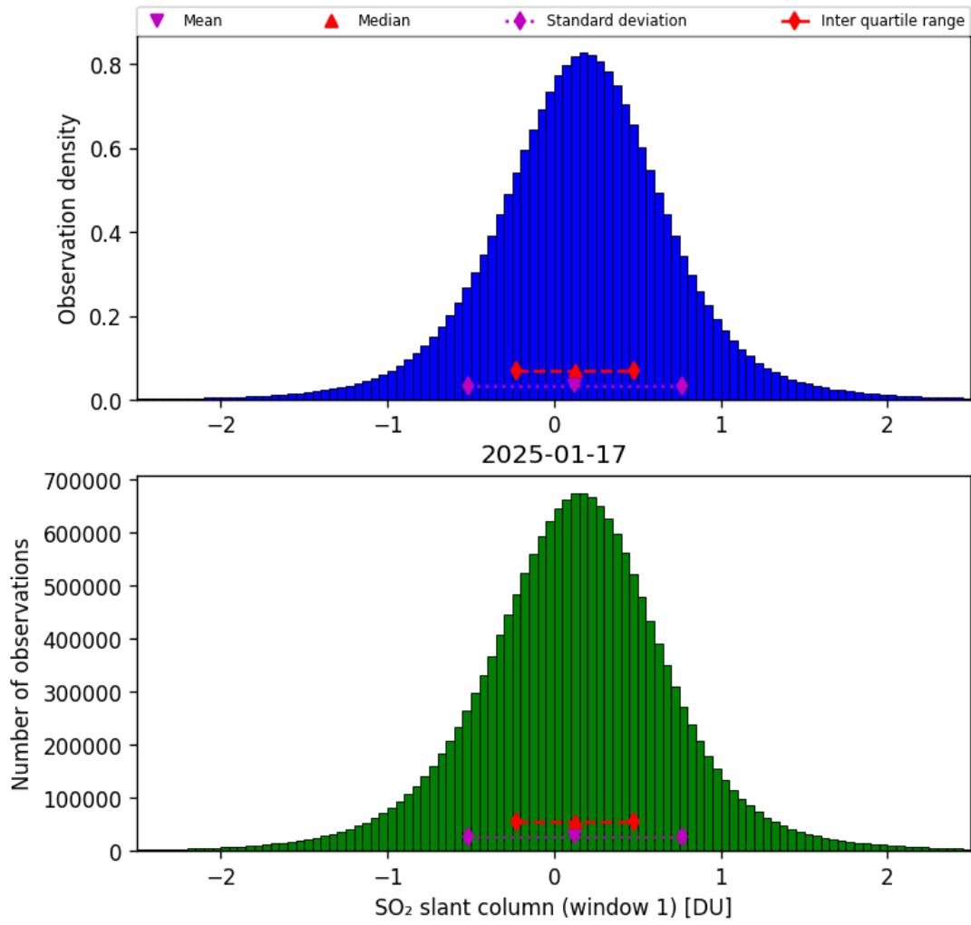
Figure 63: Histogram of “SO 2 slant column (window 1)” for 2025-01-17 to 2025-01-18
