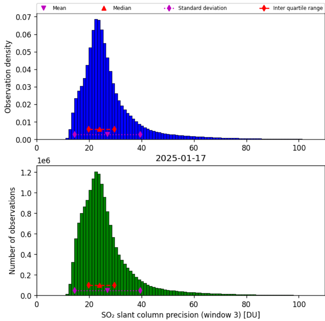
Figure 72: Histogram of “SO 2 slant column precision (window 3)” for 2025-01-17 to 2025-01-18
