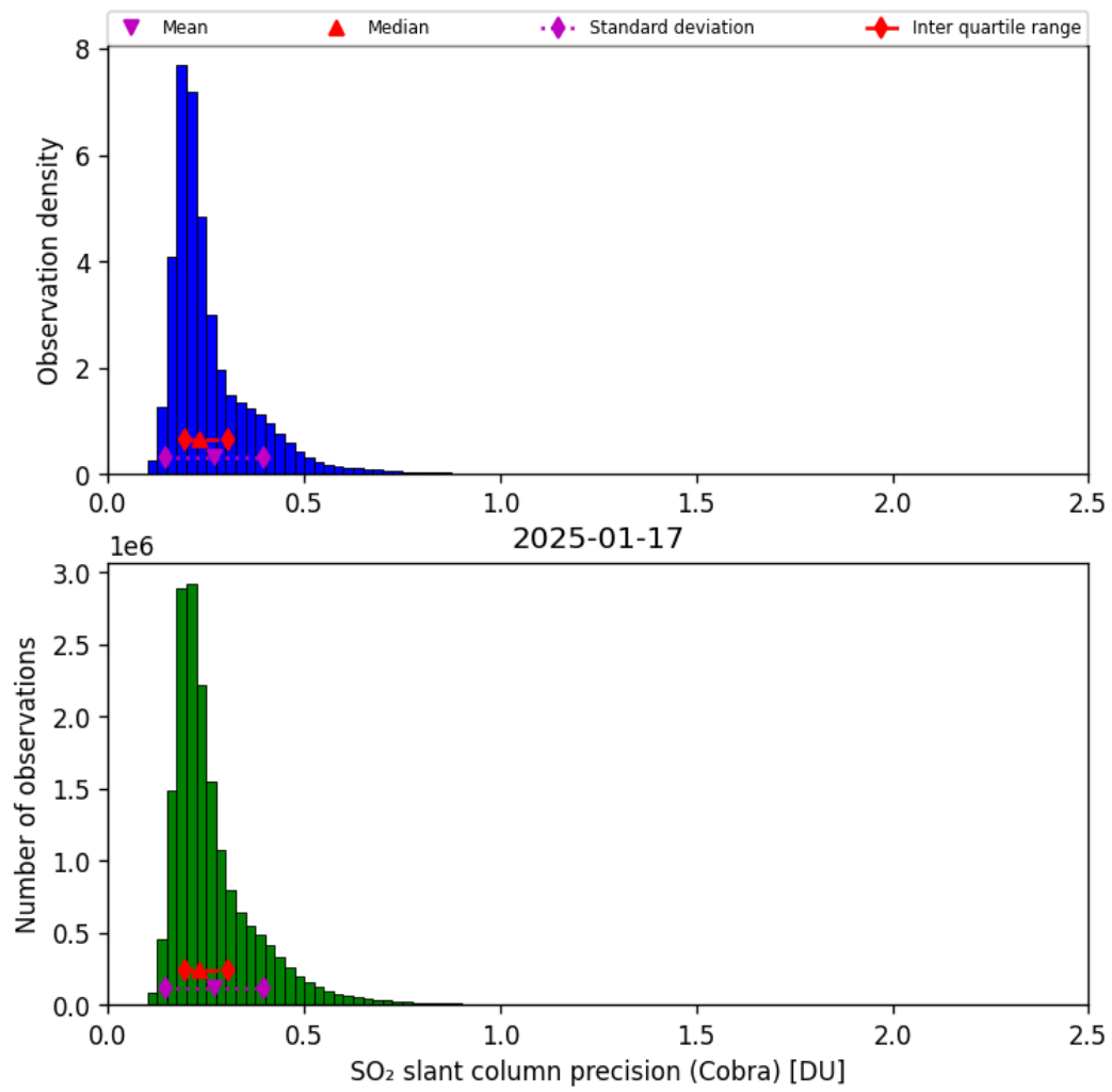
Figure 62: Histogram of “SO 2 slant column precision (Cobra)” for 2025-01-17 to 2025-01-18
