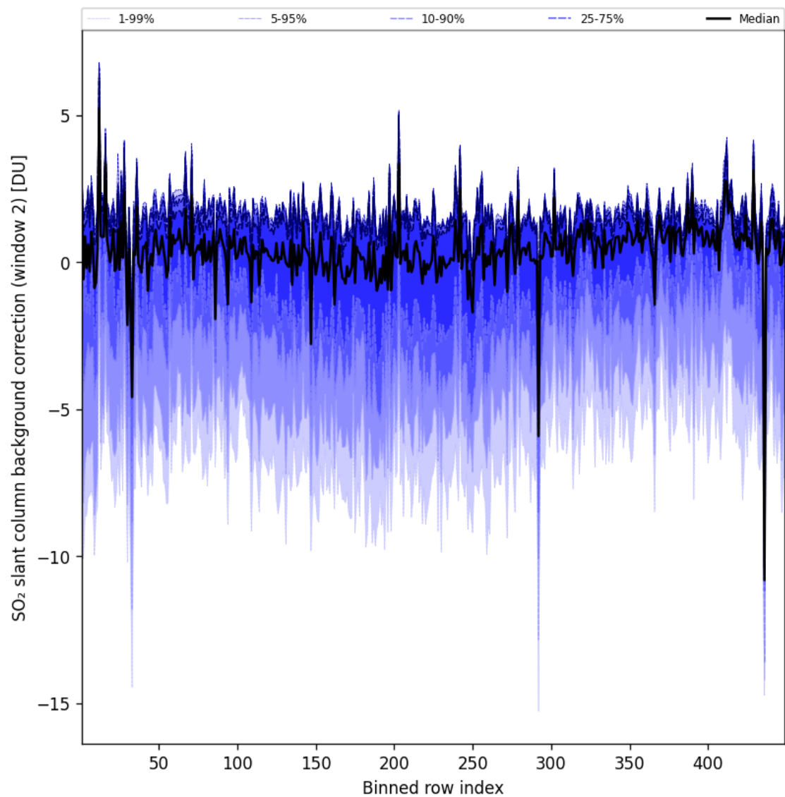
Figure 97: Along track statistics of “SO 2 slant column background correction (window 2)” for 2025-01-17 to 2025-01-18
