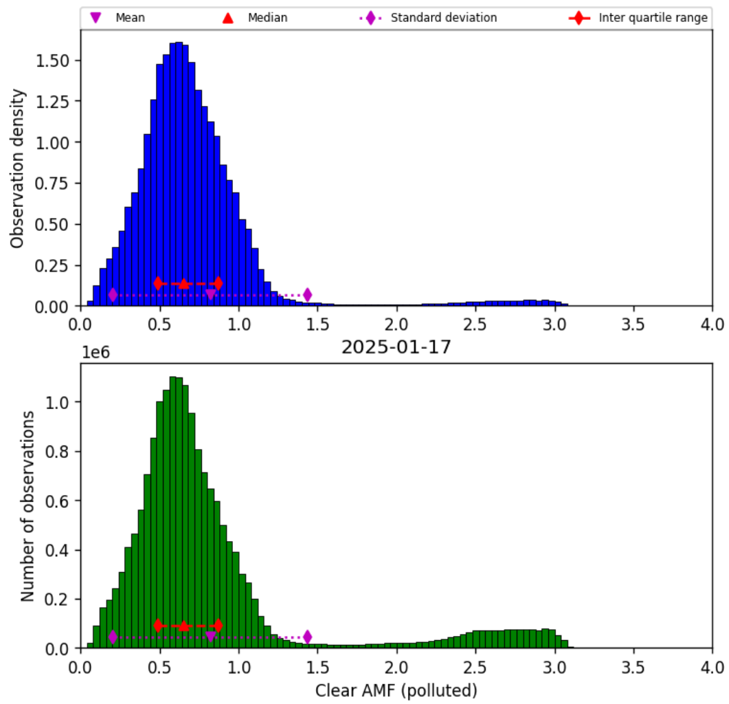
Figure 82: Histogram of “Clear AMF (polluted)” for 2025-01-17 to 2025-01-18
