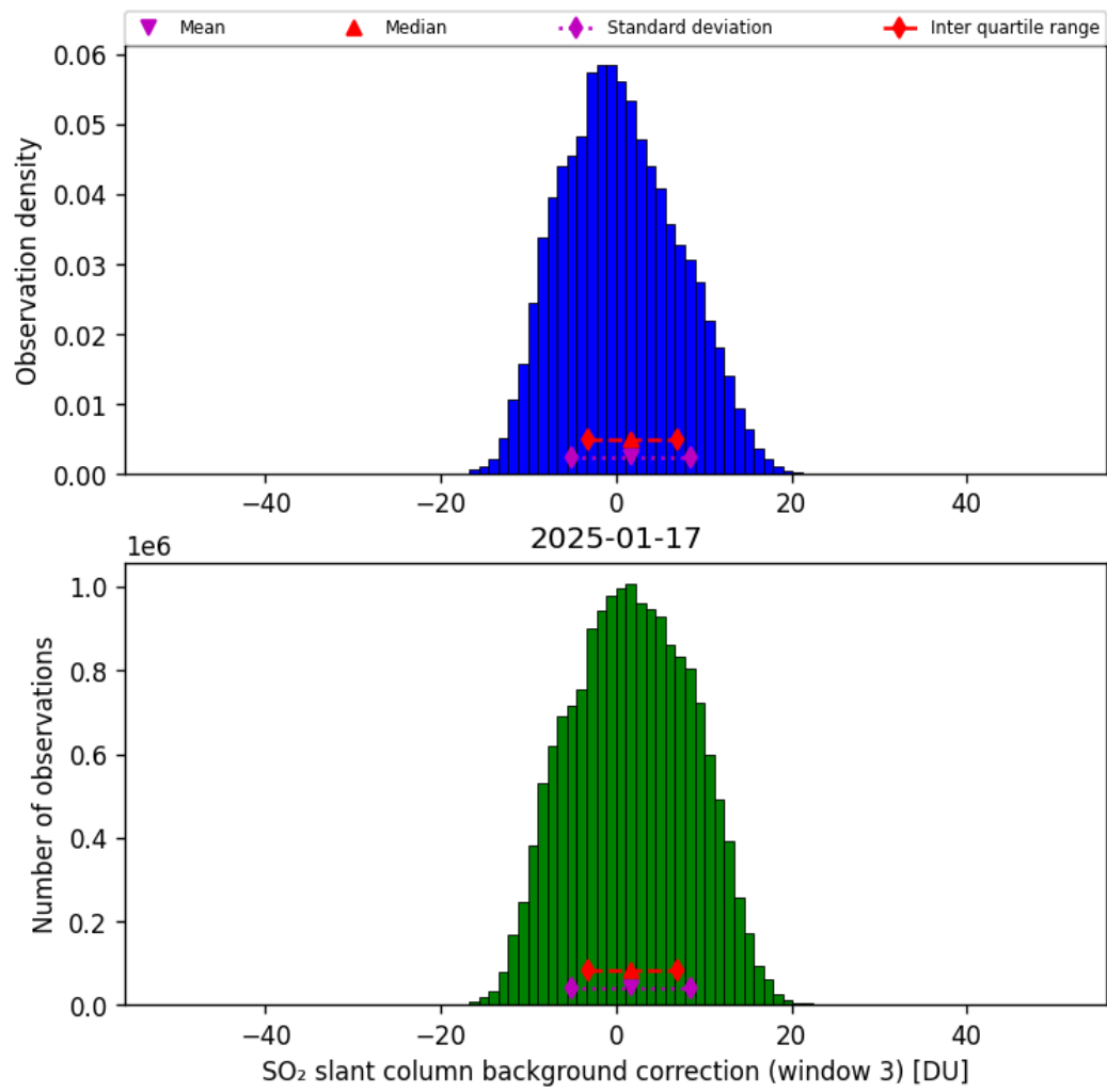
Figure 74: Histogram of “SO 2 slant column background correction (window 3)” for 2025-01-17 to 2025-01-18
