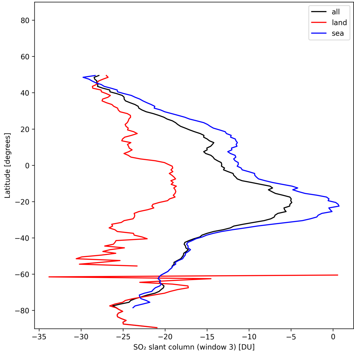
Figure 44: Zonal average of “SO 2 slant column (window 3)” for 2025-01-17 to 2025-01-18.
