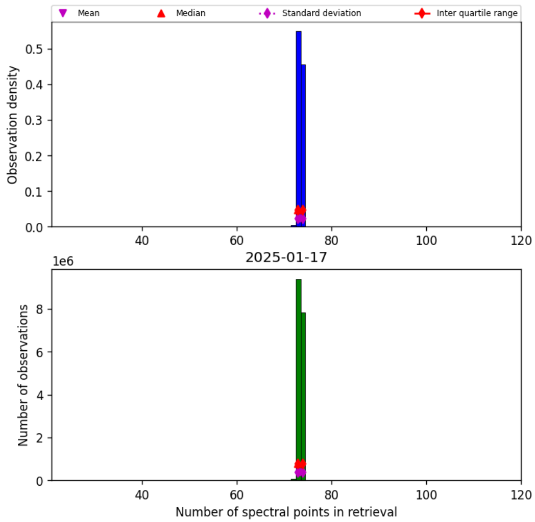
Figure 83: Histogram of “Number of spectral points in retrieval” for 2025-01-17 to 2025-01-18
