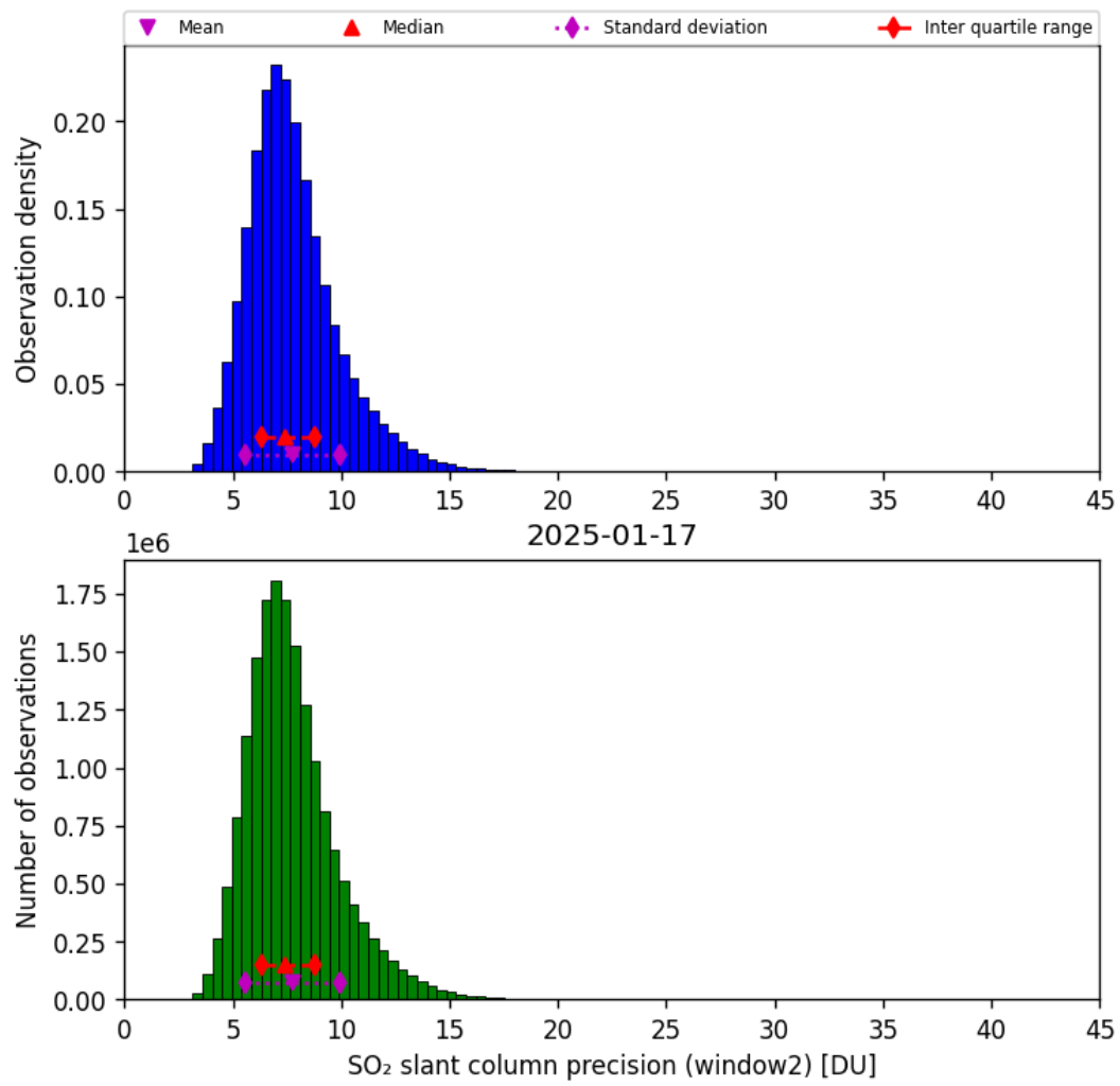
Figure 68: Histogram of “SO 2 slant column precision (window2)” for 2025-01-17 to 2025-01-18
