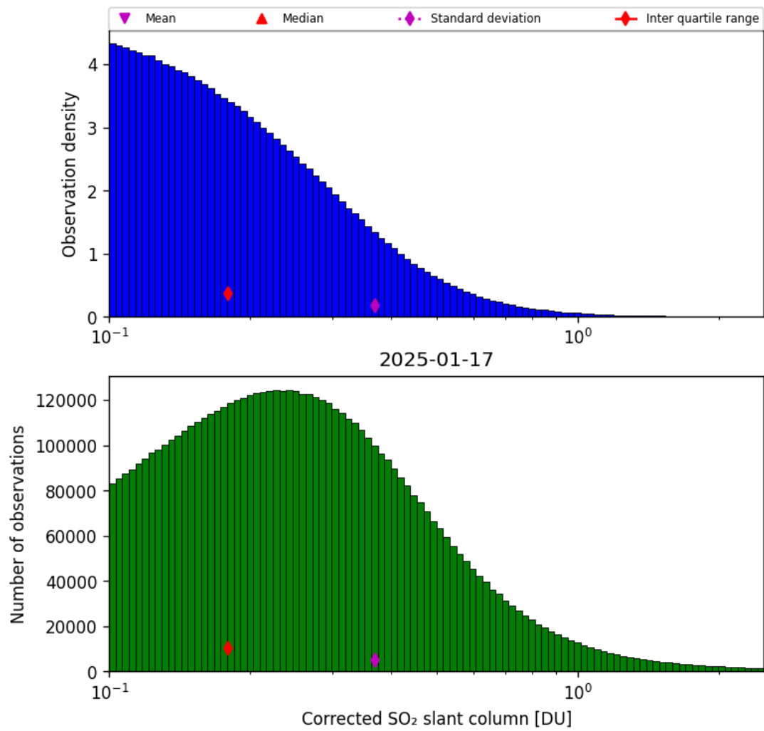
Figure 60: Histogram of “Corrected SO 2 slant column” for 2025-01-17 to 2025-01-18
