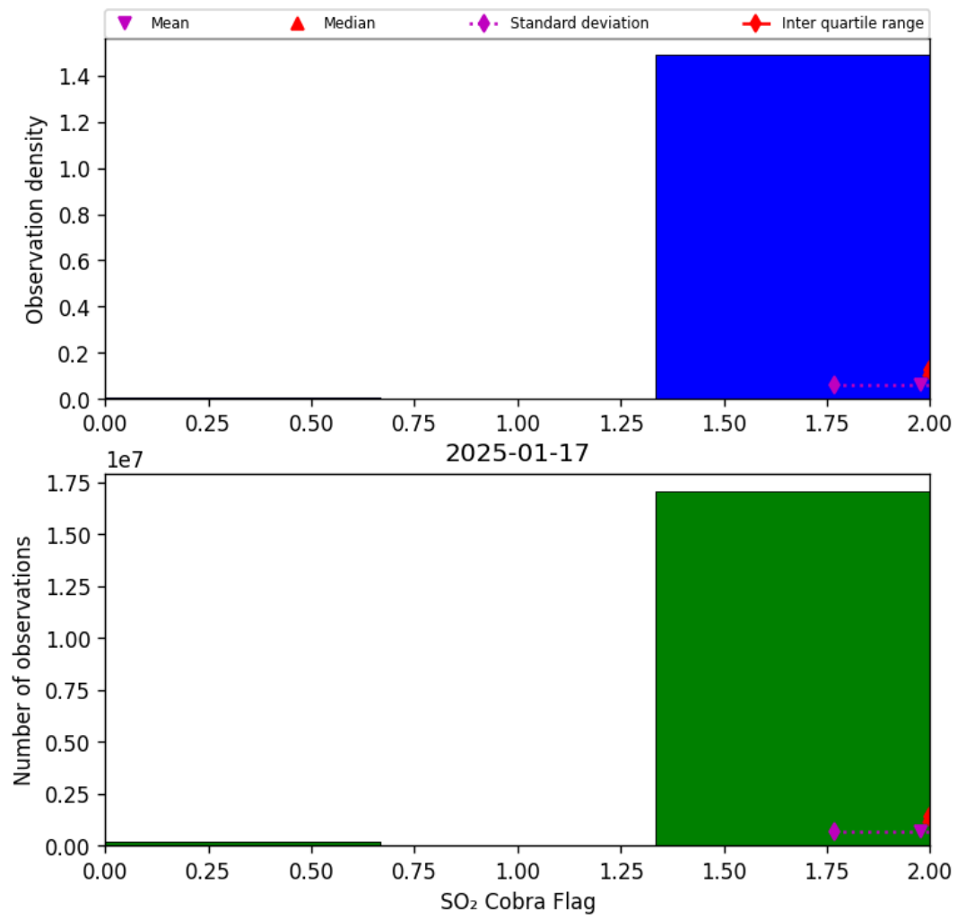
Figure 75: Histogram of “SO 2 Cobra Flag” for 2025-01-17 to 2025-01-18
