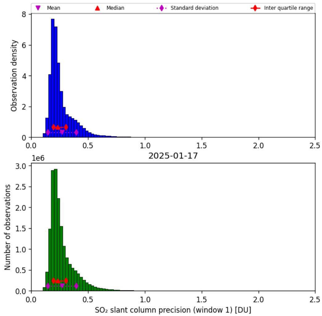
Figure 64: Histogram of “SO 2 slant column precision (window 1)” for 2025-01-17 to 2025-01-18
