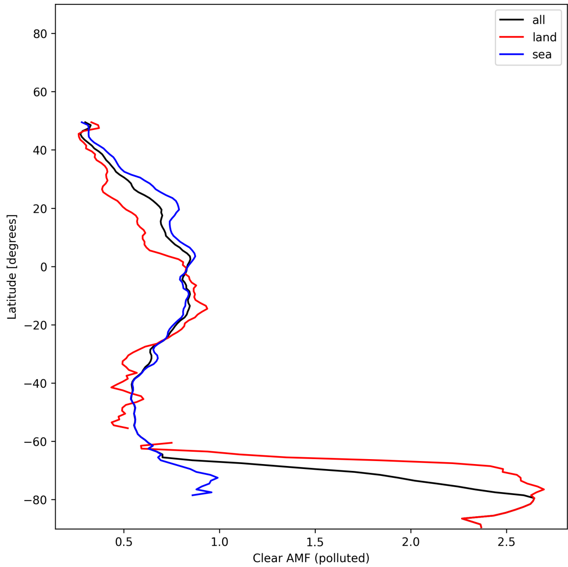
Figure 55: Zonal average of “Clear AMF (polluted)” for 2025-01-17 to 2025-01-18.
