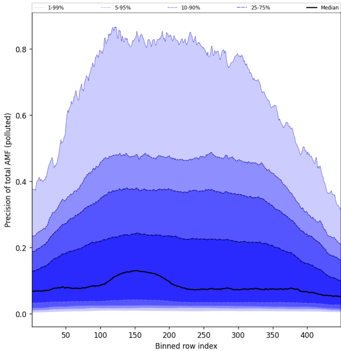
Figure 108: Along track statistics of “Precision of total AMF (polluted)” for 2025-01-17 to 2025-01-18
