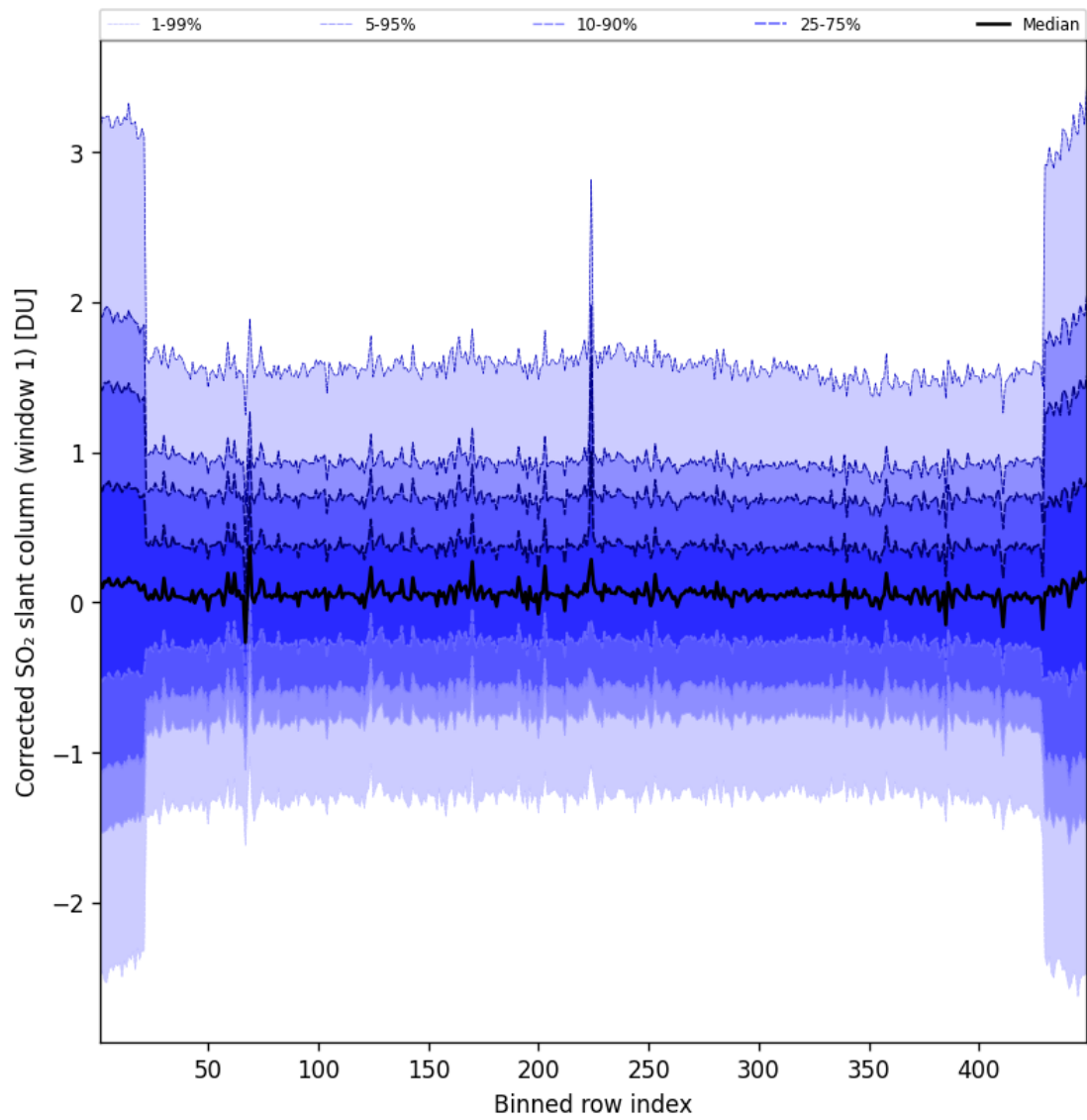
Figure 92: Along track statistics of “Corrected SO 2 slant column (window 1)” for 2025-01-17 to 2025-01-18
