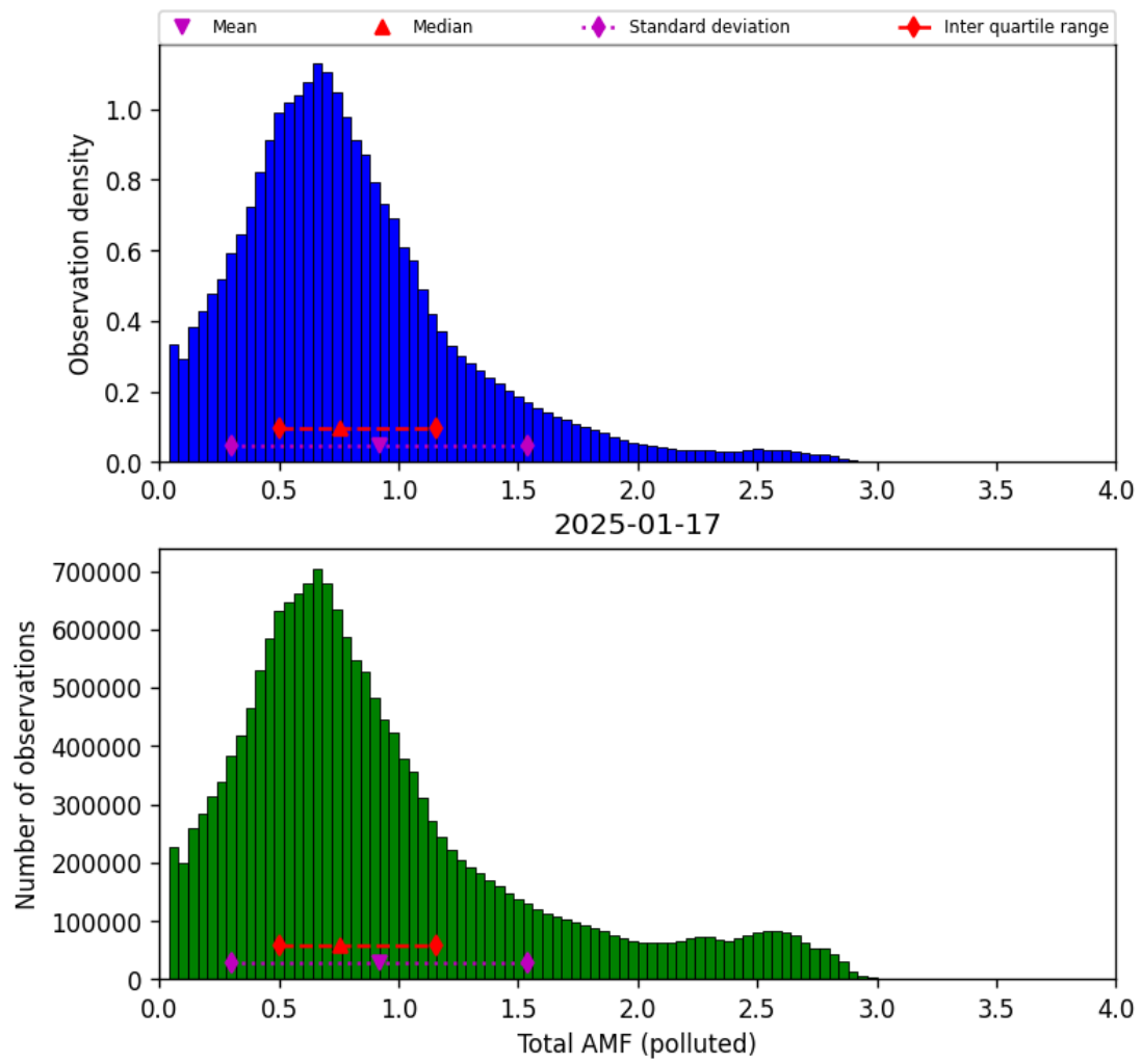
Figure 80: Histogram of “Total AMF (polluted)” for 2025-01-17 to 2025-01-18
