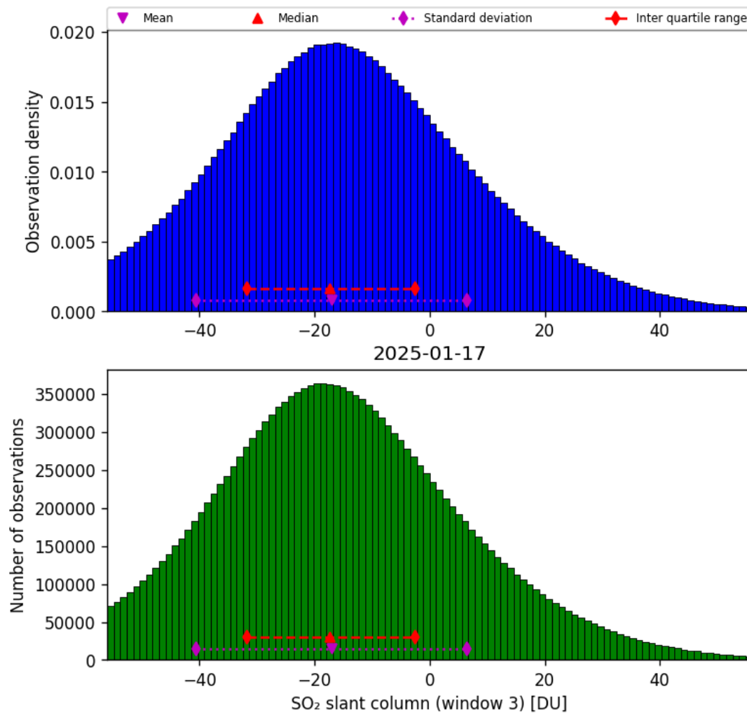
Figure 71: Histogram of “SO 2 slant column (window 3)” for 2025-01-17 to 2025-01-18
