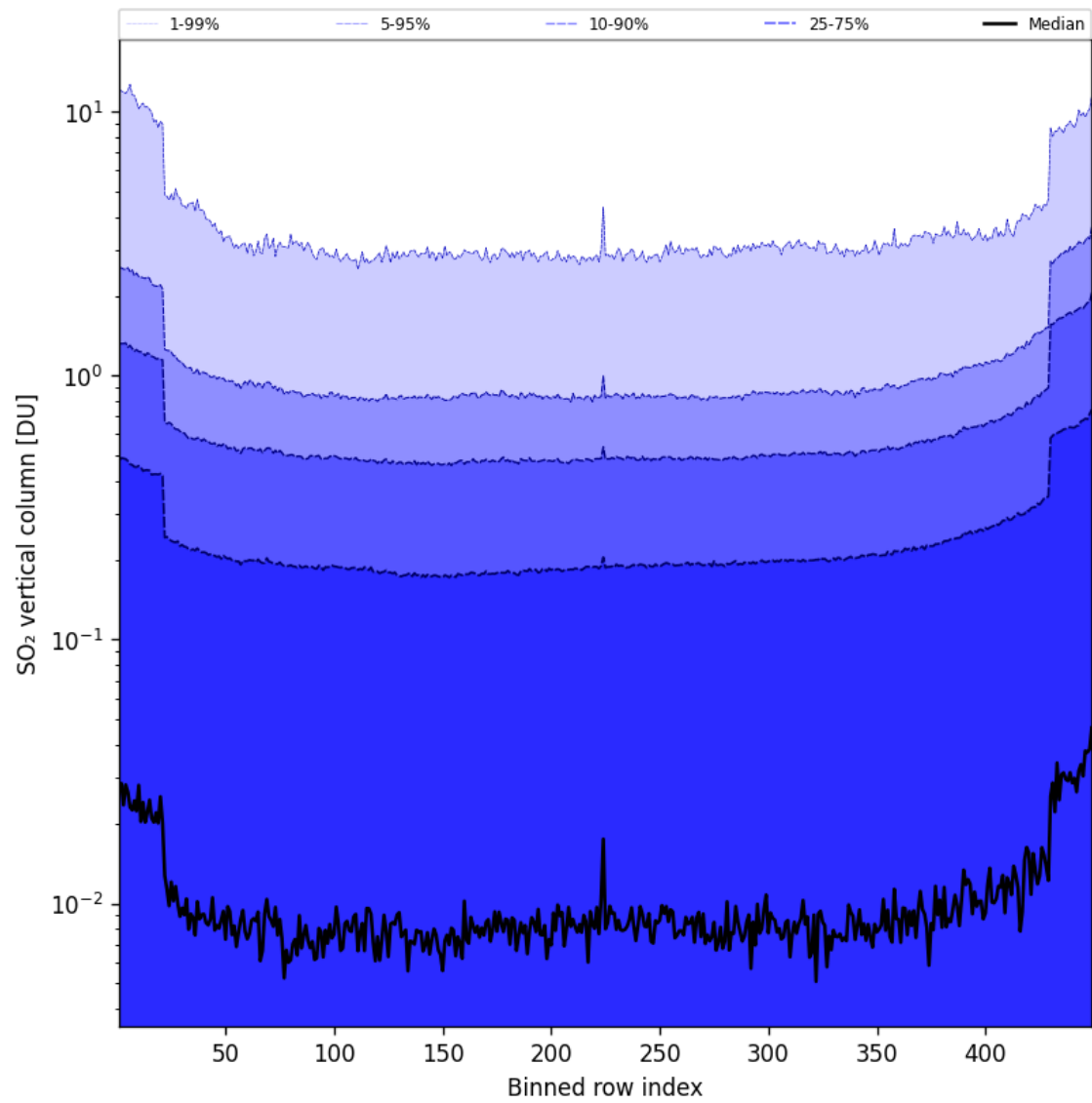
Figure 85: Along track statistics of “SO 2 vertical column” for 2025-01-17 to 2025-01-18
