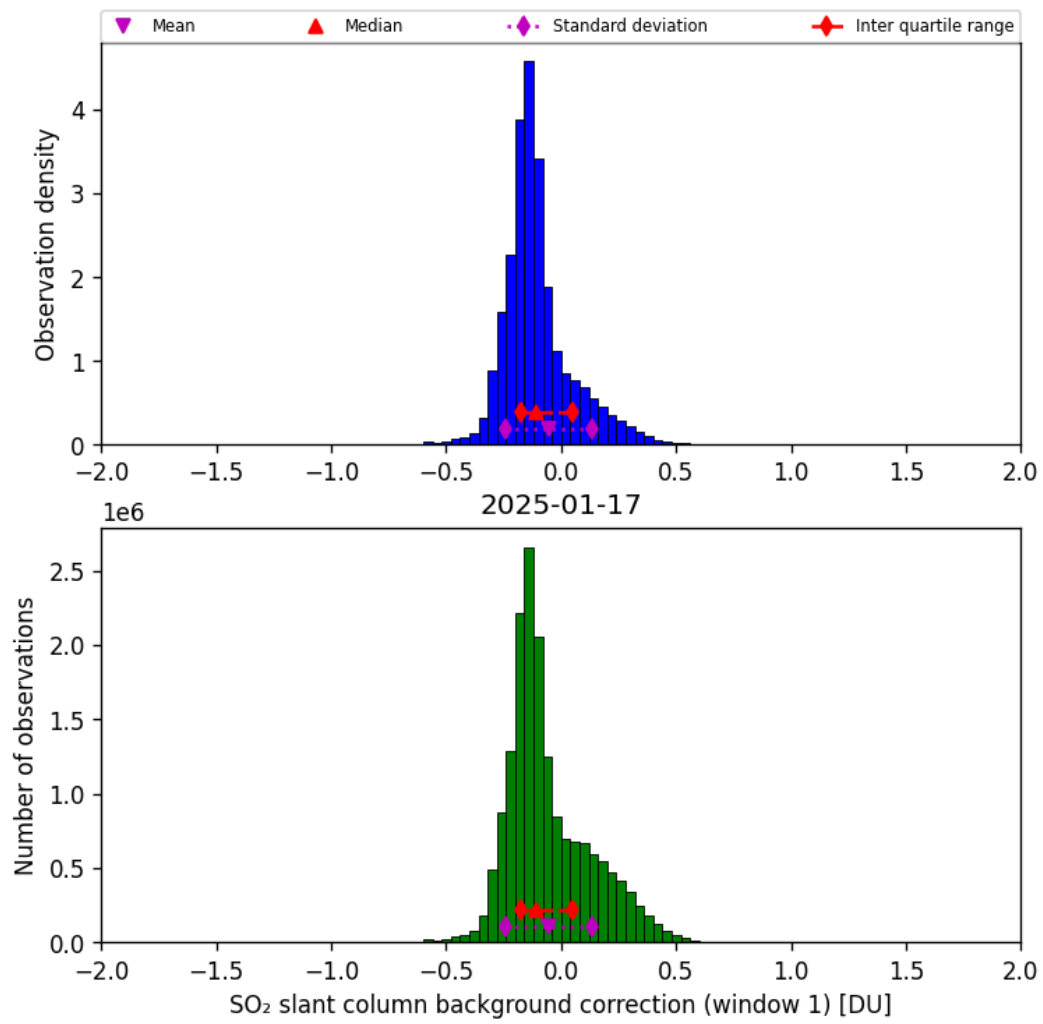
Figure 66: Histogram of “SO 2 slant column background correction (window 1)” for 2025-01-17 to 2025-01-18
