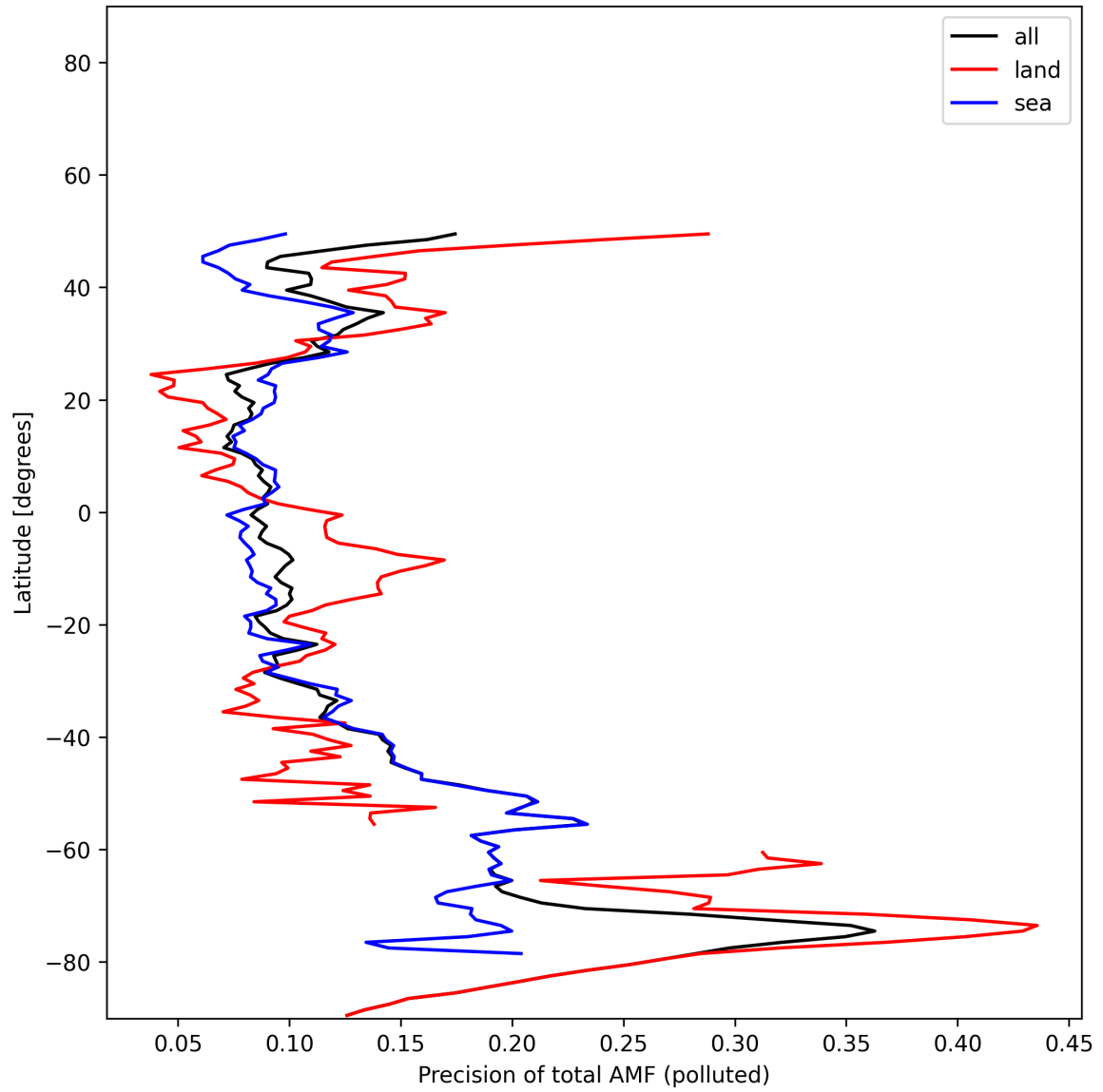
Figure 54: Zonal average of “Precision of total AMF (polluted)” for 2025-01-17 to 2025-01-18.
