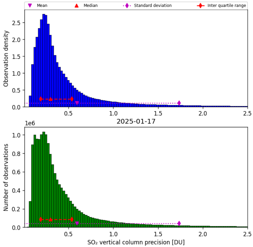
Figure 59: Histogram of “SO 2 vertical column precision” for 2025-01-17 to 2025-01-18
