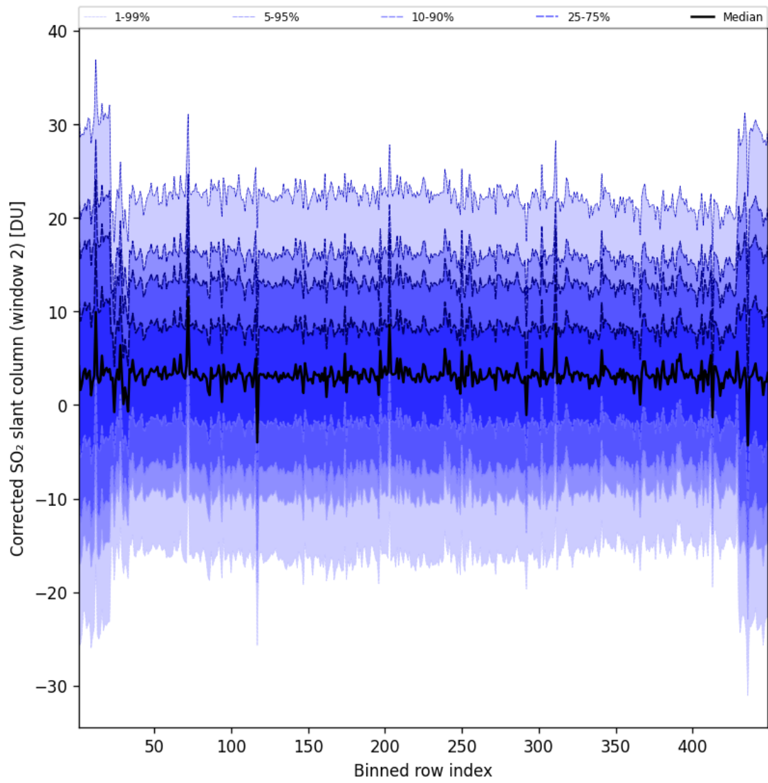
Figure 96: Along track statistics of “Corrected SO 2 slant column (window 2)” for 2025-01-17 to 2025-01-18
