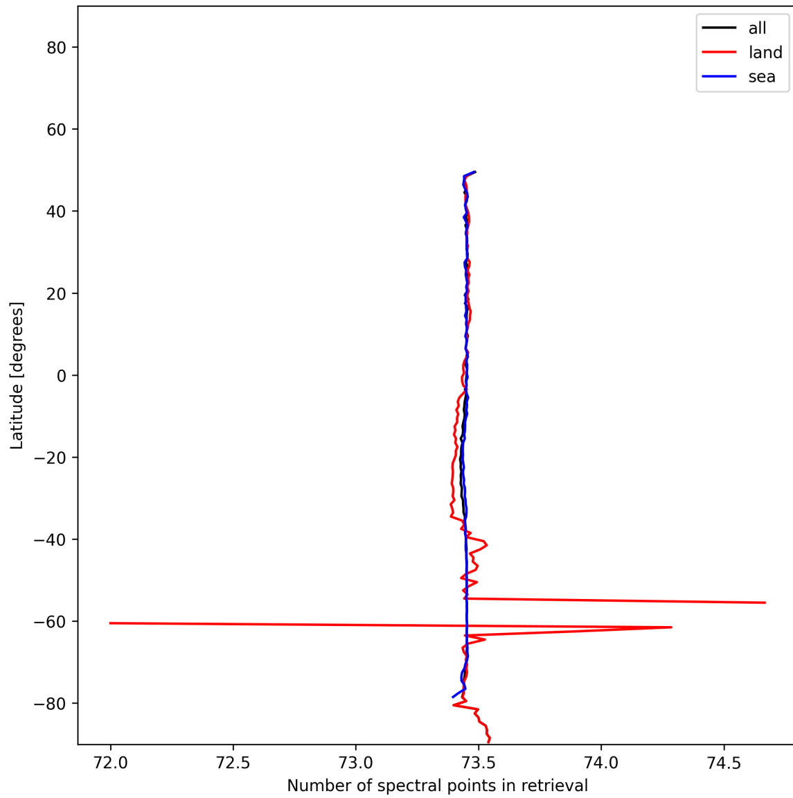
Figure 56: Zonal average of “Number of spectral points in retrieval” for 2025-01-17 to 2025-01-18.
