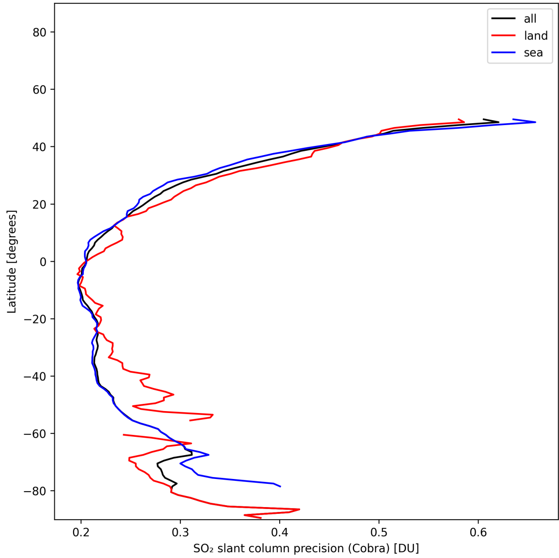
Figure 35: Zonal average of “SO 2 slant column precision (Cobra)” for 2025-01-17 to 2025-01-18.
