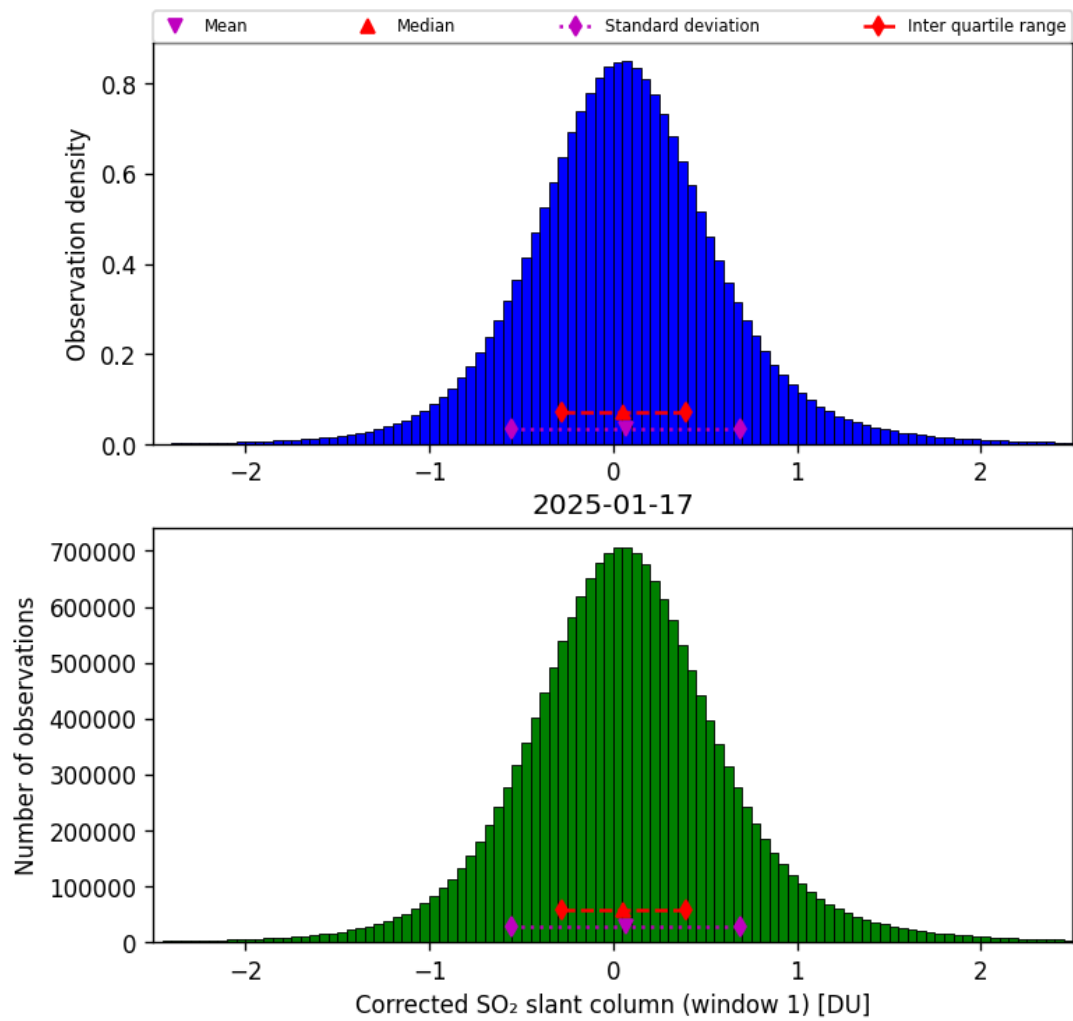
Figure 65: Histogram of “Corrected SO 2 slant column (window 1)” for 2025-01-17 to 2025-01-18
