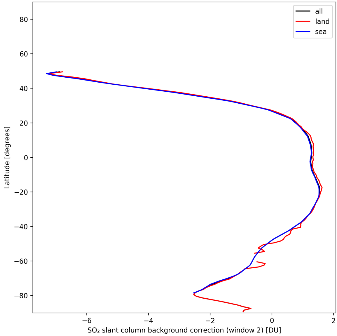
Figure 43: Zonal average of “SO 2 slant column background correction (window 2)” for 2025-01-17 to 2025-01-18.
