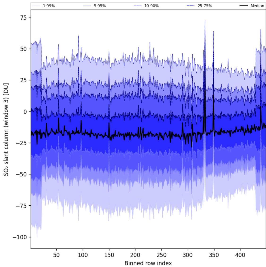
Figure 98: Along track statistics of “SO 2 slant column (window 3)” for 2025-01-17 to 2025-01-18
