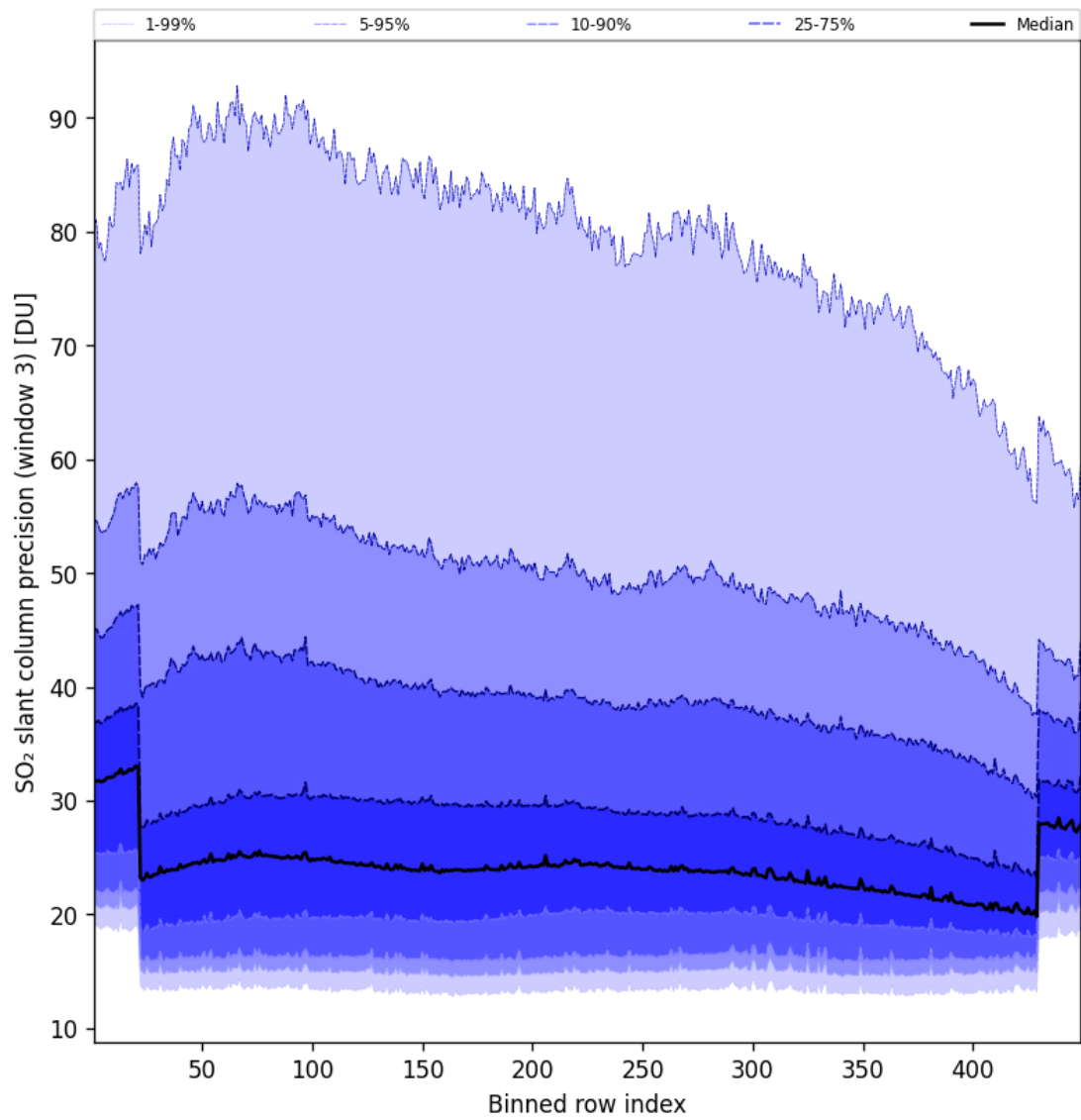
Figure 99: Along track statistics of “SO 2 slant column precision (window 3)” for 2025-01-17 to 2025-01-18
