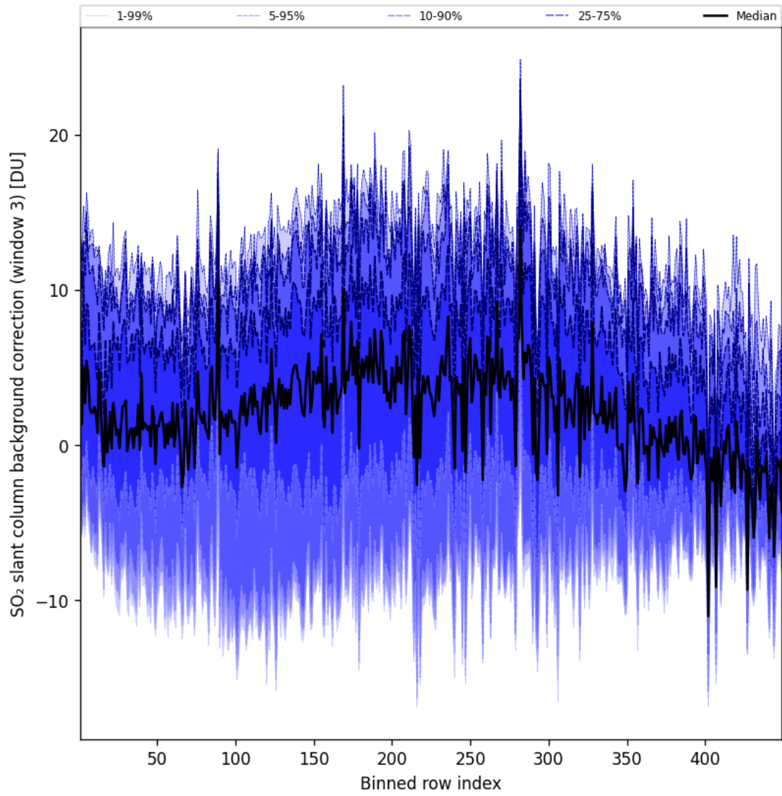
Figure 101: Along track statistics of “SO 2 slant column background correction (window 3)” for 2025-01-17 to 2025-01-18
