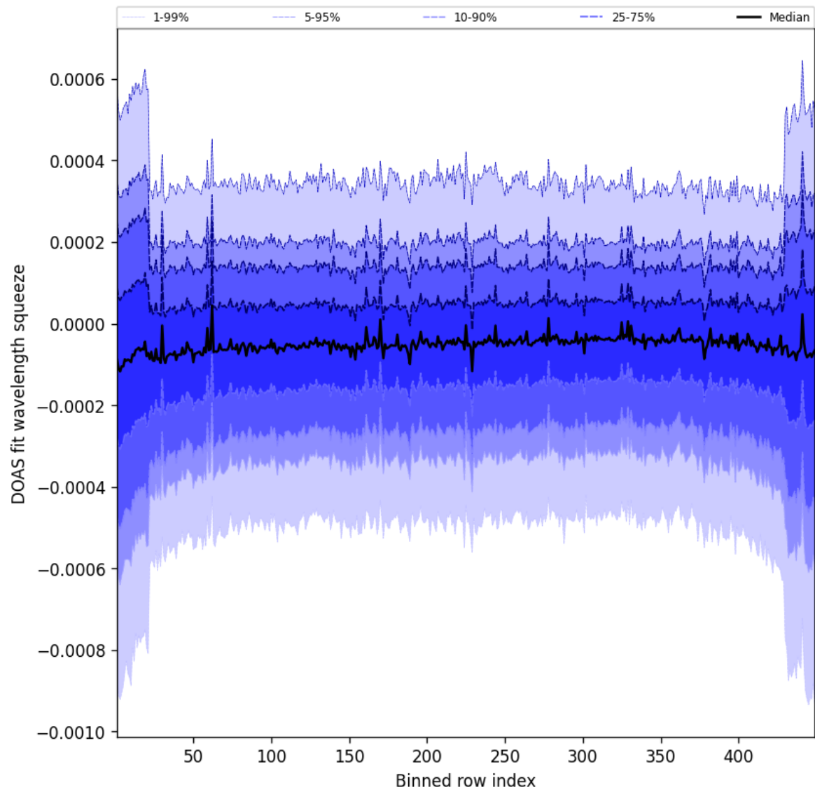
Figure 105: Along track statistics of “DOAS fit wavelength squeeze” for 2025-01-17 to 2025-01-18
