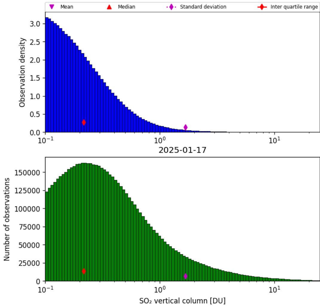
Figure 58: Histogram of “SO 2 vertical column” for 2025-01-17 to 2025-01-18
