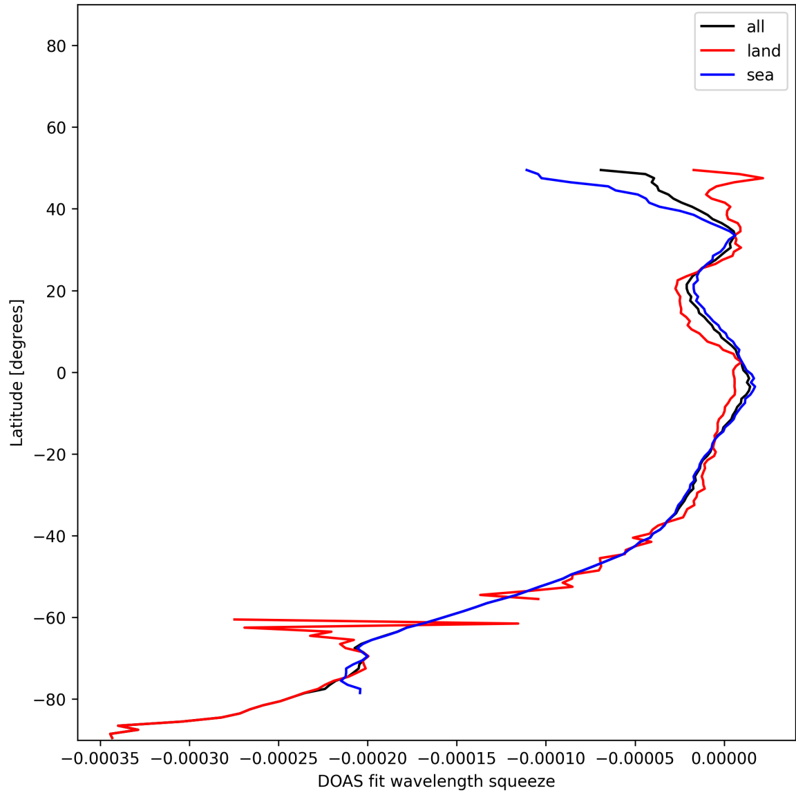
Figure 51: Zonal average of “DOAS fit wavelength squeeze” for 2025-01-17 to 2025-01-18.
