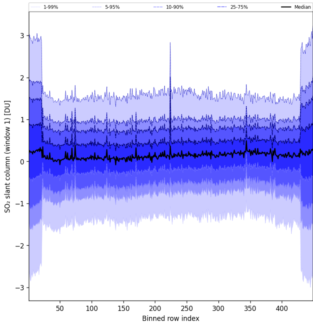
Figure 90: Along track statistics of “SO 2 slant column (window 1)” for 2025-01-17 to 2025-01-18
