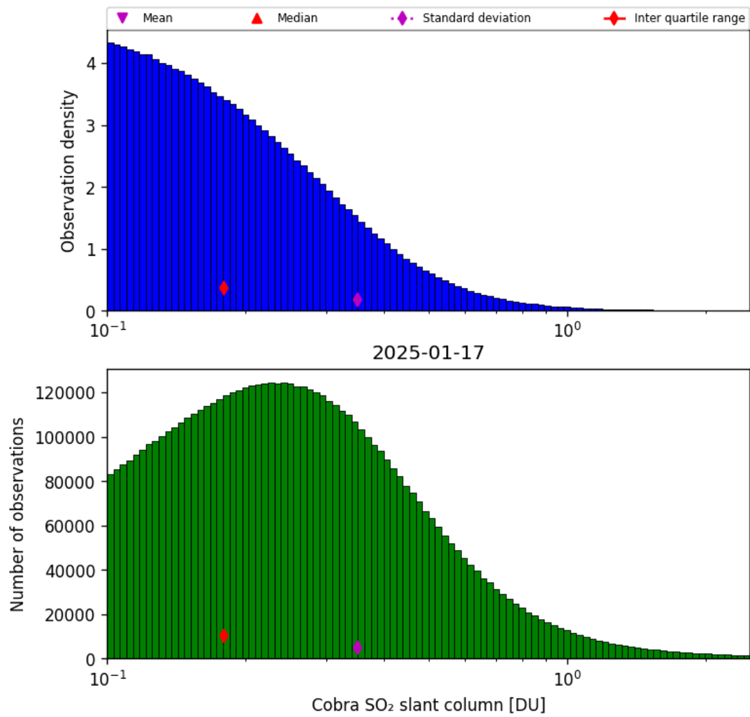
Figure 61: Histogram of “Cobra SO 2 slant column” for 2025-01-17 to 2025-01-18
