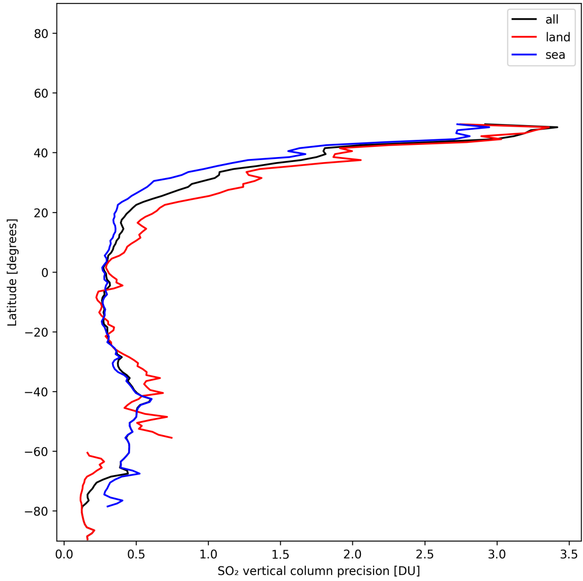
Figure 32: Zonal average of “SO 2 vertical column precision” for 2025-01-17 to 2025-01-18.
