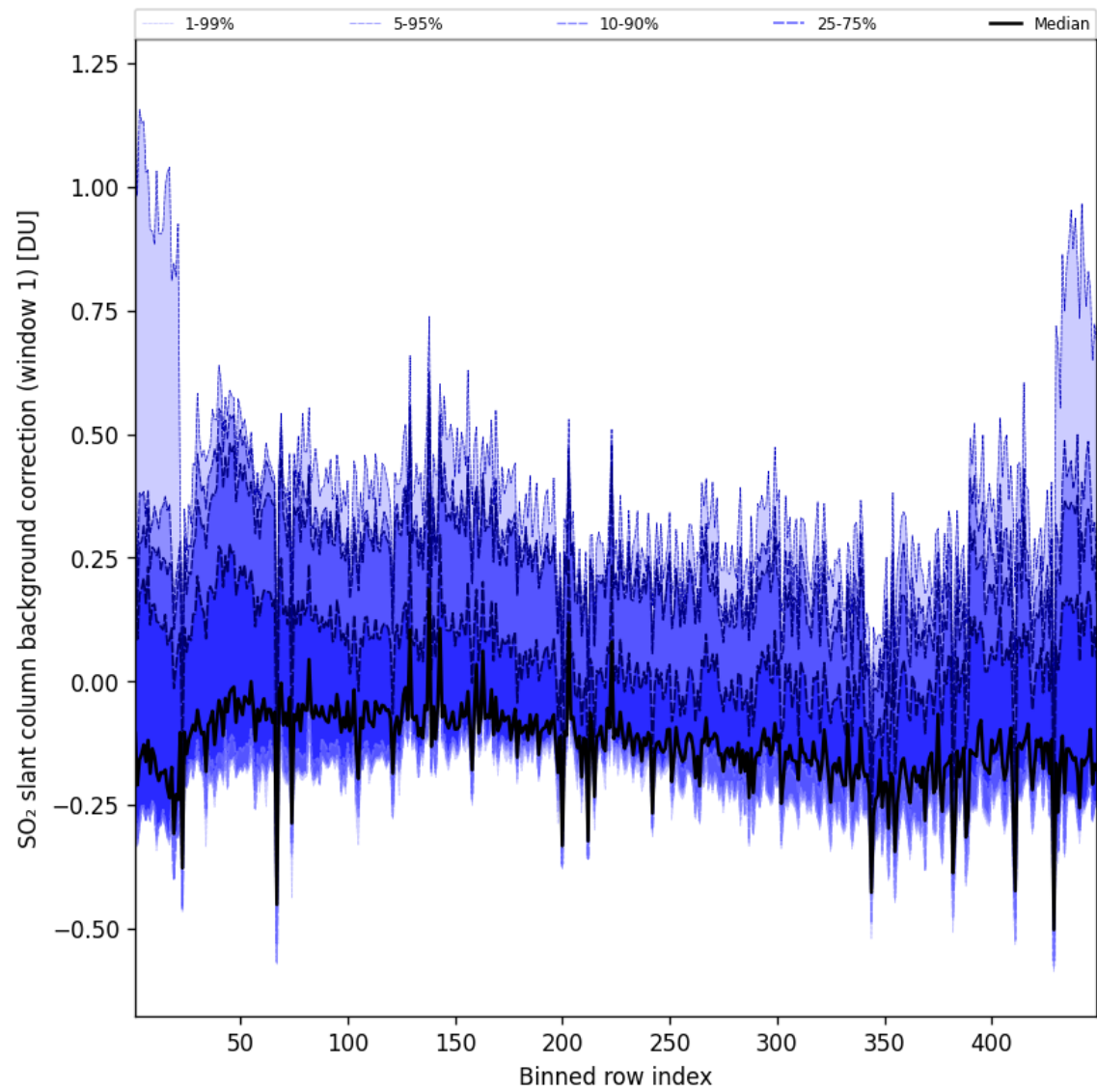
Figure 93: Along track statistics of “SO 2 slant column background correction (window 1)” for 2025-01-17 to 2025-01-18
