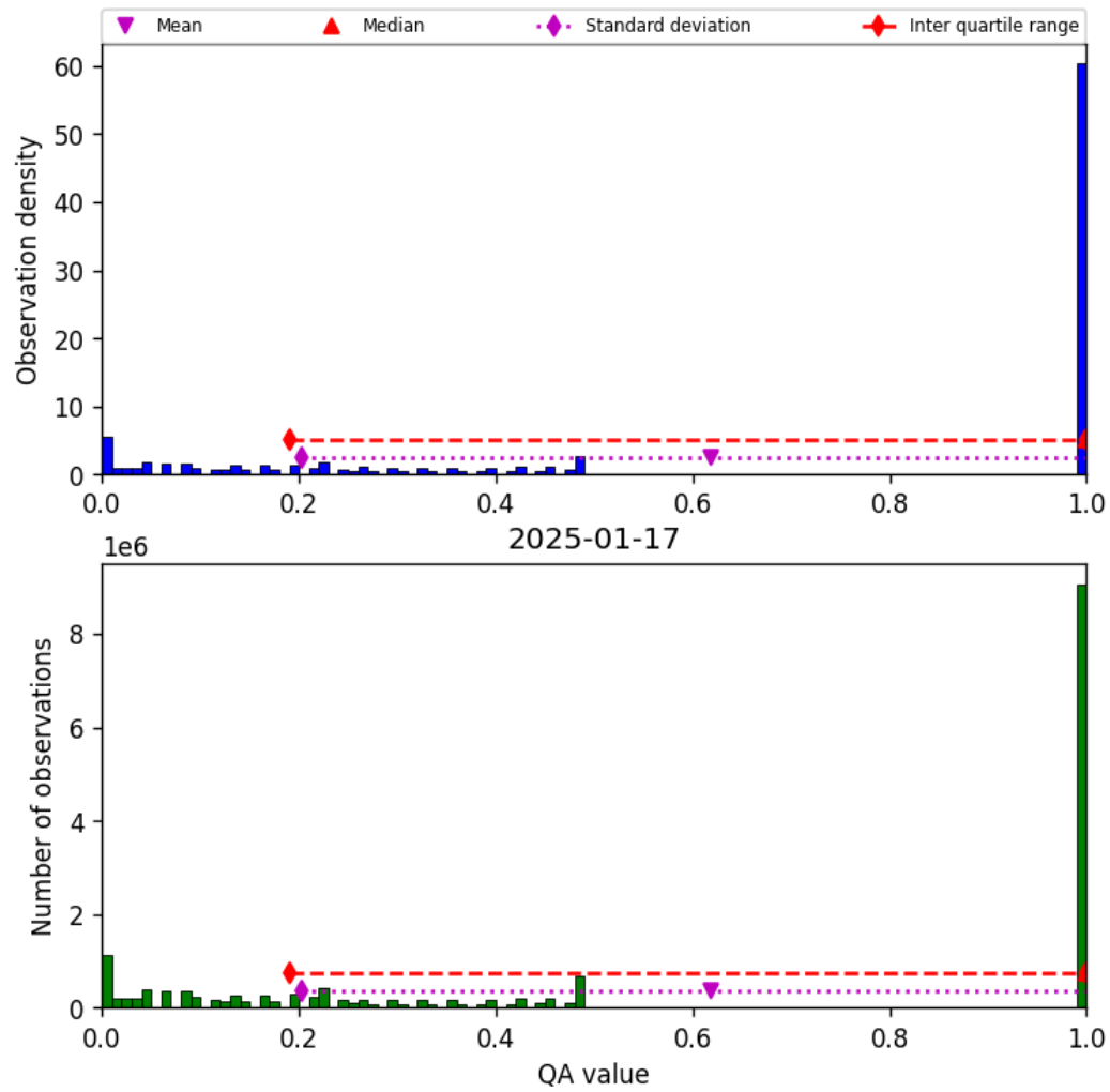
Figure 57: Histogram of “QA value” for 2025-01-17 to 2025-01-18
