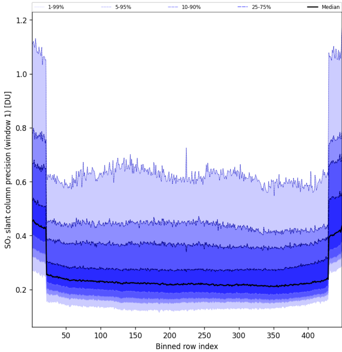
Figure 91: Along track statistics of “SO 2 slant column precision (window 1)” for 2025-01-17 to 2025-01-18
