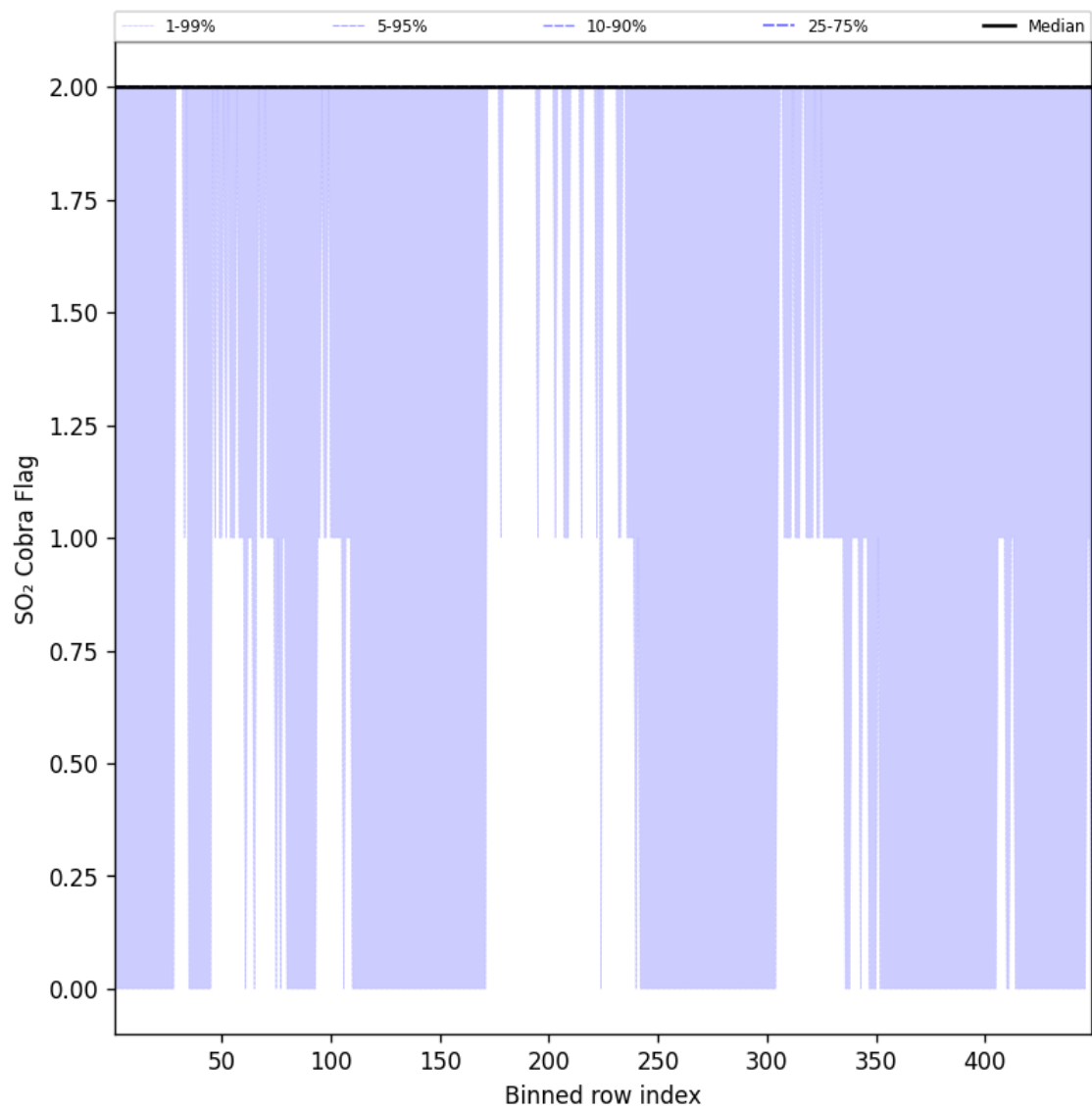
Figure 102: Along track statistics of “SO 2 Cobra Flag” for 2025-01-17 to 2025-01-18
