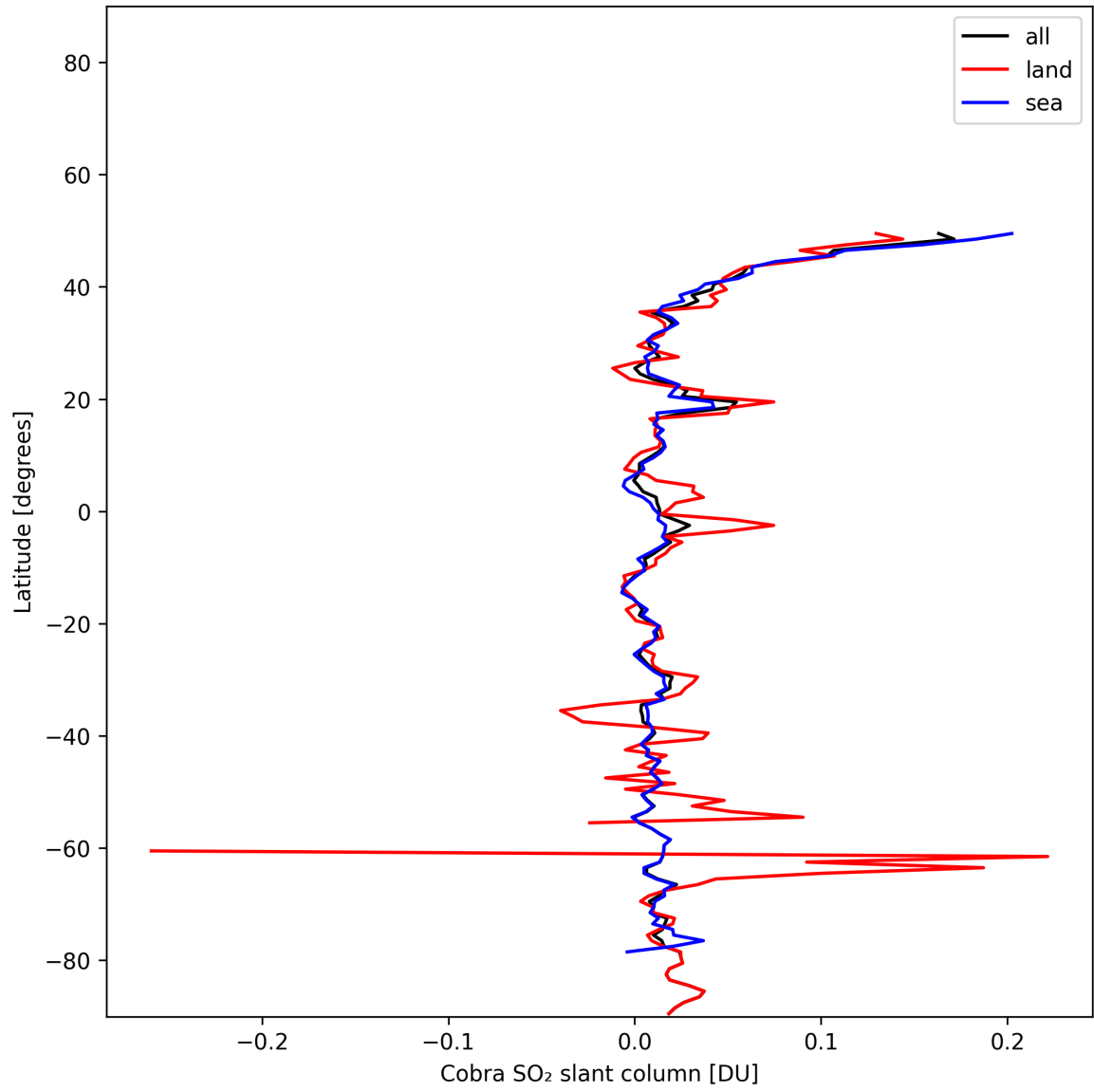
Figure 34: Zonal average of “Cobra SO 2 slant column” for 2025-01-17 to 2025-01-18.
