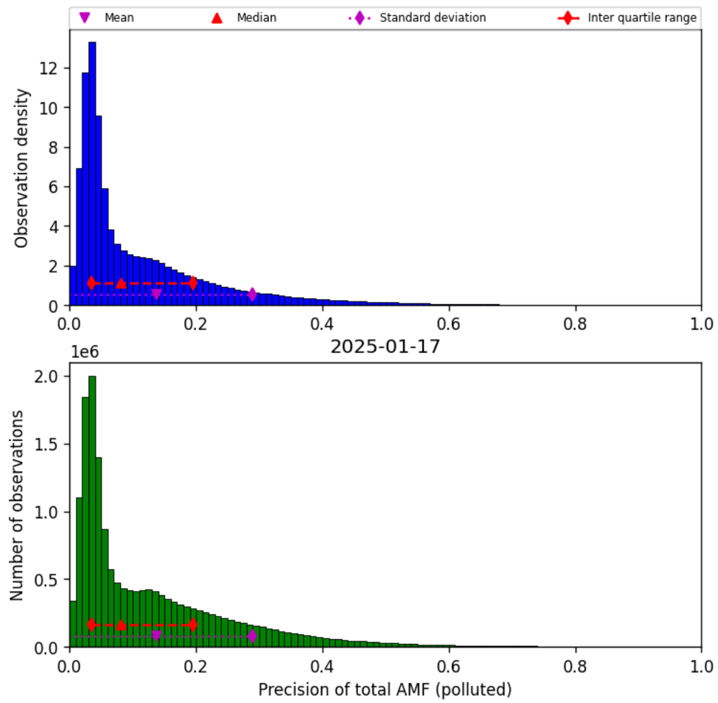
Figure 81: Histogram of “Precision of total AMF (polluted)” for 2025-01-17 to 2025-01-18
