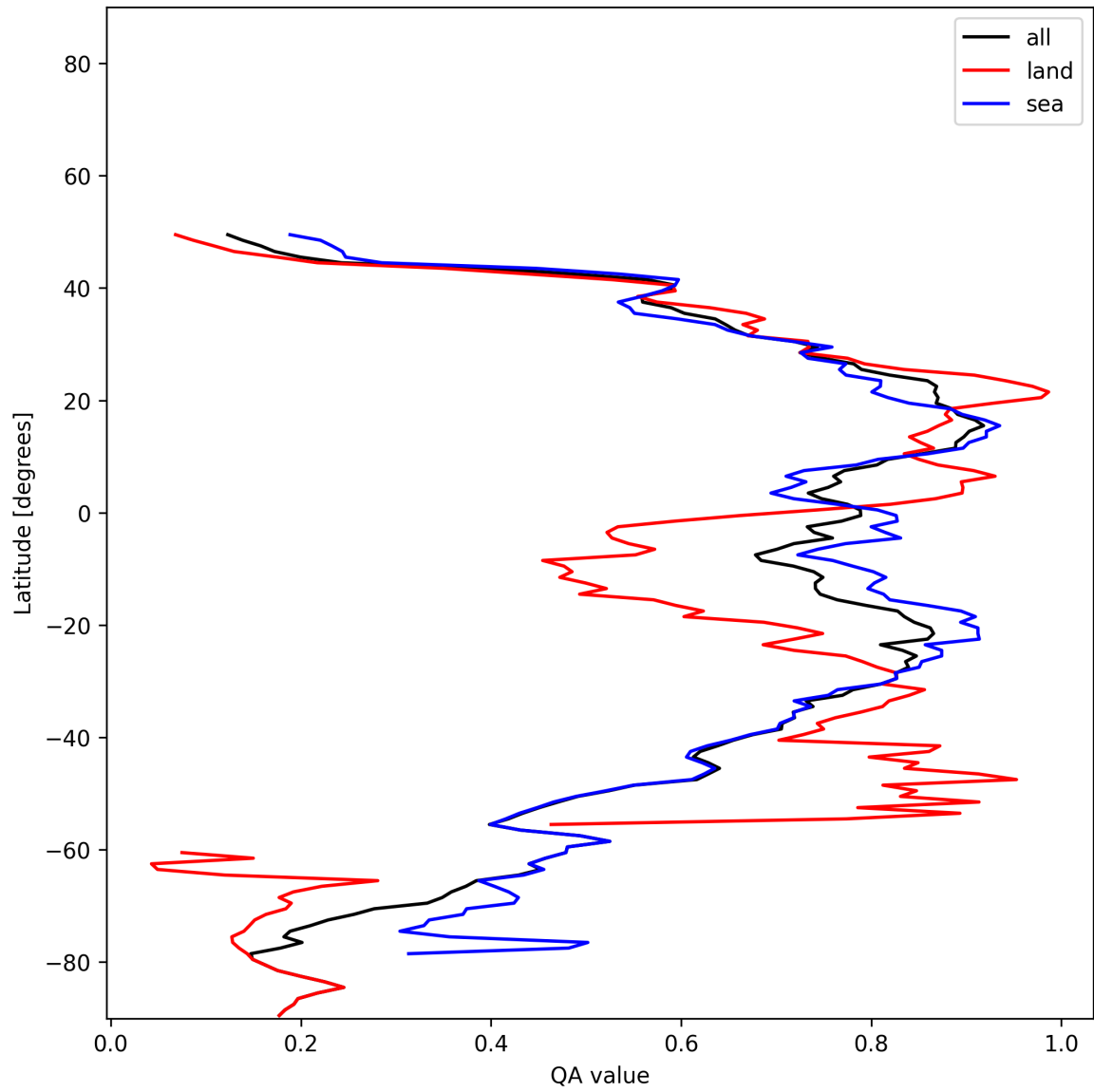
Figure 30: Zonal average of “QA value” for 2025-01-17 to 2025-01-18.
