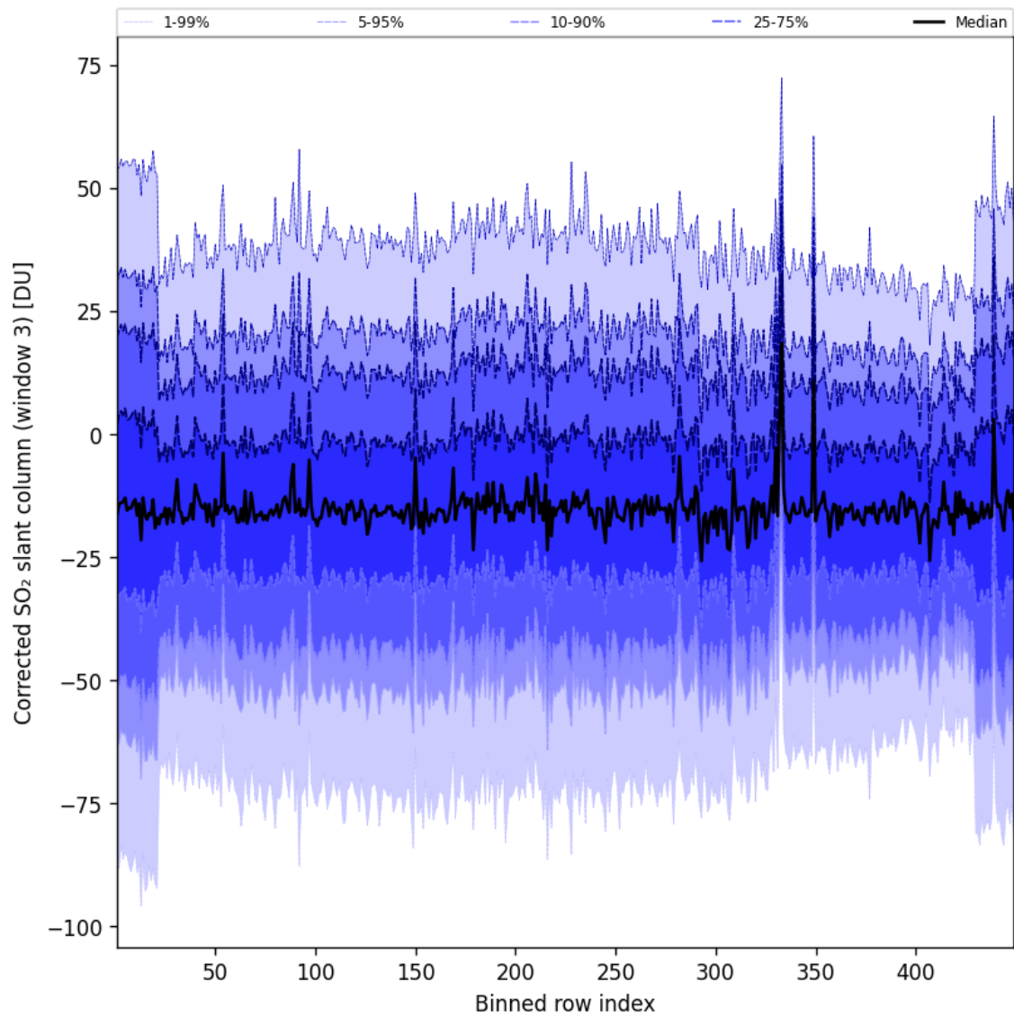
Figure 100: Along track statistics of “Corrected SO 2 slant column (window 3)” for 2025-01-17 to 2025-01-18
