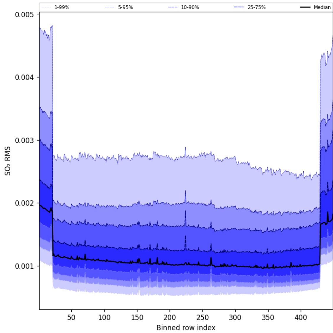
Figure 106: Along track statistics of “SO 2 RMS” for 2025-01-17 to 2025-01-18
