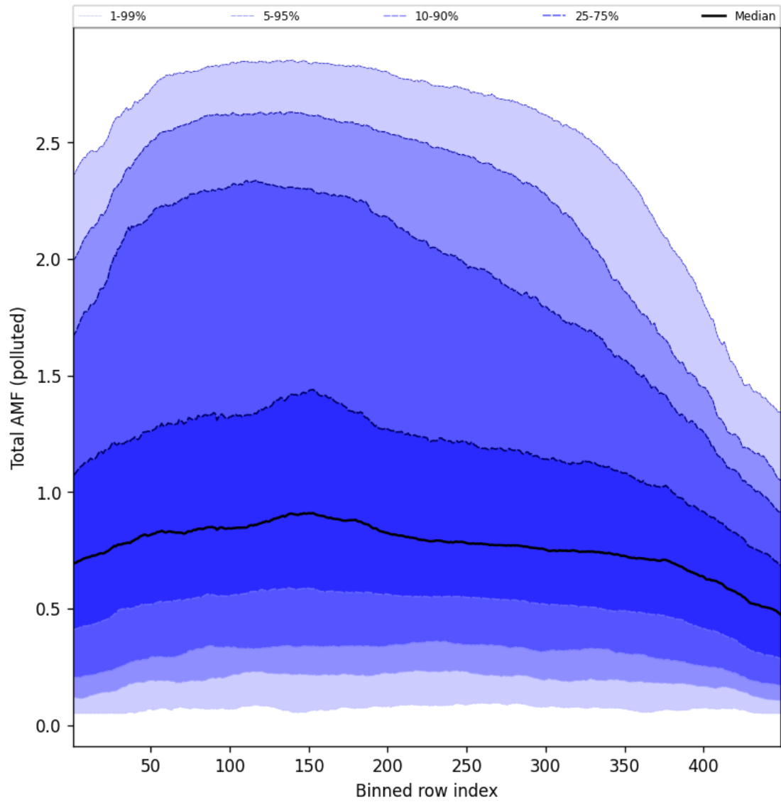
Figure 107: Along track statistics of “Total AMF (polluted)” for 2025-01-17 to 2025-01-18
