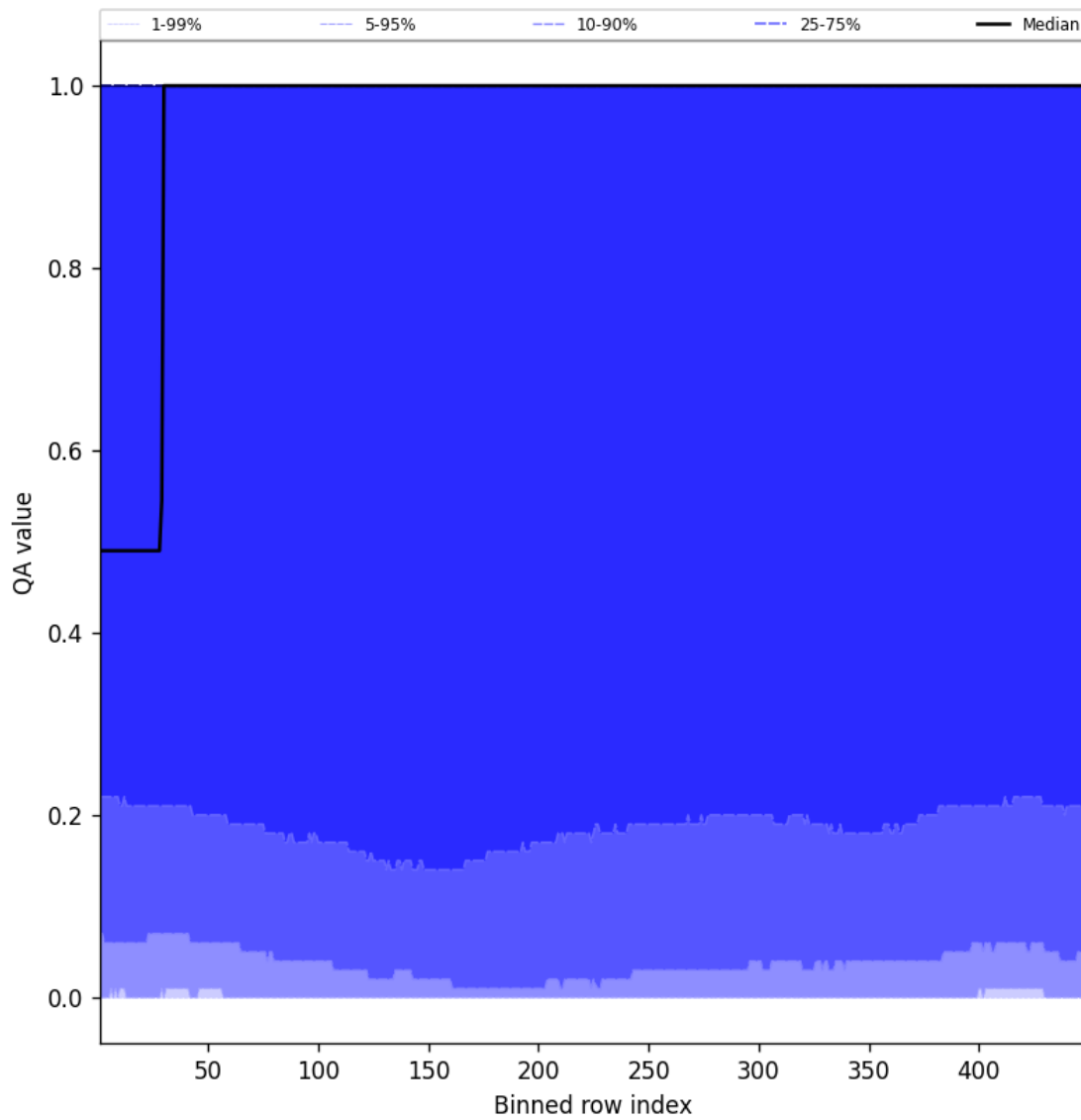
Figure 84: Along track statistics of “QA value” for 2025-01-17 to 2025-01-18
