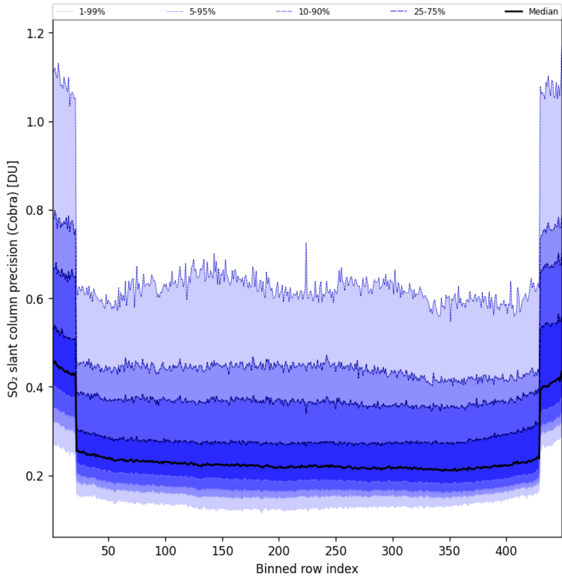
Figure 89: Along track statistics of “SO 2 slant column precision (Cobra)” for 2025-01-17 to 2025-01-18
