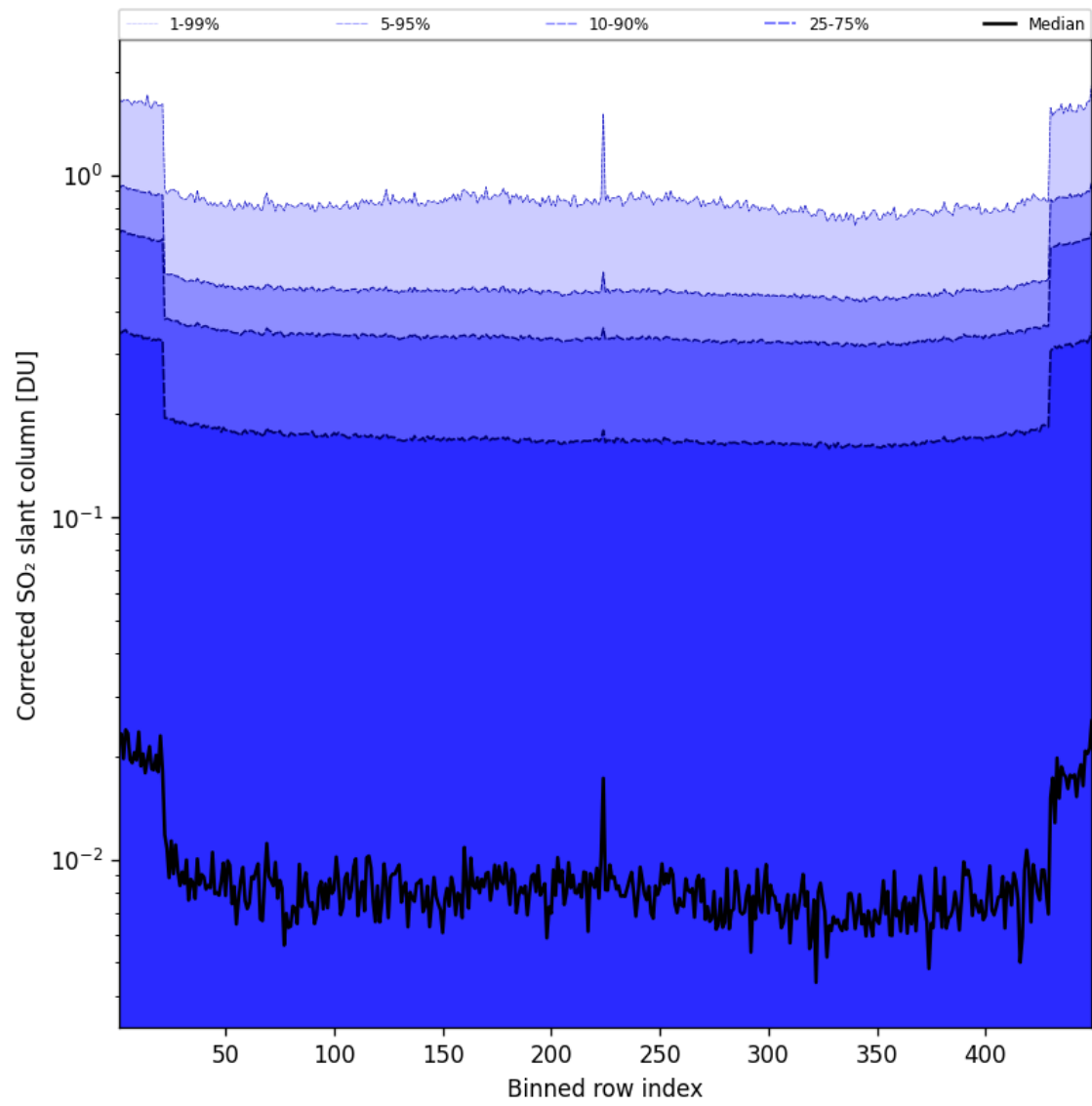
Figure 87: Along track statistics of “Corrected SO 2 slant column” for 2025-01-17 to 2025-01-18
