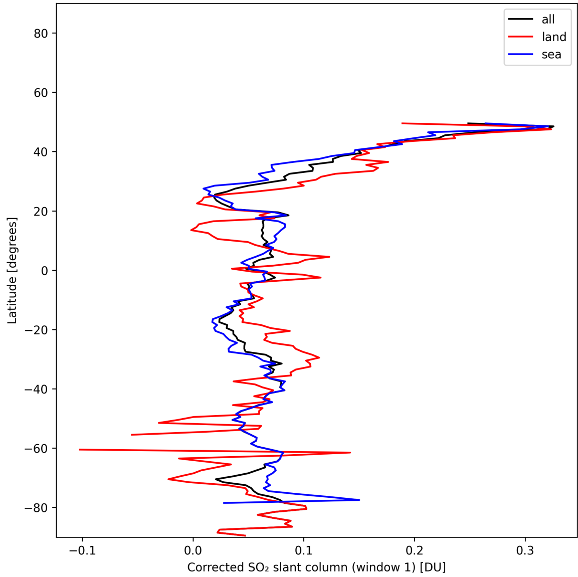
Figure 38: Zonal average of “Corrected SO 2 slant column (window 1)” for 2025-01-17 to 2025-01-18.
