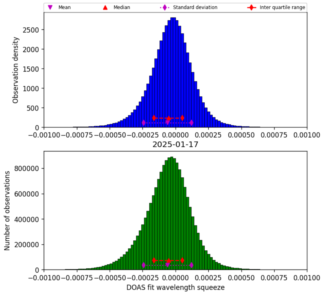
Figure 78: Histogram of “DOAS fit wavelength squeeze” for 2025-01-17 to 2025-01-18
