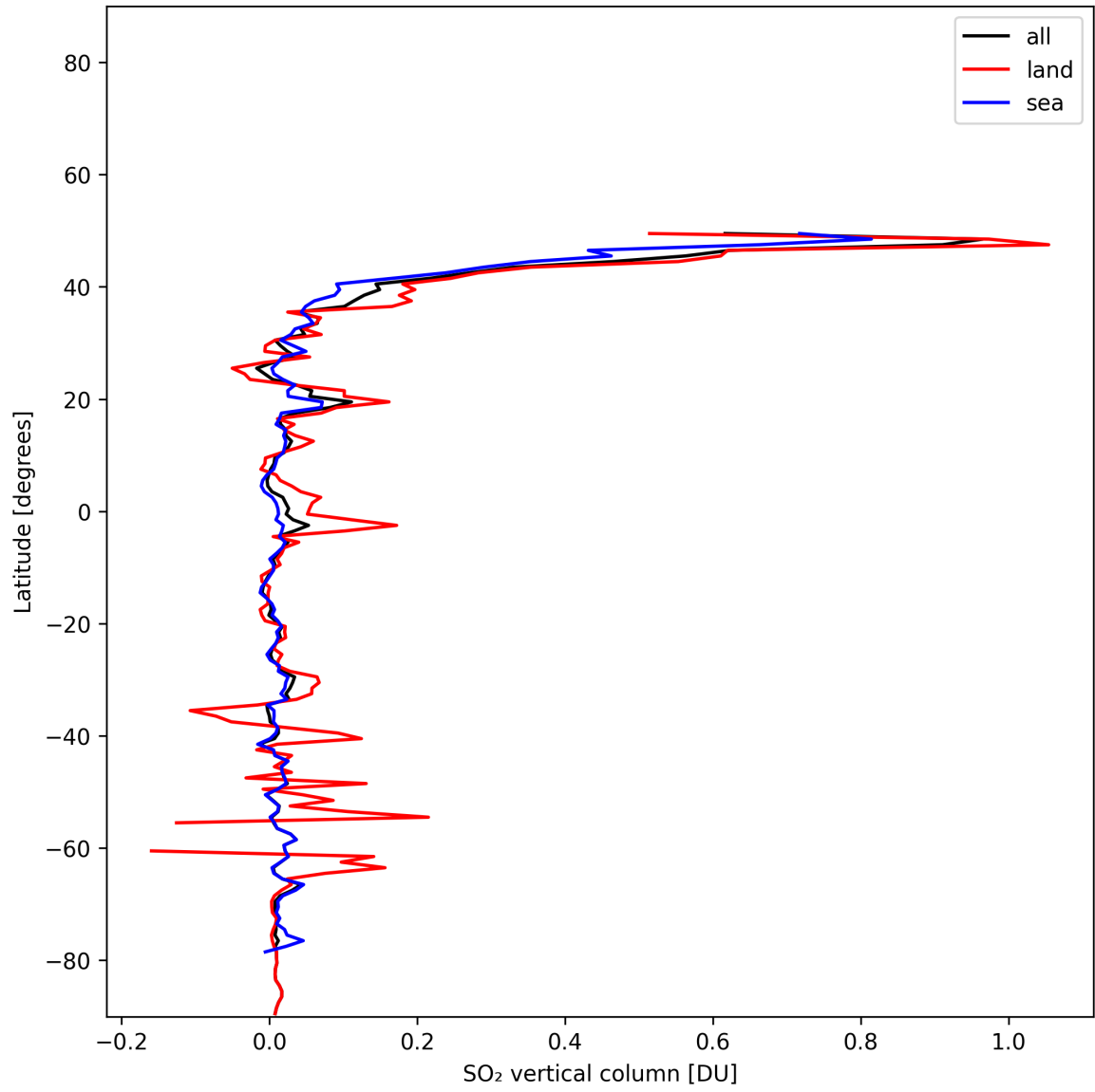
Figure 31: Zonal average of “SO 2 vertical column” for 2025-01-17 to 2025-01-18.
