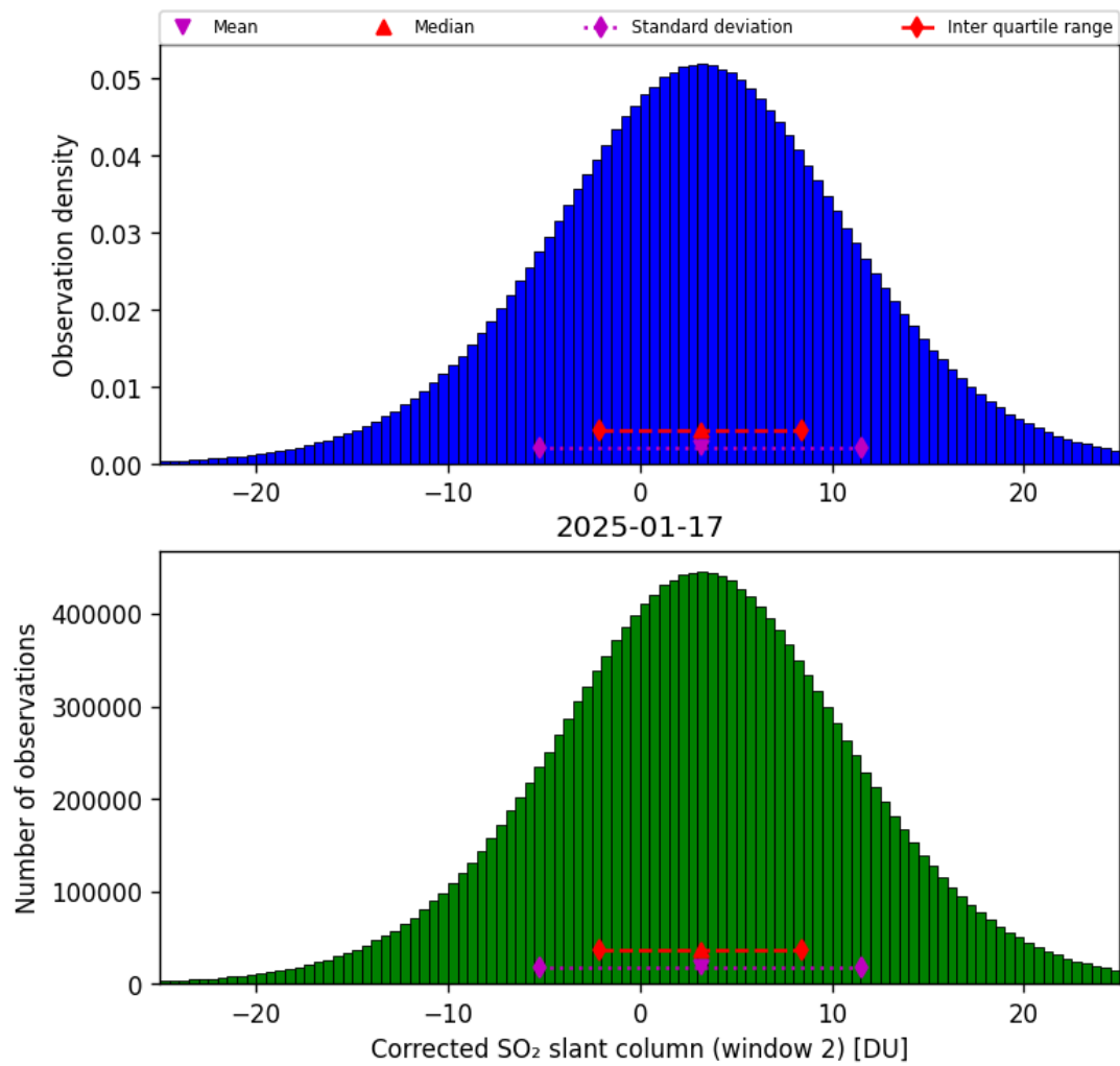
Figure 69: Histogram of “Corrected SO 2 slant column (window 2)” for 2025-01-17 to 2025-01-18
