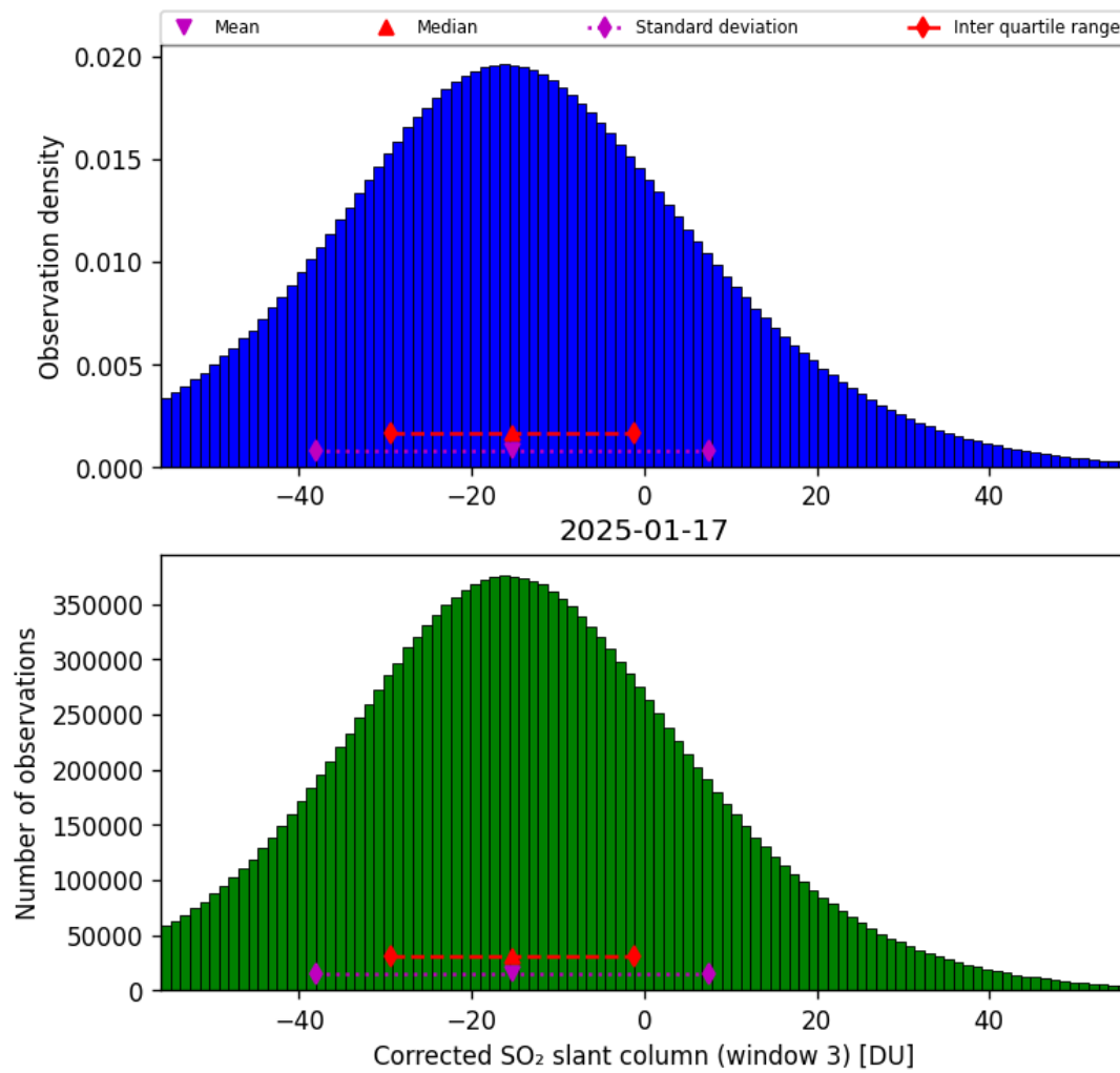
Figure 73: Histogram of “Corrected SO 2 slant column (window 3)” for 2025-01-17 to 2025-01-18
