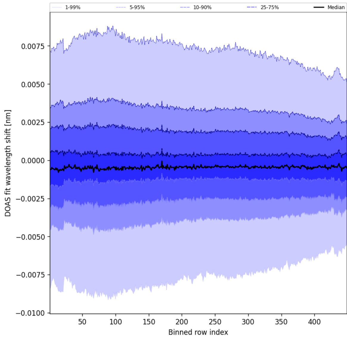
Figure 104: Along track statistics of “DOAS fit wavelength shift” for 2025-01-17 to 2025-01-18
