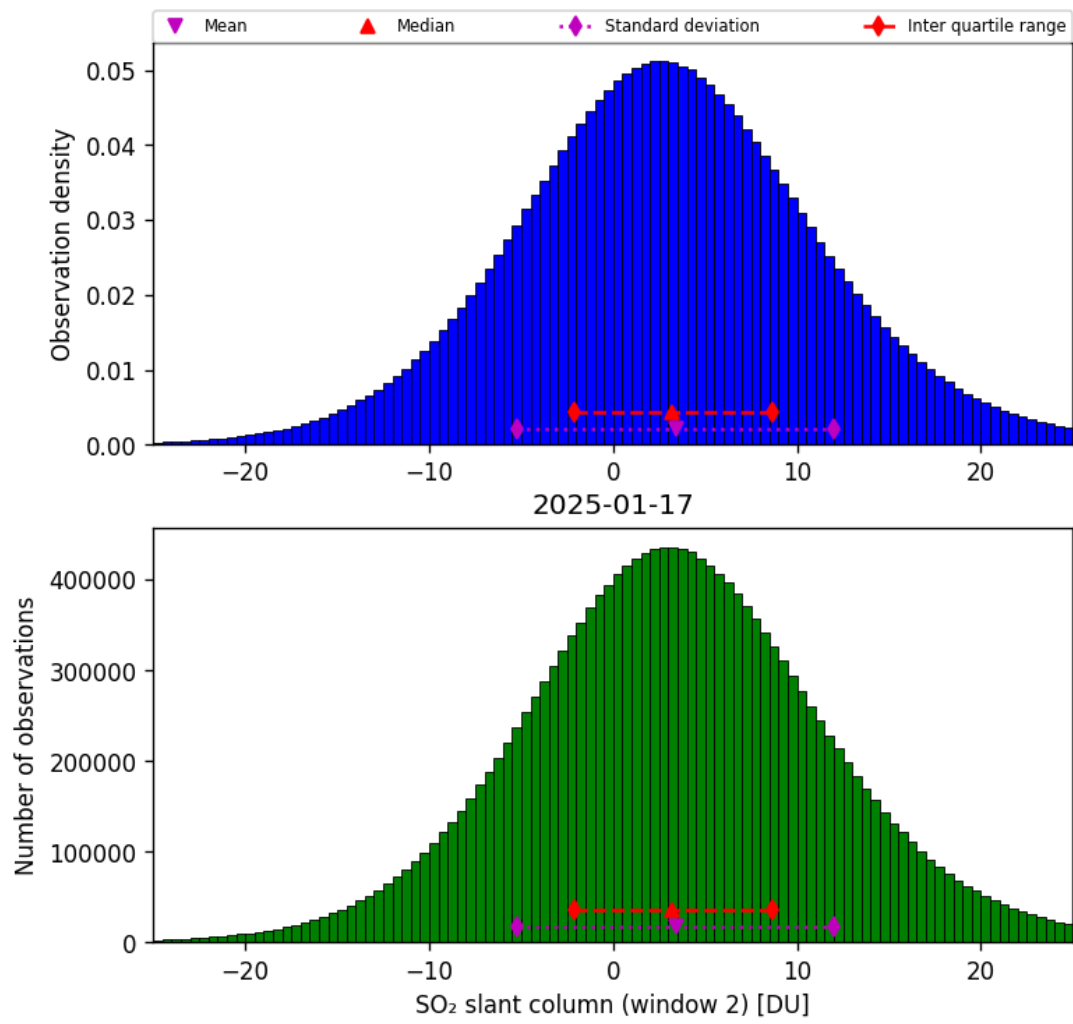
Figure 67: Histogram of “SO 2 slant column (window 2)” for 2025-01-17 to 2025-01-18
