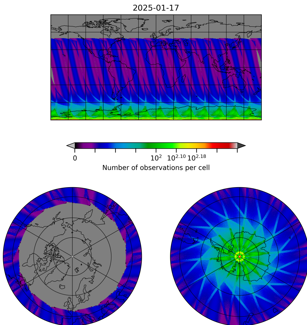
Figure 29: Map of the number of observations for 2025-01-17 to 2025-01-18
