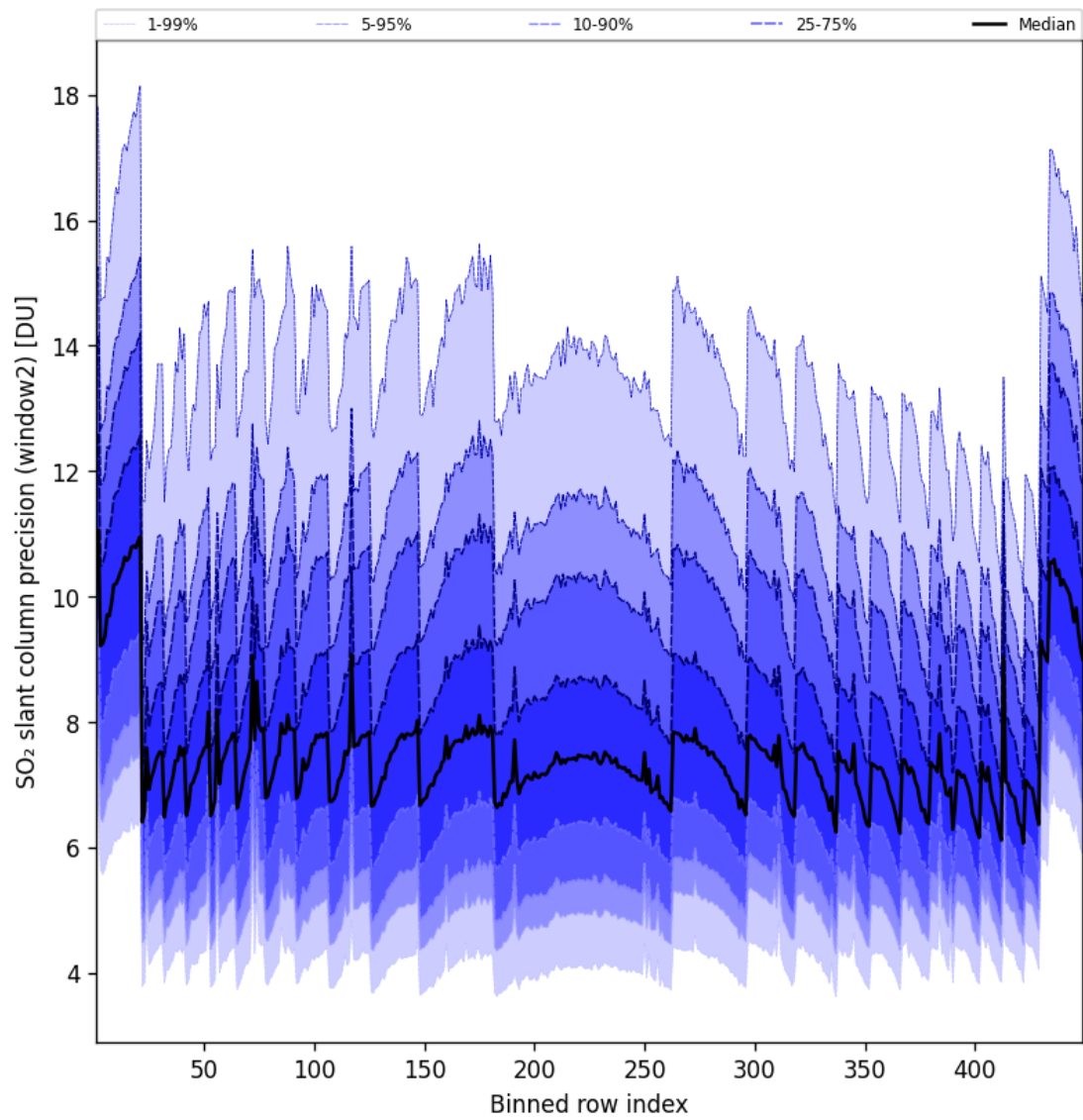
Figure 95: Along track statistics of “SO 2 slant column precision (window2)” for 2025-01-17 to 2025-01-18
