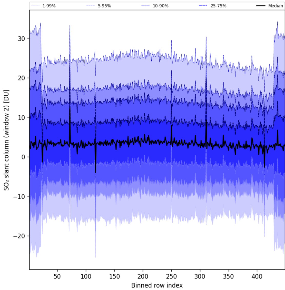
Figure 94: Along track statistics of “SO 2 slant column (window 2)” for 2025-01-17 to 2025-01-18
