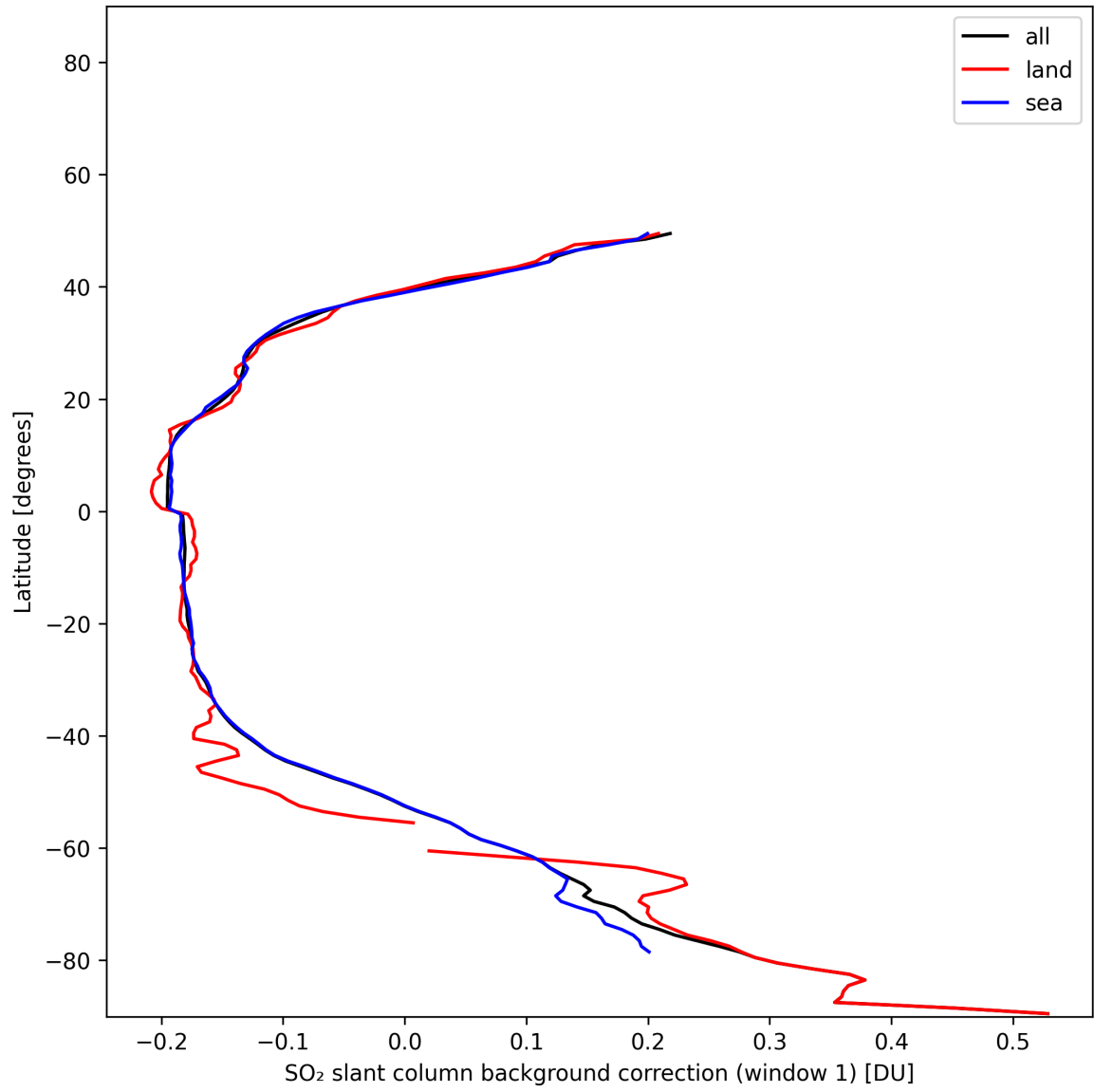
Figure 39: Zonal average of "SO 2 slant column background correction (window 1)" for 2025-01-17 to 2025-01-18.
