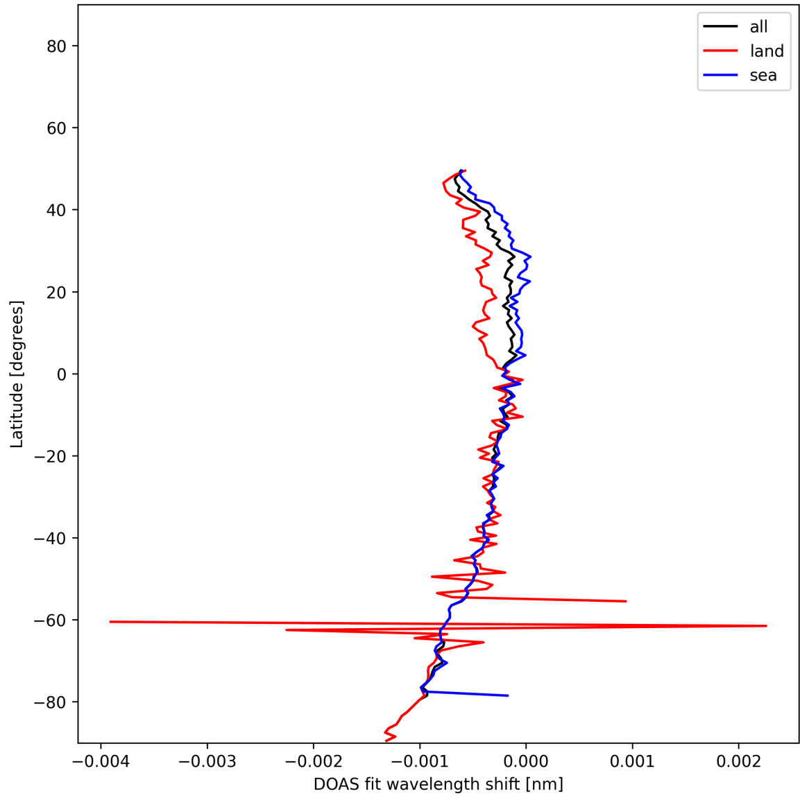
Figure 50: Zonal average of “DOAS fit wavelength shift” for 2025-01-17 to 2025-01-18.
