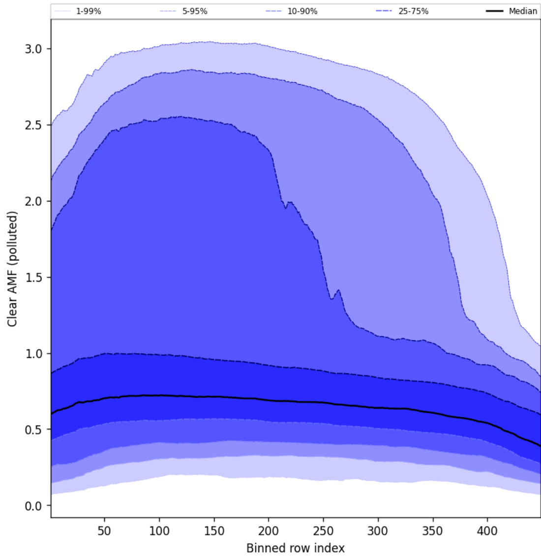
Figure 109: Along track statistics of “Clear AMF (polluted)” for 2025-01-17 to 2025-01-18
