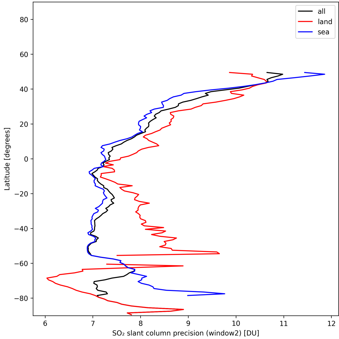
Figure 41: Zonal average of “SO 2 slant column precision (window2)” for 2025-01-17 to 2025-01-18.
