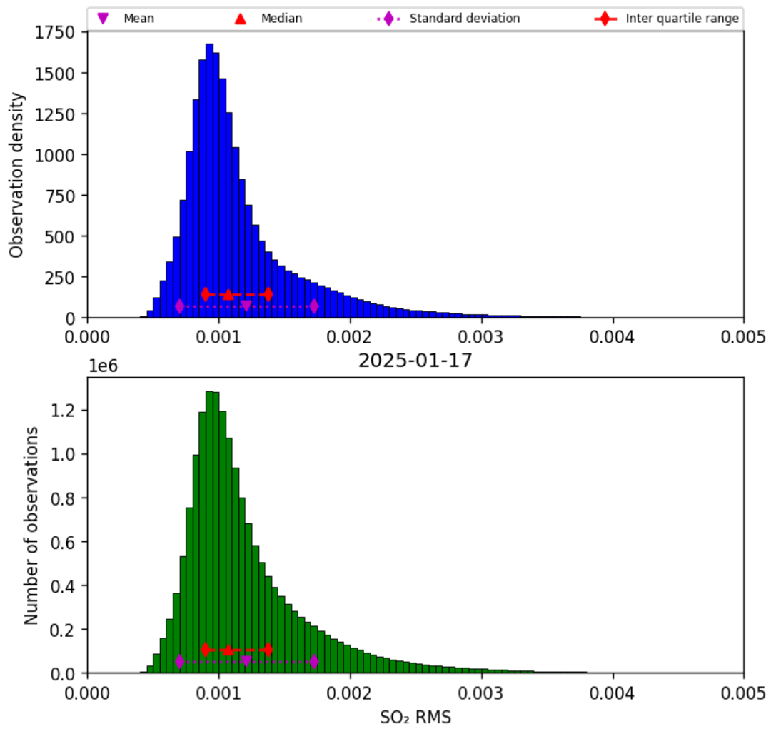
Figure 79: Histogram of “SO 2 RMS” for 2025-01-17 to 2025-01-18
