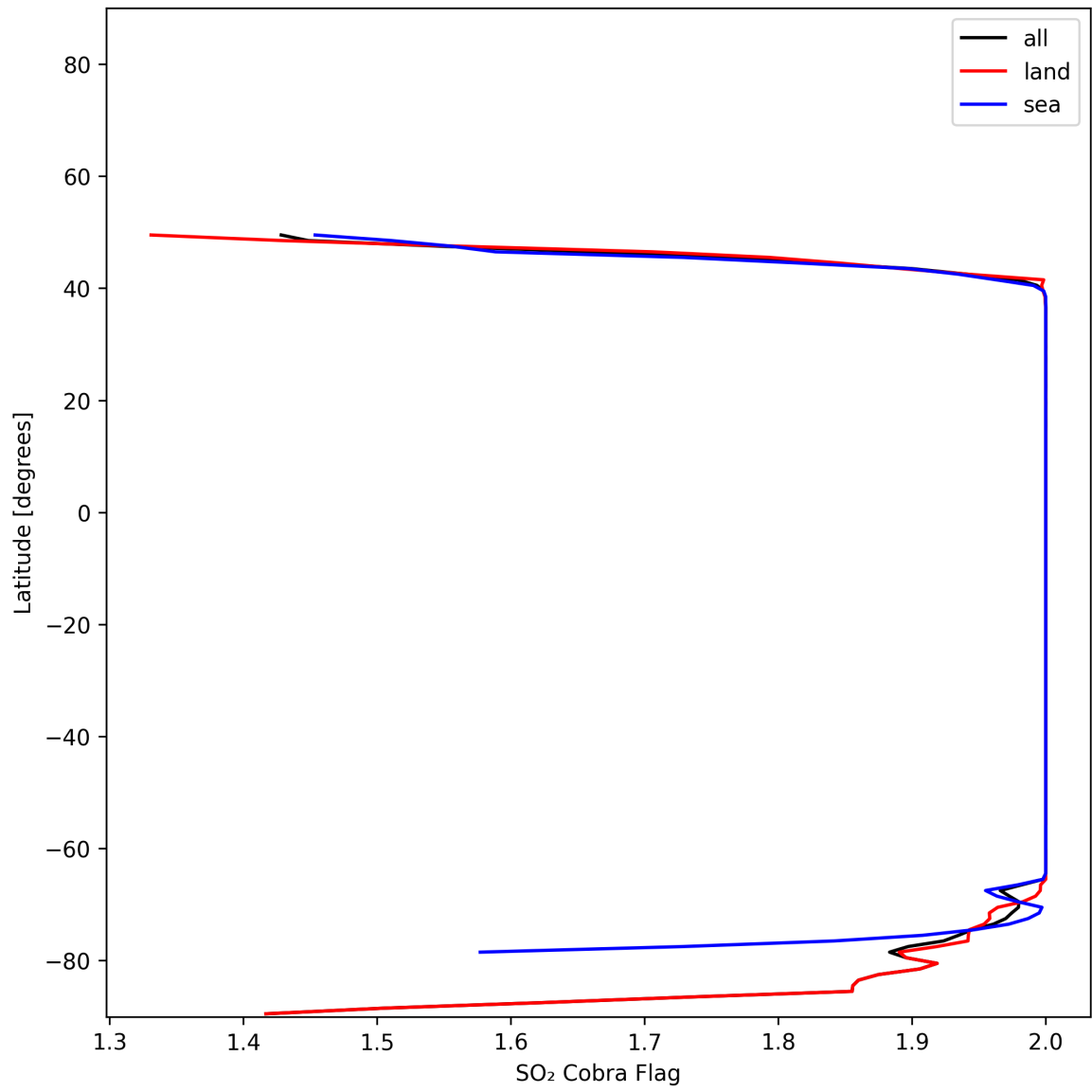
Figure 48: Zonal average of "SO 2 Cobra Flag" for 2025-01-17 to 2025-01-18.
