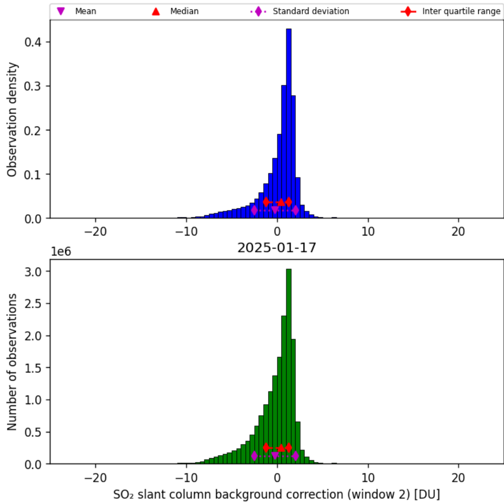
Figure 70: Histogram of “SO 2 slant column background correction (window 2)” for 2025-01-17 to 2025-01-18
