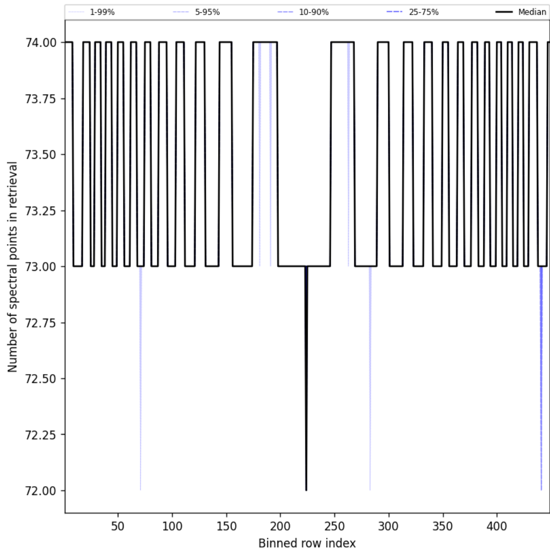
Figure 110: Along track statistics of “Number of spectral points in retrieval” for 2025-01-17 to 2025-01-18
