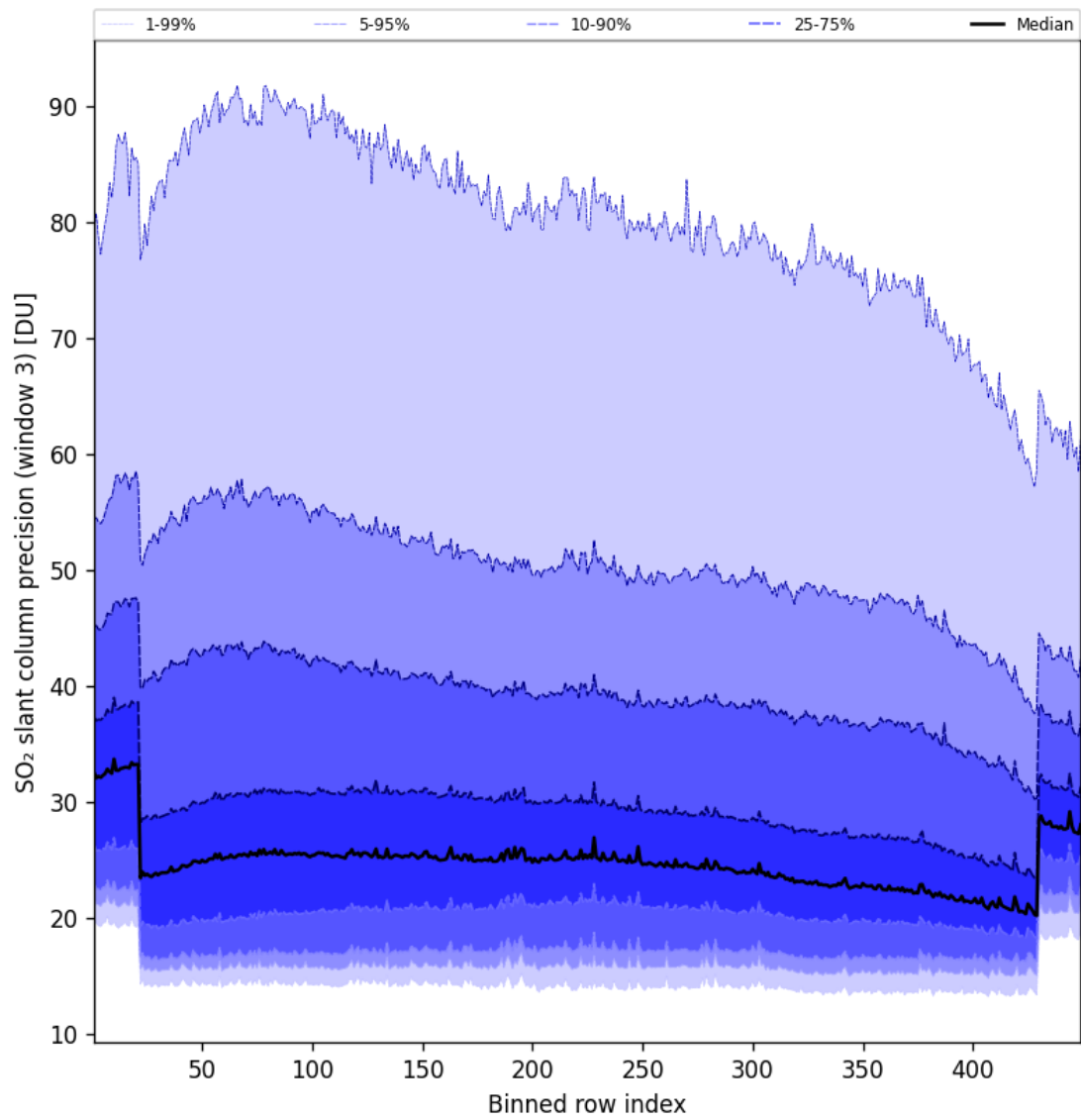
Figure 99: Along track statistics of “SO 2 slant column precision (window 3)” for 2025-01-21 to 2025-01-21
