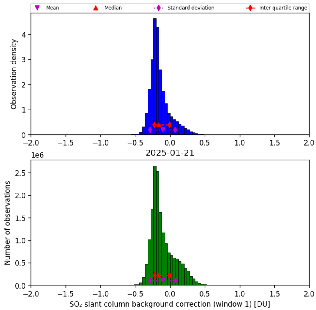
Figure 66: Histogram of “SO 2 slant column background correction (window 1)” for 2025-01-21 to 2025-01-21
