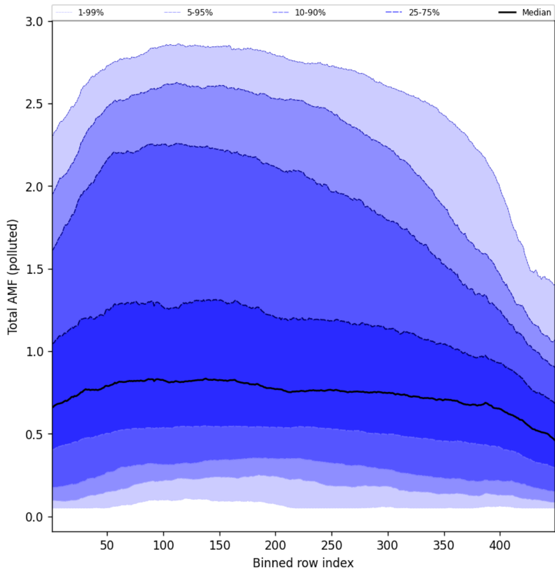
Figure 107: Along track statistics of “Total AMF (polluted)” for 2025-01-21 to 2025-01-21
