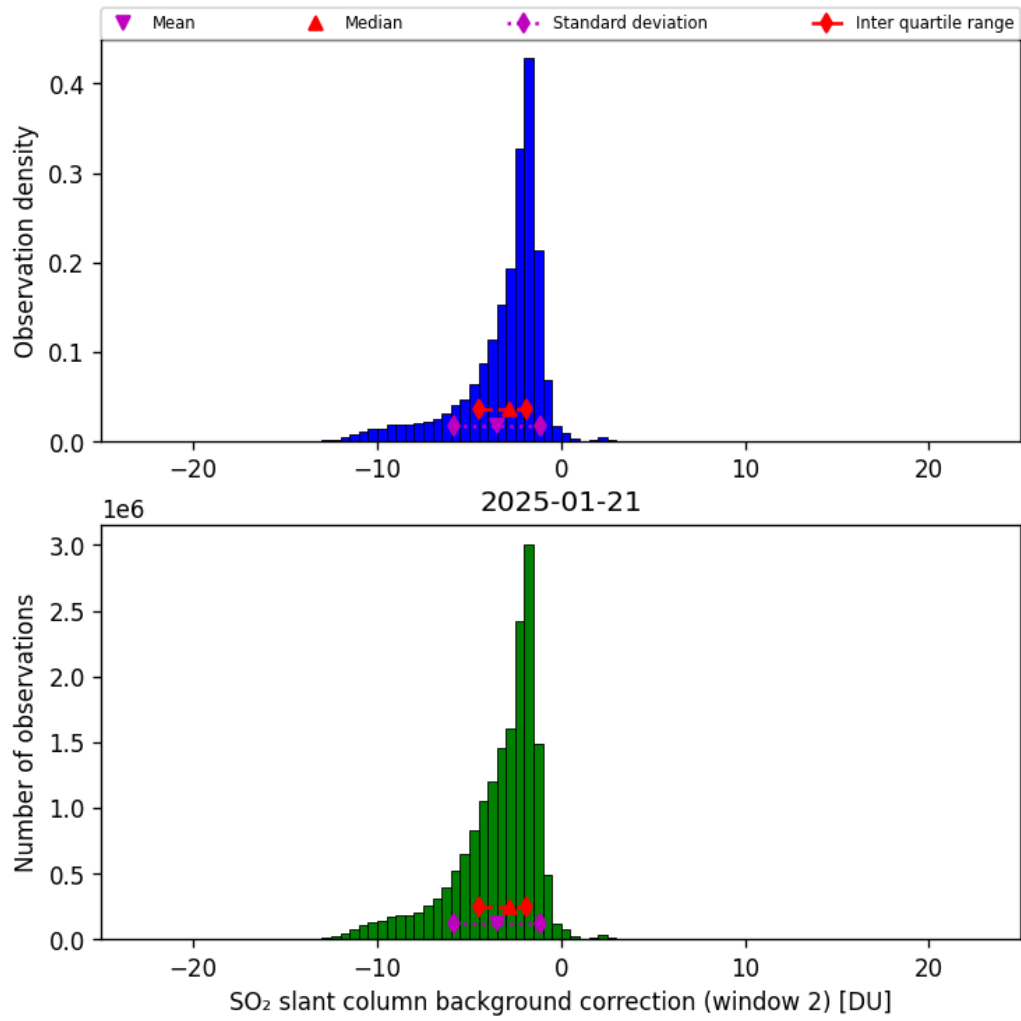
Figure 70: Histogram of “SO 2 slant column background correction (window 2)” for 2025-01-21 to 2025-01-21
