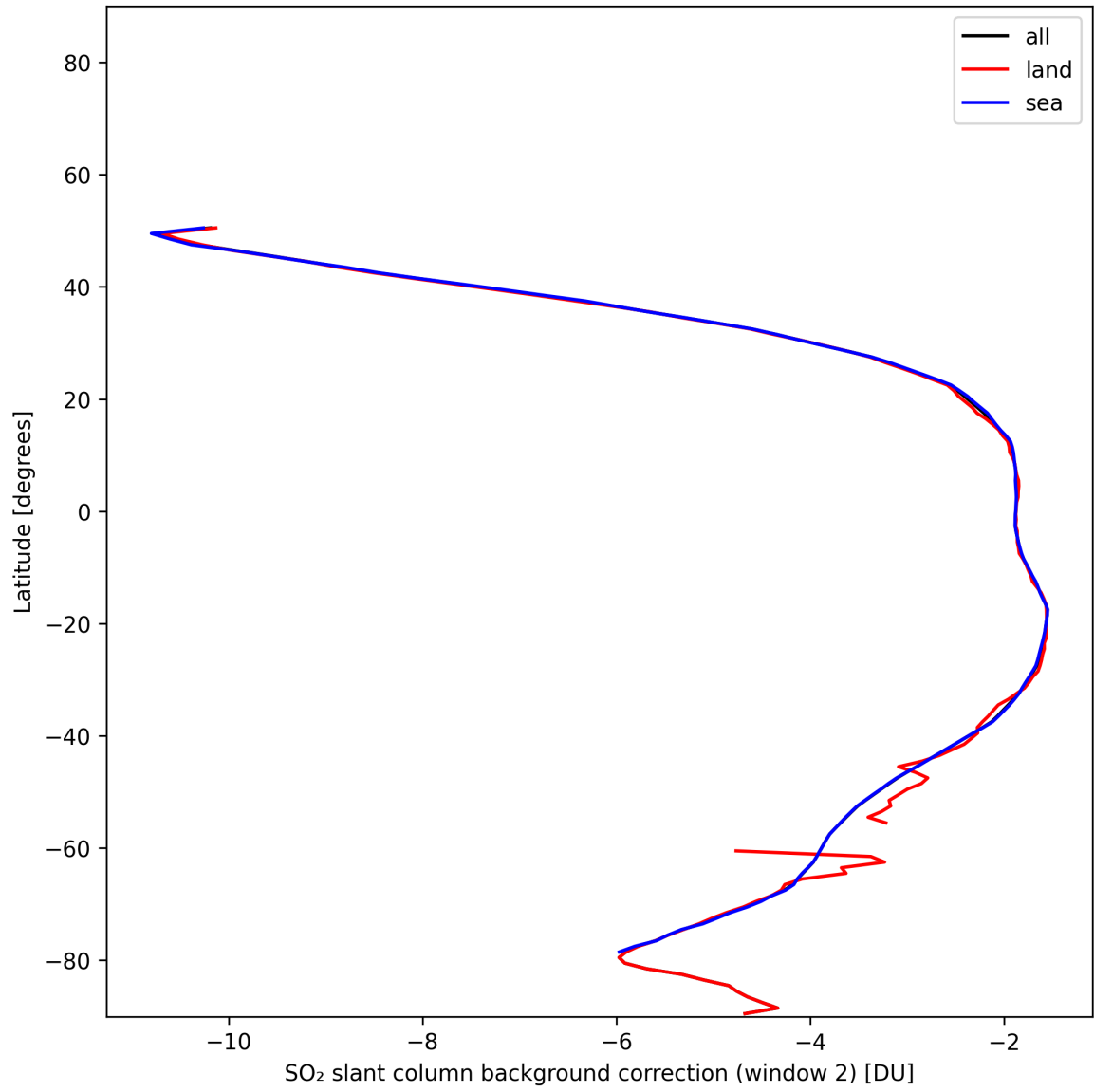
Figure 43: Zonal average of “SO 2 slant column background correction (window 2)” for 2025-01-21 to 2025-01-21.
