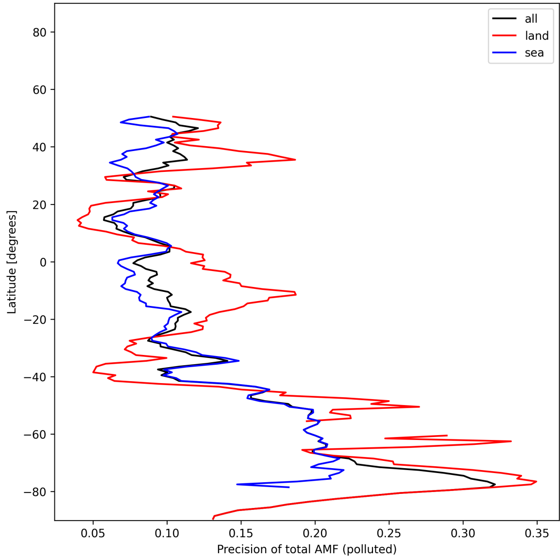
Figure 54: Zonal average of “Precision of total AMF (polluted)” for 2025-01-21 to 2025-01-21.
