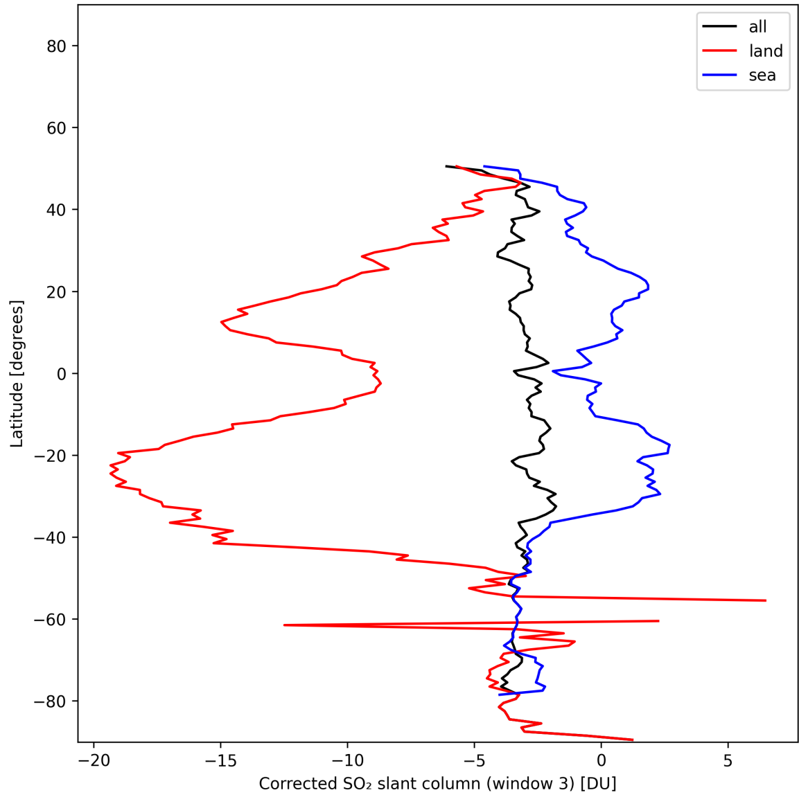
Figure 46: Zonal average of “Corrected SO 2 slant column (window 3)” for 2025-01-21 to 2025-01-21.
