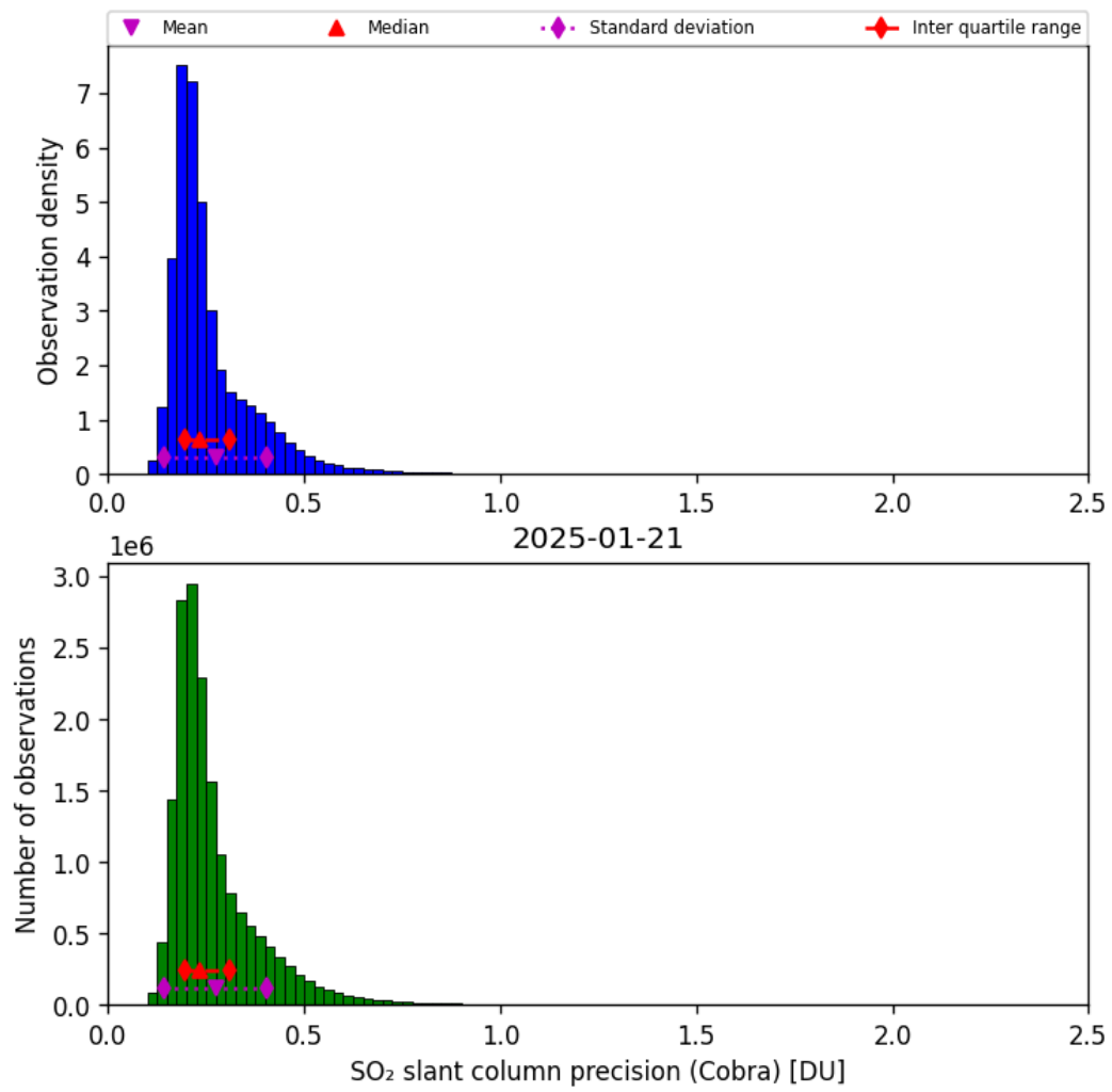
Figure 62: Histogram of “SO 2 slant column precision (Cobra)” for 2025-01-21 to 2025-01-21
