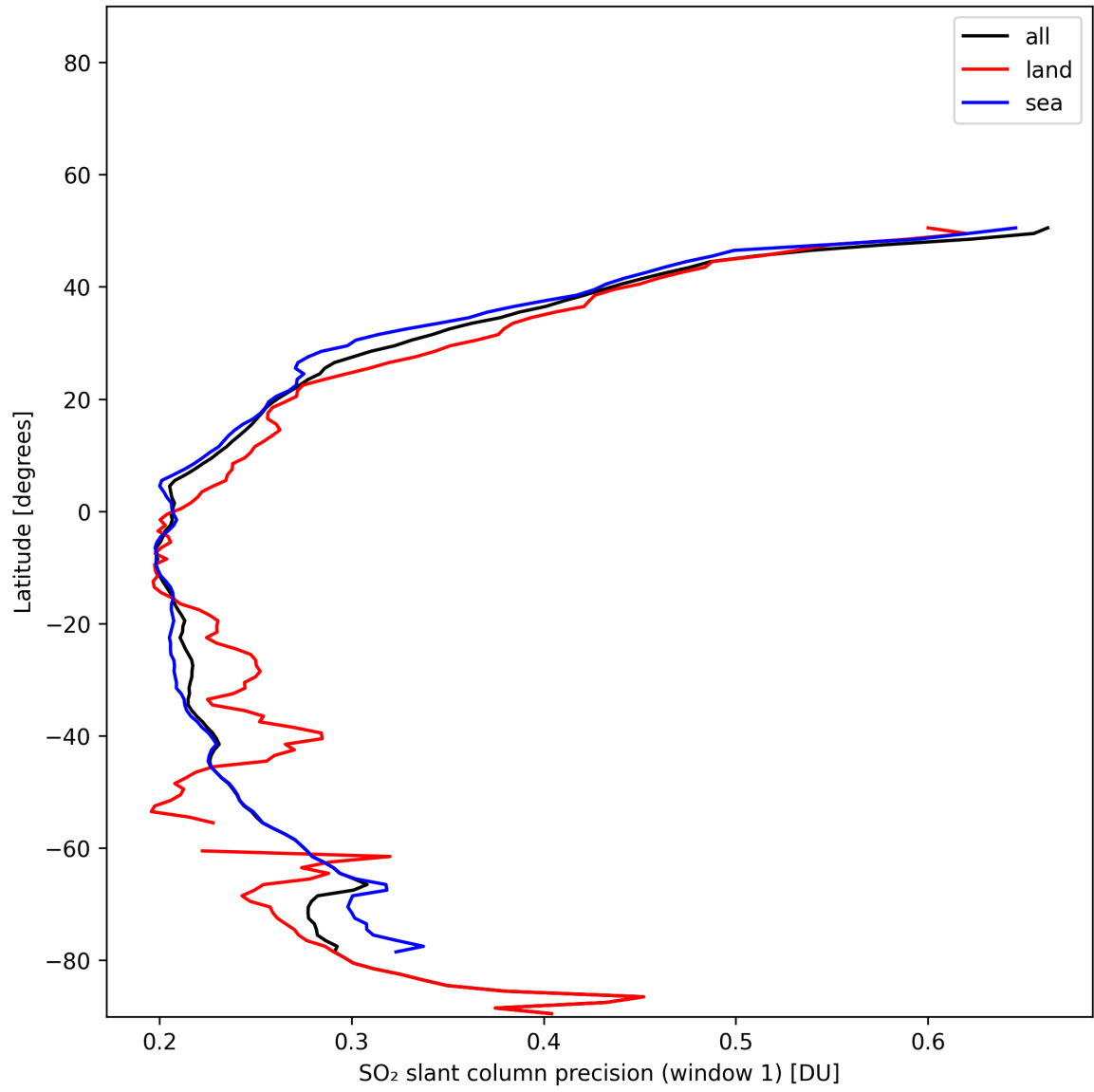
Figure 37: Zonal average of “SO 2 slant column precision (window 1)” for 2025-01-21 to 2025-01-21.
