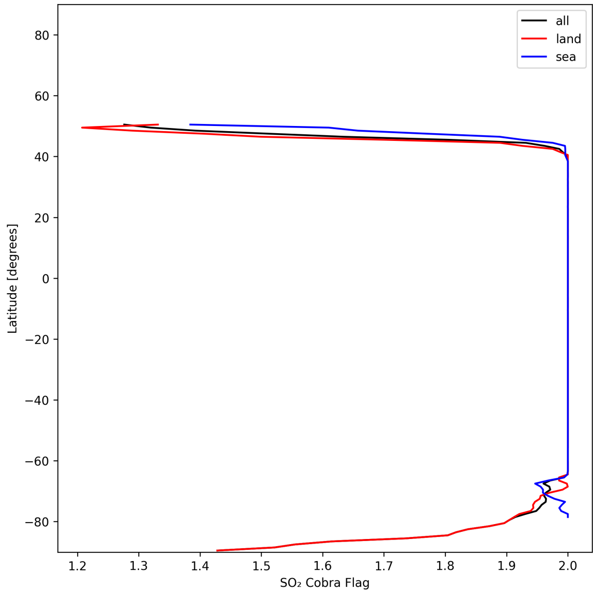
Figure 48: Zonal average of "SO 2 Cobra Flag" for 2025-01-21 to 2025-01-21.
