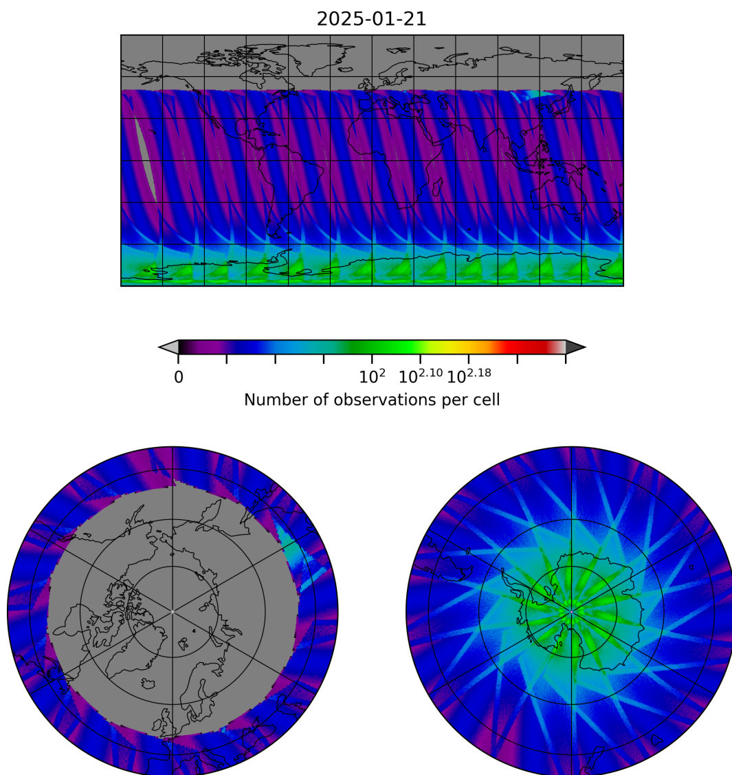
Figure 29: Map of the number of observations for 2025-01-21 to 2025-01-21
