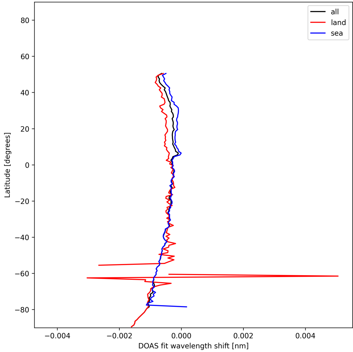
Figure 50: Zonal average of "DOAS fit wavelength shift" for 2025-01-21 to 2025-01-21.
