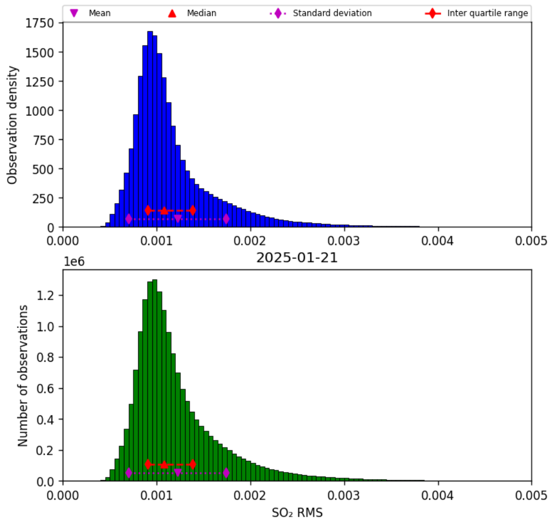
Figure 79: Histogram of “SO 2 RMS” for 2025-01-21 to 2025-01-21
