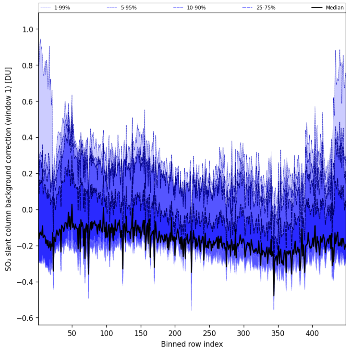
Figure 93: Along track statistics of “SO 2 slant column background correction (window 1)” for 2025-01-21 to 2025-01-21
