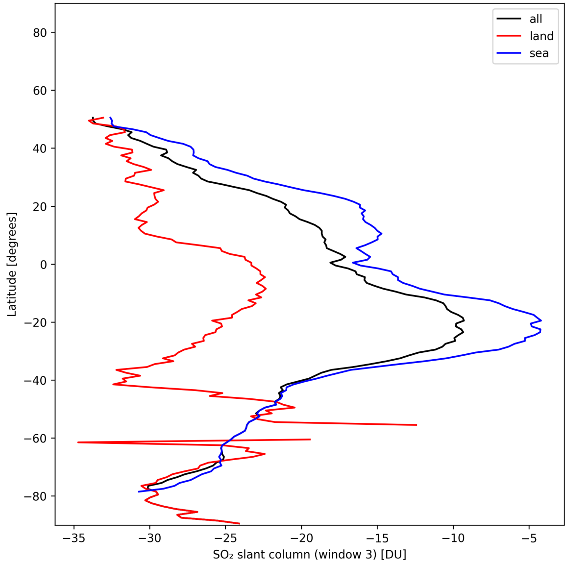
Figure 44: Zonal average of “SO 2 slant column (window 3)” for 2025-01-21 to 2025-01-21.
