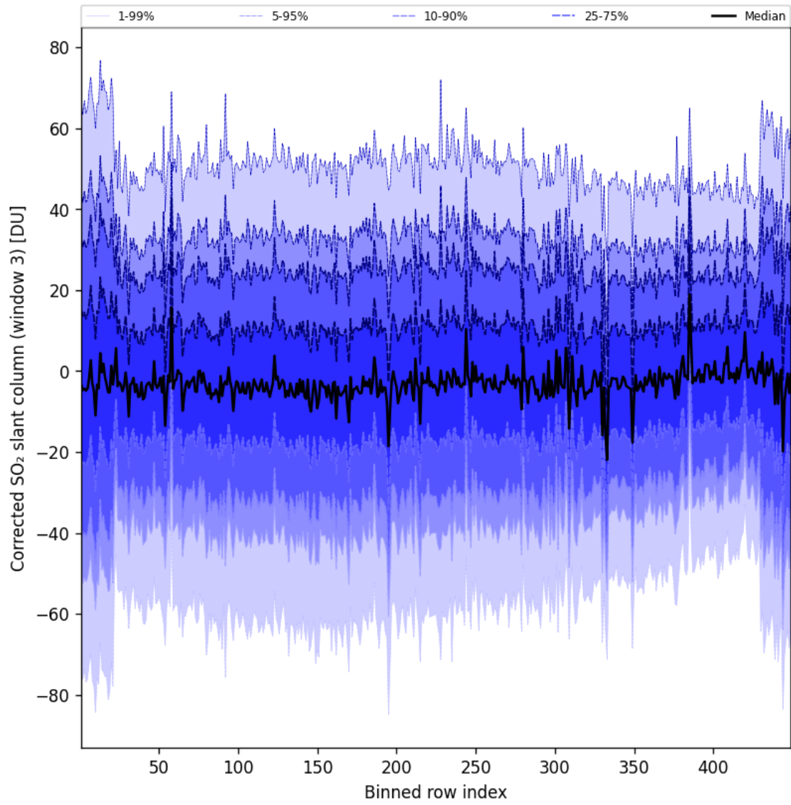
Figure 100: Along track statistics of “Corrected SO 2 slant column (window 3)” for 2025-01-21 to 2025-01-21
