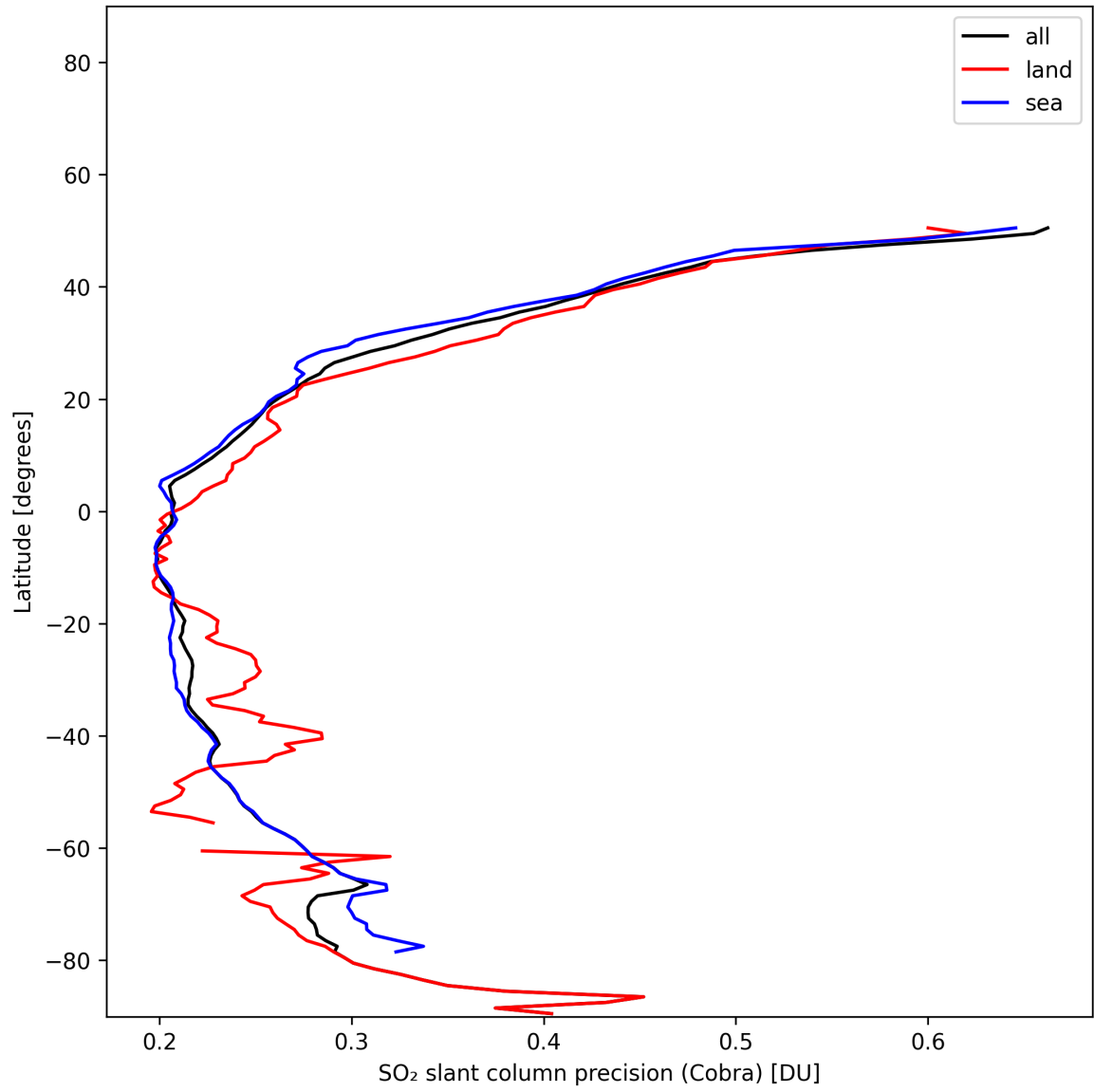
Figure 35: Zonal average of “SO 2 slant column precision (Cobra)” for 2025-01-21 to 2025-01-21.
