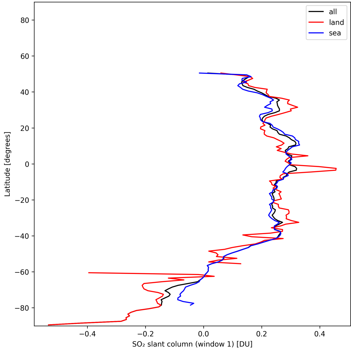
Figure 36: Zonal average of “SO 2 slant column (window 1)” for 2025-01-21 to 2025-01-21.
