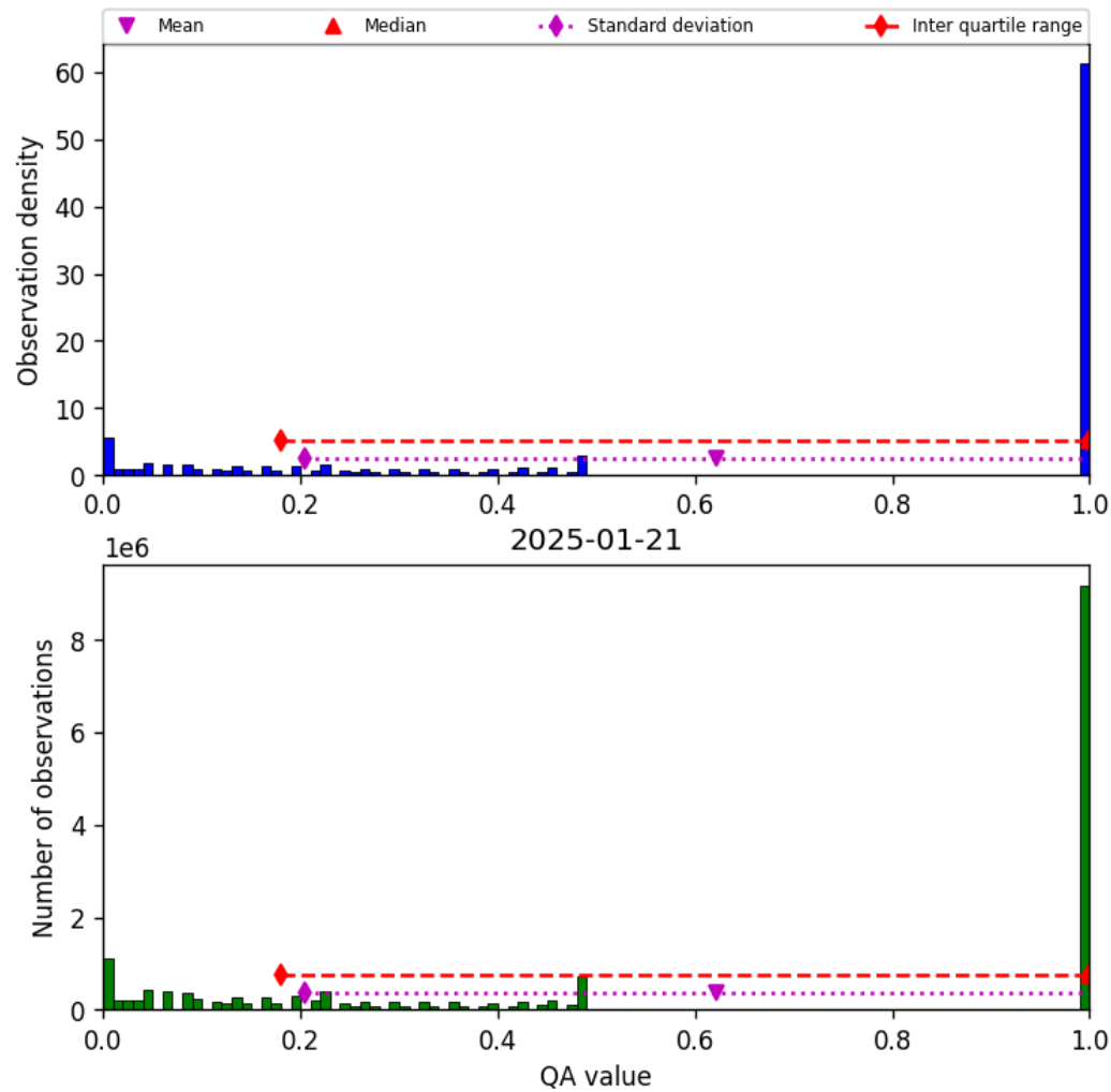
Figure 57: Histogram of “QA value” for 2025-01-21 to 2025-01-21
