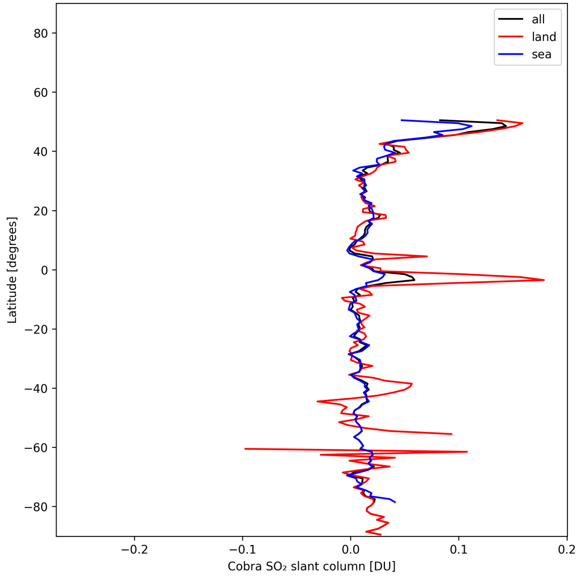
Figure 34: Zonal average of “Cobra SO 2 slant column” for 2025-01-21 to 2025-01-21.
