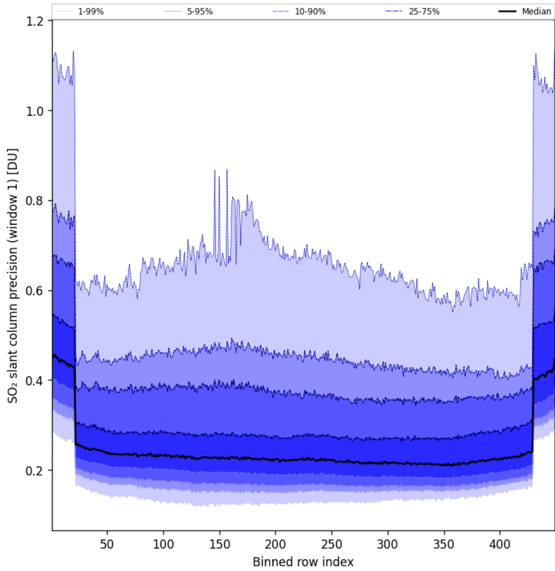
Figure 91: Along track statistics of "SO 2 slant column precision (window 1)" for 2025-01-21 to 2025-01-21
