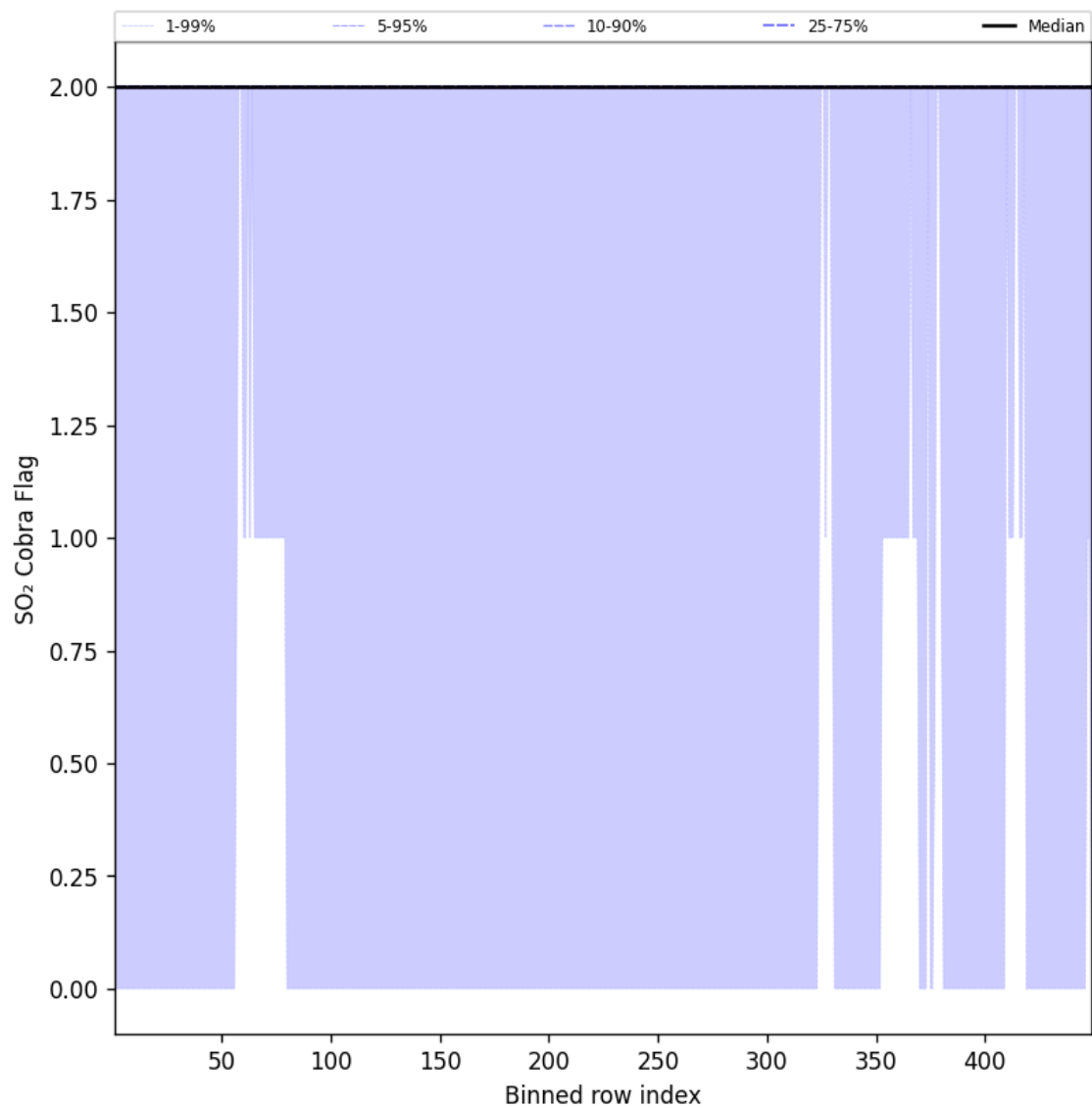
Figure 102: Along track statistics of “SO 2 Cobra Flag” for 2025-01-21 to 2025-01-21
