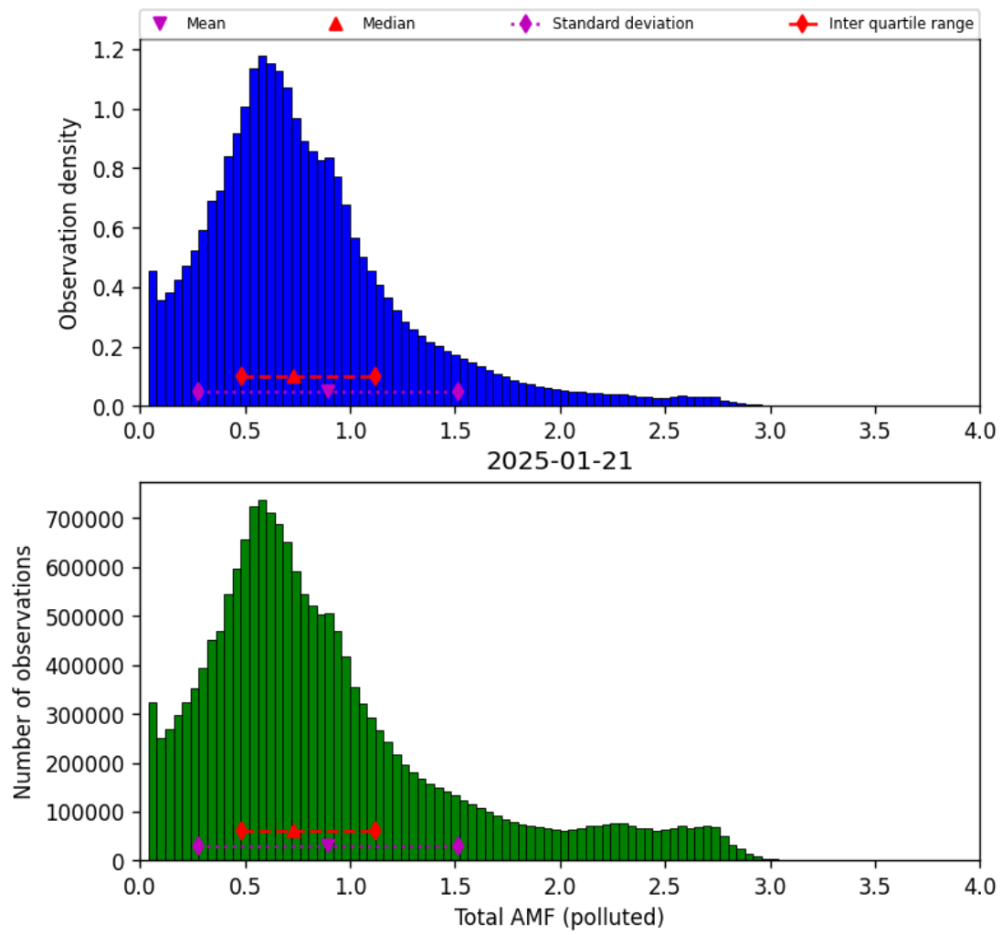
Figure 80: Histogram of “Total AMF (polluted)” for 2025-01-21 to 2025-01-21
