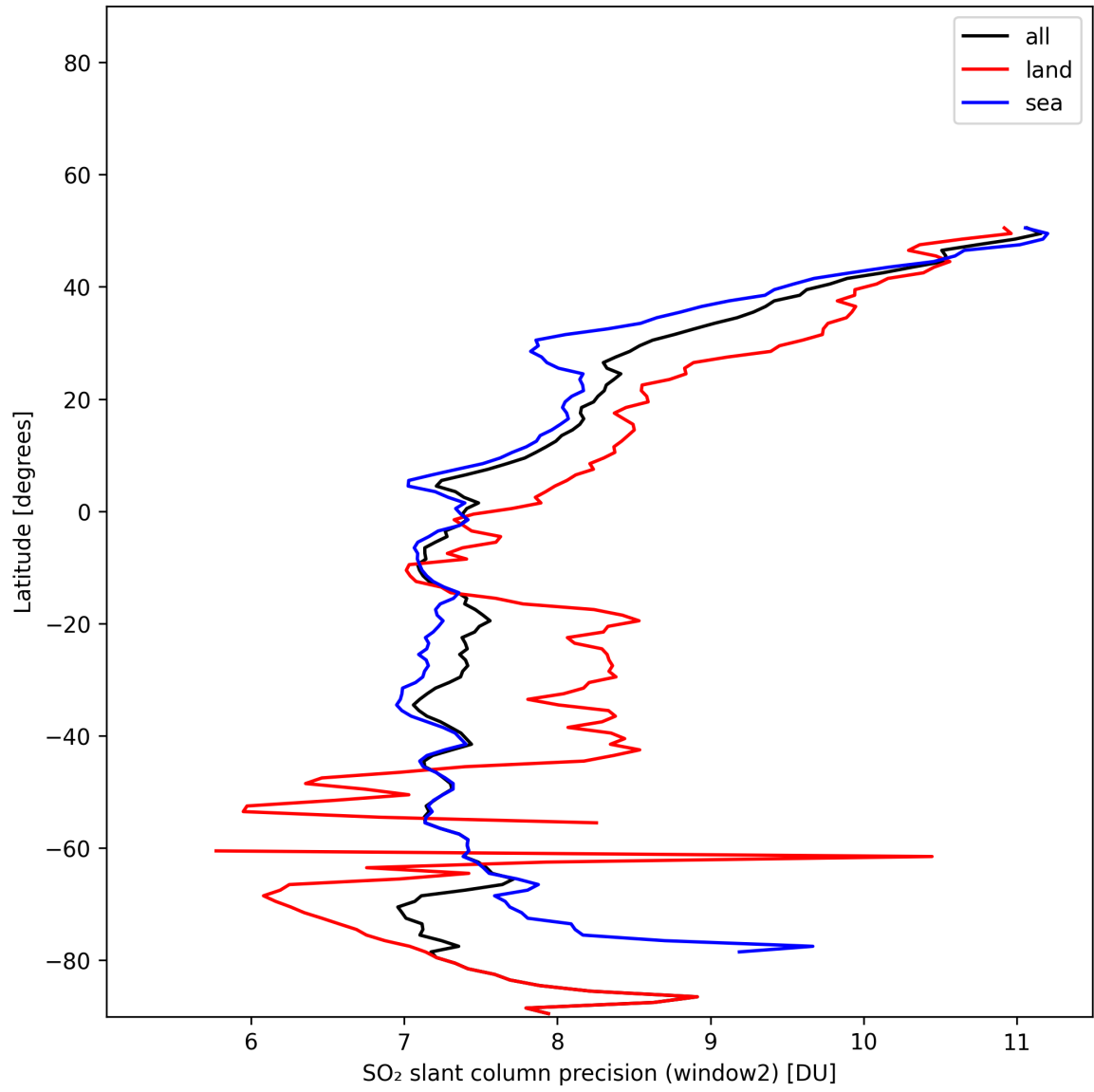
Figure 41: Zonal average of “SO 2 slant column precision (window2)” for 2025-01-21 to 2025-01-21.
