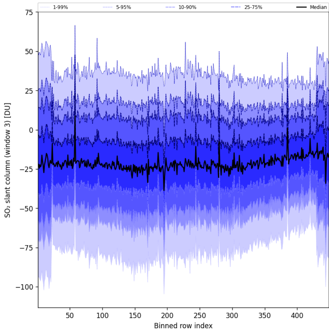
Figure 98: Along track statistics of “SO 2 slant column (window 3)” for 2025-01-21 to 2025-01-21
