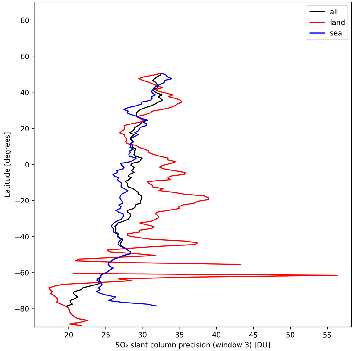
Figure 45: Zonal average of “SO 2 slant column precision (window 3)” for 2025-01-21 to 2025-01-21.
