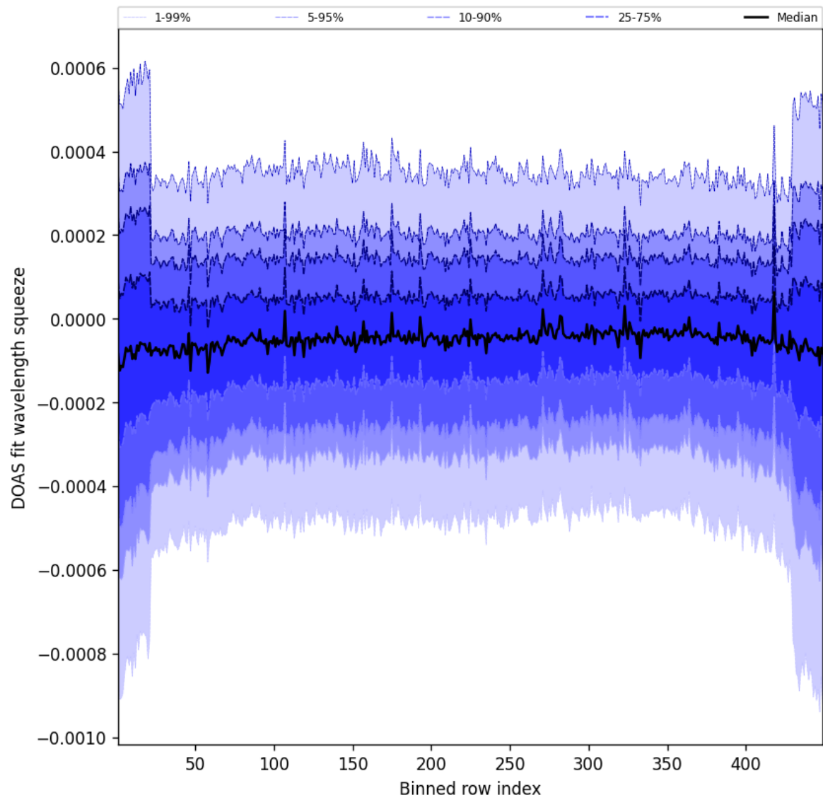
Figure 105: Along track statistics of “DOAS fit wavelength squeeze” for 2025-01-21 to 2025-01-21
