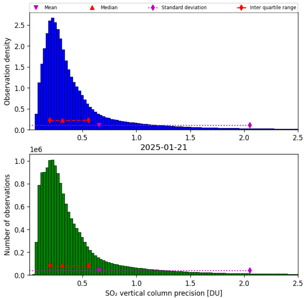
Figure 59: Histogram of “SO 2 vertical column precision” for 2025-01-21 to 2025-01-21
