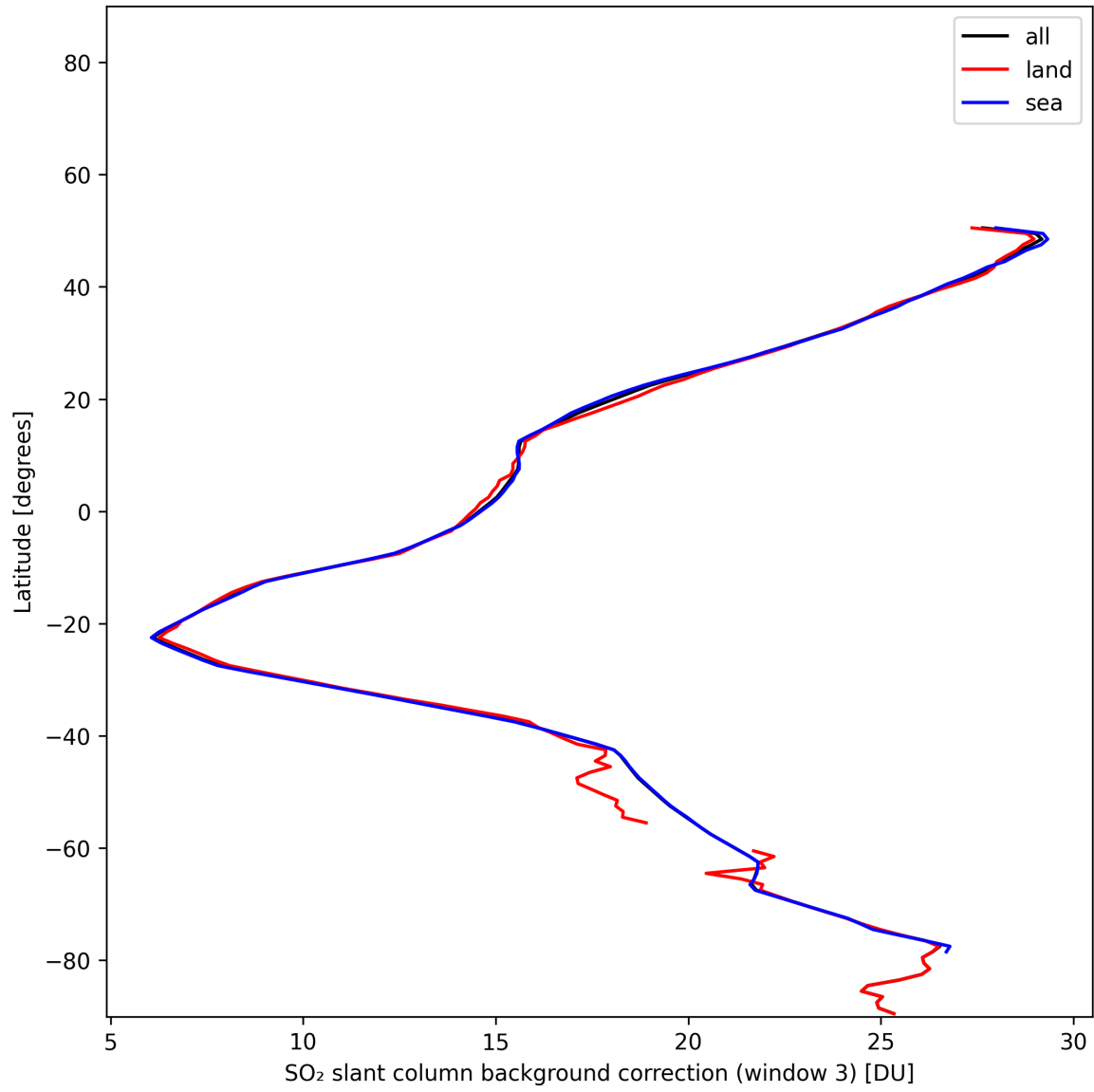
Figure 47: Zonal average of “SO 2 slant column background correction (window 3)” for 2025-01-21 to 2025-01-21.
