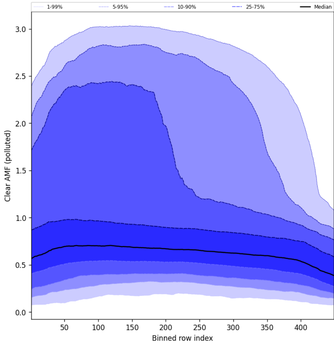
Figure 109: Along track statistics of “Clear AMF (polluted)” for 2025-01-21 to 2025-01-21
