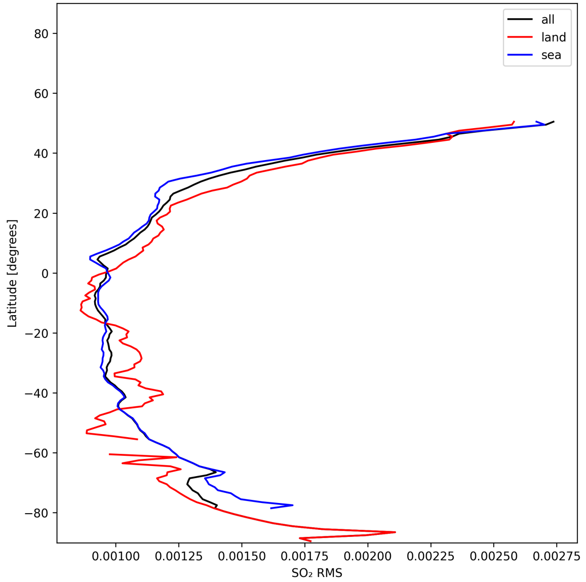
Figure 52: Zonal average of “SO 2 RMS” for 2025-01-21 to 2025-01-21.
