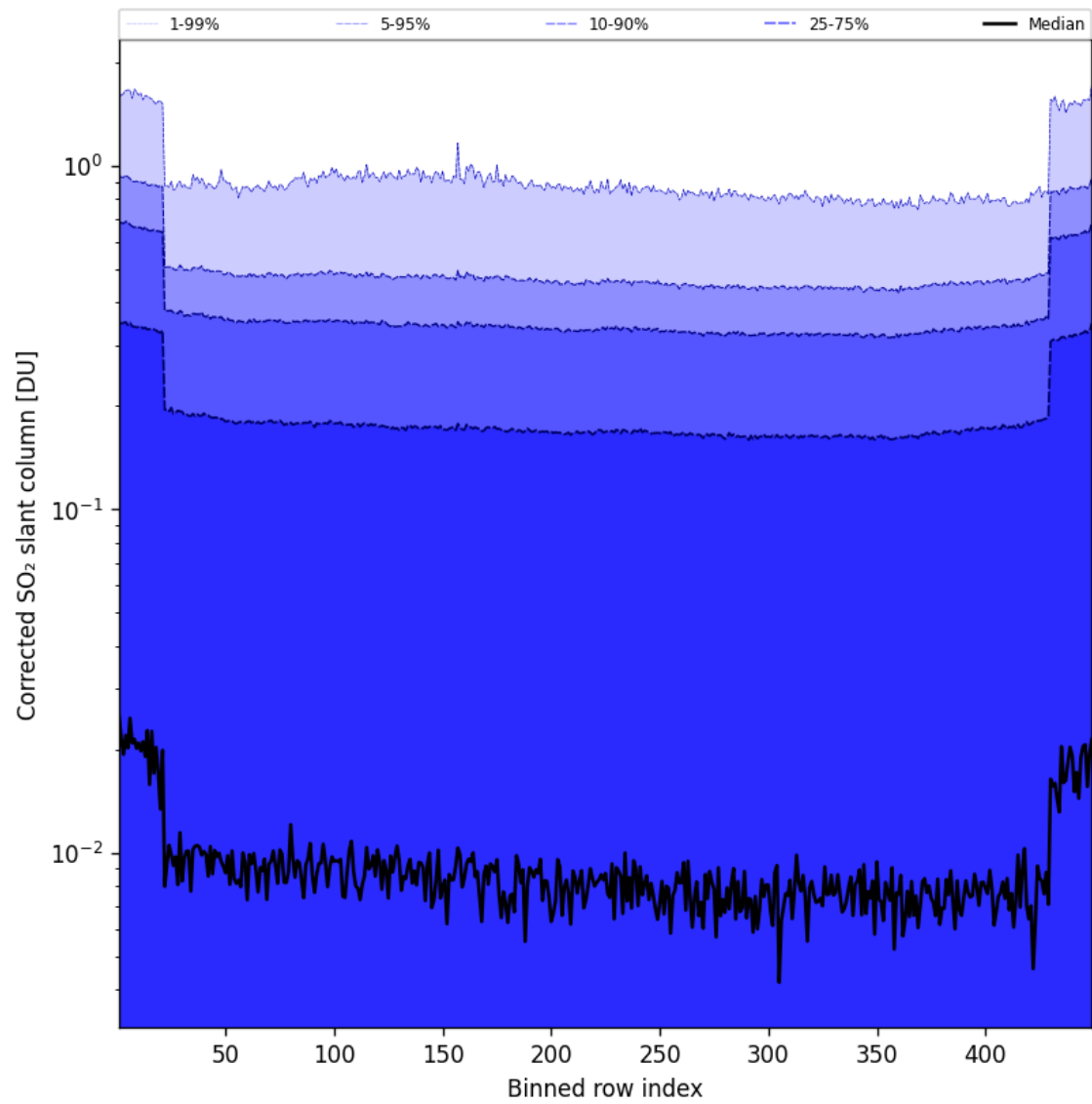
Figure 87: Along track statistics of “Corrected SO 2 slant column” for 2025-01-21 to 2025-01-21
