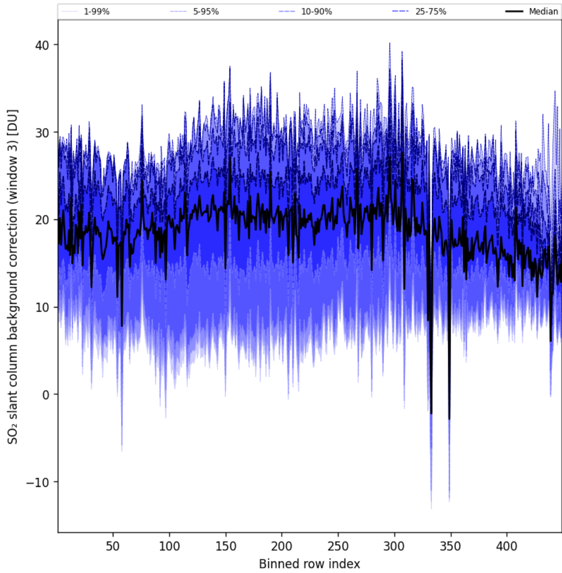
Figure 101: Along track statistics of “SO 2 slant column background correction (window 3)” for 2025-01-21 to 2025-01-21
