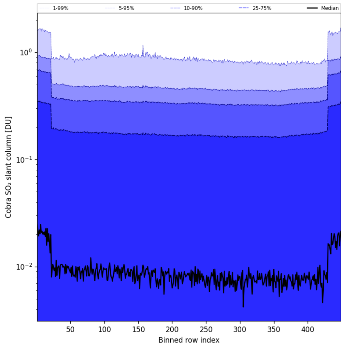
Figure 88: Along track statistics of “Cobra SO 2 slant column” for 2025-01-21 to 2025-01-21
