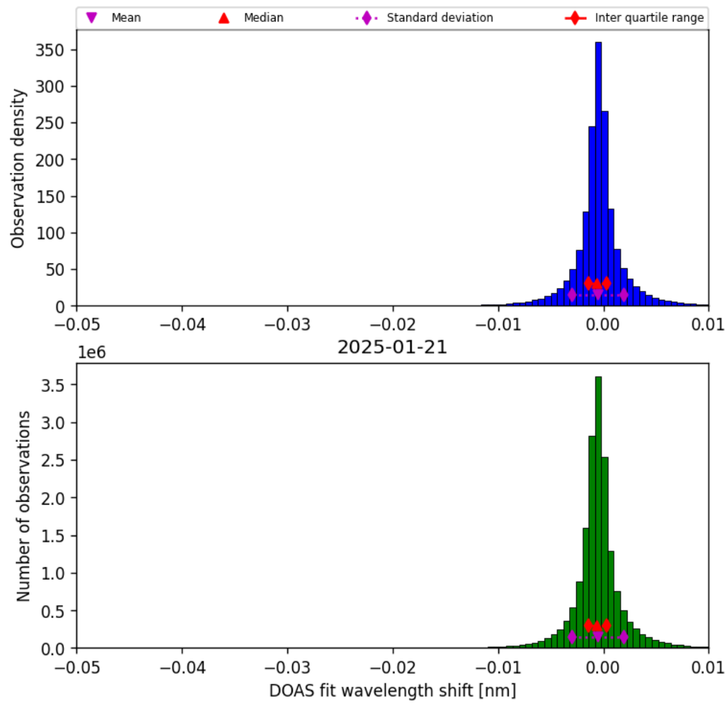
Figure 77: Histogram of “DOAS fit wavelength shift” for 2025-01-21 to 2025-01-21
