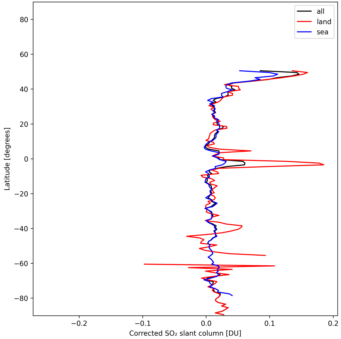
Figure 33: Zonal average of “Corrected SO 2 slant column” for 2025-01-21 to 2025-01-21.
