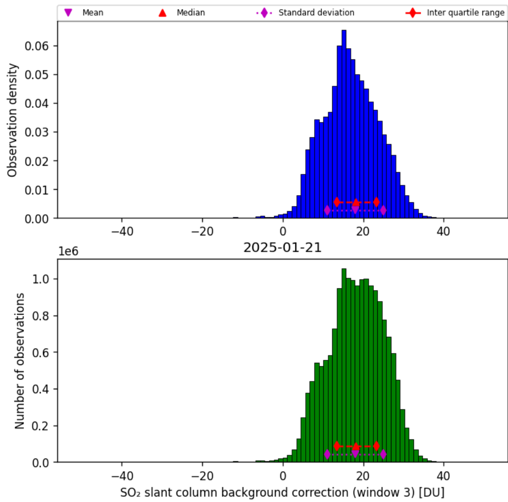
Figure 74: Histogram of “SO 2 slant column background correction (window 3)” for 2025-01-21 to 2025-01-21
