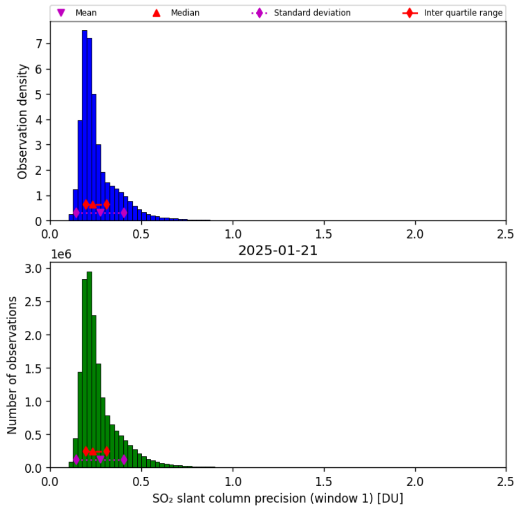
Figure 64: Histogram of “SO 2 slant column precision (window 1)” for 2025-01-21 to 2025-01-21
