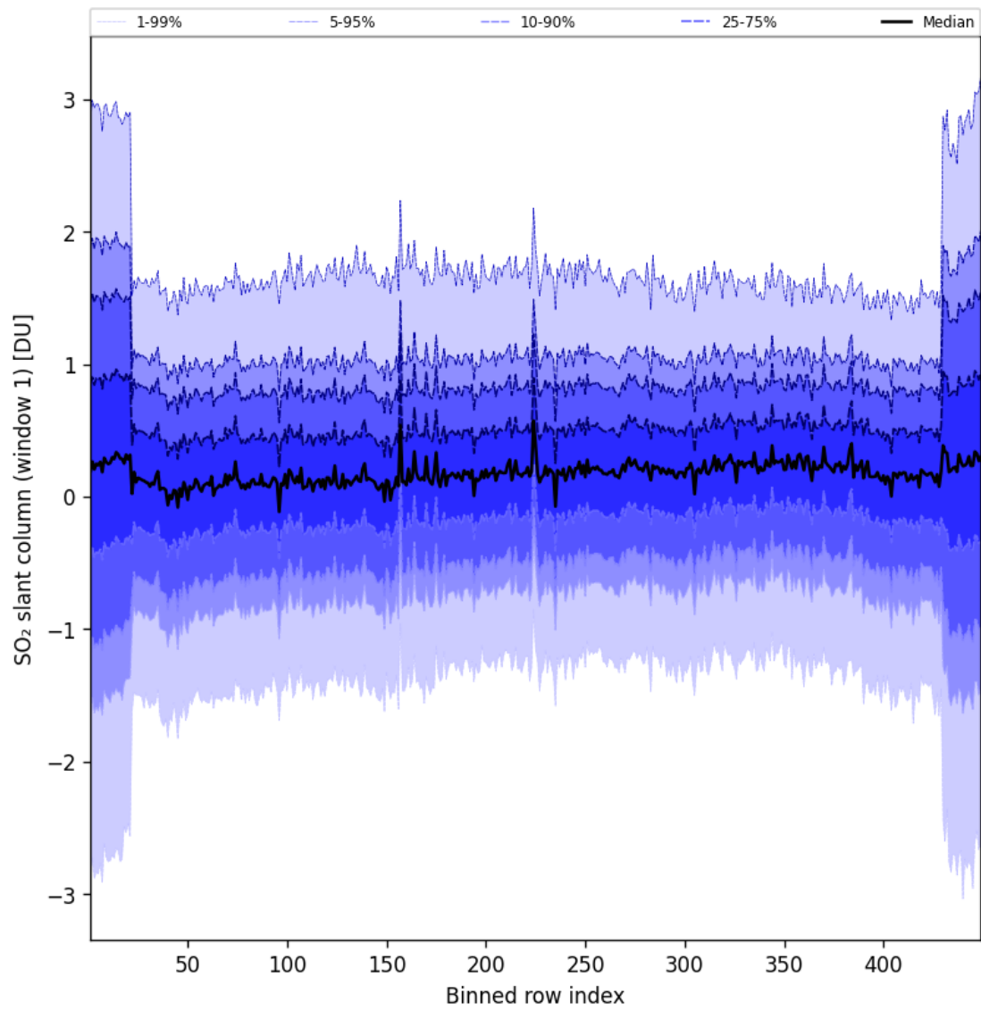
Figure 90: Along track statistics of “SO 2 slant column (window 1)” for 2025-01-21 to 2025-01-21
