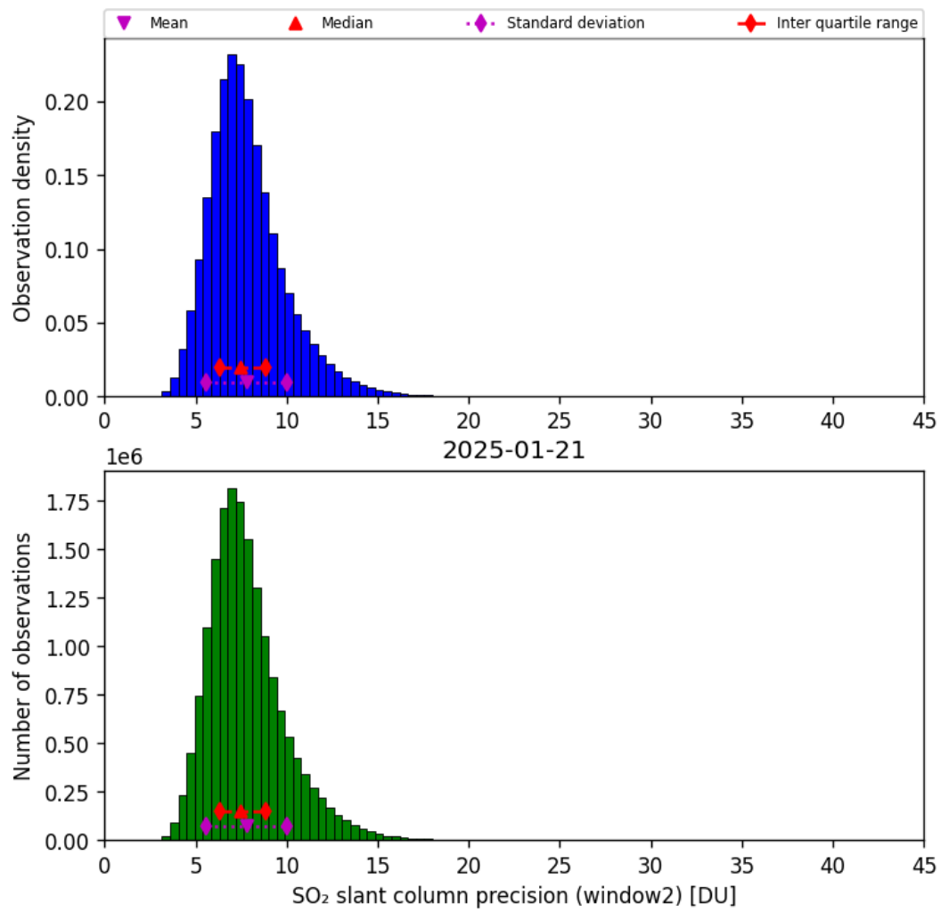
Figure 68: Histogram of “SO 2 slant column precision (window2)” for 2025-01-21 to 2025-01-21
