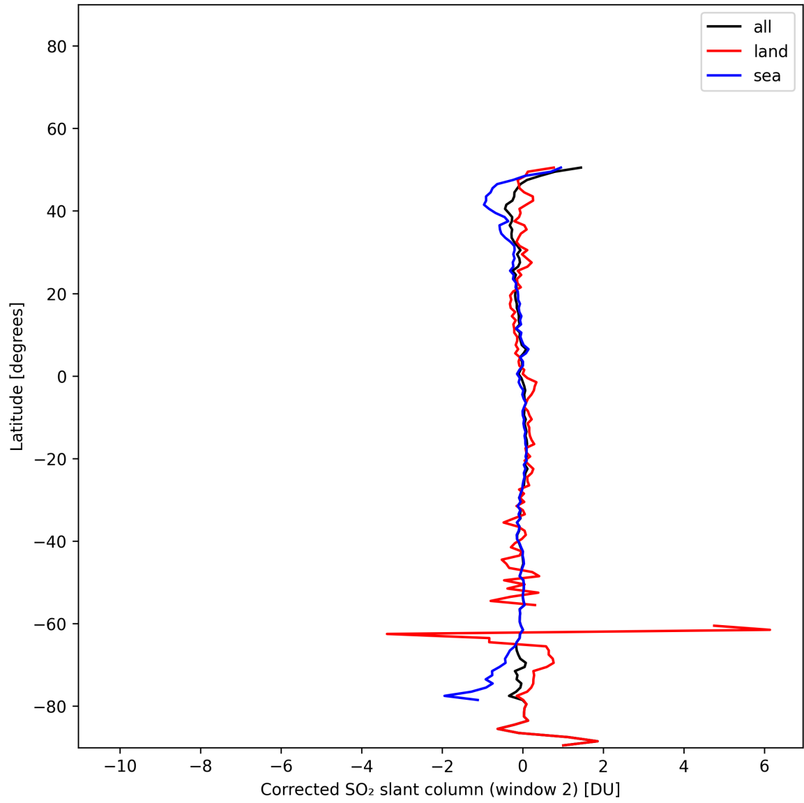
Figure 42: Zonal average of “Corrected SO 2 slant column (window 2)” for 2025-01-21 to 2025-01-21.
