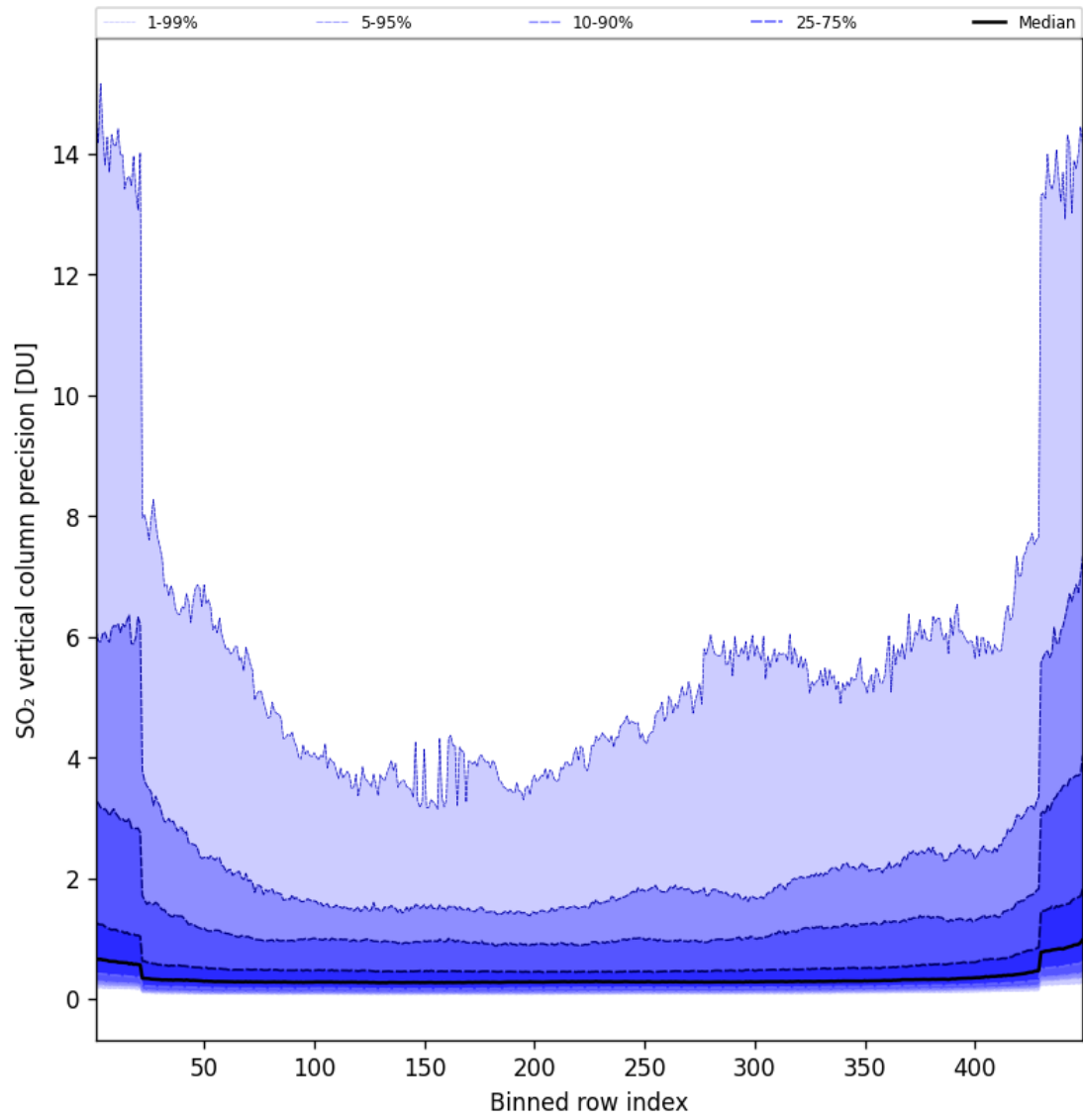
Figure 86: Along track statistics of “SO 2 vertical column precision” for 2025-01-21 to 2025-01-21
