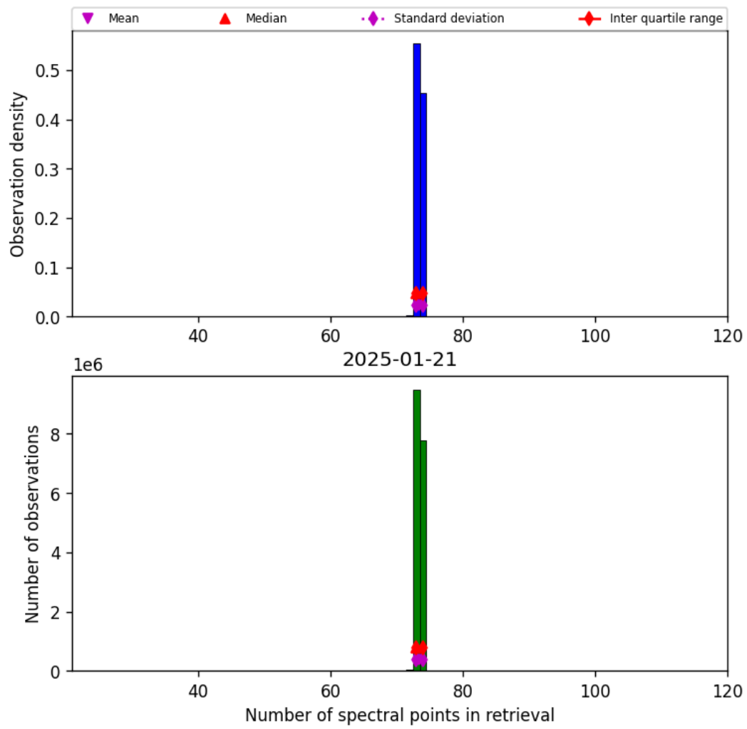
Figure 83: Histogram of “Number of spectral points in retrieval” for 2025-01-21 to 2025-01-21
