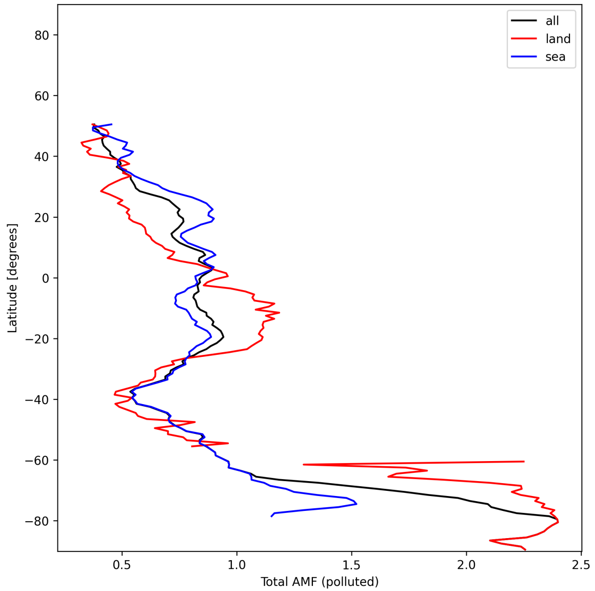
Figure 53: Zonal average of “Total AMF (polluted)” for 2025-01-21 to 2025-01-21.
