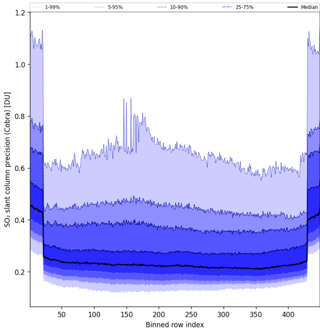
Figure 89: Along track statistics of “SO 2 slant column precision (Cobra)” for 2025-01-21 to 2025-01-21
