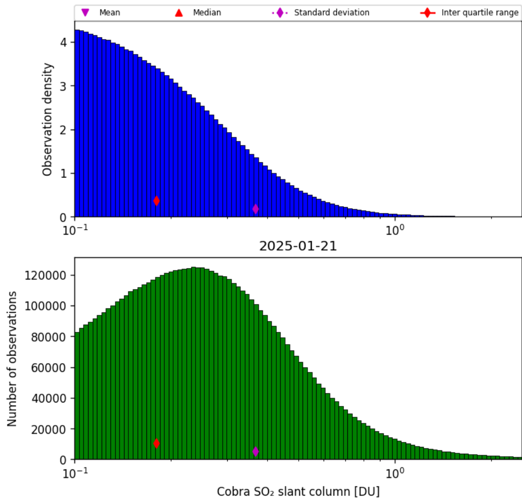
Figure 61: Histogram of “Cobra SO 2 slant column” for 2025-01-21 to 2025-01-21
