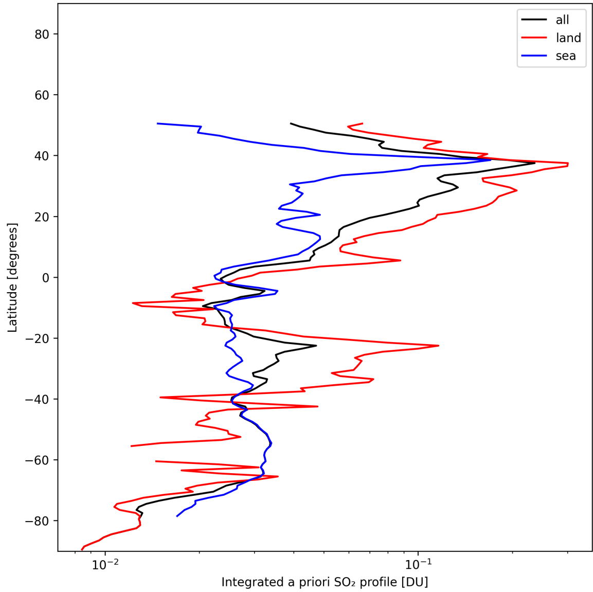
Figure 49: Zonal average of “Integrated a priori SO 2 profile” for 2025-01-21 to 2025-01-21.
