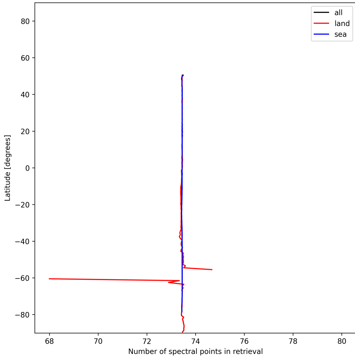
Figure 56: Zonal average of “Number of spectral points in retrieval” for 2025-01-21 to 2025-01-21.
