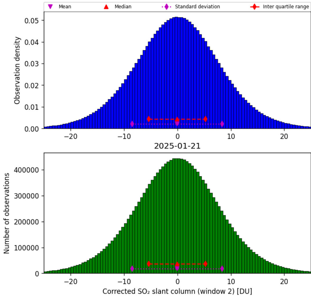
Figure 69: Histogram of “Corrected SO 2 slant column (window 2)” for 2025-01-21 to 2025-01-21
