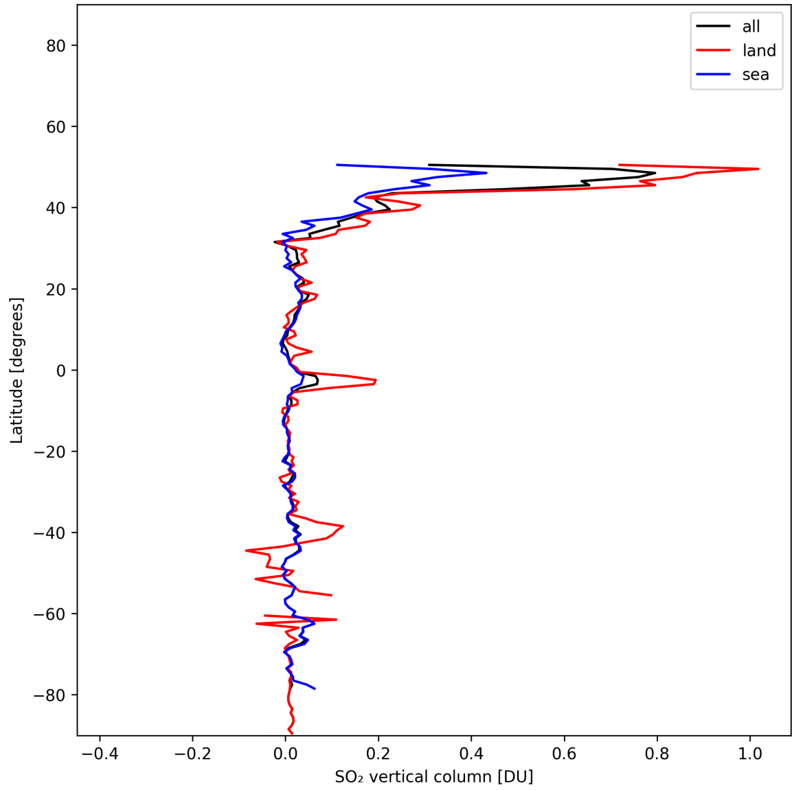
Figure 31: Zonal average of “SO 2 vertical column” for 2025-01-21 to 2025-01-21.
