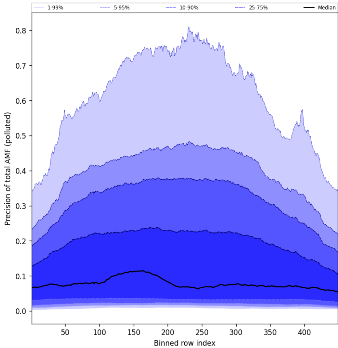
Figure 108: Along track statistics of “Precision of total AMF (polluted)” for 2025-01-21 to 2025-01-21
