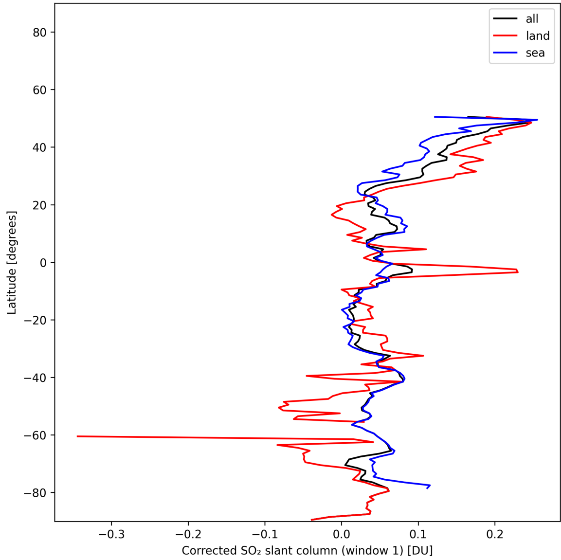
Figure 38: Zonal average of “Corrected SO 2 slant column (window 1)” for 2025-01-21 to 2025-01-21.
