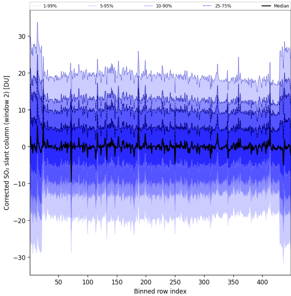
Figure 96: Along track statistics of “Corrected SO 2 slant column (window 2)” for 2025-01-21 to 2025-01-21
