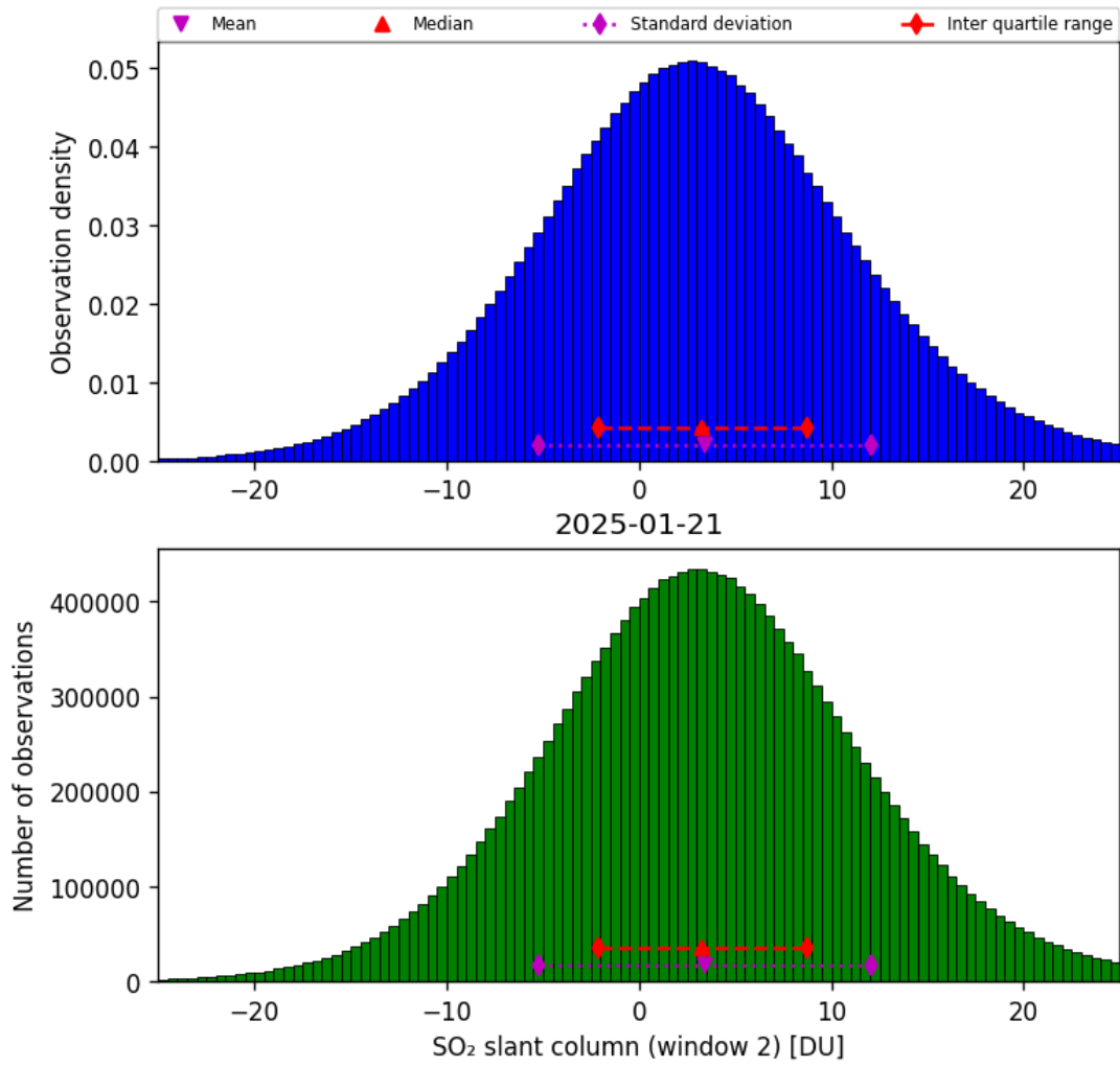
Figure 67: Histogram of “SO 2 slant column (window 2)” for 2025-01-21 to 2025-01-21
