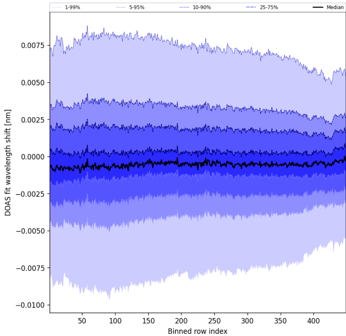
Figure 104: Along track statistics of “DOAS fit wavelength shift” for 2025-01-21 to 2025-01-21
