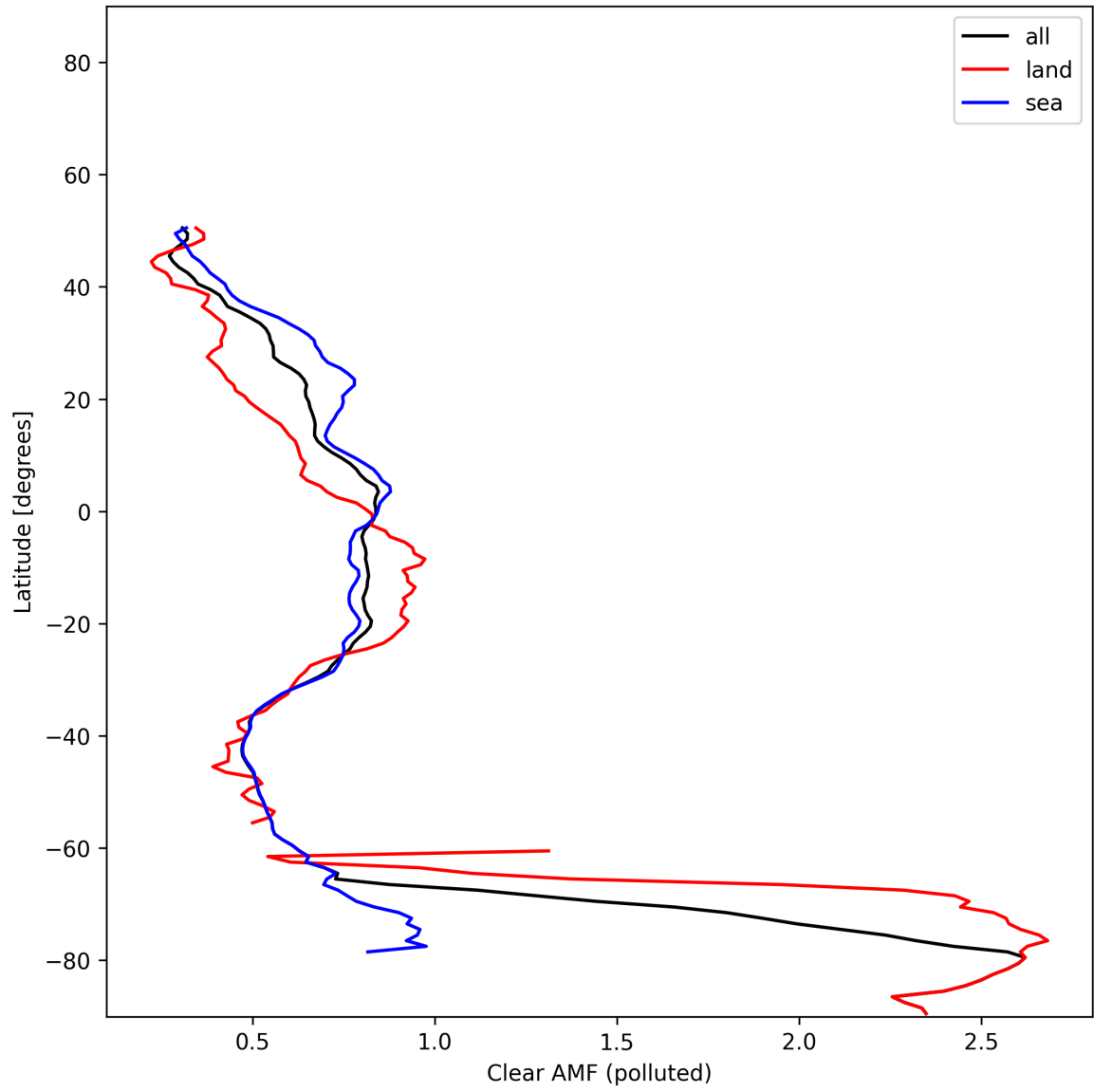
Figure 55: Zonal average of “Clear AMF (polluted)” for 2025-01-21 to 2025-01-21.
