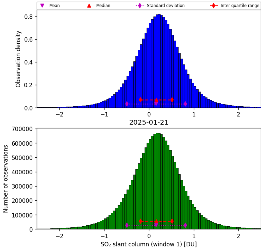
Figure 63: Histogram of “SO 2 slant column (window 1)” for 2025-01-21 to 2025-01-21
