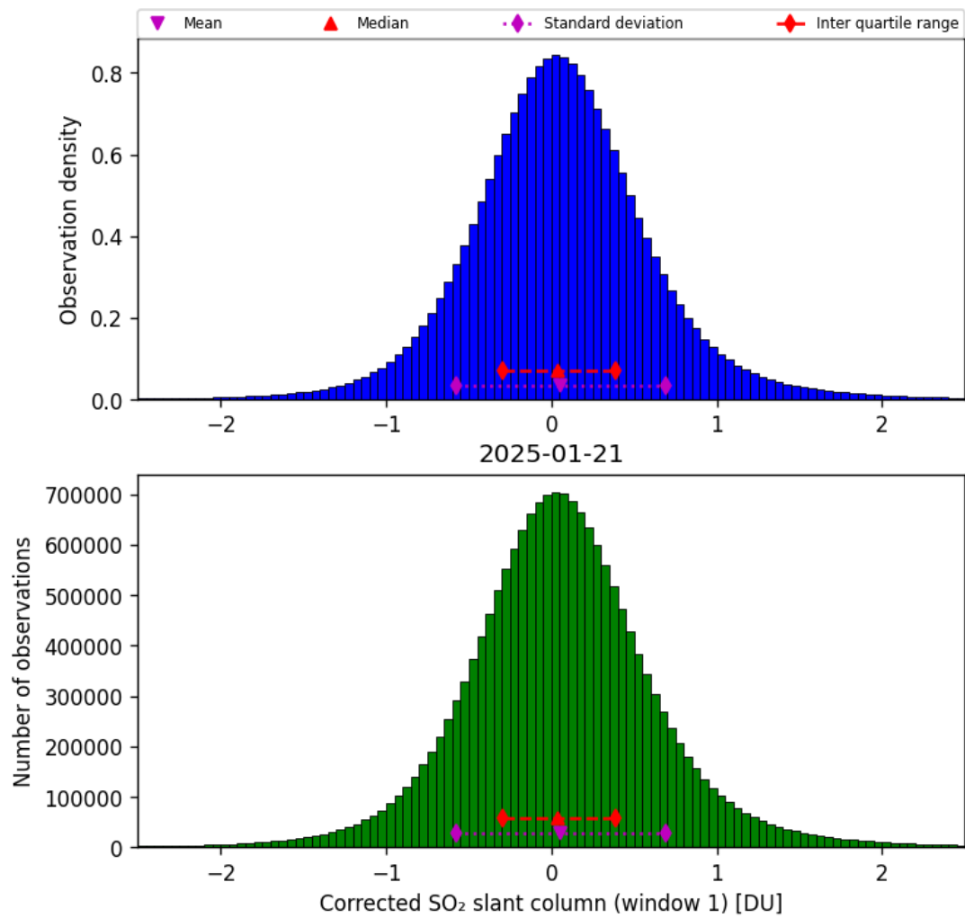
Figure 65: Histogram of “Corrected SO 2 slant column (window 1)” for 2025-01-21 to 2025-01-21
