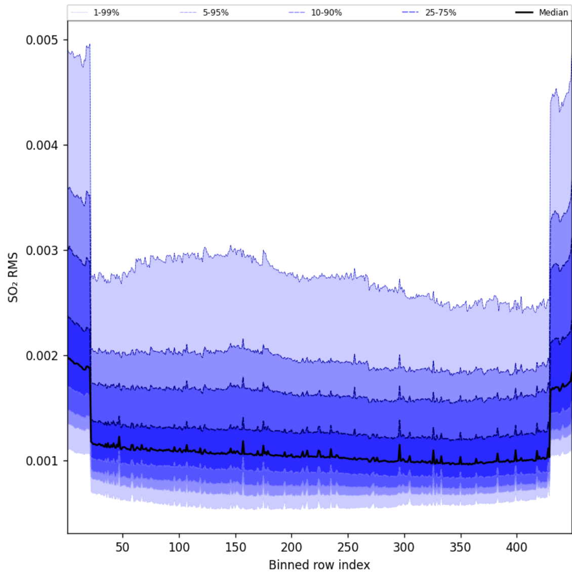
Figure 106: Along track statistics of “SO 2 RMS” for 2025-01-21 to 2025-01-21
