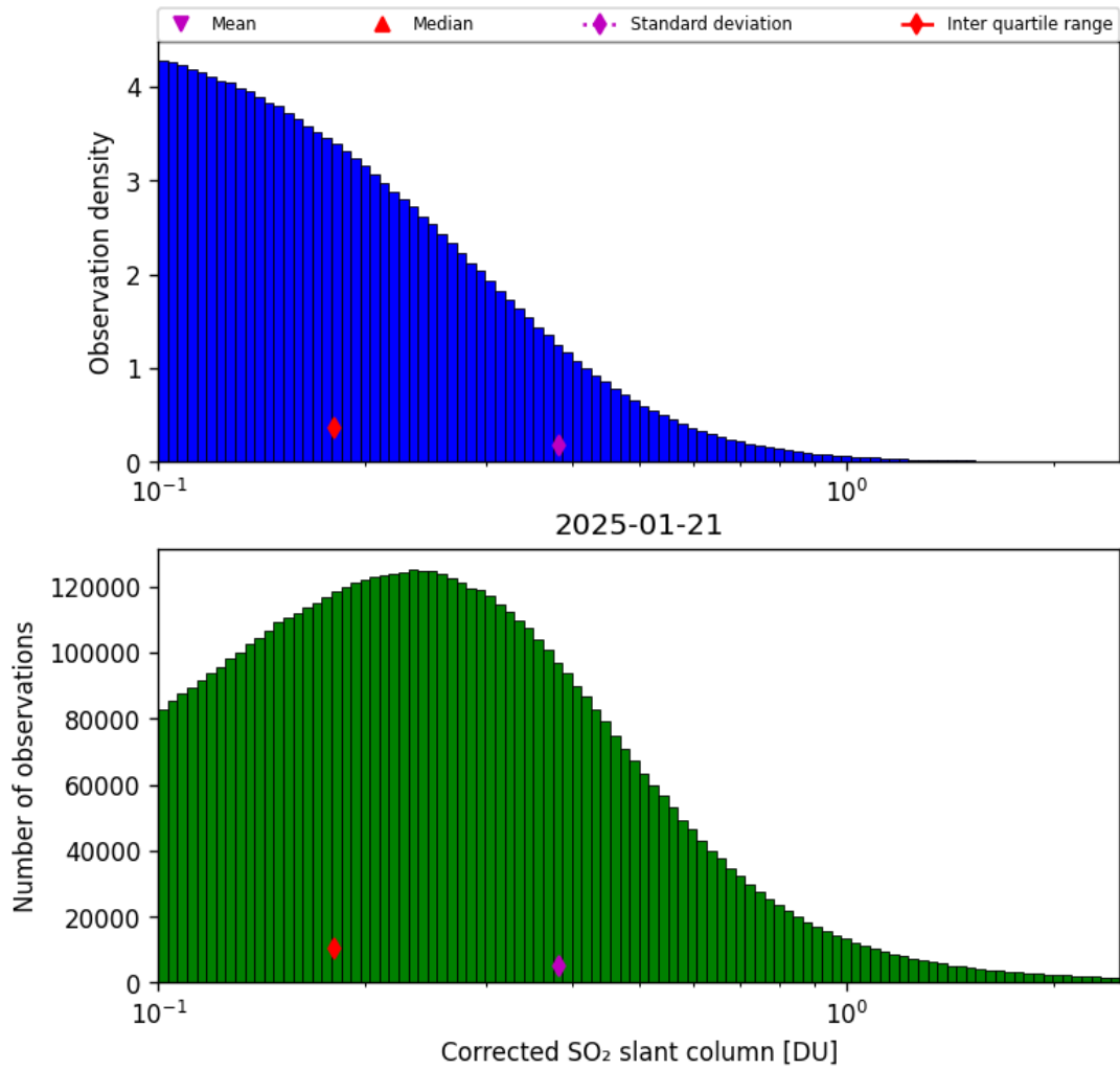
Figure 60: Histogram of “Corrected SO 2 slant column” for 2025-01-21 to 2025-01-21
