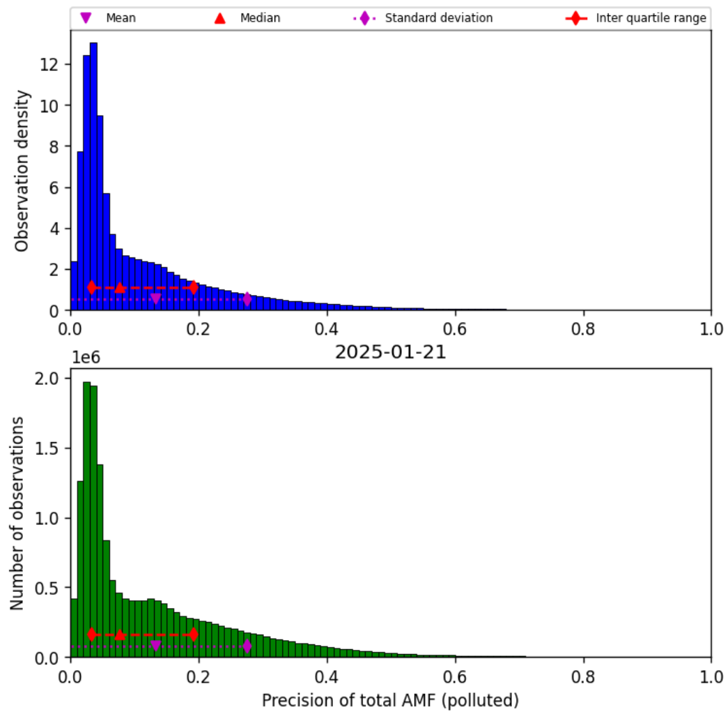
Figure 81: Histogram of “Precision of total AMF (polluted)” for 2025-01-21 to 2025-01-21
