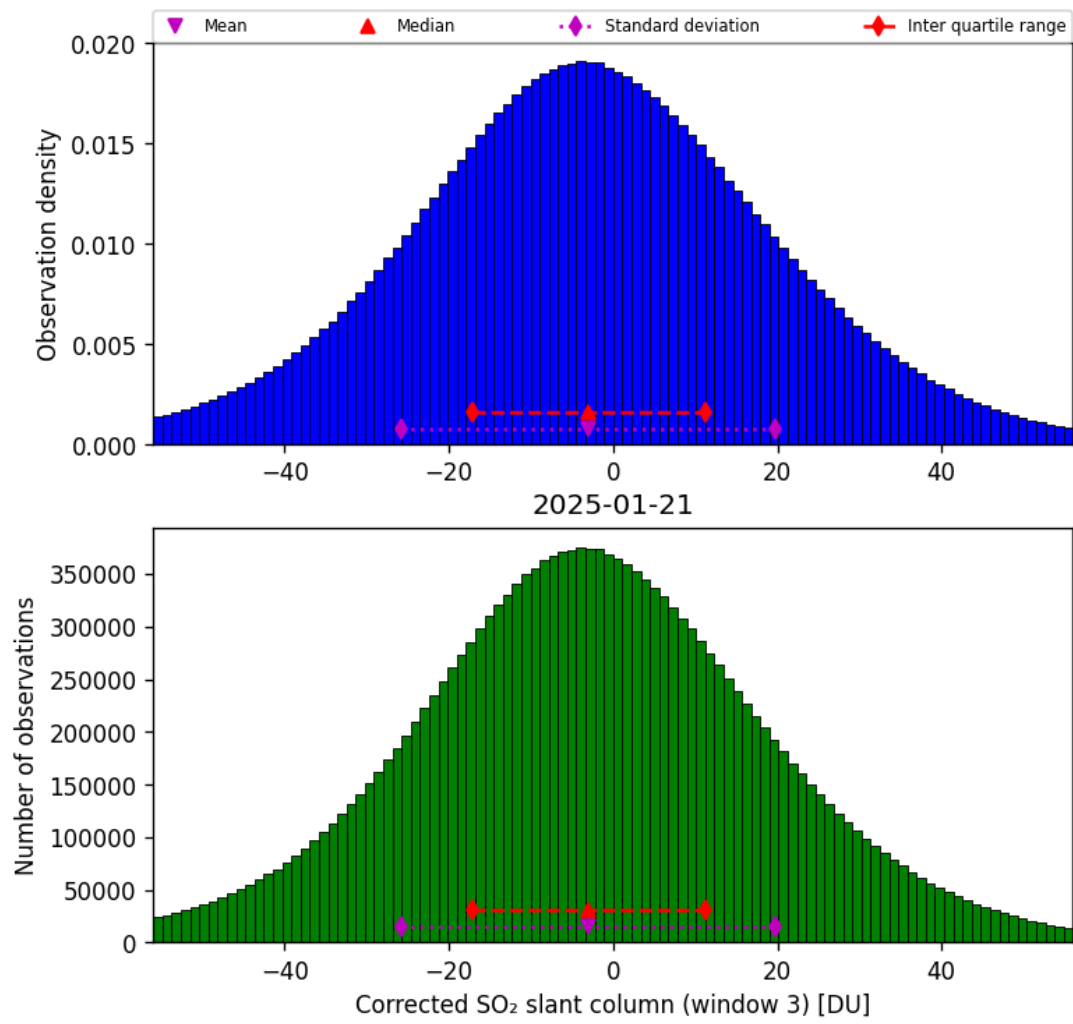
Figure 73: Histogram of “Corrected SO 2 slant column (window 3)” for 2025-01-21 to 2025-01-21
