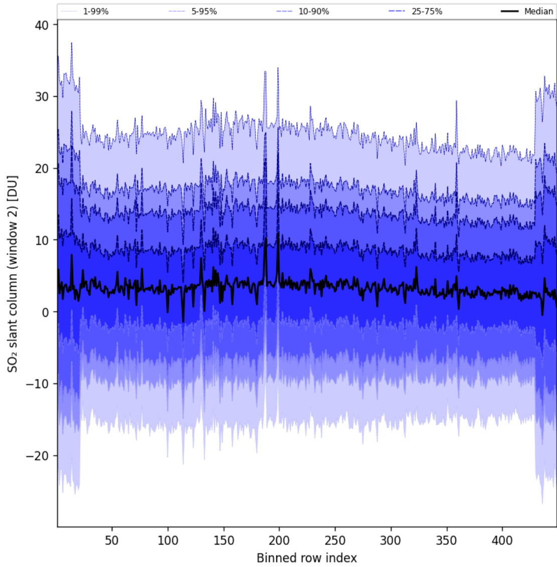
Figure 94: Along track statistics of “SO 2 slant column (window 2)” for 2025-01-21 to 2025-01-21
