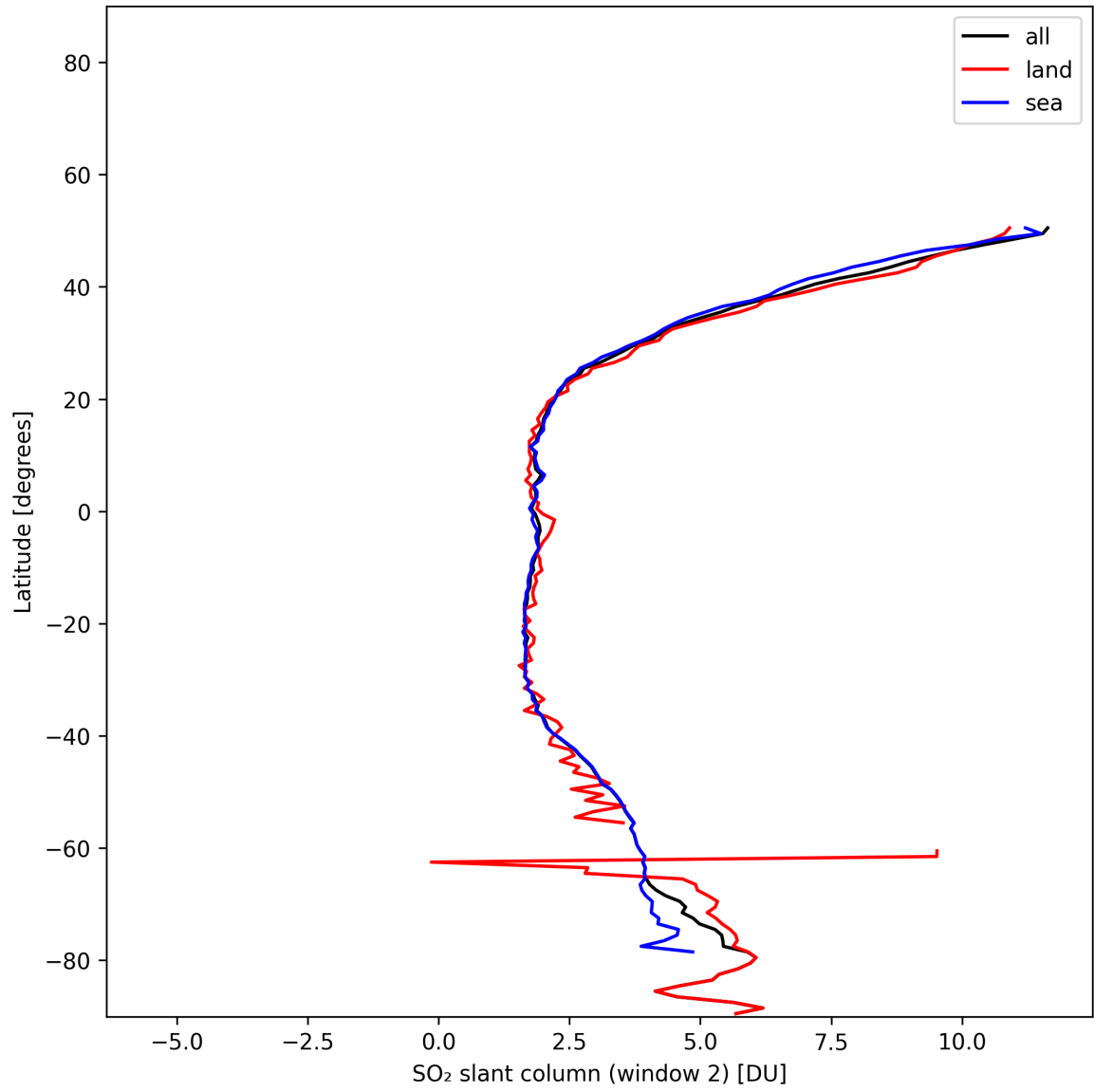
Figure 40: Zonal average of “SO 2 slant column (window 2)” for 2025-01-21 to 2025-01-21.
