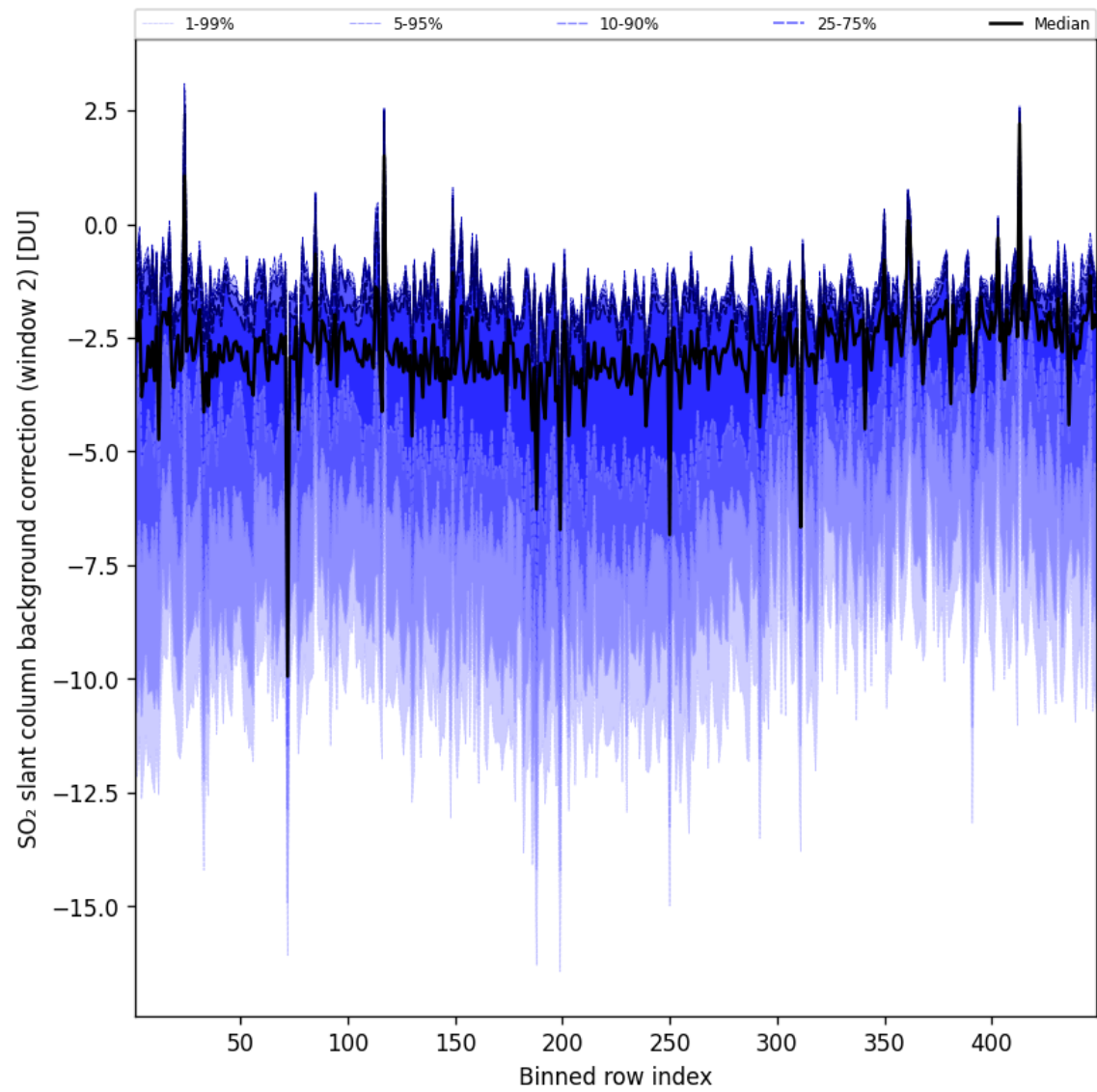
Figure 97: Along track statistics of “SO 2 slant column background correction (window 2)” for 2025-01-21 to 2025-01-21
