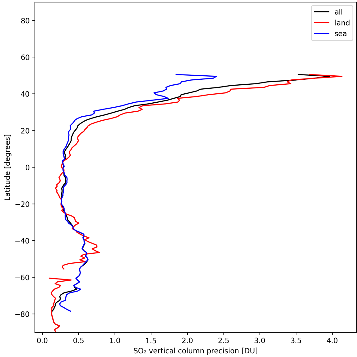
Figure 32: Zonal average of “SO 2 vertical column precision” for 2025-01-21 to 2025-01-21.
