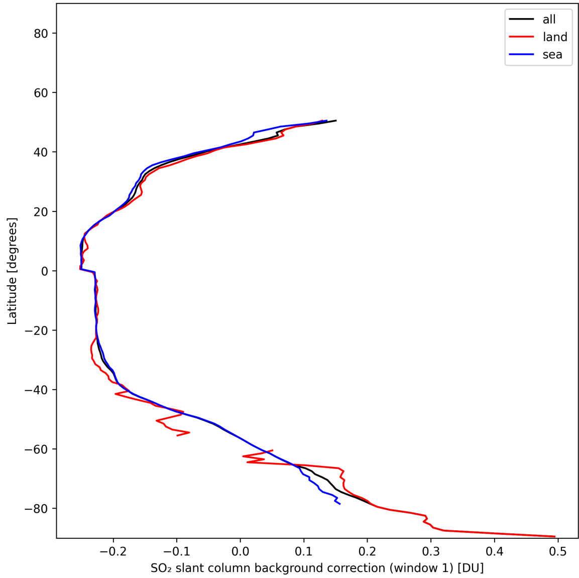
Figure 39: Zonal average of "SO 2 slant column background correction (window 1)" for 2025-01-21 to 2025-01-21.
