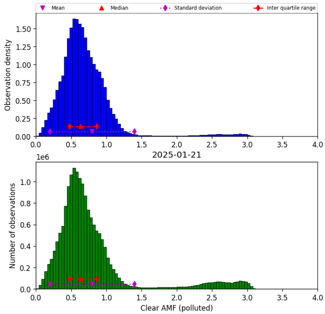
Figure 82: Histogram of “Clear AMF (polluted)” for 2025-01-21 to 2025-01-21
