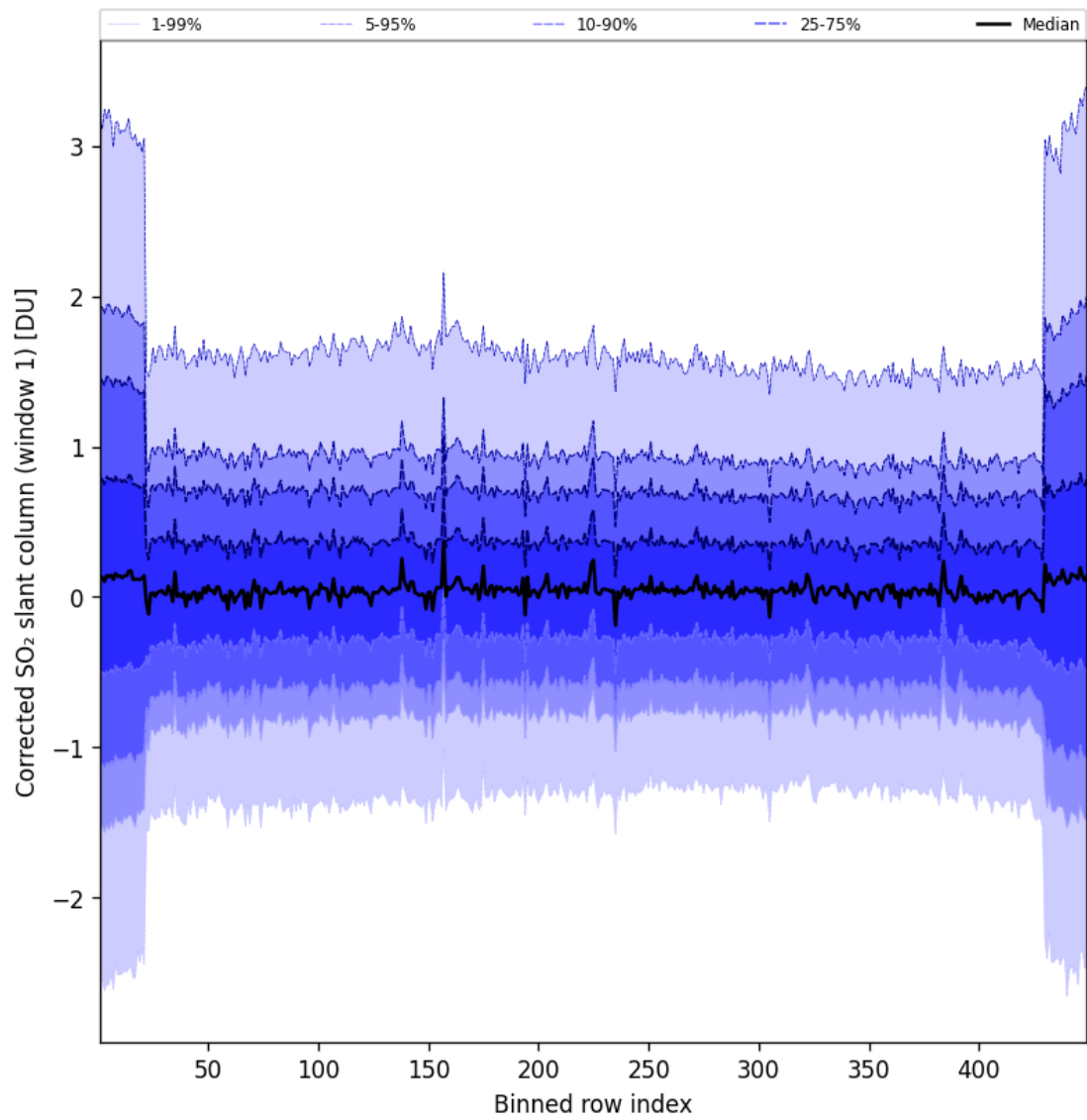
Figure 92: Along track statistics of “Corrected SO 2 slant column (window 1)” for 2025-01-21 to 2025-01-21
