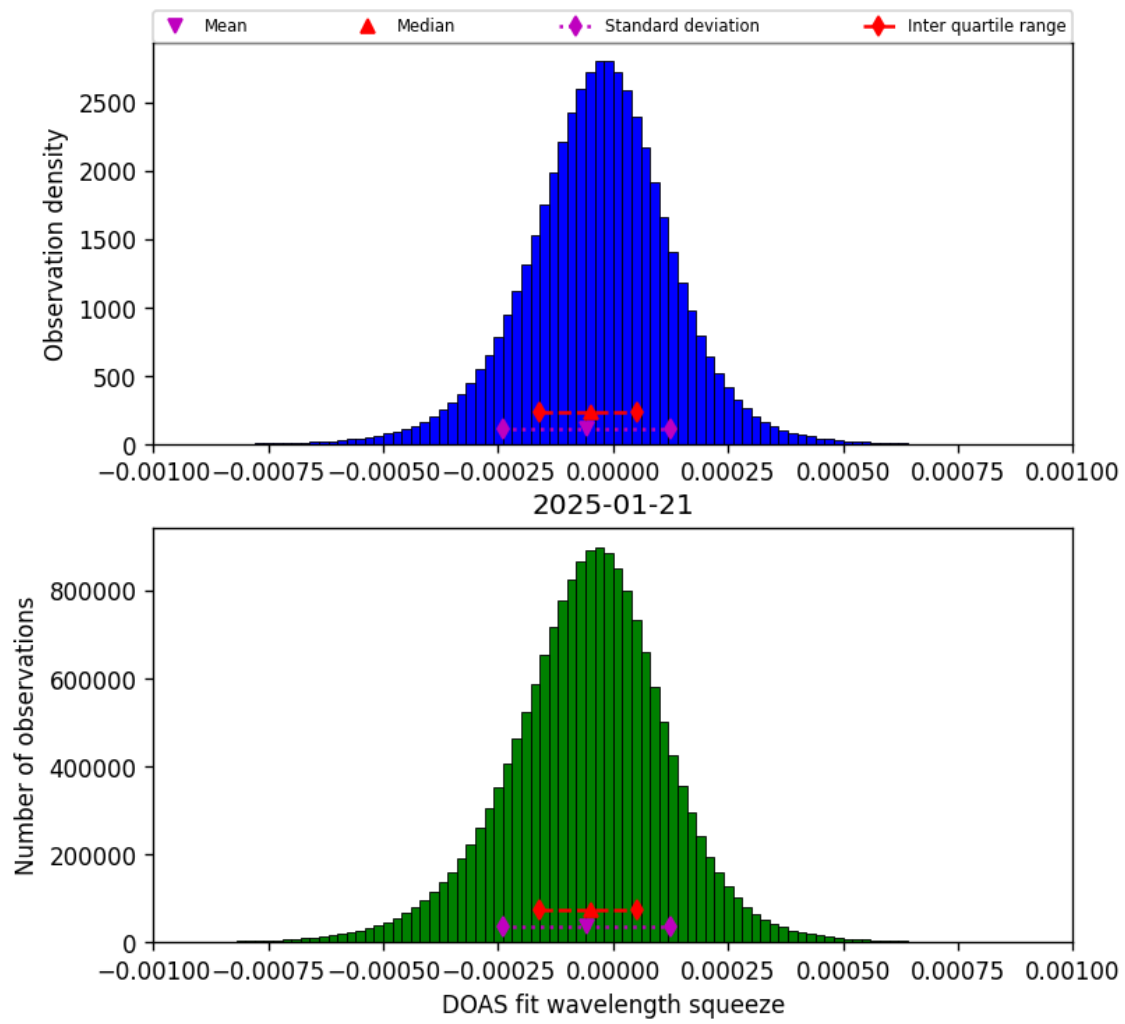
Figure 78: Histogram of “DOAS fit wavelength squeeze” for 2025-01-21 to 2025-01-21
