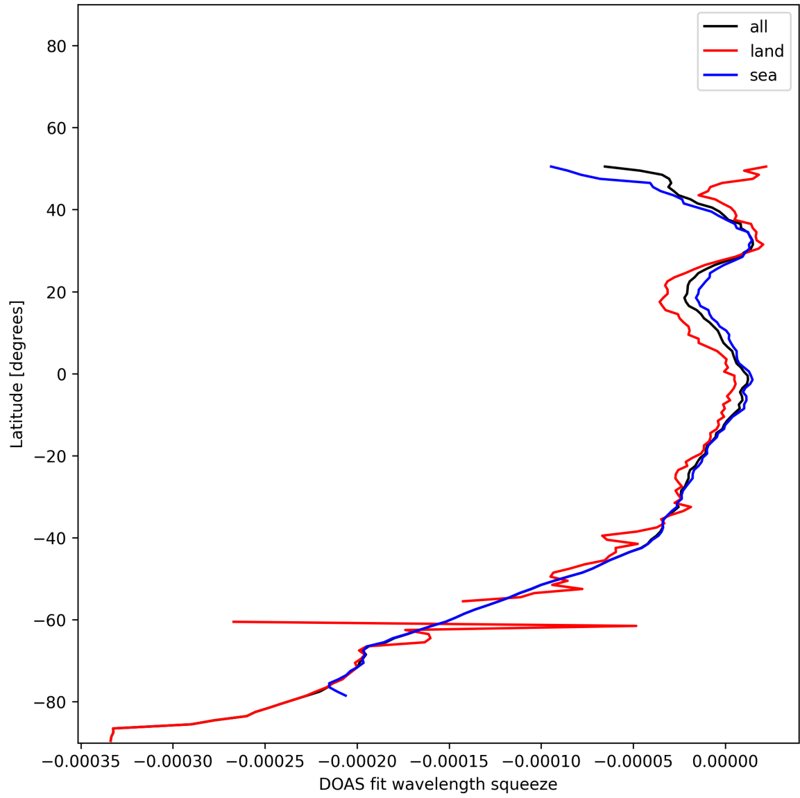
Figure 51: Zonal average of “DOAS fit wavelength squeeze” for 2025-01-21 to 2025-01-21.
