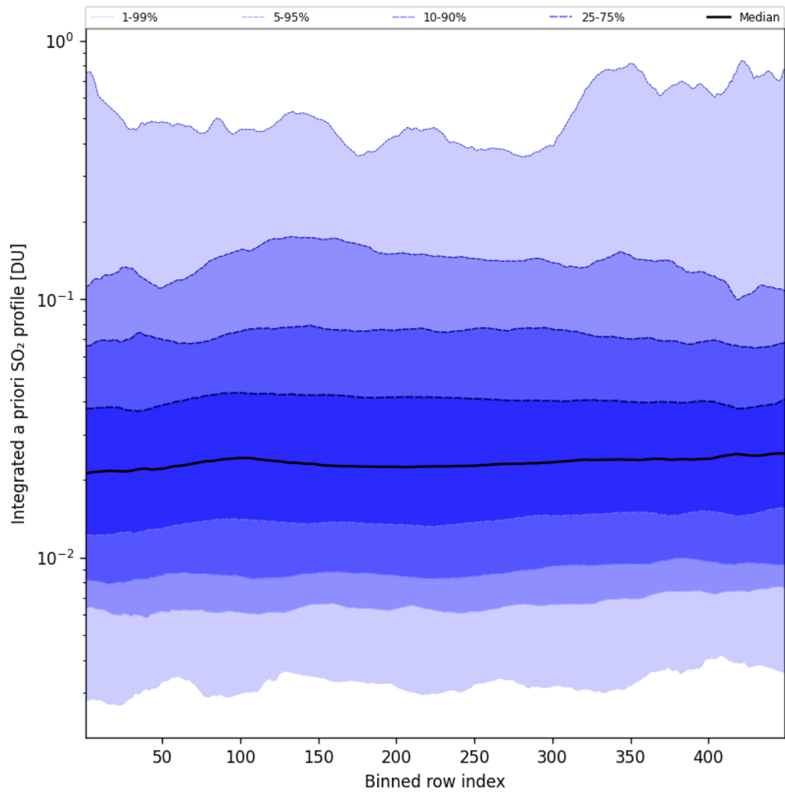
Figure 103: Along track statistics of “Integrated a priori SO 2 profile” for 2025-01-21 to 2025-01-21
