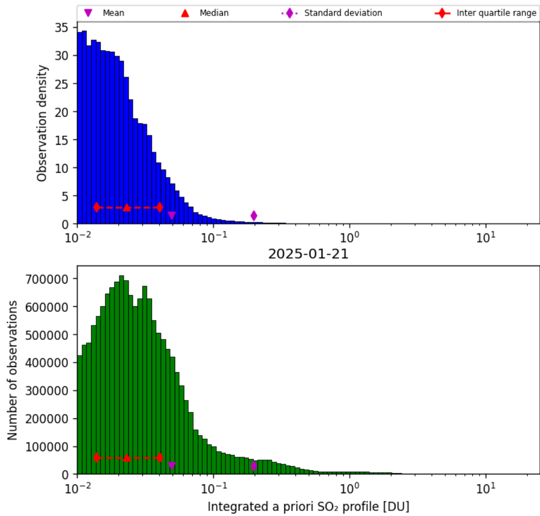
Figure 76: Histogram of “Integrated a priori SO 2 profile” for 2025-01-21 to 2025-01-21
