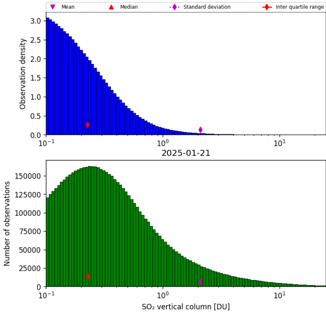
Figure 58: Histogram of “SO 2 vertical column” for 2025-01-21 to 2025-01-21
