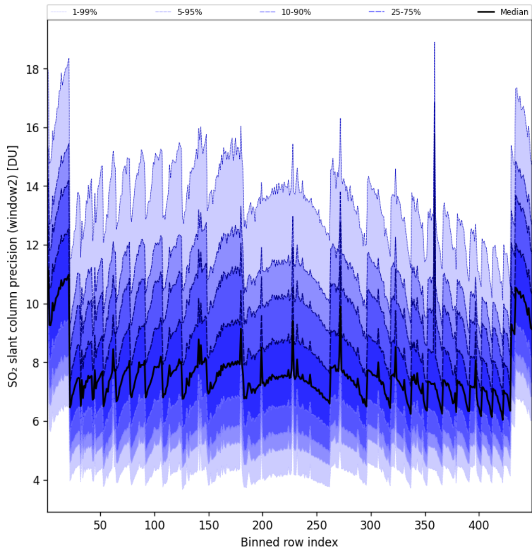
Figure 95: Along track statistics of “SO 2 slant column precision (window2)” for 2025-01-21 to 2025-01-21
