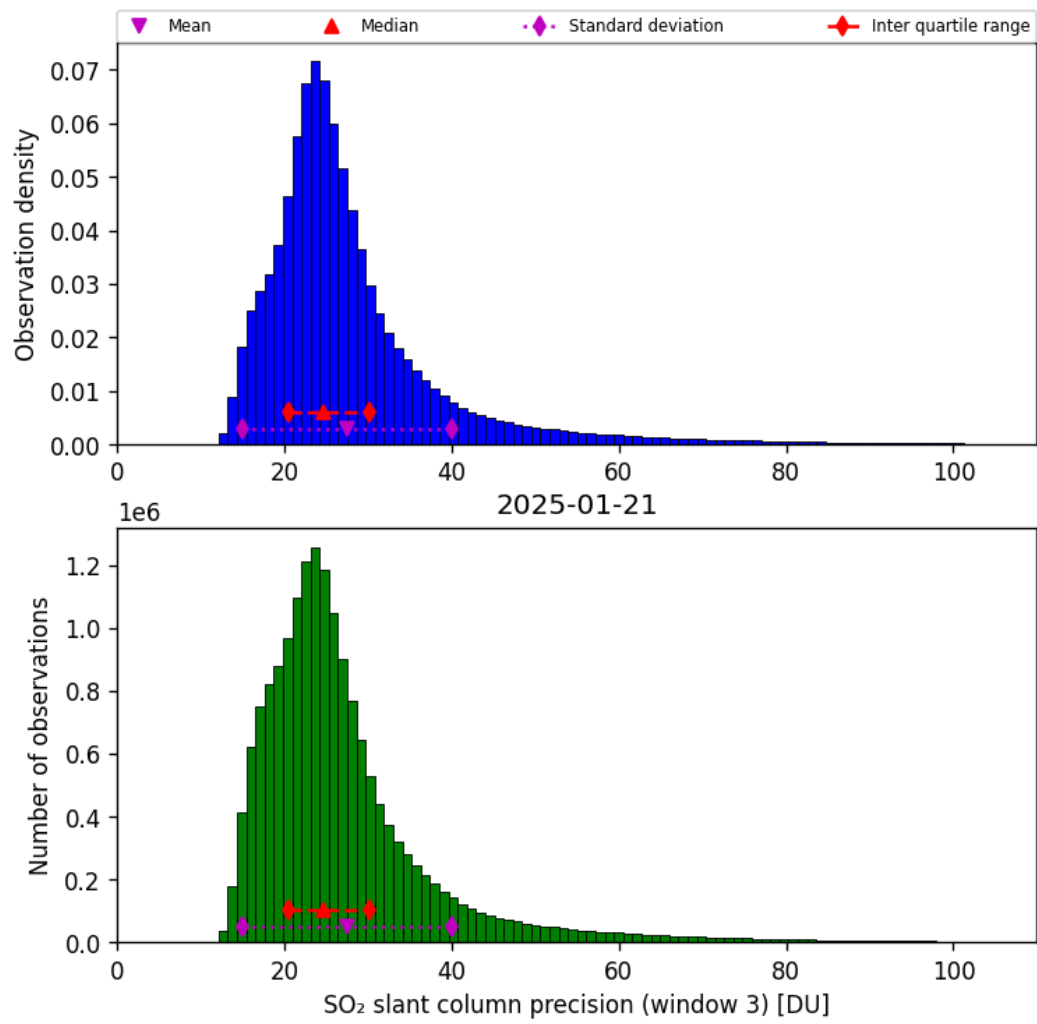
Figure 72: Histogram of “SO 2 slant column precision (window 3)” for 2025-01-21 to 2025-01-21
