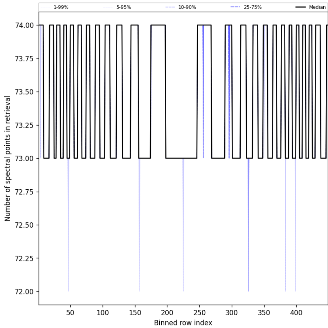
Figure 110: Along track statistics of “Number of spectral points in retrieval” for 2025-01-21 to 2025-01-21
