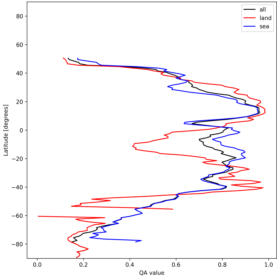
Figure 30: Zonal average of “QA value” for 2025-01-21 to 2025-01-21.
