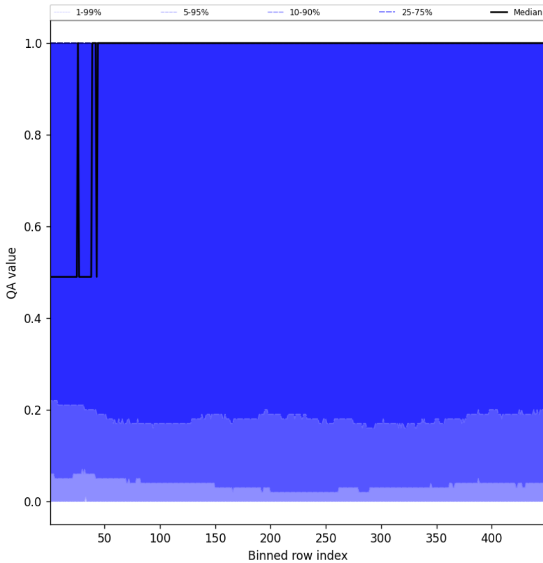
Figure 84: Along track statistics of “QA value” for 2025-01-21 to 2025-01-21
