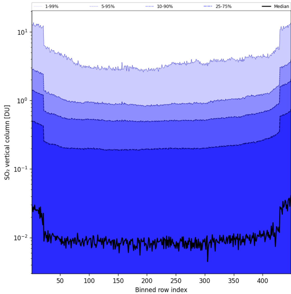
Figure 85: Along track statistics of “SO 2 vertical column” for 2025-01-21 to 2025-01-21
