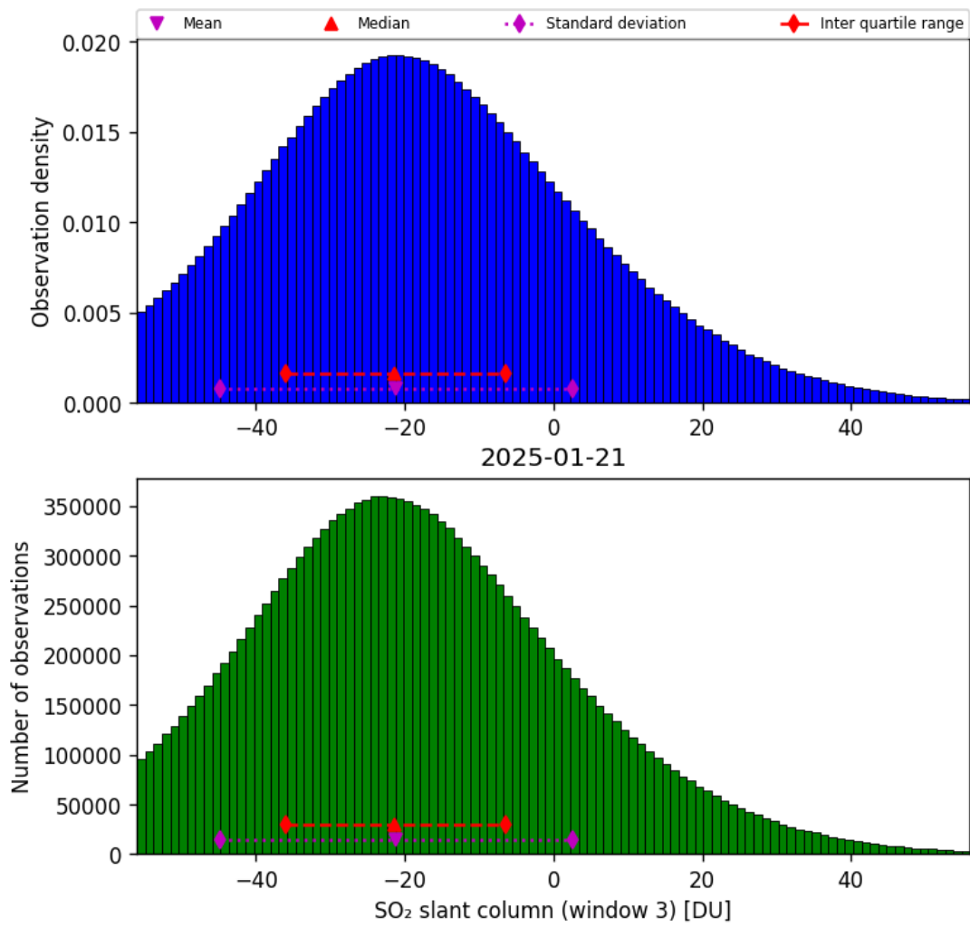
Figure 71: Histogram of “SO 2 slant column (window 3)” for 2025-01-21 to 2025-01-21
