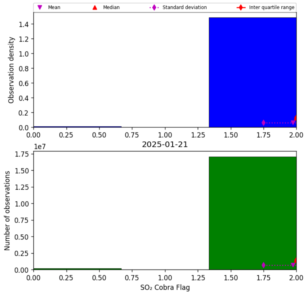
Figure 75: Histogram of “SO 2 Cobra Flag” for 2025-01-21 to 2025-01-21
