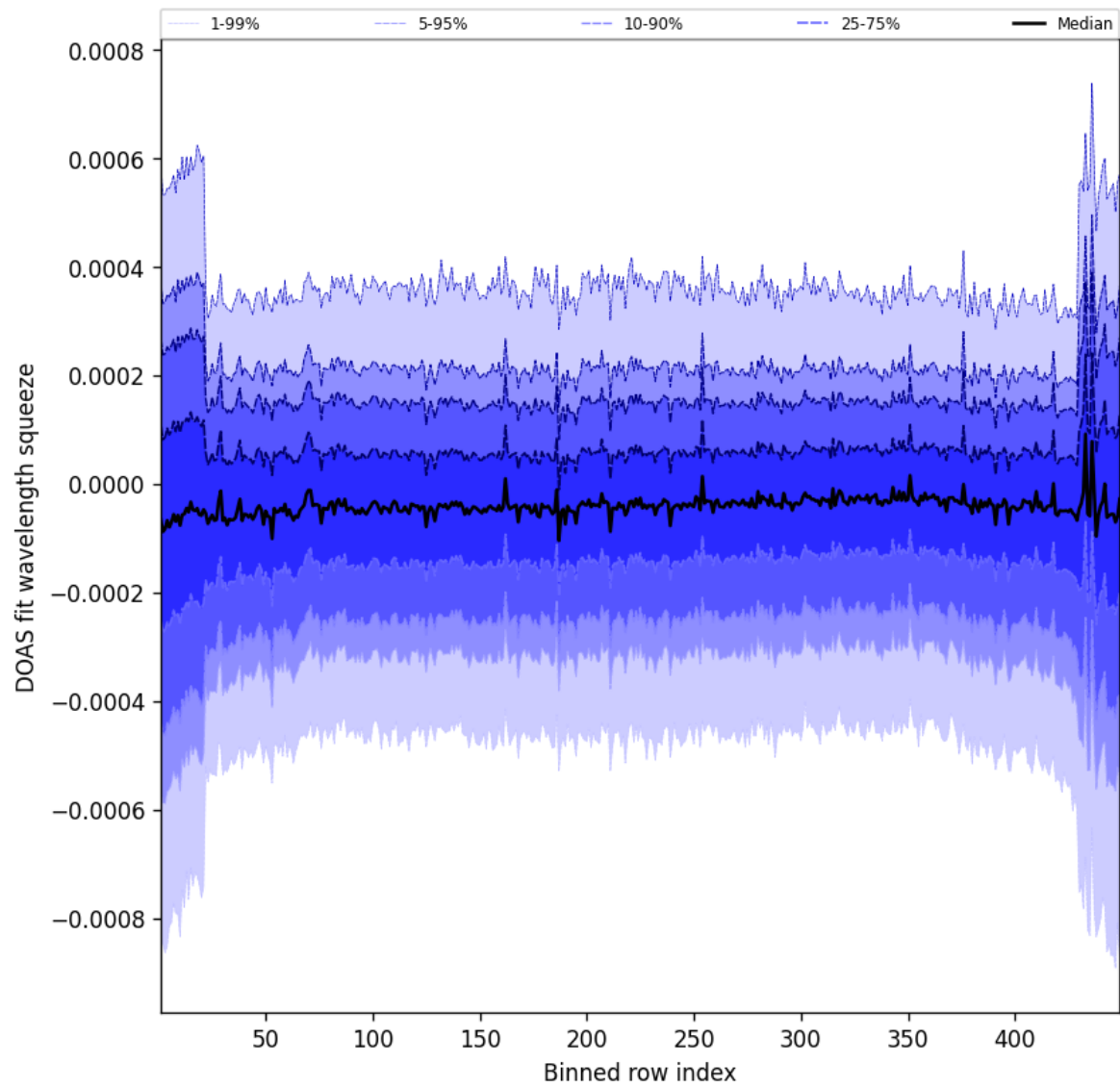
Figure 105: Along track statistics of “DOAS fit wavelength squeeze” for 2025-01-25 to 2025-01-26
