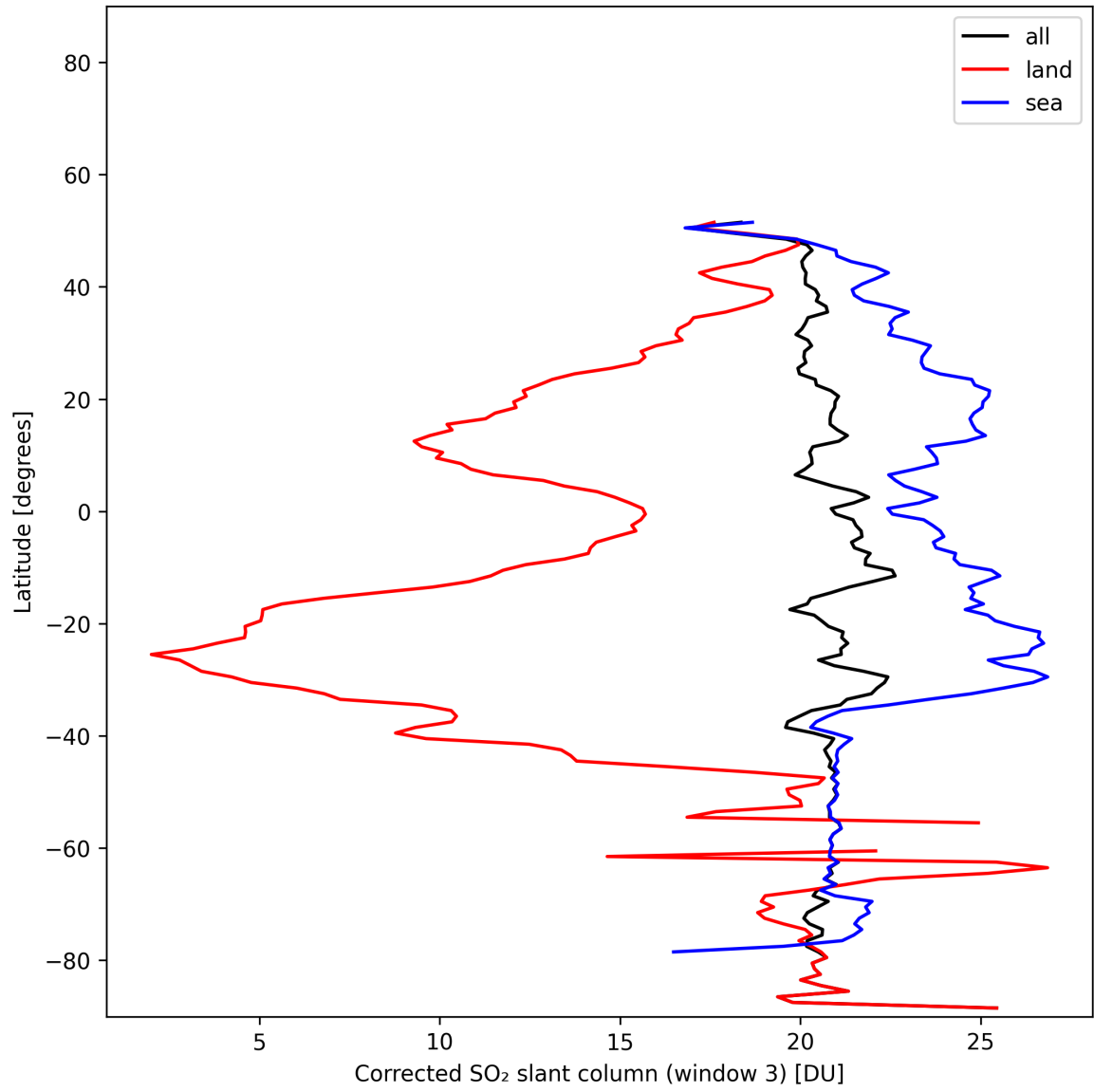
Figure 46: Zonal average of “Corrected SO 2 slant column (window 3)” for 2025-01-25 to 2025-01-26.
