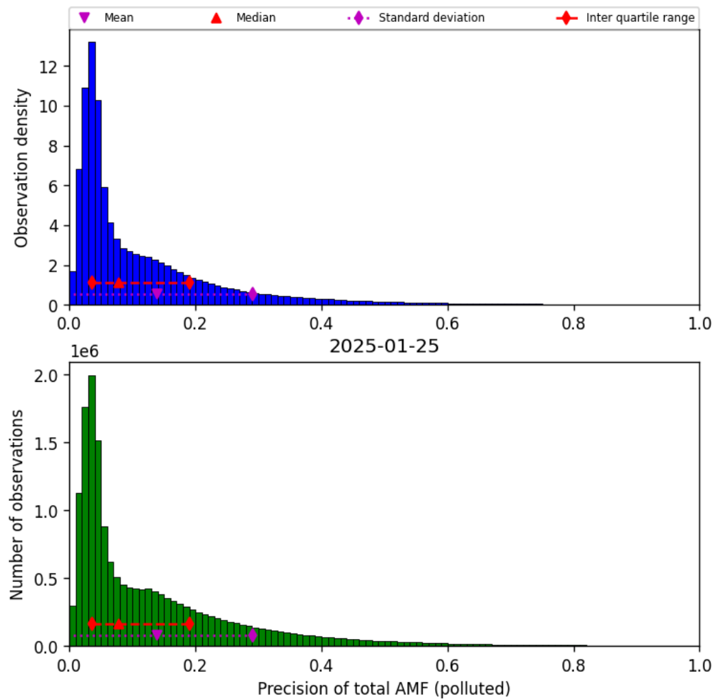
Figure 81: Histogram of “Precision of total AMF (polluted)” for 2025-01-25 to 2025-01-26
