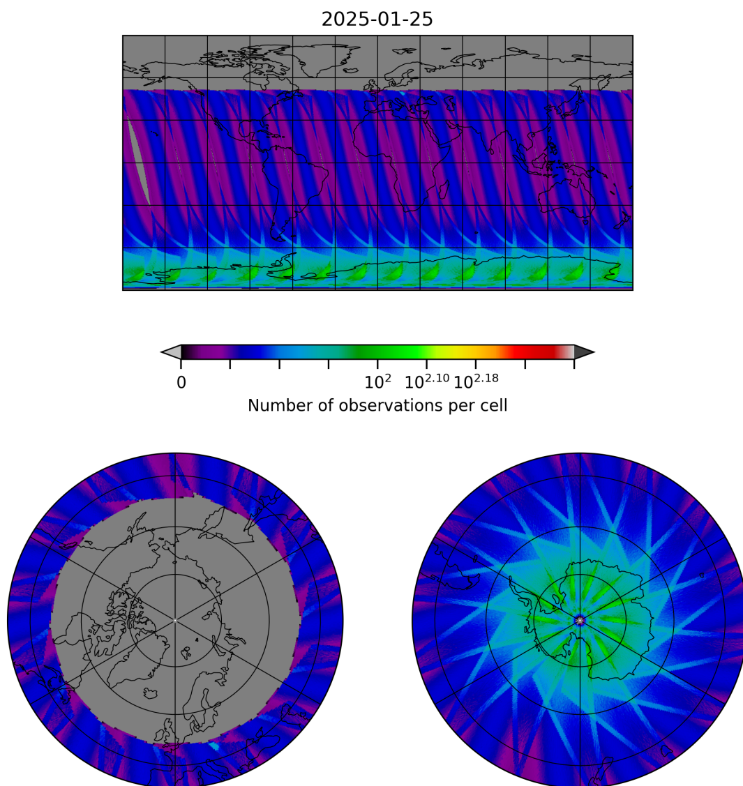
Figure 29: Map of the number of observations for 2025-01-25 to 2025-01-26
