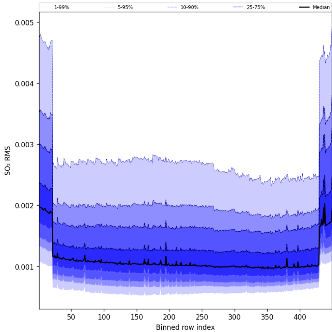
Figure 106: Along track statistics of “SO 2 RMS” for 2025-01-25 to 2025-01-26
