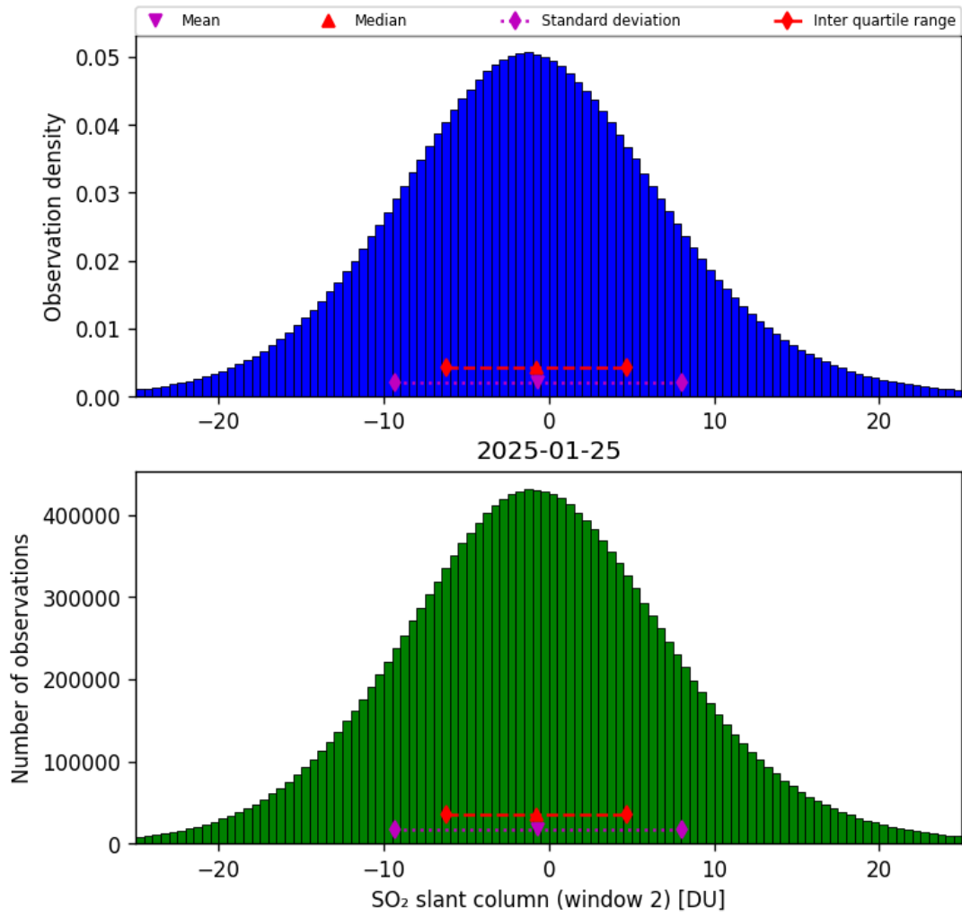
Figure 67: Histogram of “SO 2 slant column (window 2)” for 2025-01-25 to 2025-01-26
