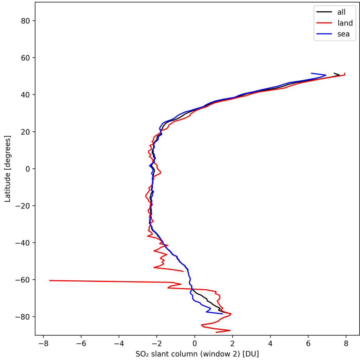
Figure 40: Zonal average of “SO 2 slant column (window 2)” for 2025-01-25 to 2025-01-26.
