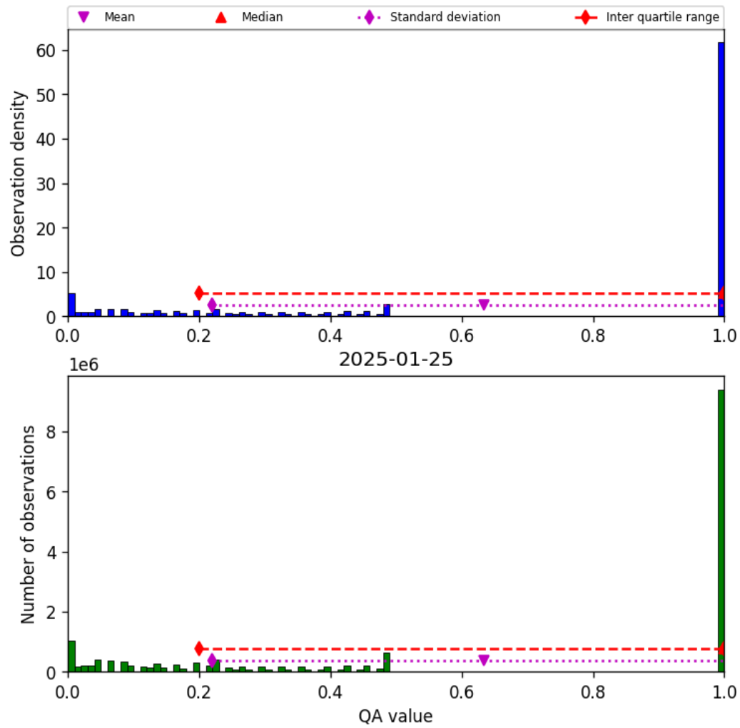
Figure 57: Histogram of “QA value” for 2025-01-25 to 2025-01-26
