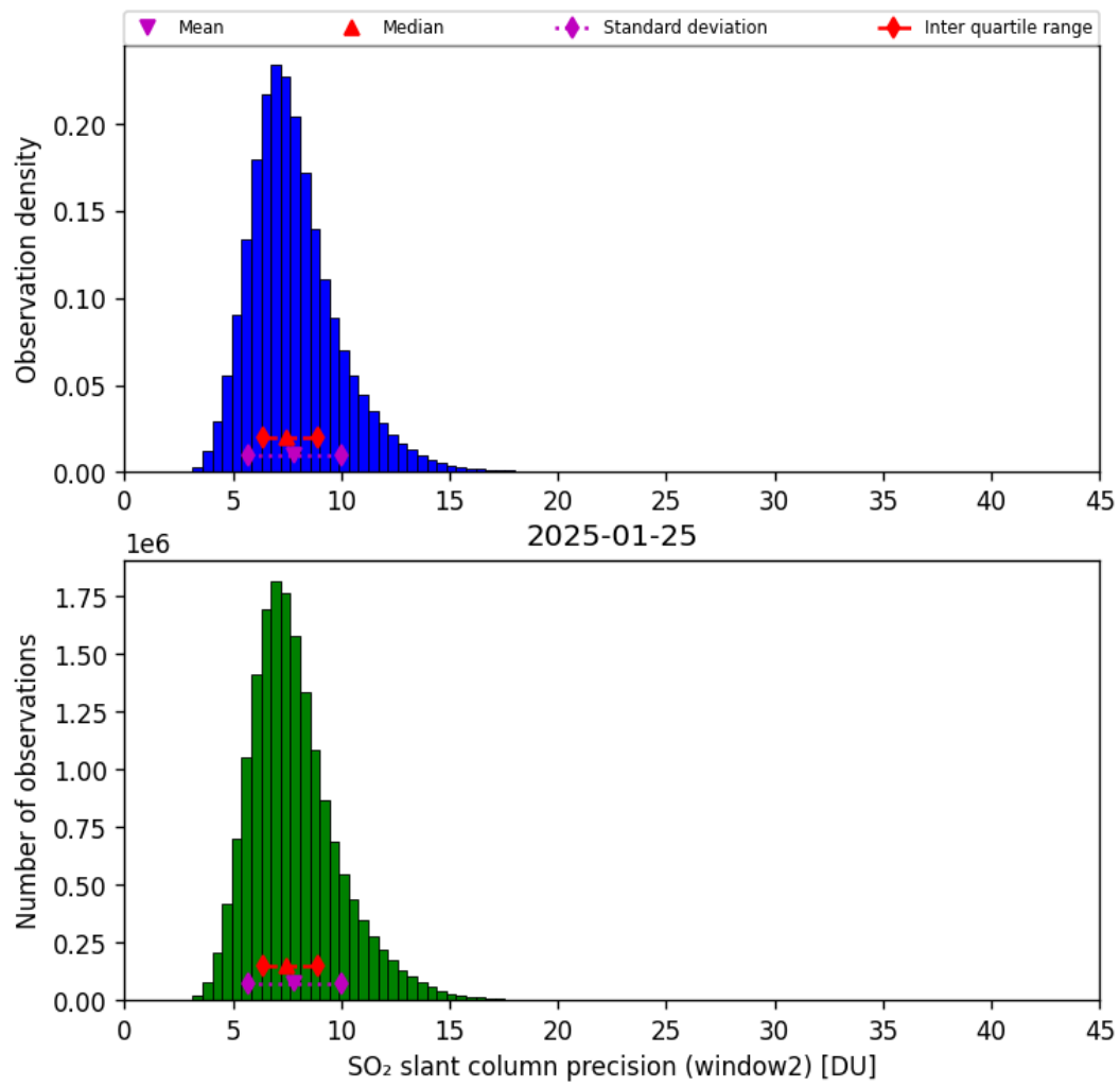
Figure 68: Histogram of “SO 2 slant column precision (window2)” for 2025-01-25 to 2025-01-26
