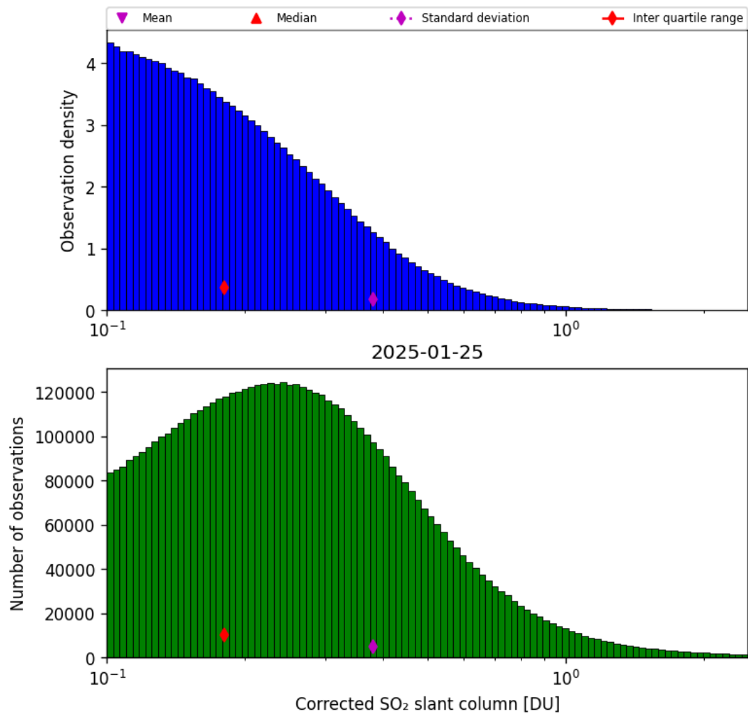
Figure 60: Histogram of “Corrected SO 2 slant column” for 2025-01-25 to 2025-01-26
