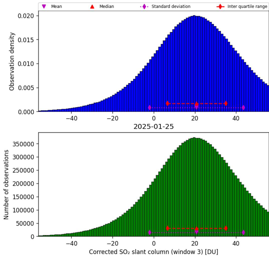
Figure 73: Histogram of “Corrected SO 2 slant column (window 3)” for 2025-01-25 to 2025-01-26
