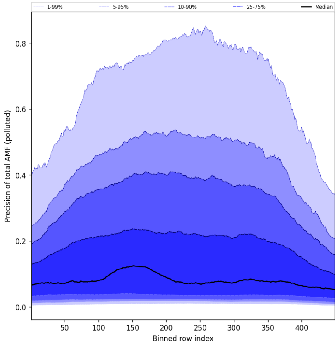
Figure 108: Along track statistics of “Precision of total AMF (polluted)” for 2025-01-25 to 2025-01-26
