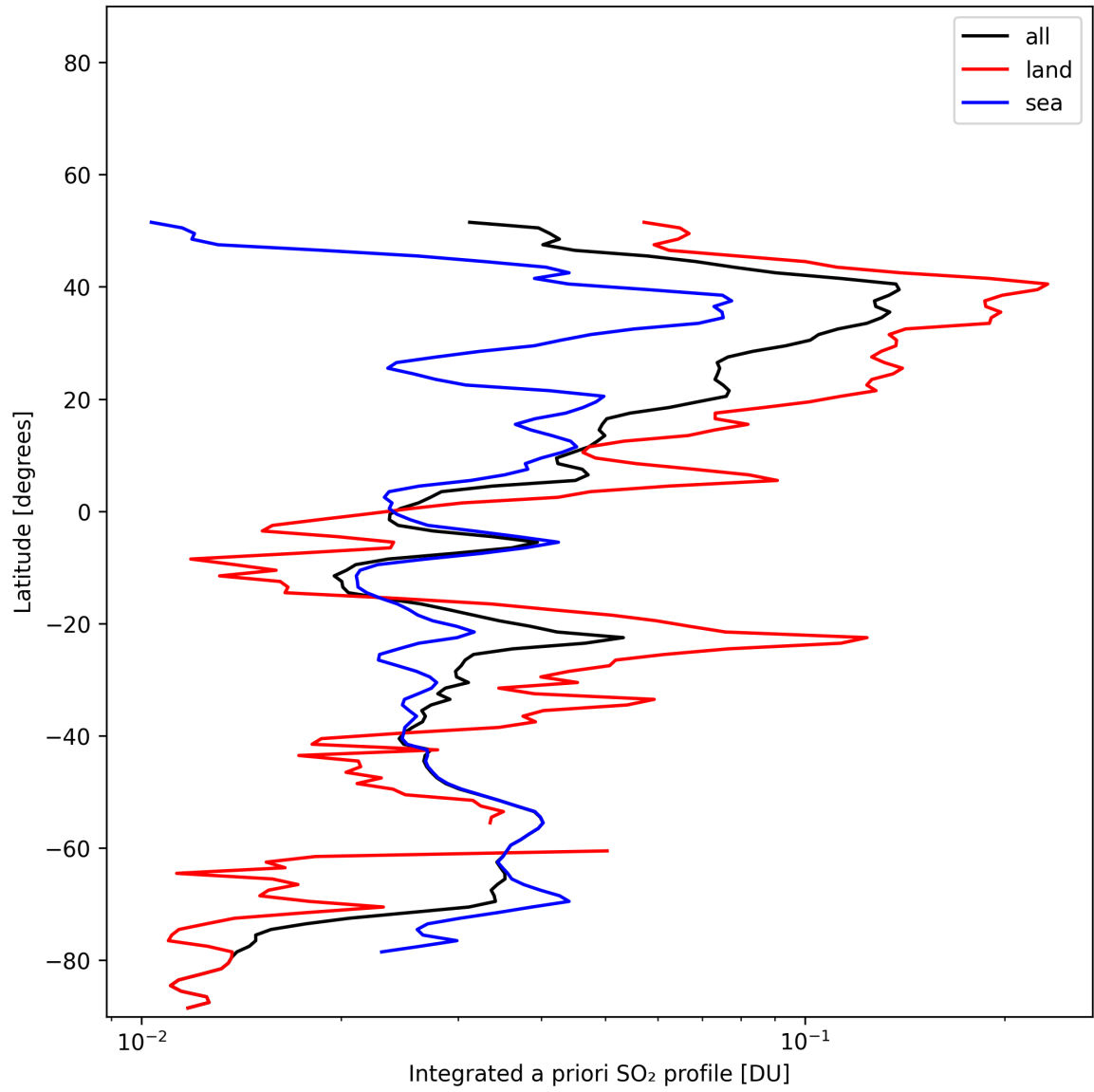
Figure 49: Zonal average of “Integrated a priori SO 2 profile” for 2025-01-25 to 2025-01-26.
