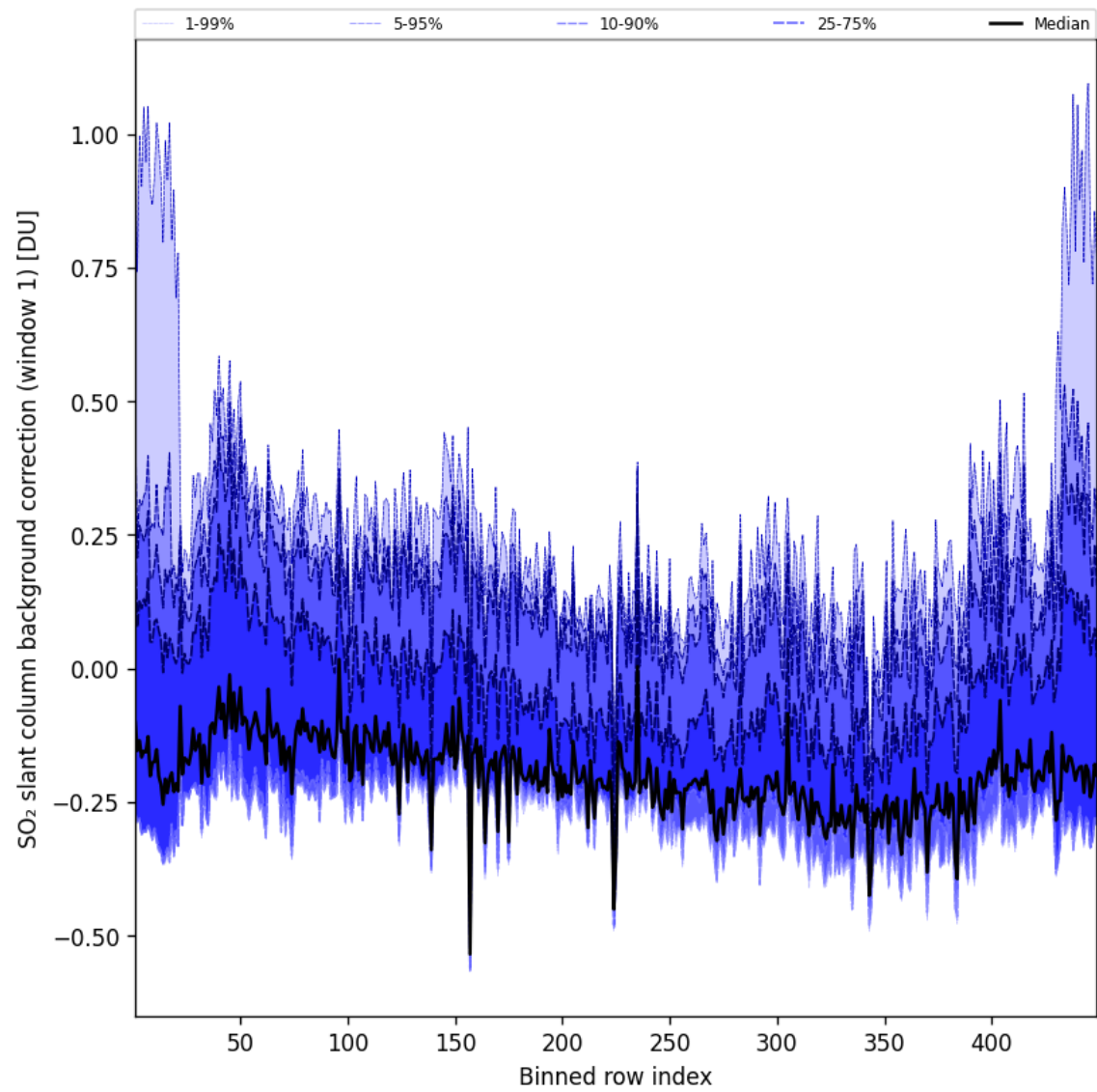
Figure 93: Along track statistics of “SO 2 slant column background correction (window 1)” for 2025-01-25 to 2025-01-26
