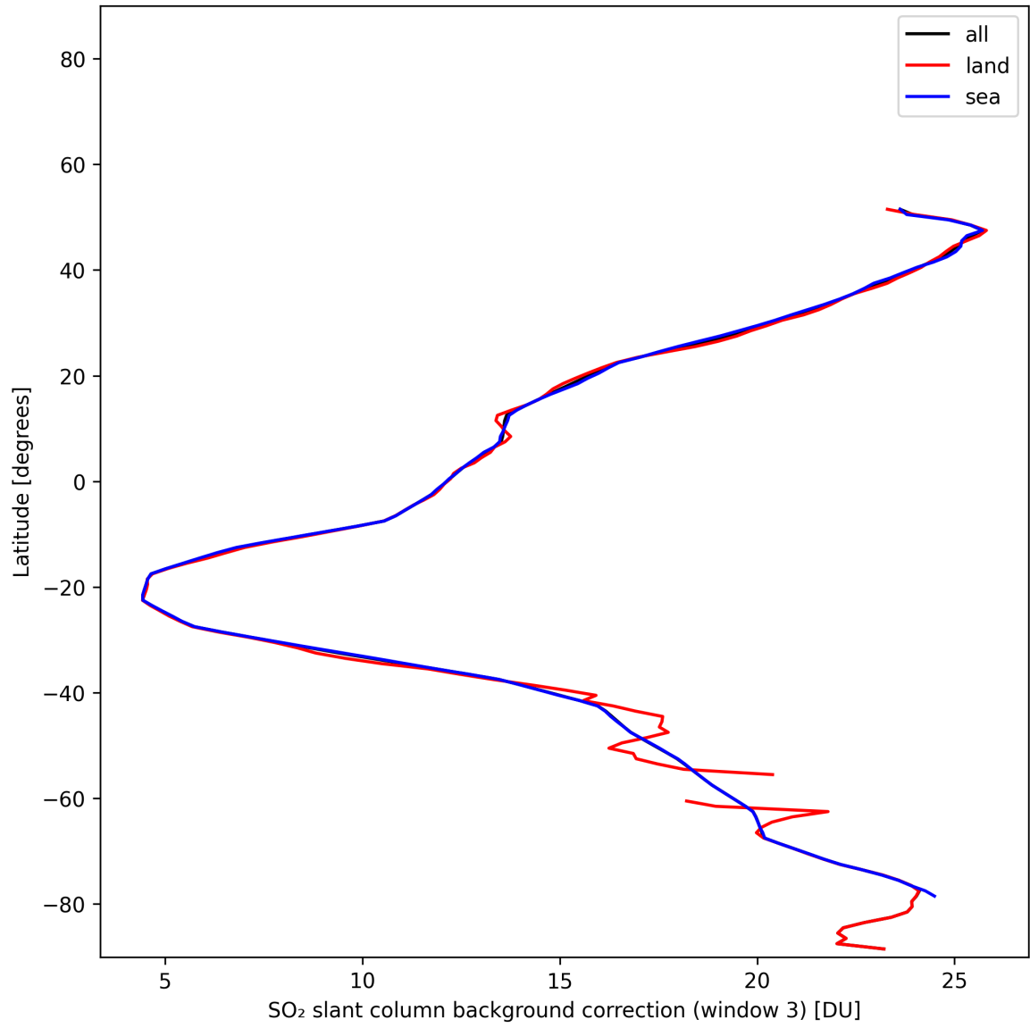
Figure 47: Zonal average of “SO 2 slant column background correction (window 3)” for 2025-01-25 to 2025-01-26.
