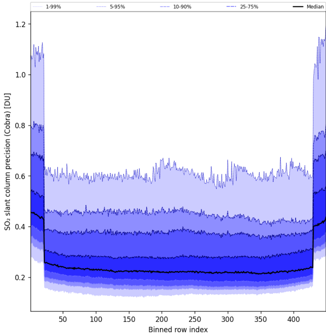
Figure 89: Along track statistics of “SO 2 slant column precision (Cobra)” for 2025-01-25 to 2025-01-26
