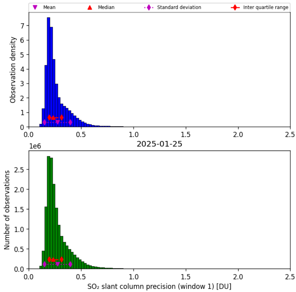
Figure 64: Histogram of “SO 2 slant column precision (window 1)” for 2025-01-25 to 2025-01-26
