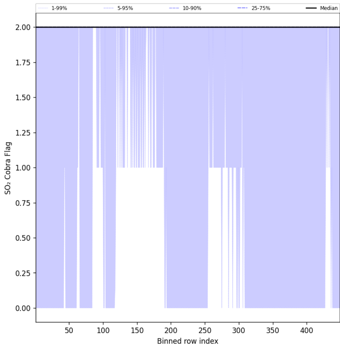
Figure 102: Along track statistics of “SO 2 Cobra Flag” for 2025-01-25 to 2025-01-26
