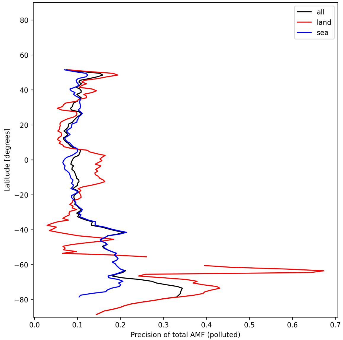
Figure 54: Zonal average of “Precision of total AMF (polluted)” for 2025-01-25 to 2025-01-26.
