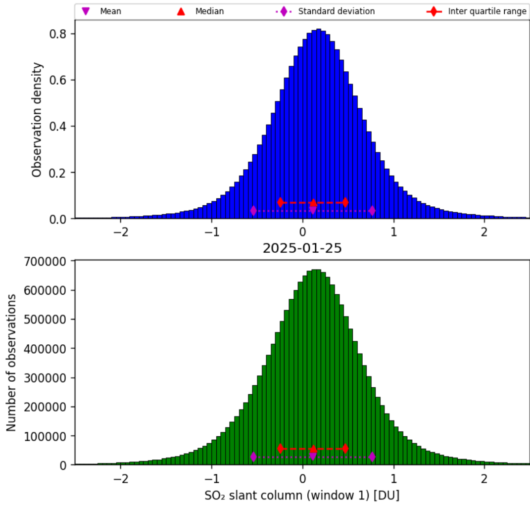
Figure 63: Histogram of “SO 2 slant column (window 1)” for 2025-01-25 to 2025-01-26
