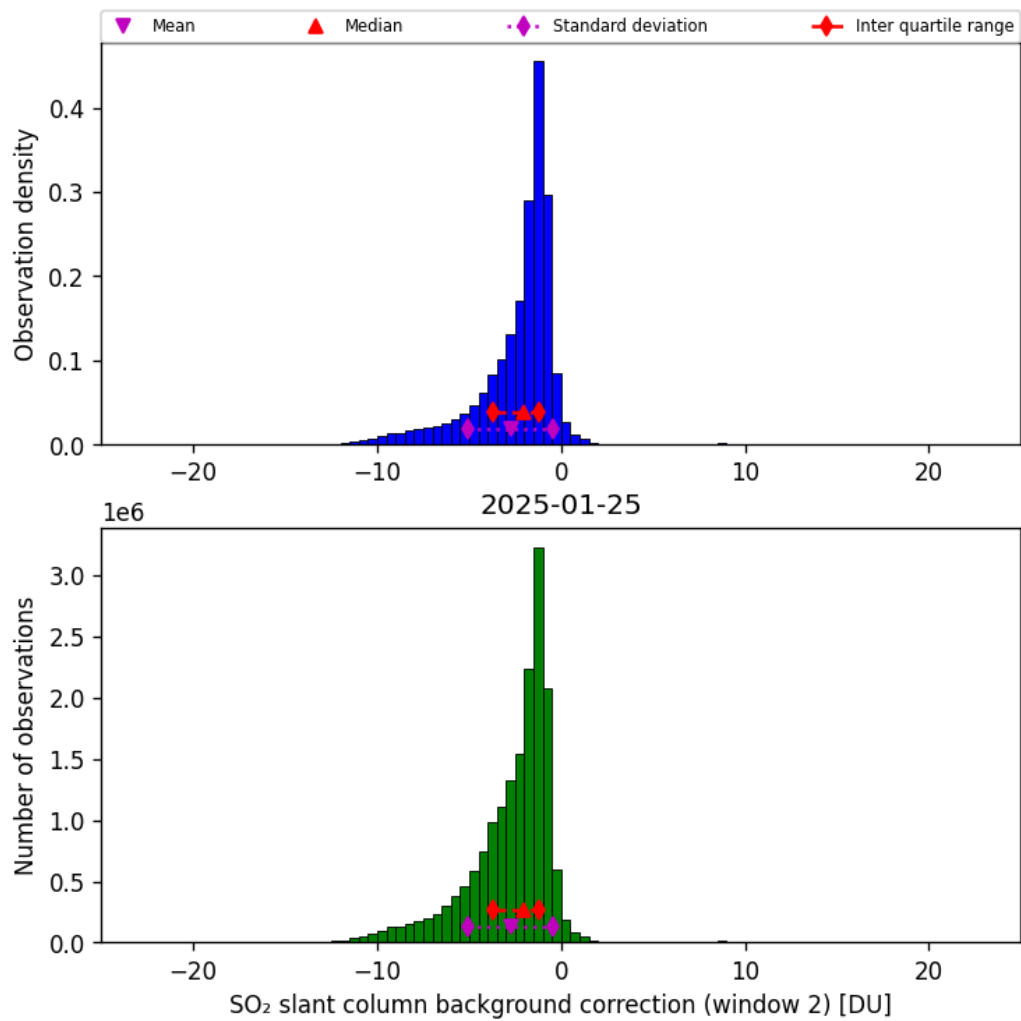
Figure 70: Histogram of “SO 2 slant column background correction (window 2)” for 2025-01-25 to 2025-01-26
