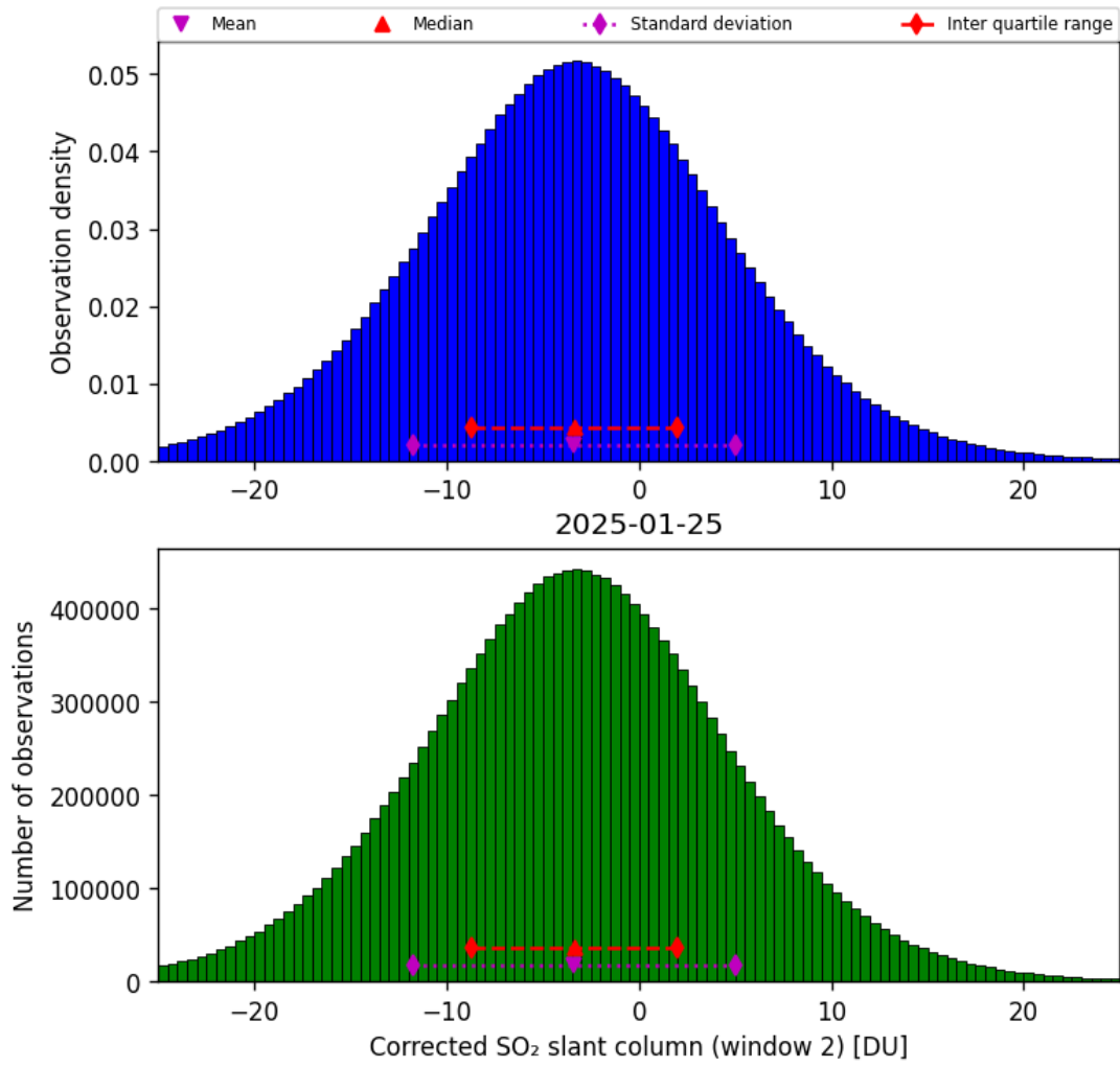
Figure 69: Histogram of “Corrected SO 2 slant column (window 2)” for 2025-01-25 to 2025-01-26
