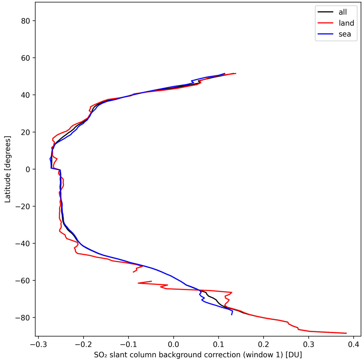
Figure 39: Zonal average of “SO 2 slant column background correction (window 1)” for 2025-01-25 to 2025-01-26.
