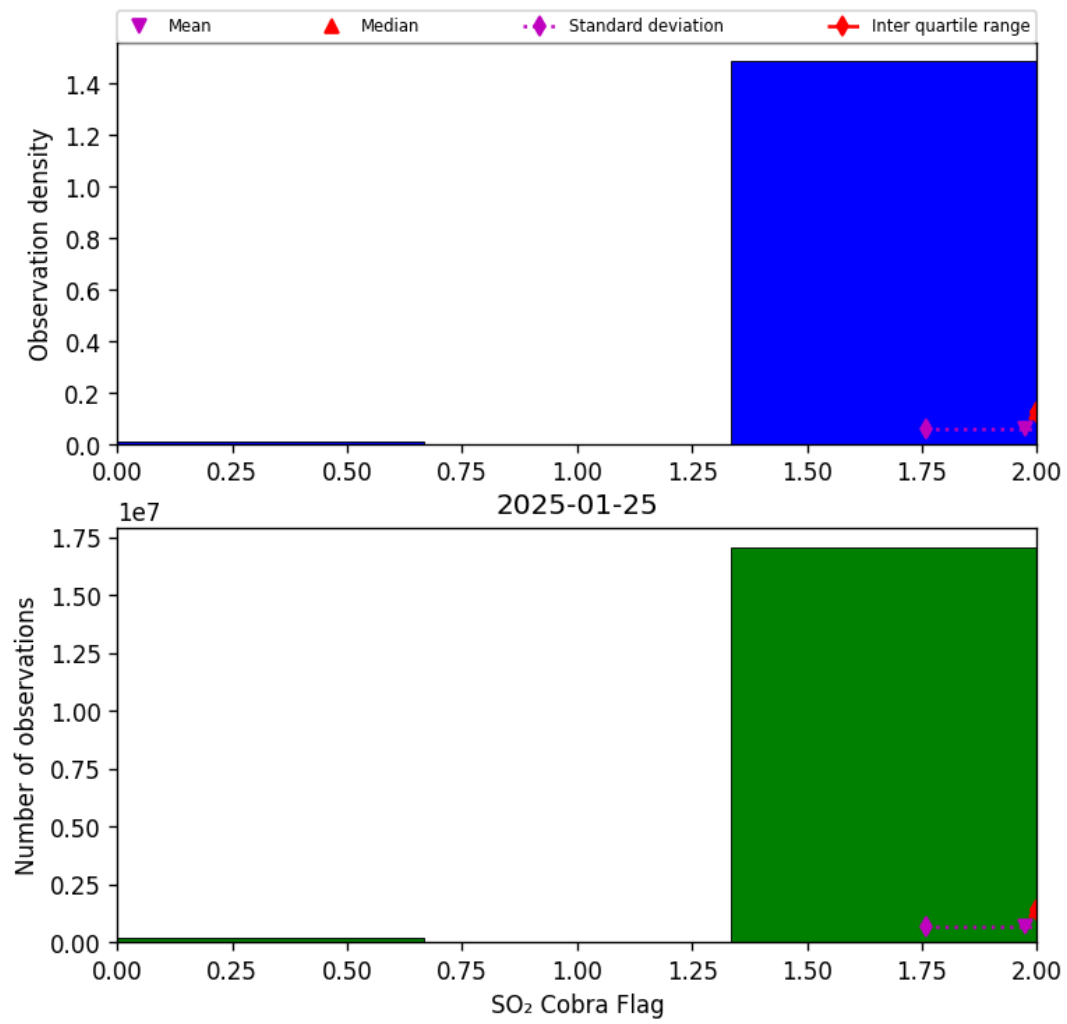
Figure 75: Histogram of “SO 2 Cobra Flag” for 2025-01-25 to 2025-01-26
