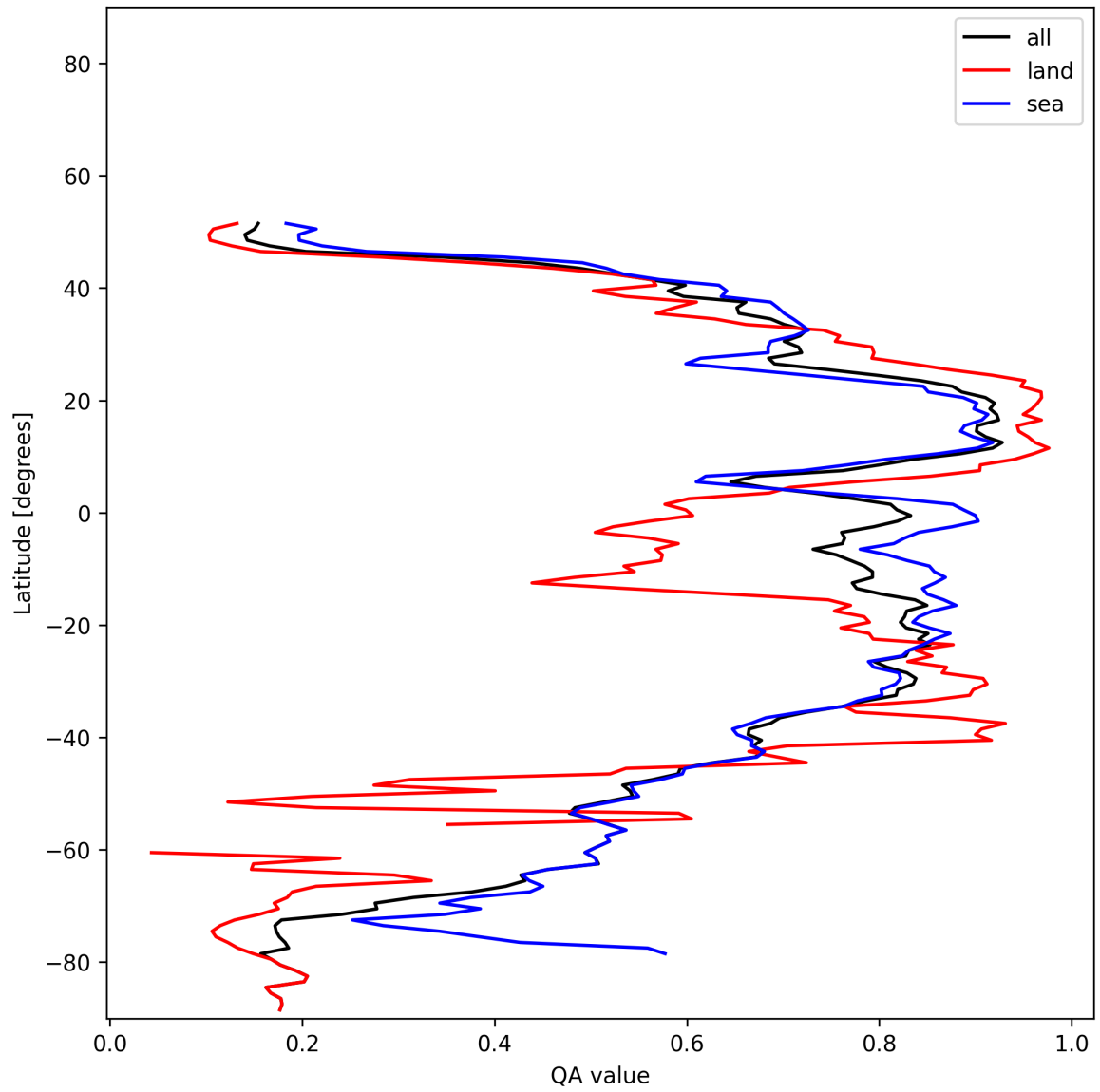
Figure 30: Zonal average of “QA value” for 2025-01-25 to 2025-01-26.
