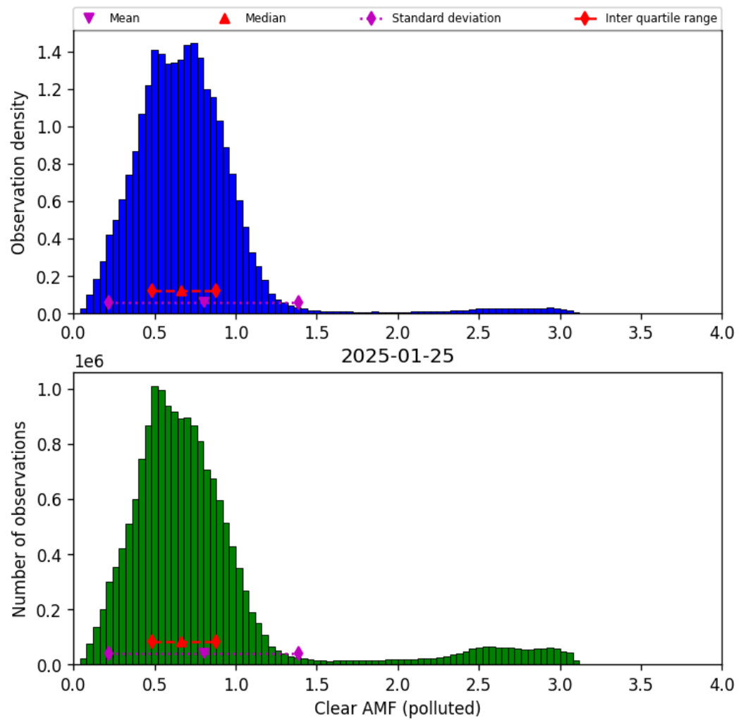
Figure 82: Histogram of “Clear AMF (polluted)” for 2025-01-25 to 2025-01-26
