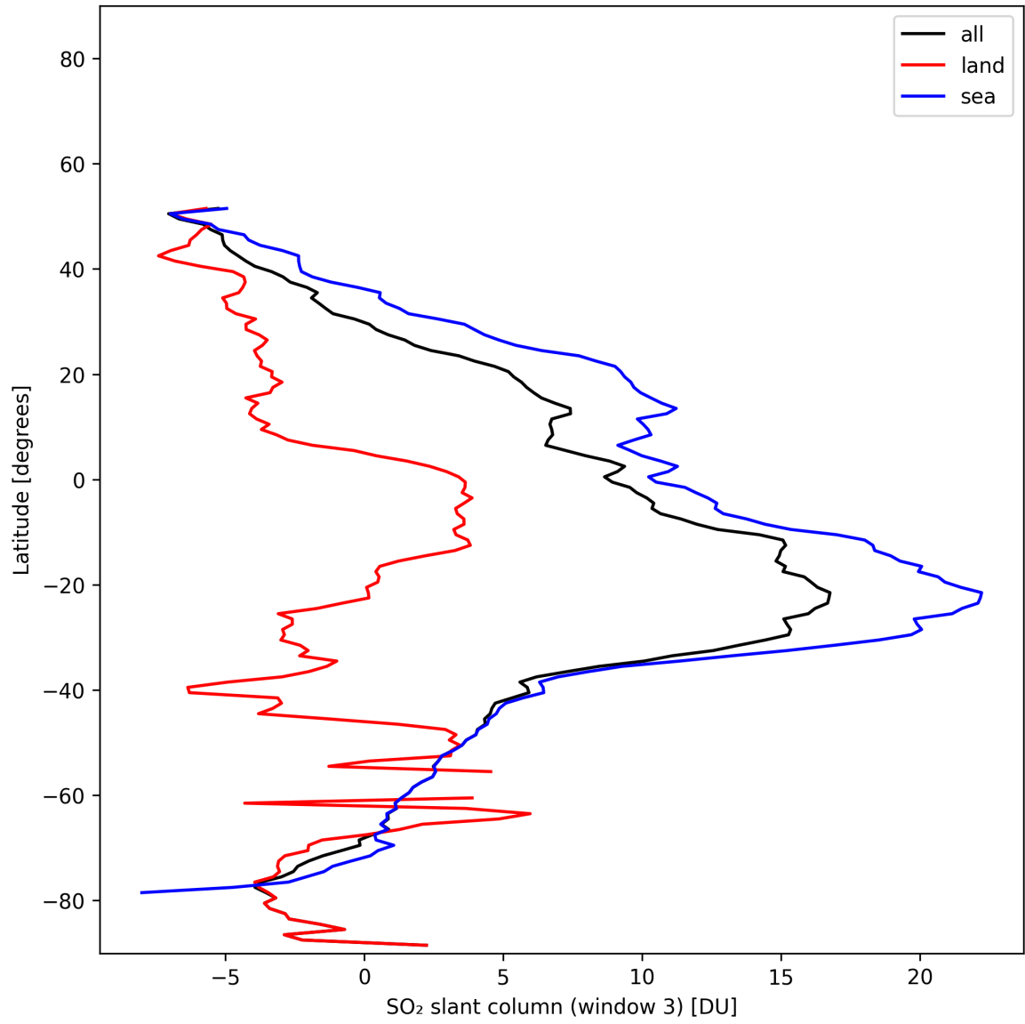
Figure 44: Zonal average of “SO 2 slant column (window 3)” for 2025-01-25 to 2025-01-26.
