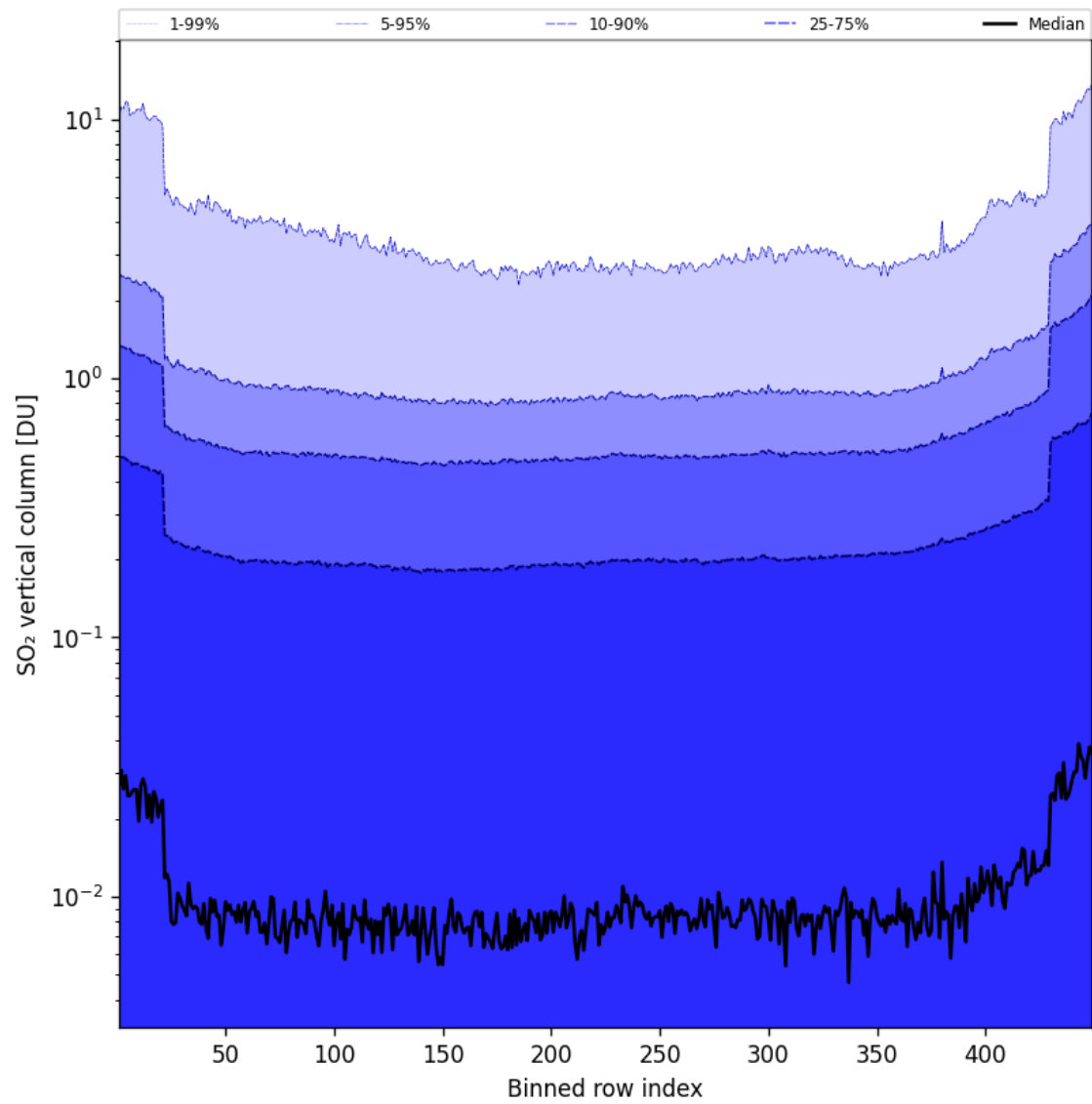
Figure 85: Along track statistics of “SO 2 vertical column” for 2025-01-25 to 2025-01-26
