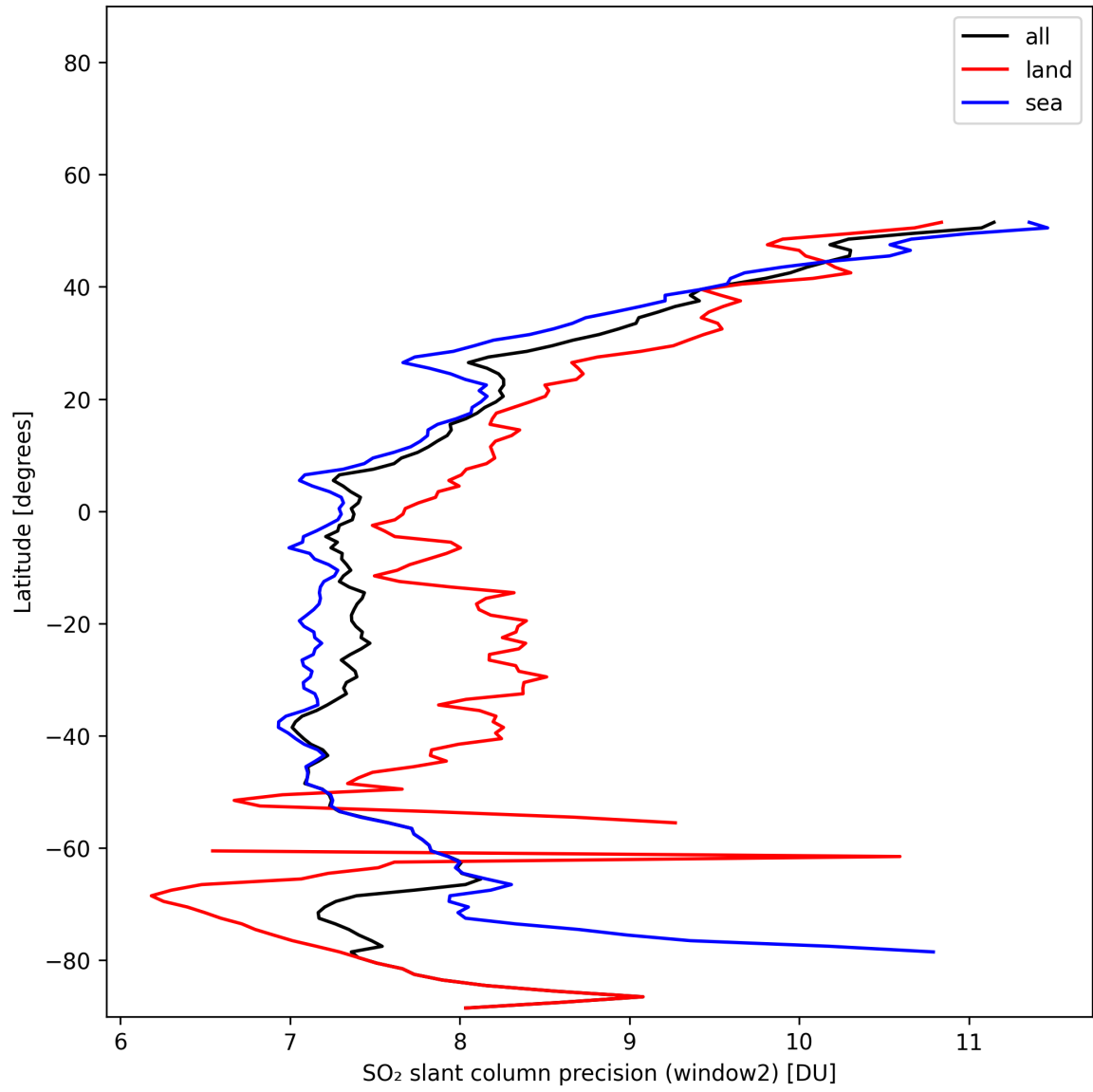
Figure 41: Zonal average of "SO 2 slant column precision (window2)" for 2025-01-25 to 2025-01-26.
