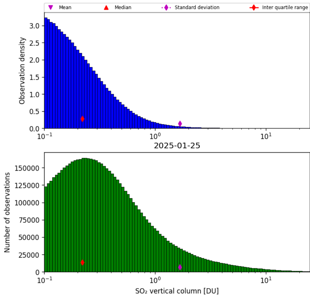
Figure 58: Histogram of “SO 2 vertical column” for 2025-01-25 to 2025-01-26
