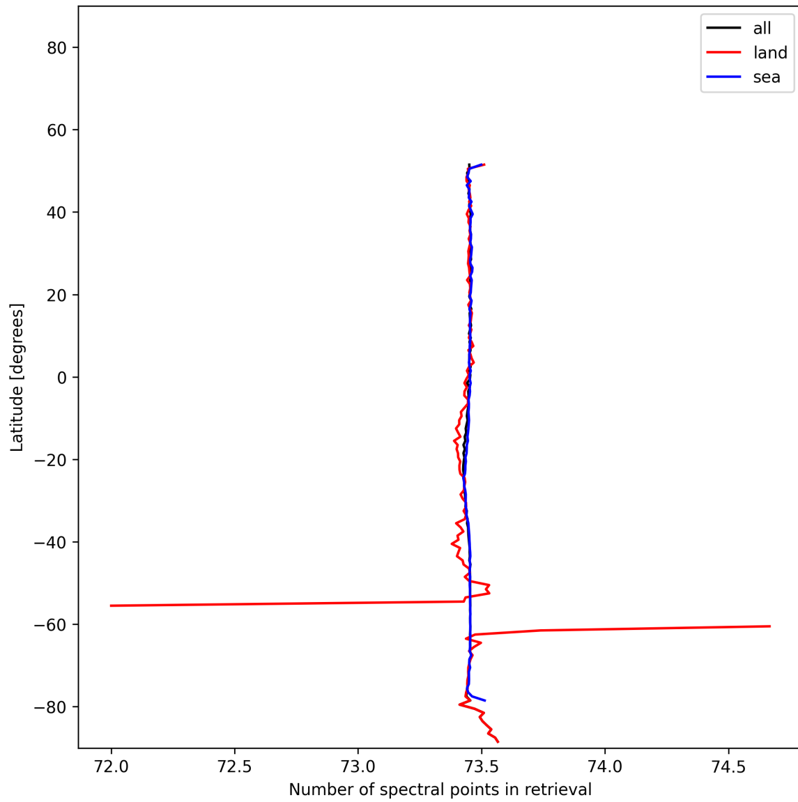
Figure 56: Zonal average of “Number of spectral points in retrieval” for 2025-01-25 to 2025-01-26.
