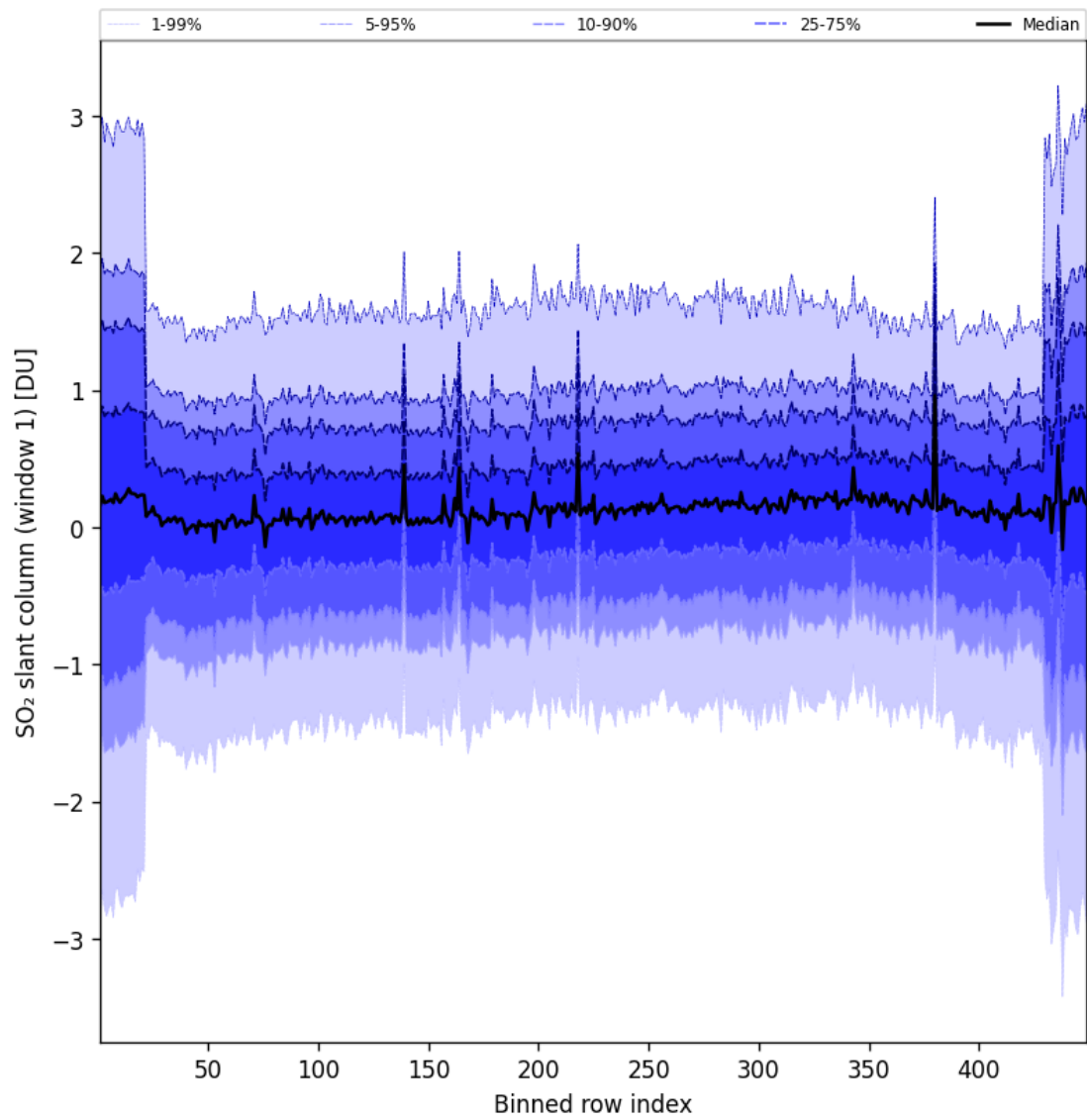
Figure 90: Along track statistics of “SO 2 slant column (window 1)” for 2025-01-25 to 2025-01-26
