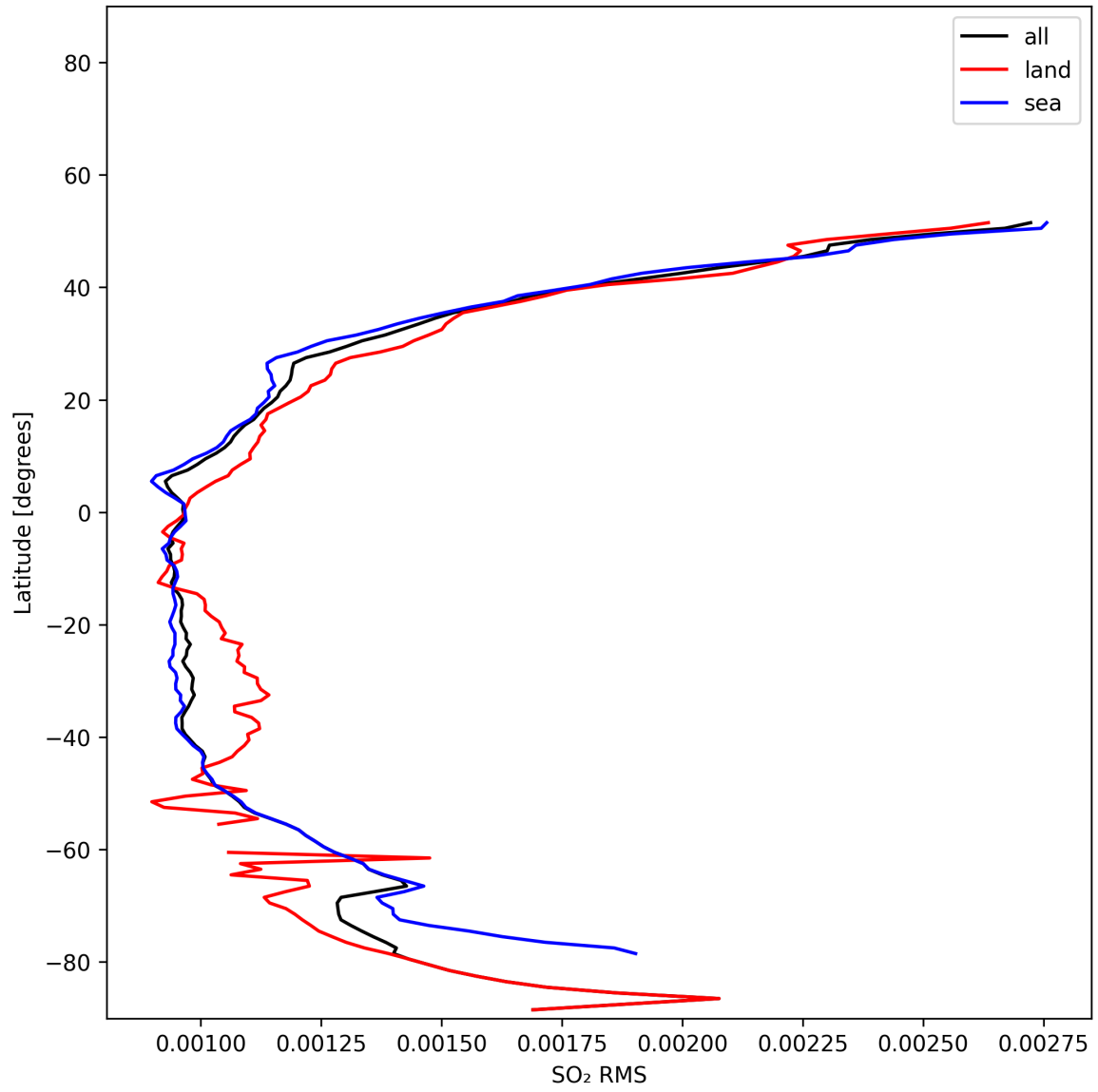
Figure 52: Zonal average of “SO 2 RMS” for 2025-01-25 to 2025-01-26.
