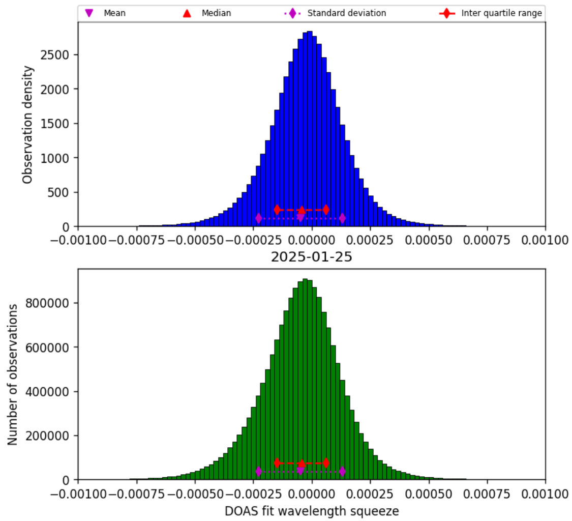
Figure 78: Histogram of “DOAS fit wavelength squeeze” for 2025-01-25 to 2025-01-26
