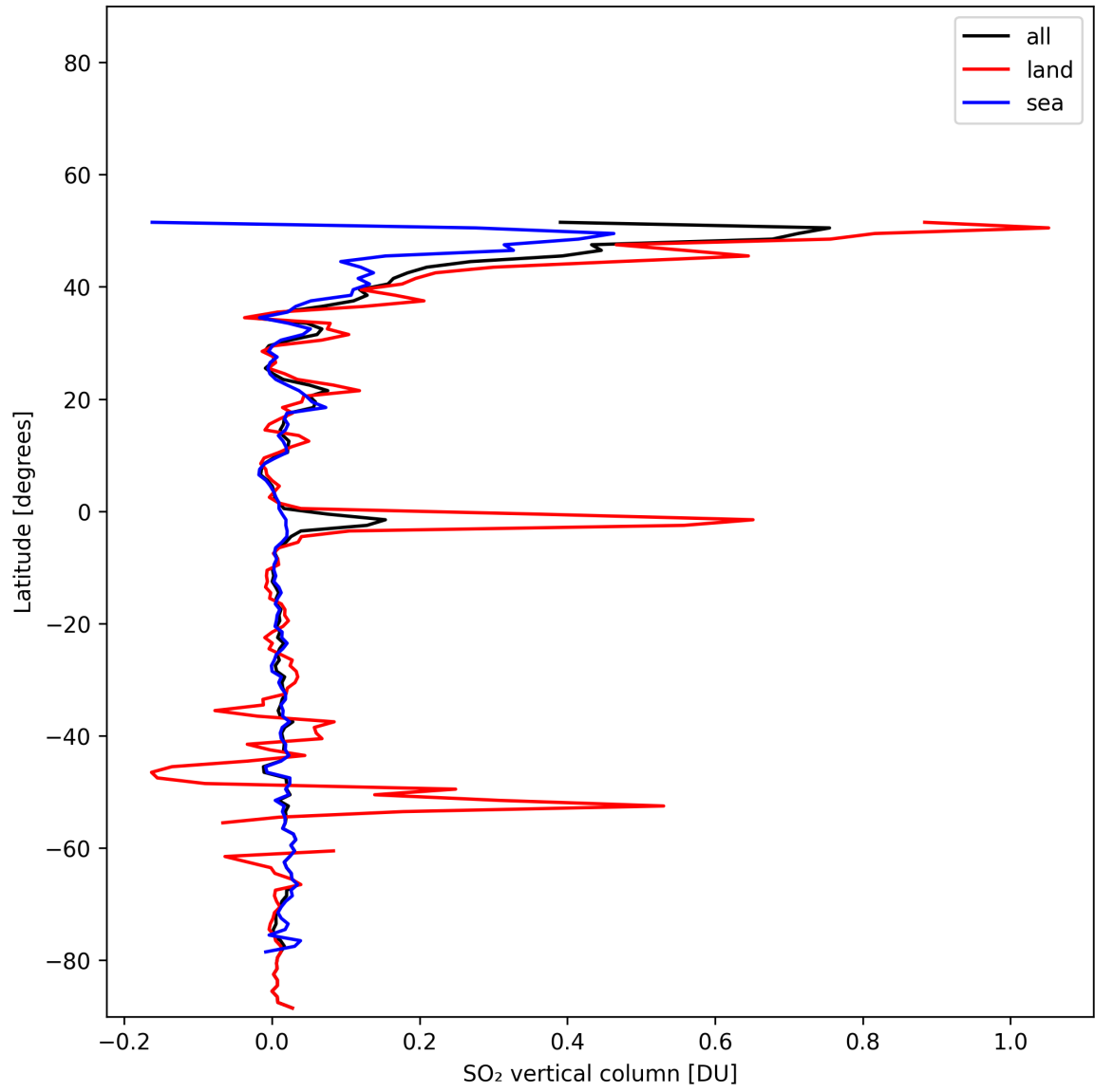
Figure 31: Zonal average of “SO 2 vertical column” for 2025-01-25 to 2025-01-26.
