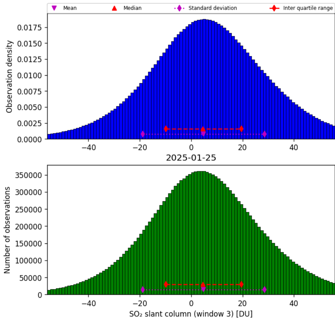
Figure 71: Histogram of “SO 2 slant column (window 3)” for 2025-01-25 to 2025-01-26
