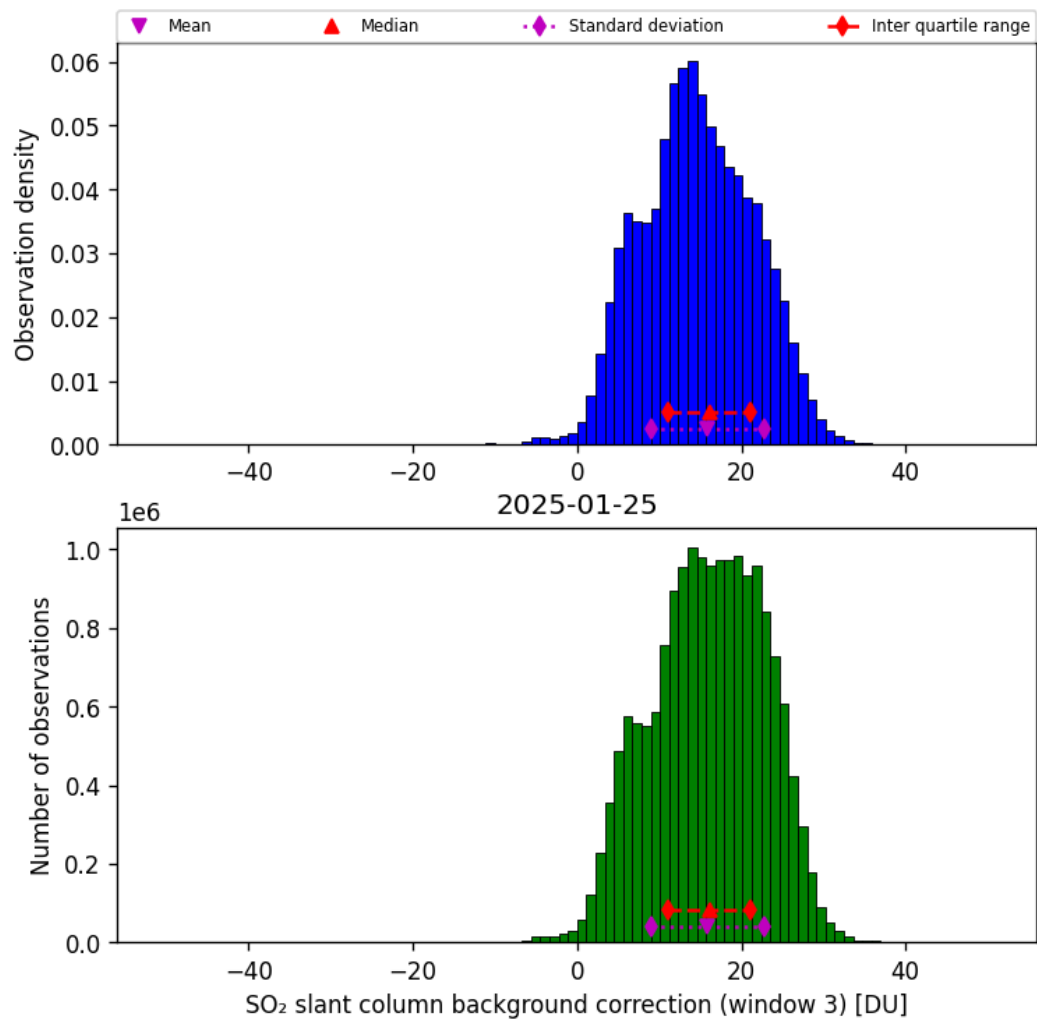
Figure 74: Histogram of “SO 2 slant column background correction (window 3)” for 2025-01-25 to 2025-01-26
