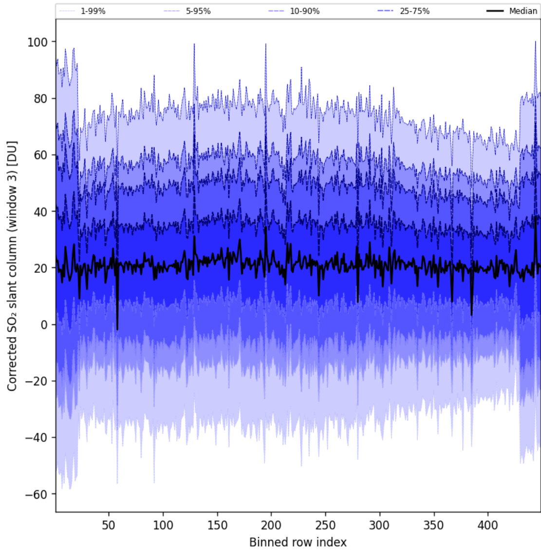
Figure 100: Along track statistics of “Corrected SO 2 slant column (window 3)” for 2025-01-25 to 2025-01-26
