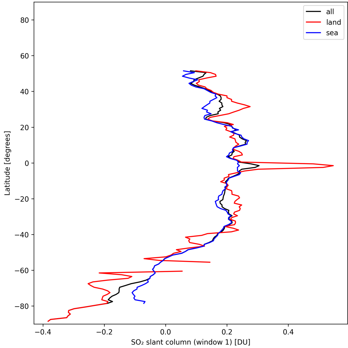
Figure 36: Zonal average of “SO 2 slant column (window 1)” for 2025-01-25 to 2025-01-26.
