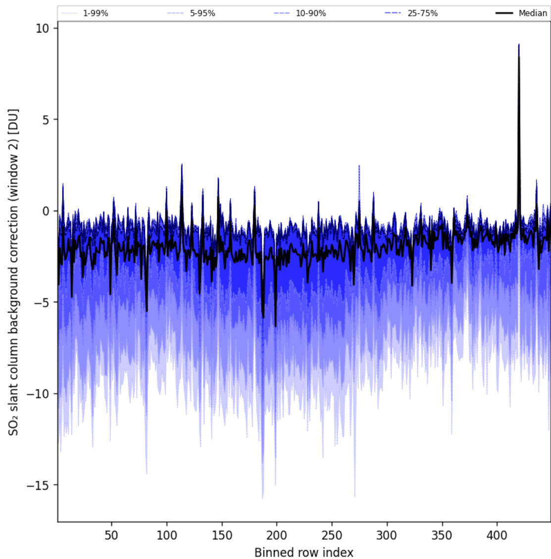
Figure 97: Along track statistics of “SO 2 slant column background correction (window 2)” for 2025-01-25 to 2025-01-26
