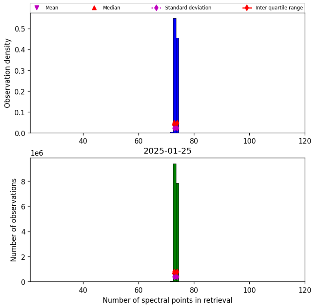
Figure 83: Histogram of “Number of spectral points in retrieval” for 2025-01-25 to 2025-01-26
