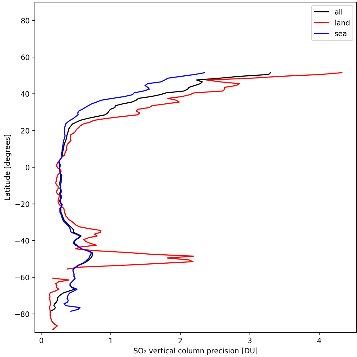
Figure 32: Zonal average of “SO 2 vertical column precision” for 2025-01-25 to 2025-01-26.
