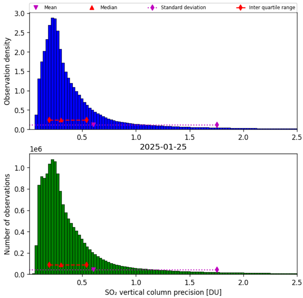
Figure 59: Histogram of “SO 2 vertical column precision” for 2025-01-25 to 2025-01-26
