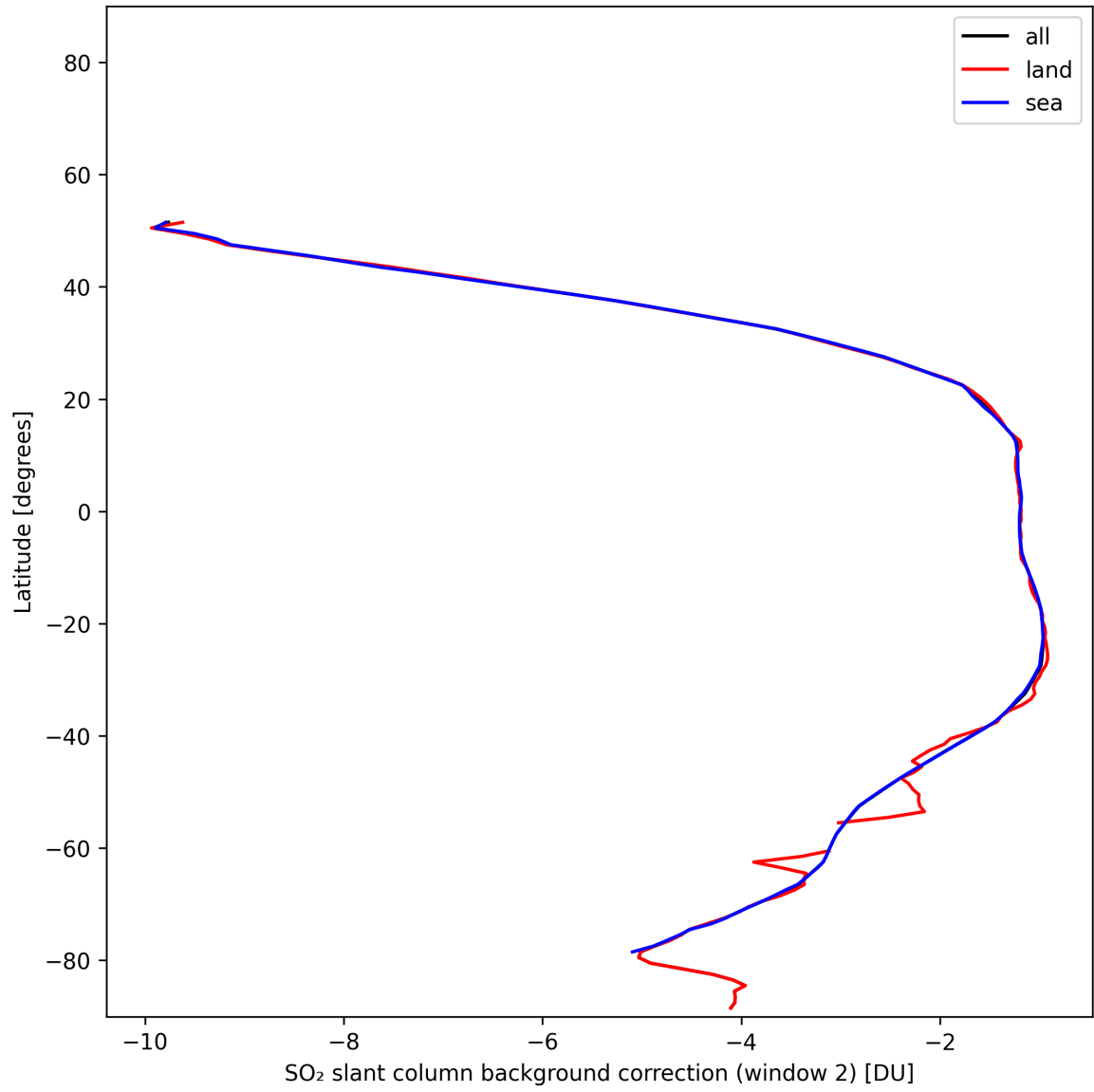
Figure 43: Zonal average of “SO 2 slant column background correction (window 2)” for 2025-01-25 to 2025-01-26.
