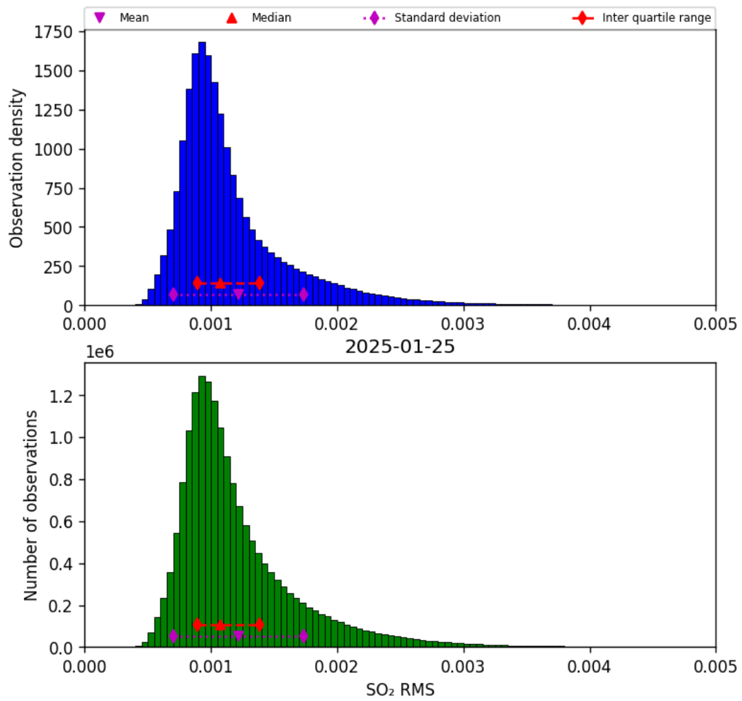
Figure 79: Histogram of “SO 2 RMS” for 2025-01-25 to 2025-01-26
