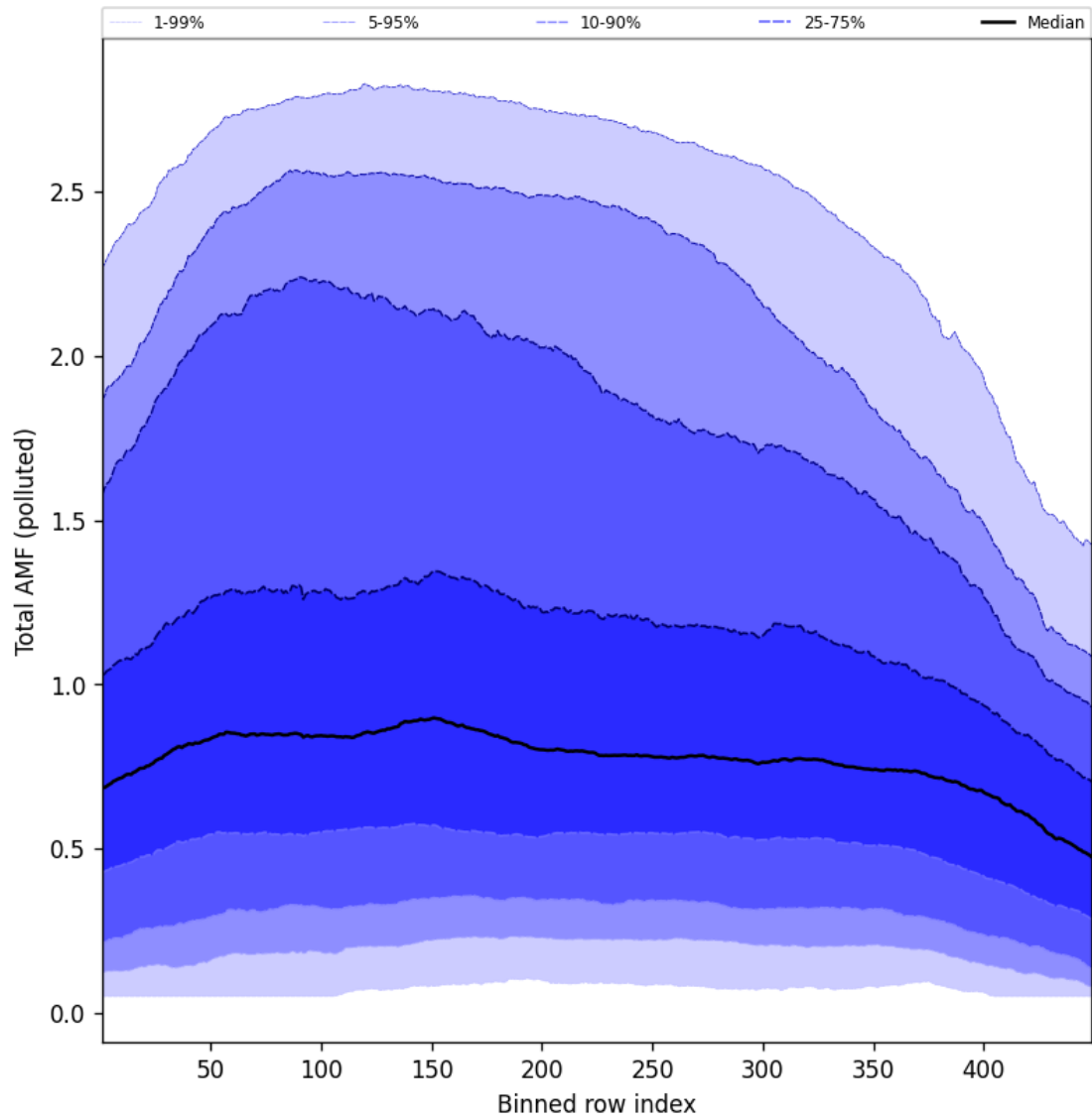
Figure 107: Along track statistics of “Total AMF (polluted)” for 2025-01-25 to 2025-01-26
