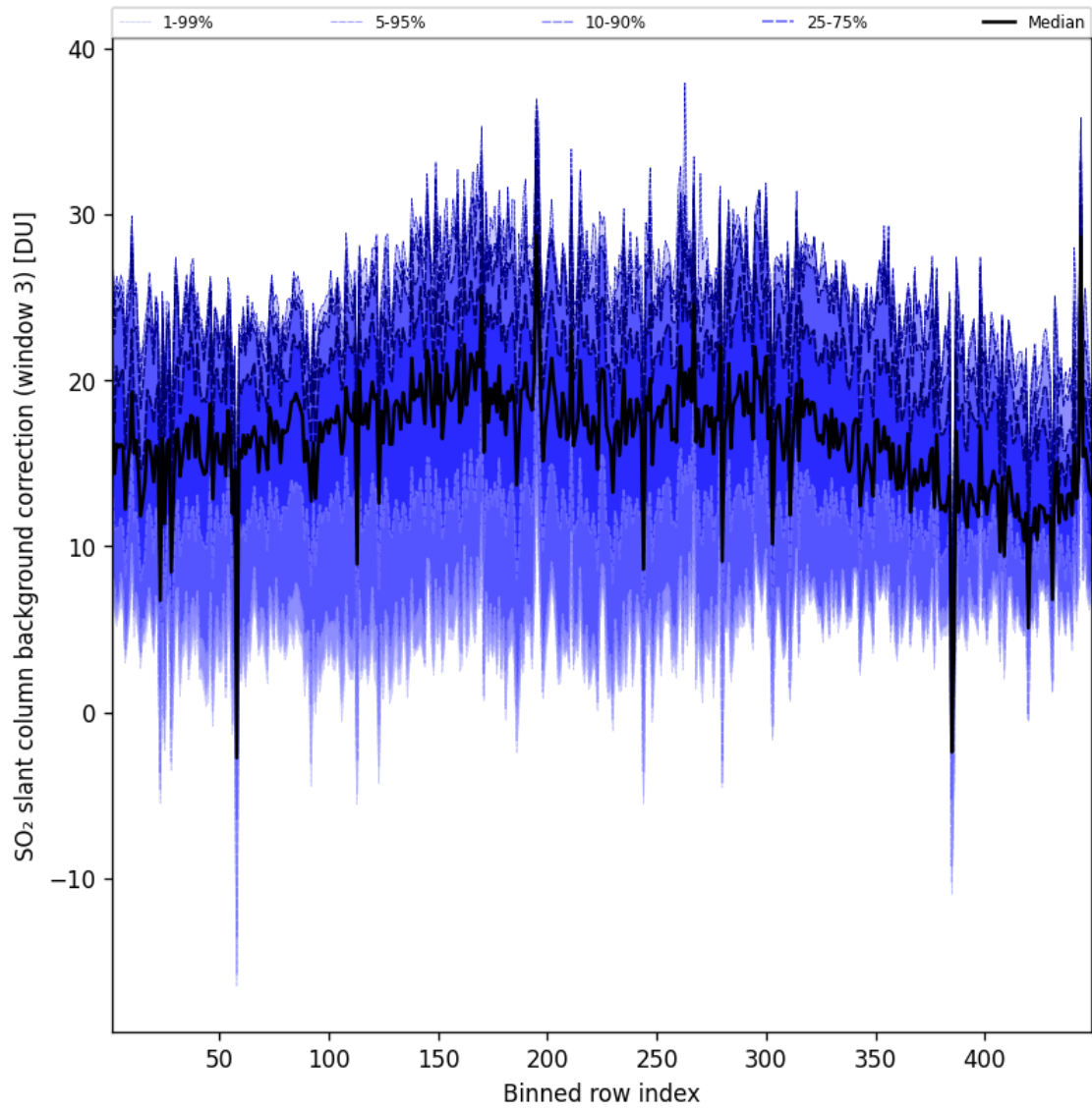
Figure 101: Along track statistics of “SO 2 slant column background correction (window 3)” for 2025-01-25 to 2025-01-26
