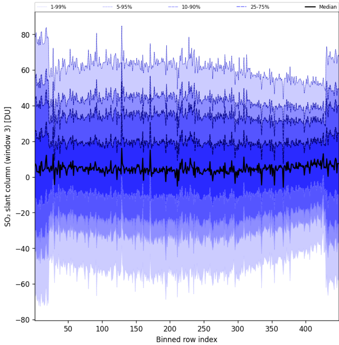
Figure 98: Along track statistics of “SO 2 slant column (window 3)” for 2025-01-25 to 2025-01-26
