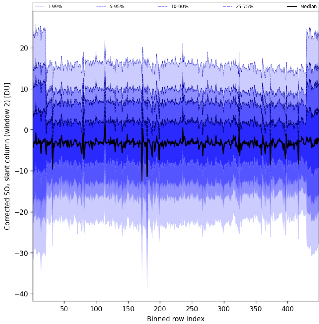
Figure 96: Along track statistics of “Corrected SO 2 slant column (window 2)” for 2025-01-25 to 2025-01-26
