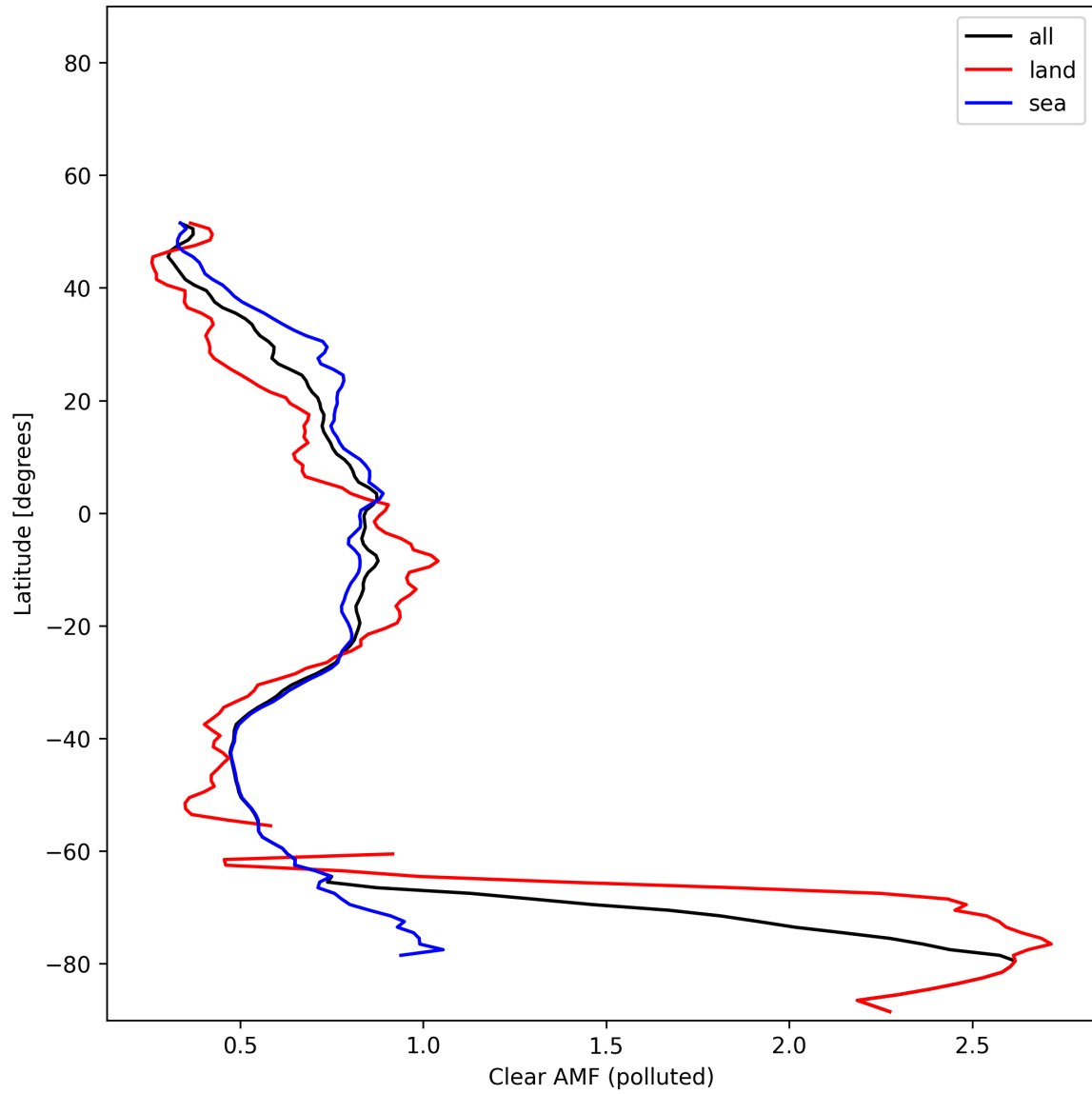
Figure 55: Zonal average of “Clear AMF (polluted)” for 2025-01-25 to 2025-01-26.
