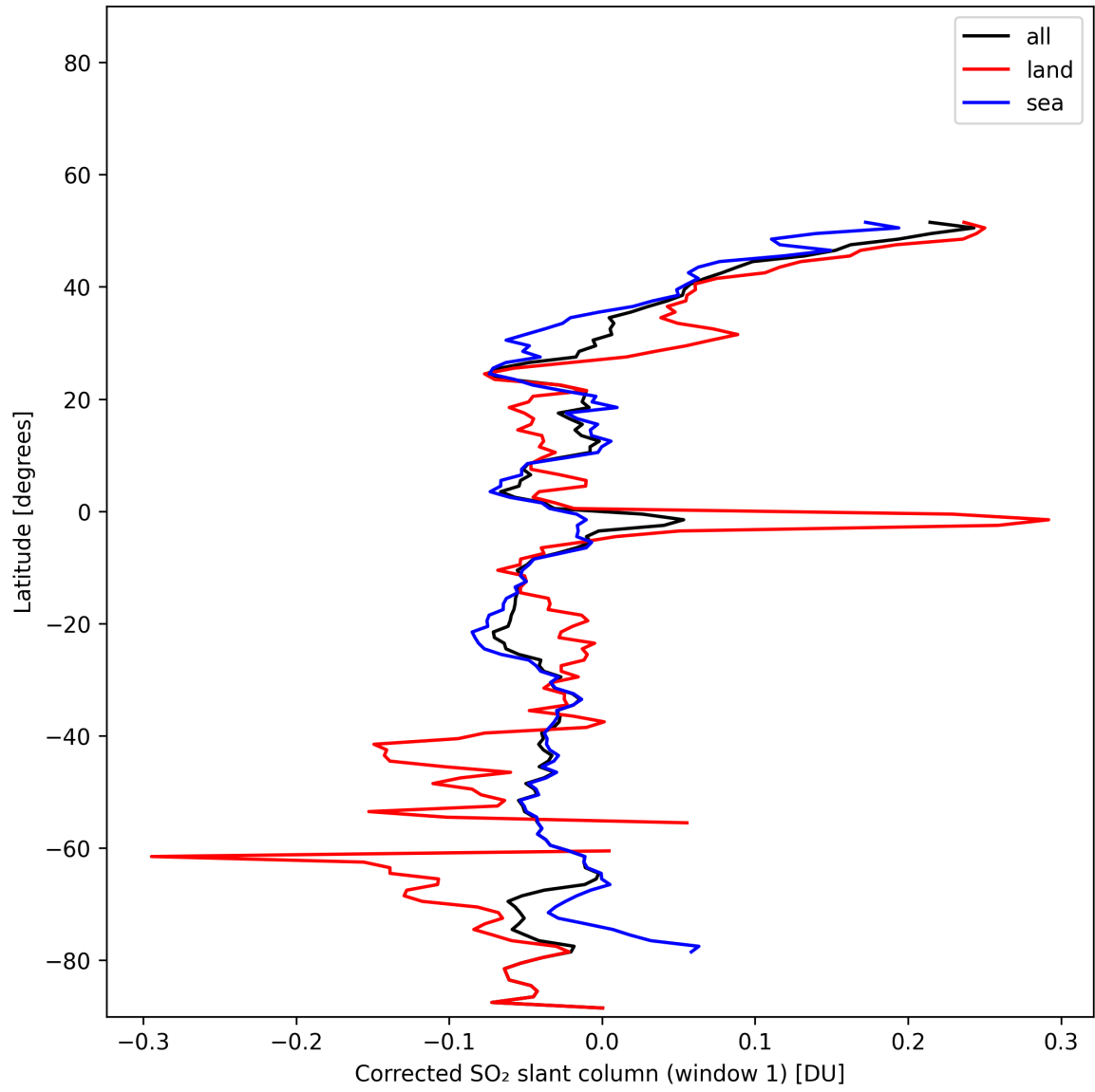
Figure 38: Zonal average of “Corrected SO 2 slant column (window 1)” for 2025-01-25 to 2025-01-26.
