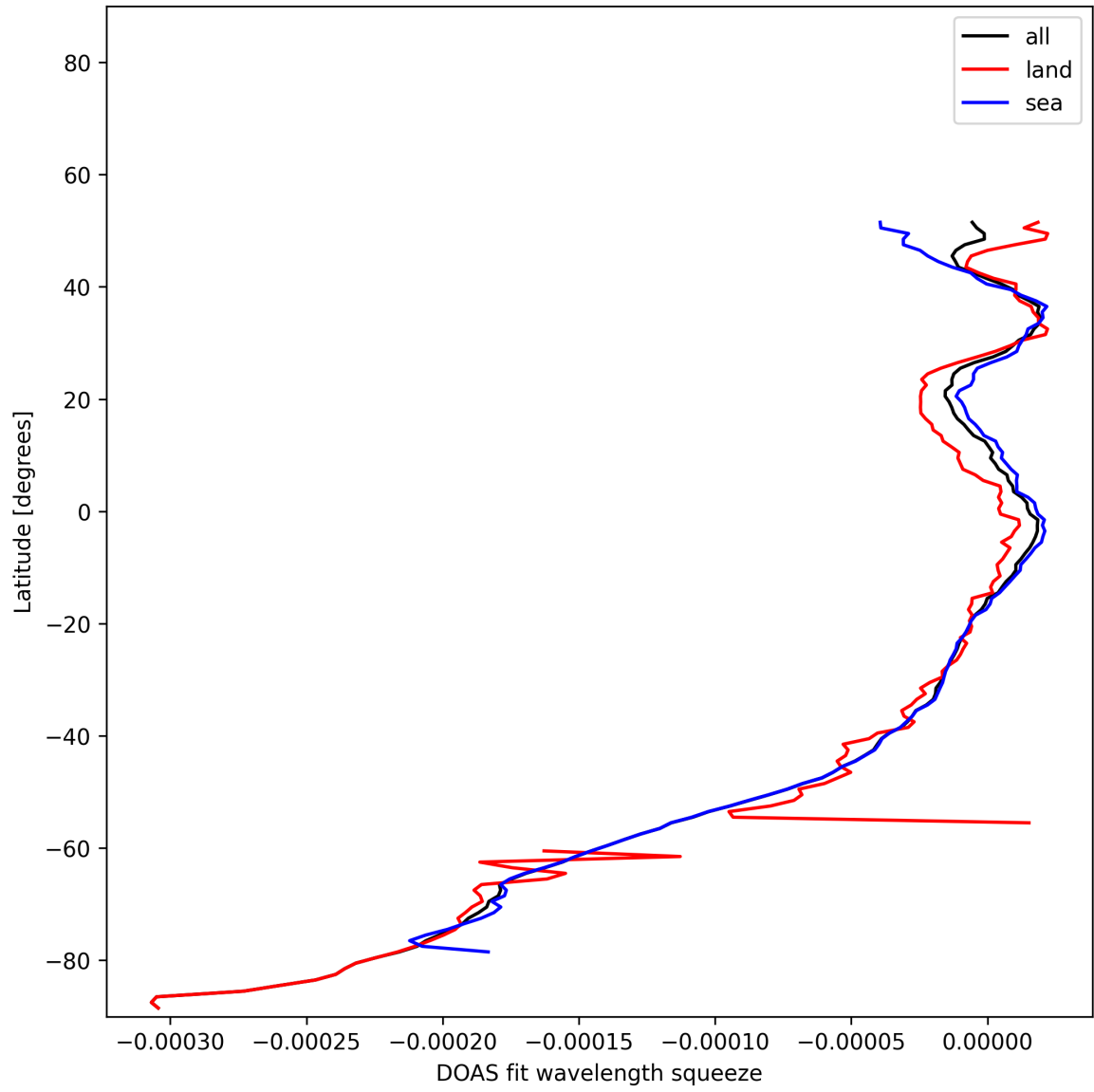
Figure 51: Zonal average of “DOAS fit wavelength squeeze” for 2025-01-25 to 2025-01-26.
