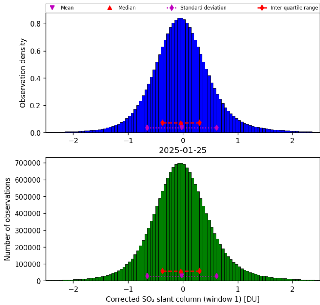
Figure 65: Histogram of “Corrected SO 2 slant column (window 1)” for 2025-01-25 to 2025-01-26
