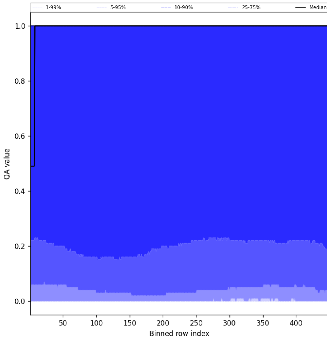
Figure 84: Along track statistics of “QA value” for 2025-01-25 to 2025-01-26
