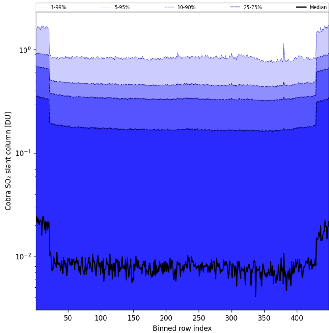
Figure 88: Along track statistics of “Cobra SO 2 slant column” for 2025-01-25 to 2025-01-26
