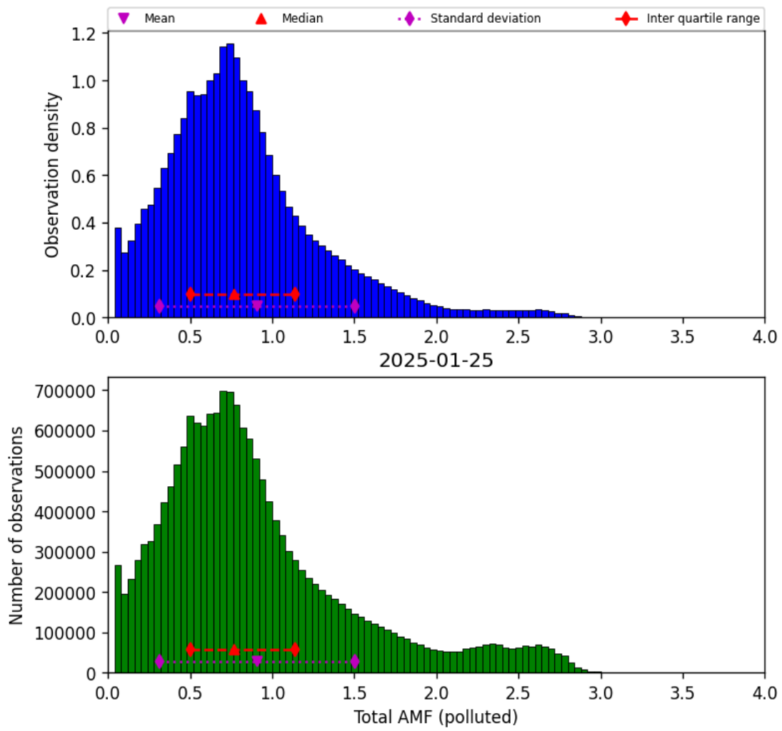
Figure 80: Histogram of “Total AMF (polluted)” for 2025-01-25 to 2025-01-26
