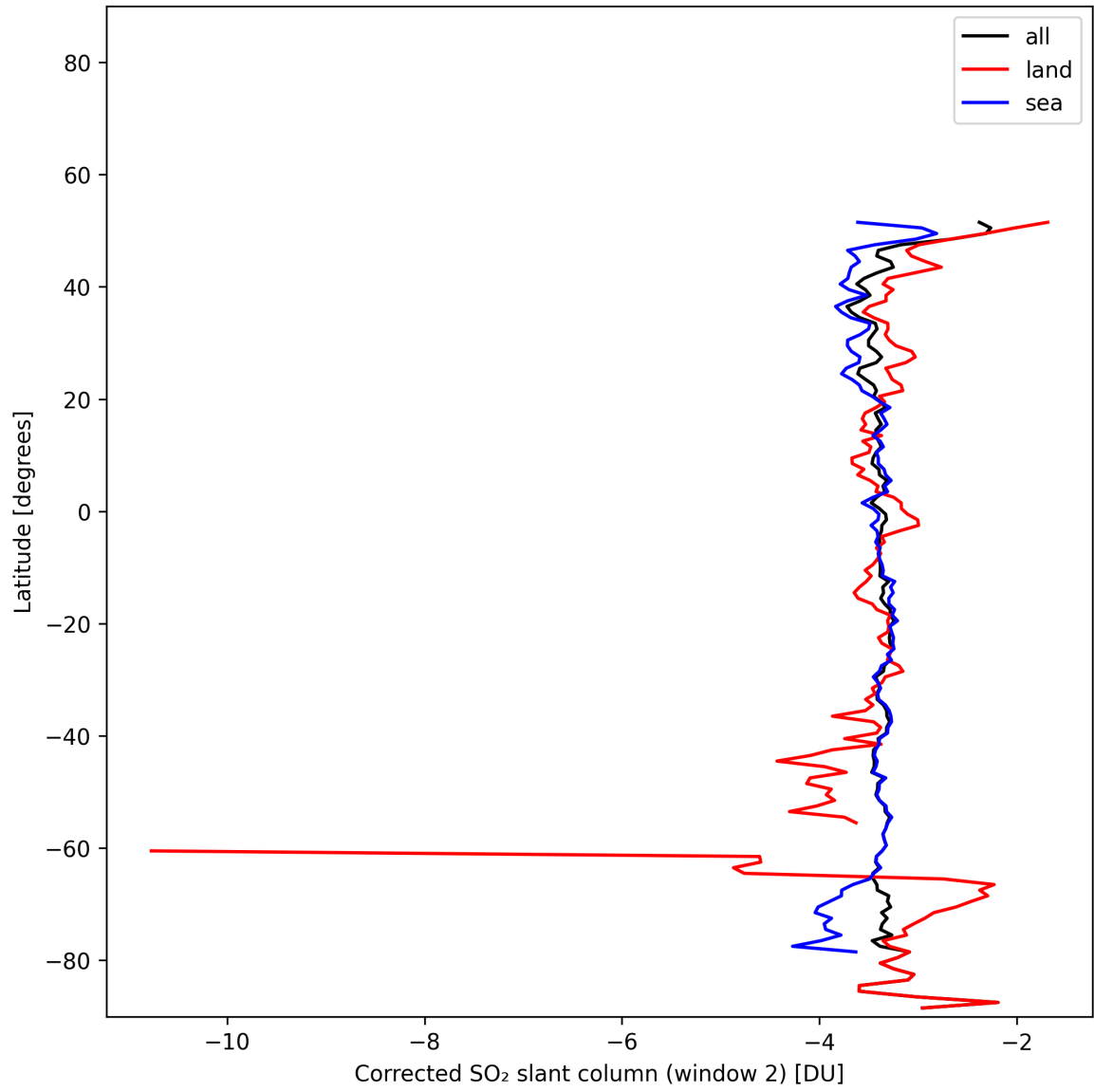
Figure 42: Zonal average of “Corrected SO 2 slant column (window 2)” for 2025-01-25 to 2025-01-26.
