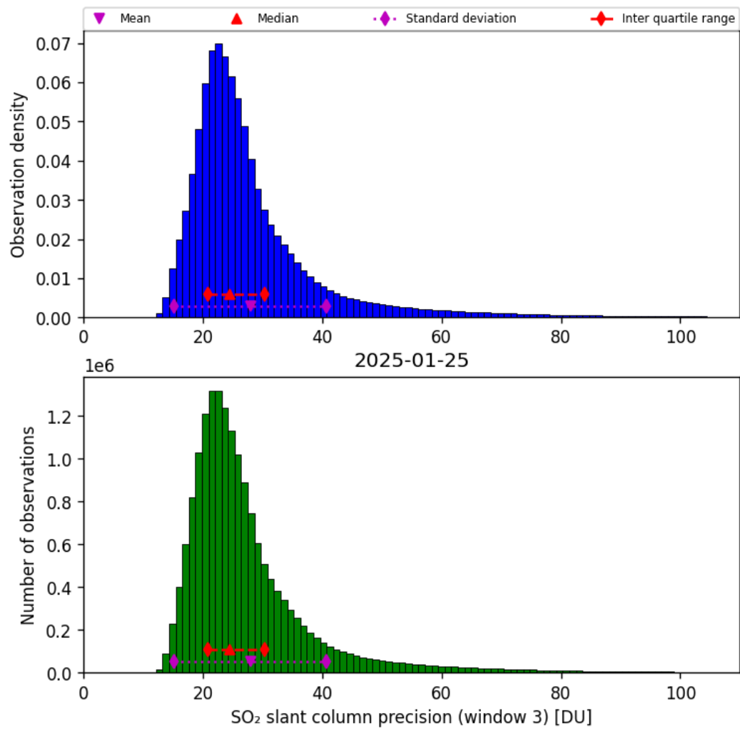
Figure 72: Histogram of “SO 2 slant column precision (window 3)” for 2025-01-25 to 2025-01-26
