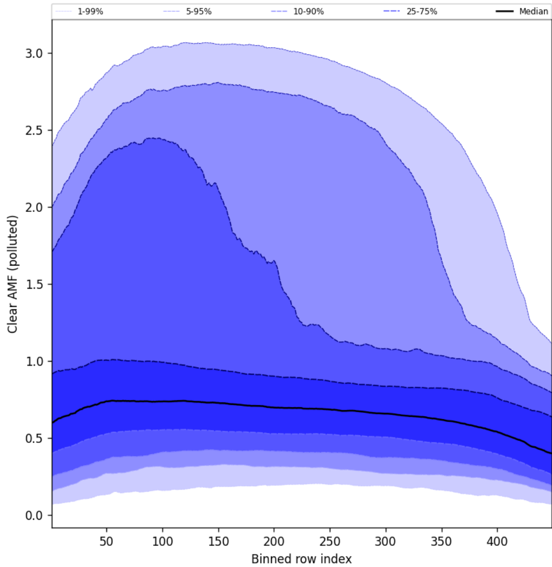
Figure 109: Along track statistics of “Clear AMF (polluted)” for 2025-01-25 to 2025-01-26
