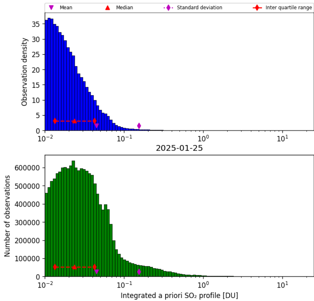
Figure 76: Histogram of “Integrated a priori SO 2 profile” for 2025-01-25 to 2025-01-26
