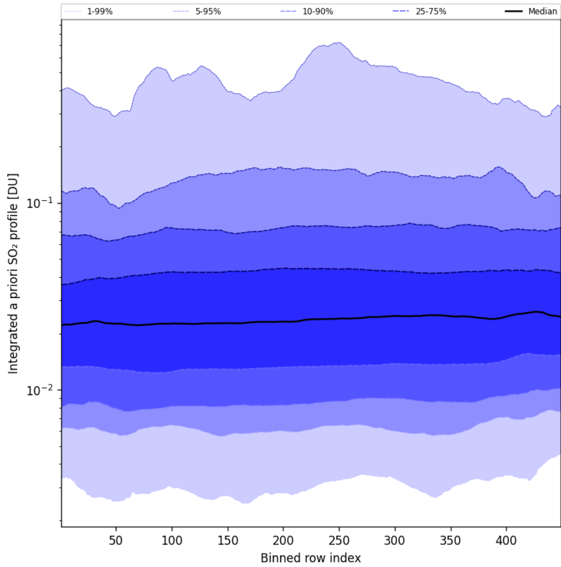
Figure 103: Along track statistics of “Integrated a priori SO 2 profile” for 2025-01-25 to 2025-01-26
