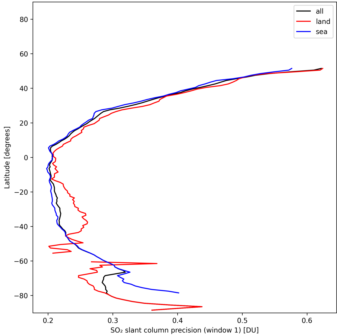
Figure 37: Zonal average of “SO 2 slant column precision (window 1)” for 2025-01-25 to 2025-01-26.
