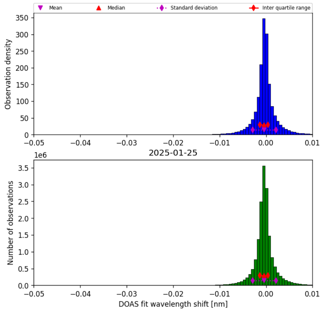
Figure 77: Histogram of “DOAS fit wavelength shift” for 2025-01-25 to 2025-01-26
