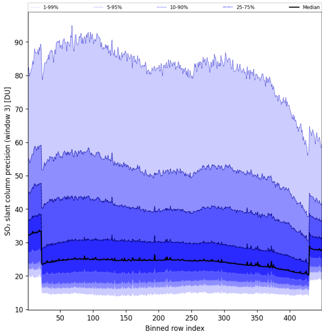
Figure 99: Along track statistics of “SO 2 slant column precision (window 3)” for 2025-01-25 to 2025-01-26
