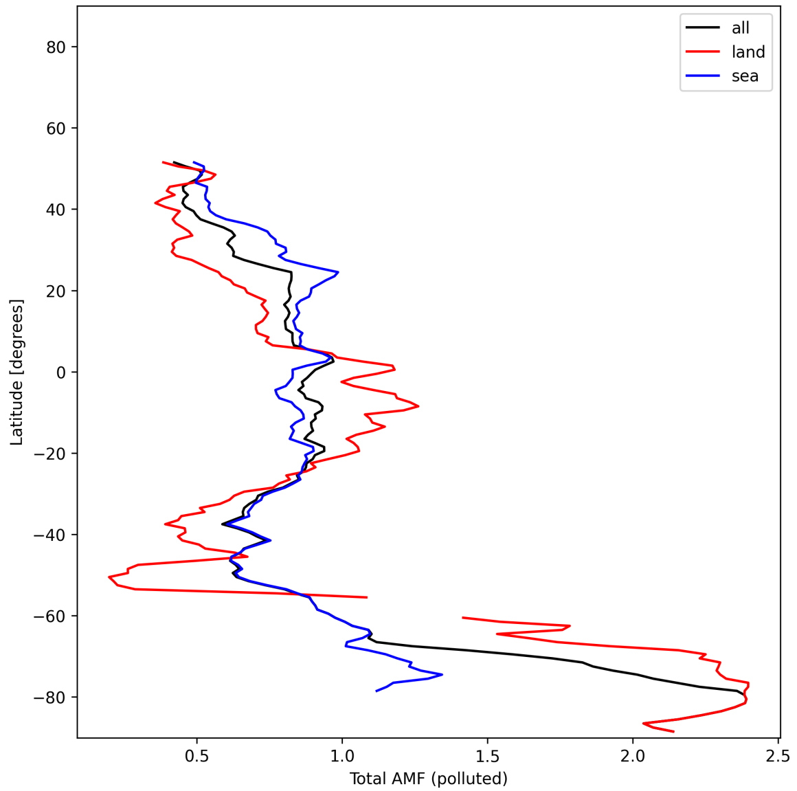
Figure 53: Zonal average of “Total AMF (polluted)” for 2025-01-25 to 2025-01-26.
