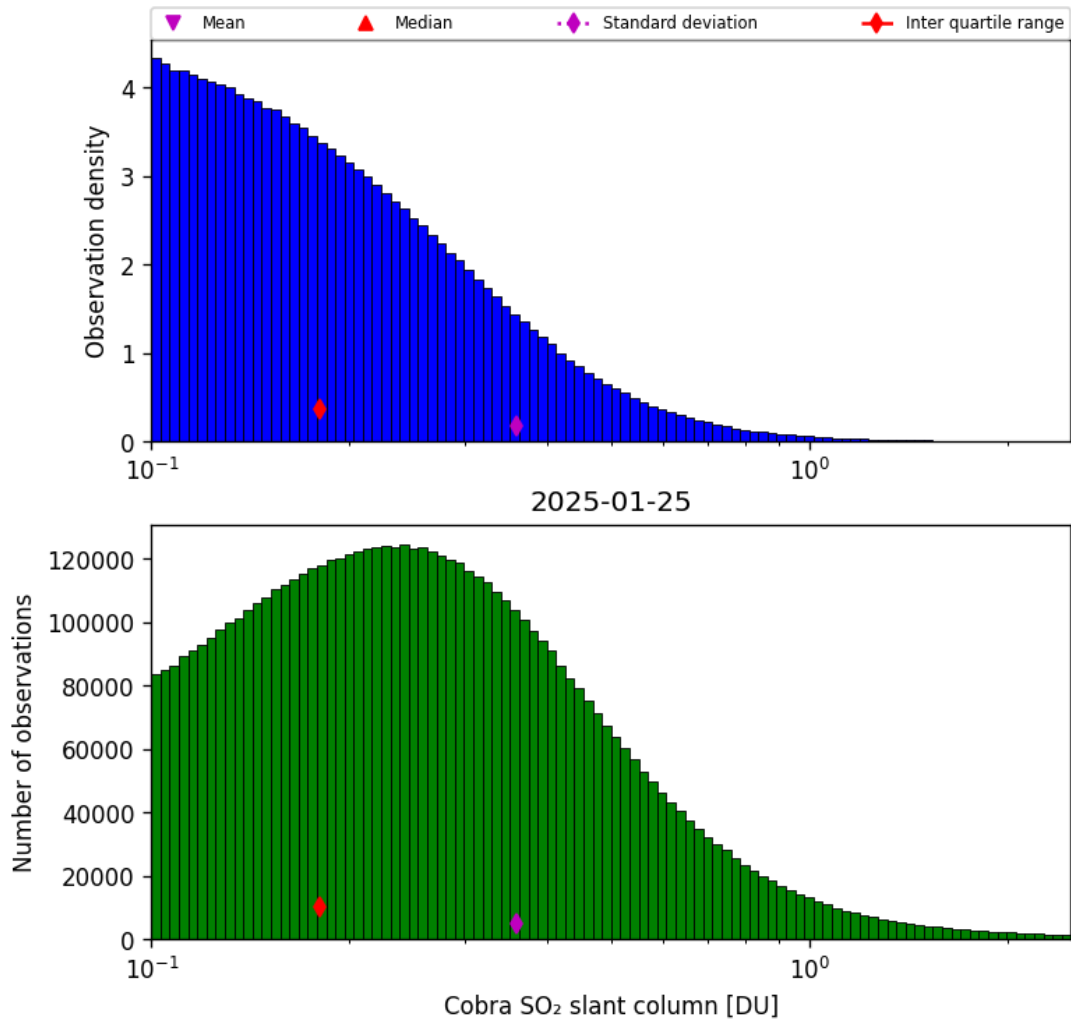
Figure 61: Histogram of “Cobra SO 2 slant column” for 2025-01-25 to 2025-01-26
