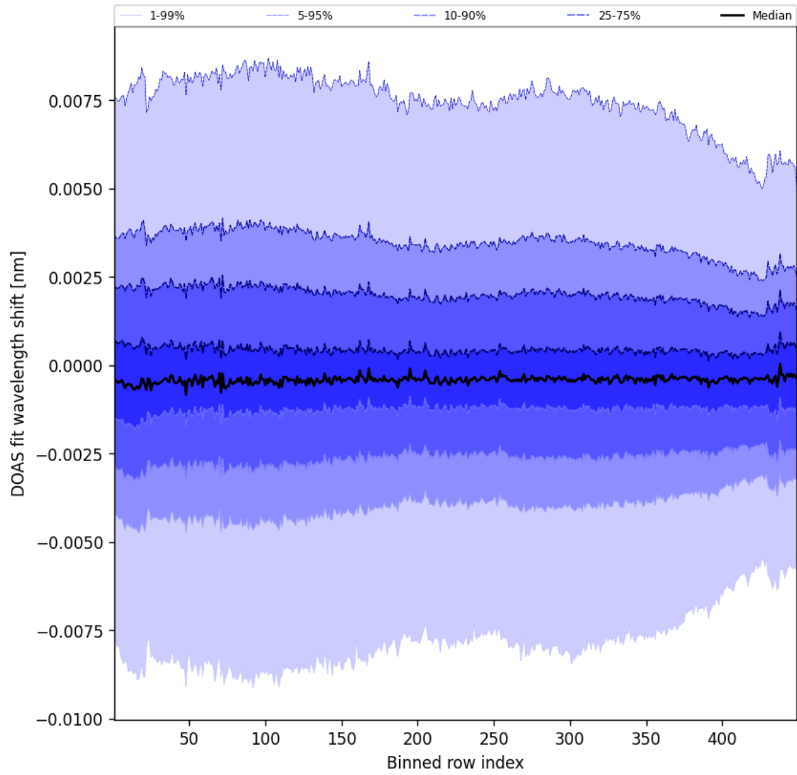
Figure 104: Along track statistics of “DOAS fit wavelength shift” for 2025-01-25 to 2025-01-26
