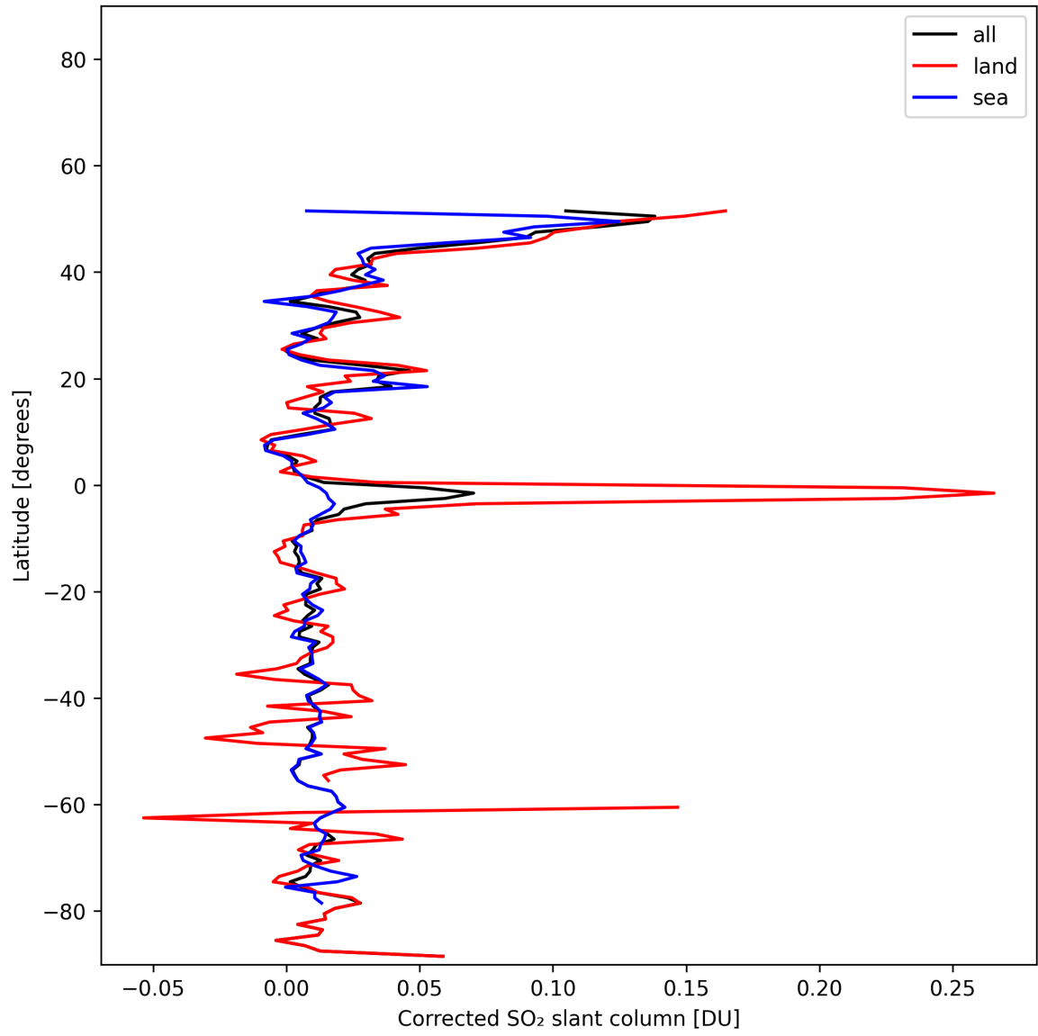
Figure 33: Zonal average of “Corrected SO 2 slant column” for 2025-01-25 to 2025-01-26.
