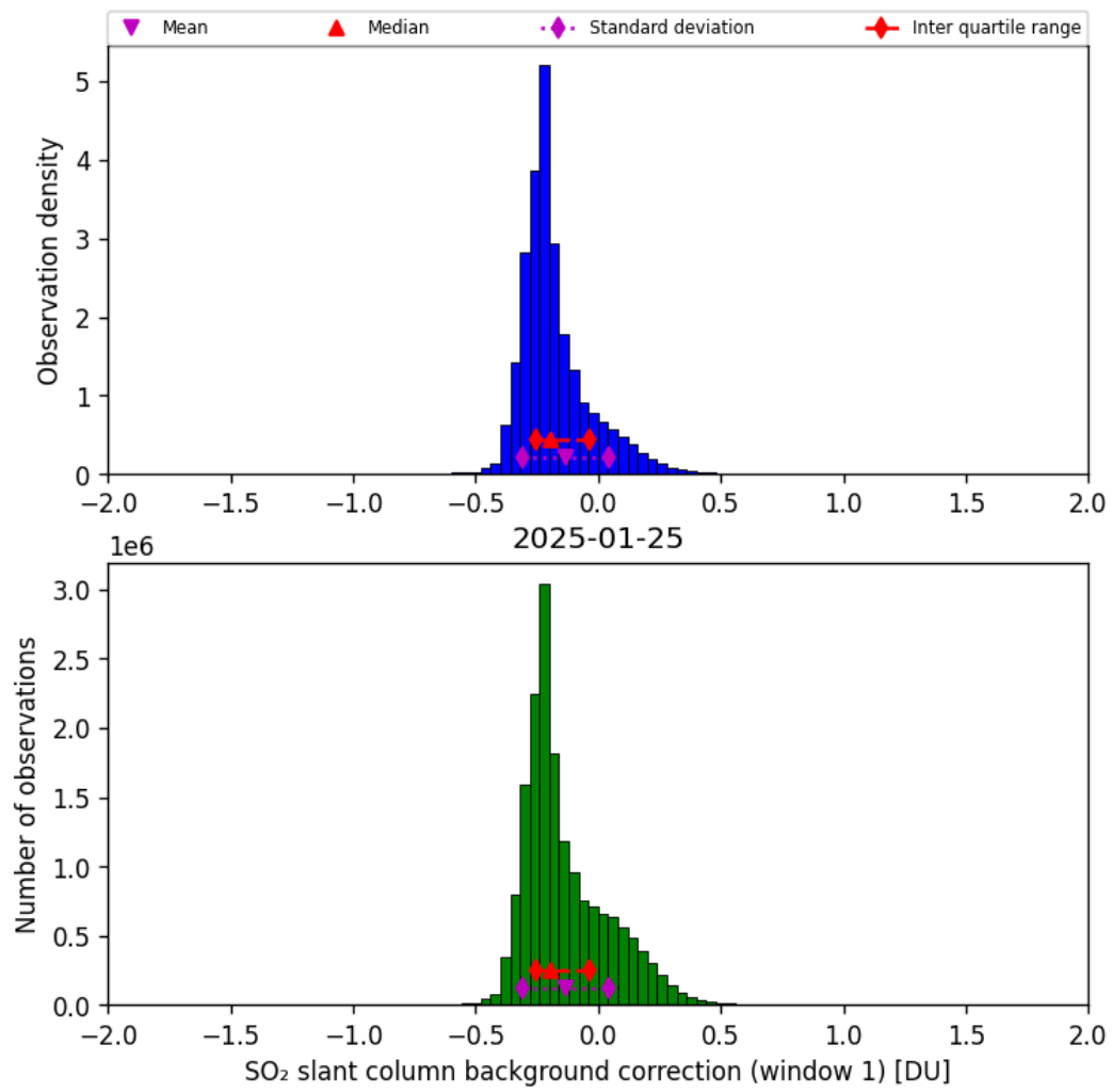
Figure 66: Histogram of “SO 2 slant column background correction (window 1)” for 2025-01-25 to 2025-01-26
