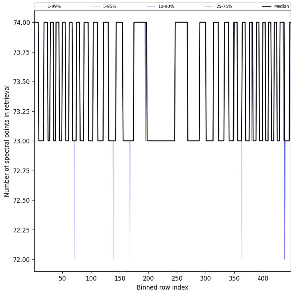
Figure 110: Along track statistics of “Number of spectral points in retrieval” for 2025-01-25 to 2025-01-26
