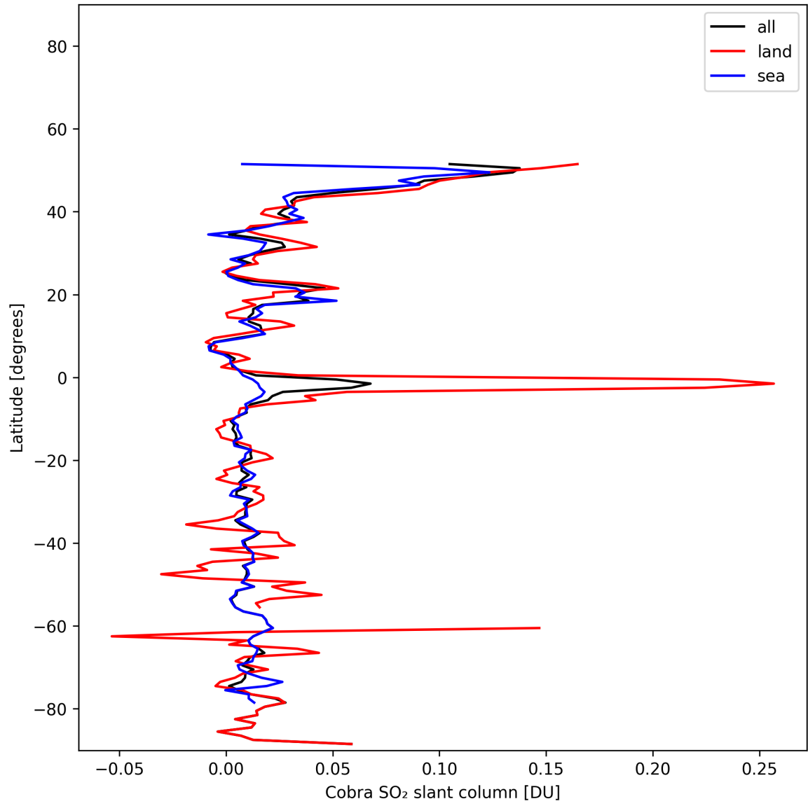
Figure 34: Zonal average of “Cobra SO 2 slant column” for 2025-01-25 to 2025-01-26.
