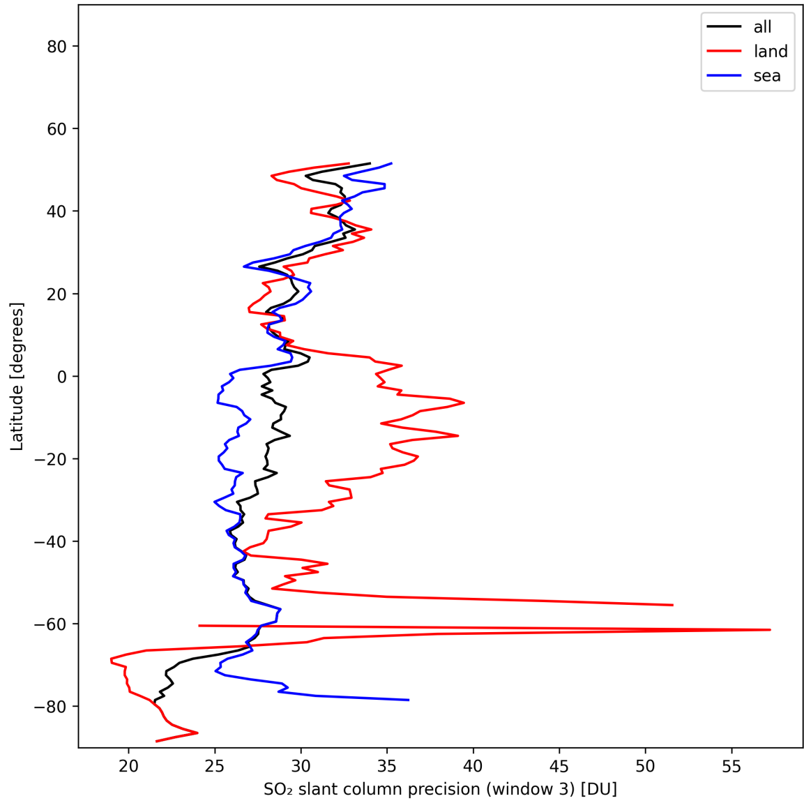
Figure 45: Zonal average of “SO 2 slant column precision (window 3)” for 2025-01-25 to 2025-01-26.
