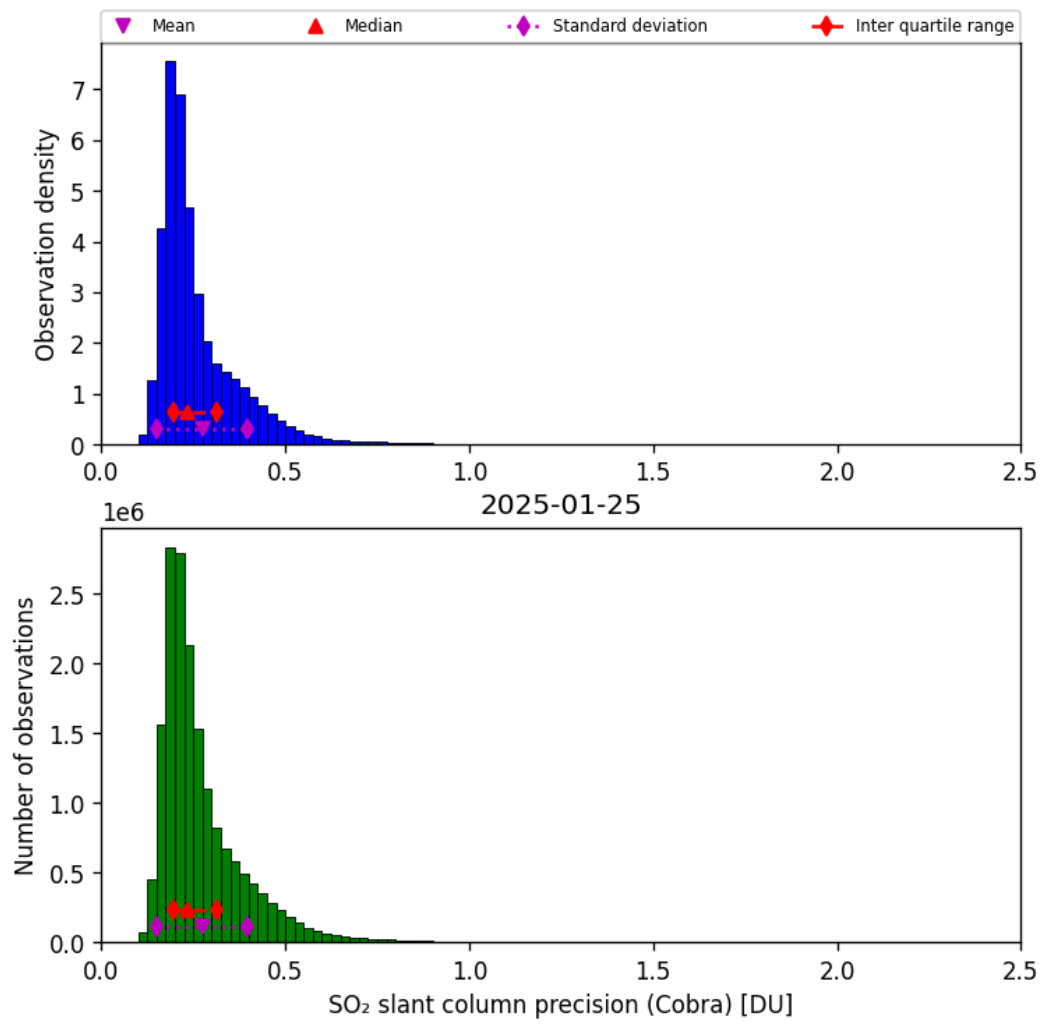
Figure 62: Histogram of “SO 2 slant column precision (Cobra)” for 2025-01-25 to 2025-01-26
