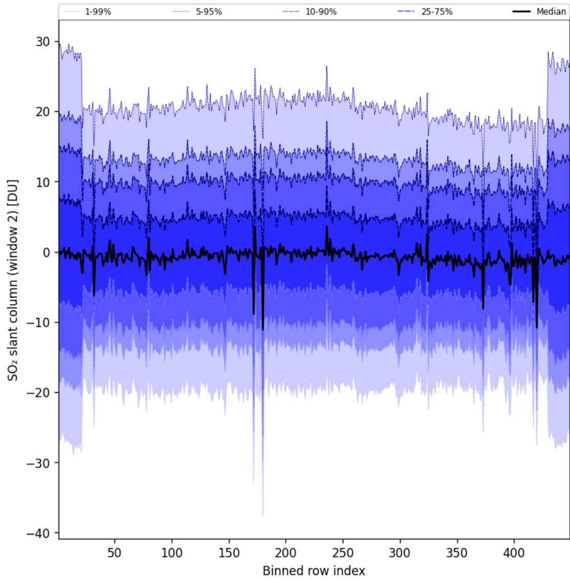
Figure 94: Along track statistics of “SO 2 slant column (window 2)” for 2025-01-25 to 2025-01-26
