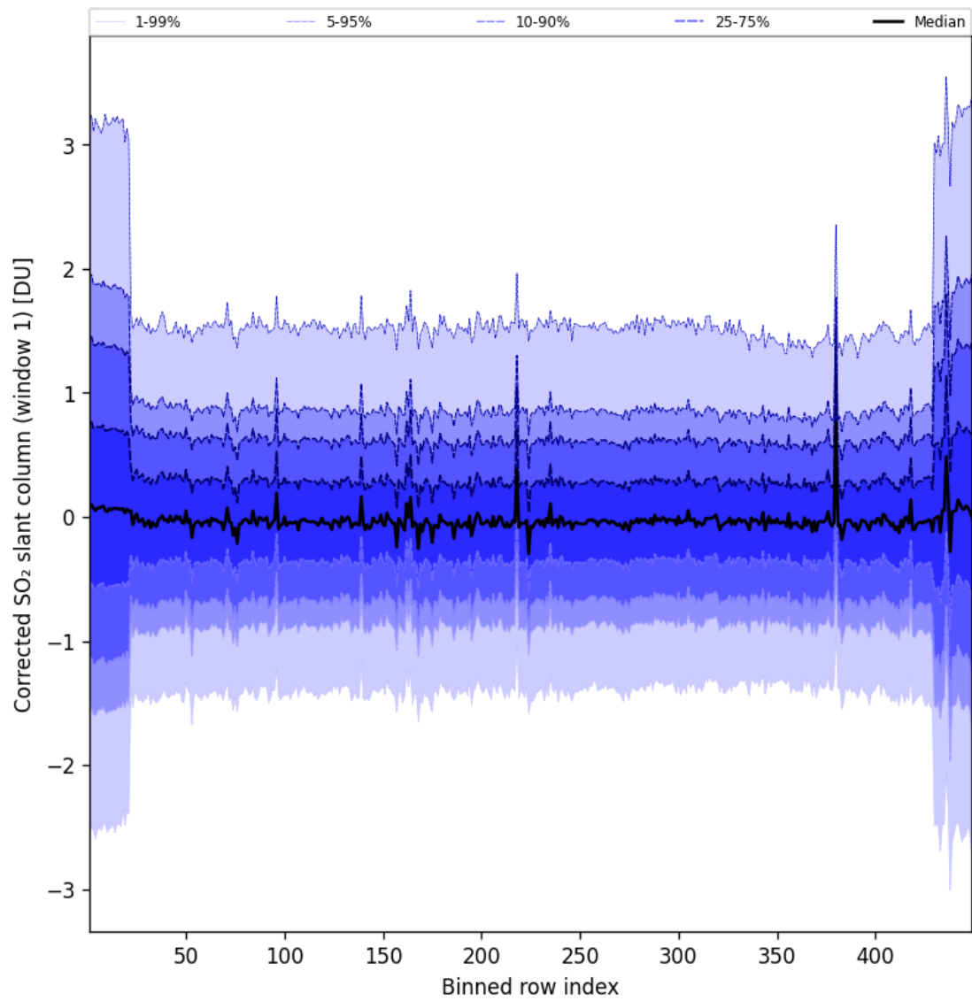
Figure 92: Along track statistics of “Corrected SO 2 slant column (window 1)” for 2025-01-25 to 2025-01-26
