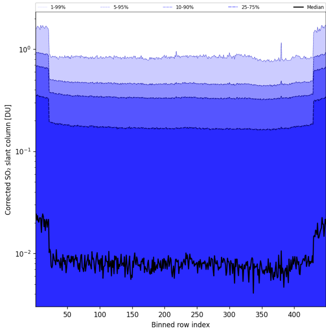
Figure 87: Along track statistics of “Corrected SO 2 slant column” for 2025-01-25 to 2025-01-26
