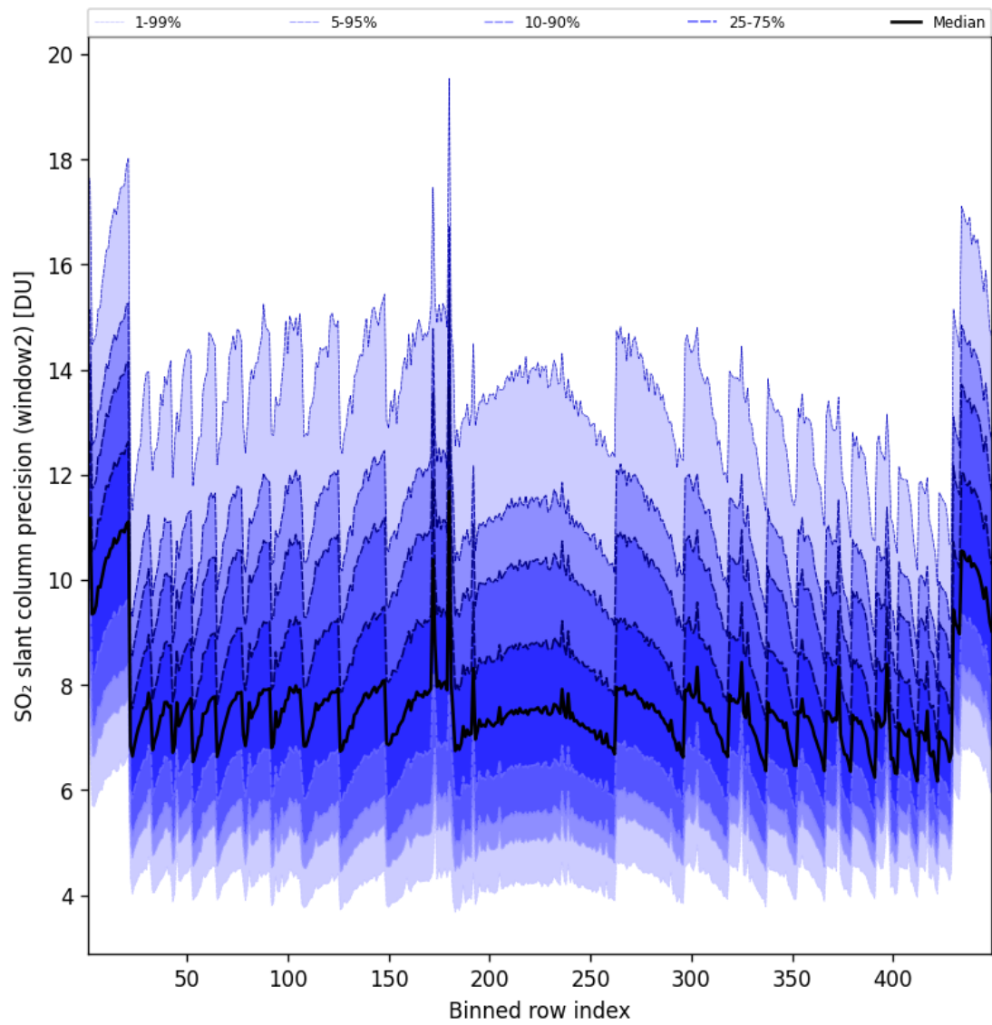
Figure 95: Along track statistics of “SO 2 slant column precision (window2)” for 2025-01-25 to 2025-01-26
