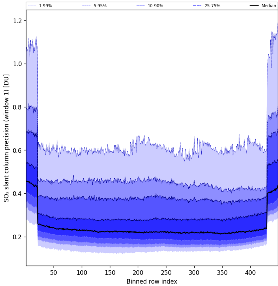
Figure 91: Along track statistics of “SO 2 slant column precision (window 1)” for 2025-01-25 to 2025-01-26
