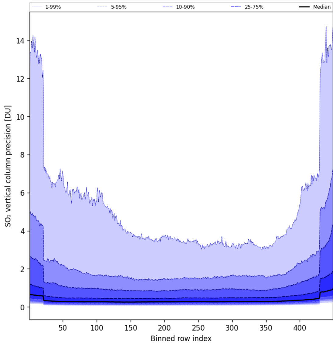
Figure 86: Along track statistics of “SO 2 vertical column precision” for 2025-01-25 to 2025-01-26
