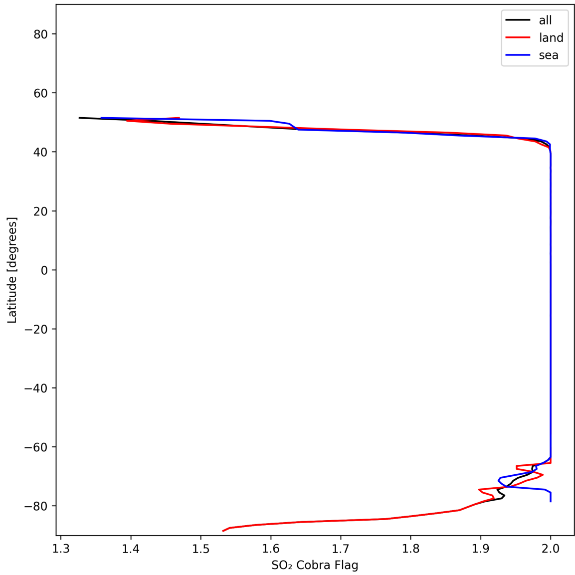
Figure 48: Zonal average of "SO 2 Cobra Flag" for 2025-01-25 to 2025-01-26.
