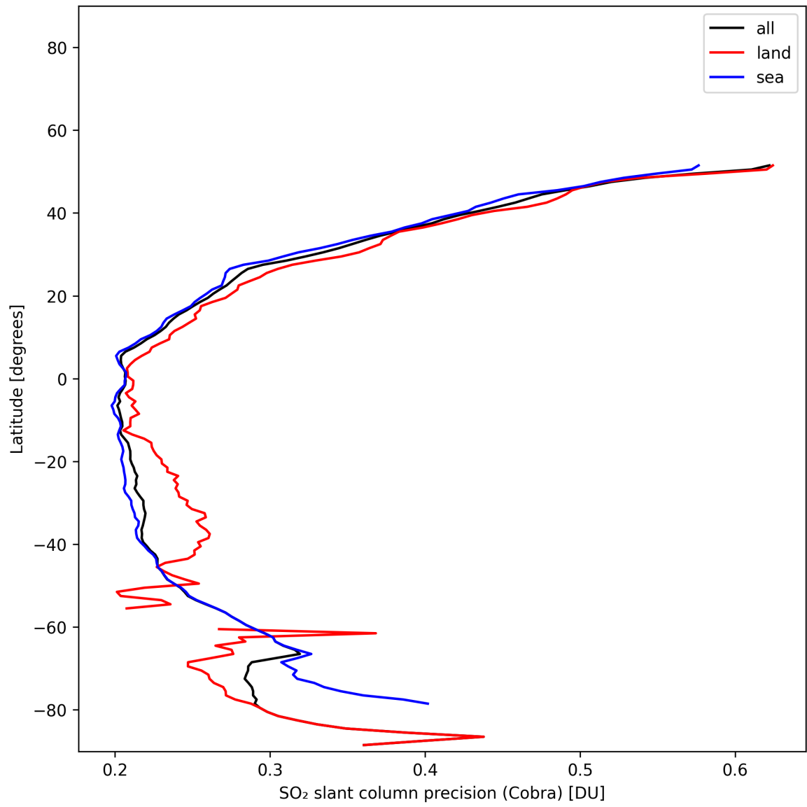
Figure 35: Zonal average of “SO 2 slant column precision (Cobra)” for 2025-01-25 to 2025-01-26.
