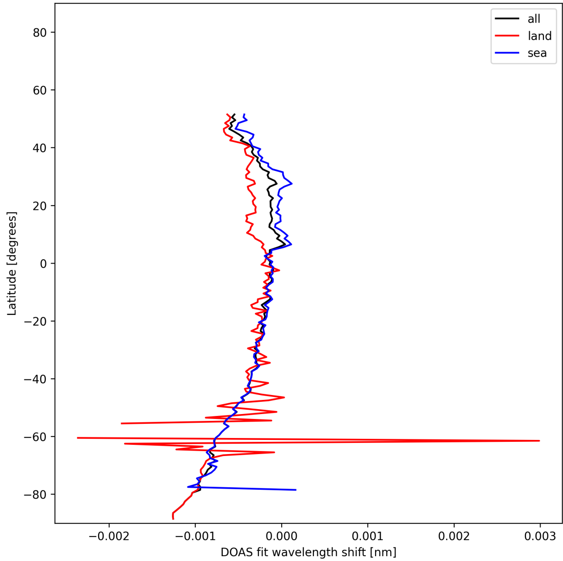
Figure 50: Zonal average of “DOAS fit wavelength shift” for 2025-01-25 to 2025-01-26.
