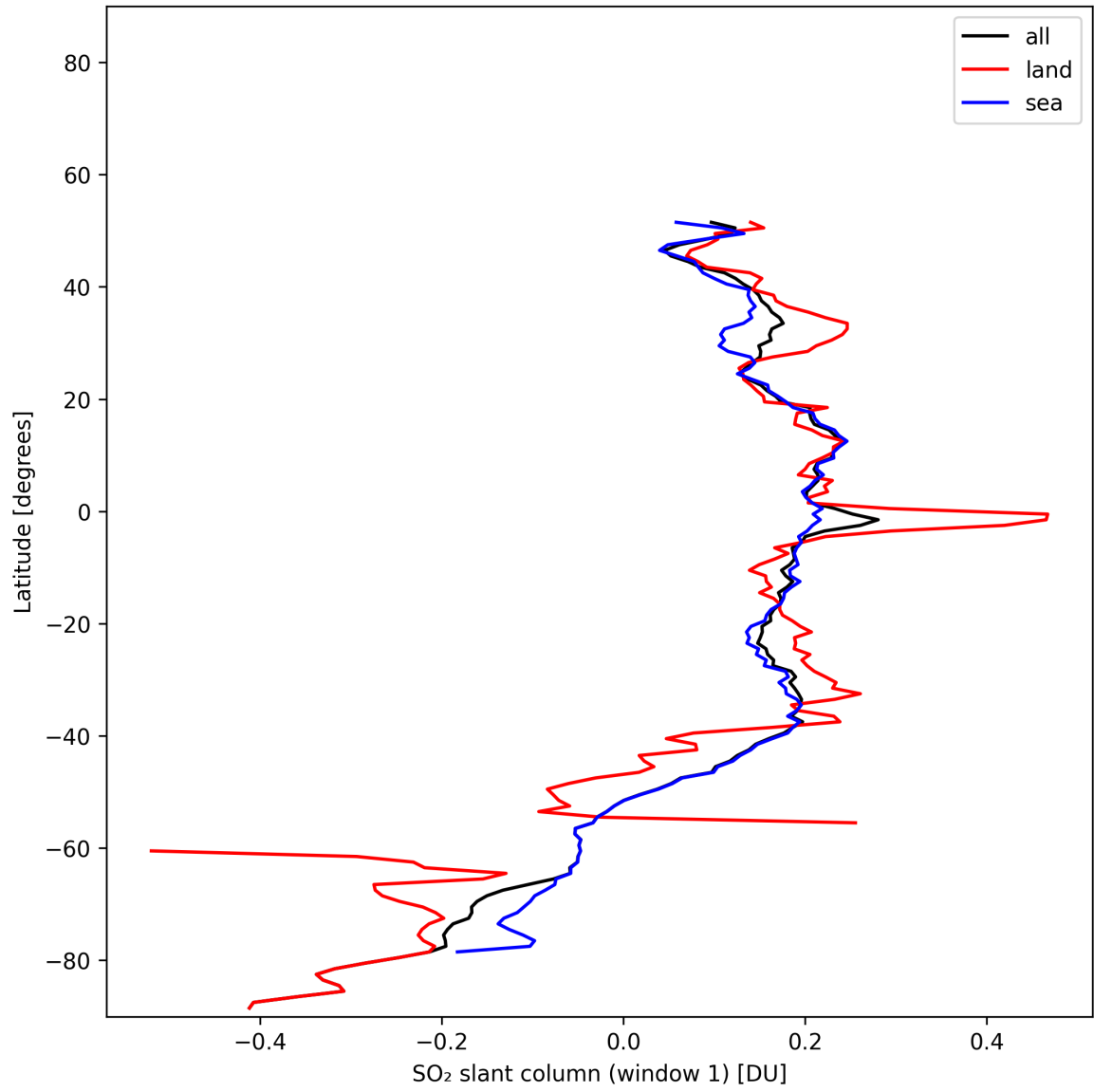
Figure 36: Zonal average of “SO 2 slant column (window 1)” for 2025-01-26 to 2025-01-26.
