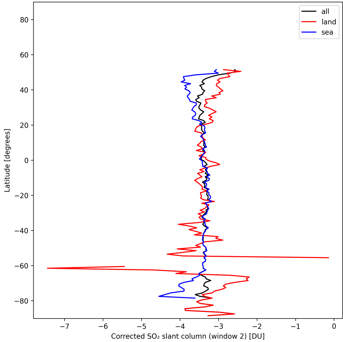
Figure 42: Zonal average of “Corrected SO 2 slant column (window 2)” for 2025-01-26 to 2025-01-26.
