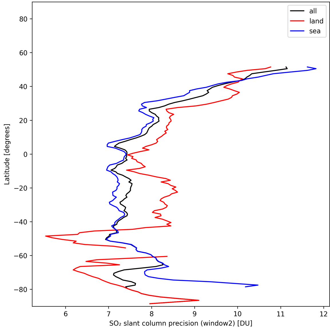
Figure 41: Zonal average of “SO 2 slant column precision (window2)” for 2025-01-26 to 2025-01-26.
