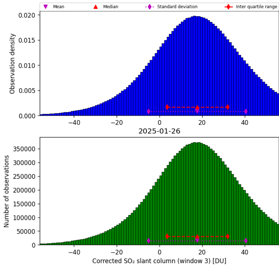
Figure 73: Histogram of “Corrected SO 2 slant column (window 3)” for 2025-01-26 to 2025-01-26
