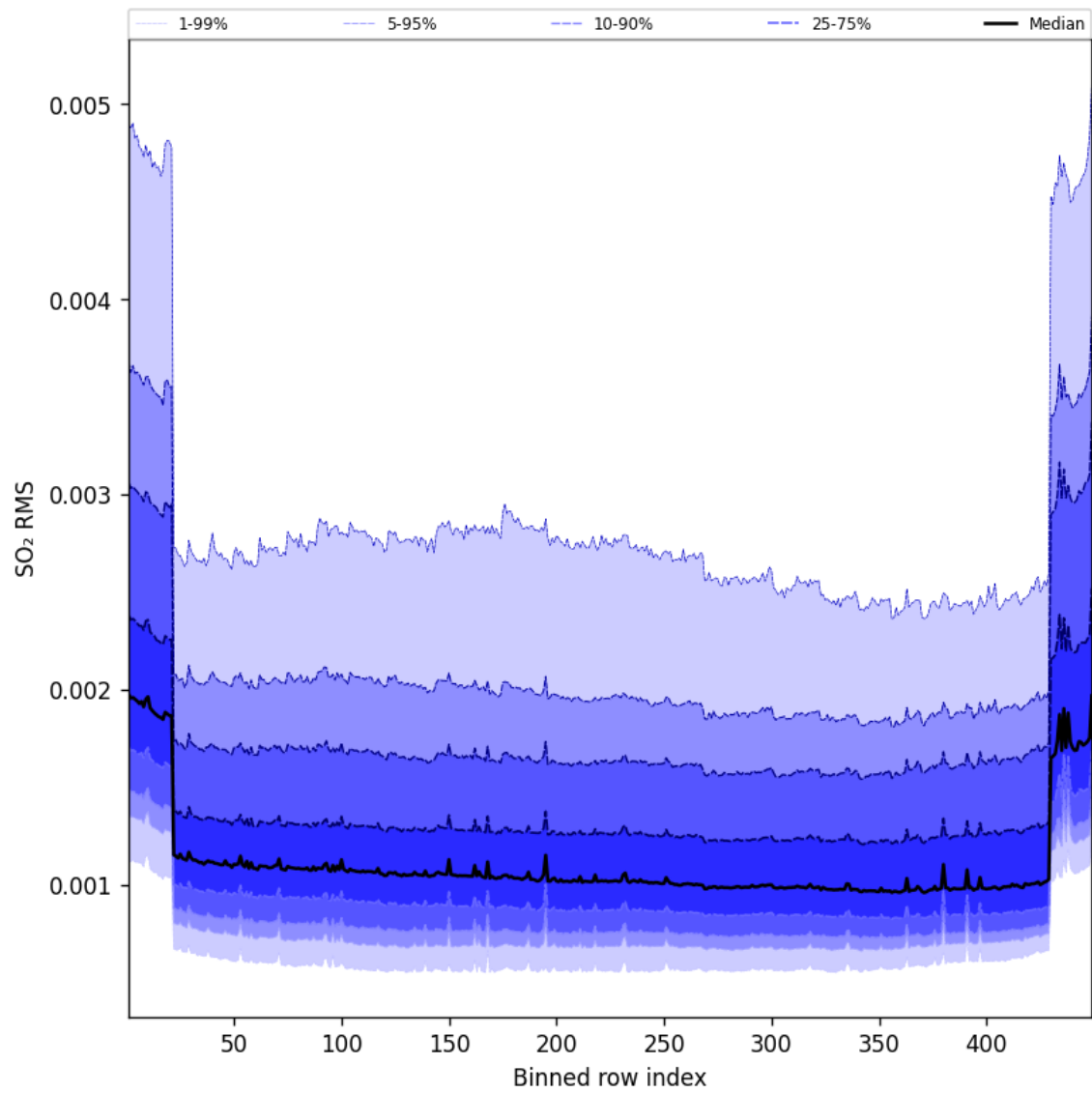
Figure 106: Along track statistics of “SO 2 RMS” for 2025-01-26 to 2025-01-26
