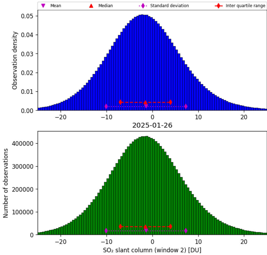
Figure 67: Histogram of “SO 2 slant column (window 2)” for 2025-01-26 to 2025-01-26
