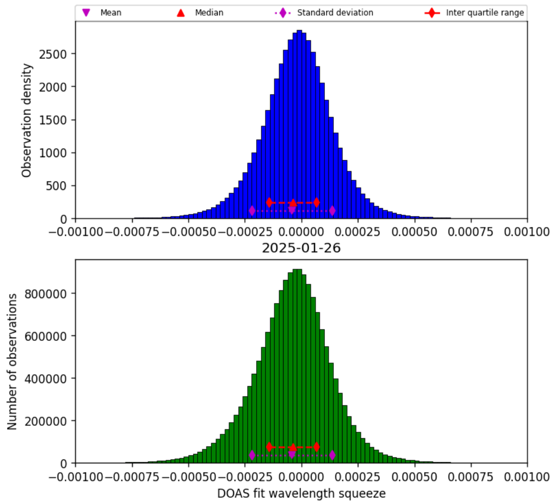
Figure 78: Histogram of “DOAS fit wavelength squeeze” for 2025-01-26 to 2025-01-26
