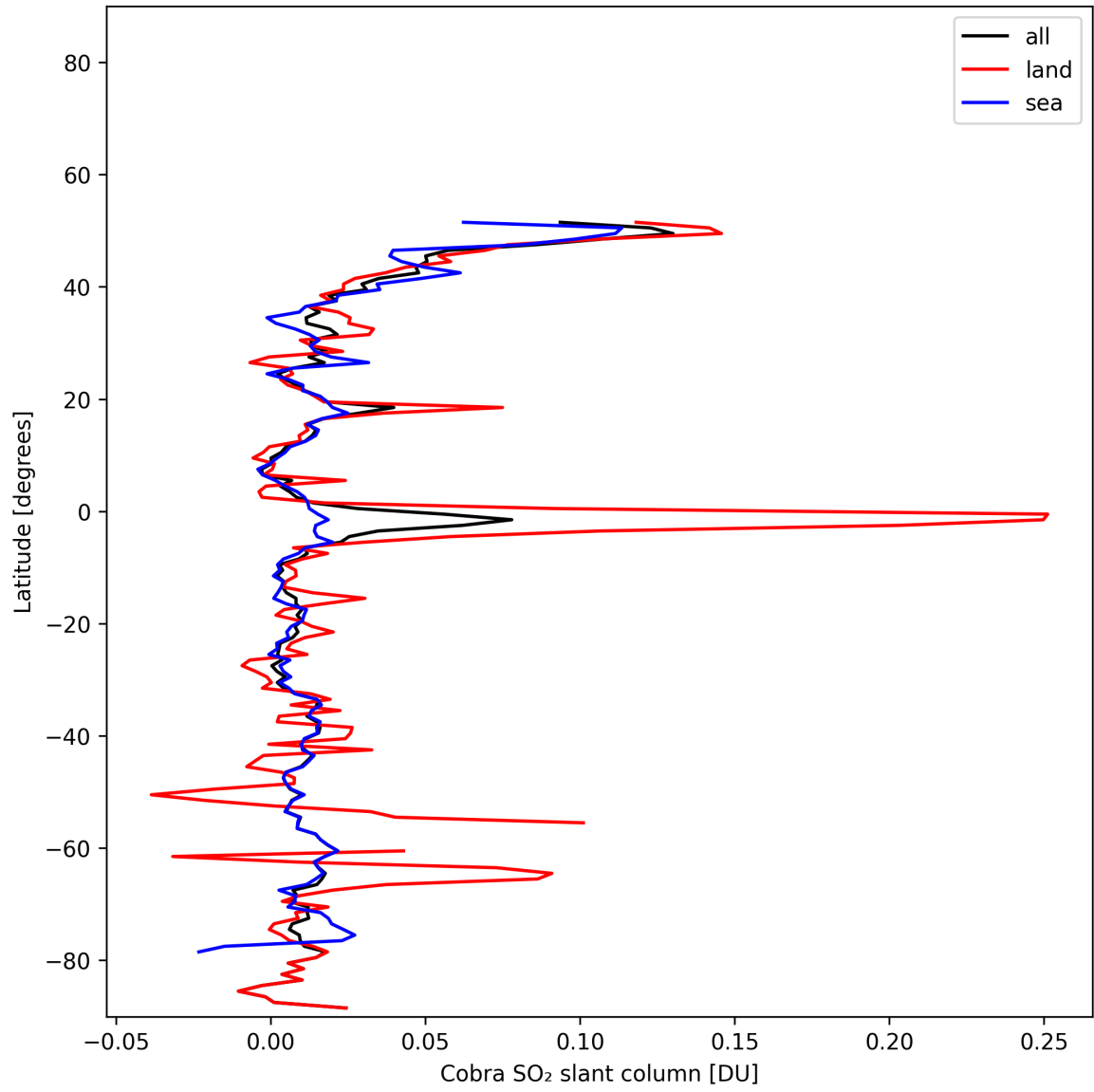
Figure 34: Zonal average of “Cobra SO 2 slant column” for 2025-01-26 to 2025-01-26.
