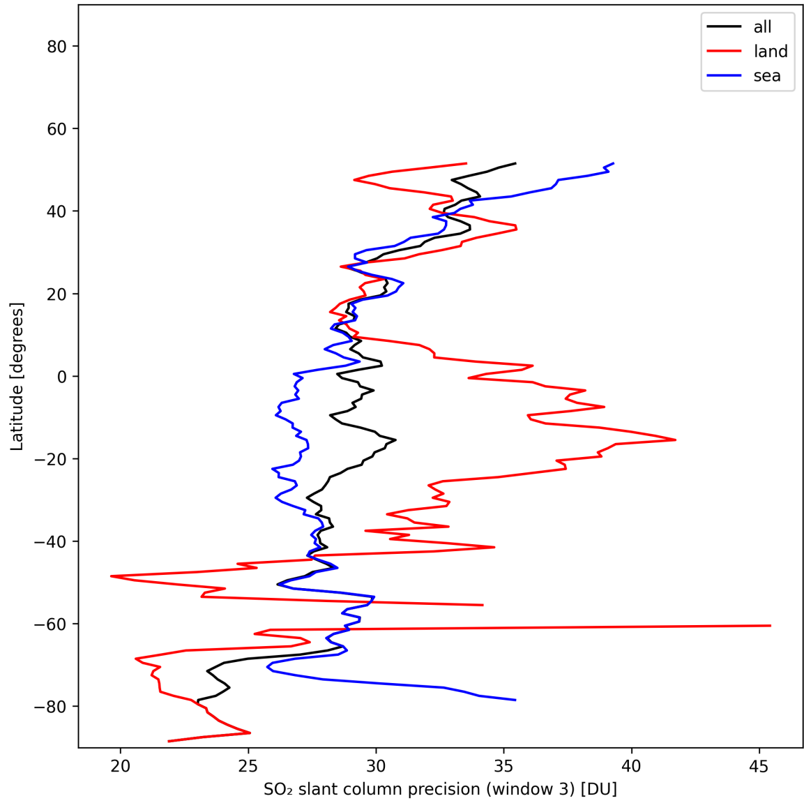
Figure 45: Zonal average of “SO 2 slant column precision (window 3)” for 2025-01-26 to 2025-01-26.
