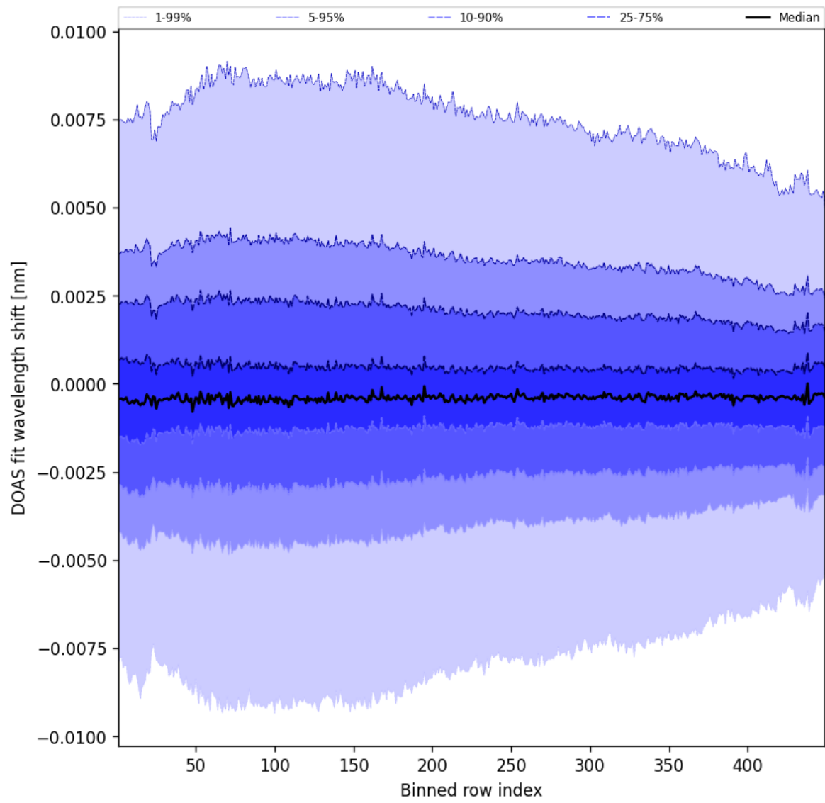
Figure 104: Along track statistics of “DOAS fit wavelength shift” for 2025-01-26 to 2025-01-26
