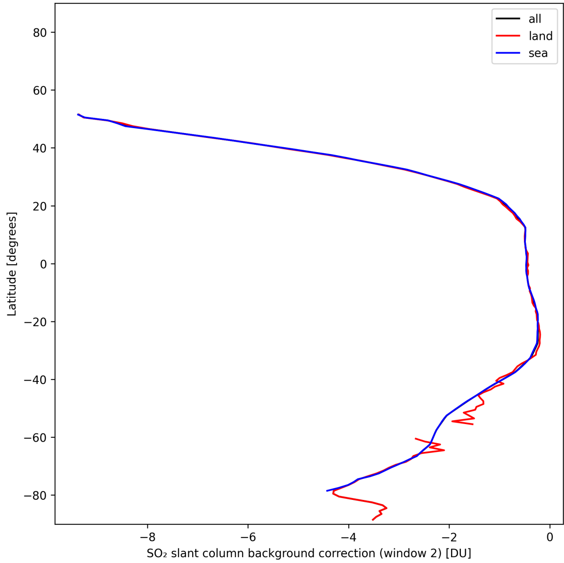
Figure 43: Zonal average of “SO 2 slant column background correction (window 2)” for 2025-01-26 to 2025-01-26.
