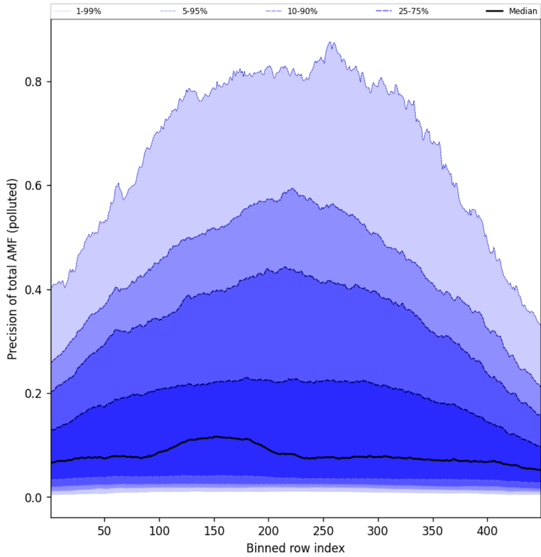
Figure 108: Along track statistics of “Precision of total AMF (polluted)” for 2025-01-26 to 2025-01-26
