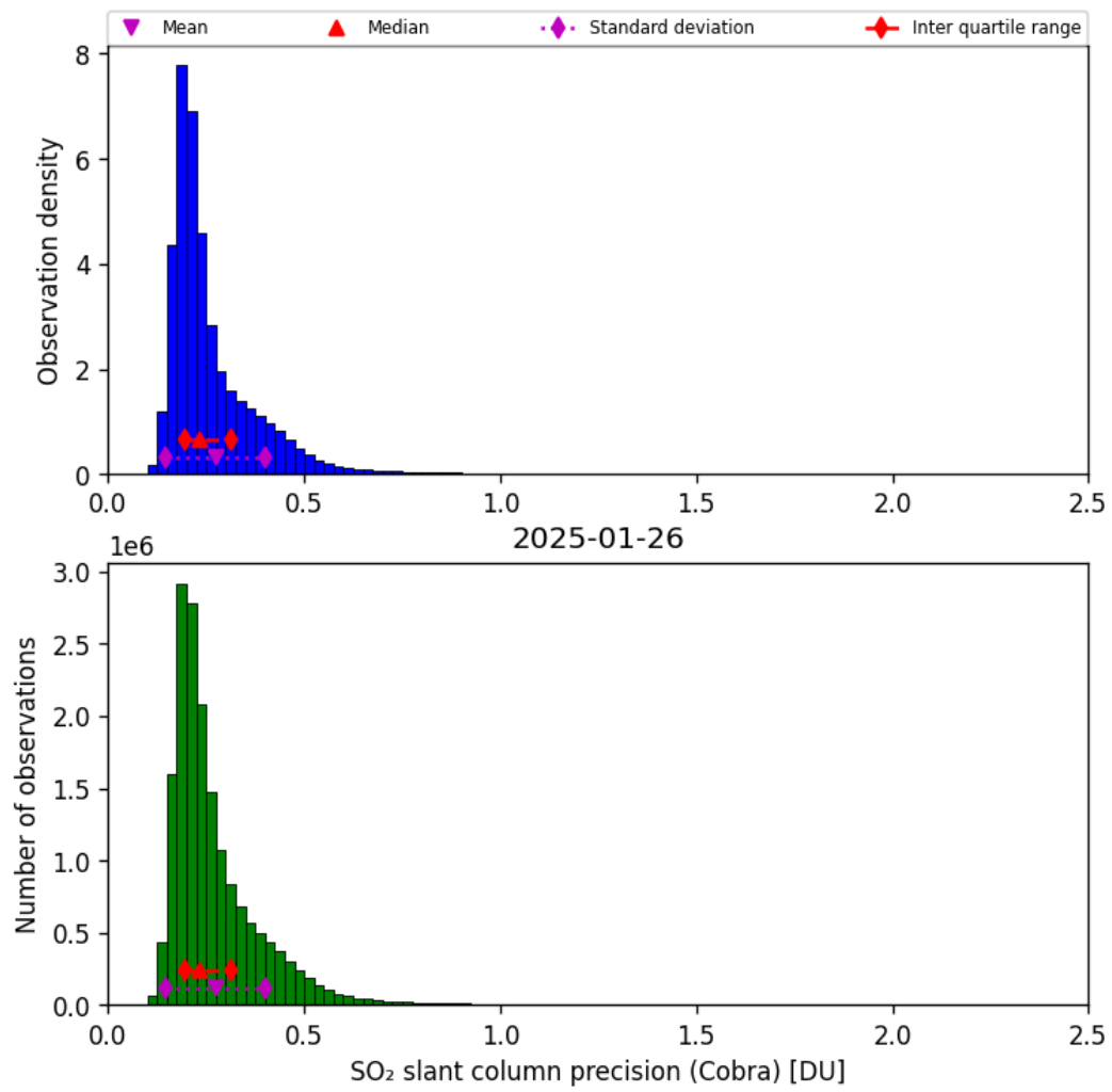
Figure 62: Histogram of “SO 2 slant column precision (Cobra)” for 2025-01-26 to 2025-01-26
