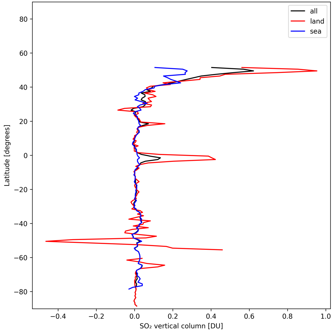
Figure 31: Zonal average of “SO 2 vertical column” for 2025-01-26 to 2025-01-26.
