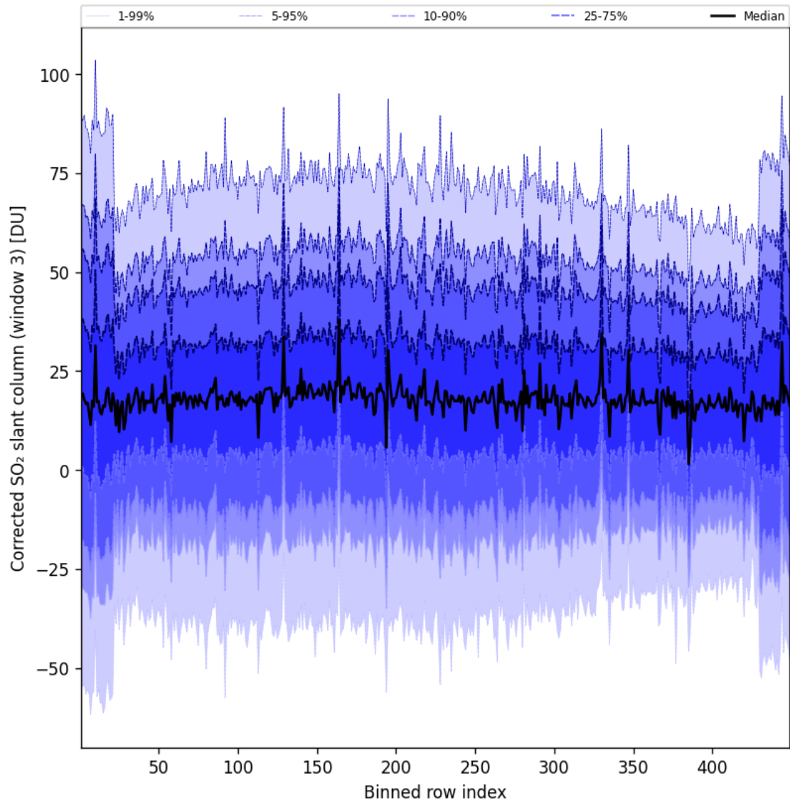
Figure 100: Along track statistics of “Corrected SO 2 slant column (window 3)” for 2025-01-26 to 2025-01-26
