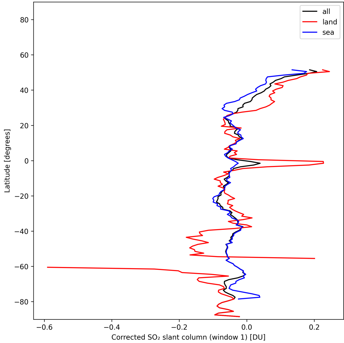
Figure 38: Zonal average of “Corrected SO 2 slant column (window 1)” for 2025-01-26 to 2025-01-26.
