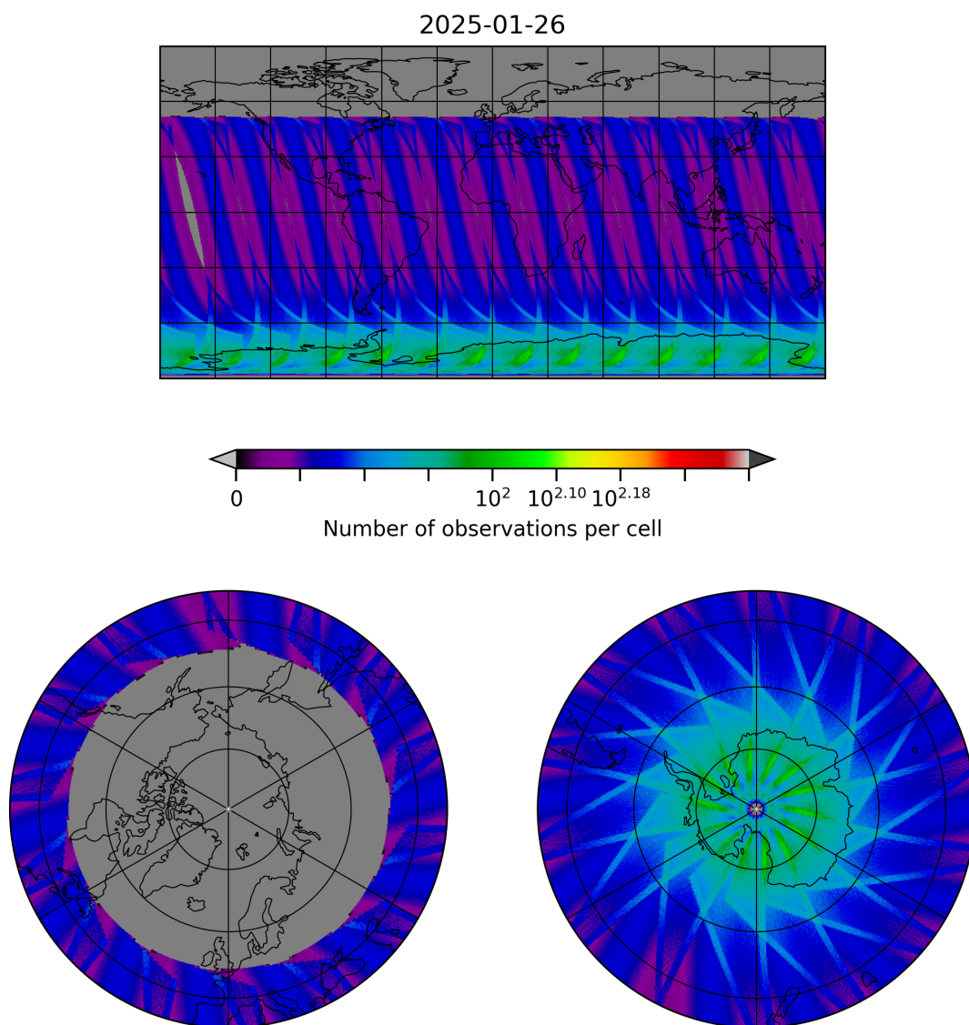
Figure 29: Map of the number of observations for 2025-01-26 to 2025-01-26
