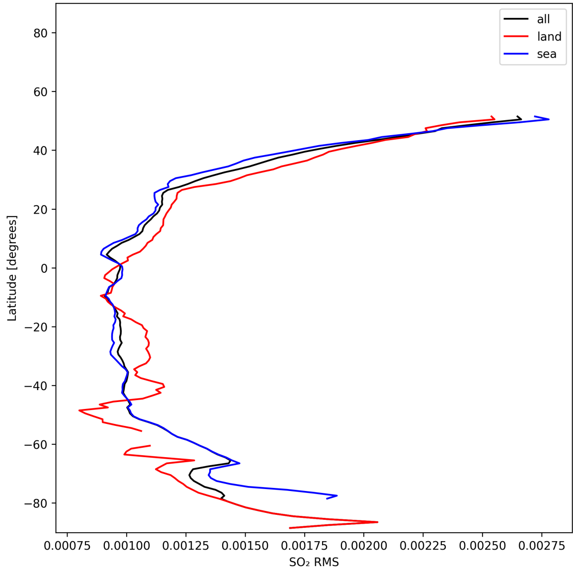
Figure 52: Zonal average of “SO 2 RMS” for 2025-01-26 to 2025-01-26.
