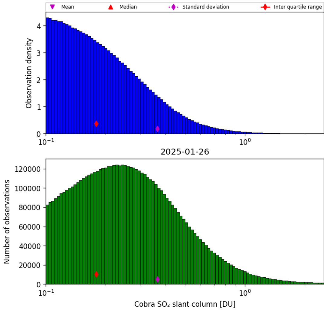
Figure 61: Histogram of “Cobra SO 2 slant column” for 2025-01-26 to 2025-01-26
