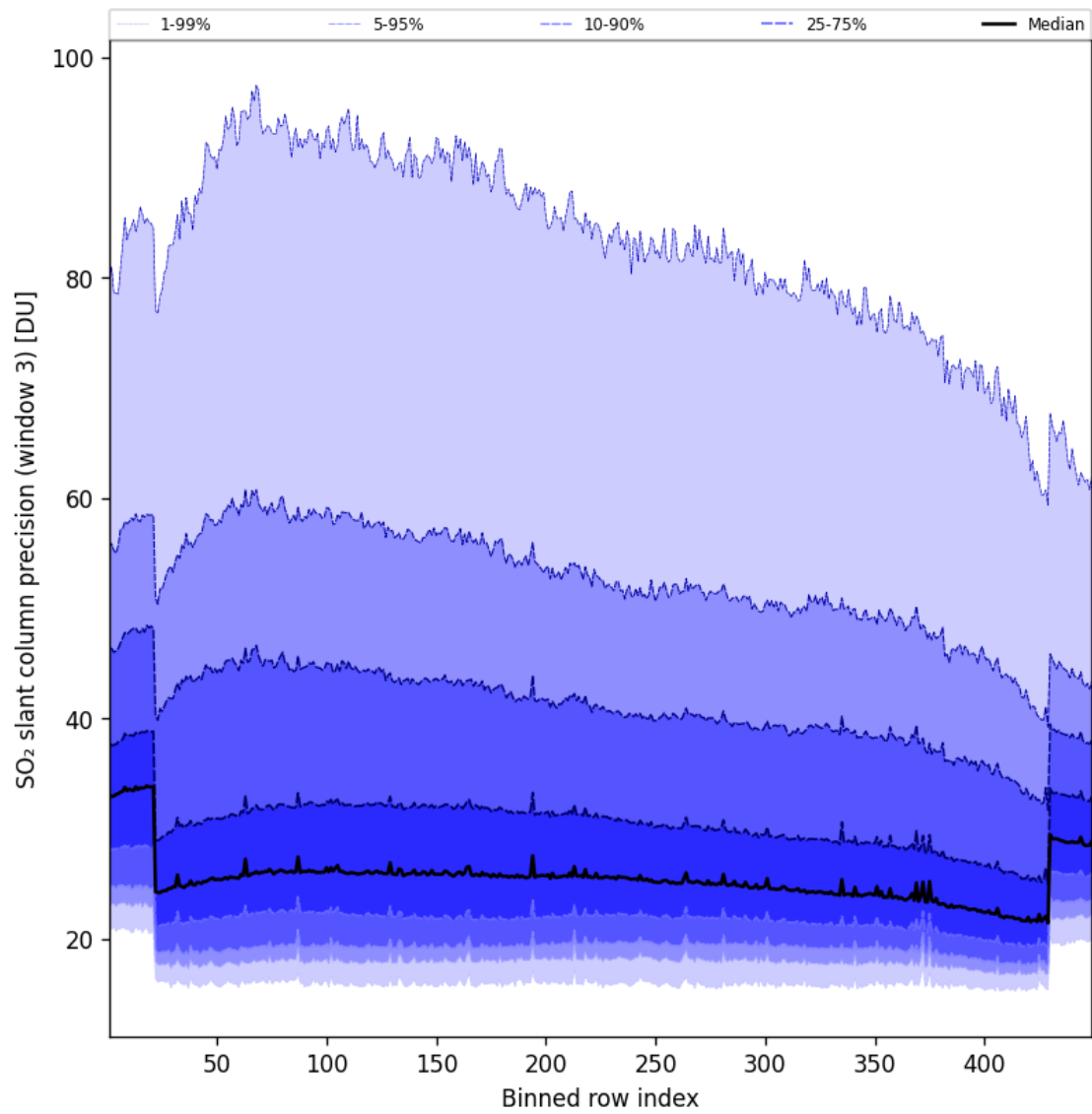
Figure 99: Along track statistics of “SO 2 slant column precision (window 3)” for 2025-01-26 to 2025-01-26
