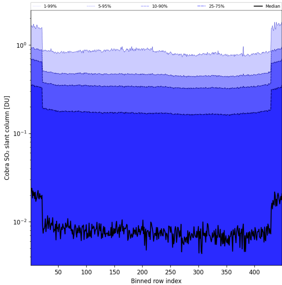
Figure 88: Along track statistics of “Cobra SO 2 slant column” for 2025-01-26 to 2025-01-26
