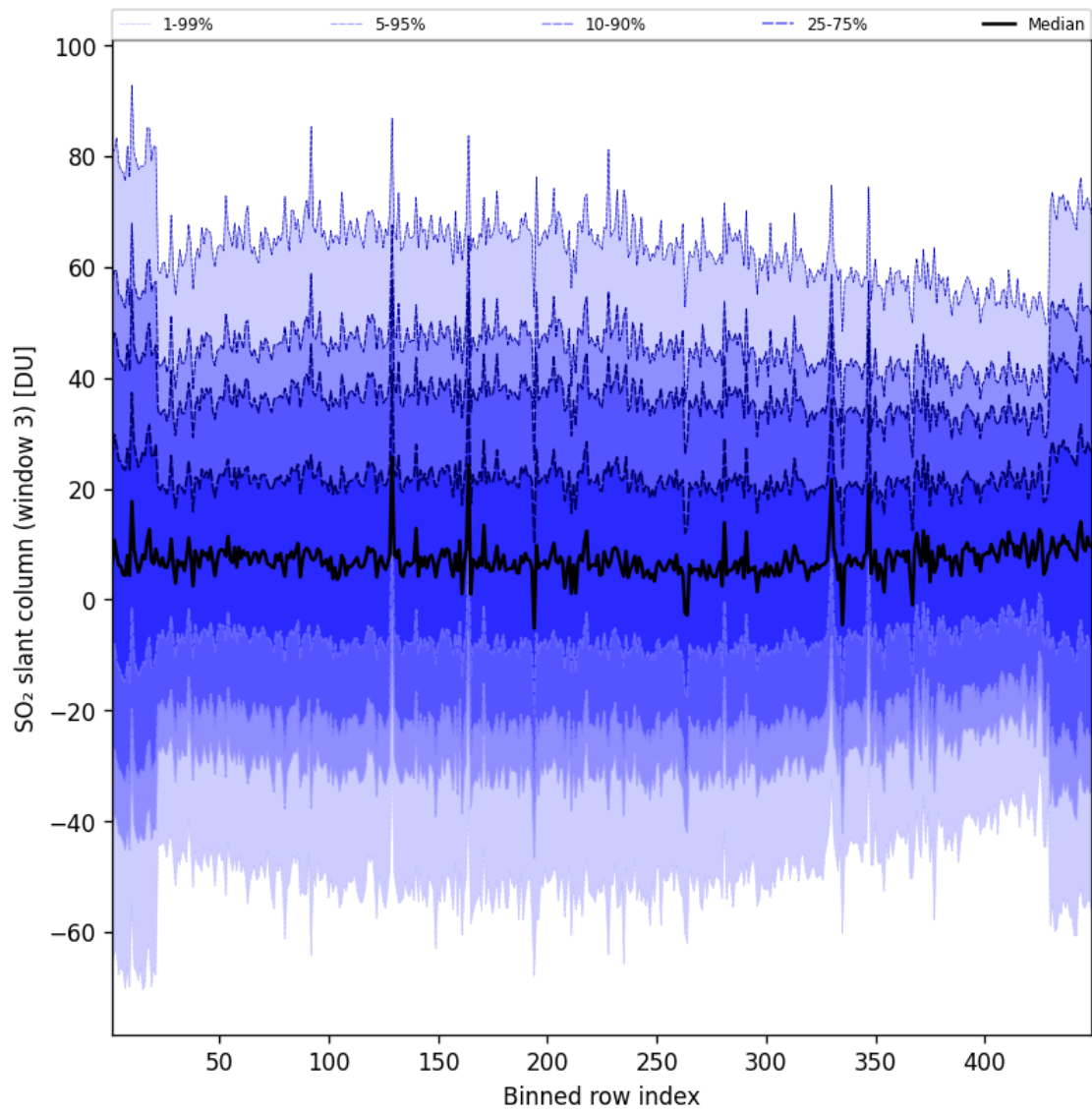
Figure 98: Along track statistics of “SO 2 slant column (window 3)” for 2025-01-26 to 2025-01-26
