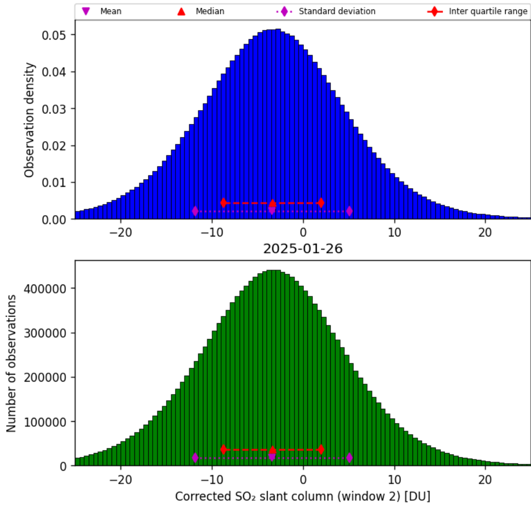
Figure 69: Histogram of “Corrected SO 2 slant column (window 2)” for 2025-01-26 to 2025-01-26
