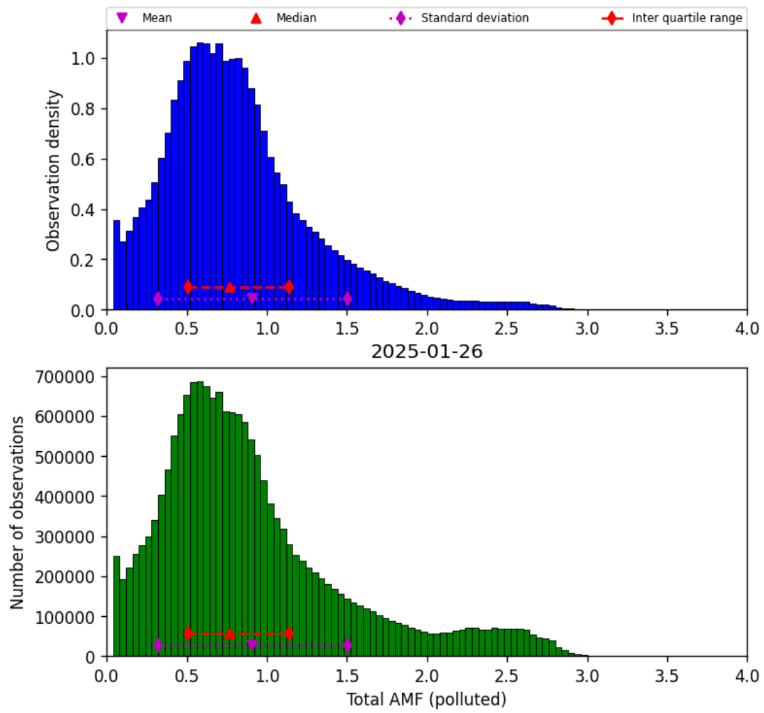
Figure 80: Histogram of “Total AMF (polluted)” for 2025-01-26 to 2025-01-26
