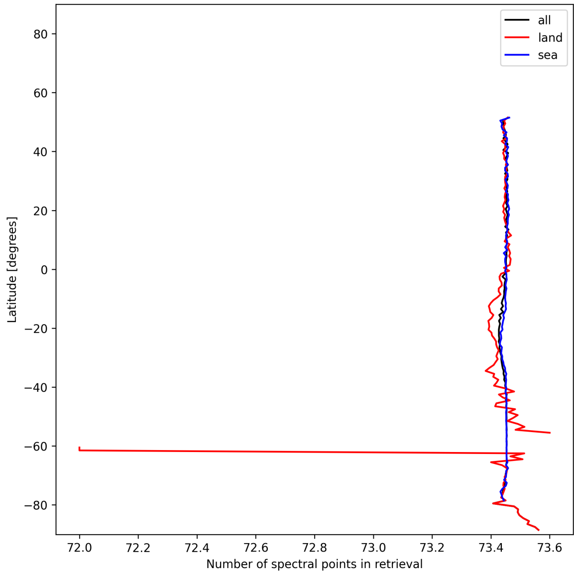
Figure 56: Zonal average of “Number of spectral points in retrieval” for 2025-01-26 to 2025-01-26.
