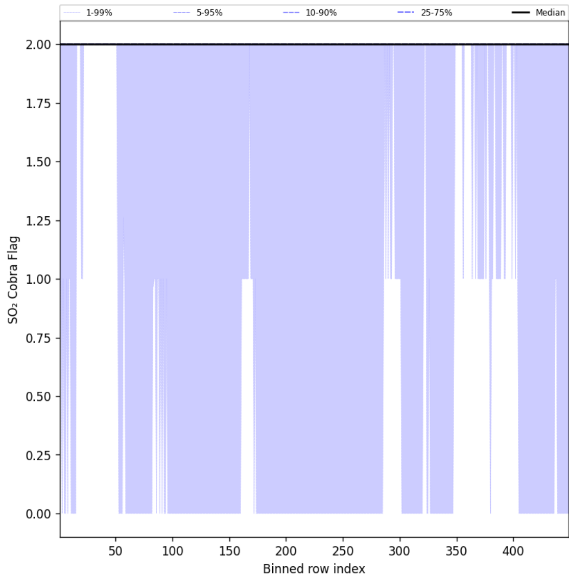
Figure 102: Along track statistics of “SO 2 Cobra Flag” for 2025-01-26 to 2025-01-26
