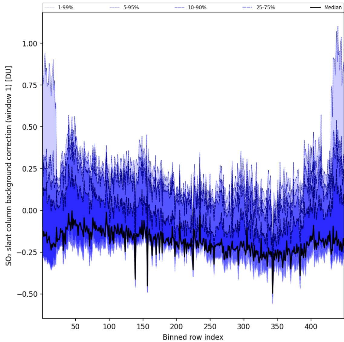
Figure 93: Along track statistics of “SO 2 slant column background correction (window 1)” for 2025-01-26 to 2025-01-26
