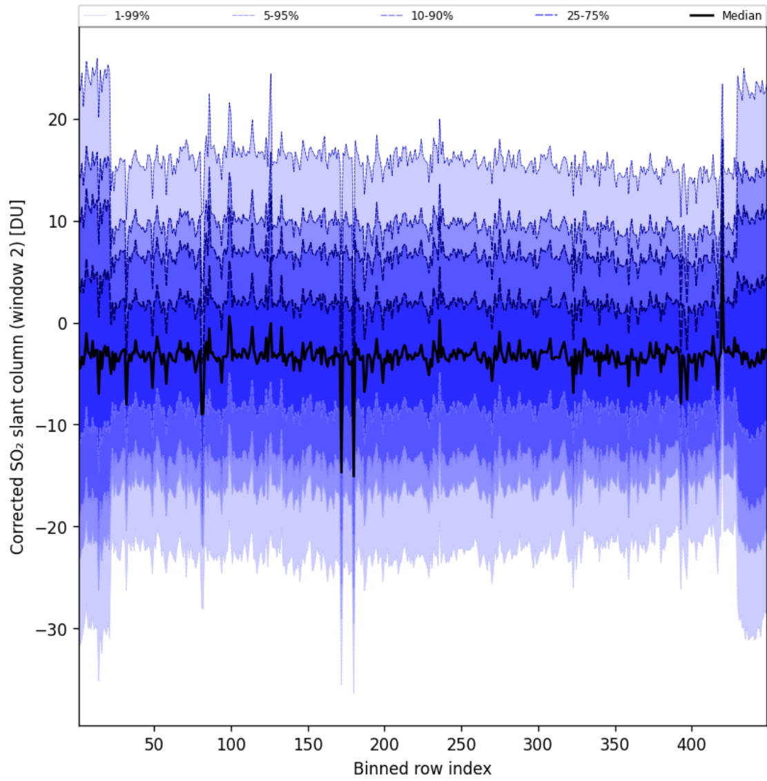
Figure 96: Along track statistics of “Corrected SO 2 slant column (window 2)” for 2025-01-26 to 2025-01-26
