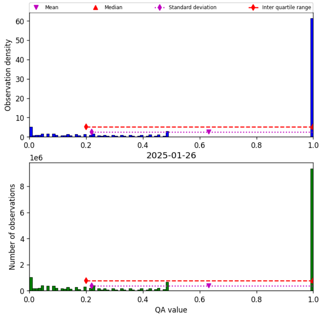
Figure 57: Histogram of “QA value” for 2025-01-26 to 2025-01-26
