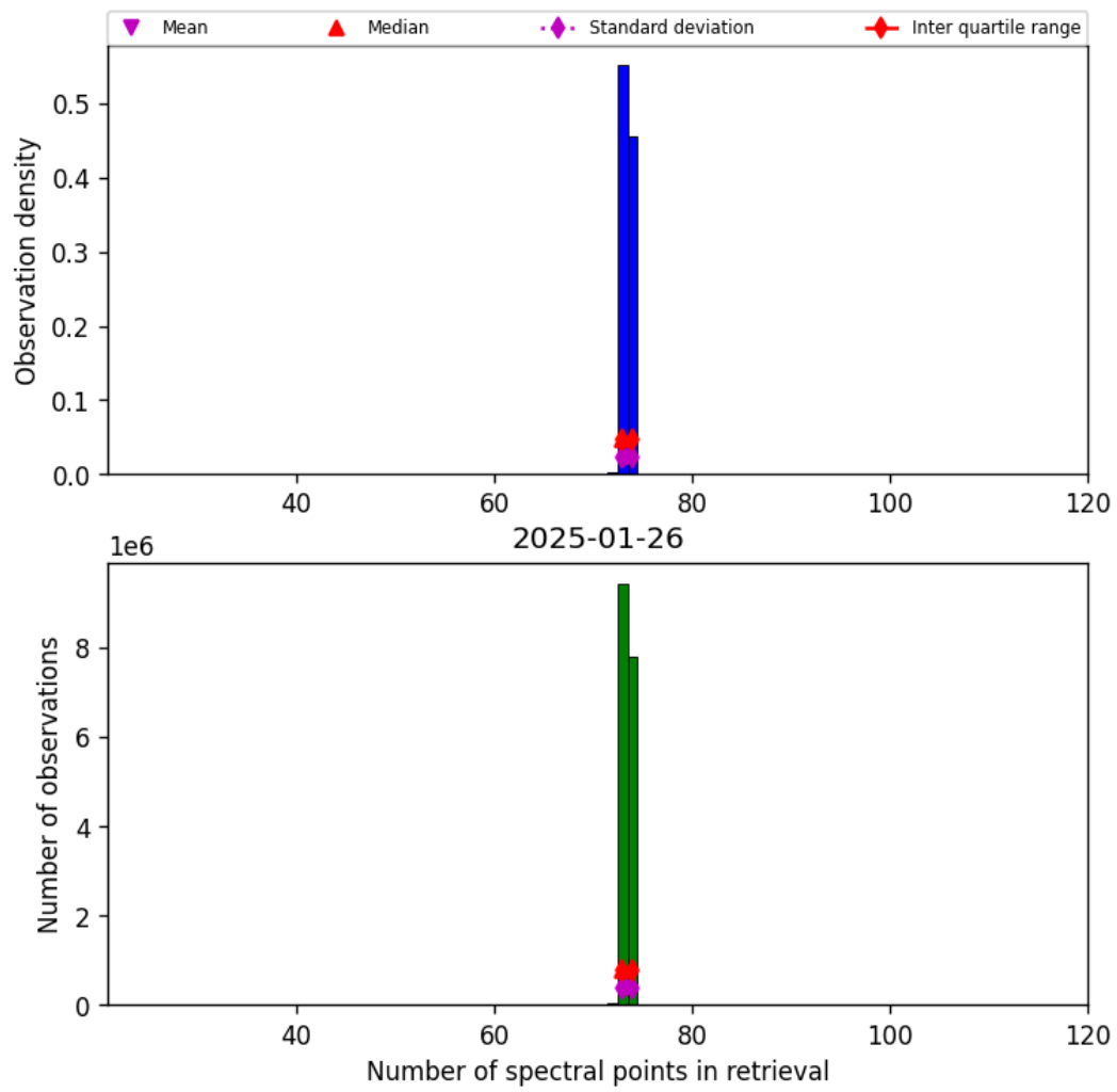
Figure 83: Histogram of “Number of spectral points in retrieval” for 2025-01-26 to 2025-01-26
