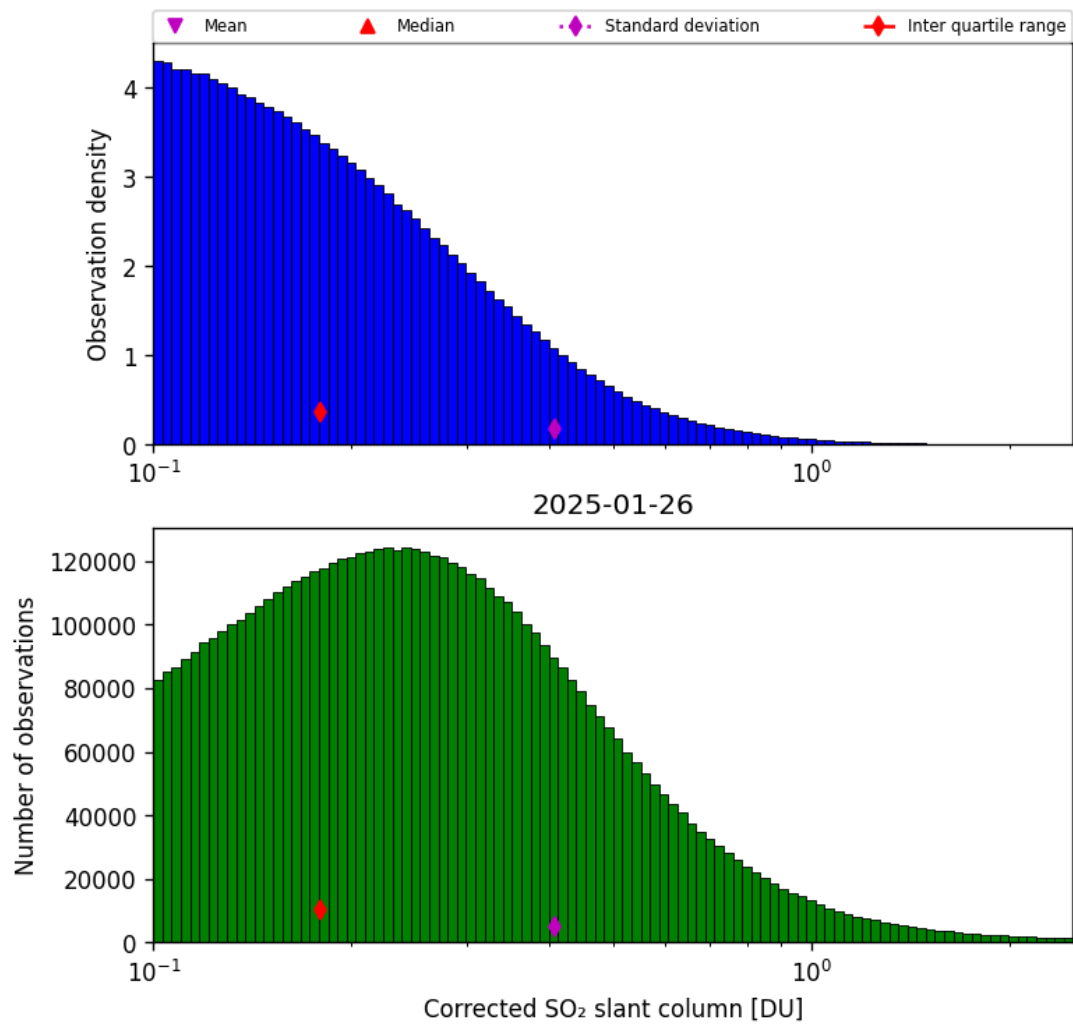
Figure 60: Histogram of “Corrected SO 2 slant column” for 2025-01-26 to 2025-01-26
