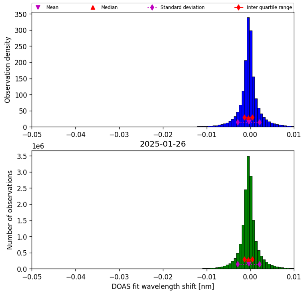
Figure 77: Histogram of “DOAS fit wavelength shift” for 2025-01-26 to 2025-01-26
