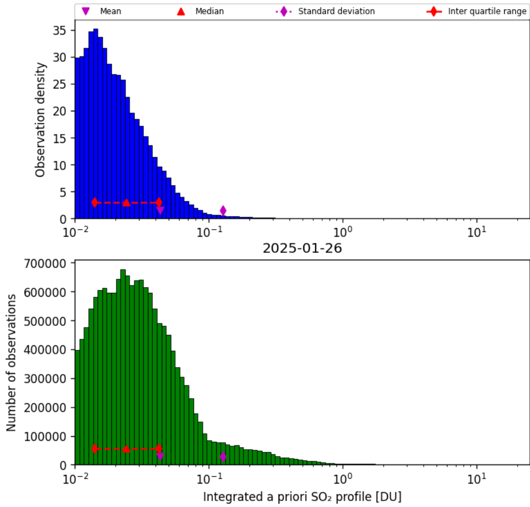
Figure 76: Histogram of “Integrated a priori SO 2 profile” for 2025-01-26 to 2025-01-26
