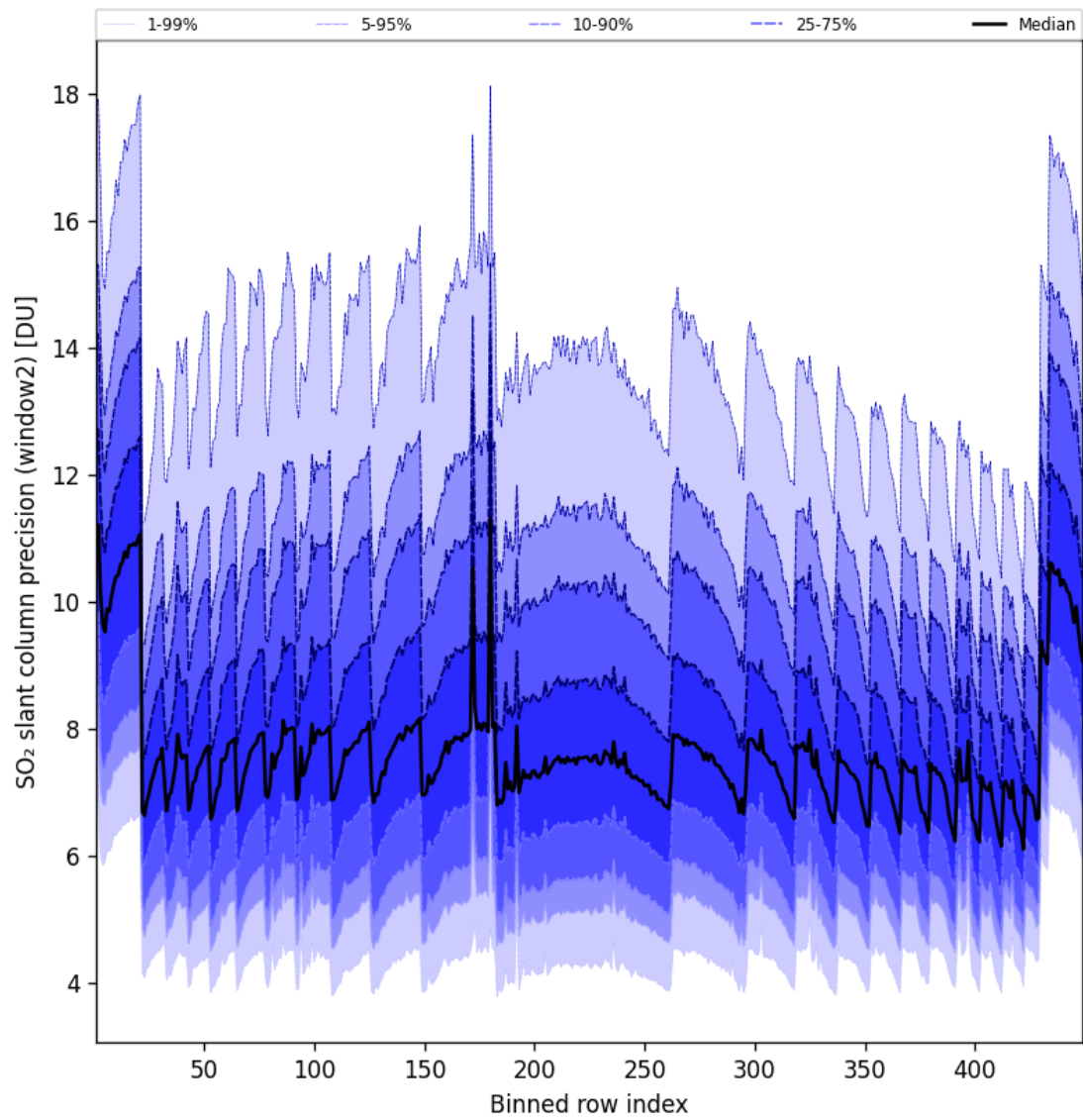
Figure 95: Along track statistics of “SO 2 slant column precision (window2)” for 2025-01-26 to 2025-01-26
