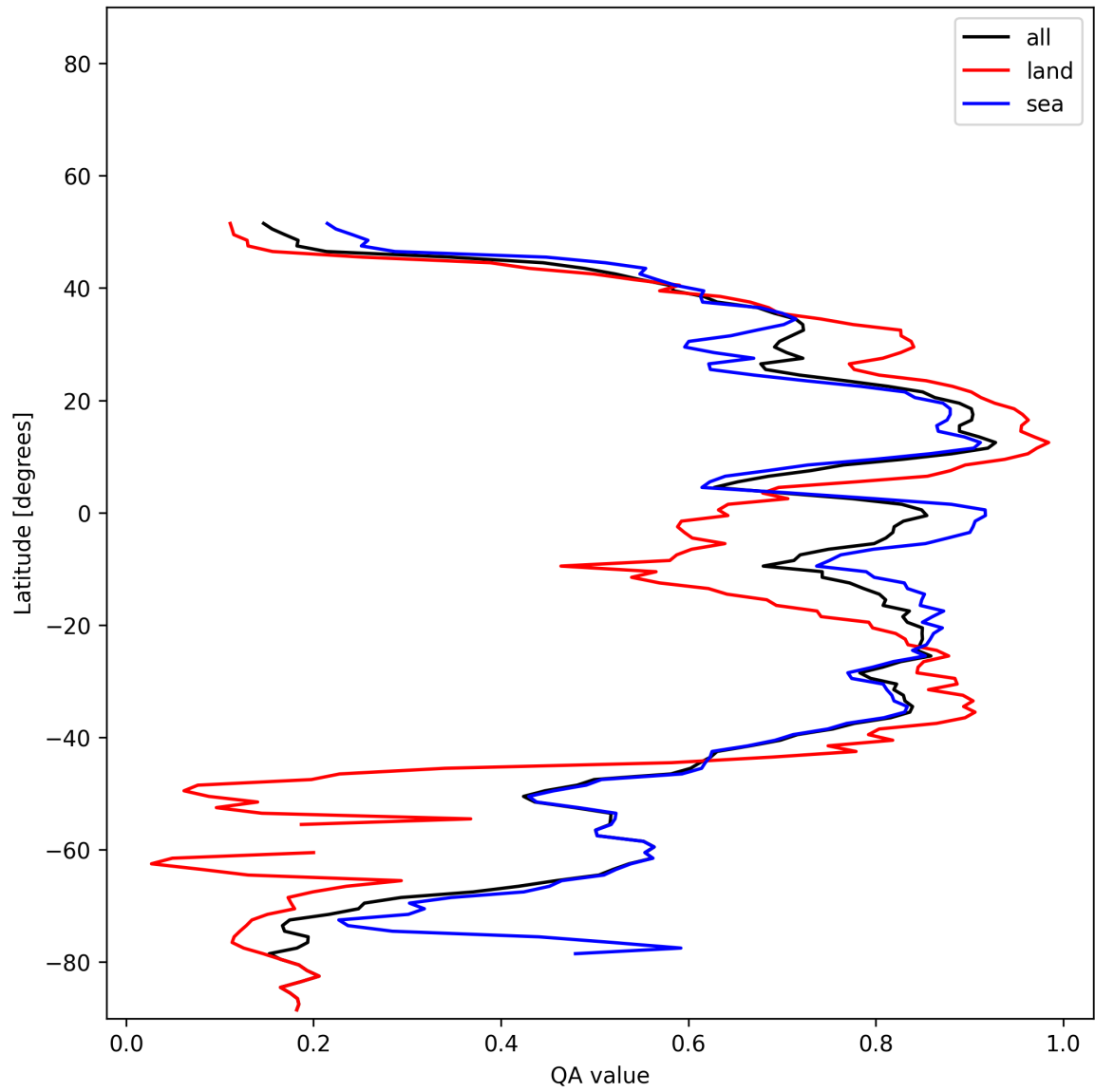
Figure 30: Zonal average of “QA value” for 2025-01-26 to 2025-01-26.
