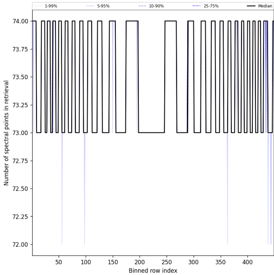
Figure 110: Along track statistics of “Number of spectral points in retrieval” for 2025-01-26 to 2025-01-26
