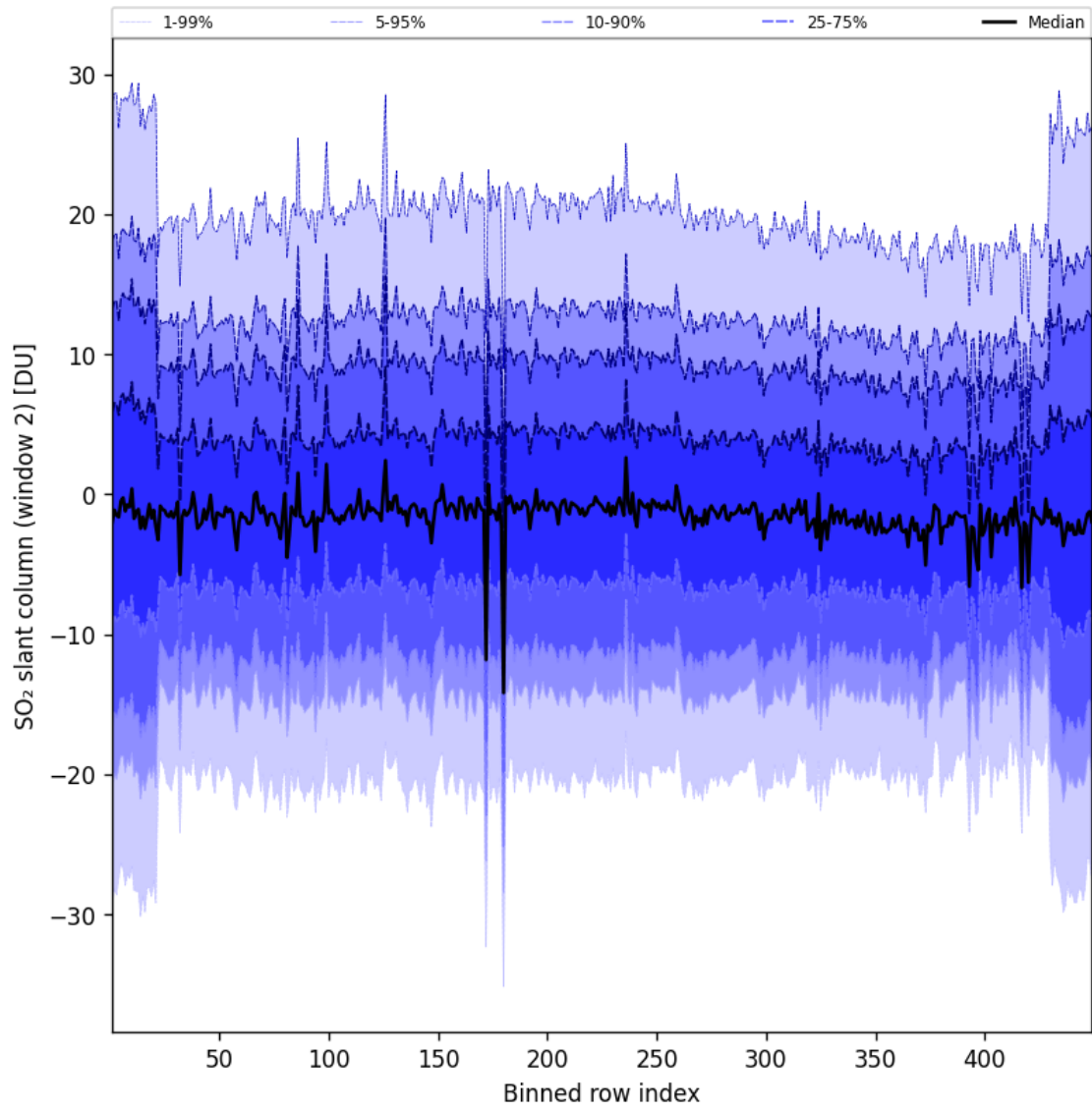
Figure 94: Along track statistics of “SO 2 slant column (window 2)” for 2025-01-26 to 2025-01-26
