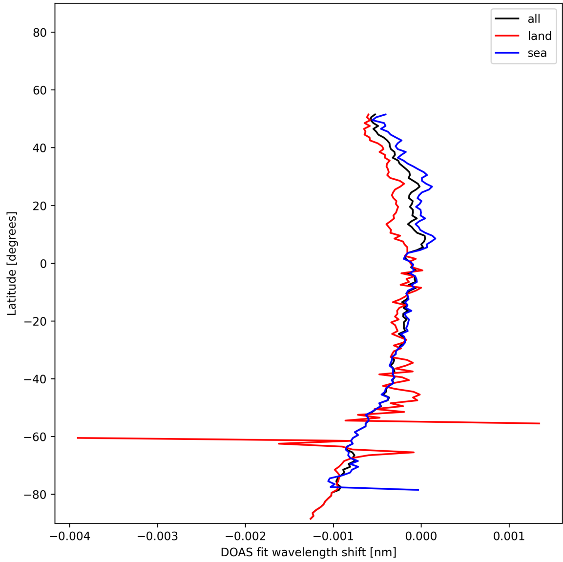
Figure 50: Zonal average of "DOAS fit wavelength shift" for 2025-01-26 to 2025-01-26.
