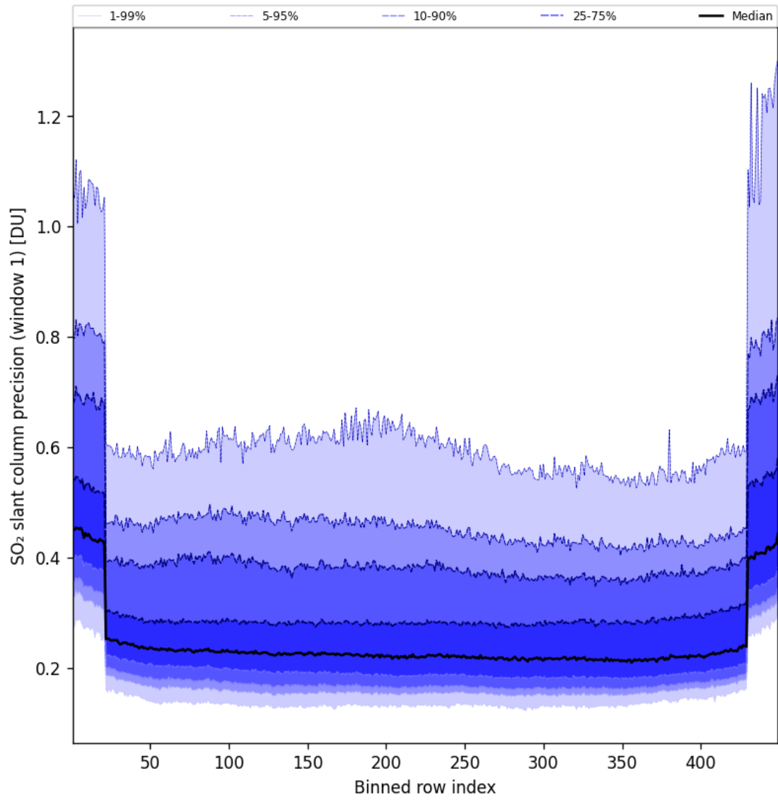
Figure 91: Along track statistics of “SO 2 slant column precision (window 1)” for 2025-01-26 to 2025-01-26
