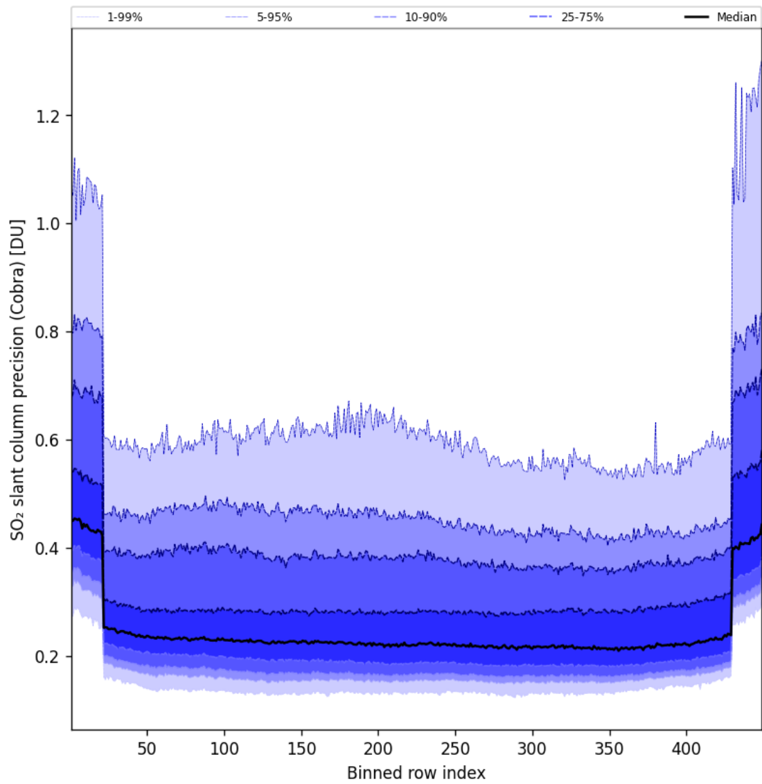
Figure 89: Along track statistics of “SO 2 slant column precision (Cobra)” for 2025-01-26 to 2025-01-26
