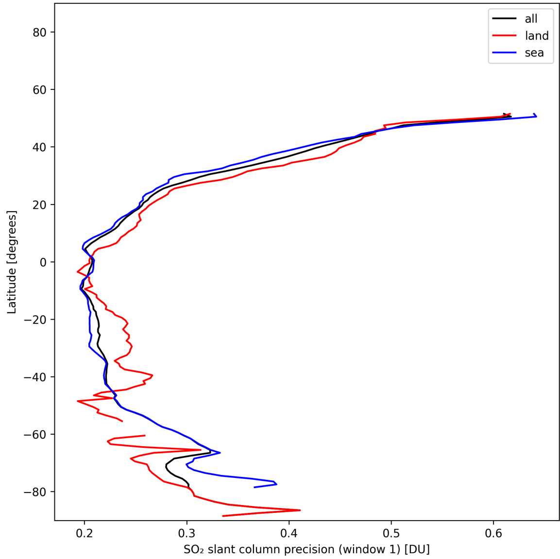
Figure 37: Zonal average of “SO 2 slant column precision (window 1)” for 2025-01-26 to 2025-01-26.
