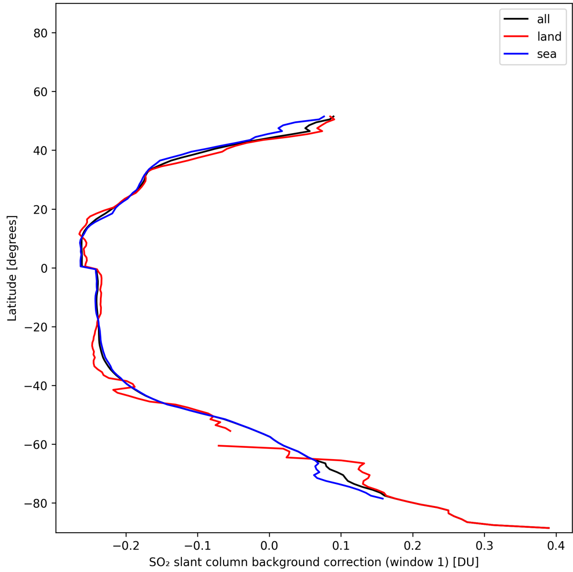
Figure 39: Zonal average of “SO 2 slant column background correction (window 1)” for 2025-01-26 to 2025-01-26.
