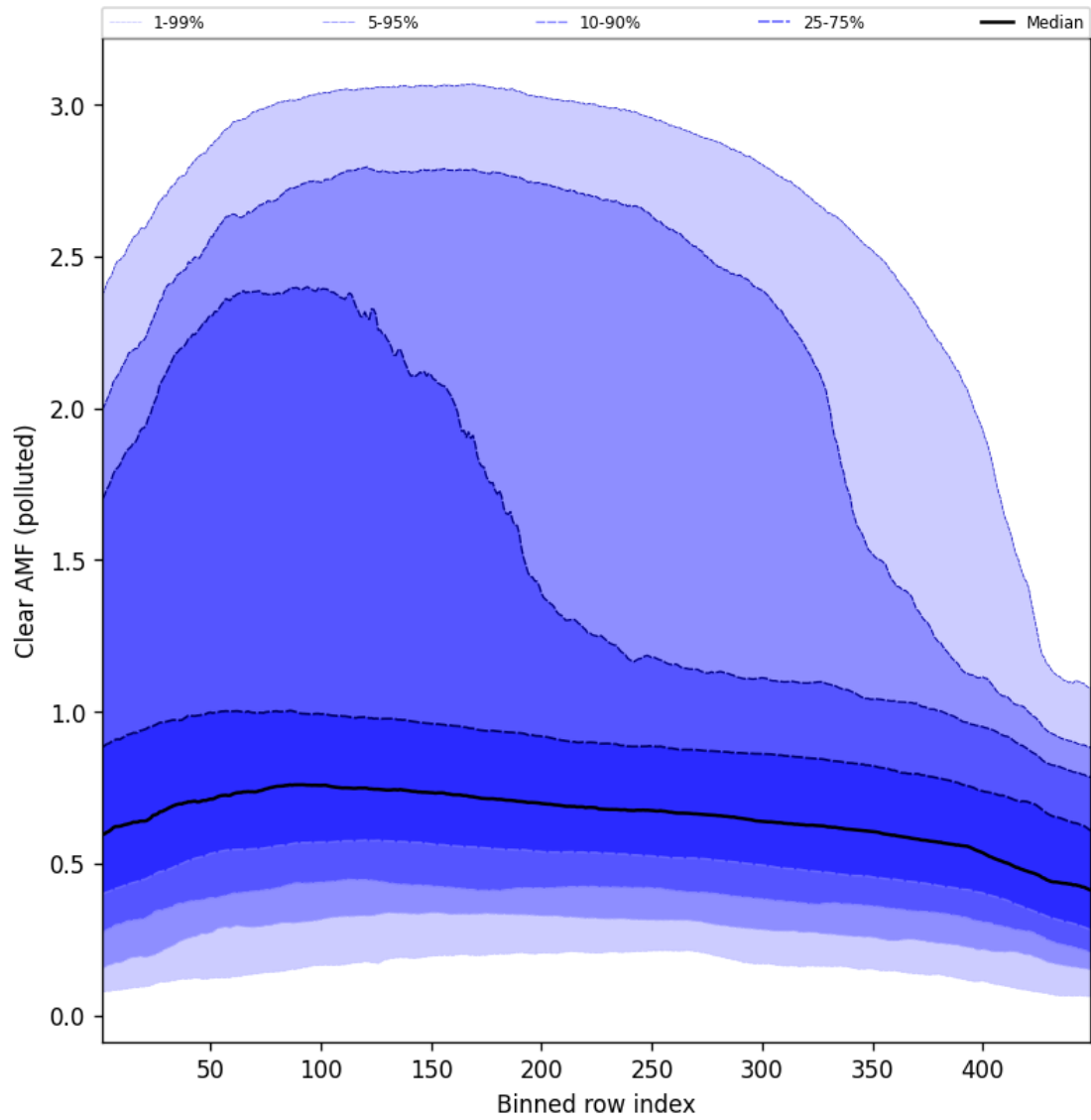
Figure 109: Along track statistics of “Clear AMF (polluted)” for 2025-01-26 to 2025-01-26
