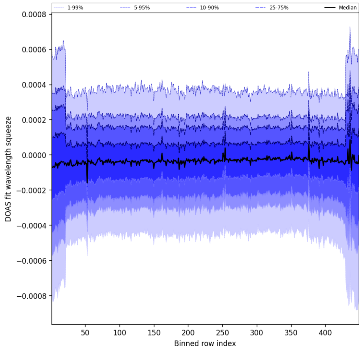
Figure 105: Along track statistics of “DOAS fit wavelength squeeze” for 2025-01-26 to 2025-01-26
