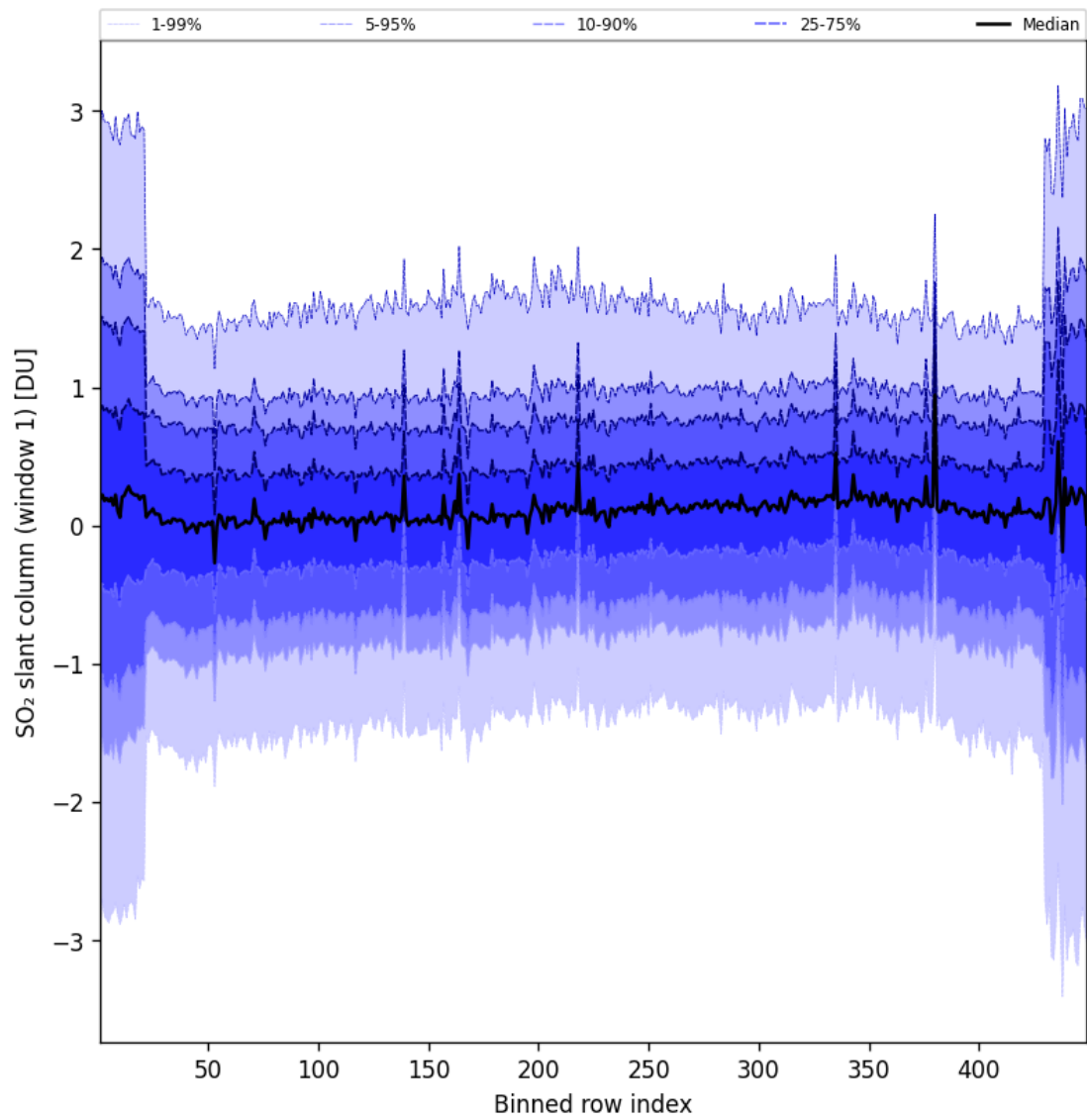
Figure 90: Along track statistics of “SO 2 slant column (window 1)” for 2025-01-26 to 2025-01-26
