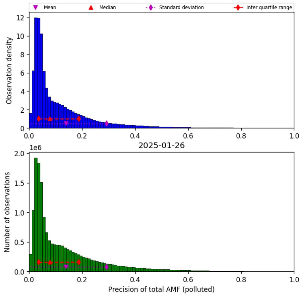
Figure 81: Histogram of “Precision of total AMF (polluted)” for 2025-01-26 to 2025-01-26
