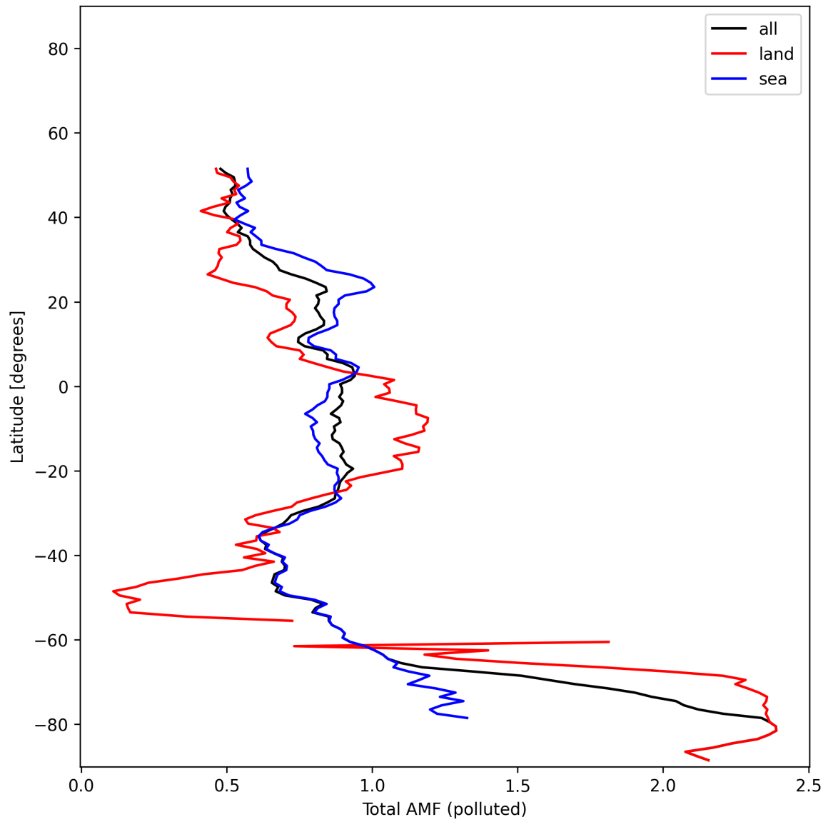
Figure 53: Zonal average of “Total AMF (polluted)” for 2025-01-26 to 2025-01-26.
