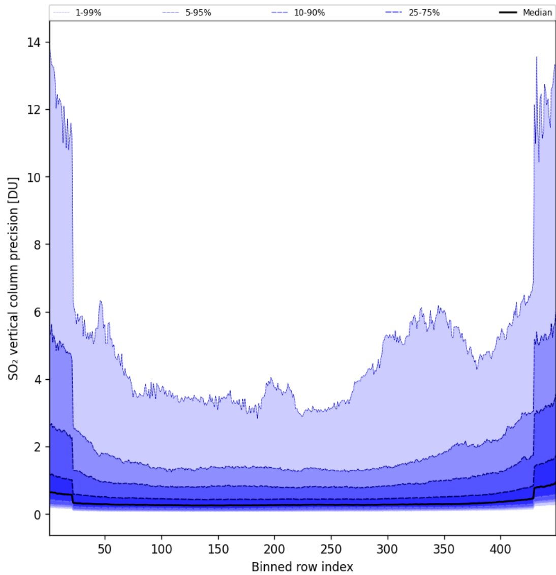
Figure 86: Along track statistics of “SO 2 vertical column precision” for 2025-01-26 to 2025-01-26
