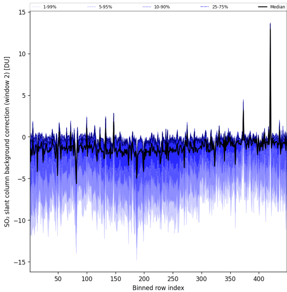
Figure 97: Along track statistics of “SO 2 slant column background correction (window 2)” for 2025-01-26 to 2025-01-26
