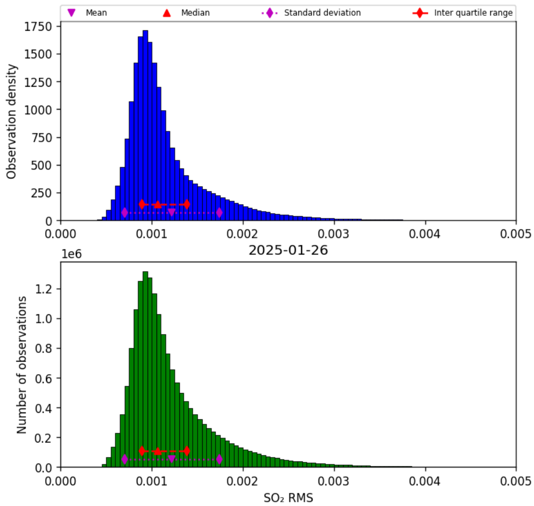
Figure 79: Histogram of “SO 2 RMS” for 2025-01-26 to 2025-01-26
