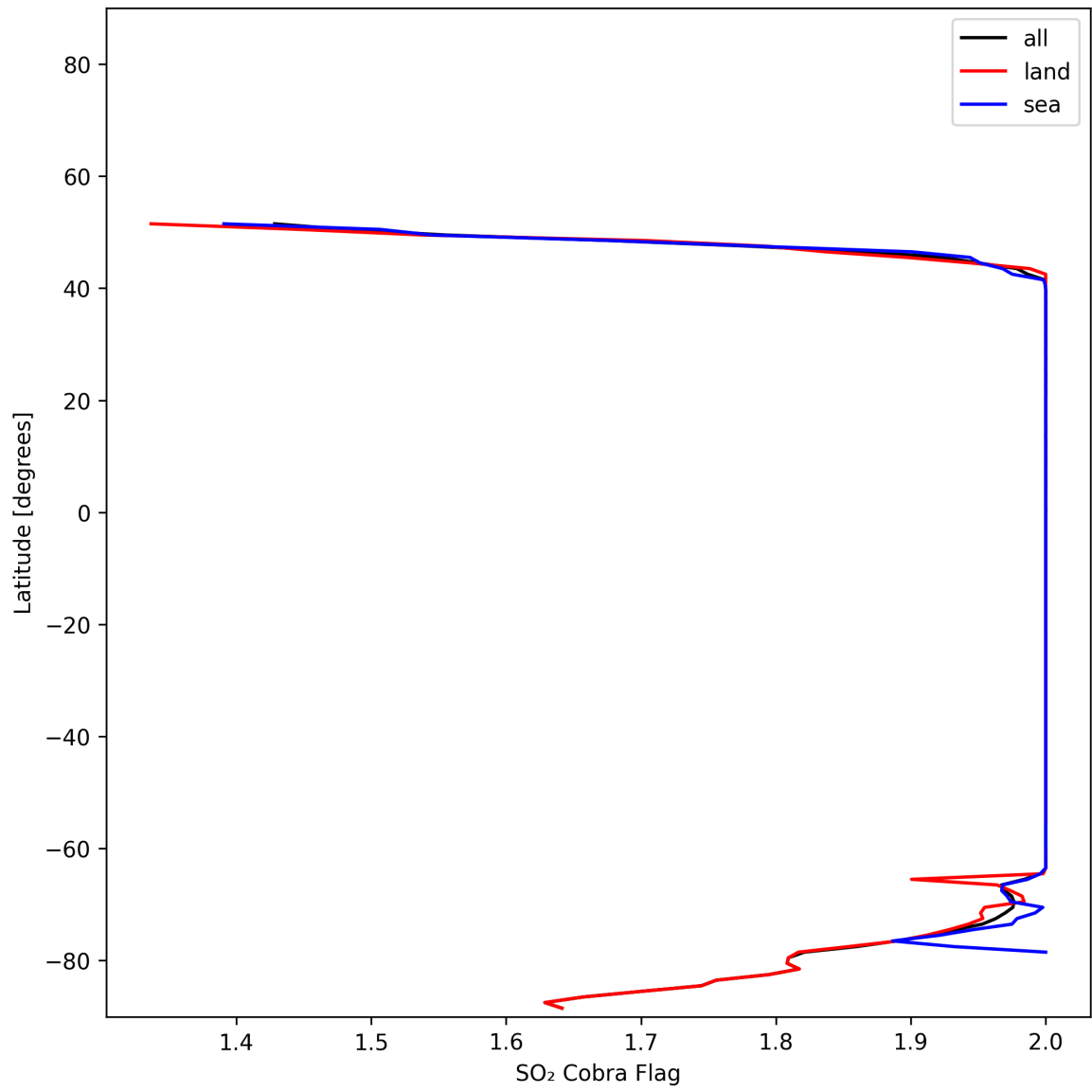
Figure 48: Zonal average of "SO 2 Cobra Flag" for 2025-01-26 to 2025-01-26.
