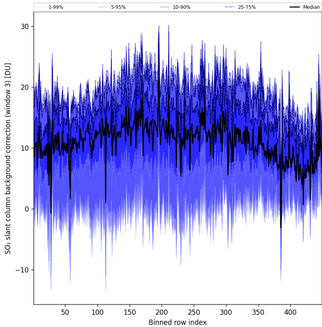
Figure 101: Along track statistics of “SO 2 slant column background correction (window 3)” for 2025-01-26 to 2025-01-26
