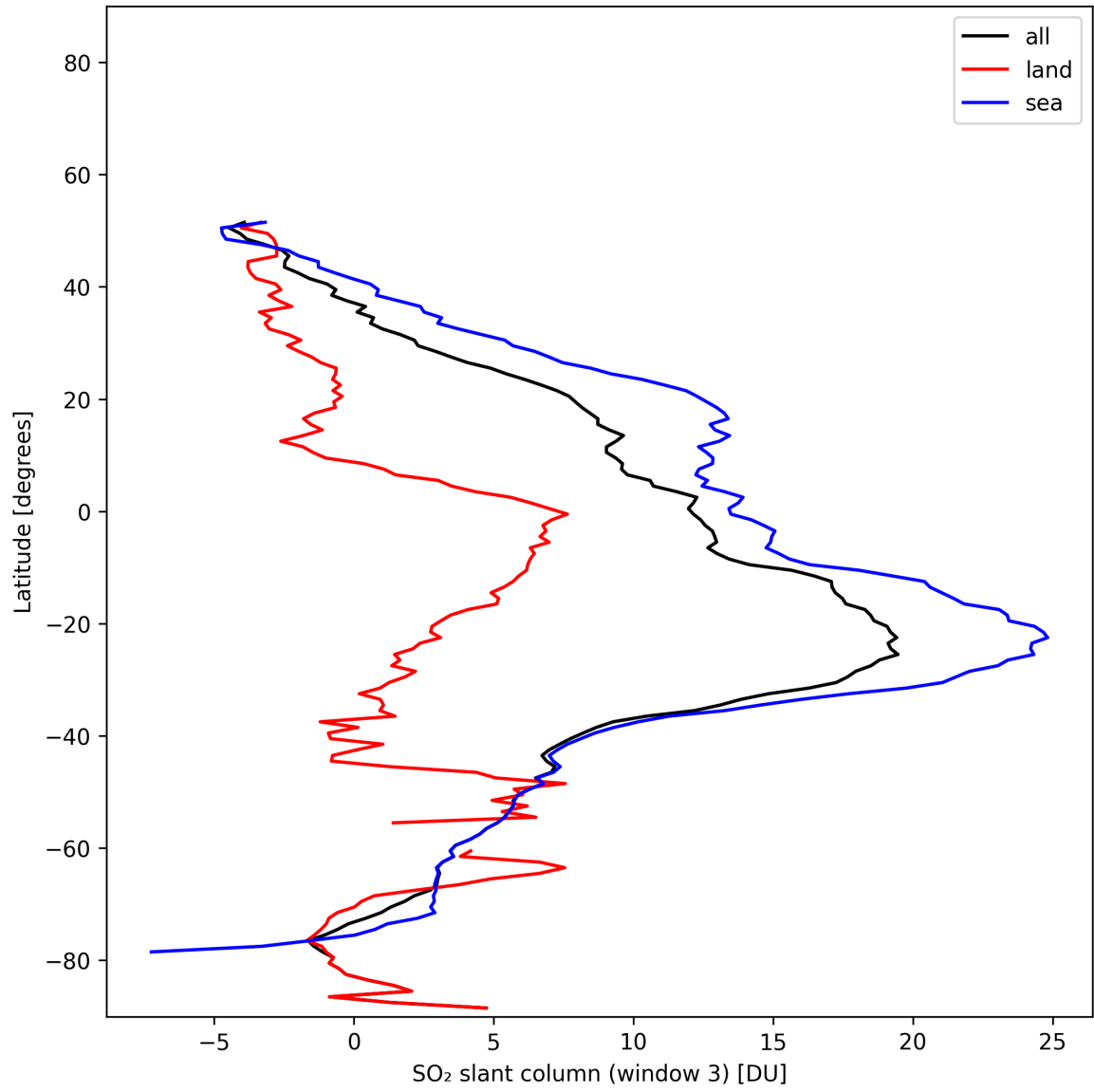
Figure 44: Zonal average of “SO 2 slant column (window 3)” for 2025-01-26 to 2025-01-26.
