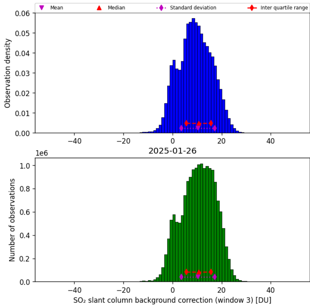
Figure 74: Histogram of “SO 2 slant column background correction (window 3)” for 2025-01-26 to 2025-01-26
