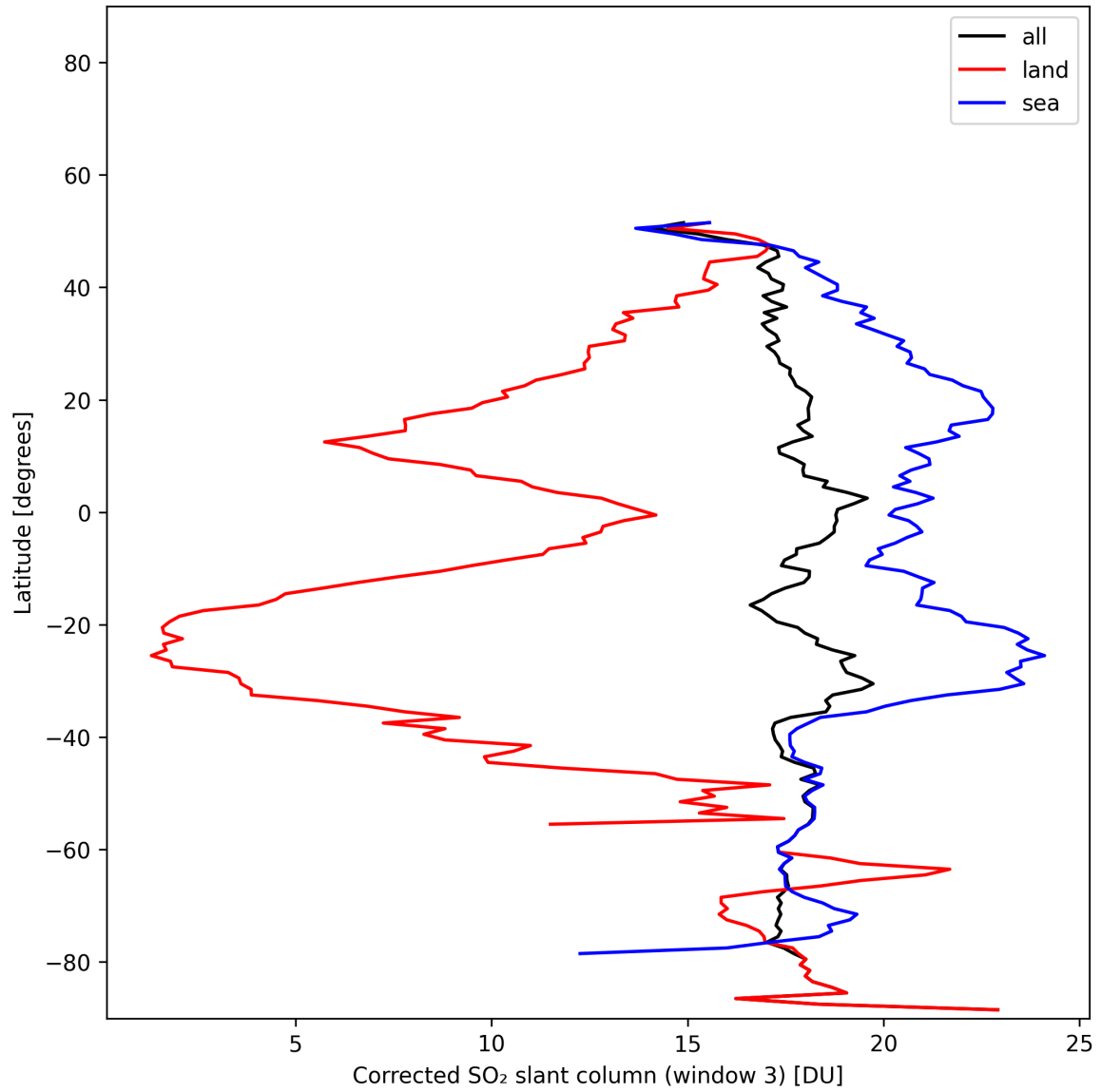
Figure 46: Zonal average of “Corrected SO 2 slant column (window 3)” for 2025-01-26 to 2025-01-26.
