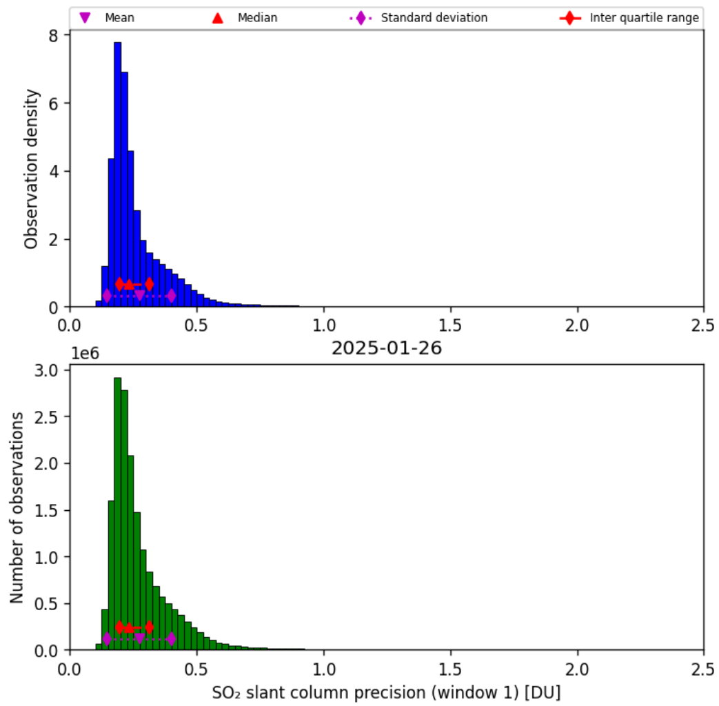
Figure 64: Histogram of “SO 2 slant column precision (window 1)” for 2025-01-26 to 2025-01-26
