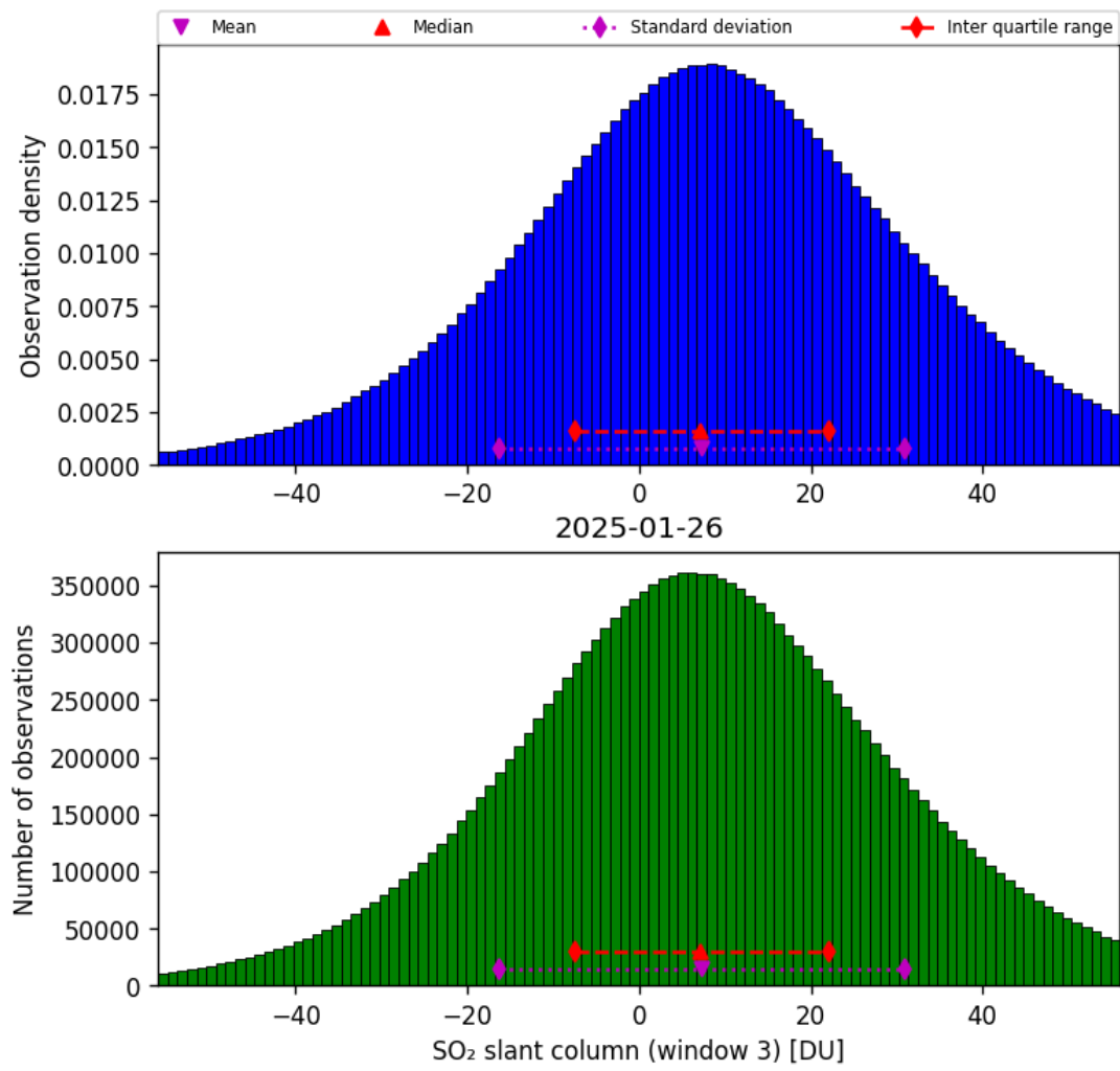
Figure 71: Histogram of “SO 2 slant column (window 3)” for 2025-01-26 to 2025-01-26
