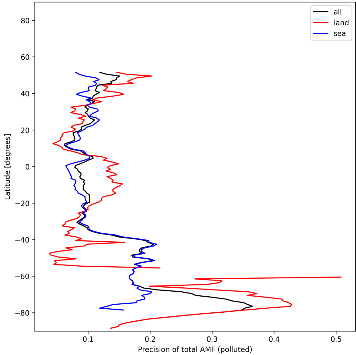
Figure 54: Zonal average of “Precision of total AMF (polluted)” for 2025-01-26 to 2025-01-26.
