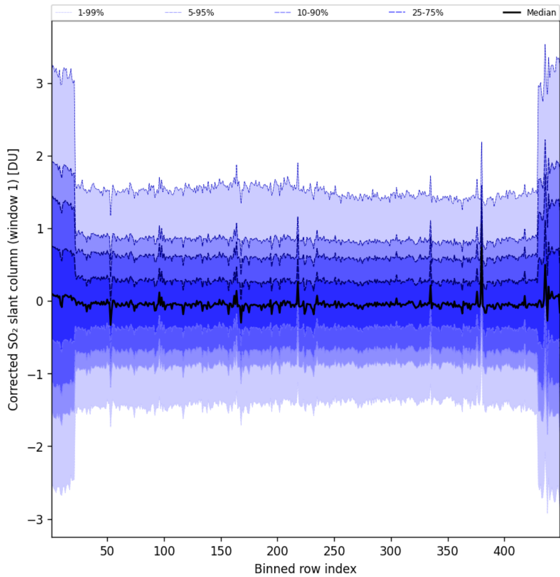
Figure 92: Along track statistics of “Corrected SO 2 slant column (window 1)” for 2025-01-26 to 2025-01-26
