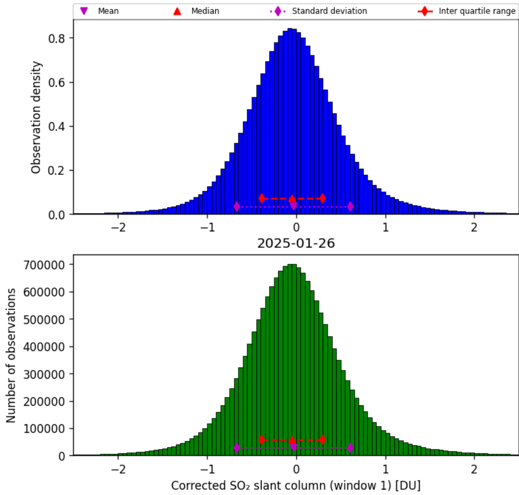
Figure 65: Histogram of “Corrected SO 2 slant column (window 1)” for 2025-01-26 to 2025-01-26
