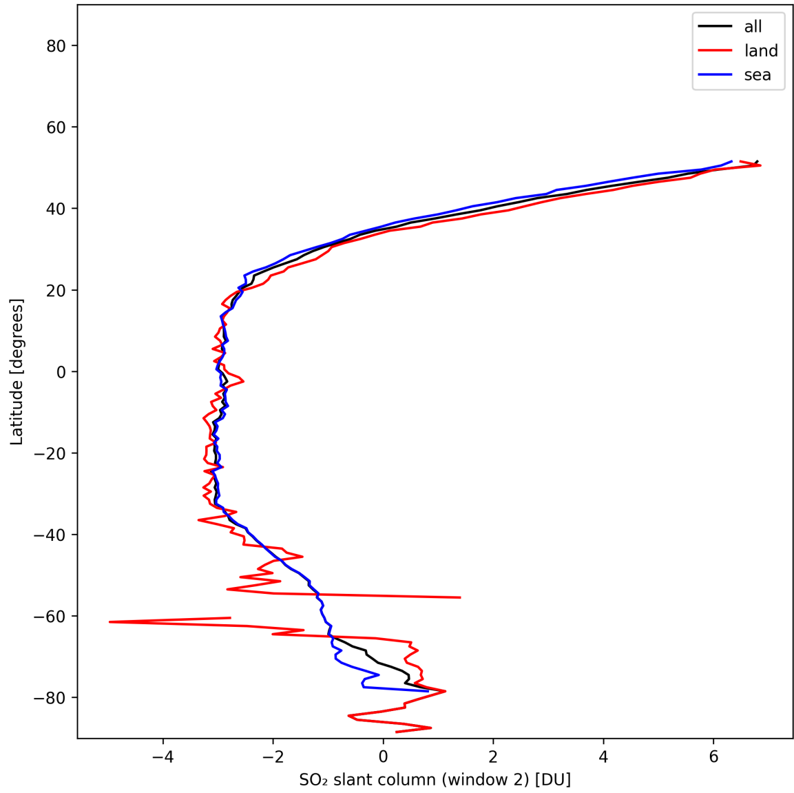
Figure 40: Zonal average of “SO 2 slant column (window 2)” for 2025-01-26 to 2025-01-26.
