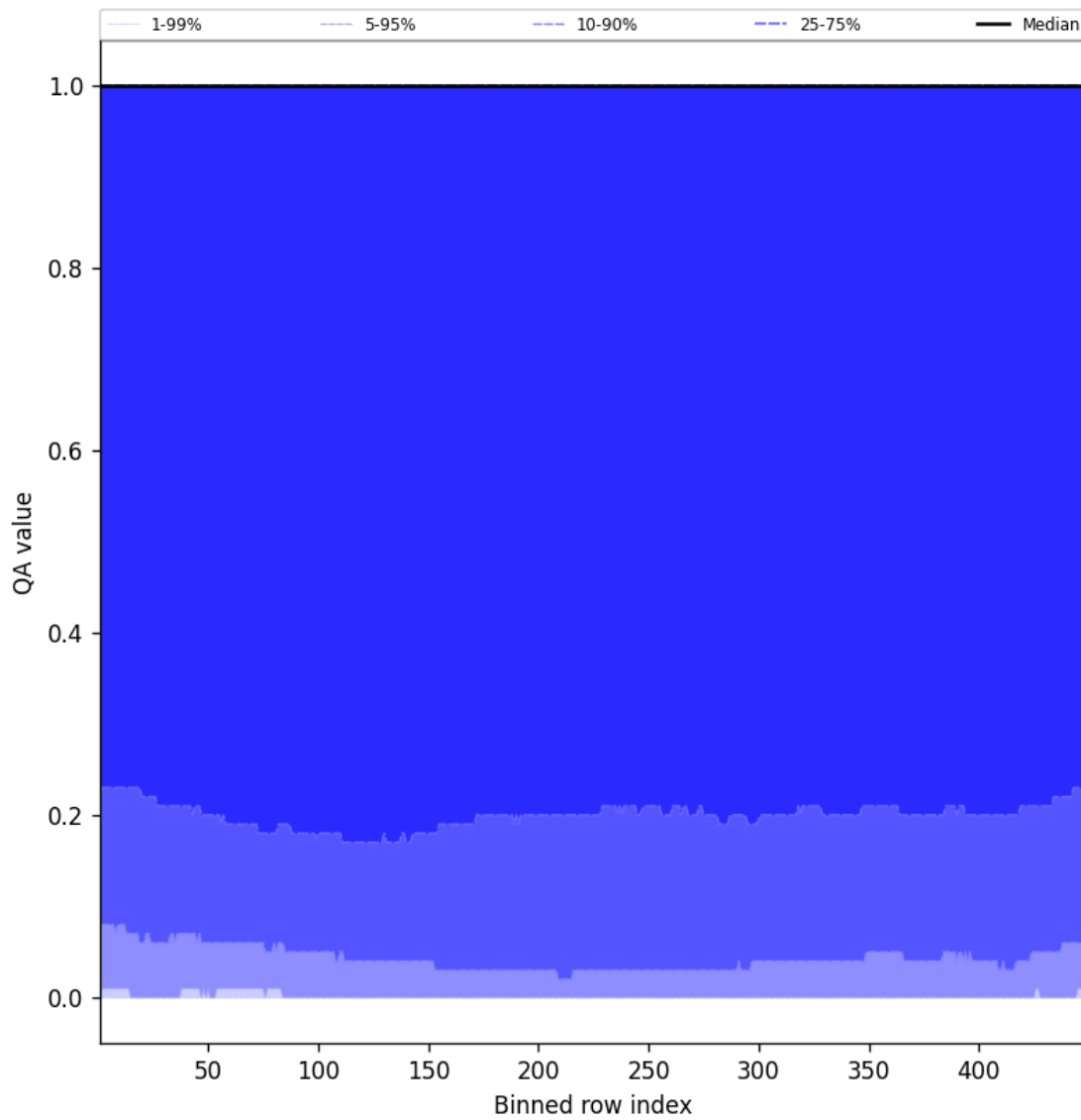
Figure 84: Along track statistics of “QA value” for 2025-01-26 to 2025-01-26
