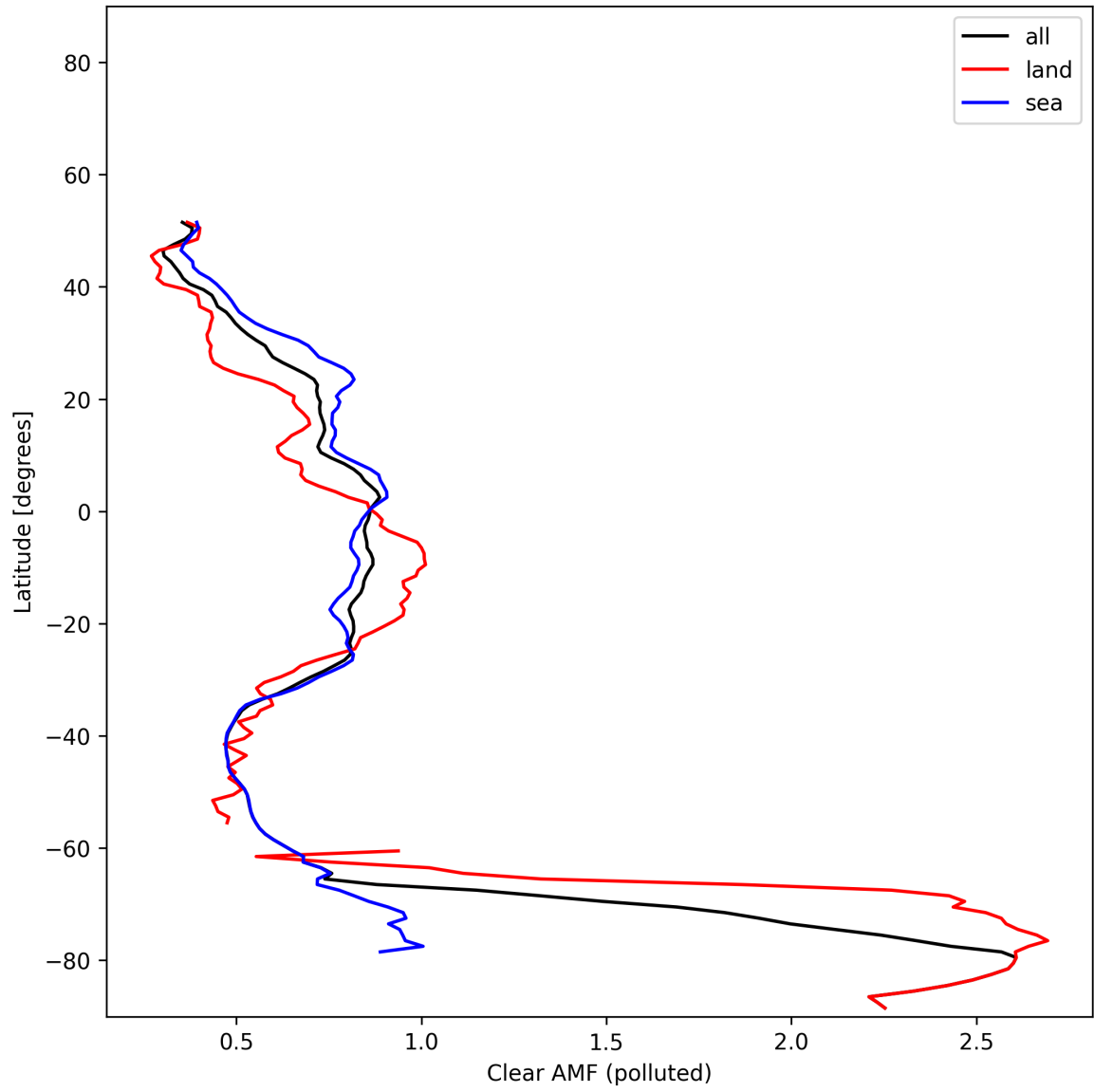
Figure 55: Zonal average of “Clear AMF (polluted)” for 2025-01-26 to 2025-01-26.
