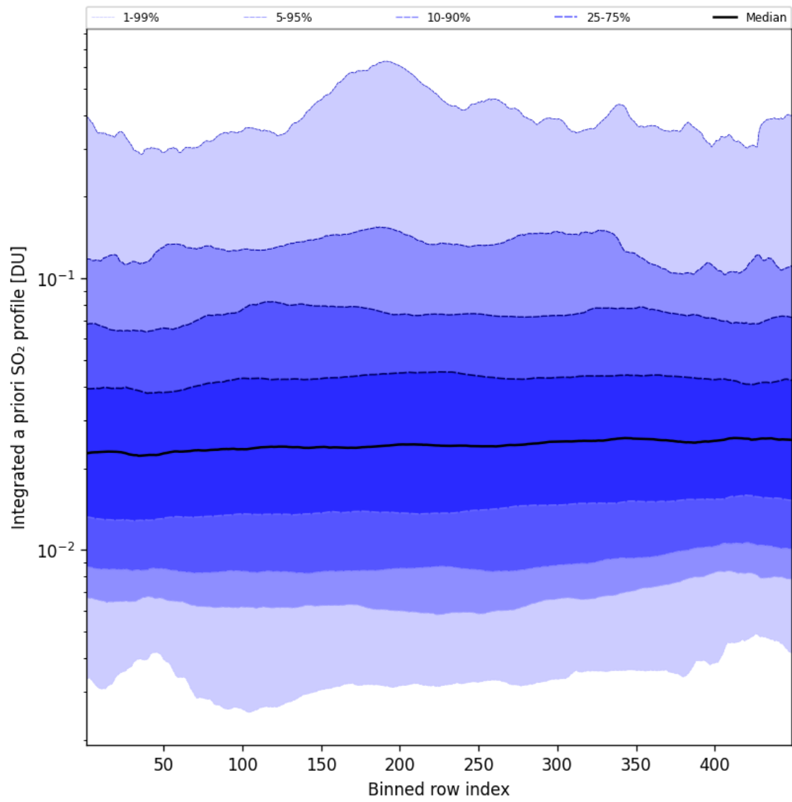
Figure 103: Along track statistics of “Integrated a priori SO 2 profile” for 2025-01-26 to 2025-01-26
