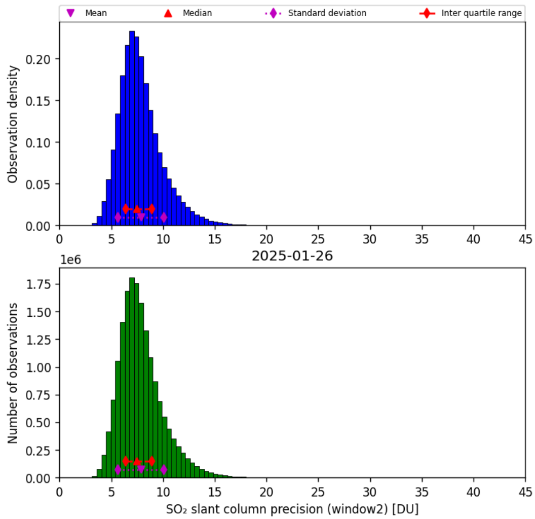
Figure 68: Histogram of “SO 2 slant column precision (window2)” for 2025-01-26 to 2025-01-26
