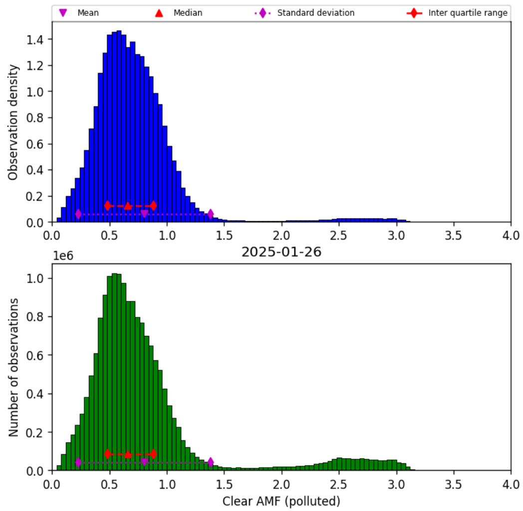
Figure 82: Histogram of “Clear AMF (polluted)” for 2025-01-26 to 2025-01-26
