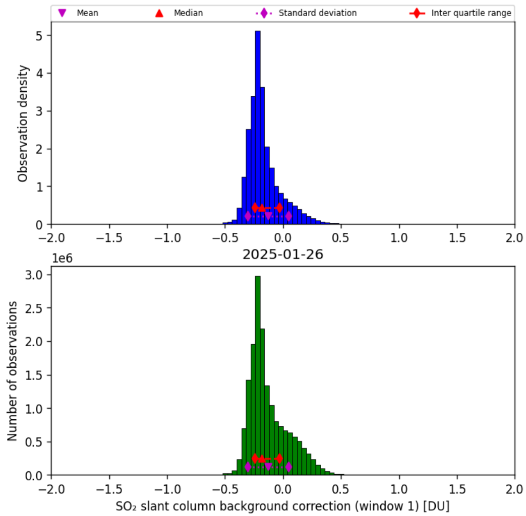
Figure 66: Histogram of “SO 2 slant column background correction (window 1)” for 2025-01-26 to 2025-01-26
