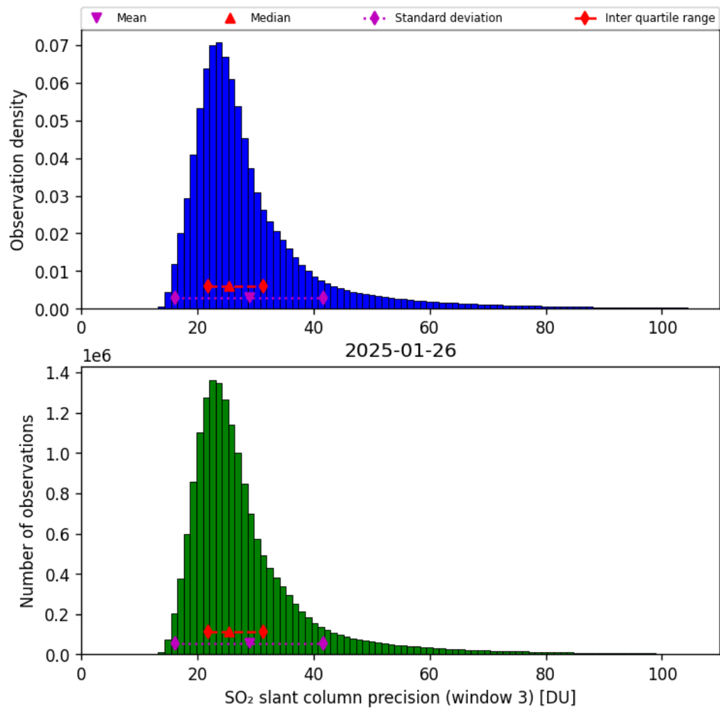
Figure 72: Histogram of “SO 2 slant column precision (window 3)” for 2025-01-26 to 2025-01-26
