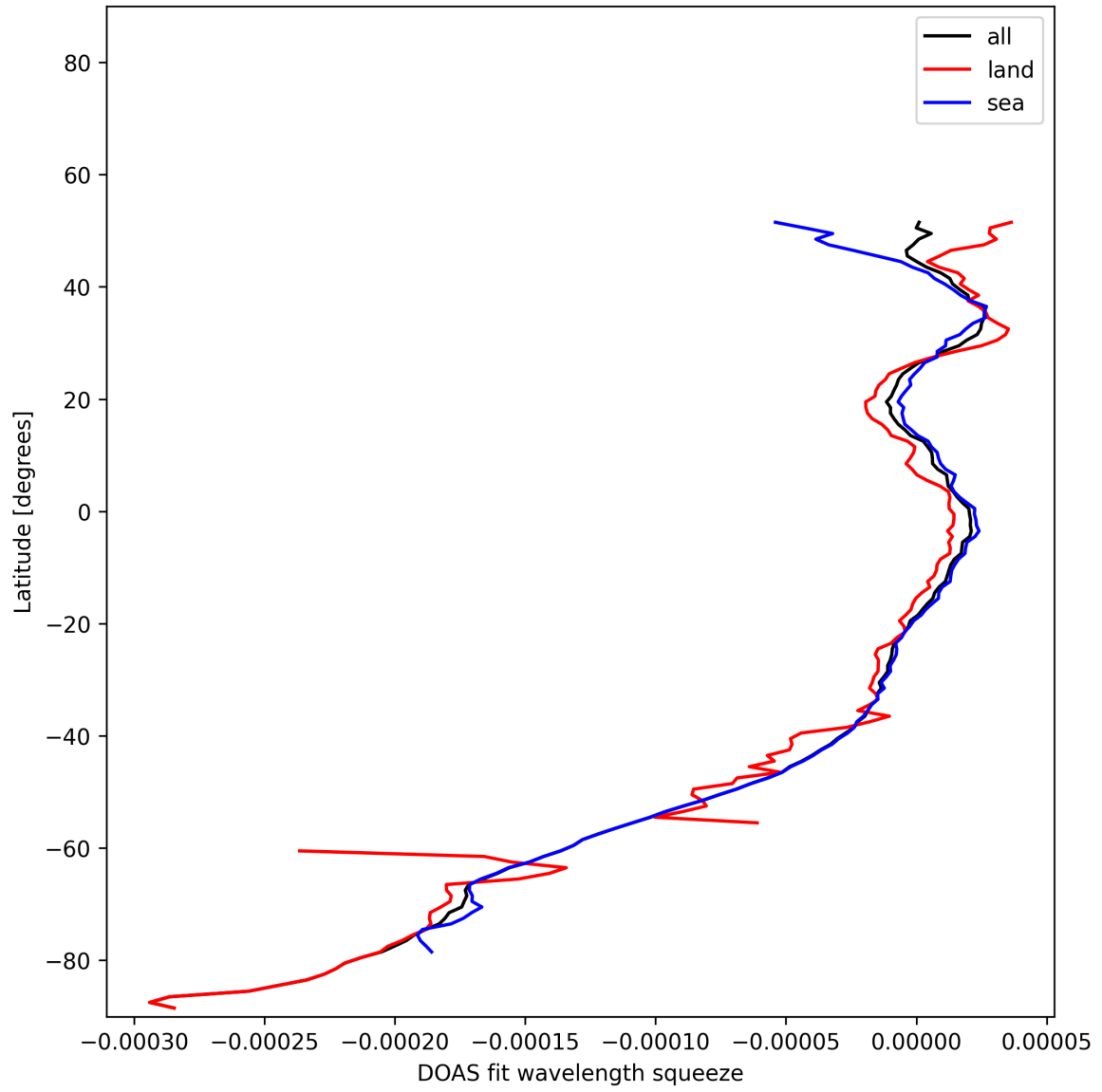
Figure 51: Zonal average of “DOAS fit wavelength squeeze” for 2025-01-26 to 2025-01-26.
