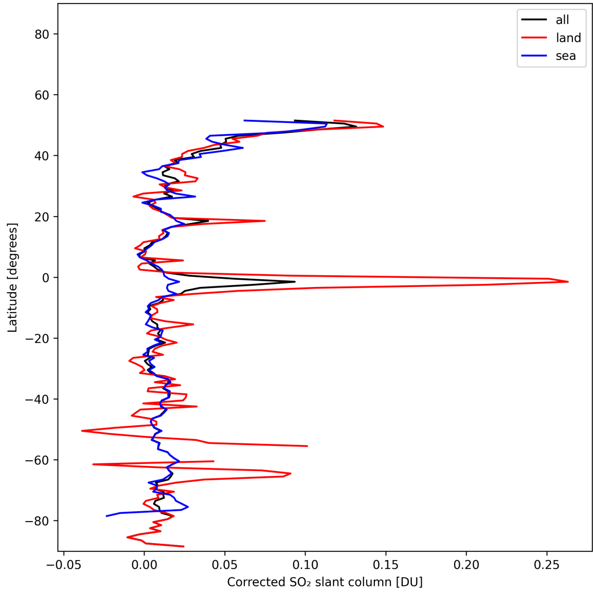
Figure 33: Zonal average of “Corrected SO 2 slant column” for 2025-01-26 to 2025-01-26.
