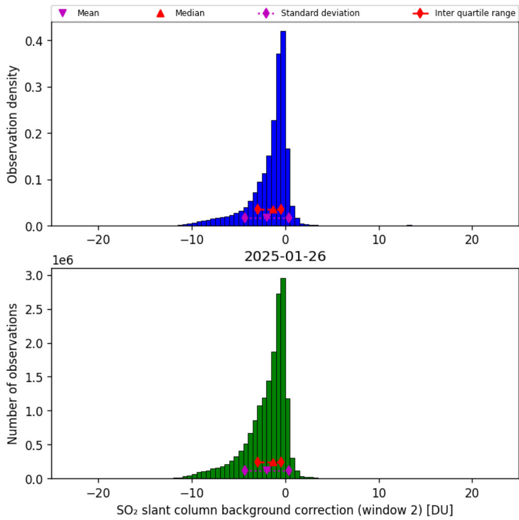
Figure 70: Histogram of “SO 2 slant column background correction (window 2)” for 2025-01-26 to 2025-01-26
