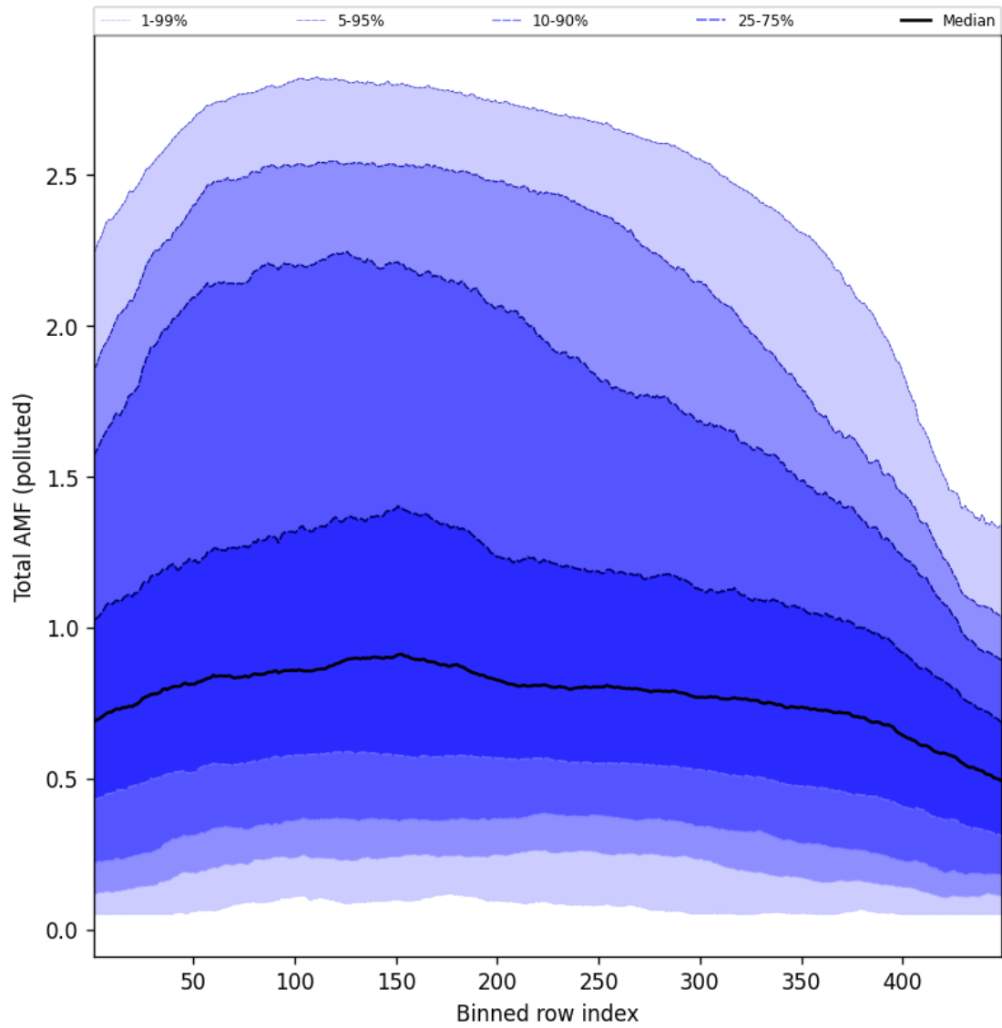
Figure 107: Along track statistics of “Total AMF (polluted)” for 2025-01-26 to 2025-01-26
