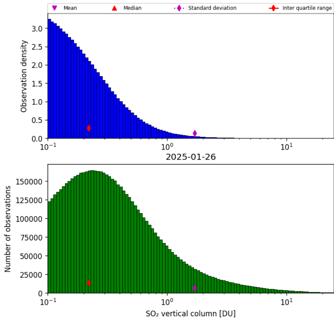
Figure 58: Histogram of “SO 2 vertical column” for 2025-01-26 to 2025-01-26
