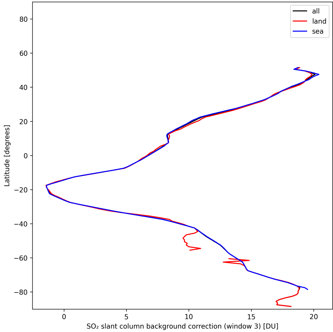
Figure 47: Zonal average of “SO 2 slant column background correction (window 3)” for 2025-01-26 to 2025-01-26.
