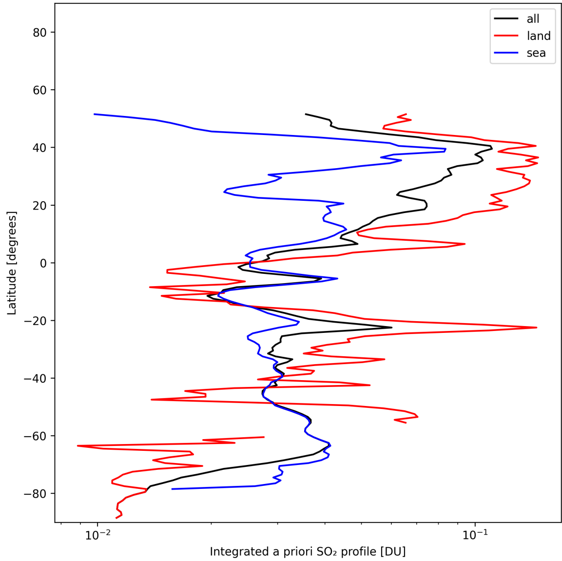
Figure 49: Zonal average of “Integrated a priori SO 2 profile” for 2025-01-26 to 2025-01-26.
