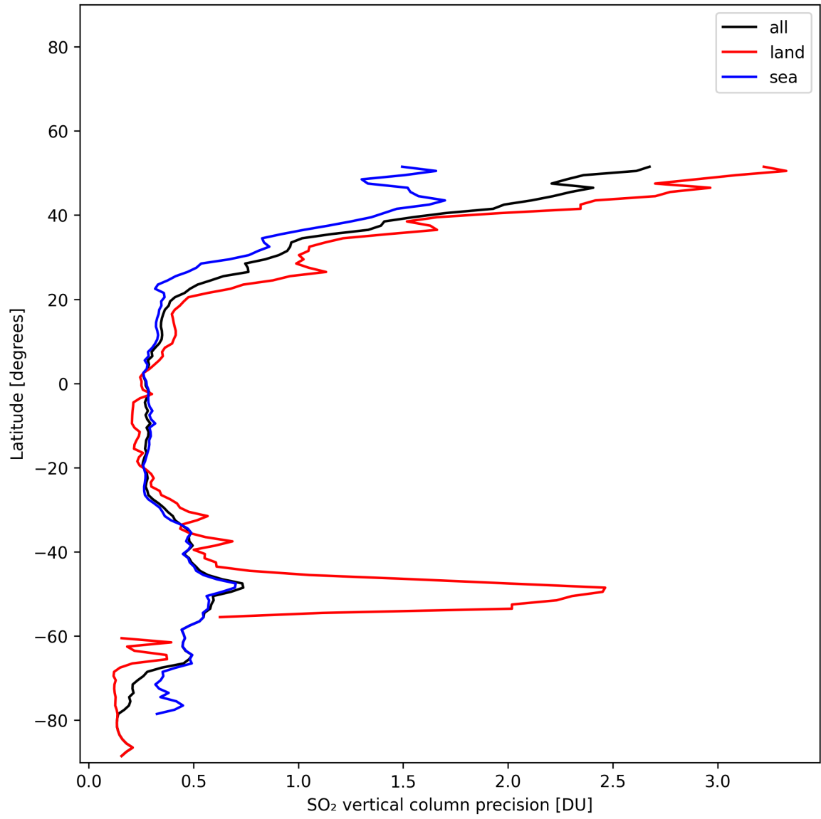
Figure 32: Zonal average of “SO 2 vertical column precision” for 2025-01-26 to 2025-01-26.
