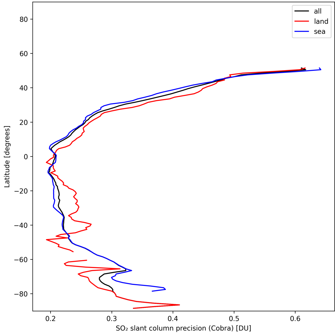
Figure 35: Zonal average of “SO 2 slant column precision (Cobra)” for 2025-01-26 to 2025-01-26.
