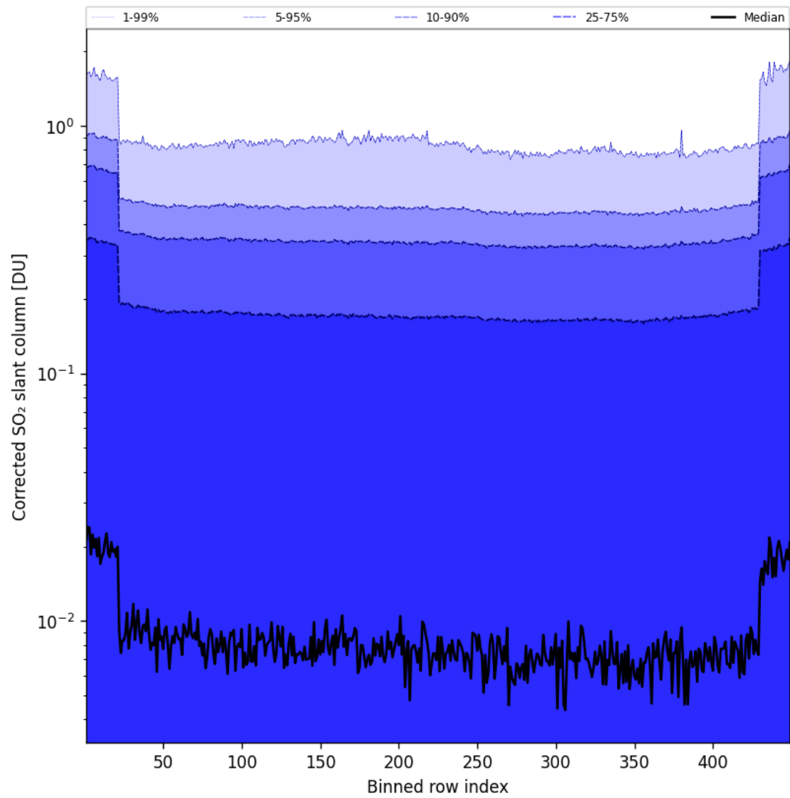
Figure 87: Along track statistics of “Corrected SO 2 slant column” for 2025-01-26 to 2025-01-26
