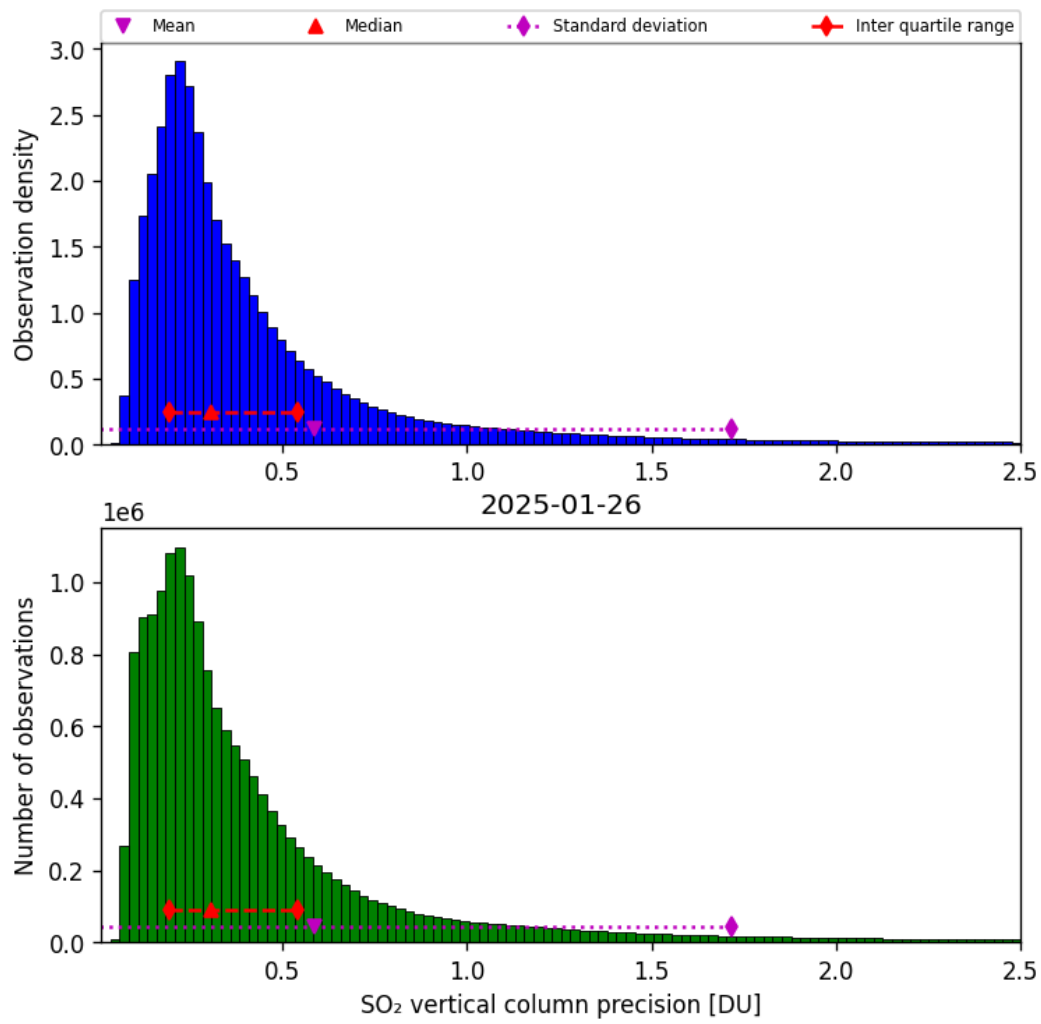
Figure 59: Histogram of “SO 2 vertical column precision” for 2025-01-26 to 2025-01-26
