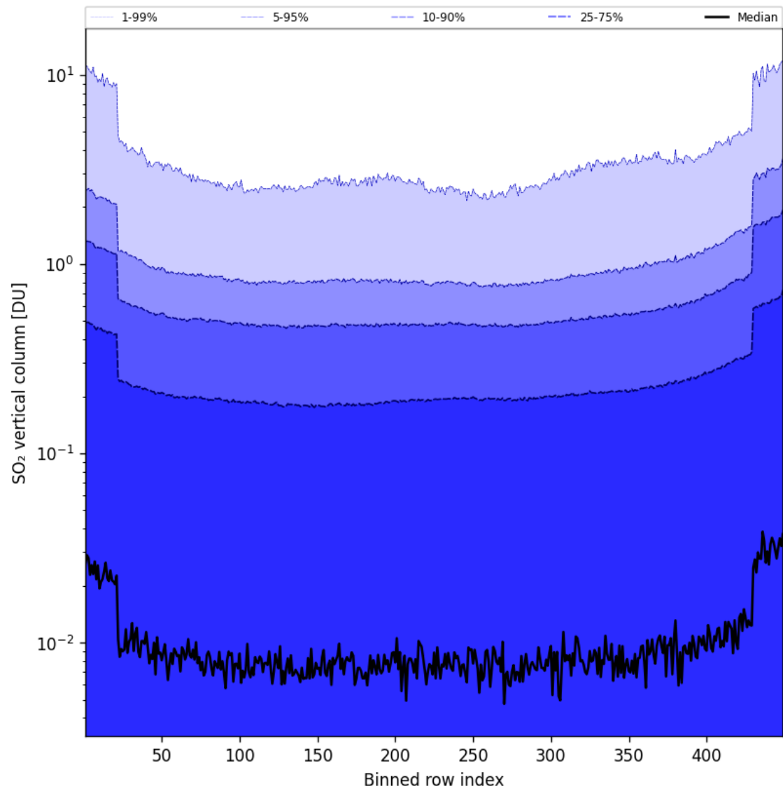
Figure 85: Along track statistics of “SO 2 vertical column” for 2025-01-26 to 2025-01-26
