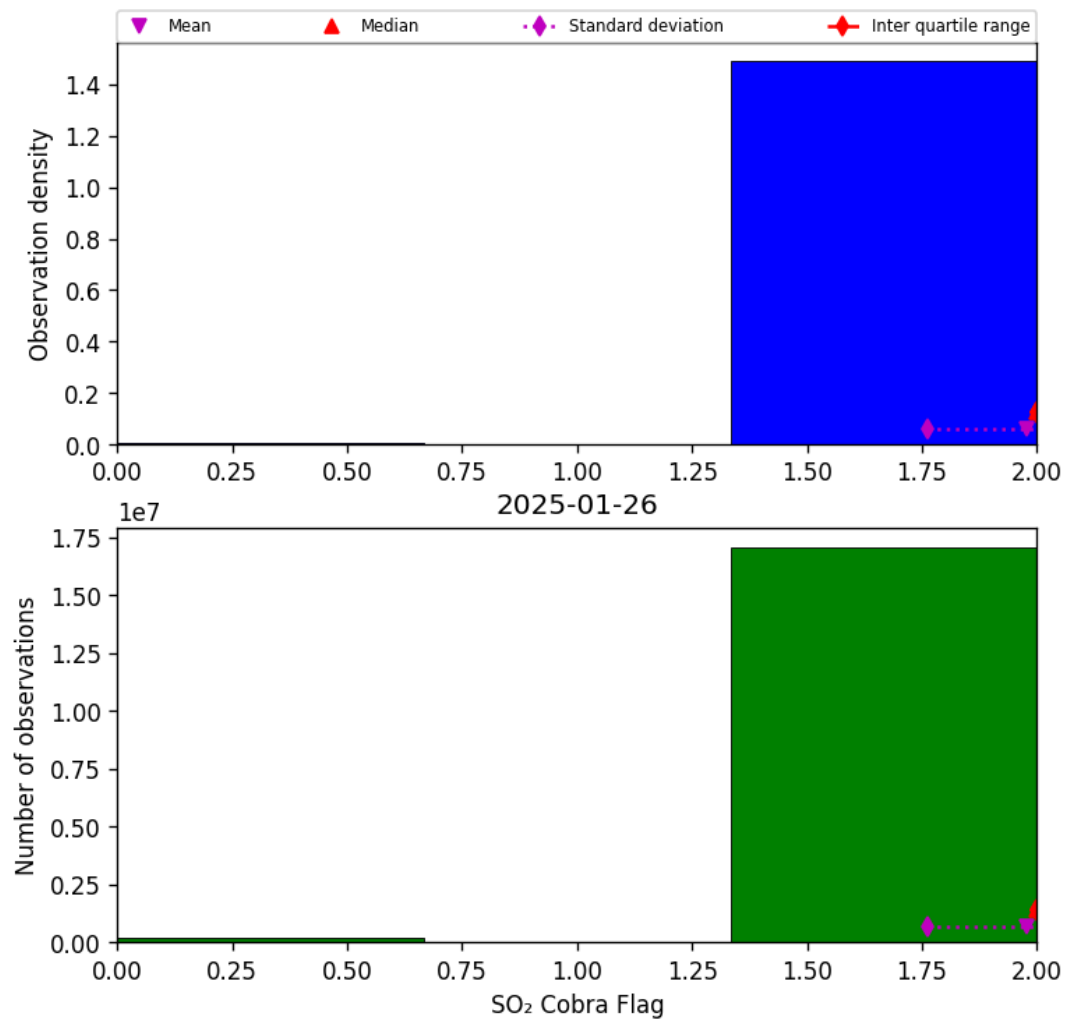
Figure 75: Histogram of “SO 2 Cobra Flag” for 2025-01-26 to 2025-01-26
