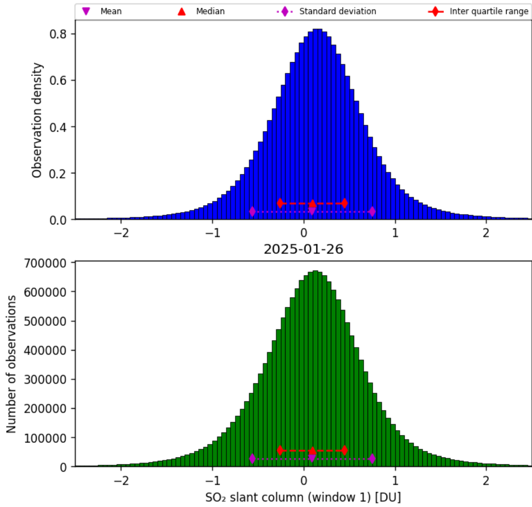
Figure 63: Histogram of “SO 2 slant column (window 1)” for 2025-01-26 to 2025-01-26
