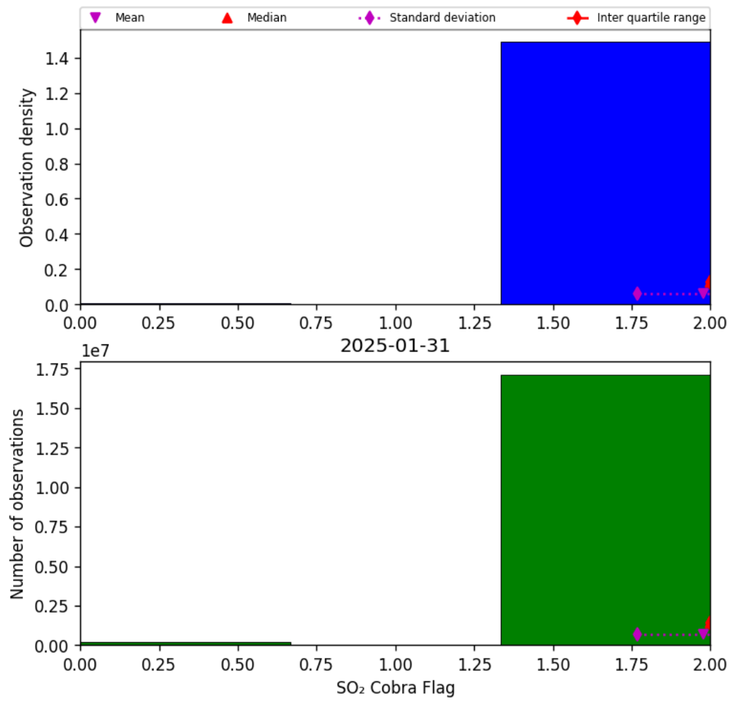
Figure 75: Histogram of "SO 2 Cobra Flag" for 2025-01-31 to 2025-01-31
