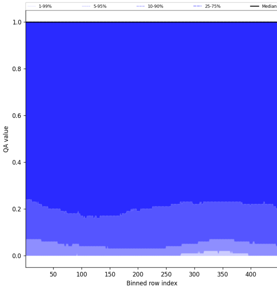
Figure 84: Along track statistics of “QA value” for 2025-01-31 to 2025-01-31
