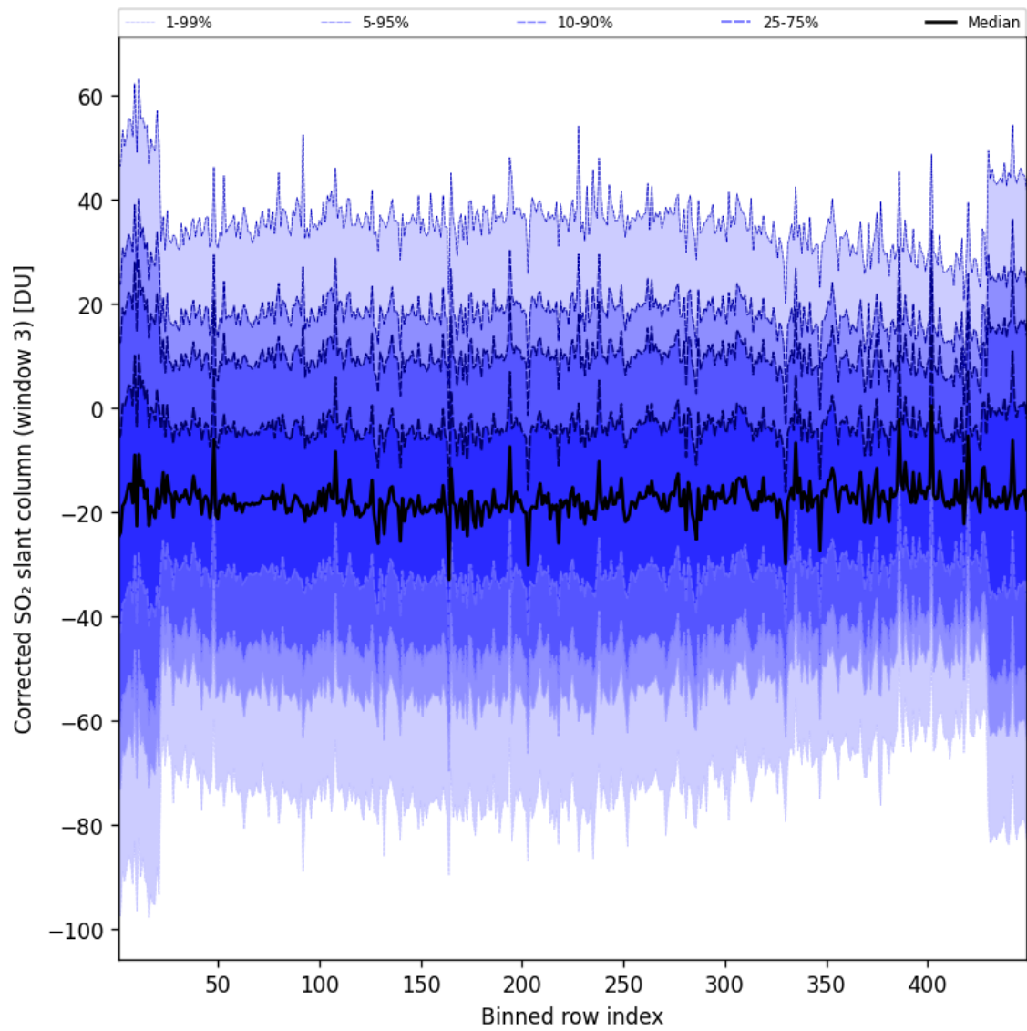
Figure 100: Along track statistics of "Corrected SO 2 slant column (window 3)" for 2025-01-31 to 2025-01-31
