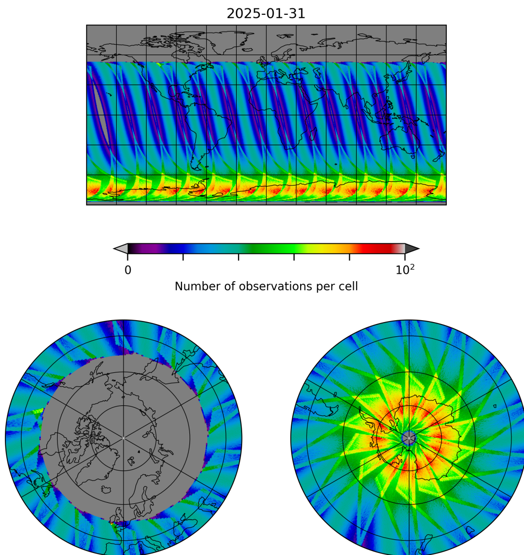
Figure 29: Map of the number of observations for 2025-01-31 to 2025-01-31
