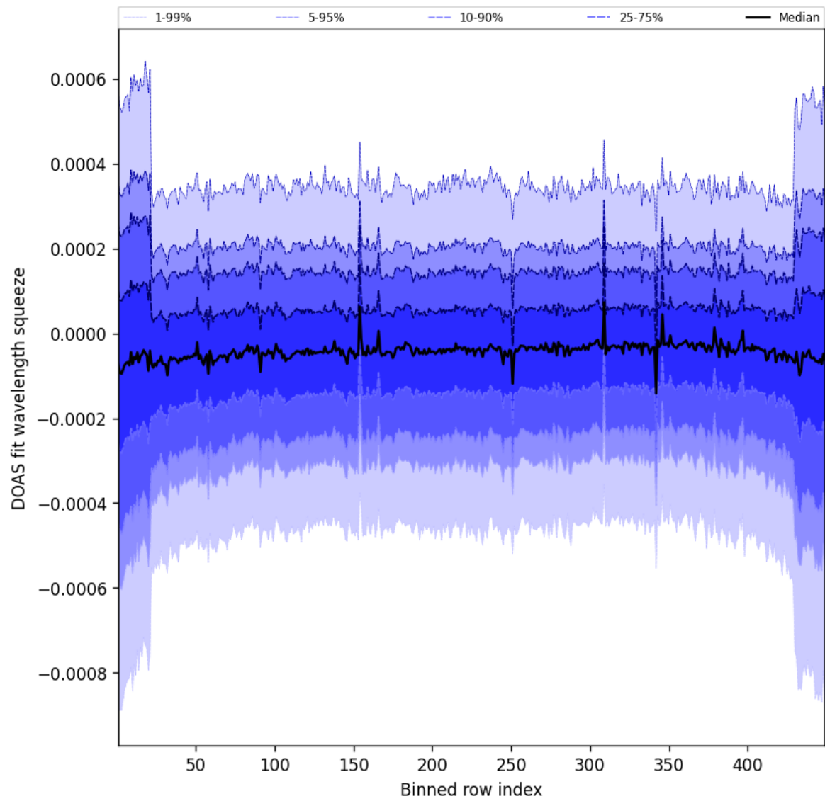
Figure 105: Along track statistics of “DOAS fit wavelength squeeze” for 2025-01-31 to 2025-01-31
