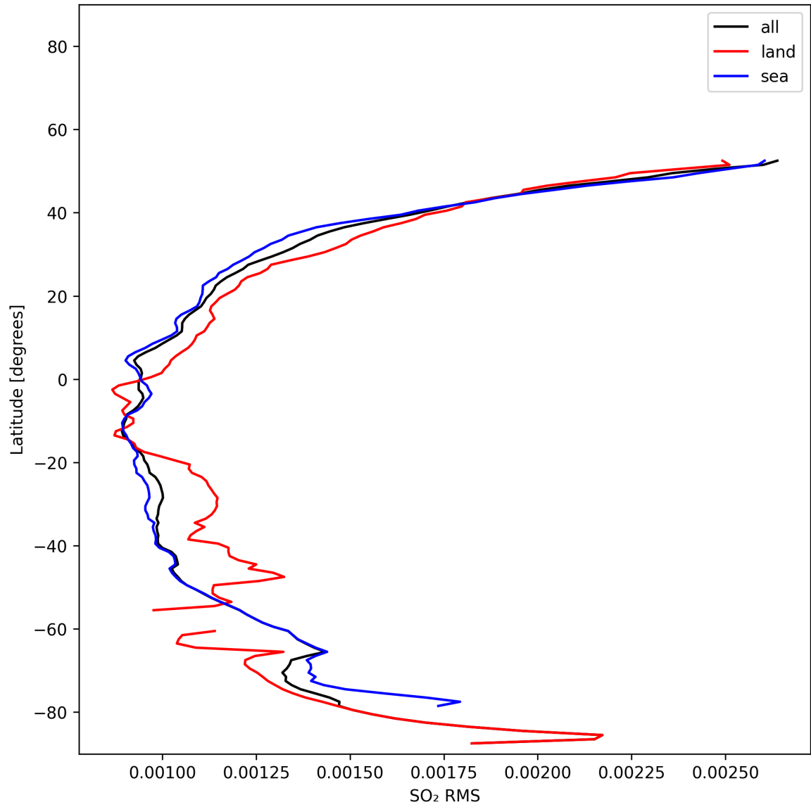
Figure 52: Zonal average of “SO 2 RMS” for 2025-01-31 to 2025-01-31.
