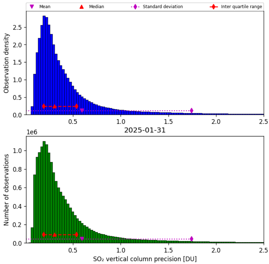
Figure 59: Histogram of “SO 2 vertical column precision” for 2025-01-31 to 2025-01-31
