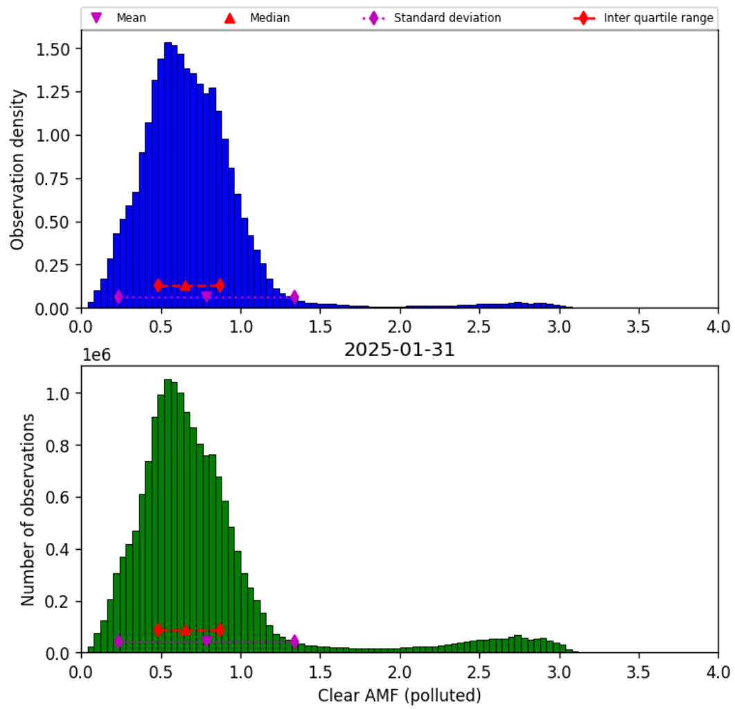
Figure 82: Histogram of “Clear AMF (polluted)” for 2025-01-31 to 2025-01-31
