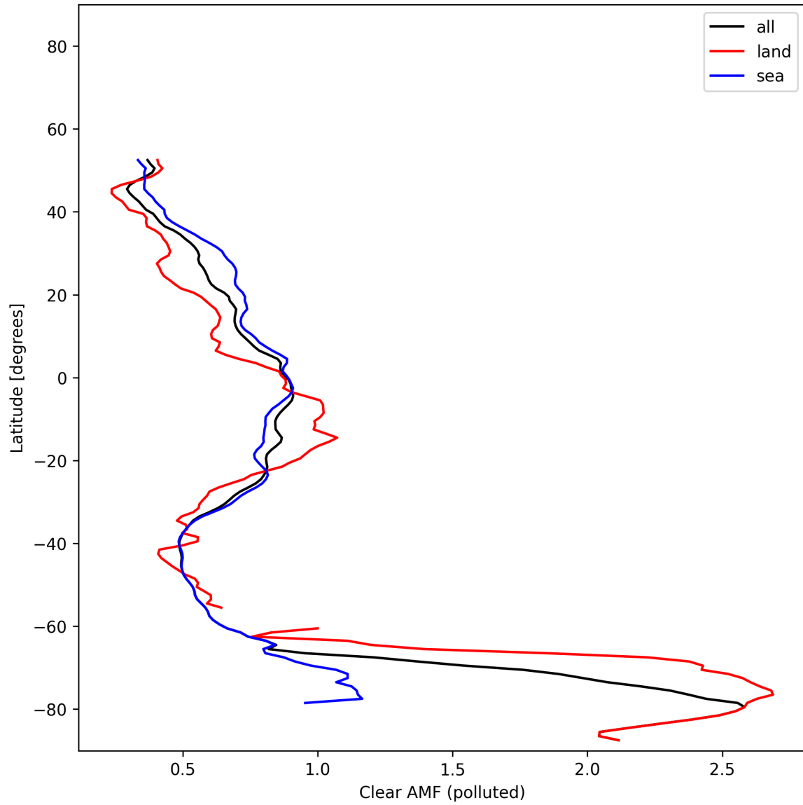
Figure 55: Zonal average of “Clear AMF (polluted)” for 2025-01-31 to 2025-01-31.
