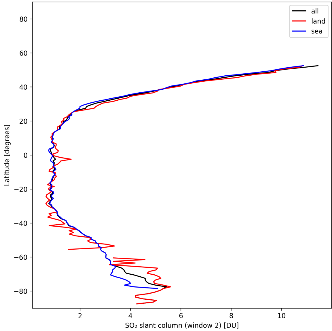
Figure 40: Zonal average of “SO 2 slant column (window 2)” for 2025-01-31 to 2025-01-31.
