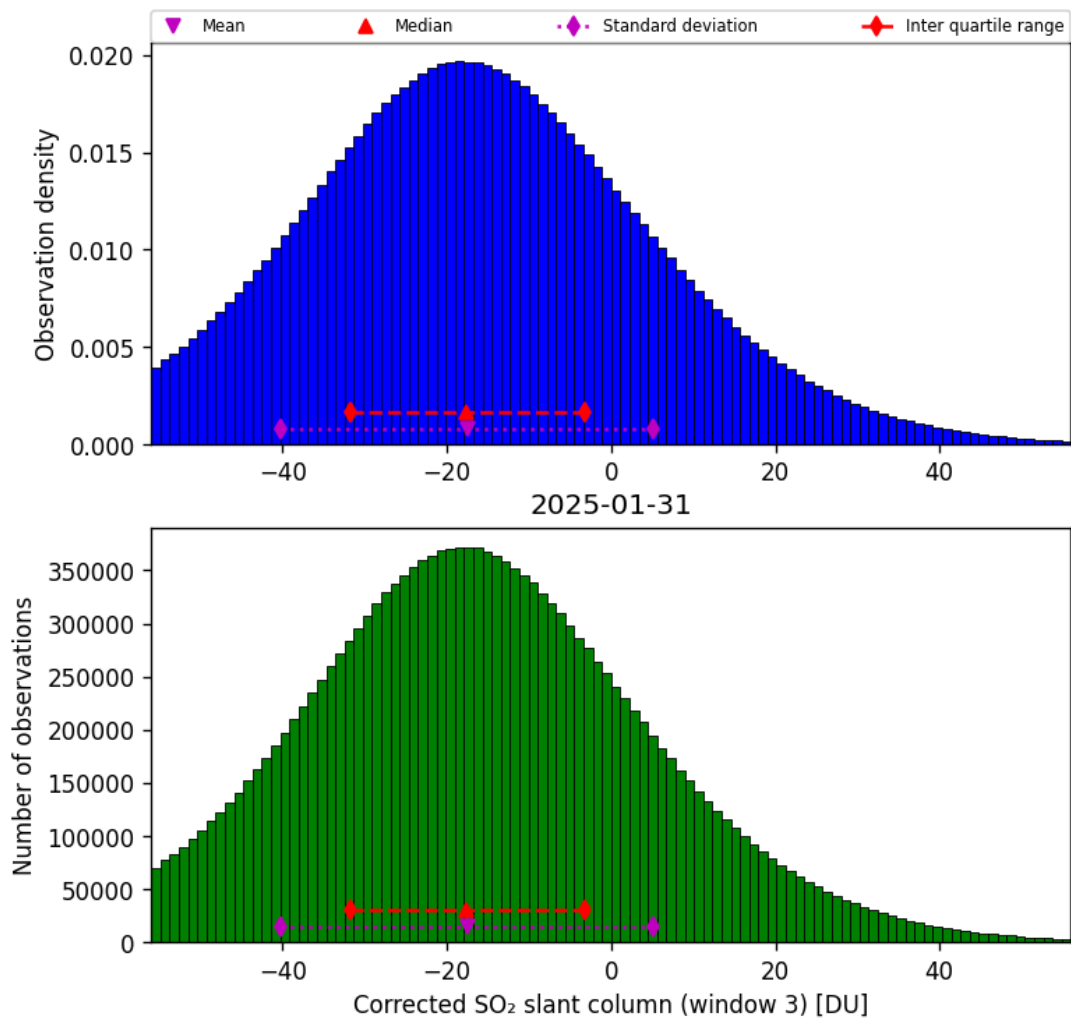
Figure 73: Histogram of “Corrected SO 2 slant column (window 3)” for 2025-01-31 to 2025-01-31
