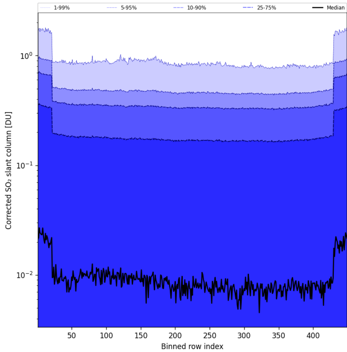
Figure 87: Along track statistics of “Corrected SO 2 slant column” for 2025-01-31 to 2025-01-31
