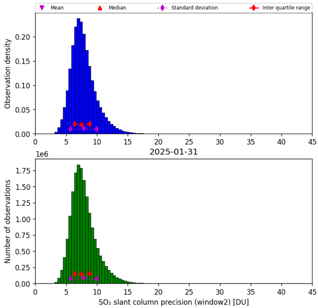
Figure 68: Histogram of “SO 2 slant column precision (window2)” for 2025-01-31 to 2025-01-31
