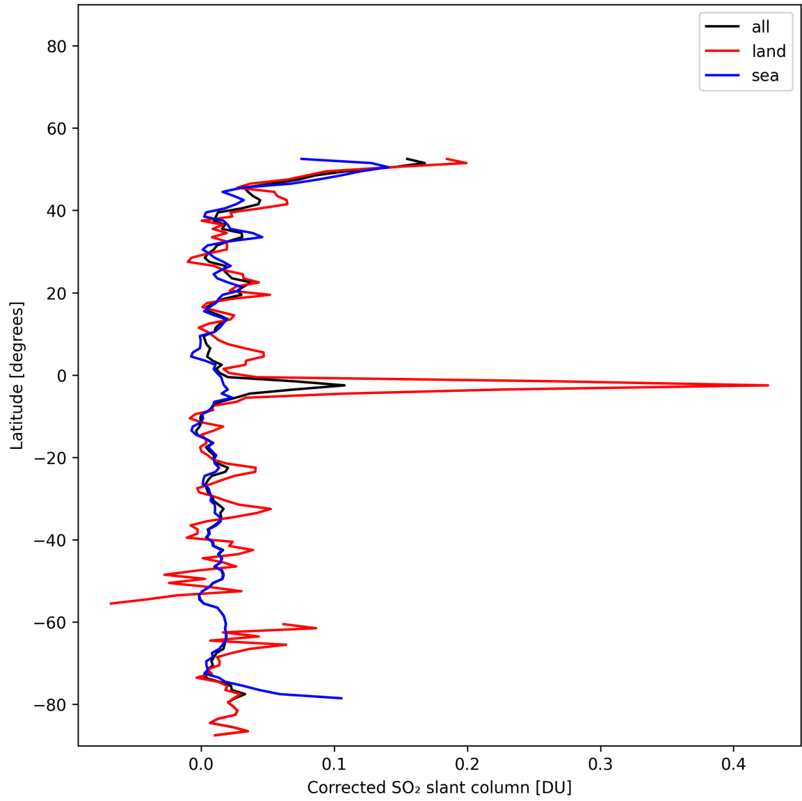
Figure 33: Zonal average of “Corrected SO 2 slant column” for 2025-01-31 to 2025-01-31.
