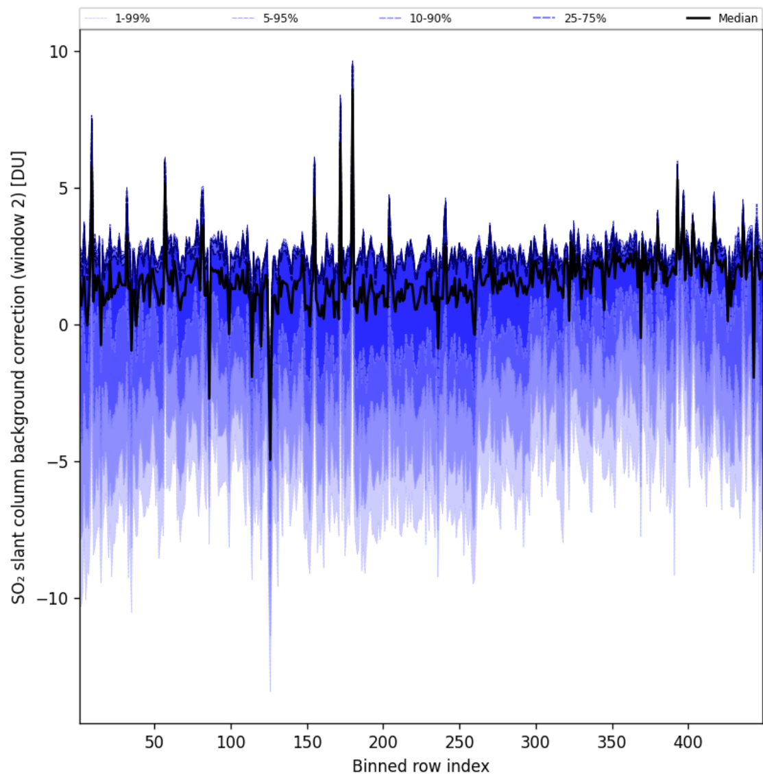
Figure 97: Along track statistics of “SO 2 slant column background correction (window 2)” for 2025-01-31 to 2025-01-31
