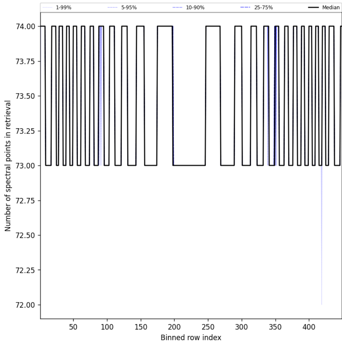
Figure 110: Along track statistics of “Number of spectral points in retrieval” for 2025-01-31 to 2025-01-31
