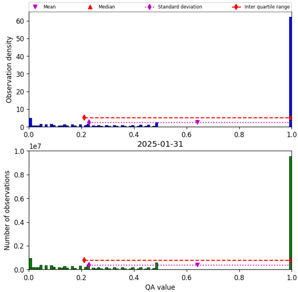
Figure 57: Histogram of “QA value” for 2025-01-31 to 2025-01-31
