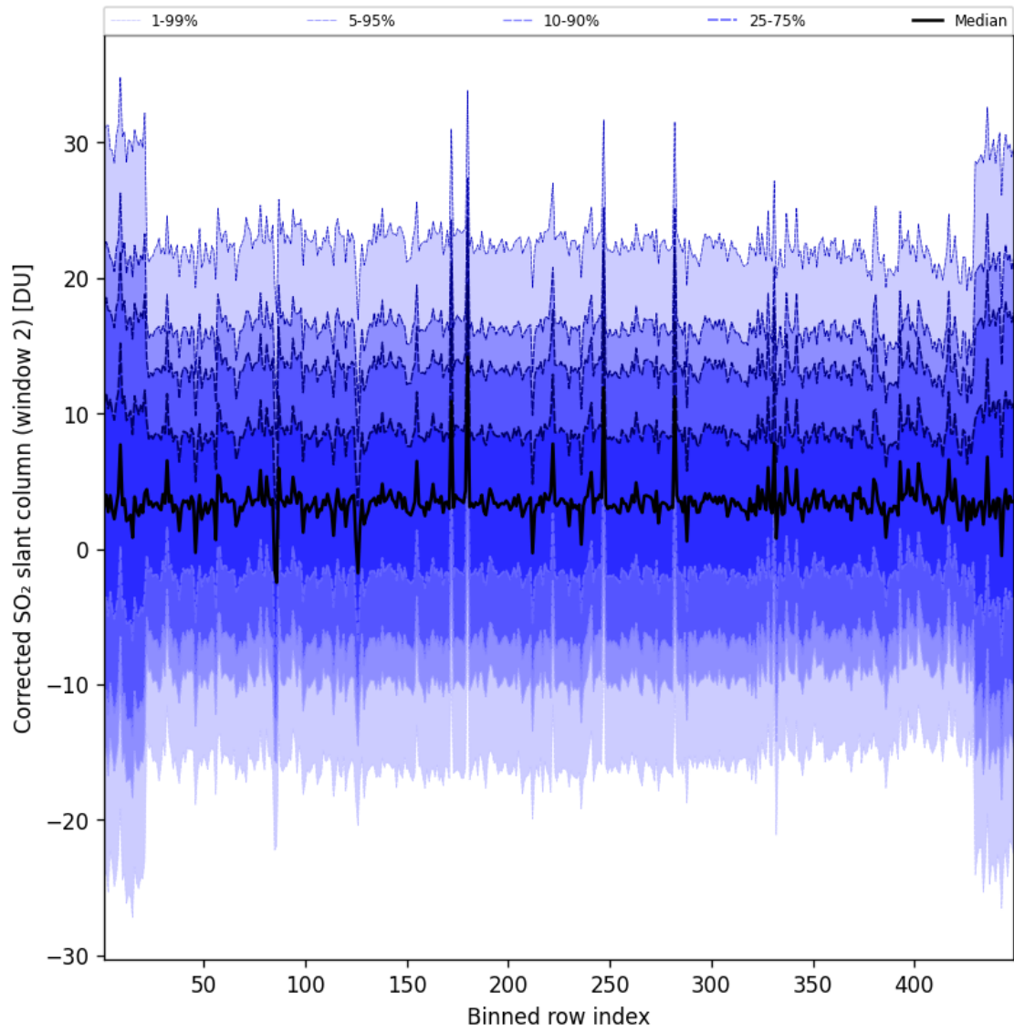
Figure 96: Along track statistics of “Corrected SO 2 slant column (window 2)” for 2025-01-31 to 2025-01-31
