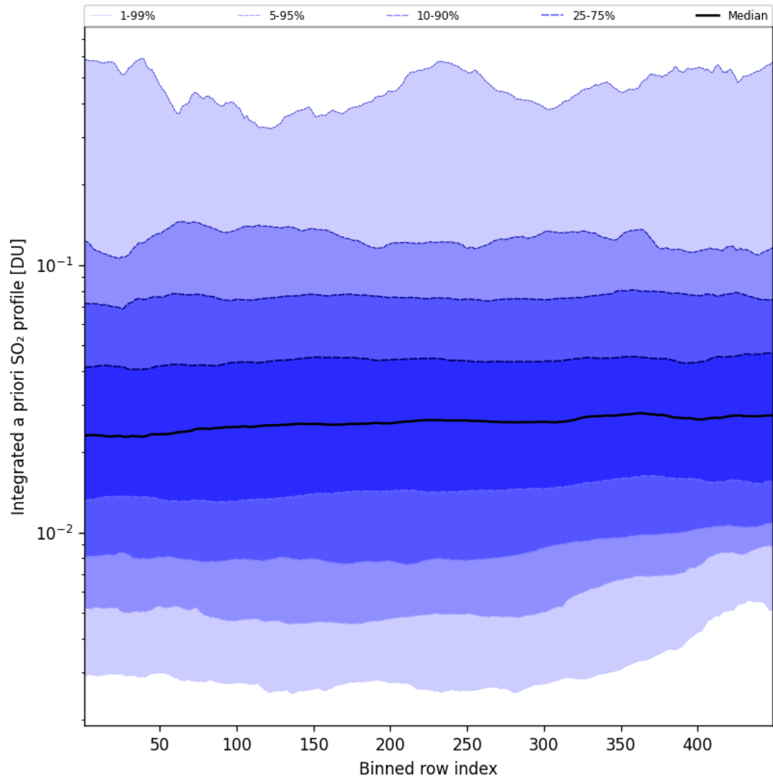
Figure 103: Along track statistics of “Integrated a priori SO 2 profile” for 2025-01-31 to 2025-01-31
