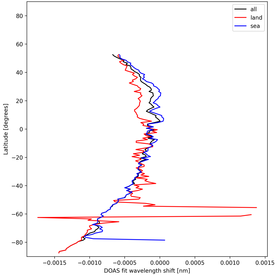
Figure 50: Zonal average of “DOAS fit wavelength shift” for 2025-01-31 to 2025-01-31.
