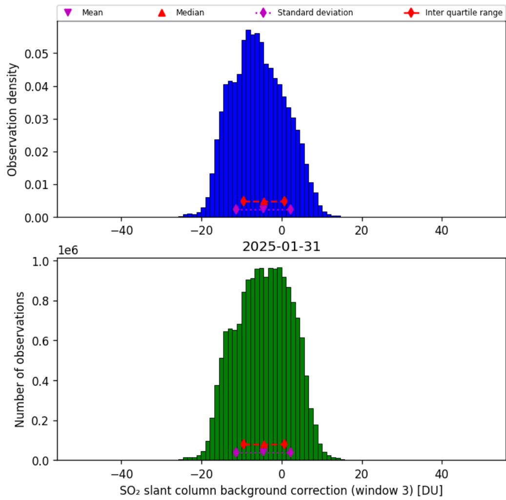
Figure 74: Histogram of “SO 2 slant column background correction (window 3)” for 2025-01-31 to 2025-01-31
