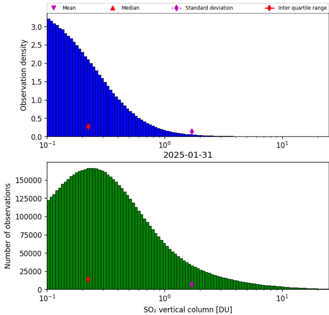
Figure 58: Histogram of “SO 2 vertical column” for 2025-01-31 to 2025-01-31
