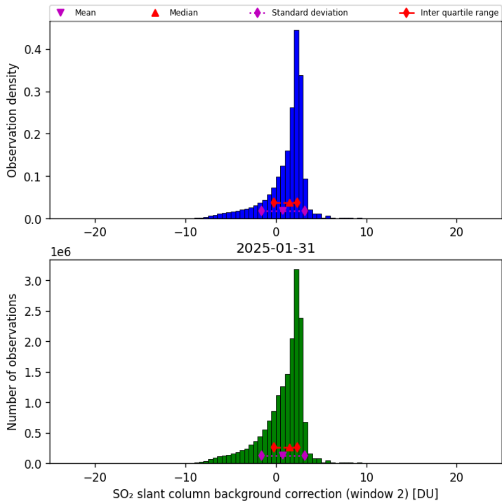
Figure 70: Histogram of “SO 2 slant column background correction (window 2)” for 2025-01-31 to 2025-01-31
