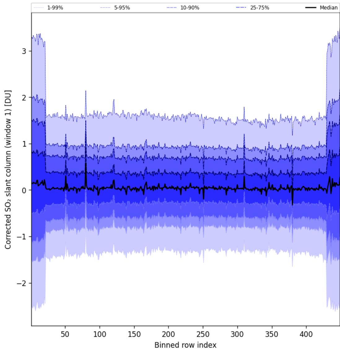
Figure 92: Along track statistics of "Corrected SO 2 slant column (window 1)" for 2025-01-31 to 2025-01-31
