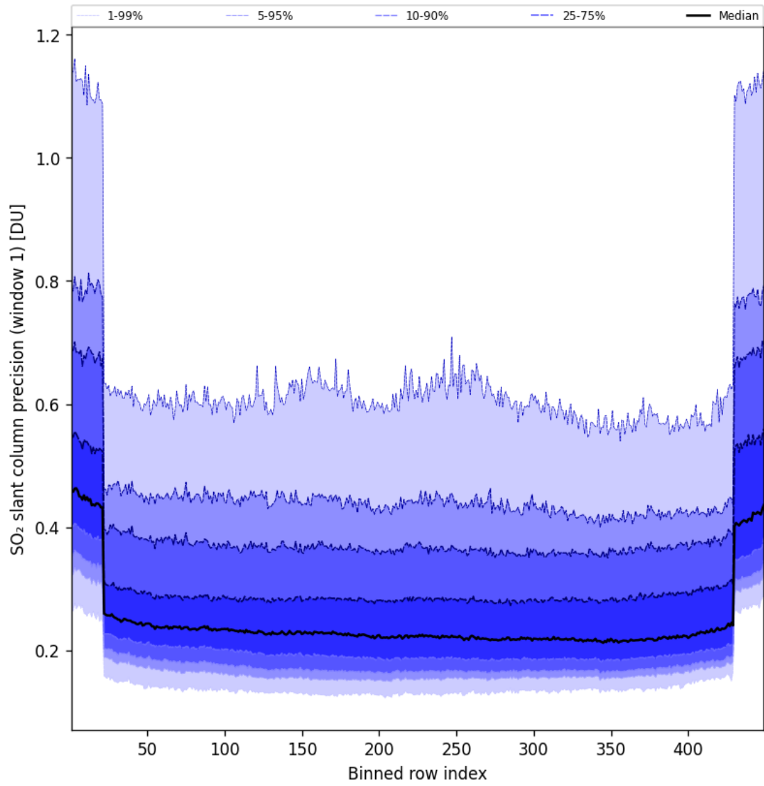
Figure 91: Along track statistics of “SO 2 slant column precision (window 1)” for 2025-01-31 to 2025-01-31
