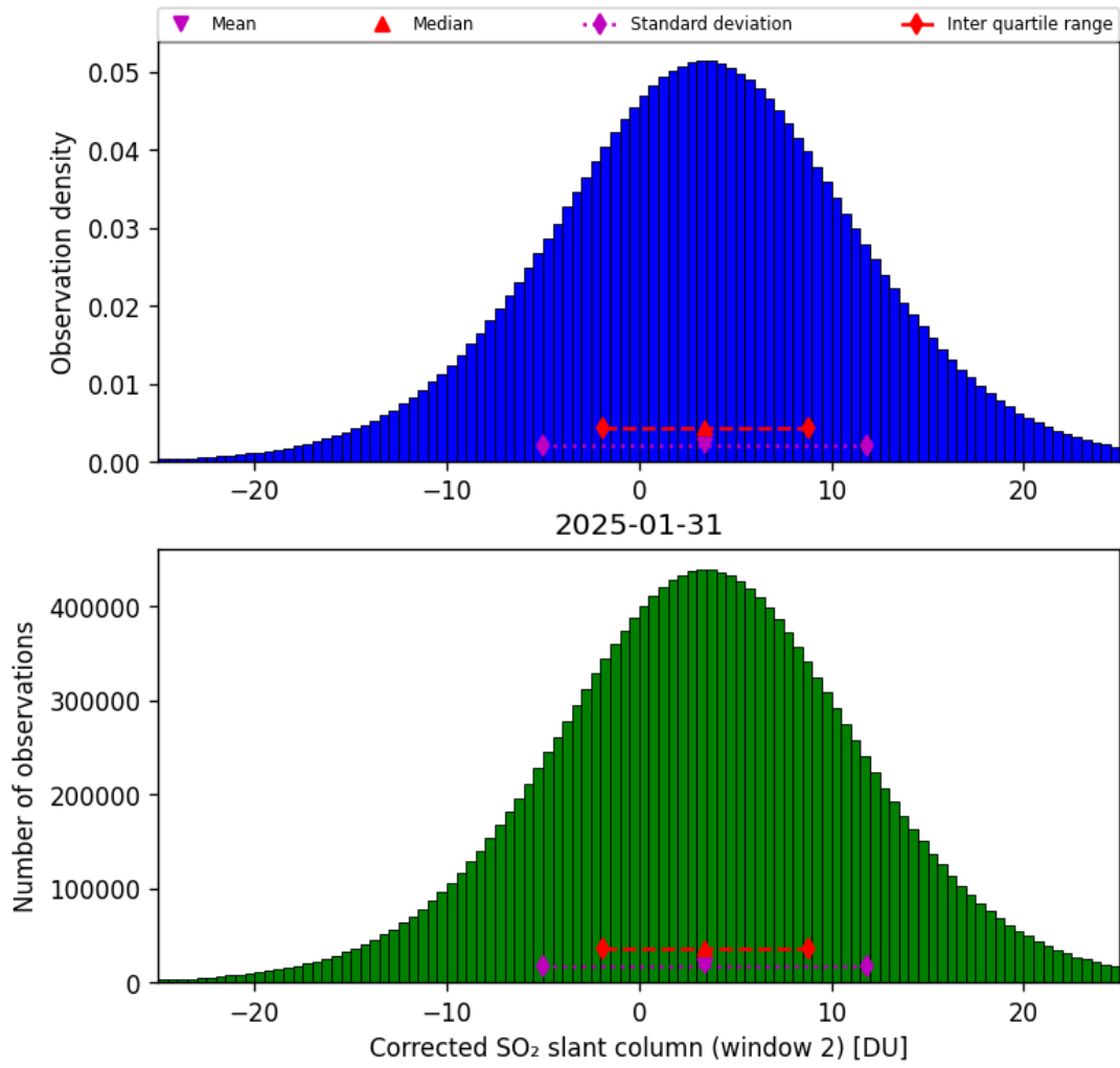
Figure 69: Histogram of “Corrected SO 2 slant column (window 2)” for 2025-01-31 to 2025-01-31
