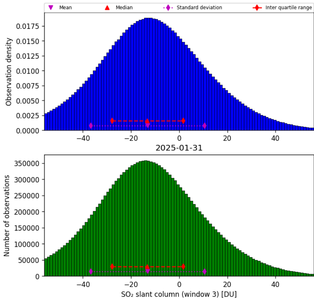
Figure 71: Histogram of “SO 2 slant column (window 3)” for 2025-01-31 to 2025-01-31
