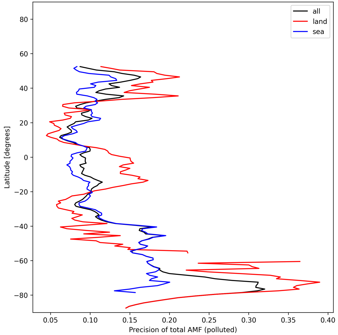
Figure 54: Zonal average of “Precision of total AMF (polluted)” for 2025-01-31 to 2025-01-31.
