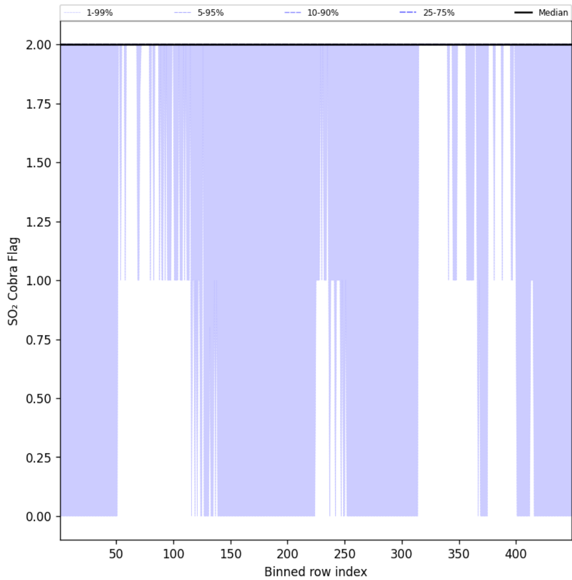
Figure 102: Along track statistics of “SO 2 Cobra Flag” for 2025-01-31 to 2025-01-31
