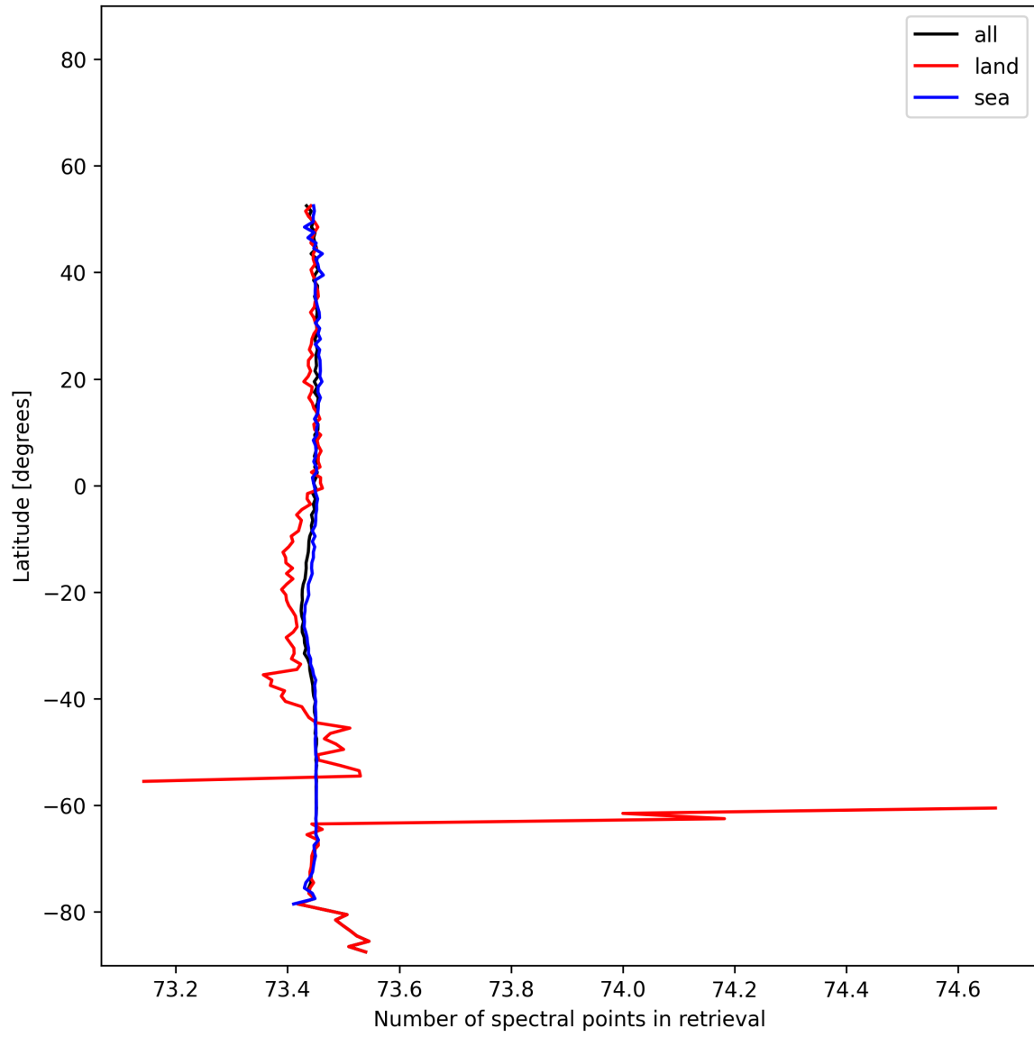
Figure 56: Zonal average of “Number of spectral points in retrieval” for 2025-01-31 to 2025-01-31.
