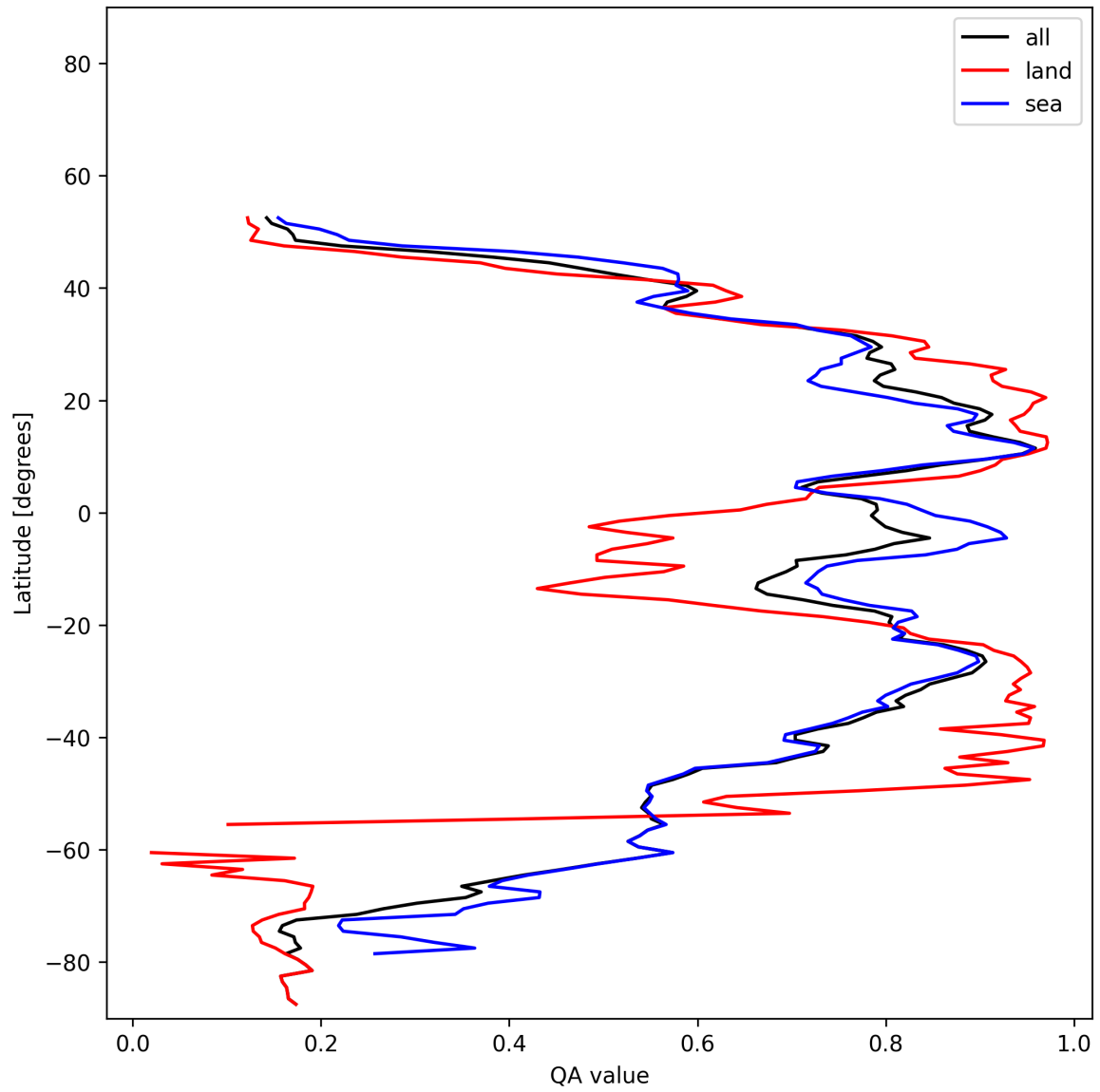
Figure 30: Zonal average of “QA value” for 2025-01-31 to 2025-01-31.
