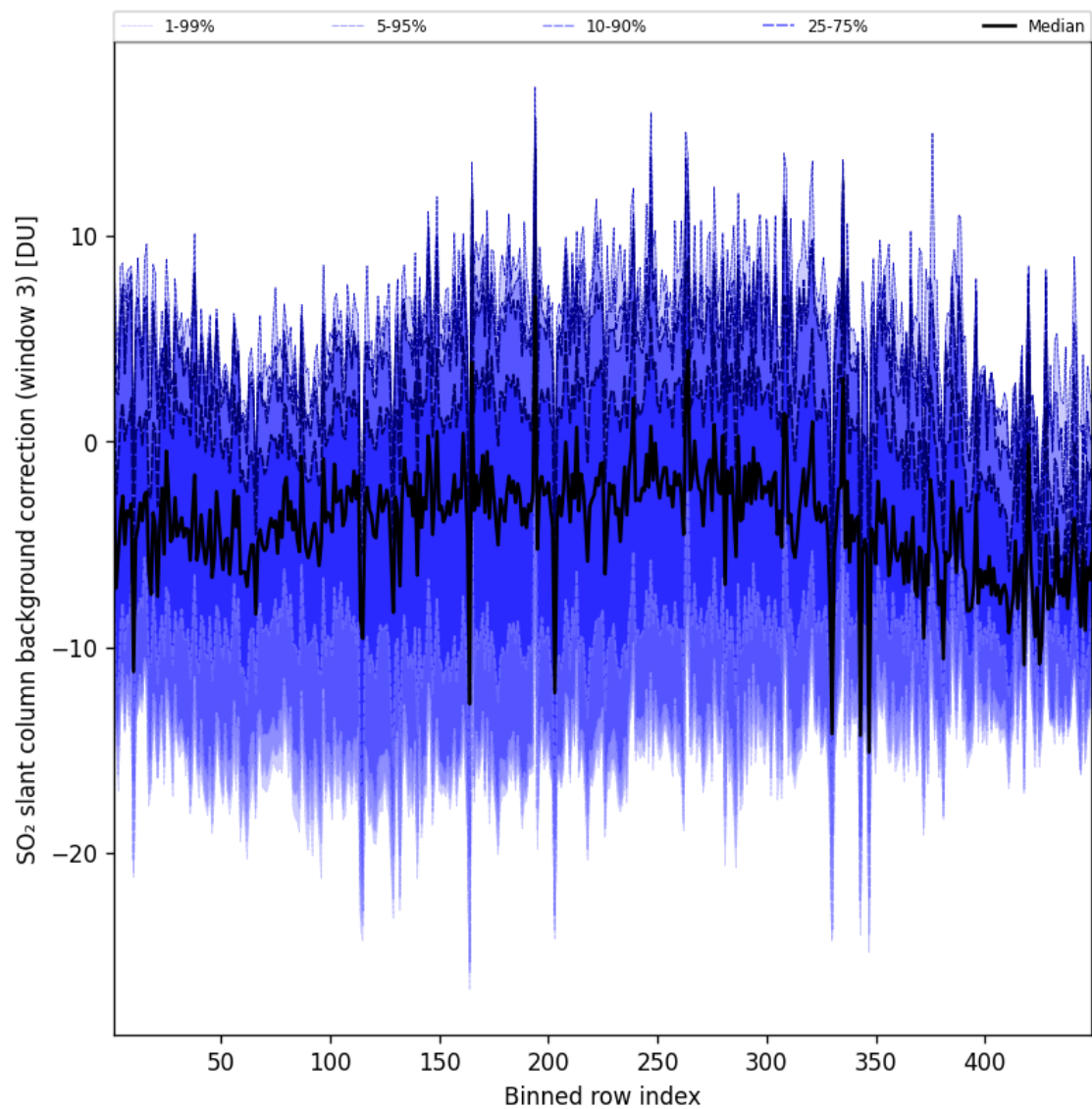
Figure 101: Along track statistics of “SO 2 slant column background correction (window 3)” for 2025-01-31 to 2025-01-31
