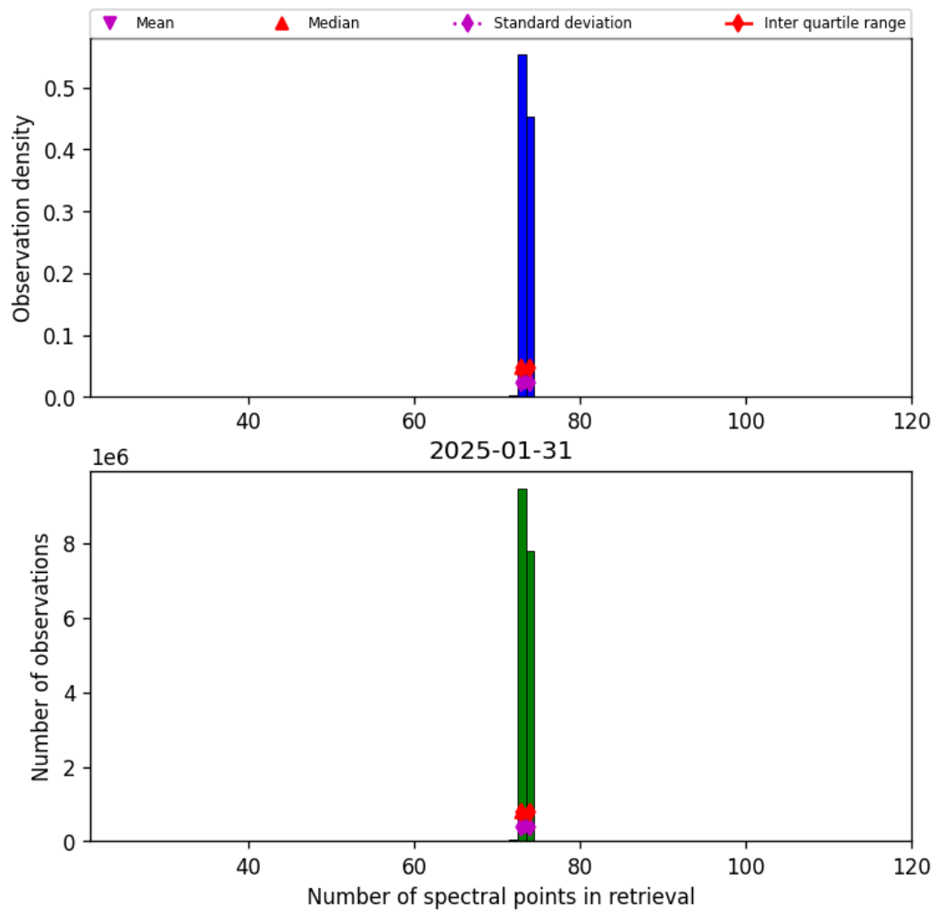
Figure 83: Histogram of “Number of spectral points in retrieval” for 2025-01-31 to 2025-01-31
