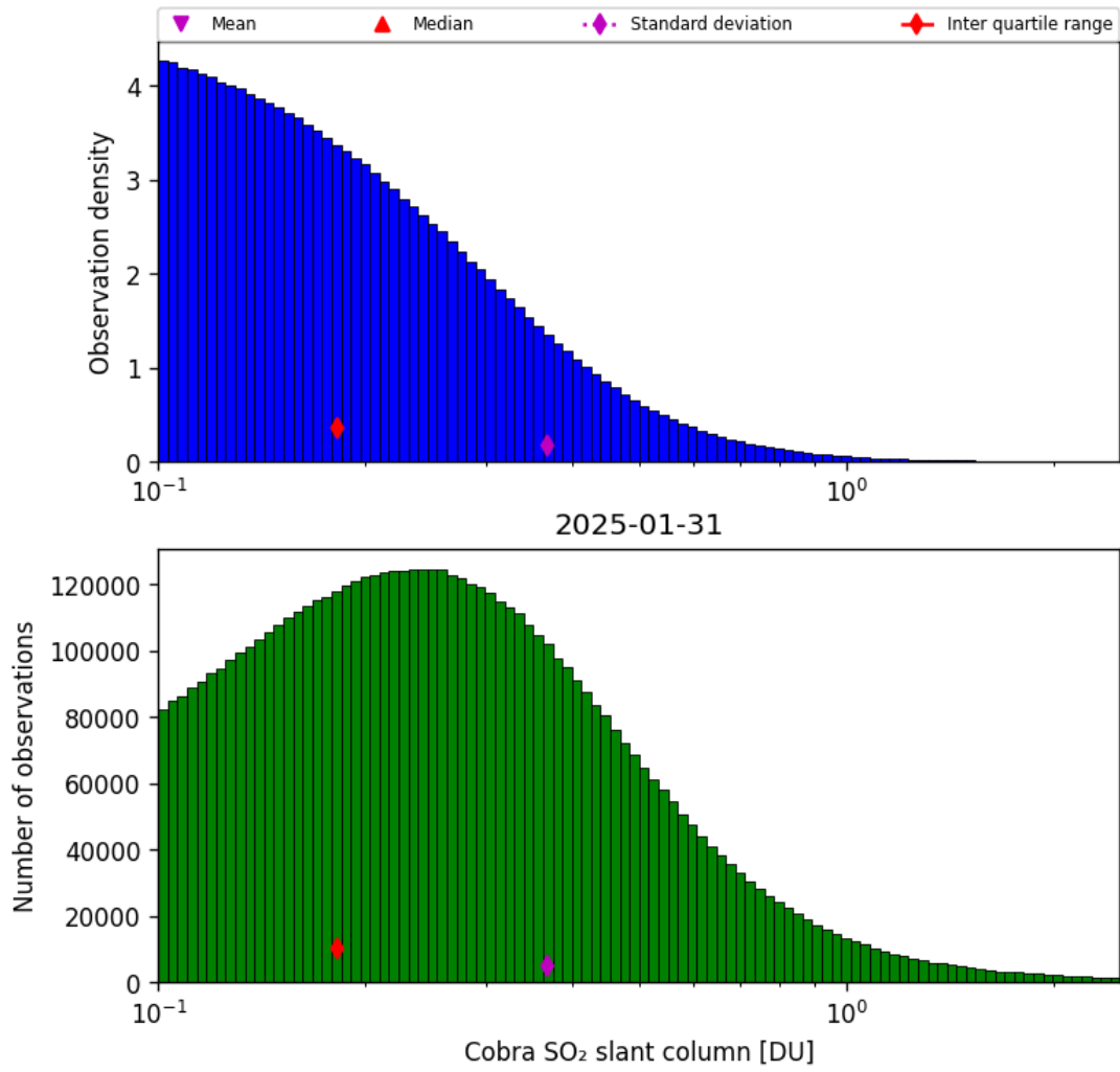
Figure 61: Histogram of “Cobra SO 2 slant column” for 2025-01-31 to 2025-01-31
