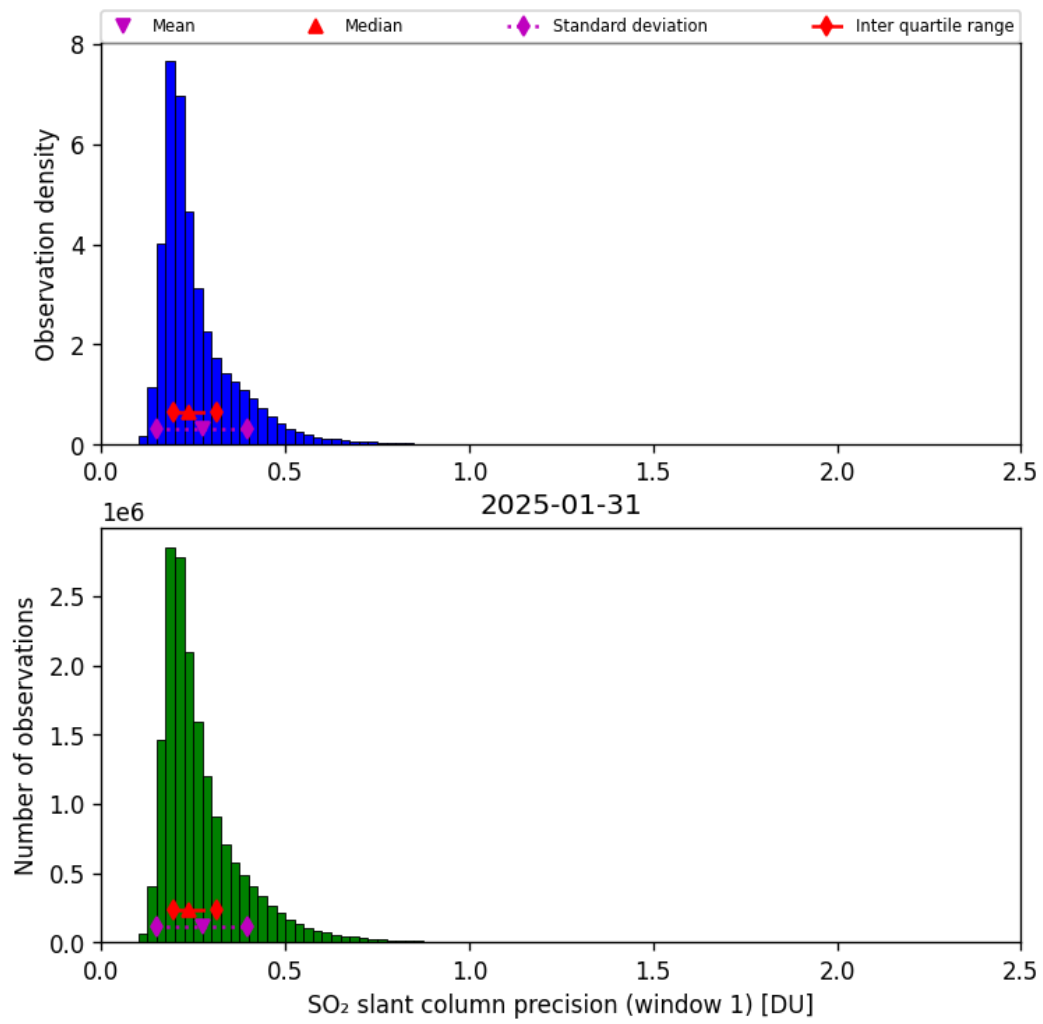
Figure 64: Histogram of “SO 2 slant column precision (window 1)” for 2025-01-31 to 2025-01-31
