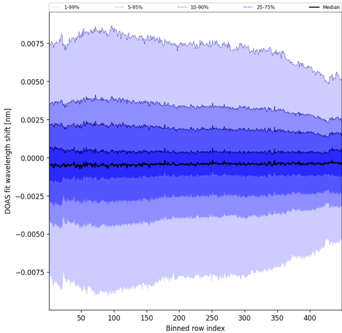
Figure 104: Along track statistics of “DOAS fit wavelength shift” for 2025-01-31 to 2025-01-31
