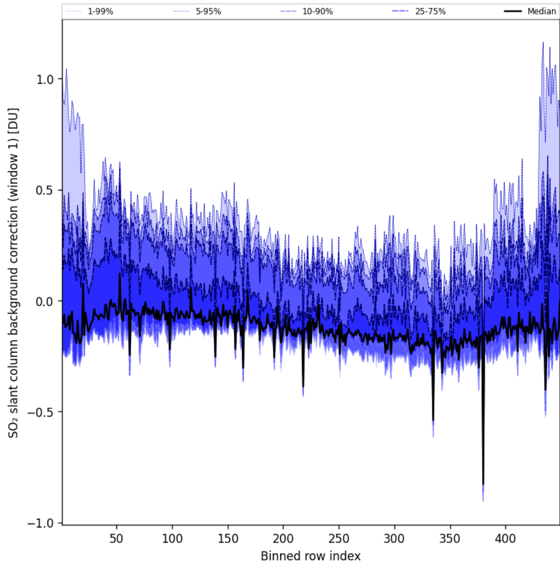
Figure 93: Along track statistics of “SO 2 slant column background correction (window 1)” for 2025-01-31 to 2025-01-31
