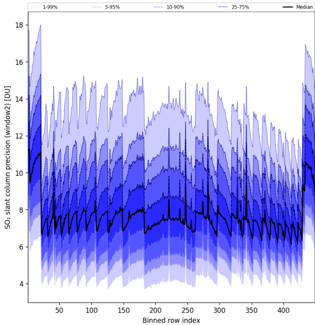
Figure 95: Along track statistics of “SO 2 slant column precision (window2)” for 2025-01-31 to 2025-01-31
