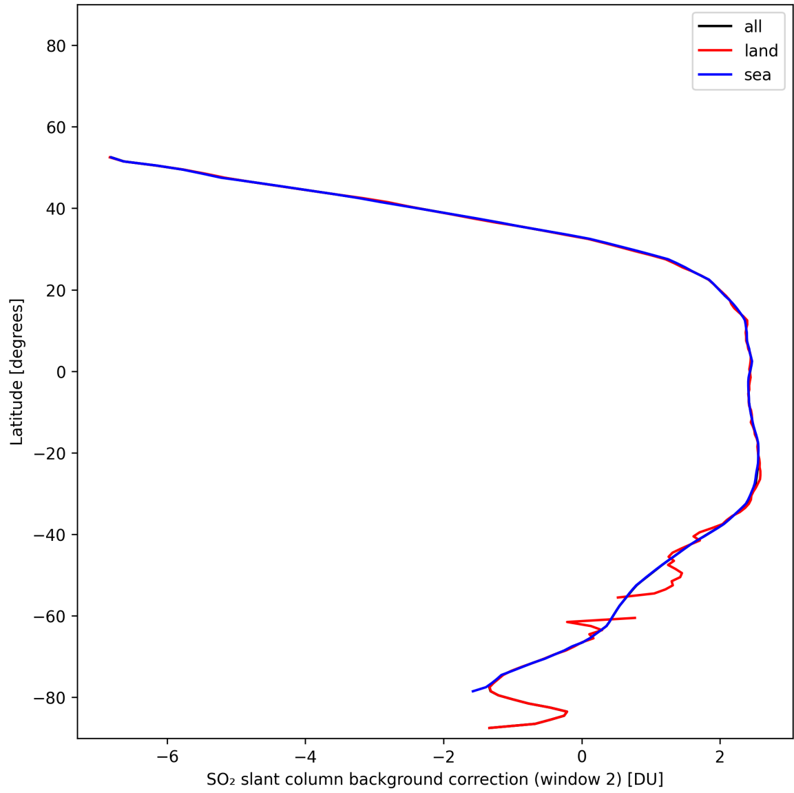
Figure 43: Zonal average of “SO 2 slant column background correction (window 2)” for 2025-01-31 to 2025-01-31.
