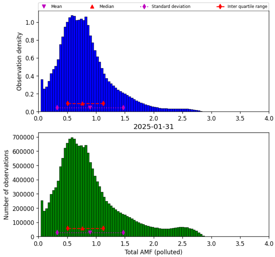
Figure 80: Histogram of “Total AMF (polluted)” for 2025-01-31 to 2025-01-31
