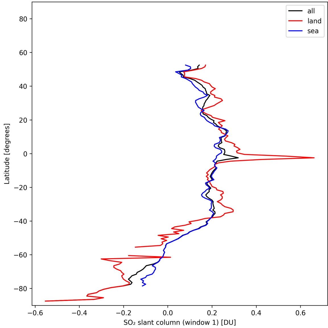
Figure 36: Zonal average of “SO 2 slant column (window 1)” for 2025-01-31 to 2025-01-31.
