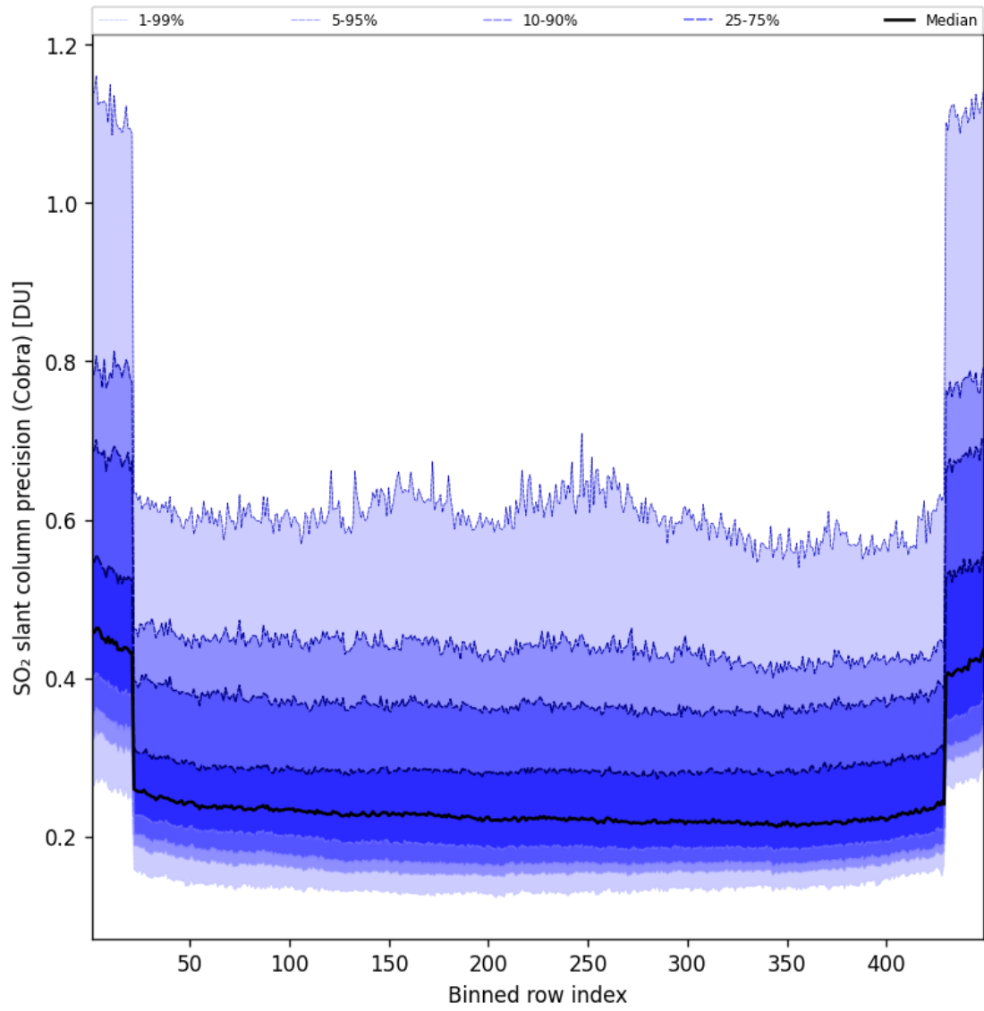
Figure 89: Along track statistics of “SO 2 slant column precision (Cobra)” for 2025-01-31 to 2025-01-31
