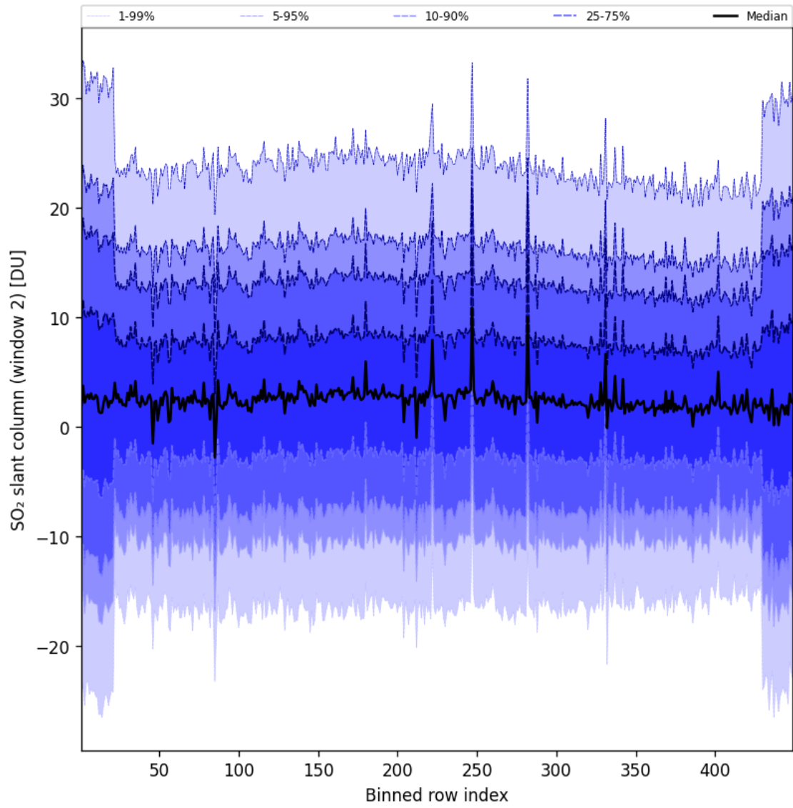
Figure 94: Along track statistics of “SO 2 slant column (window 2)” for 2025-01-31 to 2025-01-31
