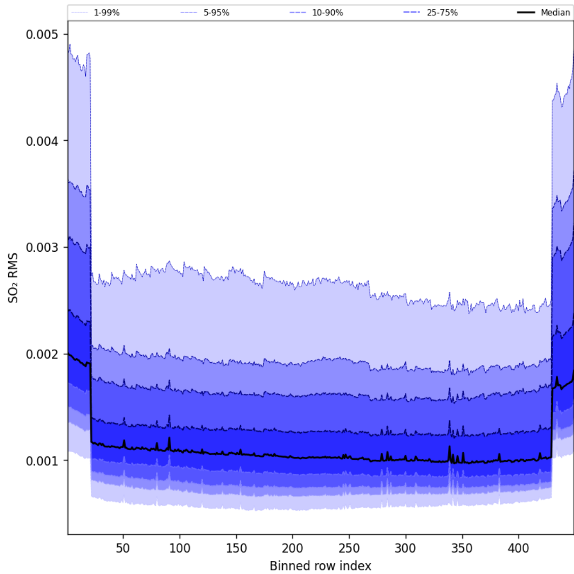
Figure 106: Along track statistics of “SO 2 RMS” for 2025-01-31 to 2025-01-31
