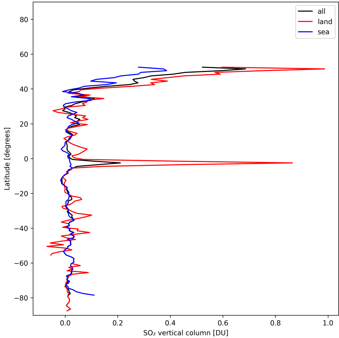
Figure 31: Zonal average of “SO 2 vertical column” for 2025-01-31 to 2025-01-31.
