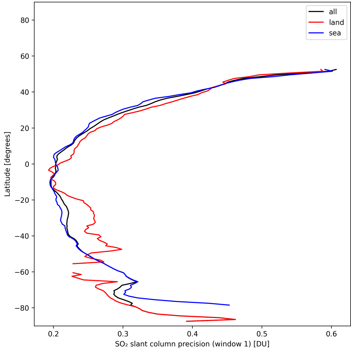
Figure 37: Zonal average of “SO 2 slant column precision (window 1)” for 2025-01-31 to 2025-01-31.
