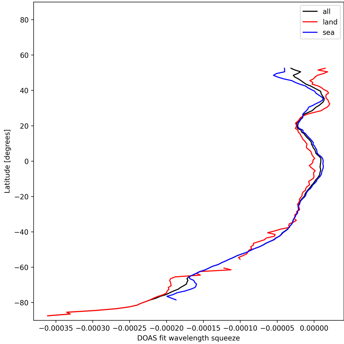
Figure 51: Zonal average of “DOAS fit wavelength squeeze” for 2025-01-31 to 2025-01-31.
