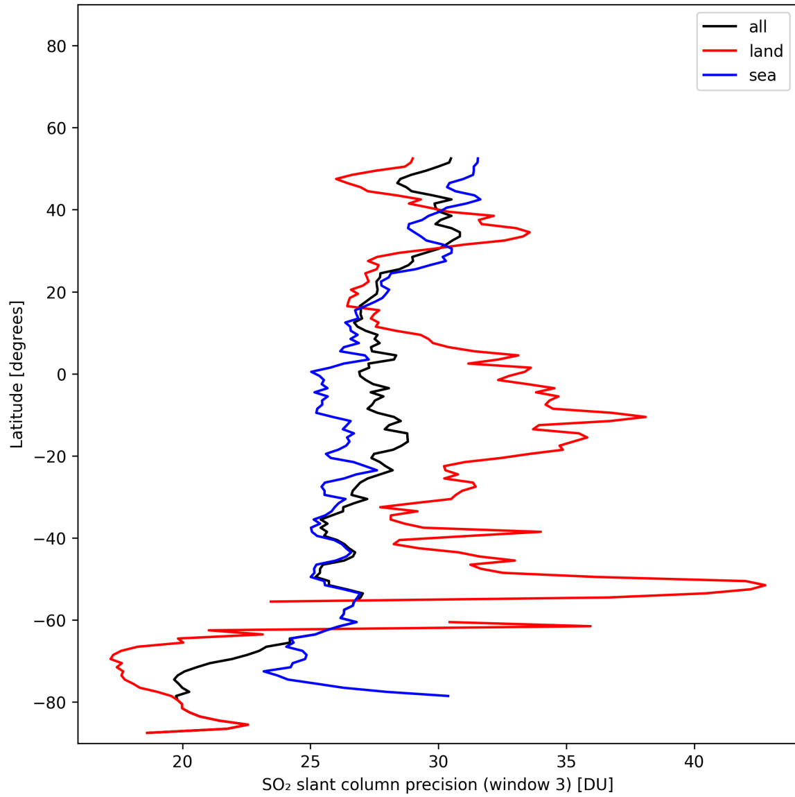
Figure 45: Zonal average of “SO 2 slant column precision (window 3)” for 2025-01-31 to 2025-01-31.
