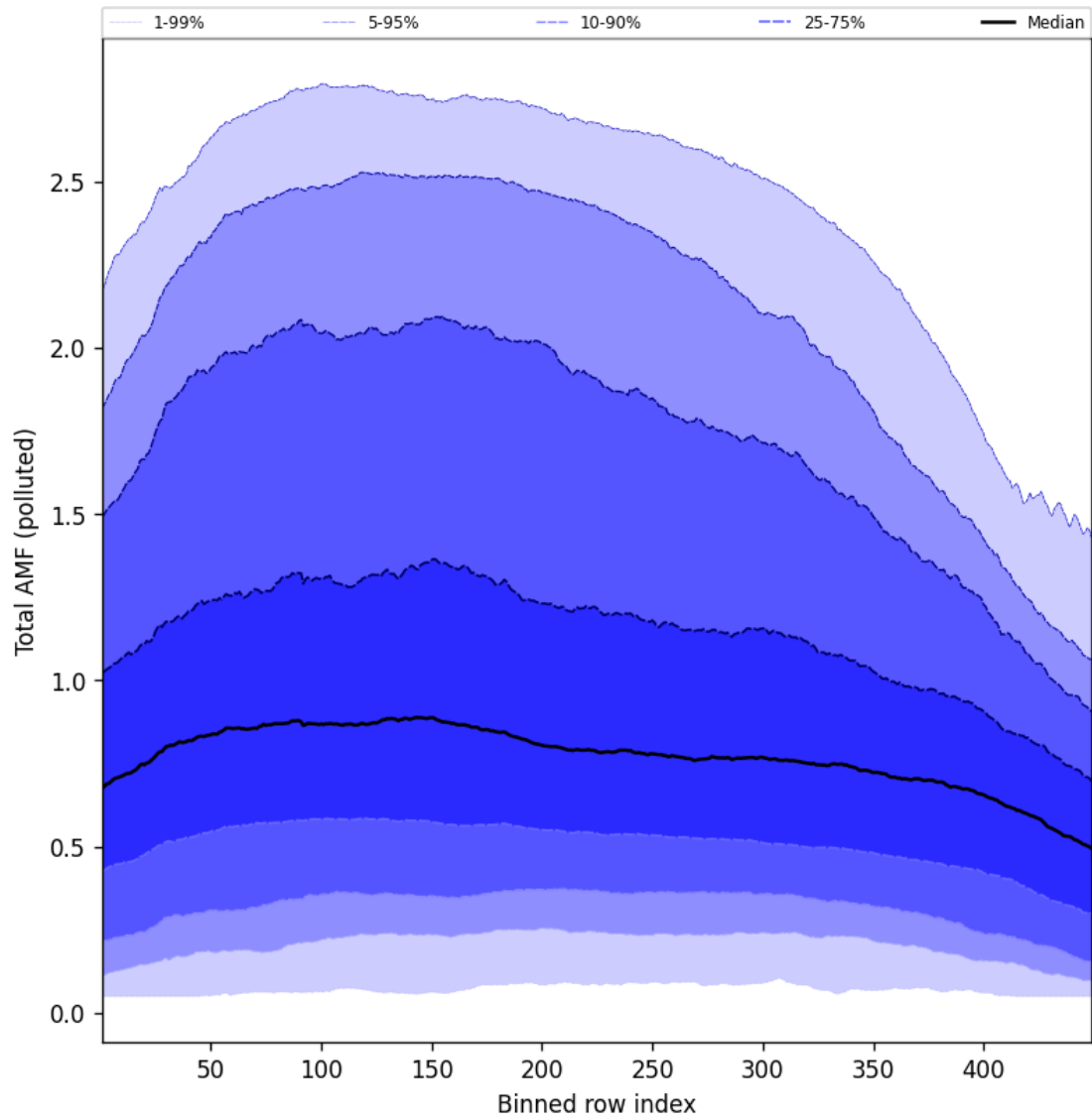
Figure 107: Along track statistics of “Total AMF (polluted)” for 2025-01-31 to 2025-01-31
