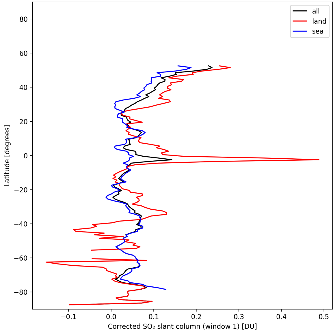
Figure 38: Zonal average of “Corrected SO 2 slant column (window 1)” for 2025-01-31 to 2025-01-31.
