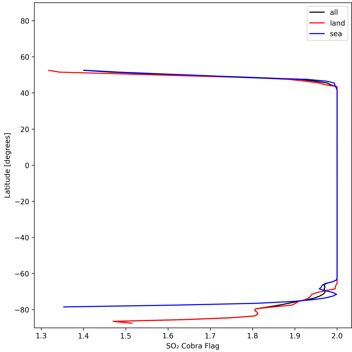
Figure 48: Zonal average of "SO 2 Cobra Flag" for 2025-01-31 to 2025-01-31.
