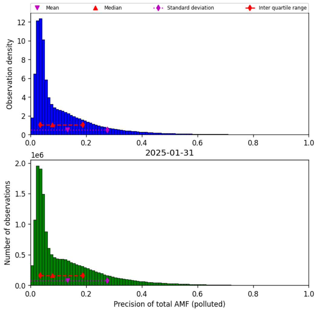
Figure 81: Histogram of “Precision of total AMF (polluted)” for 2025-01-31 to 2025-01-31
