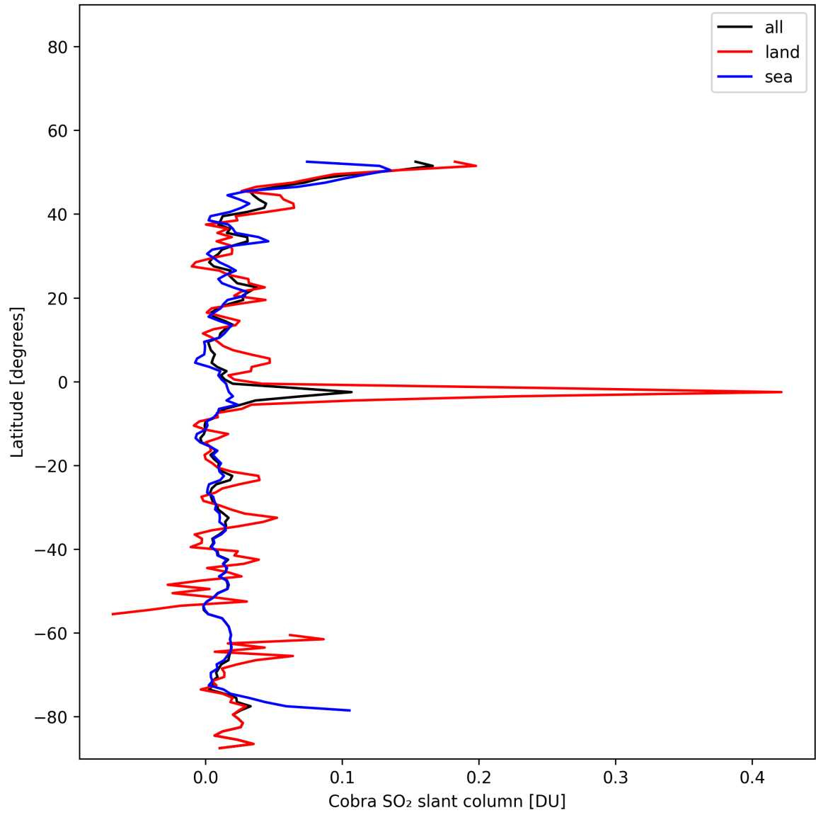
Figure 34: Zonal average of “Cobra SO 2 slant column” for 2025-01-31 to 2025-01-31.
