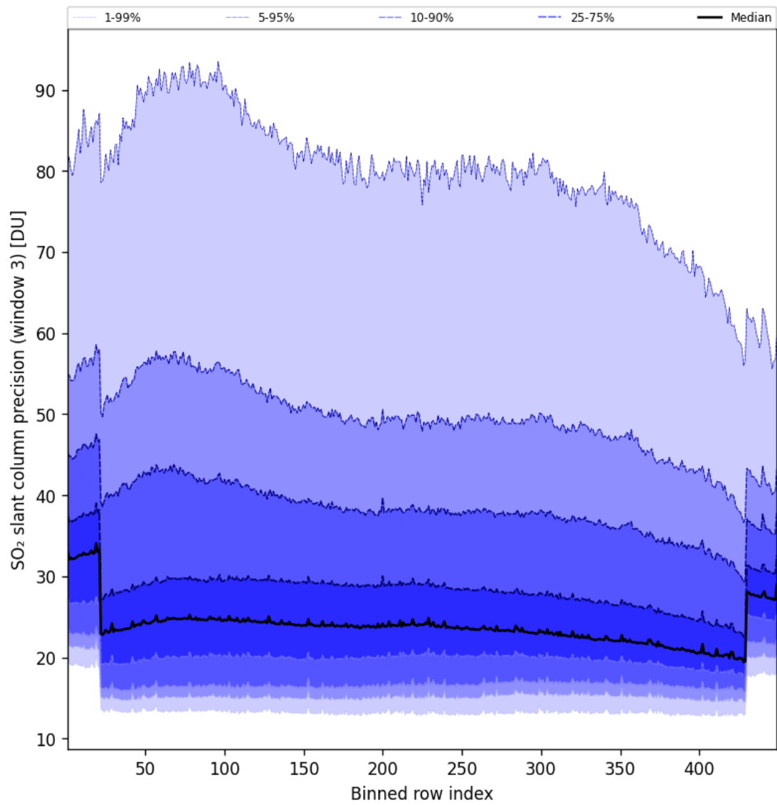
Figure 99: Along track statistics of “SO 2 slant column precision (window 3)” for 2025-01-31 to 2025-01-31
