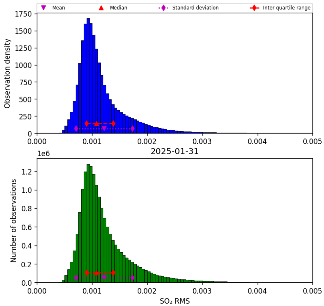
Figure 79: Histogram of “SO 2 RMS” for 2025-01-31 to 2025-01-31
