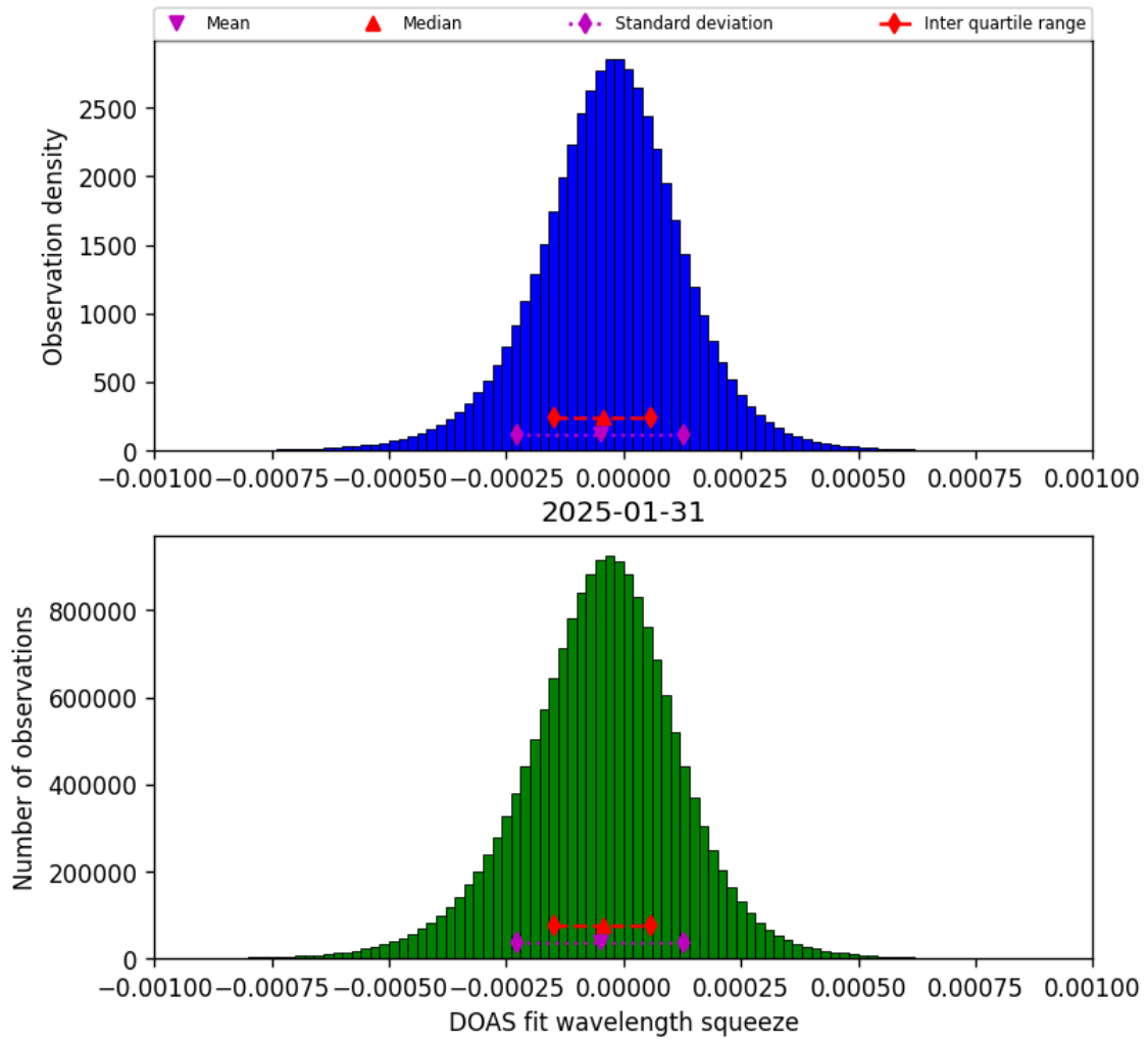
Figure 78: Histogram of “DOAS fit wavelength squeeze” for 2025-01-31 to 2025-01-31
