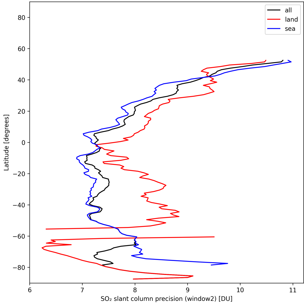
Figure 41: Zonal average of “SO 2 slant column precision (window2)” for 2025-01-31 to 2025-01-31.
