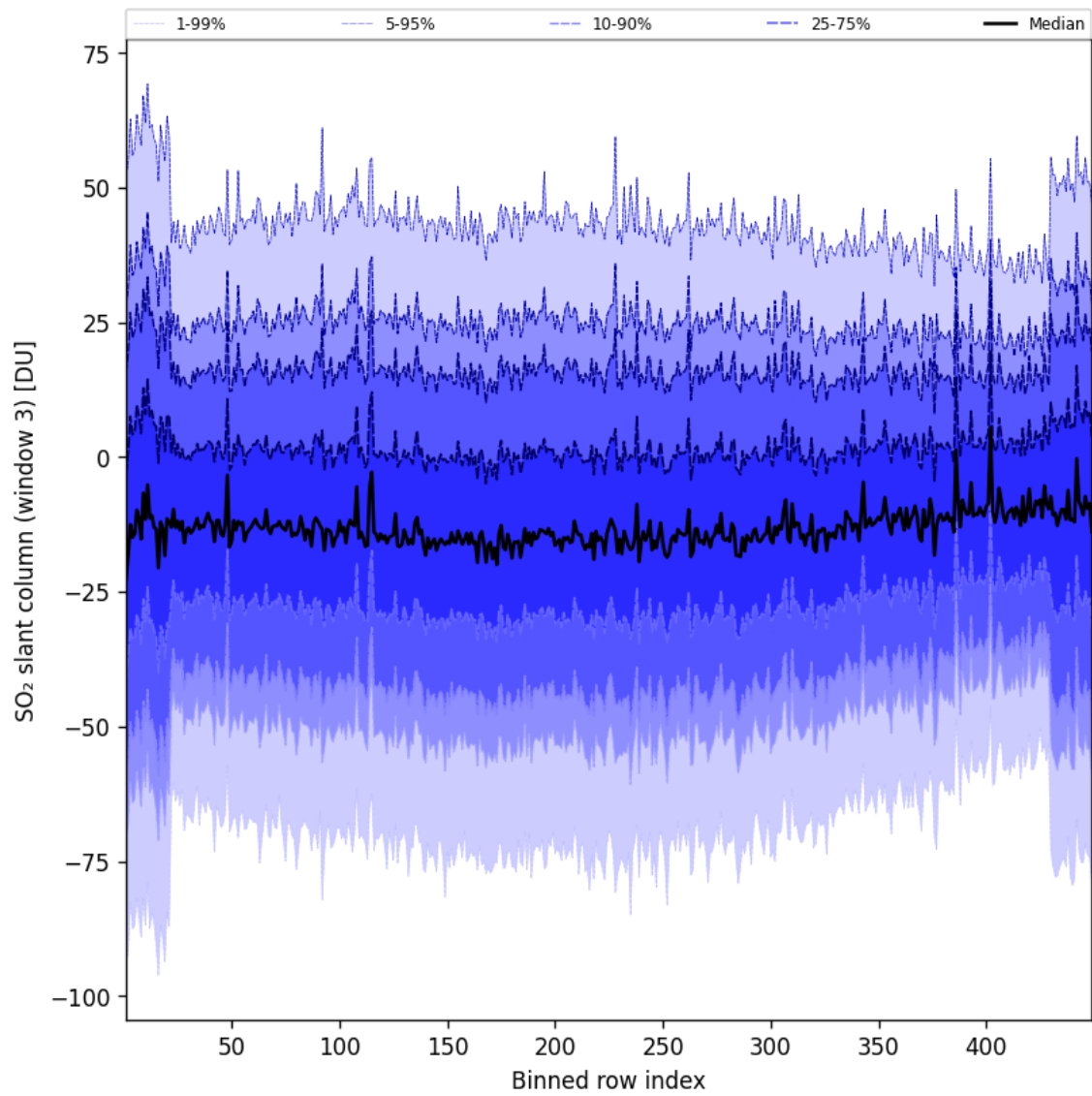
Figure 98: Along track statistics of “SO 2 slant column (window 3)” for 2025-01-31 to 2025-01-31
