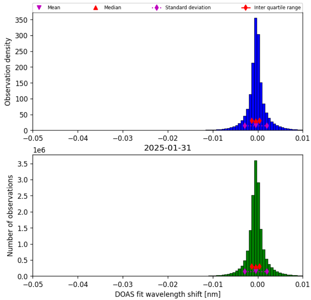
Figure 77: Histogram of “DOAS fit wavelength shift” for 2025-01-31 to 2025-01-31
