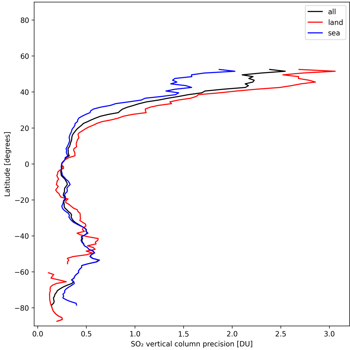
Figure 32: Zonal average of “SO 2 vertical column precision” for 2025-01-31 to 2025-01-31.
