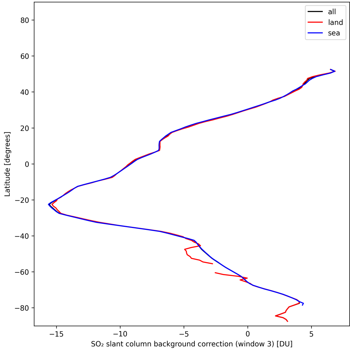
Figure 47: Zonal average of “SO 2 slant column background correction (window 3)” for 2025-01-31 to 2025-01-31.
