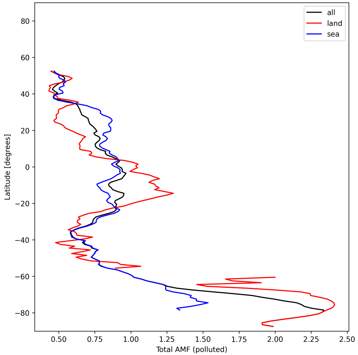
Figure 53: Zonal average of “Total AMF (polluted)” for 2025-01-31 to 2025-01-31.
