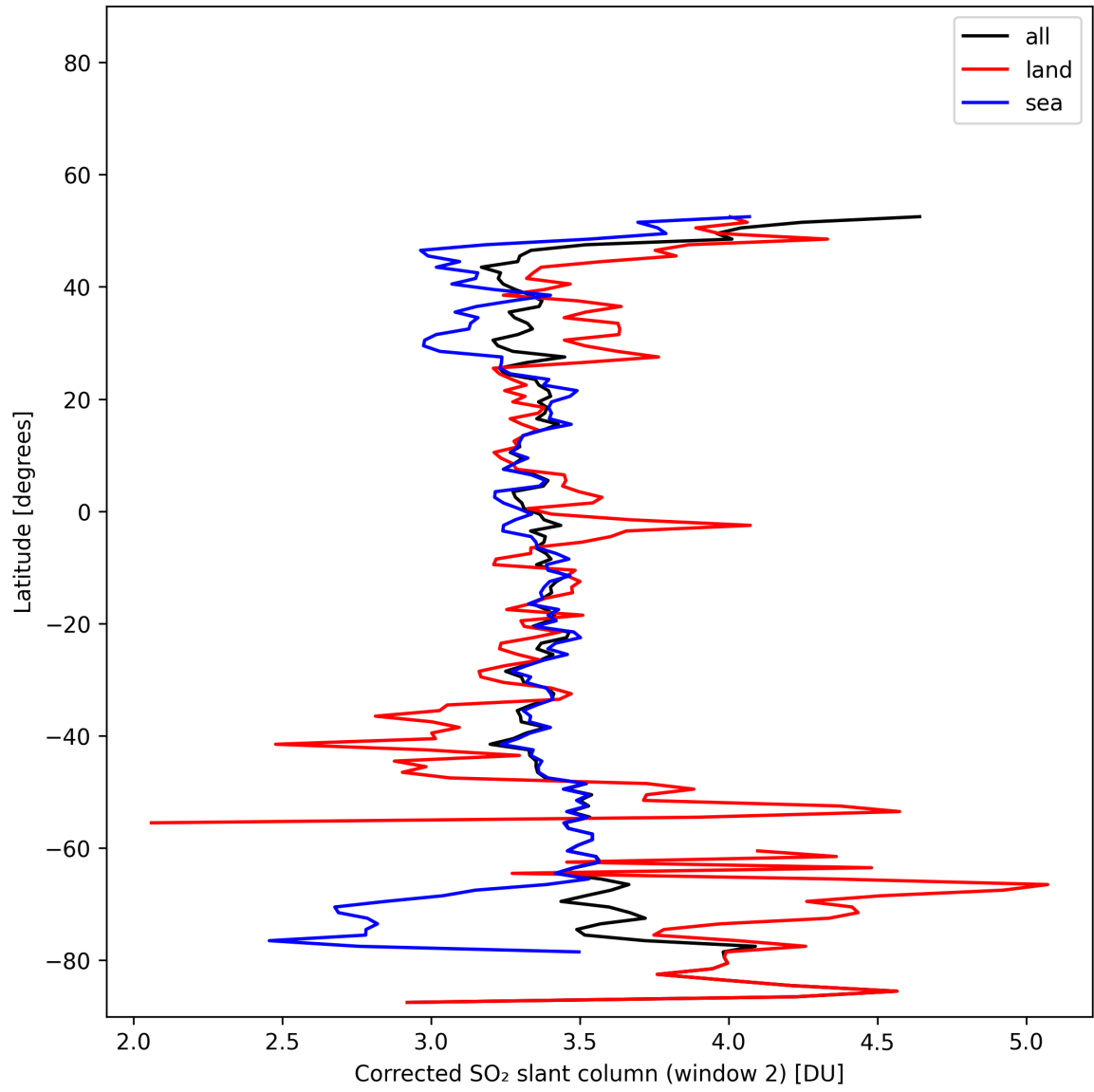
Figure 42: Zonal average of “Corrected SO 2 slant column (window 2)” for 2025-01-31 to 2025-01-31.
