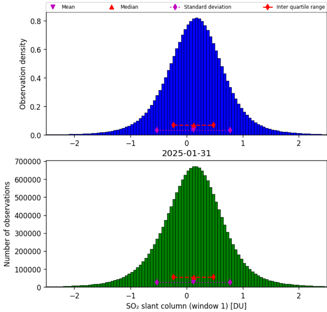
Figure 63: Histogram of “SO 2 slant column (window 1)” for 2025-01-31 to 2025-01-31
