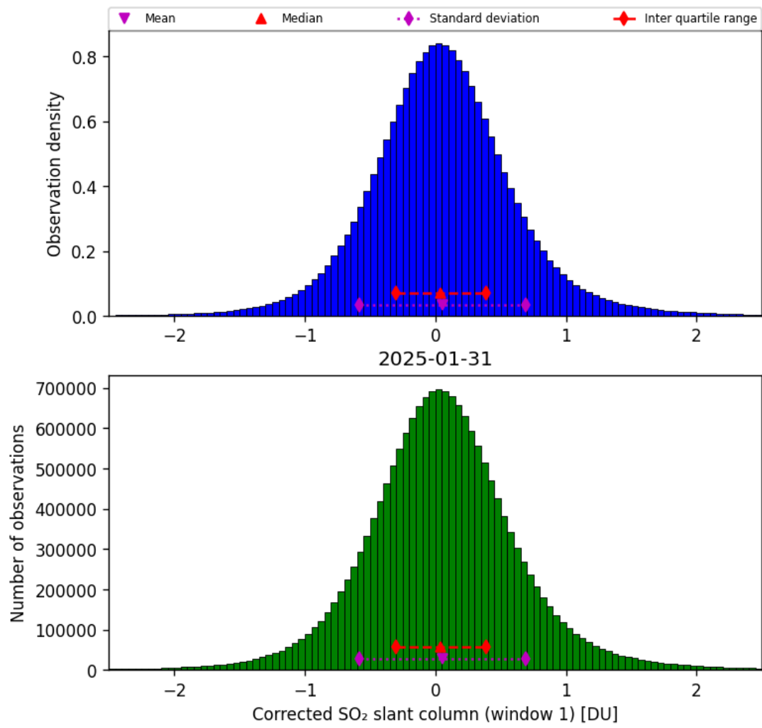
Figure 65: Histogram of “Corrected SO 2 slant column (window 1)” for 2025-01-31 to 2025-01-31
