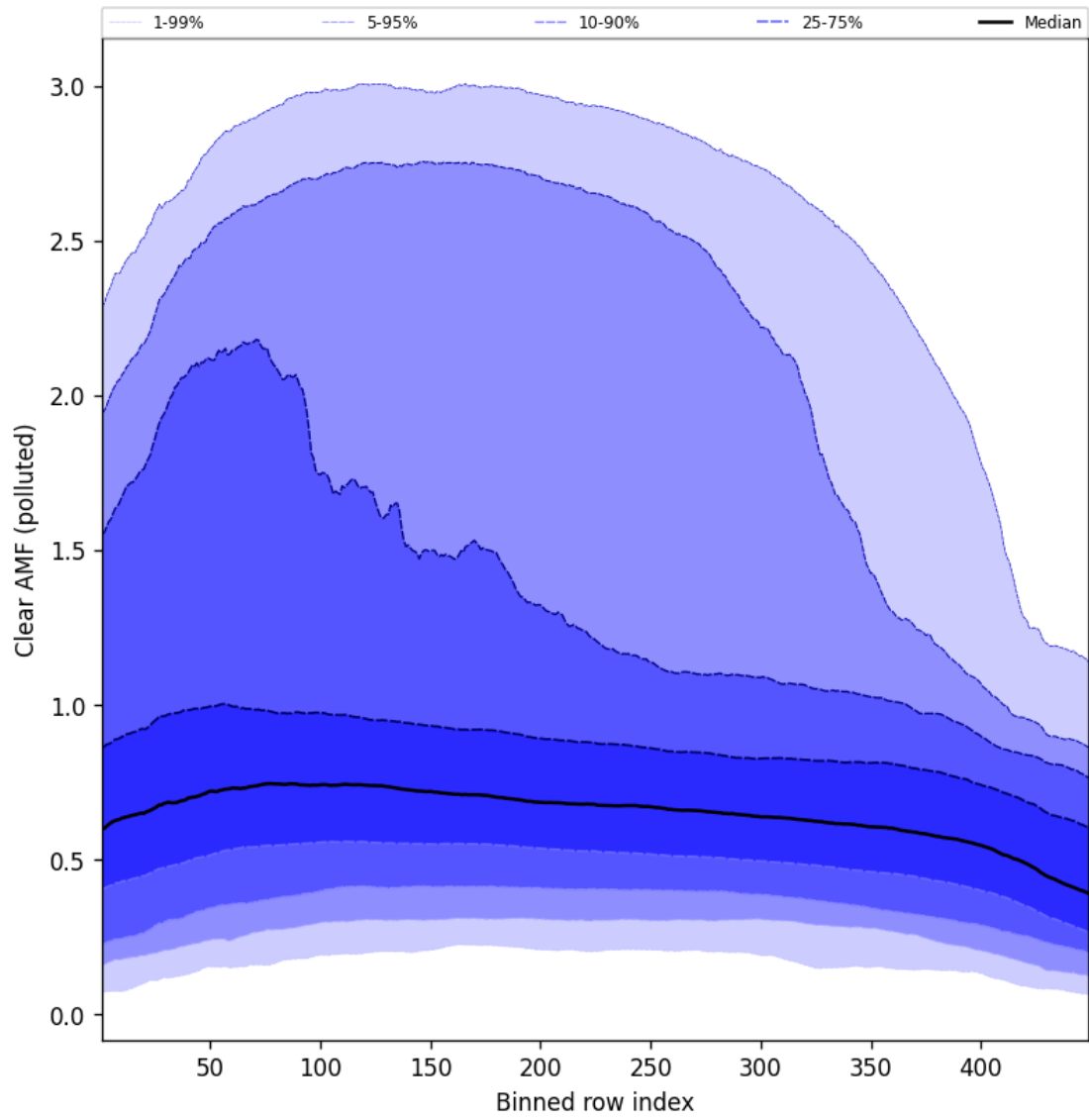
Figure 109: Along track statistics of “Clear AMF (polluted)” for 2025-01-31 to 2025-01-31
