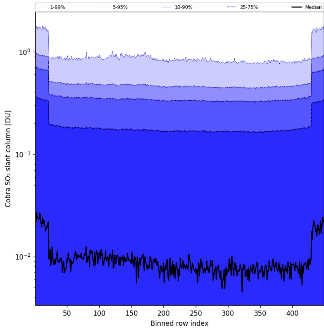
Figure 88: Along track statistics of “Cobra SO 2 slant column” for 2025-01-31 to 2025-01-31
