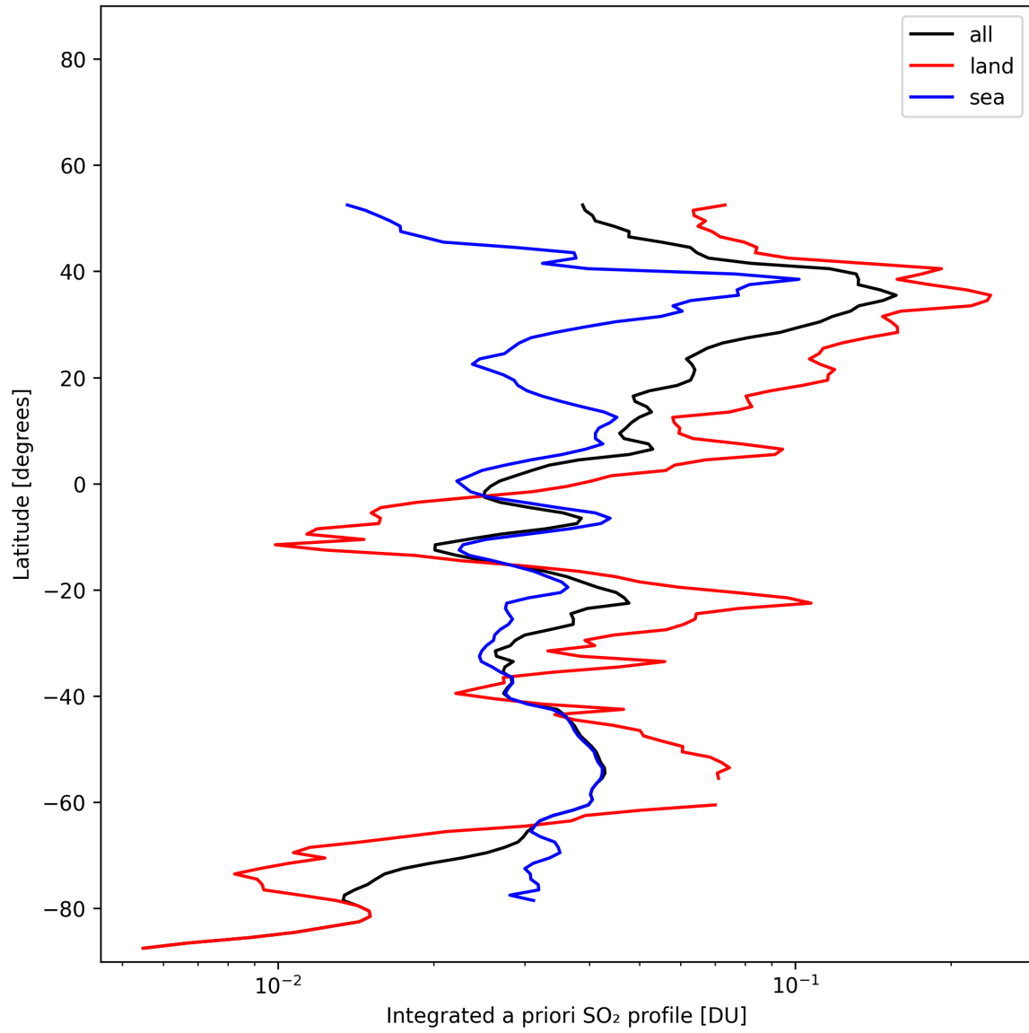
Figure 49: Zonal average of “Integrated a priori SO 2 profile” for 2025-01-31 to 2025-01-31.
