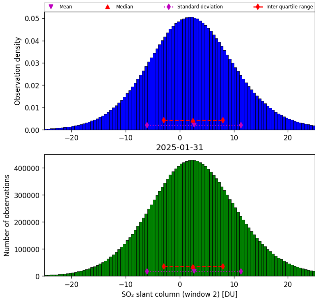
Figure 67: Histogram of “SO 2 slant column (window 2)” for 2025-01-31 to 2025-01-31
