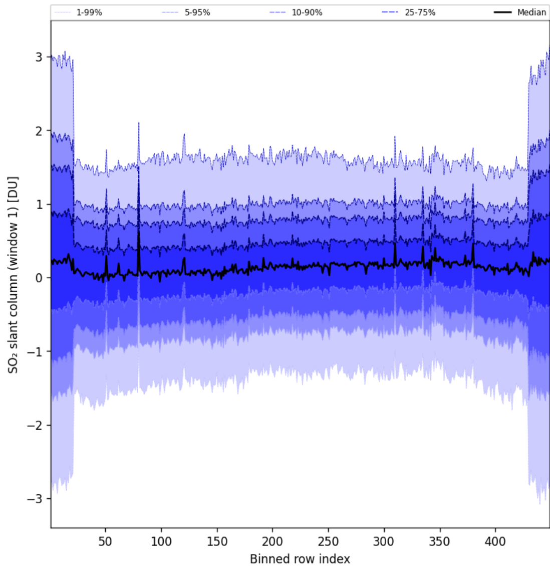
Figure 90: Along track statistics of “SO 2 slant column (window 1)” for 2025-01-31 to 2025-01-31
