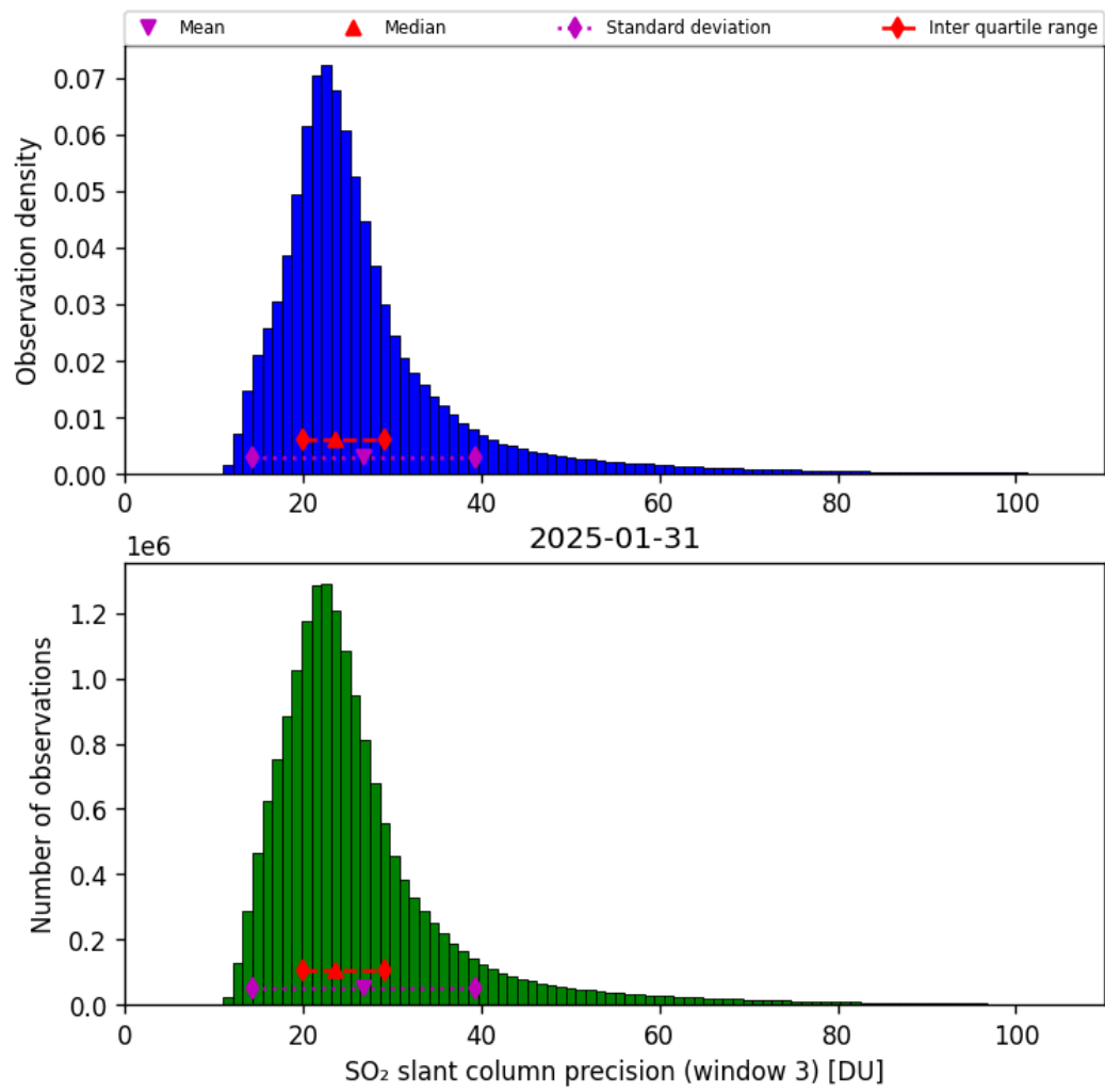
Figure 72: Histogram of “SO 2 slant column precision (window 3)” for 2025-01-31 to 2025-01-31
