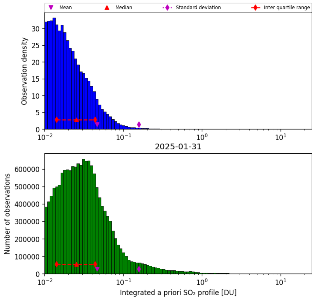
Figure 76: Histogram of “Integrated a priori SO 2 profile” for 2025-01-31 to 2025-01-31
