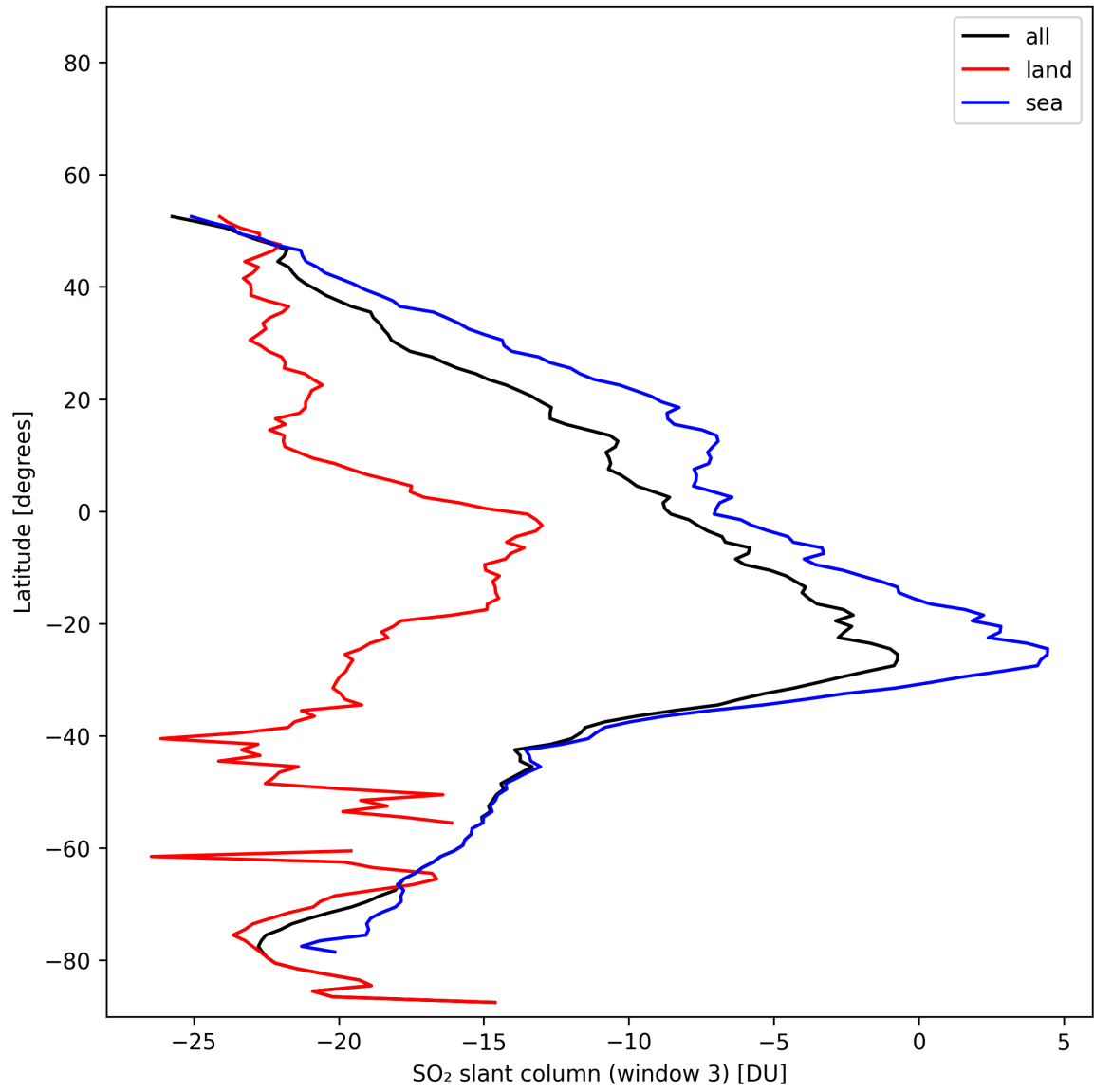
Figure 44: Zonal average of “SO 2 slant column (window 3)” for 2025-01-31 to 2025-01-31.
