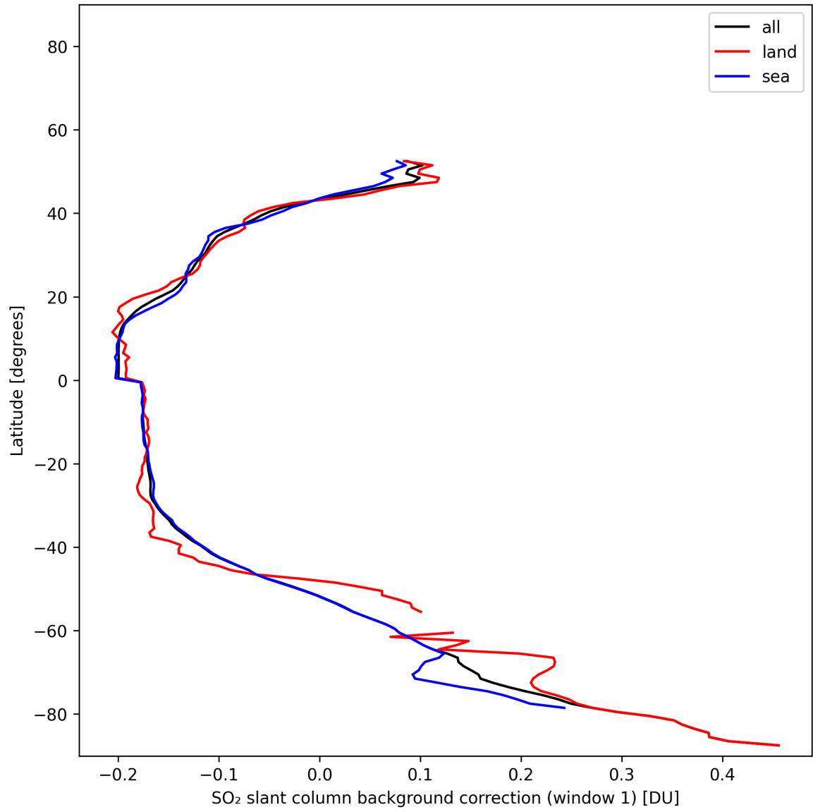
Figure 39: Zonal average of “SO 2 slant column background correction (window 1)” for 2025-01-31 to 2025-01-31.
