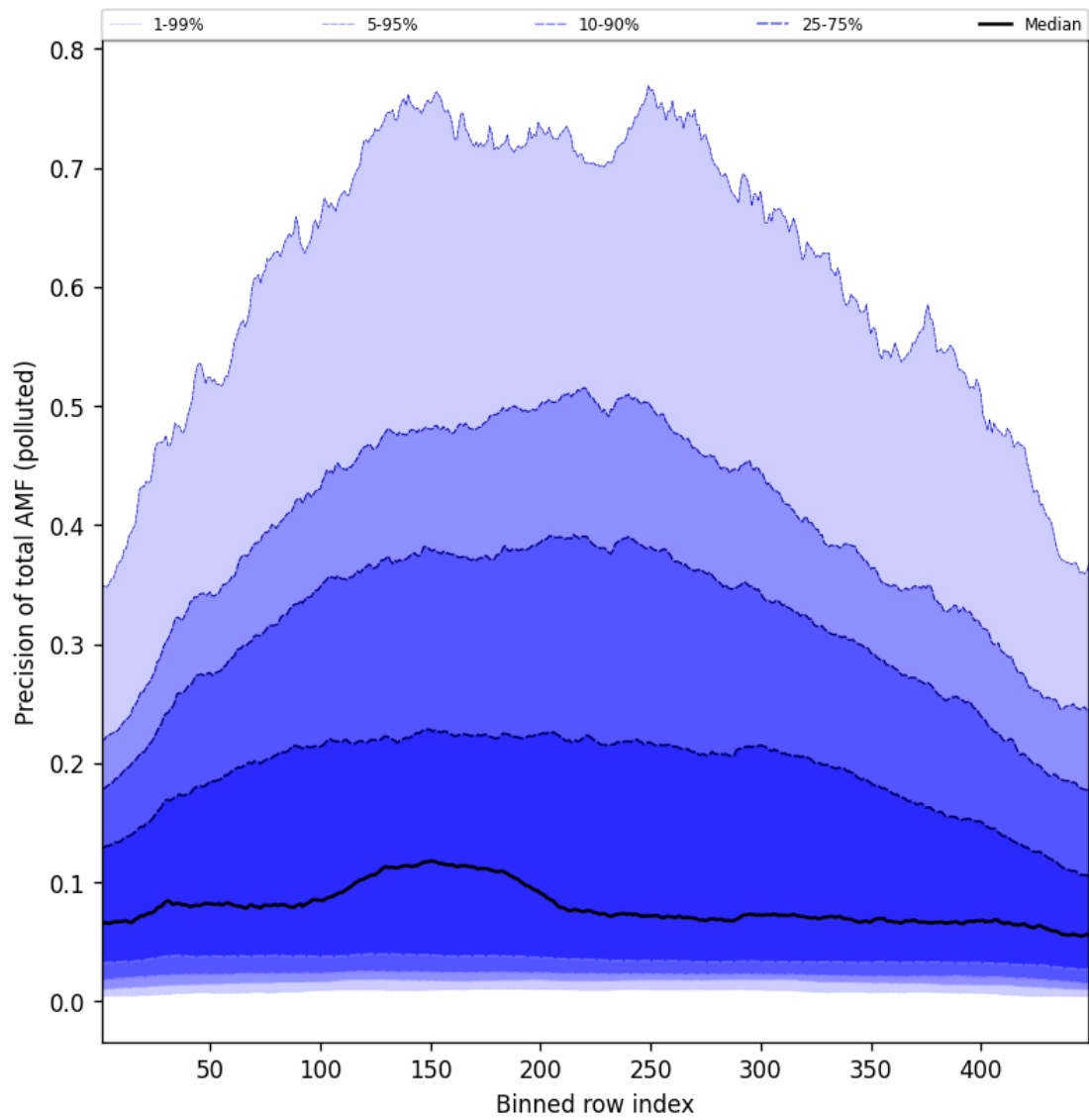
Figure 108: Along track statistics of “Precision of total AMF (polluted)” for 2025-01-31 to 2025-01-31
