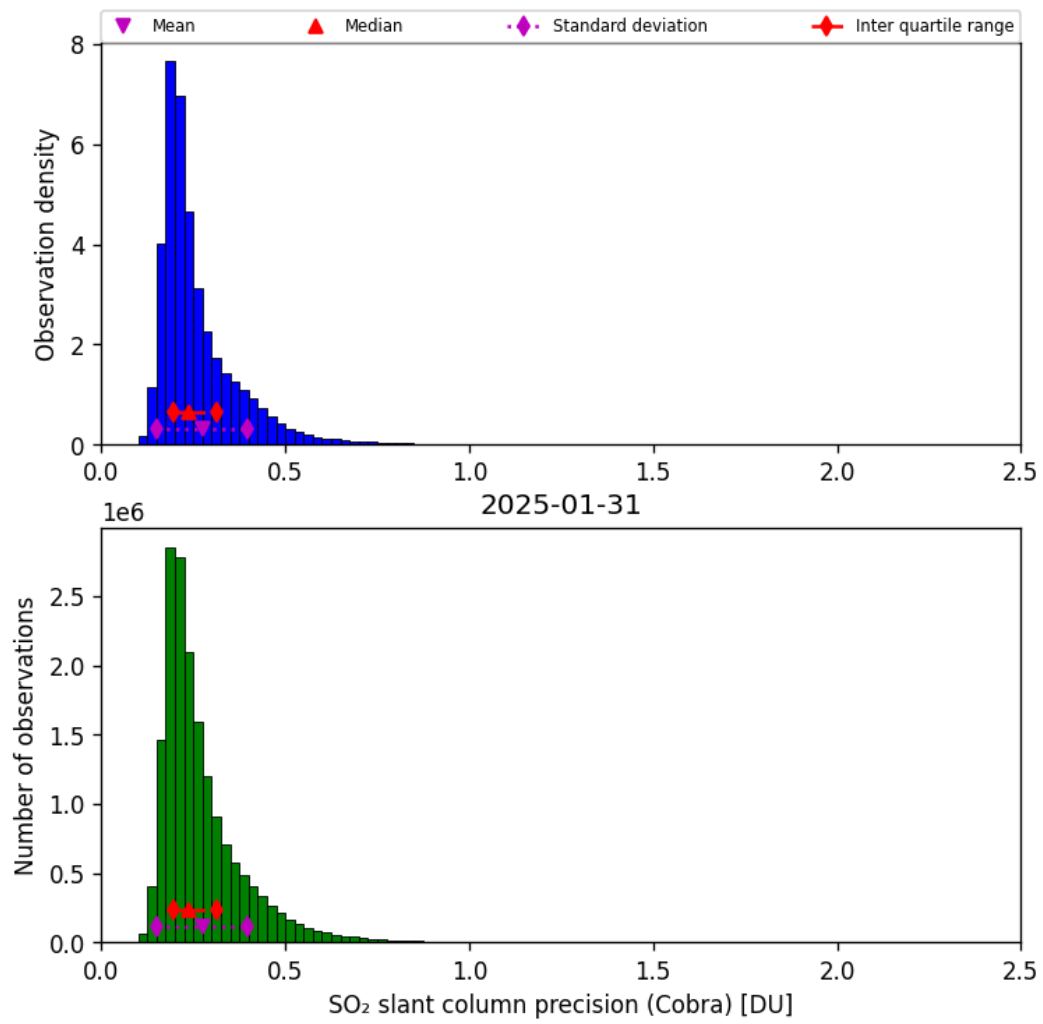
Figure 62: Histogram of “SO 2 slant column precision (Cobra)” for 2025-01-31 to 2025-01-31
