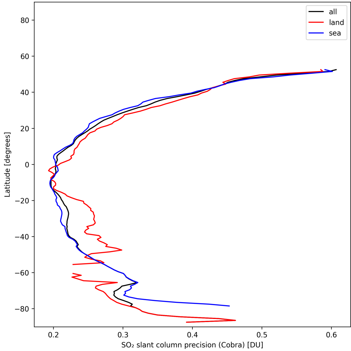
Figure 35: Zonal average of “SO 2 slant column precision (Cobra)” for 2025-01-31 to 2025-01-31.
