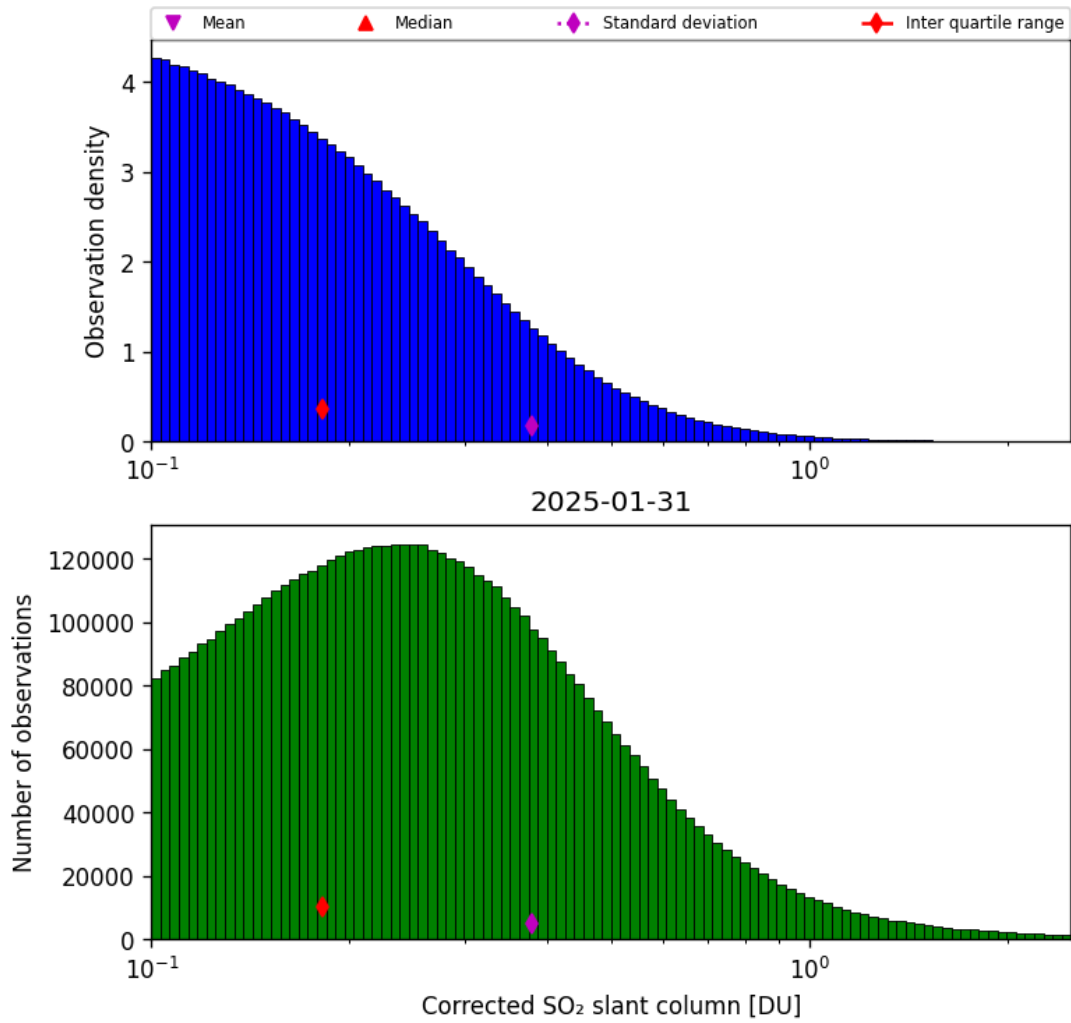
Figure 60: Histogram of "Corrected SO 2 slant column" for 2025-01-31 to 2025-01-31
