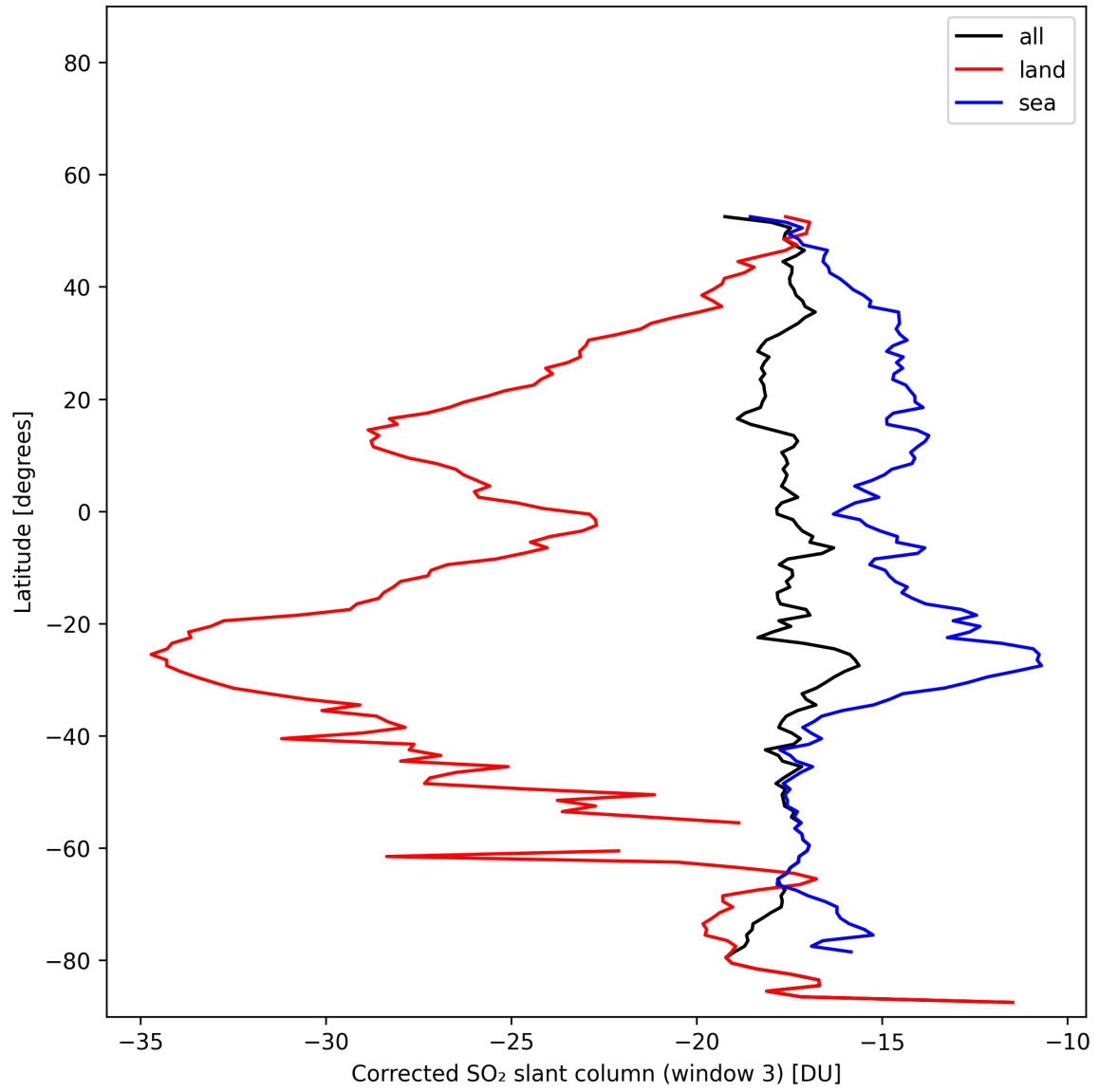
Figure 46: Zonal average of “Corrected SO 2 slant column (window 3)” for 2025-01-31 to 2025-01-31.
