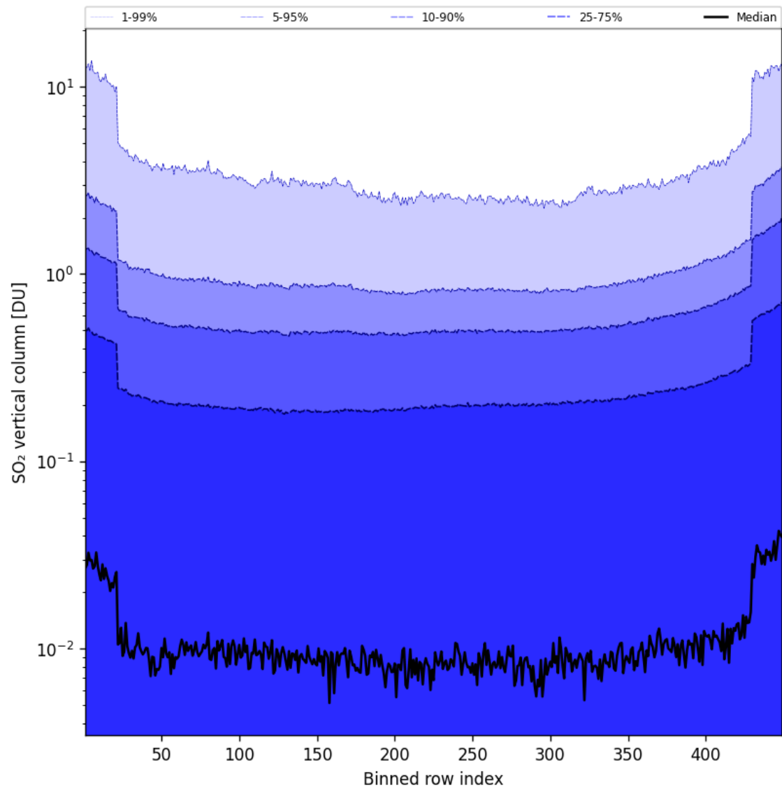
Figure 85: Along track statistics of “SO 2 vertical column” for 2025-01-31 to 2025-01-31
