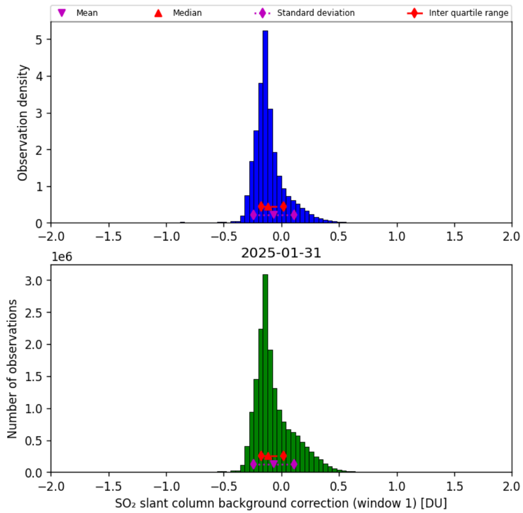
Figure 66: Histogram of “SO 2 slant column background correction (window 1)” for 2025-01-31 to 2025-01-31
