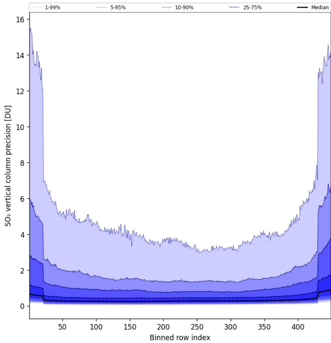
Figure 86: Along track statistics of “SO 2 vertical column precision” for 2025-01-31 to 2025-01-31
