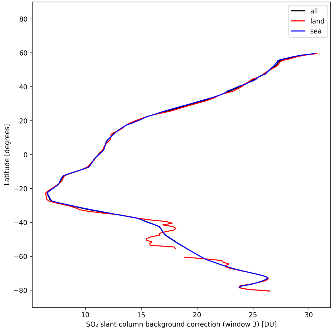
Figure 47: Zonal average of “SO 2 slant column background correction (window 3)” for 2025-02-21 to 2025-02-22.
