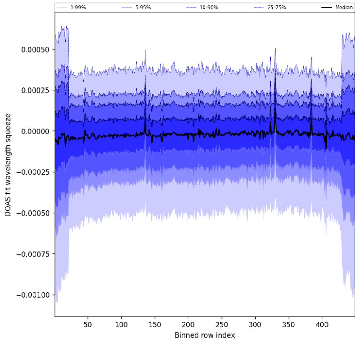
Figure 105: Along track statistics of “DOAS fit wavelength squeeze” for 2025-02-21 to 2025-02-22
