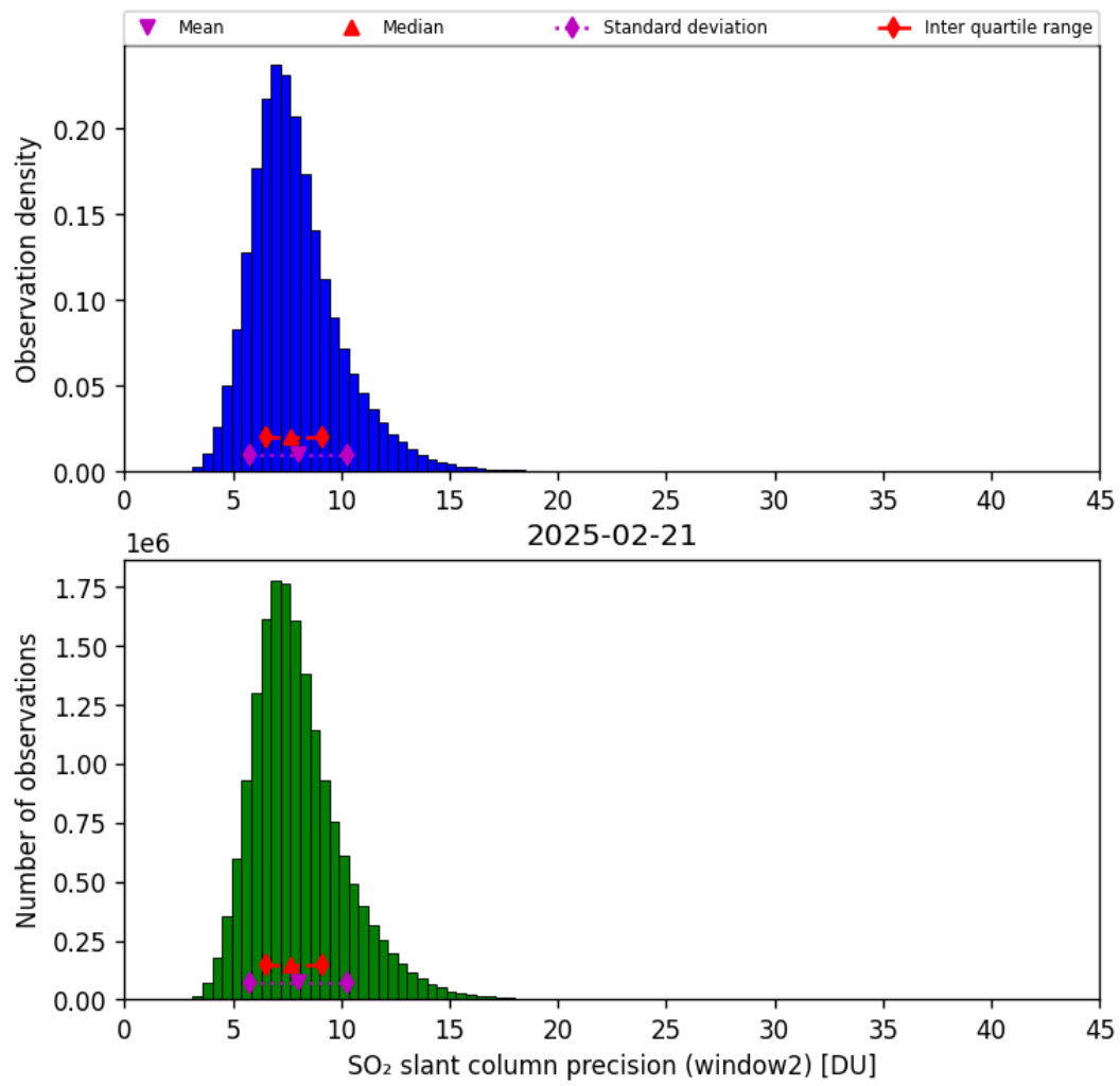
Figure 68: Histogram of “SO 2 slant column precision (window2)” for 2025-02-21 to 2025-02-22
