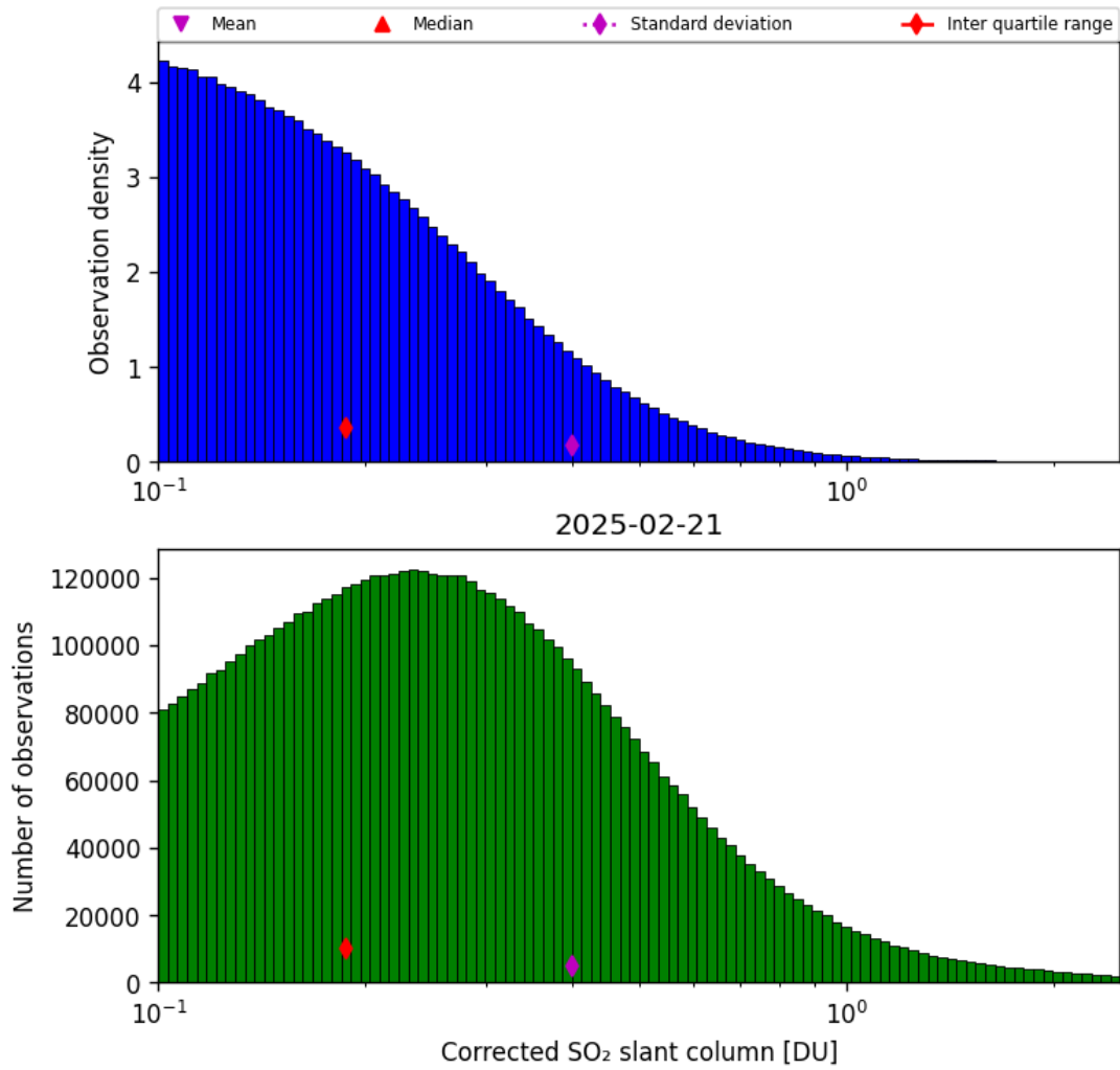
Figure 60: Histogram of “Corrected SO 2 slant column” for 2025-02-21 to 2025-02-22
