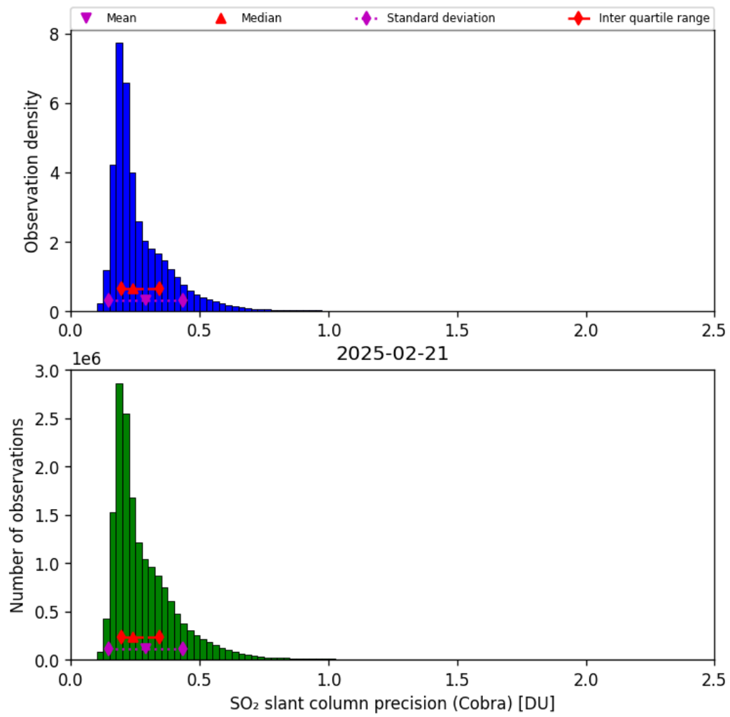
Figure 62: Histogram of “SO 2 slant column precision (Cobra)” for 2025-02-21 to 2025-02-22
