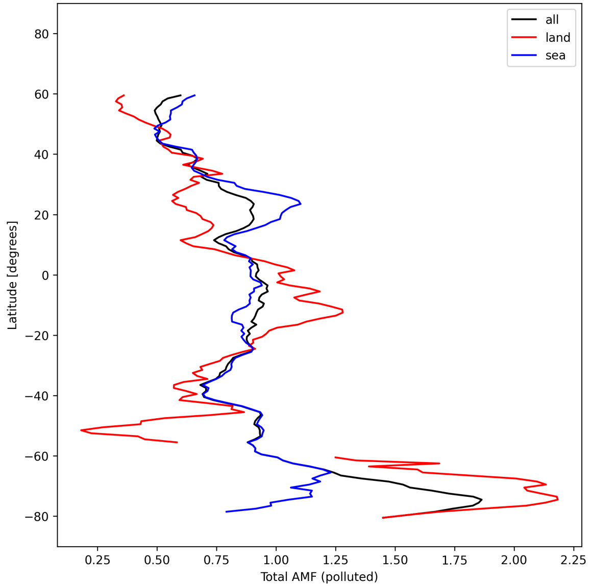
Figure 53: Zonal average of “Total AMF (polluted)” for 2025-02-21 to 2025-02-22.
