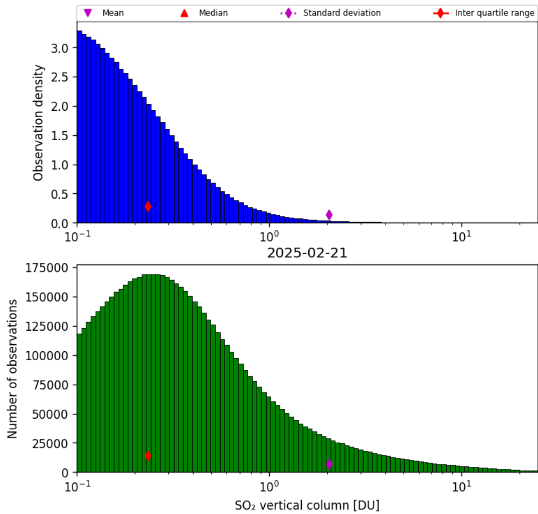
Figure 58: Histogram of “SO 2 vertical column” for 2025-02-21 to 2025-02-22
