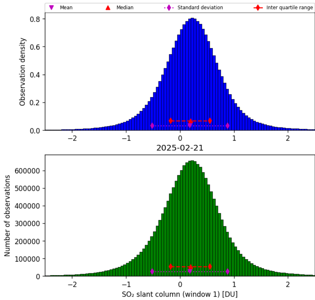
Figure 63: Histogram of “SO 2 slant column (window 1)” for 2025-02-21 to 2025-02-22
