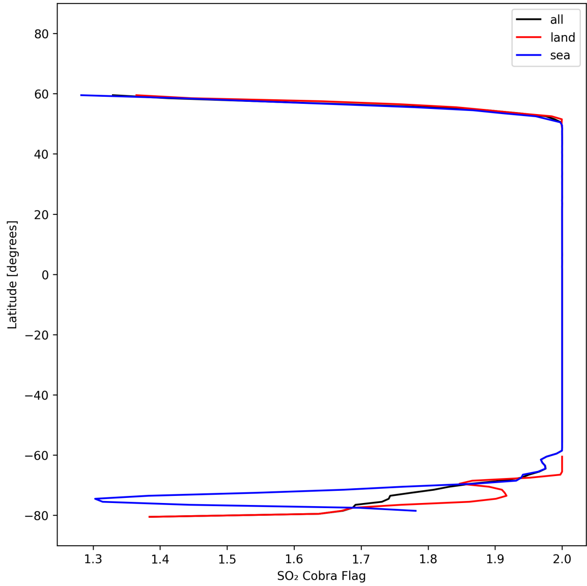
Figure 48: Zonal average of "SO 2 Cobra Flag" for 2025-02-21 to 2025-02-22.
