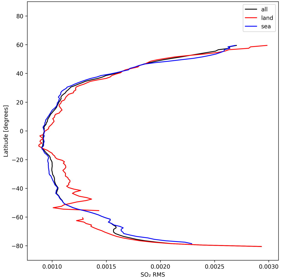
Figure 52: Zonal average of “SO 2 RMS” for 2025-02-21 to 2025-02-22.
