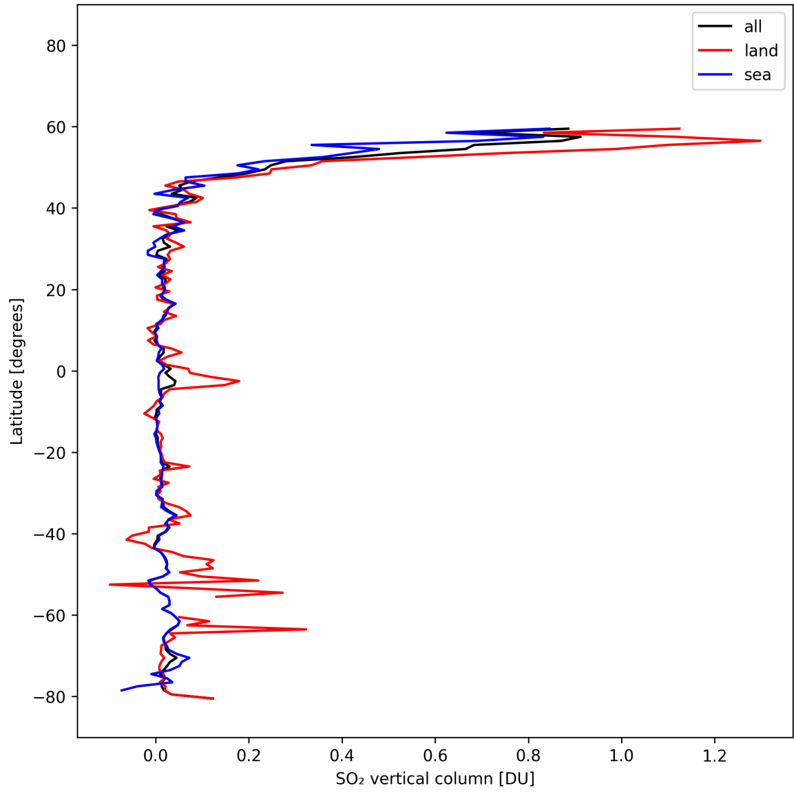
Figure 31: Zonal average of “SO 2 vertical column” for 2025-02-21 to 2025-02-22.
