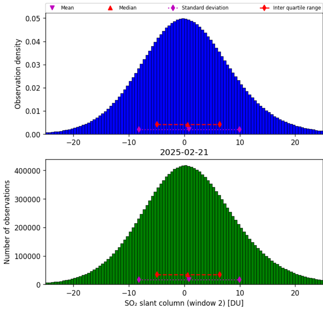
Figure 67: Histogram of “SO 2 slant column (window 2)” for 2025-02-21 to 2025-02-22
