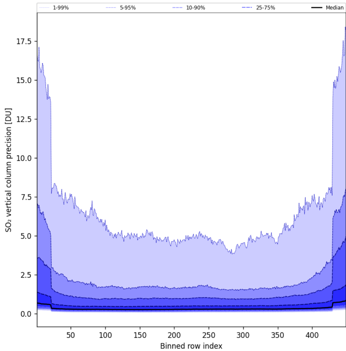
Figure 86: Along track statistics of “SO 2 vertical column precision” for 2025-02-21 to 2025-02-22
