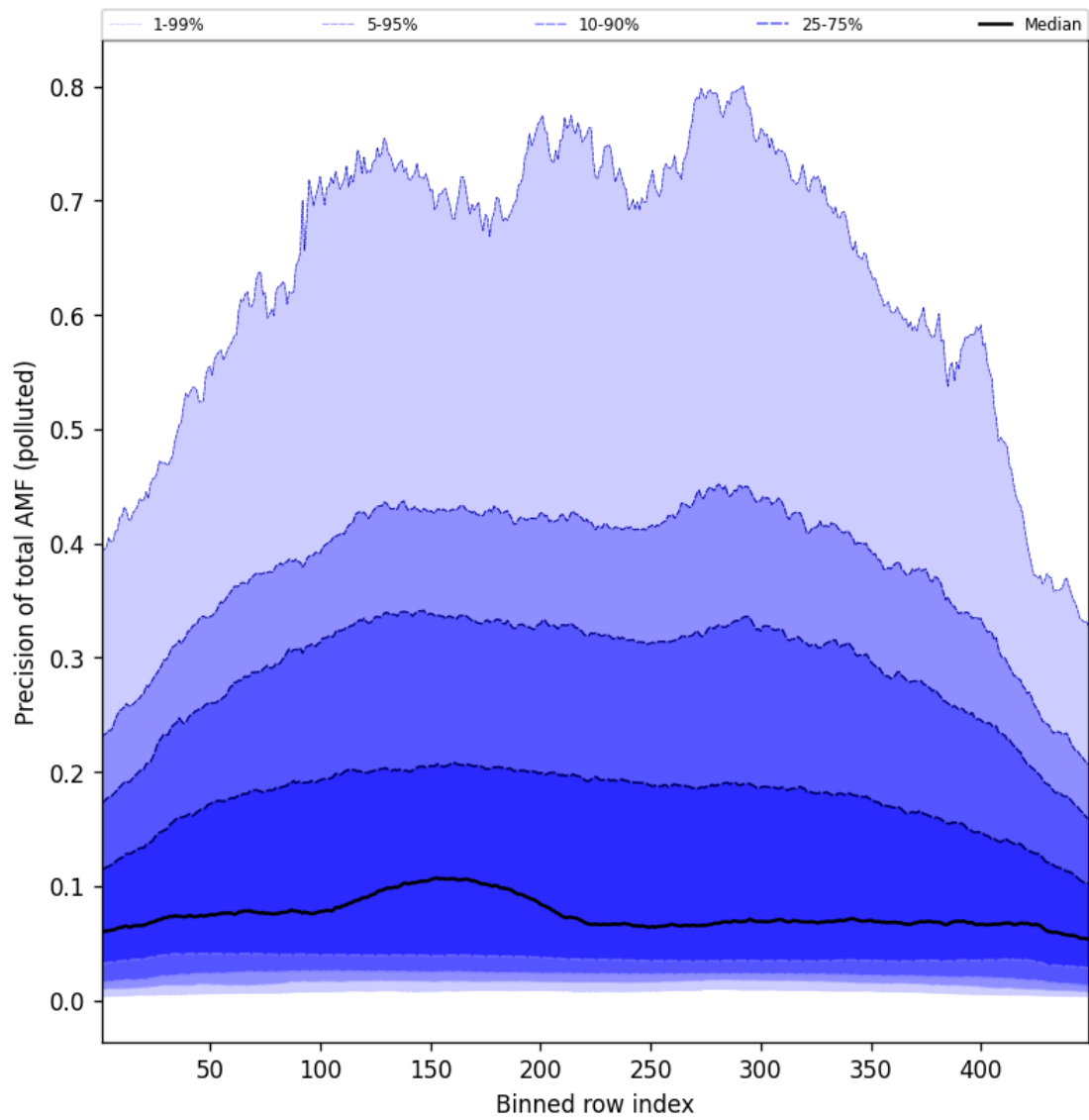
Figure 108: Along track statistics of “Precision of total AMF (polluted)” for 2025-02-21 to 2025-02-22
