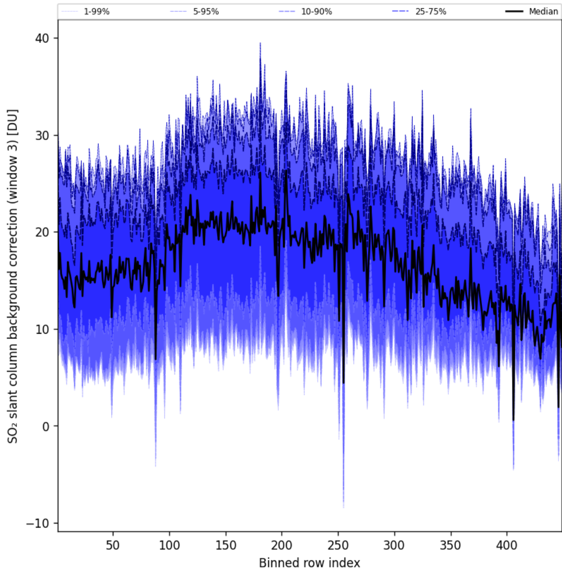
Figure 101: Along track statistics of “SO 2 slant column background correction (window 3)” for 2025-02-21 to 2025-02-22
