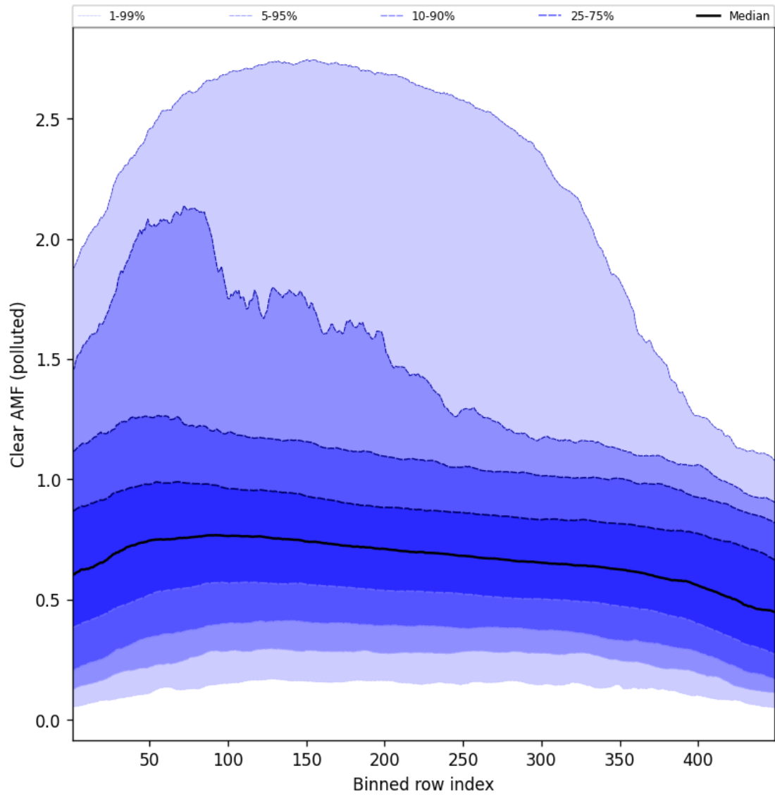
Figure 109: Along track statistics of “Clear AMF (polluted)” for 2025-02-21 to 2025-02-22
