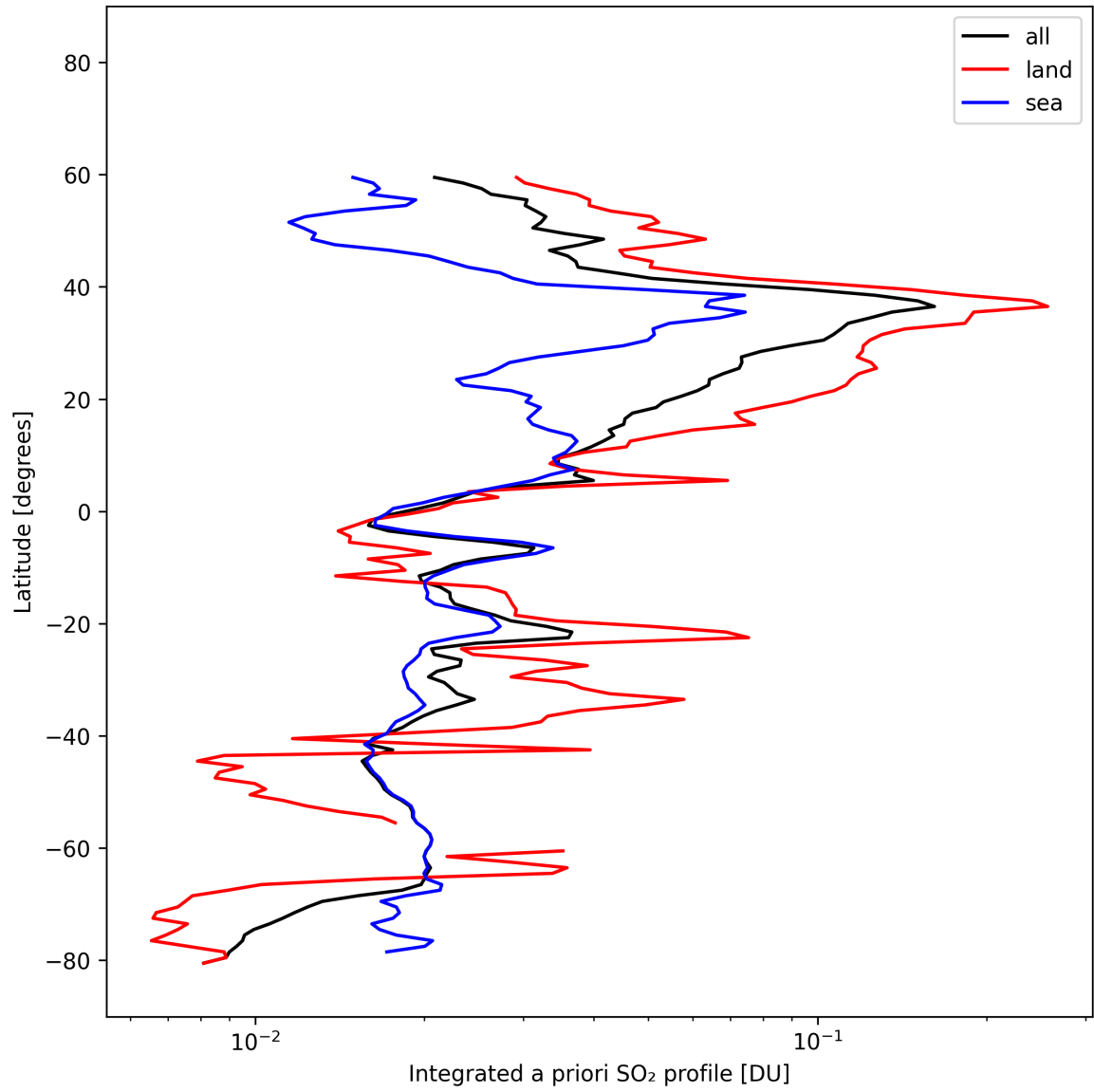
Figure 49: Zonal average of “Integrated a priori SO 2 profile” for 2025-02-21 to 2025-02-22.
