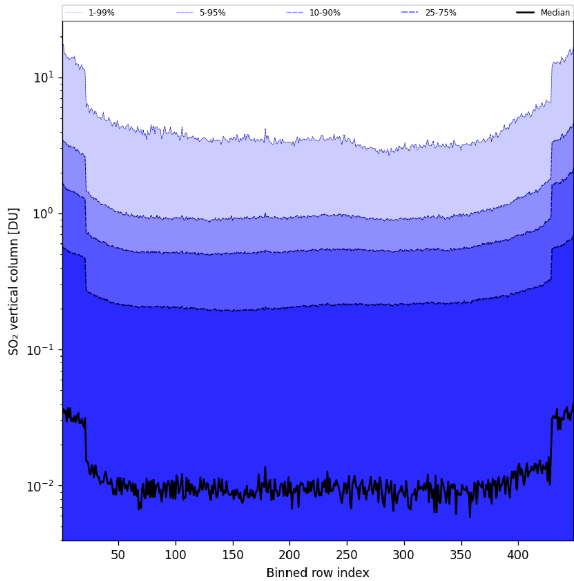
Figure 85: Along track statistics of “SO 2 vertical column” for 2025-02-21 to 2025-02-22
