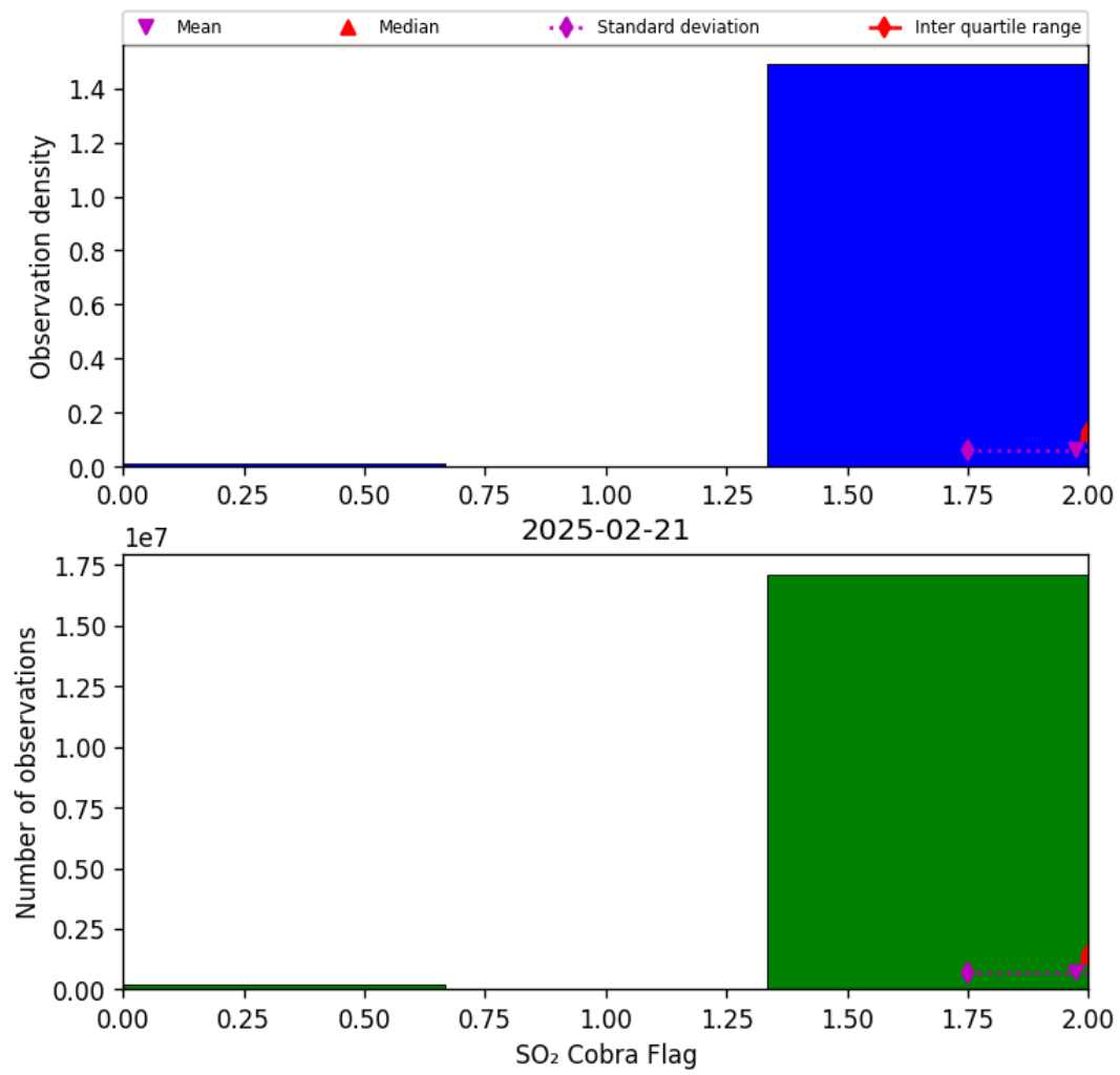
Figure 75: Histogram of “SO 2 Cobra Flag” for 2025-02-21 to 2025-02-22
