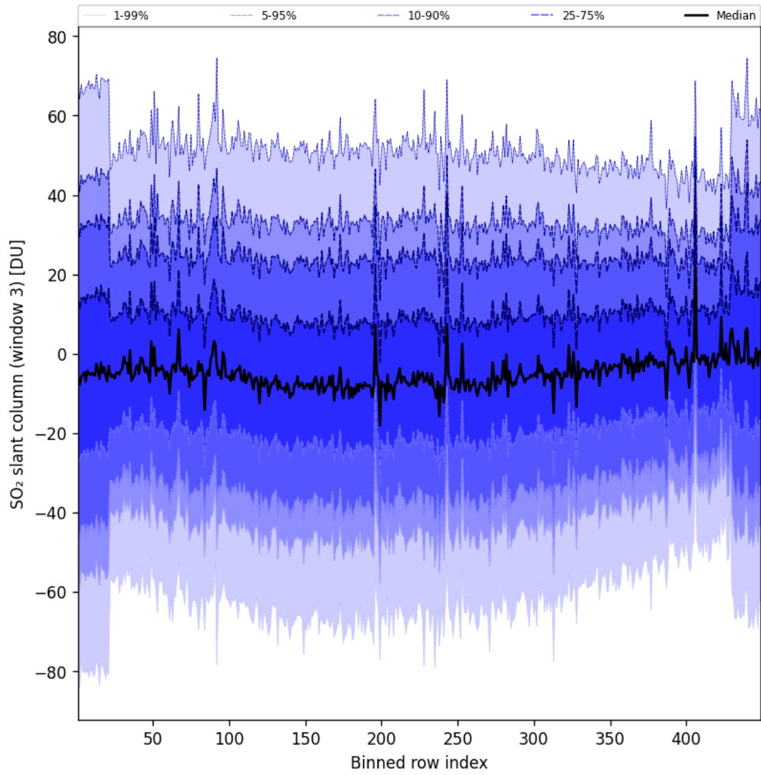
Figure 98: Along track statistics of “SO 2 slant column (window 3)” for 2025-02-21 to 2025-02-22
