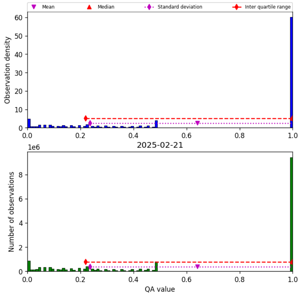
Figure 57: Histogram of “QA value” for 2025-02-21 to 2025-02-22
