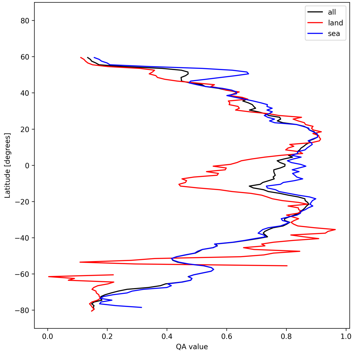
Figure 30: Zonal average of “QA value” for 2025-02-21 to 2025-02-22.
