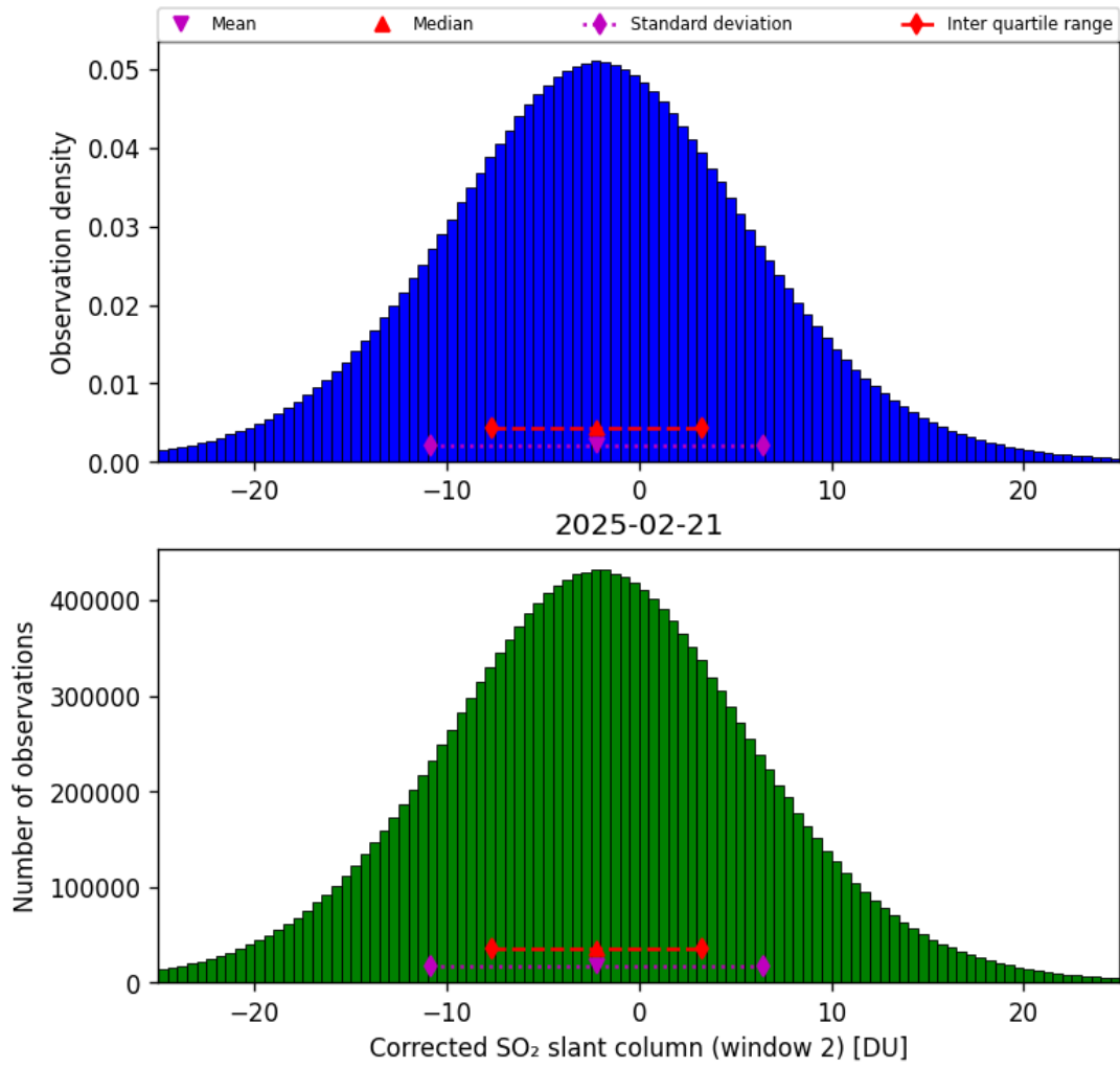
Figure 69: Histogram of “Corrected SO 2 slant column (window 2)” for 2025-02-21 to 2025-02-22
