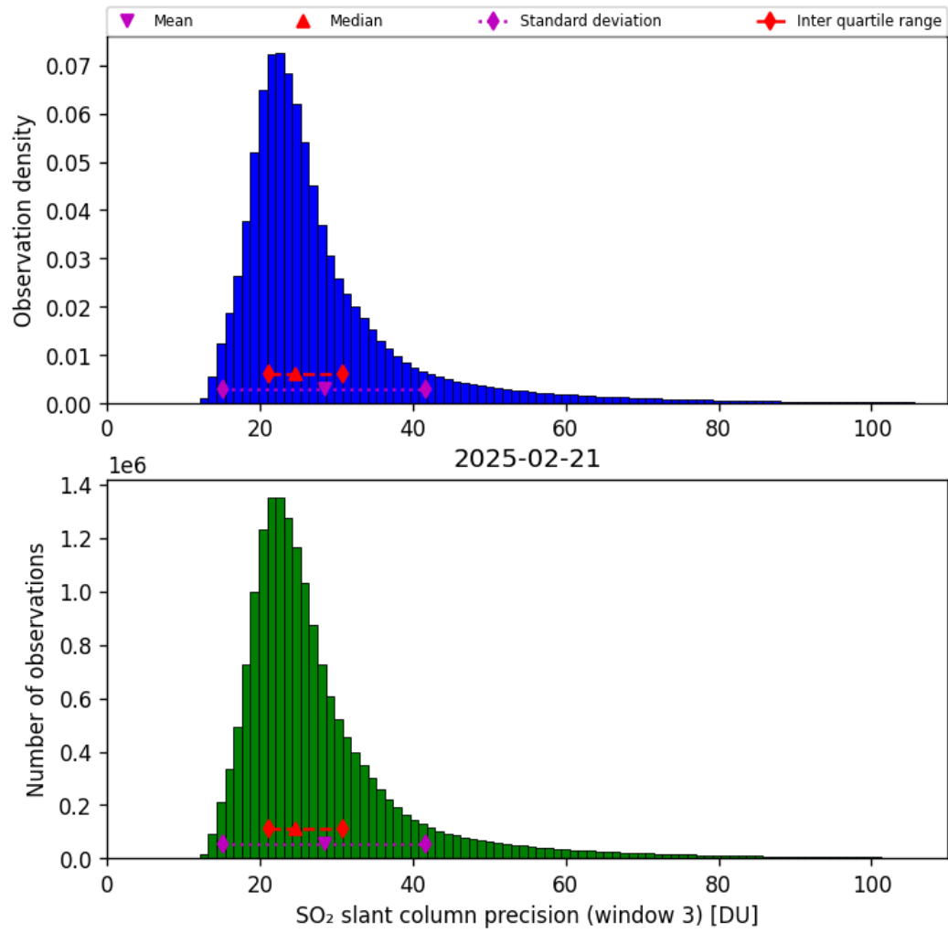
Figure 72: Histogram of “SO 2 slant column precision (window 3)” for 2025-02-21 to 2025-02-22
