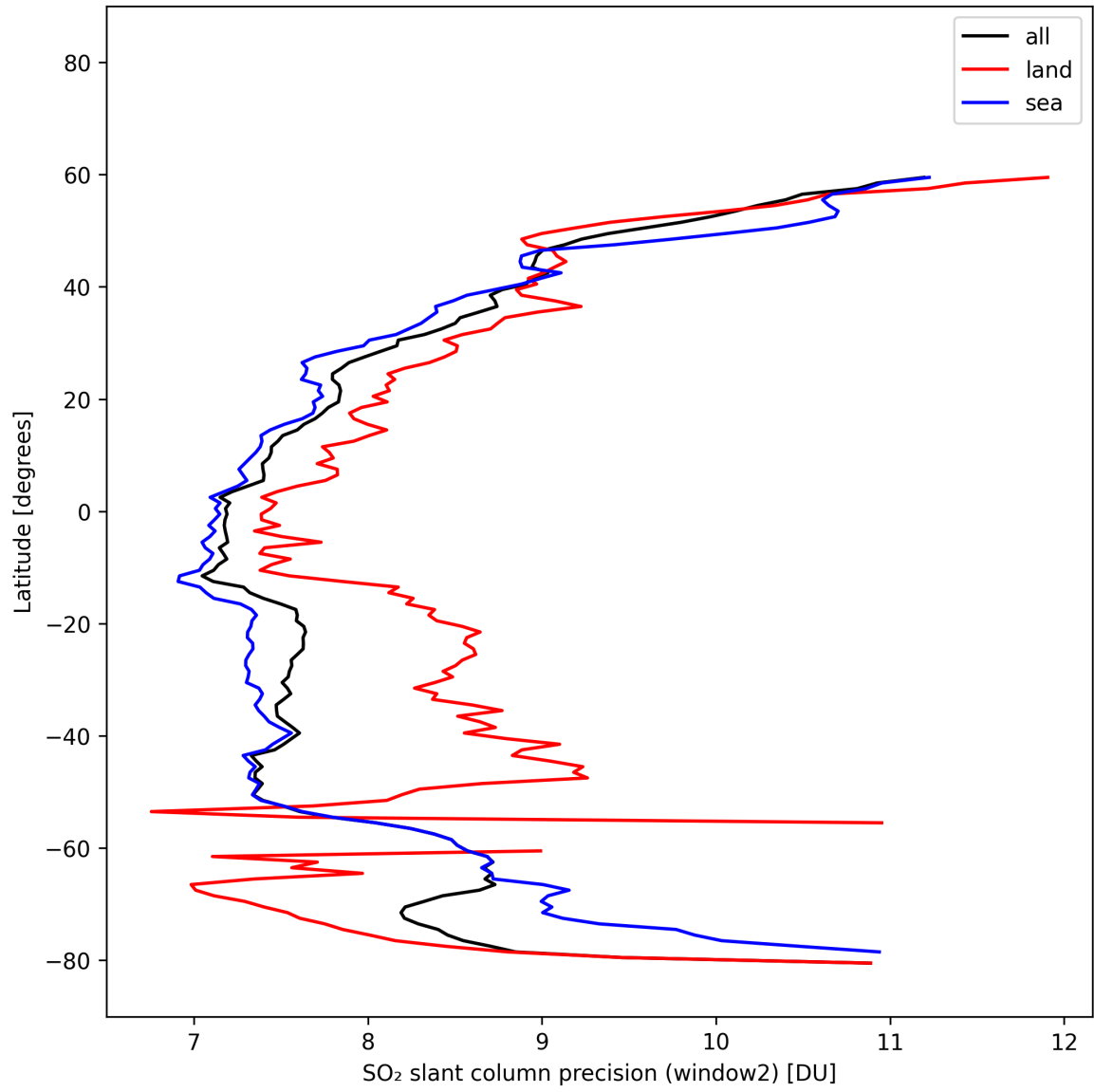
Figure 41: Zonal average of “SO 2 slant column precision (window2)” for 2025-02-21 to 2025-02-22.
