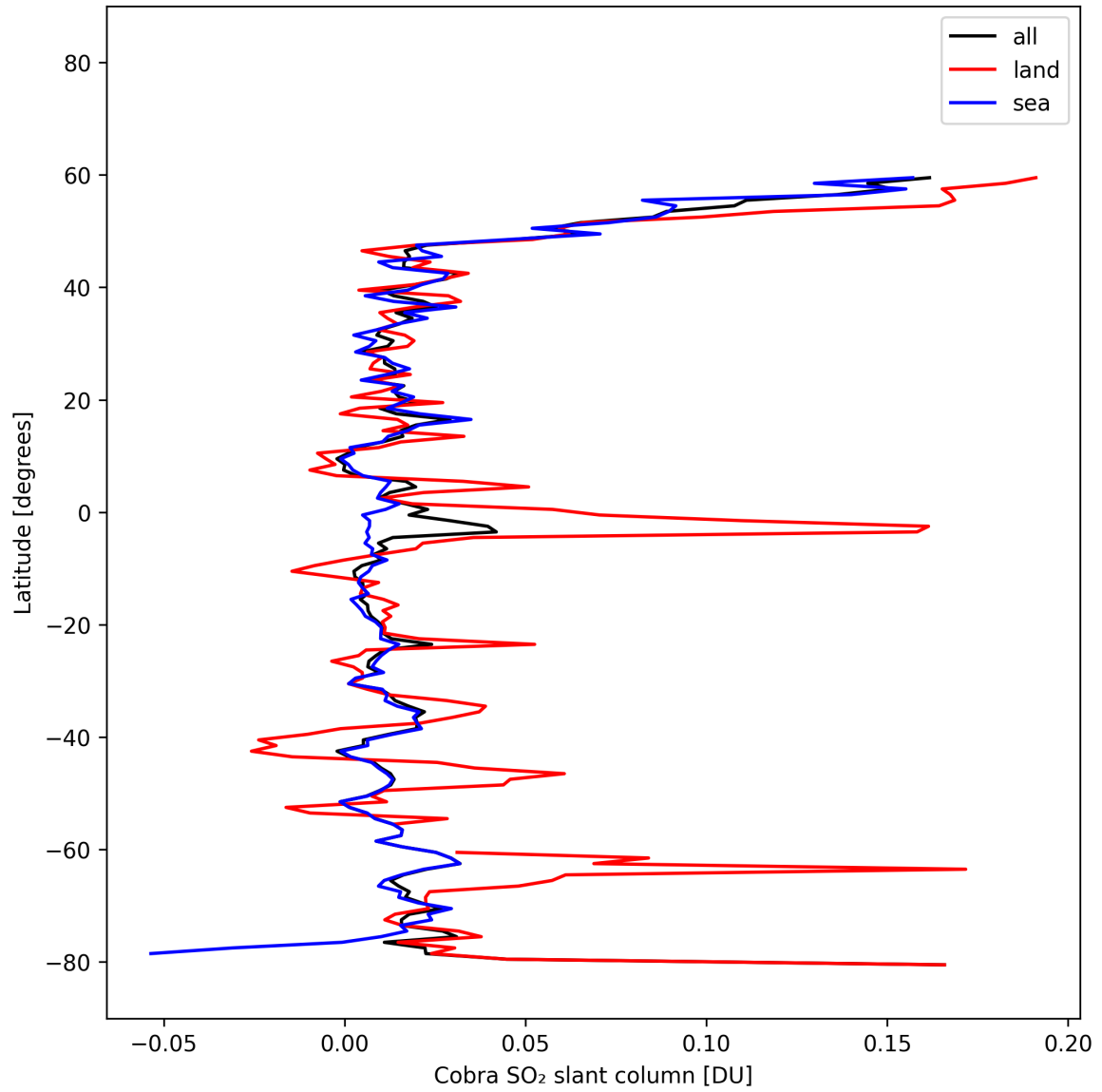
Figure 34: Zonal average of “Cobra SO 2 slant column” for 2025-02-21 to 2025-02-22.
