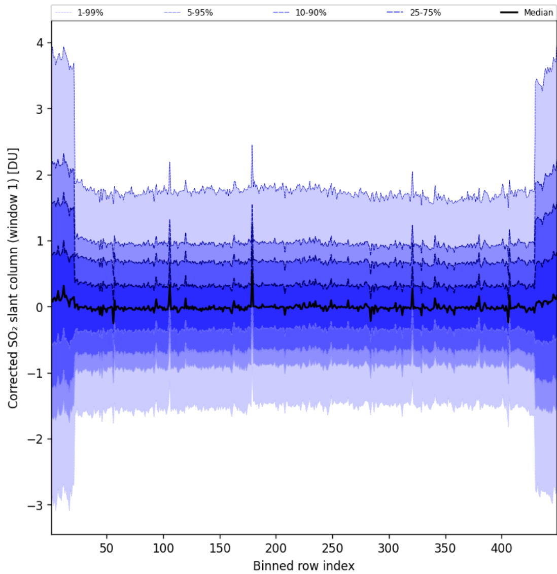
Figure 92: Along track statistics of “Corrected SO 2 slant column (window 1)” for 2025-02-21 to 2025-02-22
