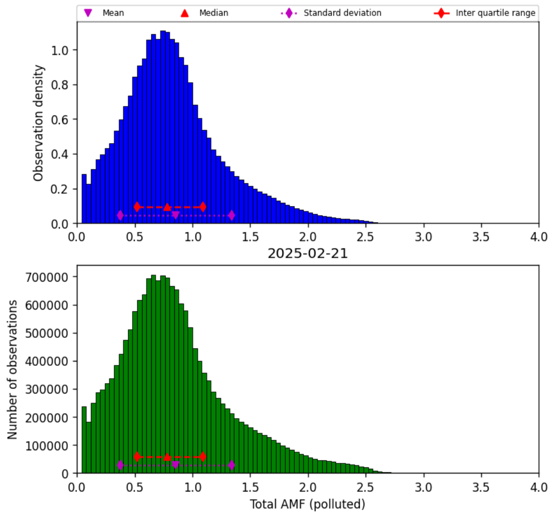
Figure 80: Histogram of “Total AMF (polluted)” for 2025-02-21 to 2025-02-22
