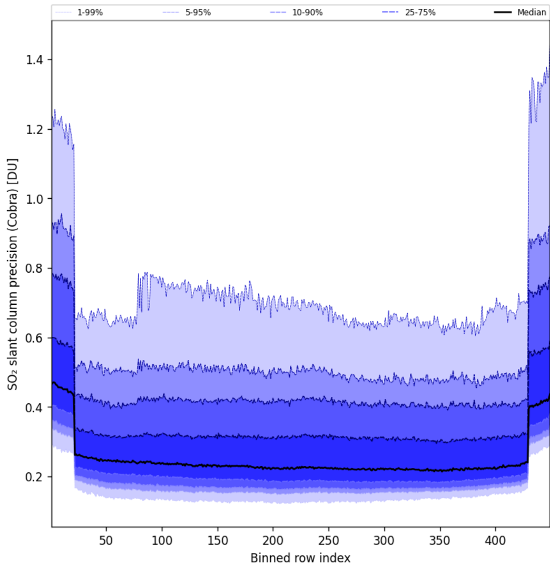
Figure 89: Along track statistics of “SO 2 slant column precision (Cobra)” for 2025-02-21 to 2025-02-22
