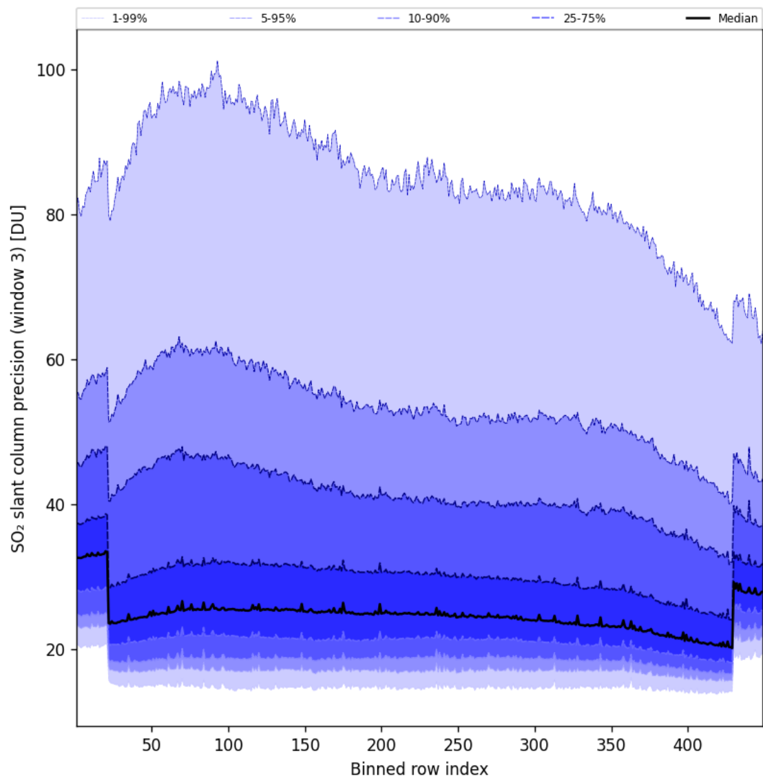
Figure 99: Along track statistics of “SO 2 slant column precision (window 3)” for 2025-02-21 to 2025-02-22
