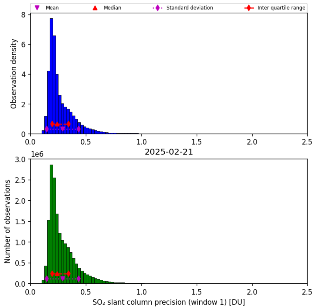
Figure 64: Histogram of “SO 2 slant column precision (window 1)” for 2025-02-21 to 2025-02-22
