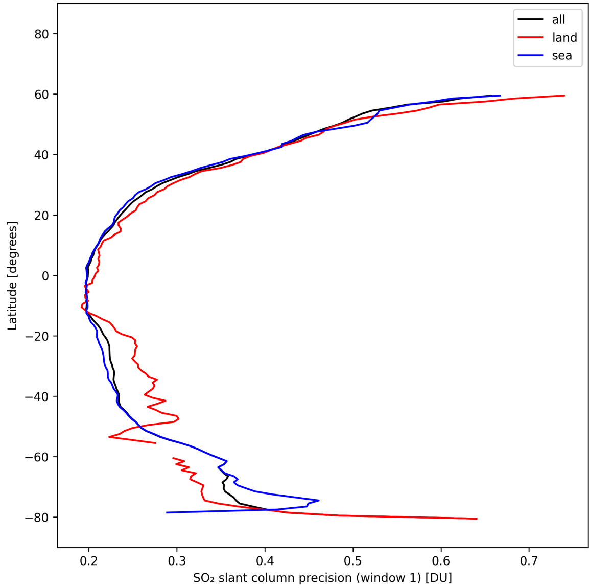
Figure 37: Zonal average of “SO 2 slant column precision (window 1)” for 2025-02-21 to 2025-02-22.
