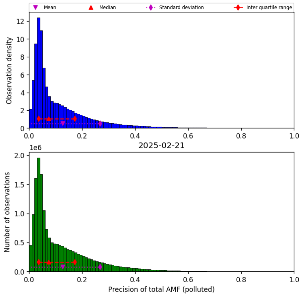
Figure 81: Histogram of “Precision of total AMF (polluted)” for 2025-02-21 to 2025-02-22
