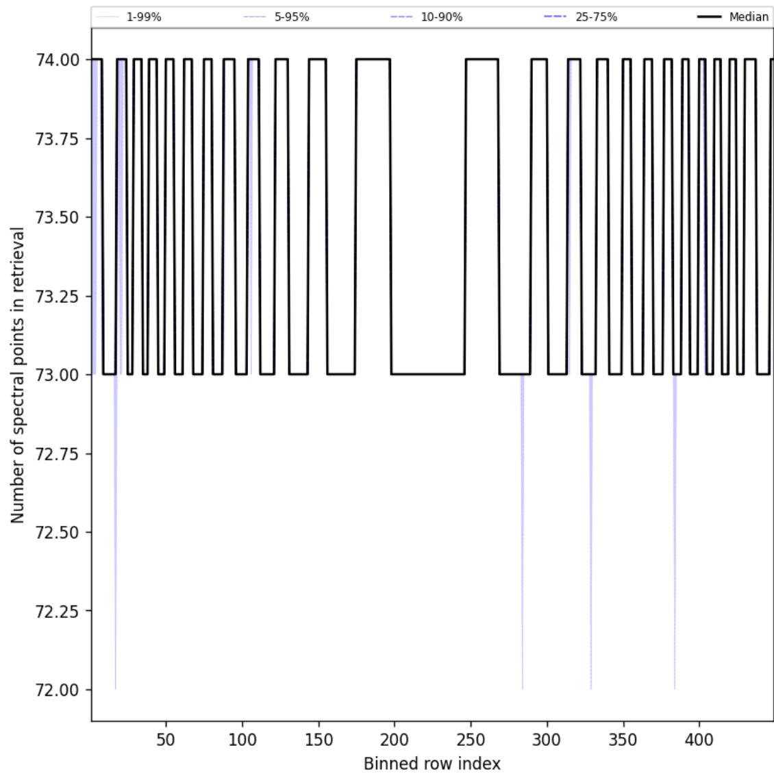
Figure 110: Along track statistics of “Number of spectral points in retrieval” for 2025-02-21 to 2025-02-22
