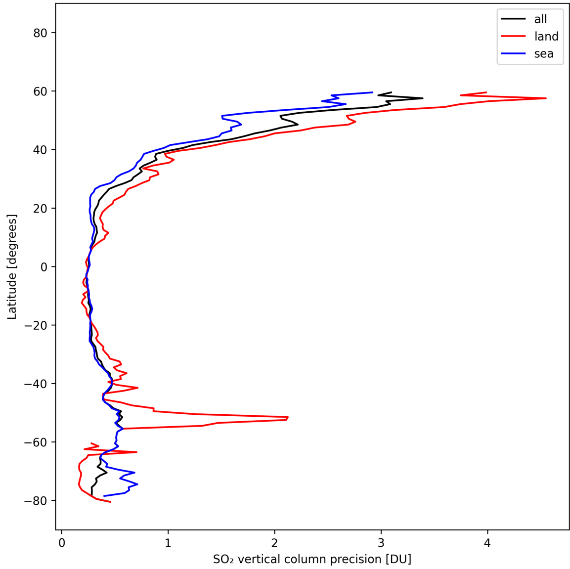
Figure 32: Zonal average of “SO 2 vertical column precision” for 2025-02-21 to 2025-02-22.
