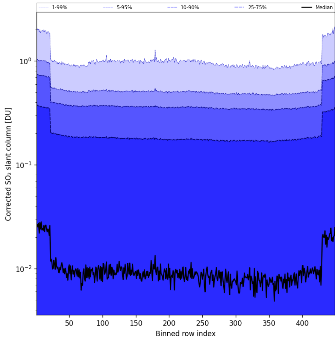
Figure 87: Along track statistics of “Corrected SO 2 slant column” for 2025-02-21 to 2025-02-22
