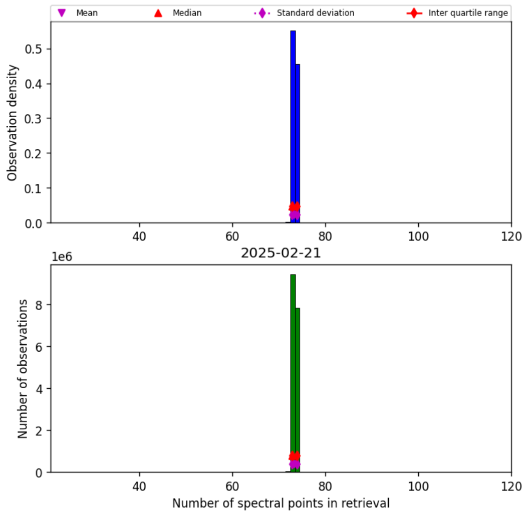
Figure 83: Histogram of “Number of spectral points in retrieval” for 2025-02-21 to 2025-02-22
