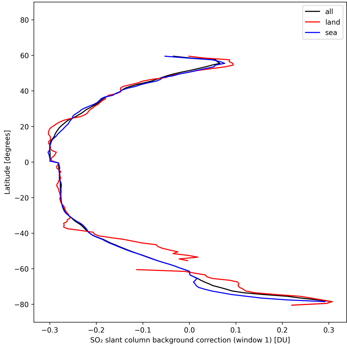
Figure 39: Zonal average of “SO 2 slant column background correction (window 1)” for 2025-02-21 to 2025-02-22.
