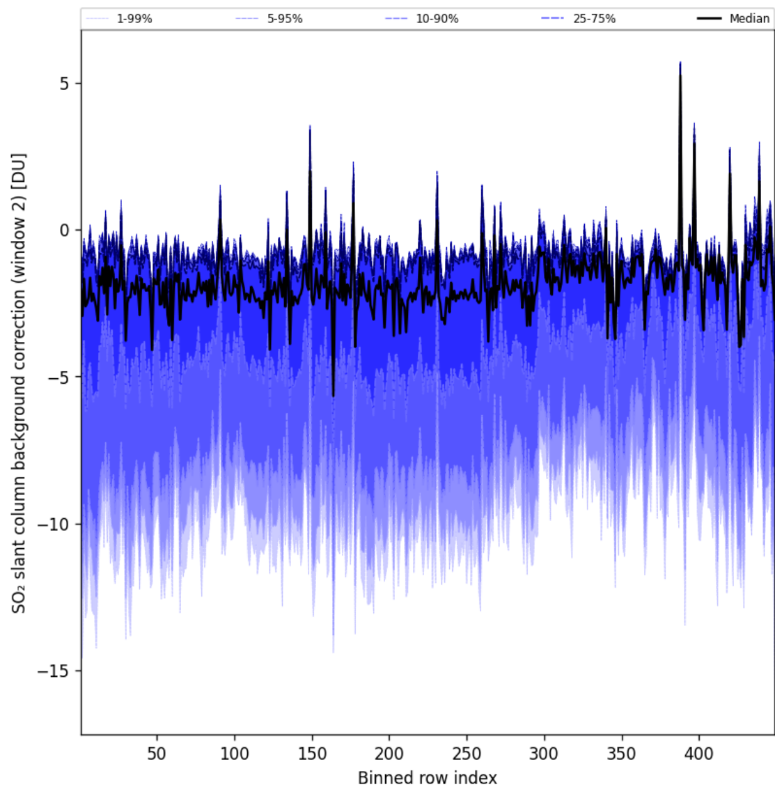
Figure 97: Along track statistics of “SO 2 slant column background correction (window 2)” for 2025-02-21 to 2025-02-22
