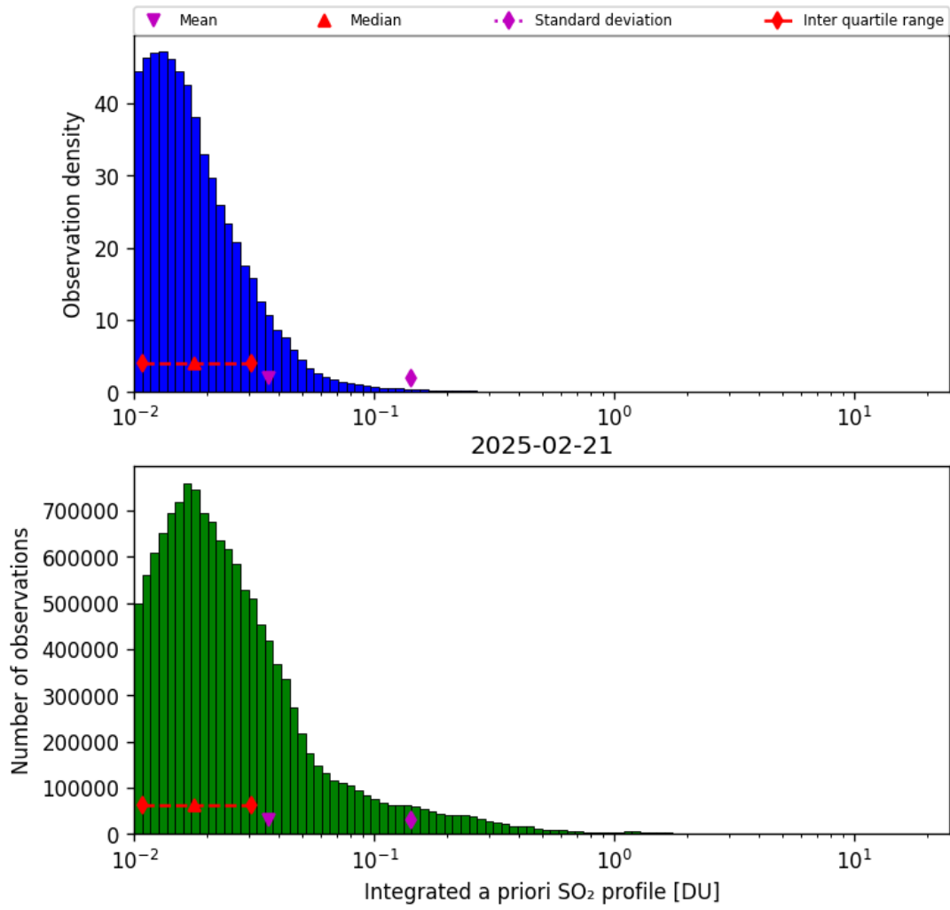
Figure 76: Histogram of “Integrated a priori SO 2 profile” for 2025-02-21 to 2025-02-22
