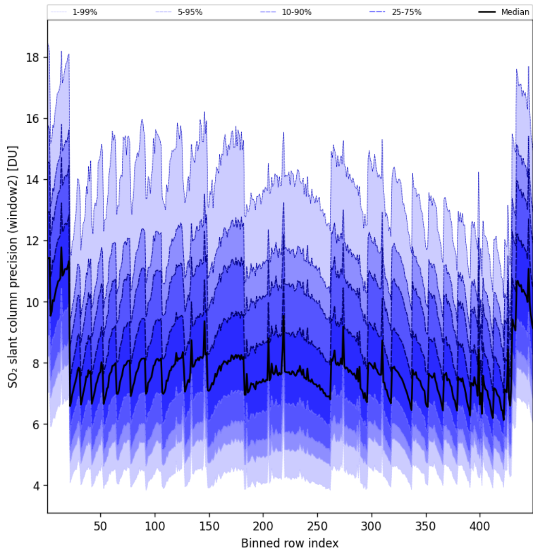
Figure 95: Along track statistics of “SO 2 slant column precision (window2)” for 2025-02-21 to 2025-02-22
