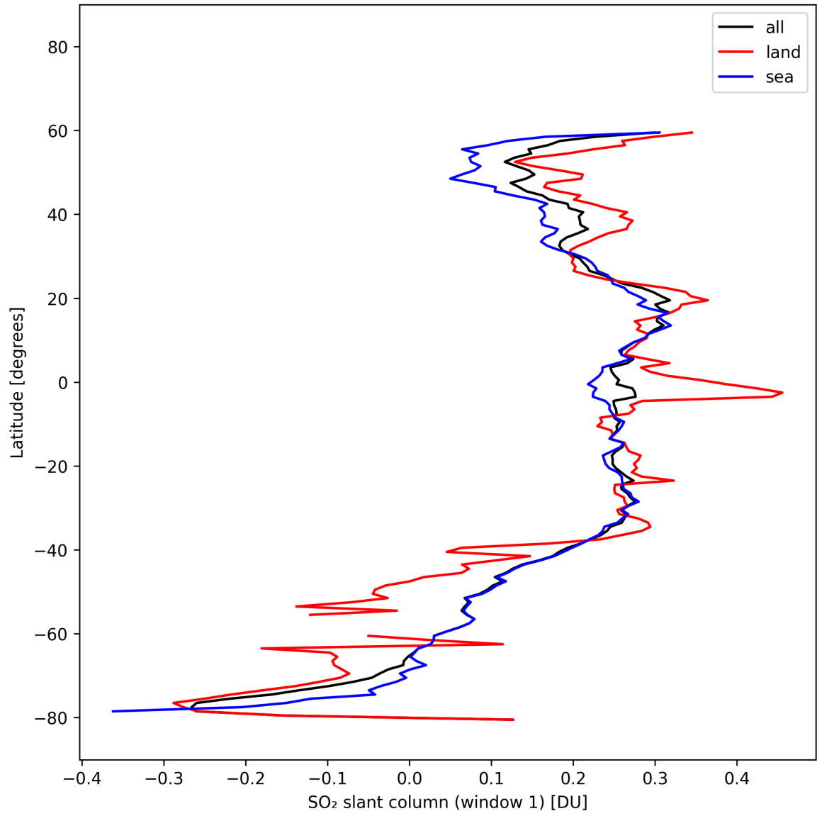
Figure 36: Zonal average of “SO 2 slant column (window 1)” for 2025-02-21 to 2025-02-22.
