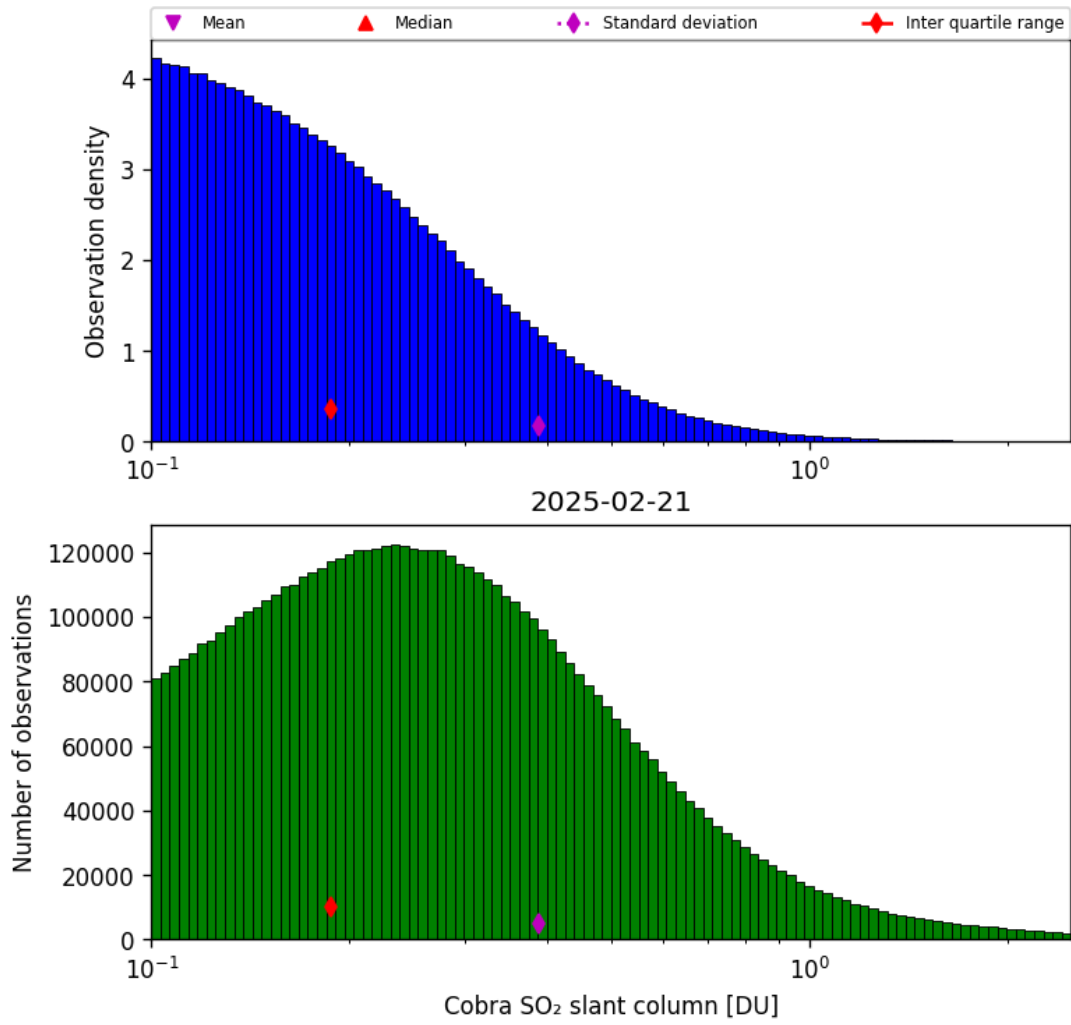
Figure 61: Histogram of “Cobra SO 2 slant column” for 2025-02-21 to 2025-02-22
