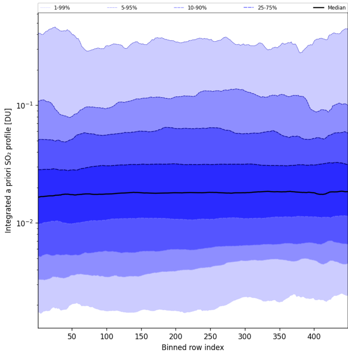
Figure 103: Along track statistics of “Integrated a priori SO 2 profile” for 2025-02-21 to 2025-02-22
