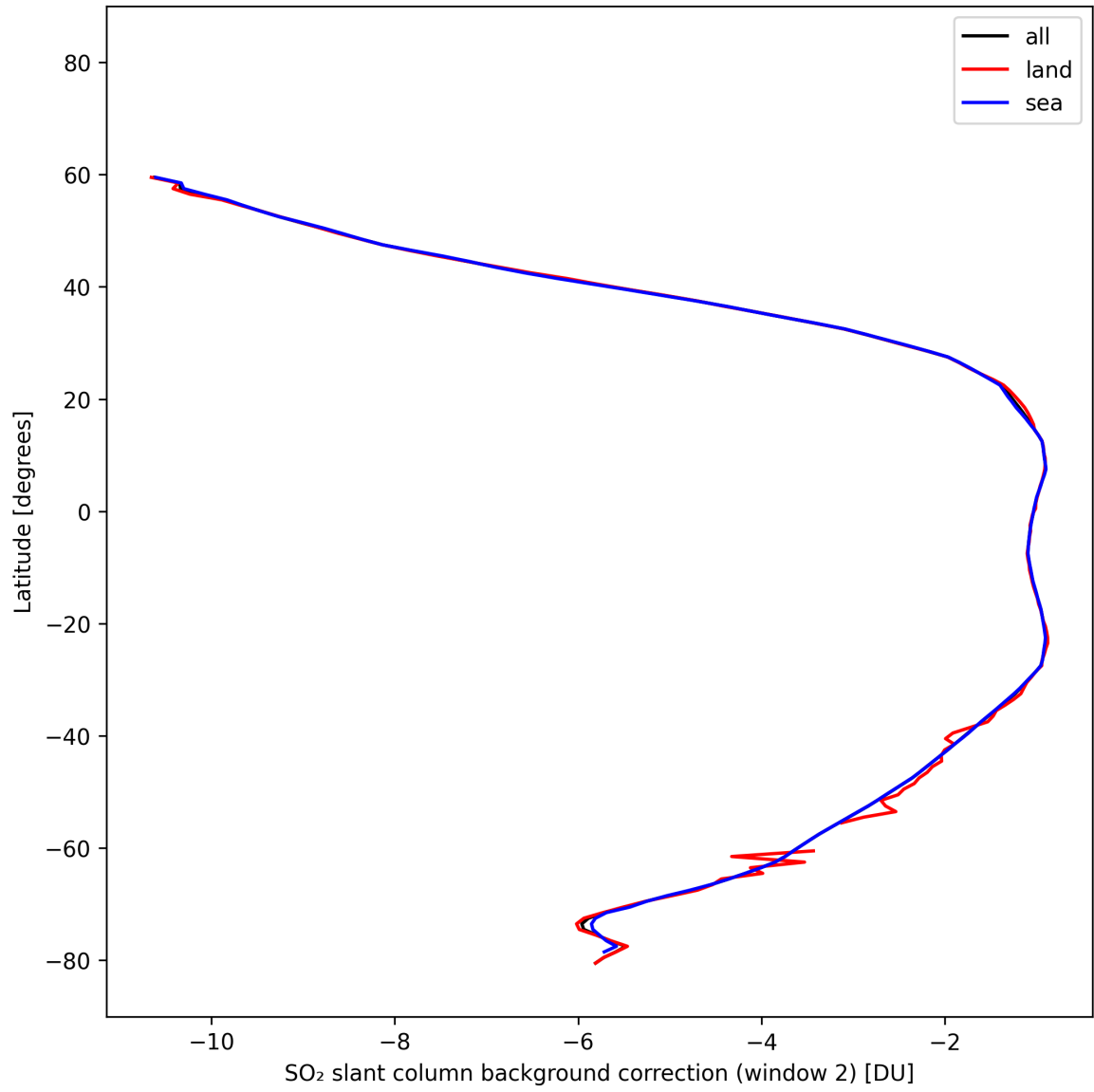
Figure 43: Zonal average of “SO 2 slant column background correction (window 2)” for 2025-02-21 to 2025-02-22.
