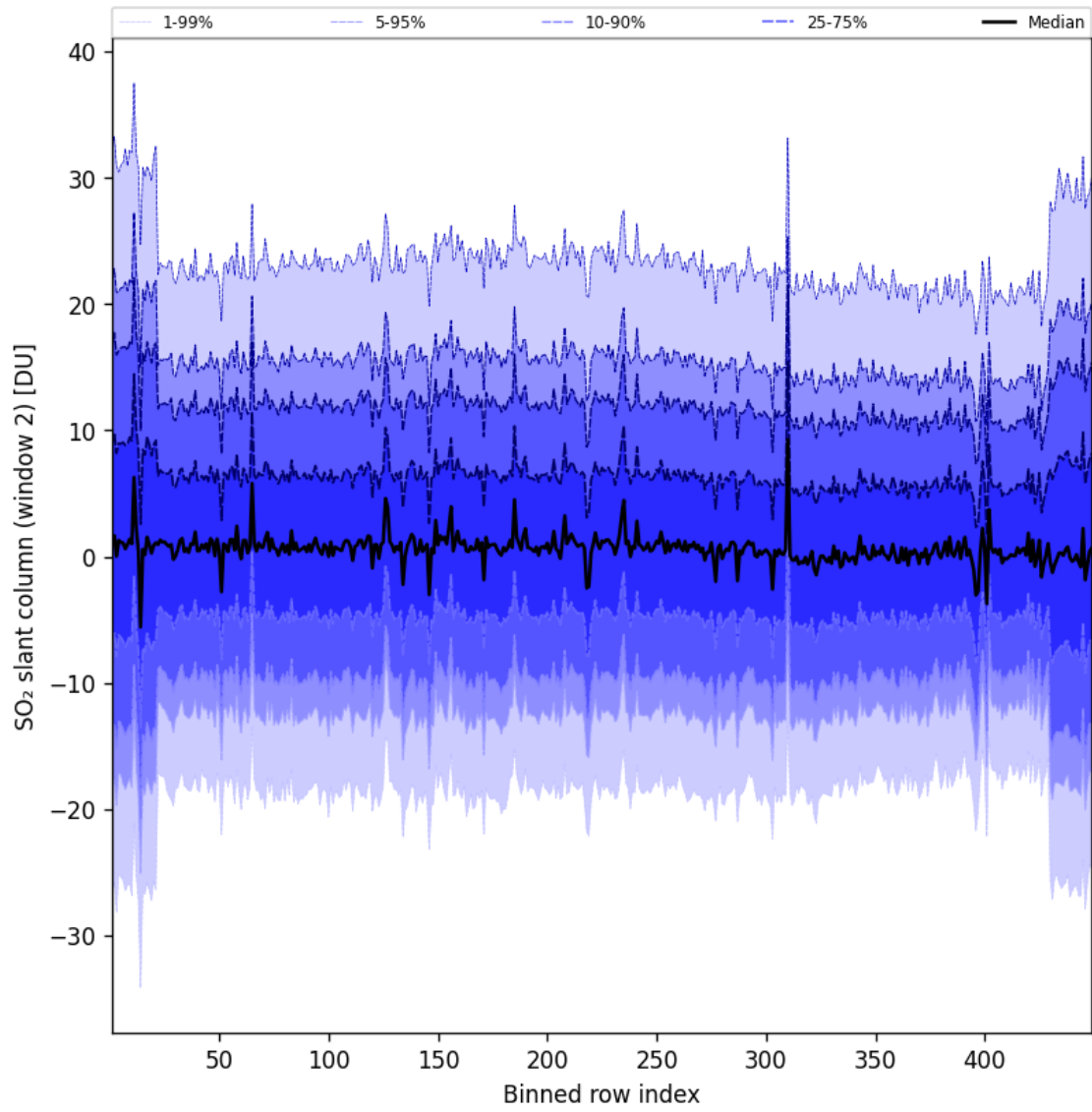
Figure 94: Along track statistics of “SO 2 slant column (window 2)” for 2025-02-21 to 2025-02-22
