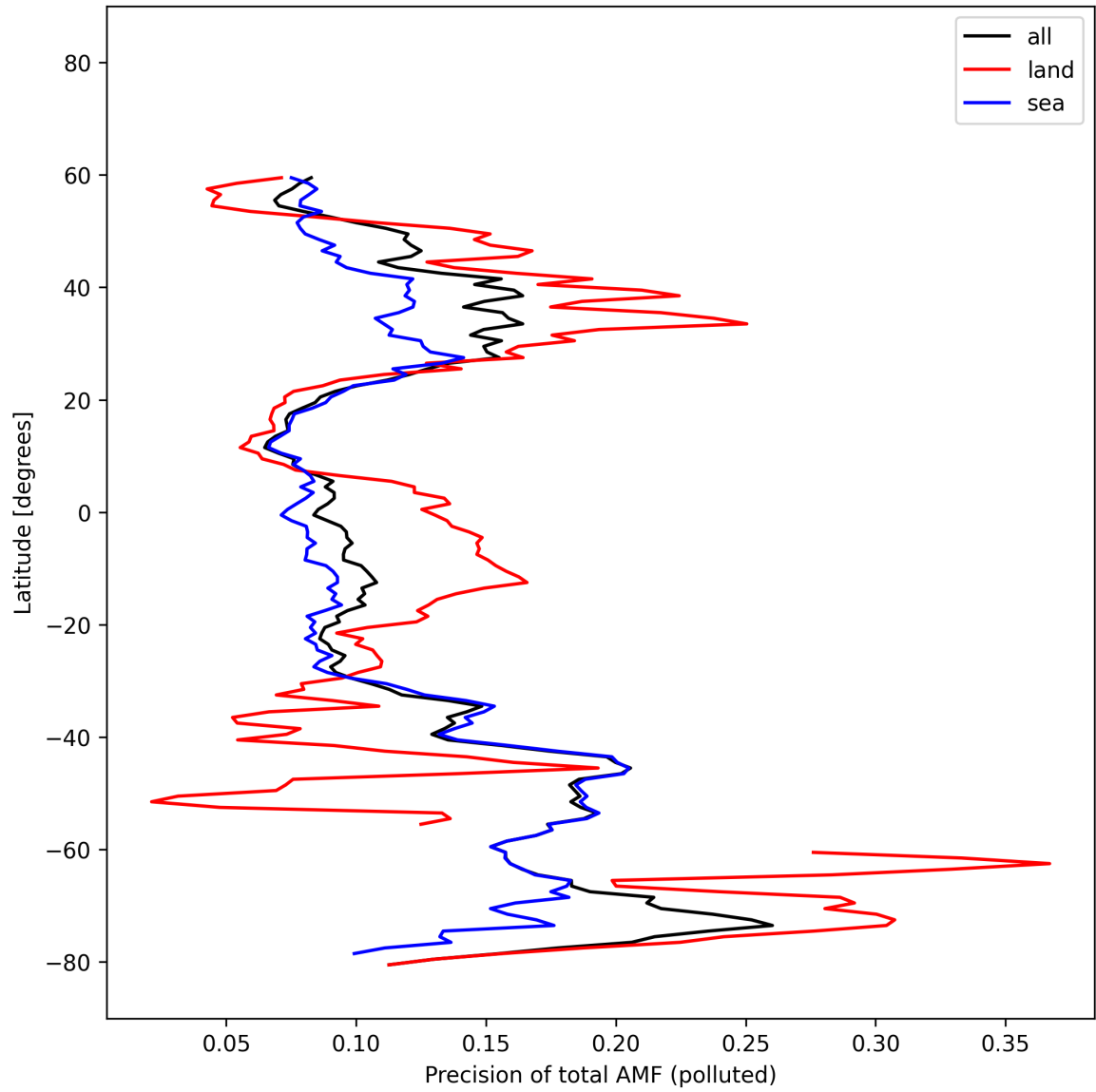
Figure 54: Zonal average of “Precision of total AMF (polluted)” for 2025-02-21 to 2025-02-22.
