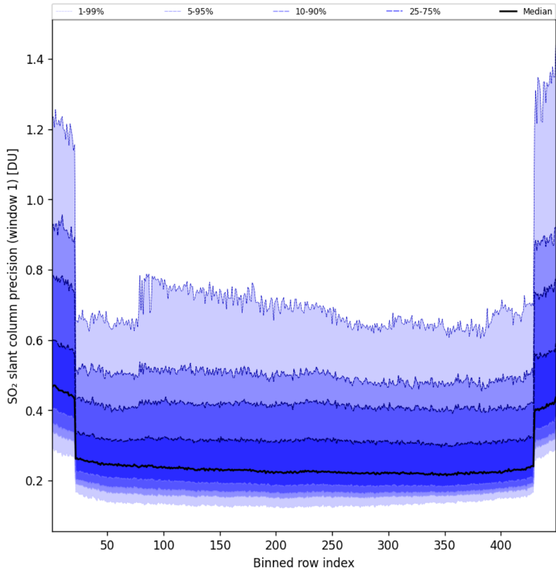
Figure 91: Along track statistics of “SO 2 slant column precision (window 1)” for 2025-02-21 to 2025-02-22
