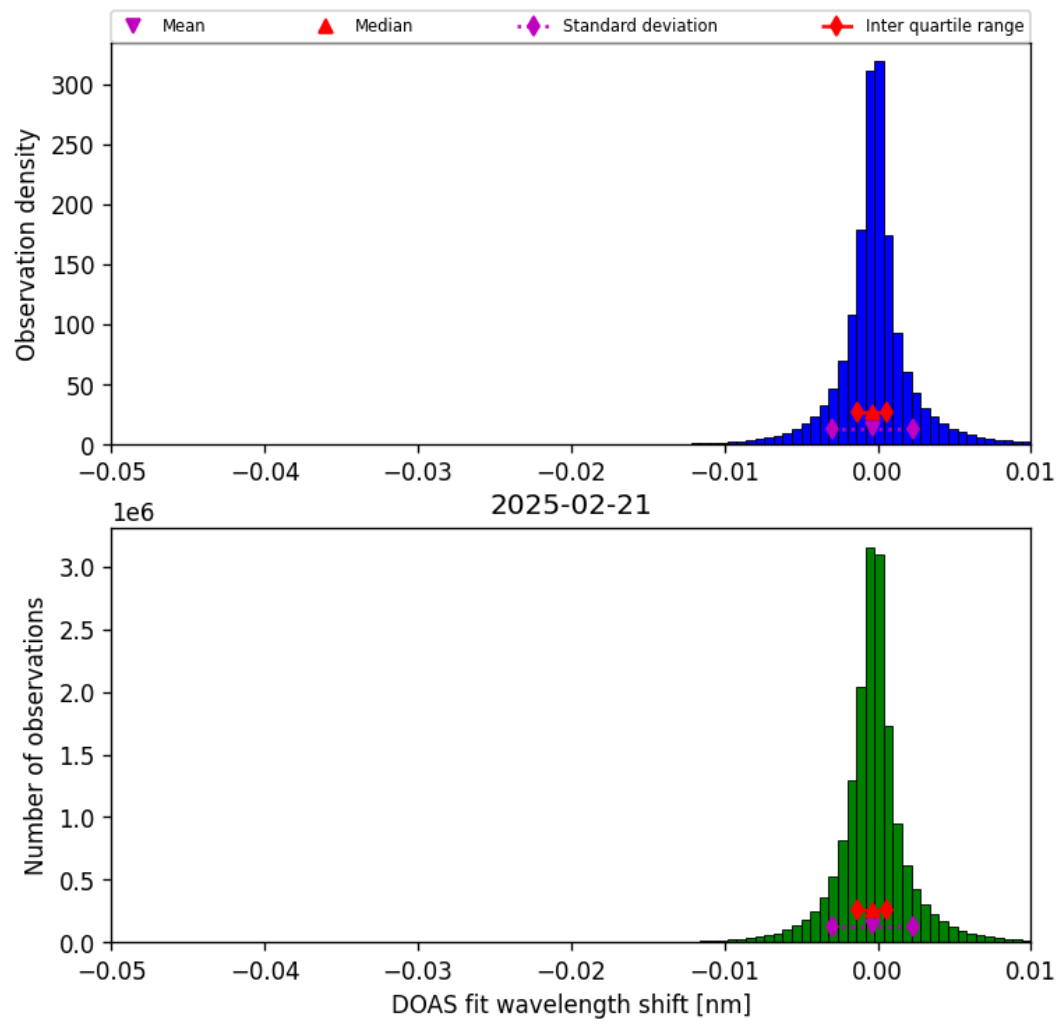
Figure 77: Histogram of “DOAS fit wavelength shift” for 2025-02-21 to 2025-02-22
