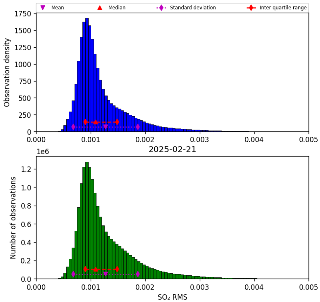
Figure 79: Histogram of “SO 2 RMS” for 2025-02-21 to 2025-02-22
