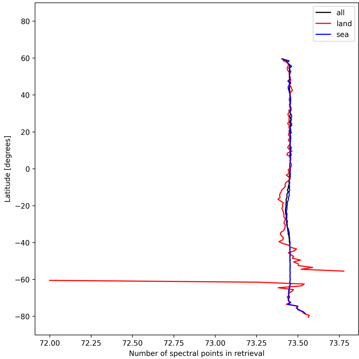
Figure 56: Zonal average of “Number of spectral points in retrieval” for 2025-02-21 to 2025-02-22.
