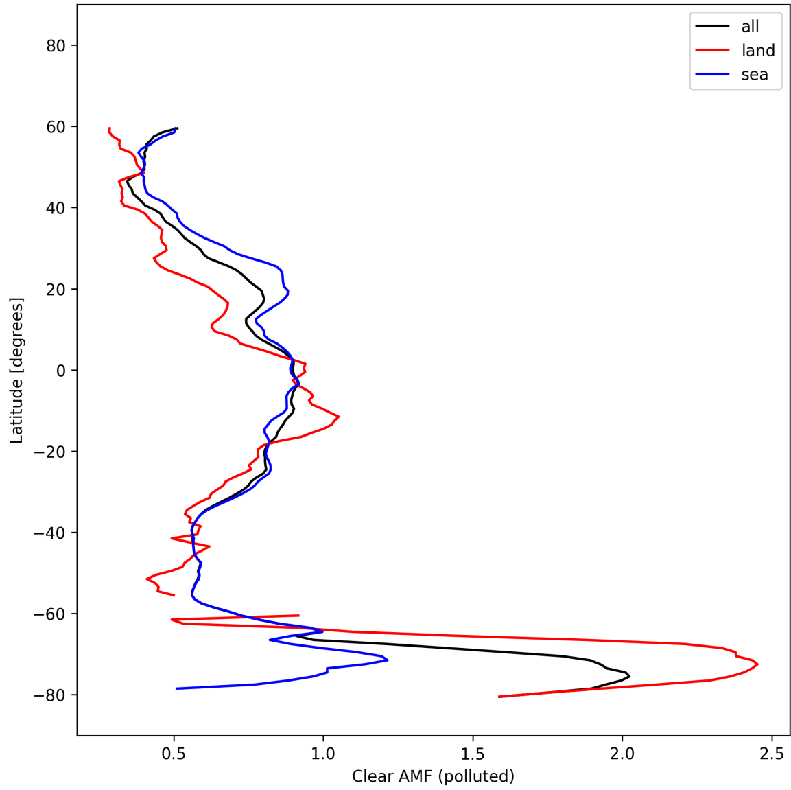
Figure 55: Zonal average of “Clear AMF (polluted)” for 2025-02-21 to 2025-02-22.
