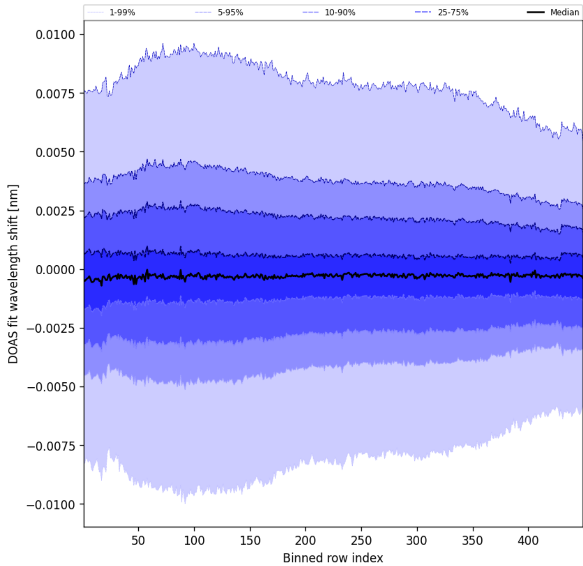
Figure 104: Along track statistics of “DOAS fit wavelength shift” for 2025-02-21 to 2025-02-22
