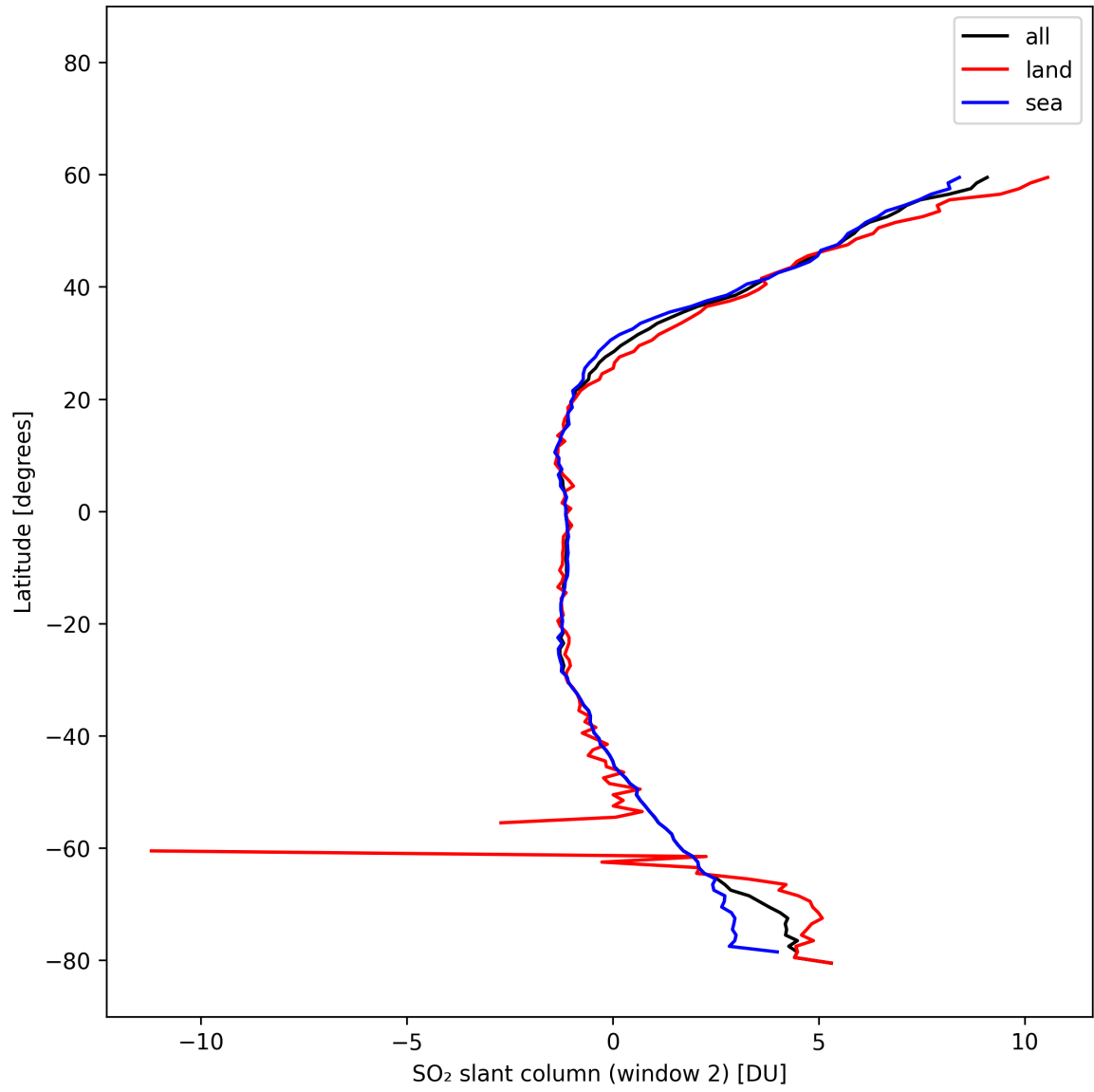
Figure 40: Zonal average of “SO 2 slant column (window 2)” for 2025-02-21 to 2025-02-22.
