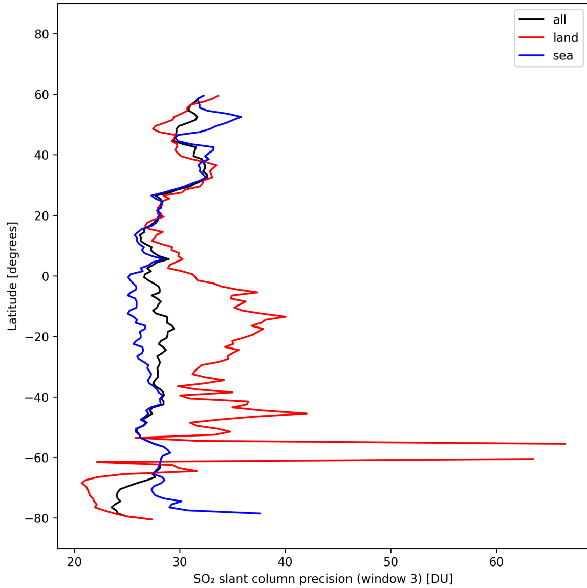
Figure 45: Zonal average of “SO 2 slant column precision (window 3)” for 2025-02-21 to 2025-02-22.
