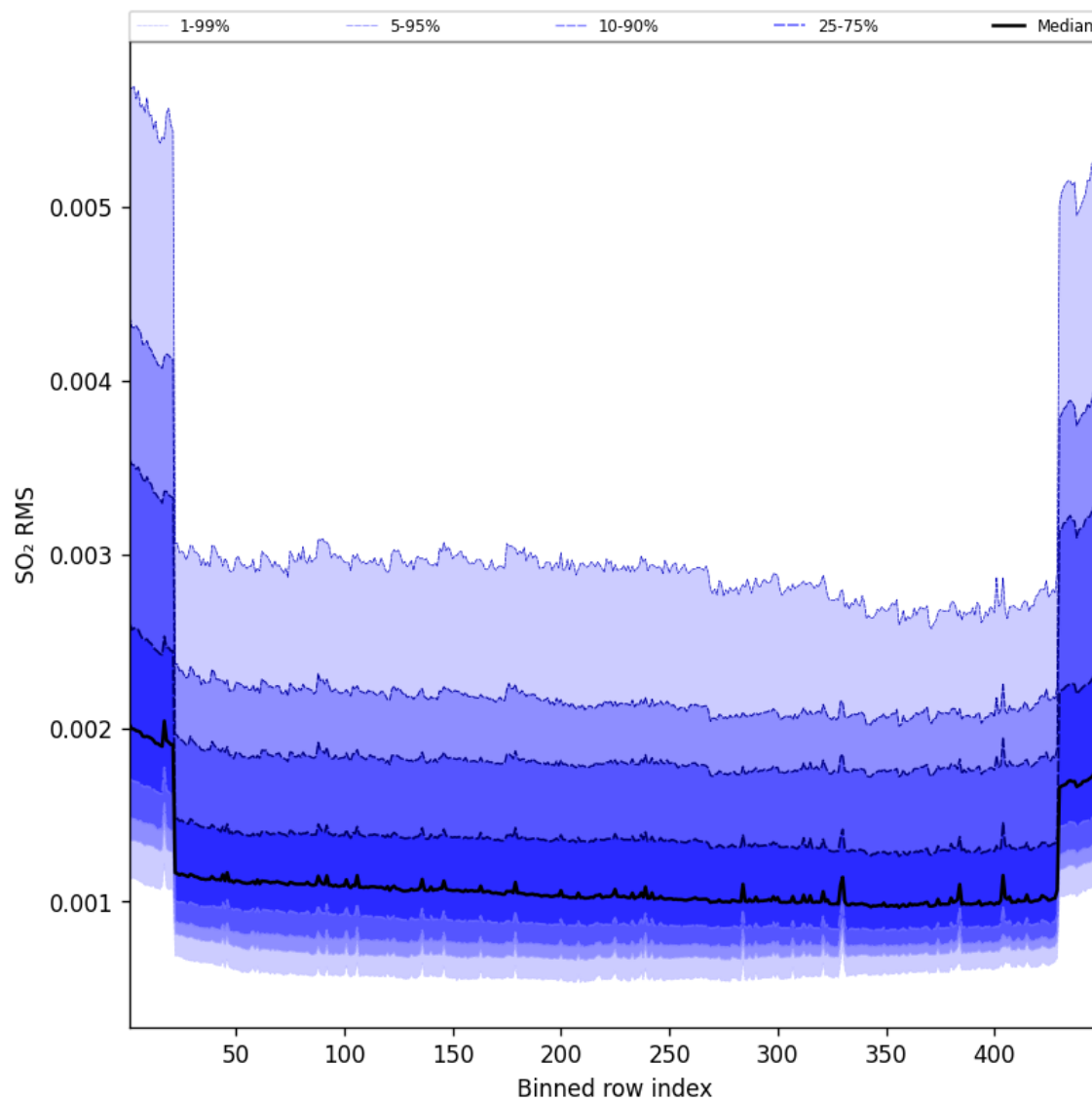
Figure 106: Along track statistics of “SO 2 RMS” for 2025-02-21 to 2025-02-22
