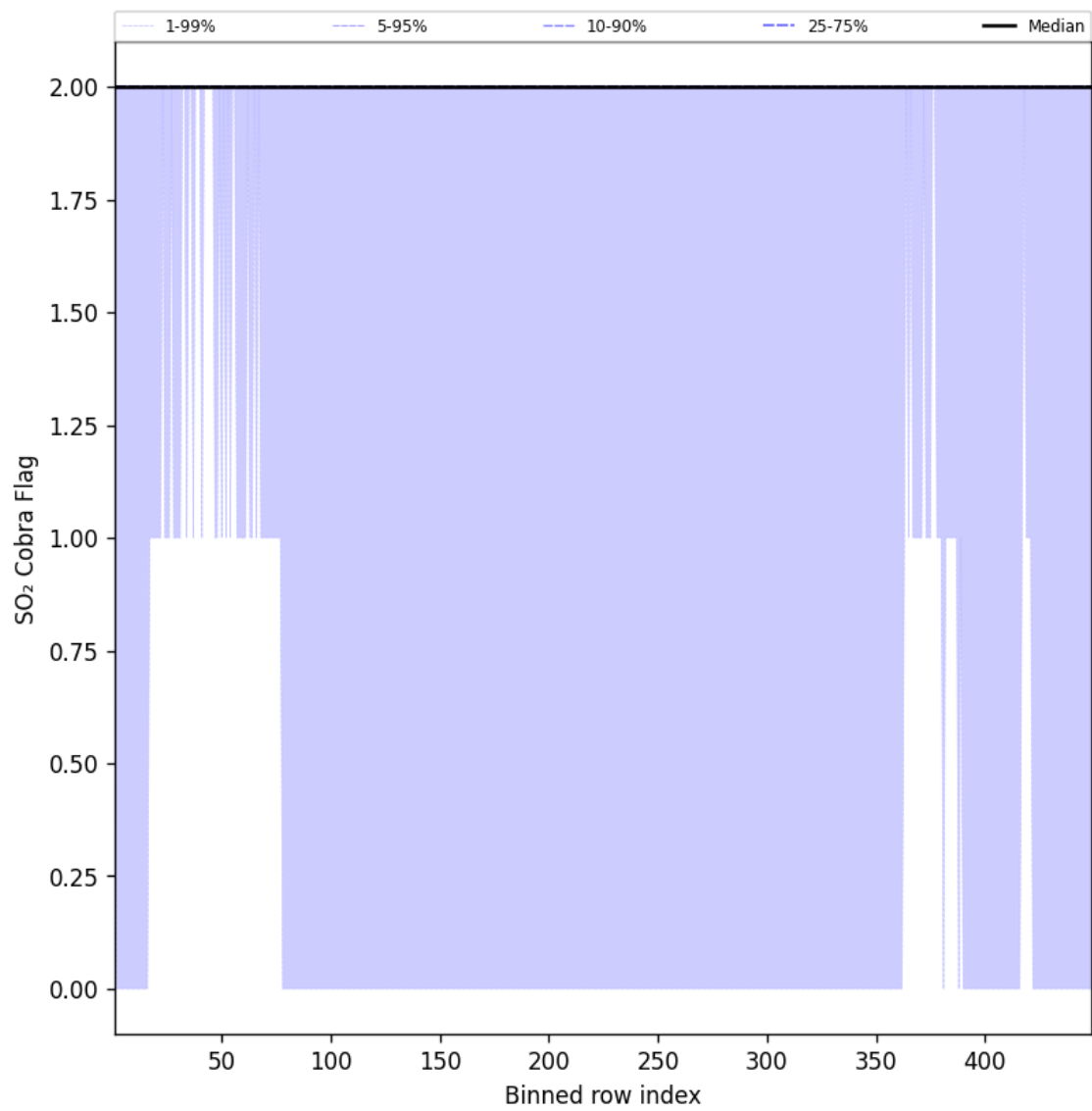
Figure 102: Along track statistics of "SO 2 Cobra Flag" for 2025-02-21 to 2025-02-22
