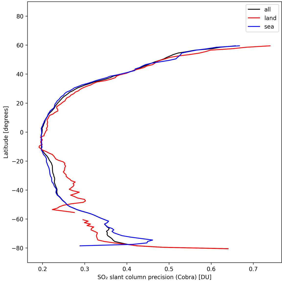
Figure 35: Zonal average of “SO 2 slant column precision (Cobra)” for 2025-02-21 to 2025-02-22.
