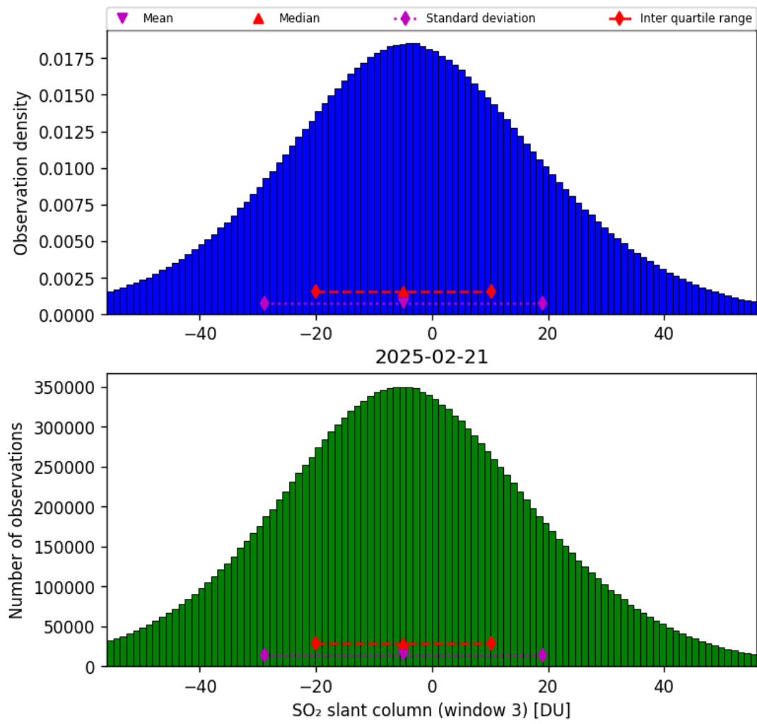
Figure 71: Histogram of “SO 2 slant column (window 3)” for 2025-02-21 to 2025-02-22
