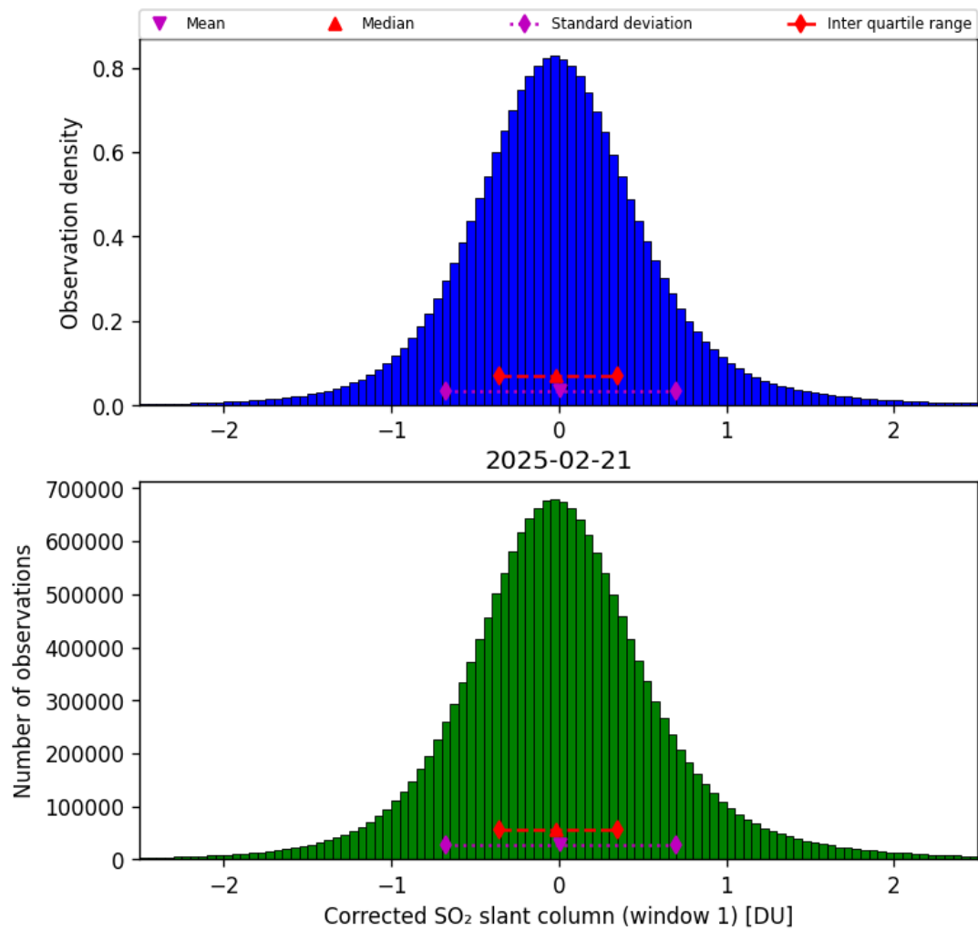
Figure 65: Histogram of “Corrected SO 2 slant column (window 1)” for 2025-02-21 to 2025-02-22
