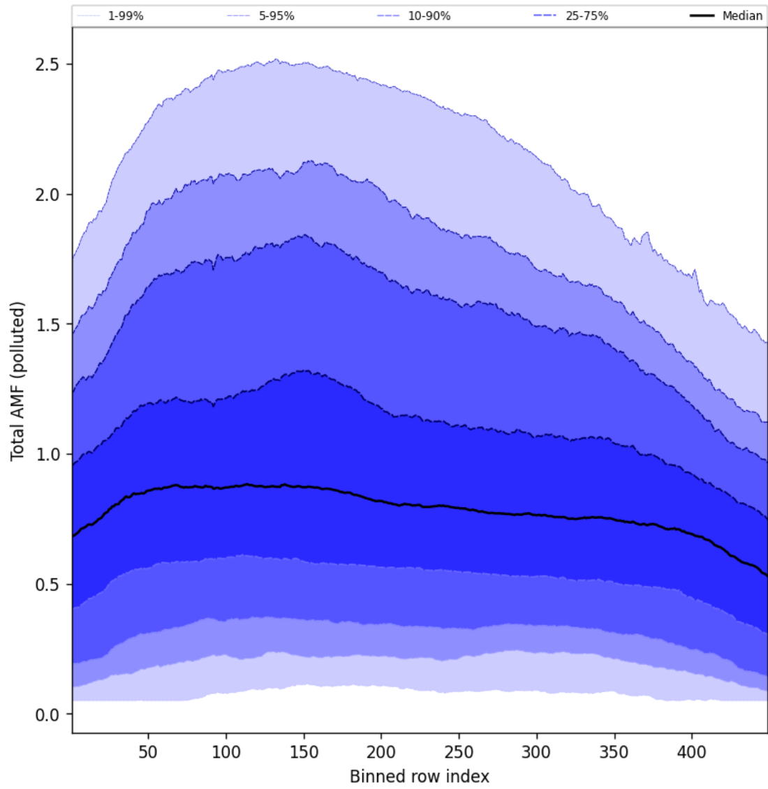
Figure 107: Along track statistics of “Total AMF (polluted)” for 2025-02-21 to 2025-02-22
