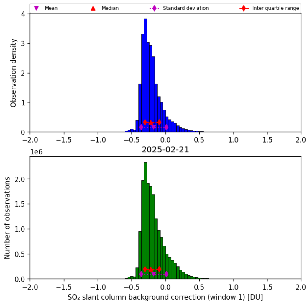
Figure 66: Histogram of “SO 2 slant column background correction (window 1)” for 2025-02-21 to 2025-02-22
