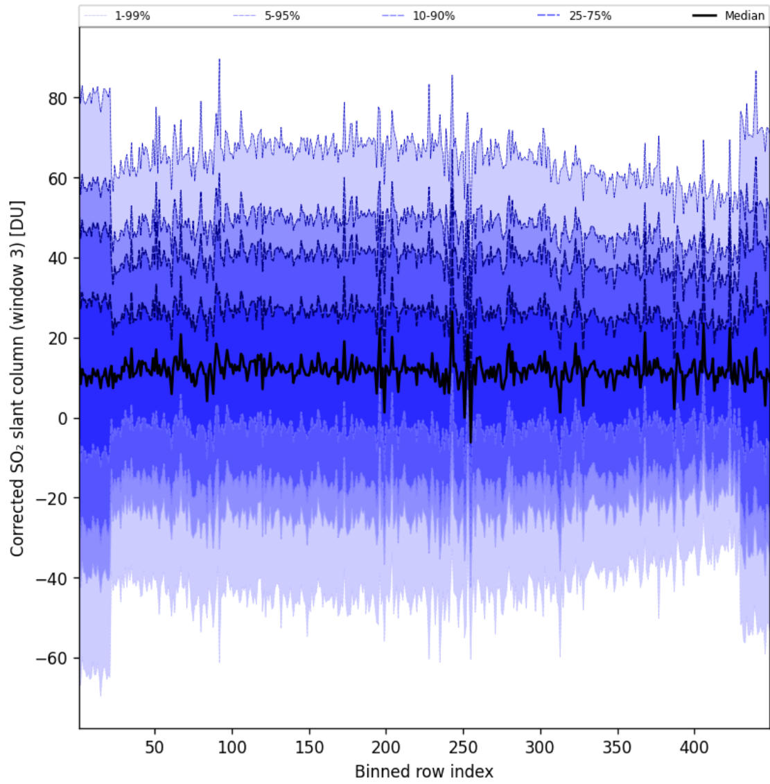
Figure 100: Along track statistics of “Corrected SO 2 slant column (window 3)” for 2025-02-21 to 2025-02-22
