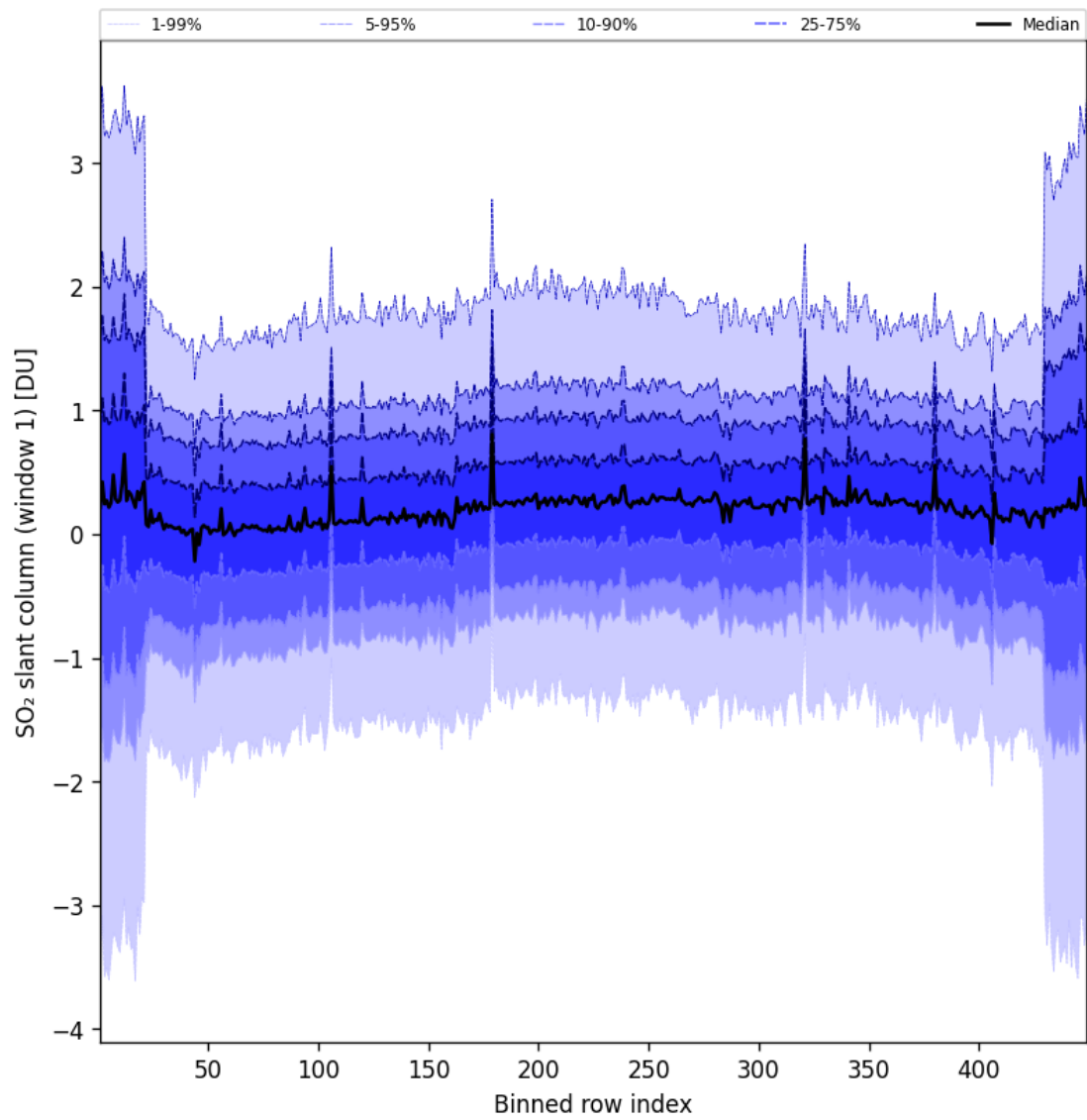
Figure 90: Along track statistics of “SO 2 slant column (window 1)” for 2025-02-21 to 2025-02-22
