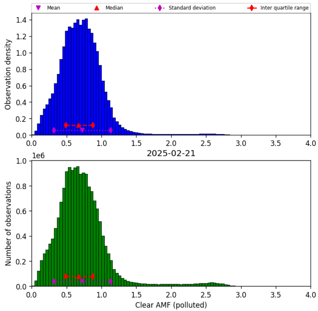
Figure 82: Histogram of “Clear AMF (polluted)” for 2025-02-21 to 2025-02-22
