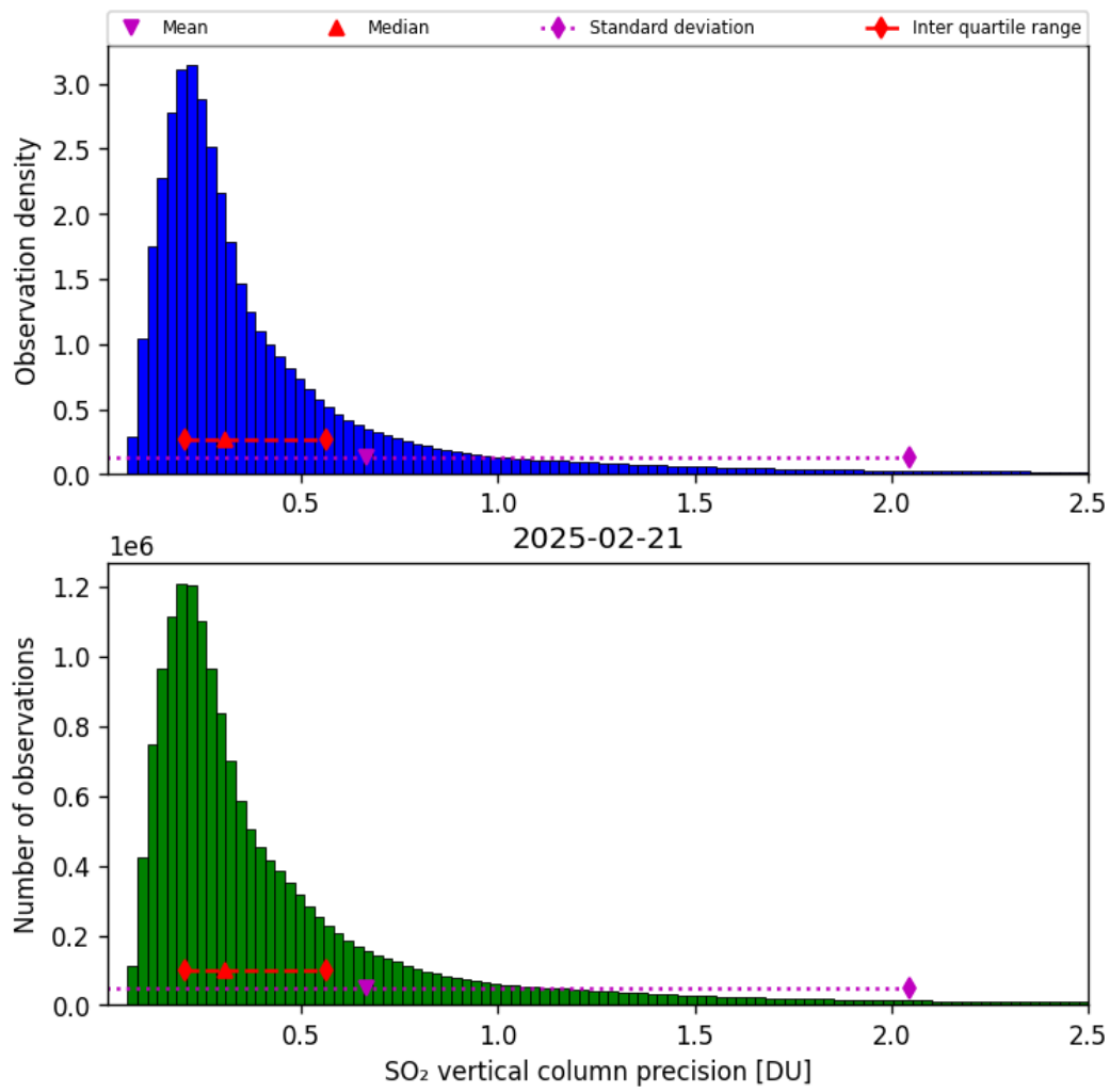
Figure 59: Histogram of “SO 2 vertical column precision” for 2025-02-21 to 2025-02-22
