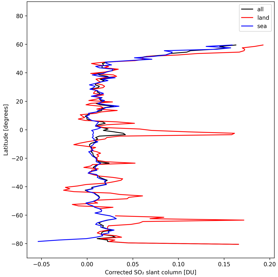
Figure 33: Zonal average of “Corrected SO 2 slant column” for 2025-02-21 to 2025-02-22.
