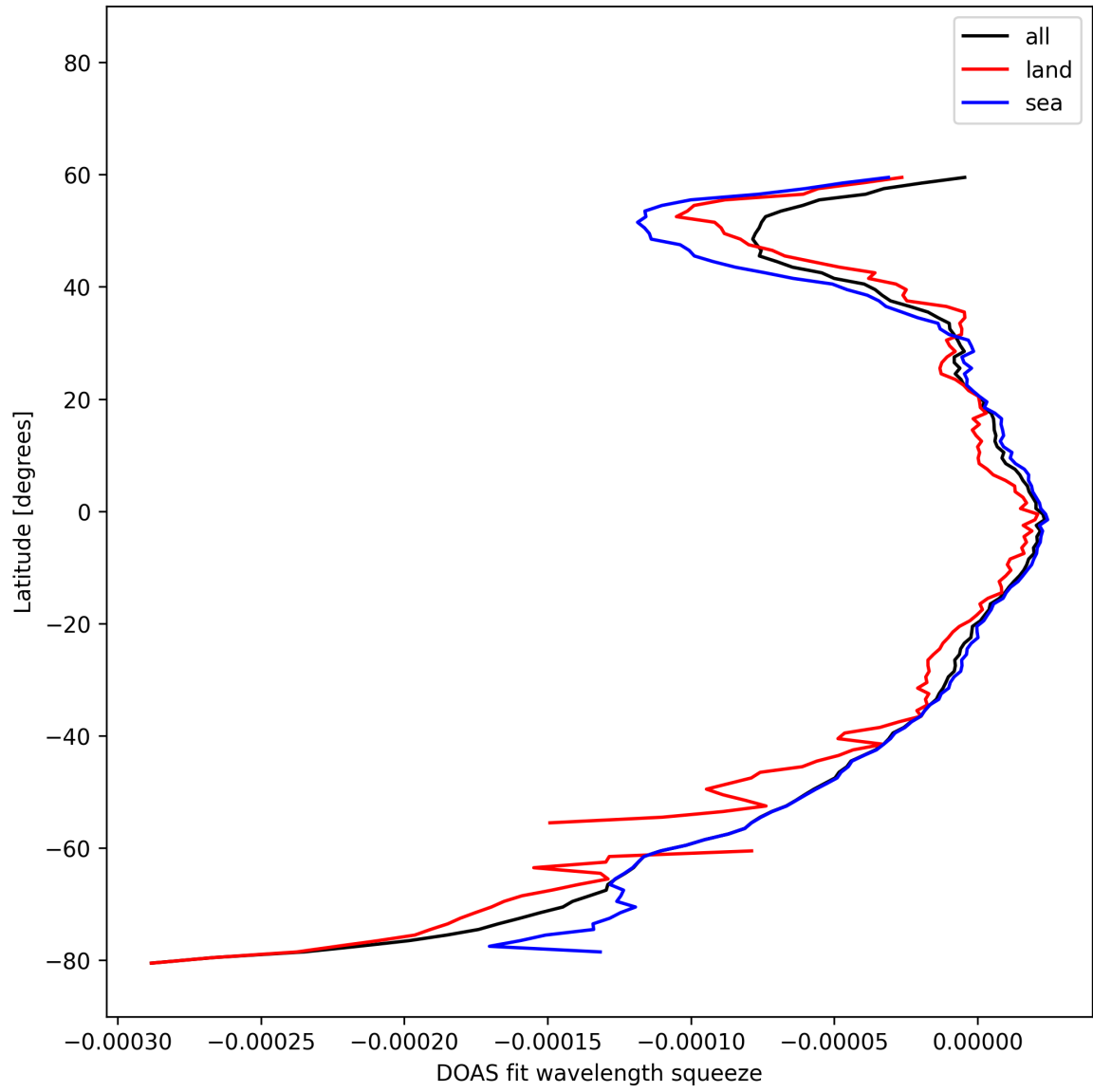
Figure 51: Zonal average of “DOAS fit wavelength squeeze” for 2025-02-21 to 2025-02-22.
