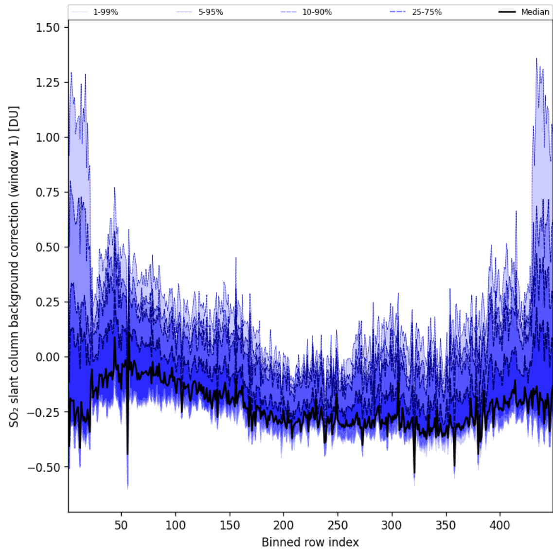
Figure 93: Along track statistics of “SO 2 slant column background correction (window 1)” for 2025-02-21 to 2025-02-22
