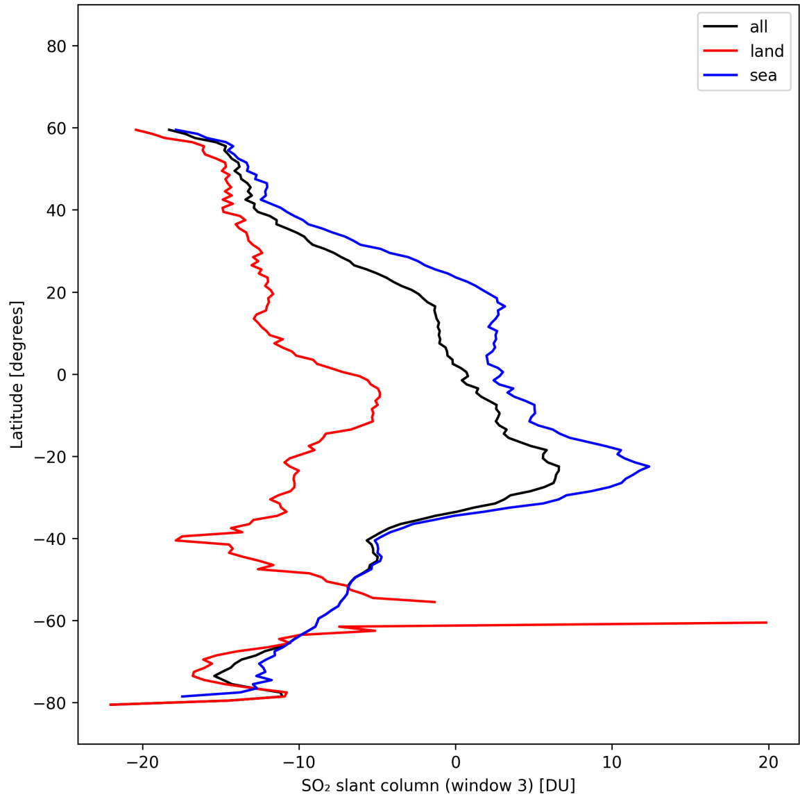
Figure 44: Zonal average of “SO 2 slant column (window 3)” for 2025-02-21 to 2025-02-22.
