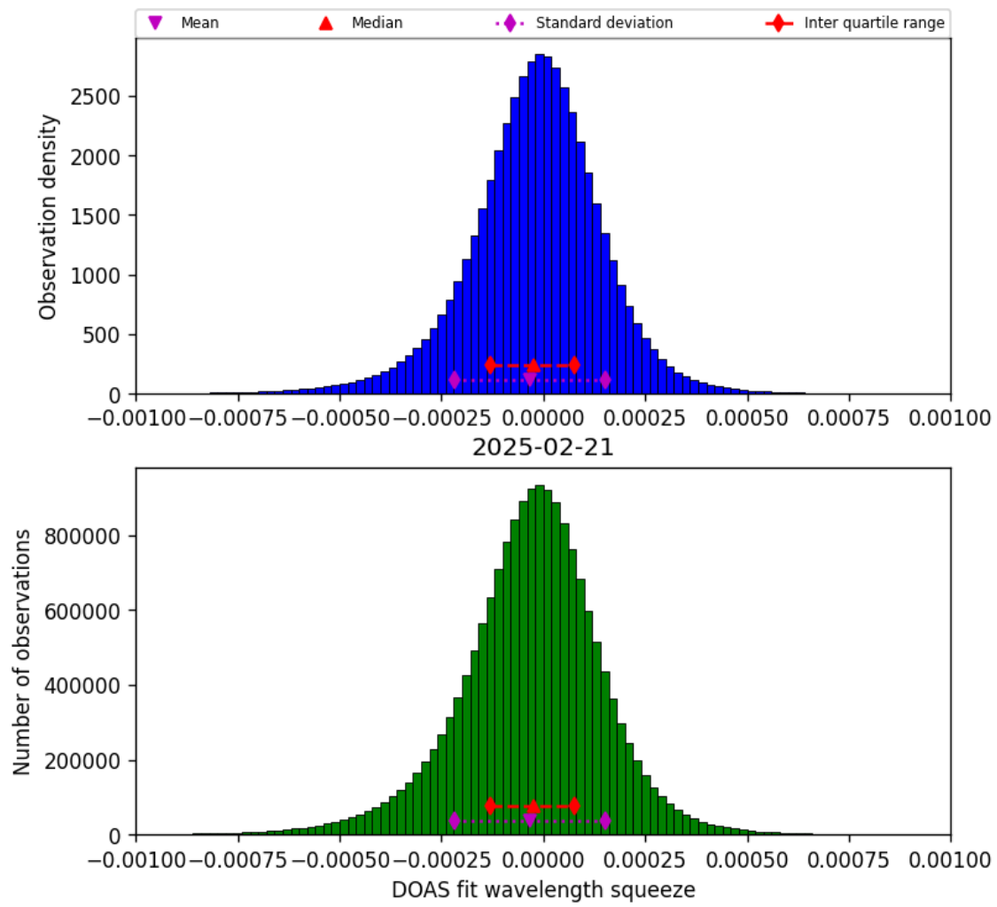
Figure 78: Histogram of “DOAS fit wavelength squeeze” for 2025-02-21 to 2025-02-22
