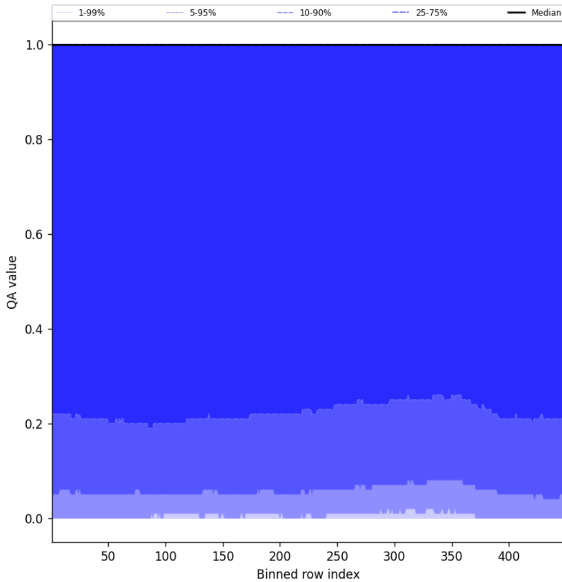
Figure 84: Along track statistics of “QA value” for 2025-02-21 to 2025-02-22
