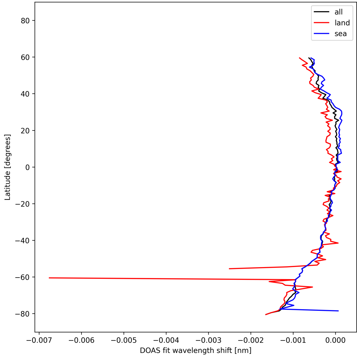
Figure 50: Zonal average of "DOAS fit wavelength shift" for 2025-02-21 to 2025-02-22.
