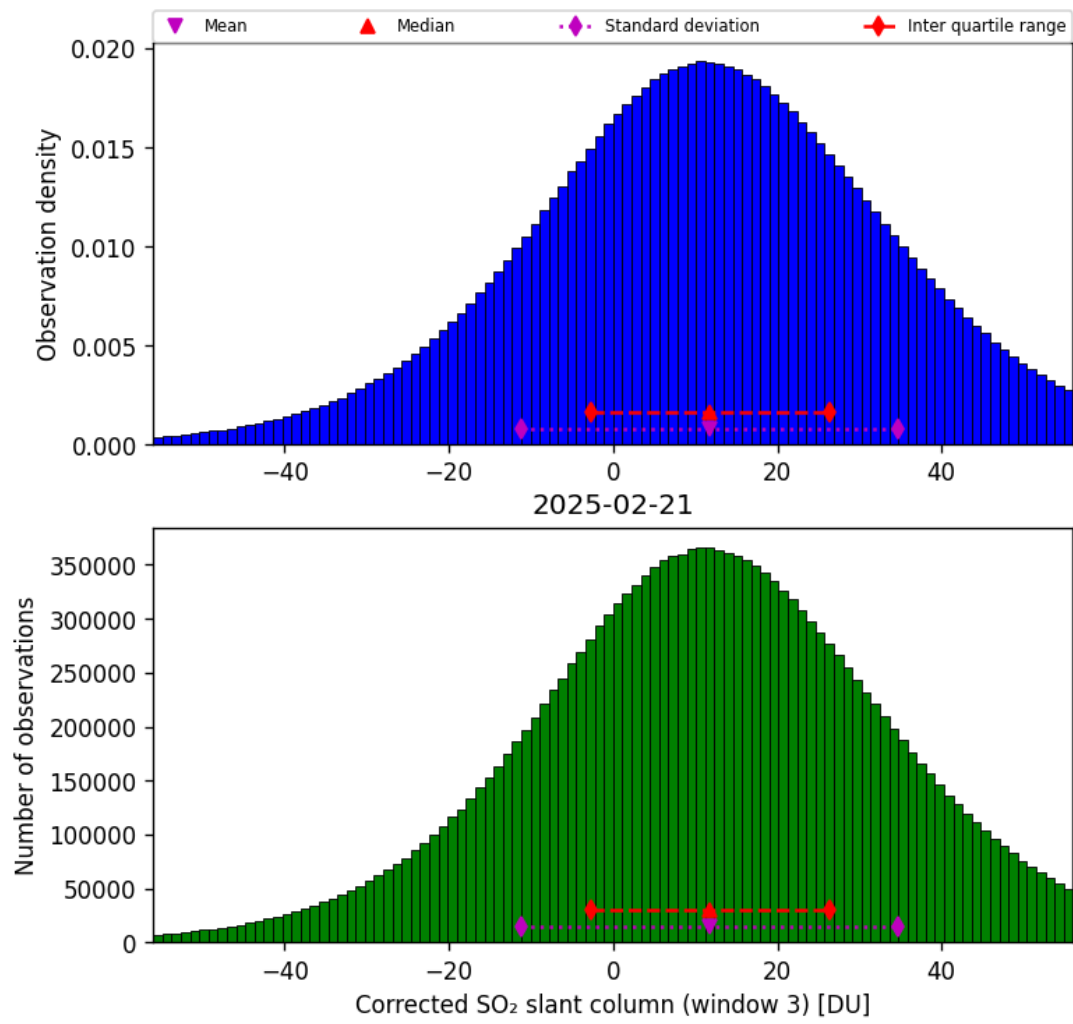
Figure 73: Histogram of “Corrected SO 2 slant column (window 3)” for 2025-02-21 to 2025-02-22
