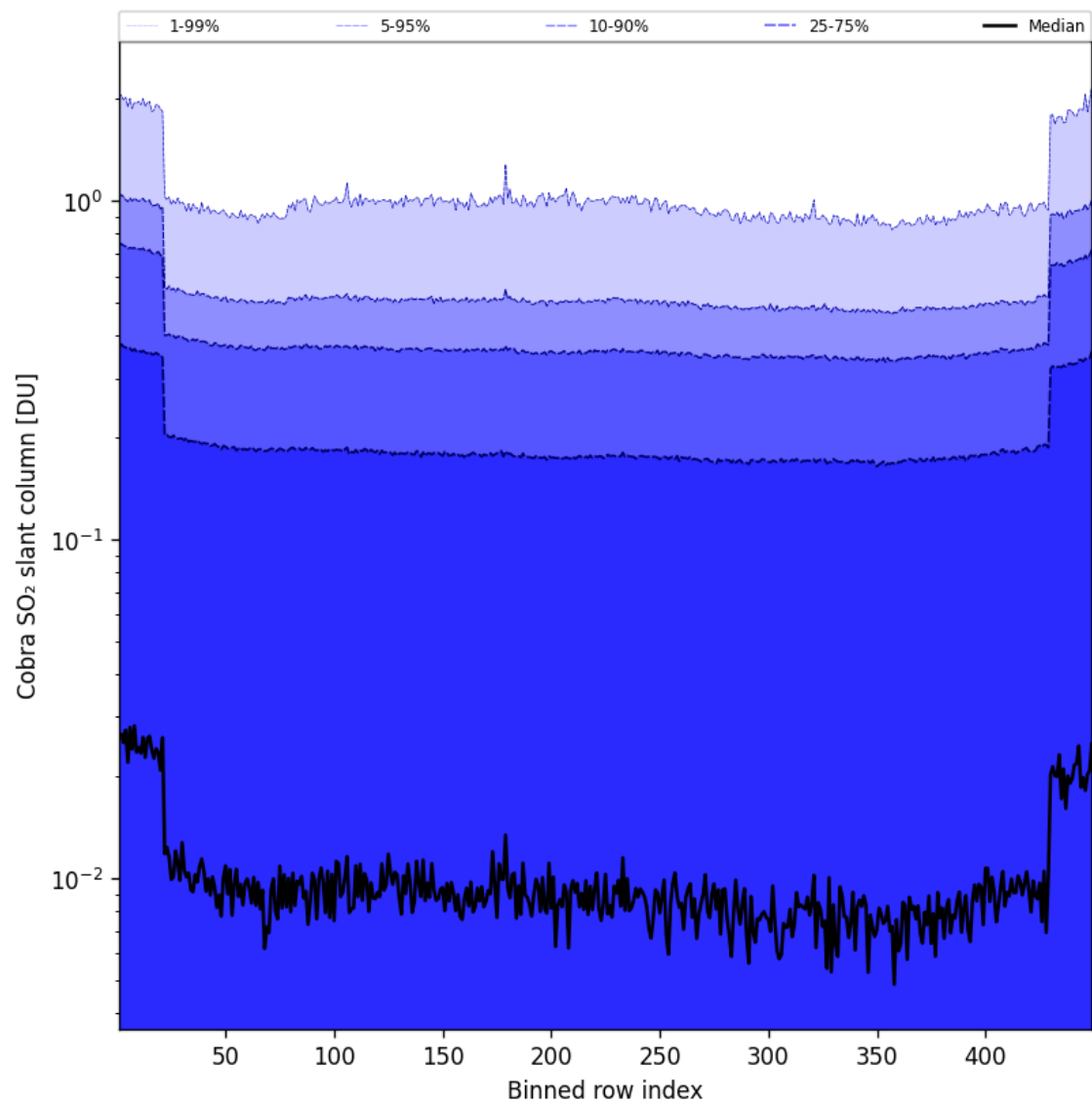
Figure 88: Along track statistics of “Cobra SO 2 slant column” for 2025-02-21 to 2025-02-22
