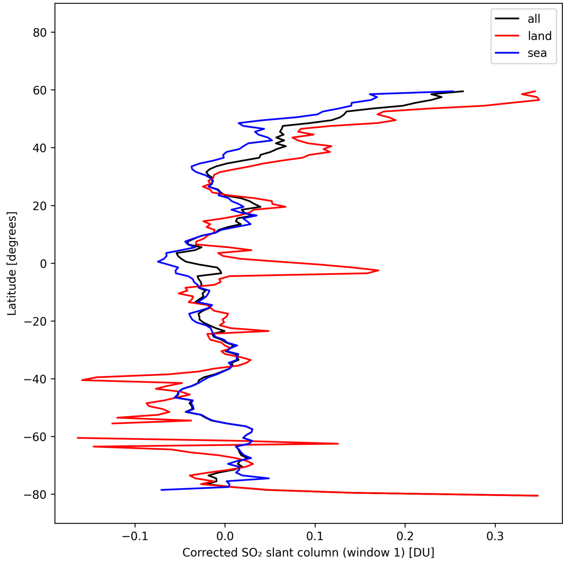
Figure 38: Zonal average of “Corrected SO 2 slant column (window 1)” for 2025-02-21 to 2025-02-22.
