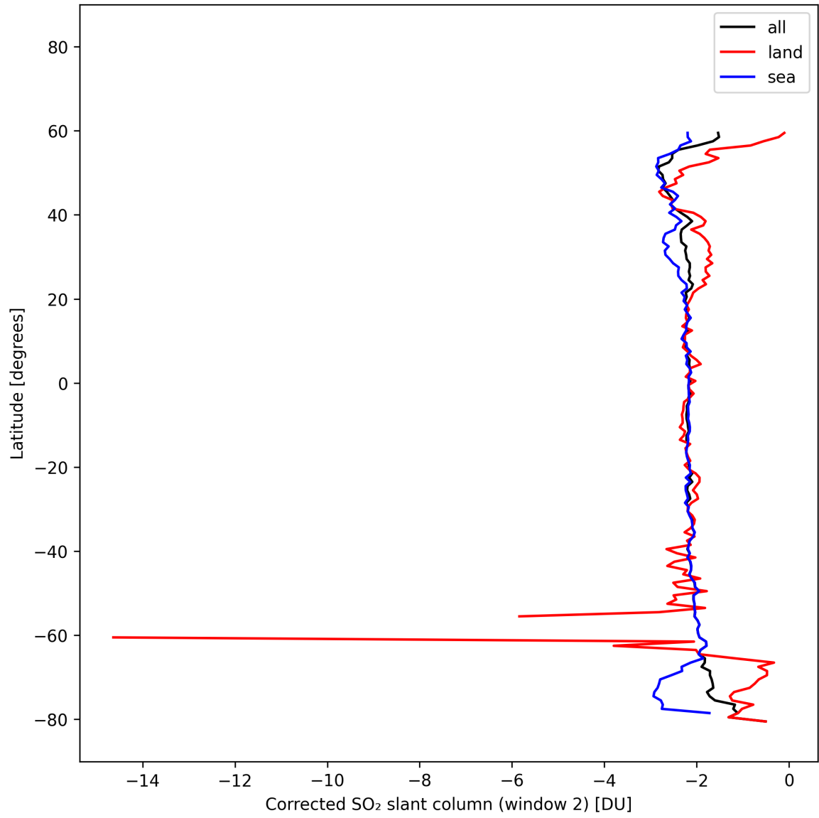
Figure 42: Zonal average of “Corrected SO 2 slant column (window 2)” for 2025-02-21 to 2025-02-22.
