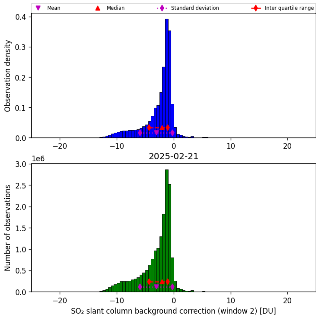
Figure 70: Histogram of “SO 2 slant column background correction (window 2)” for 2025-02-21 to 2025-02-22
