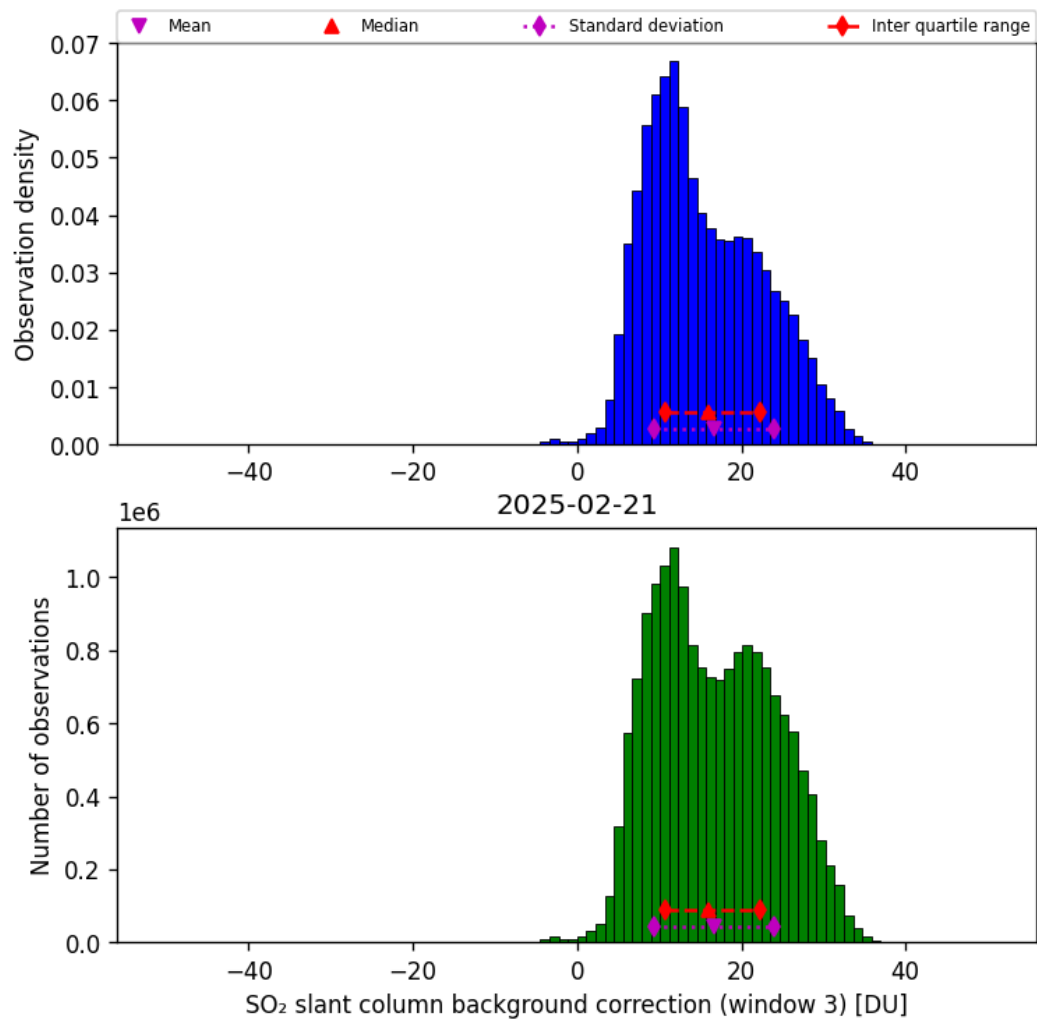
Figure 74: Histogram of “SO 2 slant column background correction (window 3)” for 2025-02-21 to 2025-02-22
