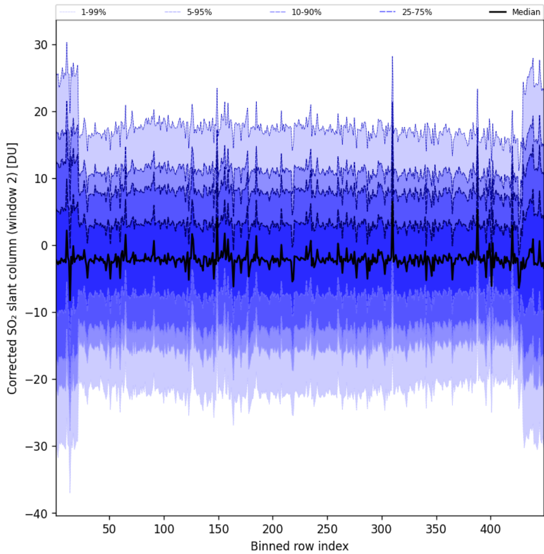
Figure 96: Along track statistics of “Corrected SO 2 slant column (window 2)” for 2025-02-21 to 2025-02-22
