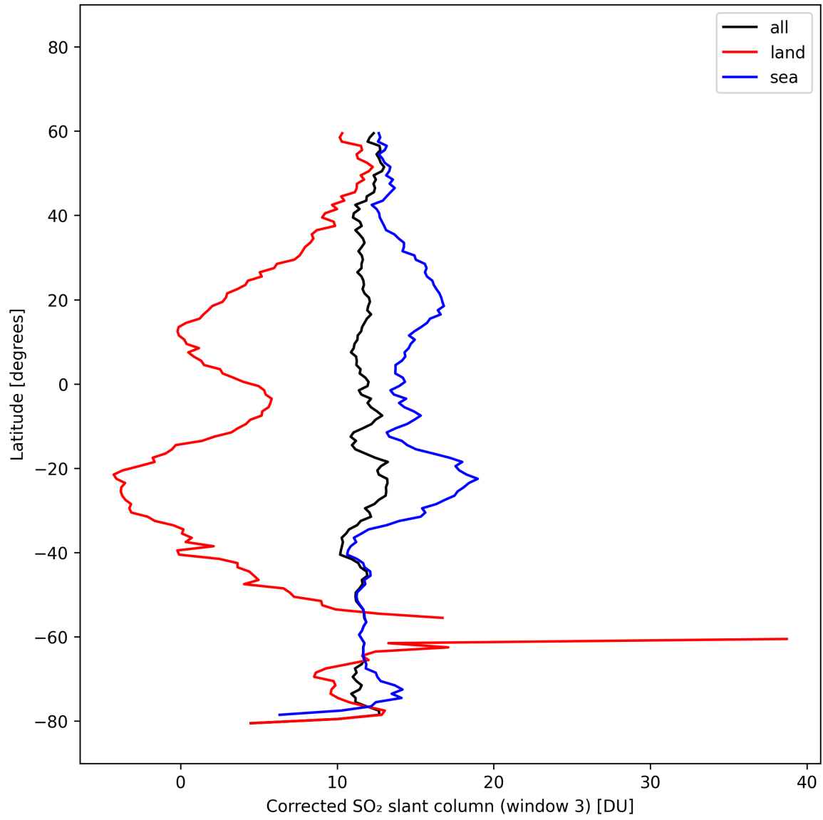
Figure 46: Zonal average of “Corrected SO 2 slant column (window 3)” for 2025-02-21 to 2025-02-22.
