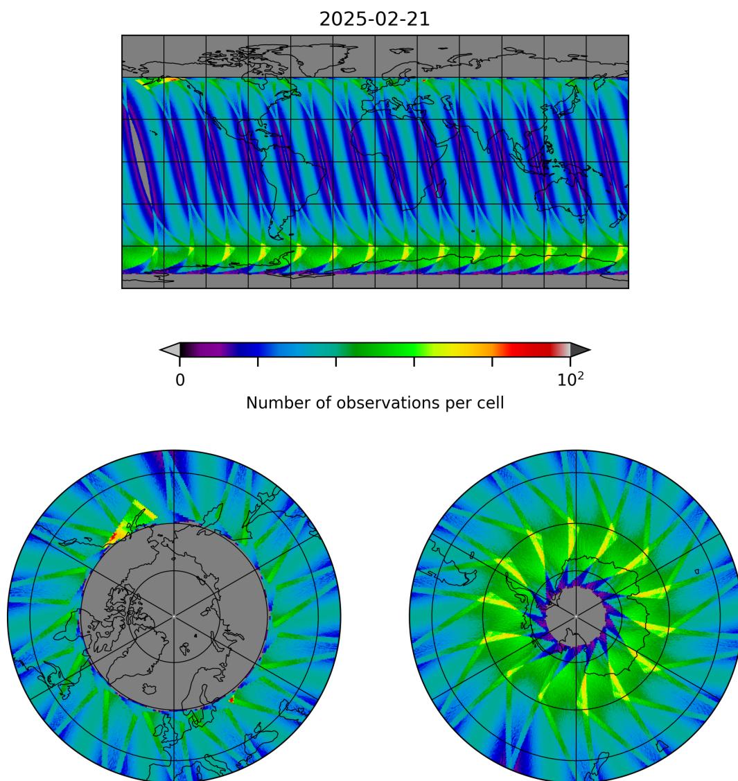
Figure 29: Map of the number of observations for 2025-02-21 to 2025-02-22
