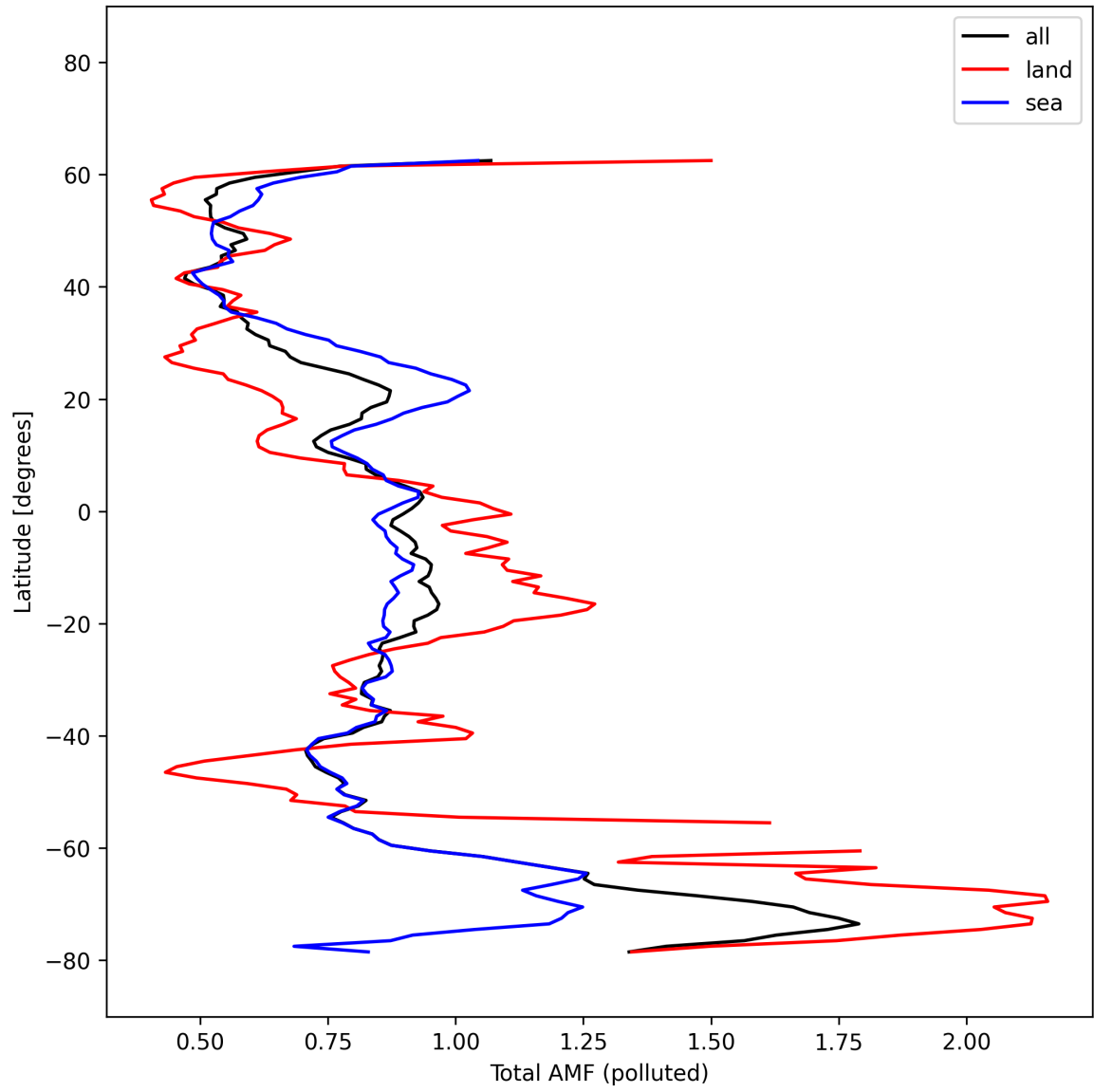
Figure 53: Zonal average of “Total AMF (polluted)” for 2025-02-27 to 2025-02-27.
