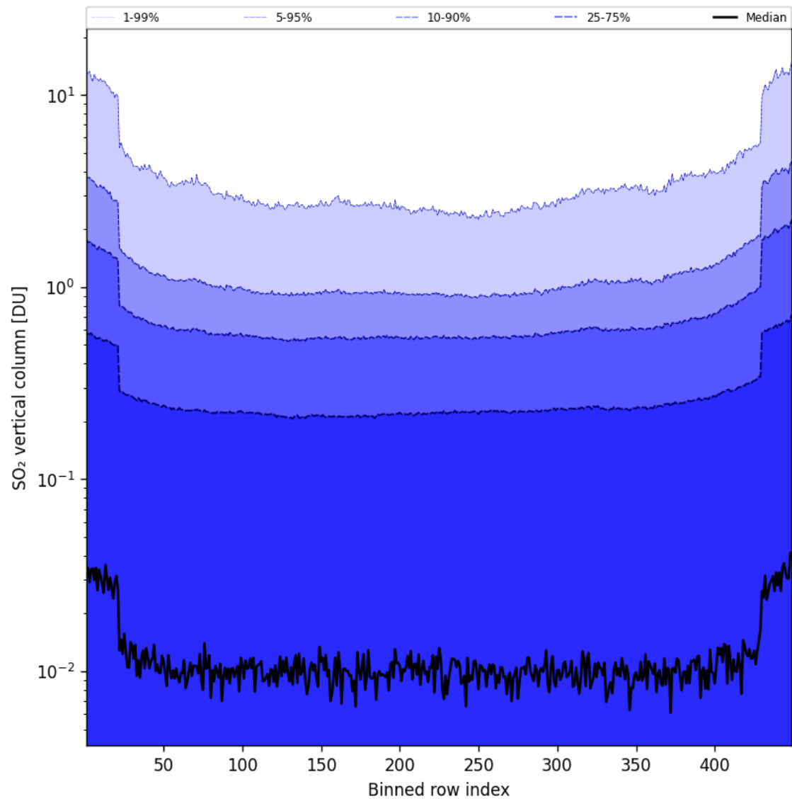
Figure 85: Along track statistics of “SO 2 vertical column” for 2025-02-27 to 2025-02-27
