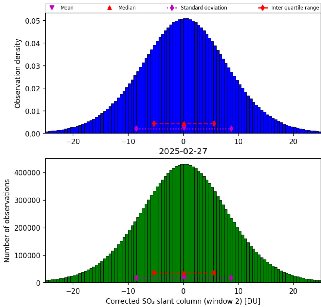
Figure 69: Histogram of “Corrected SO 2 slant column (window 2)” for 2025-02-27 to 2025-02-27
