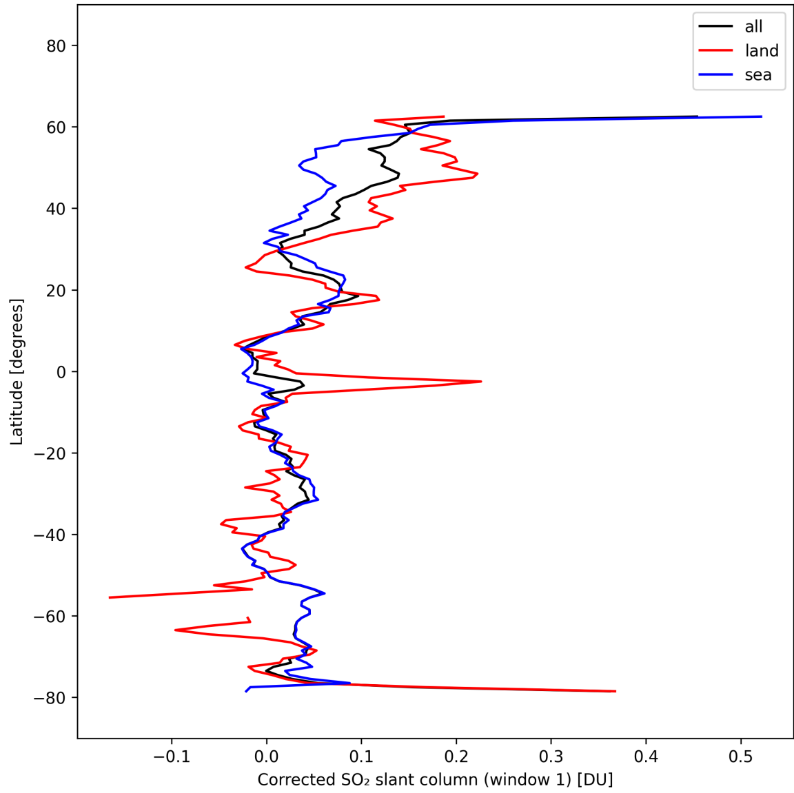
Figure 38: Zonal average of “Corrected SO 2 slant column (window 1)” for 2025-02-27 to 2025-02-27.
