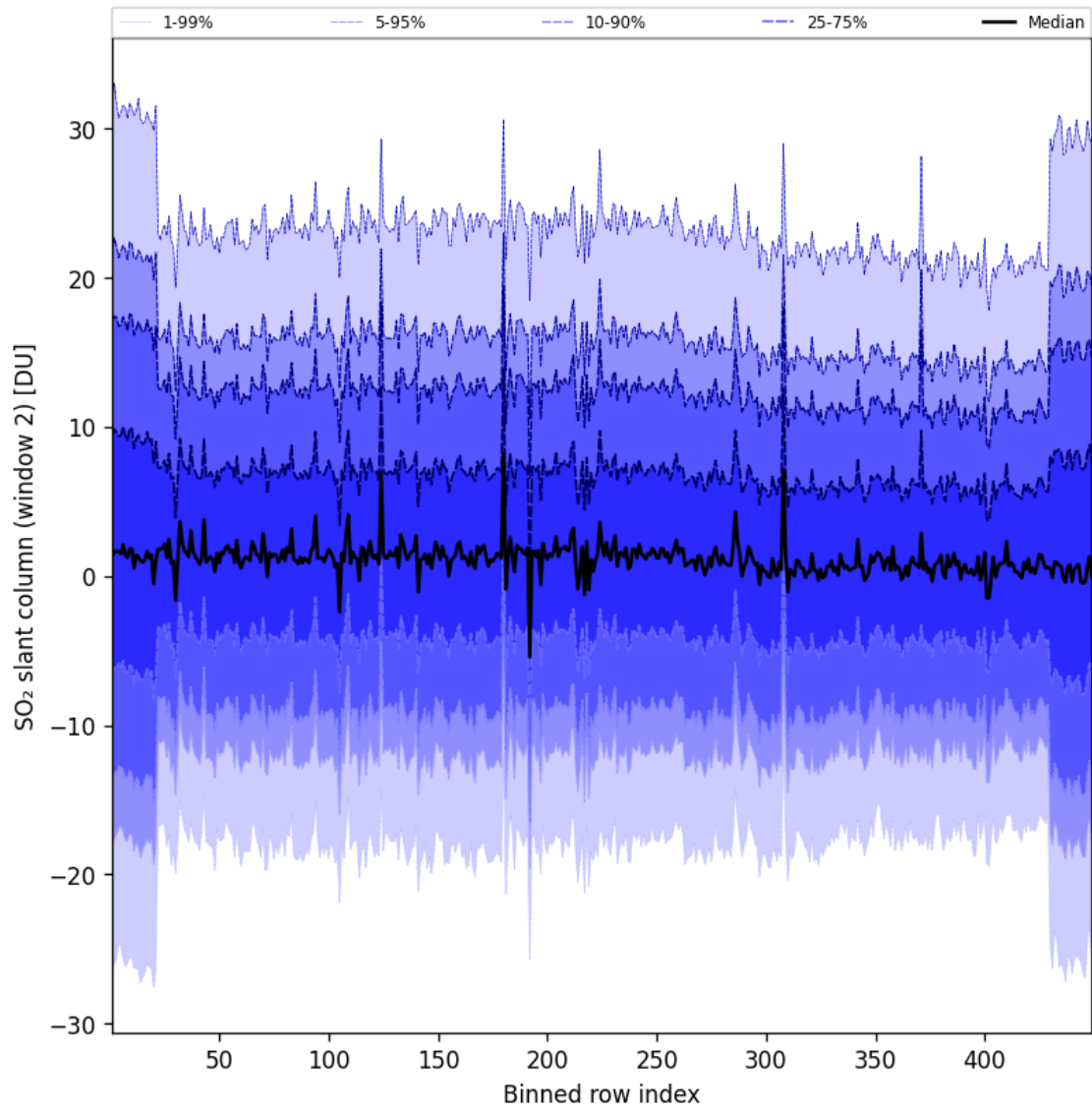
Figure 94: Along track statistics of “SO 2 slant column (window 2)” for 2025-02-27 to 2025-02-27
