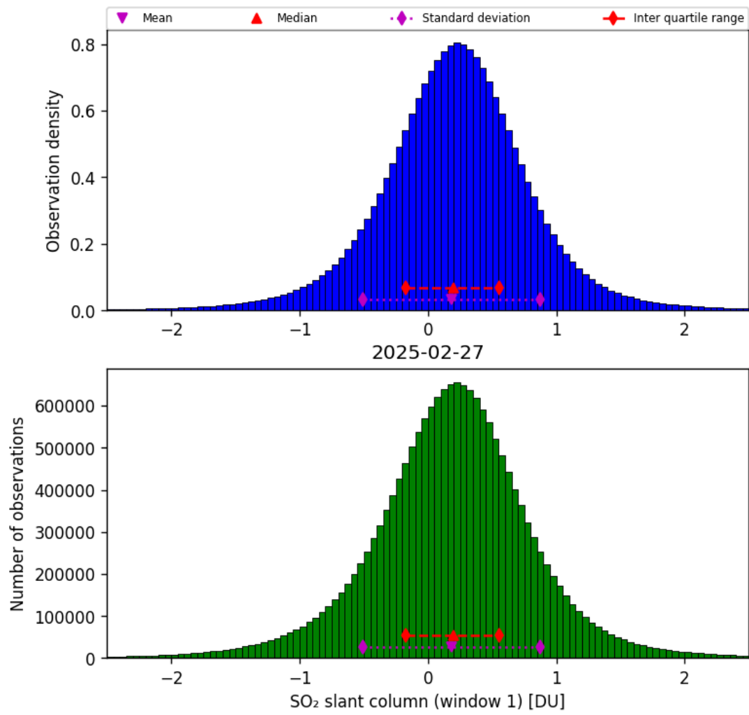
Figure 63: Histogram of “SO 2 slant column (window 1)” for 2025-02-27 to 2025-02-27
