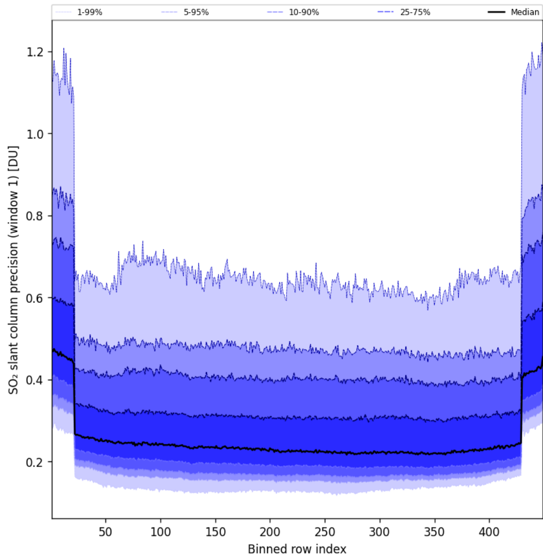
Figure 91: Along track statistics of “SO 2 slant column precision (window 1)” for 2025-02-27 to 2025-02-27
