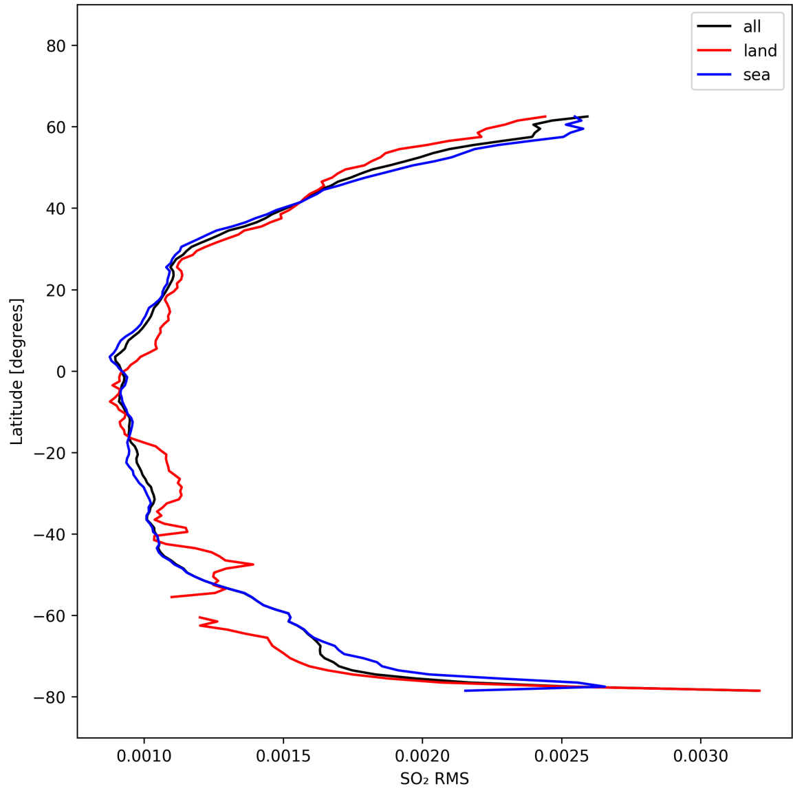
Figure 52: Zonal average of “SO 2 RMS” for 2025-02-27 to 2025-02-27.
