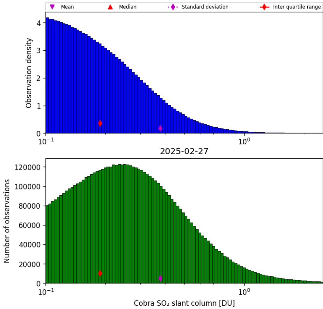
Figure 61: Histogram of “Cobra SO 2 slant column” for 2025-02-27 to 2025-02-27
