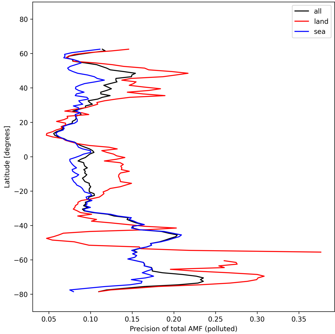
Figure 54: Zonal average of “Precision of total AMF (polluted)” for 2025-02-27 to 2025-02-27.
