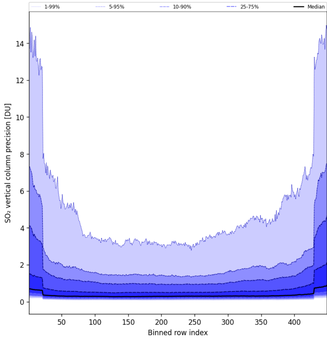
Figure 86: Along track statistics of “SO 2 vertical column precision” for 2025-02-27 to 2025-02-27
