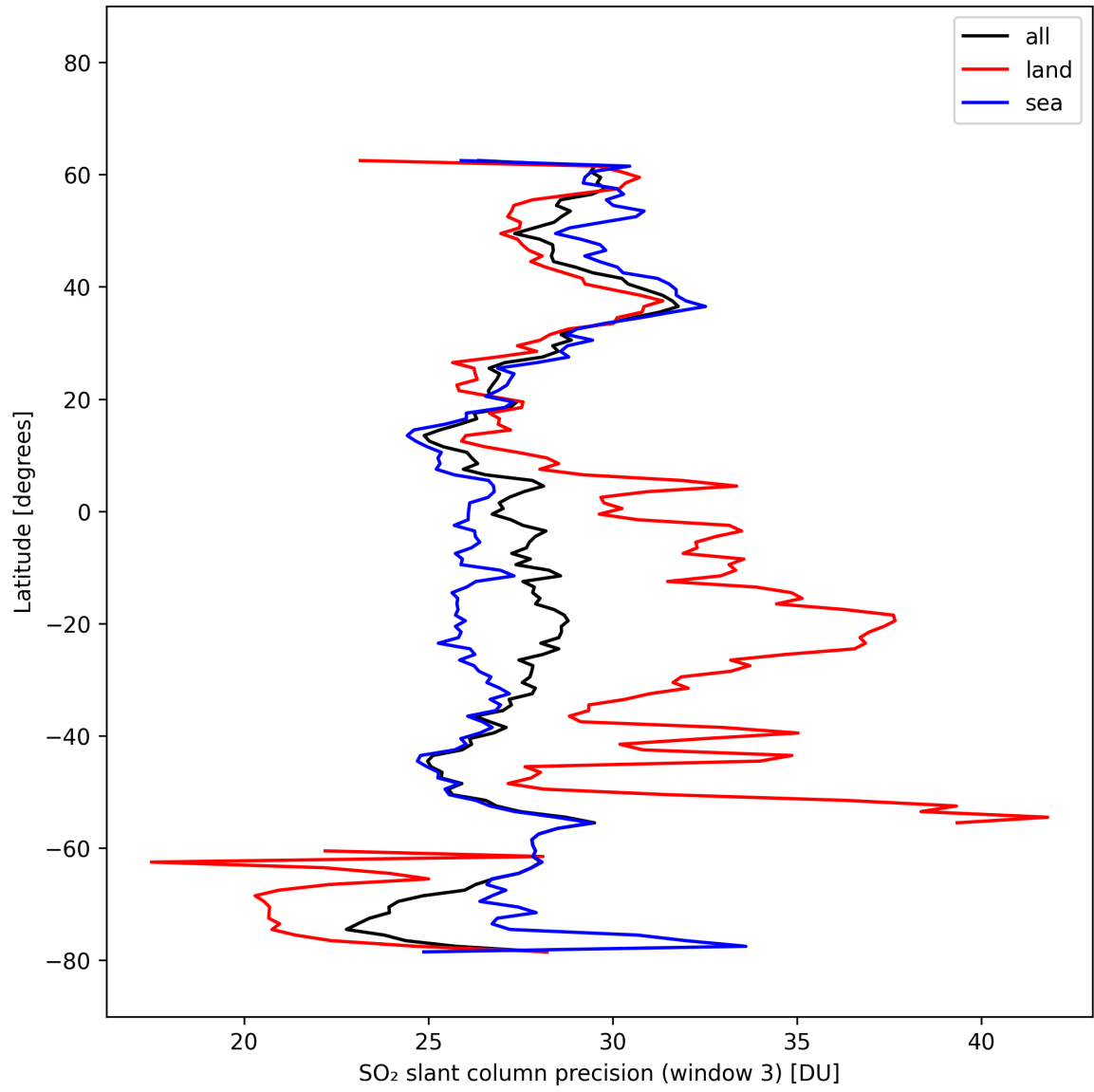
Figure 45: Zonal average of “SO 2 slant column precision (window 3)” for 2025-02-27 to 2025-02-27.
