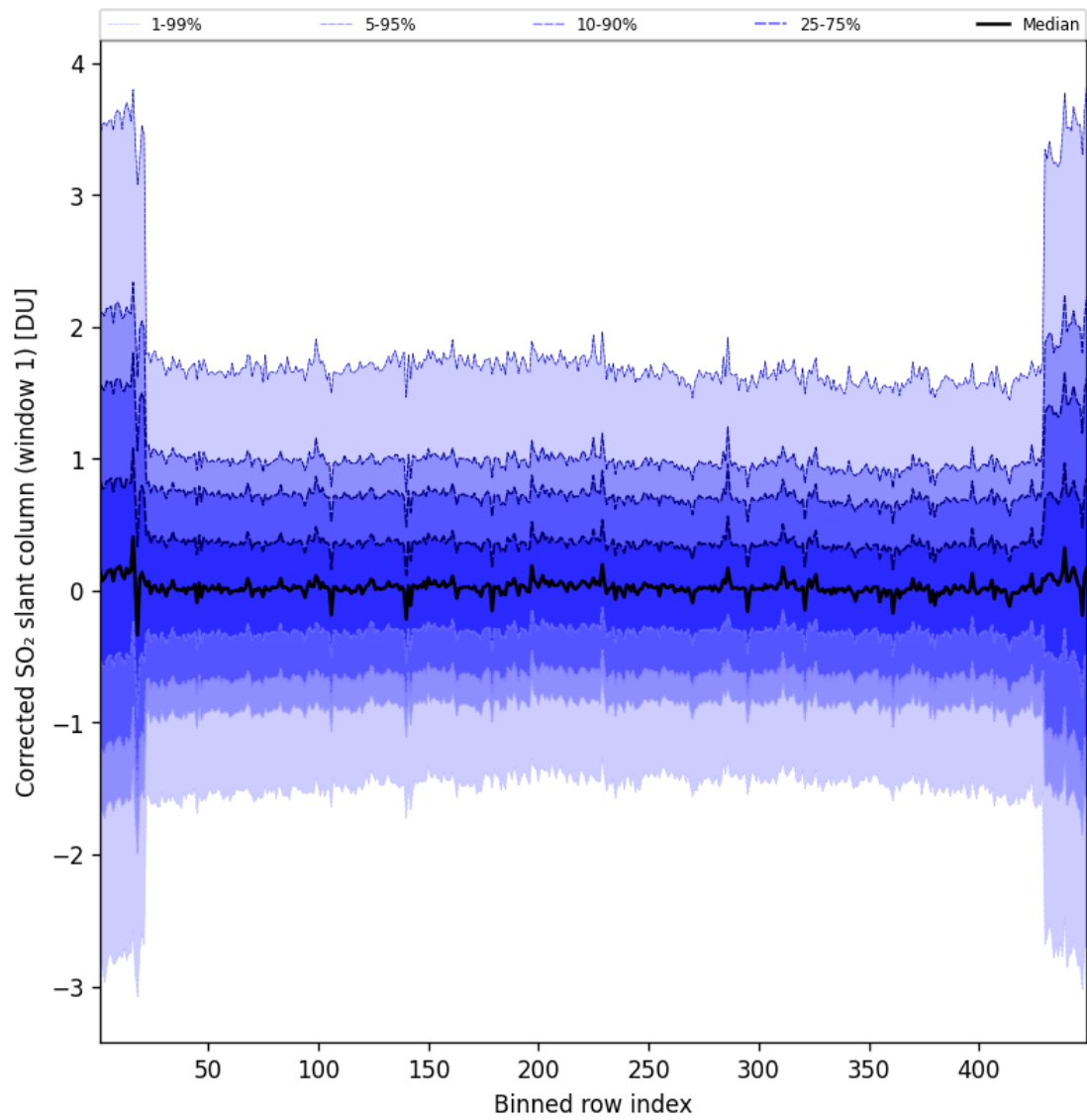
Figure 92: Along track statistics of “Corrected SO 2 slant column (window 1)” for 2025-02-27 to 2025-02-27
