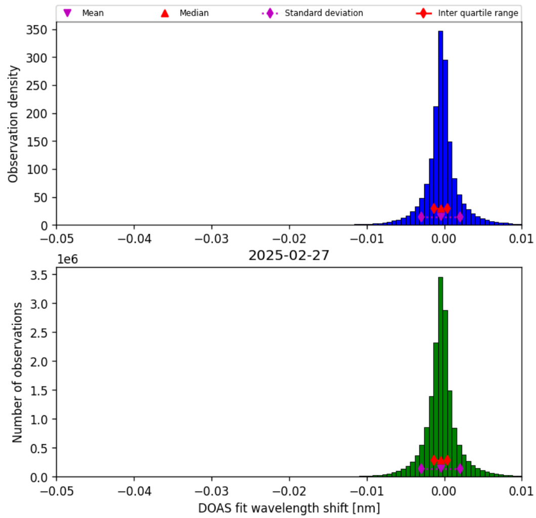
Figure 77: Histogram of “DOAS fit wavelength shift” for 2025-02-27 to 2025-02-27
