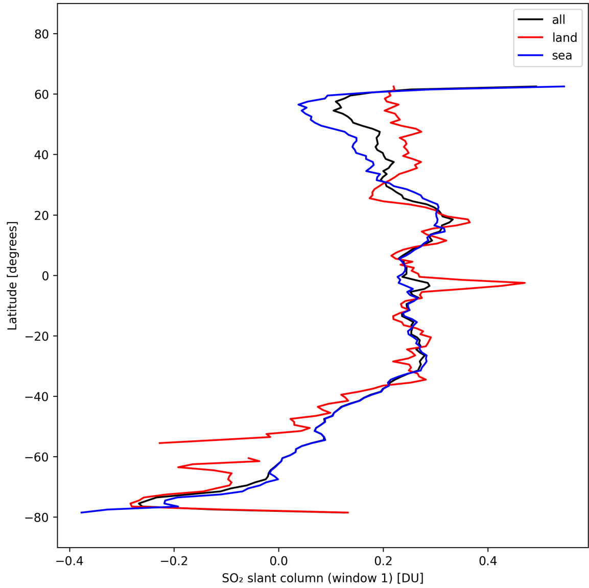
Figure 36: Zonal average of “SO 2 slant column (window 1)” for 2025-02-27 to 2025-02-27.
