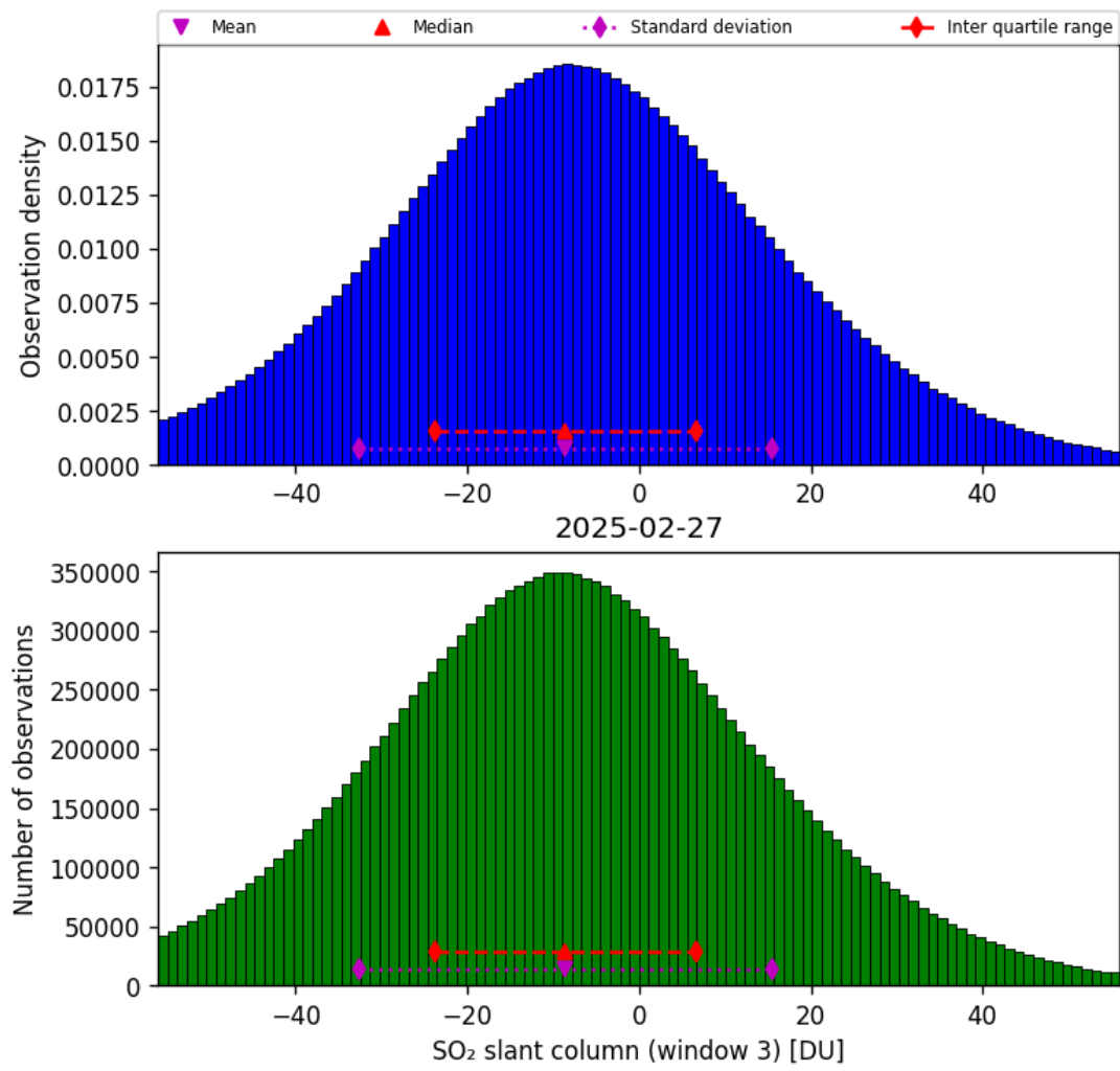
Figure 71: Histogram of “SO 2 slant column (window 3)” for 2025-02-27 to 2025-02-27
