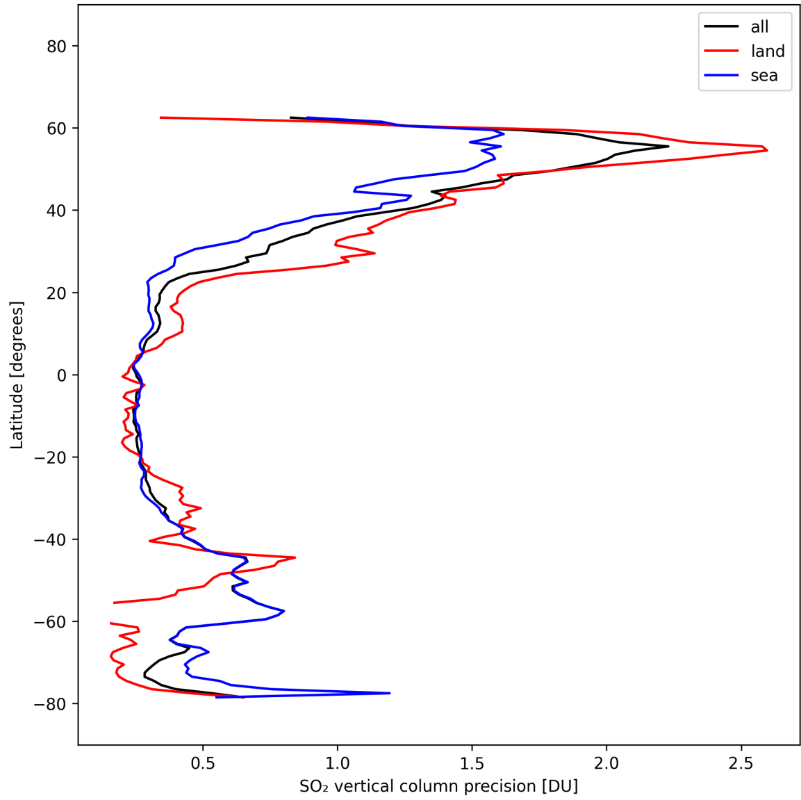
Figure 32: Zonal average of “SO 2 vertical column precision” for 2025-02-27 to 2025-02-27.
