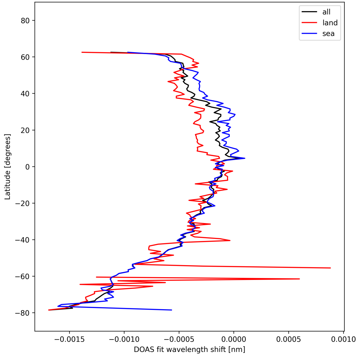
Figure 50: Zonal average of "DOAS fit wavelength shift" for 2025-02-27 to 2025-02-27.
