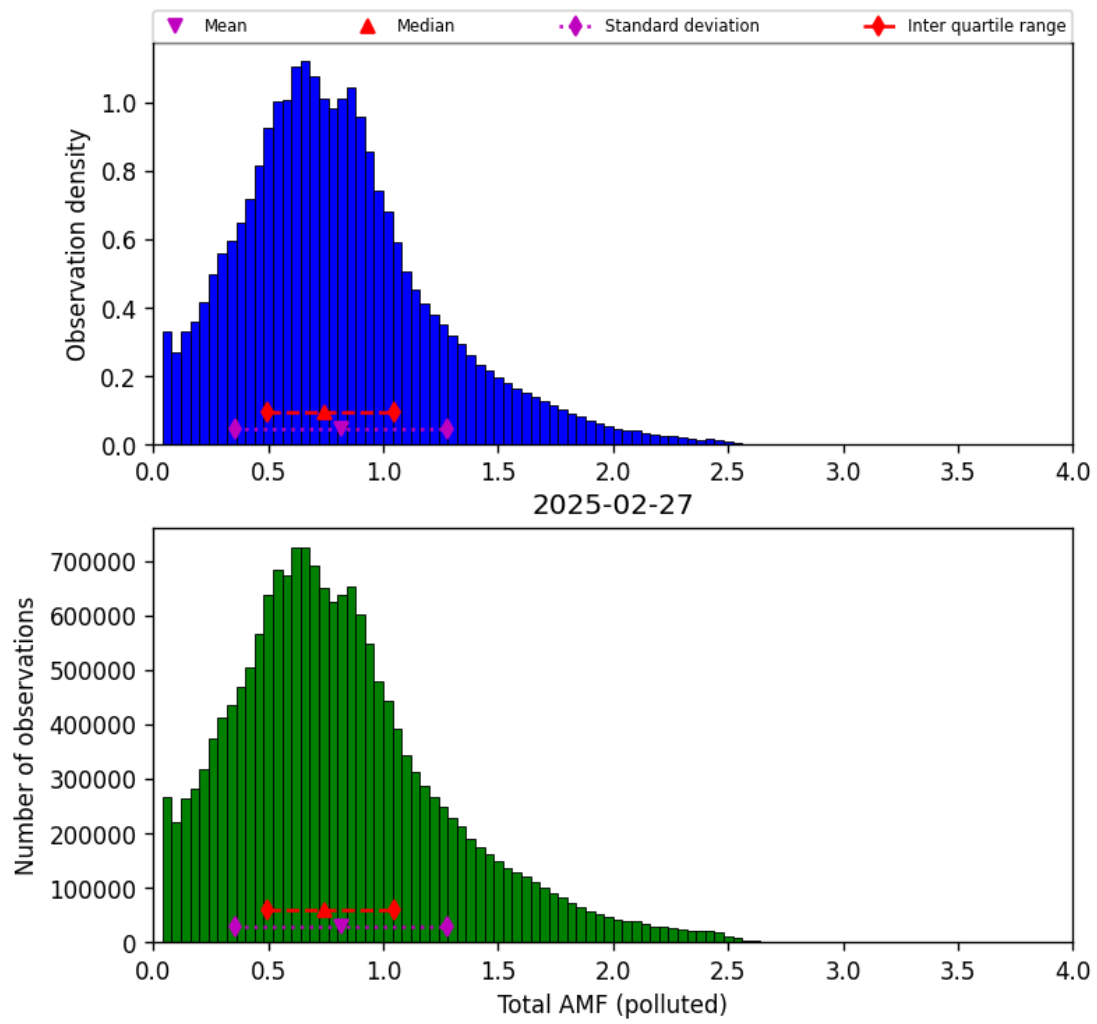
Figure 80: Histogram of “Total AMF (polluted)” for 2025-02-27 to 2025-02-27
