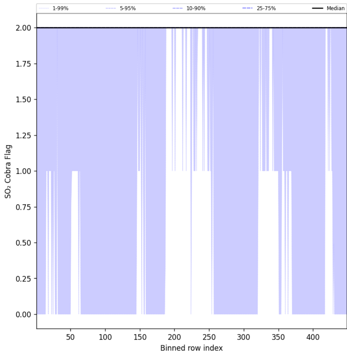
Figure 102: Along track statistics of “SO 2 Cobra Flag” for 2025-02-27 to 2025-02-27
