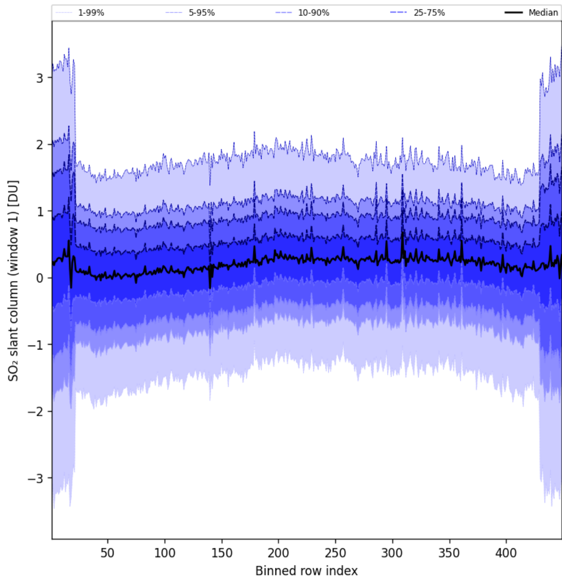
Figure 90: Along track statistics of “SO 2 slant column (window 1)” for 2025-02-27 to 2025-02-27
