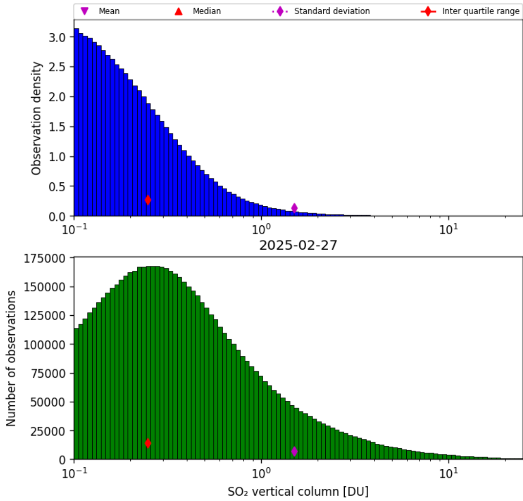
Figure 58: Histogram of “SO 2 vertical column” for 2025-02-27 to 2025-02-27
