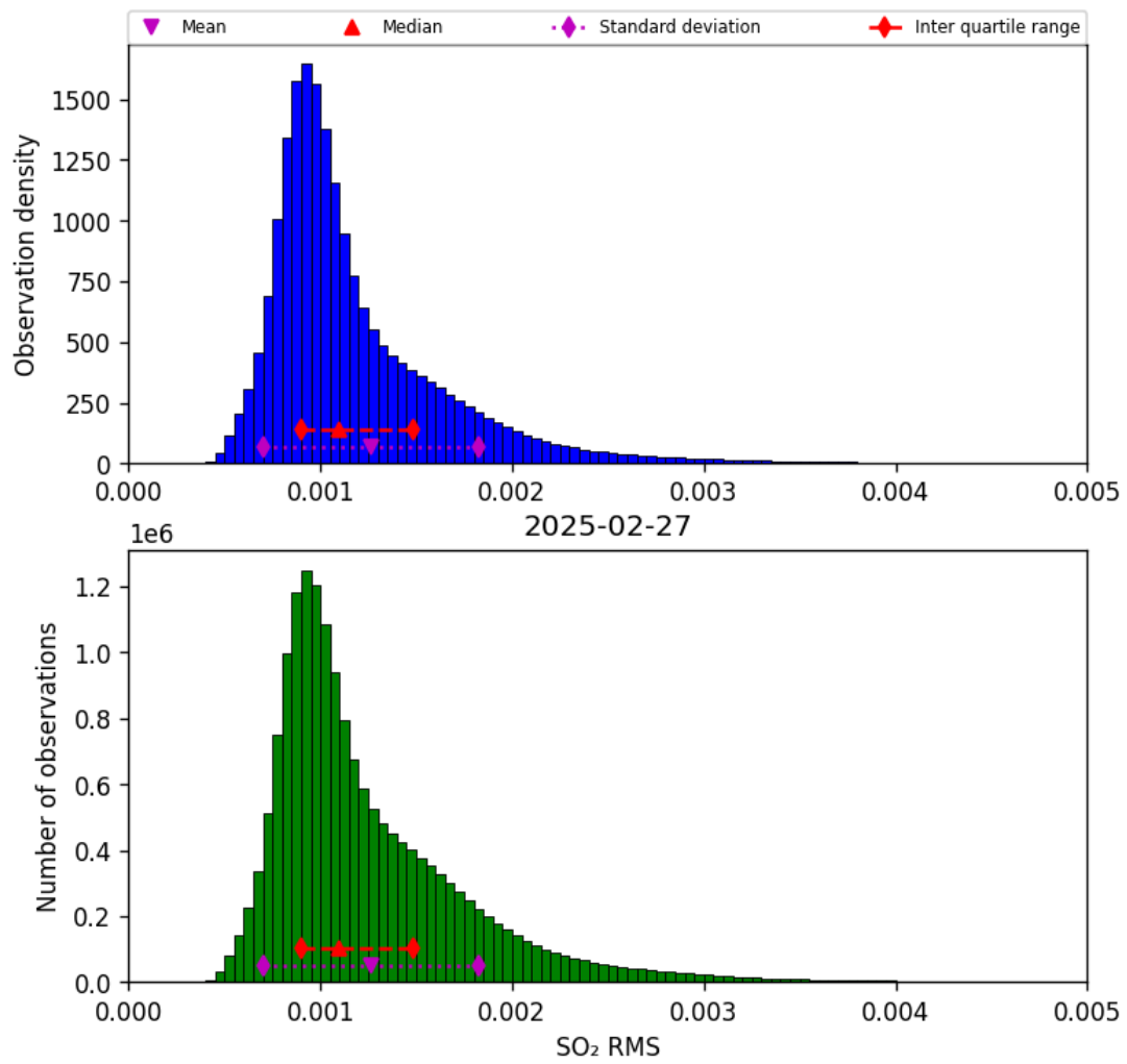
Figure 79: Histogram of “SO 2 RMS” for 2025-02-27 to 2025-02-27
