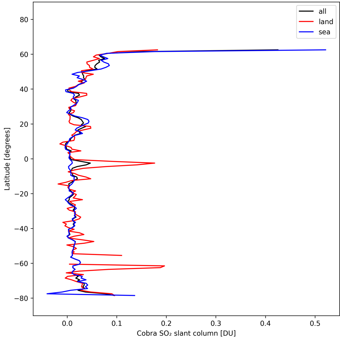
Figure 34: Zonal average of “Cobra SO 2 slant column” for 2025-02-27 to 2025-02-27.
