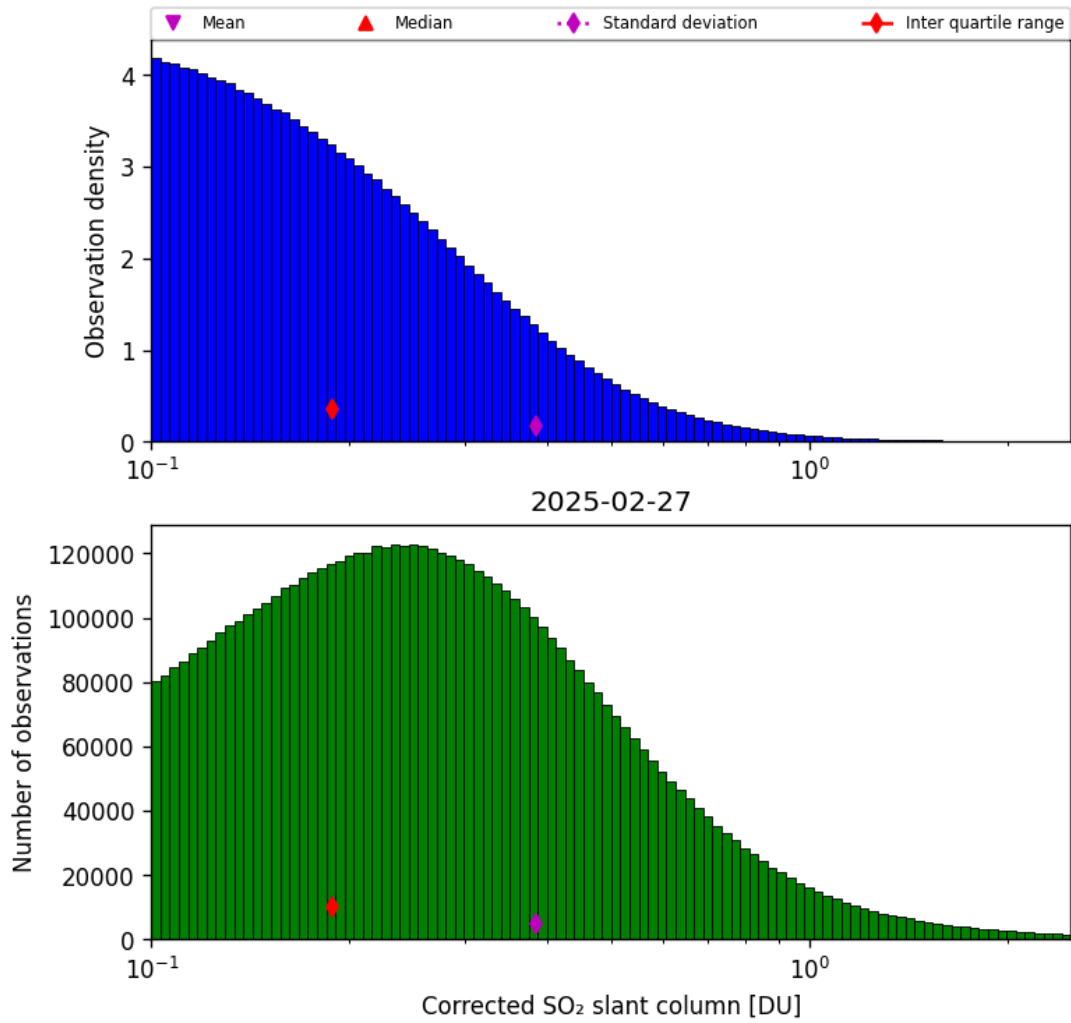
Figure 60: Histogram of “Corrected SO 2 slant column” for 2025-02-27 to 2025-02-27
