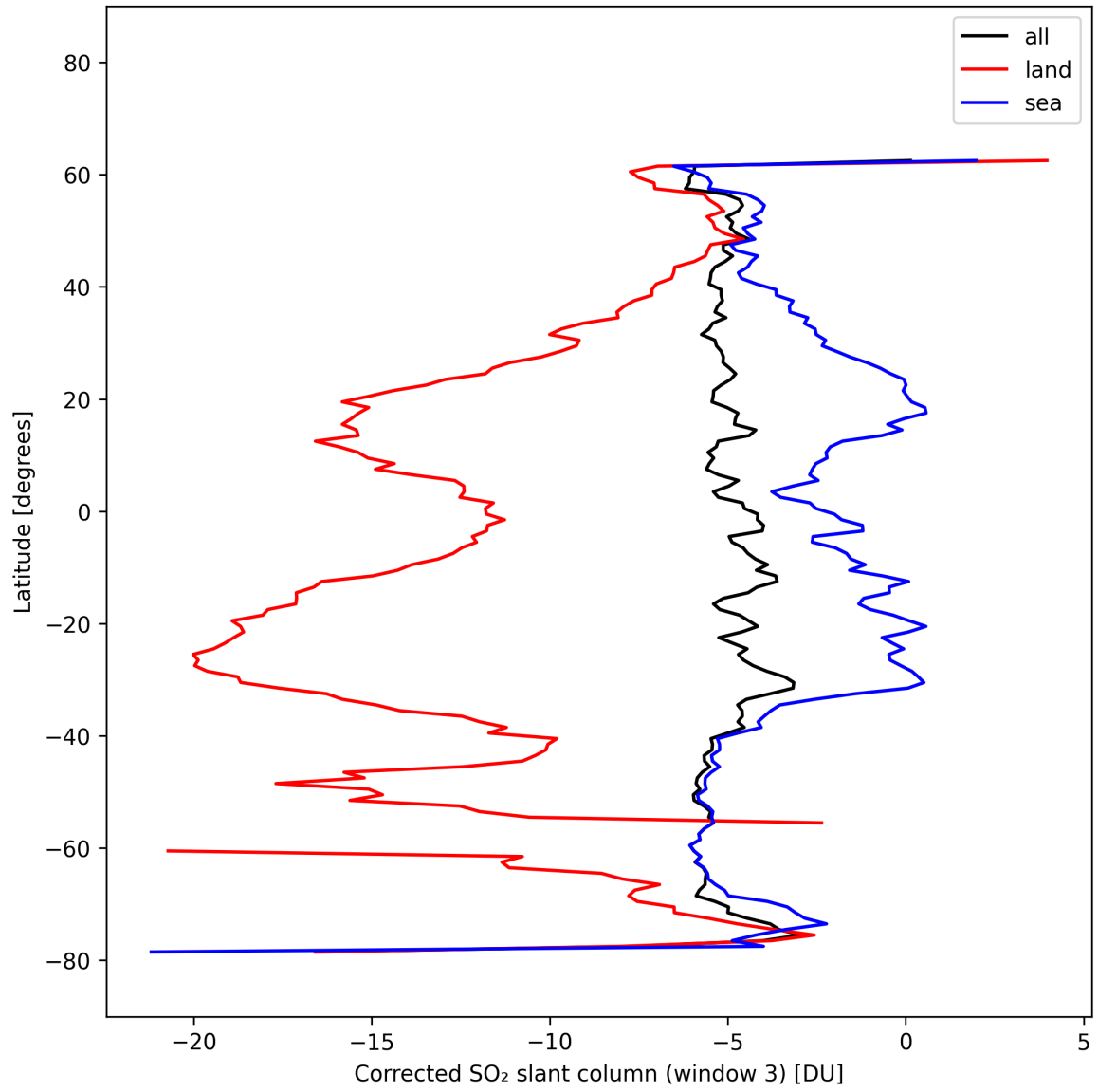
Figure 46: Zonal average of “Corrected SO 2 slant column (window 3)” for 2025-02-27 to 2025-02-27.
