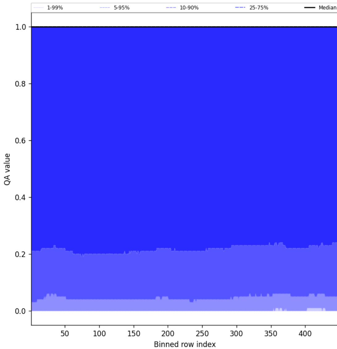
Figure 84: Along track statistics of “QA value” for 2025-02-27 to 2025-02-27
