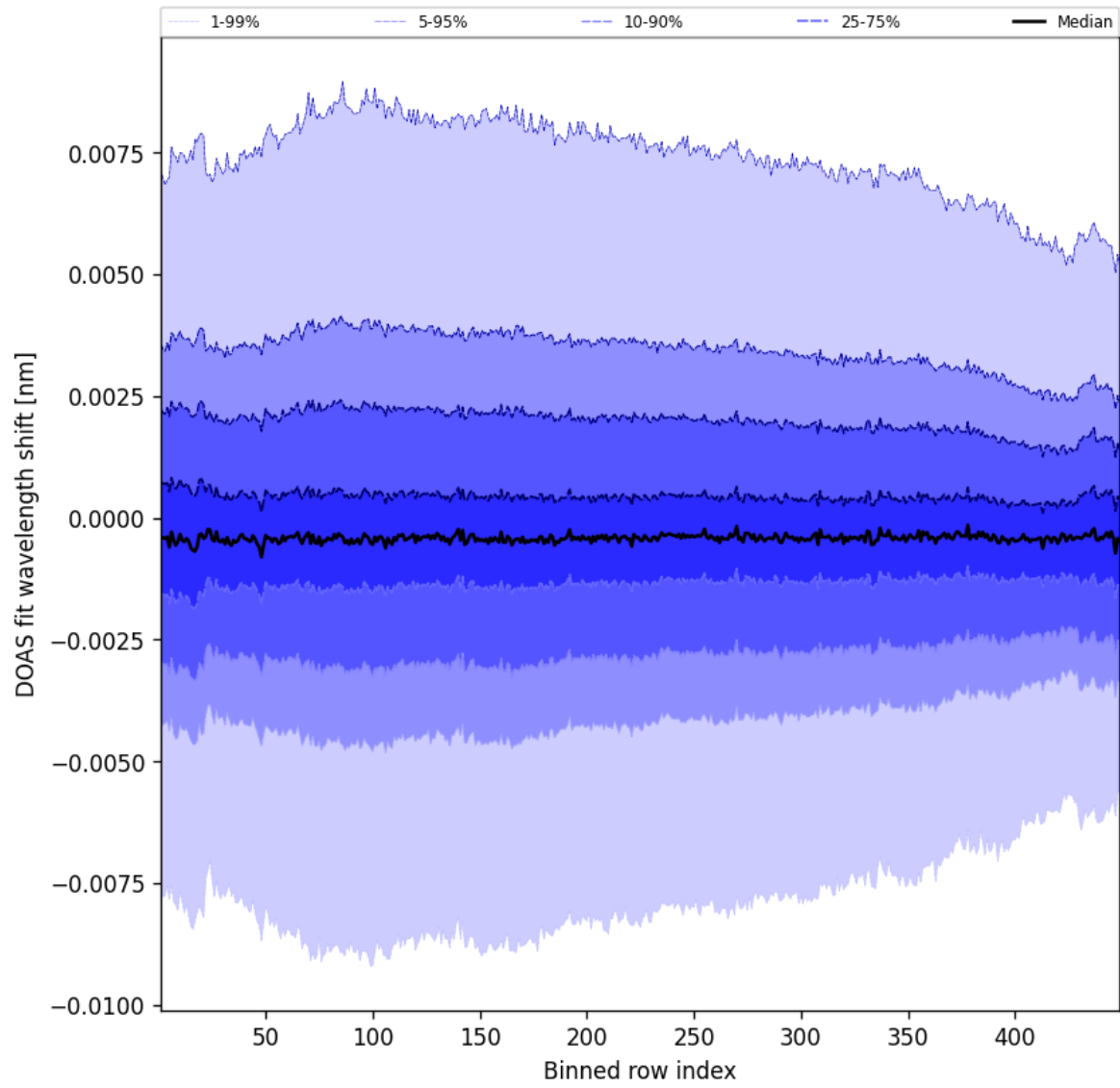
Figure 104: Along track statistics of “DOAS fit wavelength shift” for 2025-02-27 to 2025-02-27
