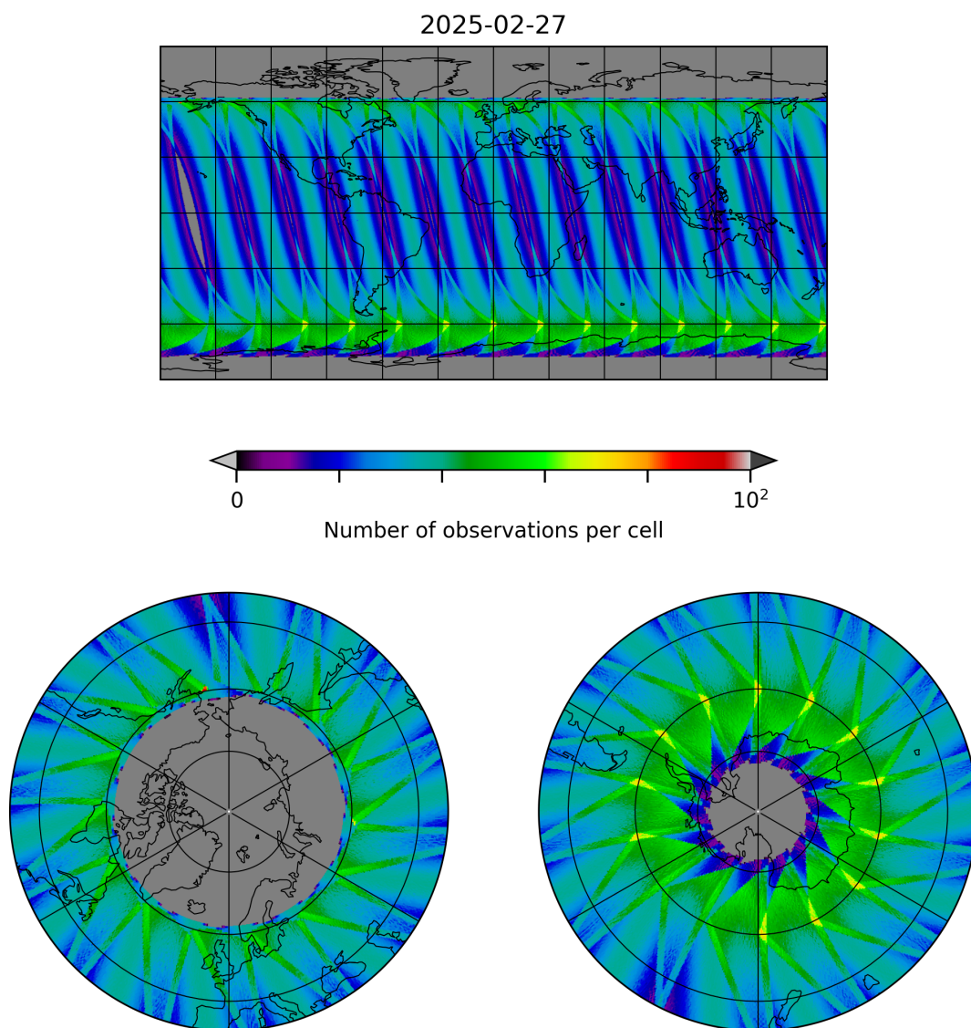
Figure 29: Map of the number of observations for 2025-02-27 to 2025-02-27
