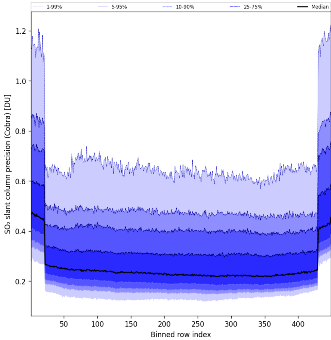
Figure 89: Along track statistics of “SO 2 slant column precision (Cobra)” for 2025-02-27 to 2025-02-27
