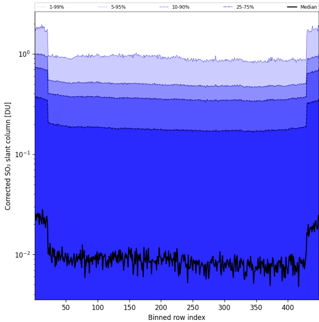
Figure 87: Along track statistics of “Corrected SO 2 slant column” for 2025-02-27 to 2025-02-27
