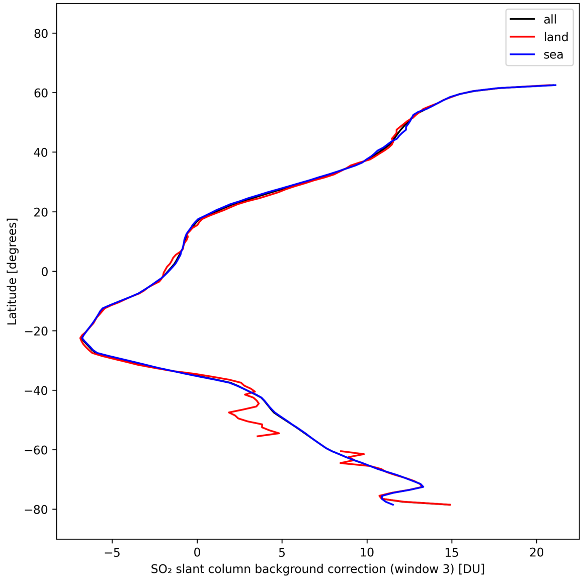
Figure 47: Zonal average of “SO 2 slant column background correction (window 3)” for 2025-02-27 to 2025-02-27.
