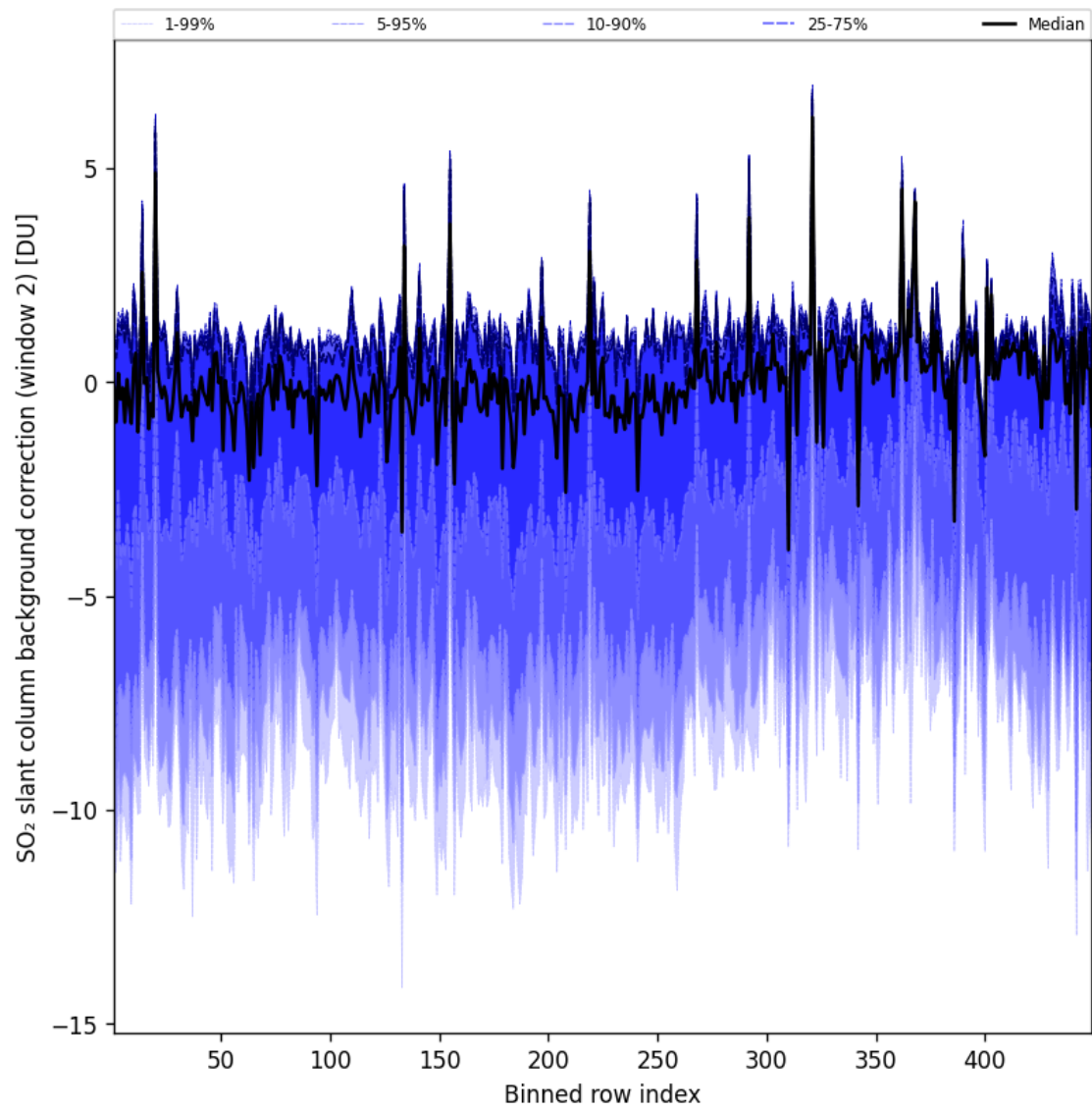
Figure 97: Along track statistics of “SO 2 slant column background correction (window 2)” for 2025-02-27 to 2025-02-27
