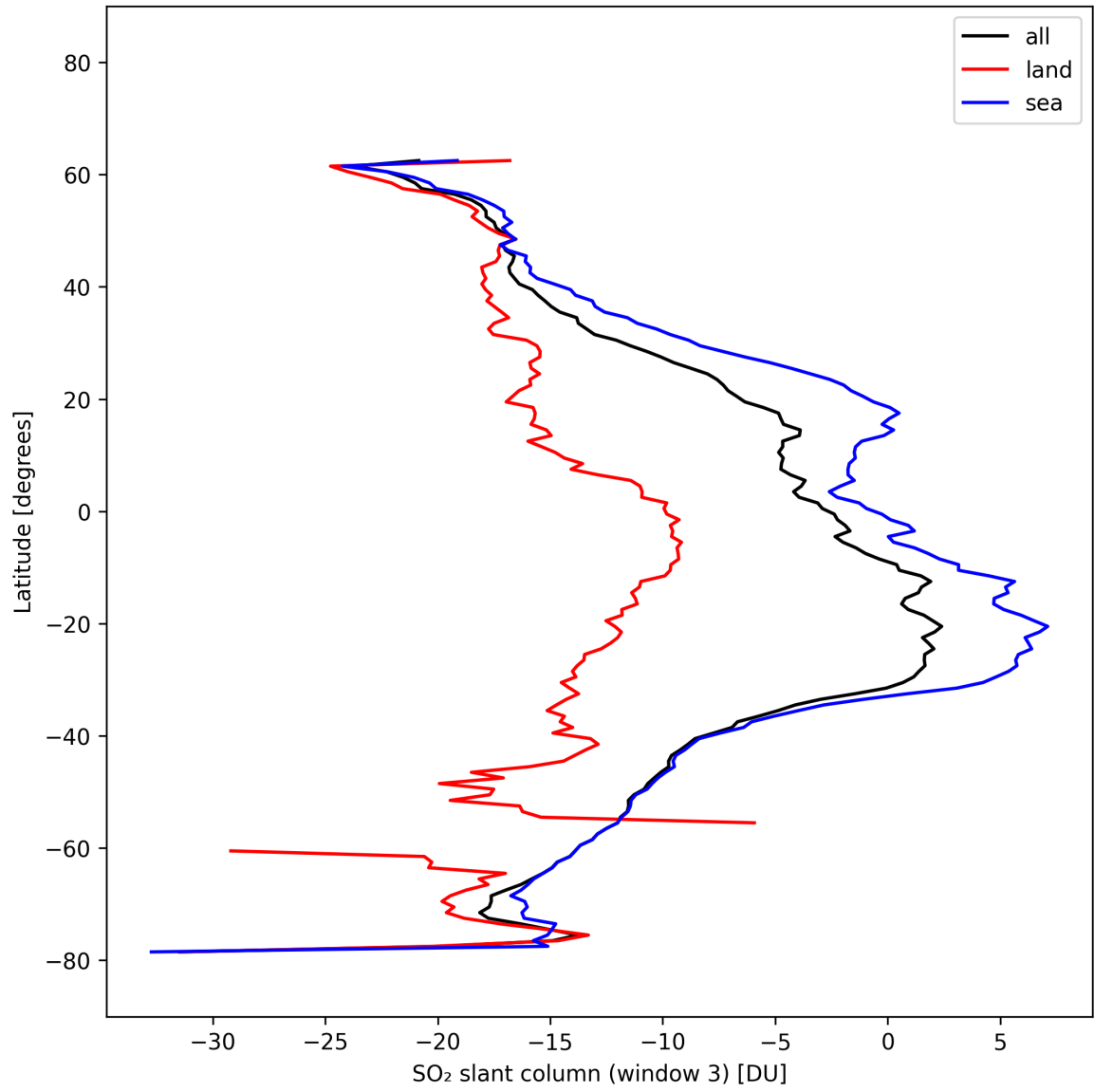
Figure 44: Zonal average of “SO 2 slant column (window 3)” for 2025-02-27 to 2025-02-27.
