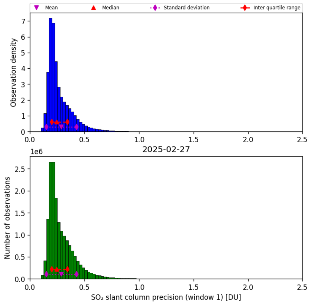
Figure 64: Histogram of “SO 2 slant column precision (window 1)” for 2025-02-27 to 2025-02-27
