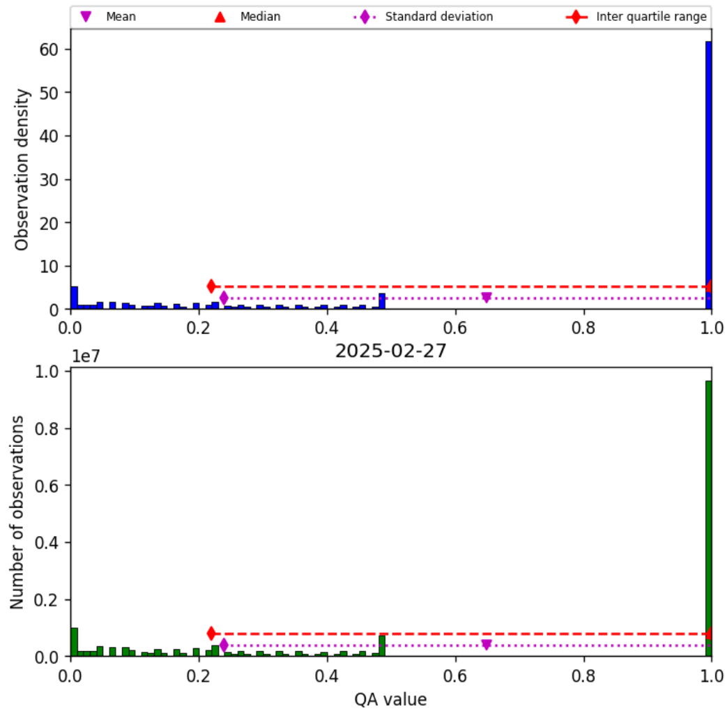
Figure 57: Histogram of “QA value” for 2025-02-27 to 2025-02-27
