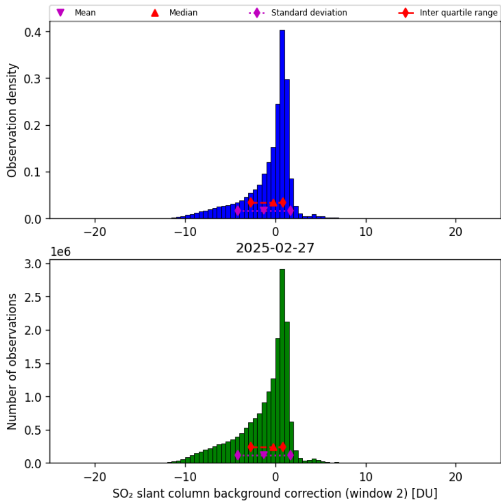
Figure 70: Histogram of “SO 2 slant column background correction (window 2)” for 2025-02-27 to 2025-02-27
