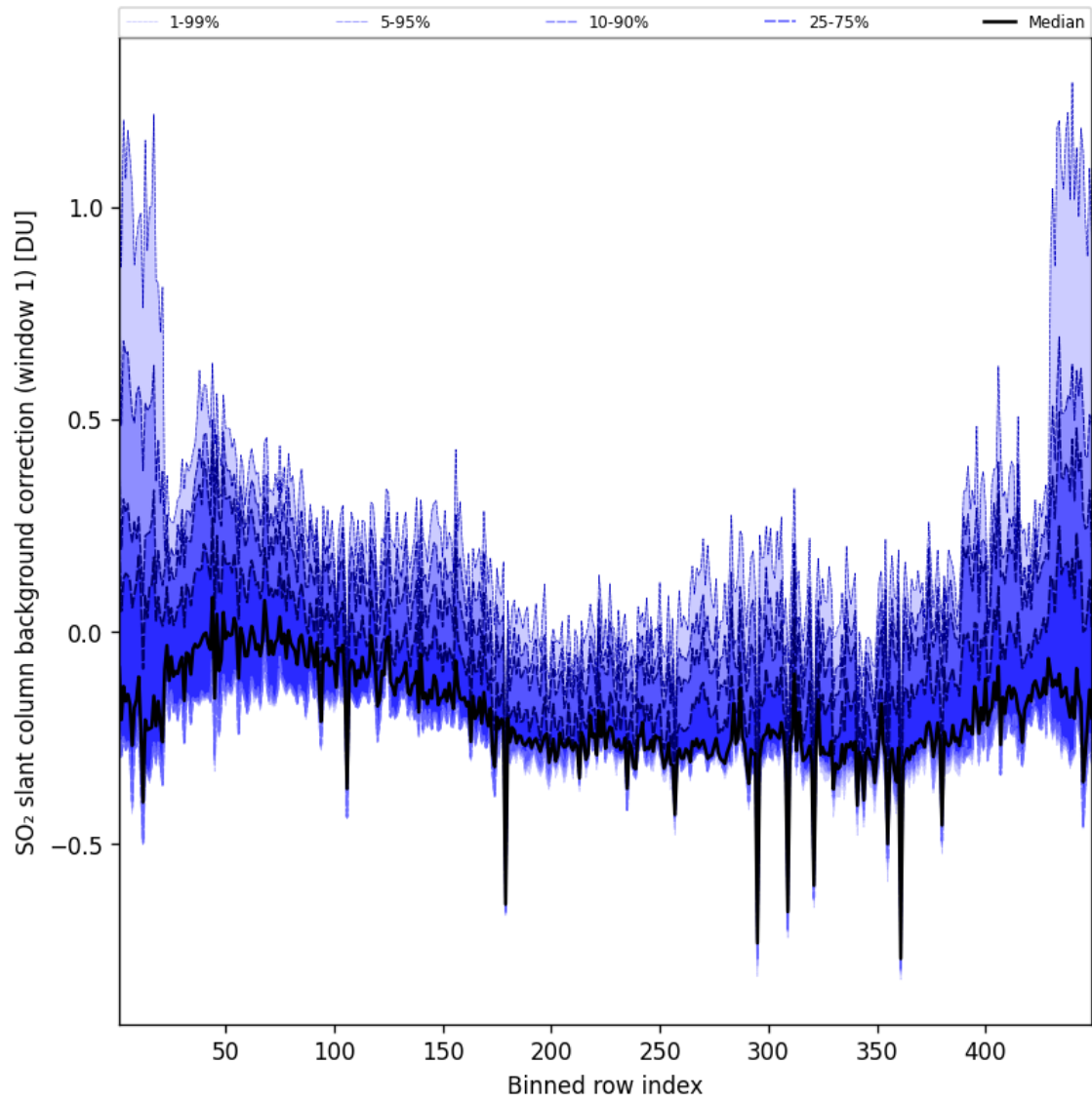
Figure 93: Along track statistics of “SO 2 slant column background correction (window 1)” for 2025-02-27 to 2025-02-27
