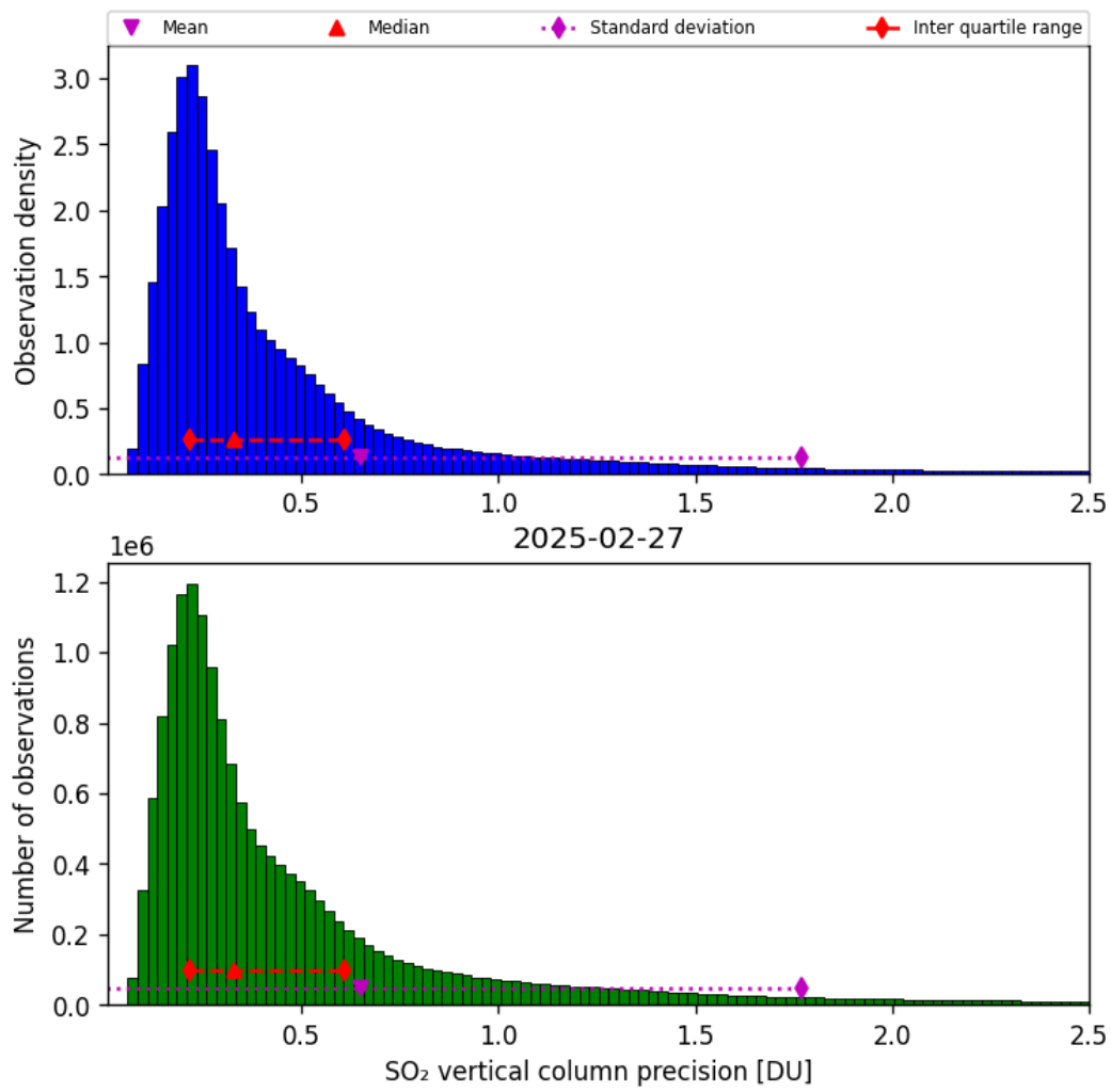
Figure 59: Histogram of "SO 2 vertical column precision" for 2025-02-27 to 2025-02-27
