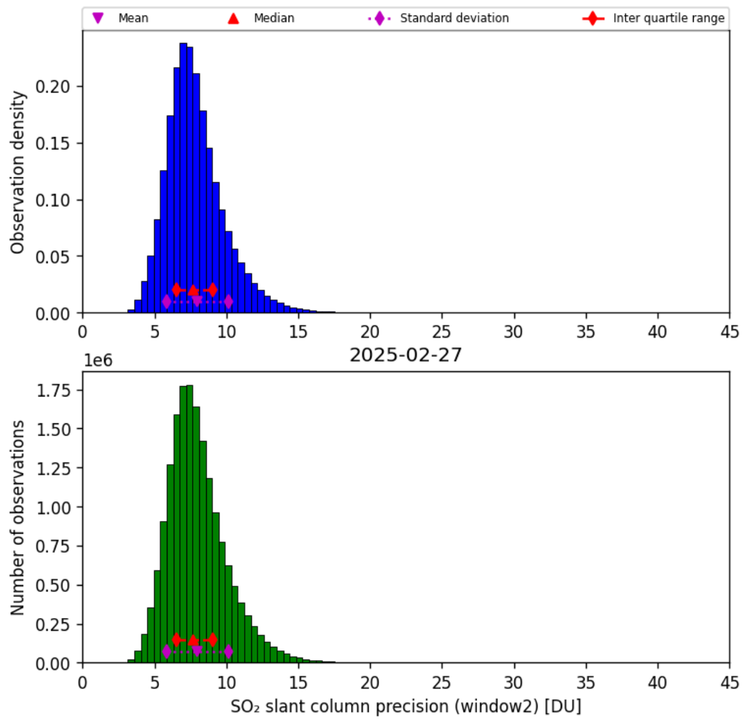
Figure 68: Histogram of “SO 2 slant column precision (window2)” for 2025-02-27 to 2025-02-27
