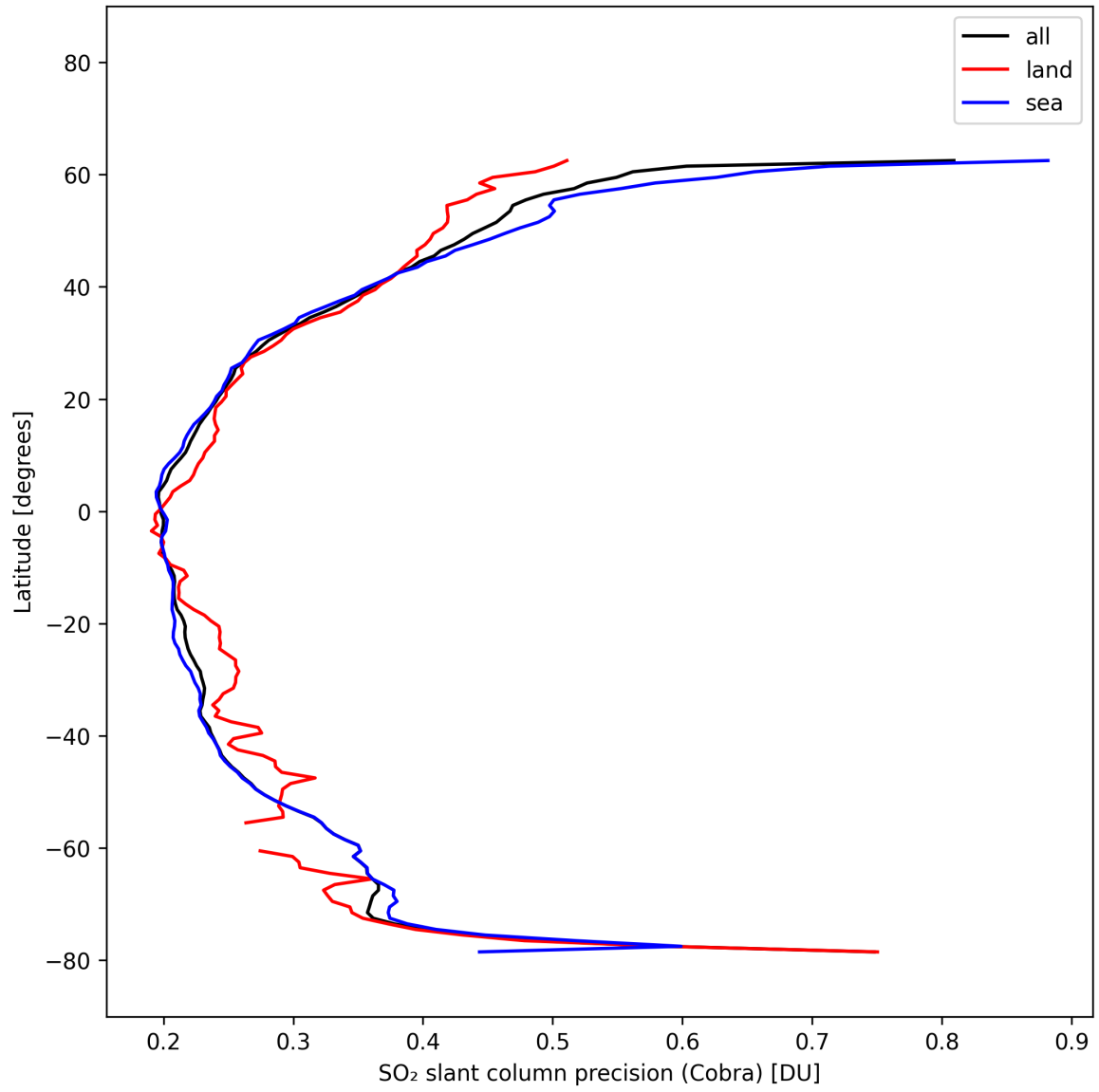
Figure 35: Zonal average of “SO 2 slant column precision (Cobra)” for 2025-02-27 to 2025-02-27.
