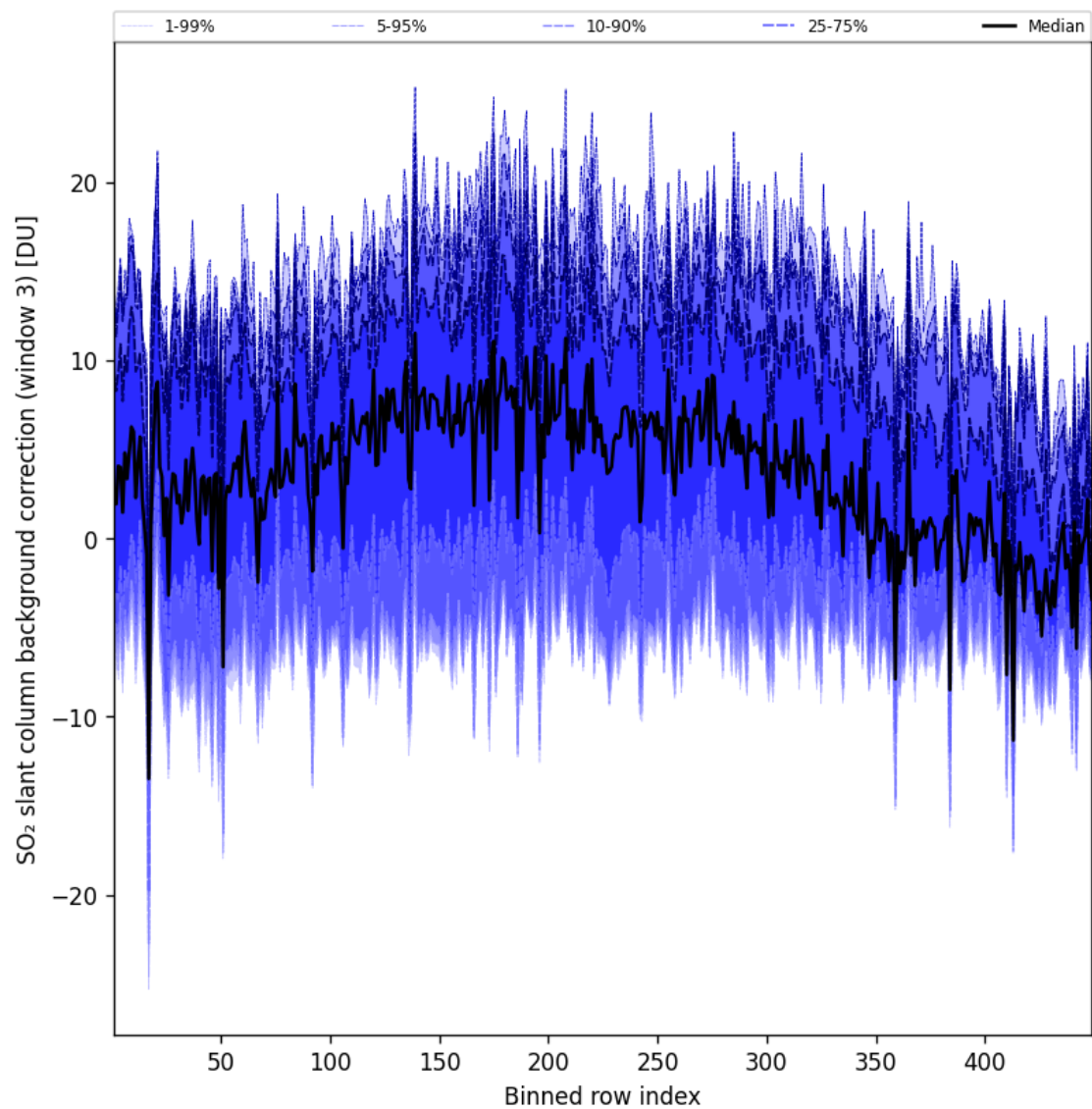
Figure 101: Along track statistics of “SO 2 slant column background correction (window 3)” for 2025-02-27 to 2025-02-27
