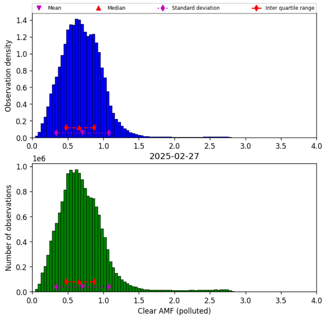
Figure 82: Histogram of “Clear AMF (polluted)” for 2025-02-27 to 2025-02-27
