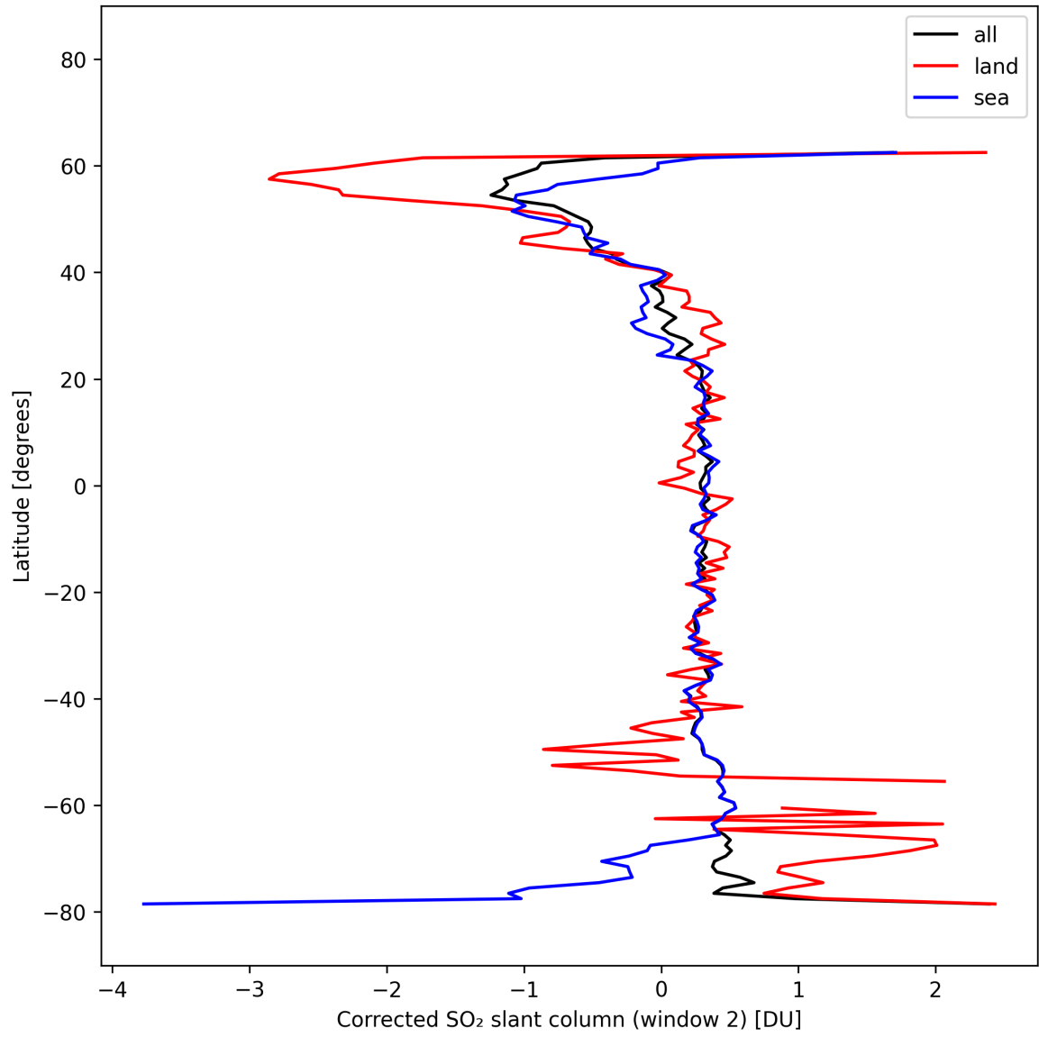
Figure 42: Zonal average of “Corrected SO 2 slant column (window 2)” for 2025-02-27 to 2025-02-27.
