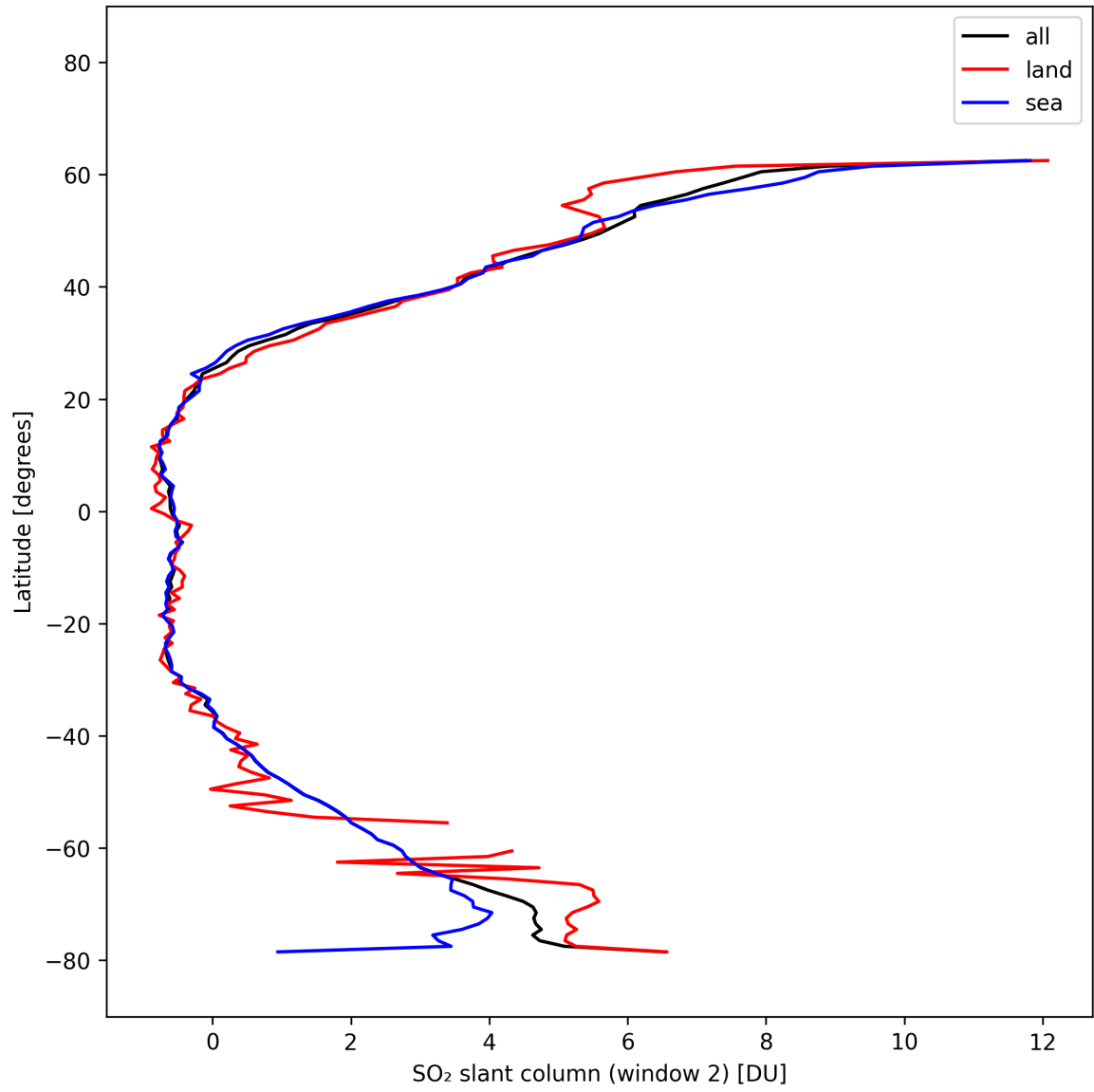
Figure 40: Zonal average of “SO 2 slant column (window 2)” for 2025-02-27 to 2025-02-27.
