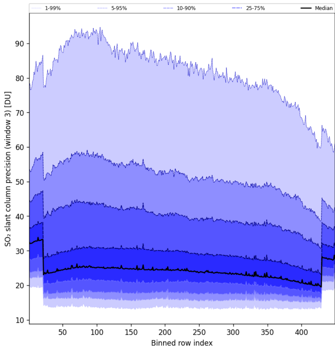
Figure 99: Along track statistics of “SO 2 slant column precision (window 3)” for 2025-02-27 to 2025-02-27
