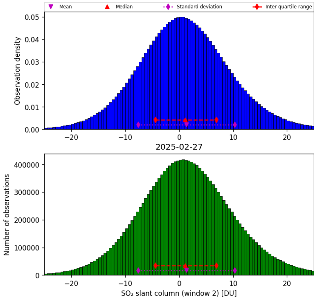
Figure 67: Histogram of “SO 2 slant column (window 2)” for 2025-02-27 to 2025-02-27
