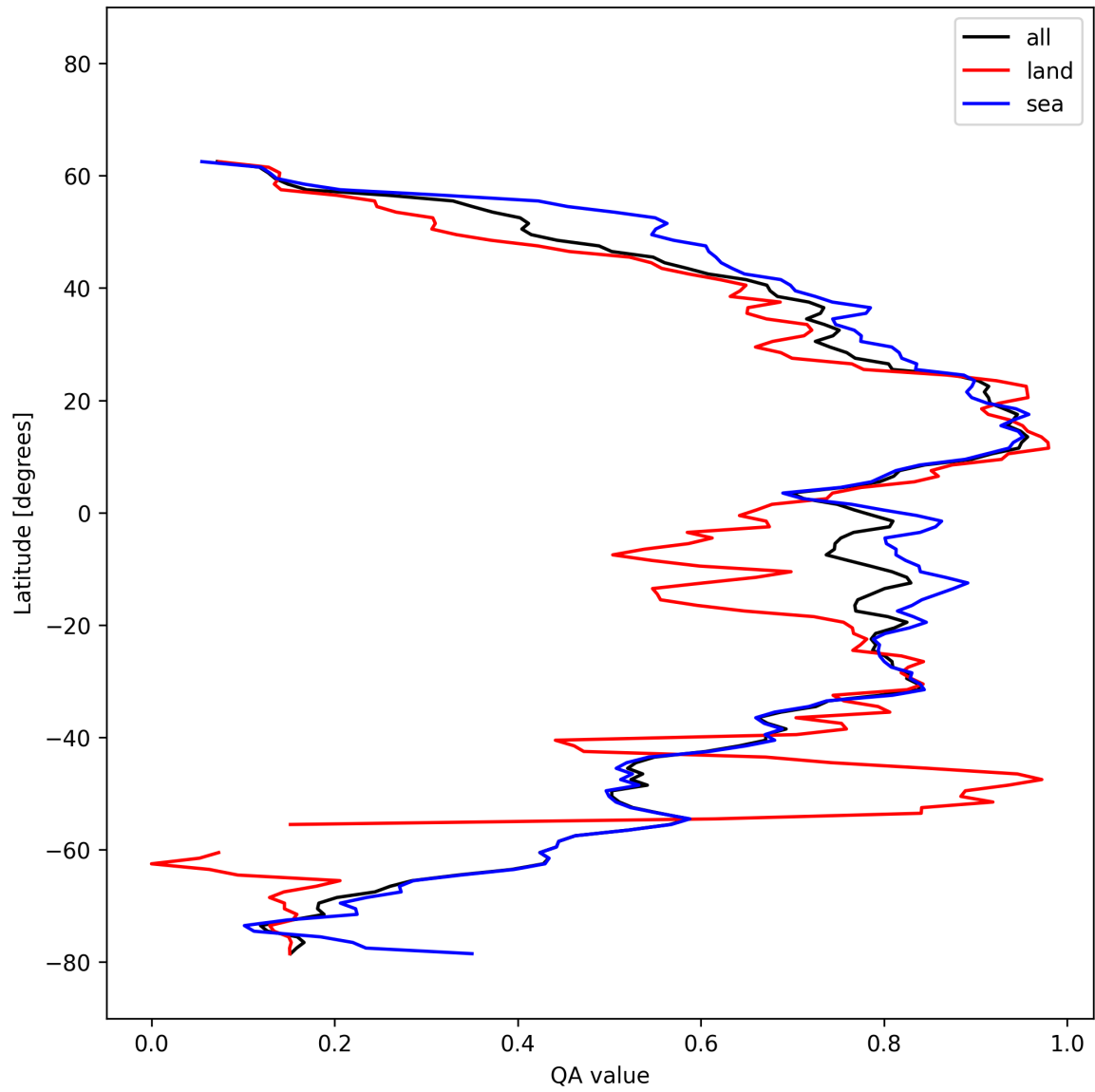
Figure 30: Zonal average of “QA value” for 2025-02-27 to 2025-02-27.
