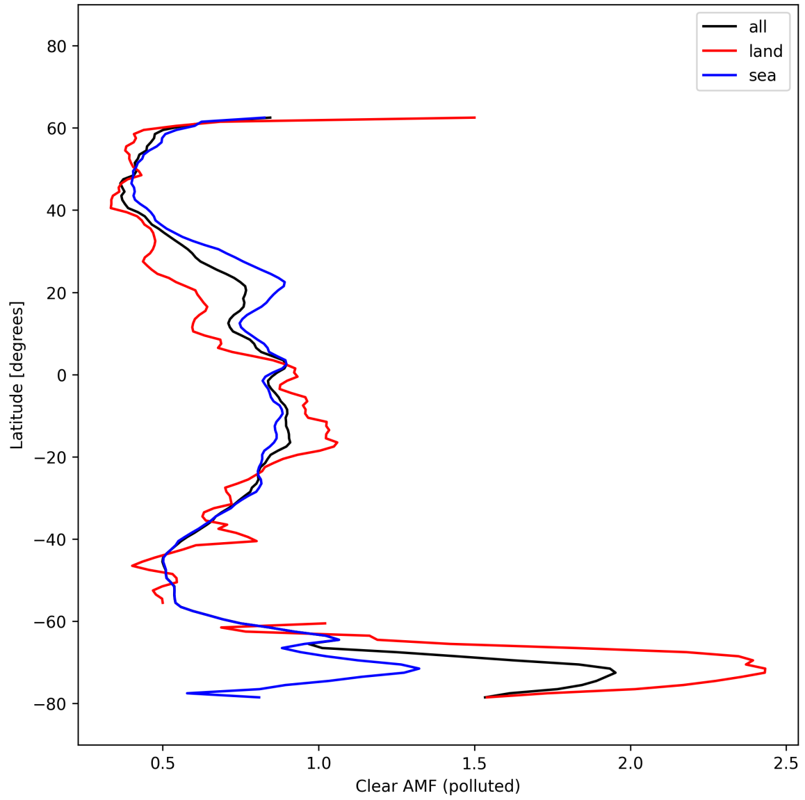
Figure 55: Zonal average of “Clear AMF (polluted)” for 2025-02-27 to 2025-02-27.
