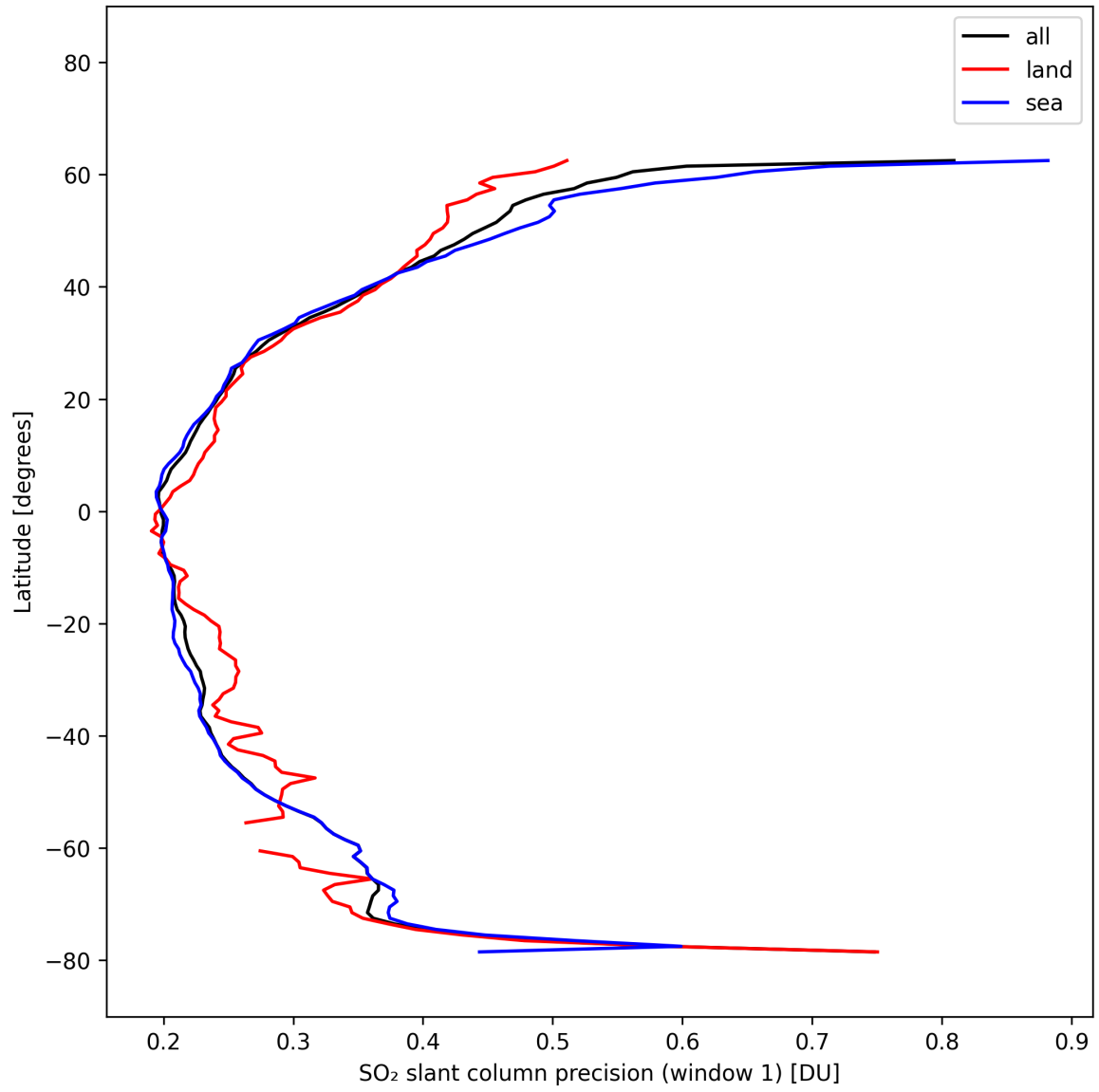
Figure 37: Zonal average of “SO 2 slant column precision (window 1)” for 2025-02-27 to 2025-02-27.
