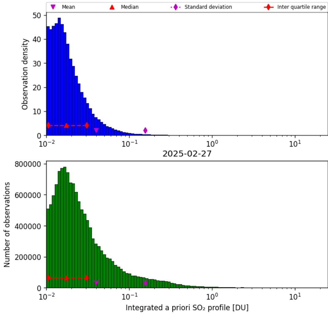
Figure 76: Histogram of “Integrated a priori SO 2 profile” for 2025-02-27 to 2025-02-27
