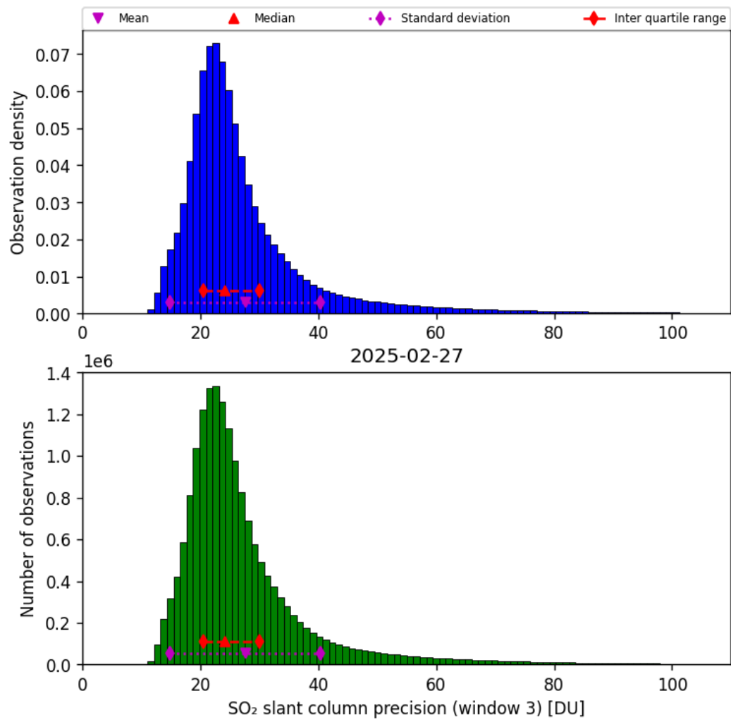
Figure 72: Histogram of “SO 2 slant column precision (window 3)” for 2025-02-27 to 2025-02-27
