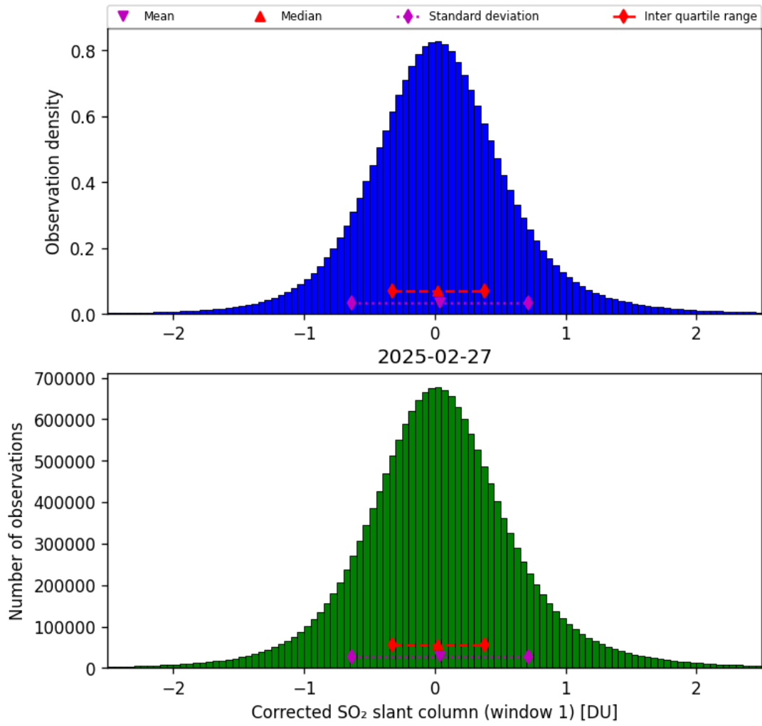
Figure 65: Histogram of “Corrected SO 2 slant column (window 1)” for 2025-02-27 to 2025-02-27
