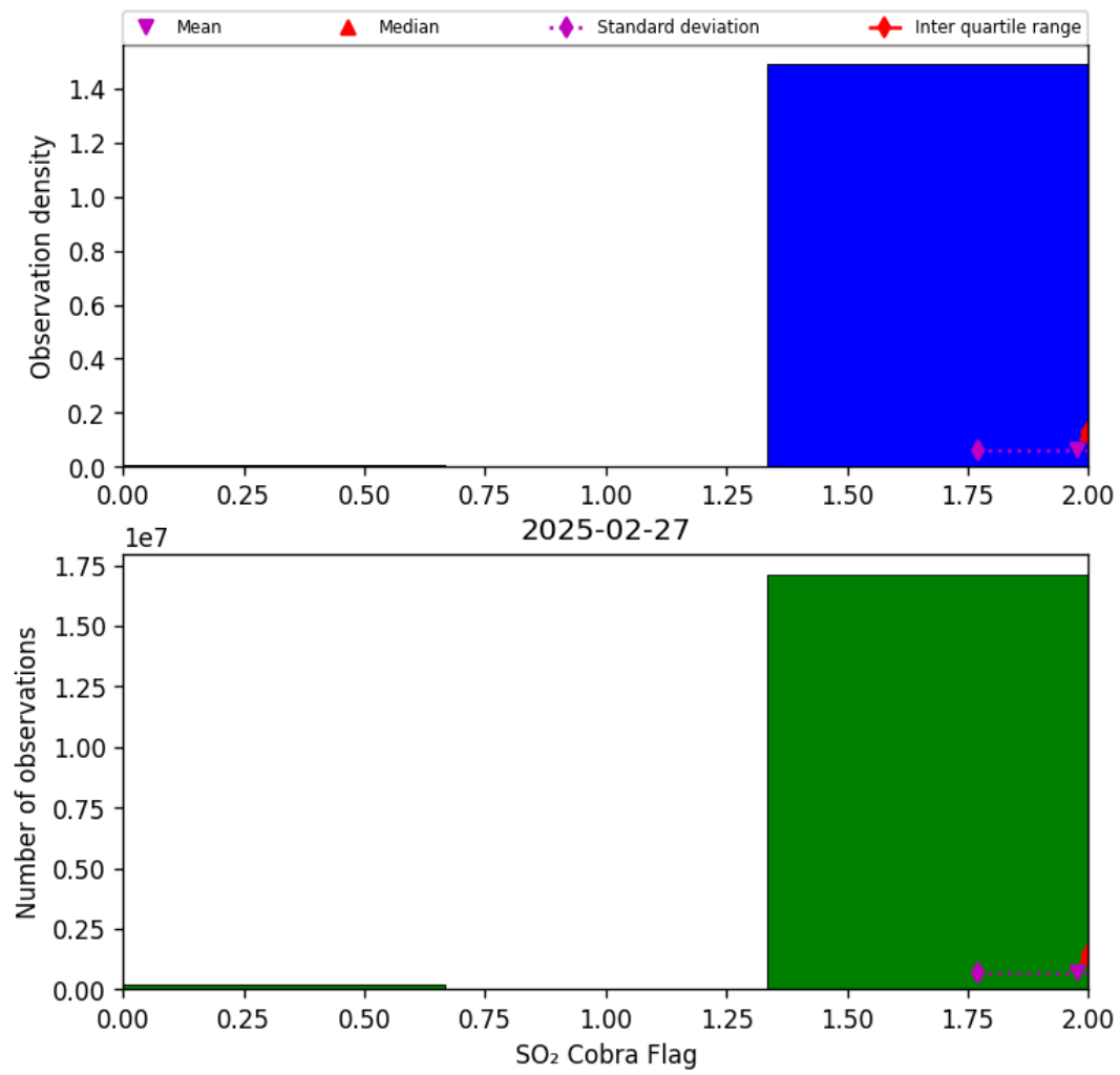
Figure 75: Histogram of “SO 2 Cobra Flag” for 2025-02-27 to 2025-02-27
