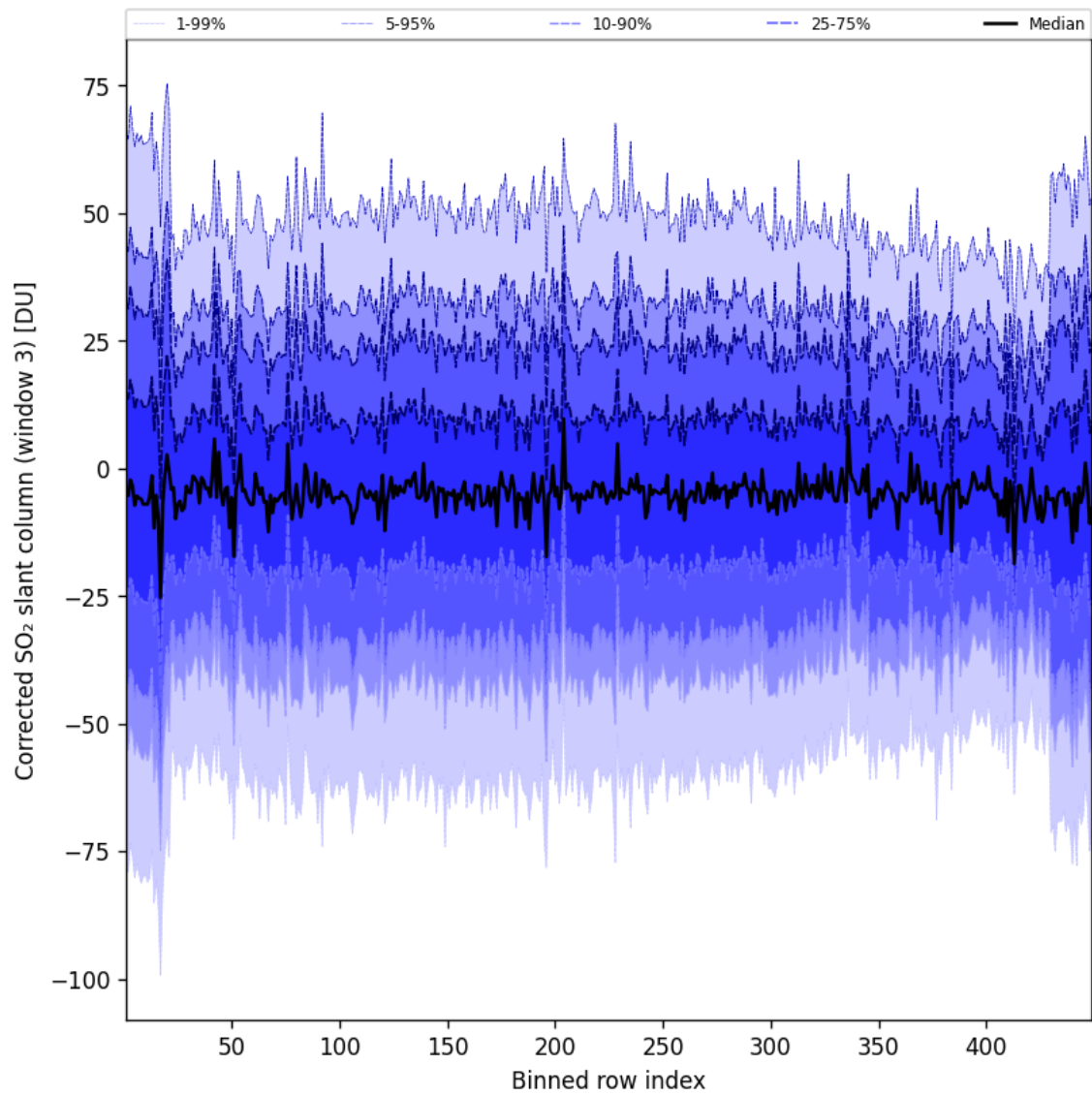
Figure 100: Along track statistics of “Corrected SO 2 slant column (window 3)” for 2025-02-27 to 2025-02-27
