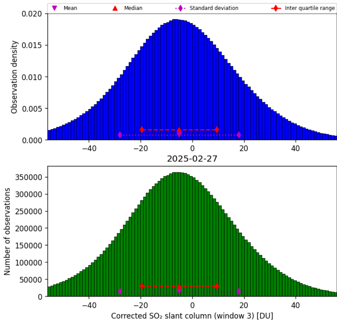
Figure 73: Histogram of “Corrected SO 2 slant column (window 3)” for 2025-02-27 to 2025-02-27
