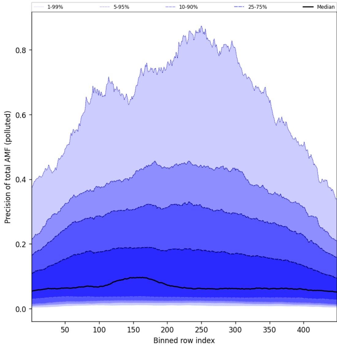
Figure 108: Along track statistics of “Precision of total AMF (polluted)” for 2025-02-27 to 2025-02-27
