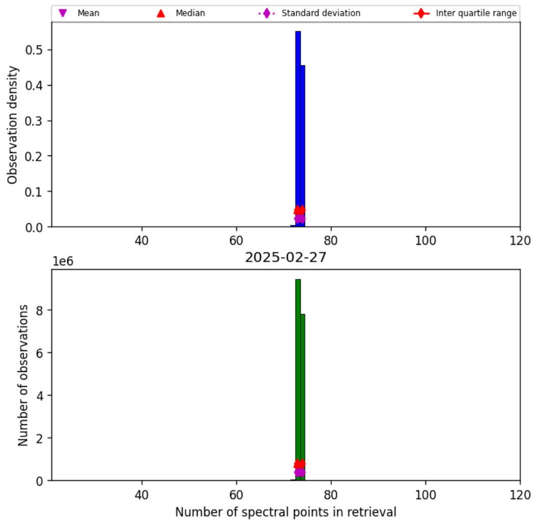
Figure 83: Histogram of "Number of spectral points in retrieval" for 2025-02-27 to 2025-02-27
