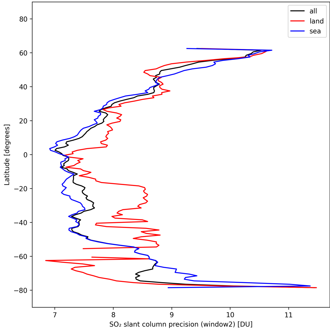
Figure 41: Zonal average of “SO 2 slant column precision (window2)” for 2025-02-27 to 2025-02-27.
