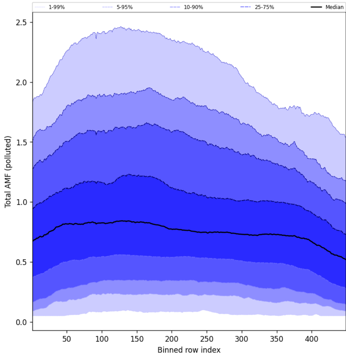
Figure 107: Along track statistics of “Total AMF (polluted)” for 2025-02-27 to 2025-02-27
