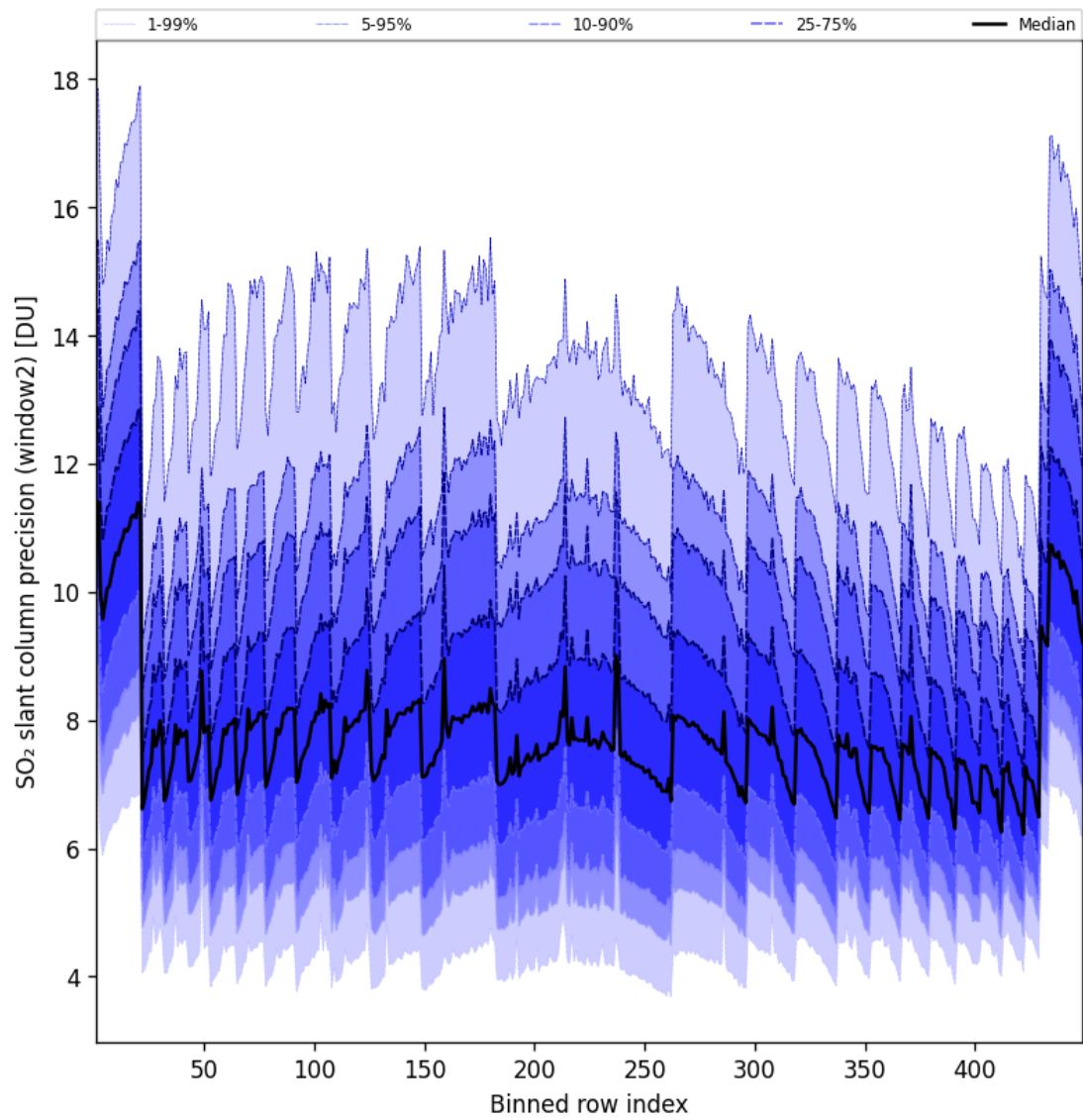
Figure 95: Along track statistics of “SO 2 slant column precision (window2)” for 2025-02-27 to 2025-02-27
