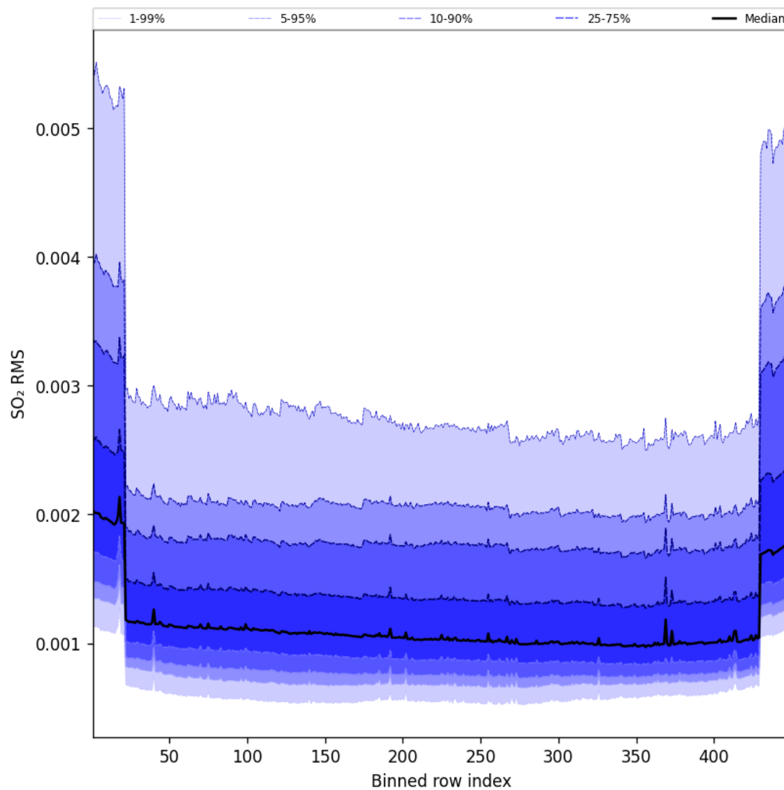
Figure 106: Along track statistics of “SO 2 RMS” for 2025-02-27 to 2025-02-27
