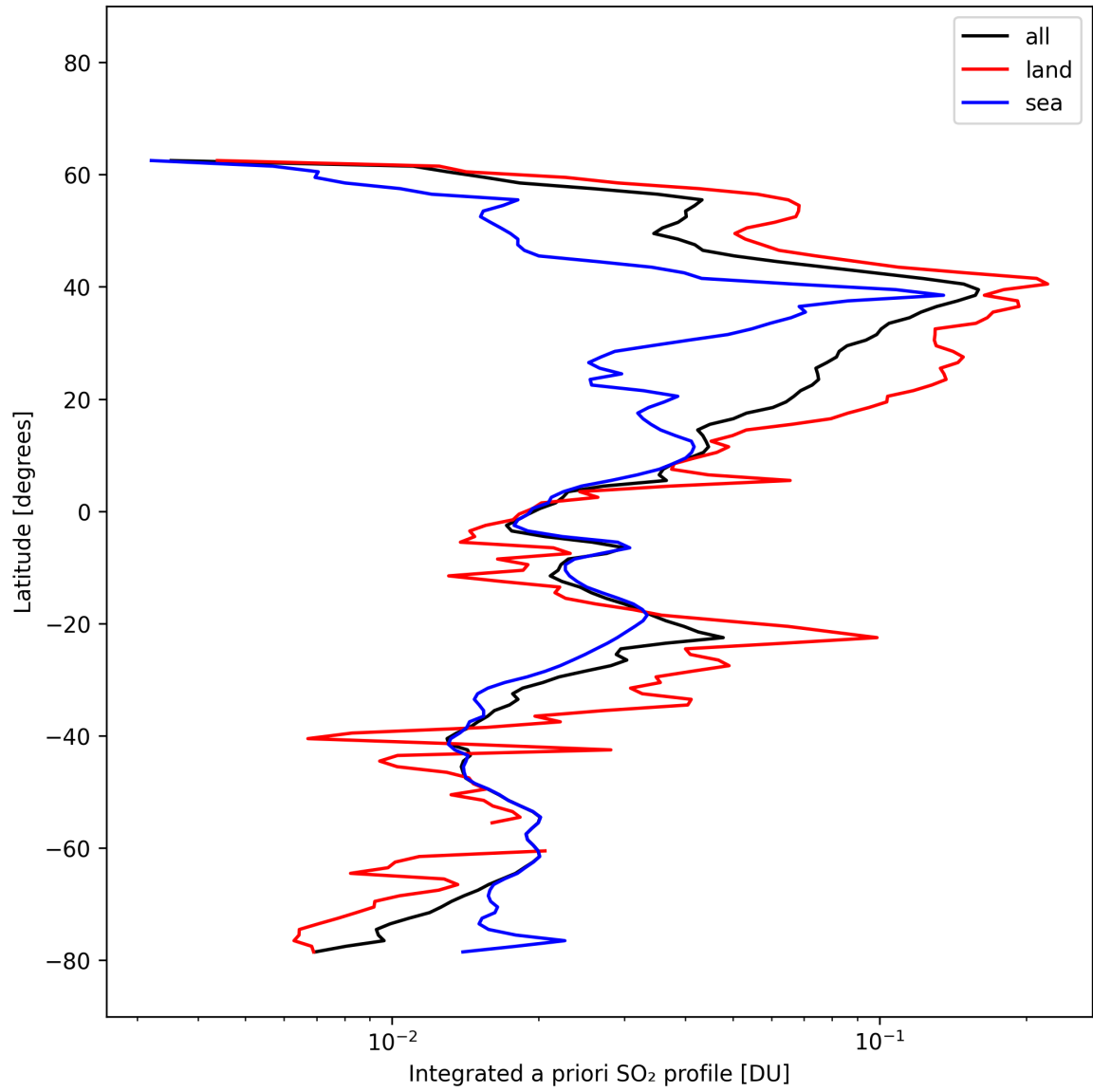
Figure 49: Zonal average of “Integrated a priori SO 2 profile” for 2025-02-27 to 2025-02-27.
