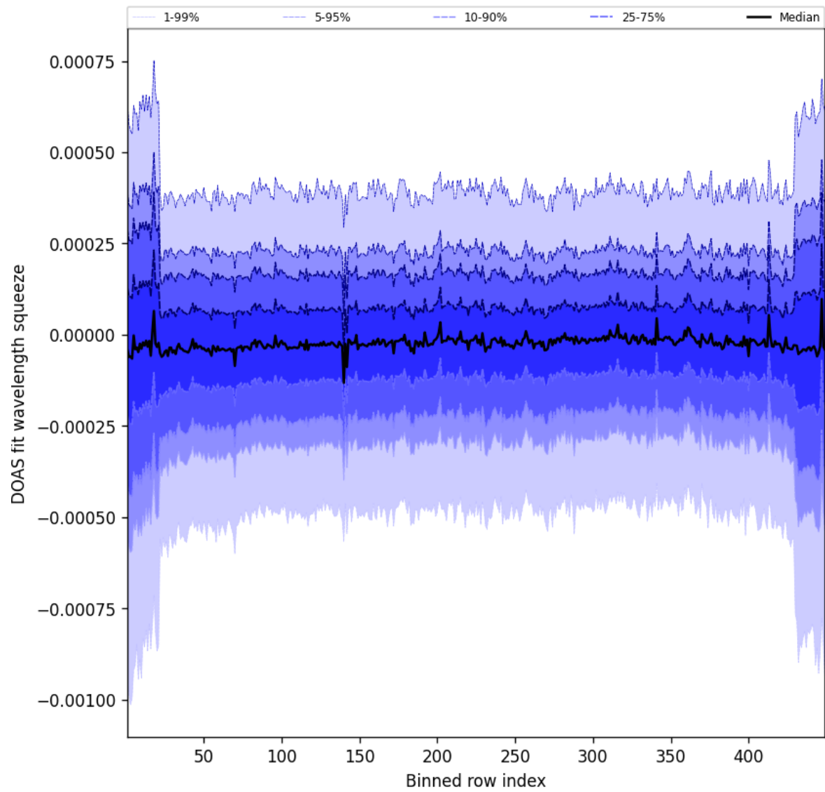
Figure 105: Along track statistics of “DOAS fit wavelength squeeze” for 2025-02-27 to 2025-02-27
