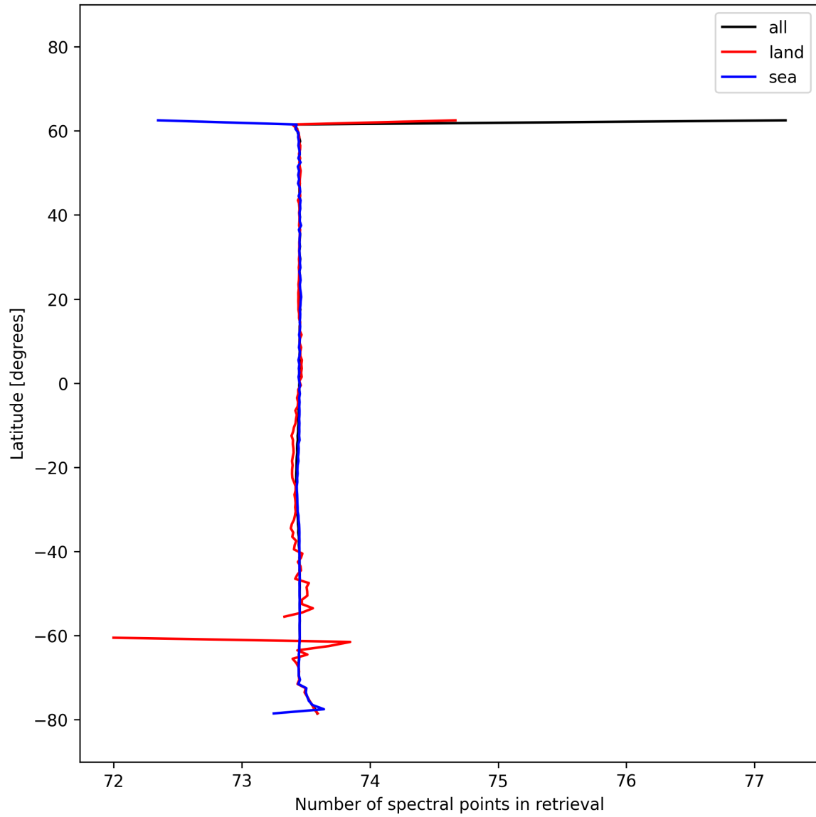
Figure 56: Zonal average of “Number of spectral points in retrieval” for 2025-02-27 to 2025-02-27.
