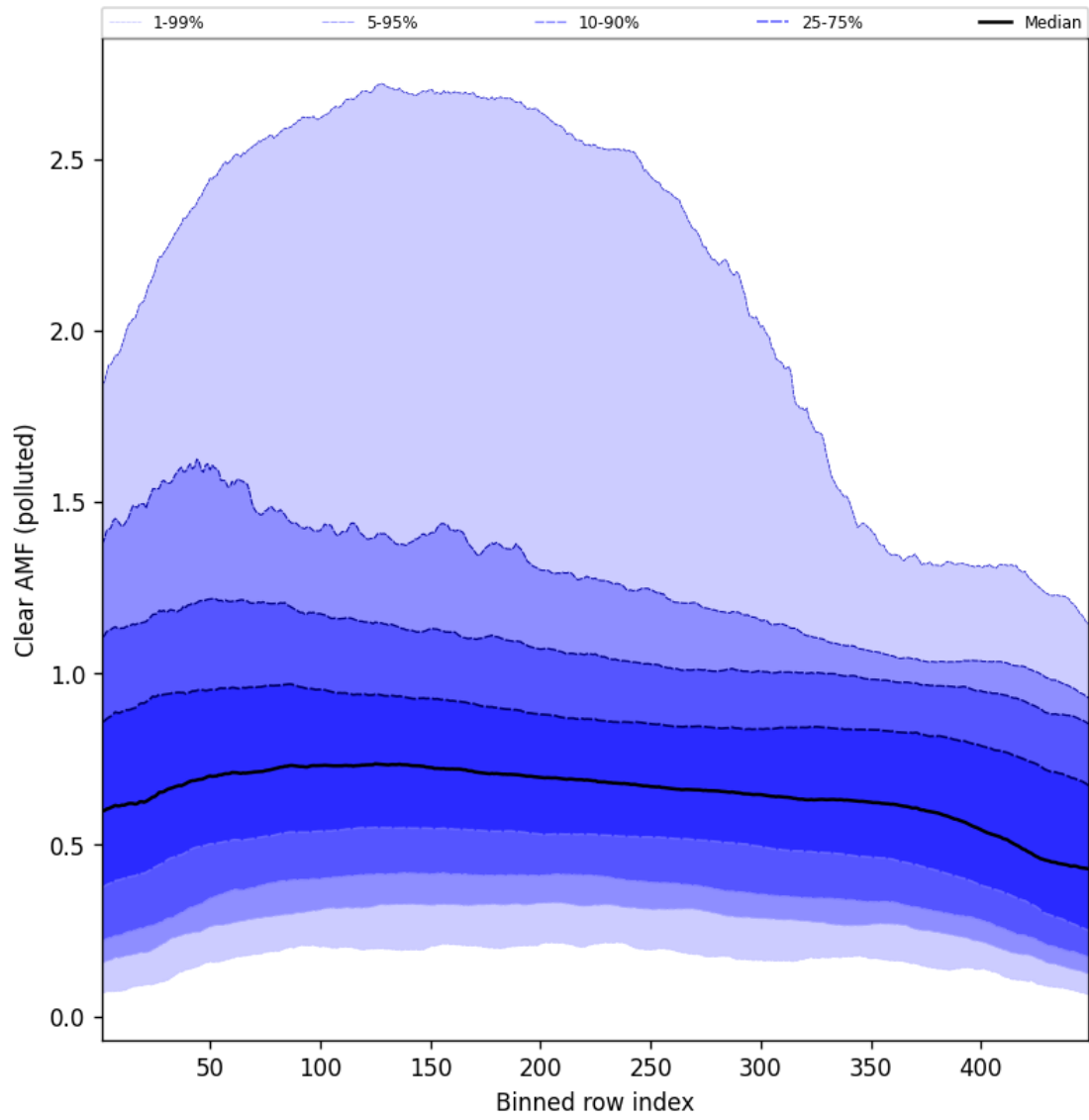
Figure 109: Along track statistics of “Clear AMF (polluted)” for 2025-02-27 to 2025-02-27
