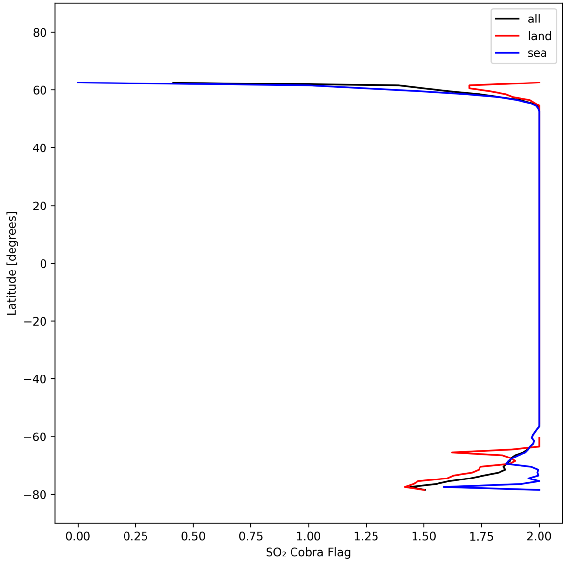
Figure 48: Zonal average of “SO 2 Cobra Flag” for 2025-02-27 to 2025-02-27.
