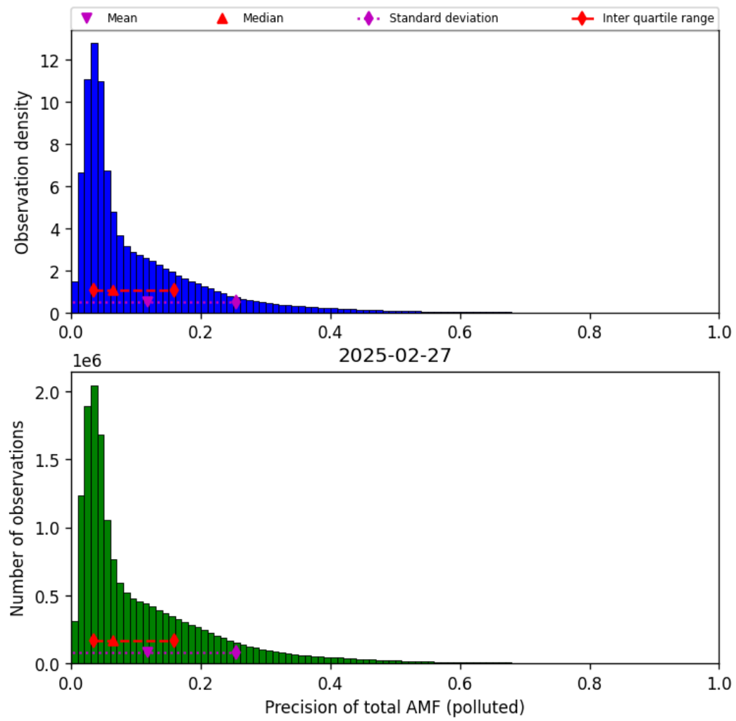
Figure 81: Histogram of “Precision of total AMF (polluted)” for 2025-02-27 to 2025-02-27
