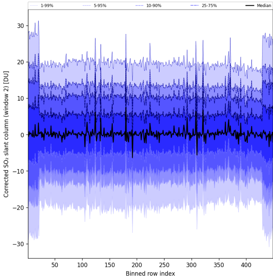
Figure 96: Along track statistics of “Corrected SO 2 slant column (window 2)” for 2025-02-27 to 2025-02-27
