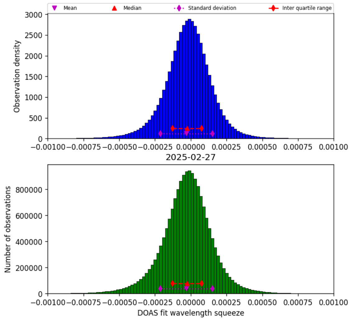
Figure 78: Histogram of “DOAS fit wavelength squeeze” for 2025-02-27 to 2025-02-27
