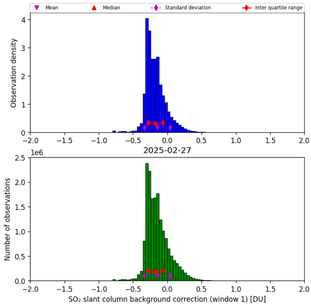
Figure 66: Histogram of “SO 2 slant column background correction (window 1)” for 2025-02-27 to 2025-02-27
