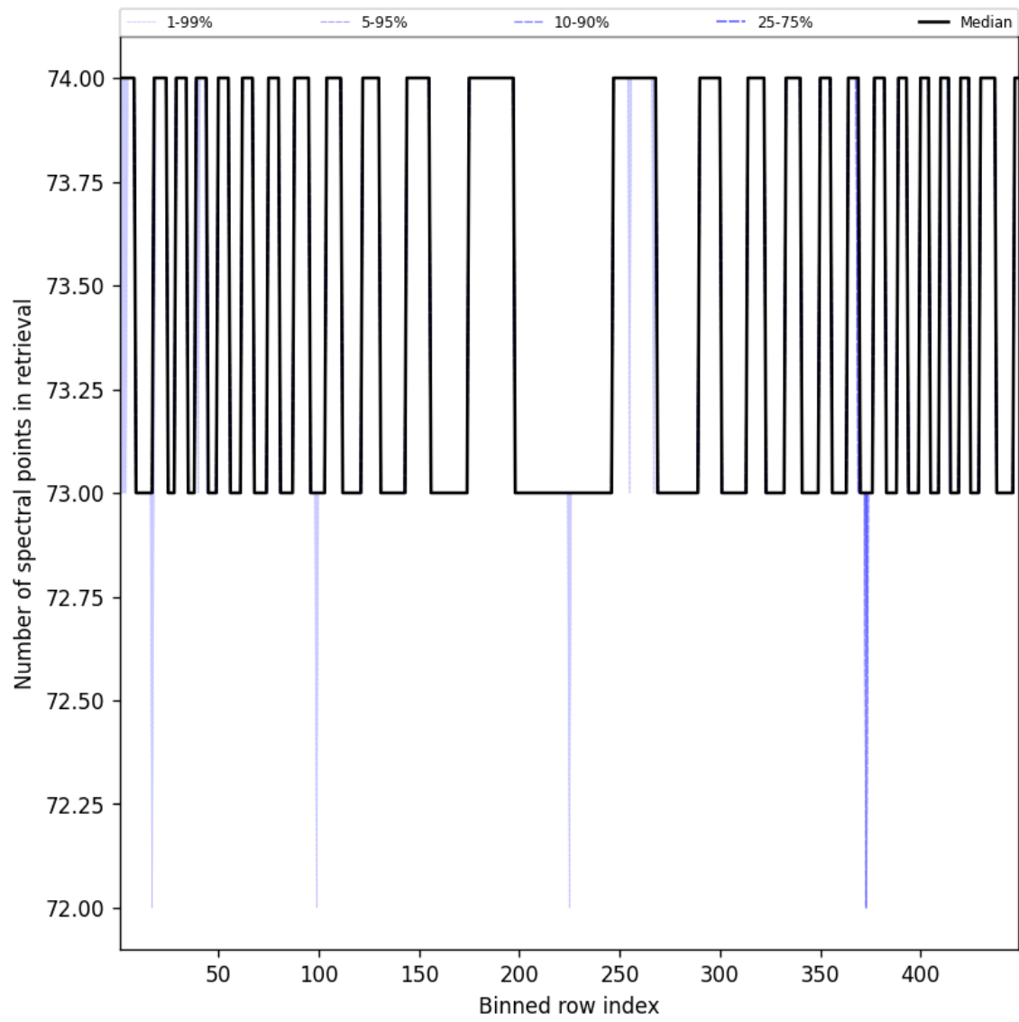
Figure 110: Along track statistics of “Number of spectral points in retrieval” for 2025-02-27 to 2025-02-27
