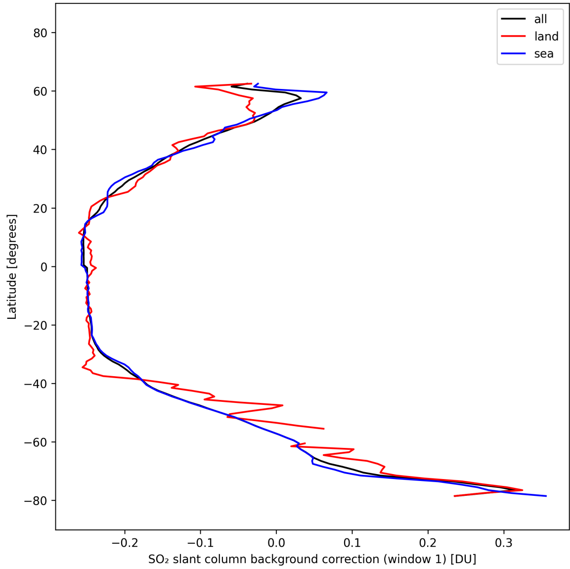
Figure 39: Zonal average of “SO 2 slant column background correction (window 1)” for 2025-02-27 to 2025-02-27.
