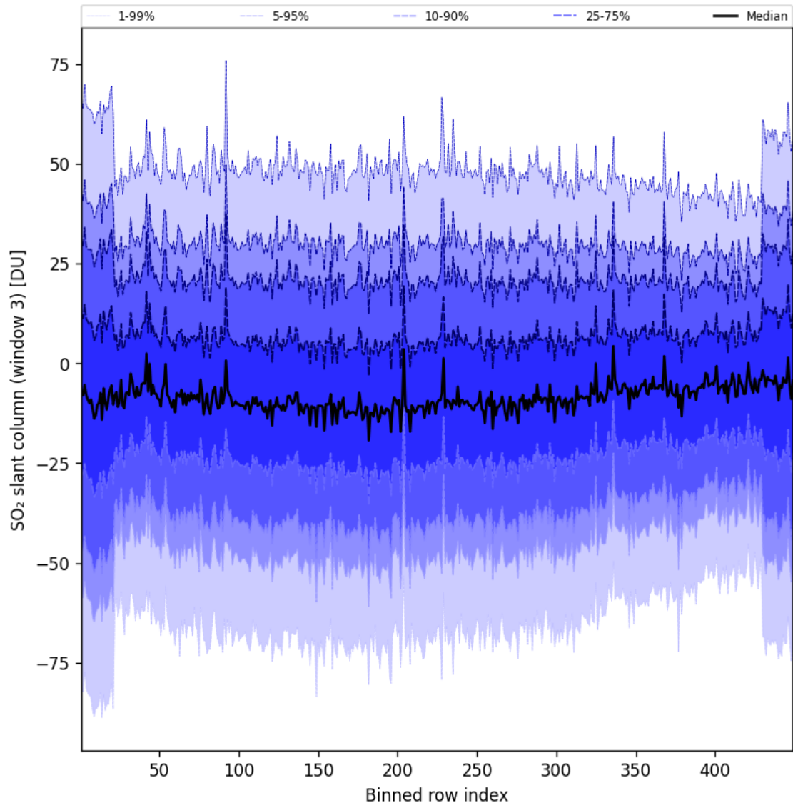
Figure 98: Along track statistics of “SO 2 slant column (window 3)” for 2025-02-27 to 2025-02-27
