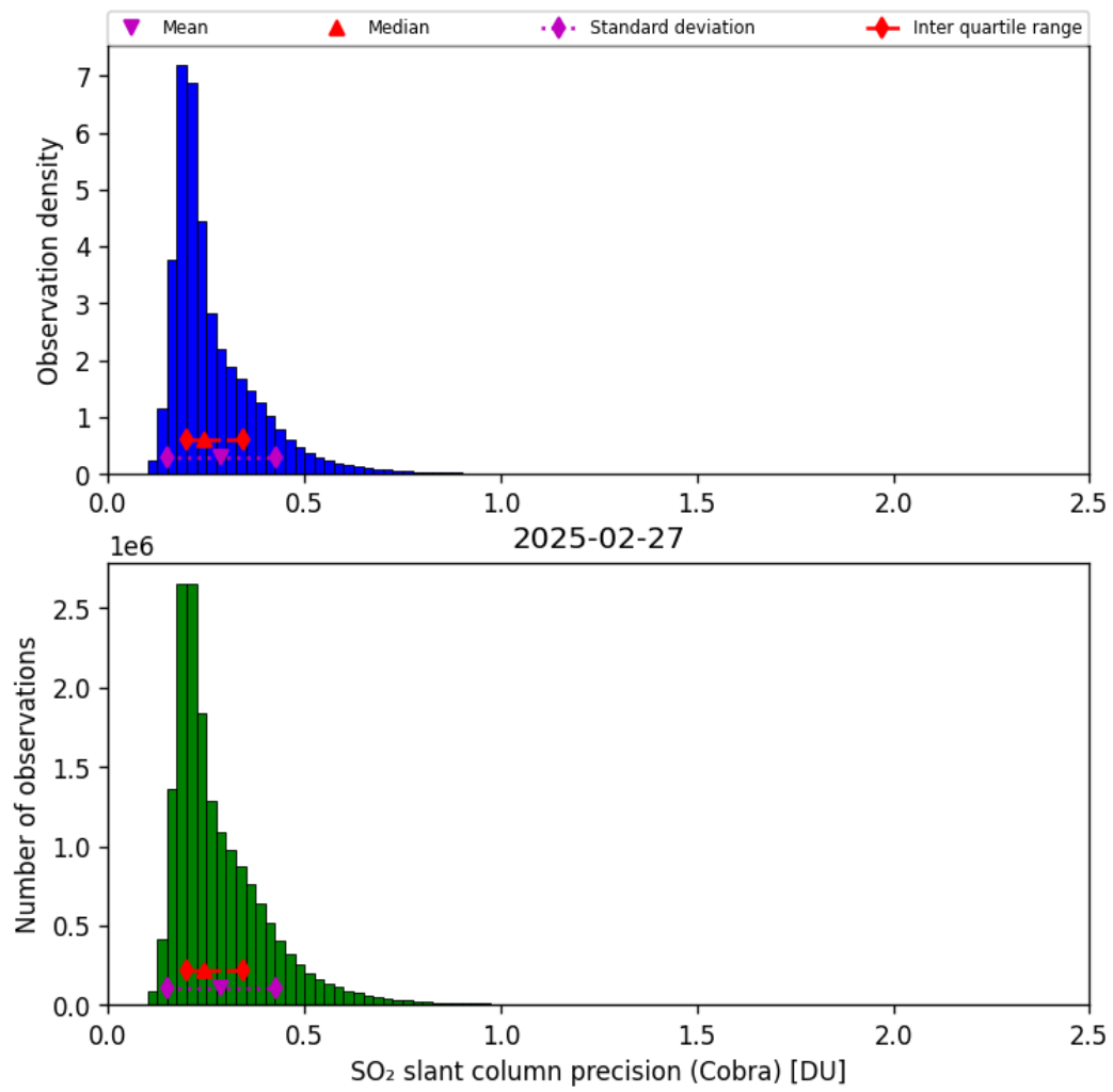
Figure 62: Histogram of “SO 2 slant column precision (Cobra)” for 2025-02-27 to 2025-02-27
