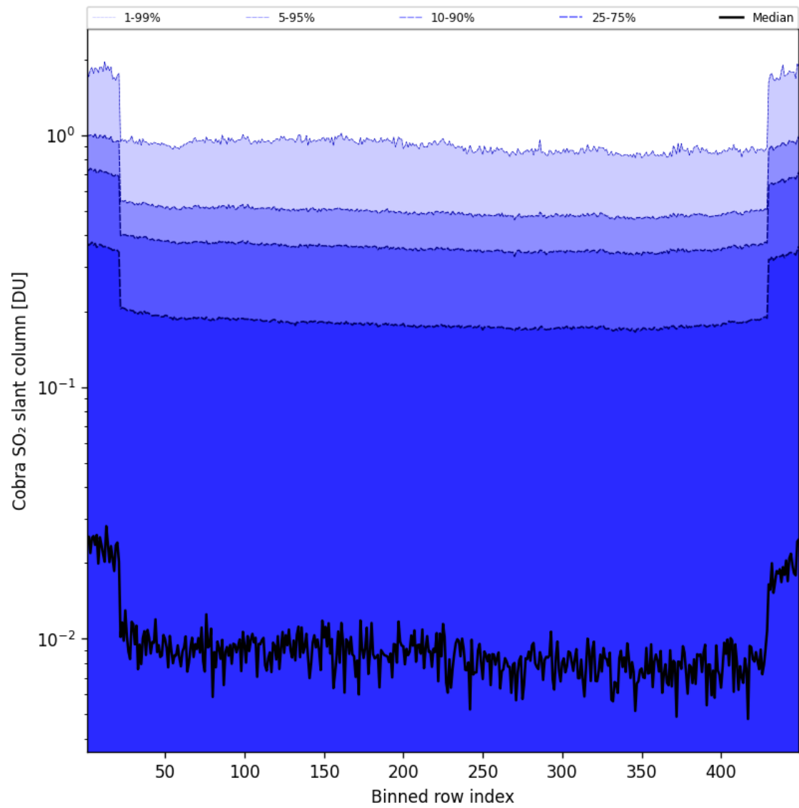
Figure 88: Along track statistics of “Cobra SO 2 slant column” for 2025-02-27 to 2025-02-27
