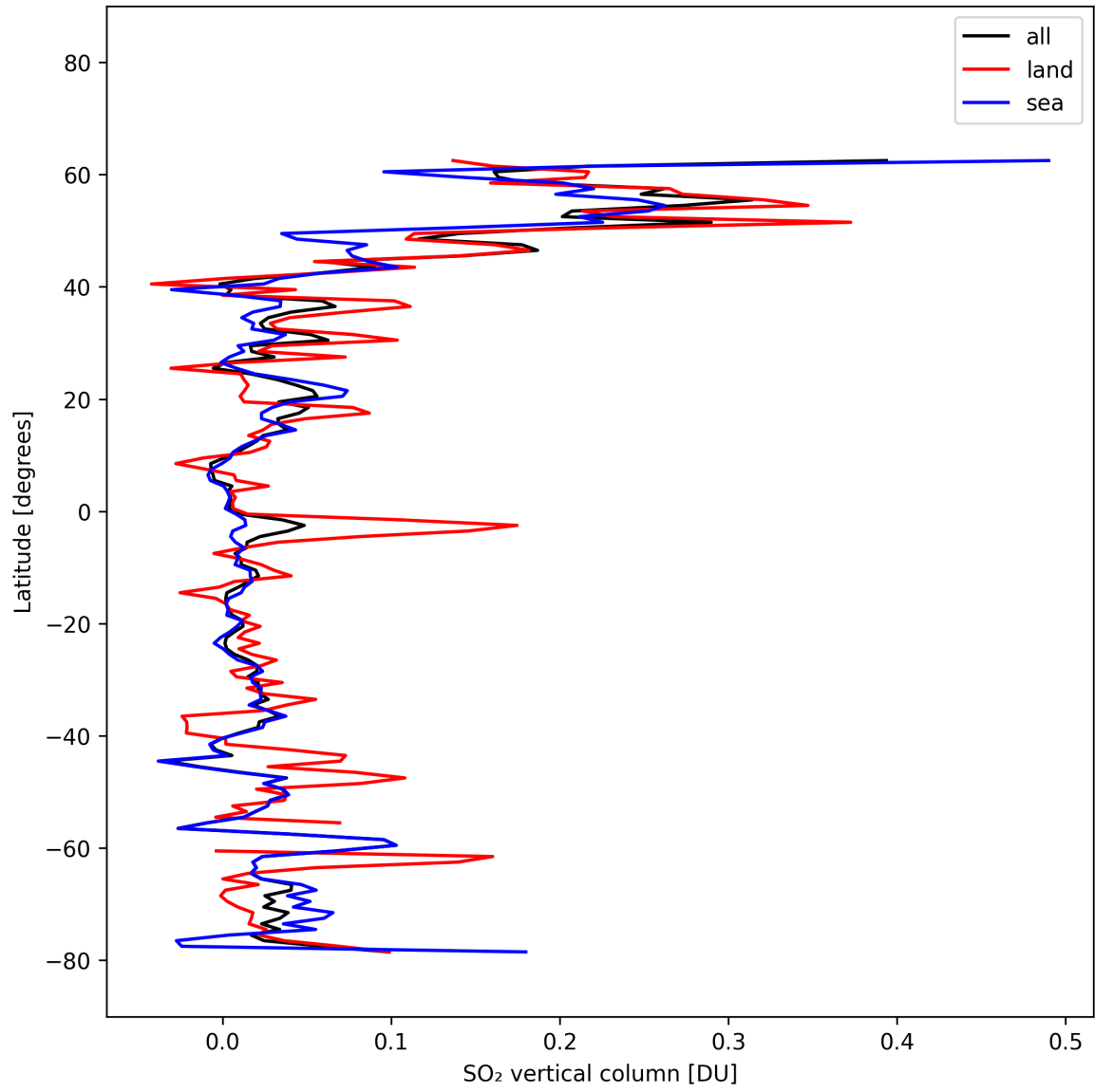
Figure 31: Zonal average of “SO 2 vertical column” for 2025-02-27 to 2025-02-27.
