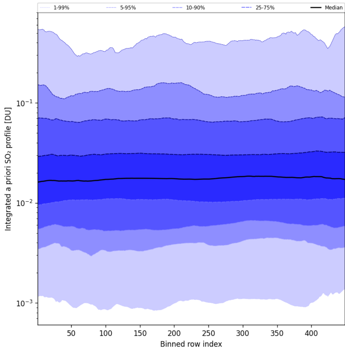
Figure 103: Along track statistics of “Integrated a priori SO 2 profile” for 2025-02-27 to 2025-02-27
