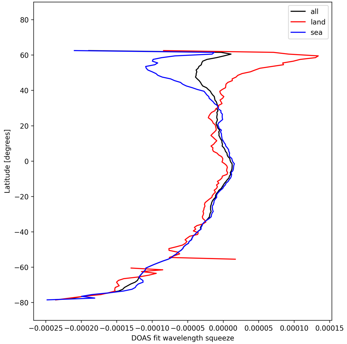
Figure 51: Zonal average of “DOAS fit wavelength squeeze” for 2025-02-27 to 2025-02-27.
