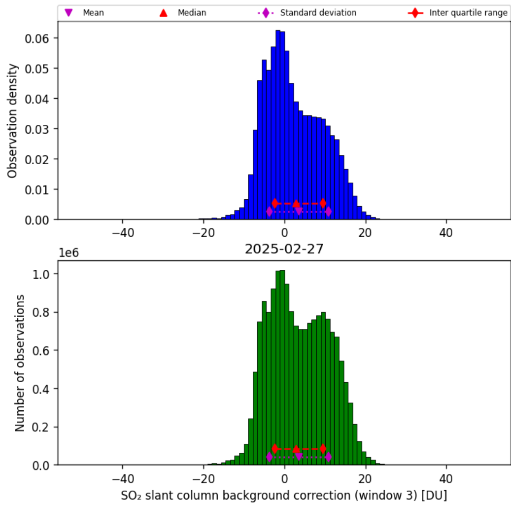
Figure 74: Histogram of “SO 2 slant column background correction (window 3)” for 2025-02-27 to 2025-02-27
