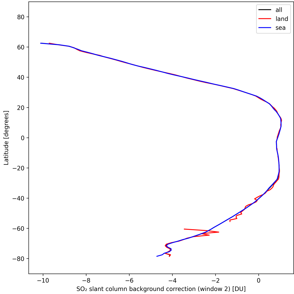
Figure 43: Zonal average of “SO 2 slant column background correction (window 2)” for 2025-02-27 to 2025-02-27.
