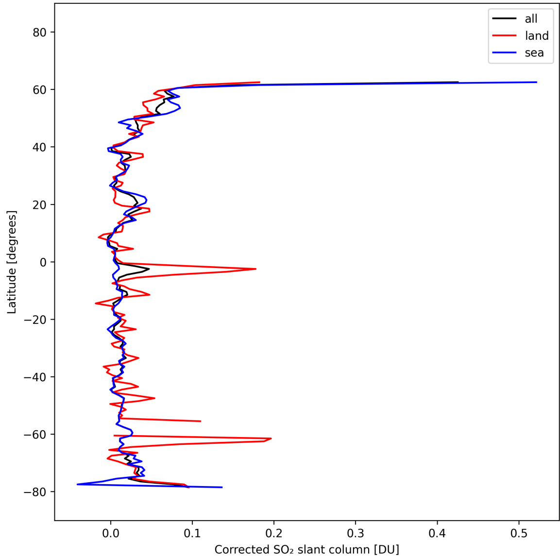
Figure 33: Zonal average of “Corrected SO 2 slant column” for 2025-02-27 to 2025-02-27.
