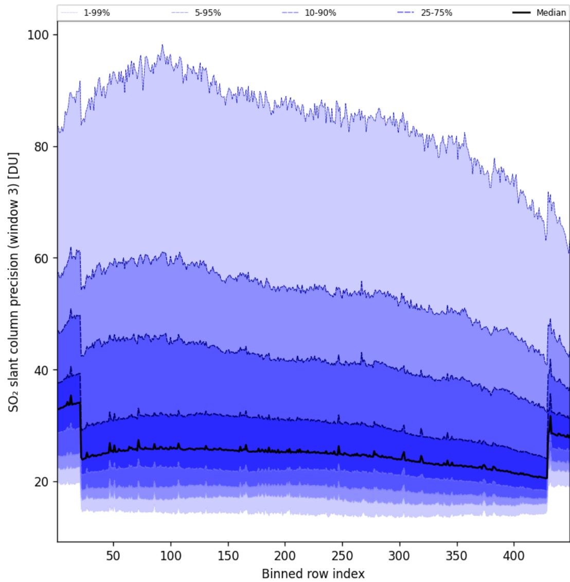
Figure 99: Along track statistics of “SO 2 slant column precision (window 3)” for 2025-04-03 to 2025-04-04
