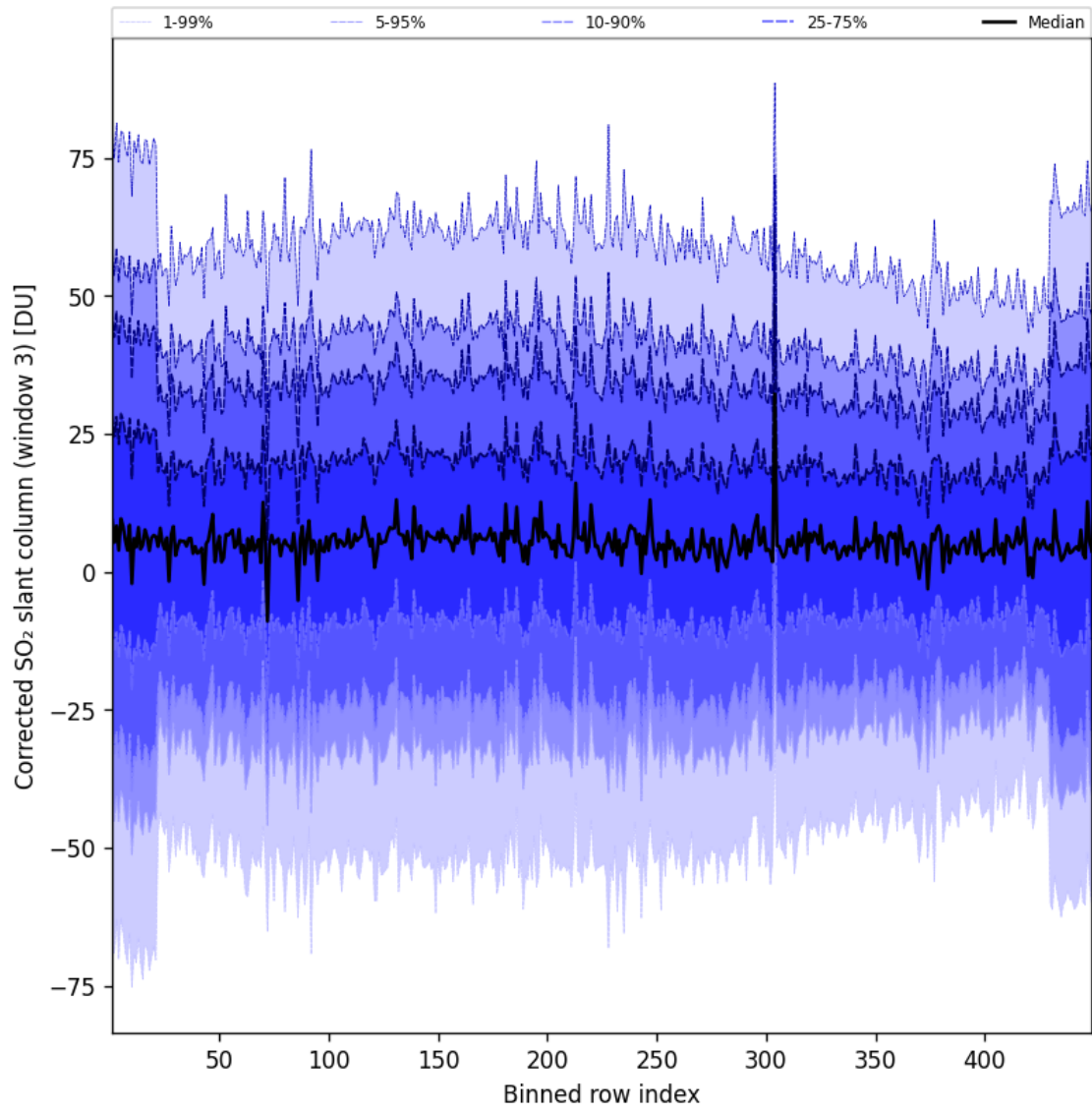
Figure 100: Along track statistics of “Corrected SO 2 slant column (window 3)” for 2025-04-03 to 2025-04-04
