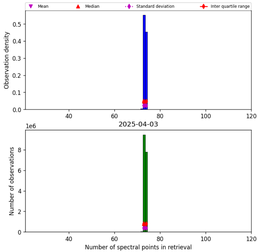
Figure 83: Histogram of “Number of spectral points in retrieval” for 2025-04-03 to 2025-04-04
