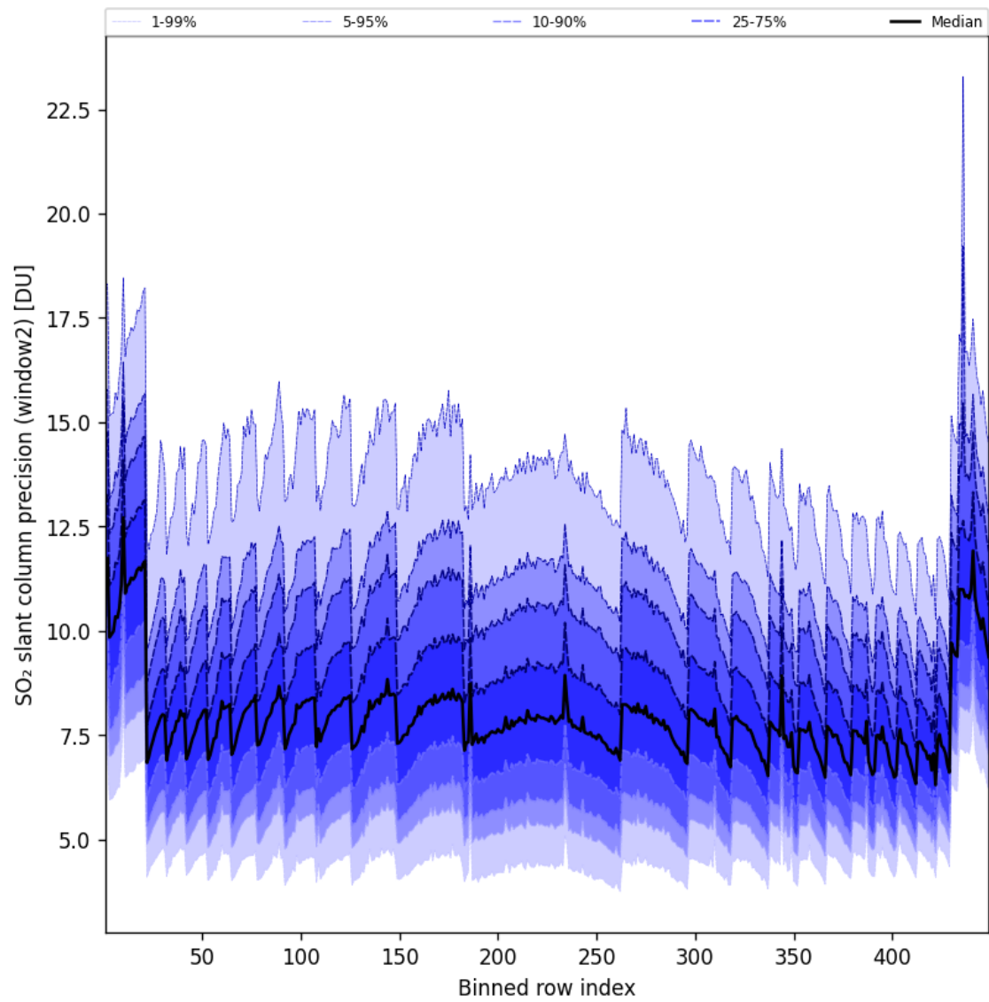
Figure 95: Along track statistics of “SO 2 slant column precision (window2)” for 2025-04-03 to 2025-04-04
