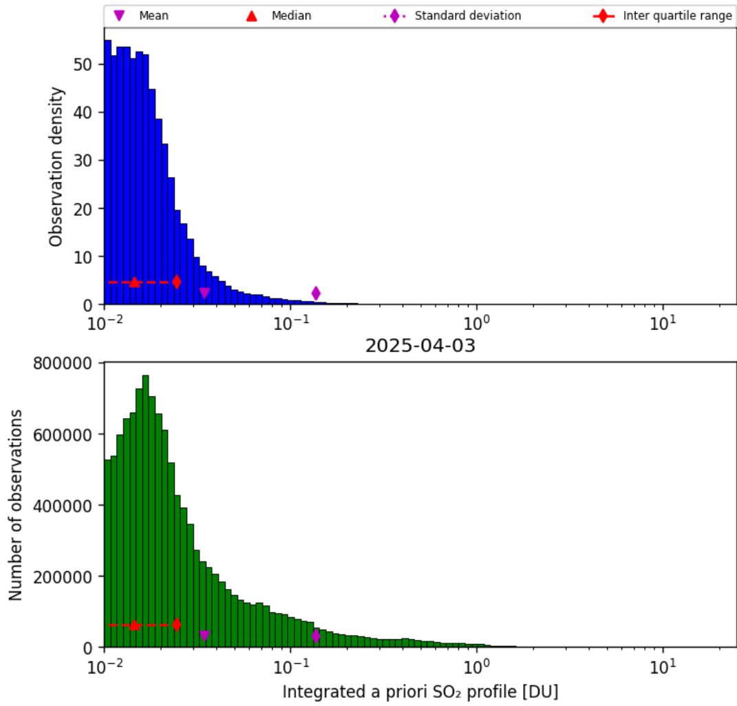
Figure 76: Histogram of “Integrated a priori SO 2 profile” for 2025-04-03 to 2025-04-04
