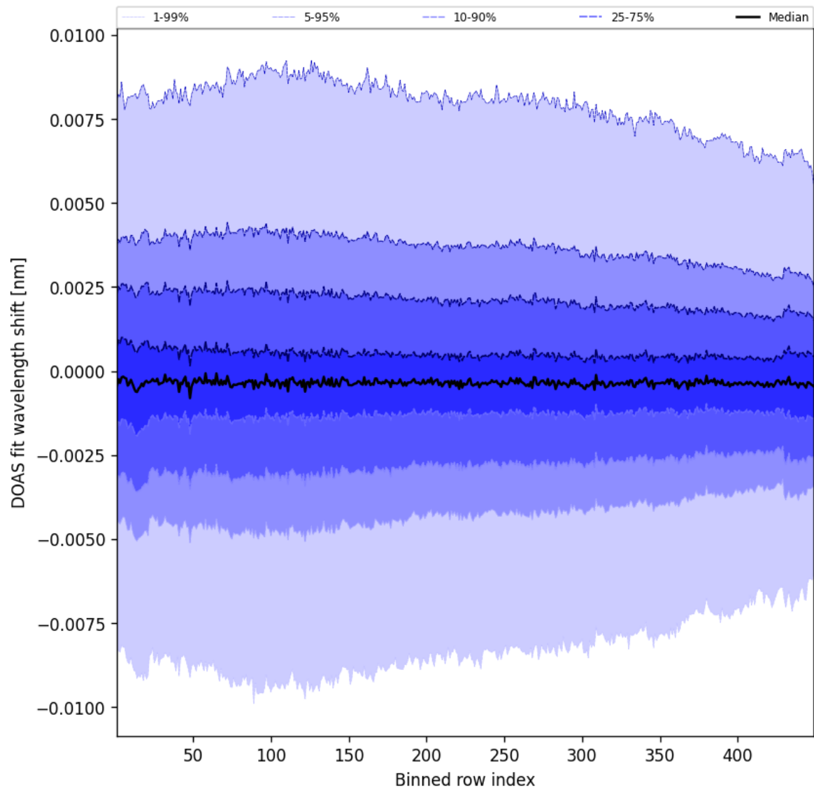
Figure 104: Along track statistics of “DOAS fit wavelength shift” for 2025-04-03 to 2025-04-04
