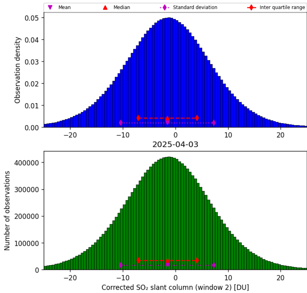
Figure 69: Histogram of “Corrected SO 2 slant column (window 2)” for 2025-04-03 to 2025-04-04
