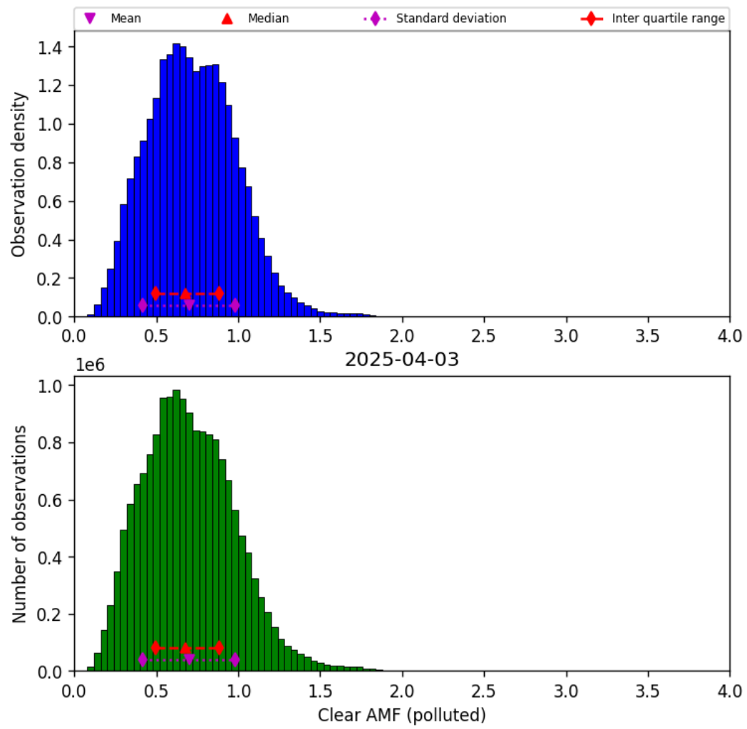
Figure 82: Histogram of “Clear AMF (polluted)” for 2025-04-03 to 2025-04-04
