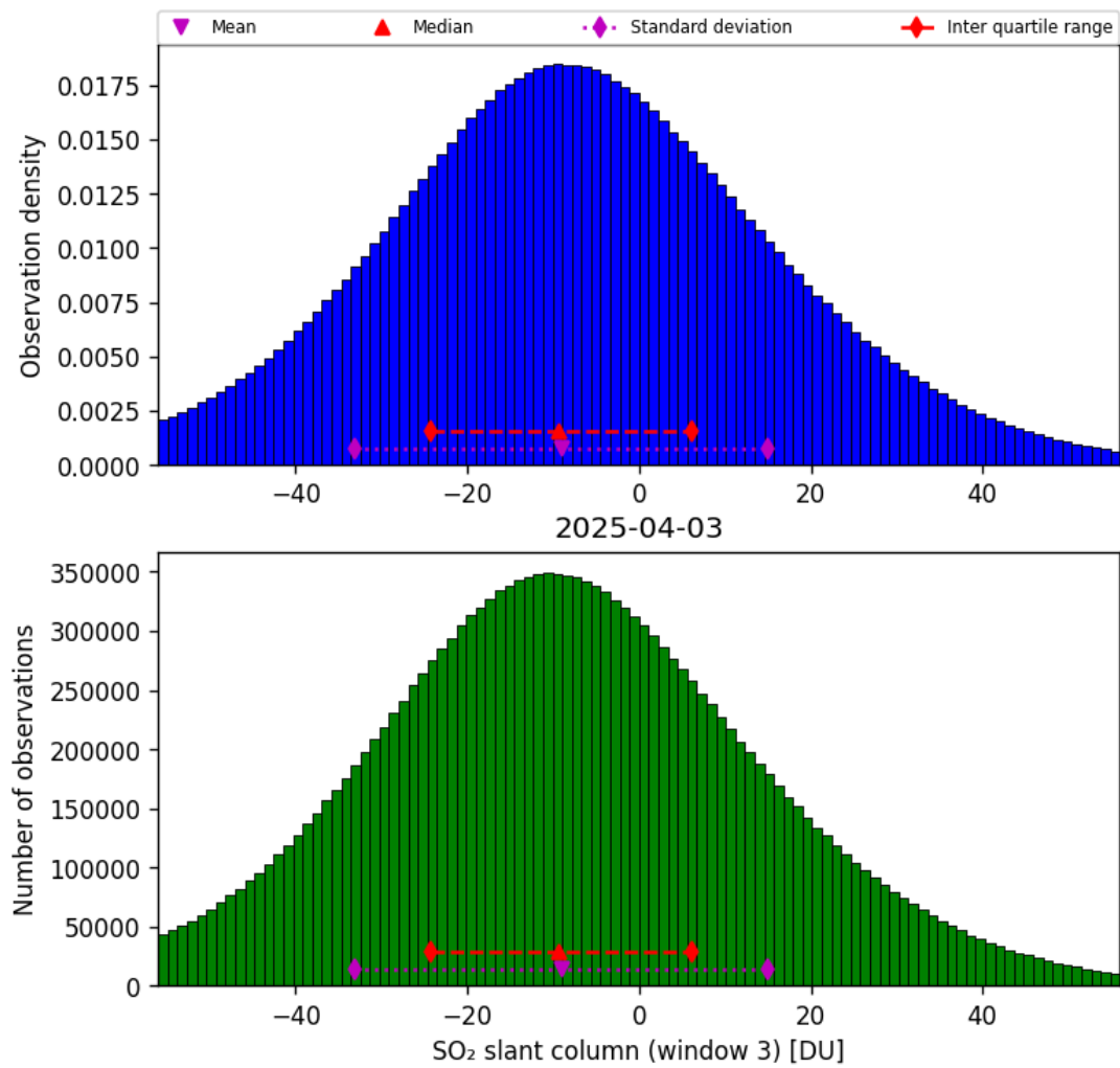
Figure 71: Histogram of “SO 2 slant column (window 3)” for 2025-04-03 to 2025-04-04
