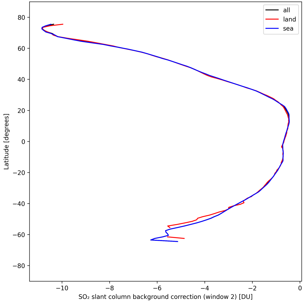
Figure 43: Zonal average of “SO 2 slant column background correction (window 2)” for 2025-04-03 to 2025-04-04.
