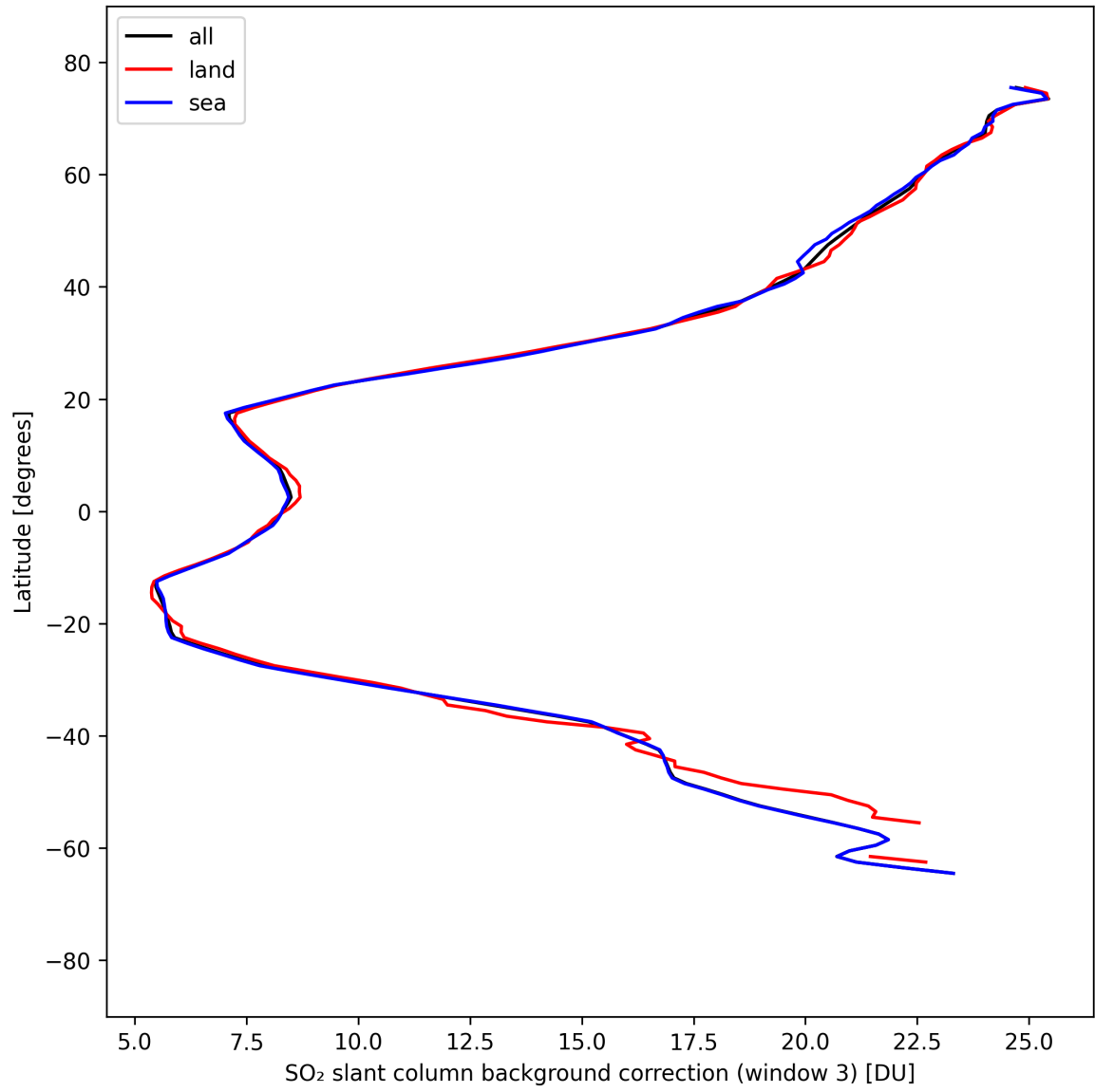
Figure 47: Zonal average of “SO 2 slant column background correction (window 3)” for 2025-04-03 to 2025-04-04.
