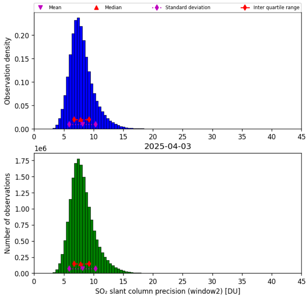
Figure 68: Histogram of “SO 2 slant column precision (window2)” for 2025-04-03 to 2025-04-04
