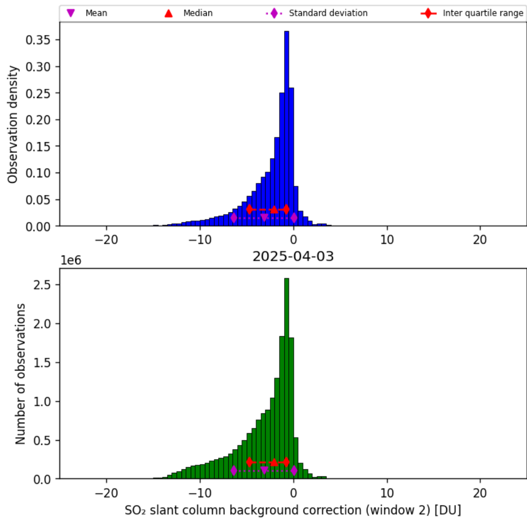
Figure 70: Histogram of “SO 2 slant column background correction (window 2)” for 2025-04-03 to 2025-04-04
