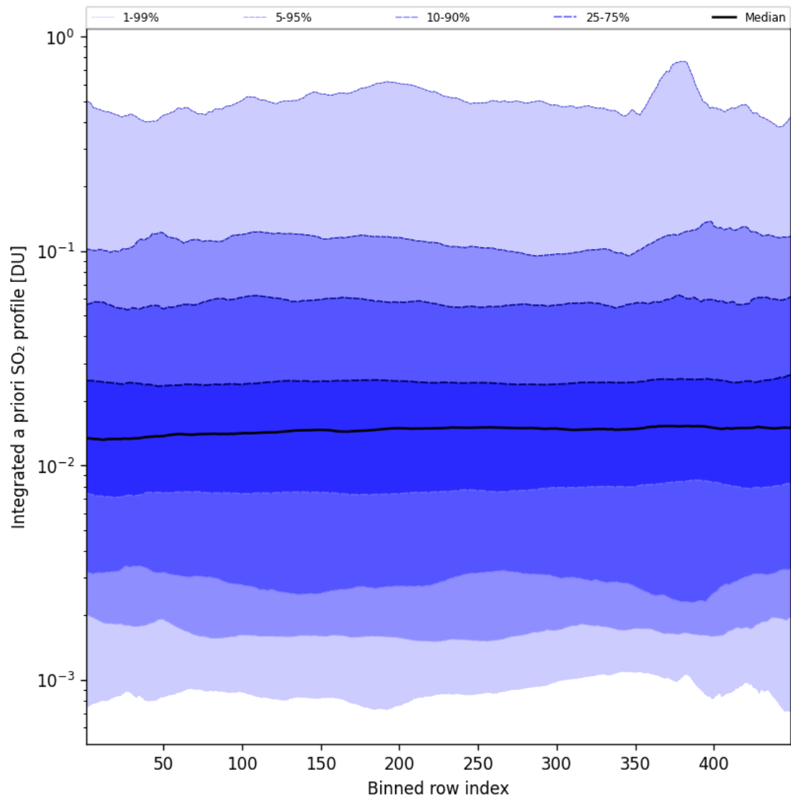
Figure 103: Along track statistics of “Integrated a priori SO 2 profile” for 2025-04-03 to 2025-04-04
