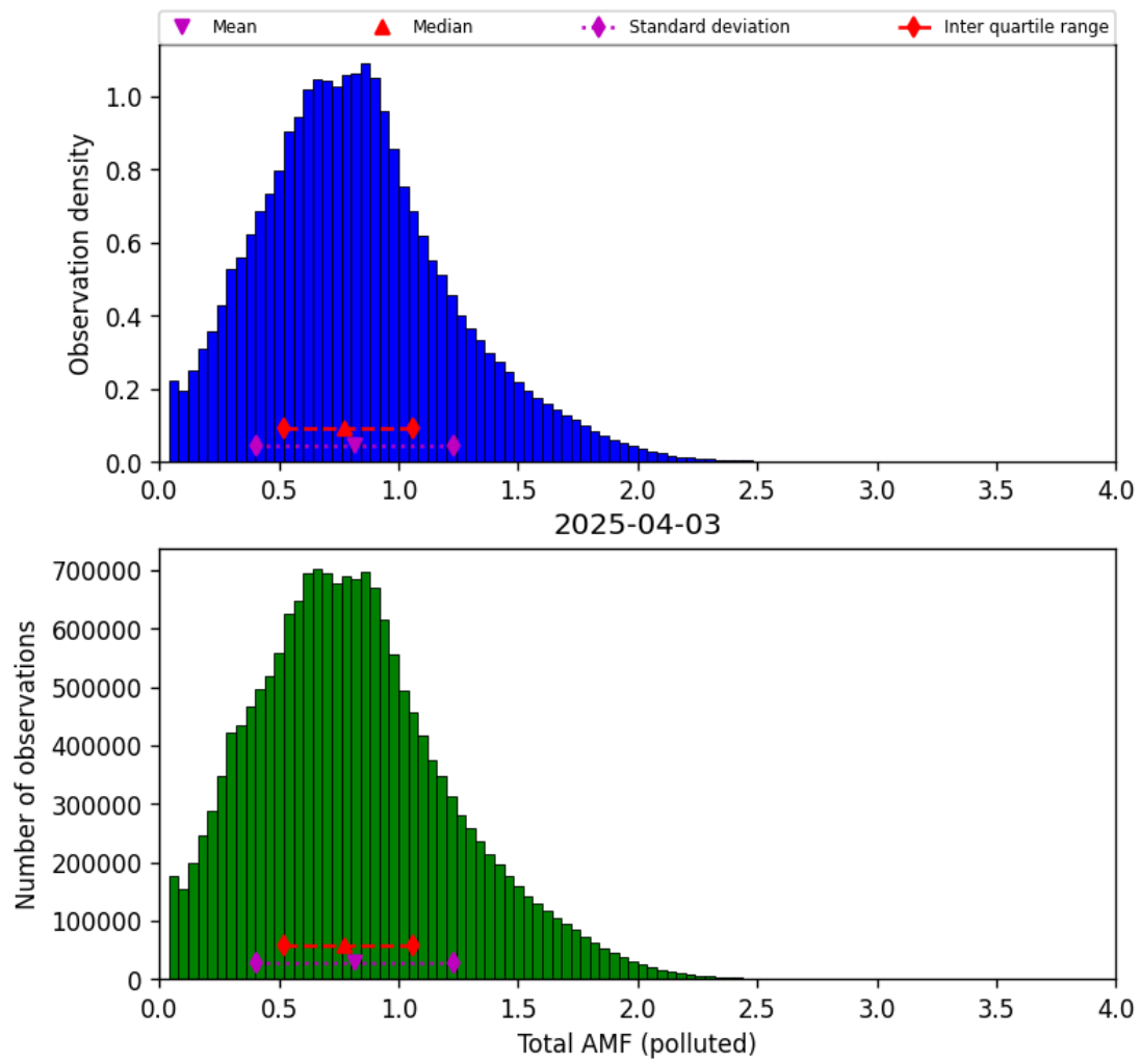
Figure 80: Histogram of “Total AMF (polluted)” for 2025-04-03 to 2025-04-04
