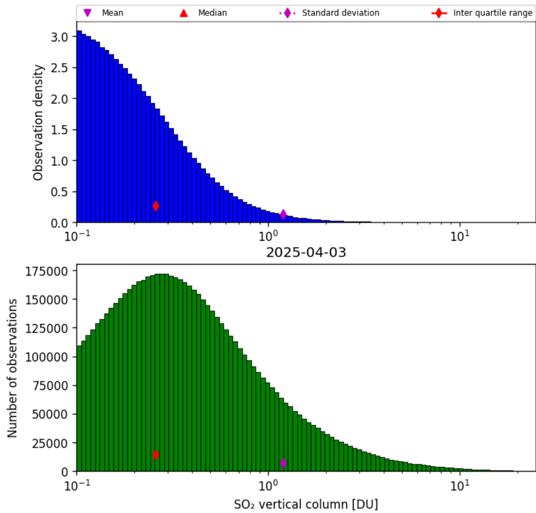
Figure 58: Histogram of “SO 2 vertical column” for 2025-04-03 to 2025-04-04
