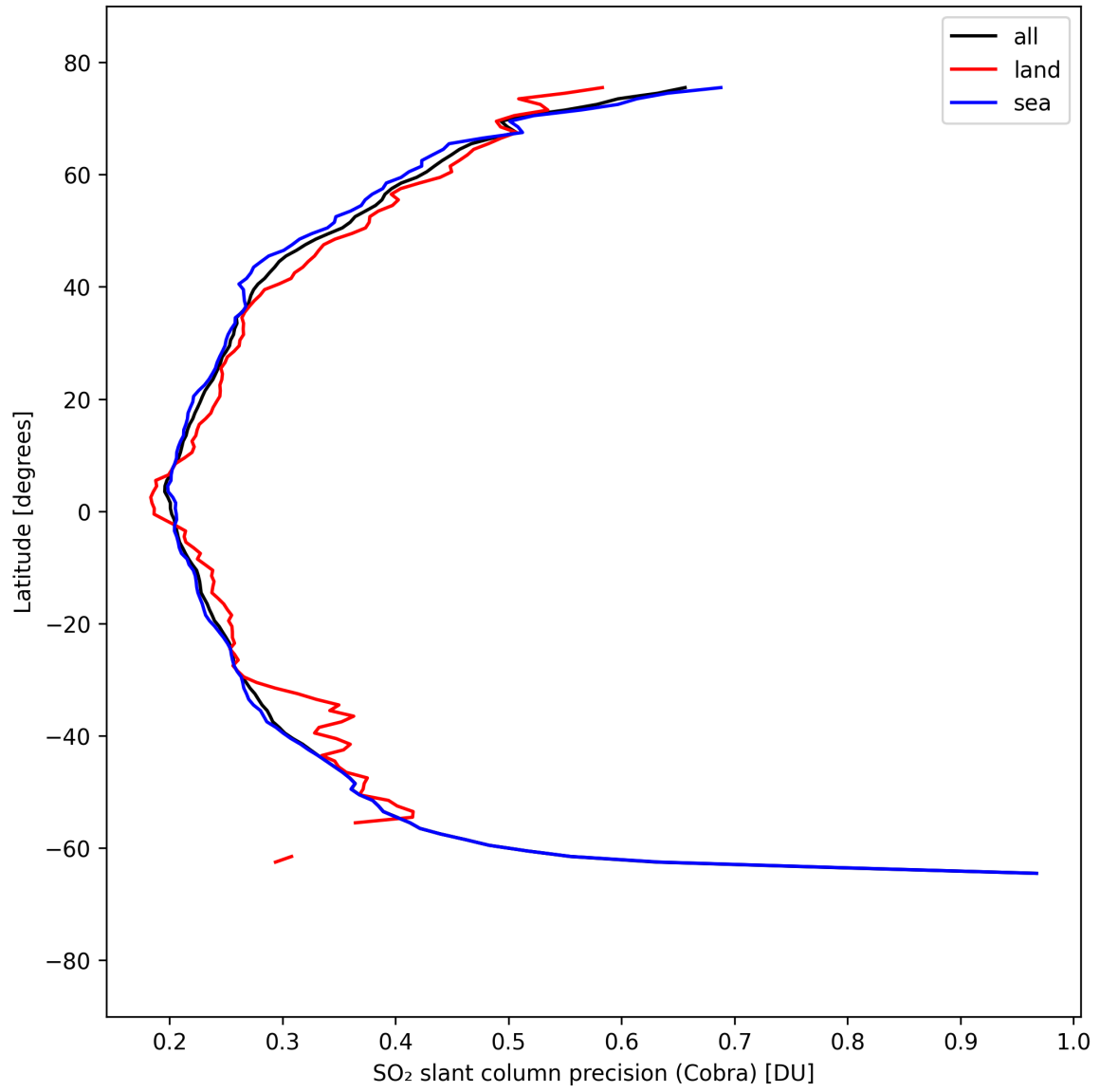
Figure 35: Zonal average of “SO 2 slant column precision (Cobra)” for 2025-04-03 to 2025-04-04.
