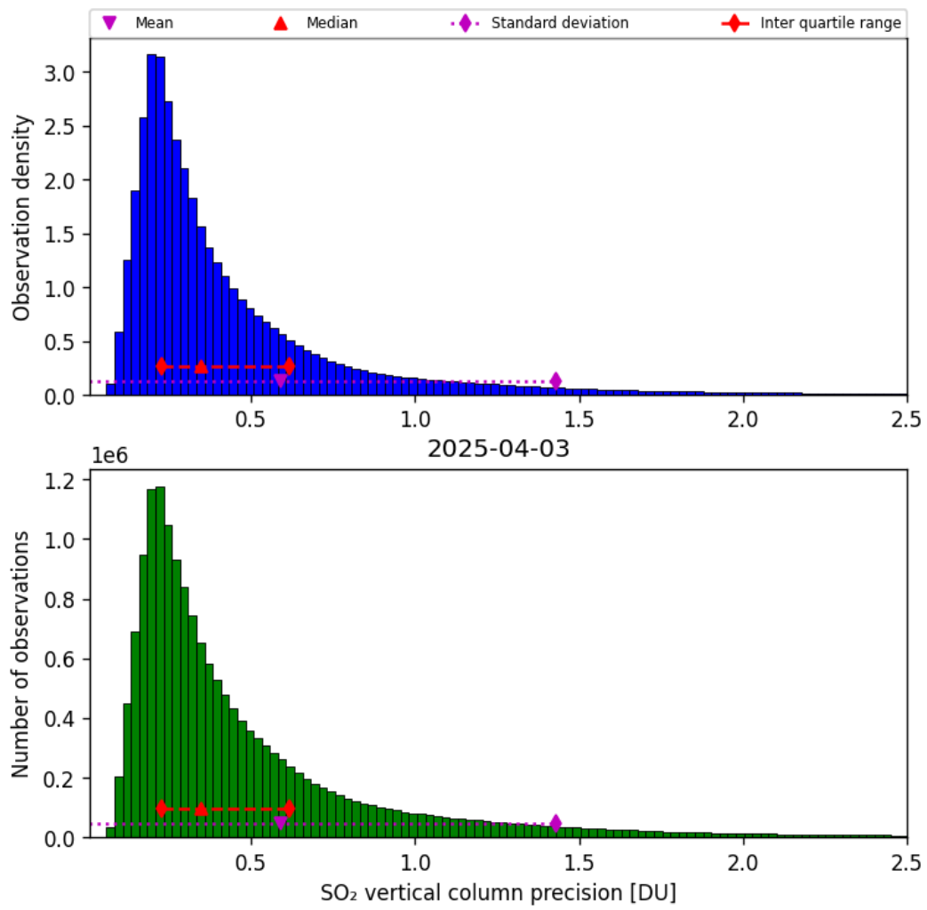
Figure 59: Histogram of “SO 2 vertical column precision” for 2025-04-03 to 2025-04-04
