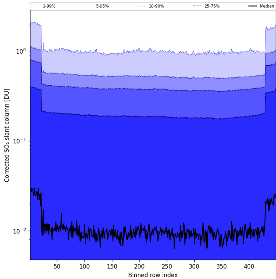
Figure 87: Along track statistics of “Corrected SO 2 slant column” for 2025-04-03 to 2025-04-04
