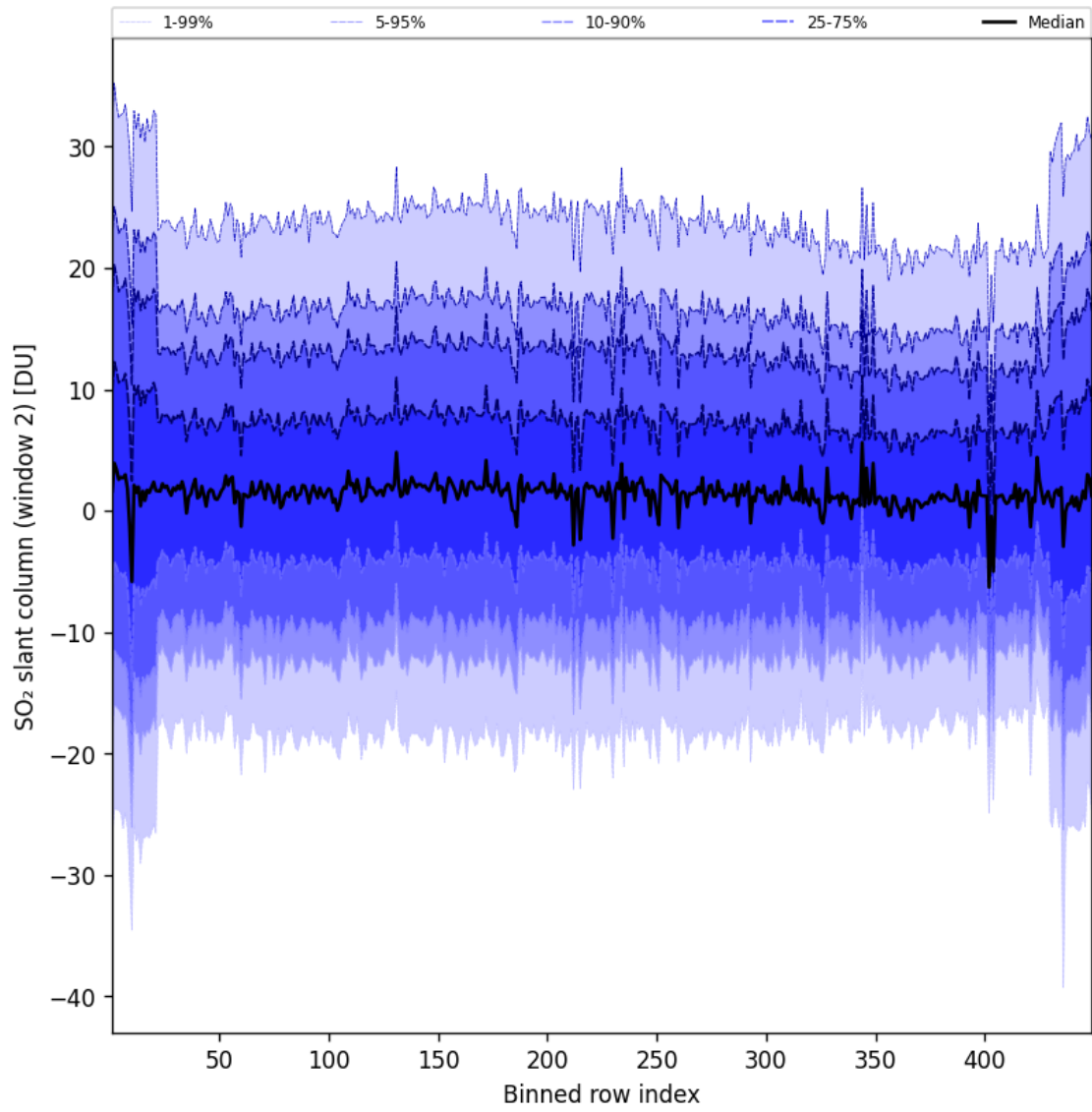
Figure 94: Along track statistics of “SO 2 slant column (window 2)” for 2025-04-03 to 2025-04-04
