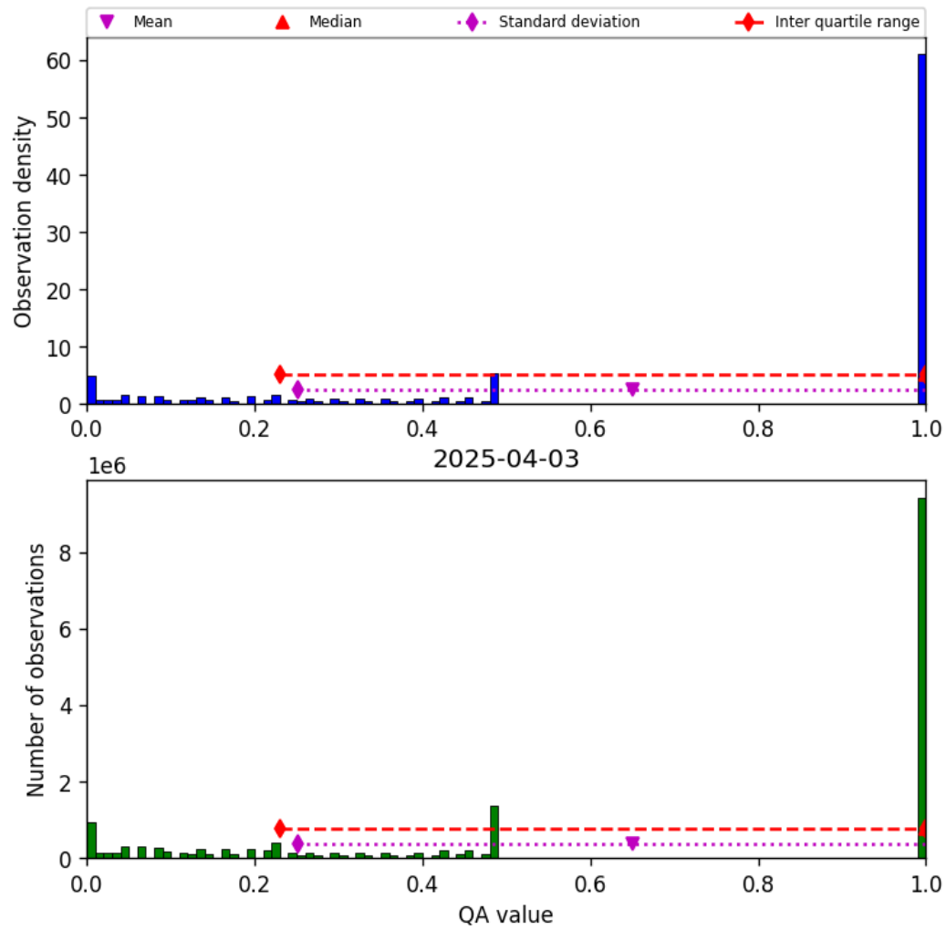
Figure 57: Histogram of “QA value” for 2025-04-03 to 2025-04-04
