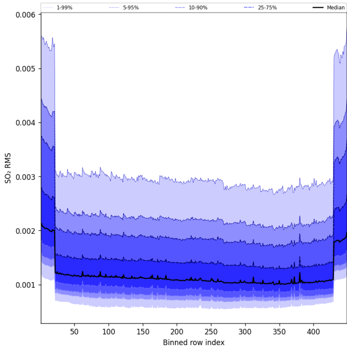
Figure 106: Along track statistics of “SO 2 RMS” for 2025-04-03 to 2025-04-04
