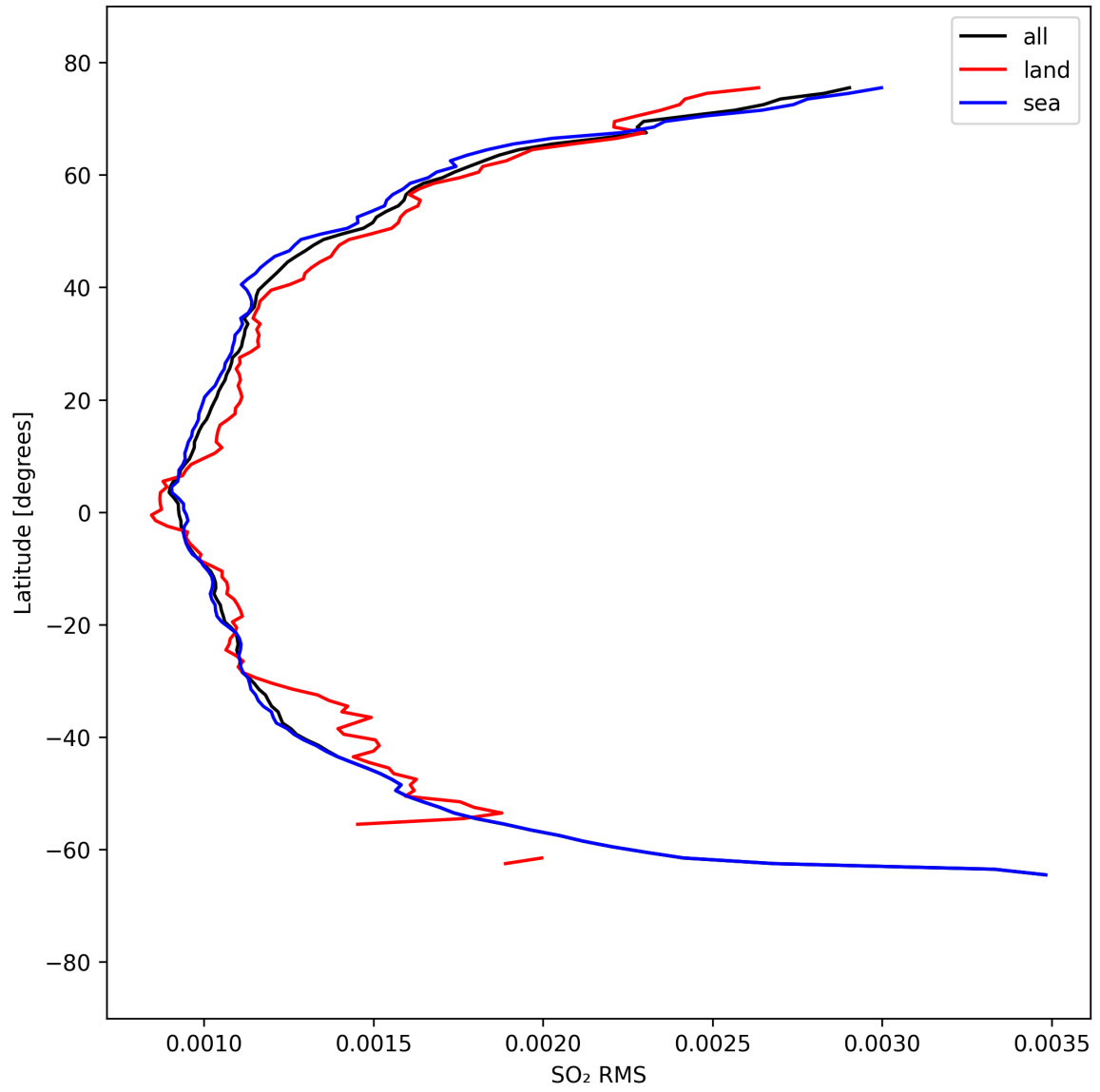
Figure 52: Zonal average of “SO 2 RMS” for 2025-04-03 to 2025-04-04.
