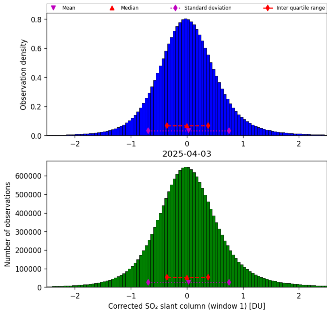
Figure 65: Histogram of “Corrected SO 2 slant column (window 1)” for 2025-04-03 to 2025-04-04
