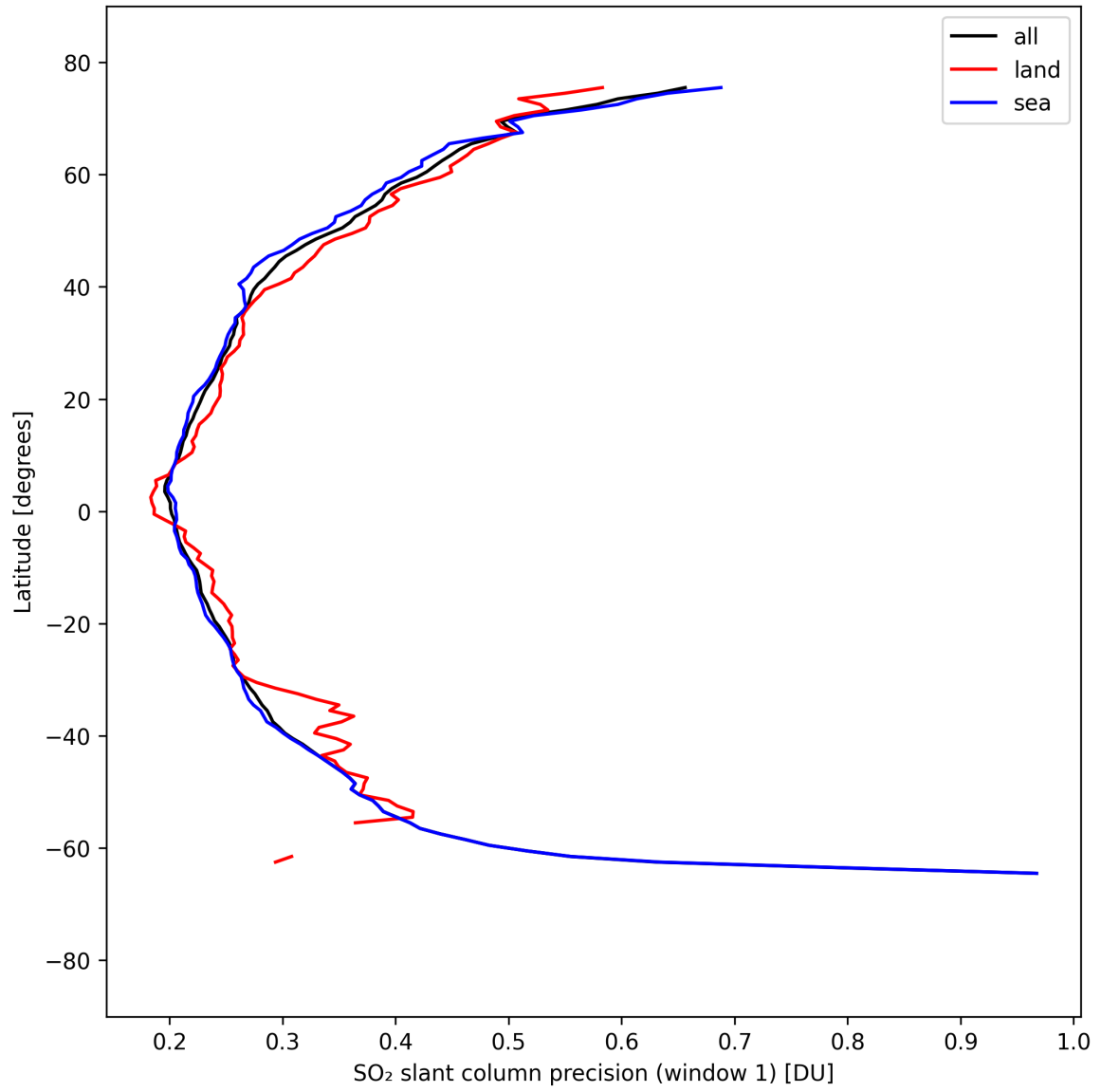
Figure 37: Zonal average of “SO 2 slant column precision (window 1)” for 2025-04-03 to 2025-04-04.
