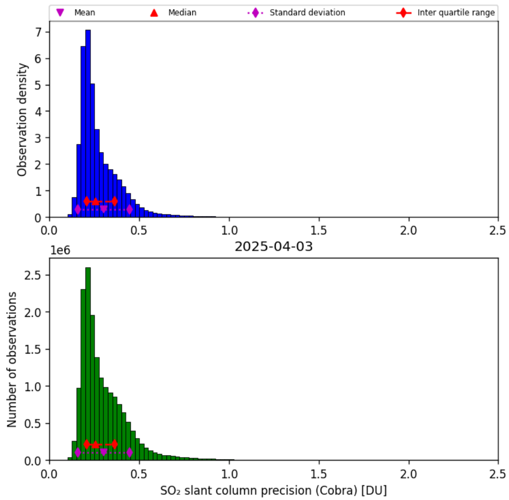
Figure 62: Histogram of “SO 2 slant column precision (Cobra)” for 2025-04-03 to 2025-04-04
