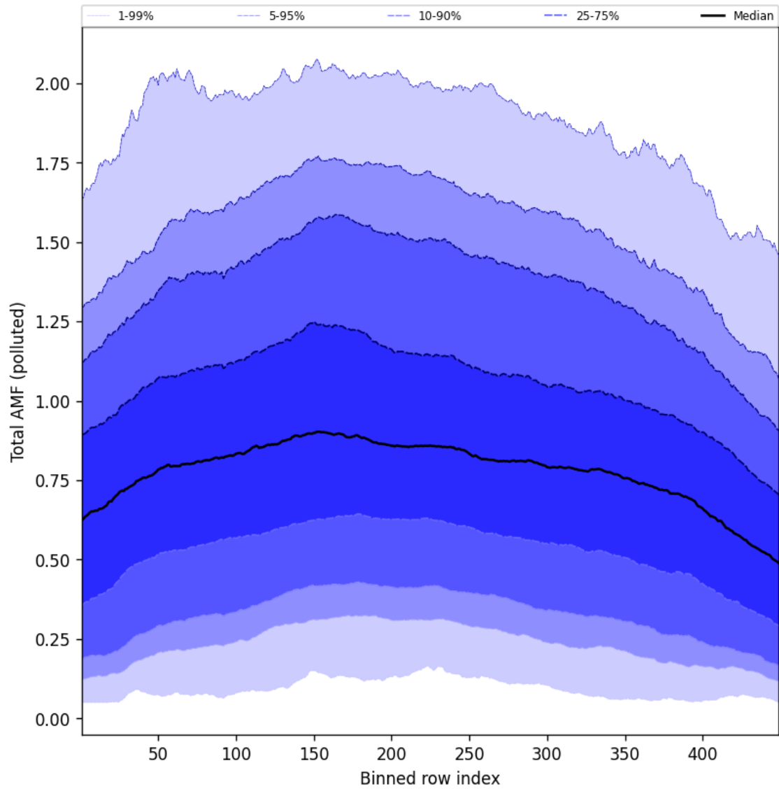
Figure 107: Along track statistics of “Total AMF (polluted)” for 2025-04-03 to 2025-04-04
