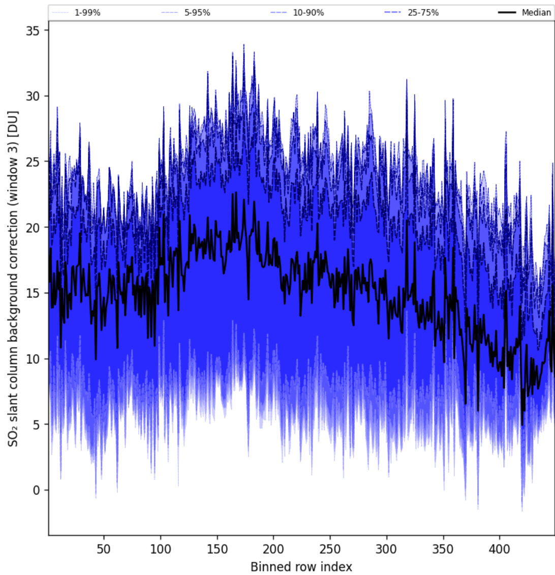
Figure 101: Along track statistics of “SO 2 slant column background correction (window 3)” for 2025-04-03 to 2025-04-04
