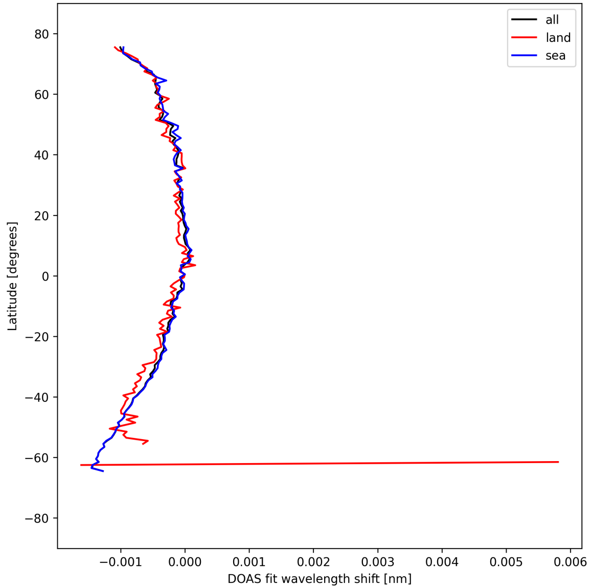
Figure 50: Zonal average of “DOAS fit wavelength shift” for 2025-04-03 to 2025-04-04.
