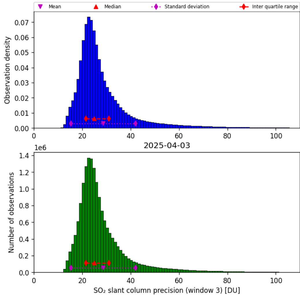
Figure 72: Histogram of “SO 2 slant column precision (window 3)” for 2025-04-03 to 2025-04-04
