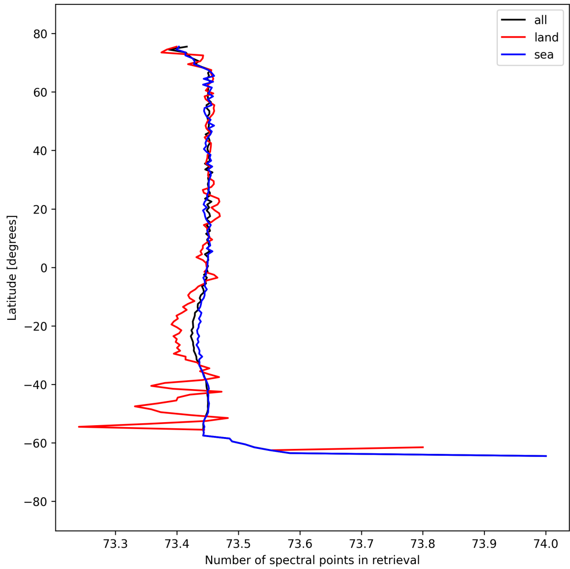
Figure 56: Zonal average of “Number of spectral points in retrieval” for 2025-04-03 to 2025-04-04.
