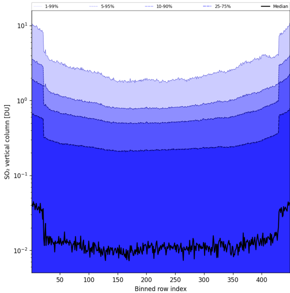
Figure 85: Along track statistics of “SO 2 vertical column” for 2025-04-03 to 2025-04-04
