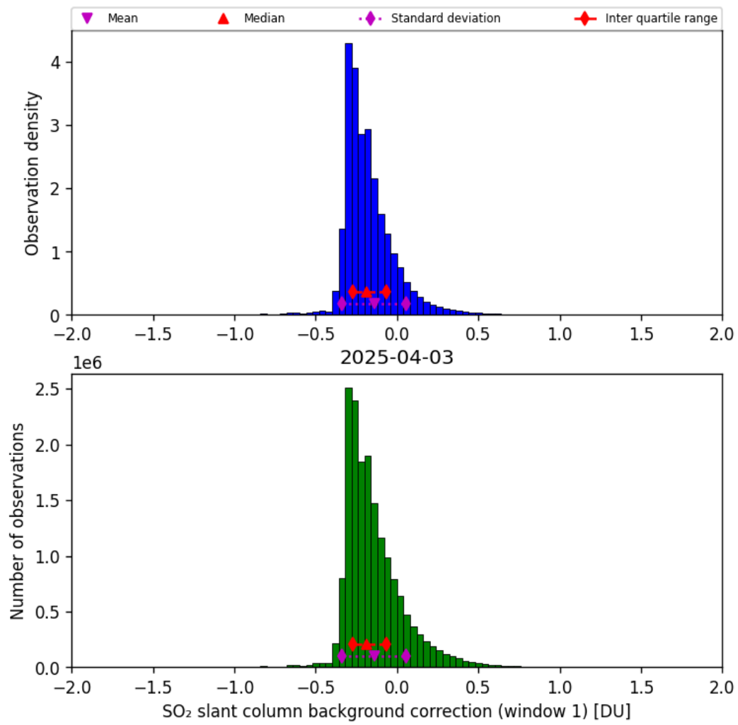
Figure 66: Histogram of “SO 2 slant column background correction (window 1)” for 2025-04-03 to 2025-04-04
