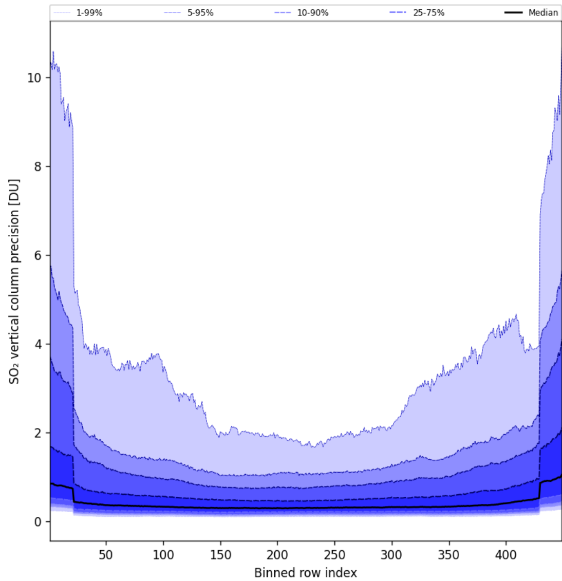
Figure 86: Along track statistics of “SO 2 vertical column precision” for 2025-04-03 to 2025-04-04
