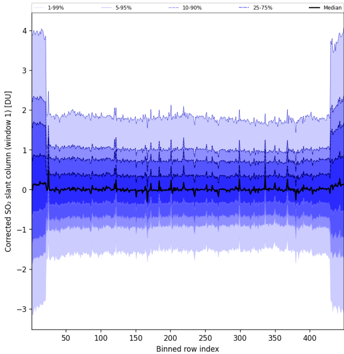
Figure 92: Along track statistics of “Corrected SO 2 slant column (window 1)” for 2025-04-03 to 2025-04-04
