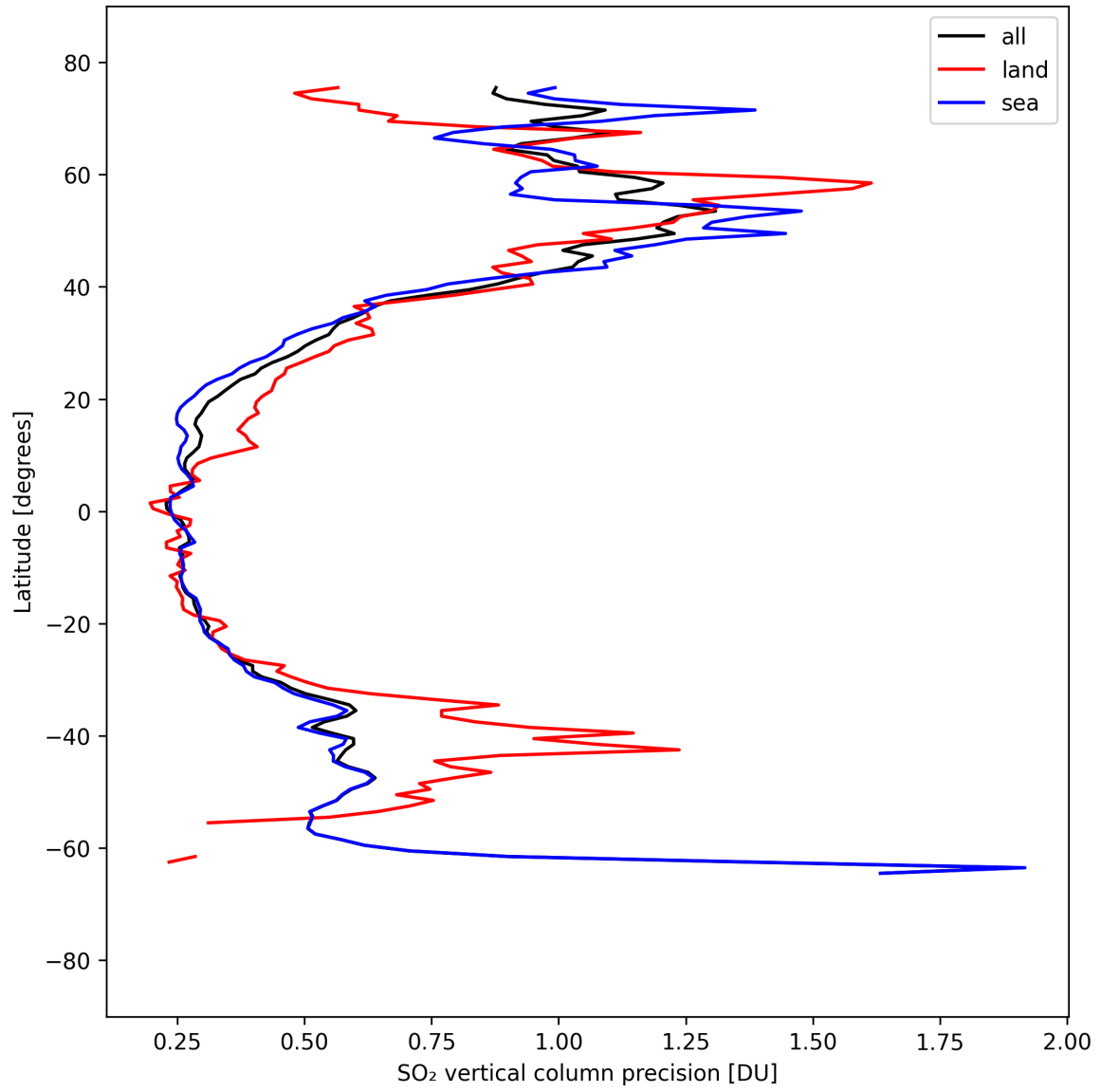
Figure 32: Zonal average of “SO 2 vertical column precision” for 2025-04-03 to 2025-04-04.
