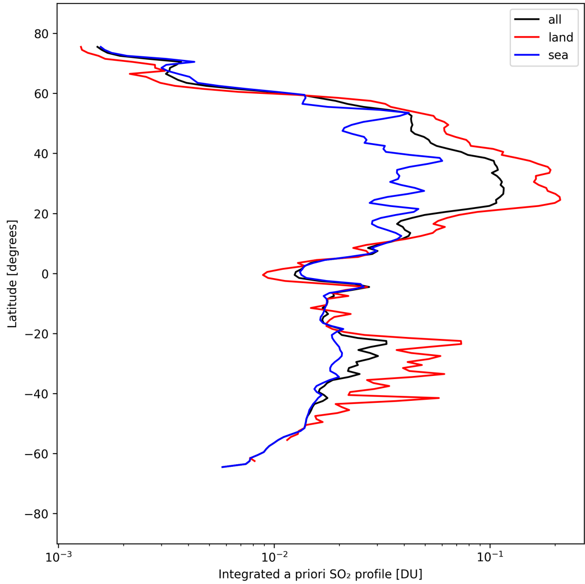
Figure 49: Zonal average of “Integrated a priori SO 2 profile” for 2025-04-03 to 2025-04-04.
