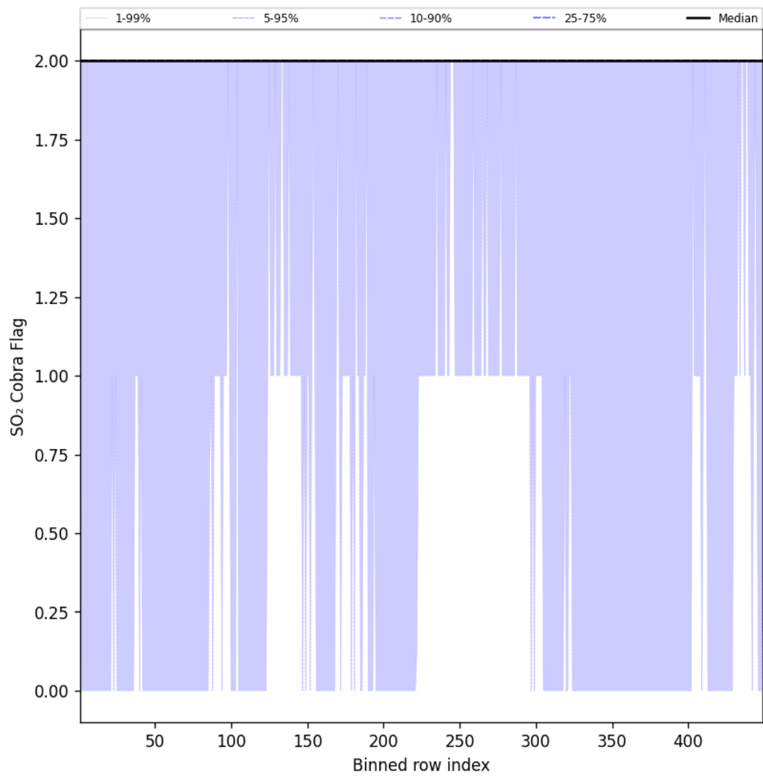
Figure 102: Along track statistics of “SO 2 Cobra Flag” for 2025-04-03 to 2025-04-04
