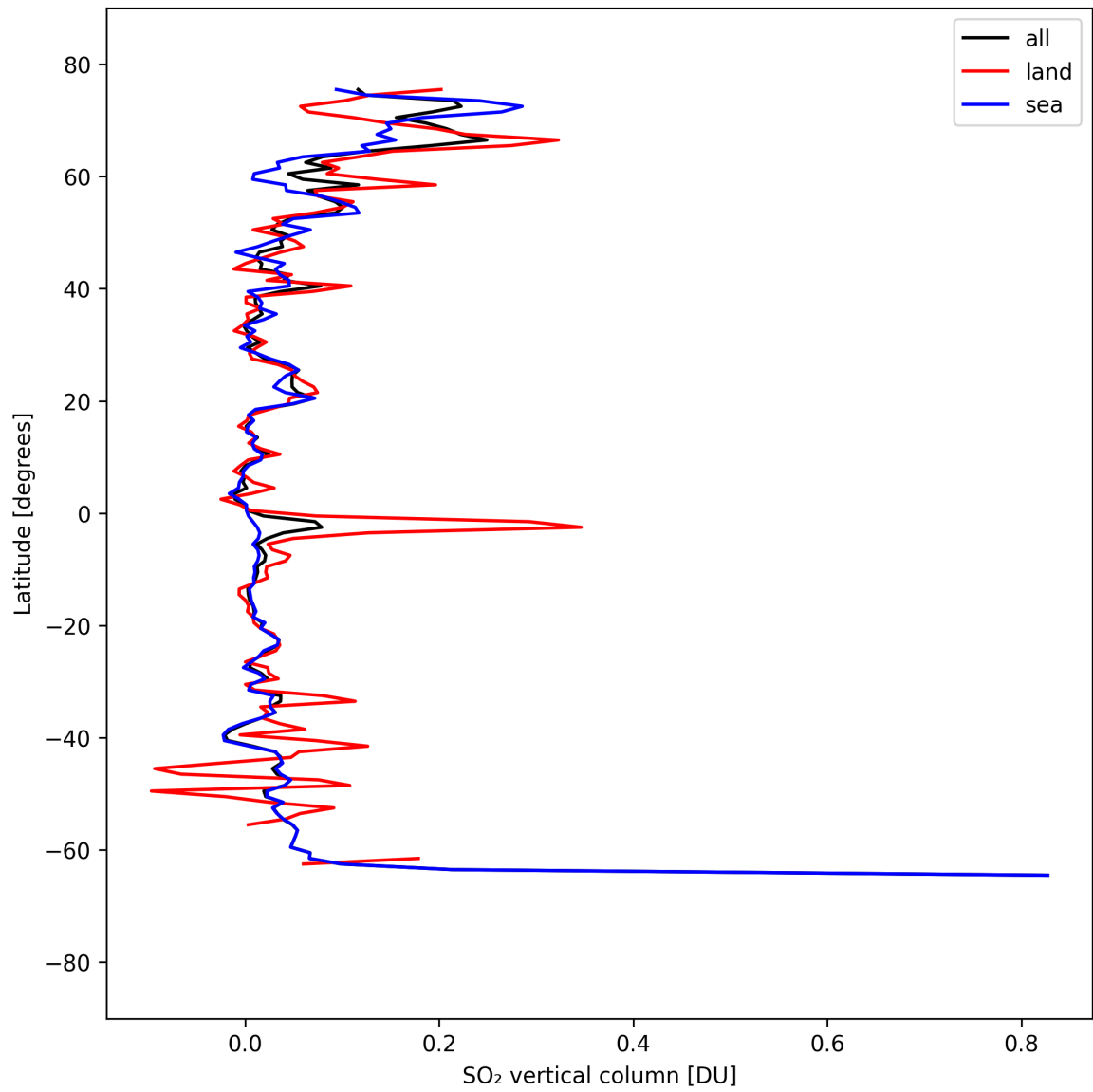
Figure 31: Zonal average of “SO 2 vertical column” for 2025-04-03 to 2025-04-04.
