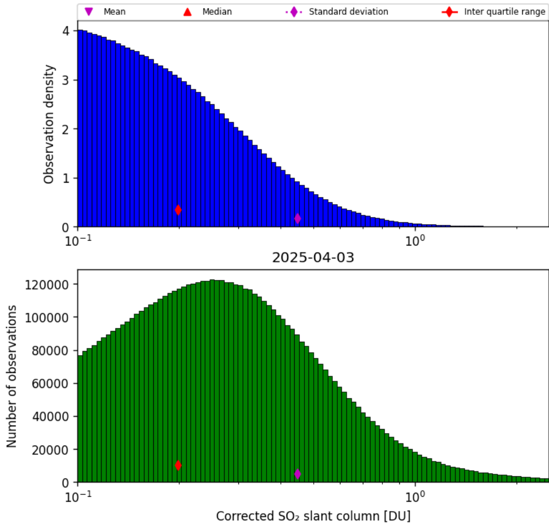
Figure 60: Histogram of “Corrected SO 2 slant column” for 2025-04-03 to 2025-04-04
