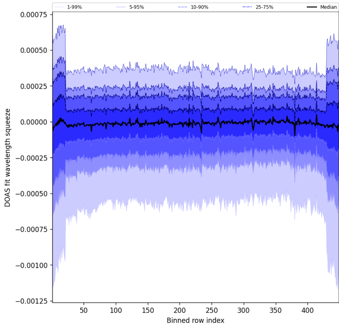
Figure 105: Along track statistics of “DOAS fit wavelength squeeze” for 2025-04-03 to 2025-04-04
