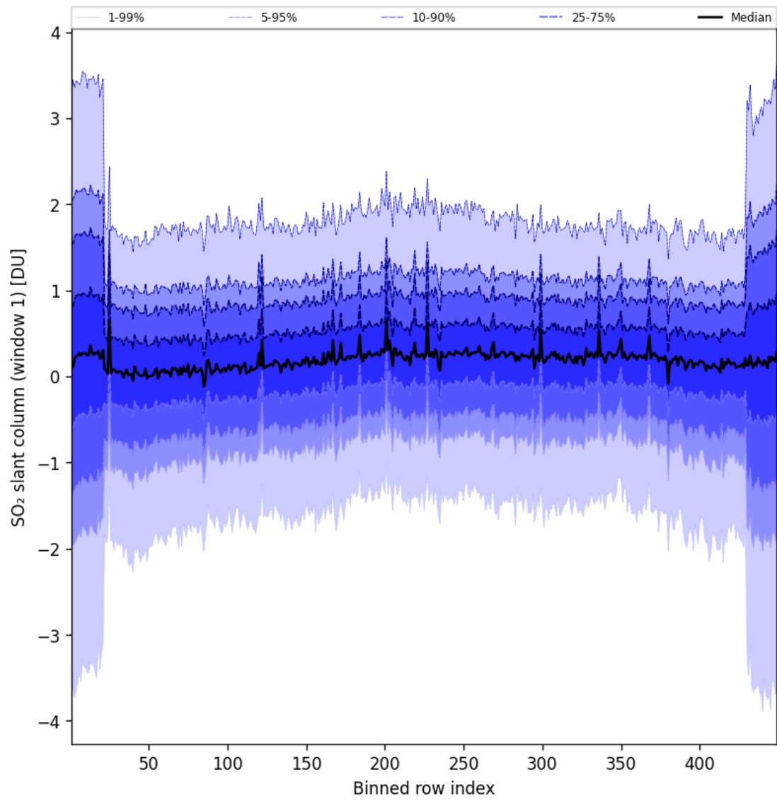
Figure 90: Along track statistics of “SO 2 slant column (window 1)” for 2025-04-03 to 2025-04-04
