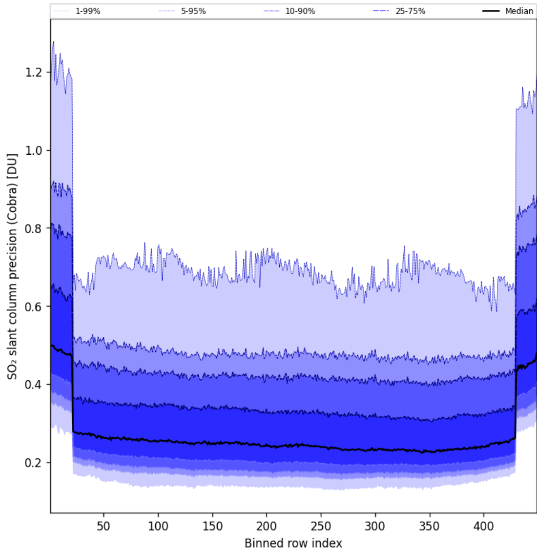
Figure 89: Along track statistics of “SO 2 slant column precision (Cobra)” for 2025-04-03 to 2025-04-04
