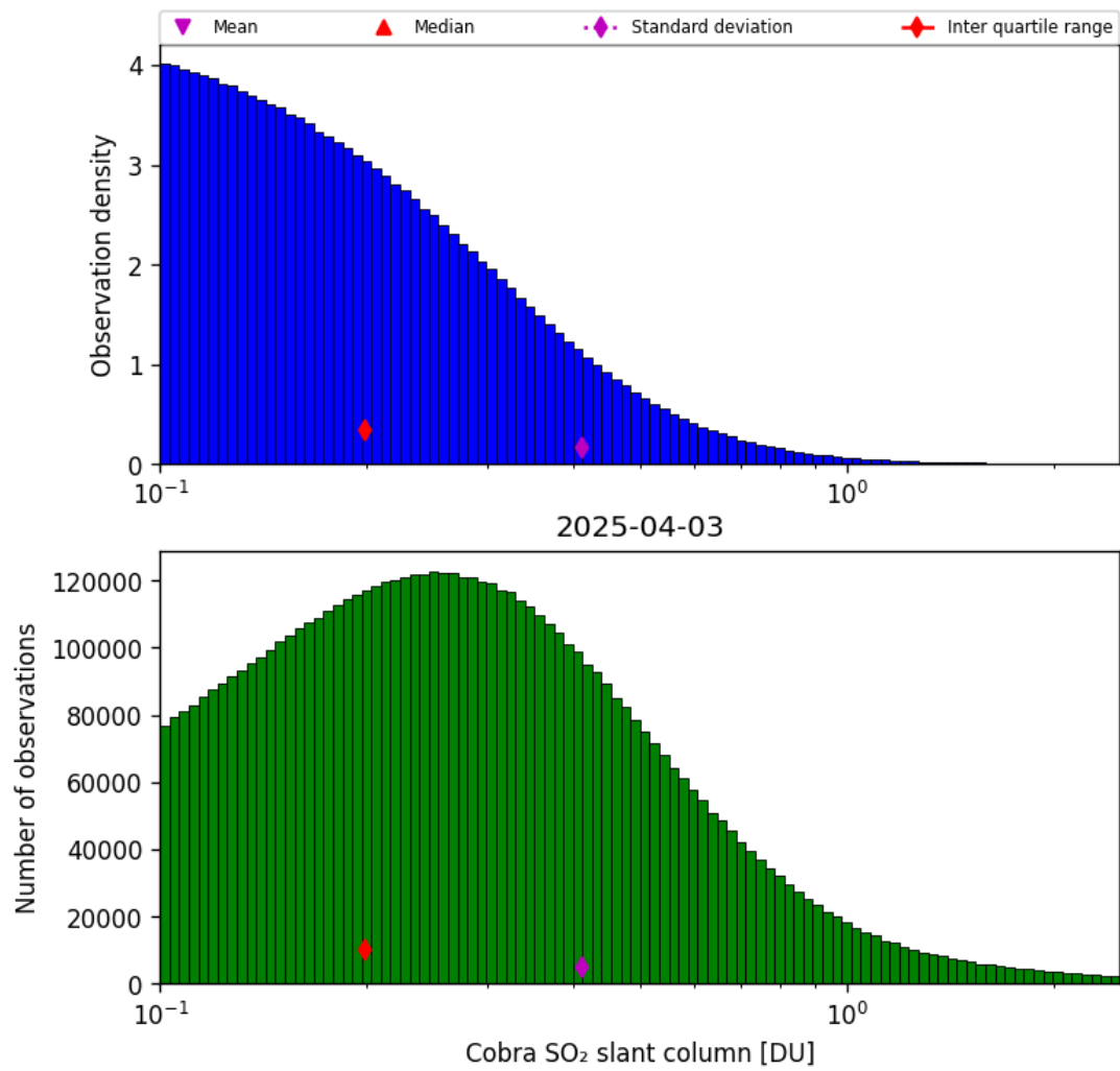
Figure 61: Histogram of “Cobra SO 2 slant column” for 2025-04-03 to 2025-04-04
