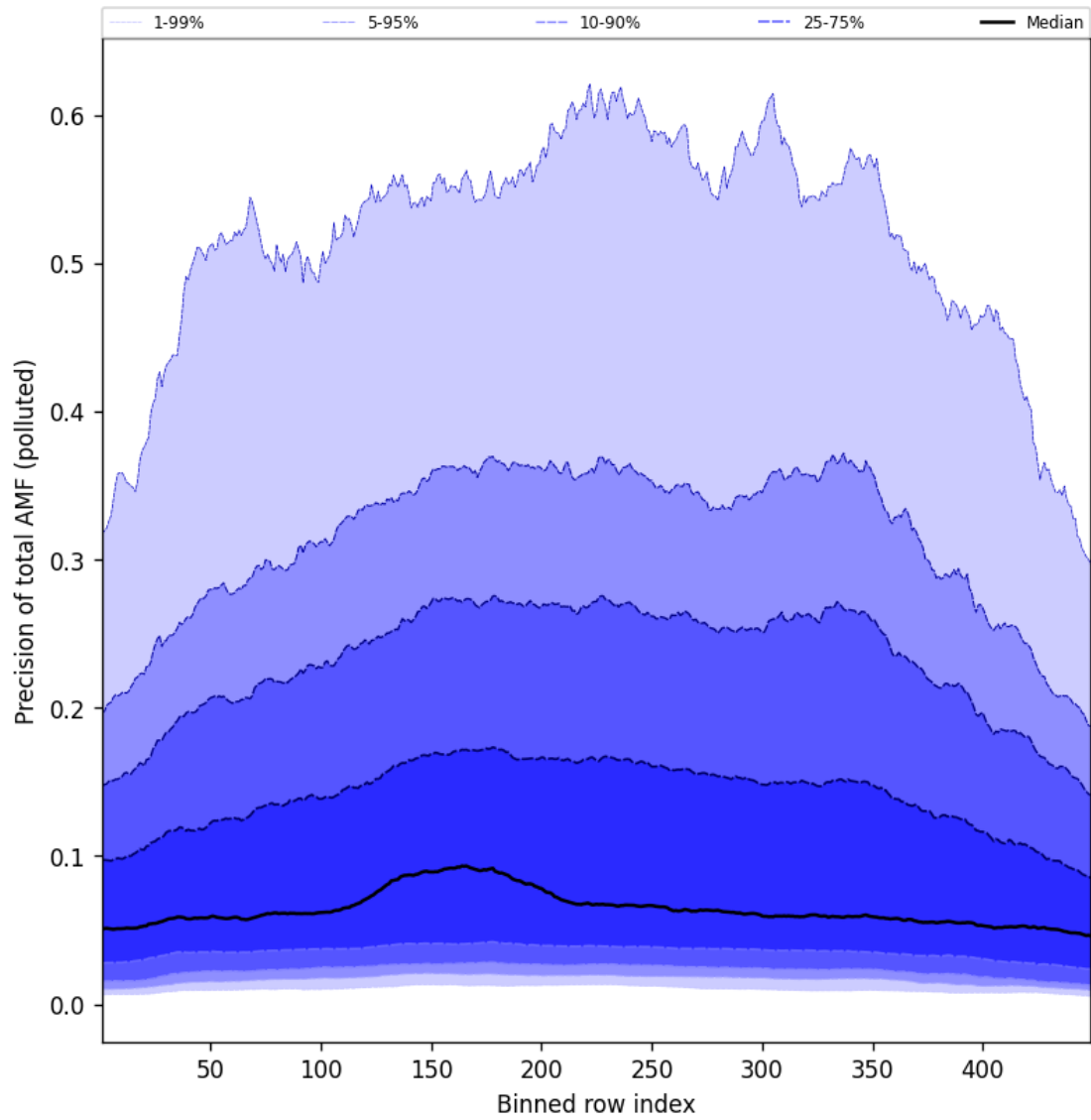
Figure 108: Along track statistics of “Precision of total AMF (polluted)” for 2025-04-03 to 2025-04-04
