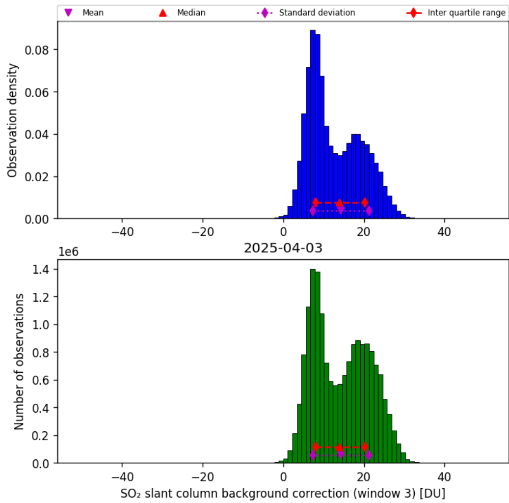
Figure 74: Histogram of “SO 2 slant column background correction (window 3)” for 2025-04-03 to 2025-04-04
