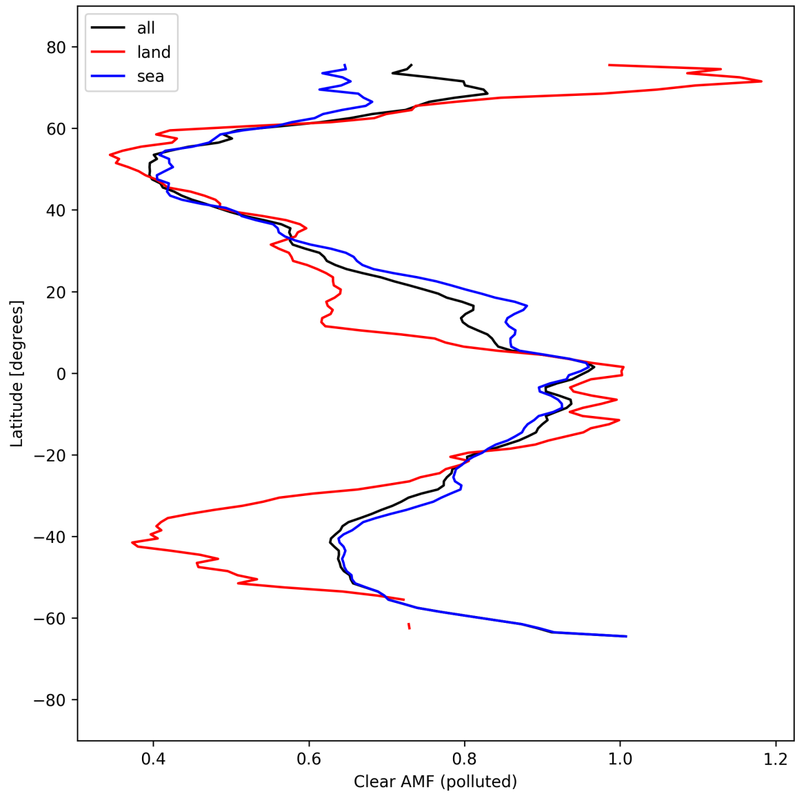
Figure 55: Zonal average of “Clear AMF (polluted)” for 2025-04-03 to 2025-04-04.
