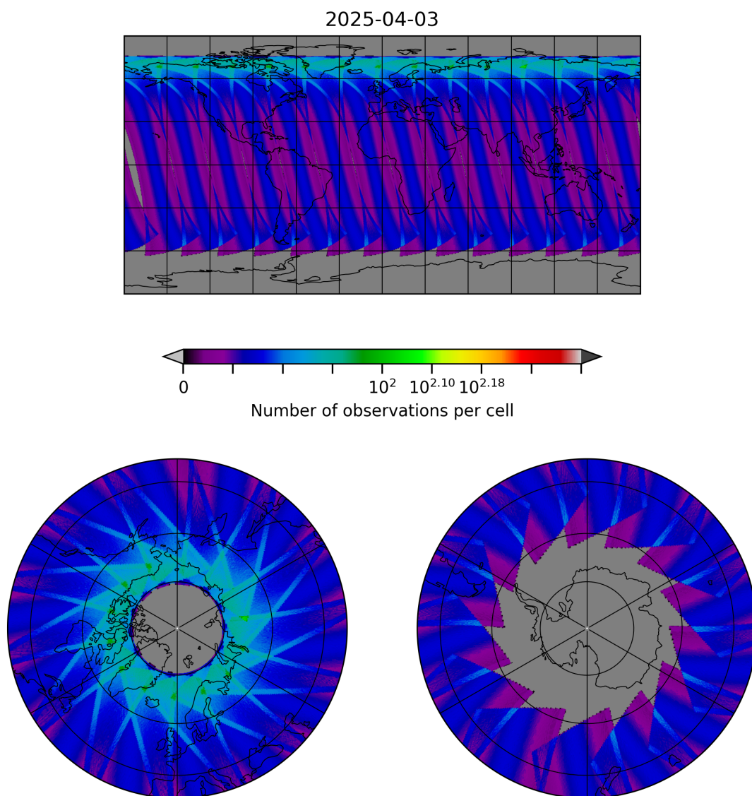
Figure 29: Map of the number of observations for 2025-04-03 to 2025-04-04
