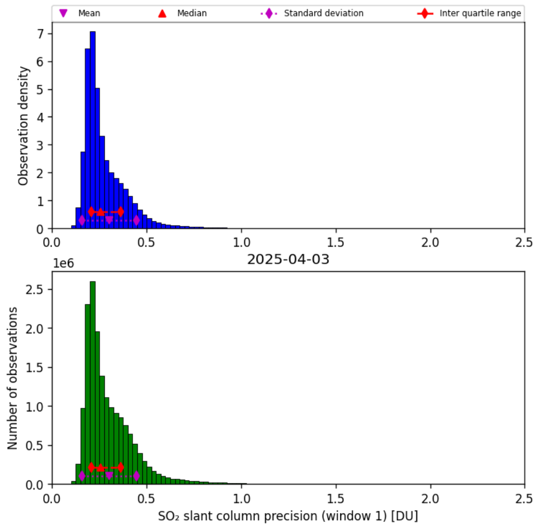
Figure 64: Histogram of “SO 2 slant column precision (window 1)” for 2025-04-03 to 2025-04-04
