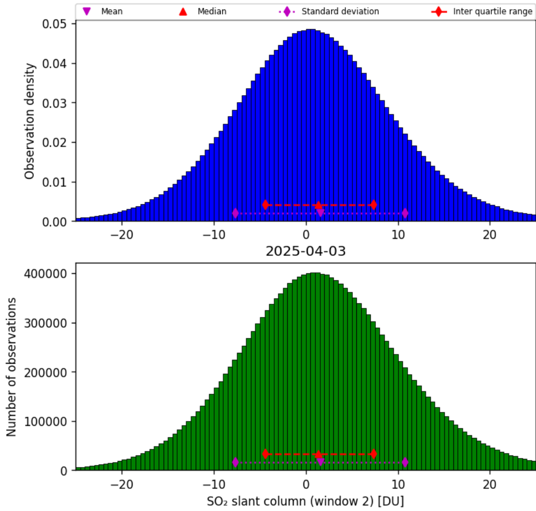
Figure 67: Histogram of “SO 2 slant column (window 2)” for 2025-04-03 to 2025-04-04
