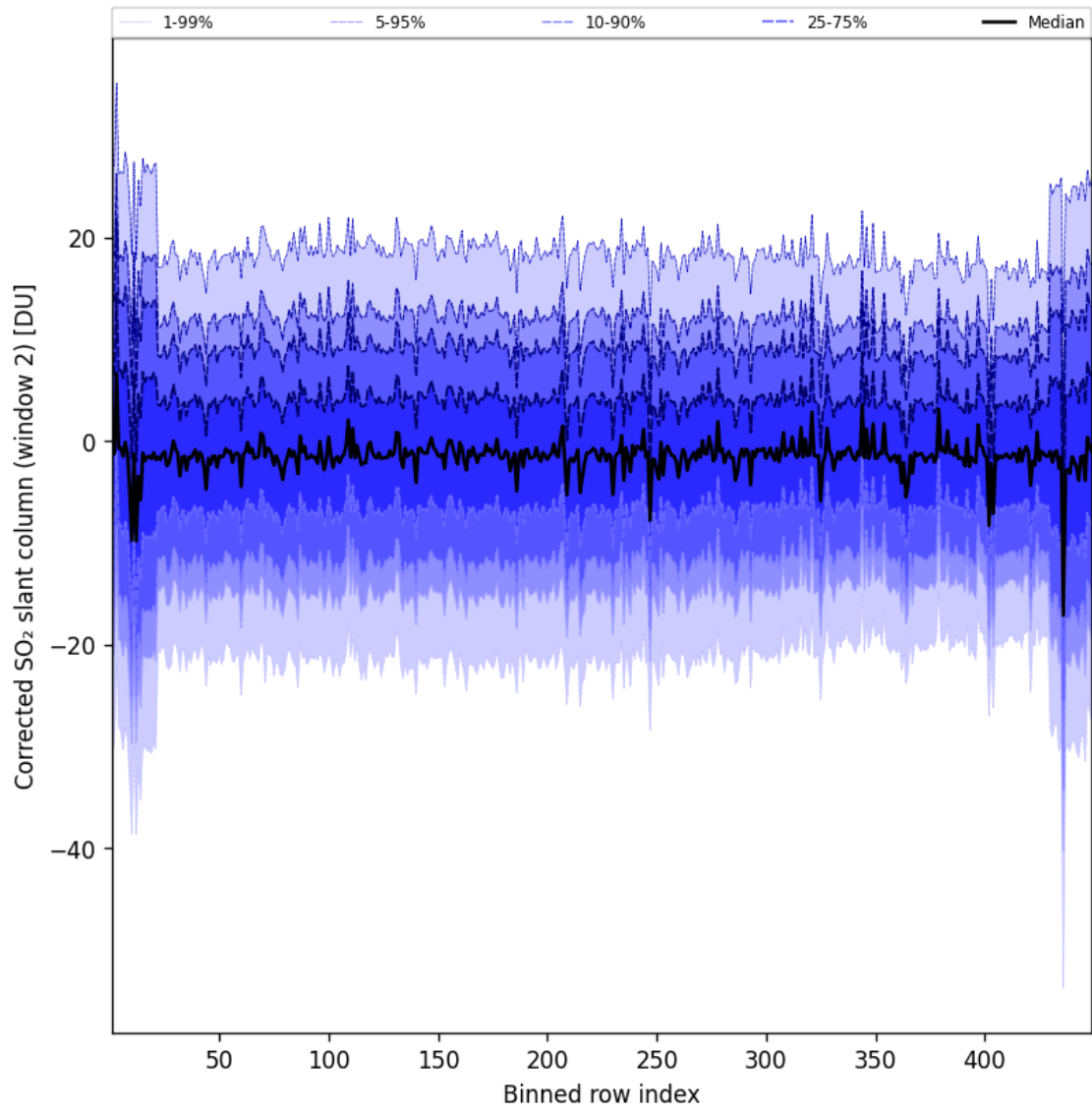
Figure 96: Along track statistics of “Corrected SO 2 slant column (window 2)” for 2025-04-03 to 2025-04-04
