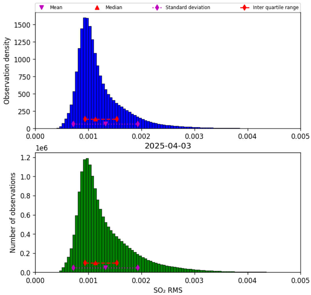
Figure 79: Histogram of “SO 2 RMS” for 2025-04-03 to 2025-04-04
