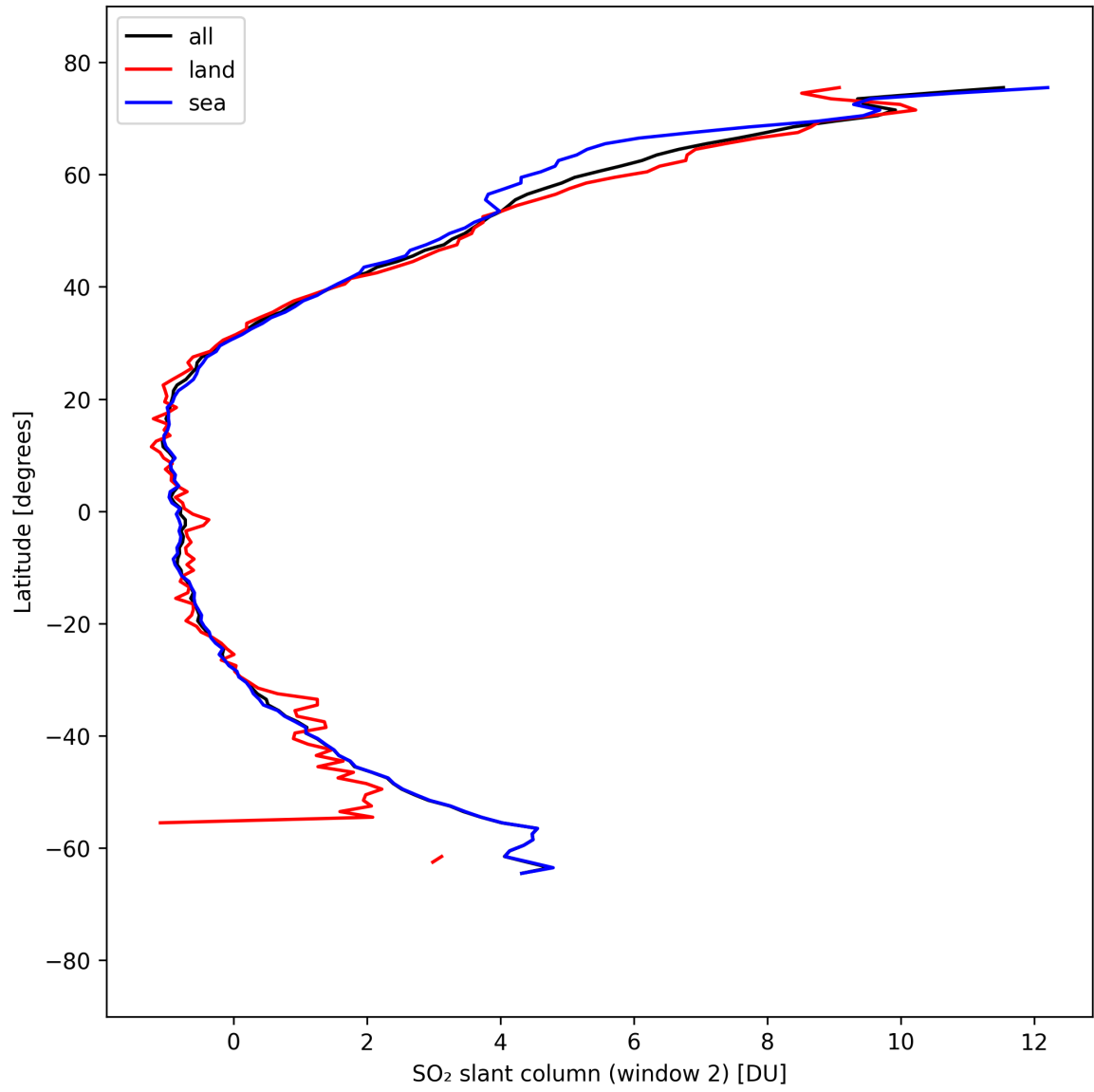
Figure 40: Zonal average of “SO 2 slant column (window 2)” for 2025-04-03 to 2025-04-04.
