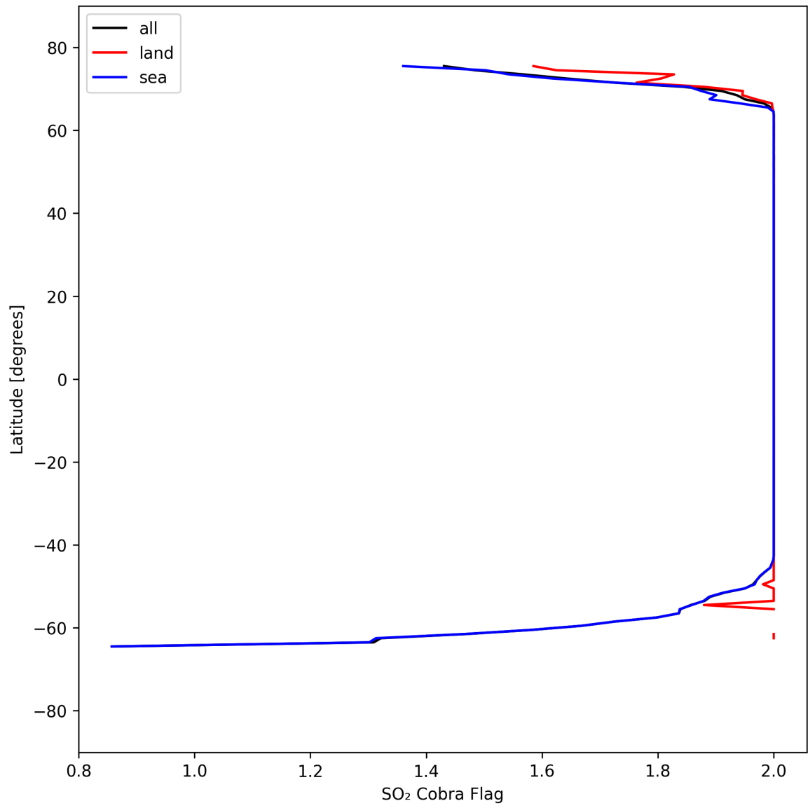
Figure 48: Zonal average of "SO 2 Cobra Flag" for 2025-04-03 to 2025-04-04.
