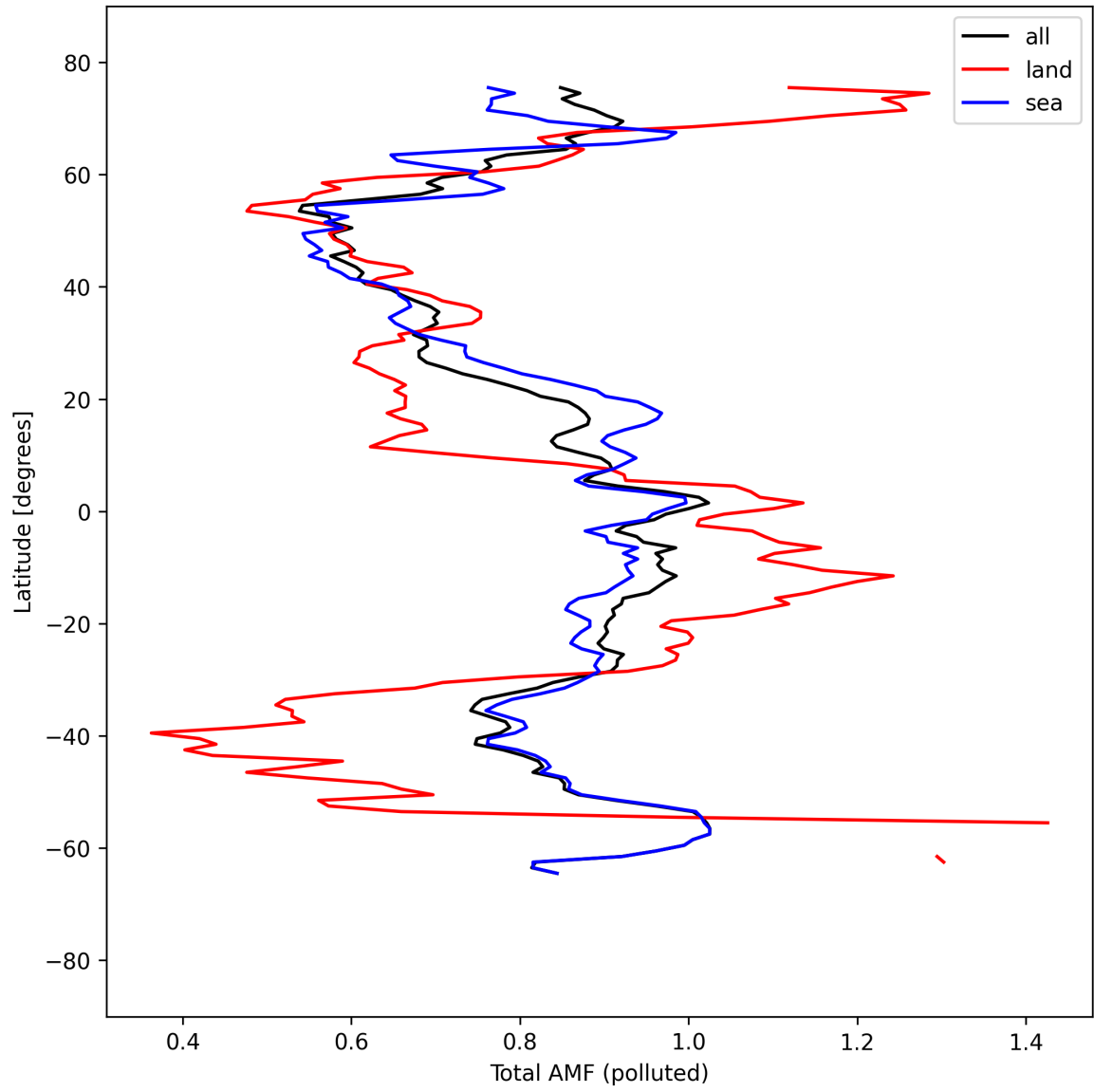
Figure 53: Zonal average of “Total AMF (polluted)” for 2025-04-03 to 2025-04-04.
