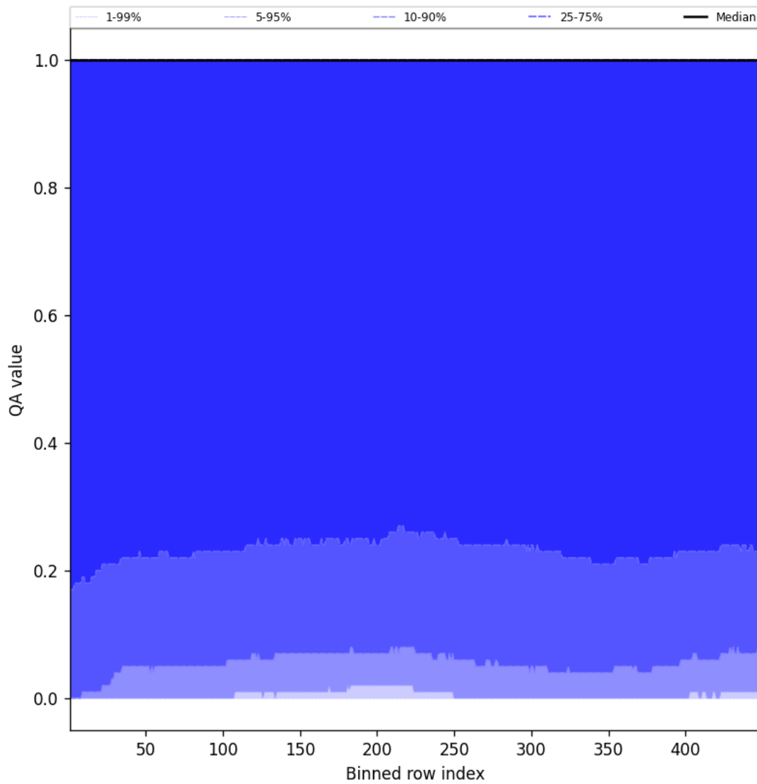
Figure 84: Along track statistics of “QA value” for 2025-04-03 to 2025-04-04
