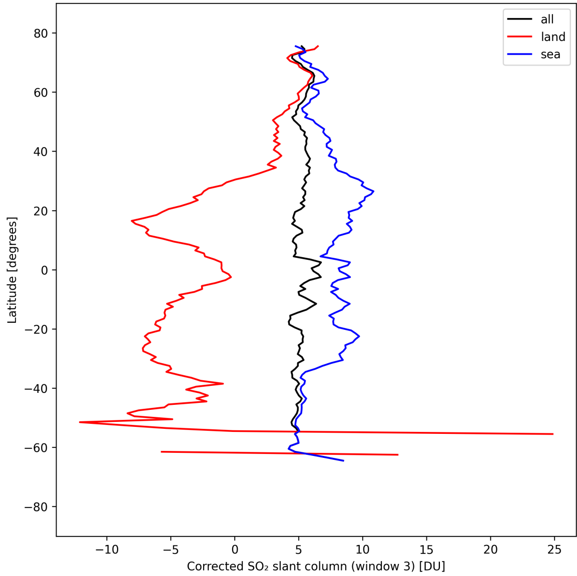
Figure 46: Zonal average of “Corrected SO 2 slant column (window 3)” for 2025-04-03 to 2025-04-04.
