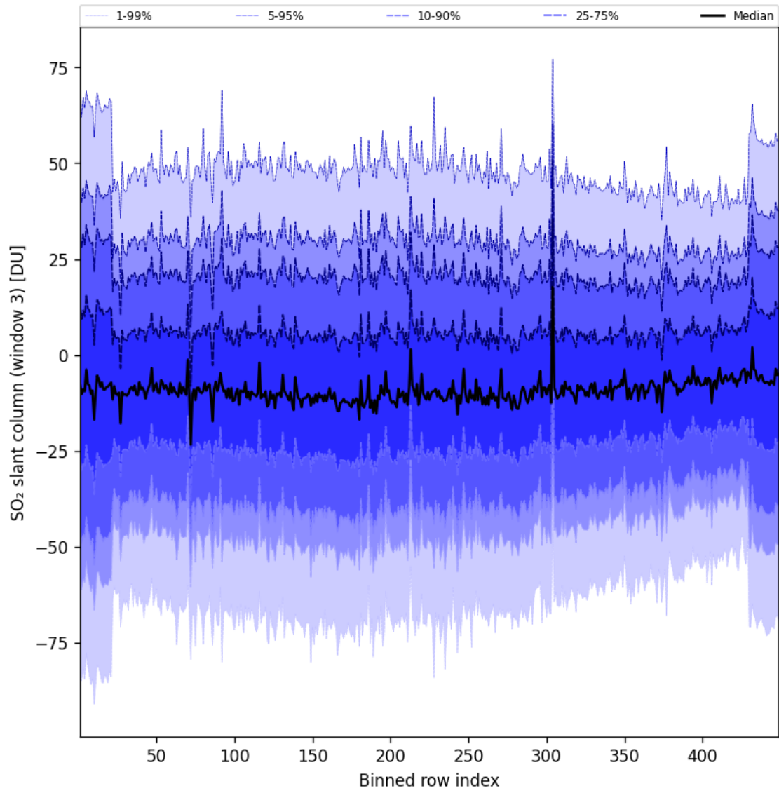
Figure 98: Along track statistics of “SO 2 slant column (window 3)” for 2025-04-03 to 2025-04-04
