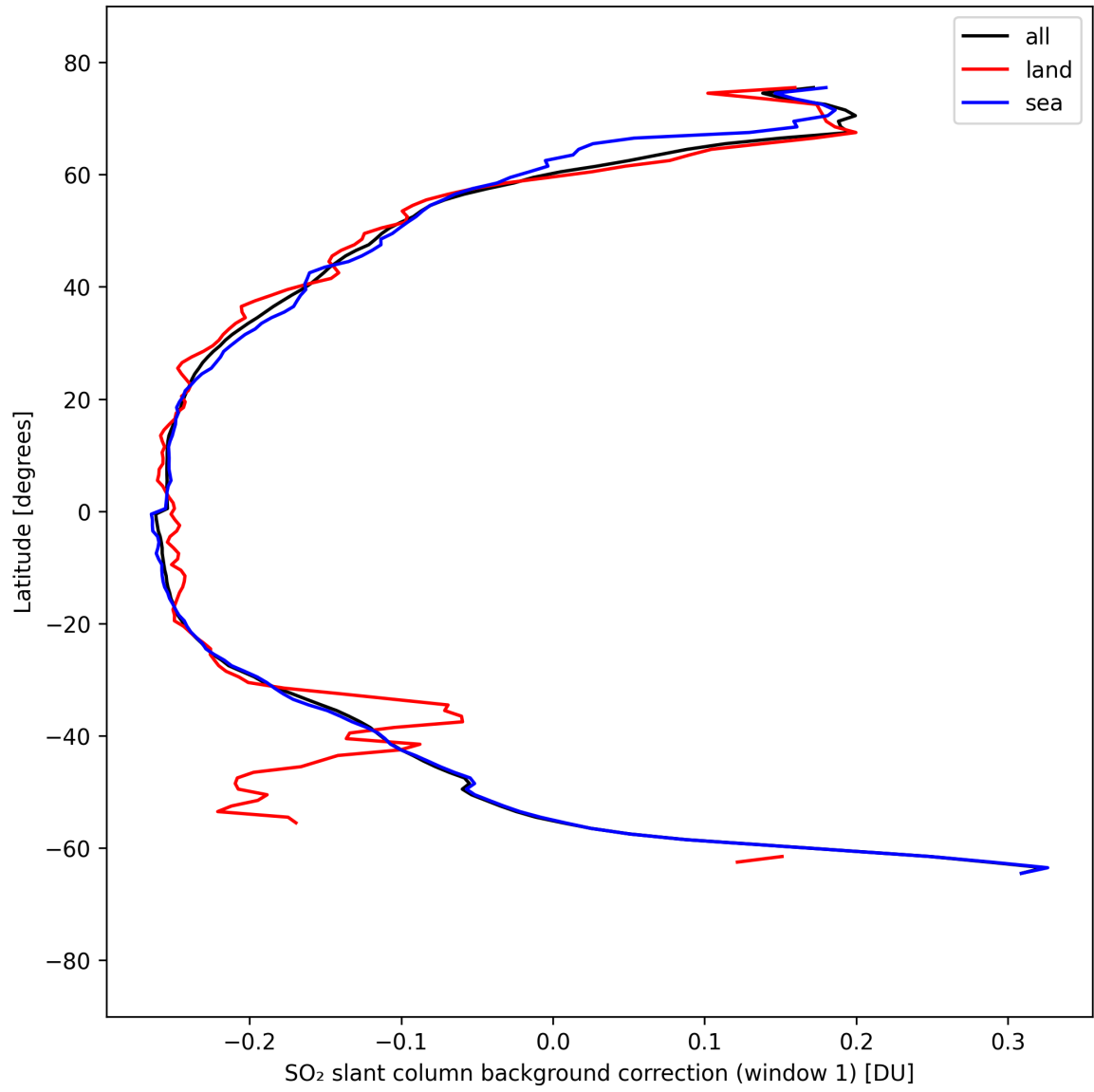
Figure 39: Zonal average of “SO 2 slant column background correction (window 1)” for 2025-04-03 to 2025-04-04.
