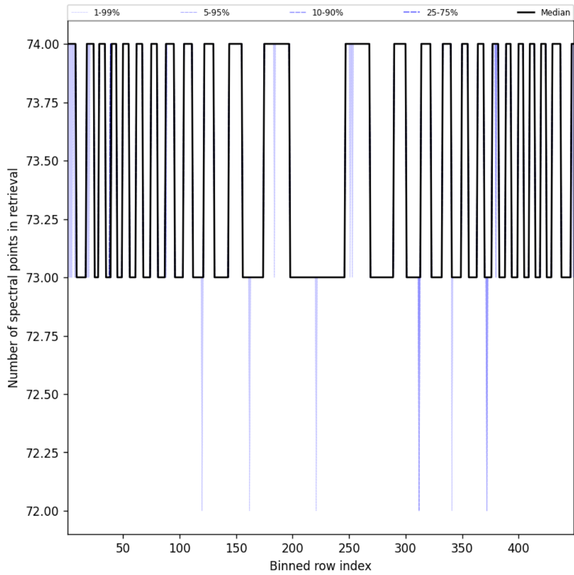
Figure 110: Along track statistics of “Number of spectral points in retrieval” for 2025-04-03 to 2025-04-04
