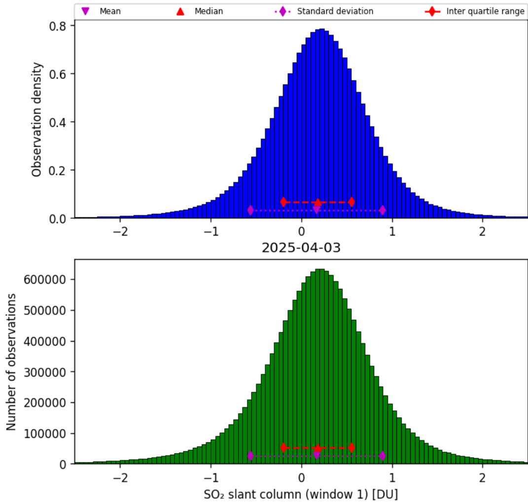
Figure 63: Histogram of “SO 2 slant column (window 1)” for 2025-04-03 to 2025-04-04
