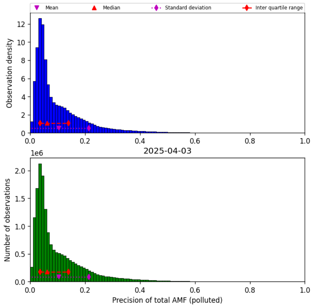
Figure 81: Histogram of “Precision of total AMF (polluted)” for 2025-04-03 to 2025-04-04
