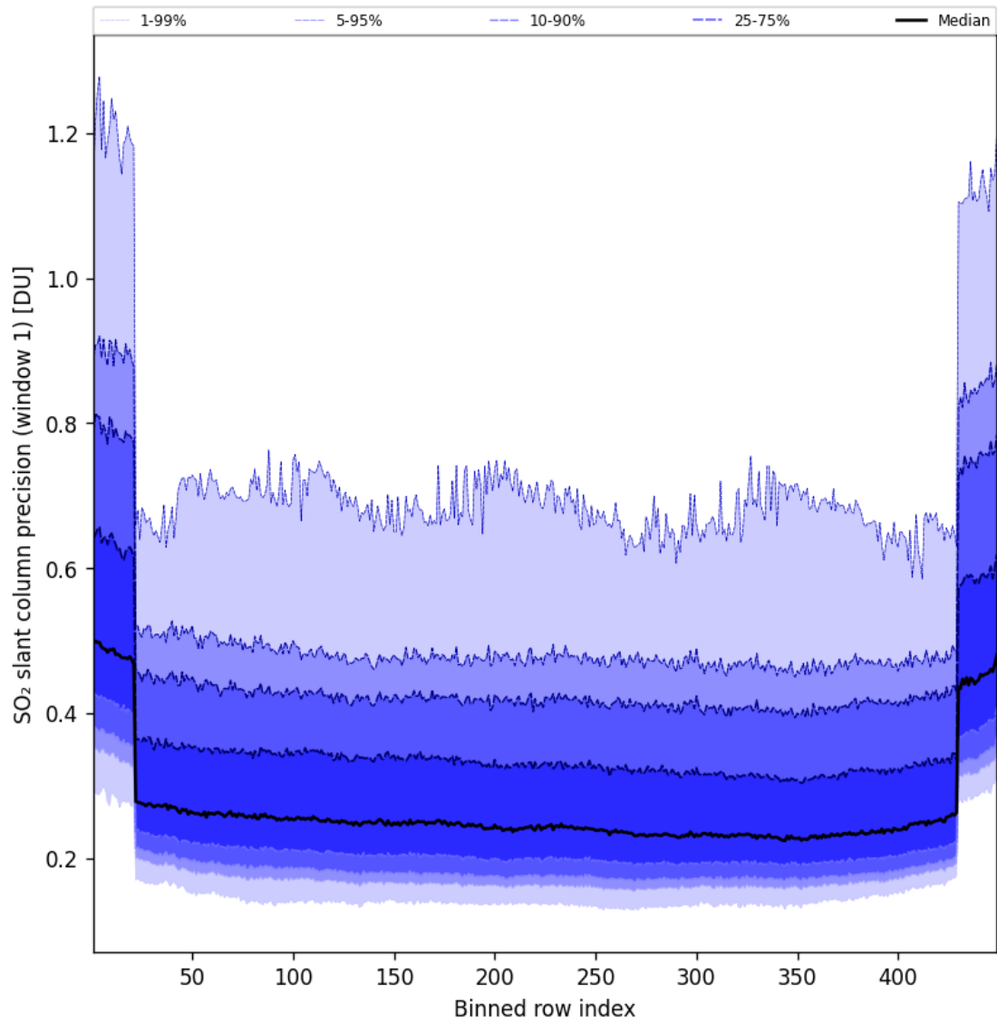
Figure 91: Along track statistics of “SO 2 slant column precision (window 1)” for 2025-04-03 to 2025-04-04
