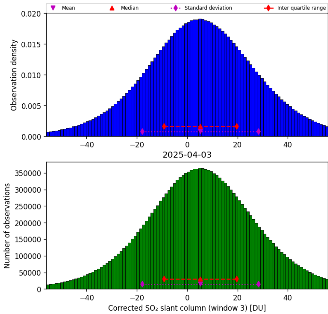
Figure 73: Histogram of “Corrected SO 2 slant column (window 3)” for 2025-04-03 to 2025-04-04
