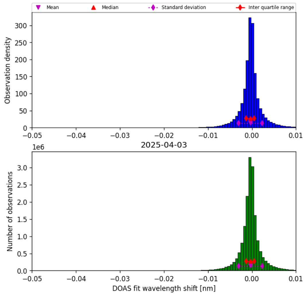
Figure 77: Histogram of “DOAS fit wavelength shift” for 2025-04-03 to 2025-04-04
