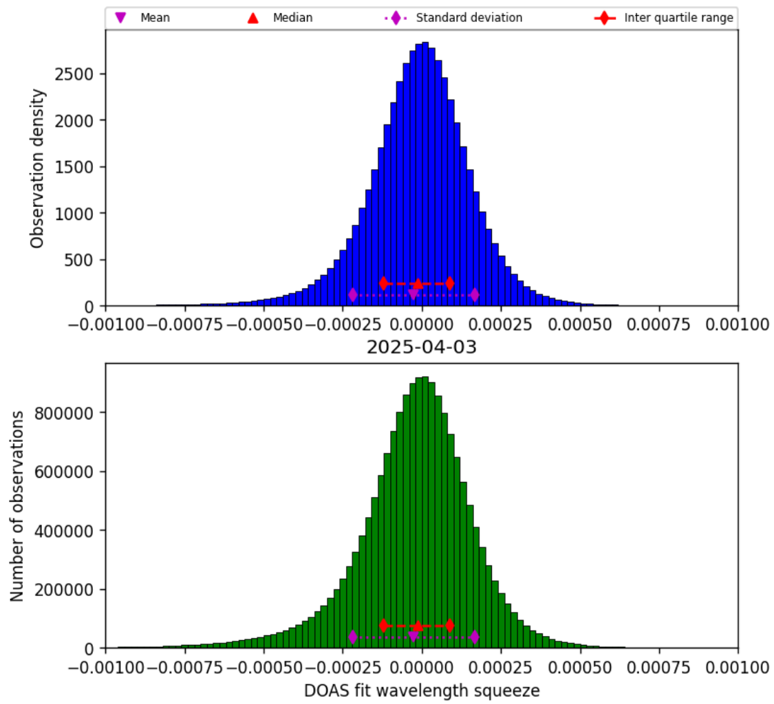
Figure 78: Histogram of “DOAS fit wavelength squeeze” for 2025-04-03 to 2025-04-04
