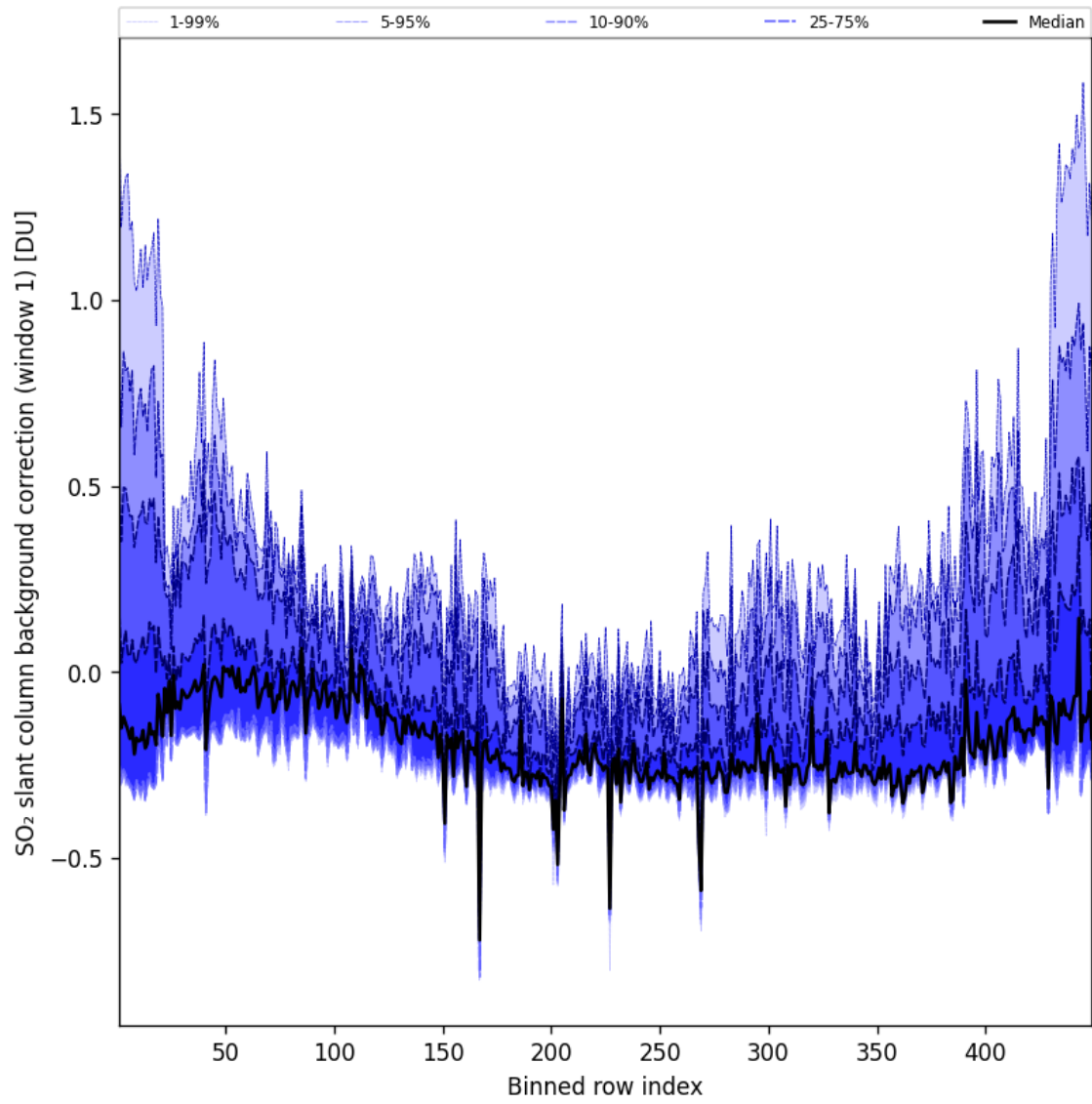
Figure 93: Along track statistics of “SO 2 slant column background correction (window 1)” for 2025-04-03 to 2025-04-04
