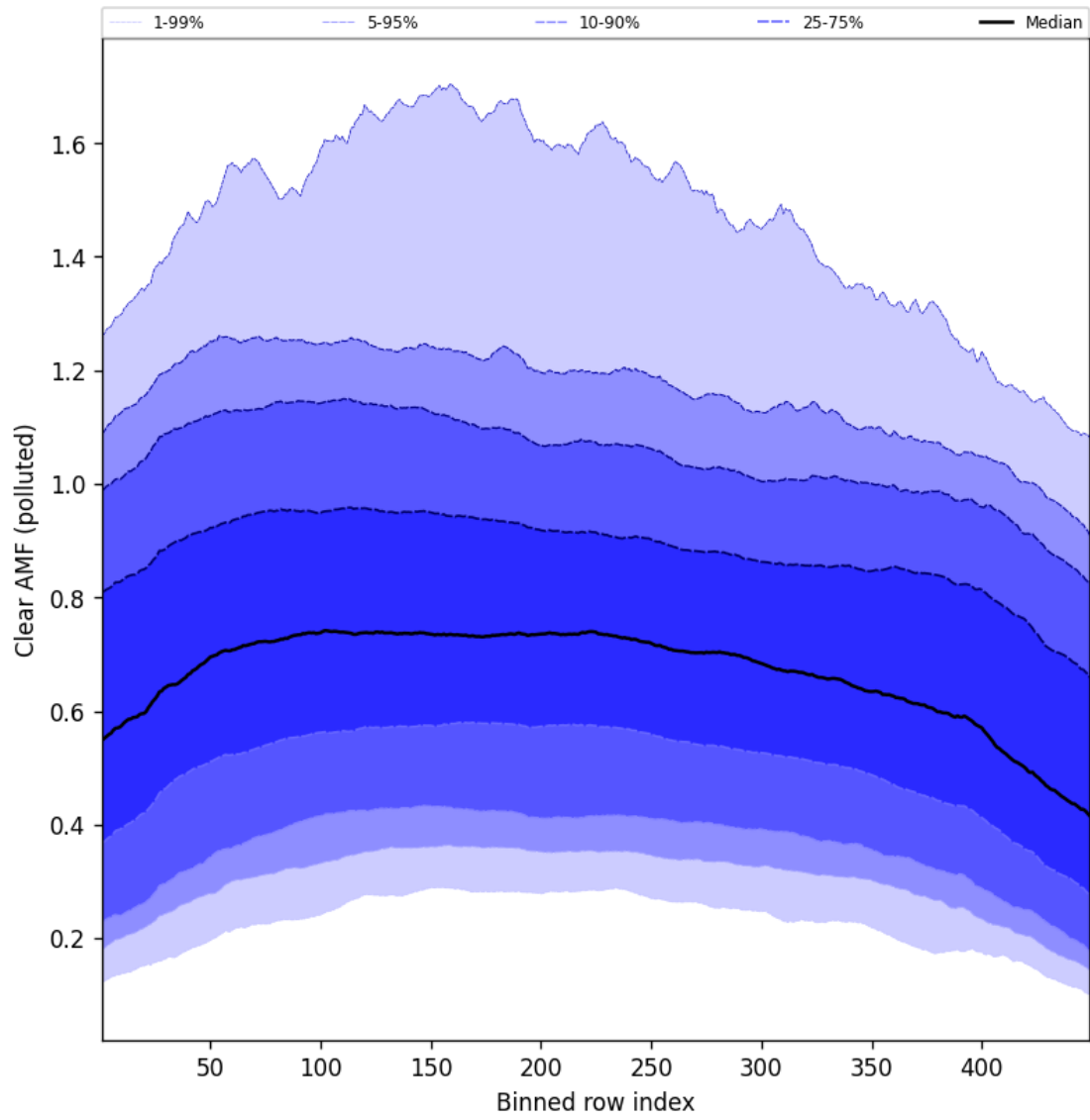
Figure 109: Along track statistics of “Clear AMF (polluted)” for 2025-04-03 to 2025-04-04
