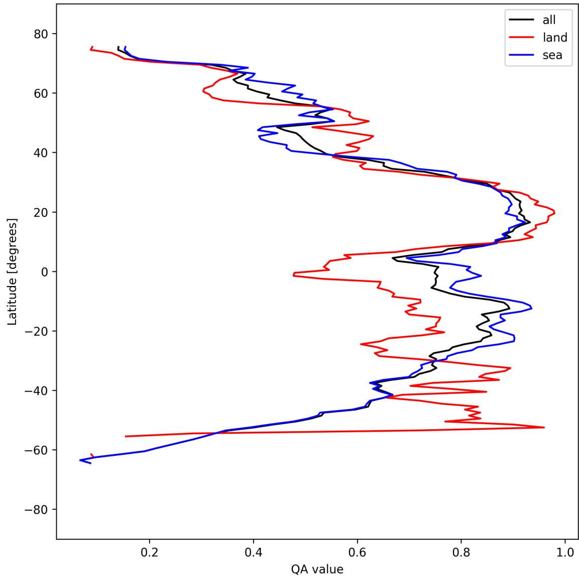
Figure 30: Zonal average of “QA value” for 2025-04-03 to 2025-04-04.
