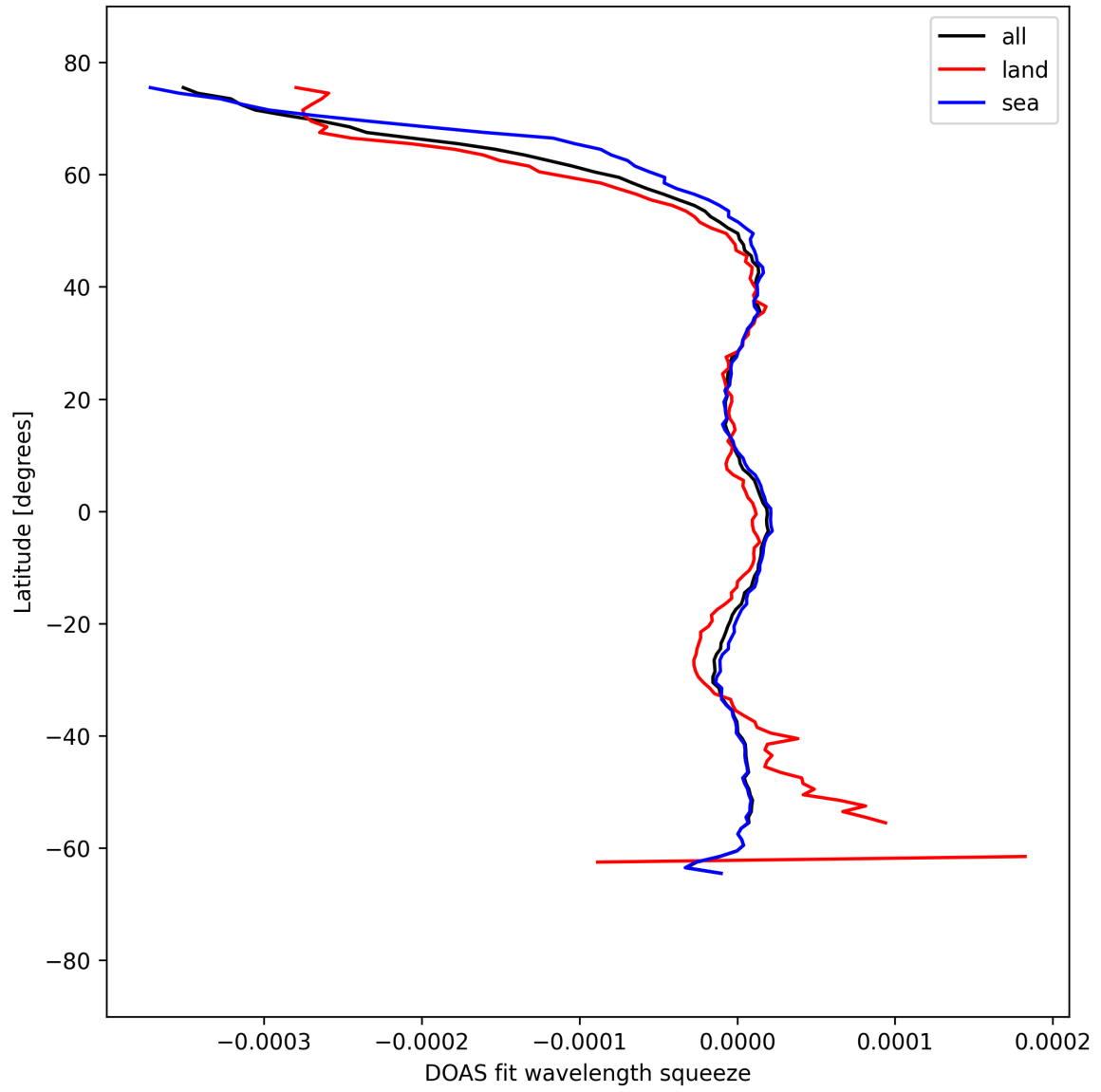
Figure 51: Zonal average of “DOAS fit wavelength squeeze” for 2025-04-03 to 2025-04-04.
