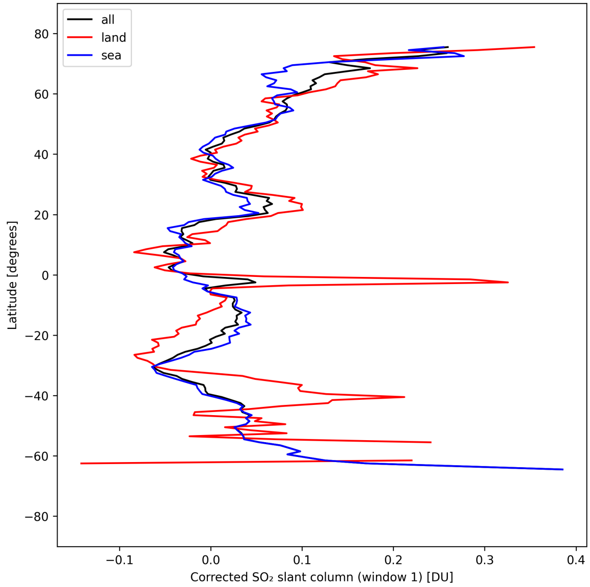
Figure 38: Zonal average of “Corrected SO 2 slant column (window 1)” for 2025-04-03 to 2025-04-04.
