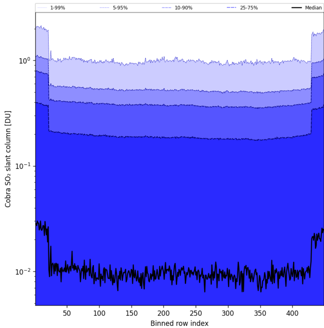
Figure 88: Along track statistics of "Cobra SO 2 slant column" for 2025-04-03 to 2025-04-04
