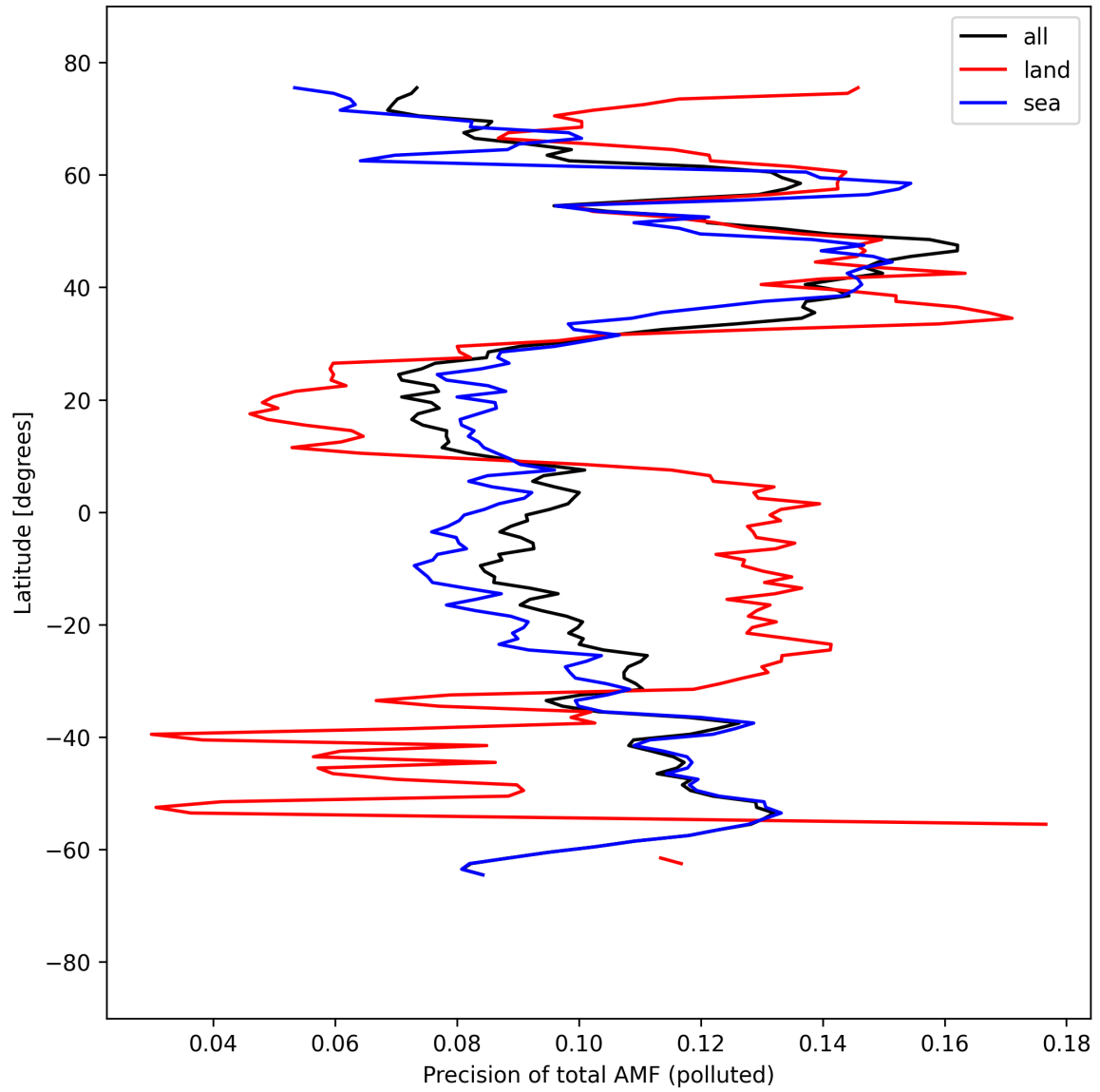
Figure 54: Zonal average of “Precision of total AMF (polluted)” for 2025-04-03 to 2025-04-04.
