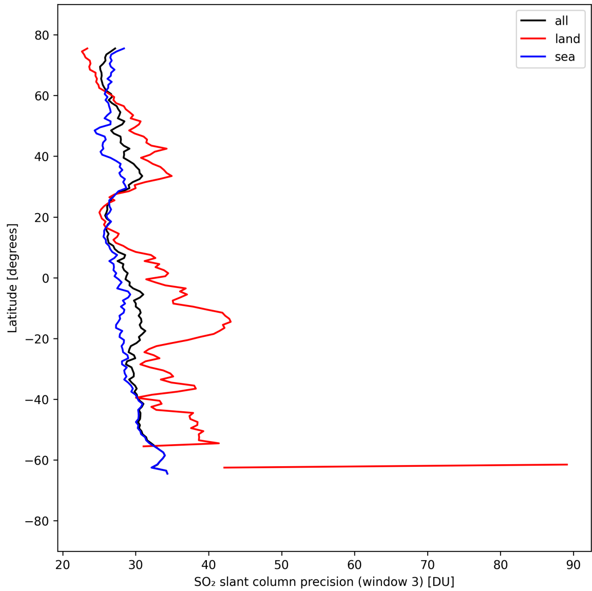
Figure 45: Zonal average of “SO 2 slant column precision (window 3)” for 2025-04-03 to 2025-04-04.
