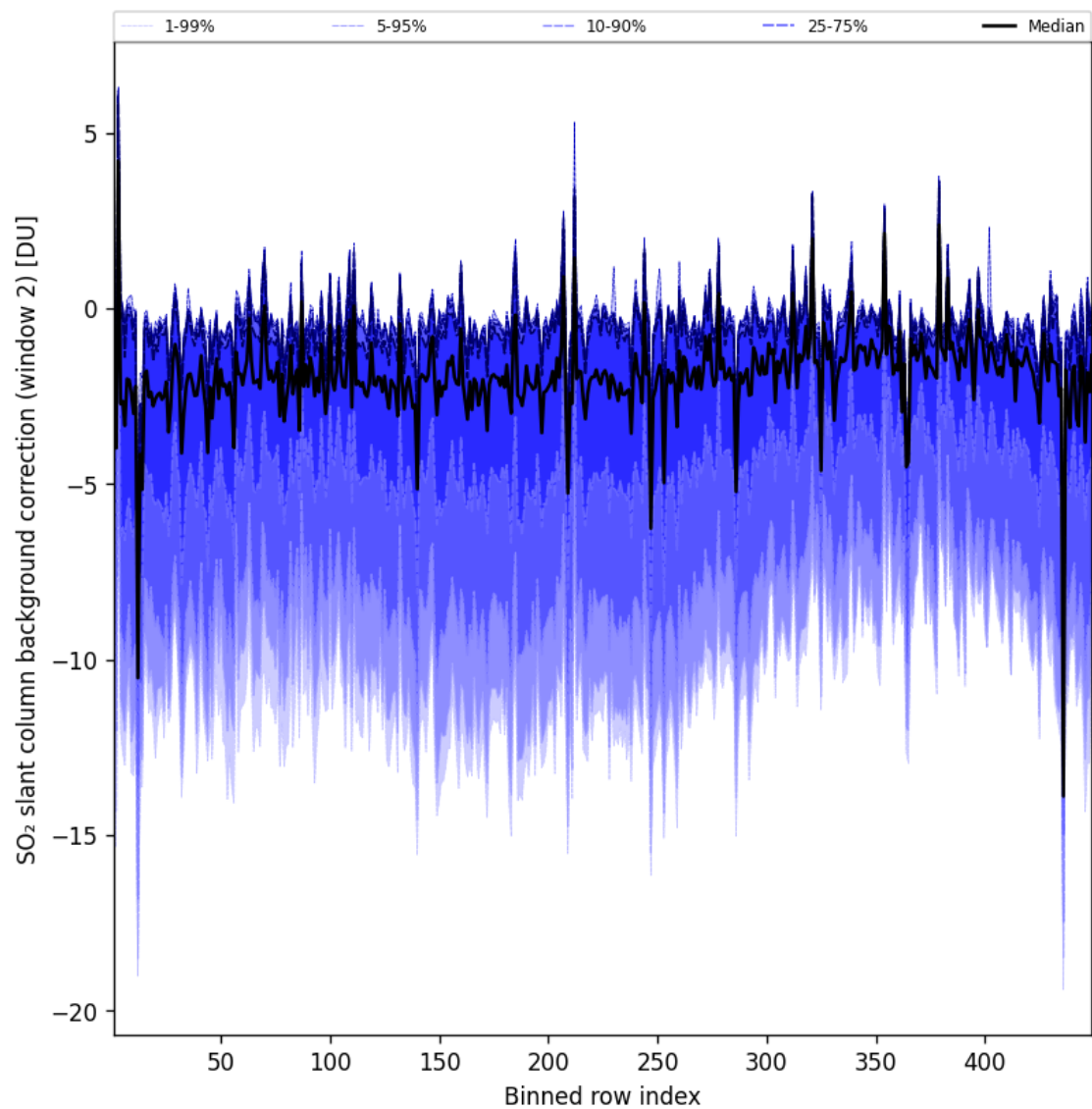
Figure 97: Along track statistics of “SO 2 slant column background correction (window 2)” for 2025-04-03 to 2025-04-04
