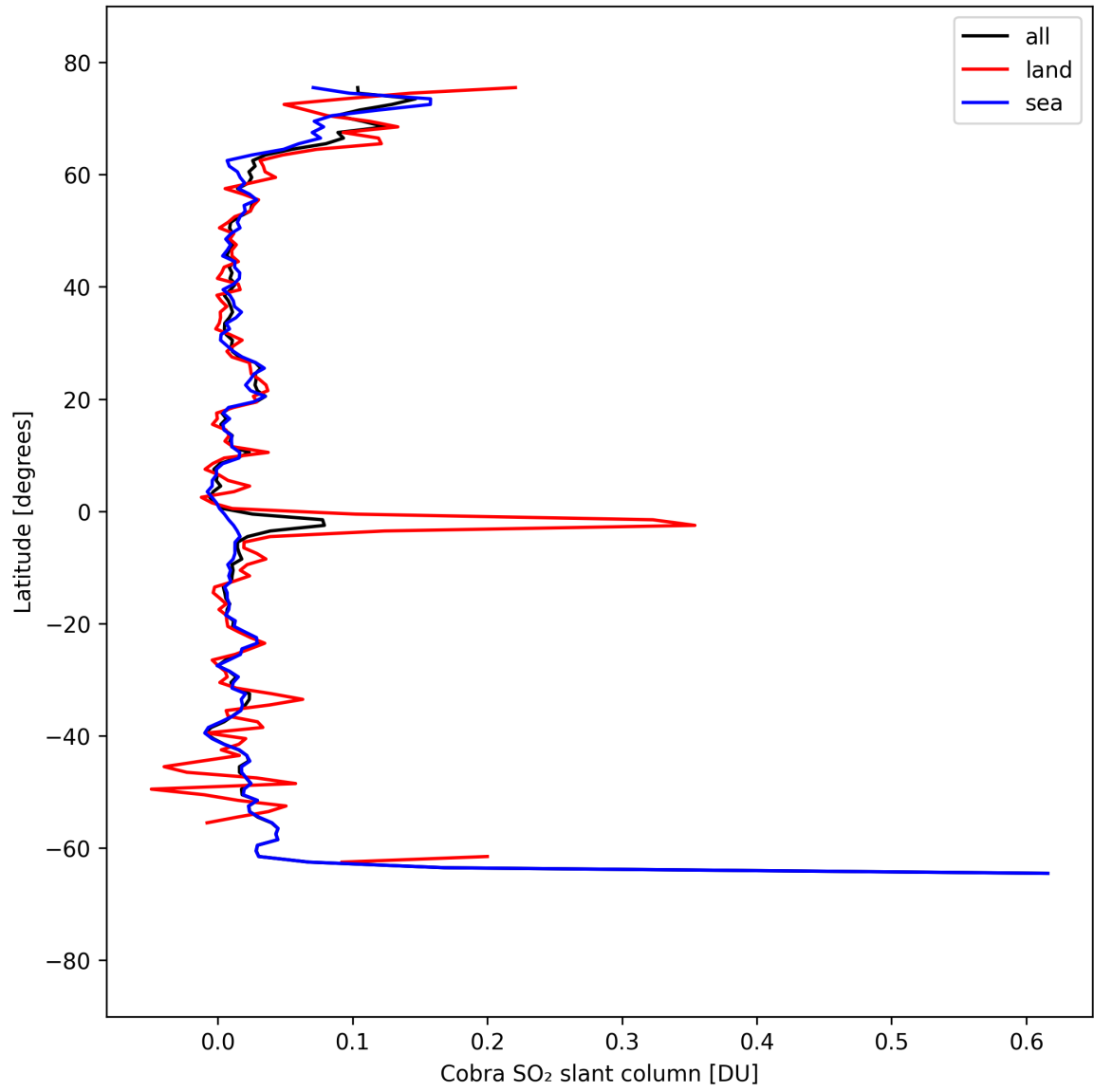
Figure 34: Zonal average of “Cobra SO 2 slant column” for 2025-04-03 to 2025-04-04.
