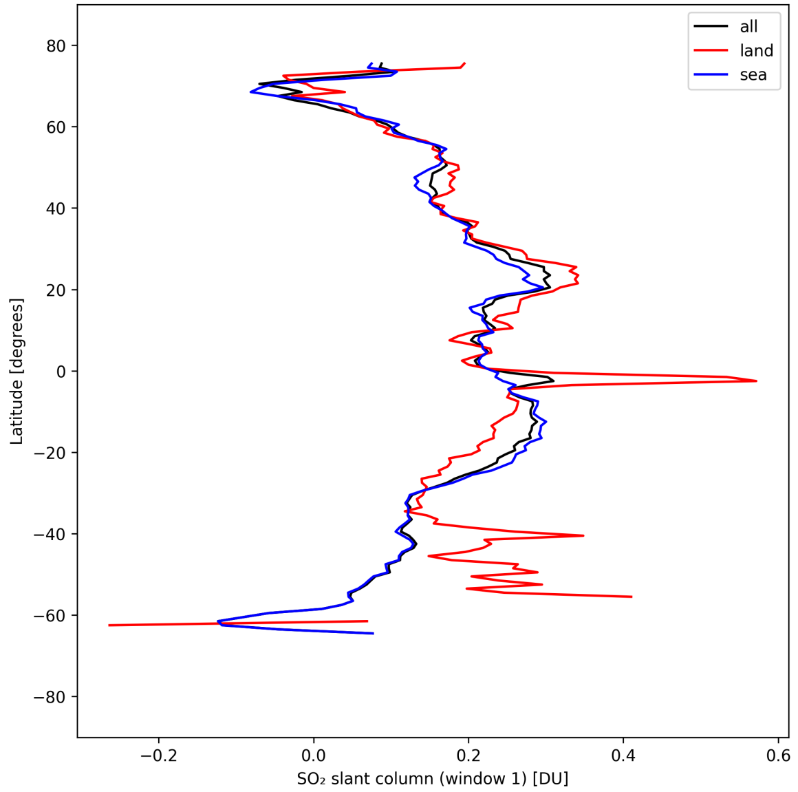
Figure 36: Zonal average of “SO 2 slant column (window 1)” for 2025-04-03 to 2025-04-04.
