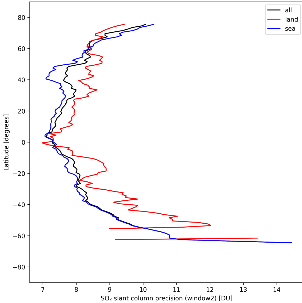
Figure 41: Zonal average of “SO 2 slant column precision (window2)” for 2025-04-03 to 2025-04-04.
