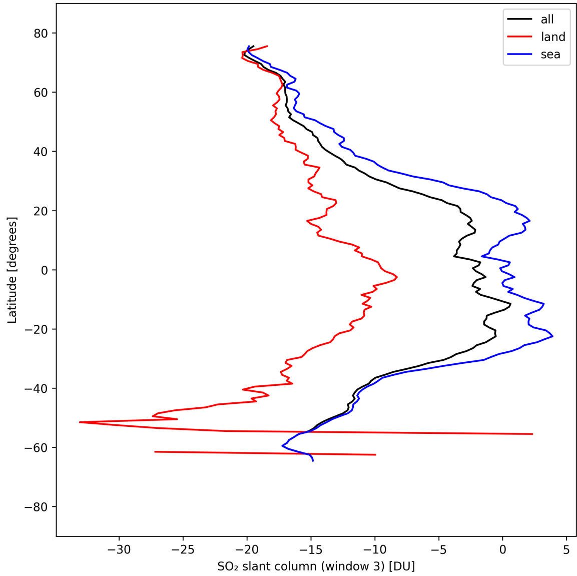
Figure 44: Zonal average of “SO 2 slant column (window 3)” for 2025-04-03 to 2025-04-04.
