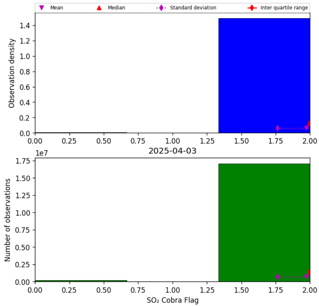
Figure 75: Histogram of “SO 2 Cobra Flag” for 2025-04-03 to 2025-04-04
