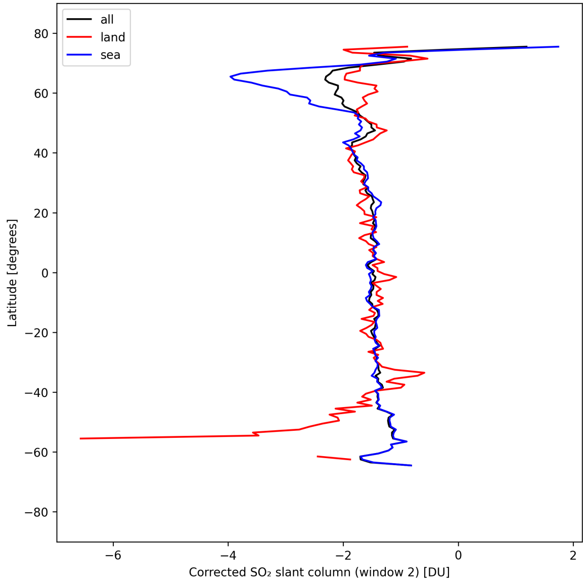
Figure 42: Zonal average of “Corrected SO 2 slant column (window 2)” for 2025-04-03 to 2025-04-04.
