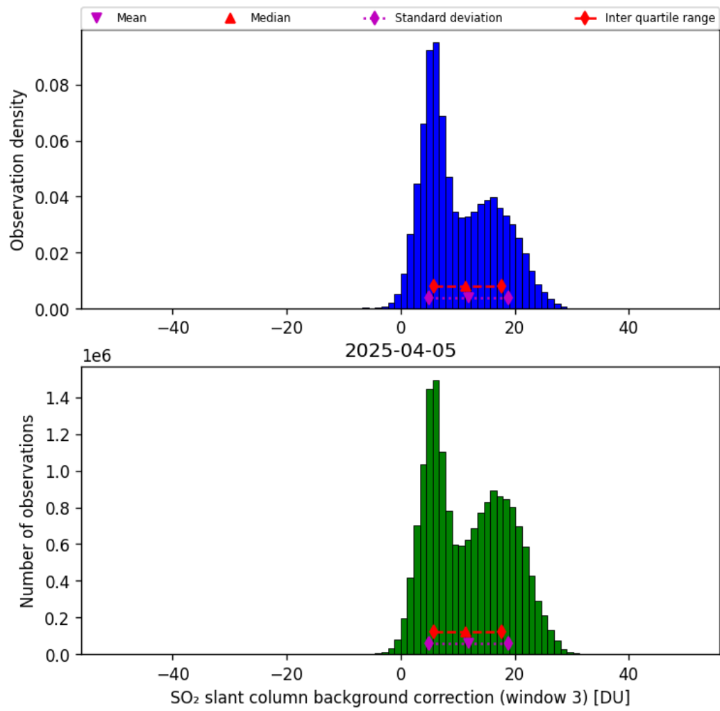
Figure 74: Histogram of “SO 2 slant column background correction (window 3)” for 2025-04-05 to 2025-04-06
