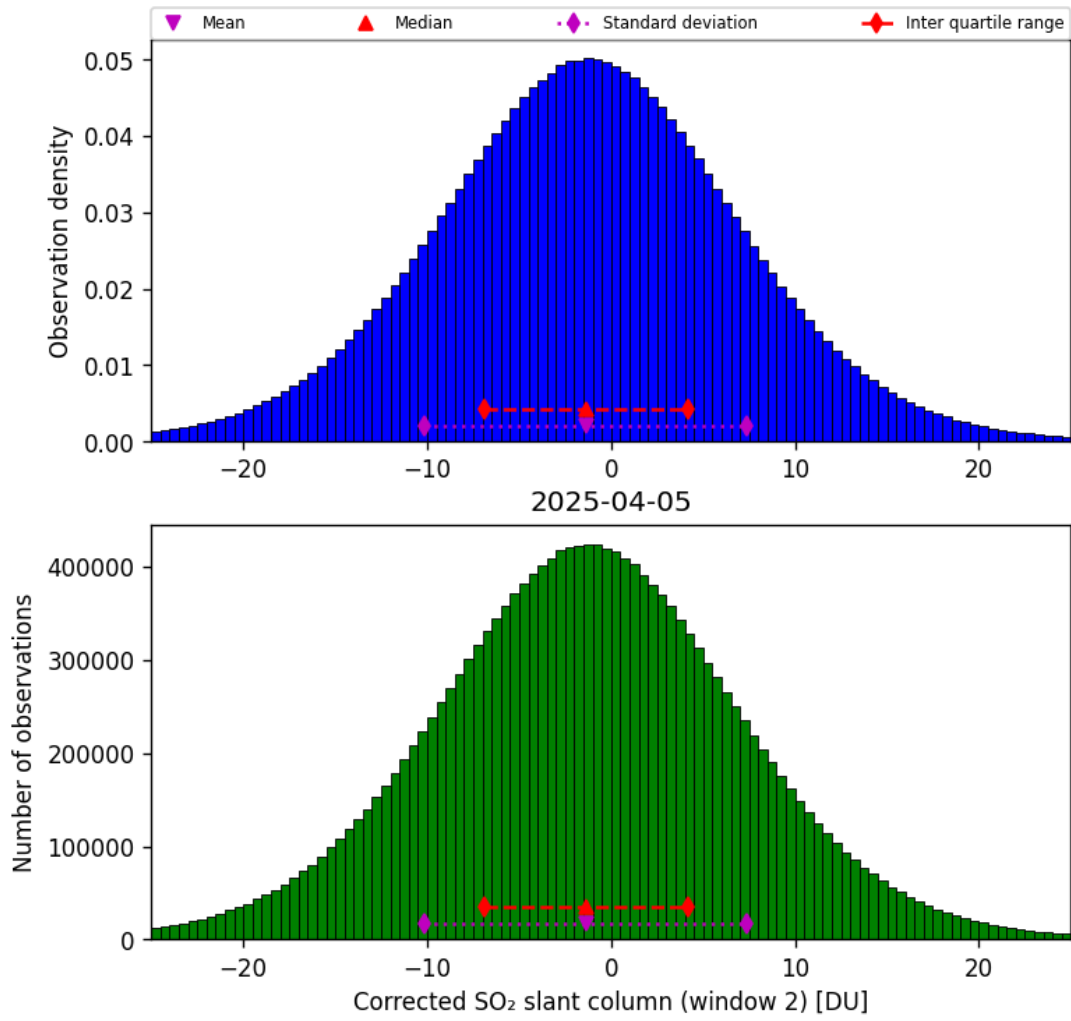
Figure 69: Histogram of “Corrected SO 2 slant column (window 2)” for 2025-04-05 to 2025-04-06
