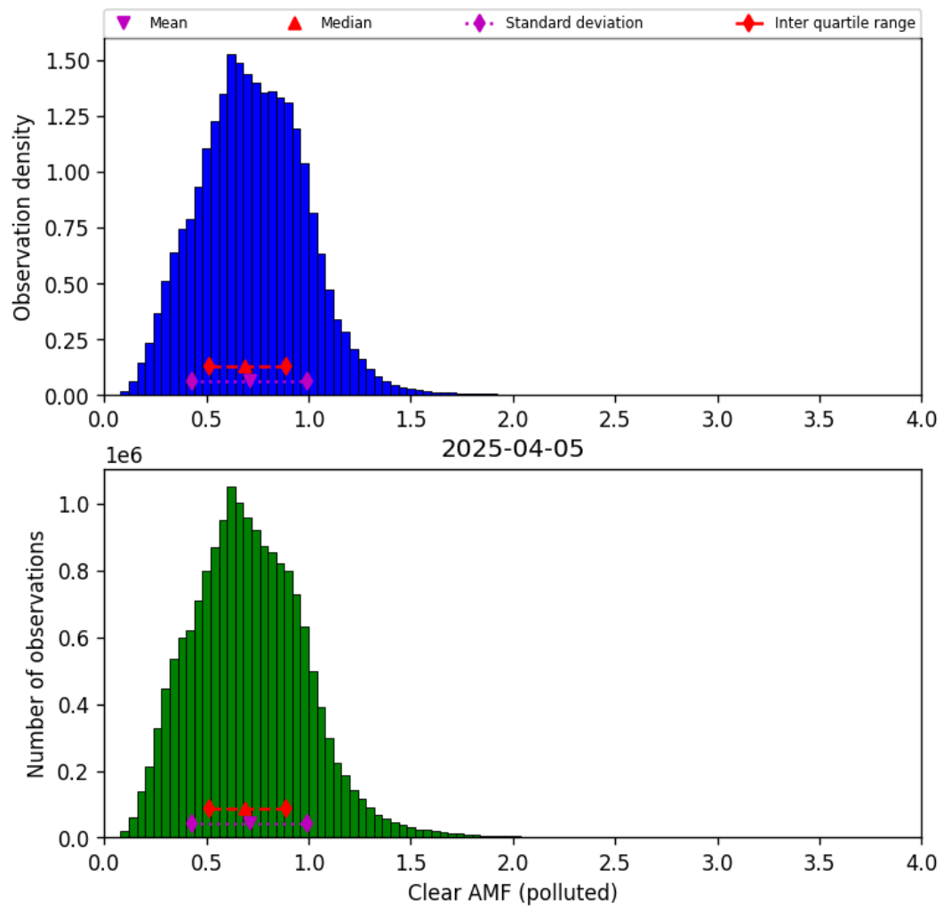
Figure 82: Histogram of “Clear AMF (polluted)” for 2025-04-05 to 2025-04-06
