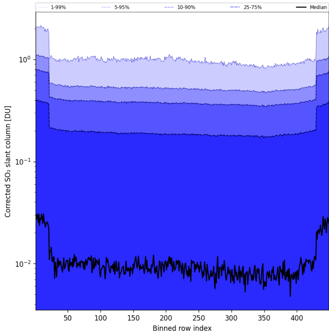
Figure 87: Along track statistics of "Corrected SO 2 slant column" for 2025-04-05 to 2025-04-06
