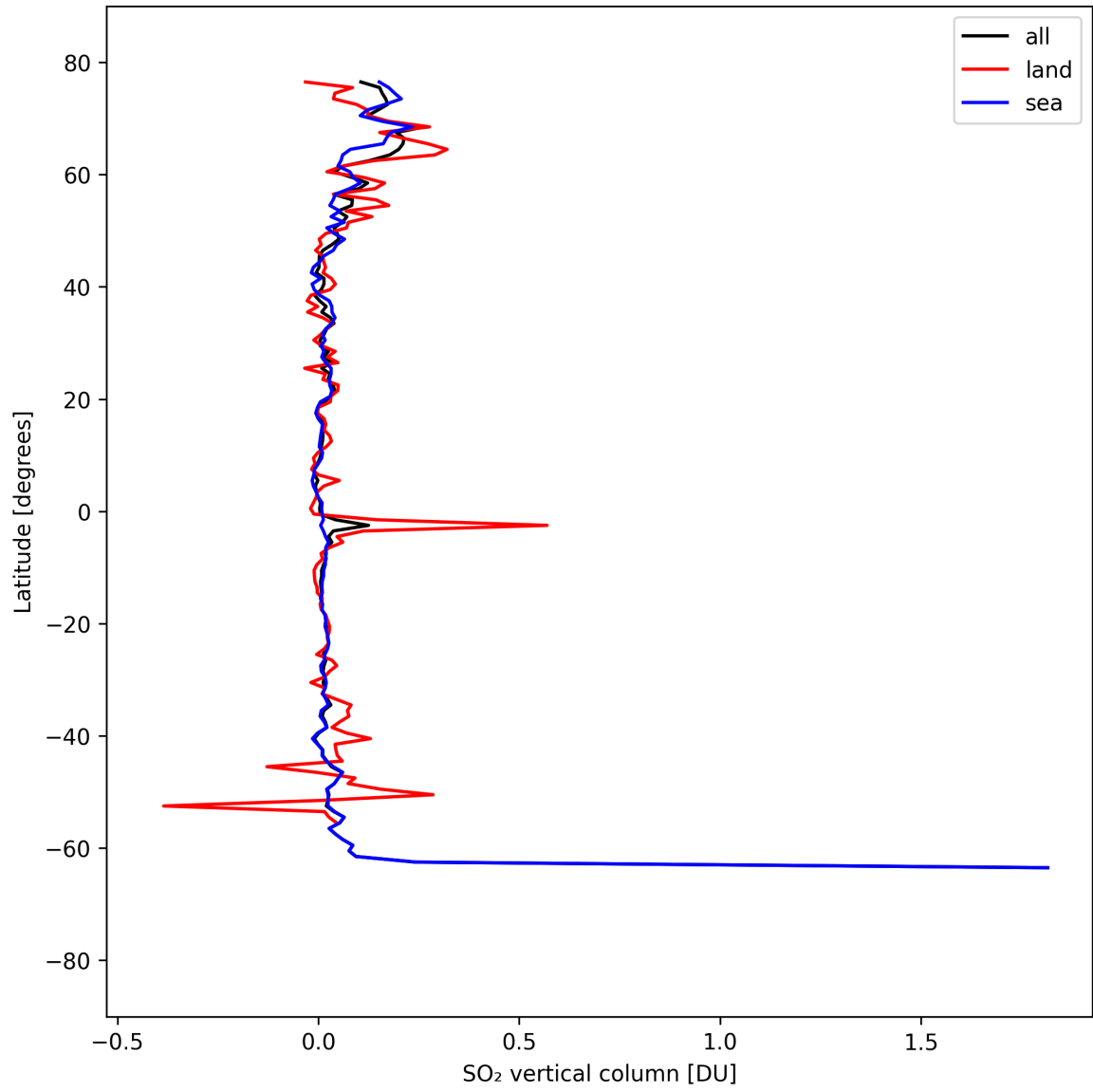
Figure 31: Zonal average of “SO 2 vertical column” for 2025-04-05 to 2025-04-06.
