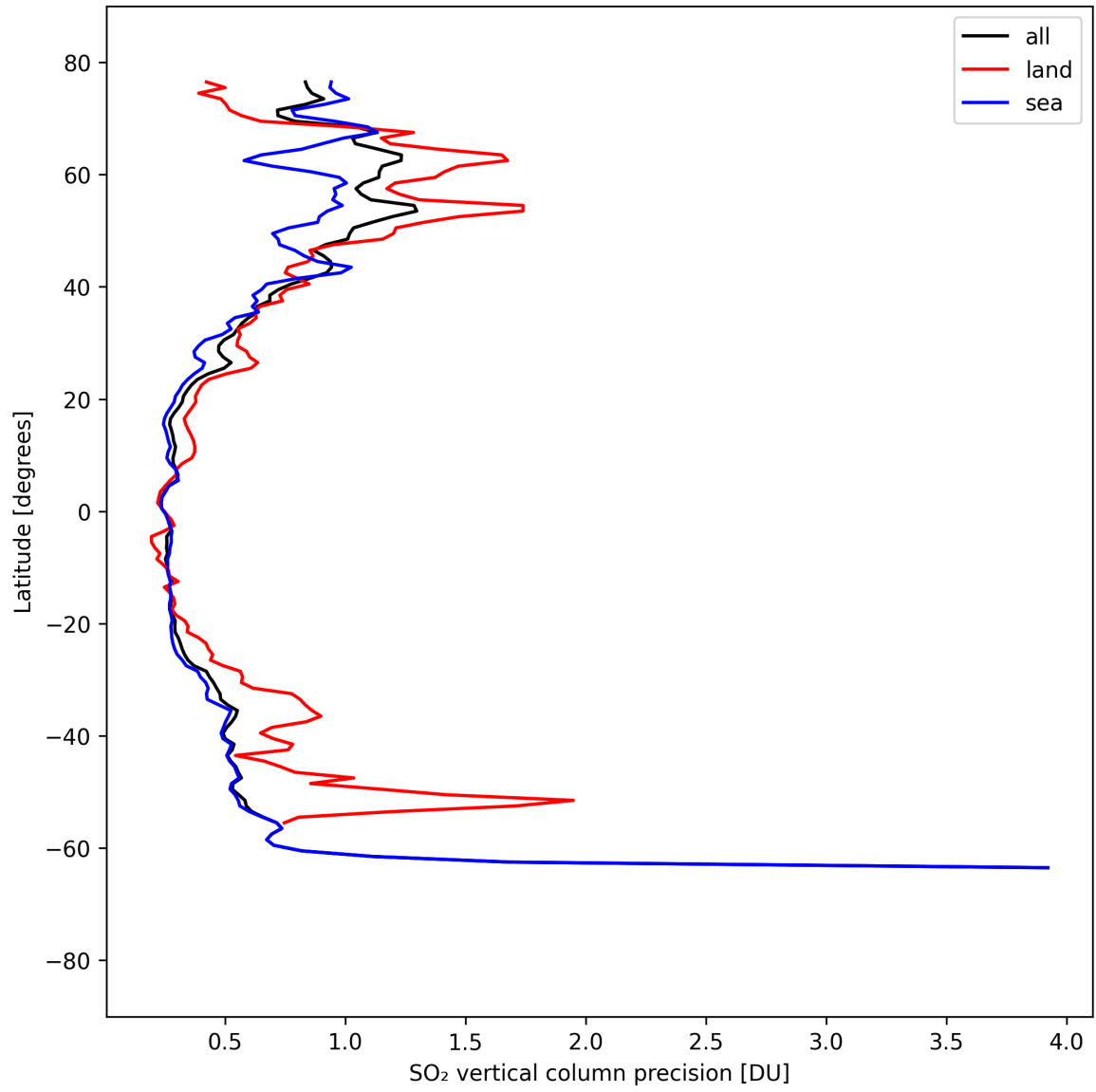
Figure 32: Zonal average of “SO 2 vertical column precision” for 2025-04-05 to 2025-04-06.
