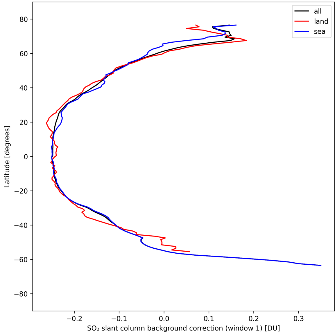
Figure 39: Zonal average of “SO 2 slant column background correction (window 1)” for 2025-04-05 to 2025-04-06.
