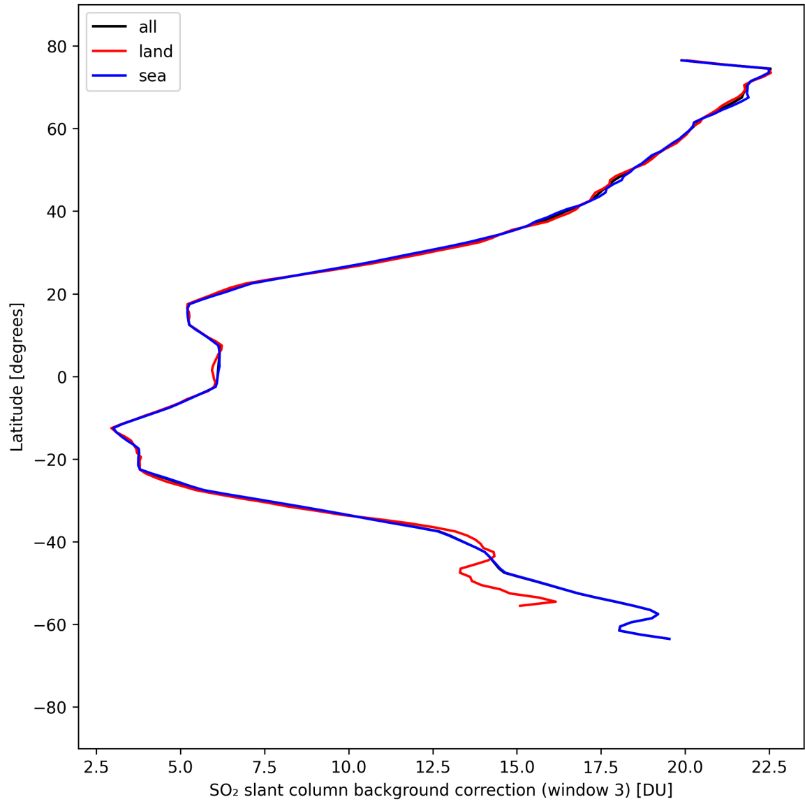
Figure 47: Zonal average of “SO 2 slant column background correction (window 3)” for 2025-04-05 to 2025-04-06.
