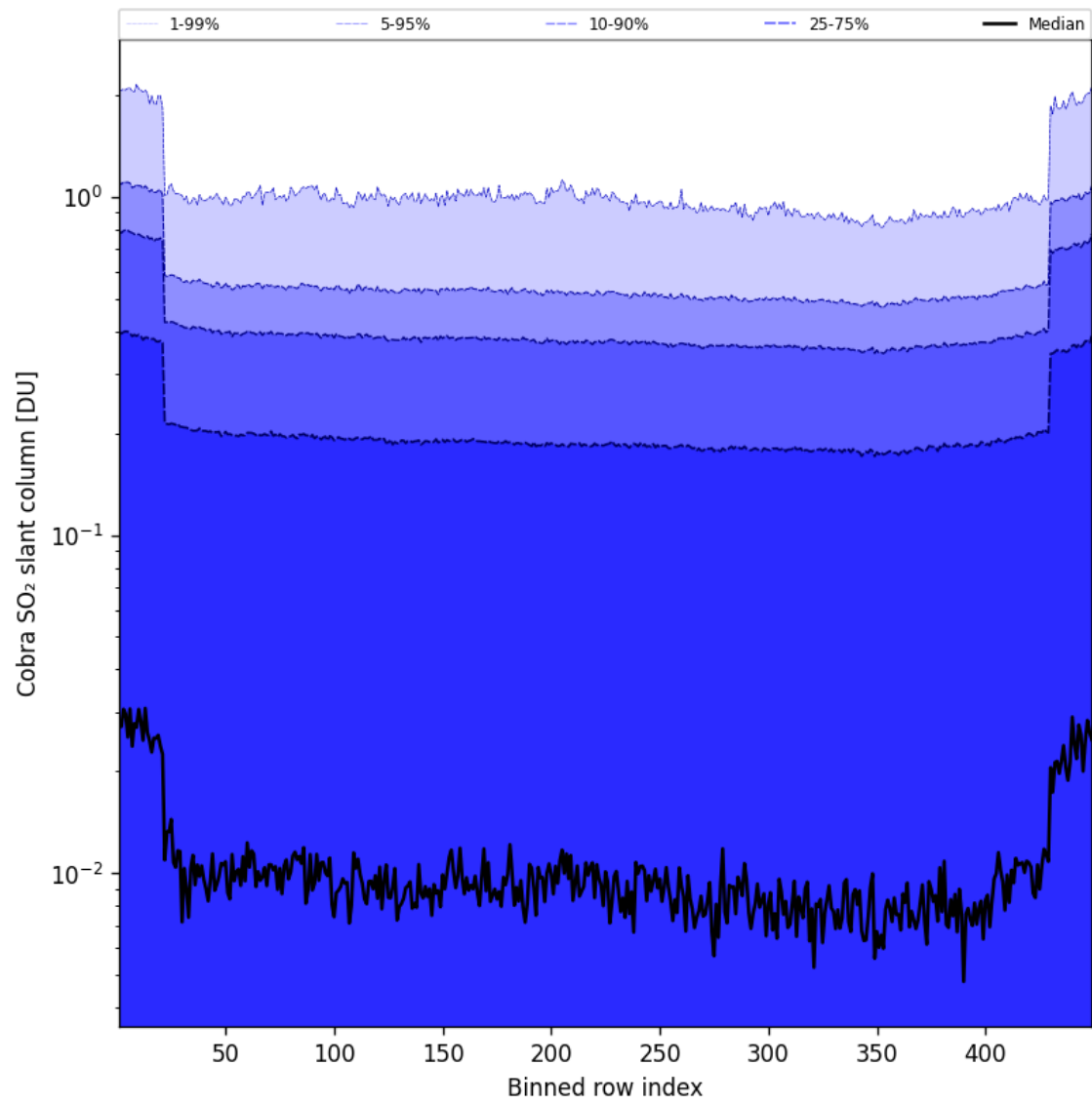
Figure 88: Along track statistics of “Cobra SO 2 slant column” for 2025-04-05 to 2025-04-06
