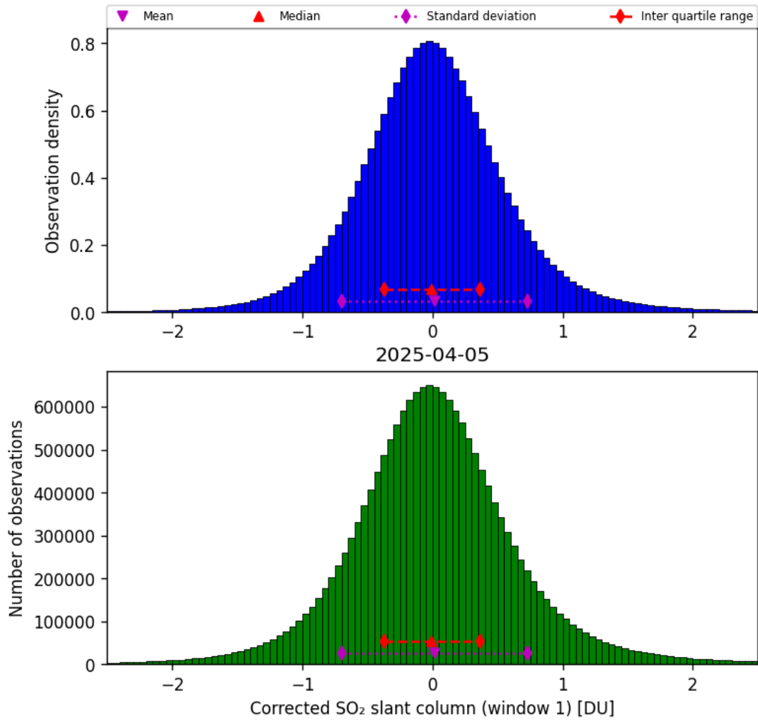
Figure 65: Histogram of “Corrected SO 2 slant column (window 1)” for 2025-04-05 to 2025-04-06
