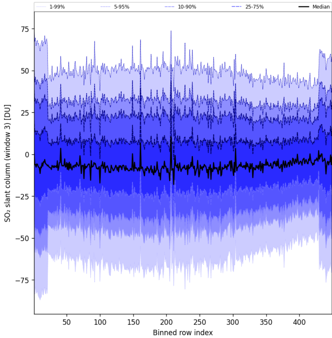
Figure 98: Along track statistics of “SO 2 slant column (window 3)” for 2025-04-05 to 2025-04-06
