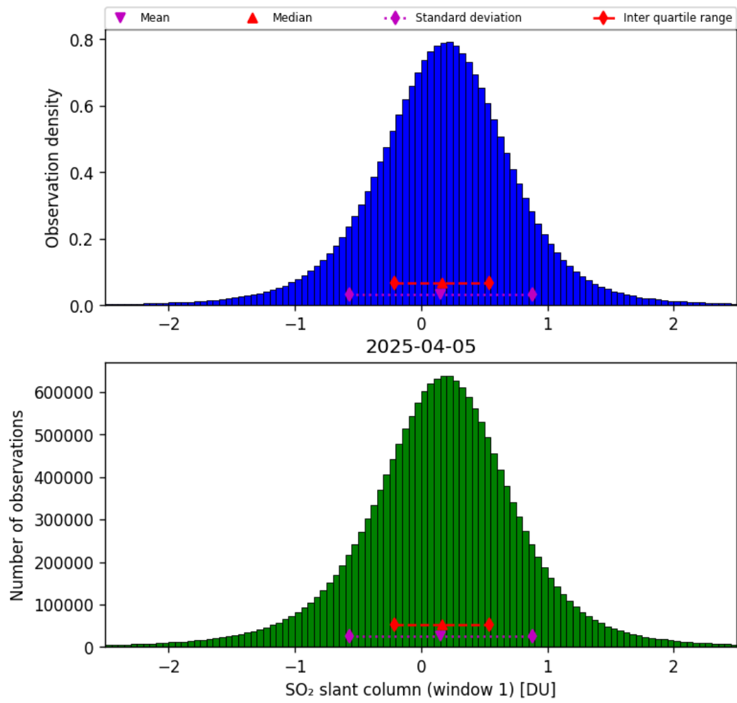
Figure 63: Histogram of “SO 2 slant column (window 1)” for 2025-04-05 to 2025-04-06
