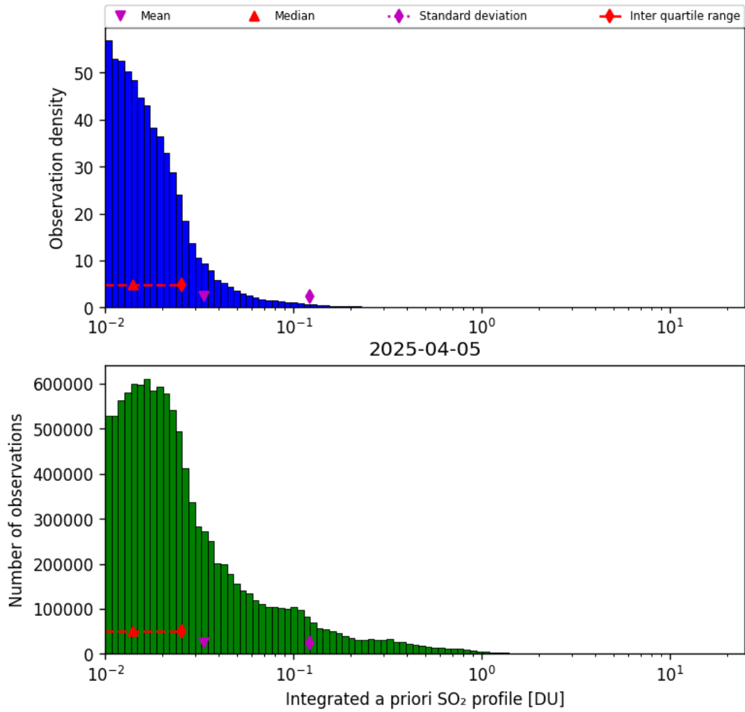
Figure 76: Histogram of “Integrated a priori SO 2 profile” for 2025-04-05 to 2025-04-06
