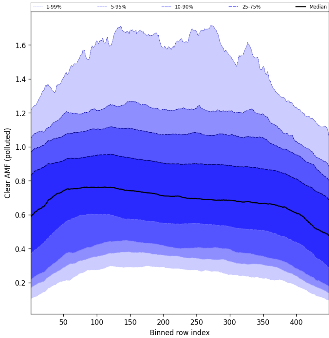
Figure 109: Along track statistics of “Clear AMF (polluted)” for 2025-04-05 to 2025-04-06
