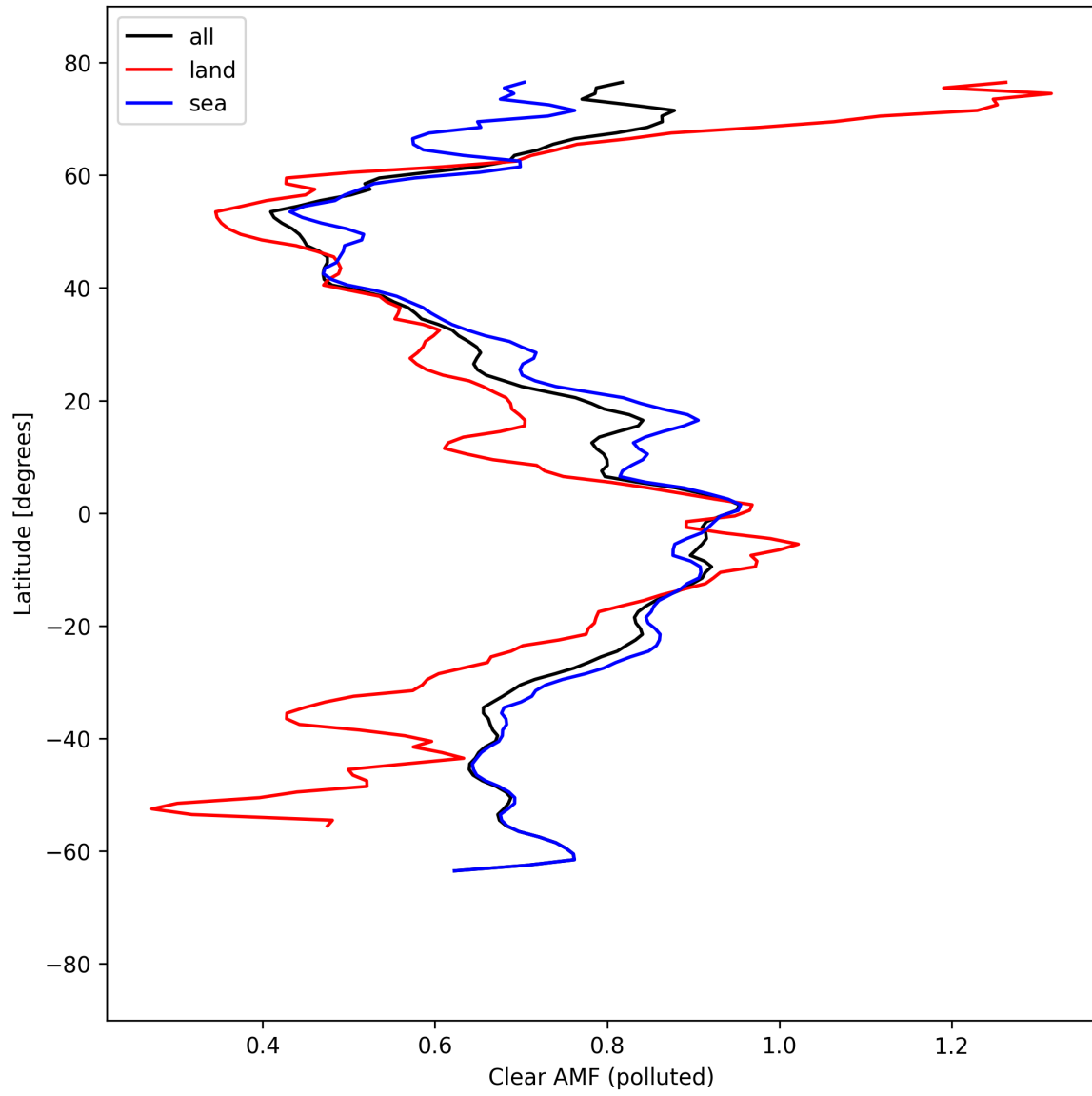
Figure 55: Zonal average of “Clear AMF (polluted)” for 2025-04-05 to 2025-04-06.
