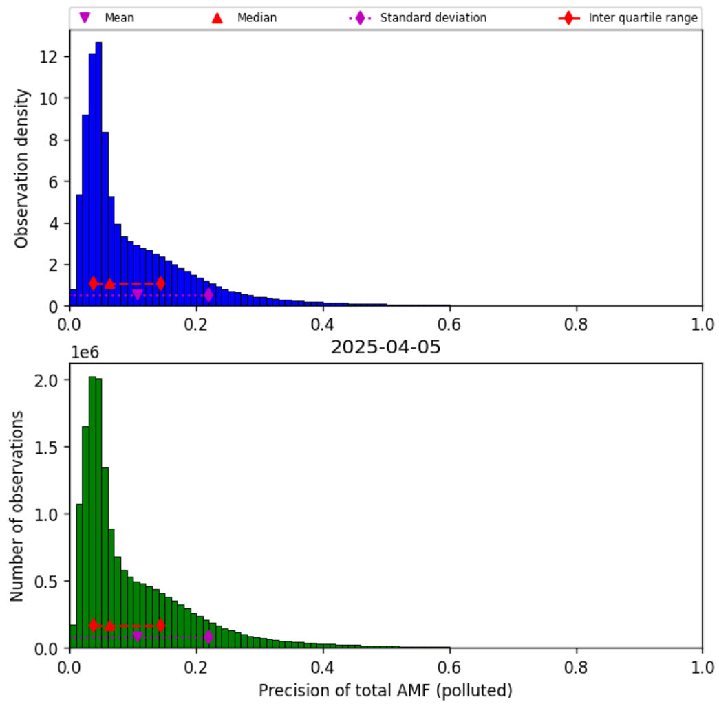
Figure 81: Histogram of “Precision of total AMF (polluted)” for 2025-04-05 to 2025-04-06
