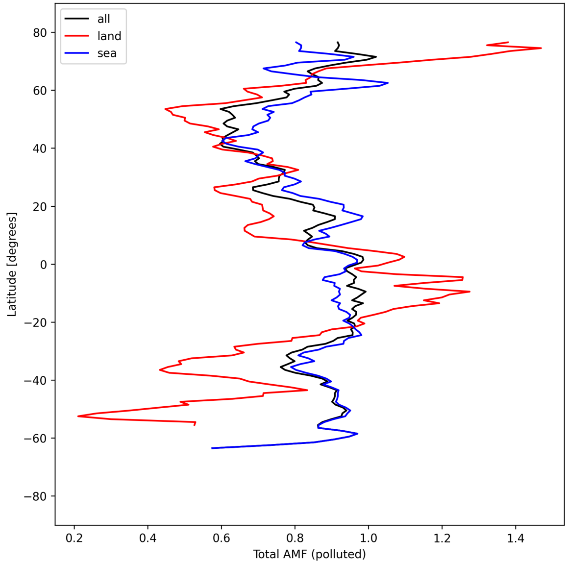
Figure 53: Zonal average of “Total AMF (polluted)” for 2025-04-05 to 2025-04-06.
