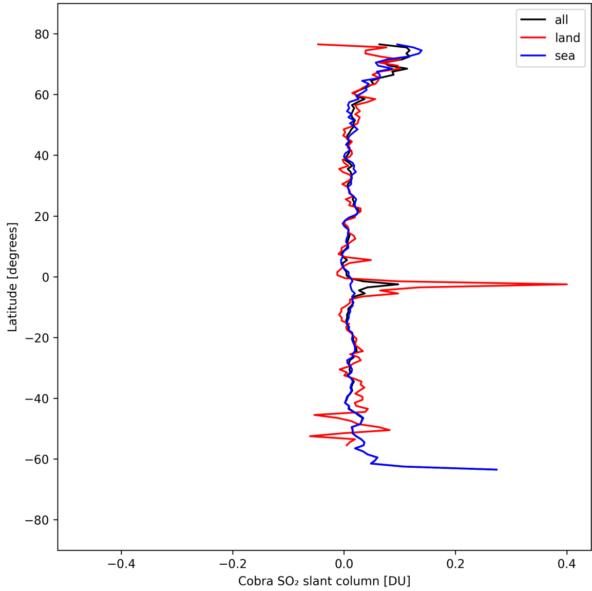
Figure 34: Zonal average of “Cobra SO 2 slant column” for 2025-04-05 to 2025-04-06.
