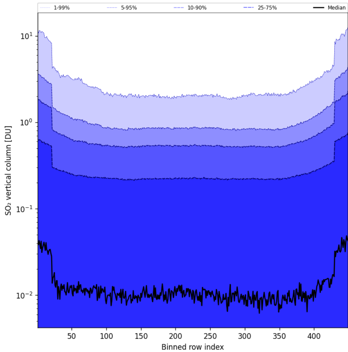
Figure 85: Along track statistics of “SO 2 vertical column” for 2025-04-05 to 2025-04-06
