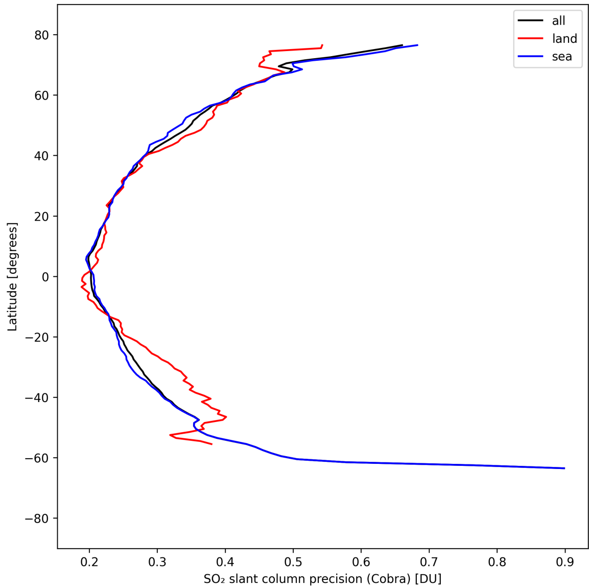
Figure 35: Zonal average of “SO 2 slant column precision (Cobra)” for 2025-04-05 to 2025-04-06.
