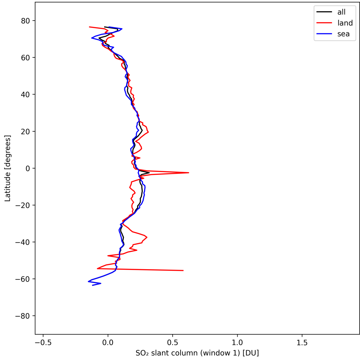
Figure 36: Zonal average of “SO 2 slant column (window 1)” for 2025-04-05 to 2025-04-06.
