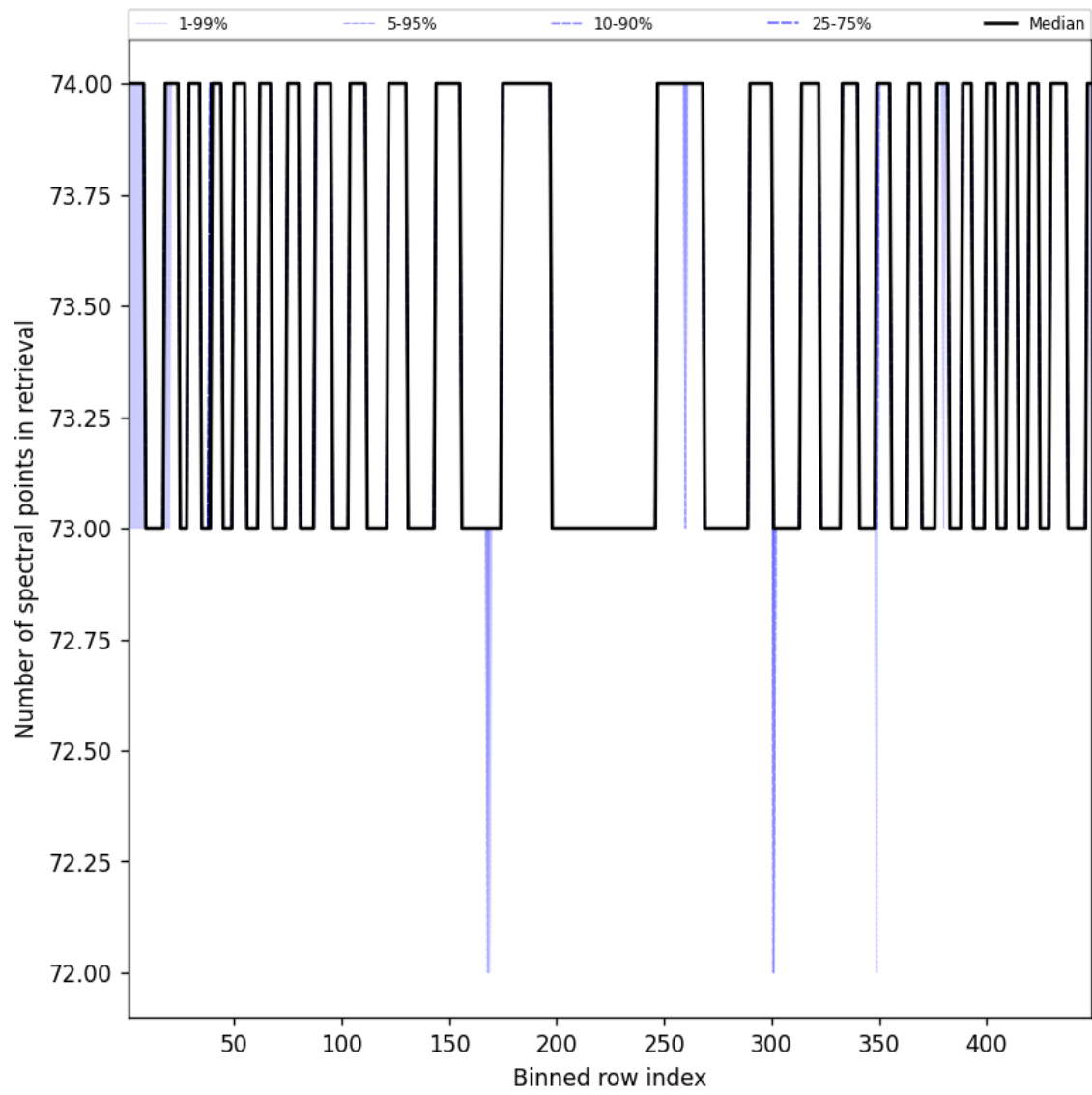
Figure 110: Along track statistics of “Number of spectral points in retrieval” for 2025-04-05 to 2025-04-06
