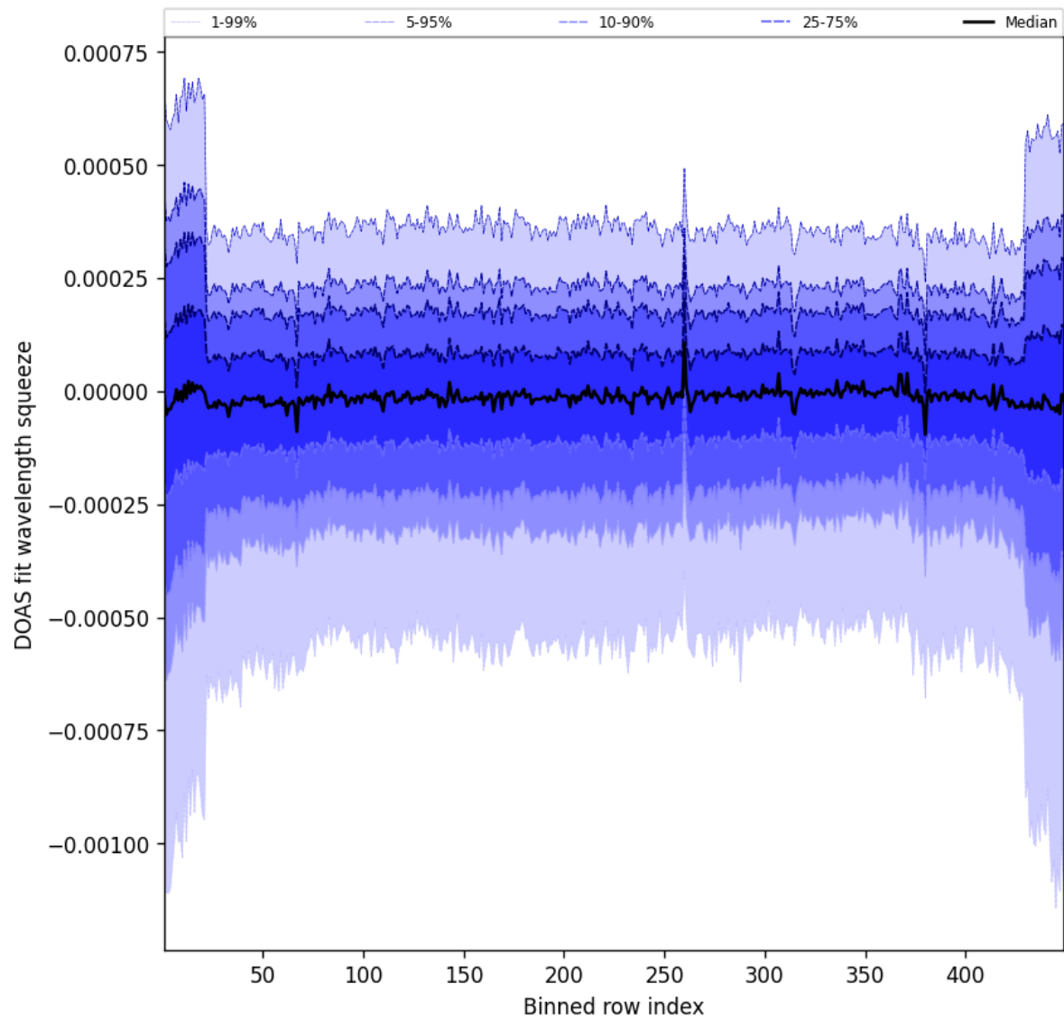
Figure 105: Along track statistics of “DOAS fit wavelength squeeze” for 2025-04-05 to 2025-04-06
