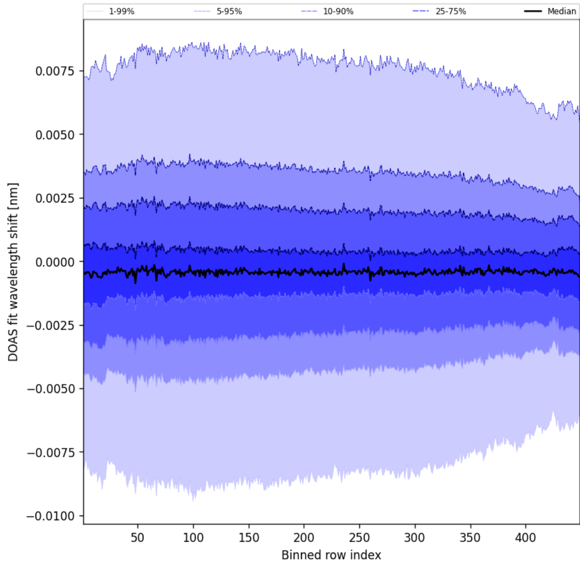
Figure 104: Along track statistics of “DOAS fit wavelength shift” for 2025-04-05 to 2025-04-06
