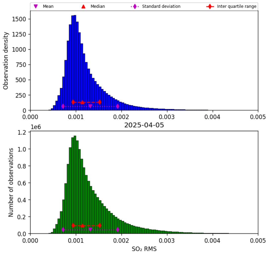
Figure 79: Histogram of “SO 2 RMS” for 2025-04-05 to 2025-04-06
