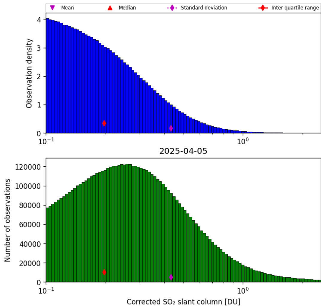
Figure 60: Histogram of “Corrected SO 2 slant column” for 2025-04-05 to 2025-04-06
