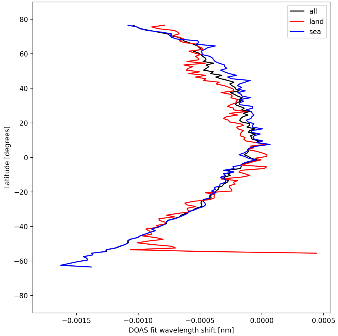
Figure 50: Zonal average of “DOAS fit wavelength shift” for 2025-04-05 to 2025-04-06.
