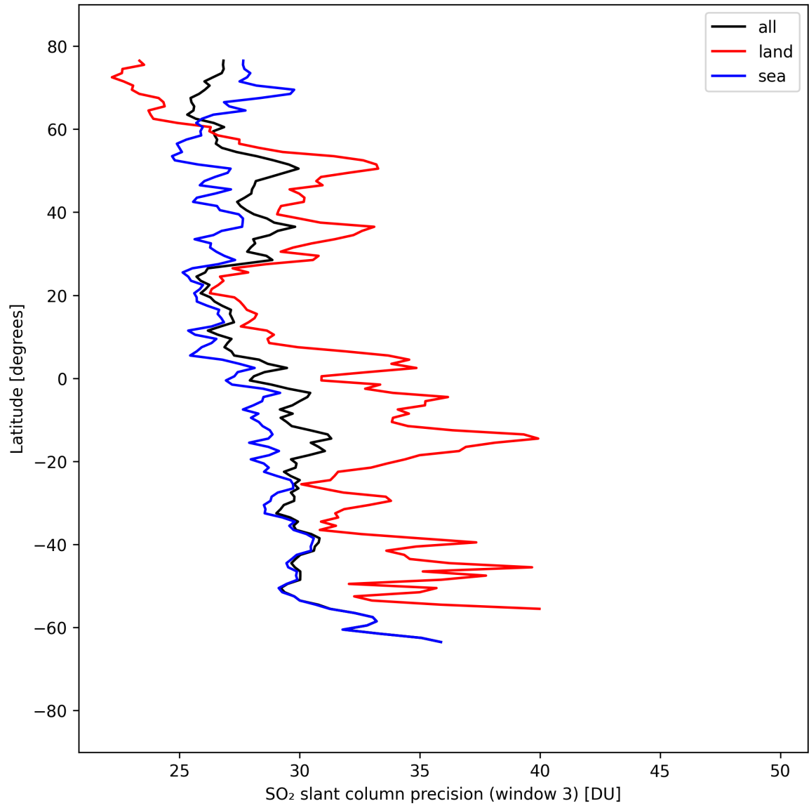
Figure 45: Zonal average of “SO 2 slant column precision (window 3)” for 2025-04-05 to 2025-04-06.
