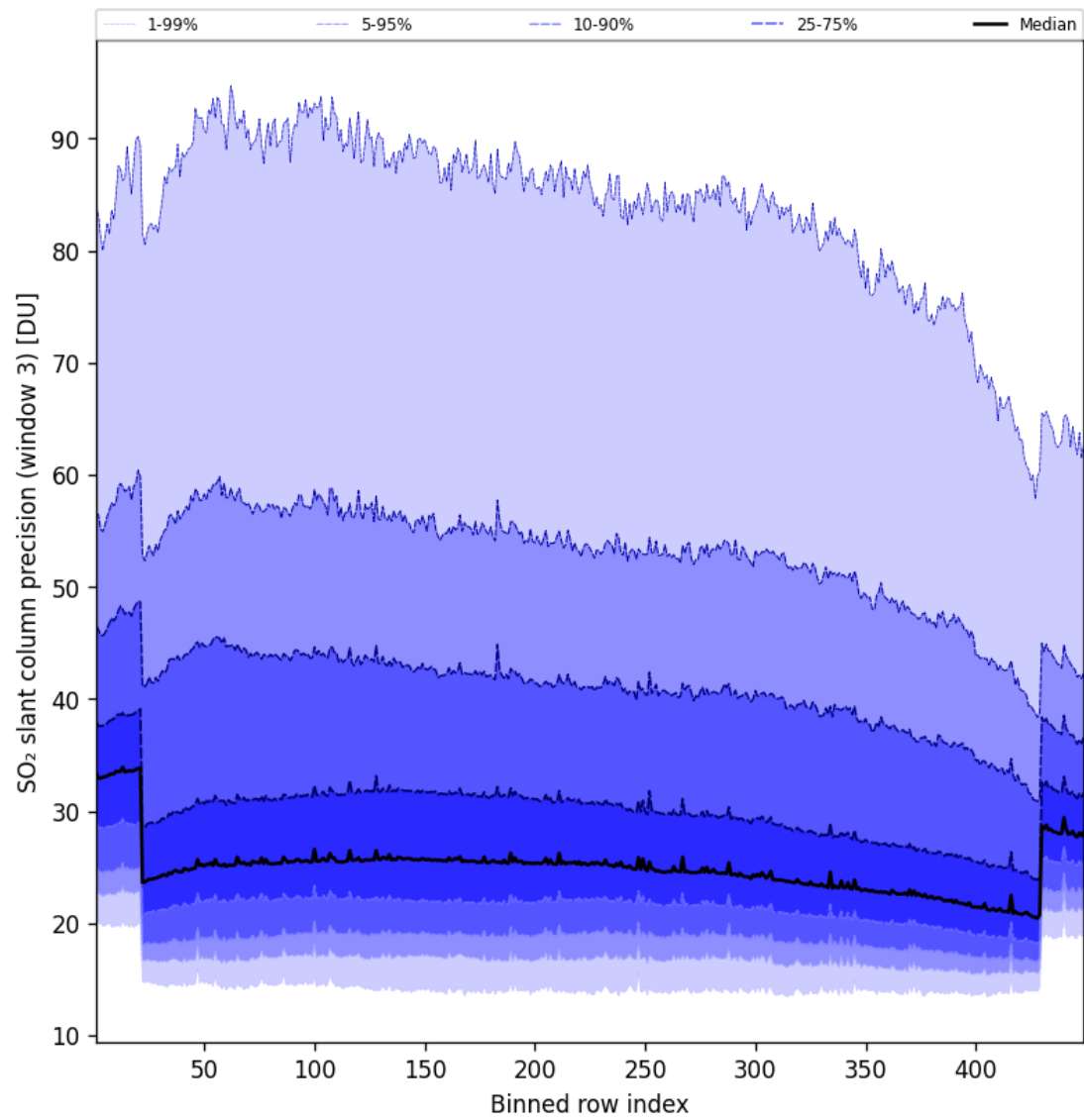
Figure 99: Along track statistics of “SO 2 slant column precision (window 3)” for 2025-04-05 to 2025-04-06
