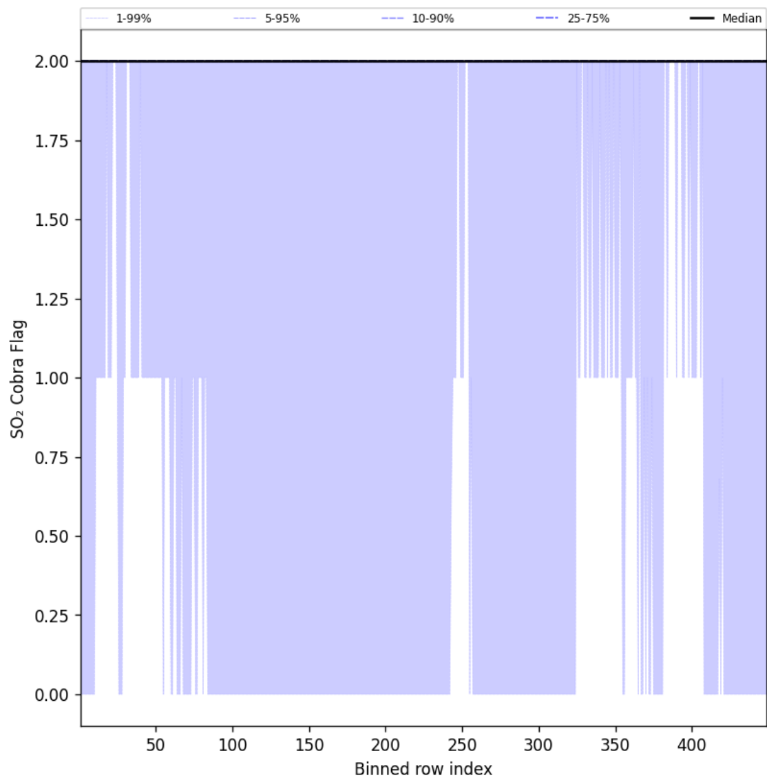
Figure 102: Along track statistics of “SO 2 Cobra Flag” for 2025-04-05 to 2025-04-06
