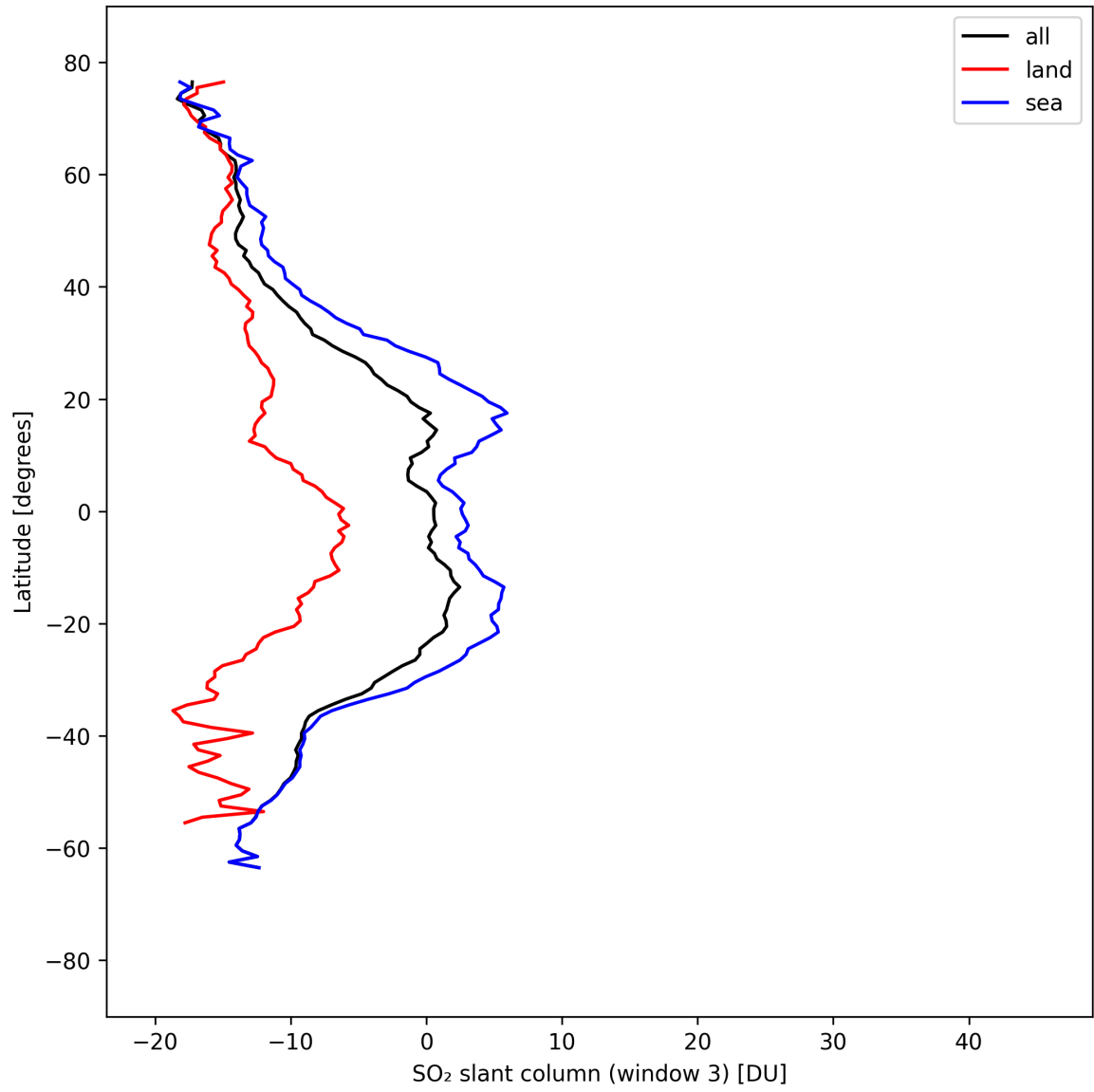
Figure 44: Zonal average of “SO 2 slant column (window 3)” for 2025-04-05 to 2025-04-06.
