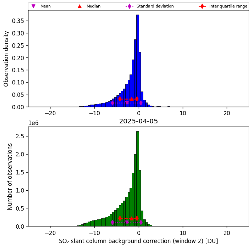
Figure 70: Histogram of “SO 2 slant column background correction (window 2)” for 2025-04-05 to 2025-04-06
