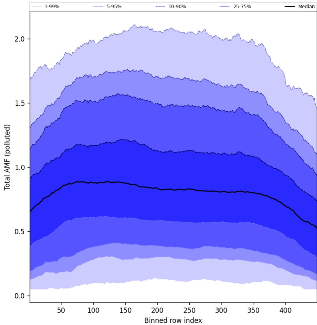
Figure 107: Along track statistics of “Total AMF (polluted)” for 2025-04-05 to 2025-04-06
