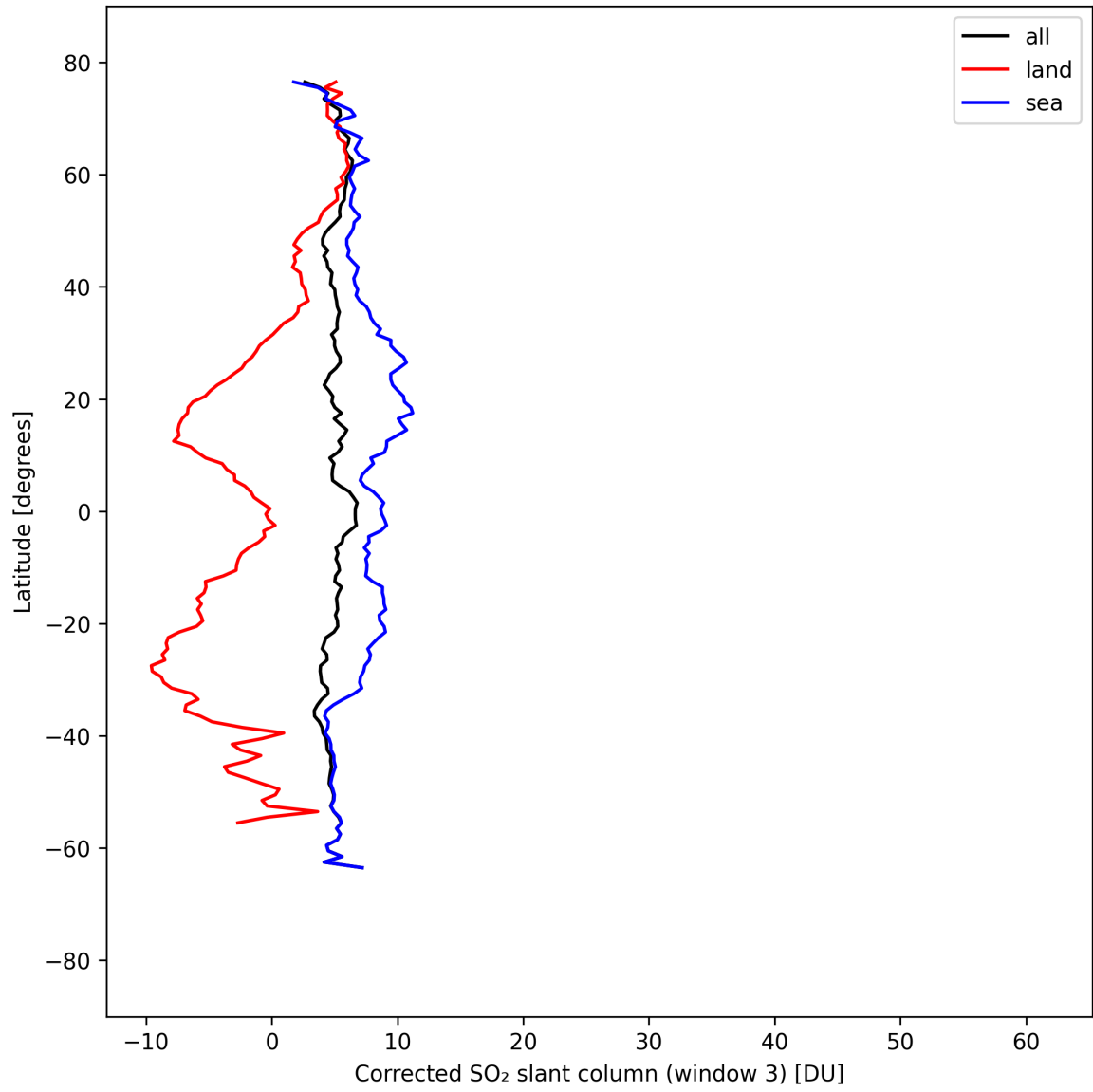
Figure 46: Zonal average of “Corrected SO 2 slant column (window 3)” for 2025-04-05 to 2025-04-06.
