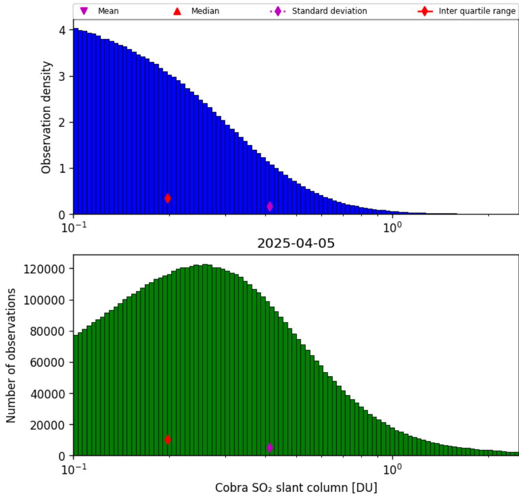
Figure 61: Histogram of “Cobra SO 2 slant column” for 2025-04-05 to 2025-04-06
