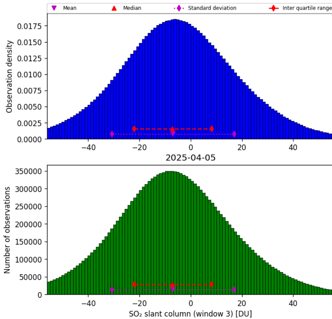
Figure 71: Histogram of “SO 2 slant column (window 3)” for 2025-04-05 to 2025-04-06
