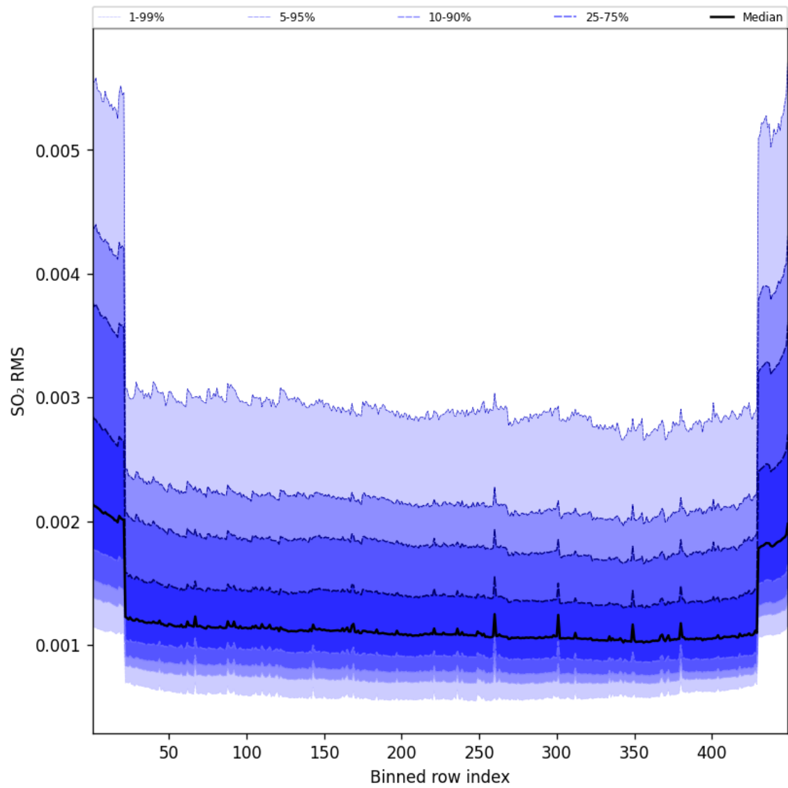
Figure 106: Along track statistics of “SO 2 RMS” for 2025-04-05 to 2025-04-06
