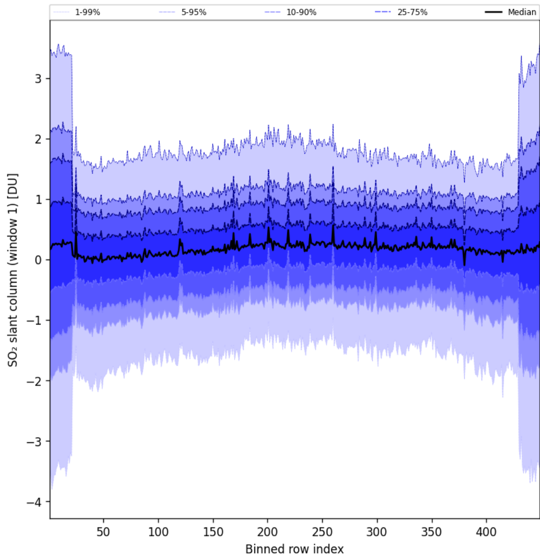
Figure 90: Along track statistics of “SO 2 slant column (window 1)” for 2025-04-05 to 2025-04-06
