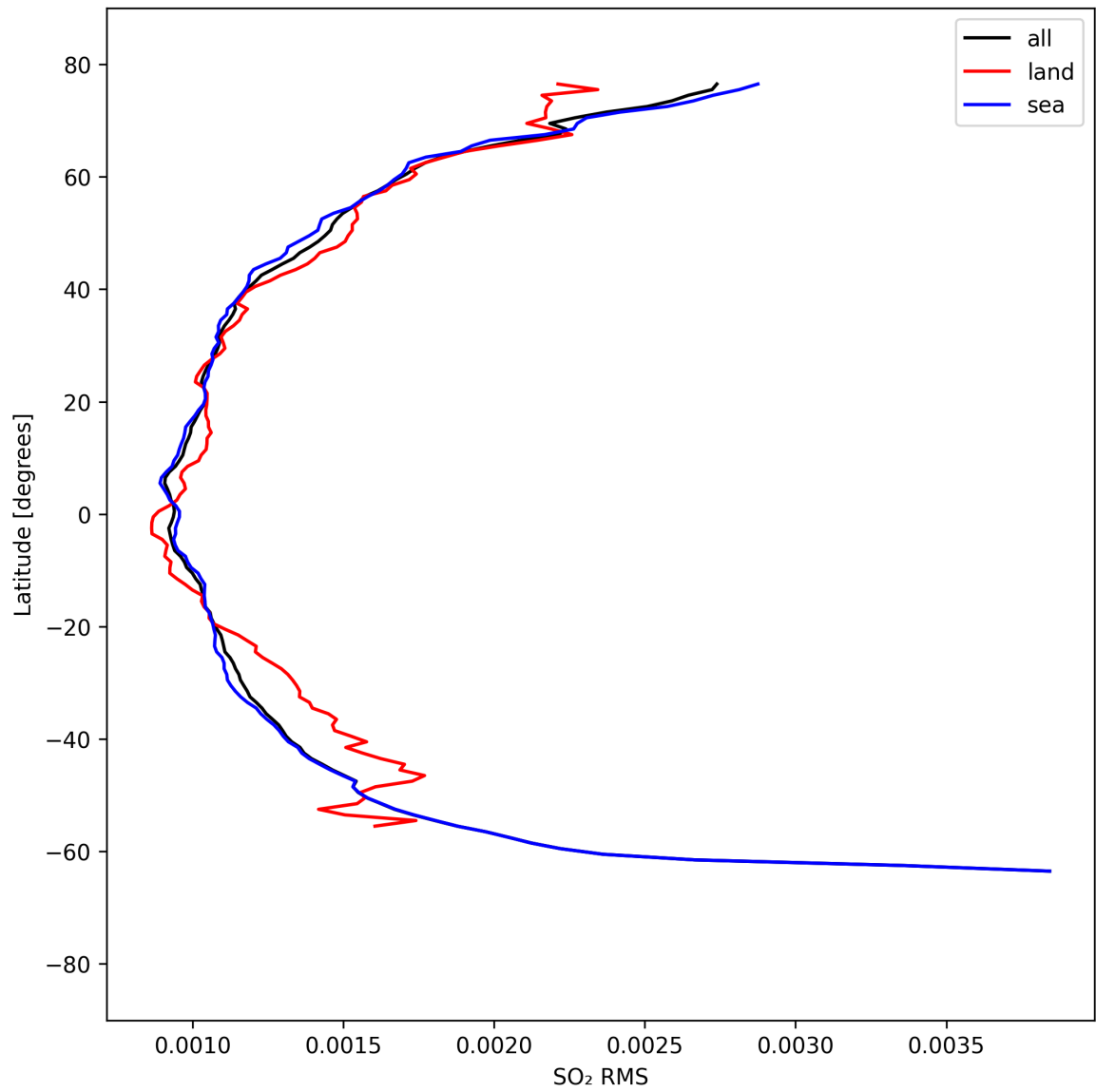
Figure 52: Zonal average of “SO 2 RMS” for 2025-04-05 to 2025-04-06.
