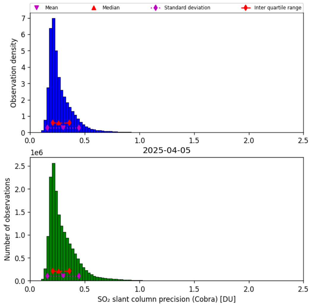
Figure 62: Histogram of “SO 2 slant column precision (Cobra)” for 2025-04-05 to 2025-04-06
