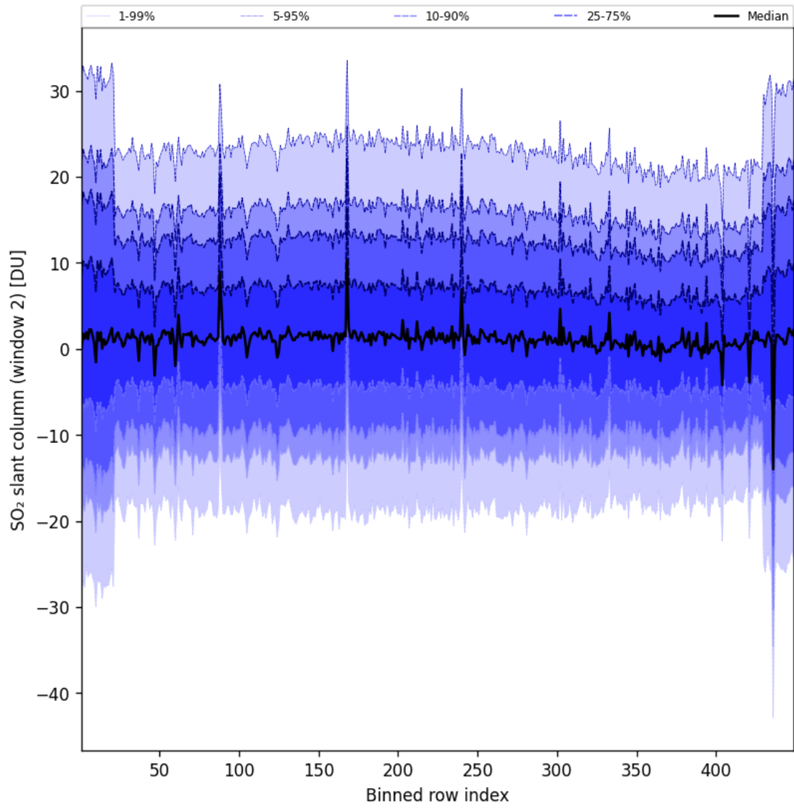
Figure 94: Along track statistics of “SO 2 slant column (window 2)” for 2025-04-05 to 2025-04-06
