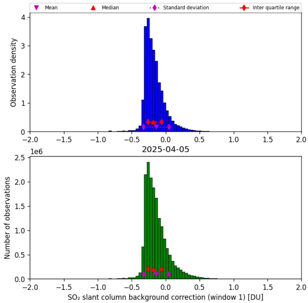
Figure 66: Histogram of “SO 2 slant column background correction (window 1)” for 2025-04-05 to 2025-04-06
