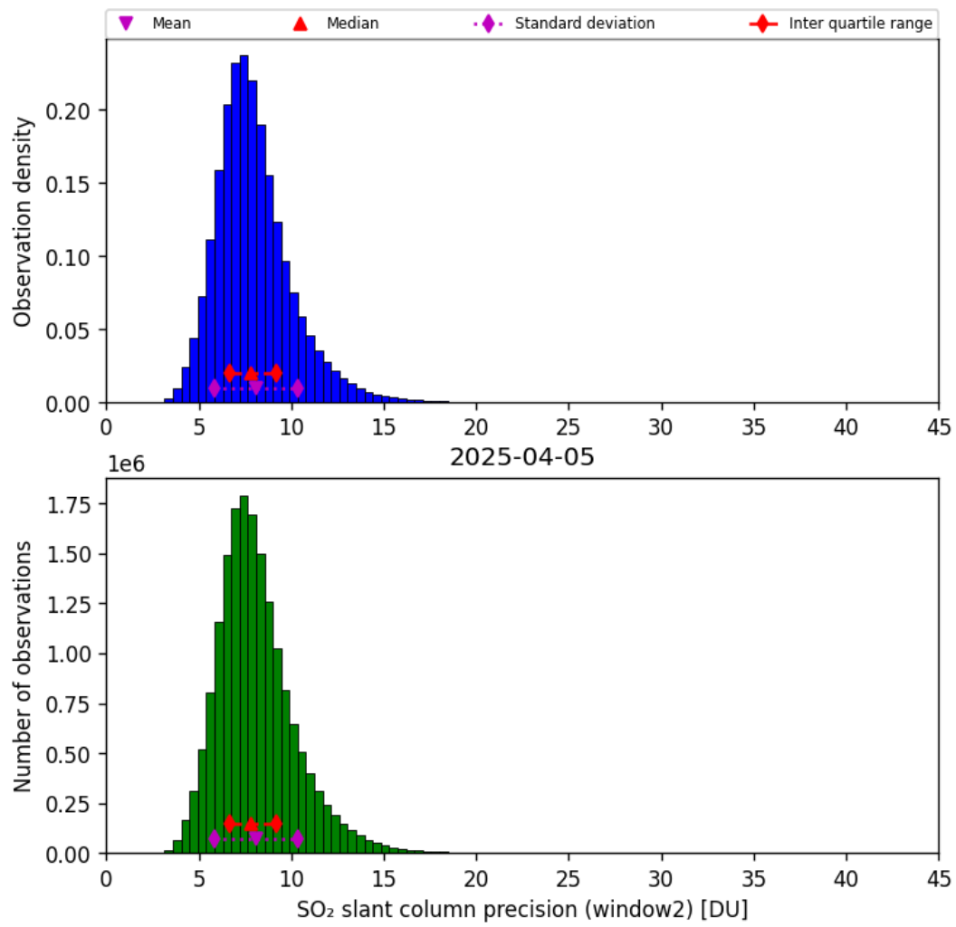
Figure 68: Histogram of “SO 2 slant column precision (window2)” for 2025-04-05 to 2025-04-06
