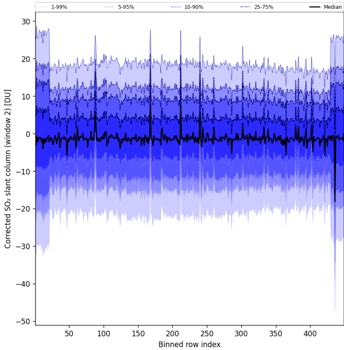
Figure 96: Along track statistics of “Corrected SO 2 slant column (window 2)” for 2025-04-05 to 2025-04-06
