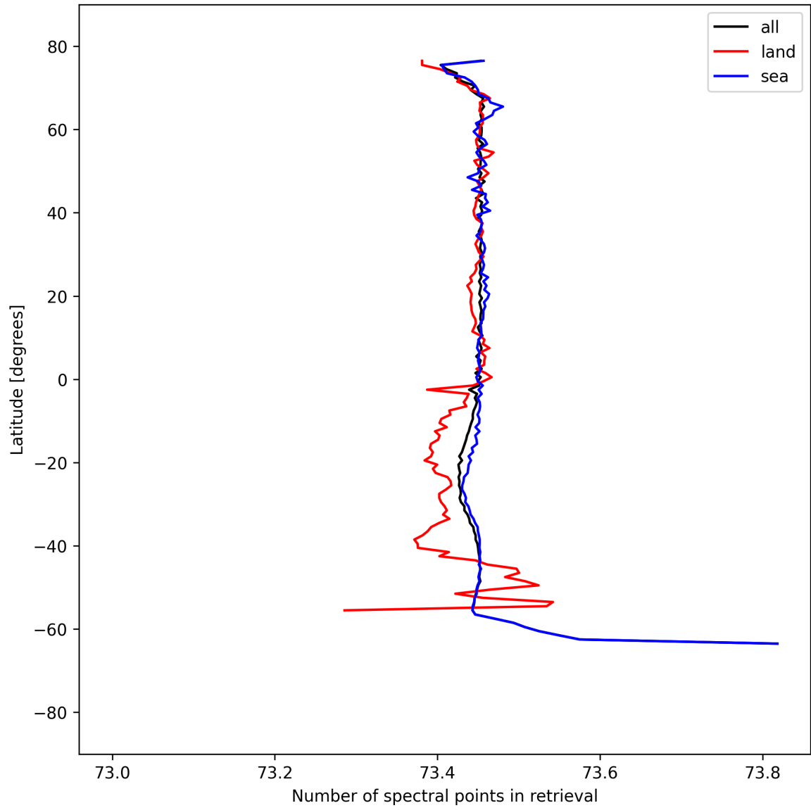
Figure 56: Zonal average of “Number of spectral points in retrieval” for 2025-04-05 to 2025-04-06.
