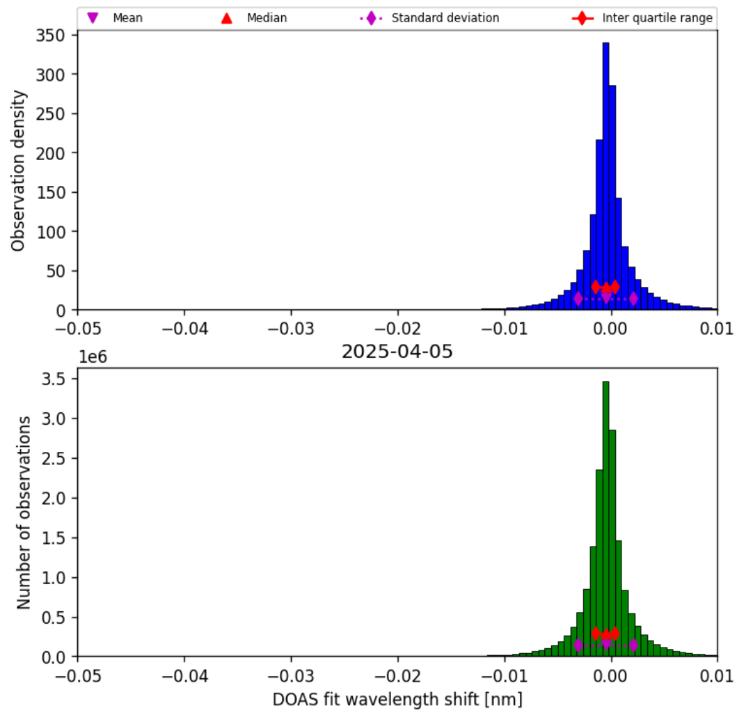
Figure 77: Histogram of “DOAS fit wavelength shift” for 2025-04-05 to 2025-04-06
