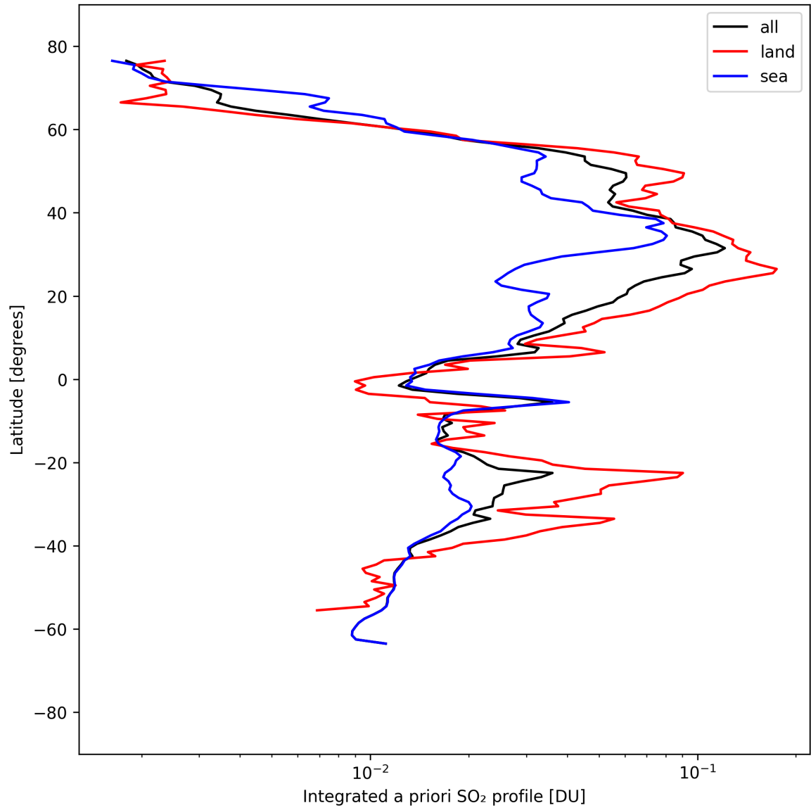
Figure 49: Zonal average of “Integrated a priori SO 2 profile” for 2025-04-05 to 2025-04-06.
