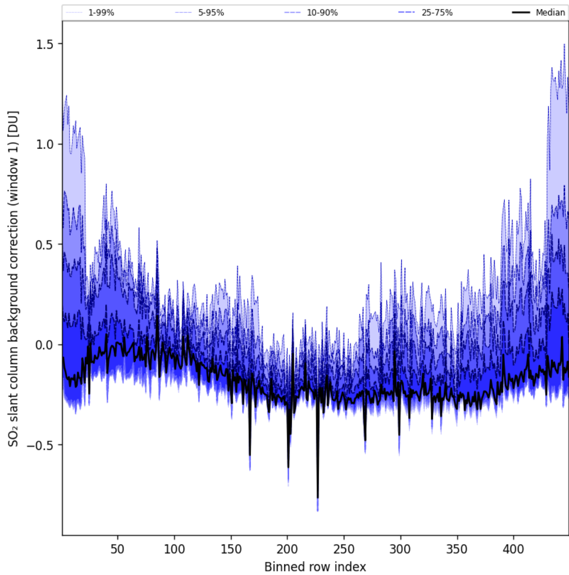
Figure 93: Along track statistics of “SO 2 slant column background correction (window 1)” for 2025-04-05 to 2025-04-06
