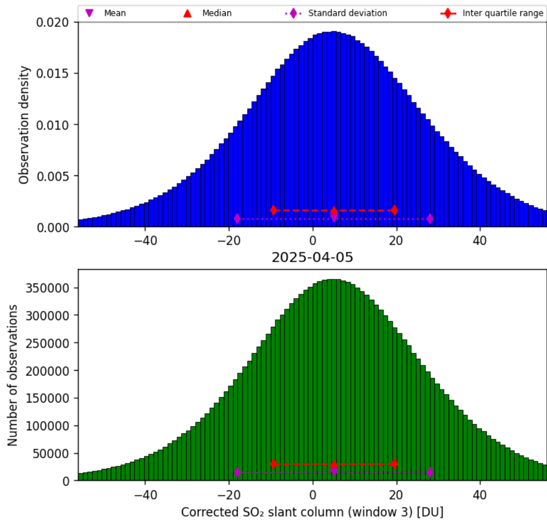
Figure 73: Histogram of “Corrected SO 2 slant column (window 3)” for 2025-04-05 to 2025-04-06
