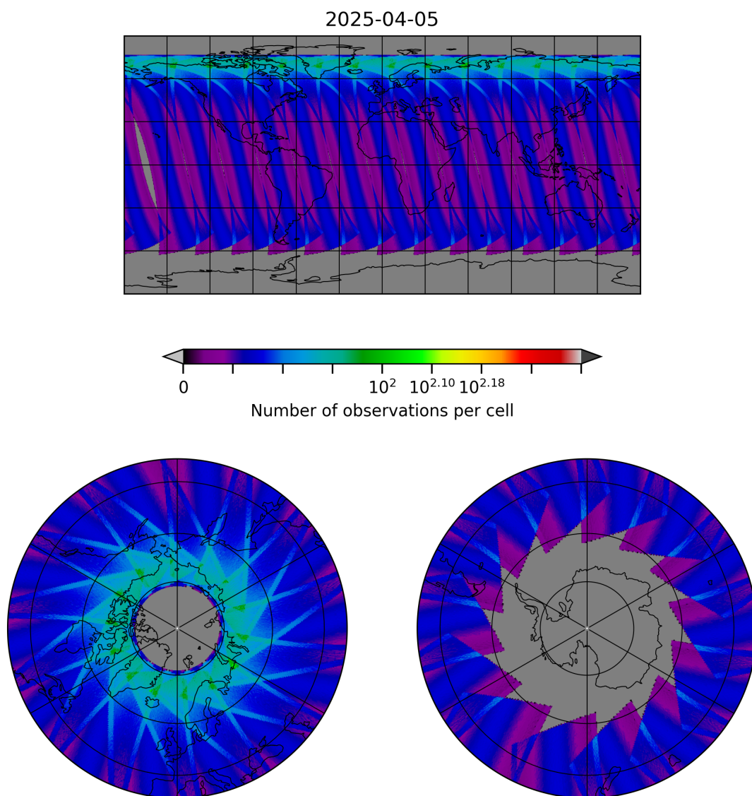
Figure 29: Map of the number of observations for 2025-04-05 to 2025-04-06
