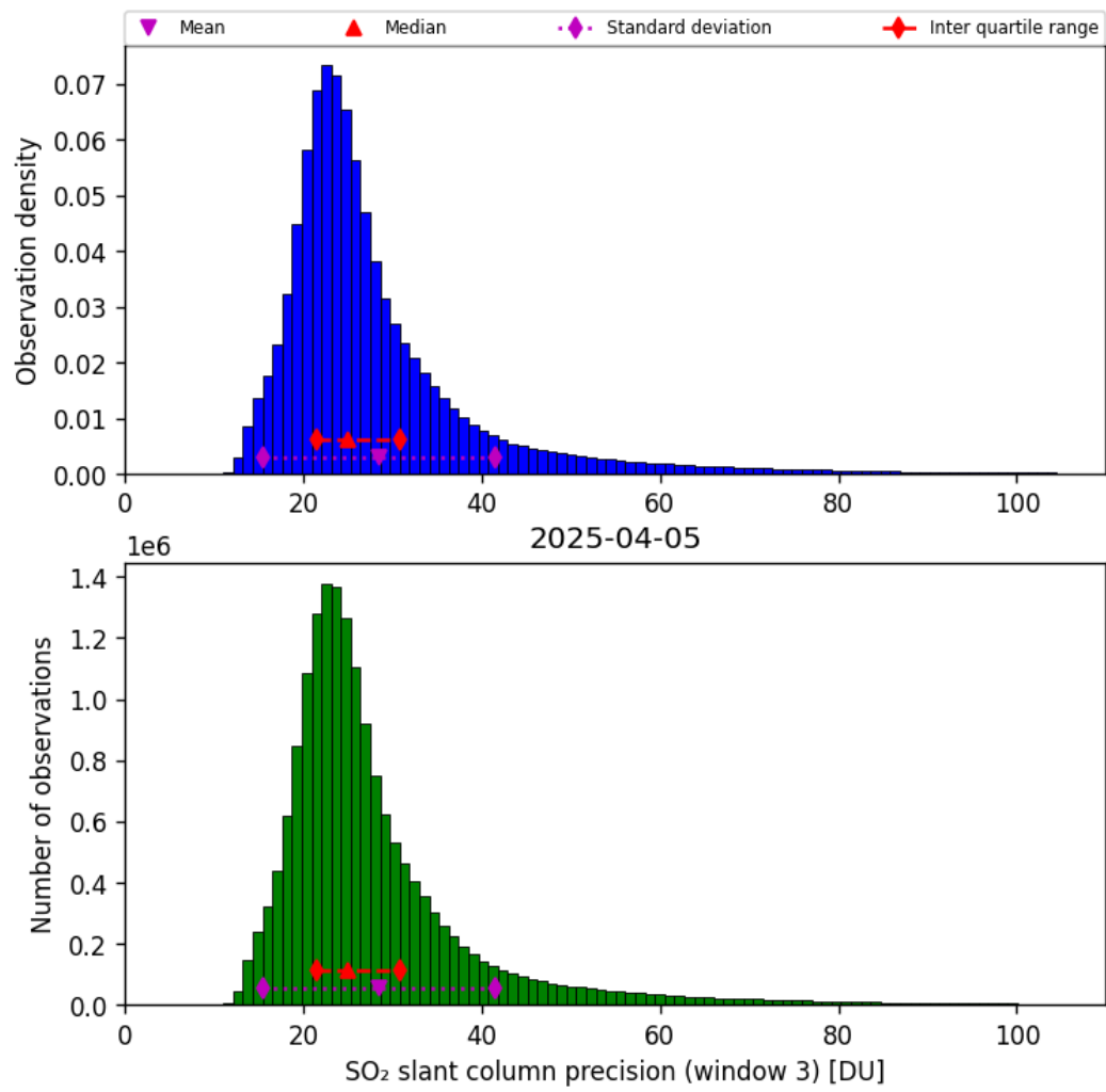
Figure 72: Histogram of “SO 2 slant column precision (window 3)” for 2025-04-05 to 2025-04-06
