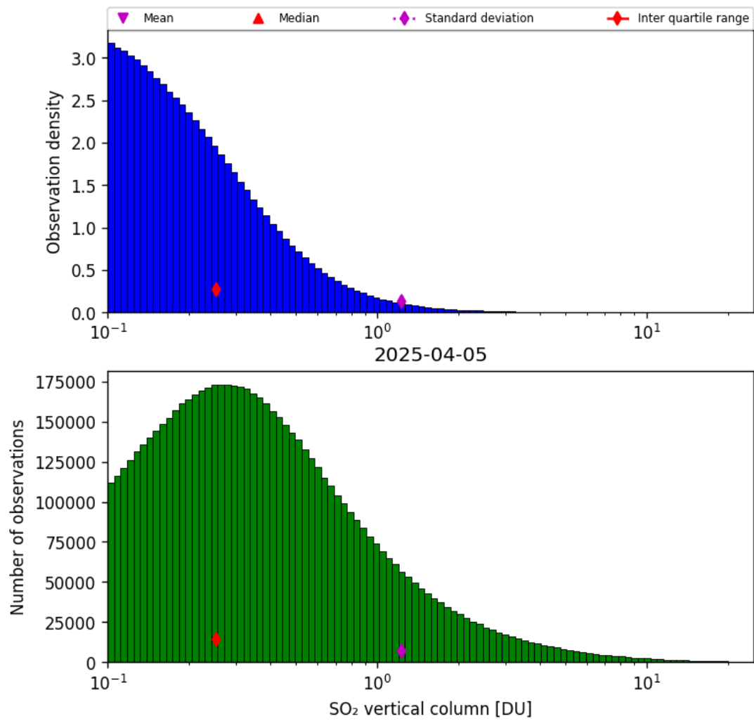
Figure 58: Histogram of “SO 2 vertical column” for 2025-04-05 to 2025-04-06
