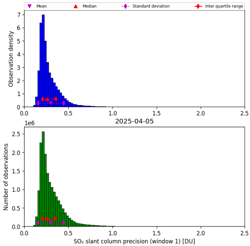
Figure 64: Histogram of “SO 2 slant column precision (window 1)” for 2025-04-05 to 2025-04-06
