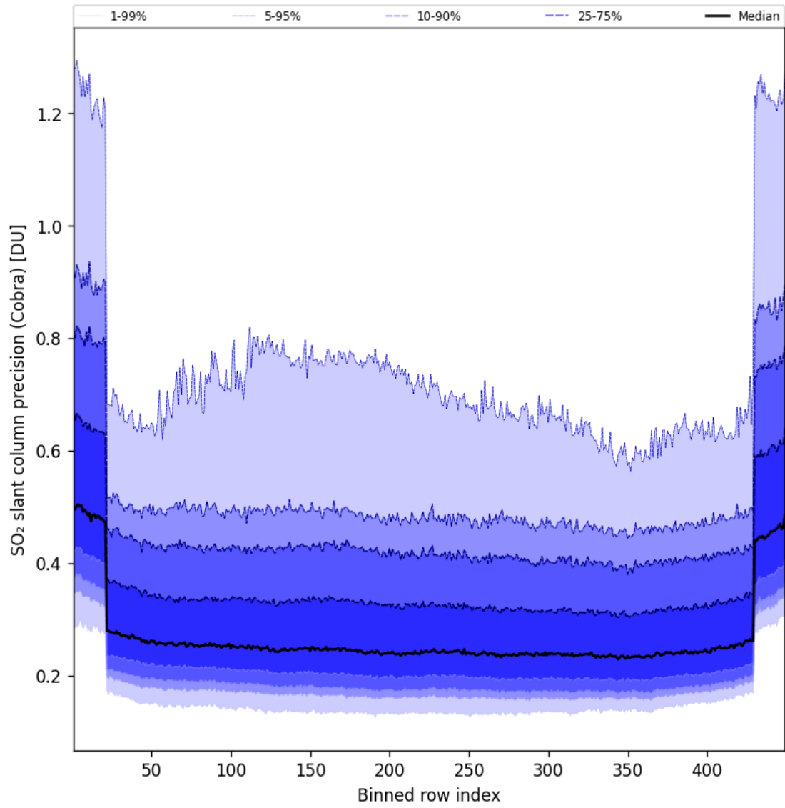
Figure 89: Along track statistics of “SO 2 slant column precision (Cobra)” for 2025-04-05 to 2025-04-06
