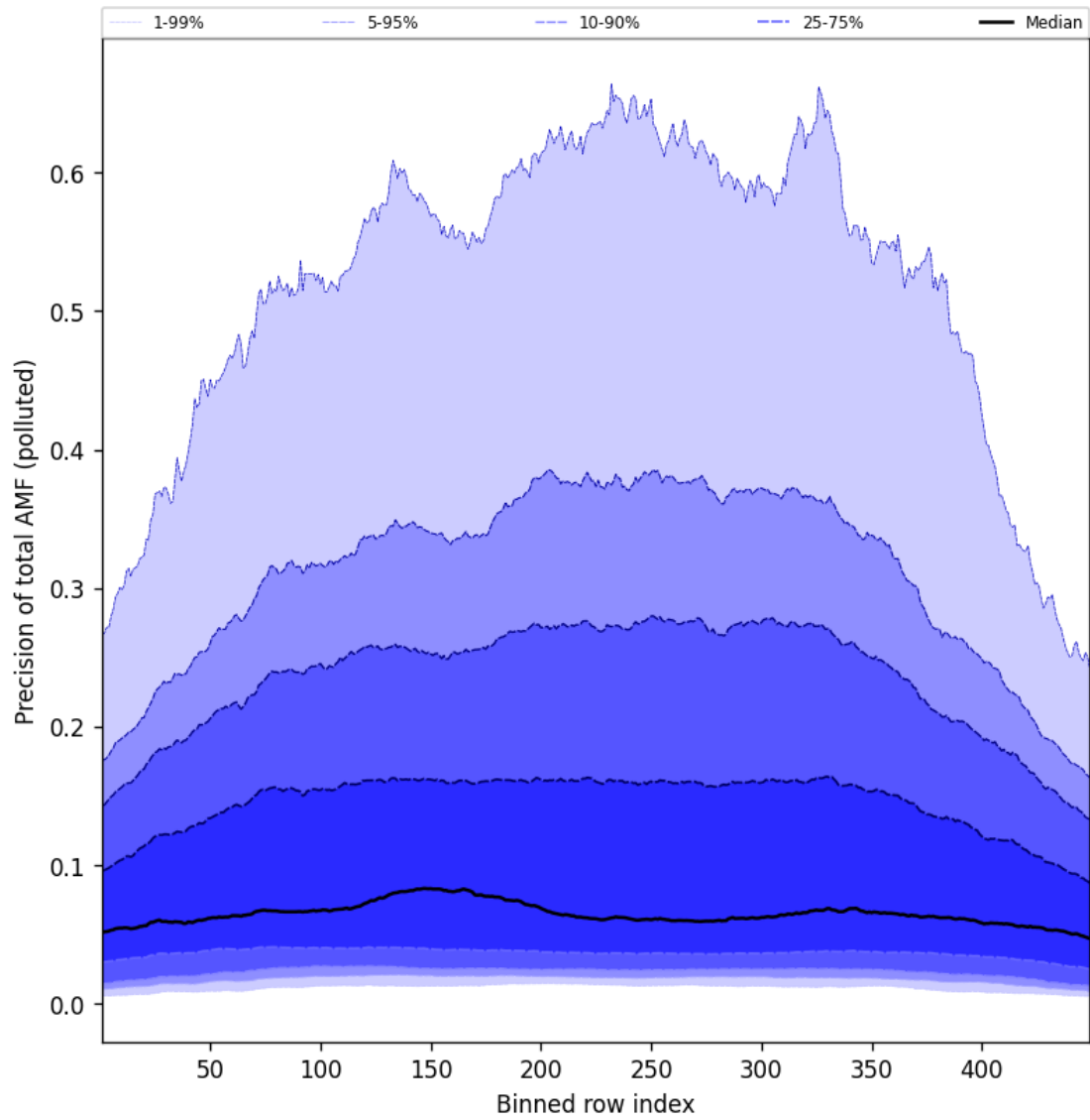
Figure 108: Along track statistics of “Precision of total AMF (polluted)” for 2025-04-05 to 2025-04-06
