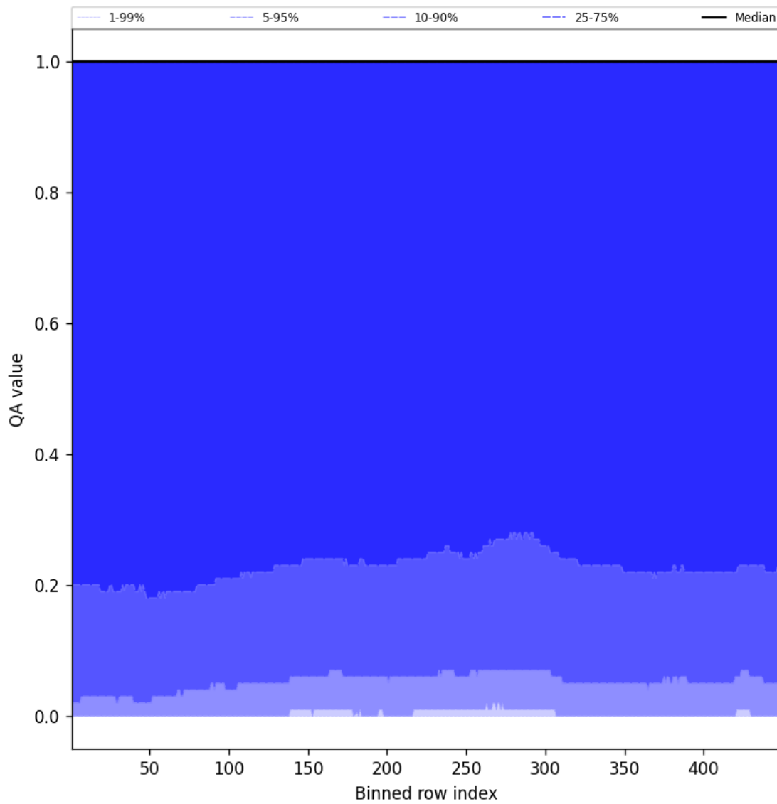
Figure 84: Along track statistics of “QA value” for 2025-04-05 to 2025-04-06
