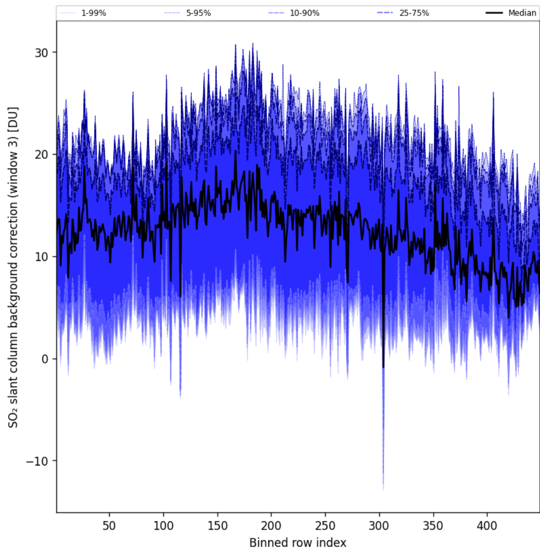
Figure 101: Along track statistics of “SO 2 slant column background correction (window 3)” for 2025-04-05 to 2025-04-06
