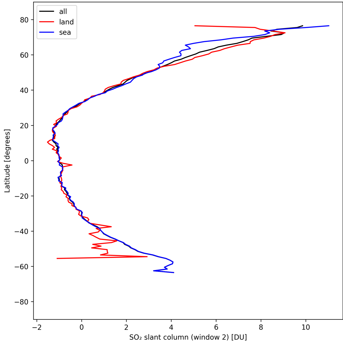
Figure 40: Zonal average of “SO 2 slant column (window 2)” for 2025-04-05 to 2025-04-06.
