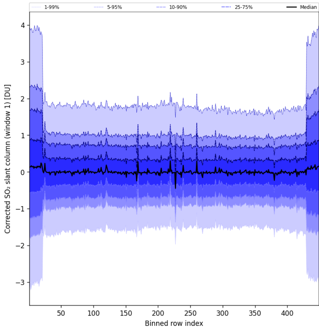
Figure 92: Along track statistics of “Corrected SO 2 slant column (window 1)” for 2025-04-05 to 2025-04-06
