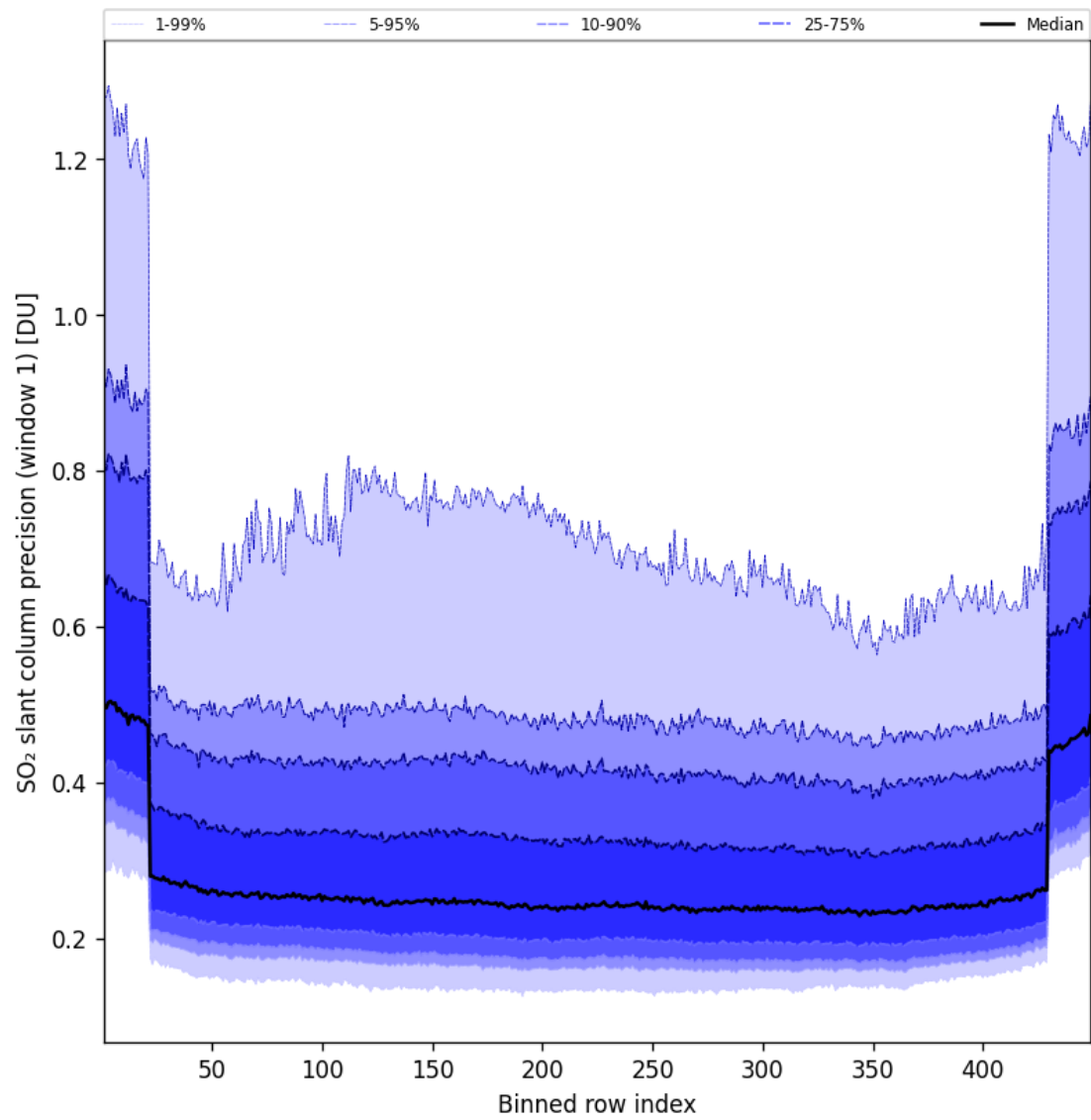
Figure 91: Along track statistics of “SO 2 slant column precision (window 1)” for 2025-04-05 to 2025-04-06
