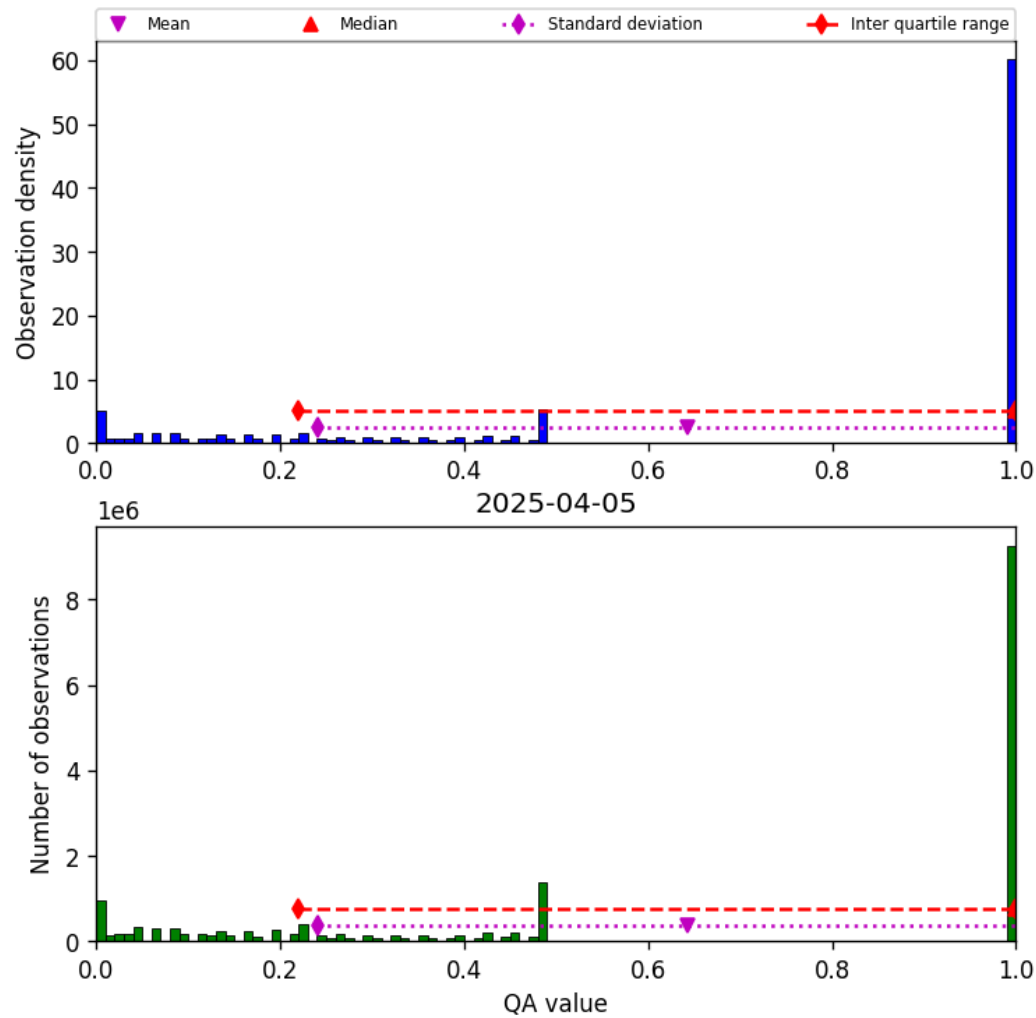
Figure 57: Histogram of “QA value” for 2025-04-05 to 2025-04-06
