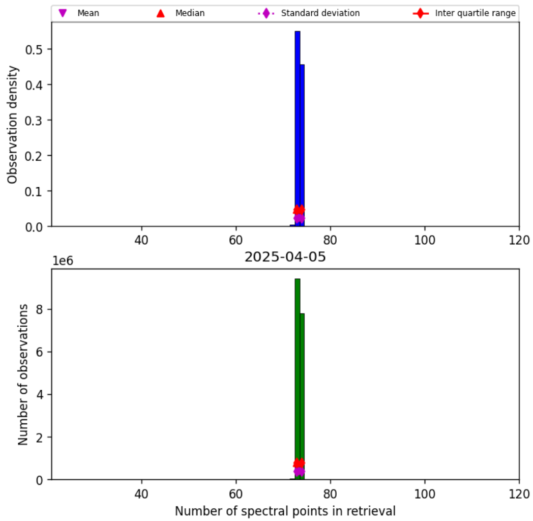
Figure 83: Histogram of “Number of spectral points in retrieval” for 2025-04-05 to 2025-04-06
