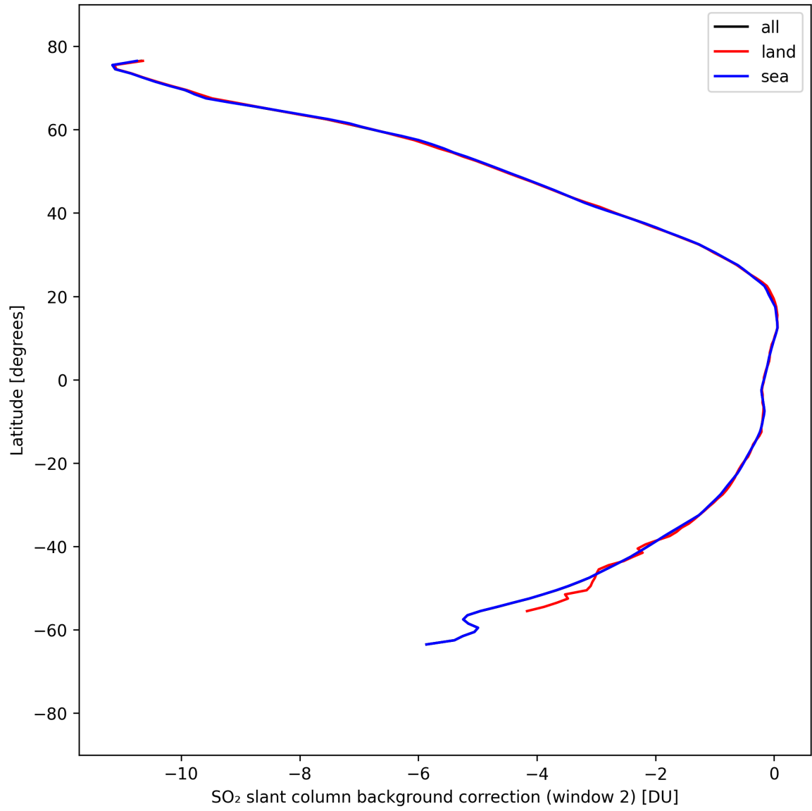
Figure 43: Zonal average of “SO 2 slant column background correction (window 2)” for 2025-04-05 to 2025-04-06.
