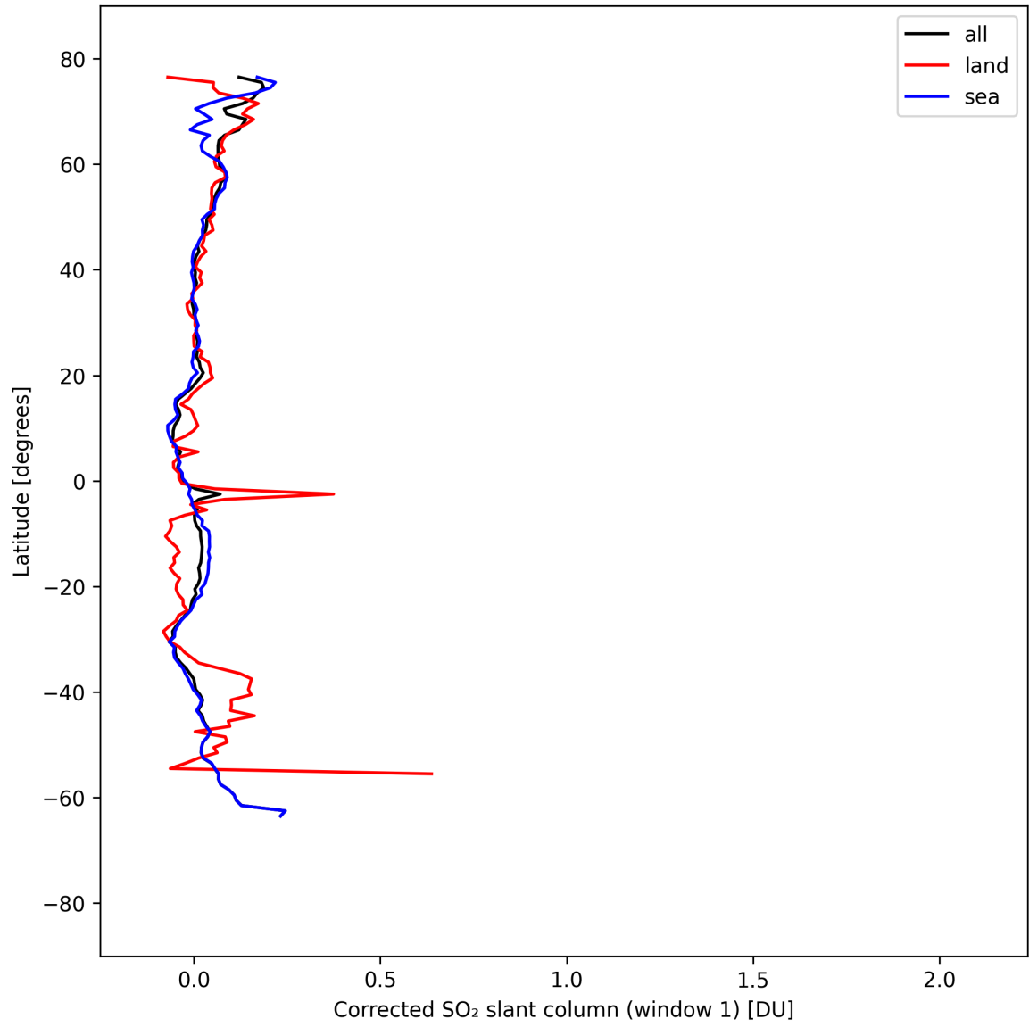
Figure 38: Zonal average of “Corrected SO 2 slant column (window 1)” for 2025-04-05 to 2025-04-06.
