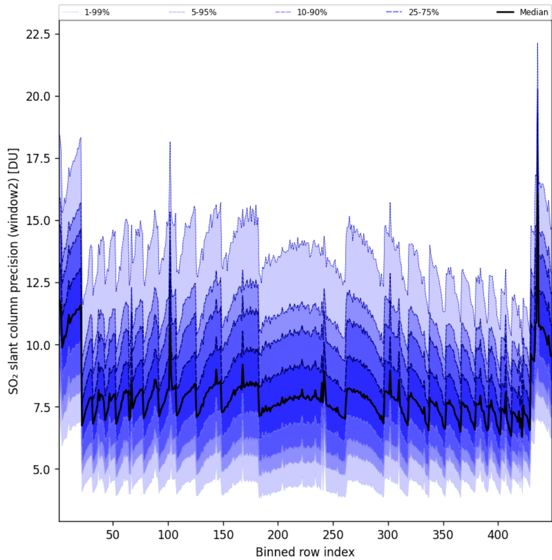
Figure 95: Along track statistics of “SO 2 slant column precision (window2)” for 2025-04-05 to 2025-04-06
