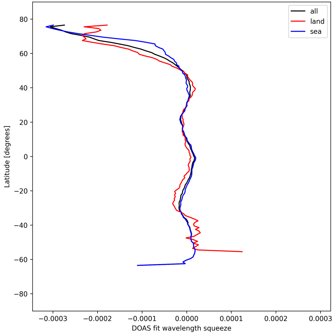
Figure 51: Zonal average of “DOAS fit wavelength squeeze” for 2025-04-05 to 2025-04-06.
