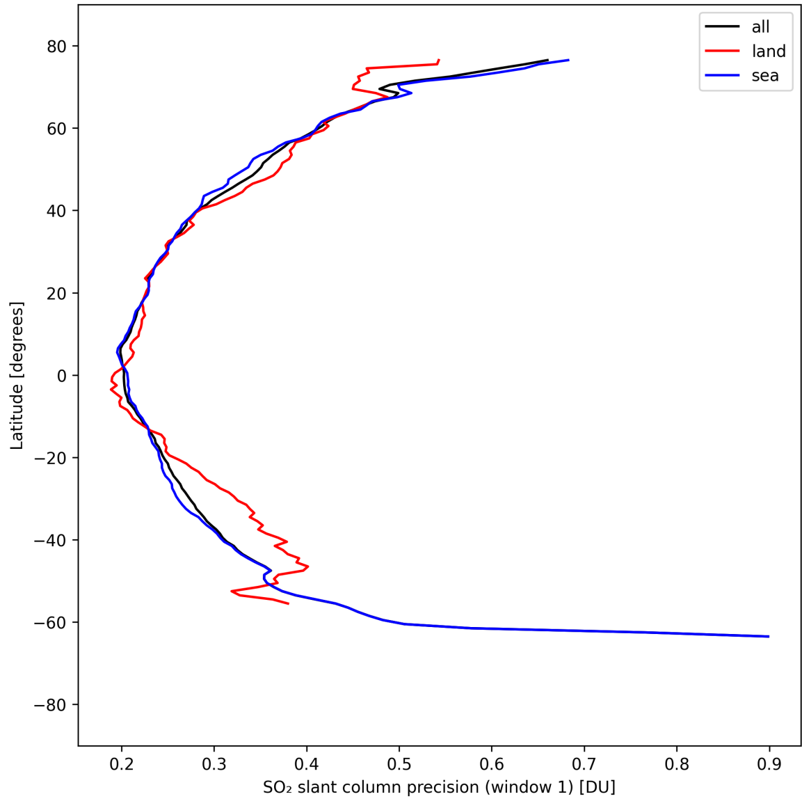
Figure 37: Zonal average of “SO 2 slant column precision (window 1)” for 2025-04-05 to 2025-04-06.
