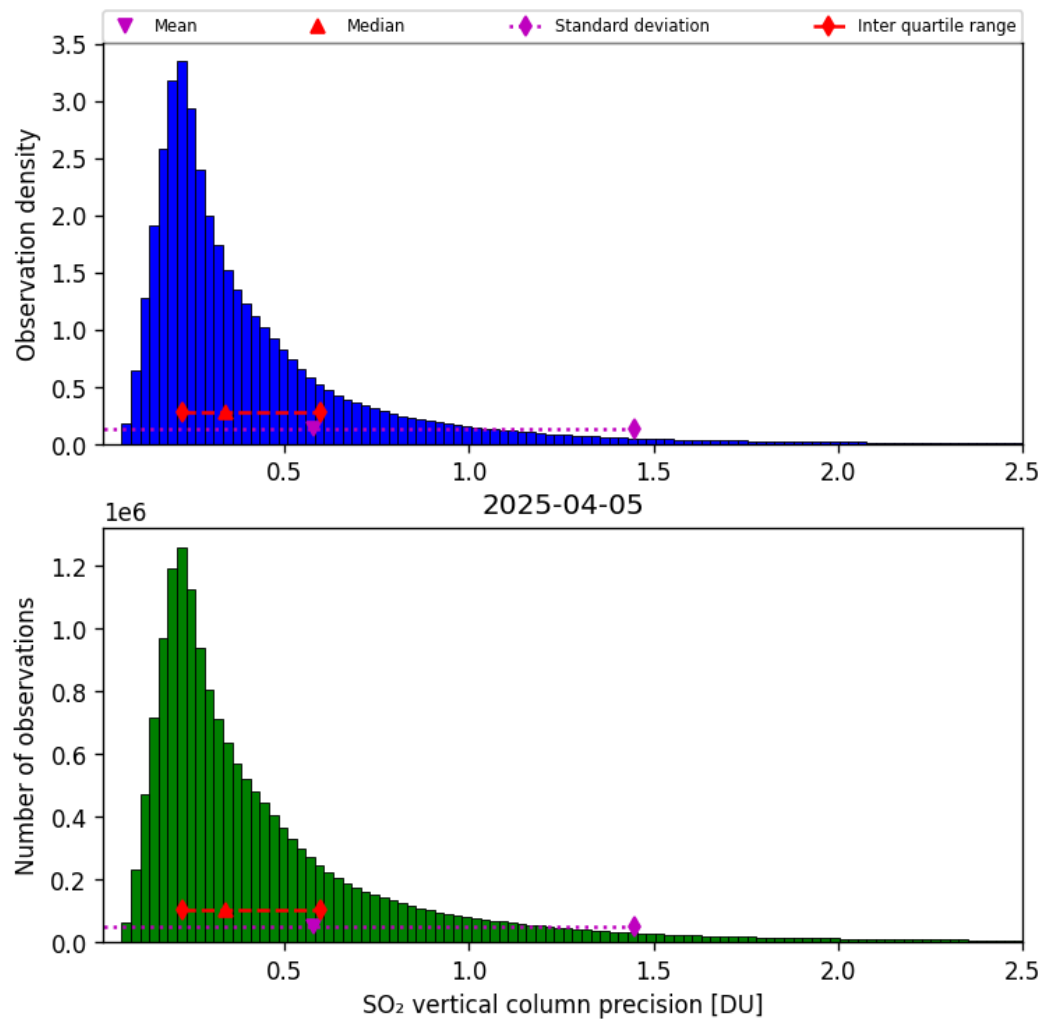
Figure 59: Histogram of “SO 2 vertical column precision” for 2025-04-05 to 2025-04-06
