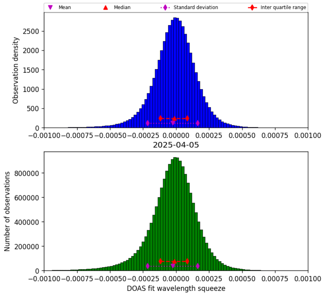
Figure 78: Histogram of “DOAS fit wavelength squeeze” for 2025-04-05 to 2025-04-06
