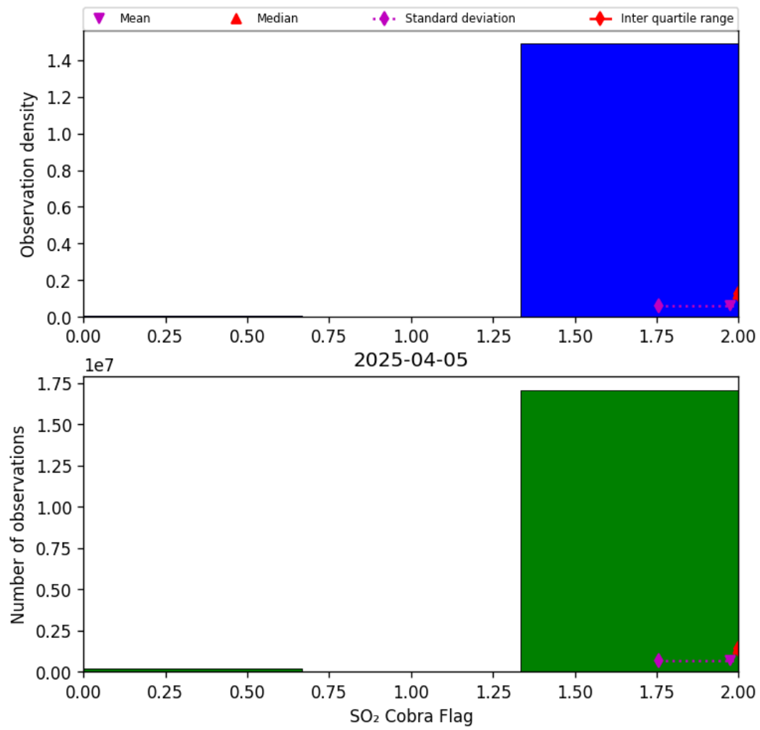
Figure 75: Histogram of “SO 2 Cobra Flag” for 2025-04-05 to 2025-04-06
