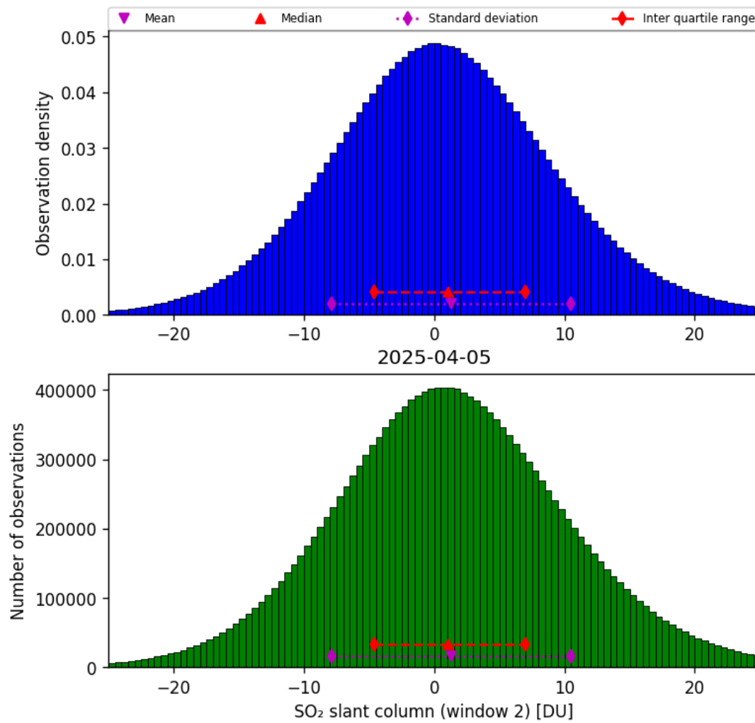
Figure 67: Histogram of “SO 2 slant column (window 2)” for 2025-04-05 to 2025-04-06
