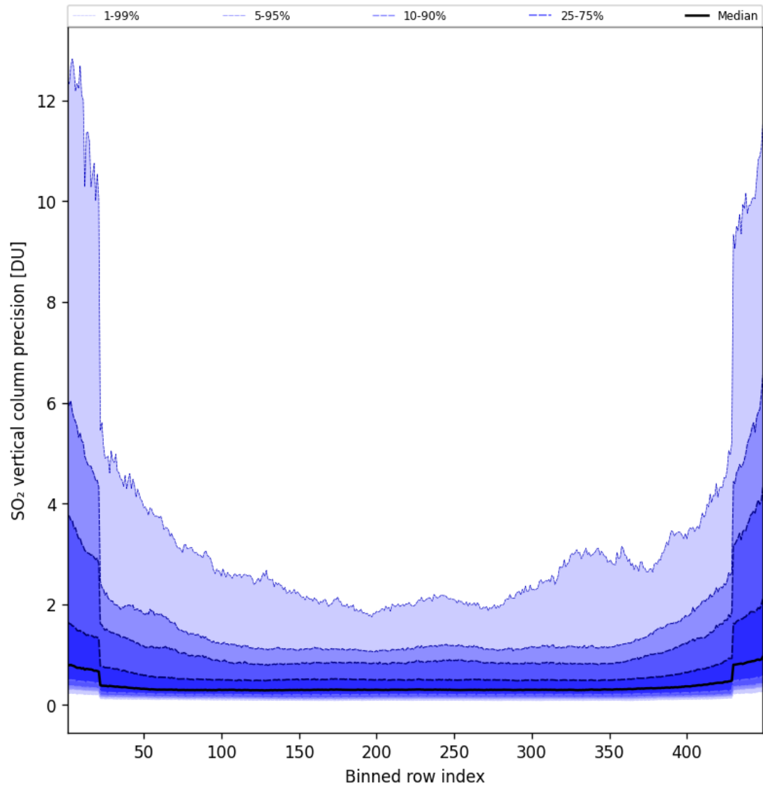
Figure 86: Along track statistics of “SO 2 vertical column precision” for 2025-04-05 to 2025-04-06
