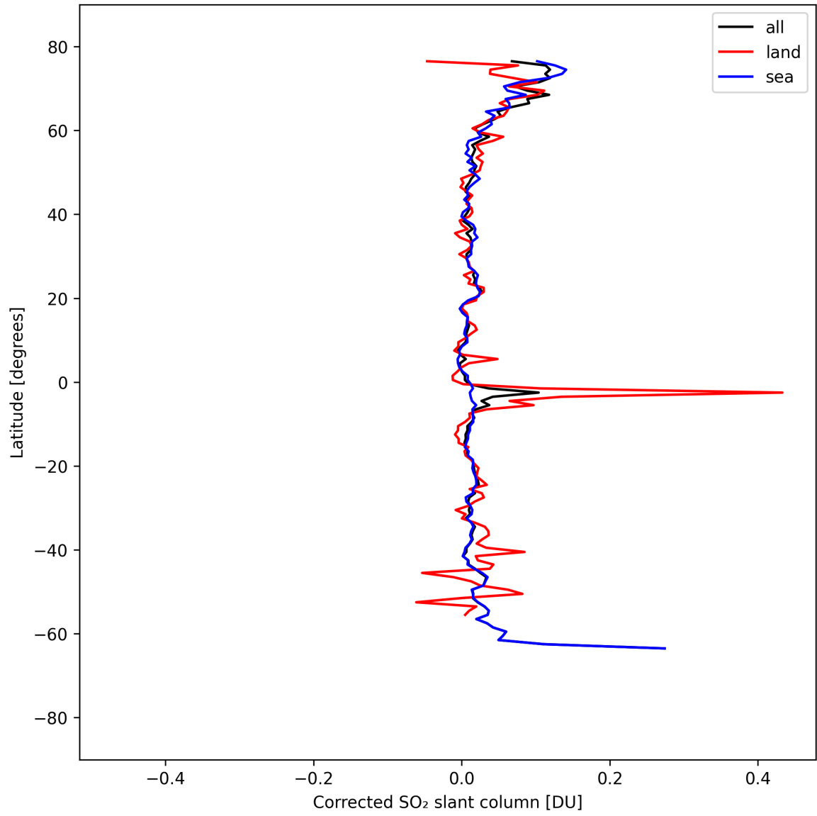
Figure 33: Zonal average of "Corrected SO 2 slant column" for 2025-04-05 to 2025-04-06.
