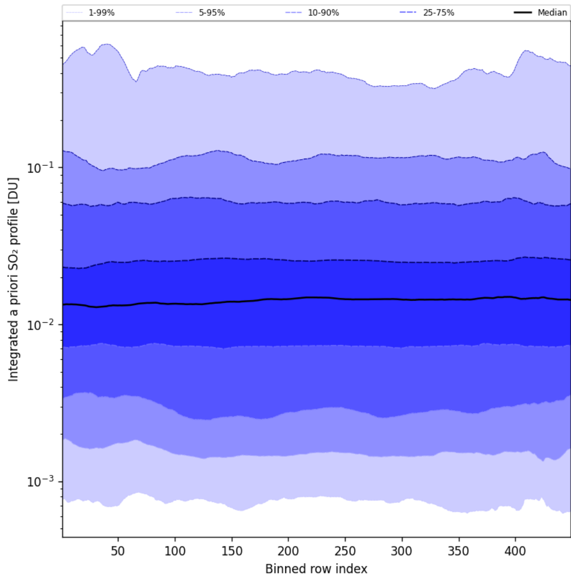
Figure 103: Along track statistics of “Integrated a priori SO 2 profile” for 2025-04-05 to 2025-04-06
