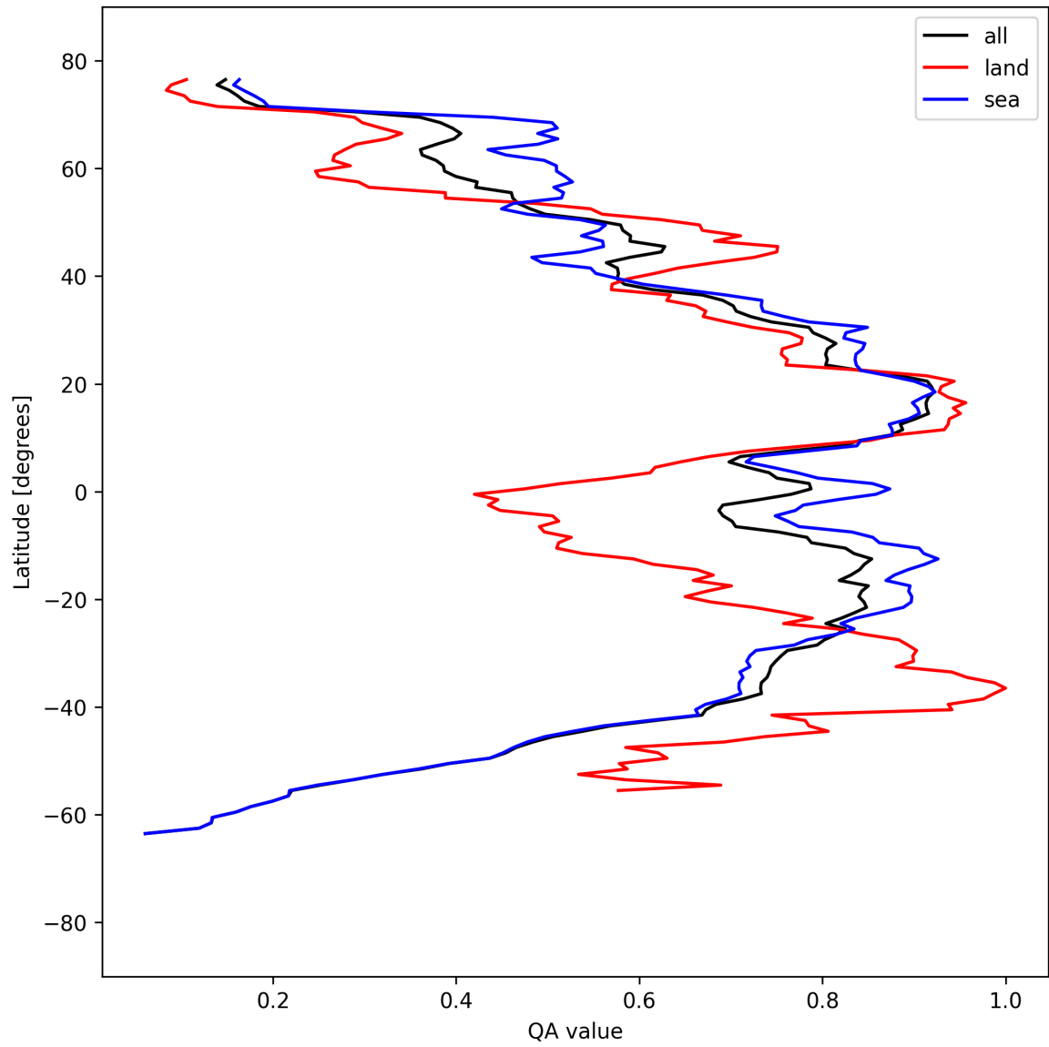
Figure 30: Zonal average of “QA value” for 2025-04-05 to 2025-04-06.
