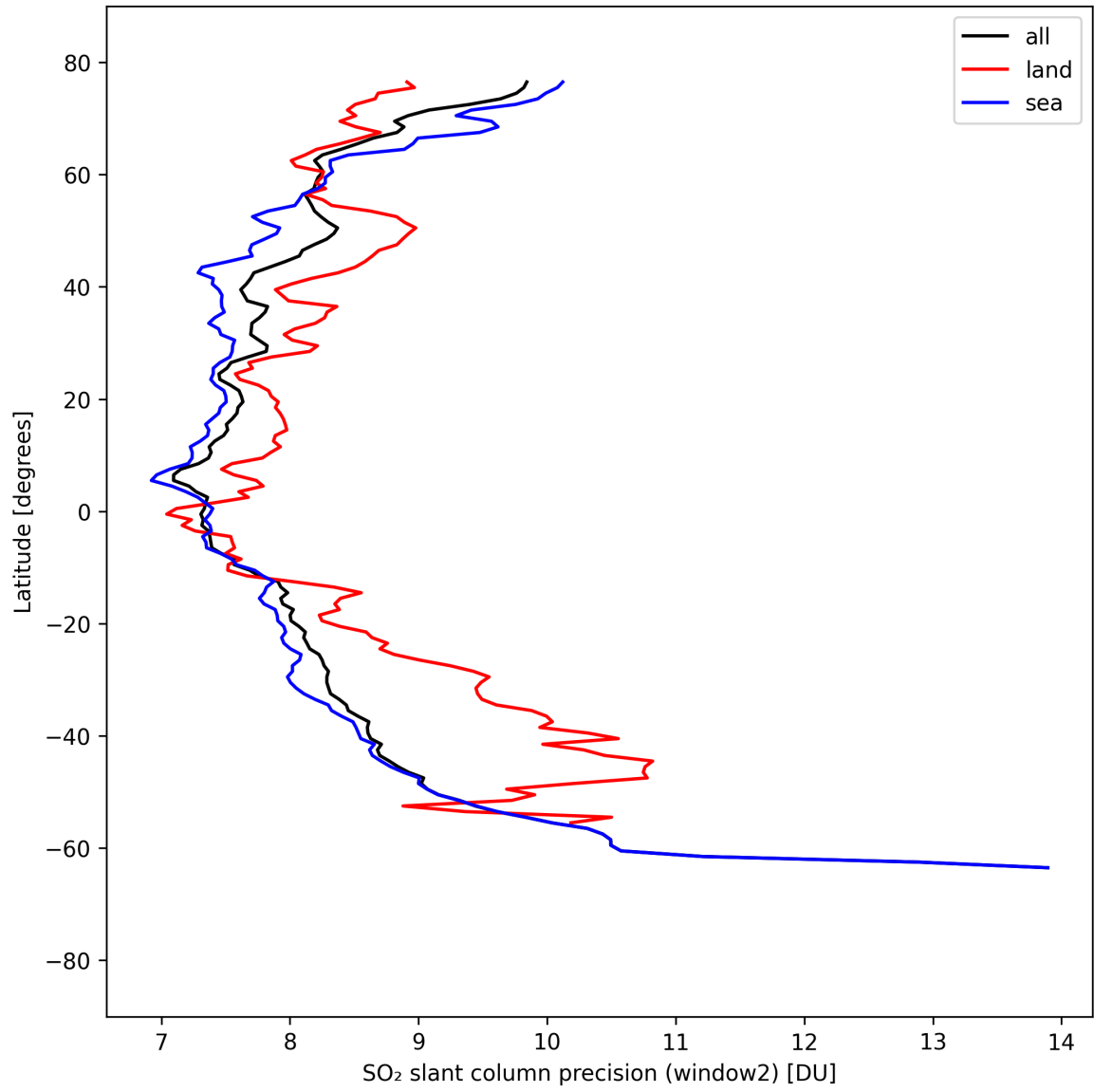
Figure 41: Zonal average of “SO 2 slant column precision (window2)” for 2025-04-05 to 2025-04-06.
