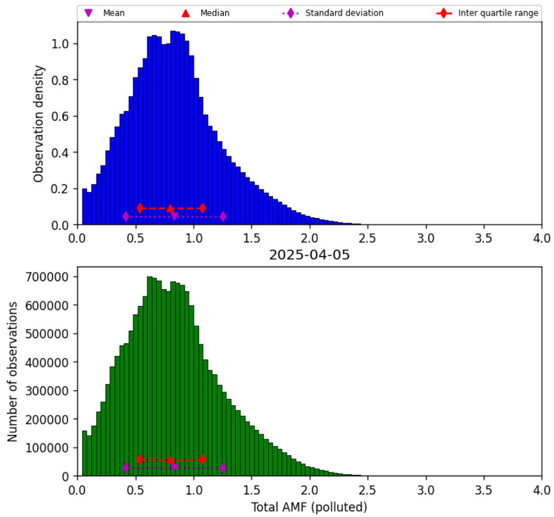
Figure 80: Histogram of “Total AMF (polluted)” for 2025-04-05 to 2025-04-06
