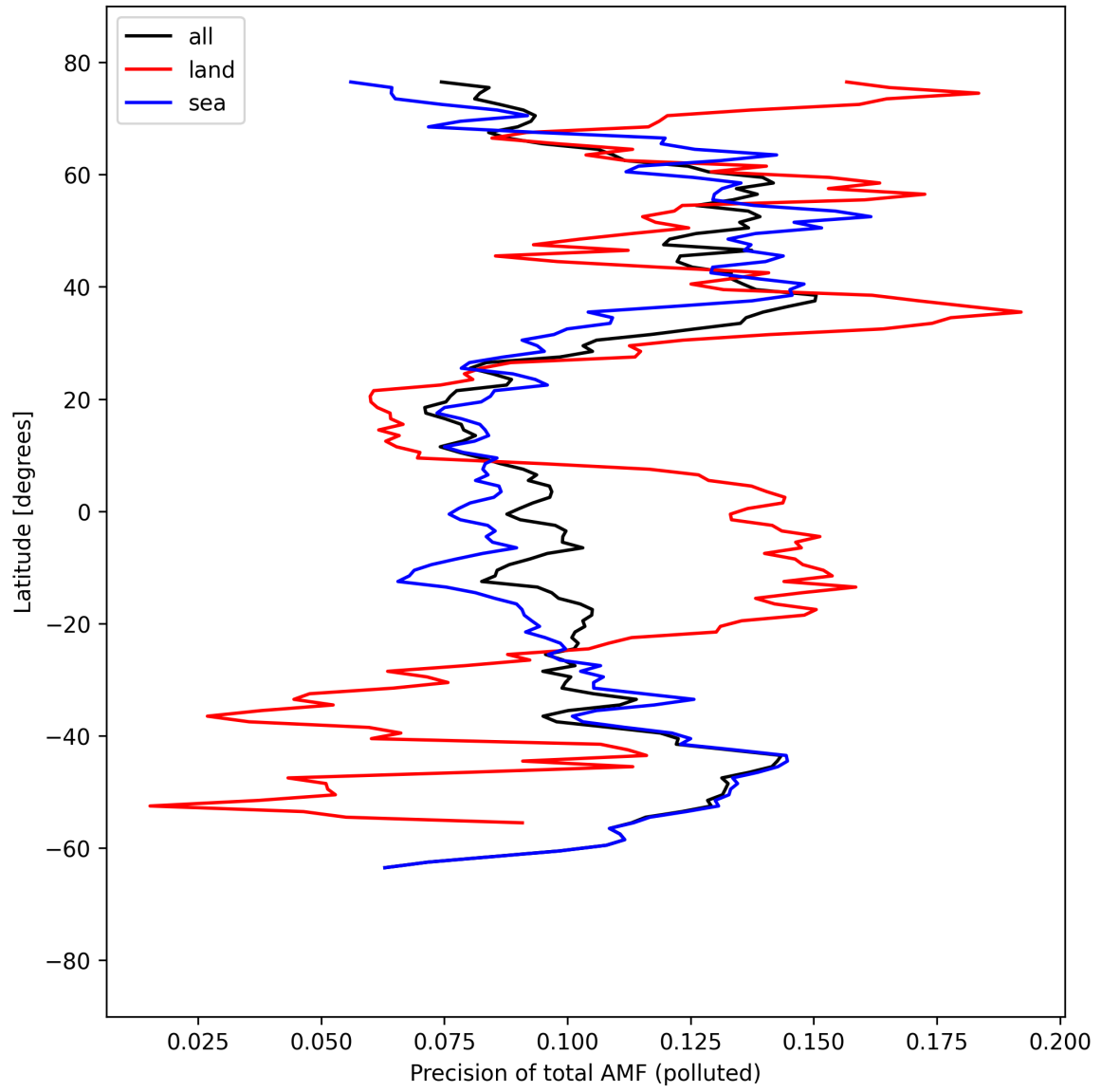
Figure 54: Zonal average of “Precision of total AMF (polluted)” for 2025-04-05 to 2025-04-06.
