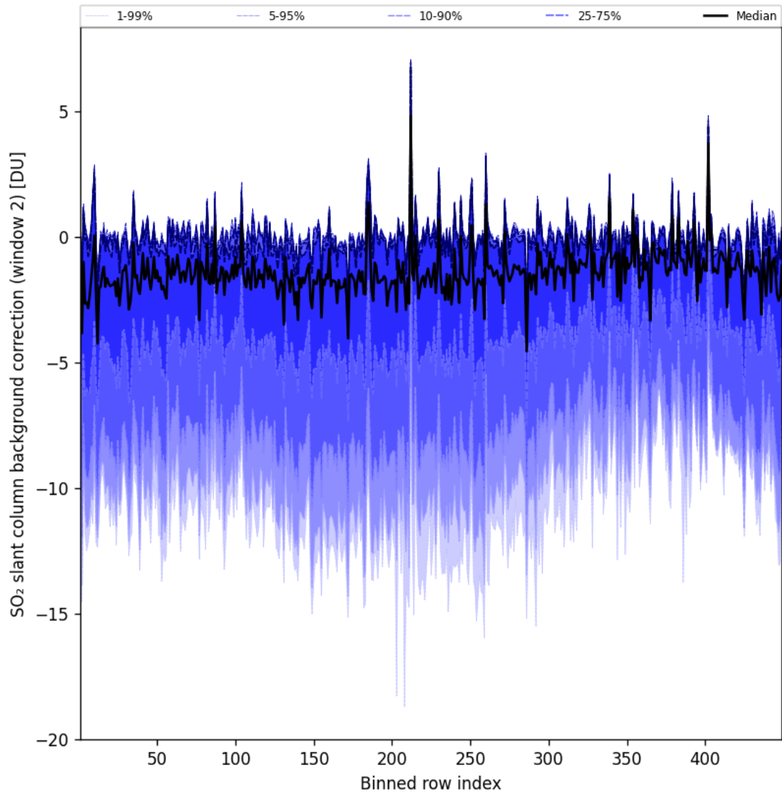
Figure 97: Along track statistics of “SO 2 slant column background correction (window 2)” for 2025-04-05 to 2025-04-06
