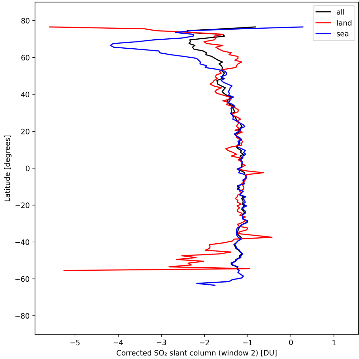
Figure 42: Zonal average of “Corrected SO 2 slant column (window 2)” for 2025-04-05 to 2025-04-06.
