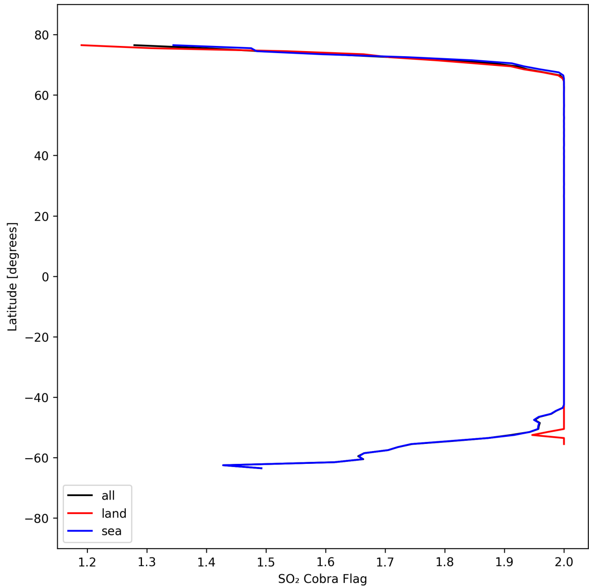
Figure 48: Zonal average of "SO 2 Cobra Flag" for 2025-04-05 to 2025-04-06.
