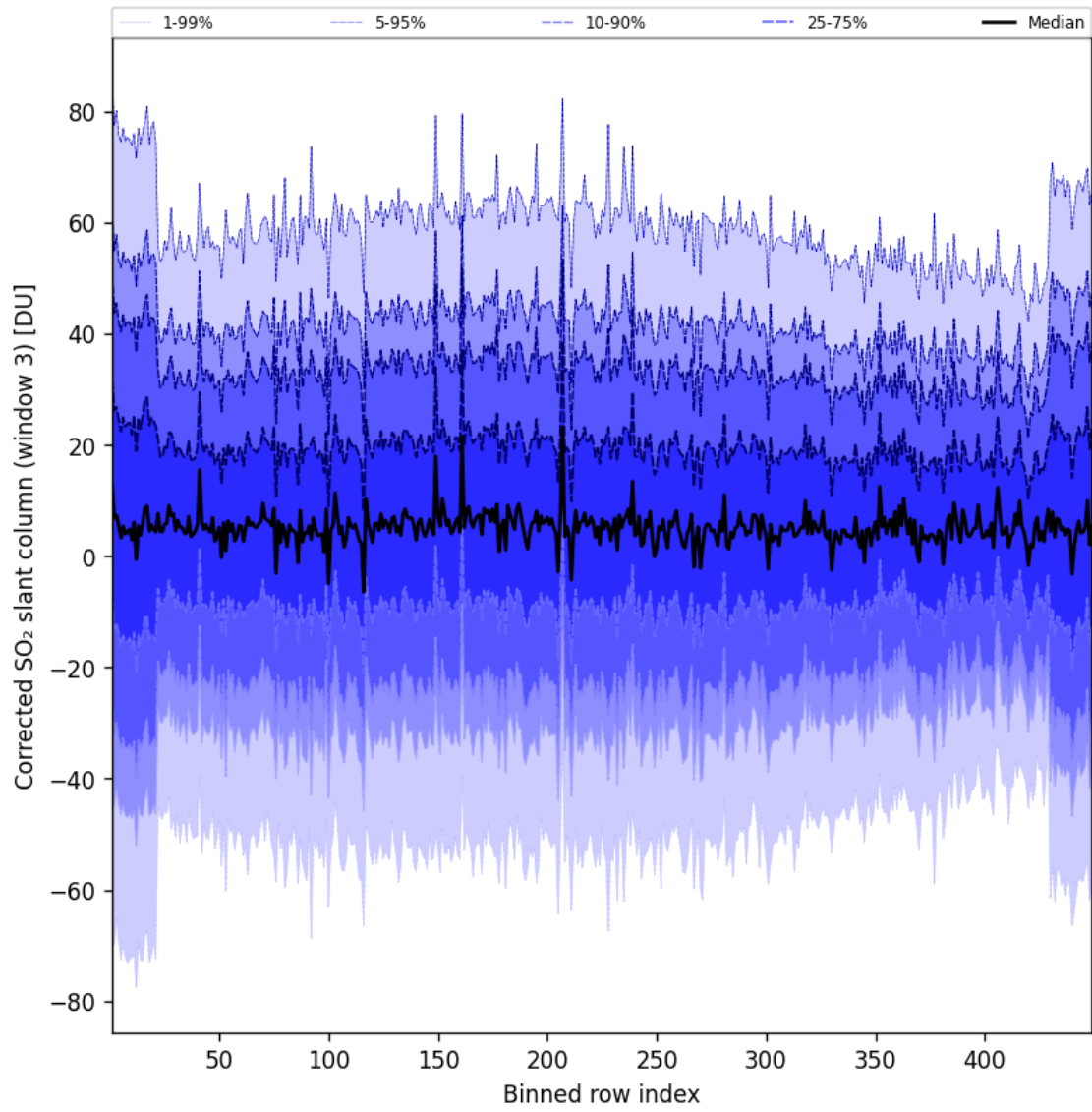
Figure 100: Along track statistics of “Corrected SO 2 slant column (window 3)” for 2025-04-05 to 2025-04-06
