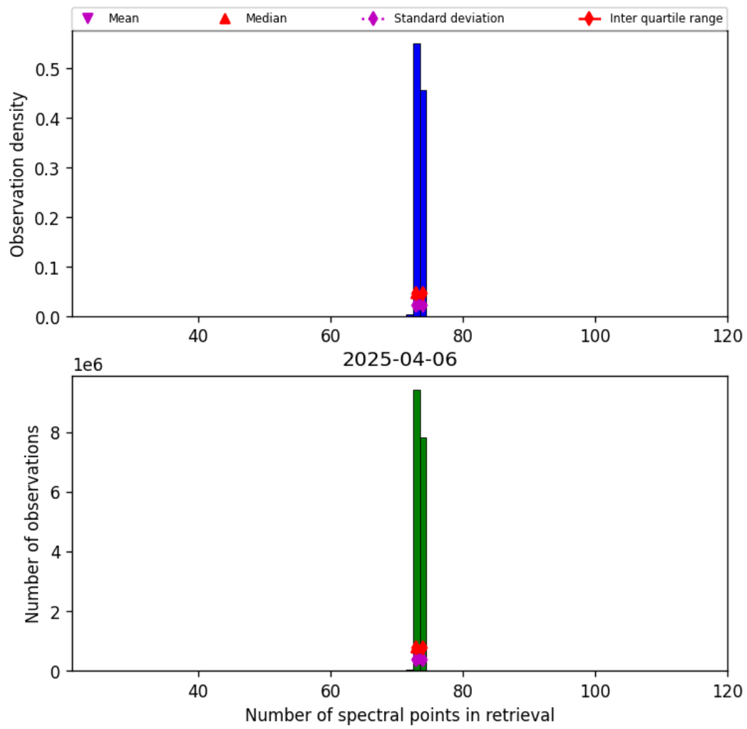
Figure 83: Histogram of “Number of spectral points in retrieval” for 2025-04-06 to 2025-04-06
