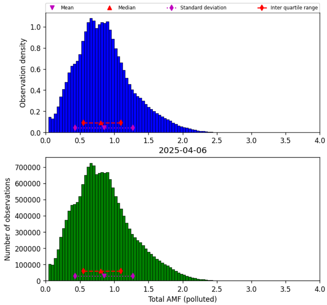
Figure 80: Histogram of “Total AMF (polluted)” for 2025-04-06 to 2025-04-06
