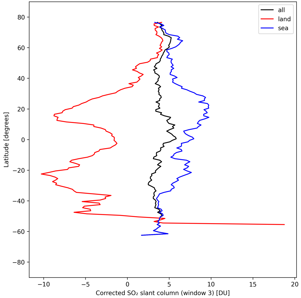
Figure 46: Zonal average of “Corrected SO 2 slant column (window 3)” for 2025-04-06 to 2025-04-06.
