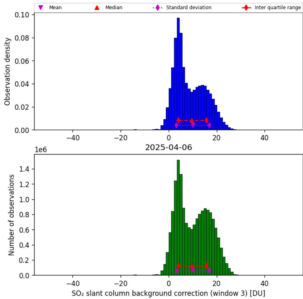
Figure 74: Histogram of “SO 2 slant column background correction (window 3)” for 2025-04-06 to 2025-04-06
