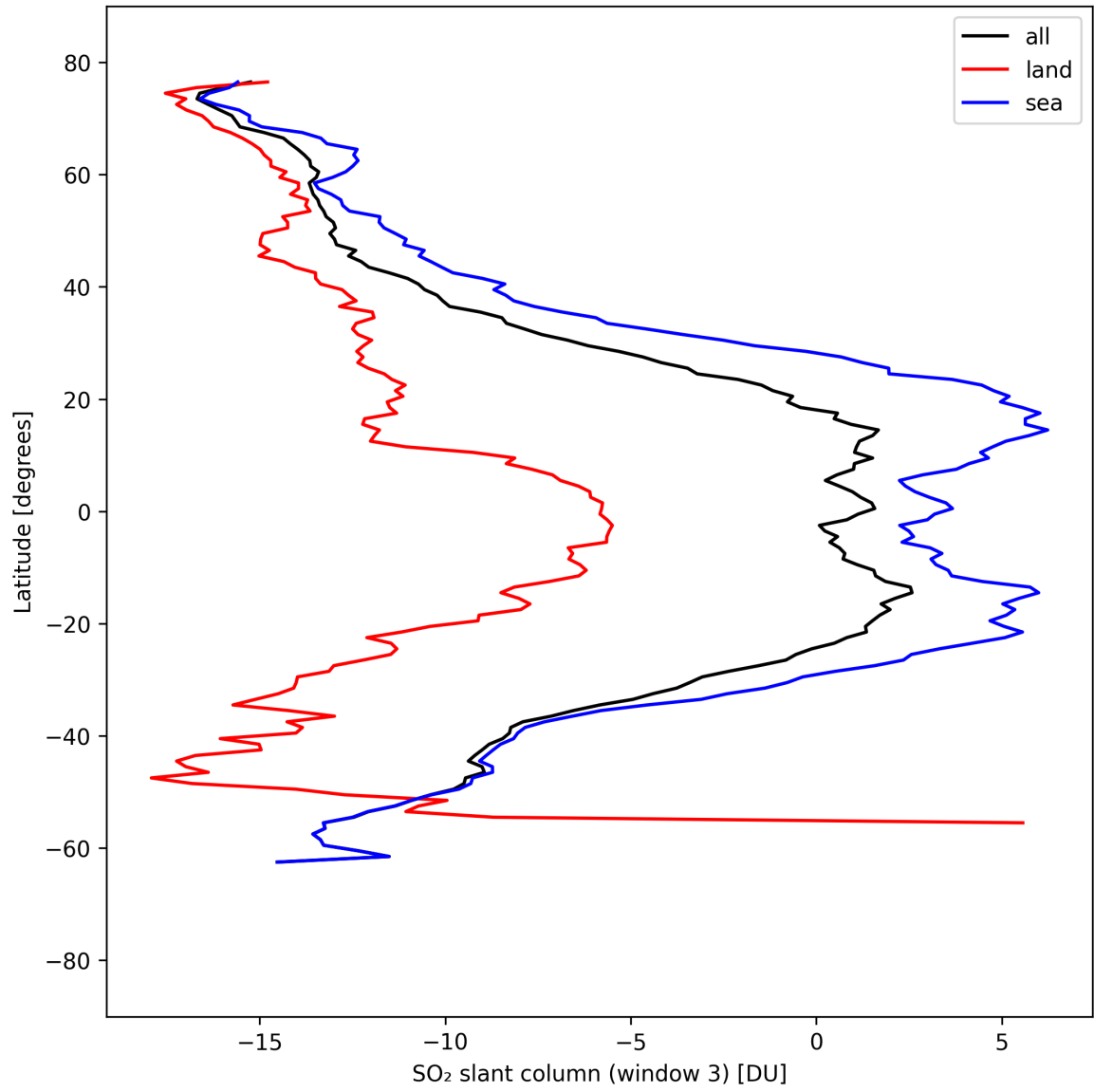
Figure 44: Zonal average of “SO 2 slant column (window 3)” for 2025-04-06 to 2025-04-06.
