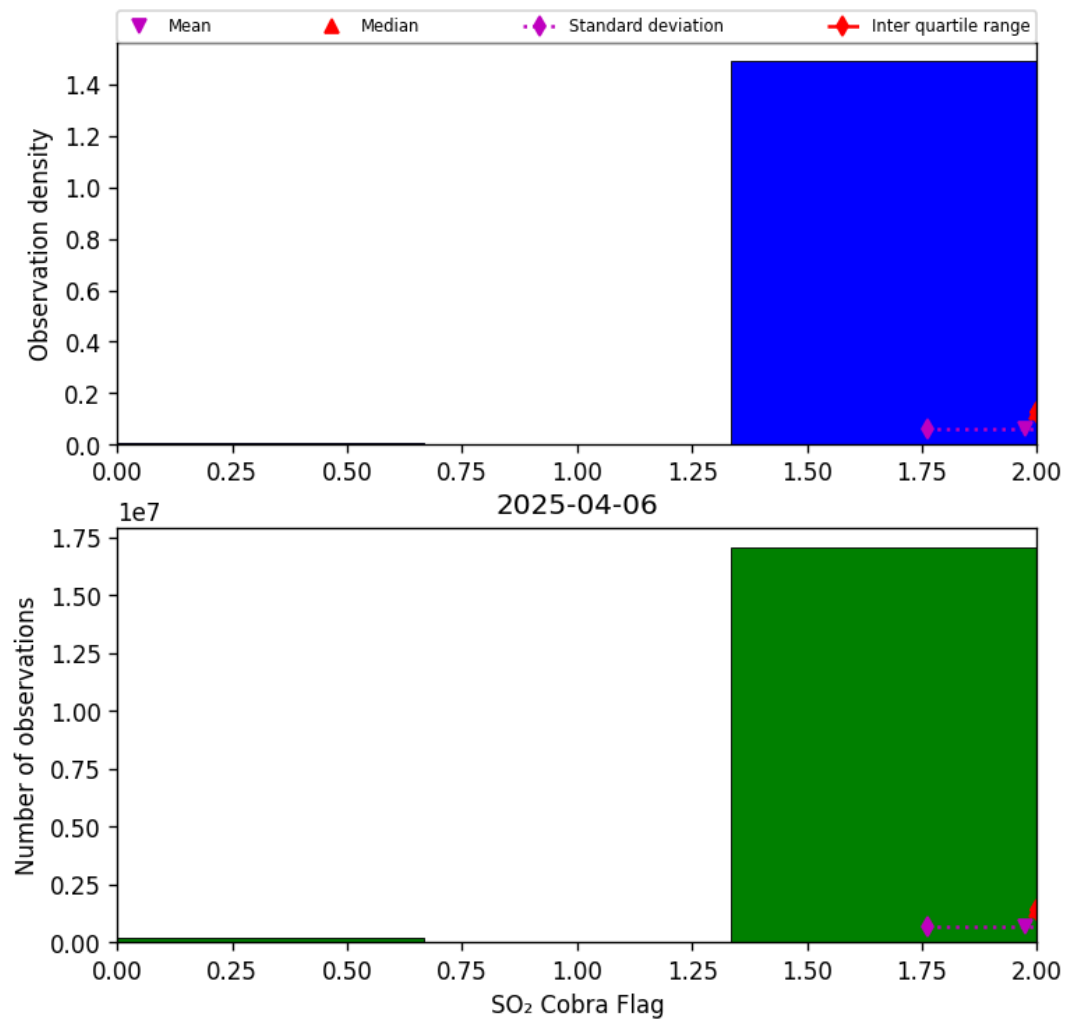
Figure 75: Histogram of “SO 2 Cobra Flag” for 2025-04-06 to 2025-04-06
