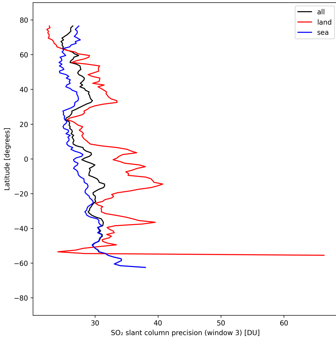
Figure 45: Zonal average of “SO 2 slant column precision (window 3)” for 2025-04-06 to 2025-04-06.
