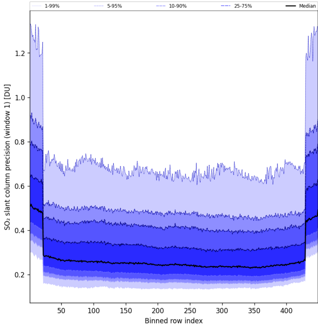
Figure 91: Along track statistics of “SO 2 slant column precision (window 1)” for 2025-04-06 to 2025-04-06
