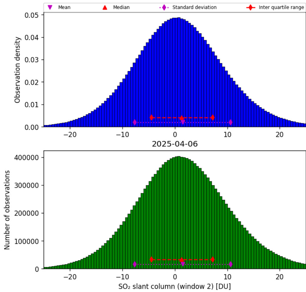
Figure 67: Histogram of “SO 2 slant column (window 2)” for 2025-04-06 to 2025-04-06
