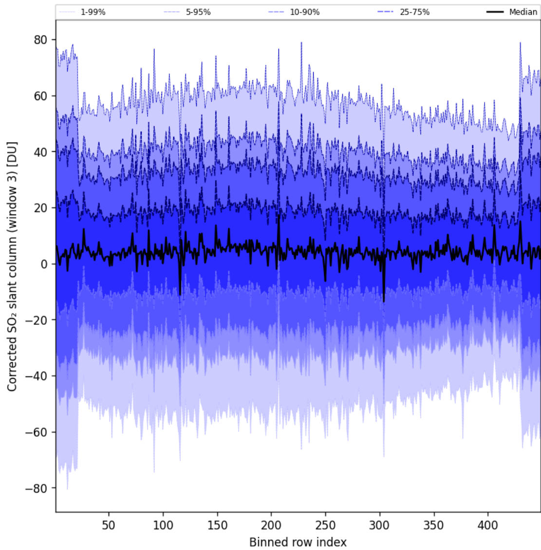
Figure 100: Along track statistics of “Corrected SO 2 slant column (window 3)” for 2025-04-06 to 2025-04-06
