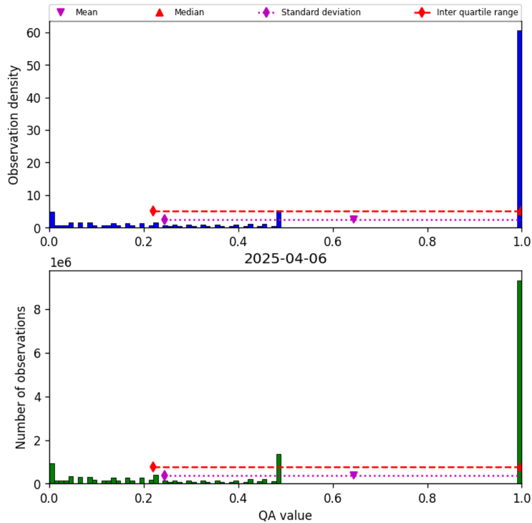
Figure 57: Histogram of “QA value” for 2025-04-06 to 2025-04-06
