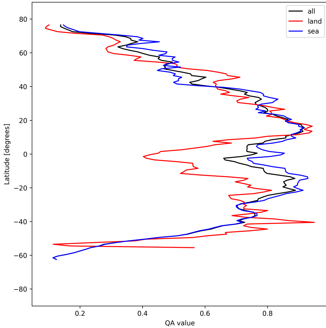
Figure 30: Zonal average of “QA value” for 2025-04-06 to 2025-04-06.
