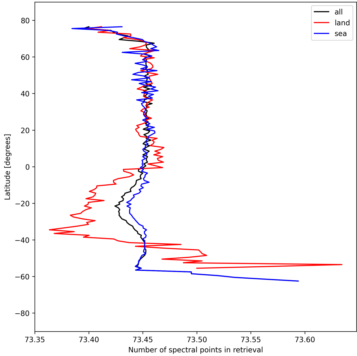
Figure 56: Zonal average of “Number of spectral points in retrieval” for 2025-04-06 to 2025-04-06.
