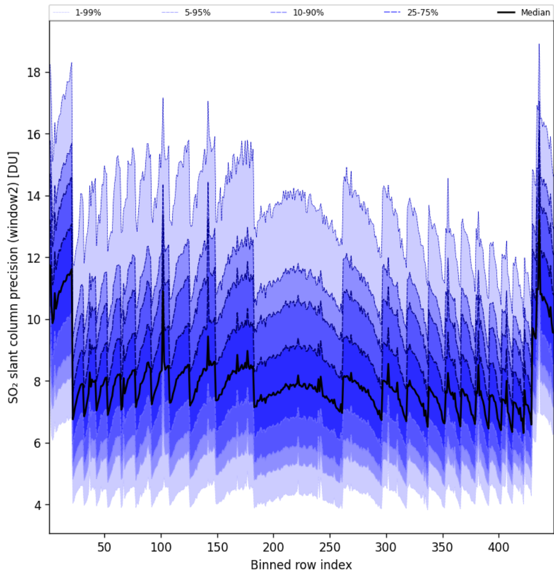
Figure 95: Along track statistics of “SO 2 slant column precision (window2)” for 2025-04-06 to 2025-04-06
