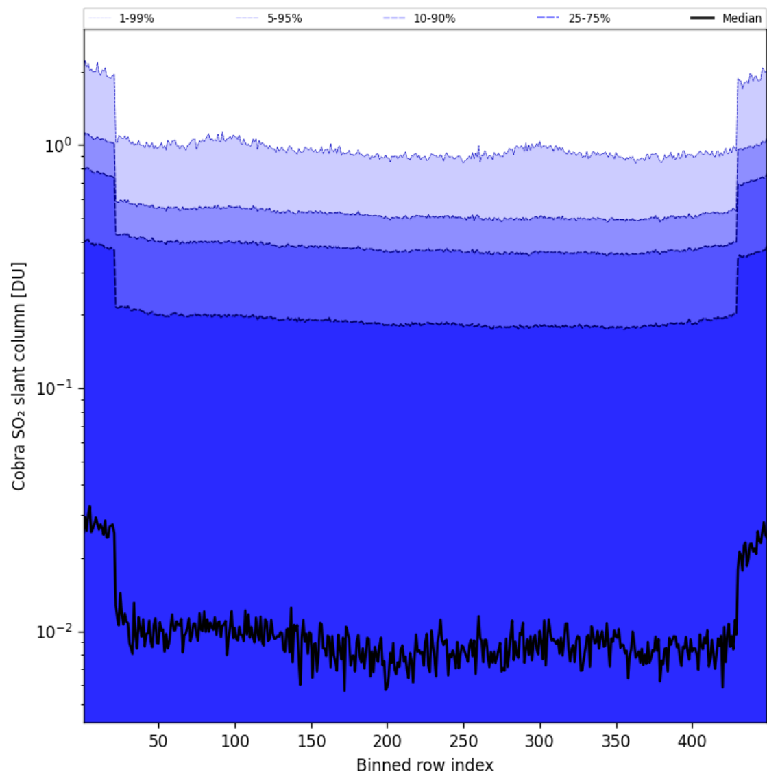
Figure 88: Along track statistics of “Cobra SO 2 slant column” for 2025-04-06 to 2025-04-06
