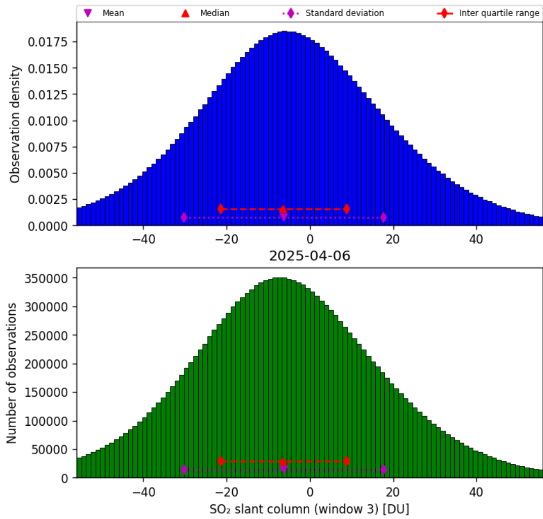
Figure 71: Histogram of “SO 2 slant column (window 3)” for 2025-04-06 to 2025-04-06
