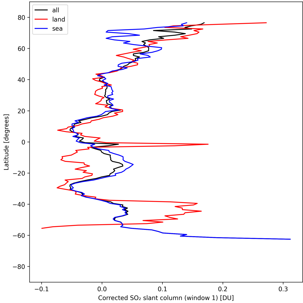
Figure 38: Zonal average of “Corrected SO 2 slant column (window 1)” for 2025-04-06 to 2025-04-06.
