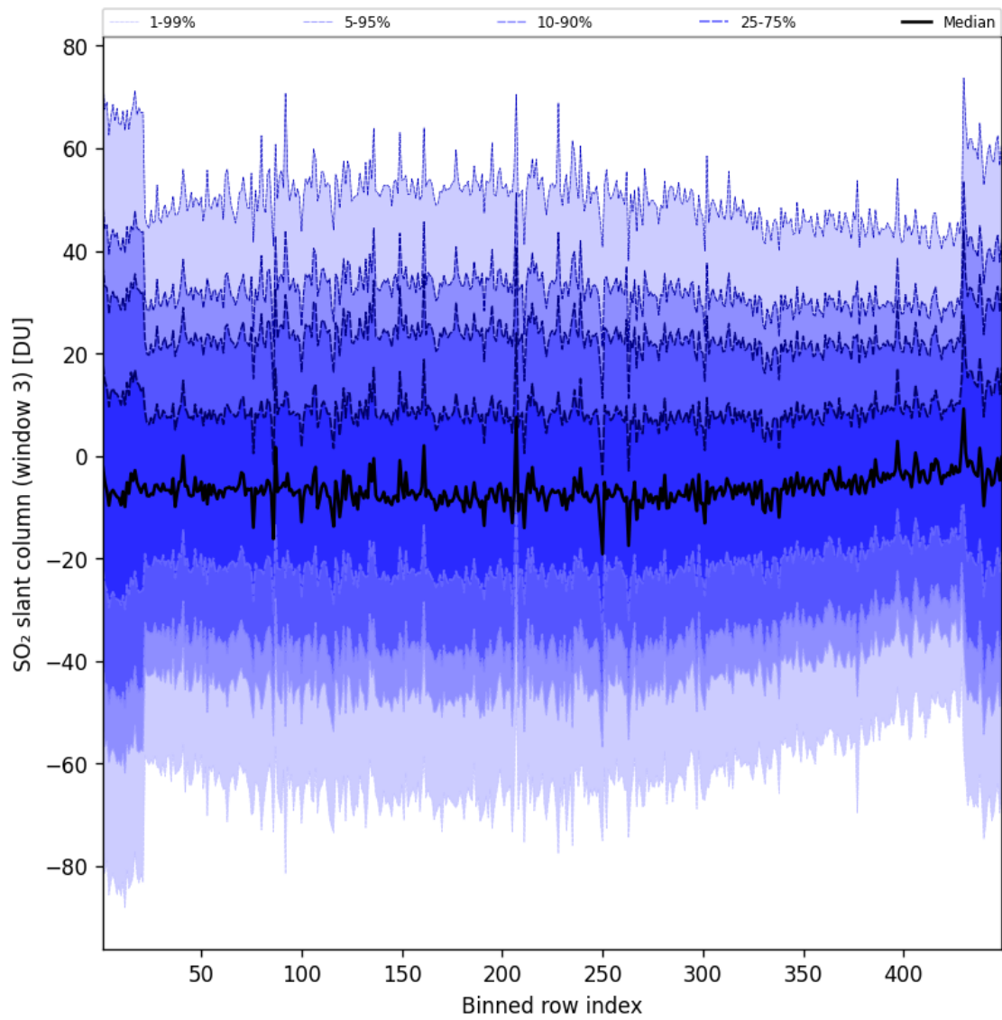
Figure 98: Along track statistics of “SO 2 slant column (window 3)” for 2025-04-06 to 2025-04-06
