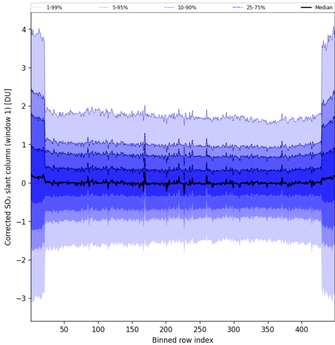
Figure 92: Along track statistics of “Corrected SO 2 slant column (window 1)” for 2025-04-06 to 2025-04-06
