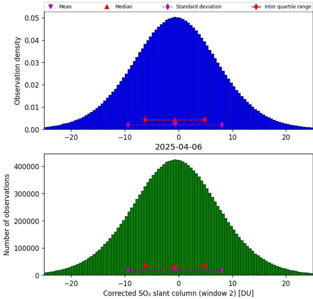
Figure 69: Histogram of “Corrected SO 2 slant column (window 2)” for 2025-04-06 to 2025-04-06
