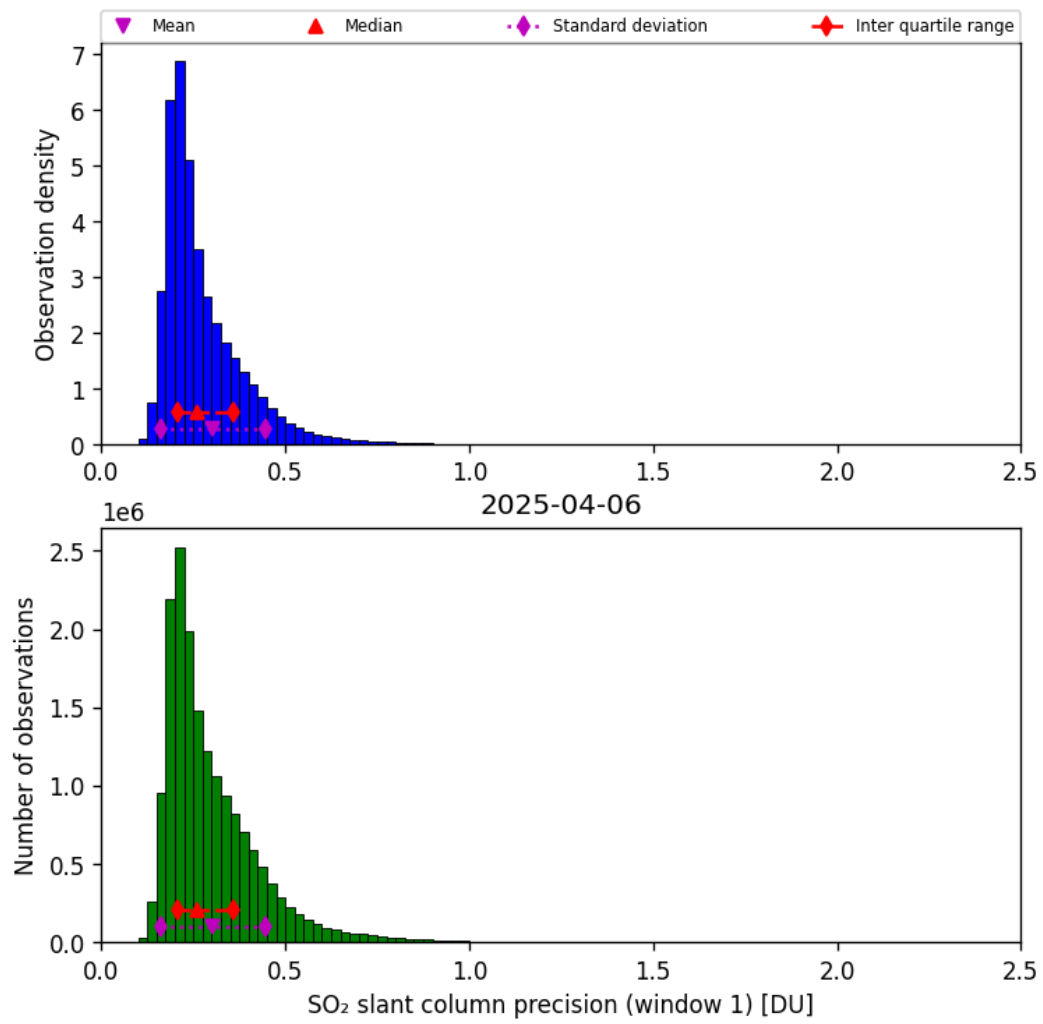
Figure 64: Histogram of “SO 2 slant column precision (window 1)” for 2025-04-06 to 2025-04-06
