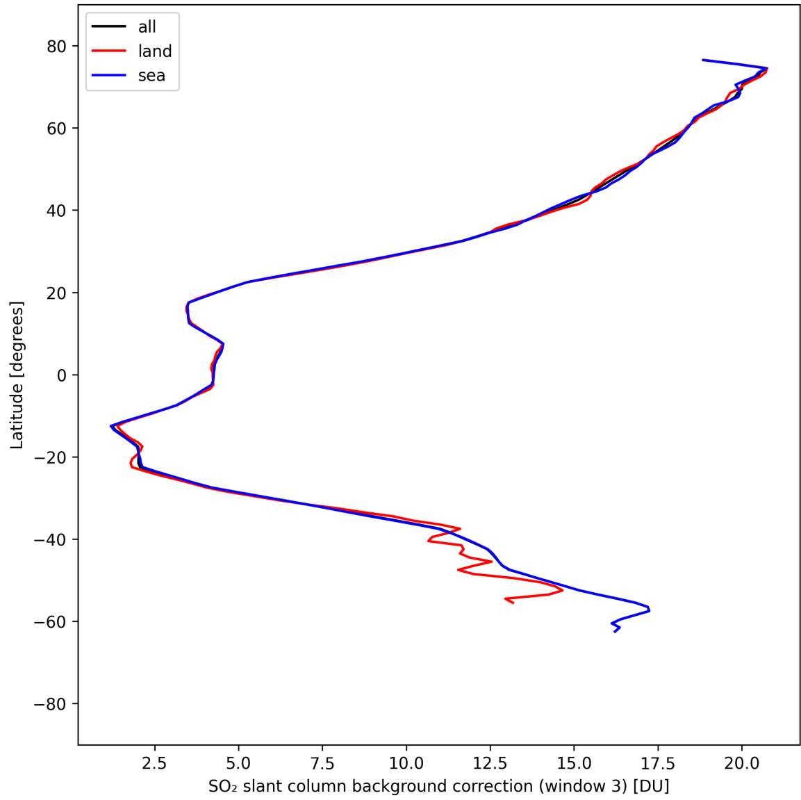
Figure 47: Zonal average of “SO 2 slant column background correction (window 3)” for 2025-04-06 to 2025-04-06.
