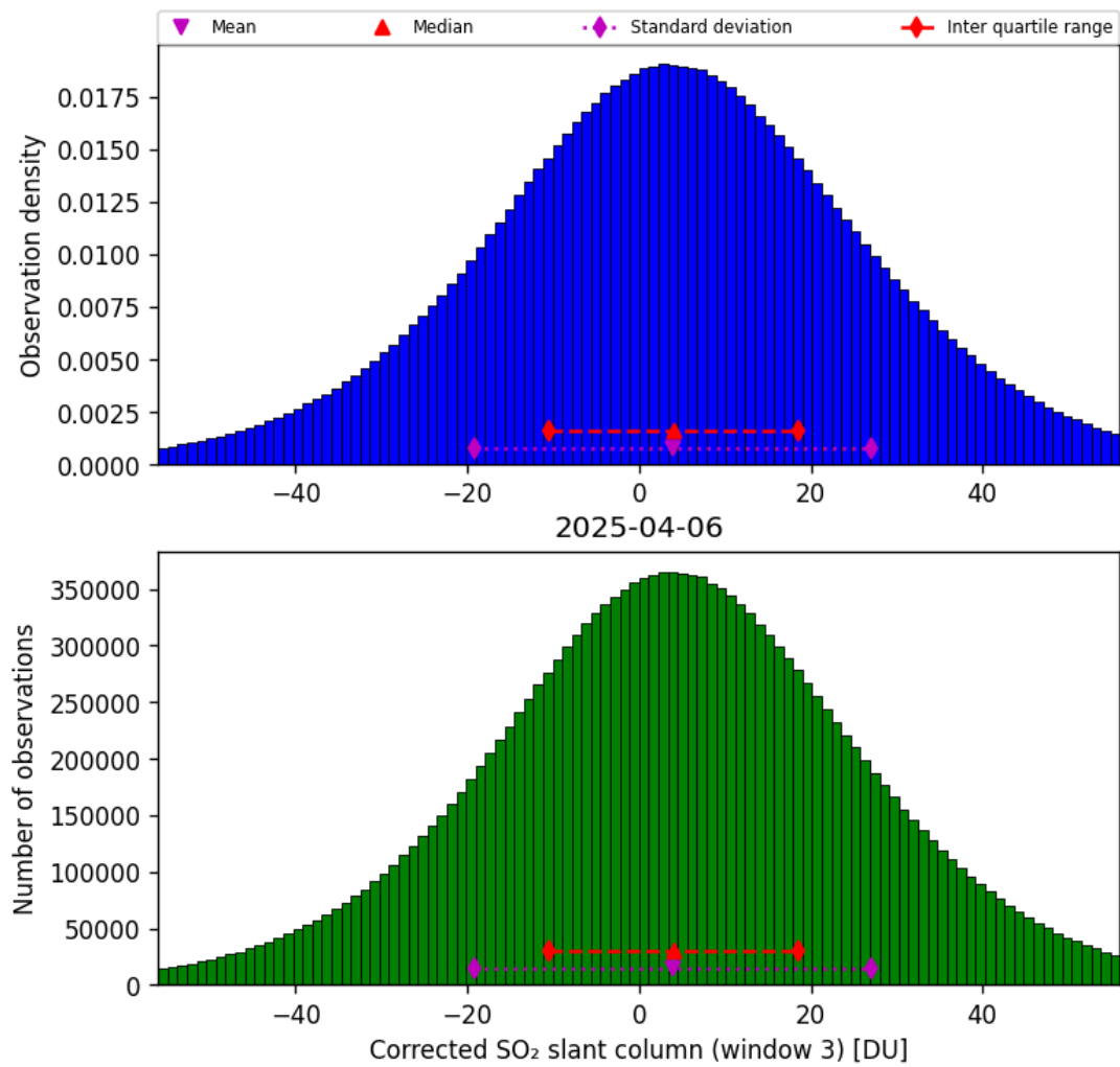
Figure 73: Histogram of “Corrected SO 2 slant column (window 3)” for 2025-04-06 to 2025-04-06
