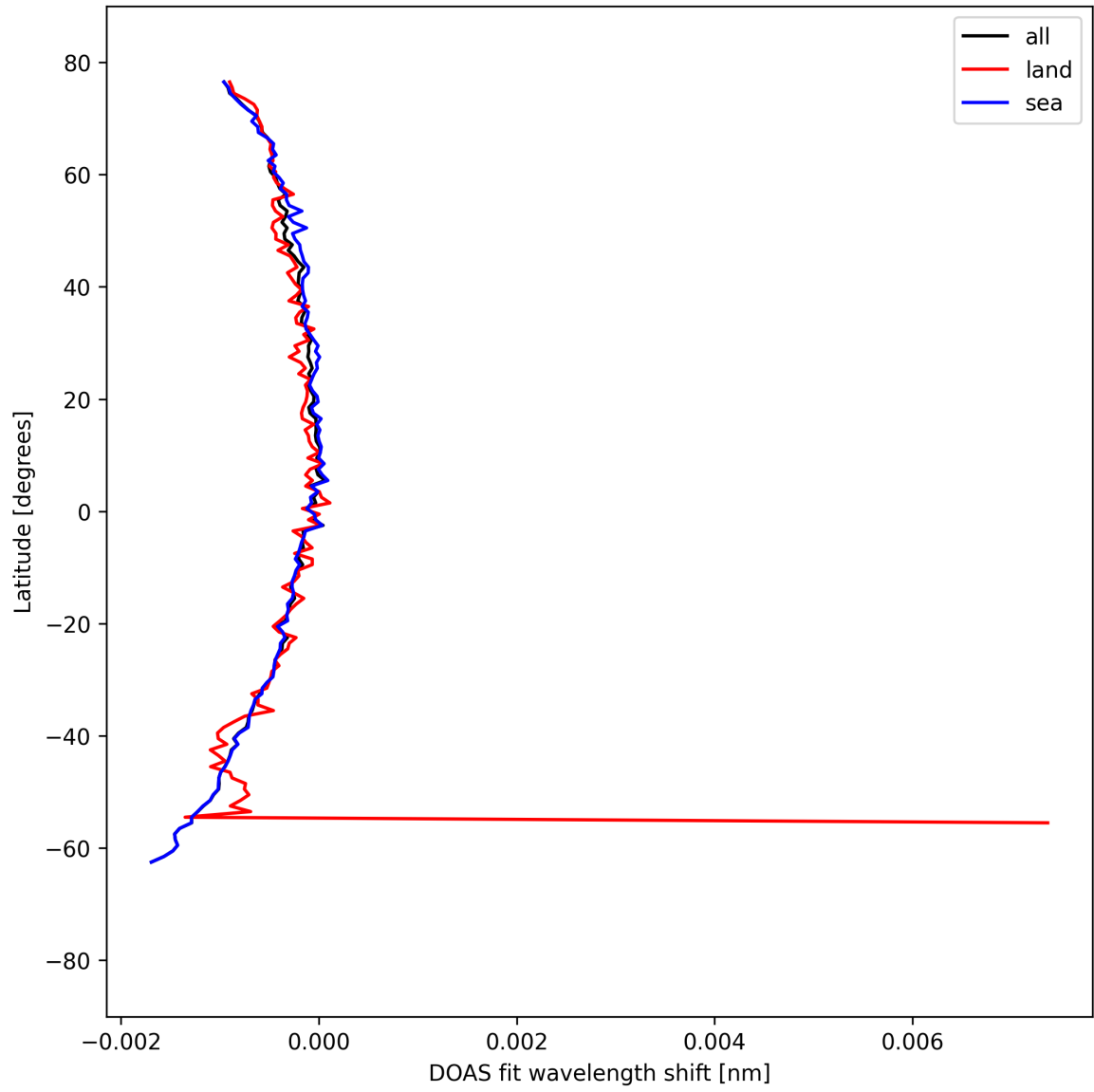
Figure 50: Zonal average of “DOAS fit wavelength shift” for 2025-04-06 to 2025-04-06.
