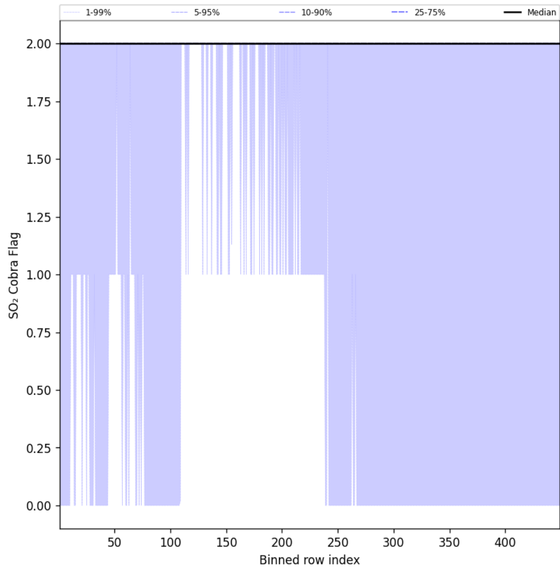
Figure 102: Along track statistics of “SO 2 Cobra Flag” for 2025-04-06 to 2025-04-06
