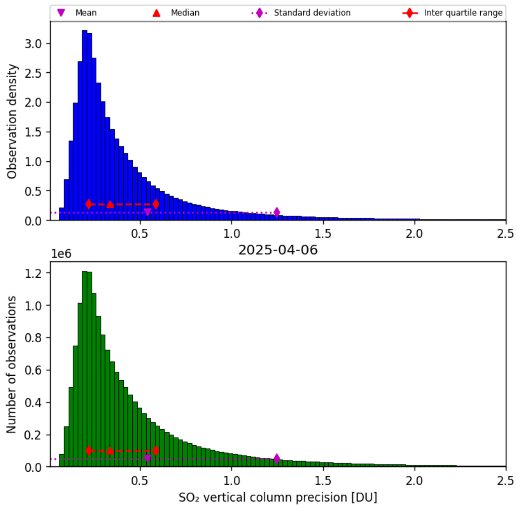
Figure 59: Histogram of “SO 2 vertical column precision” for 2025-04-06 to 2025-04-06
