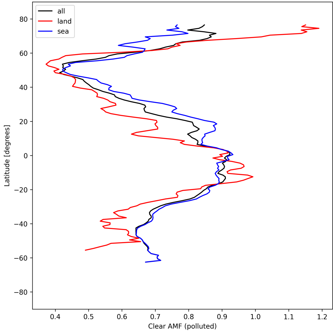
Figure 55: Zonal average of “Clear AMF (polluted)” for 2025-04-06 to 2025-04-06.
