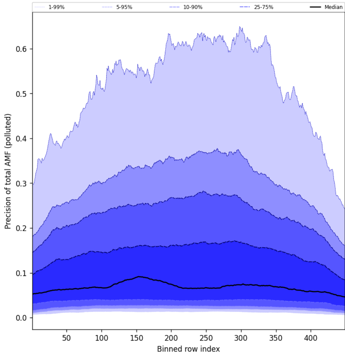
Figure 108: Along track statistics of “Precision of total AMF (polluted)” for 2025-04-06 to 2025-04-06
