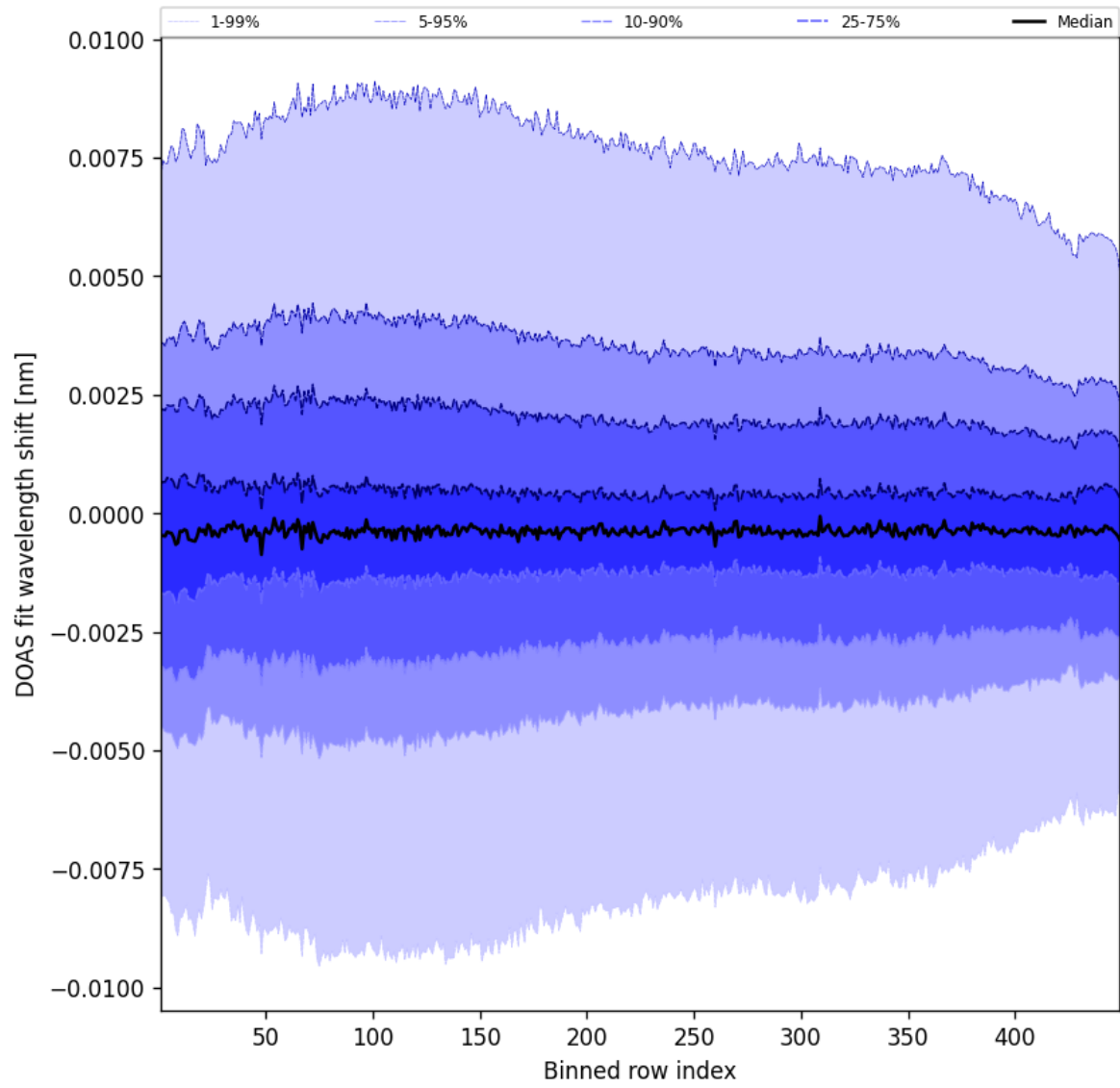
Figure 104: Along track statistics of “DOAS fit wavelength shift” for 2025-04-06 to 2025-04-06
