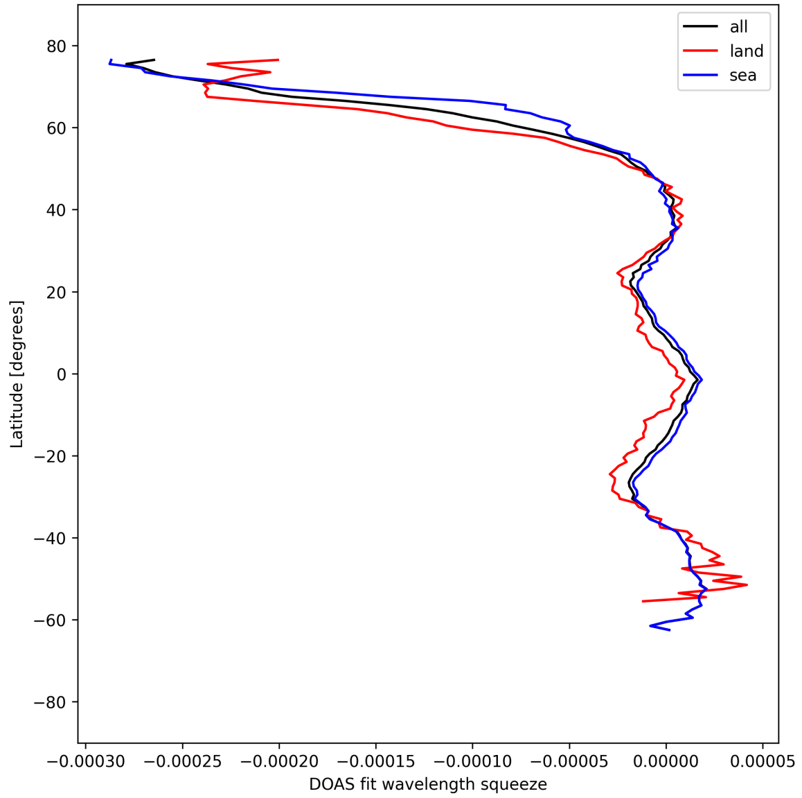
Figure 51: Zonal average of “DOAS fit wavelength squeeze” for 2025-04-06 to 2025-04-06.
