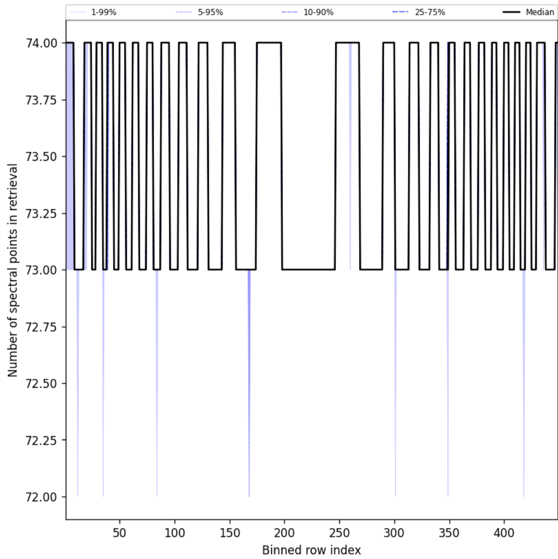
Figure 110: Along track statistics of “Number of spectral points in retrieval” for 2025-04-06 to 2025-04-06
