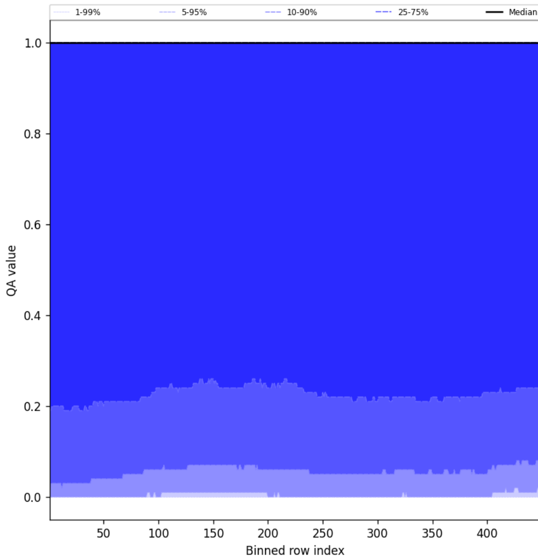
Figure 84: Along track statistics of “QA value” for 2025-04-06 to 2025-04-06
