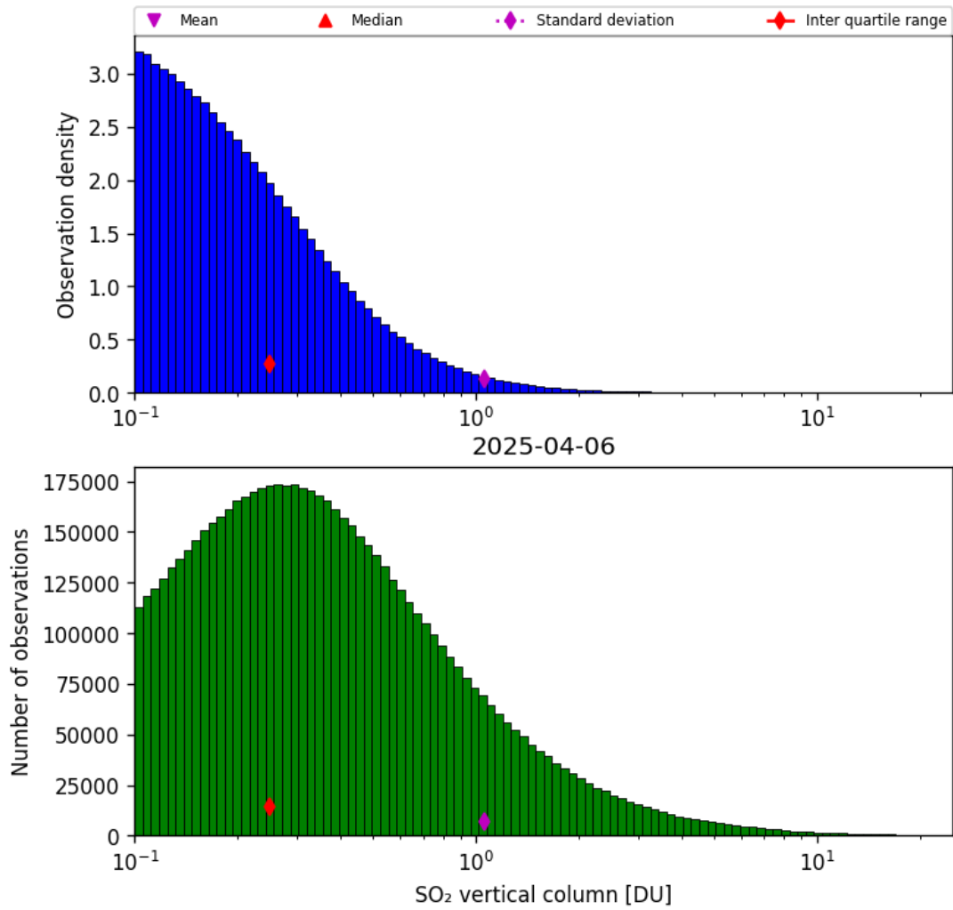
Figure 58: Histogram of “SO 2 vertical column” for 2025-04-06 to 2025-04-06
