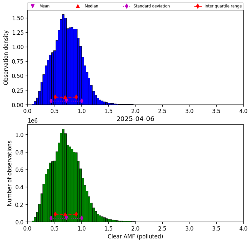
Figure 82: Histogram of “Clear AMF (polluted)” for 2025-04-06 to 2025-04-06
