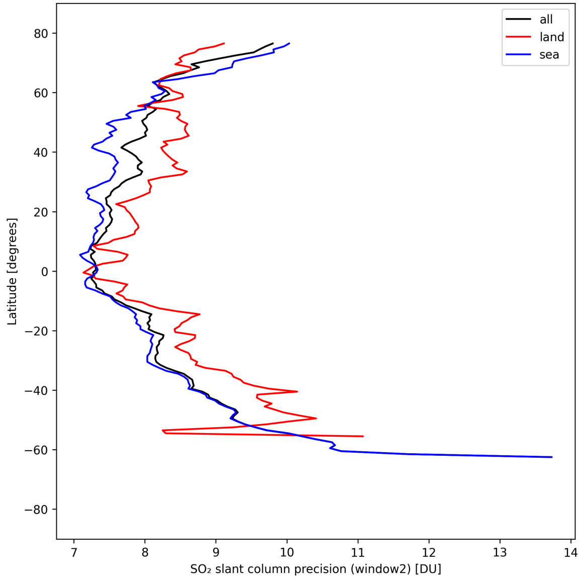
Figure 41: Zonal average of “SO 2 slant column precision (window2)” for 2025-04-06 to 2025-04-06.
