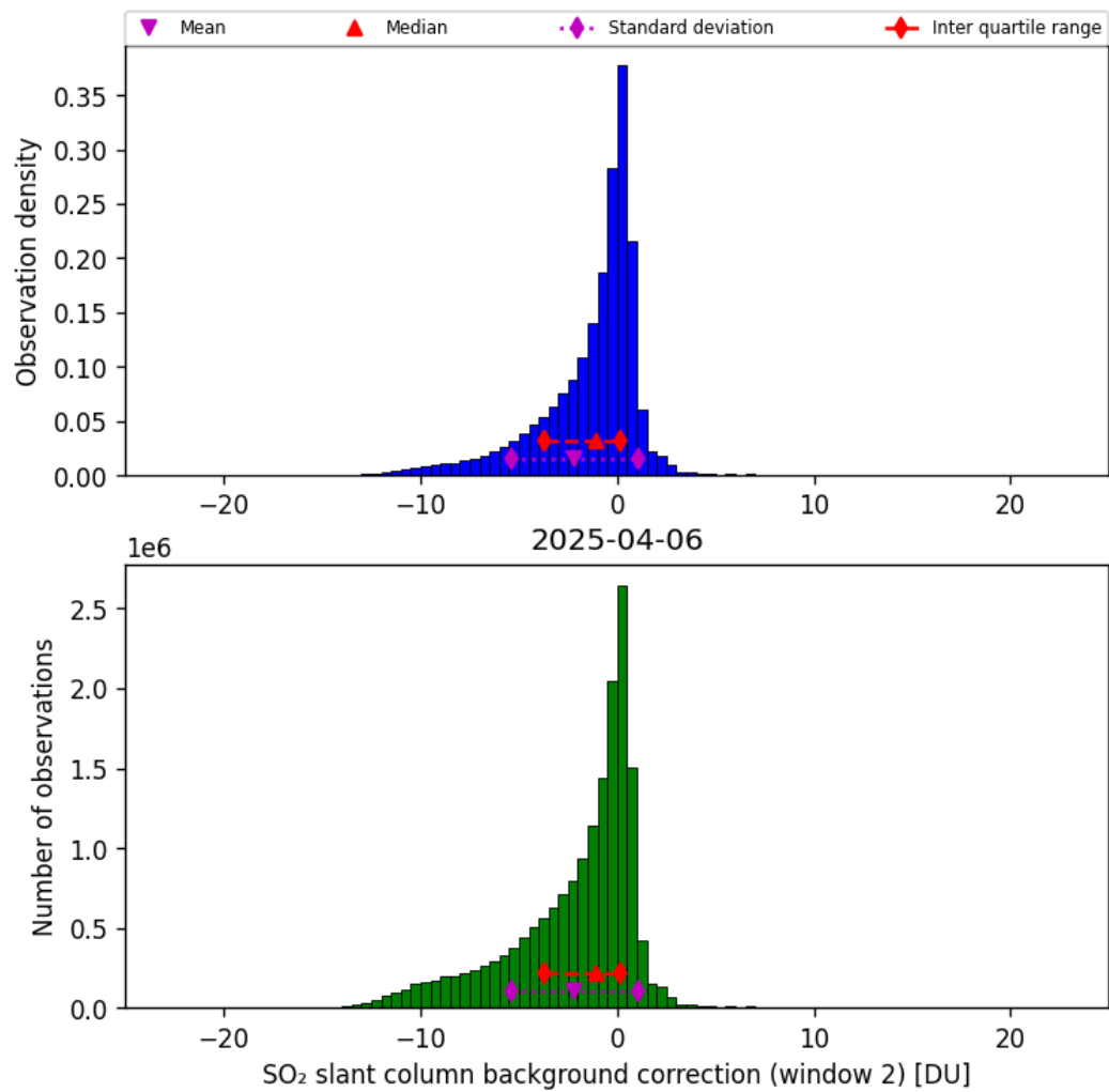
Figure 70: Histogram of “SO 2 slant column background correction (window 2)” for 2025-04-06 to 2025-04-06
