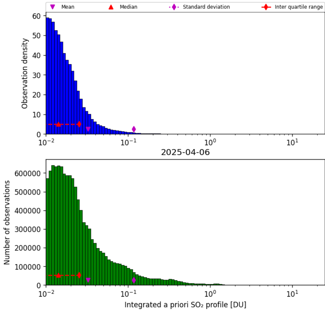
Figure 76: Histogram of “Integrated a priori SO 2 profile” for 2025-04-06 to 2025-04-06
