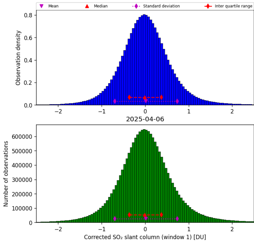
Figure 65: Histogram of “Corrected SO 2 slant column (window 1)” for 2025-04-06 to 2025-04-06
