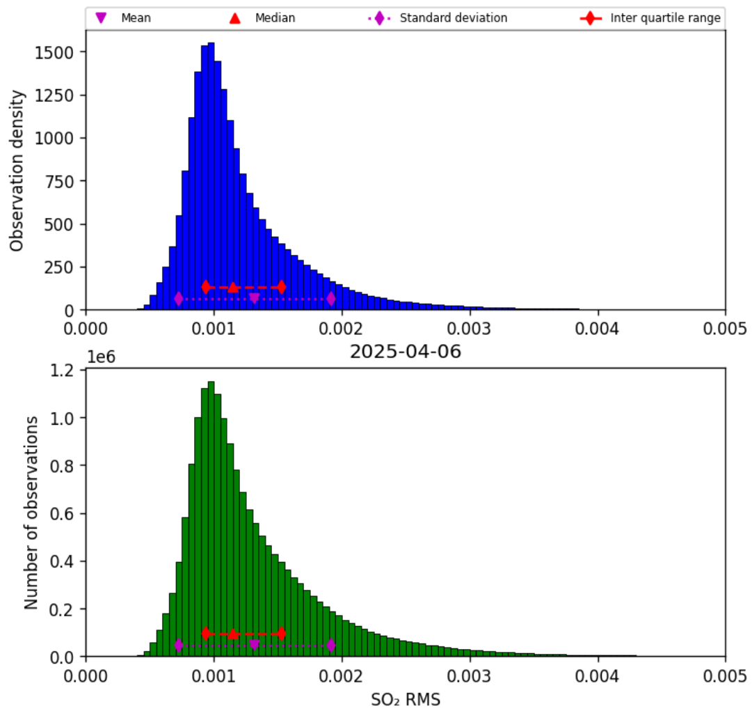
Figure 79: Histogram of “SO 2 RMS” for 2025-04-06 to 2025-04-06
