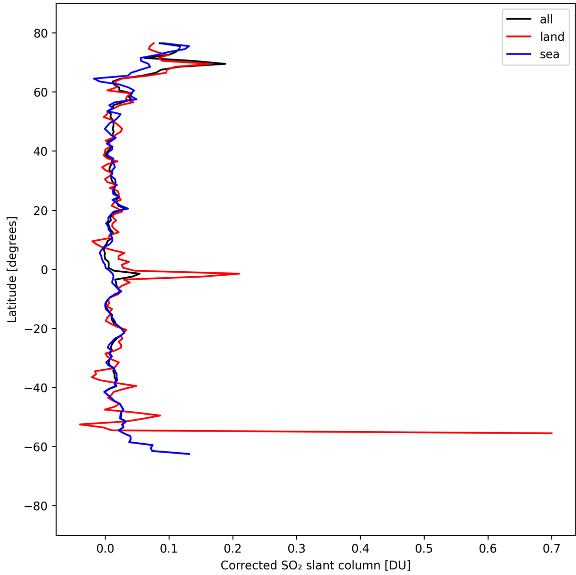
Figure 33: Zonal average of “Corrected SO 2 slant column” for 2025-04-06 to 2025-04-06.
