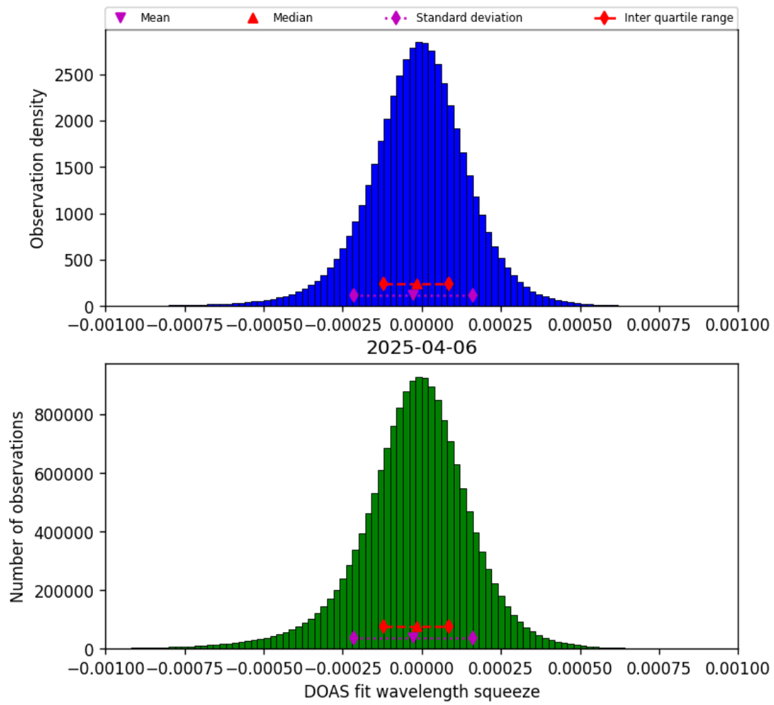
Figure 78: Histogram of “DOAS fit wavelength squeeze” for 2025-04-06 to 2025-04-06
