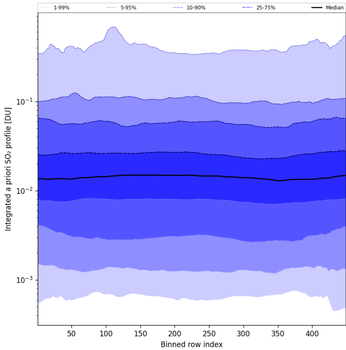
Figure 103: Along track statistics of “Integrated a priori SO 2 profile” for 2025-04-06 to 2025-04-06
