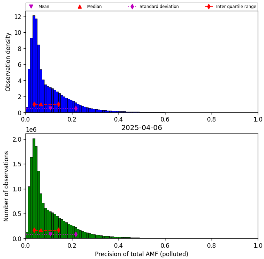
Figure 81: Histogram of “Precision of total AMF (polluted)” for 2025-04-06 to 2025-04-06
