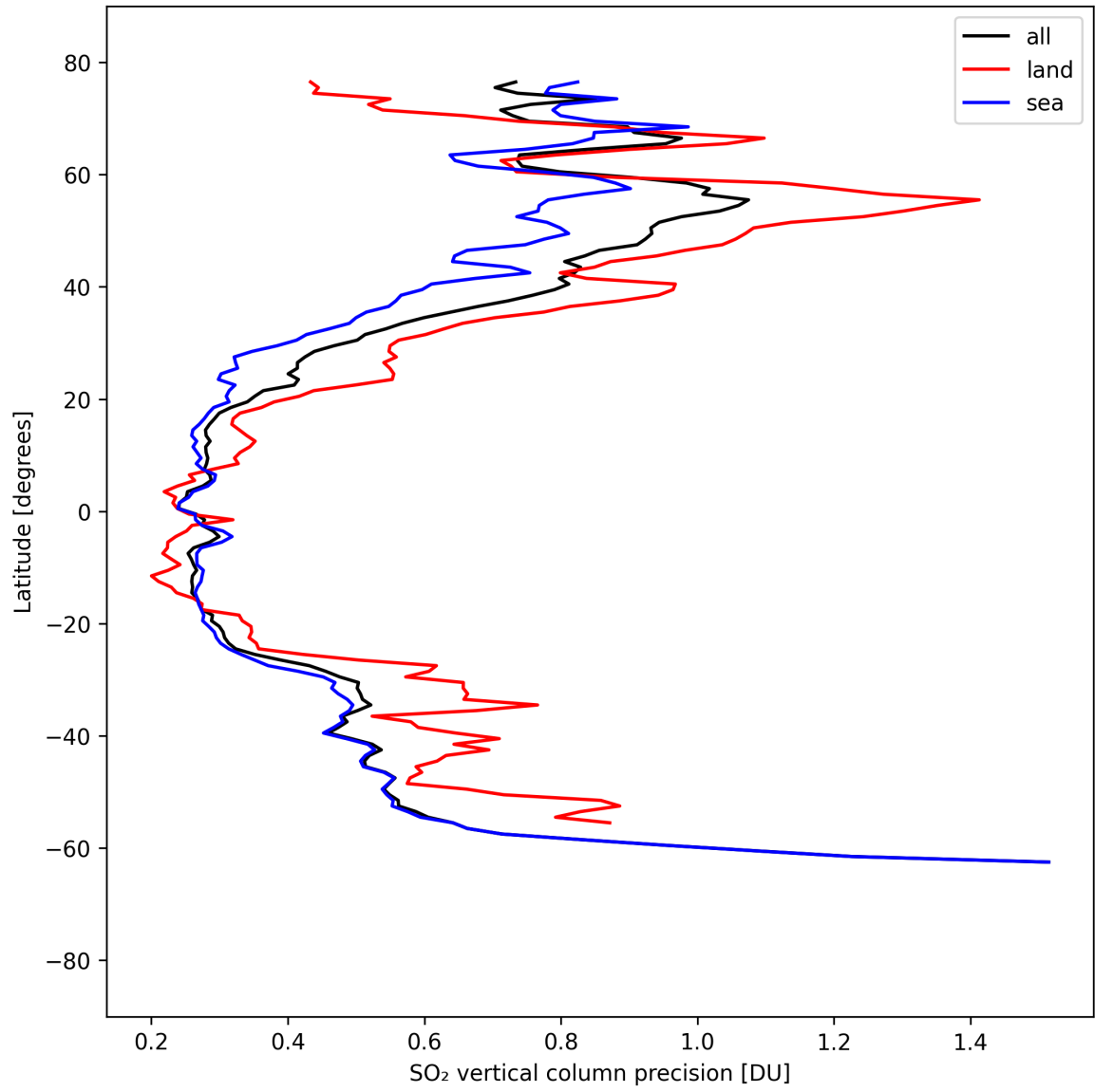
Figure 32: Zonal average of “SO 2 vertical column precision” for 2025-04-06 to 2025-04-06.
