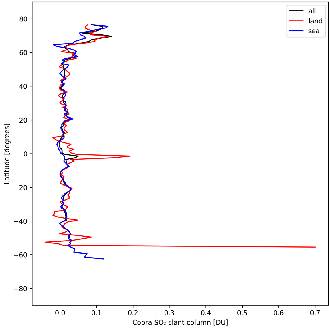
Figure 34: Zonal average of “Cobra SO 2 slant column” for 2025-04-06 to 2025-04-06.
