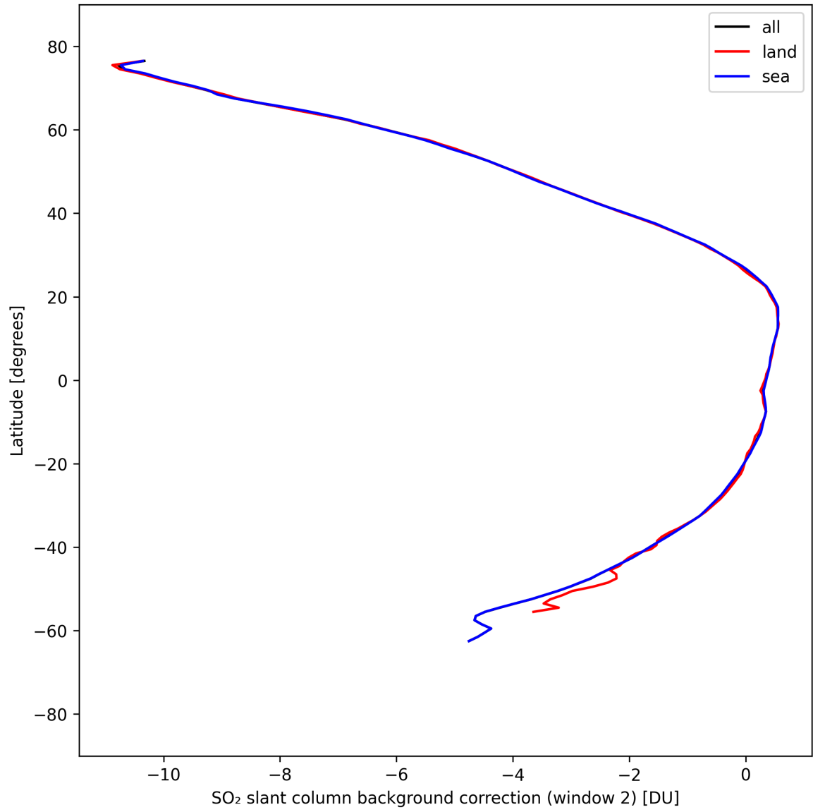
Figure 43: Zonal average of “SO 2 slant column background correction (window 2)” for 2025-04-06 to 2025-04-06.
