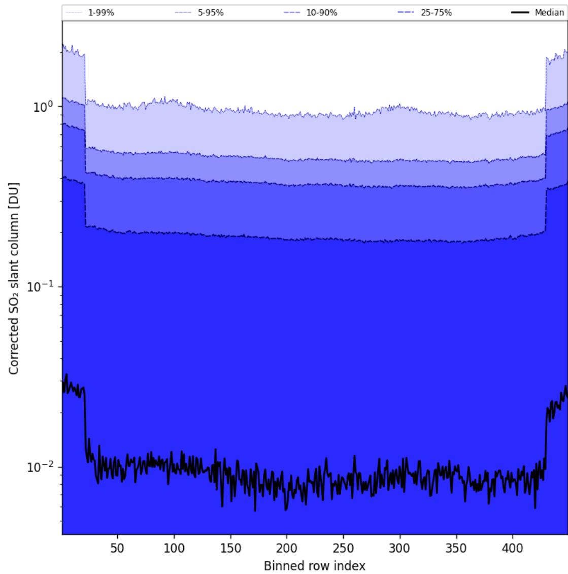
Figure 87: Along track statistics of “Corrected SO 2 slant column” for 2025-04-06 to 2025-04-06
