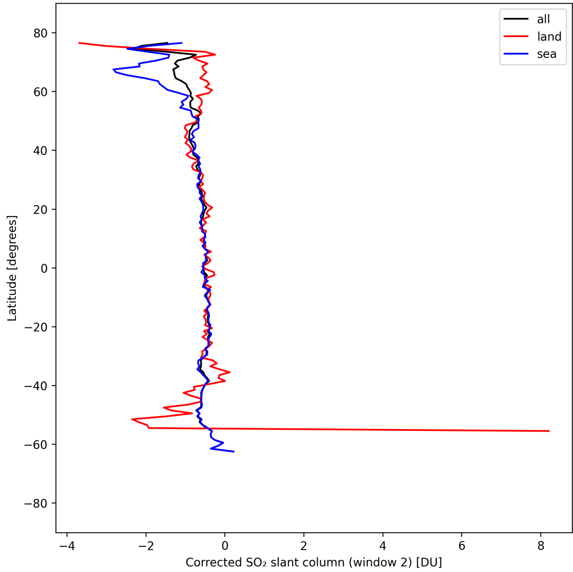
Figure 42: Zonal average of “Corrected SO 2 slant column (window 2)” for 2025-04-06 to 2025-04-06.
