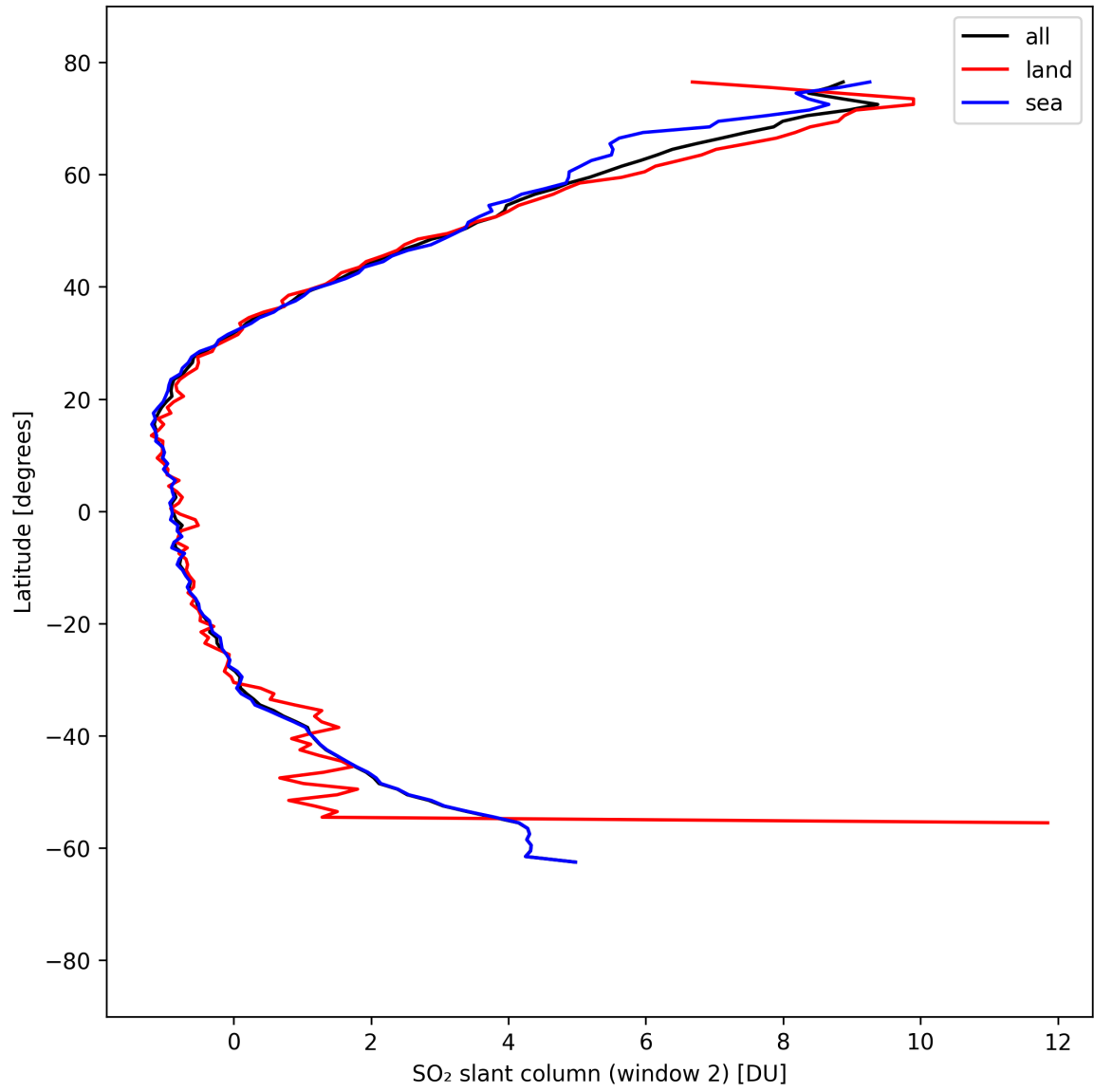
Figure 40: Zonal average of “SO 2 slant column (window 2)” for 2025-04-06 to 2025-04-06.
