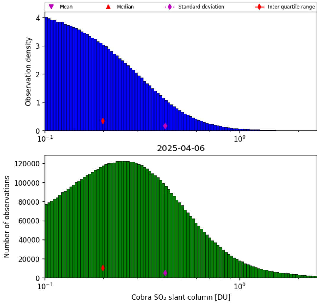
Figure 61: Histogram of “Cobra SO 2 slant column” for 2025-04-06 to 2025-04-06
