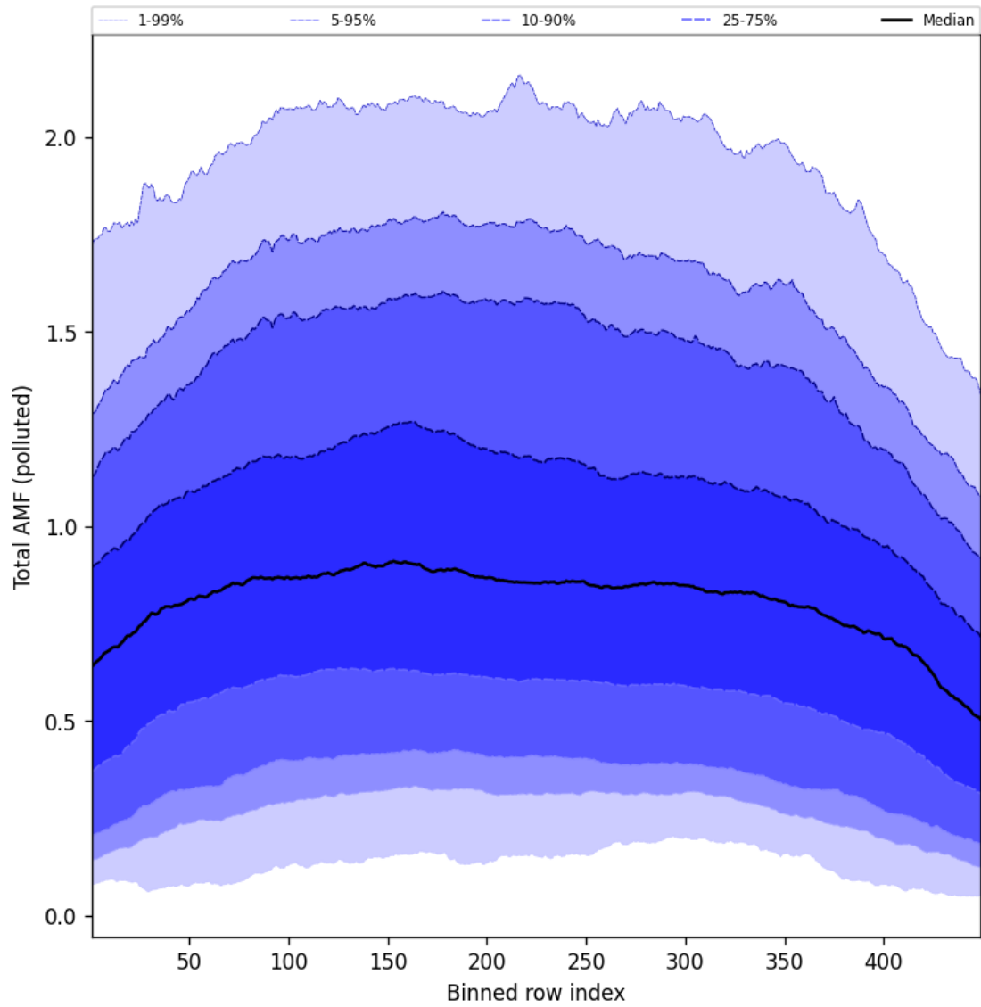
Figure 107: Along track statistics of “Total AMF (polluted)” for 2025-04-06 to 2025-04-06
