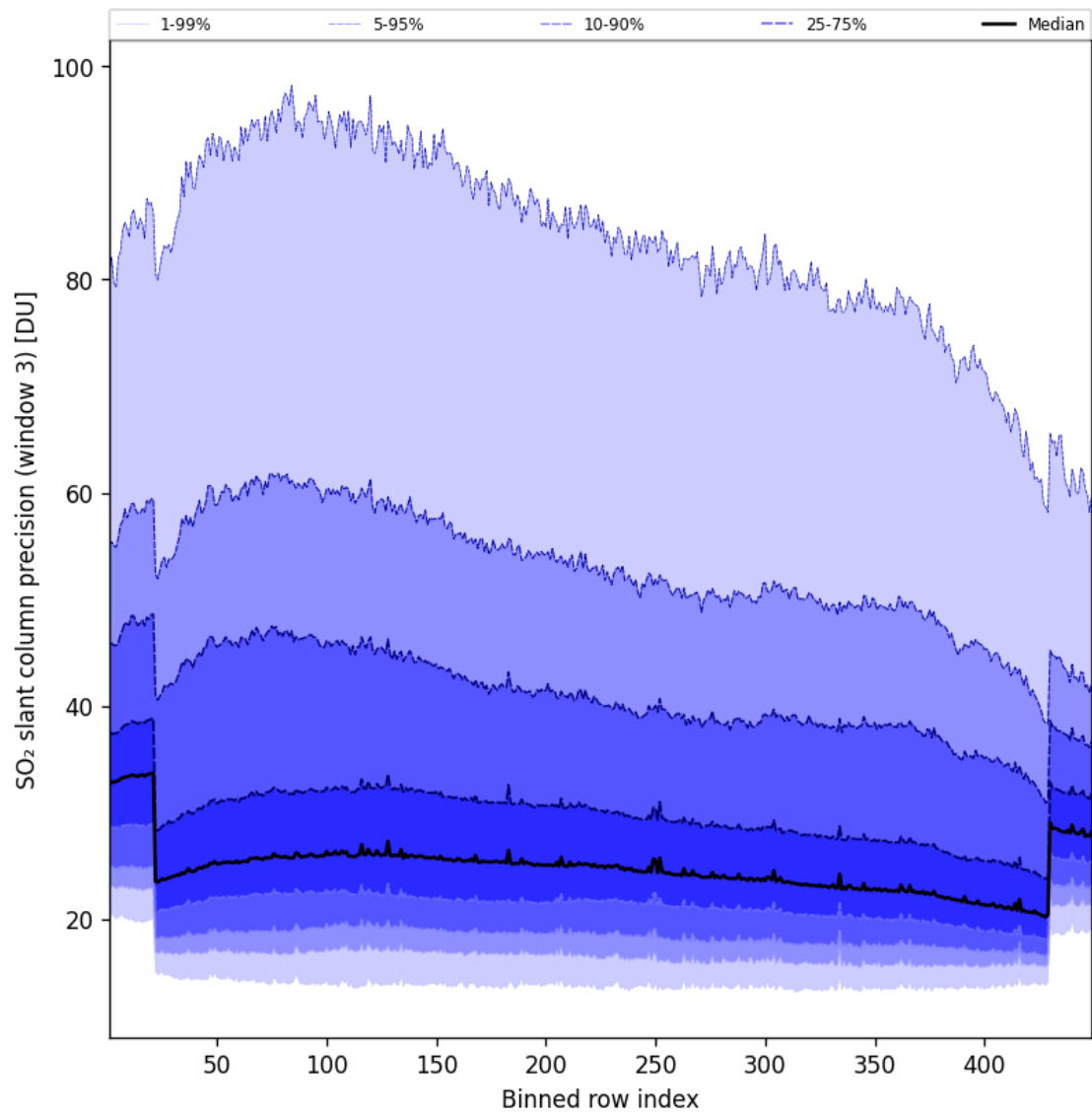
Figure 99: Along track statistics of “SO 2 slant column precision (window 3)” for 2025-04-06 to 2025-04-06
