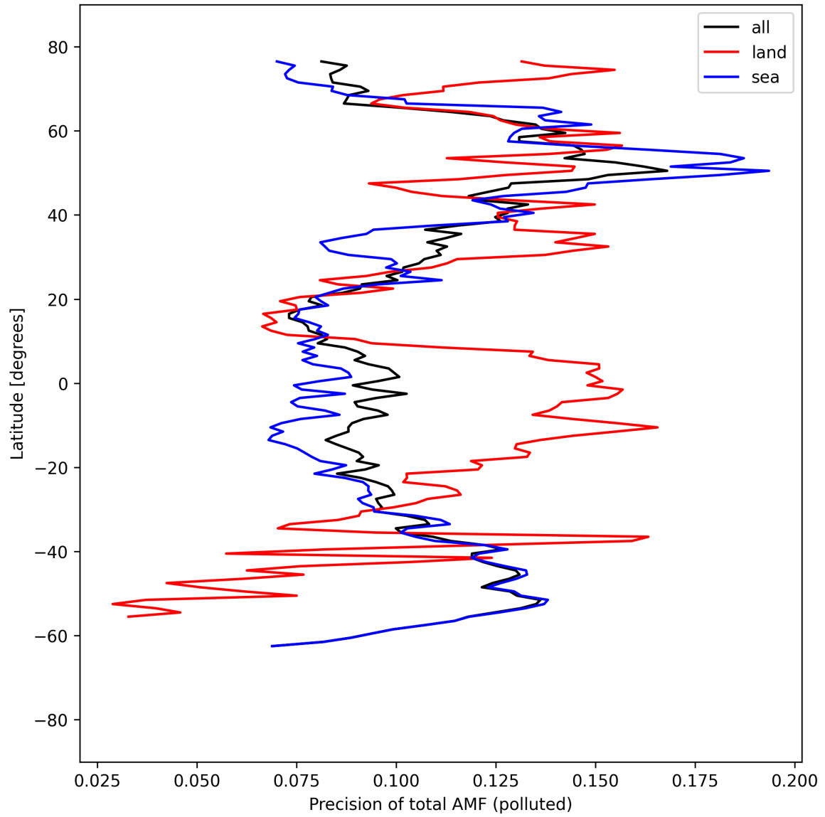
Figure 54: Zonal average of “Precision of total AMF (polluted)” for 2025-04-06 to 2025-04-06.
