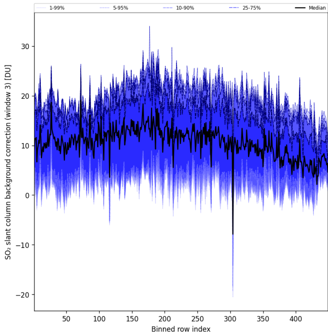
Figure 101: Along track statistics of “SO 2 slant column background correction (window 3)” for 2025-04-06 to 2025-04-06
