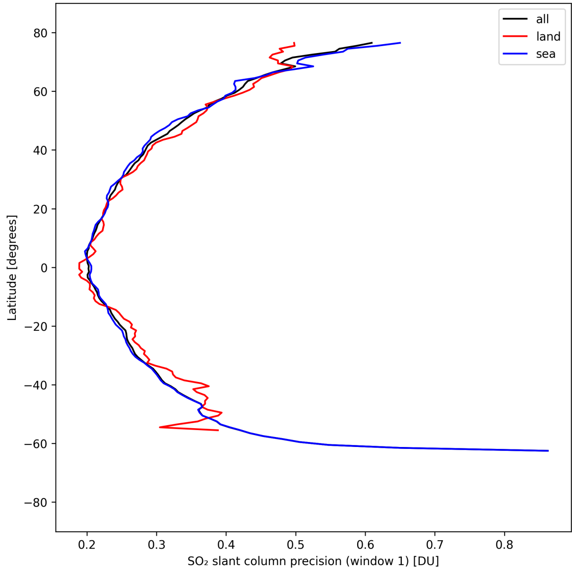
Figure 37: Zonal average of “SO 2 slant column precision (window 1)” for 2025-04-06 to 2025-04-06.
