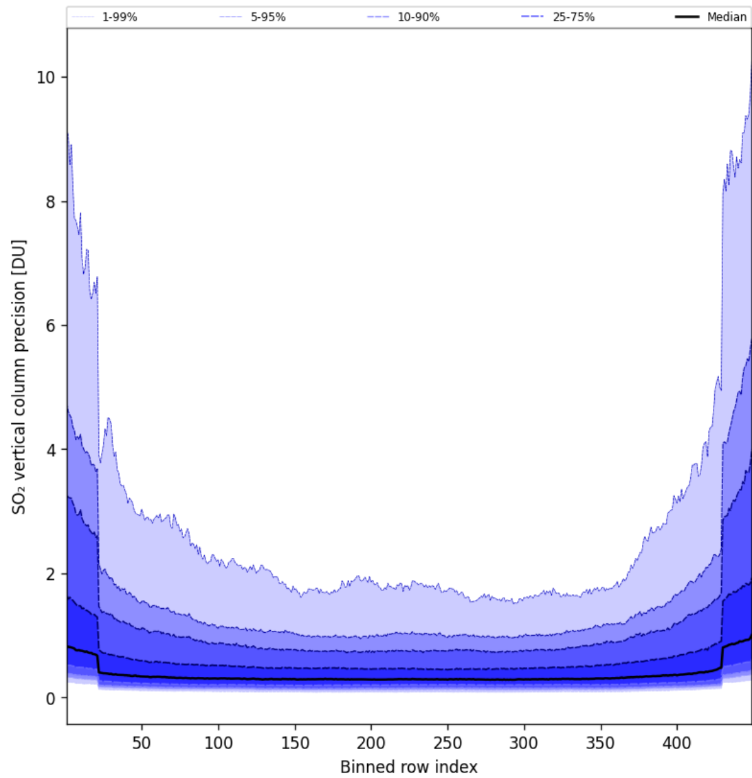
Figure 86: Along track statistics of “SO 2 vertical column precision” for 2025-04-06 to 2025-04-06
