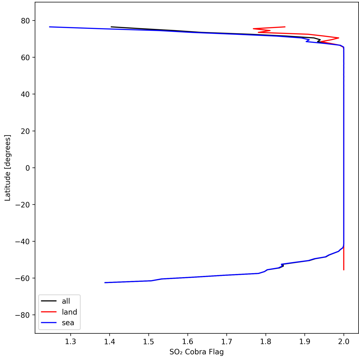
Figure 48: Zonal average of "SO 2 Cobra Flag" for 2025-04-06 to 2025-04-06.
