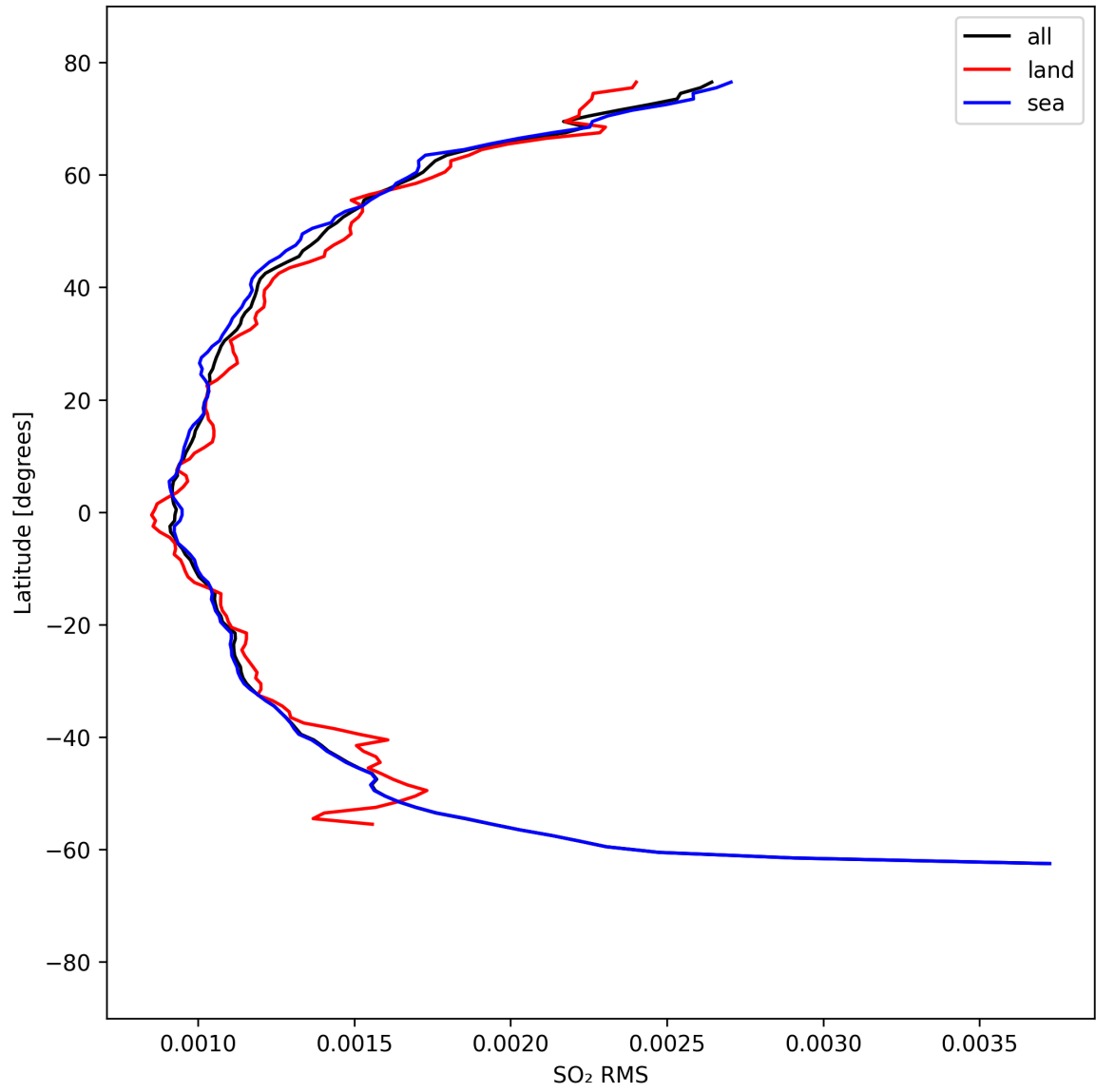
Figure 52: Zonal average of “SO 2 RMS” for 2025-04-06 to 2025-04-06.
