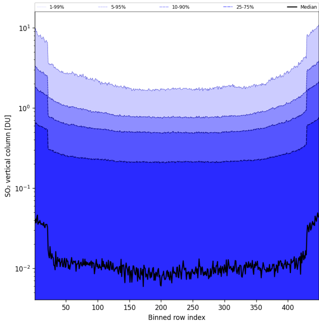
Figure 85: Along track statistics of “SO 2 vertical column” for 2025-04-06 to 2025-04-06
