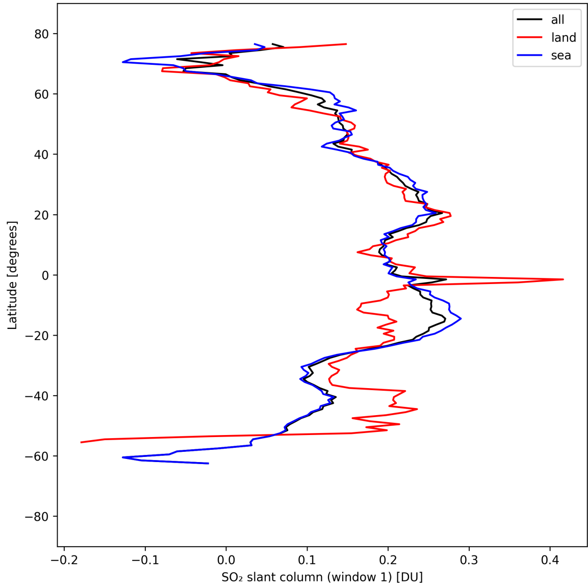
Figure 36: Zonal average of “SO 2 slant column (window 1)” for 2025-04-06 to 2025-04-06.
