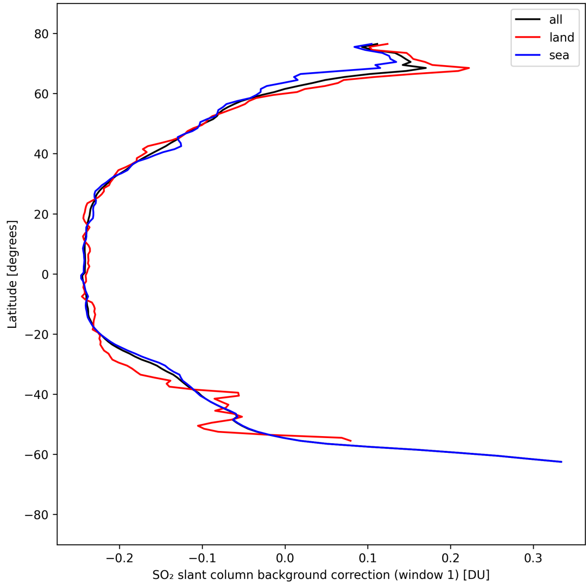
Figure 39: Zonal average of “SO 2 slant column background correction (window 1)” for 2025-04-06 to 2025-04-06.
