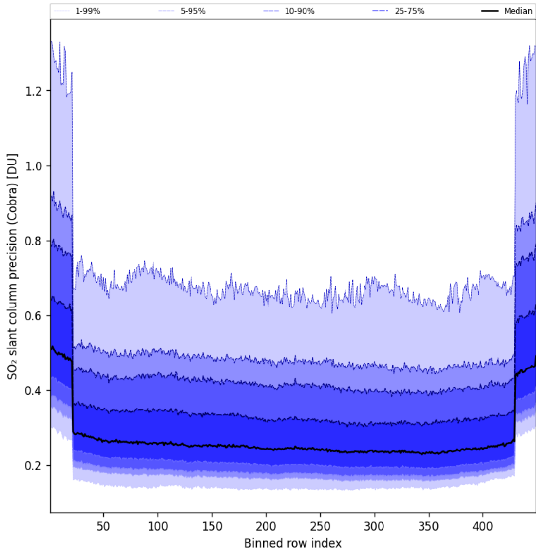
Figure 89: Along track statistics of “SO 2 slant column precision (Cobra)” for 2025-04-06 to 2025-04-06
