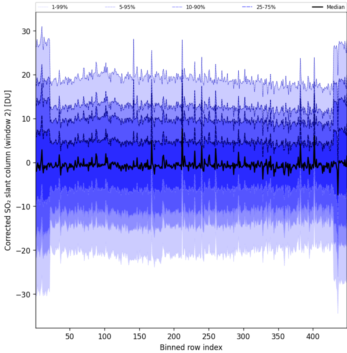
Figure 96: Along track statistics of “Corrected SO 2 slant column (window 2)” for 2025-04-06 to 2025-04-06
