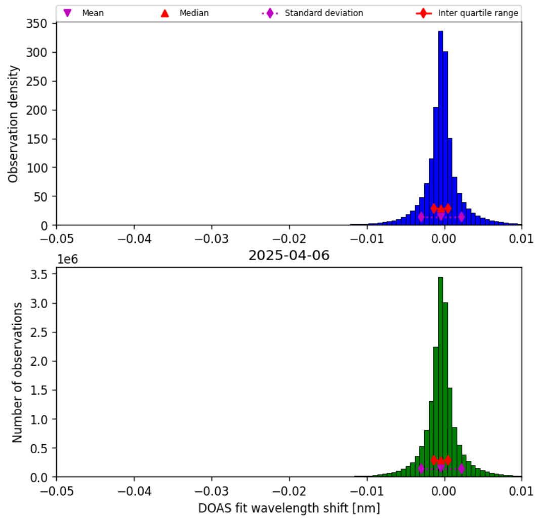
Figure 77: Histogram of “DOAS fit wavelength shift” for 2025-04-06 to 2025-04-06
