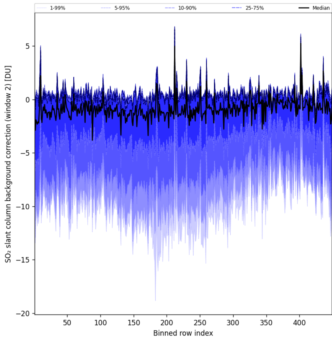
Figure 97: Along track statistics of “SO 2 slant column background correction (window 2)” for 2025-04-06 to 2025-04-06
