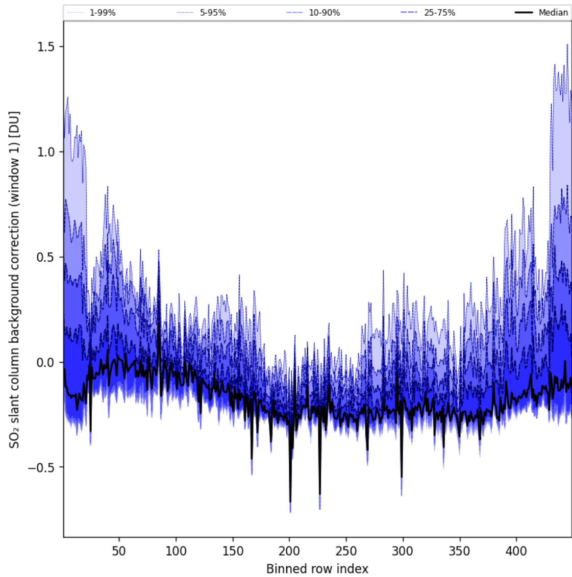
Figure 93: Along track statistics of “SO 2 slant column background correction (window 1)” for 2025-04-06 to 2025-04-06
