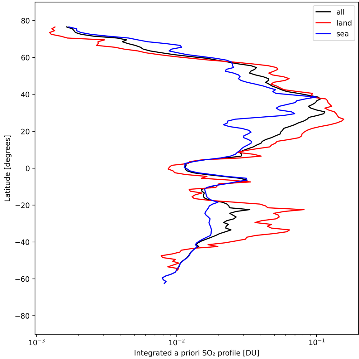
Figure 49: Zonal average of “Integrated a priori SO 2 profile” for 2025-04-06 to 2025-04-06.
