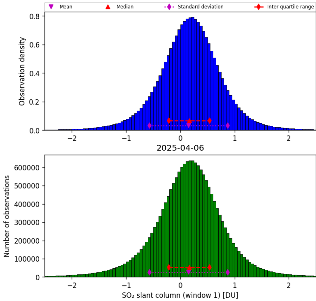
Figure 63: Histogram of “SO 2 slant column (window 1)” for 2025-04-06 to 2025-04-06
