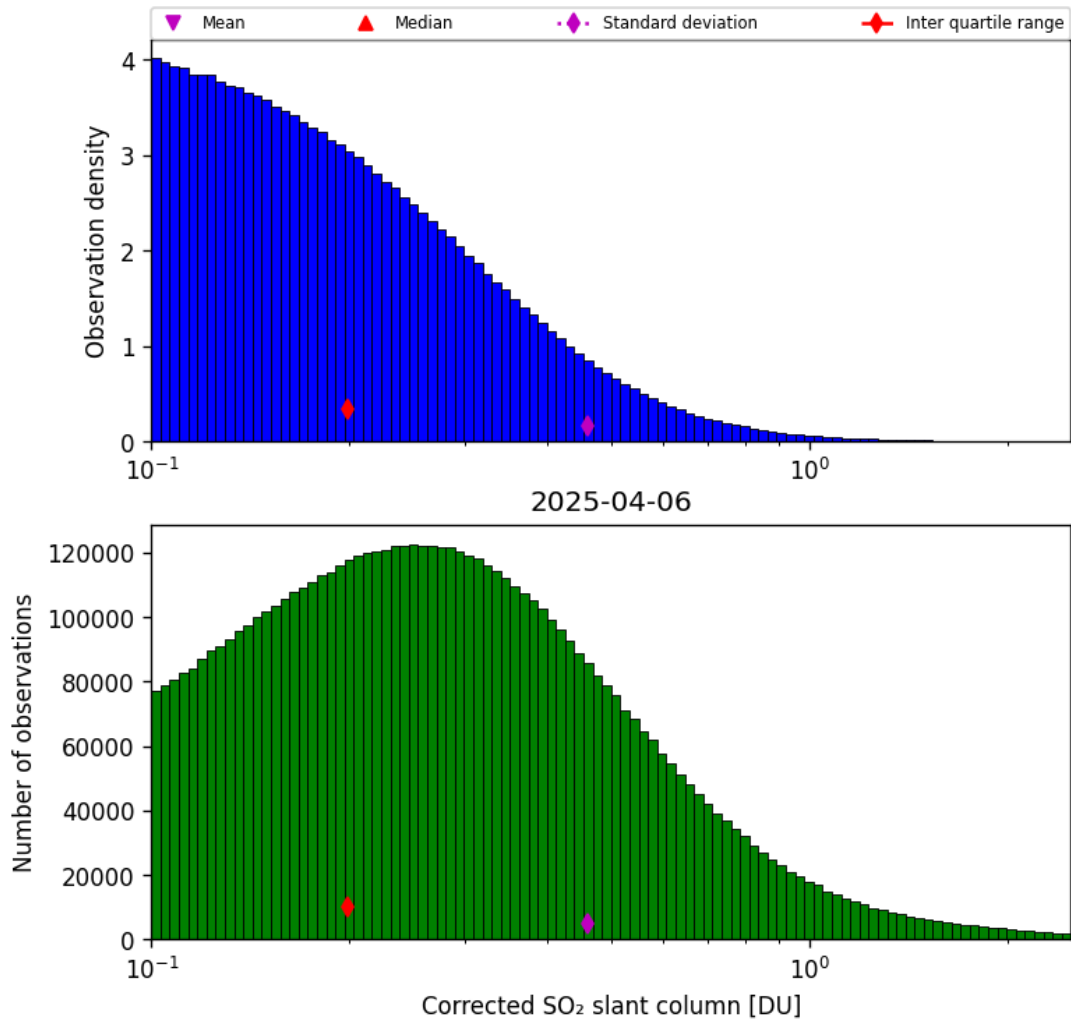
Figure 60: Histogram of “Corrected SO 2 slant column” for 2025-04-06 to 2025-04-06
