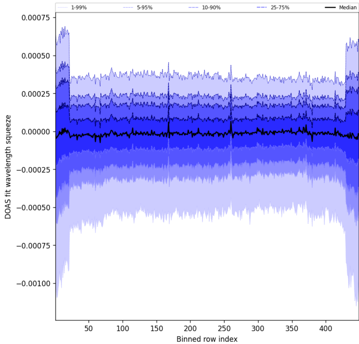
Figure 105: Along track statistics of “DOAS fit wavelength squeeze” for 2025-04-06 to 2025-04-06
