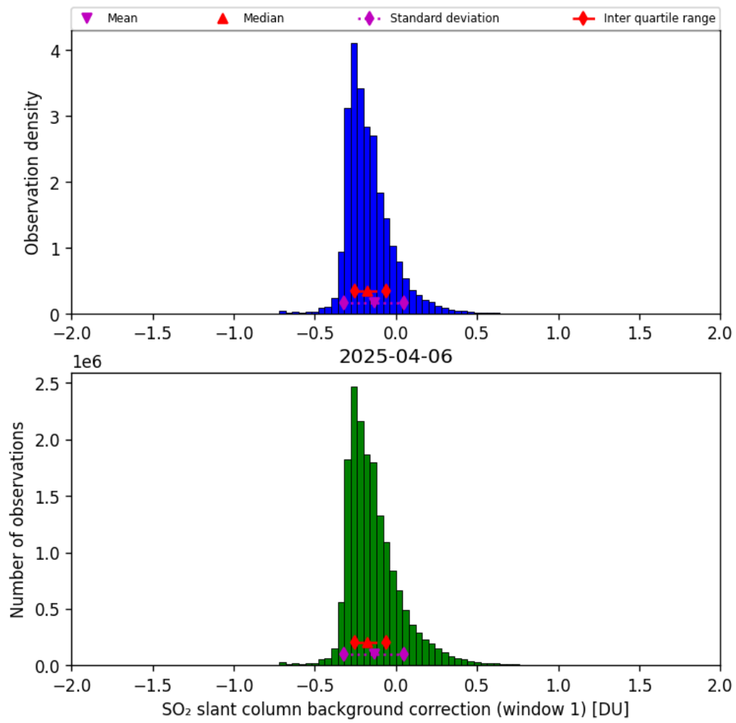
Figure 66: Histogram of “SO 2 slant column background correction (window 1)” for 2025-04-06 to 2025-04-06
