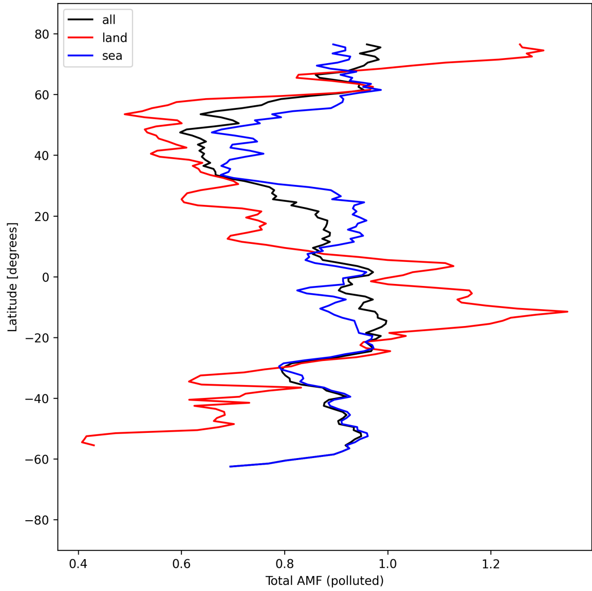
Figure 53: Zonal average of “Total AMF (polluted)” for 2025-04-06 to 2025-04-06.
