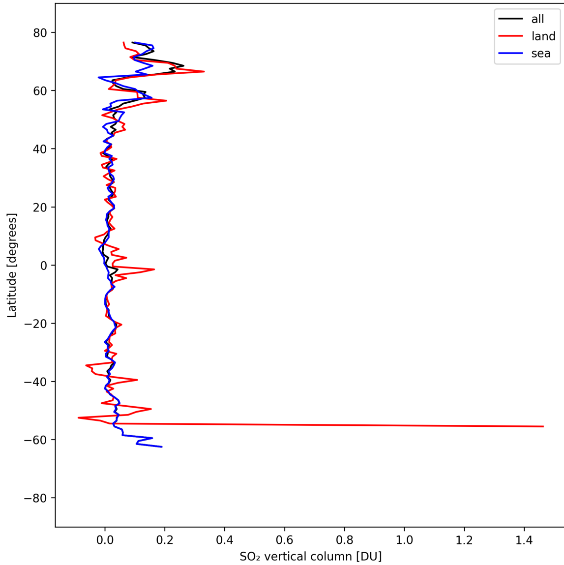
Figure 31: Zonal average of “SO 2 vertical column” for 2025-04-06 to 2025-04-06.
