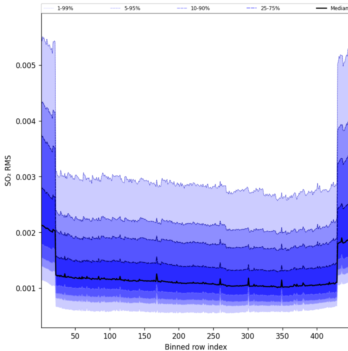
Figure 106: Along track statistics of “SO 2 RMS” for 2025-04-06 to 2025-04-06
