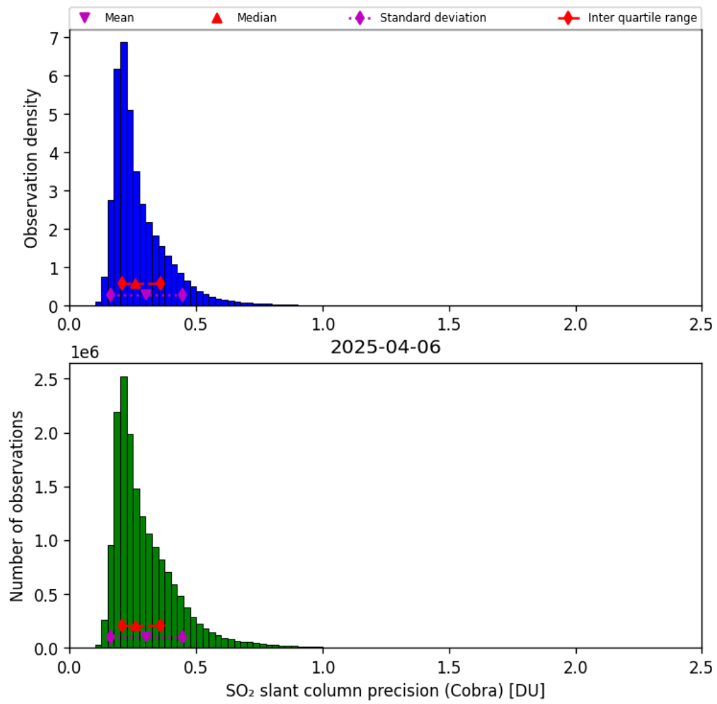
Figure 62: Histogram of “SO 2 slant column precision (Cobra)” for 2025-04-06 to 2025-04-06
