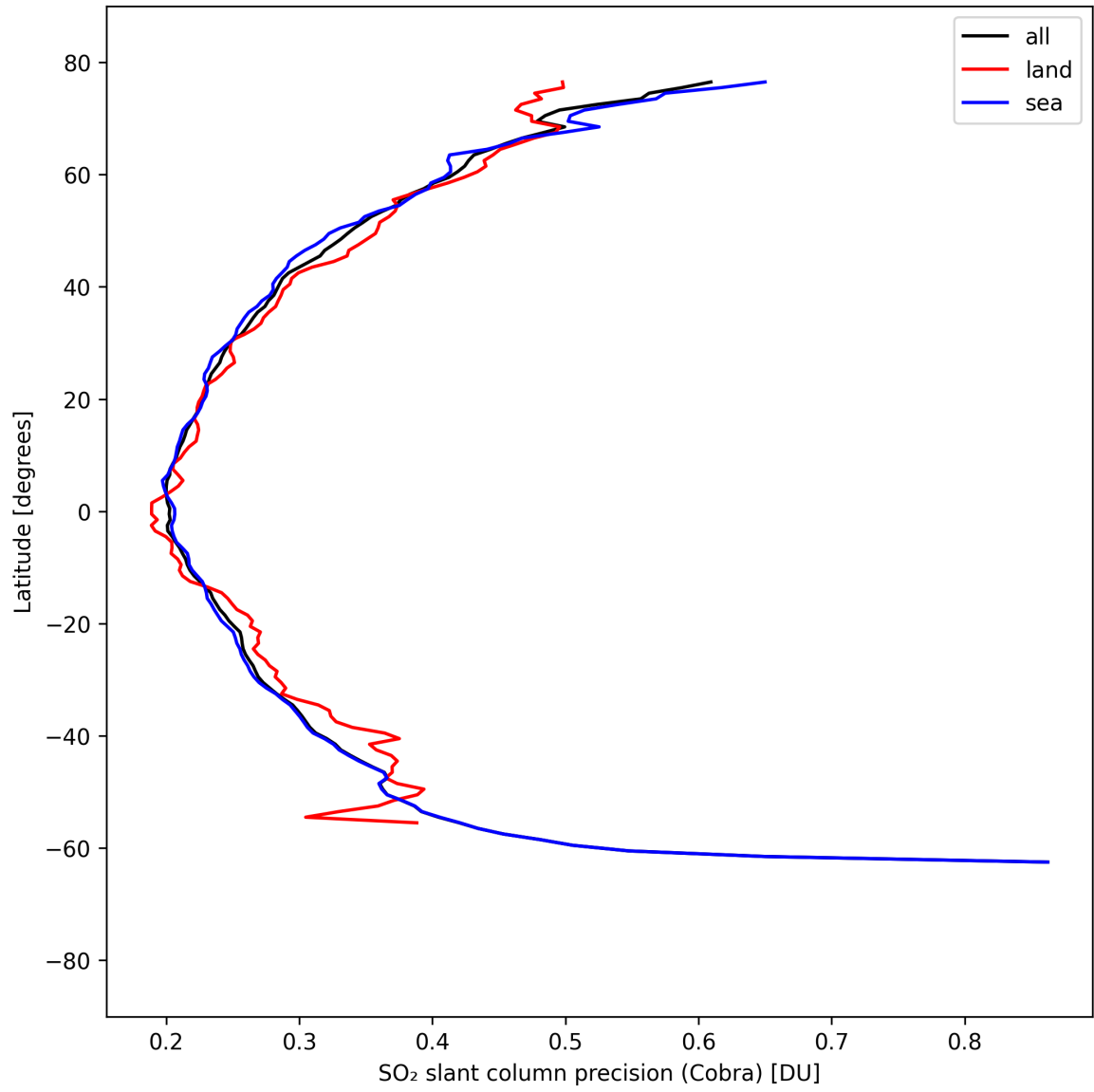
Figure 35: Zonal average of “SO 2 slant column precision (Cobra)” for 2025-04-06 to 2025-04-06.
