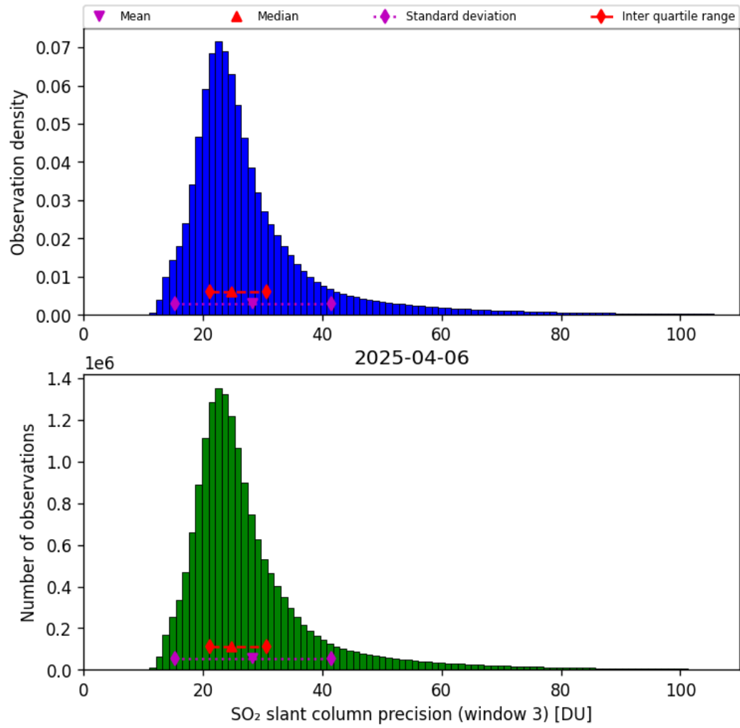
Figure 72: Histogram of “SO 2 slant column precision (window 3)” for 2025-04-06 to 2025-04-06
