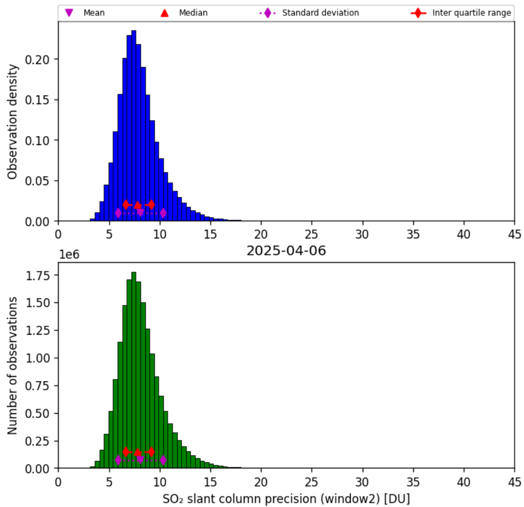
Figure 68: Histogram of “SO 2 slant column precision (window2)” for 2025-04-06 to 2025-04-06
