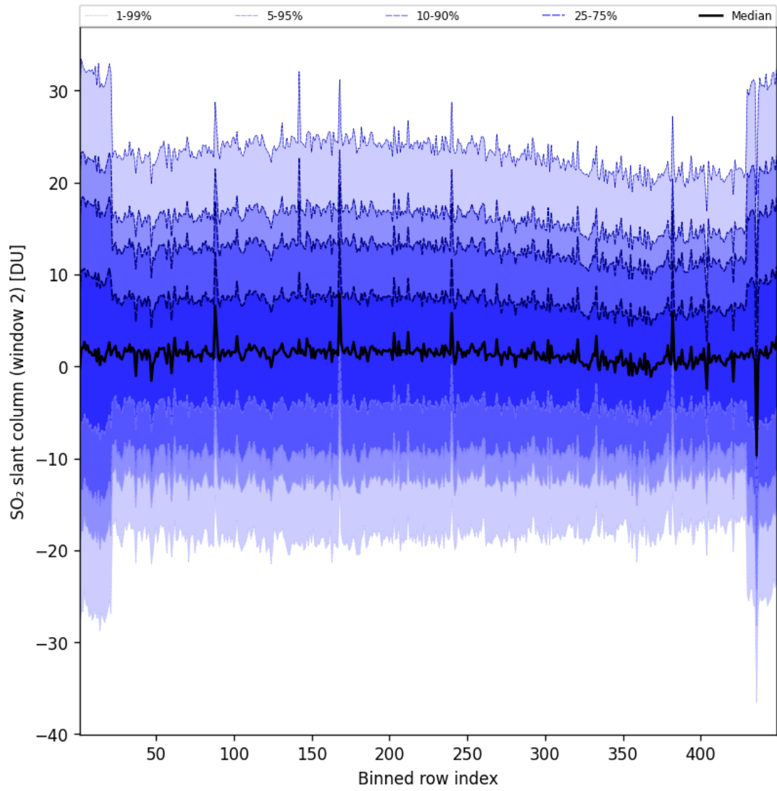
Figure 94: Along track statistics of “SO 2 slant column (window 2)” for 2025-04-06 to 2025-04-06
