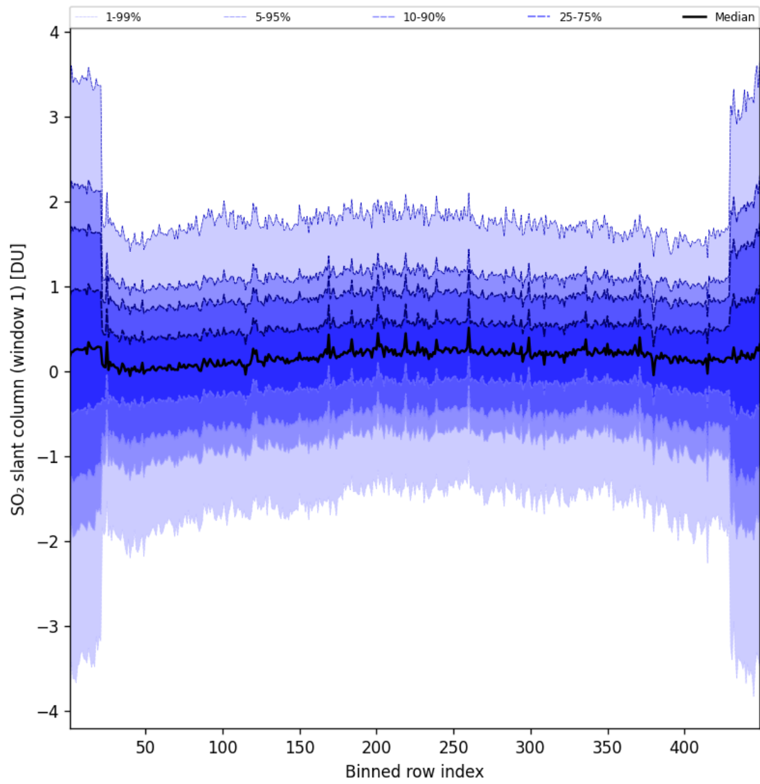
Figure 90: Along track statistics of “SO 2 slant column (window 1)” for 2025-04-06 to 2025-04-06
