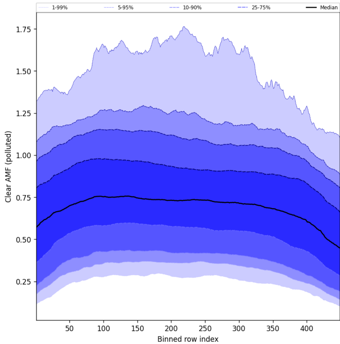
Figure 109: Along track statistics of “Clear AMF (polluted)” for 2025-04-06 to 2025-04-06
