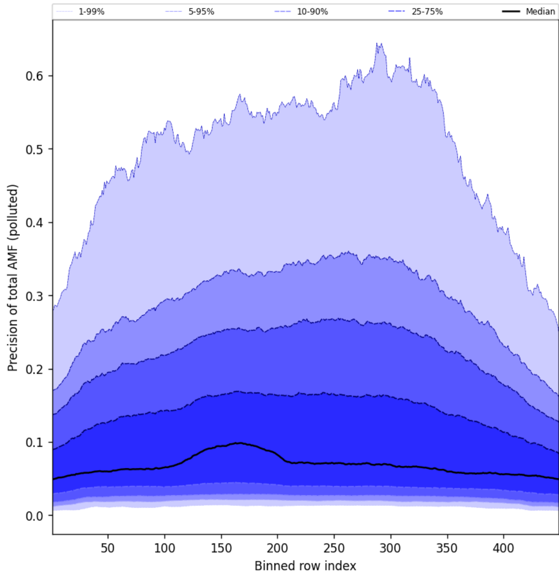
Figure 108: Along track statistics of “Precision of total AMF (polluted)” for 2025-04-08 to 2025-04-09
