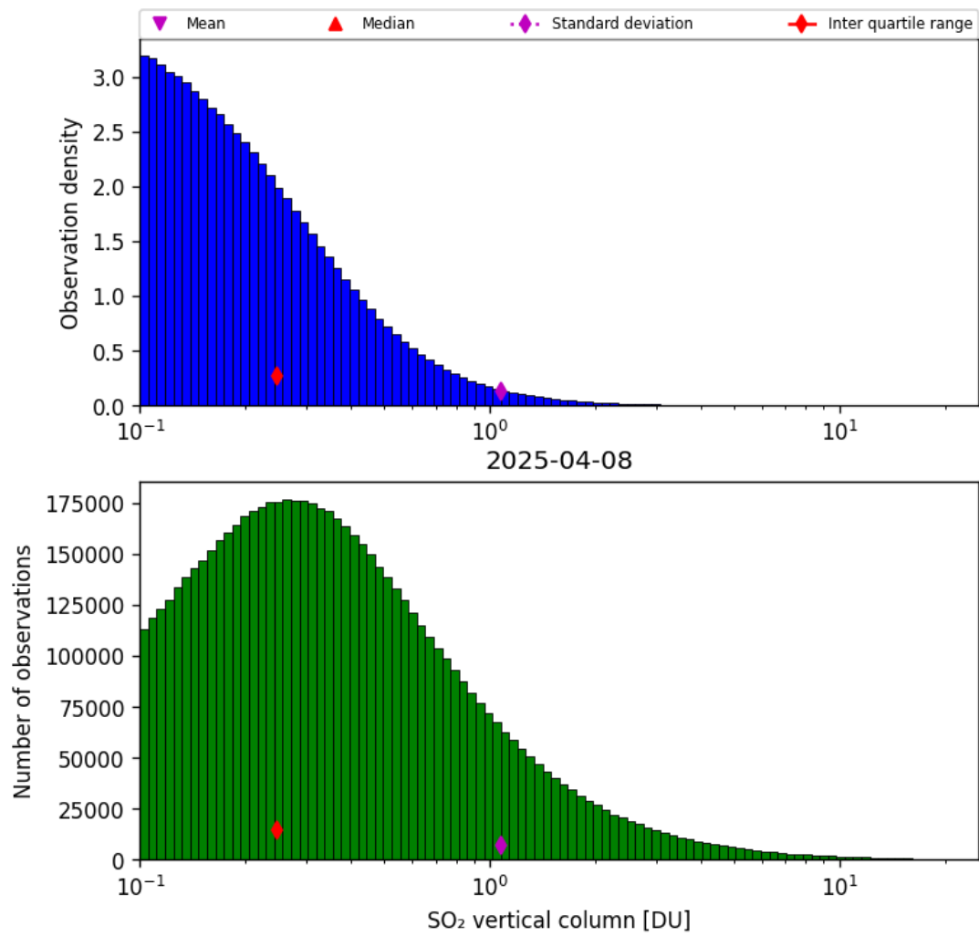
Figure 58: Histogram of “SO 2 vertical column” for 2025-04-08 to 2025-04-09
