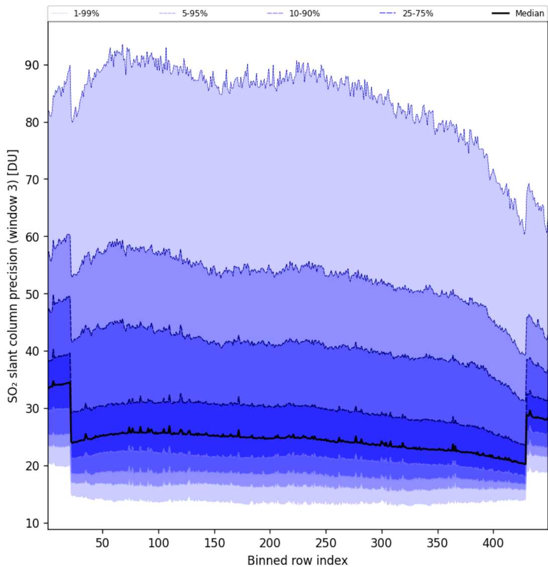
Figure 99: Along track statistics of “SO 2 slant column precision (window 3)” for 2025-04-08 to 2025-04-09
