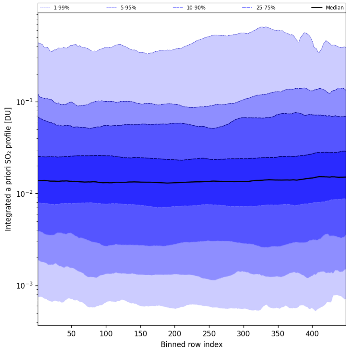
Figure 103: Along track statistics of “Integrated a priori SO 2 profile” for 2025-04-08 to 2025-04-09
