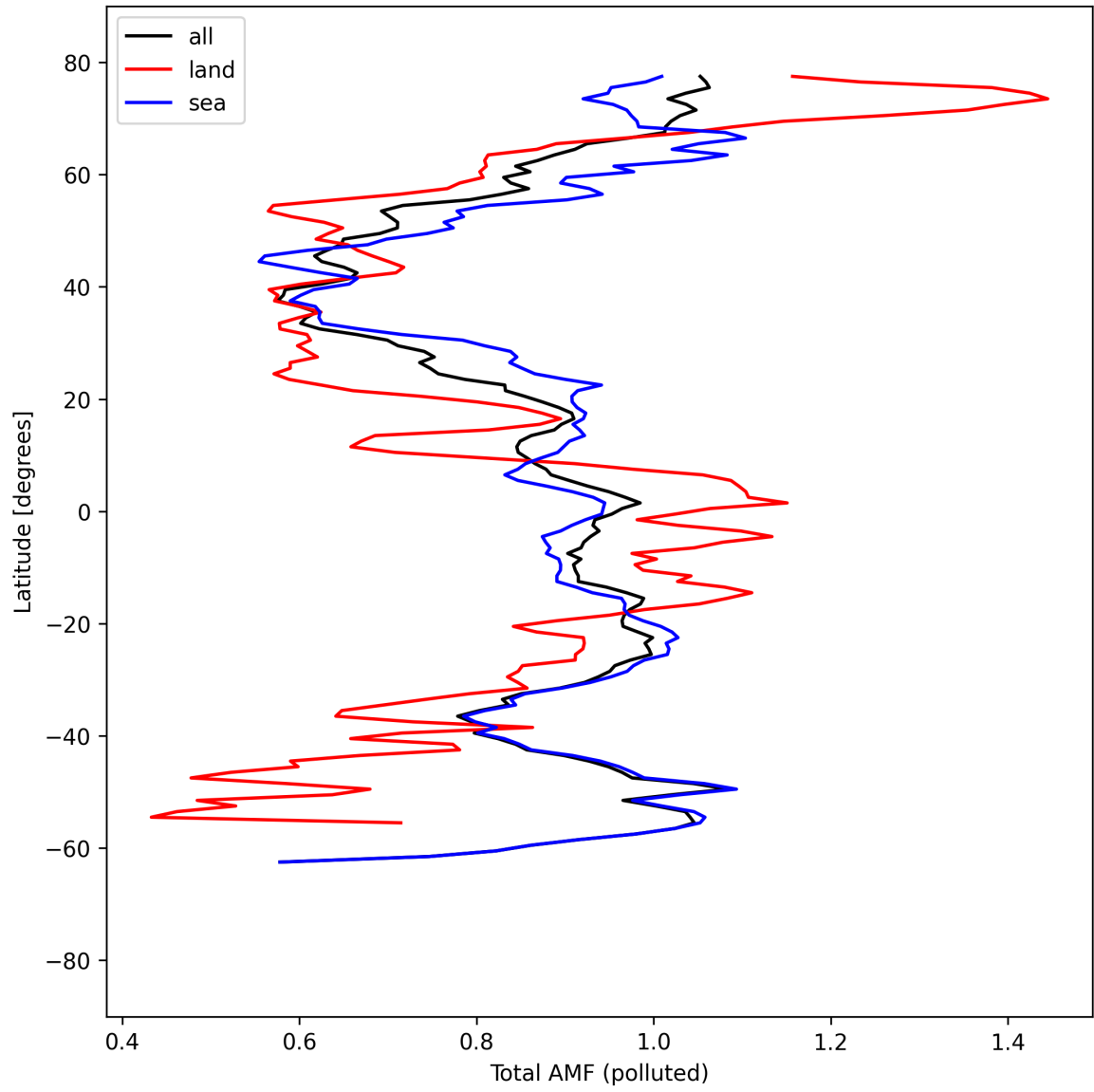
Figure 53: Zonal average of “Total AMF (polluted)” for 2025-04-08 to 2025-04-09.
