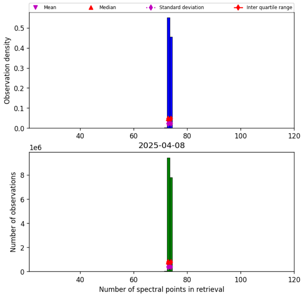
Figure 83: Histogram of “Number of spectral points in retrieval” for 2025-04-08 to 2025-04-09
