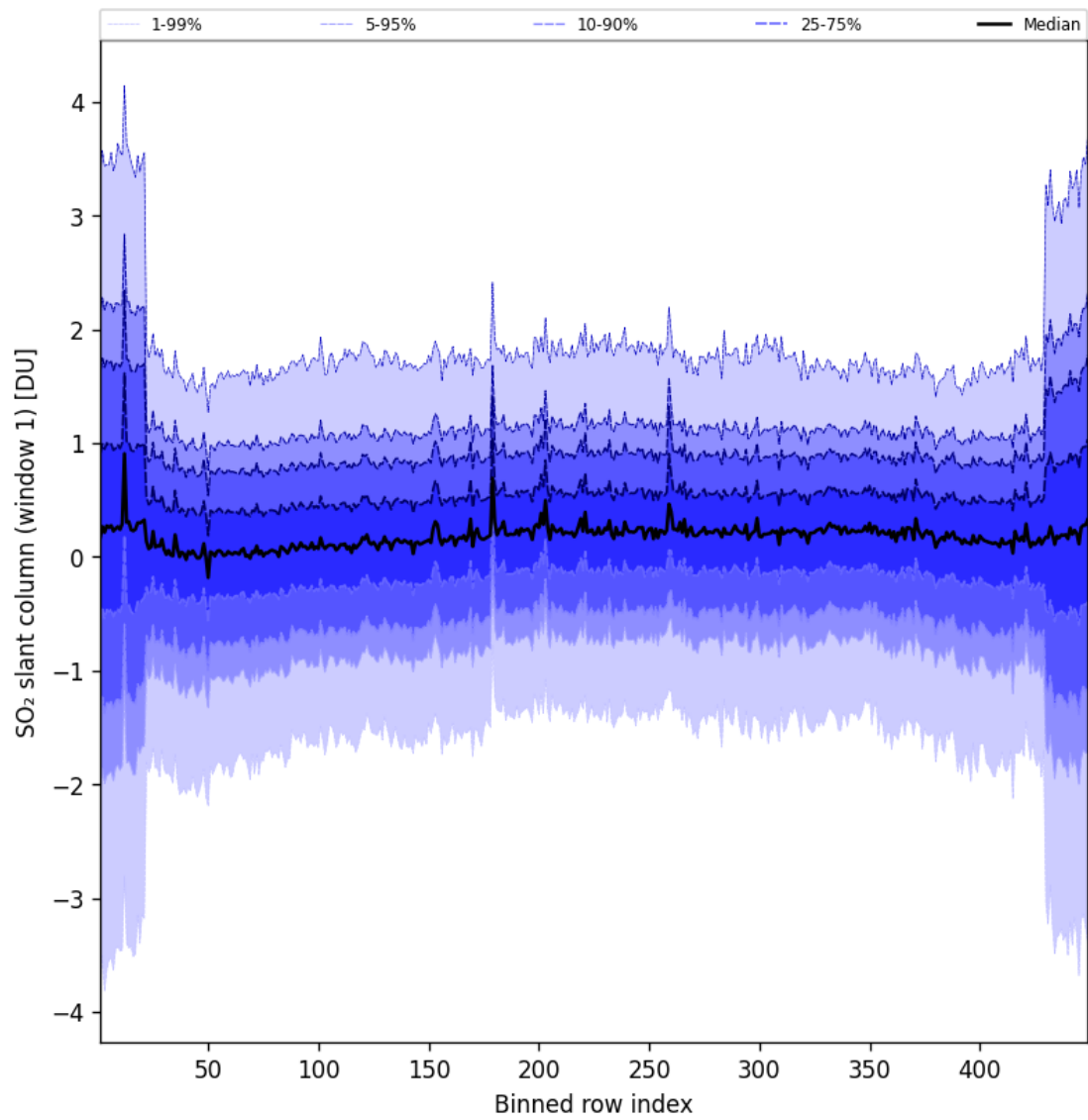
Figure 90: Along track statistics of “SO 2 slant column (window 1)” for 2025-04-08 to 2025-04-09
