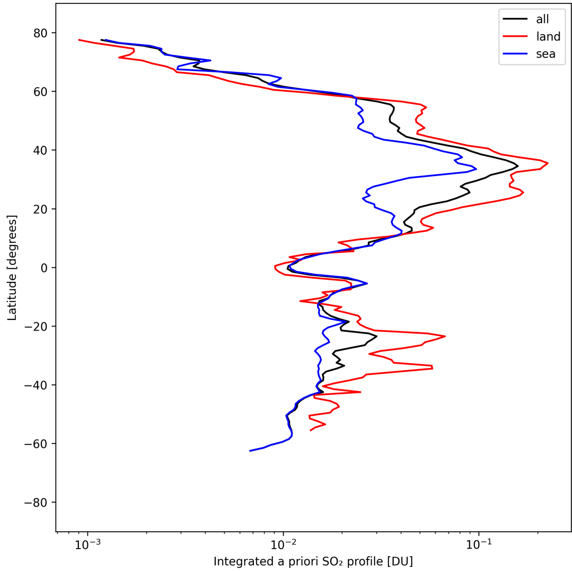
Figure 49: Zonal average of “Integrated a priori SO 2 profile” for 2025-04-08 to 2025-04-09.
