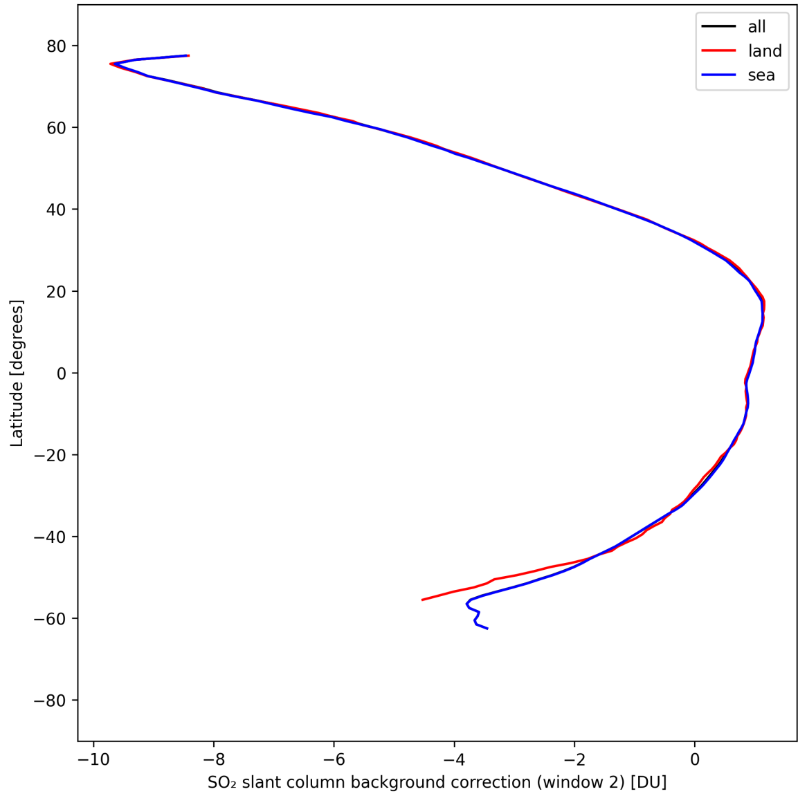
Figure 43: Zonal average of “SO 2 slant column background correction (window 2)” for 2025-04-08 to 2025-04-09.
