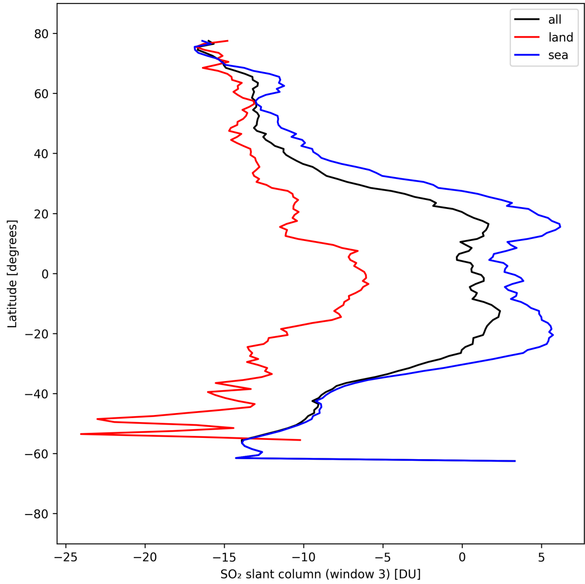
Figure 44: Zonal average of “SO 2 slant column (window 3)” for 2025-04-08 to 2025-04-09.
