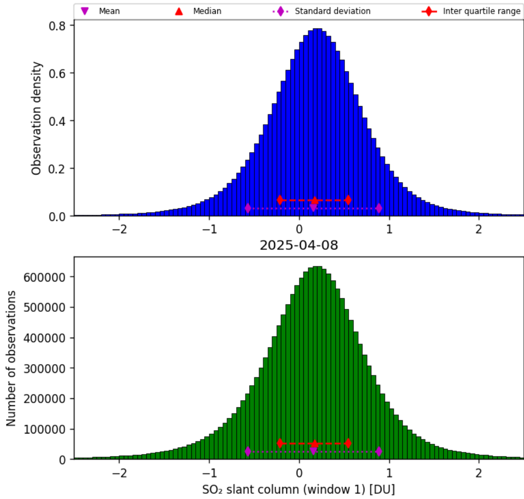
Figure 63: Histogram of “SO 2 slant column (window 1)” for 2025-04-08 to 2025-04-09
