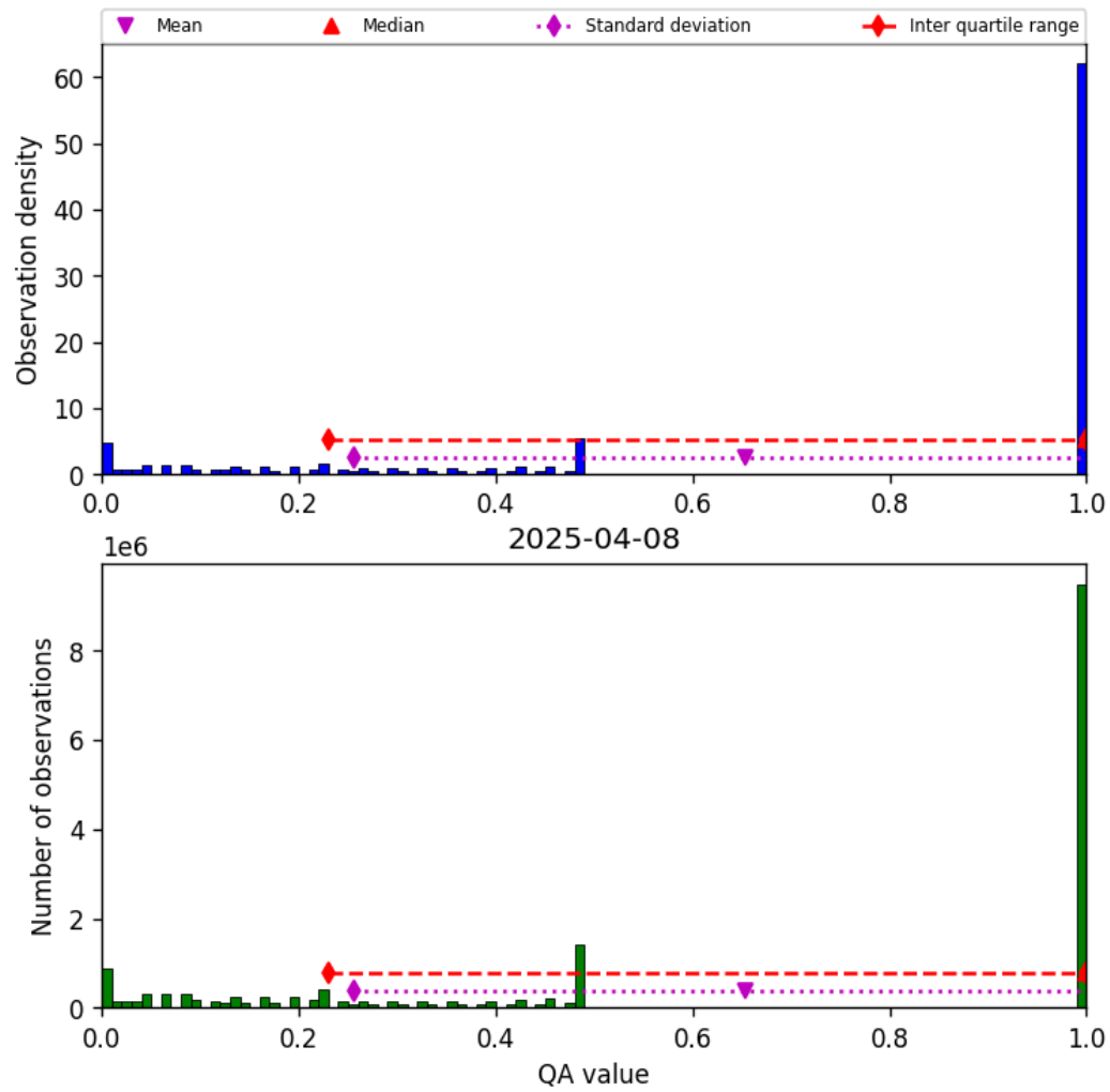
Figure 57: Histogram of “QA value” for 2025-04-08 to 2025-04-09
