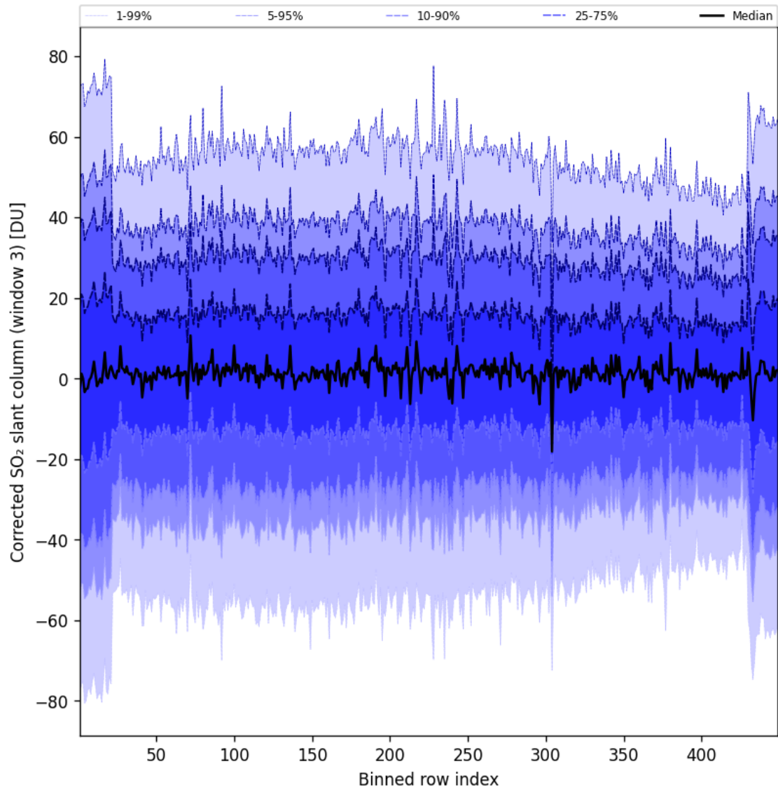
Figure 100: Along track statistics of “Corrected SO 2 slant column (window 3)” for 2025-04-08 to 2025-04-09
