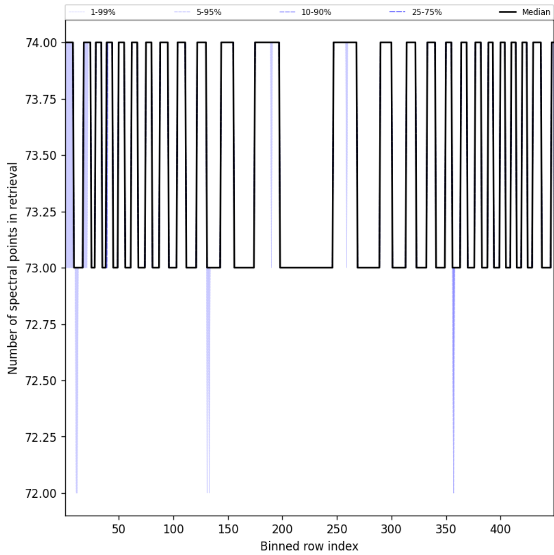
Figure 110: Along track statistics of “Number of spectral points in retrieval” for 2025-04-08 to 2025-04-09
