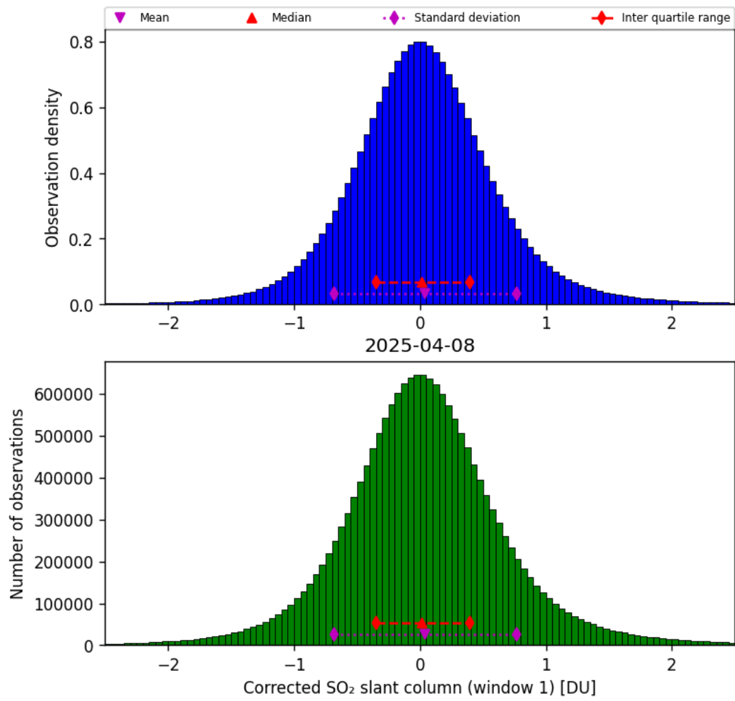
Figure 65: Histogram of “Corrected SO 2 slant column (window 1)” for 2025-04-08 to 2025-04-09
