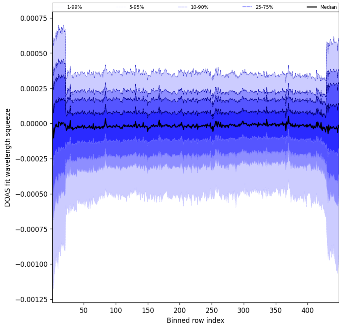
Figure 105: Along track statistics of “DOAS fit wavelength squeeze” for 2025-04-08 to 2025-04-09
