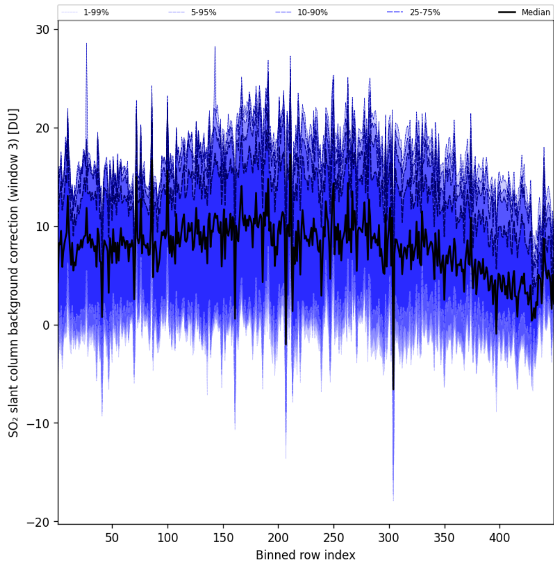
Figure 101: Along track statistics of “SO 2 slant column background correction (window 3)” for 2025-04-08 to 2025-04-09
