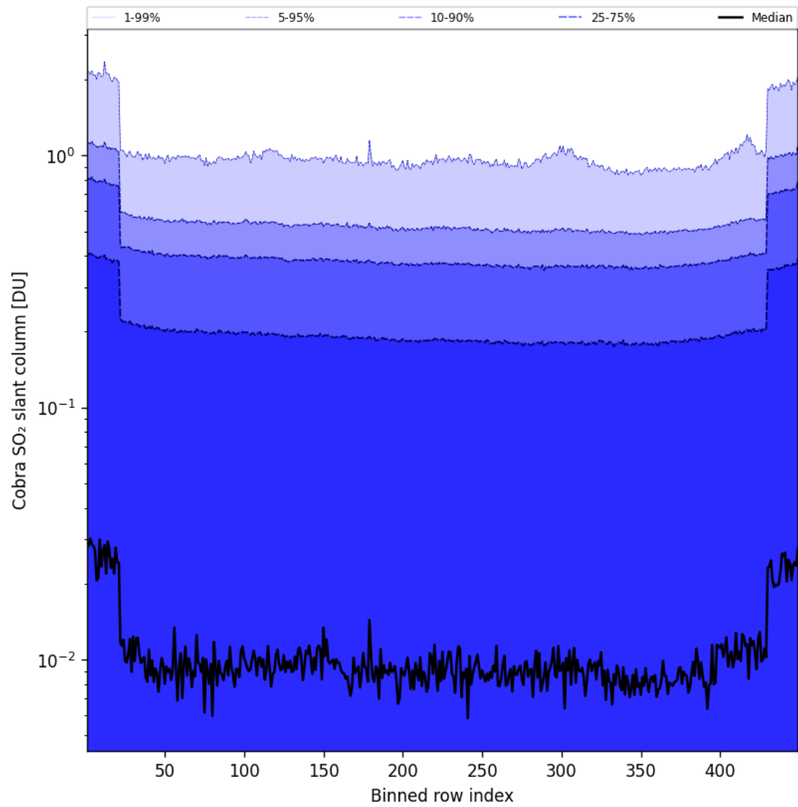
Figure 88: Along track statistics of “Cobra SO 2 slant column” for 2025-04-08 to 2025-04-09
