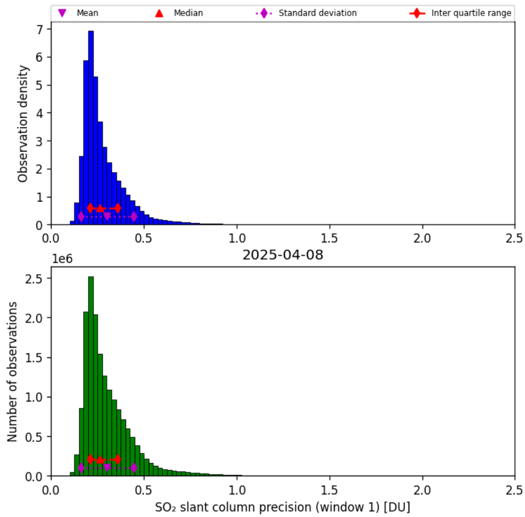
Figure 64: Histogram of “SO 2 slant column precision (window 1)” for 2025-04-08 to 2025-04-09
