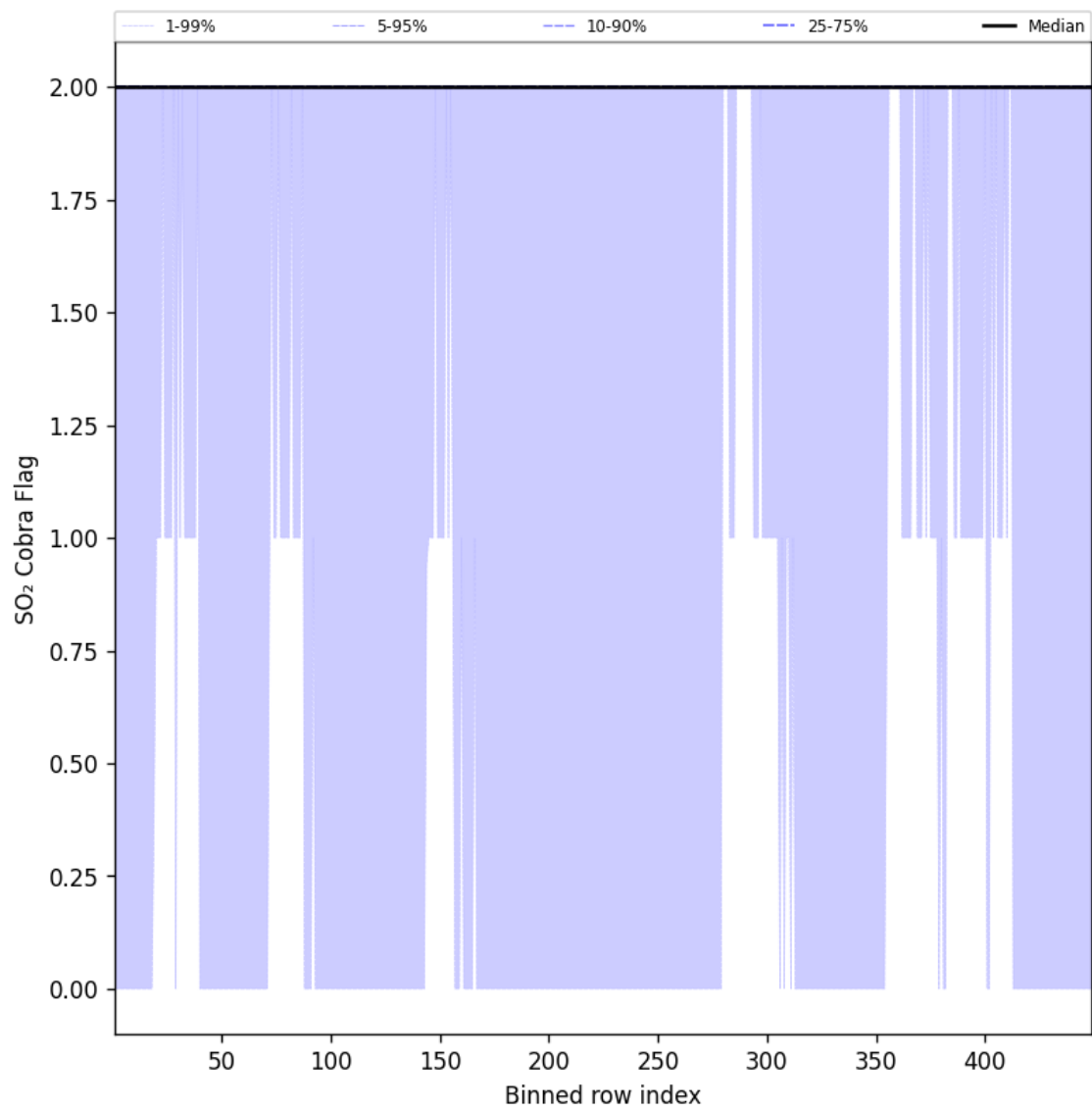
Figure 102: Along track statistics of “SO 2 Cobra Flag” for 2025-04-08 to 2025-04-09
