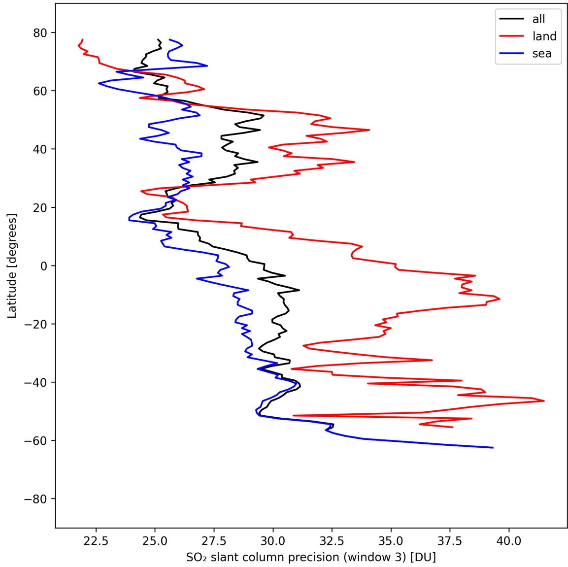
Figure 45: Zonal average of "SO 2 slant column precision (window 3)" for 2025-04-08 to 2025-04-09.
