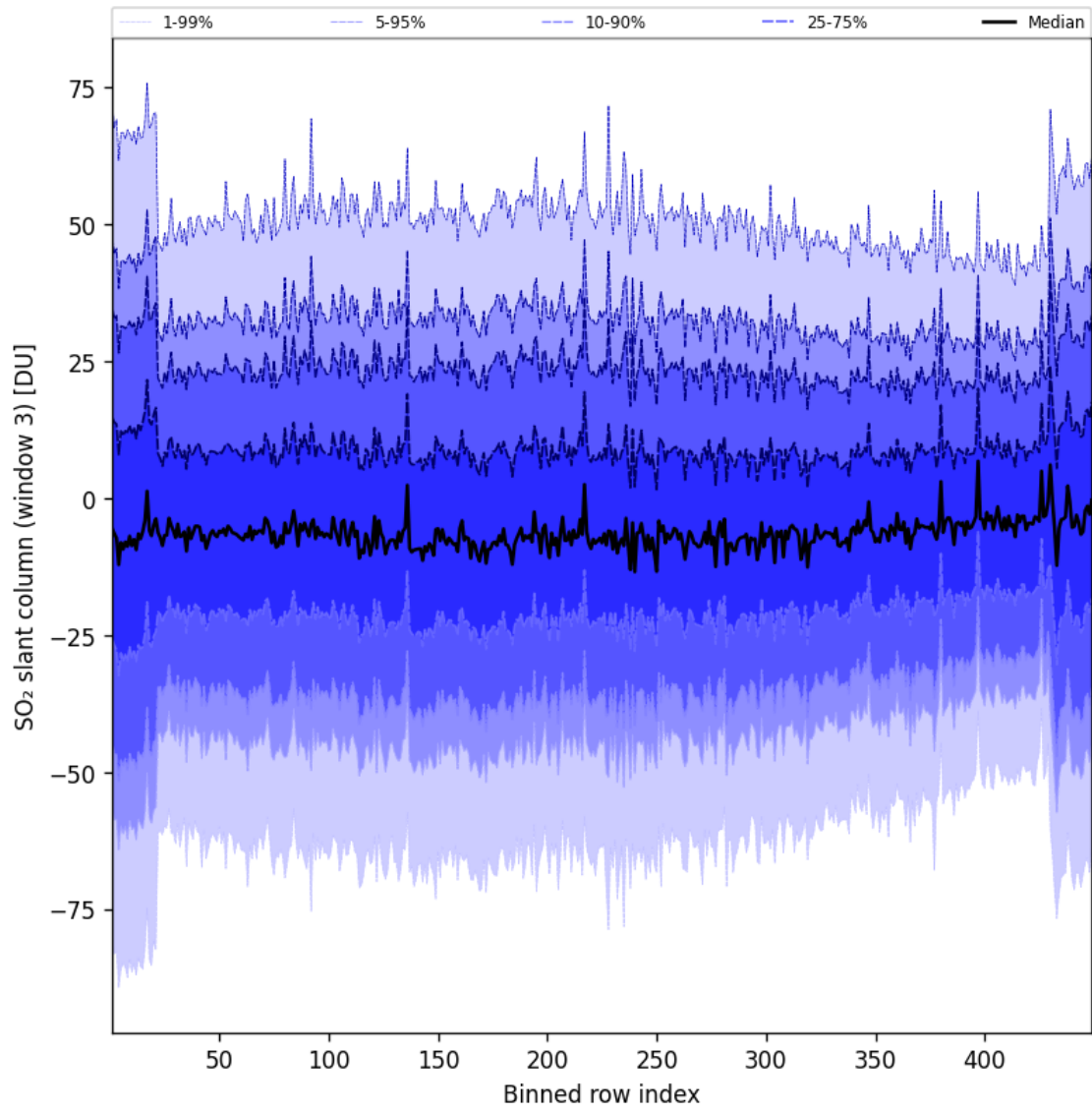
Figure 98: Along track statistics of “SO 2 slant column (window 3)” for 2025-04-08 to 2025-04-09
