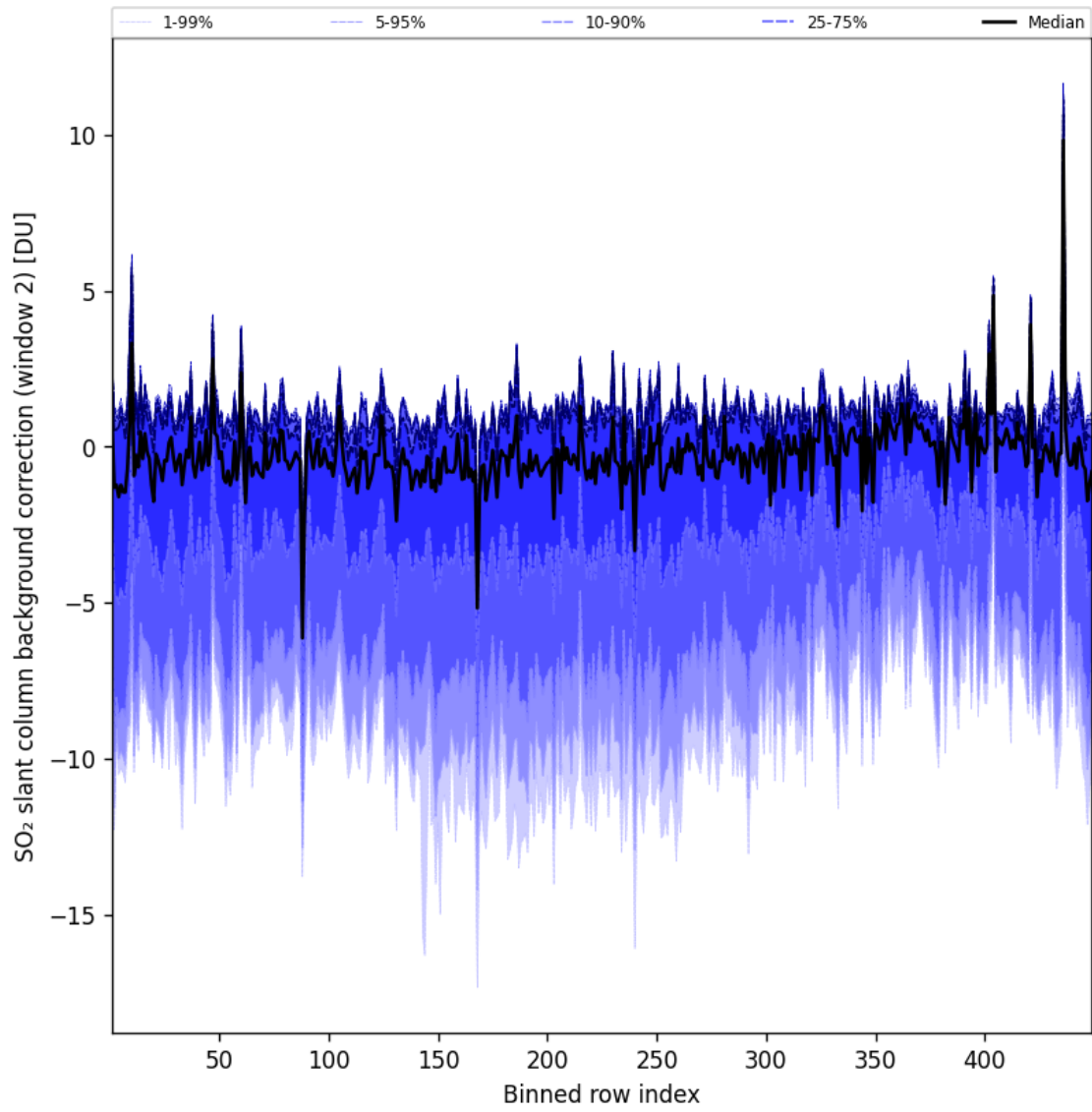
Figure 97: Along track statistics of “SO 2 slant column background correction (window 2)” for 2025-04-08 to 2025-04-09
