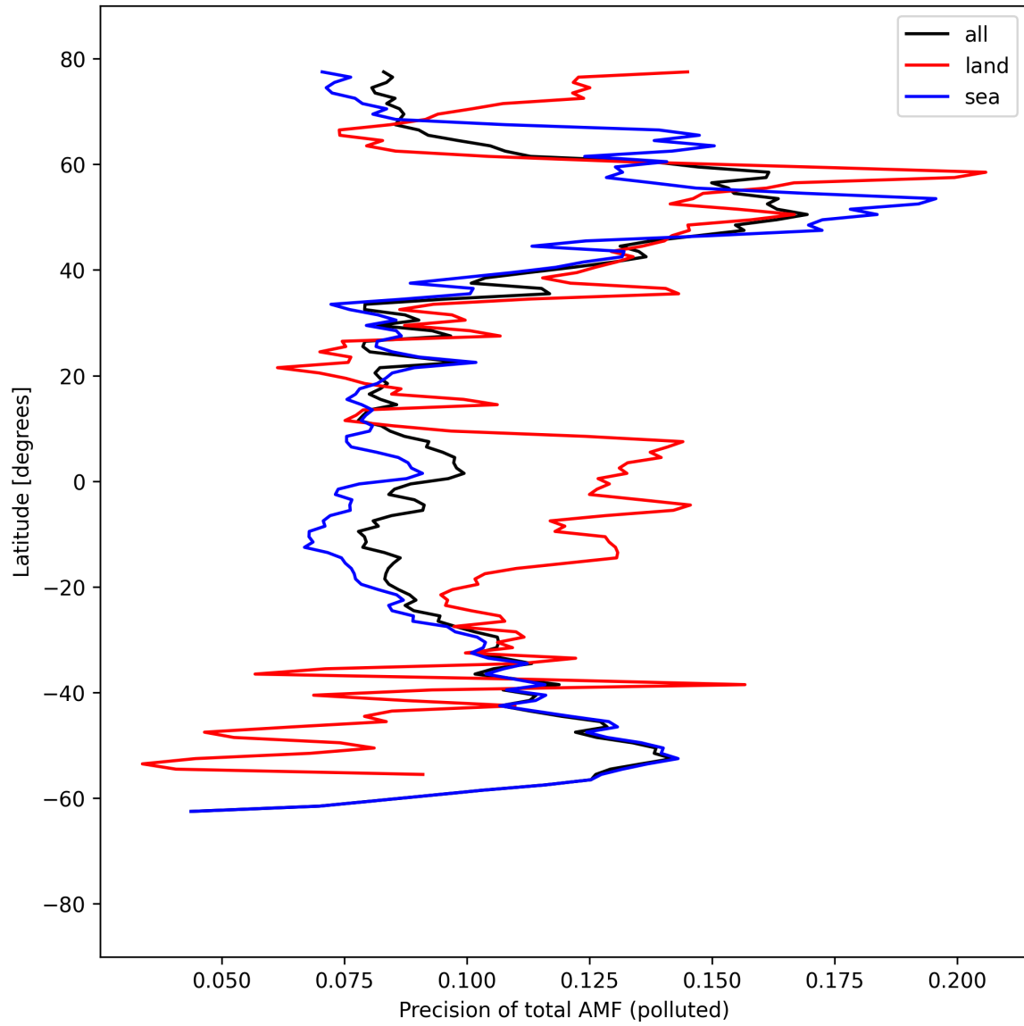
Figure 54: Zonal average of “Precision of total AMF (polluted)” for 2025-04-08 to 2025-04-09.
