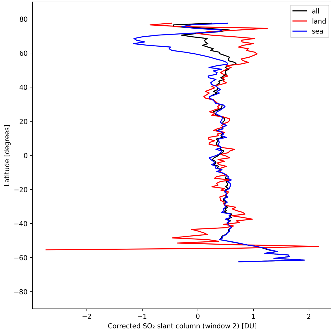
Figure 42: Zonal average of “Corrected SO 2 slant column (window 2)” for 2025-04-08 to 2025-04-09.
