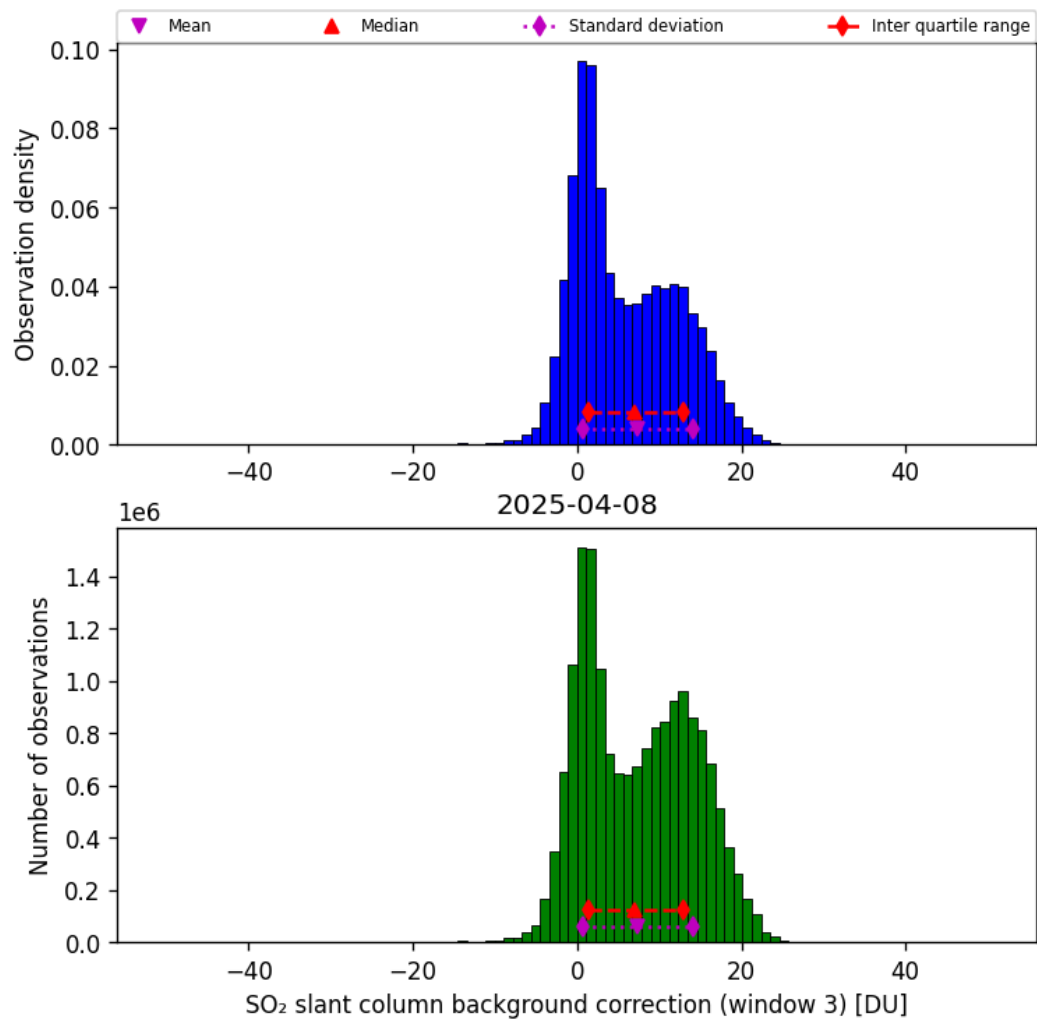
Figure 74: Histogram of “SO 2 slant column background correction (window 3)” for 2025-04-08 to 2025-04-09
