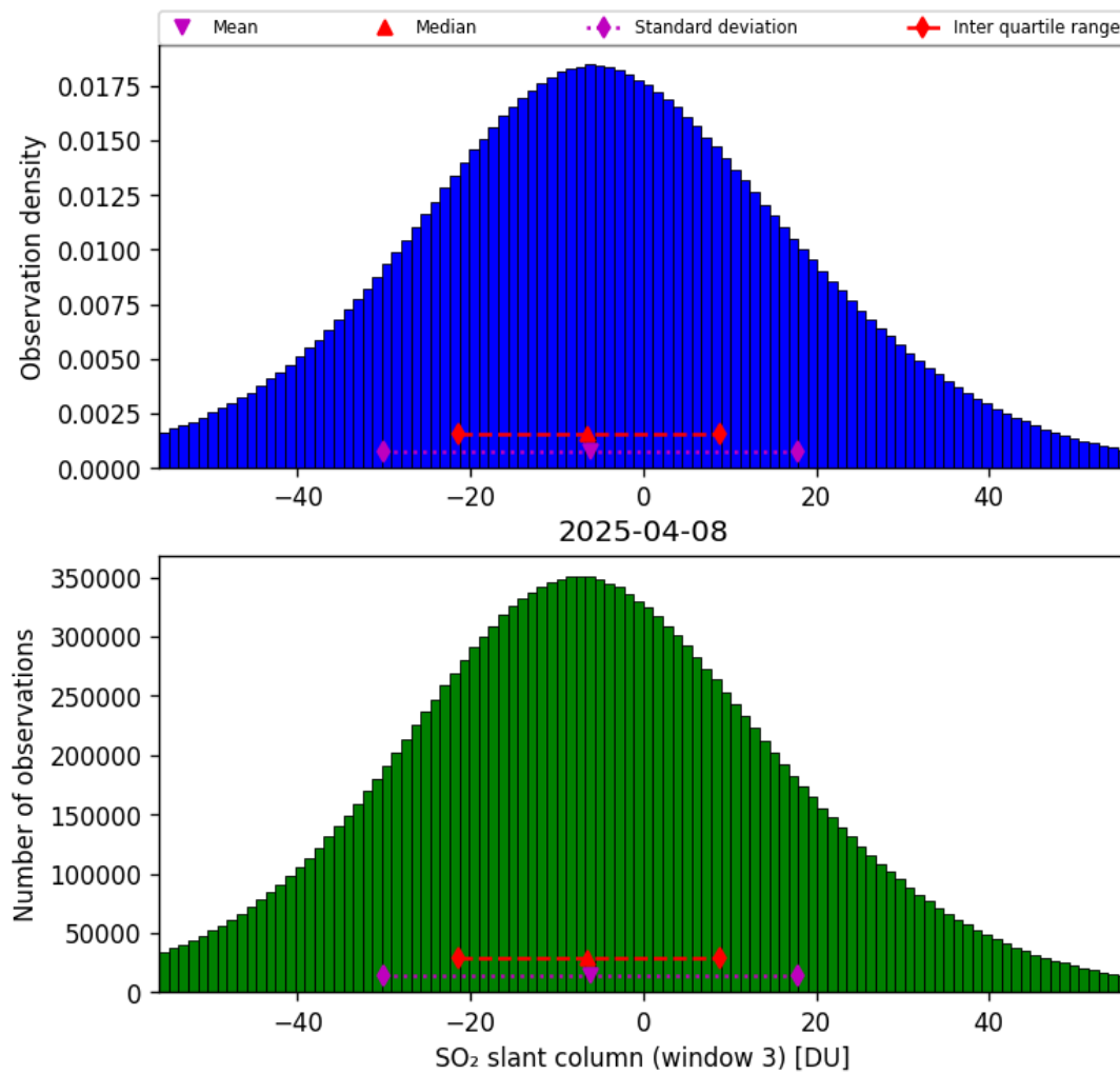
Figure 71: Histogram of “SO 2 slant column (window 3)” for 2025-04-08 to 2025-04-09
