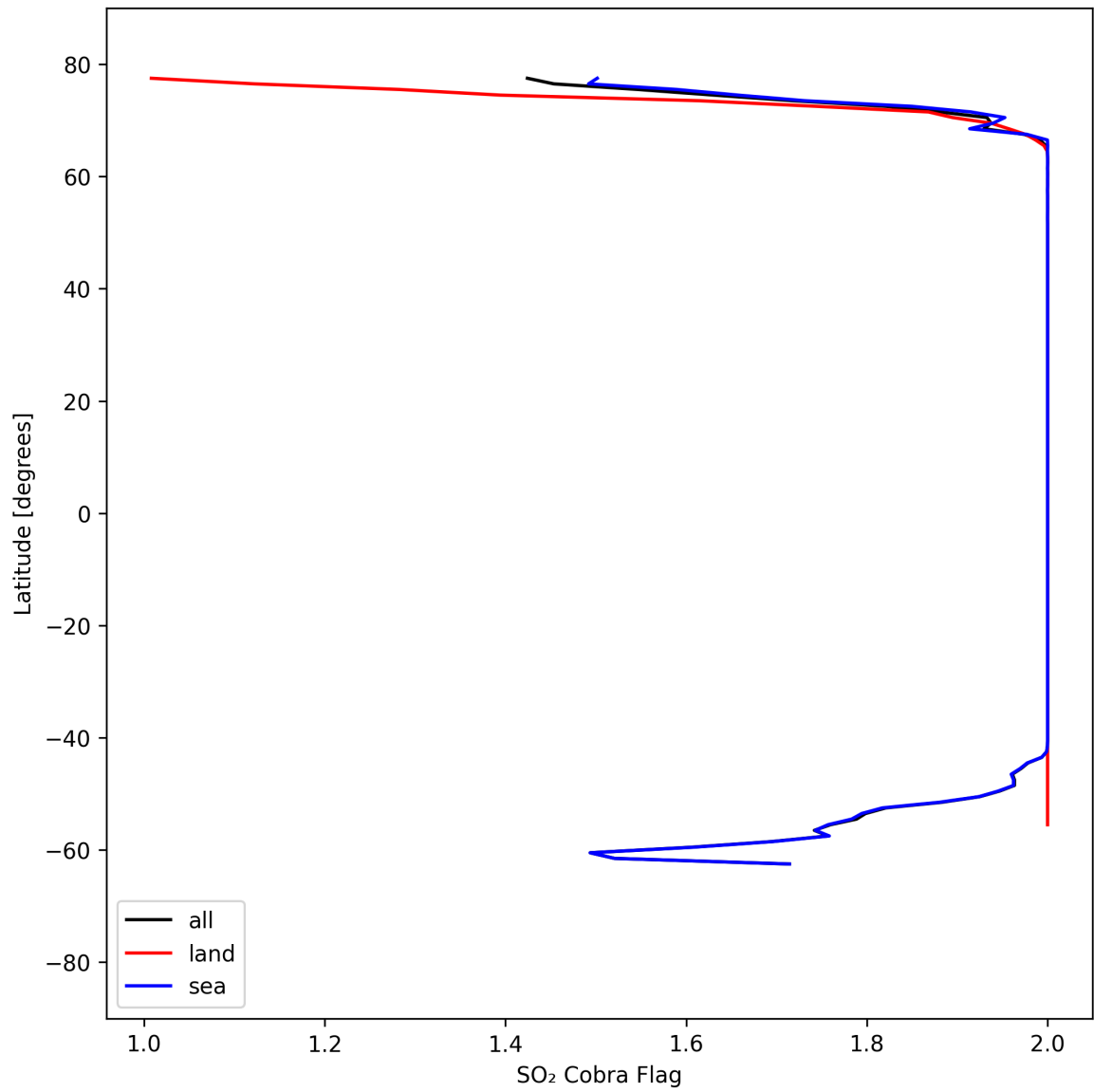
Figure 48: Zonal average of "SO 2 Cobra Flag" for 2025-04-08 to 2025-04-09.
