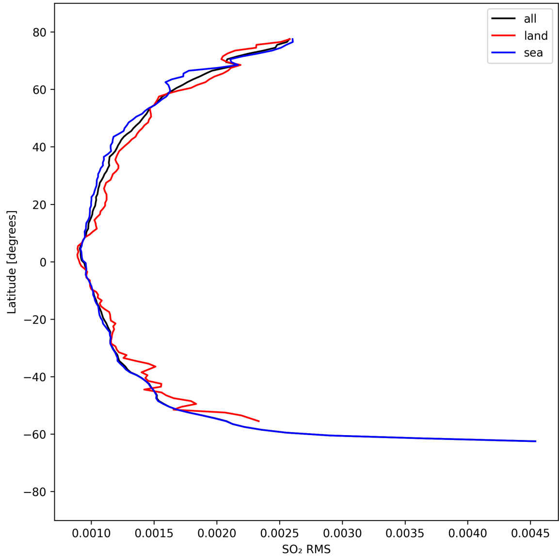
Figure 52: Zonal average of “SO 2 RMS” for 2025-04-08 to 2025-04-09.
