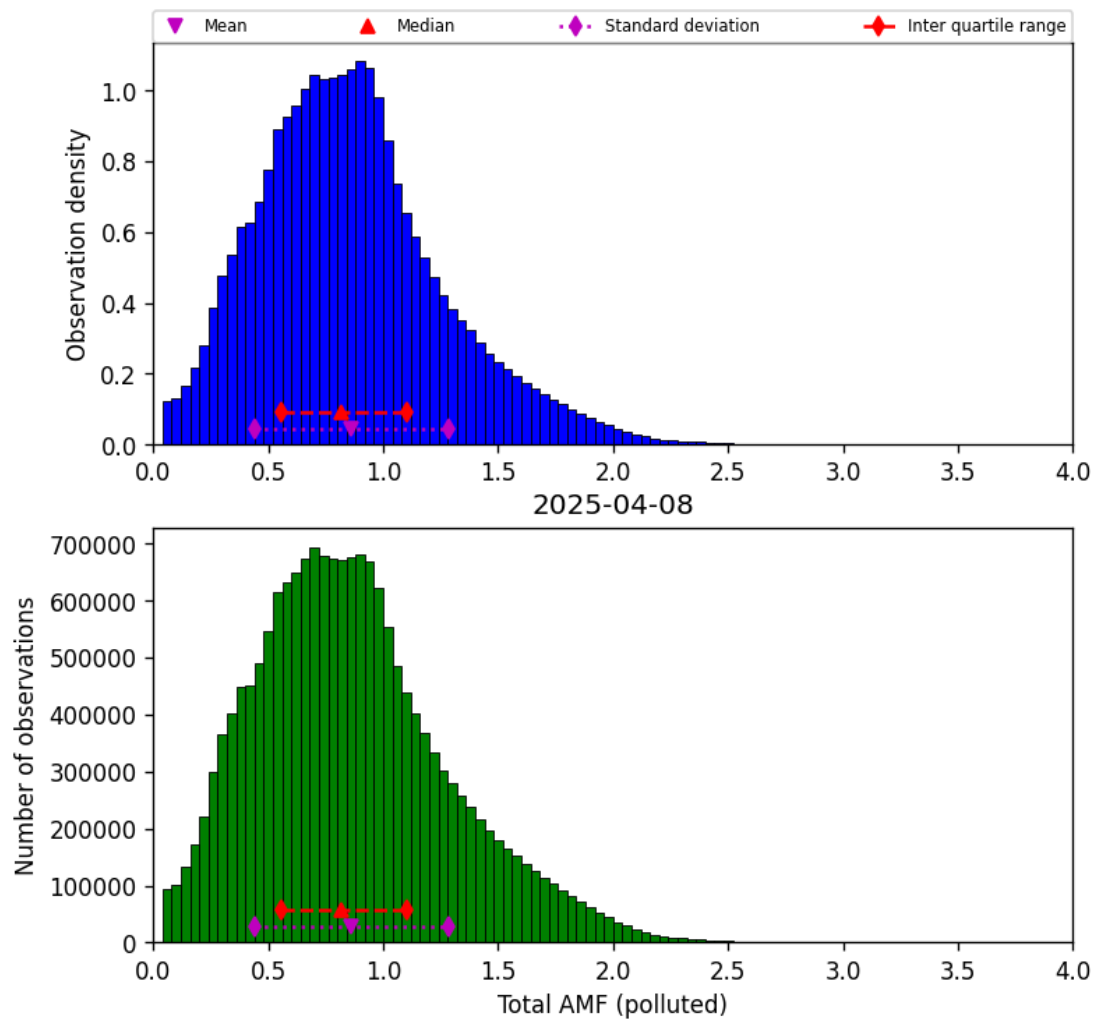
Figure 80: Histogram of “Total AMF (polluted)” for 2025-04-08 to 2025-04-09
