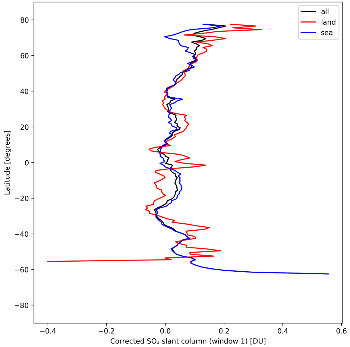
Figure 38: Zonal average of “Corrected SO 2 slant column (window 1)” for 2025-04-08 to 2025-04-09.
