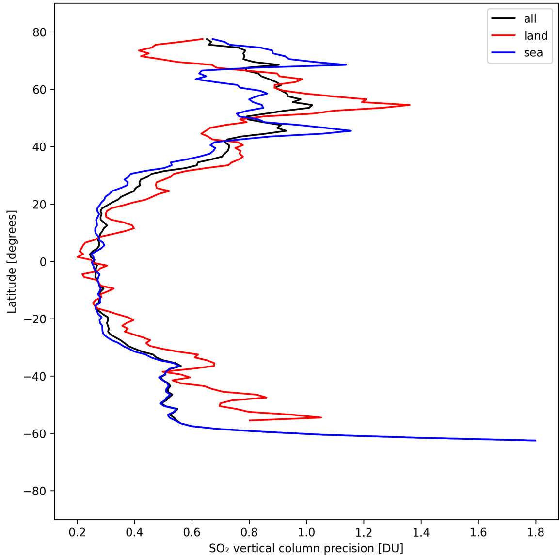
Figure 32: Zonal average of “SO 2 vertical column precision” for 2025-04-08 to 2025-04-09.
