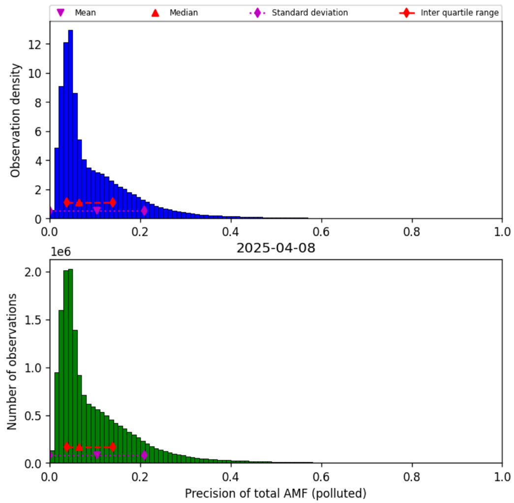
Figure 81: Histogram of “Precision of total AMF (polluted)” for 2025-04-08 to 2025-04-09
