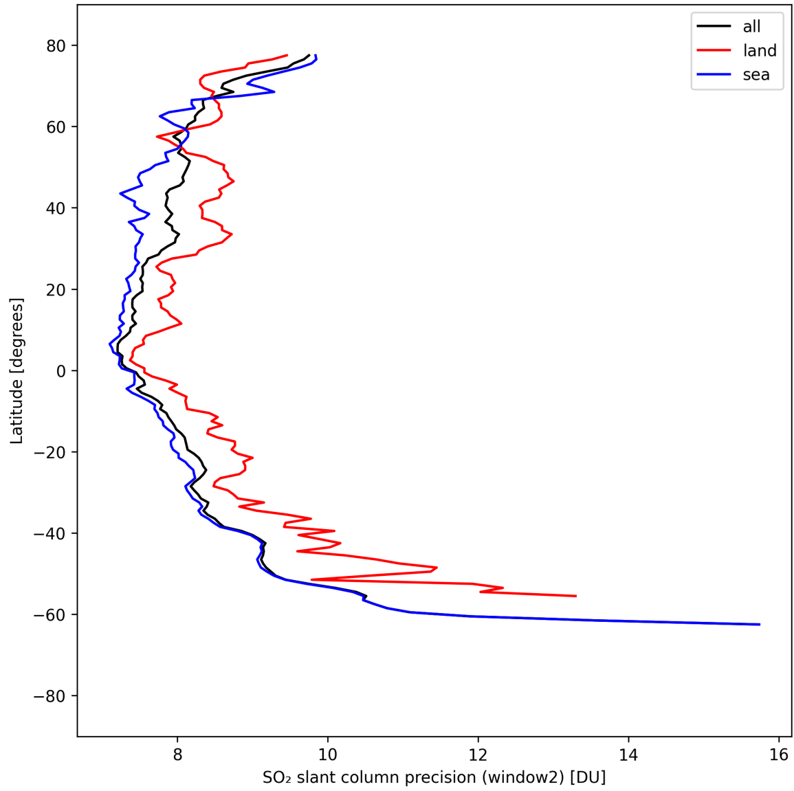
Figure 41: Zonal average of “SO 2 slant column precision (window2)” for 2025-04-08 to 2025-04-09.
