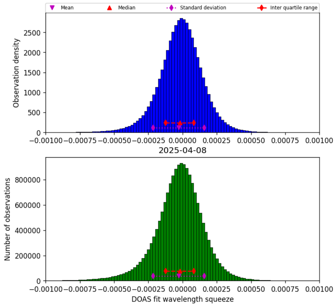
Figure 78: Histogram of “DOAS fit wavelength squeeze” for 2025-04-08 to 2025-04-09
