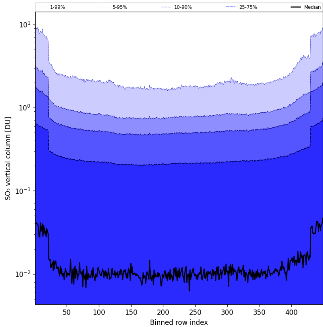
Figure 85: Along track statistics of “SO 2 vertical column” for 2025-04-08 to 2025-04-09
