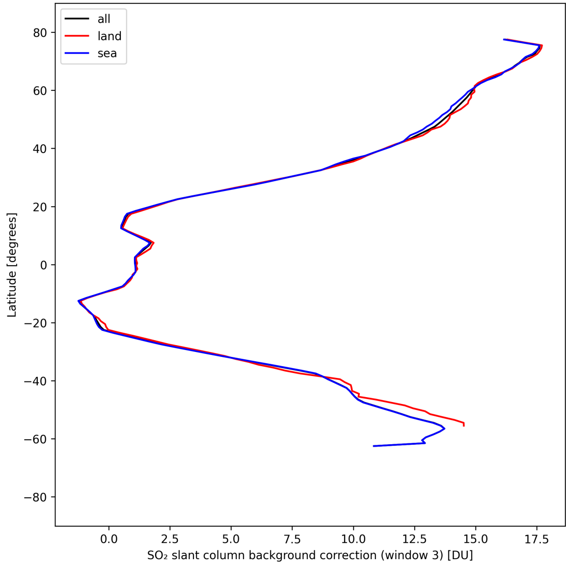
Figure 47: Zonal average of “SO 2 slant column background correction (window 3)” for 2025-04-08 to 2025-04-09.
