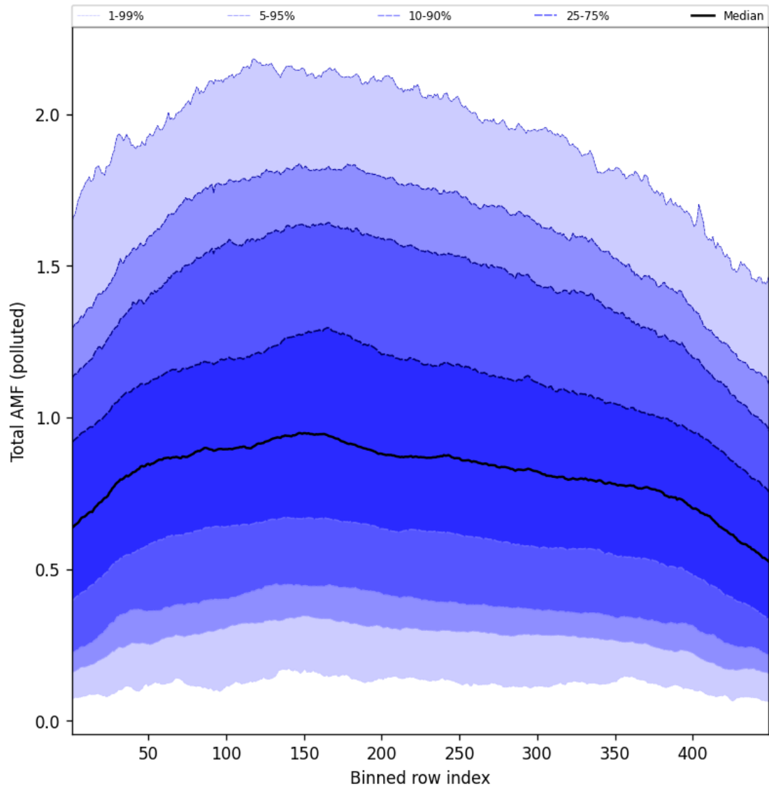
Figure 107: Along track statistics of “Total AMF (polluted)” for 2025-04-08 to 2025-04-09
