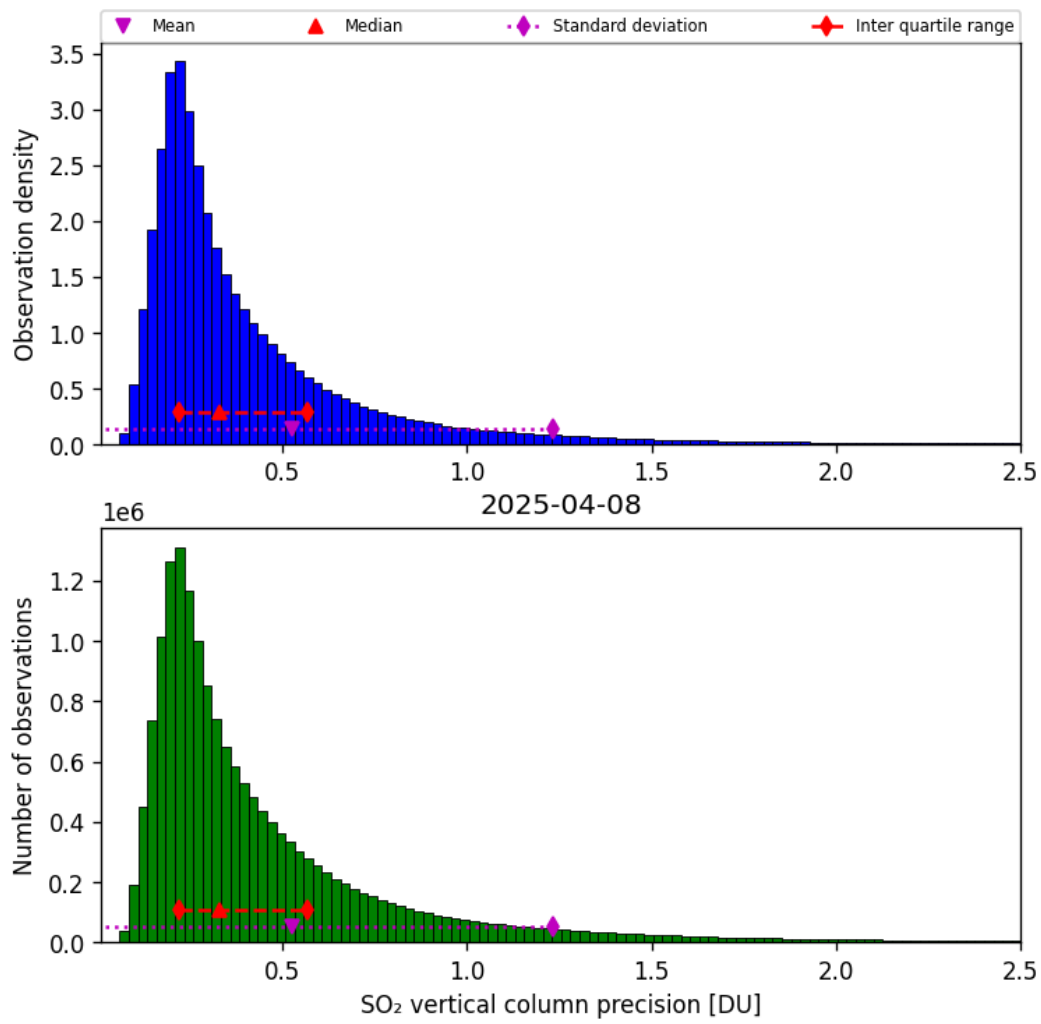
Figure 59: Histogram of “SO 2 vertical column precision” for 2025-04-08 to 2025-04-09
