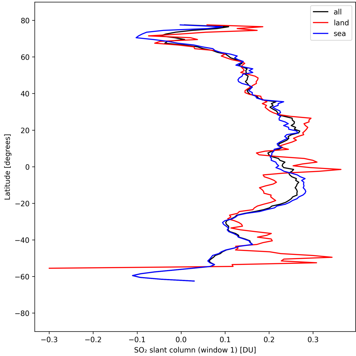
Figure 36: Zonal average of “SO 2 slant column (window 1)” for 2025-04-08 to 2025-04-09.
