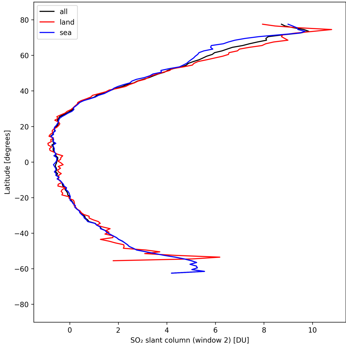
Figure 40: Zonal average of “SO 2 slant column (window 2)” for 2025-04-08 to 2025-04-09.
