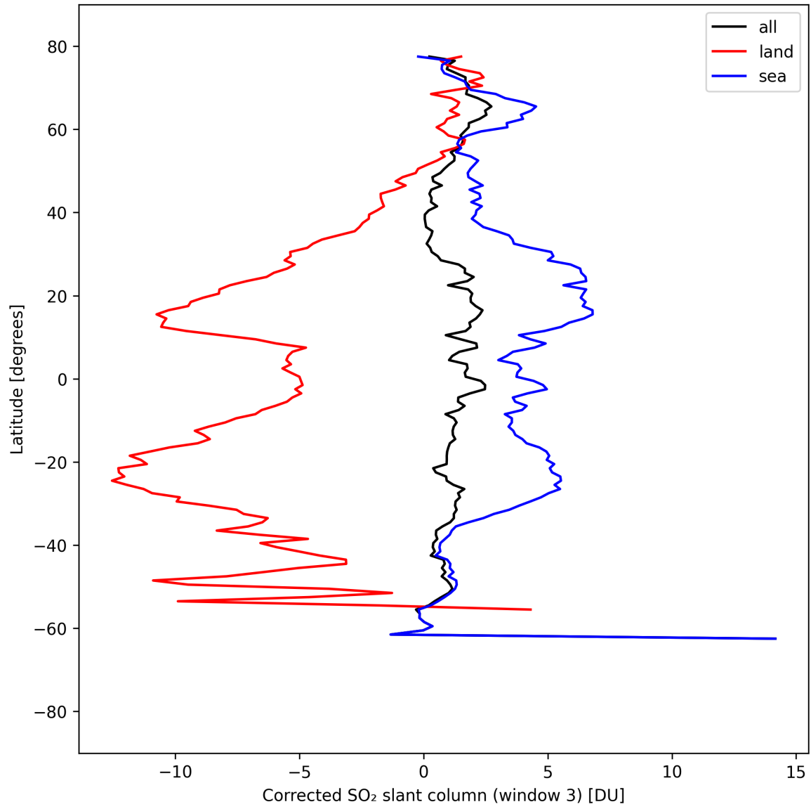
Figure 46: Zonal average of “Corrected SO 2 slant column (window 3)” for 2025-04-08 to 2025-04-09.
