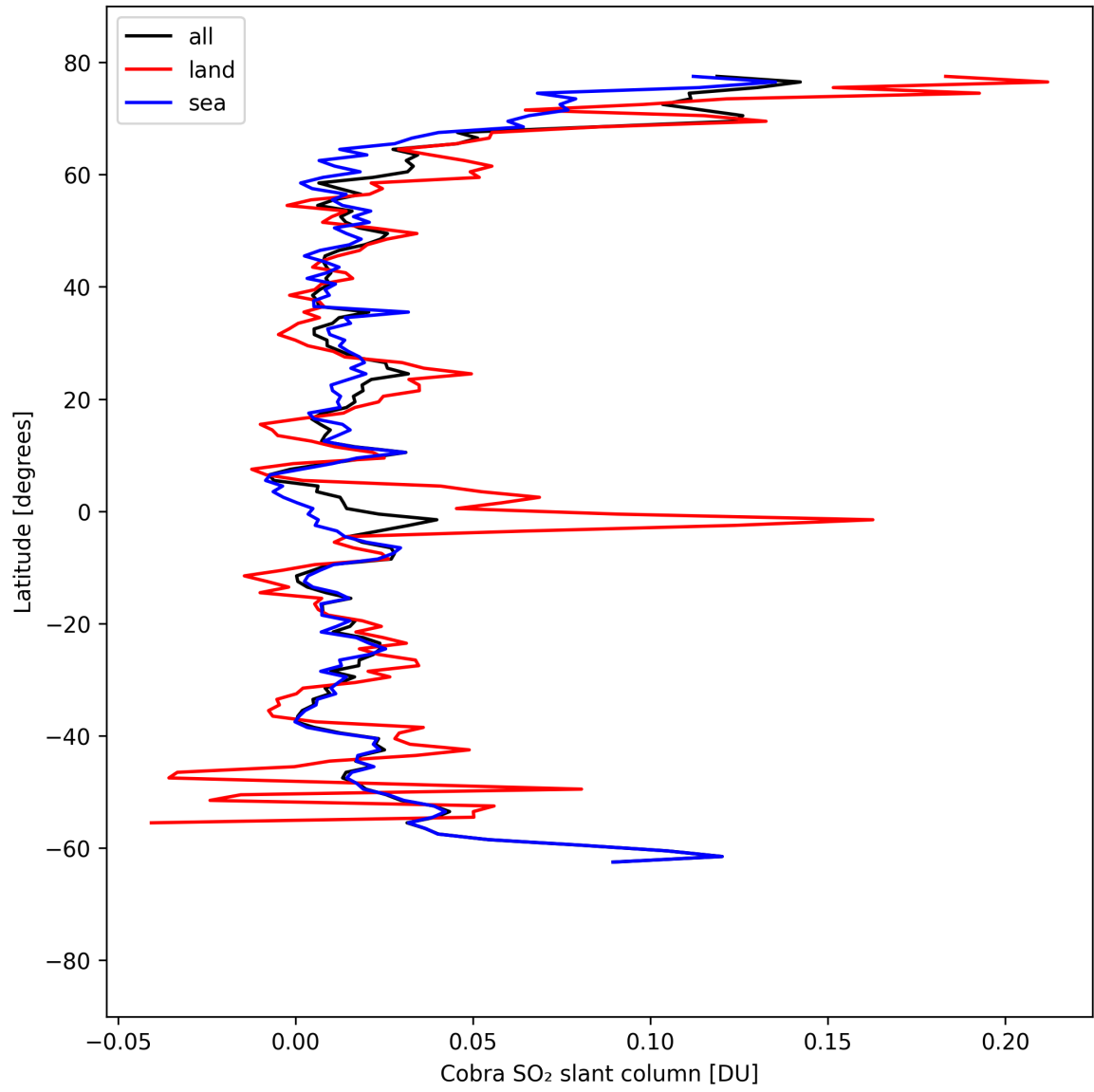
Figure 34: Zonal average of “Cobra SO 2 slant column” for 2025-04-08 to 2025-04-09.
