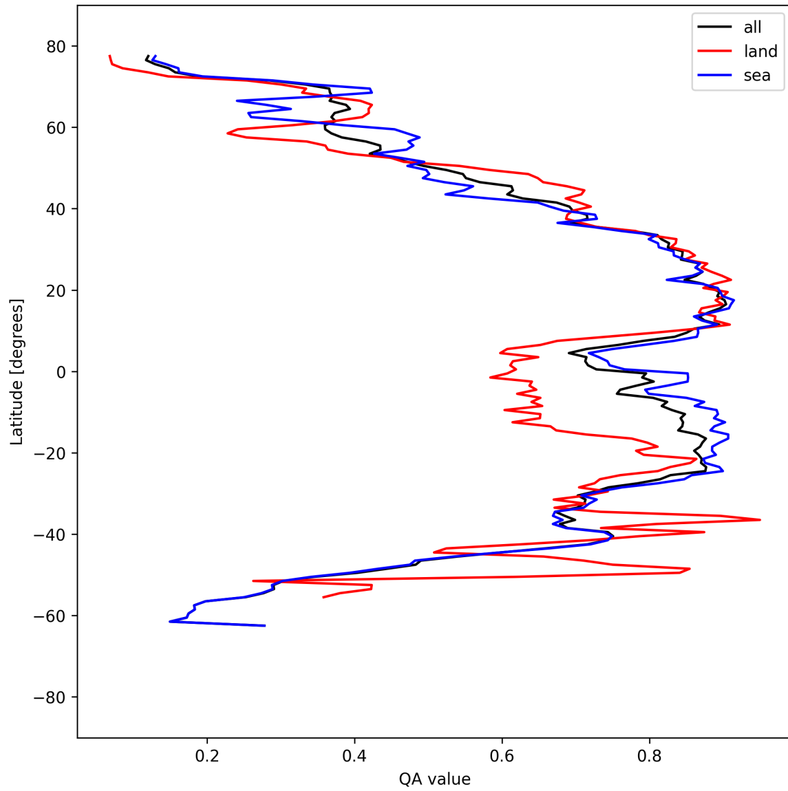
Figure 30: Zonal average of “QA value” for 2025-04-08 to 2025-04-09.
