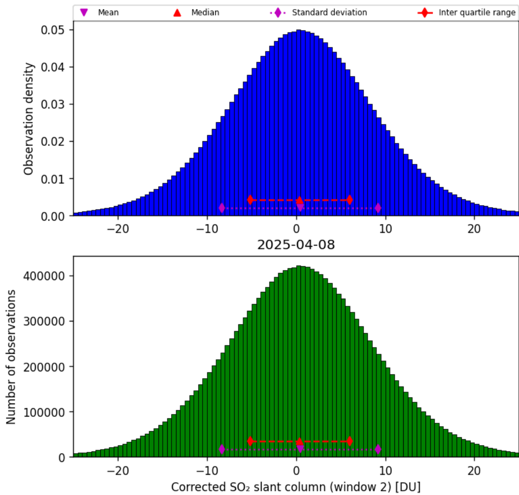
Figure 69: Histogram of “Corrected SO 2 slant column (window 2)” for 2025-04-08 to 2025-04-09
