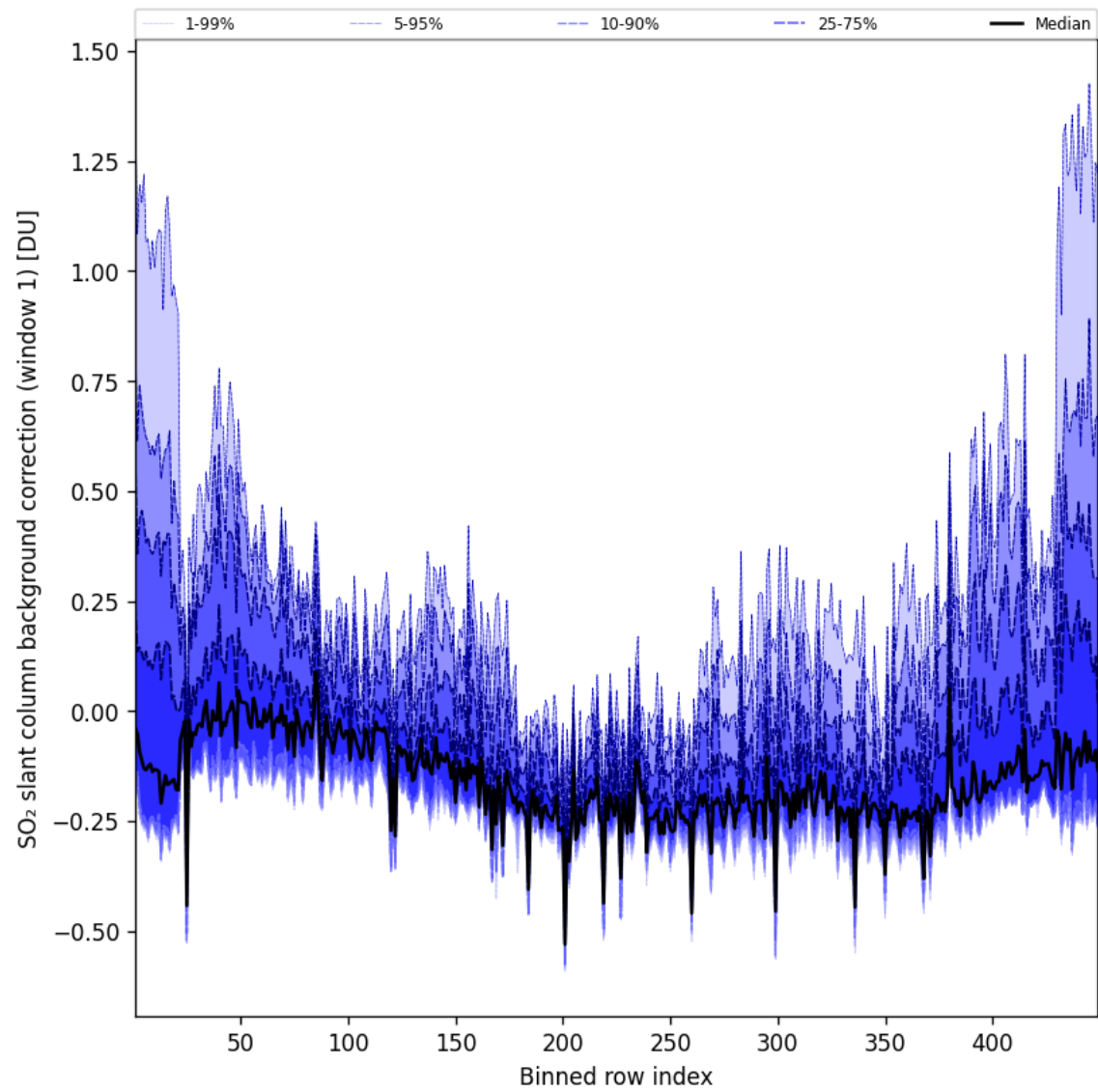
Figure 93: Along track statistics of “SO 2 slant column background correction (window 1)” for 2025-04-08 to 2025-04-09
