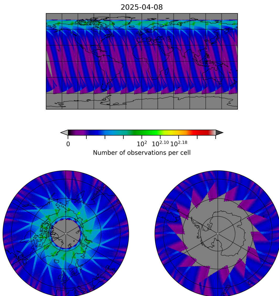
Figure 29: Map of the number of observations for 2025-04-08 to 2025-04-09
