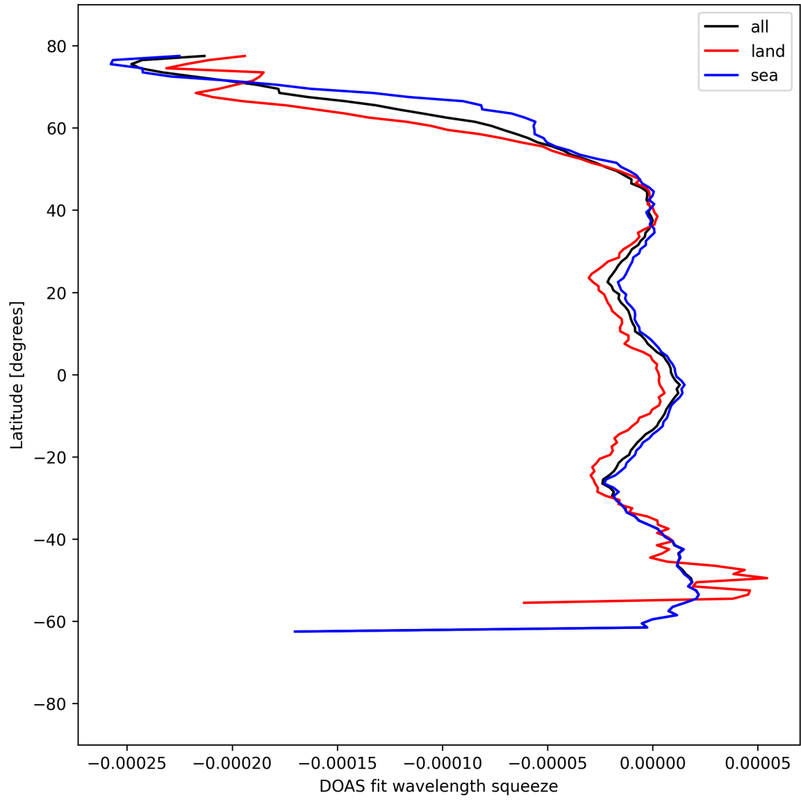
Figure 51: Zonal average of “DOAS fit wavelength squeeze” for 2025-04-08 to 2025-04-09.
