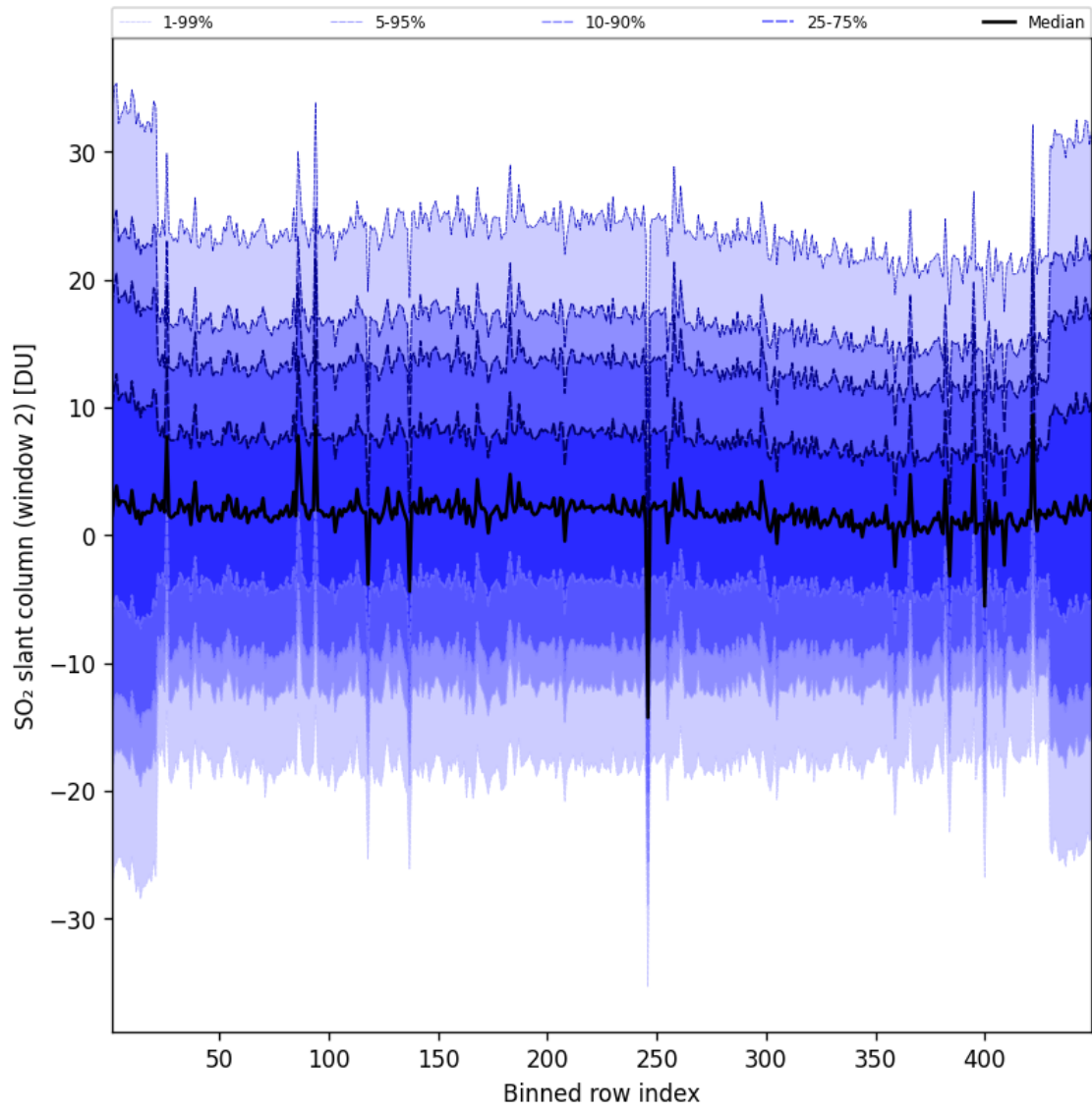
Figure 94: Along track statistics of “SO 2 slant column (window 2)” for 2025-04-08 to 2025-04-09
