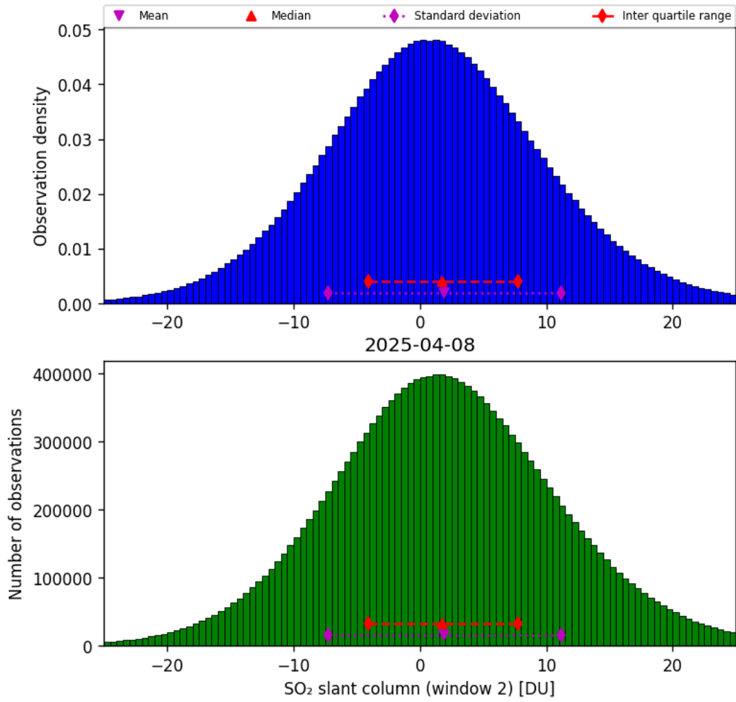
Figure 67: Histogram of “SO 2 slant column (window 2)” for 2025-04-08 to 2025-04-09
