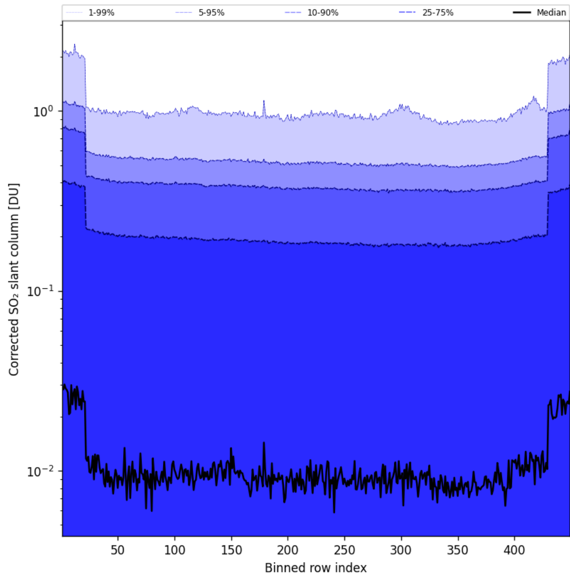
Figure 87: Along track statistics of “Corrected SO 2 slant column” for 2025-04-08 to 2025-04-09
