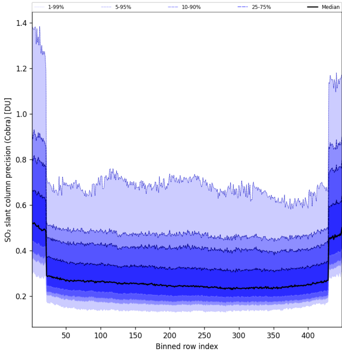
Figure 89: Along track statistics of “SO 2 slant column precision (Cobra)” for 2025-04-08 to 2025-04-09
