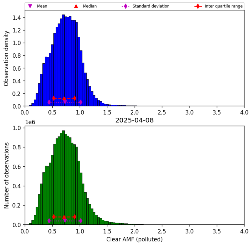
Figure 82: Histogram of “Clear AMF (polluted)” for 2025-04-08 to 2025-04-09
