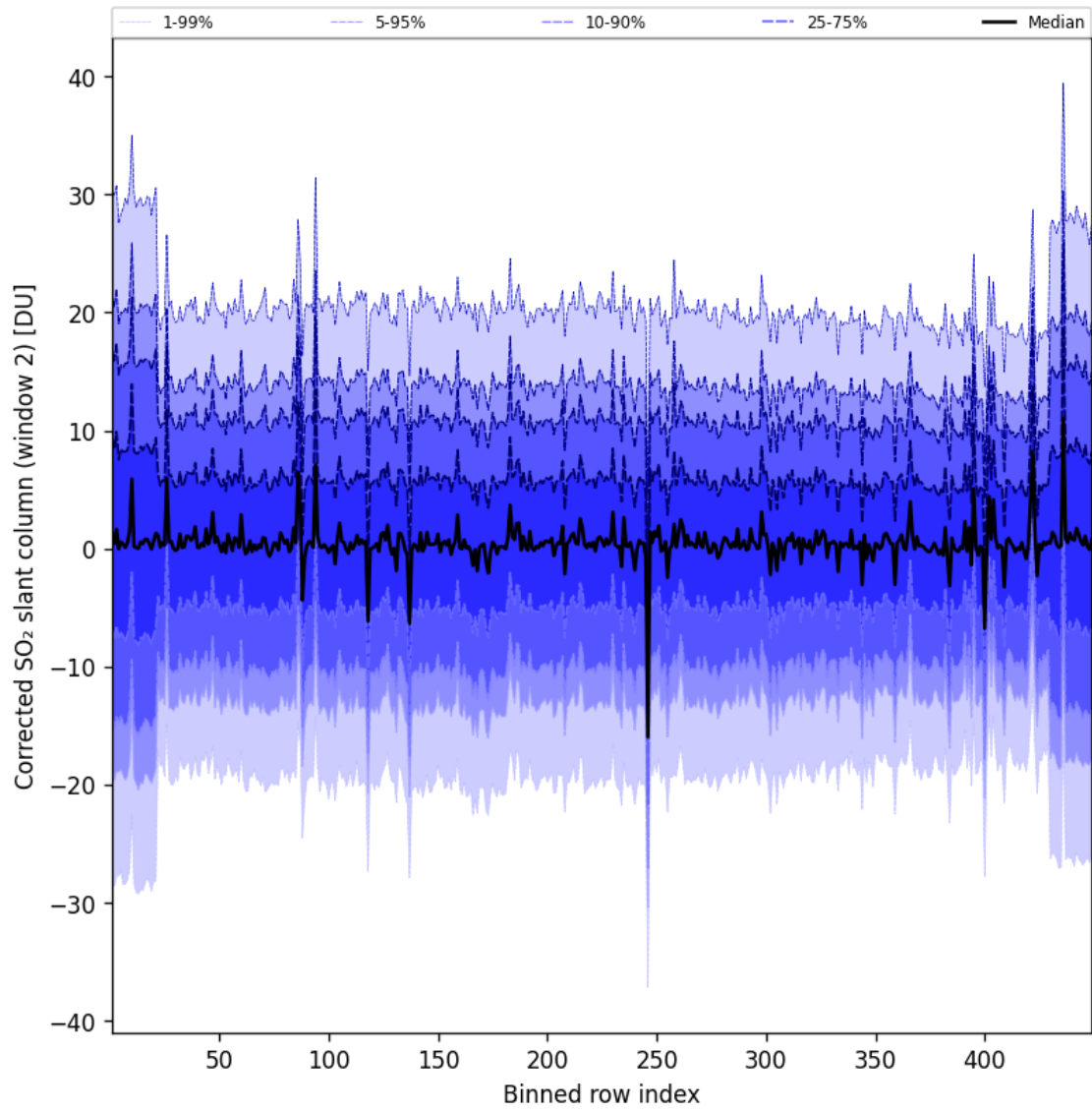
Figure 96: Along track statistics of “Corrected SO 2 slant column (window 2)” for 2025-04-08 to 2025-04-09
