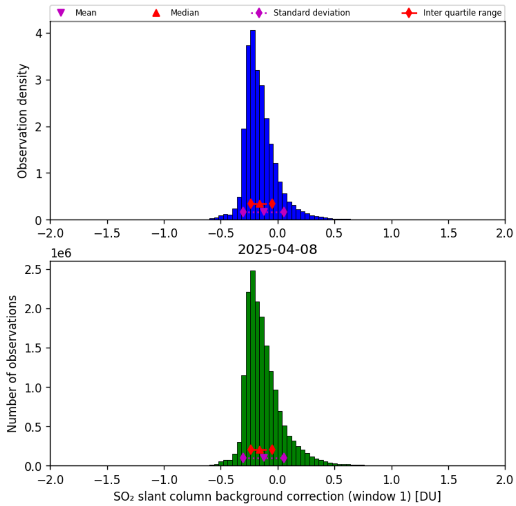
Figure 66: Histogram of “SO 2 slant column background correction (window 1)” for 2025-04-08 to 2025-04-09
