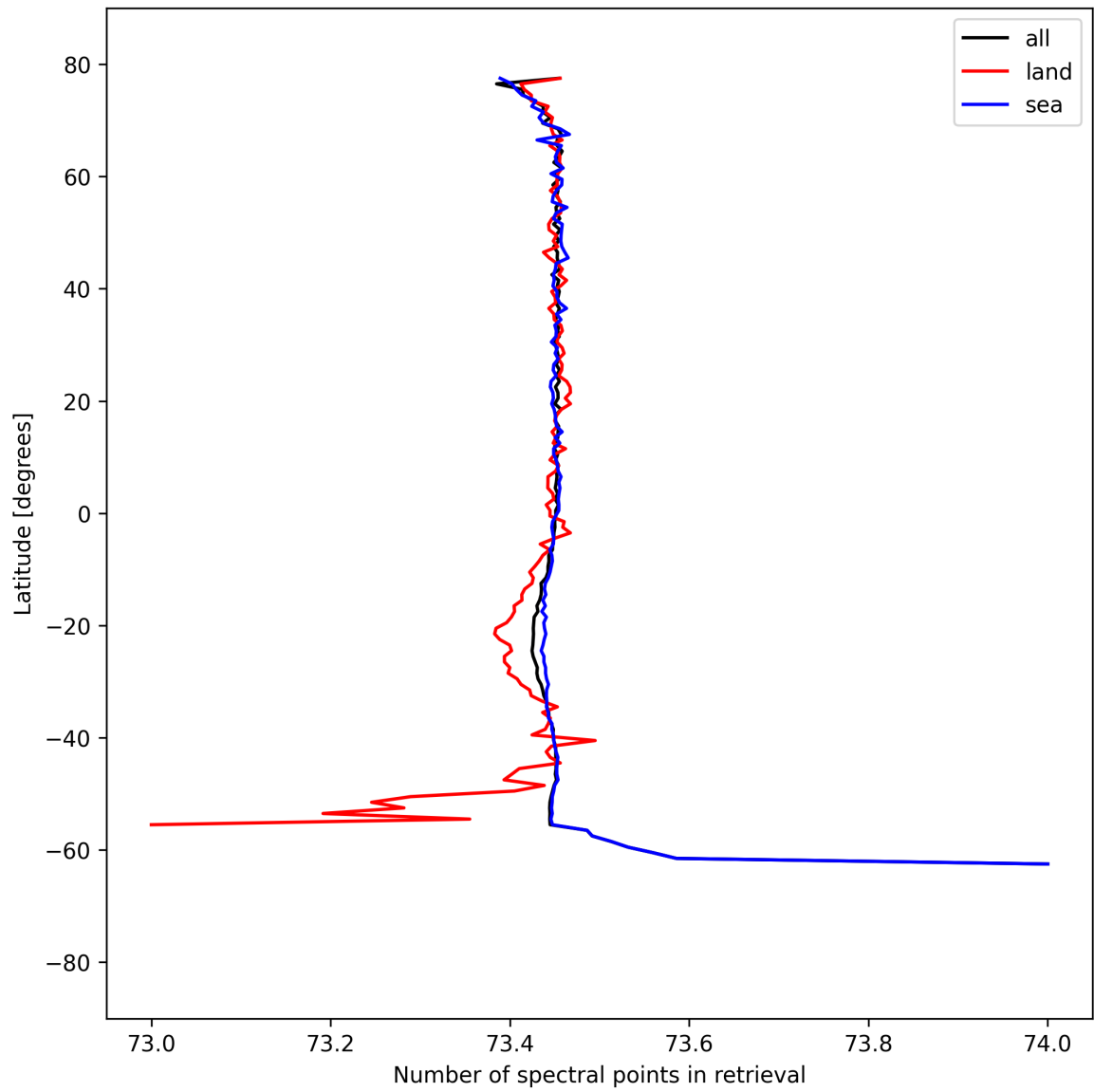
Figure 56: Zonal average of “Number of spectral points in retrieval” for 2025-04-08 to 2025-04-09.
