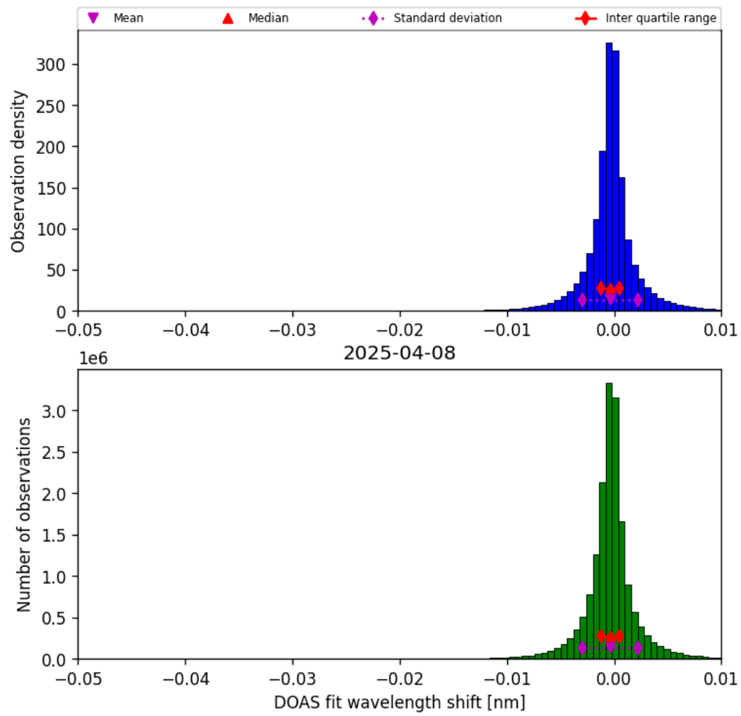
Figure 77: Histogram of “DOAS fit wavelength shift” for 2025-04-08 to 2025-04-09
