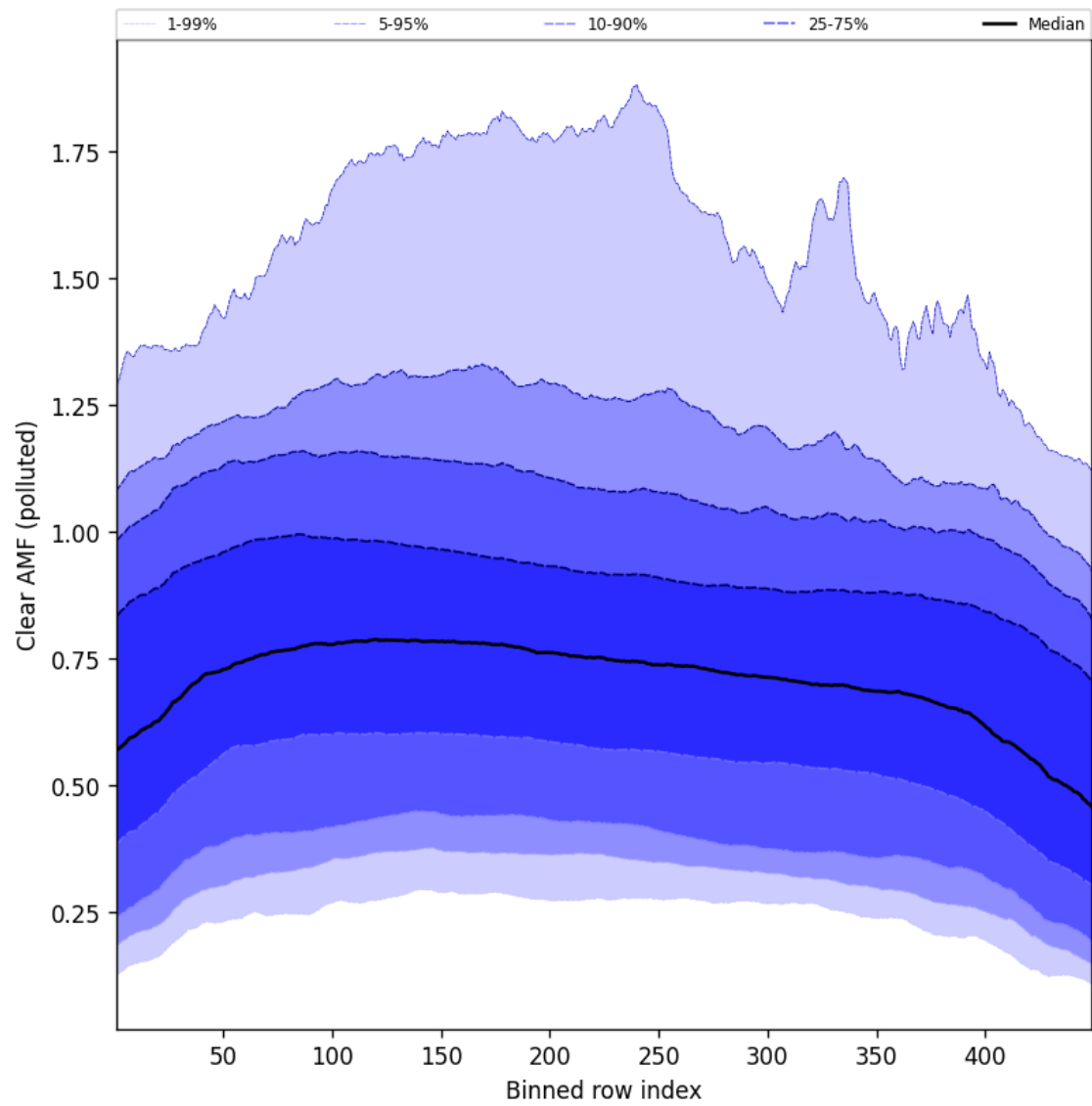
Figure 109: Along track statistics of “Clear AMF (polluted)” for 2025-04-08 to 2025-04-09
