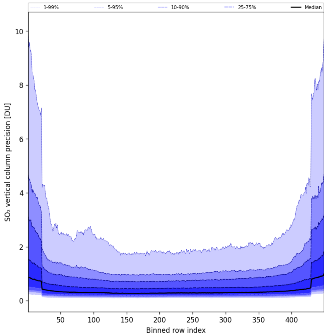
Figure 86: Along track statistics of “SO 2 vertical column precision” for 2025-04-08 to 2025-04-09
