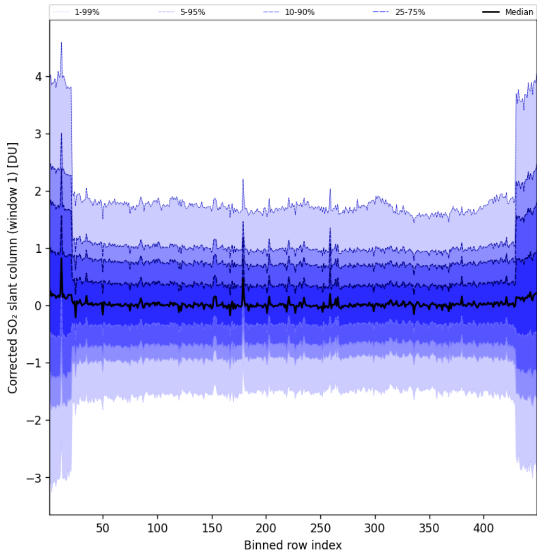
Figure 92: Along track statistics of “Corrected SO 2 slant column (window 1)” for 2025-04-08 to 2025-04-09
