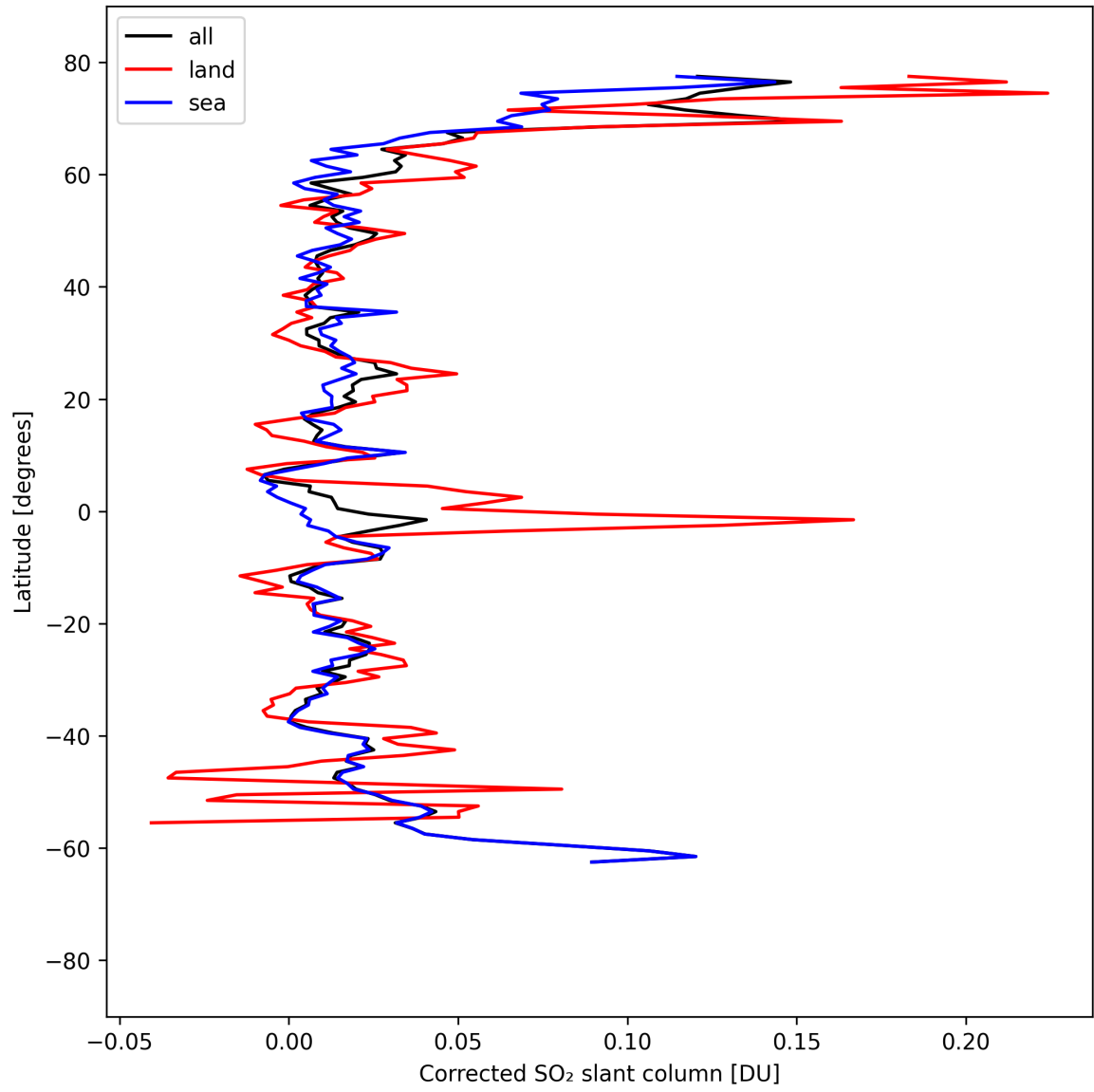
Figure 33: Zonal average of “Corrected SO 2 slant column” for 2025-04-08 to 2025-04-09.
