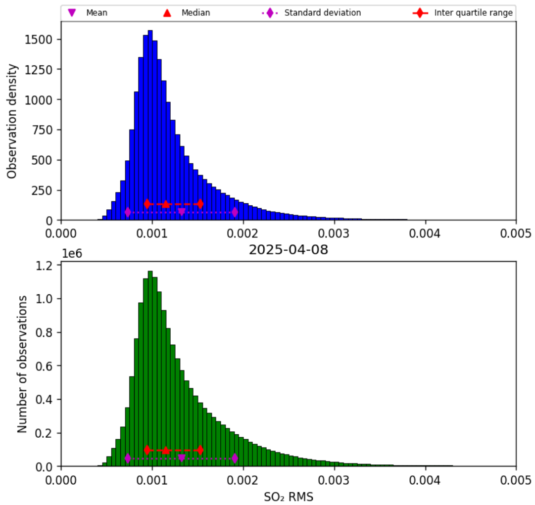
Figure 79: Histogram of “SO 2 RMS” for 2025-04-08 to 2025-04-09
