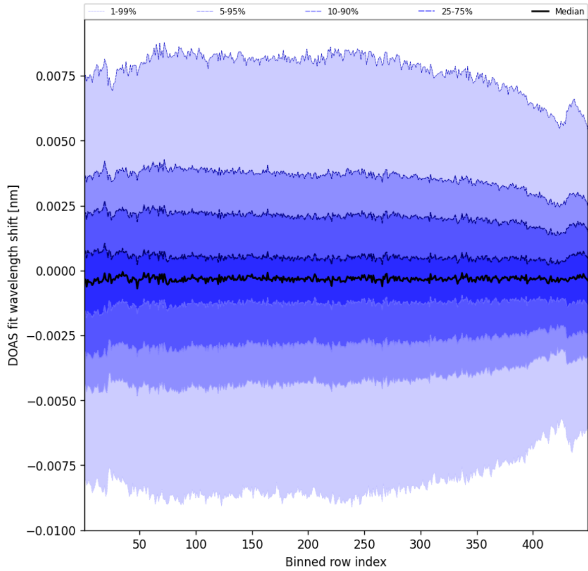
Figure 104: Along track statistics of “DOAS fit wavelength shift” for 2025-04-08 to 2025-04-09
