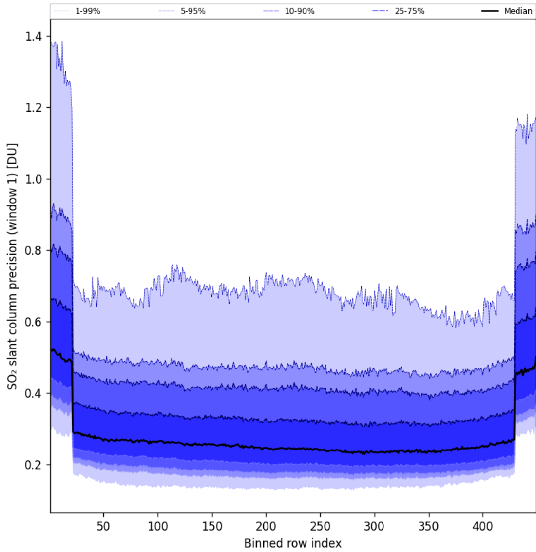
Figure 91: Along track statistics of “SO 2 slant column precision (window 1)” for 2025-04-08 to 2025-04-09
