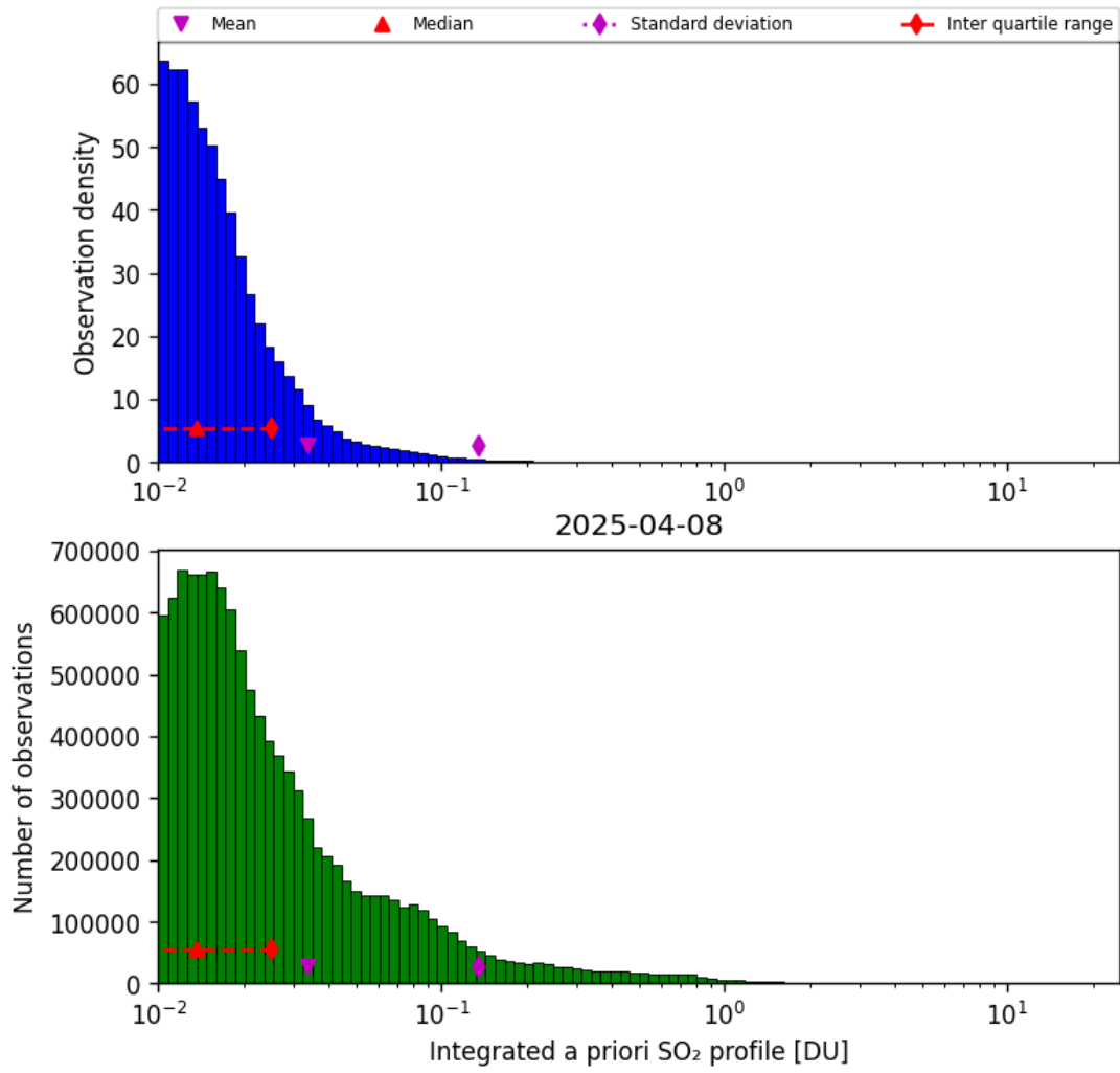
Figure 76: Histogram of “Integrated a priori SO 2 profile” for 2025-04-08 to 2025-04-09
