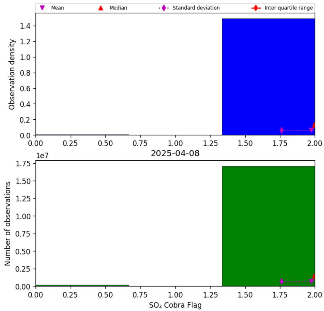
Figure 75: Histogram of "SO 2 Cobra Flag" for 2025-04-08 to 2025-04-09
