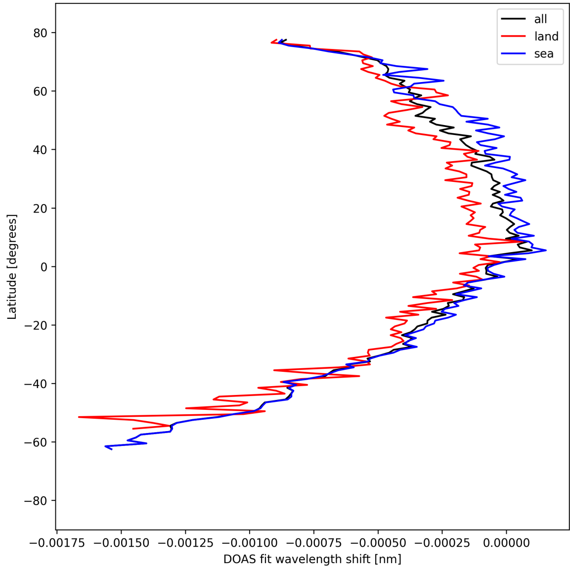
Figure 50: Zonal average of “DOAS fit wavelength shift” for 2025-04-08 to 2025-04-09.
