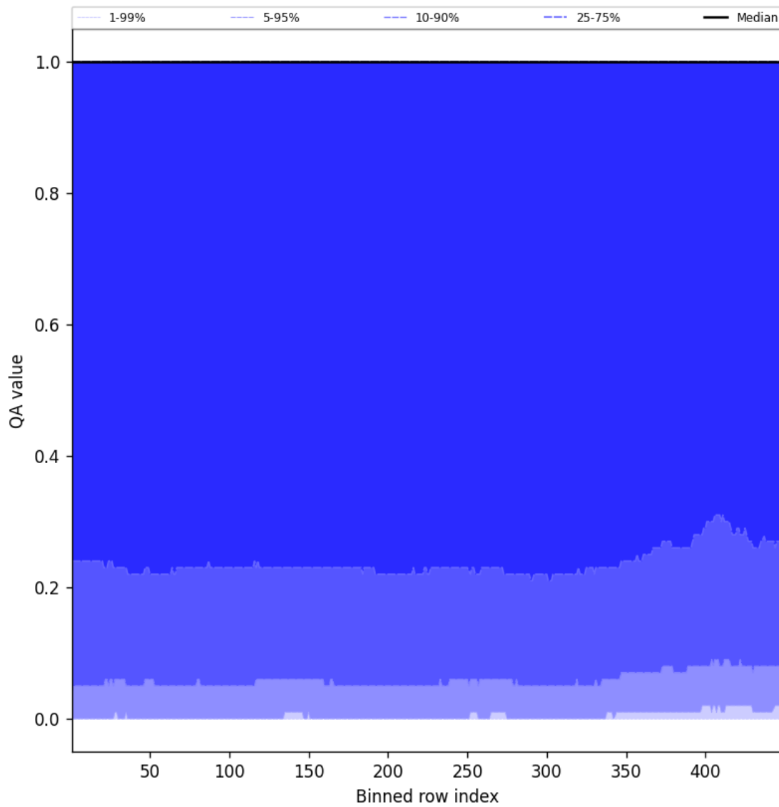
Figure 84: Along track statistics of “QA value” for 2025-04-08 to 2025-04-09
