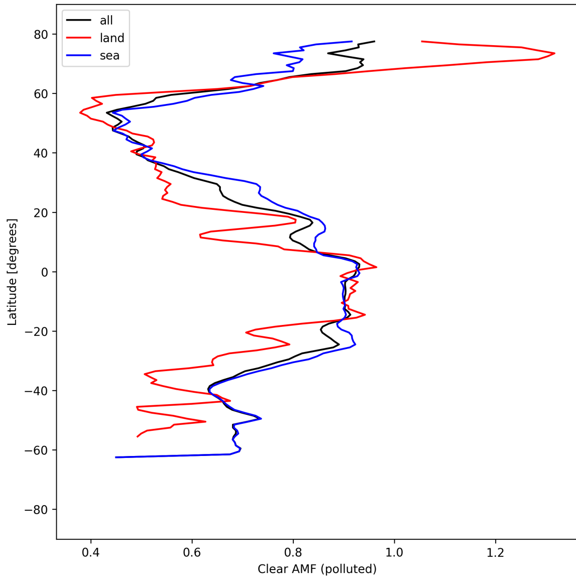
Figure 55: Zonal average of “Clear AMF (polluted)” for 2025-04-08 to 2025-04-09.
