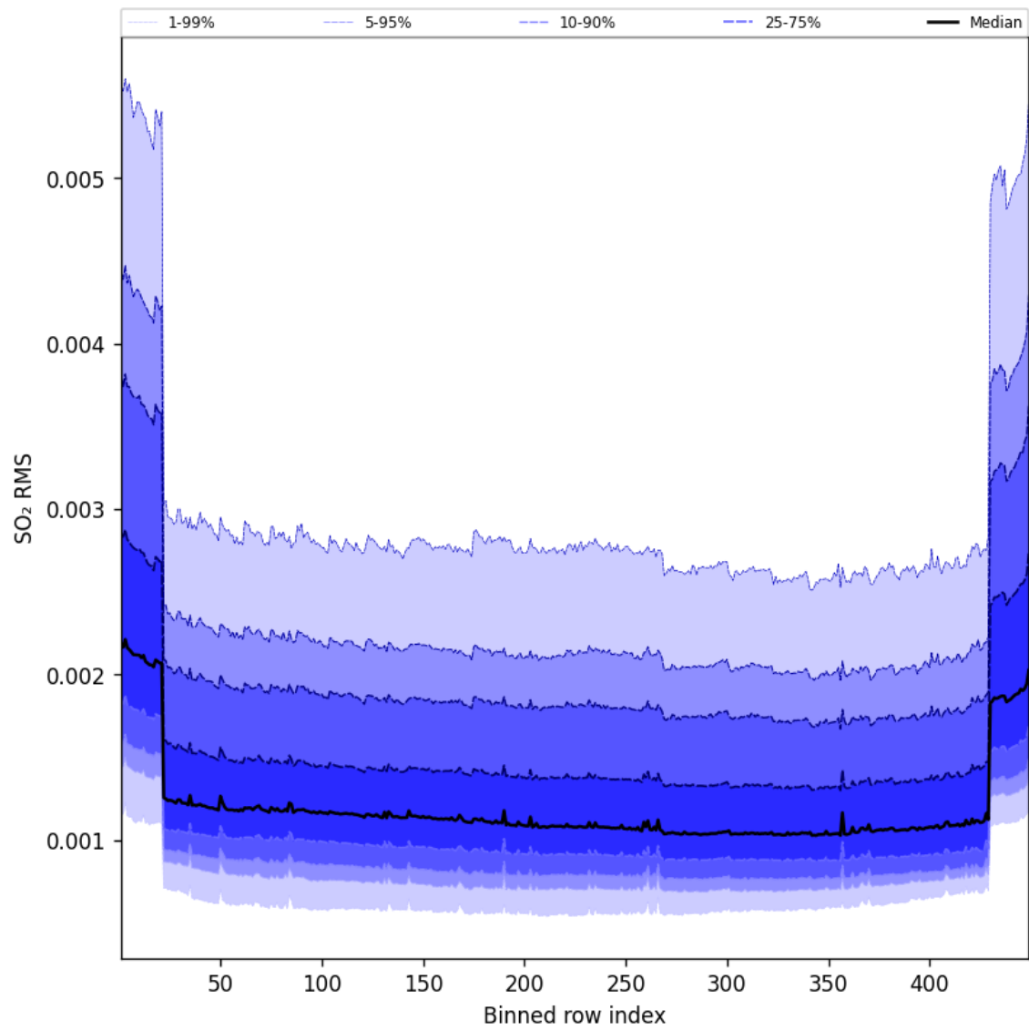
Figure 106: Along track statistics of “SO 2 RMS” for 2025-04-08 to 2025-04-09
