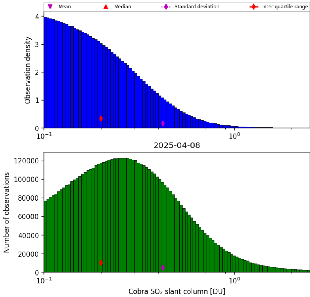
Figure 61: Histogram of “Cobra SO 2 slant column” for 2025-04-08 to 2025-04-09
