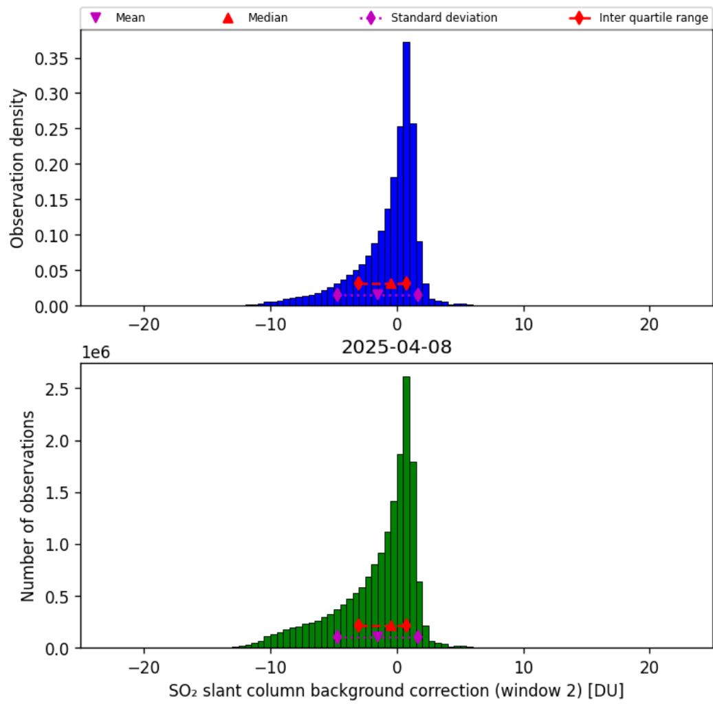
Figure 70: Histogram of “SO 2 slant column background correction (window 2)” for 2025-04-08 to 2025-04-09
