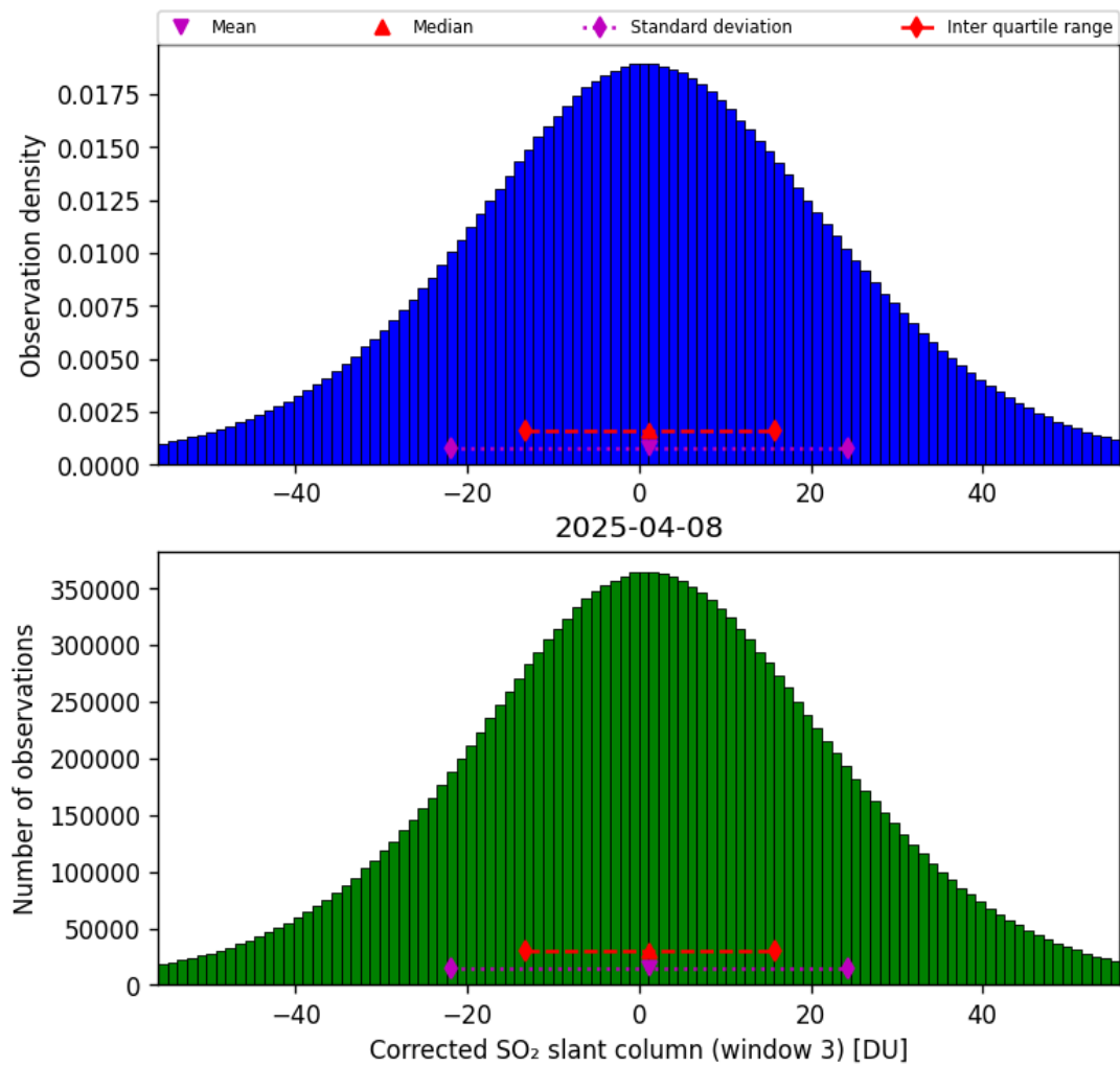
Figure 73: Histogram of “Corrected SO 2 slant column (window 3)” for 2025-04-08 to 2025-04-09
