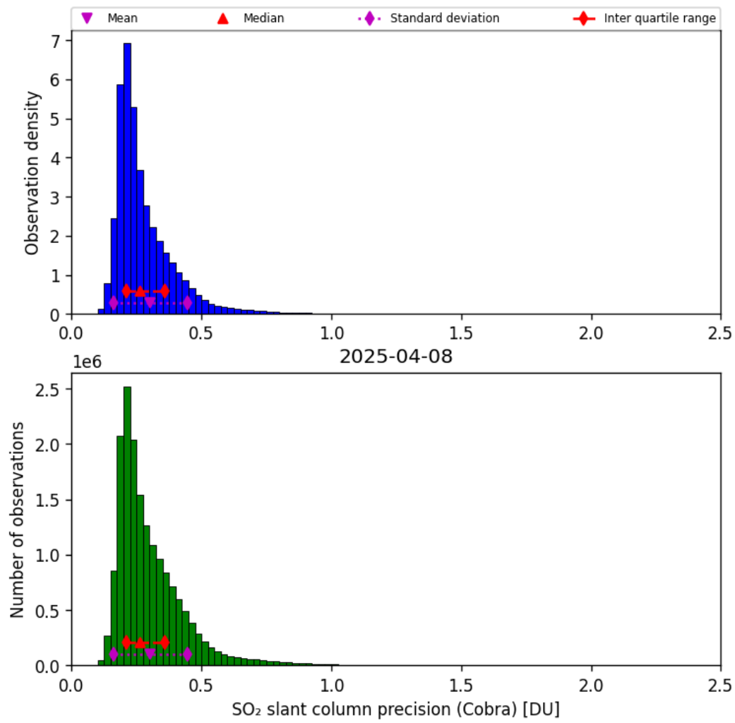
Figure 62: Histogram of “SO 2 slant column precision (Cobra)” for 2025-04-08 to 2025-04-09
