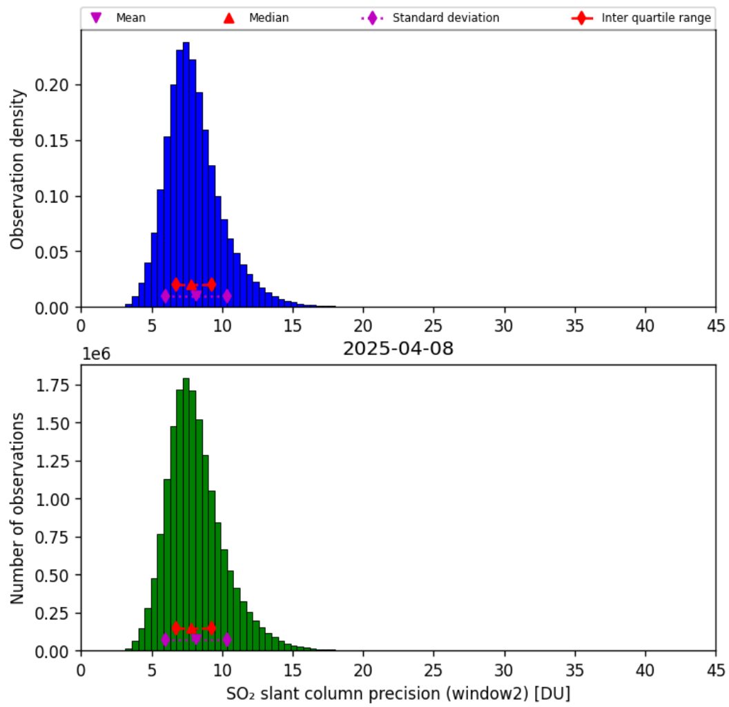
Figure 68: Histogram of “SO 2 slant column precision (window2)” for 2025-04-08 to 2025-04-09
