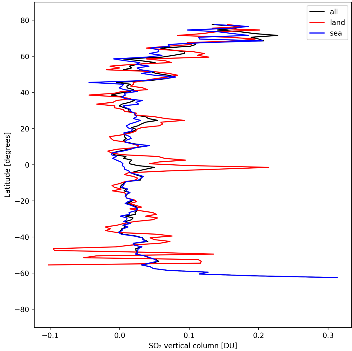
Figure 31: Zonal average of “SO 2 vertical column” for 2025-04-08 to 2025-04-09.
