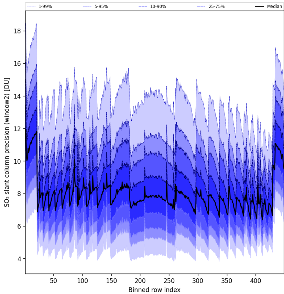
Figure 95: Along track statistics of “SO 2 slant column precision (window2)” for 2025-04-08 to 2025-04-09
