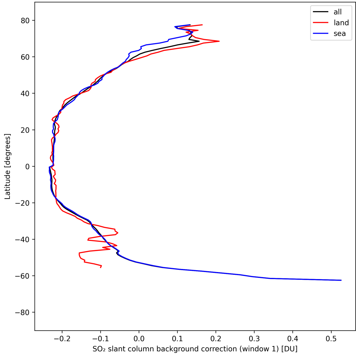
Figure 39: Zonal average of “SO 2 slant column background correction (window 1)” for 2025-04-08 to 2025-04-09.
