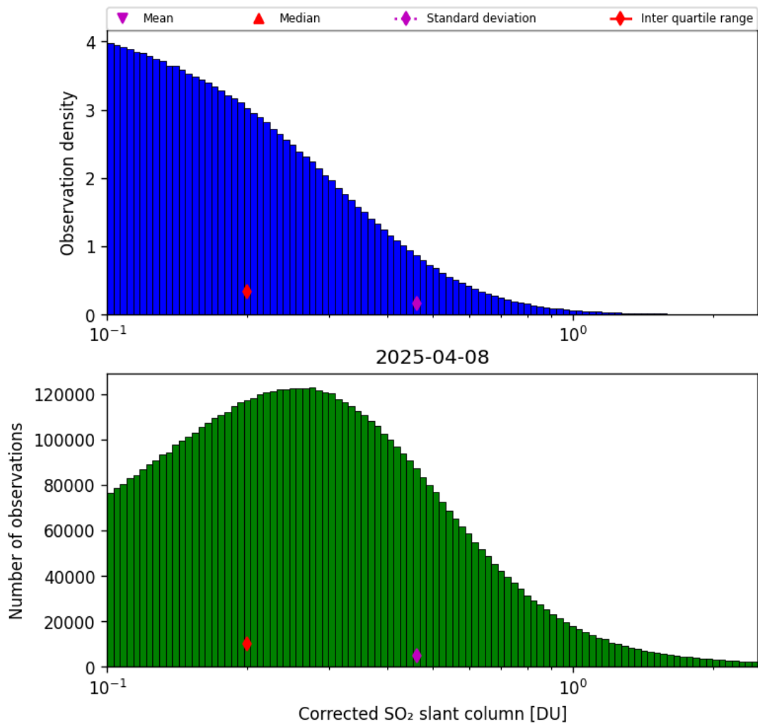
Figure 60: Histogram of “Corrected SO 2 slant column” for 2025-04-08 to 2025-04-09
