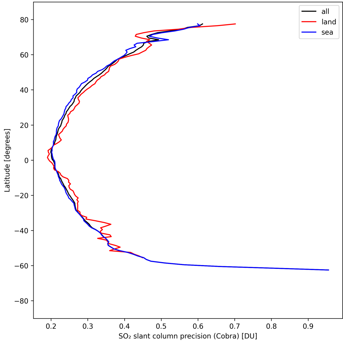
Figure 35: Zonal average of “SO 2 slant column precision (Cobra)” for 2025-04-08 to 2025-04-09.
