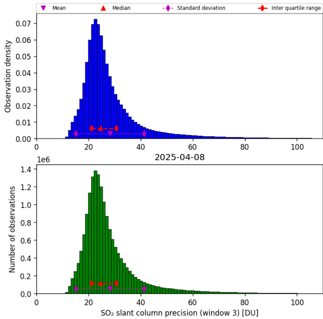
Figure 72: Histogram of “SO 2 slant column precision (window 3)” for 2025-04-08 to 2025-04-09
