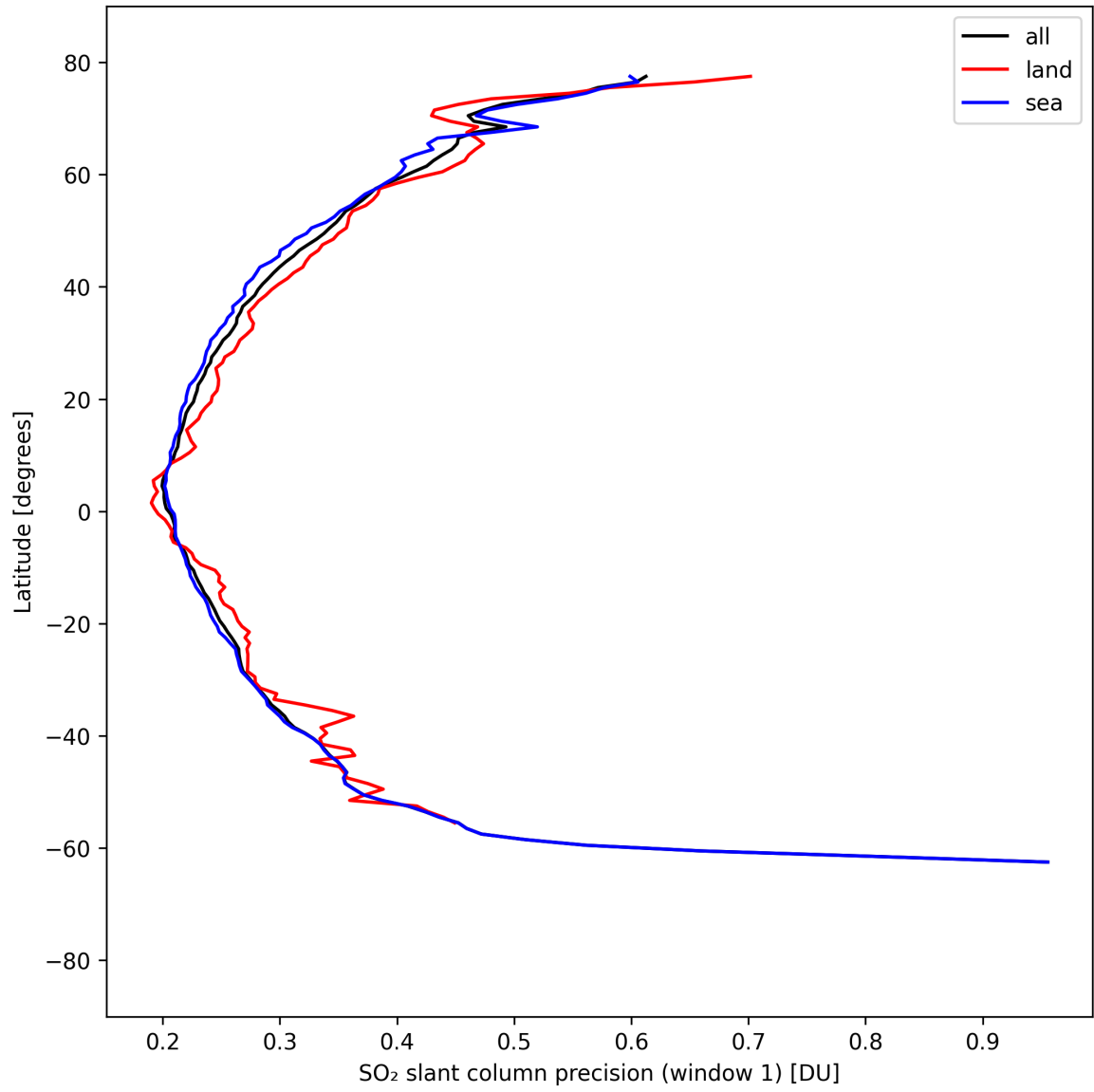
Figure 37: Zonal average of “SO 2 slant column precision (window 1)” for 2025-04-08 to 2025-04-09.
