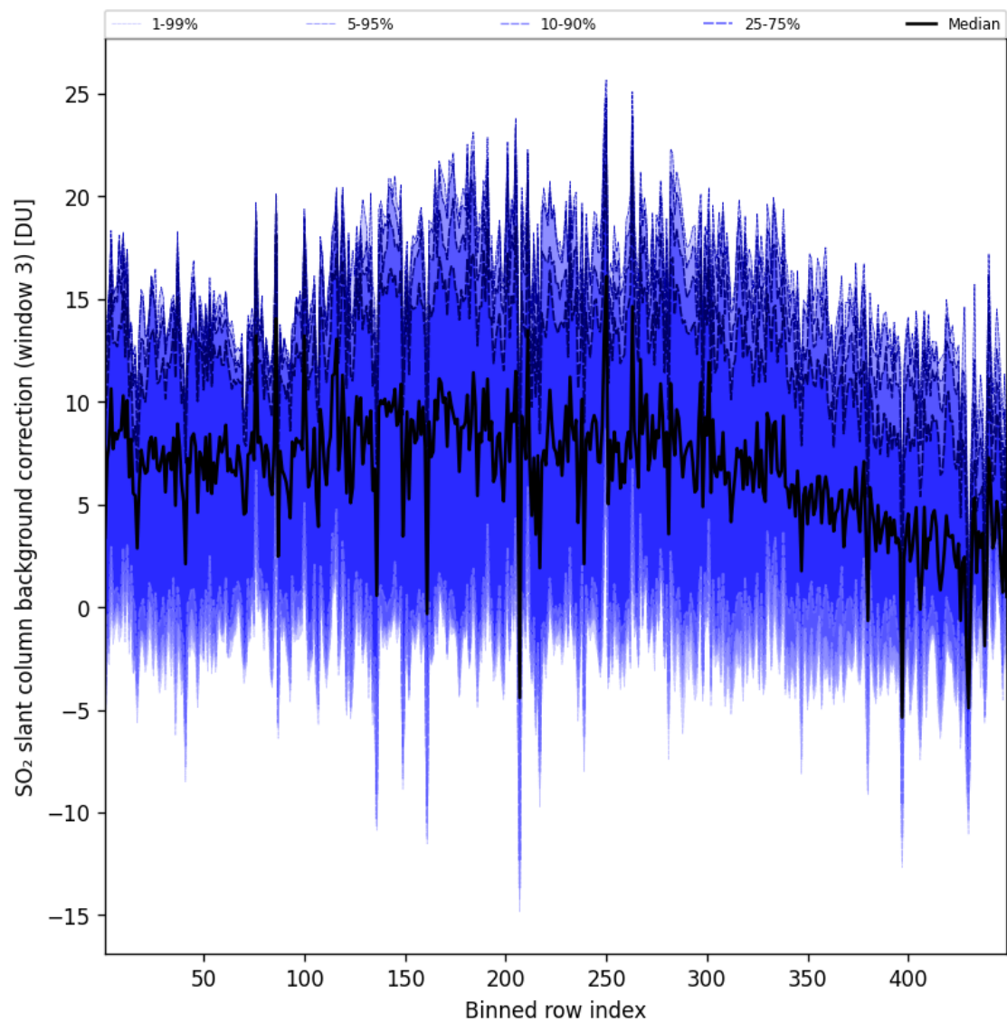
Figure 101: Along track statistics of “SO 2 slant column background correction (window 3)” for 2025-04-10 to 2025-04-11
