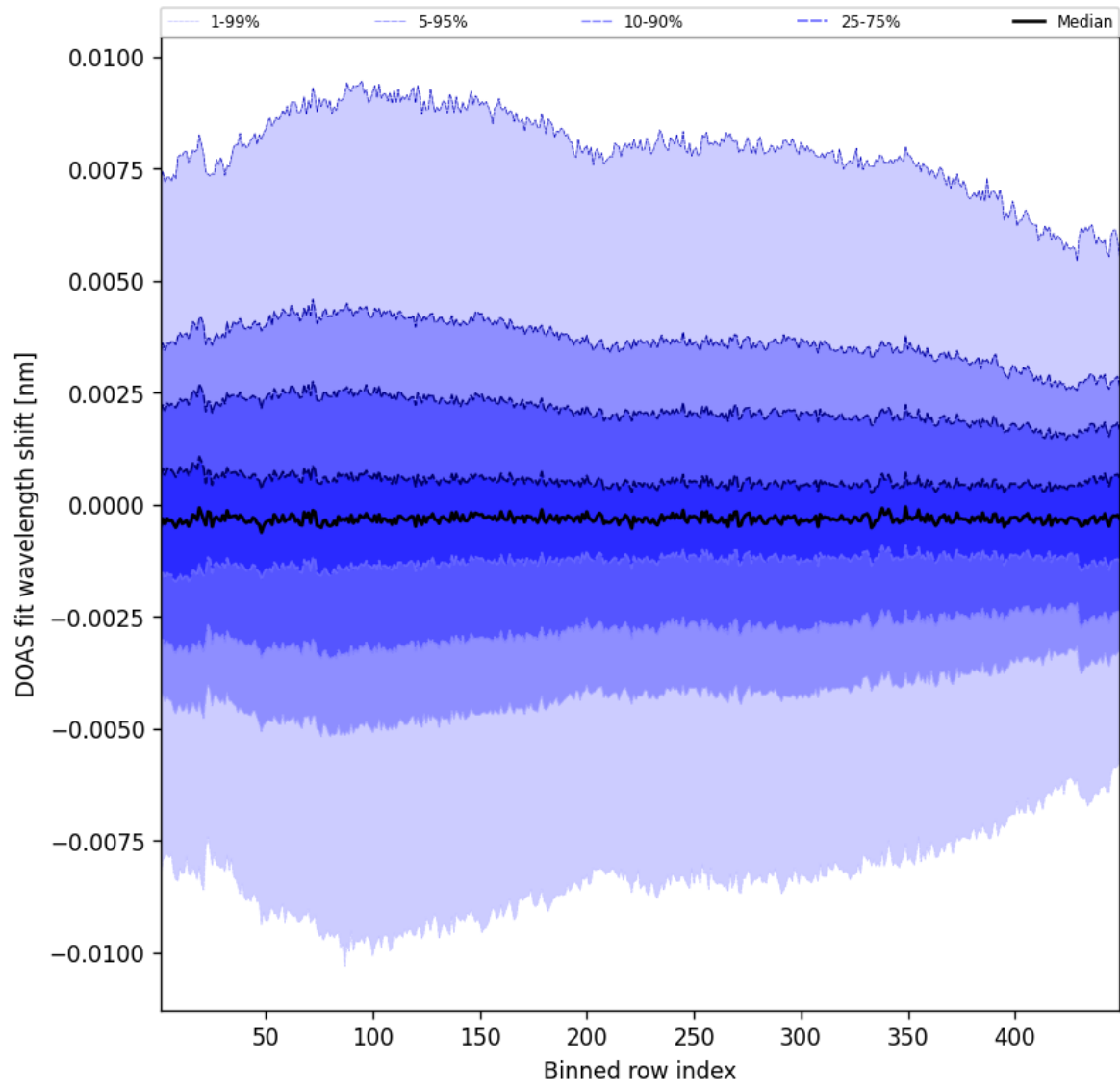
Figure 104: Along track statistics of “DOAS fit wavelength shift” for 2025-04-10 to 2025-04-11
