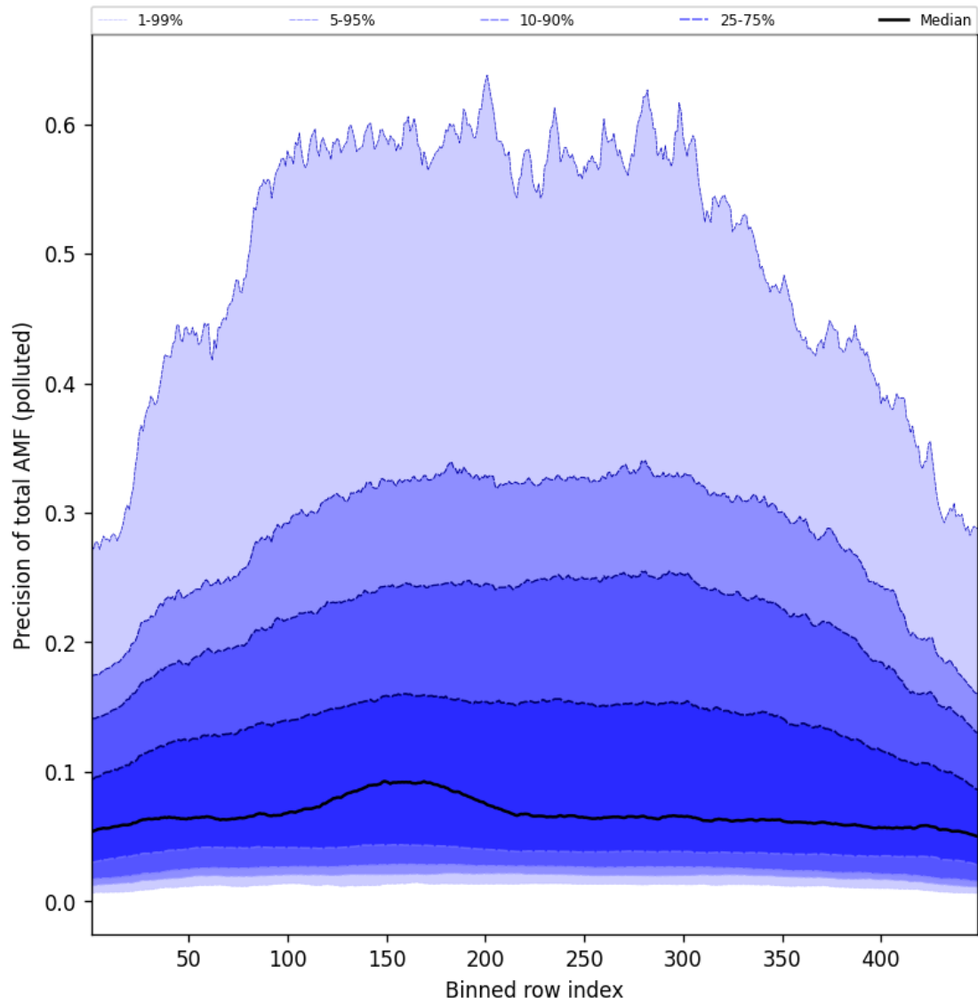
Figure 108: Along track statistics of “Precision of total AMF (polluted)” for 2025-04-10 to 2025-04-11
