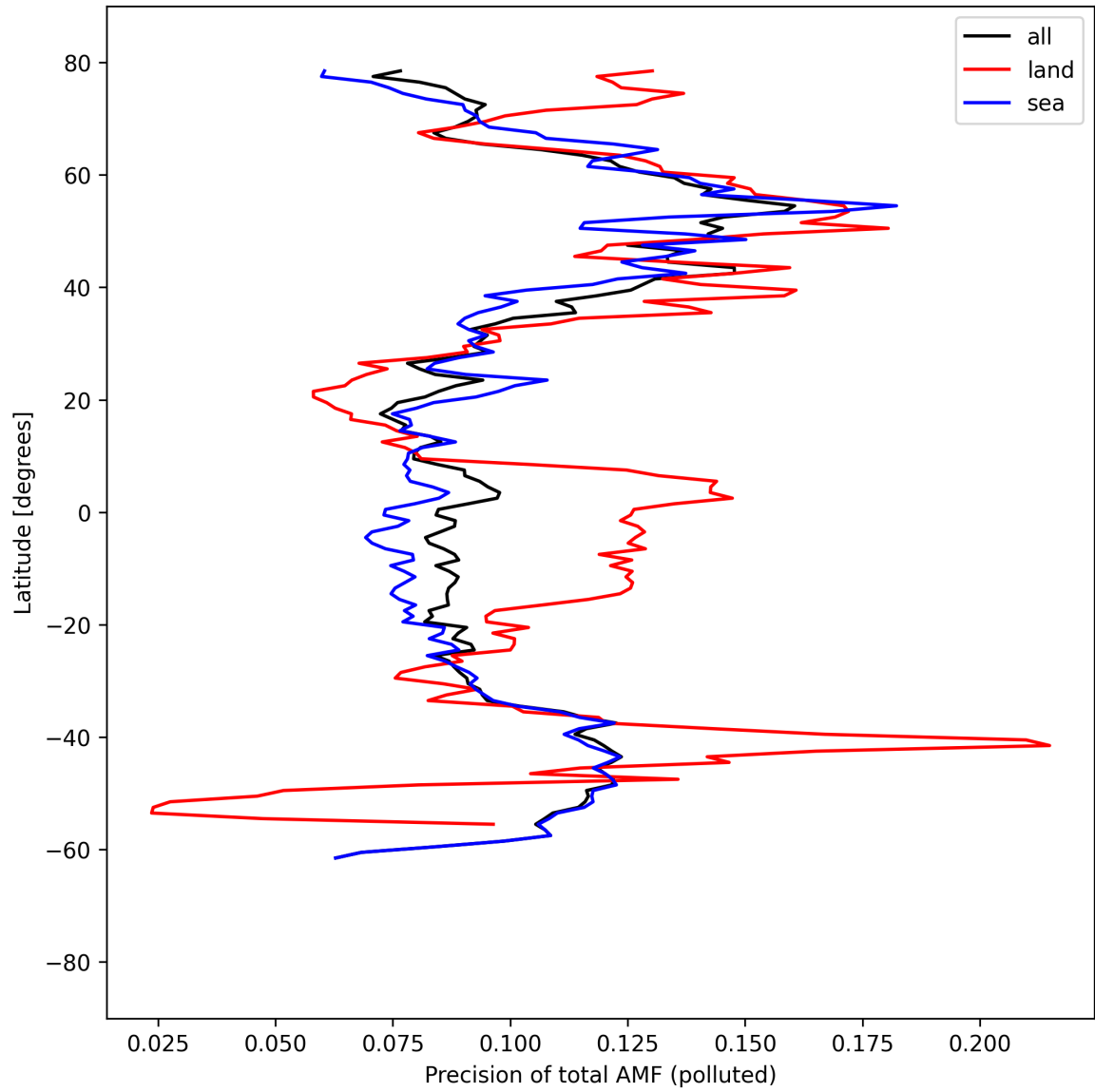
Figure 54: Zonal average of “Precision of total AMF (polluted)” for 2025-04-10 to 2025-04-11.
