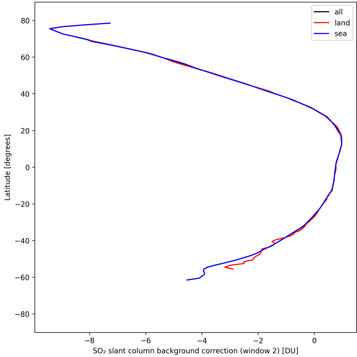
Figure 43: Zonal average of “SO 2 slant column background correction (window 2)” for 2025-04-10 to 2025-04-11.
