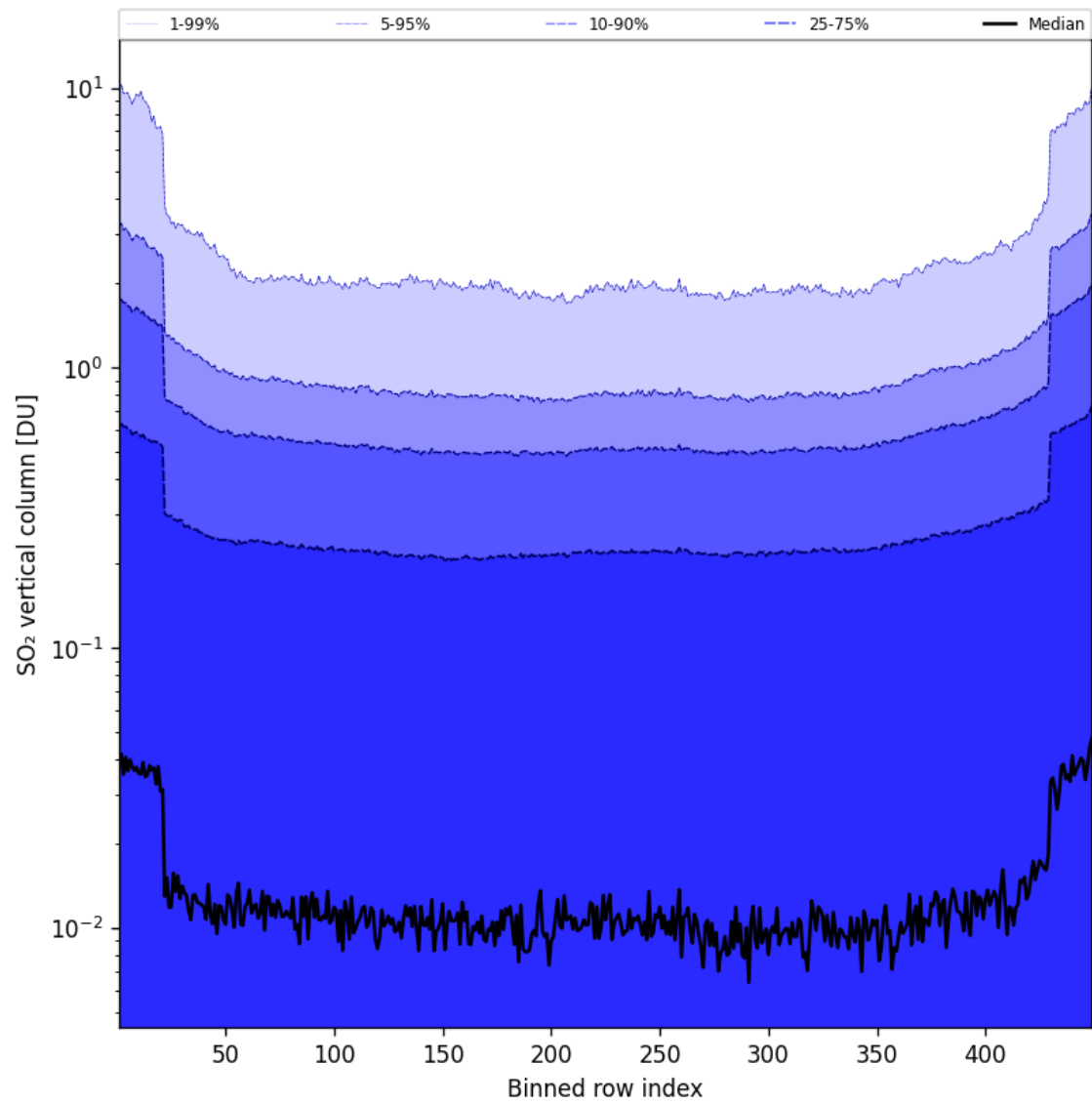
Figure 85: Along track statistics of “SO 2 vertical column” for 2025-04-10 to 2025-04-11
