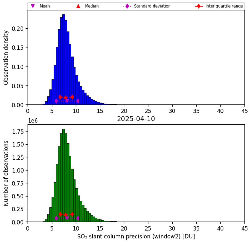
Figure 68: Histogram of “SO 2 slant column precision (window2)” for 2025-04-10 to 2025-04-11
