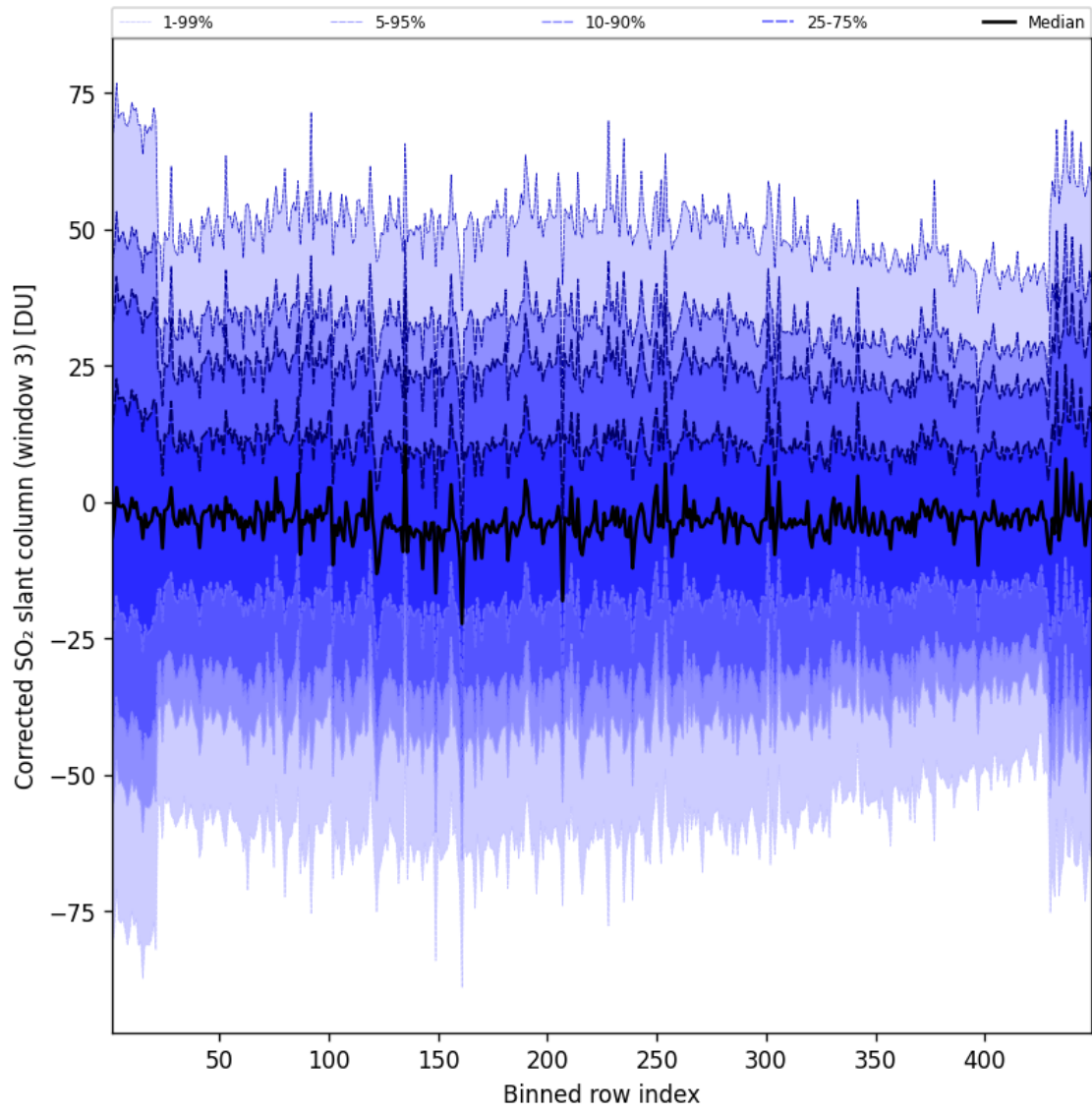
Figure 100: Along track statistics of “Corrected SO 2 slant column (window 3)” for 2025-04-10 to 2025-04-11
