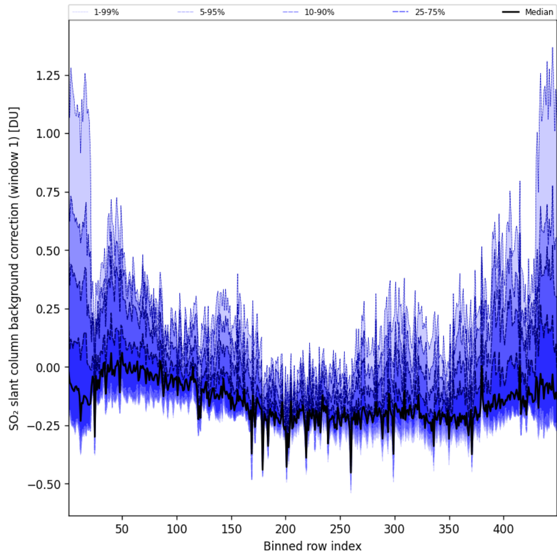
Figure 93: Along track statistics of “SO 2 slant column background correction (window 1)” for 2025-04-10 to 2025-04-11
