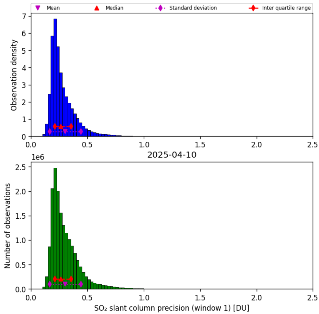
Figure 64: Histogram of “SO 2 slant column precision (window 1)” for 2025-04-10 to 2025-04-11
