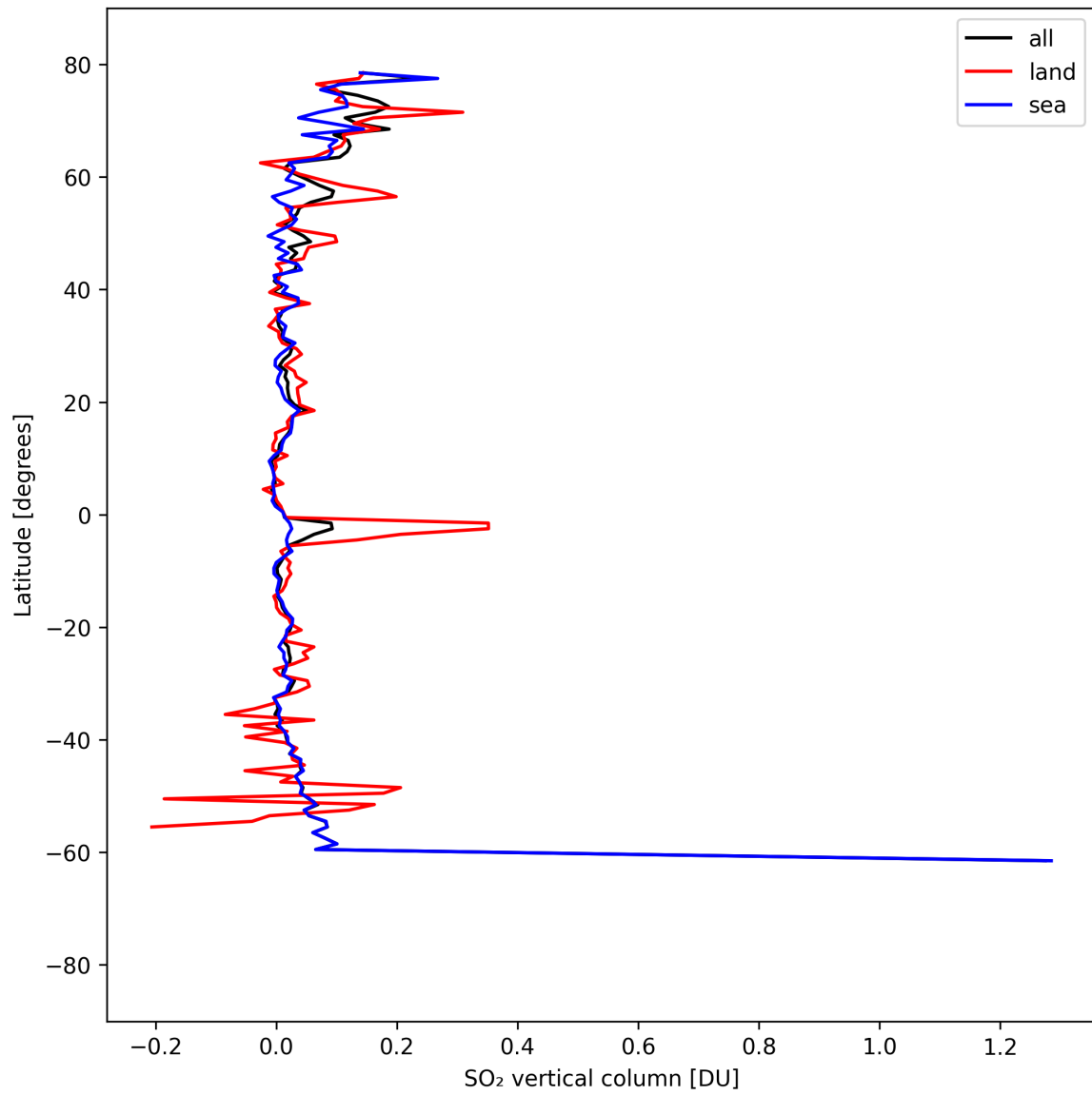
Figure 31: Zonal average of “SO 2 vertical column” for 2025-04-10 to 2025-04-11.
