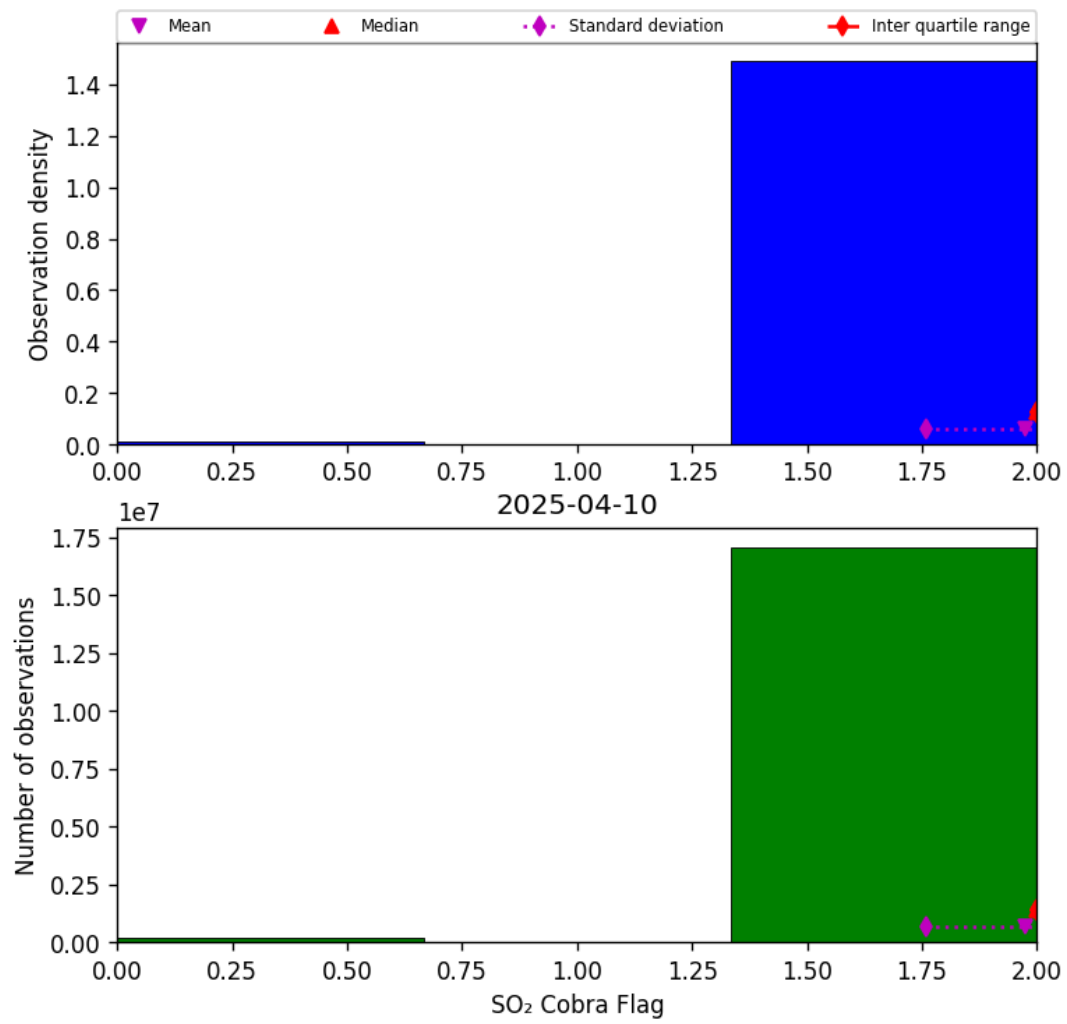
Figure 75: Histogram of “SO 2 Cobra Flag” for 2025-04-10 to 2025-04-11
