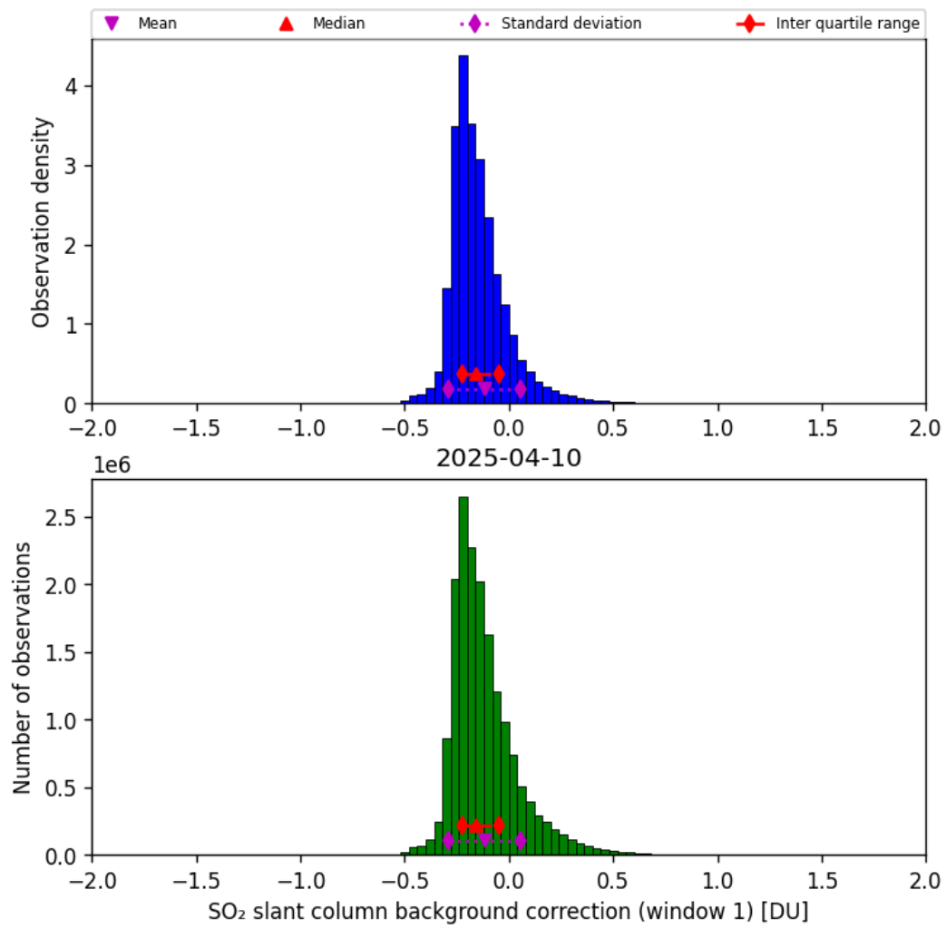
Figure 66: Histogram of “SO 2 slant column background correction (window 1)” for 2025-04-10 to 2025-04-11
