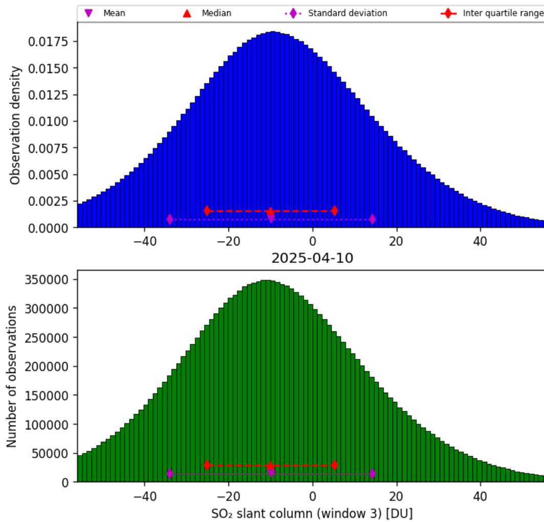
Figure 71: Histogram of “SO 2 slant column (window 3)” for 2025-04-10 to 2025-04-11
