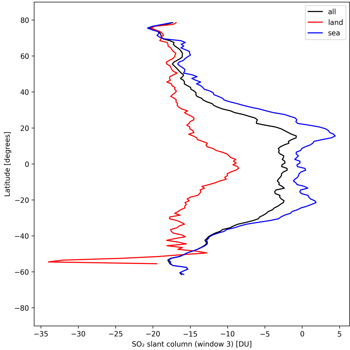
Figure 44: Zonal average of “SO 2 slant column (window 3)” for 2025-04-10 to 2025-04-11.
