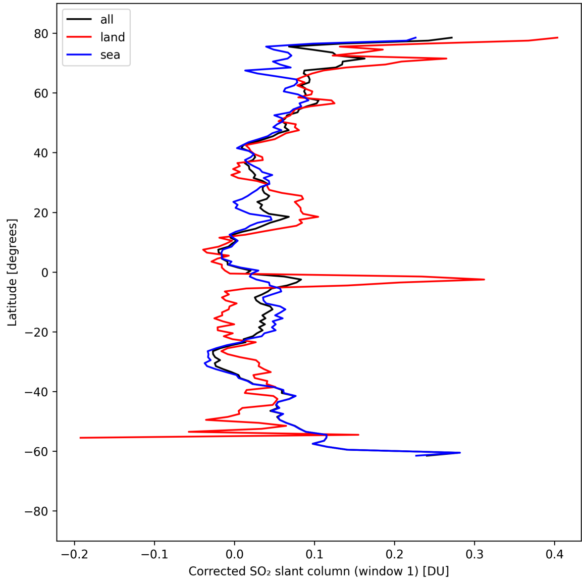
Figure 38: Zonal average of “Corrected SO 2 slant column (window 1)” for 2025-04-10 to 2025-04-11.
