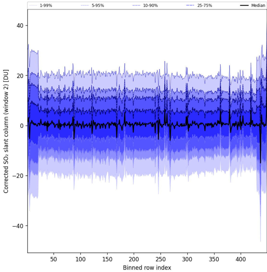
Figure 96: Along track statistics of “Corrected SO 2 slant column (window 2)” for 2025-04-10 to 2025-04-11
