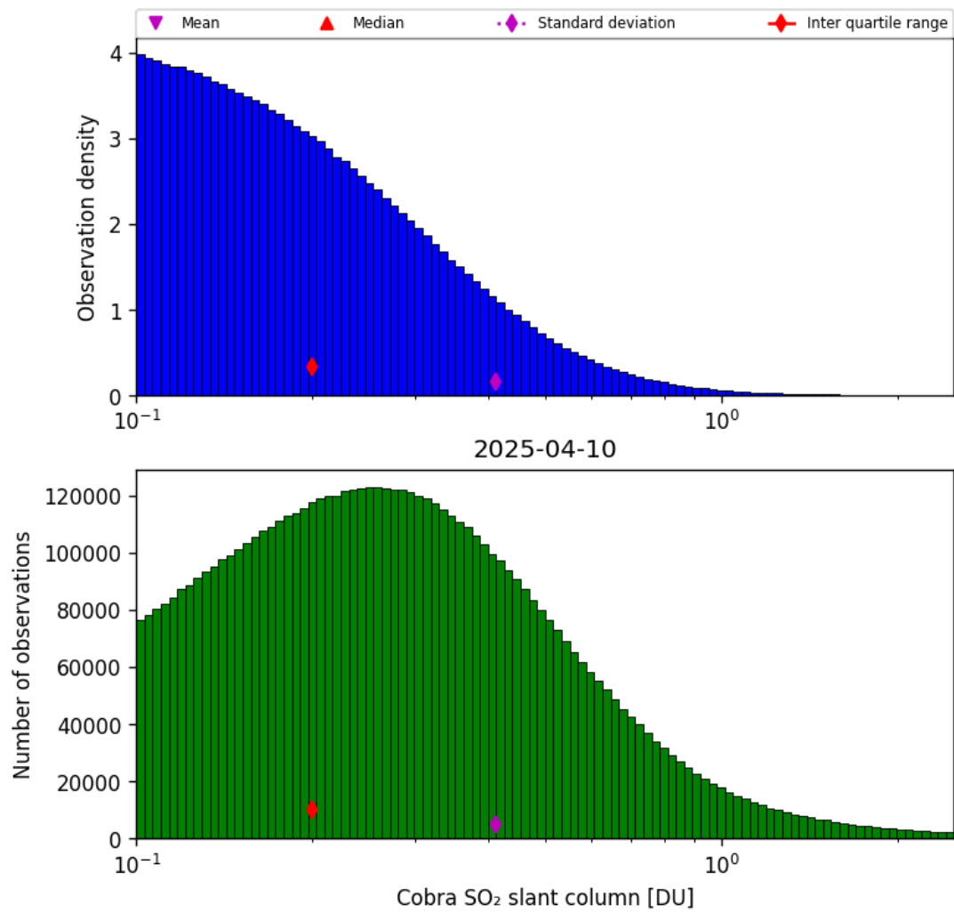
Figure 61: Histogram of “Cobra SO 2 slant column” for 2025-04-10 to 2025-04-11
