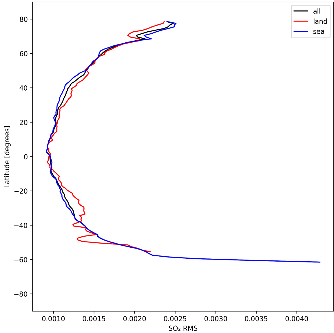
Figure 52: Zonal average of “SO 2 RMS” for 2025-04-10 to 2025-04-11.
