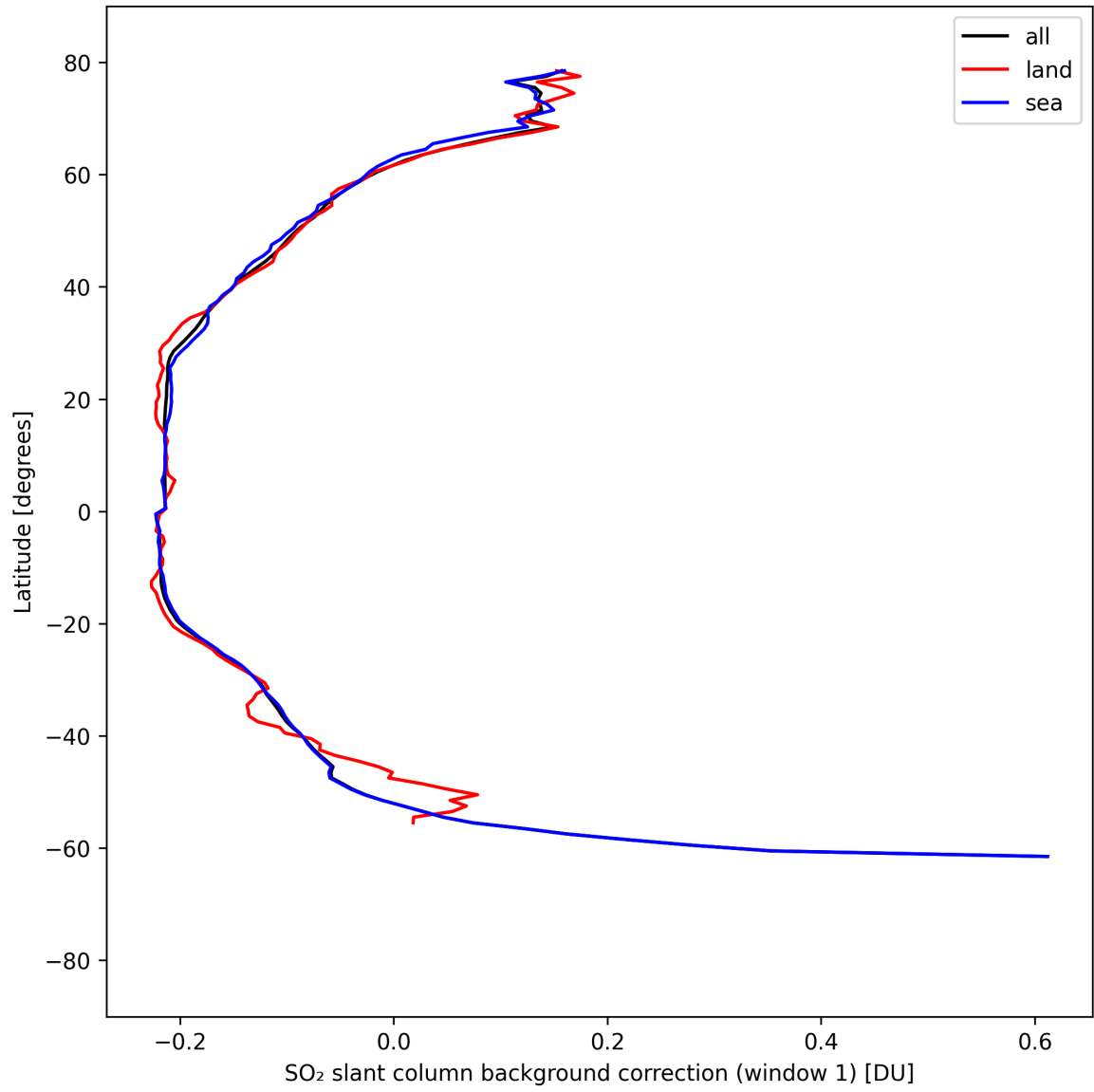
Figure 39: Zonal average of "SO 2 slant column background correction (window 1)" for 2025-04-10 to 2025-04-11.
