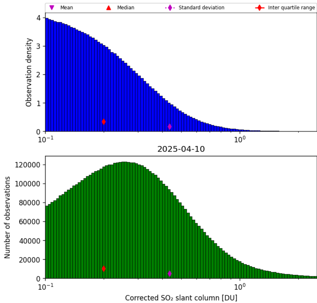
Figure 60: Histogram of “Corrected SO 2 slant column” for 2025-04-10 to 2025-04-11
