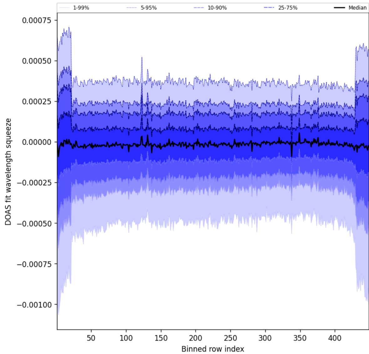
Figure 105: Along track statistics of “DOAS fit wavelength squeeze” for 2025-04-10 to 2025-04-11
