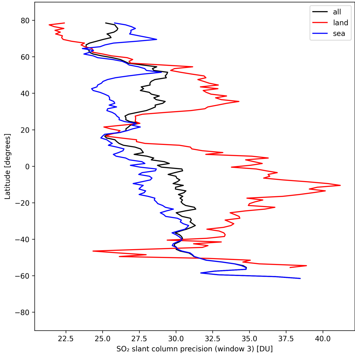
Figure 45: Zonal average of “SO 2 slant column precision (window 3)” for 2025-04-10 to 2025-04-11.
