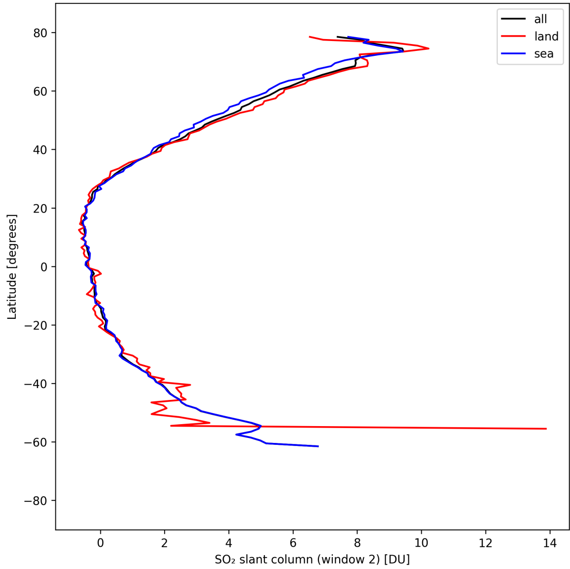
Figure 40: Zonal average of “SO 2 slant column (window 2)” for 2025-04-10 to 2025-04-11.
