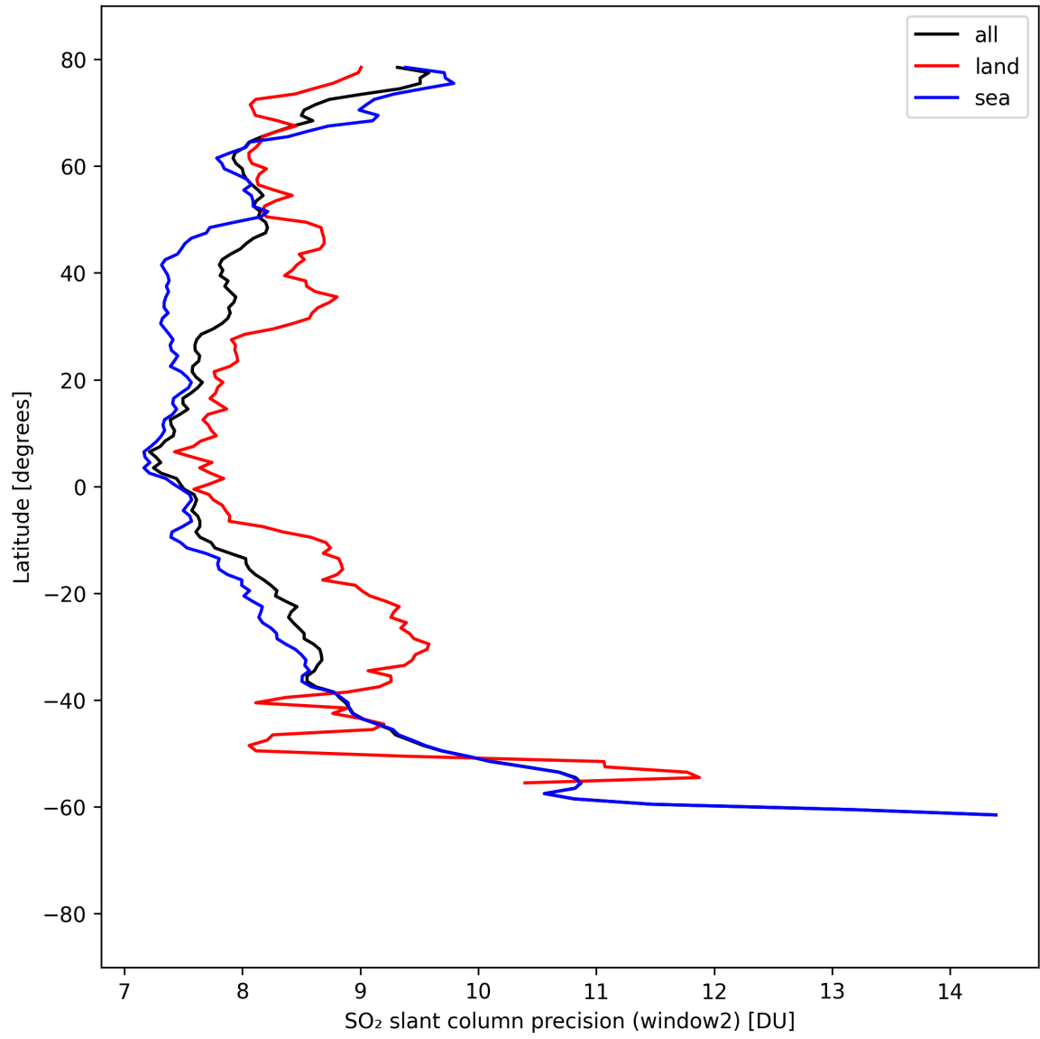
Figure 41: Zonal average of “SO 2 slant column precision (window2)” for 2025-04-10 to 2025-04-11.
