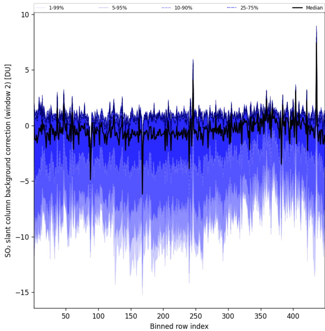
Figure 97: Along track statistics of “SO 2 slant column background correction (window 2)” for 2025-04-10 to 2025-04-11
