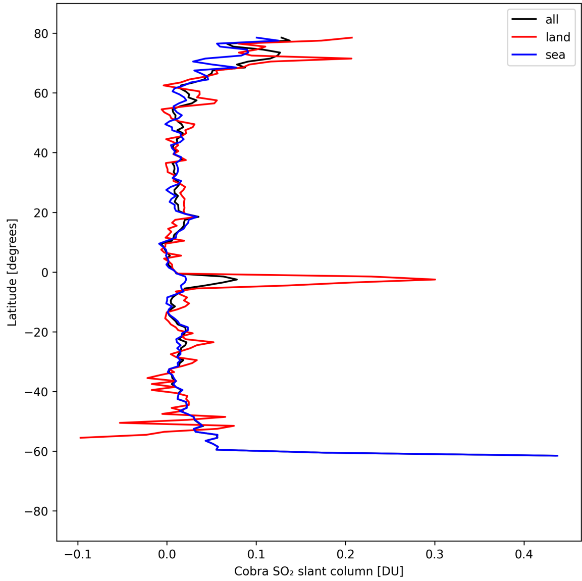
Figure 34: Zonal average of “Cobra SO 2 slant column” for 2025-04-10 to 2025-04-11.
