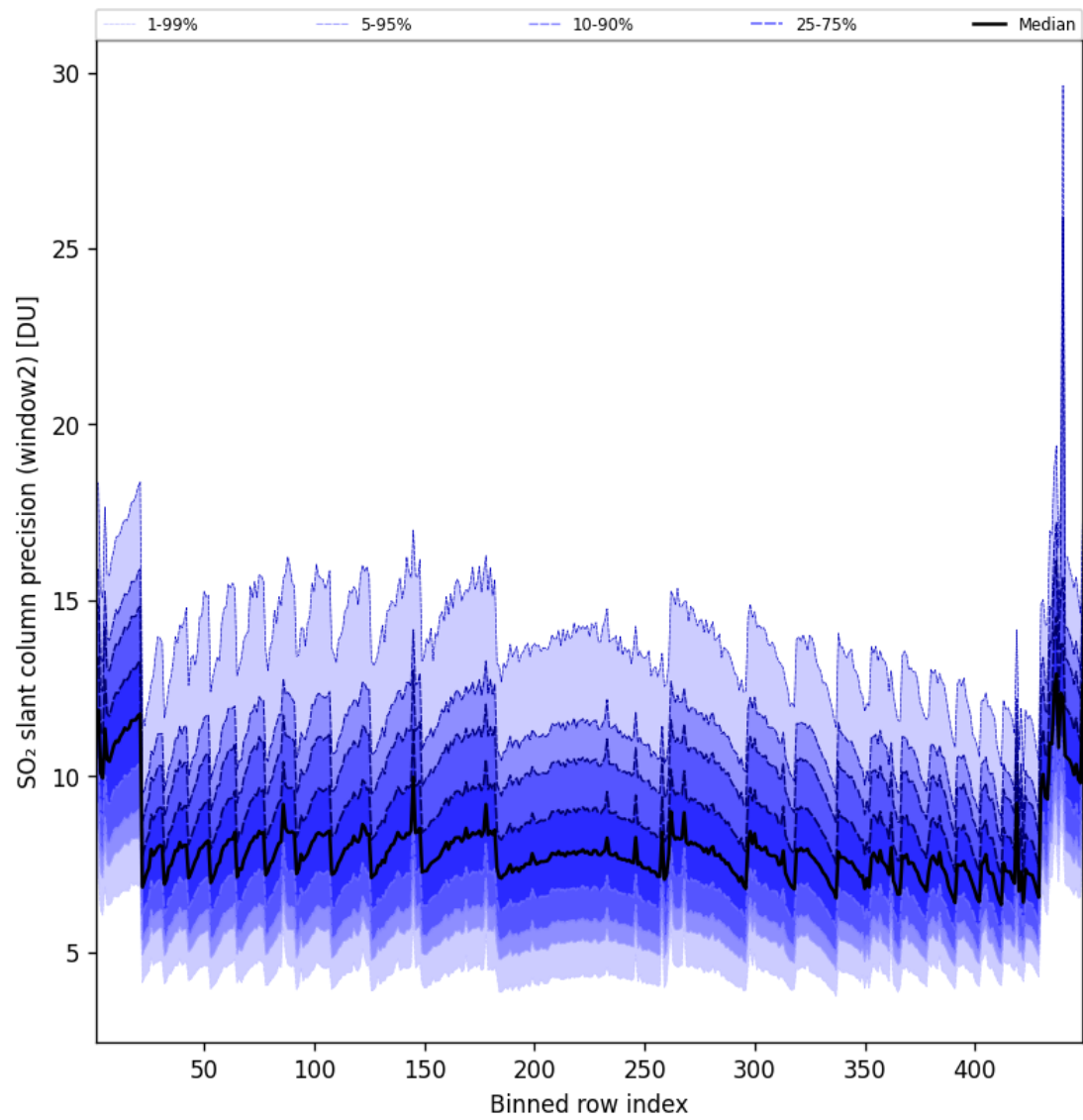
Figure 95: Along track statistics of “SO 2 slant column precision (window2)” for 2025-04-10 to 2025-04-11
