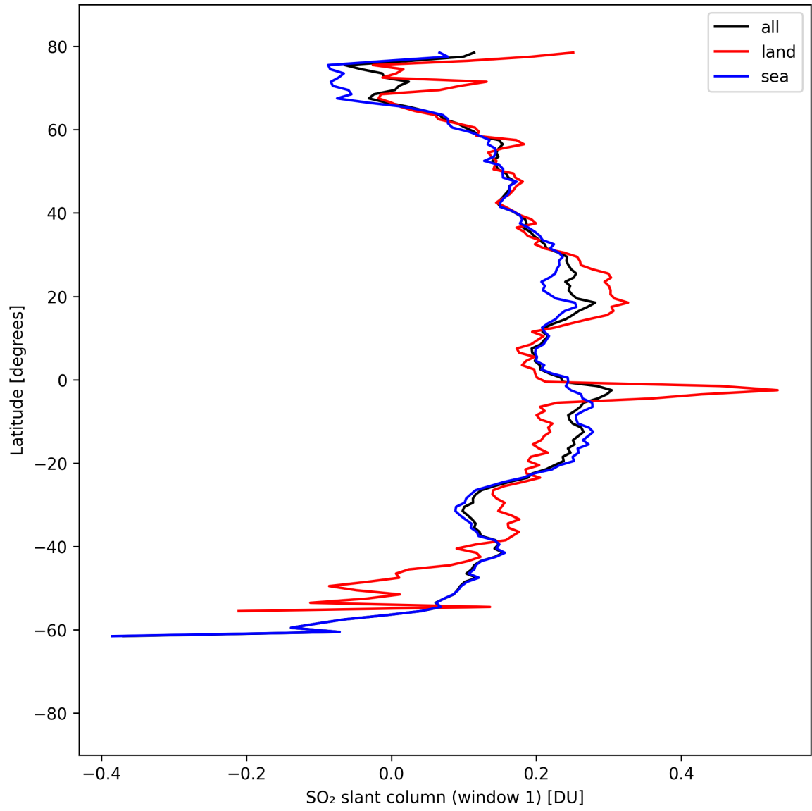
Figure 36: Zonal average of “SO 2 slant column (window 1)” for 2025-04-10 to 2025-04-11.
