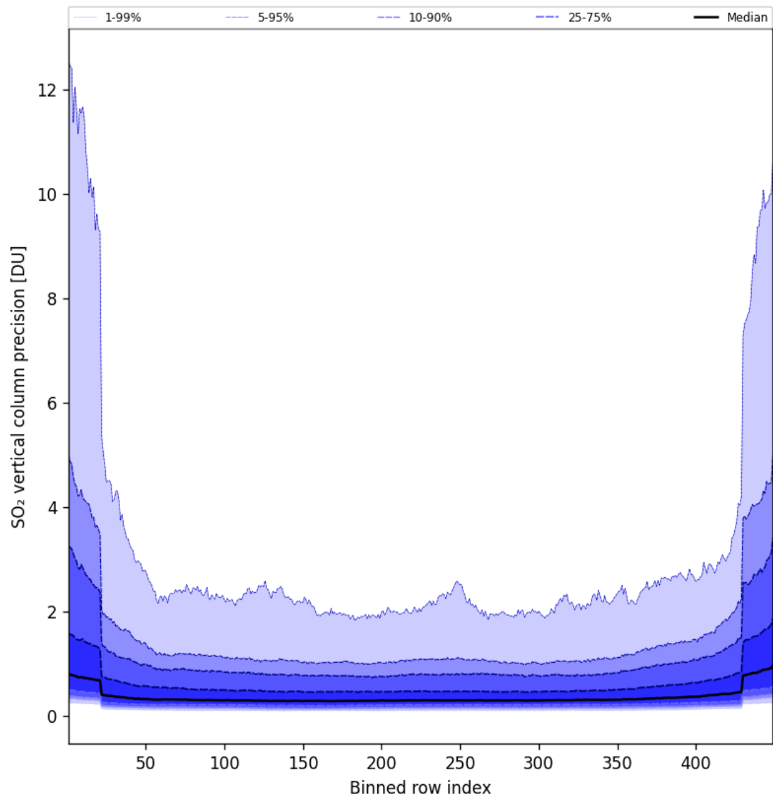
Figure 86: Along track statistics of “SO 2 vertical column precision” for 2025-04-10 to 2025-04-11
