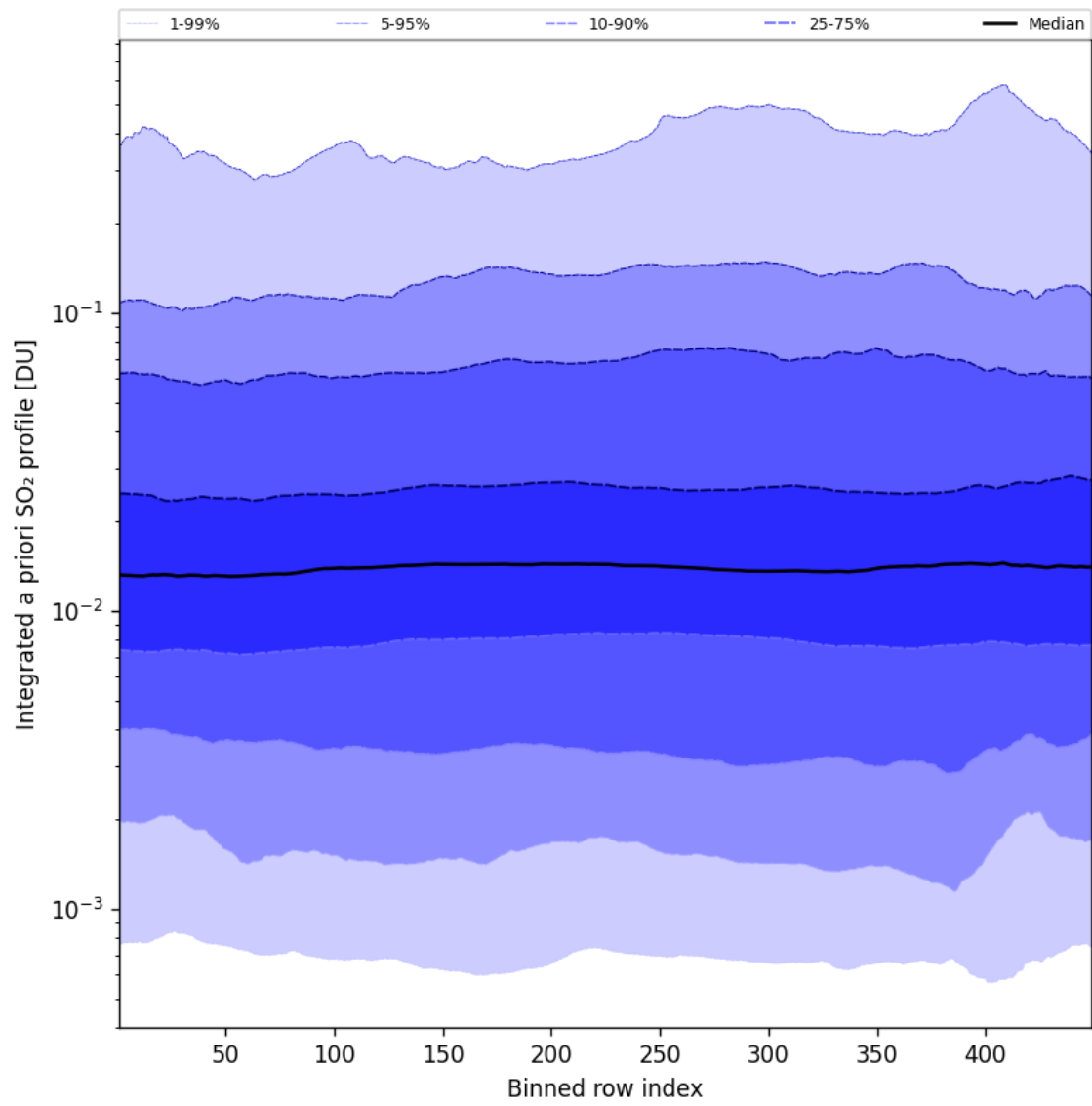
Figure 103: Along track statistics of “Integrated a priori SO 2 profile” for 2025-04-10 to 2025-04-11
