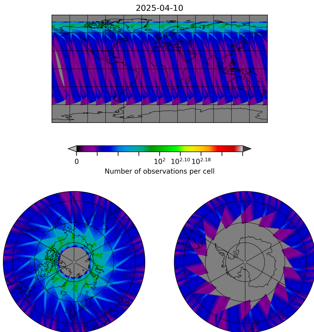
Figure 29: Map of the number of observations for 2025-04-10 to 2025-04-11
