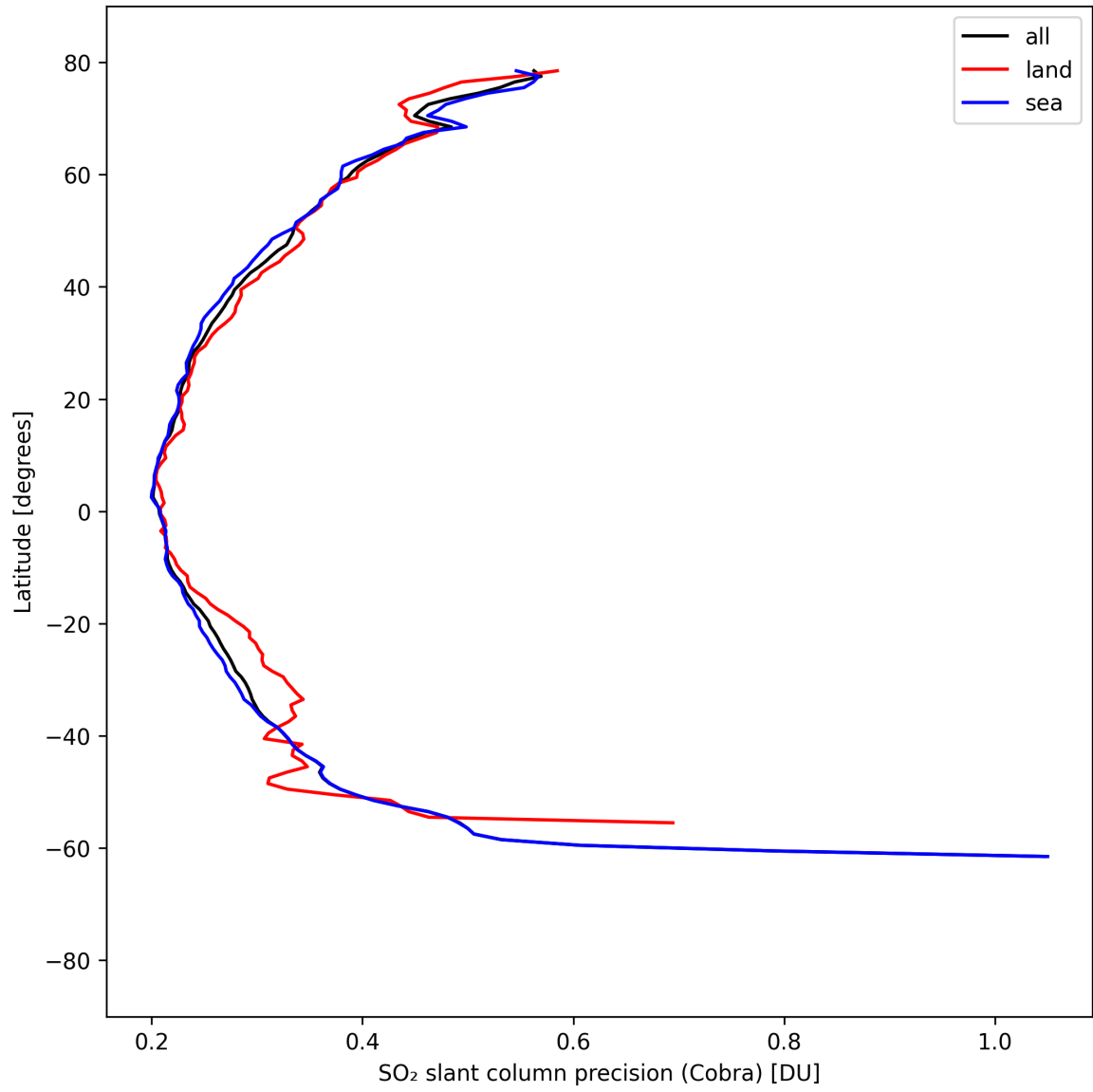
Figure 35: Zonal average of “SO 2 slant column precision (Cobra)” for 2025-04-10 to 2025-04-11.
