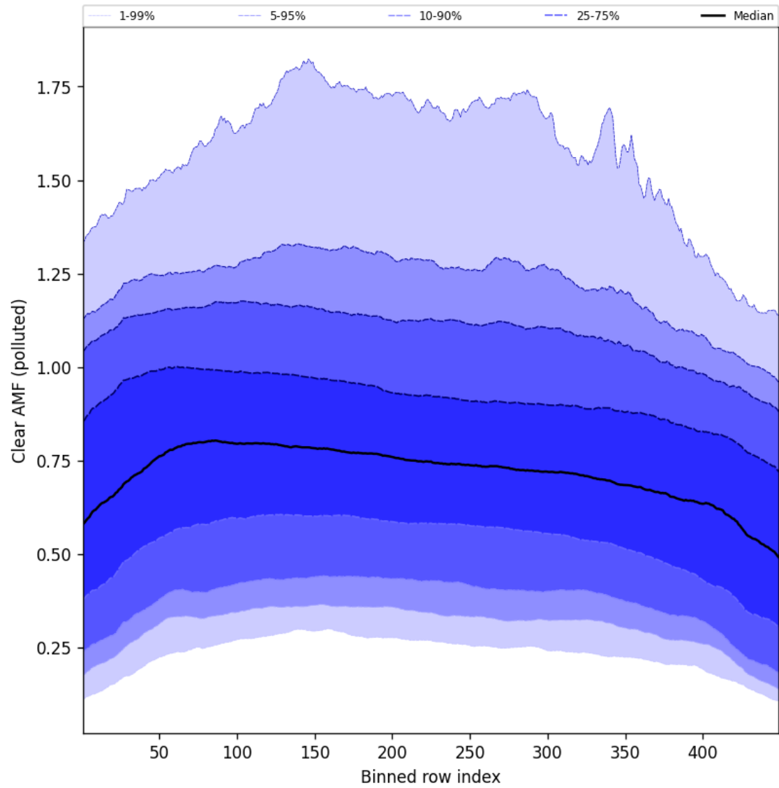
Figure 109: Along track statistics of “Clear AMF (polluted)” for 2025-04-10 to 2025-04-11
