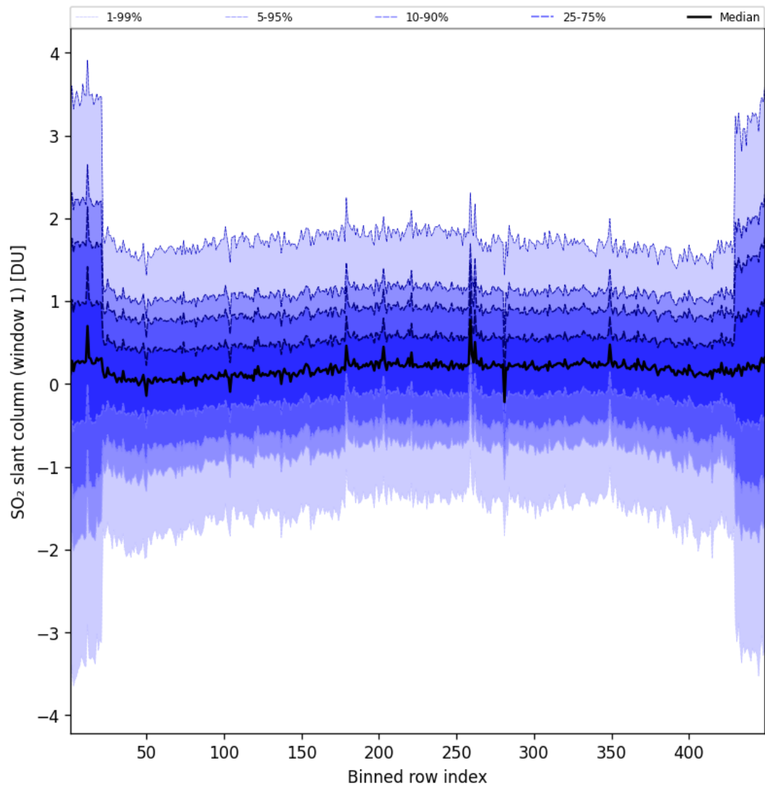
Figure 90: Along track statistics of “SO 2 slant column (window 1)” for 2025-04-10 to 2025-04-11
