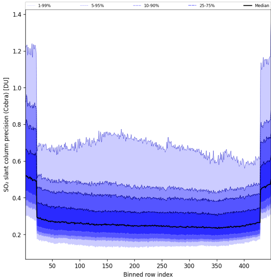
Figure 89: Along track statistics of “SO 2 slant column precision (Cobra)” for 2025-04-10 to 2025-04-11
