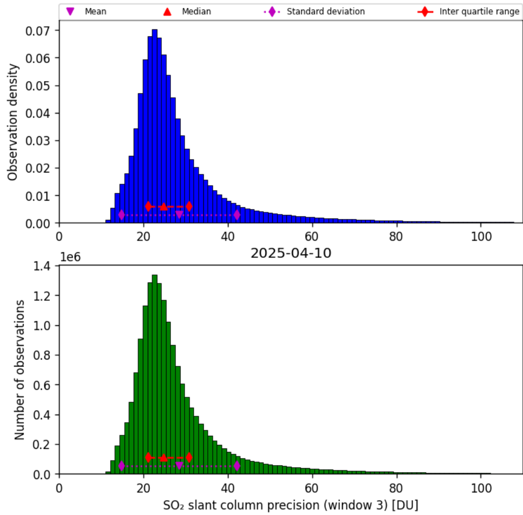
Figure 72: Histogram of “SO 2 slant column precision (window 3)” for 2025-04-10 to 2025-04-11
