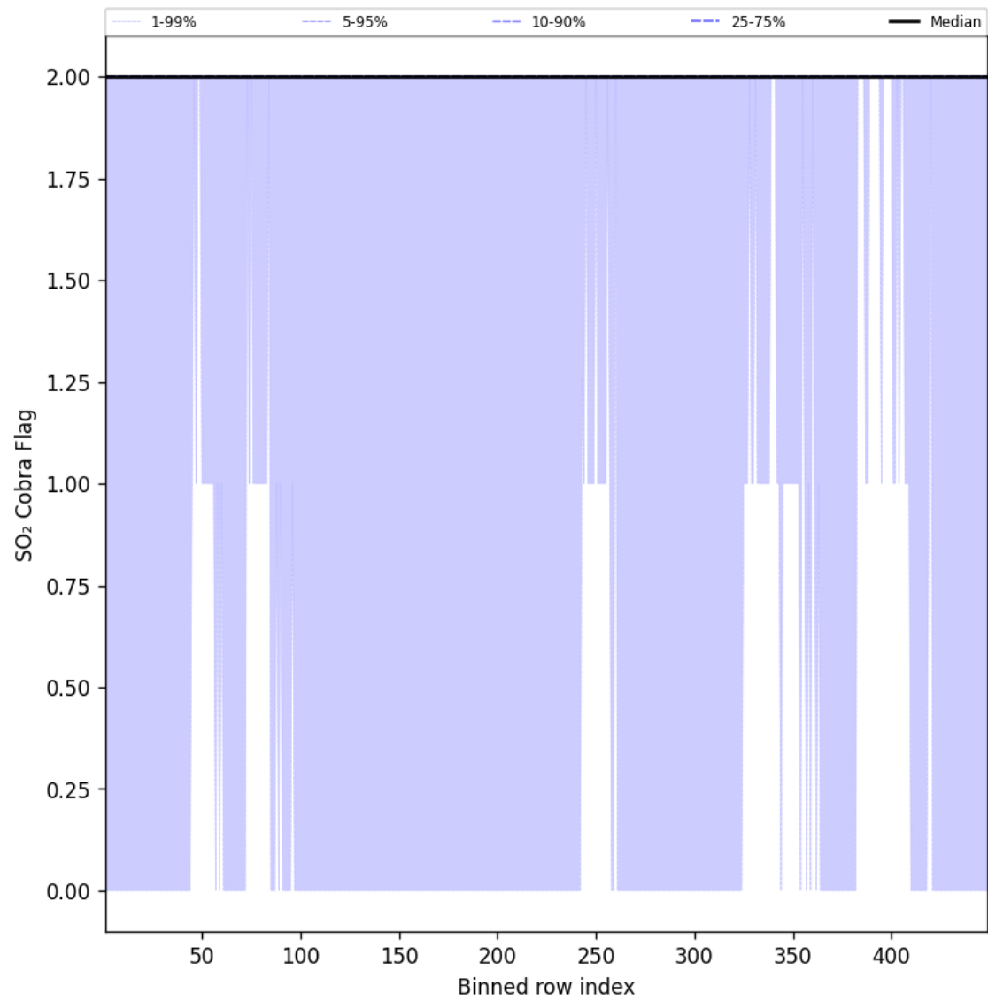
Figure 102: Along track statistics of “SO 2 Cobra Flag” for 2025-04-10 to 2025-04-11
