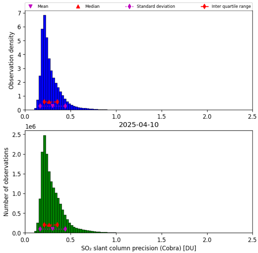
Figure 62: Histogram of “SO 2 slant column precision (Cobra)” for 2025-04-10 to 2025-04-11
