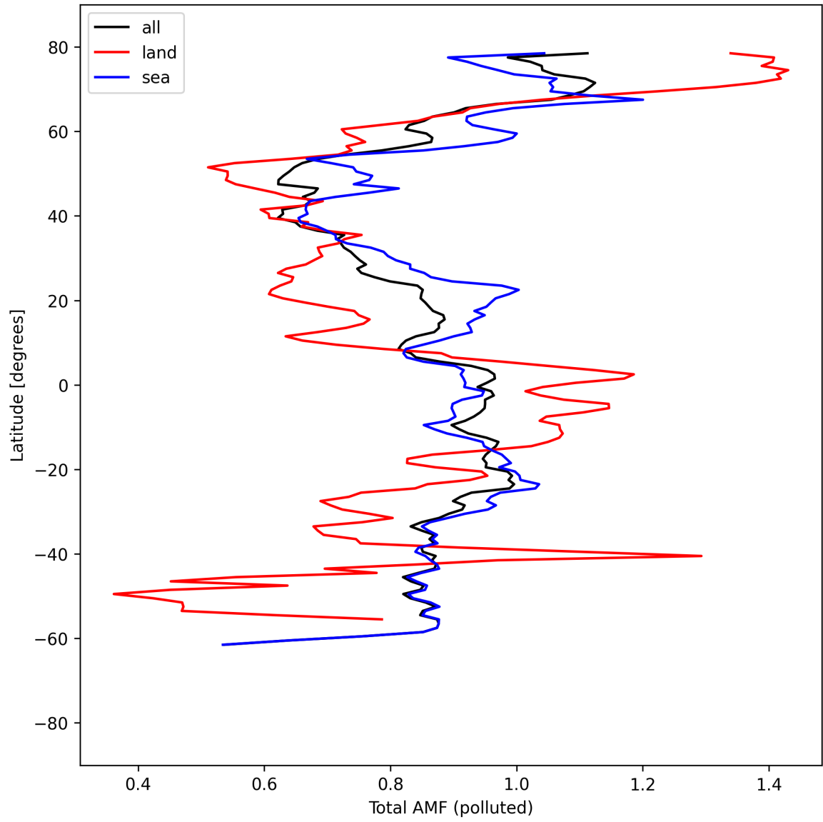
Figure 53: Zonal average of “Total AMF (polluted)” for 2025-04-10 to 2025-04-11.
