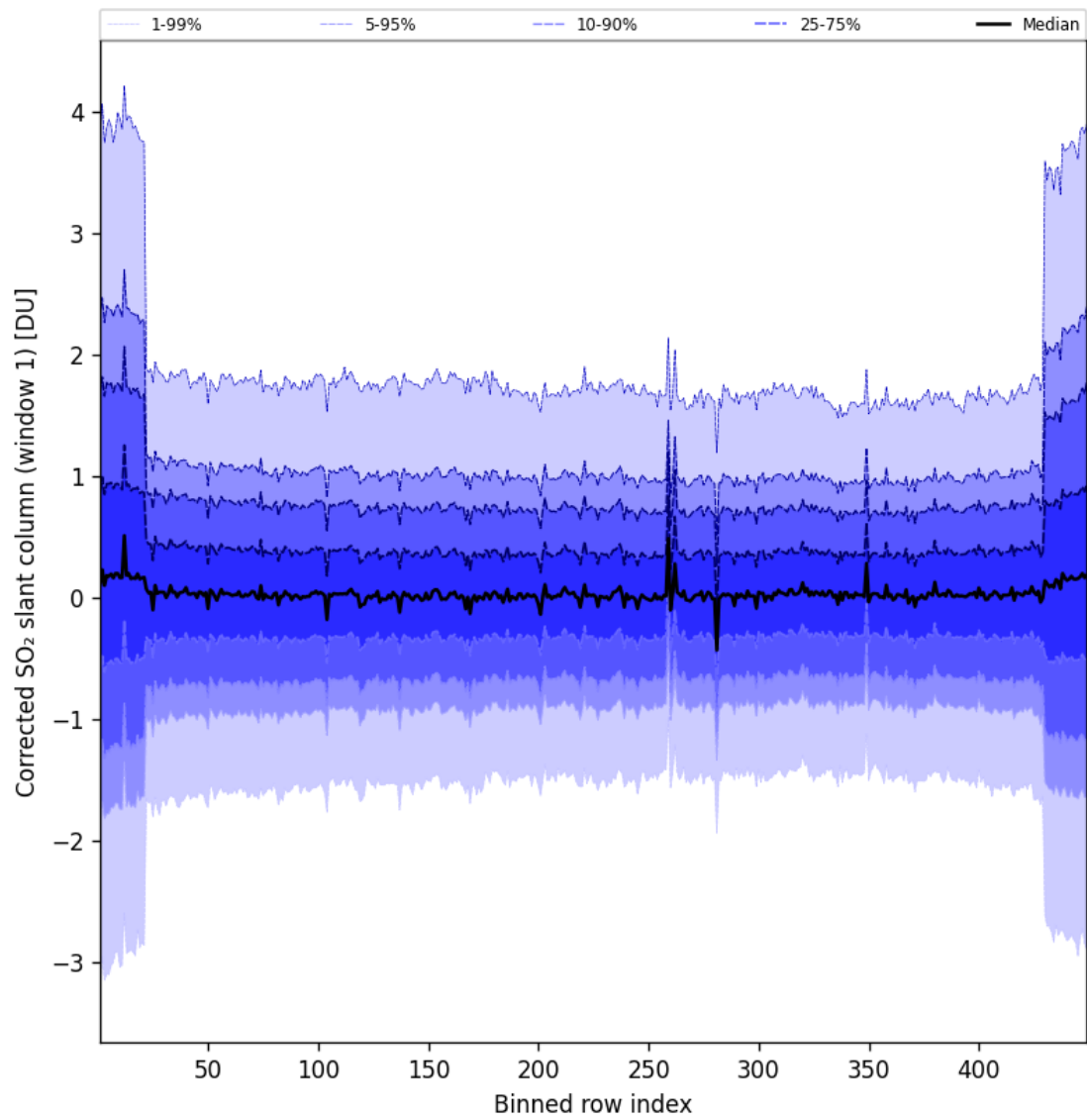
Figure 92: Along track statistics of “Corrected SO 2 slant column (window 1)” for 2025-04-10 to 2025-04-11
