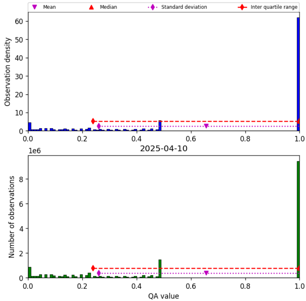
Figure 57: Histogram of “QA value” for 2025-04-10 to 2025-04-11
