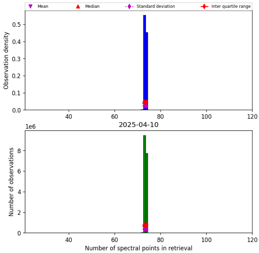
Figure 83: Histogram of “Number of spectral points in retrieval” for 2025-04-10 to 2025-04-11
