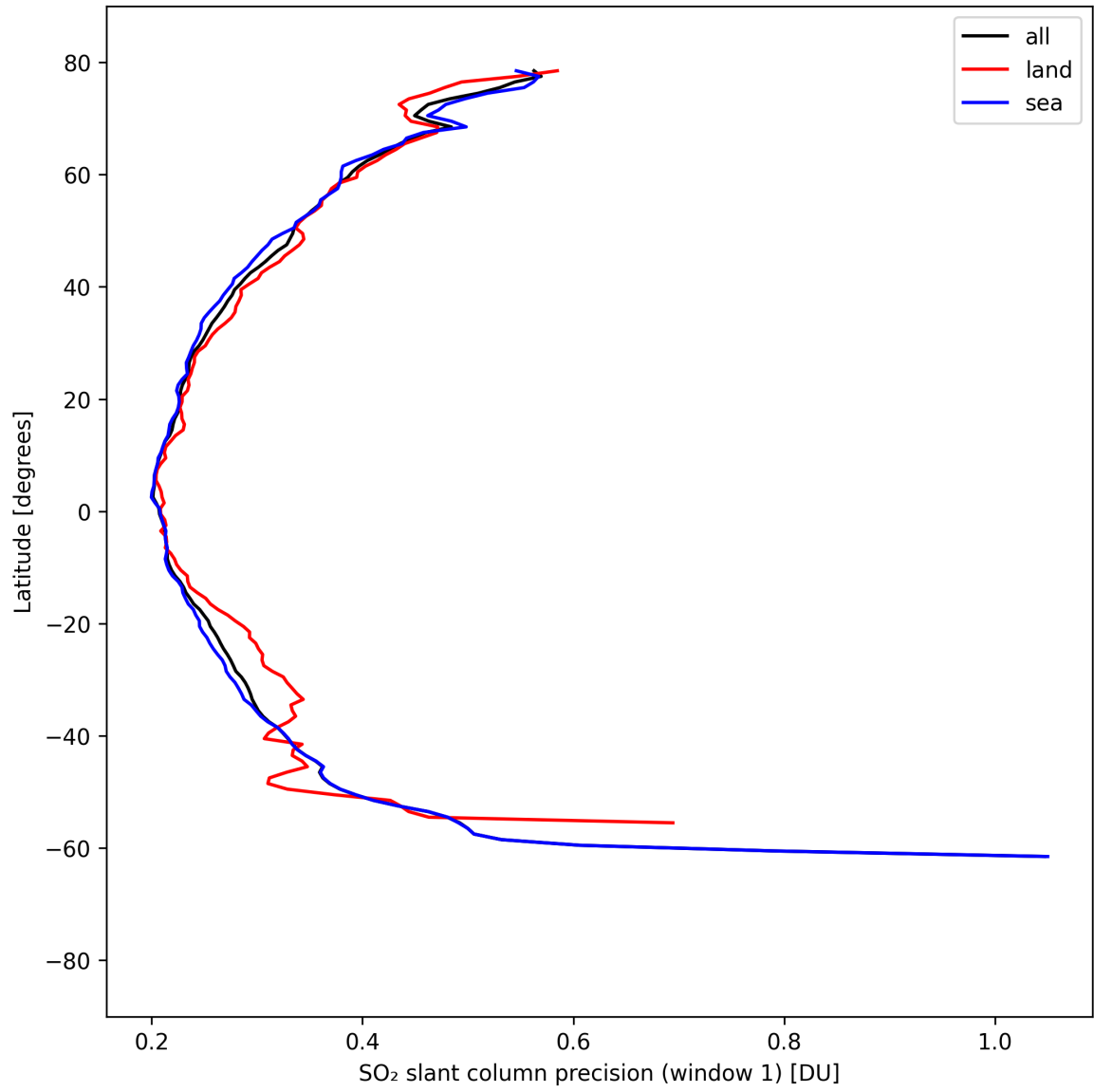
Figure 37: Zonal average of “SO 2 slant column precision (window 1)” for 2025-04-10 to 2025-04-11.
