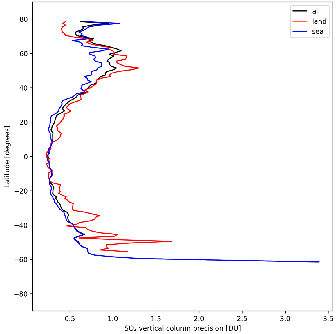
Figure 32: Zonal average of “SO 2 vertical column precision” for 2025-04-10 to 2025-04-11.
