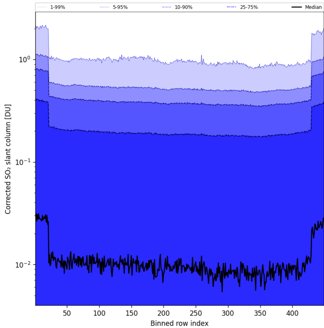
Figure 87: Along track statistics of "Corrected SO 2 slant column" for 2025-04-10 to 2025-04-11
