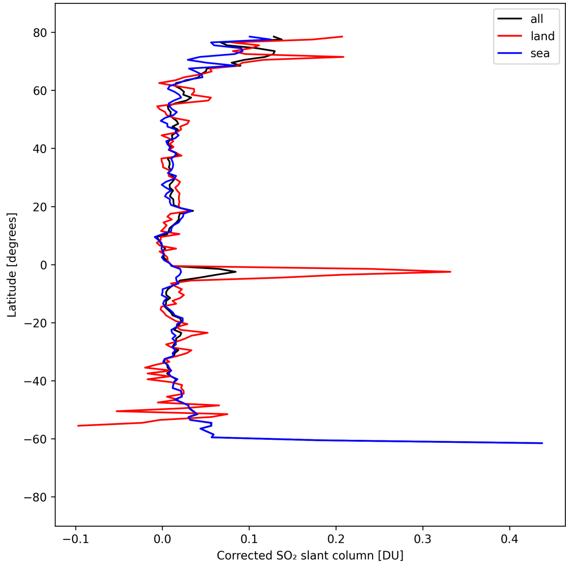
Figure 33: Zonal average of “Corrected SO 2 slant column” for 2025-04-10 to 2025-04-11.
