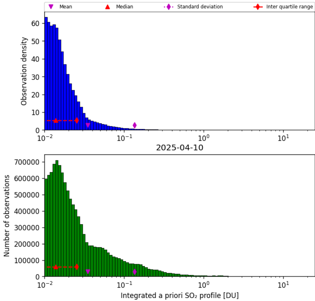
Figure 76: Histogram of “Integrated a priori SO 2 profile” for 2025-04-10 to 2025-04-11
