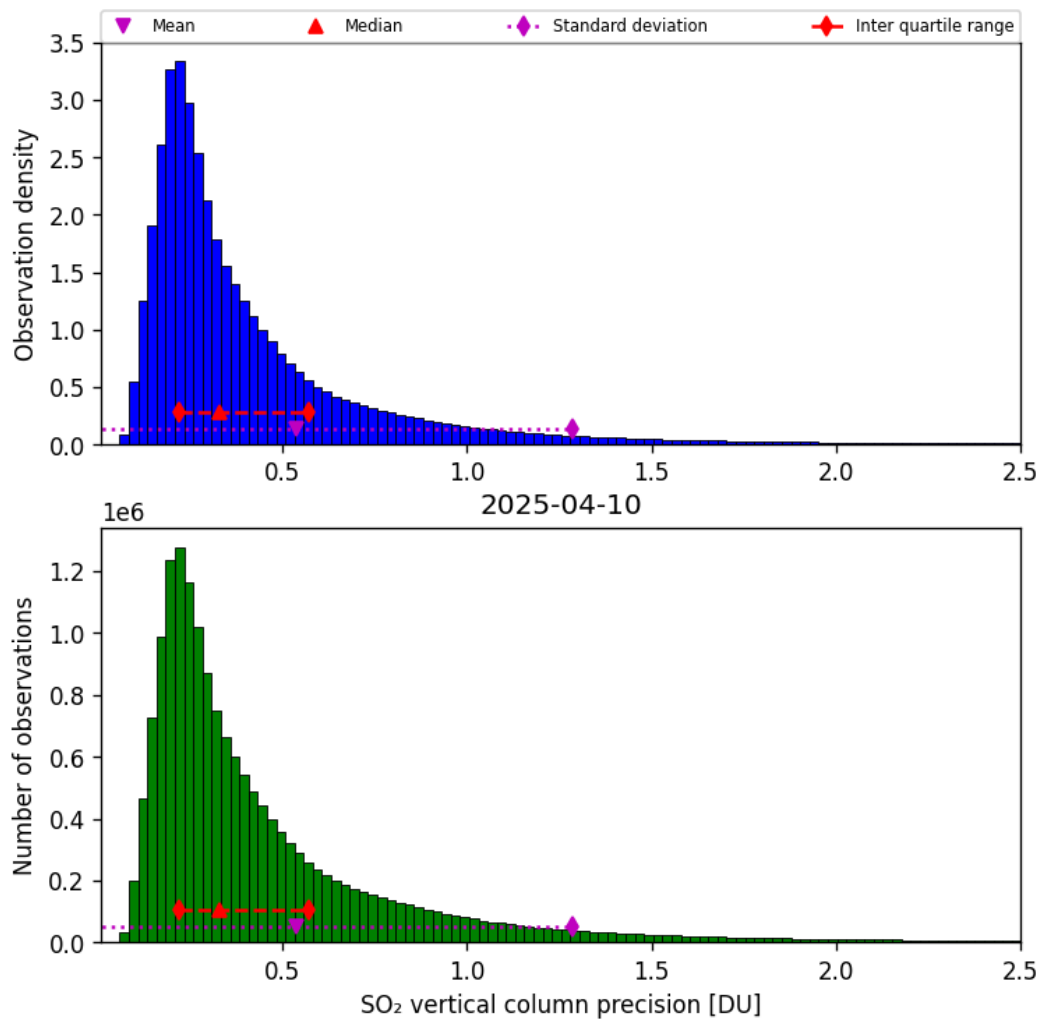
Figure 59: Histogram of “SO 2 vertical column precision” for 2025-04-10 to 2025-04-11
