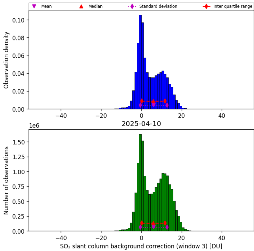
Figure 74: Histogram of “SO 2 slant column background correction (window 3)” for 2025-04-10 to 2025-04-11
