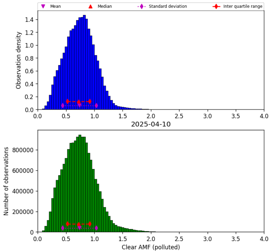
Figure 82: Histogram of “Clear AMF (polluted)” for 2025-04-10 to 2025-04-11
