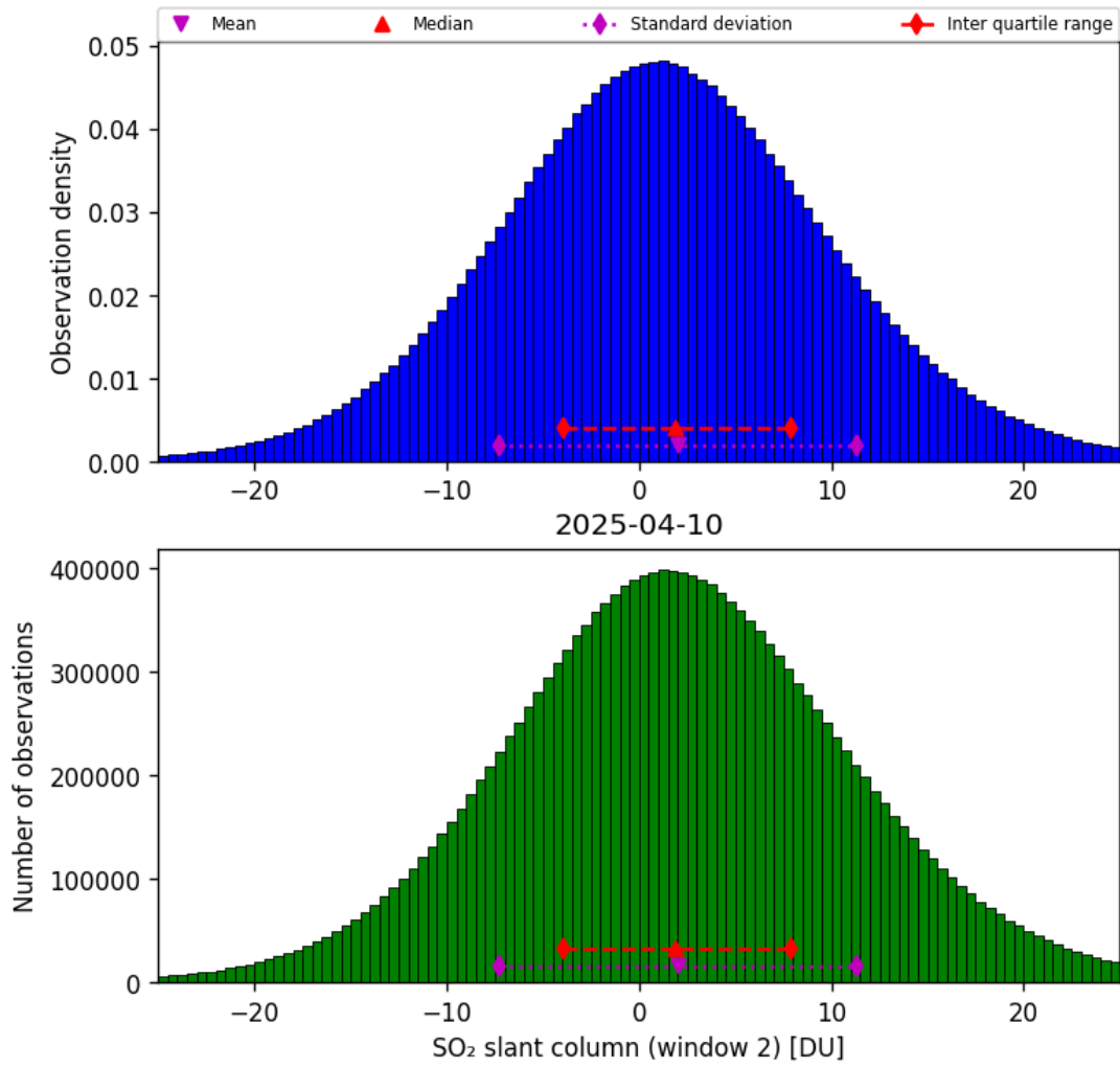
Figure 67: Histogram of “SO 2 slant column (window 2)” for 2025-04-10 to 2025-04-11
