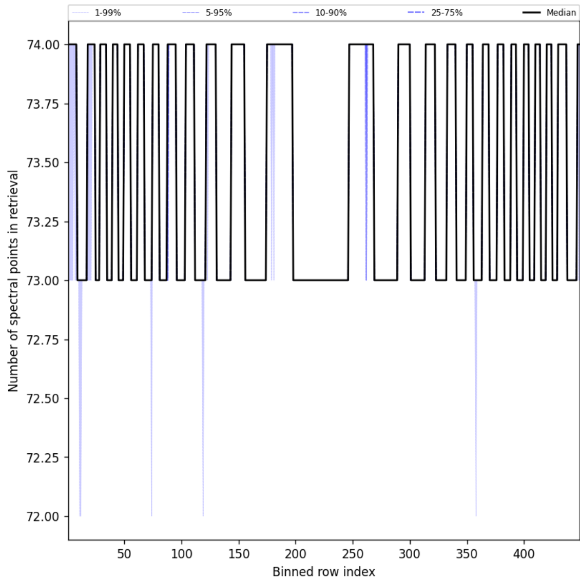
Figure 110: Along track statistics of “Number of spectral points in retrieval” for 2025-04-10 to 2025-04-11
