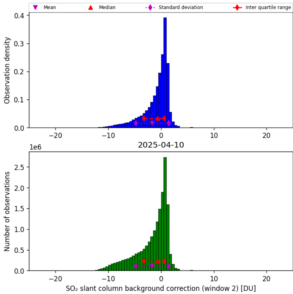
Figure 70: Histogram of “SO 2 slant column background correction (window 2)” for 2025-04-10 to 2025-04-11
