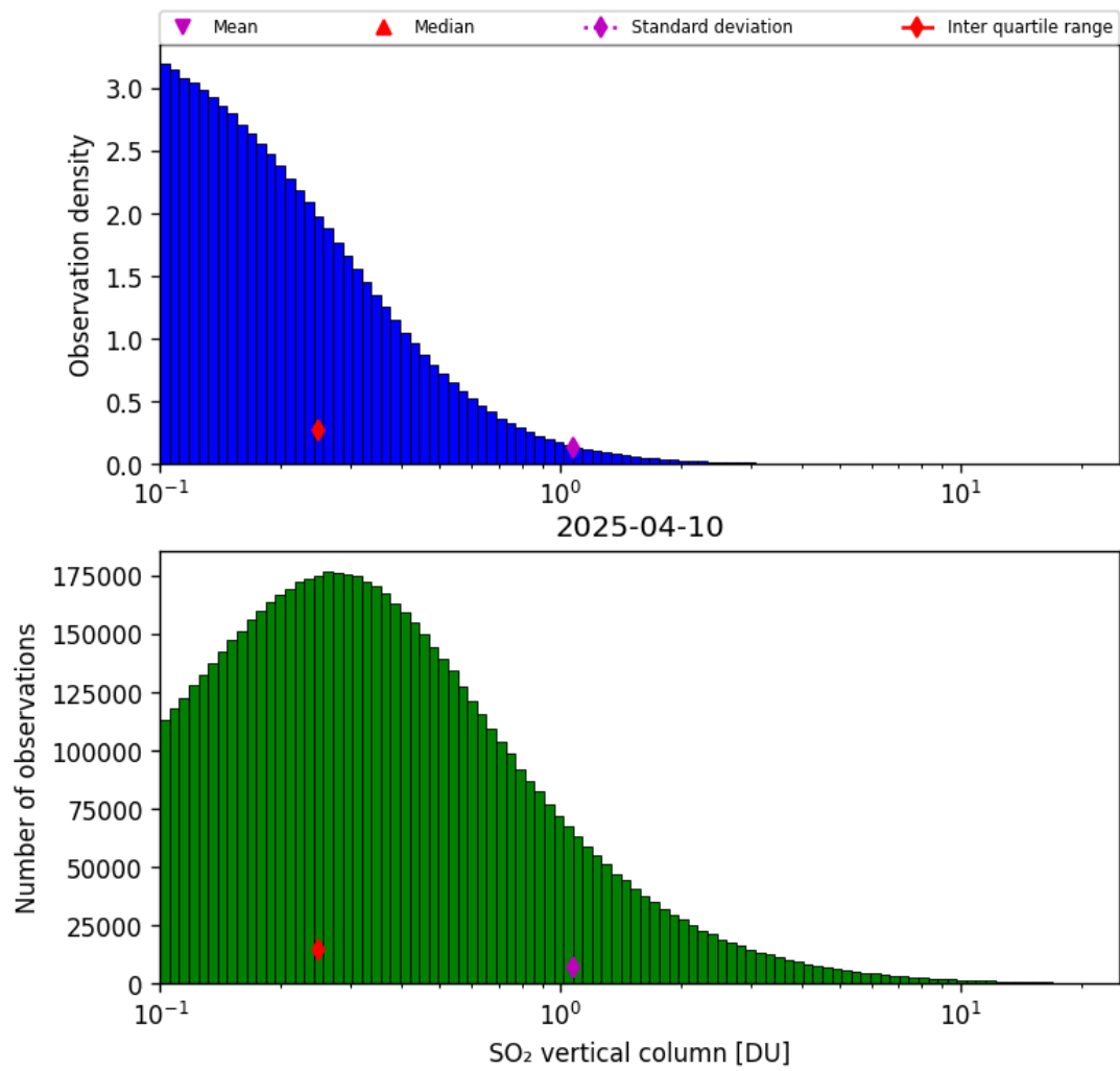
Figure 58: Histogram of “SO 2 vertical column” for 2025-04-10 to 2025-04-11
