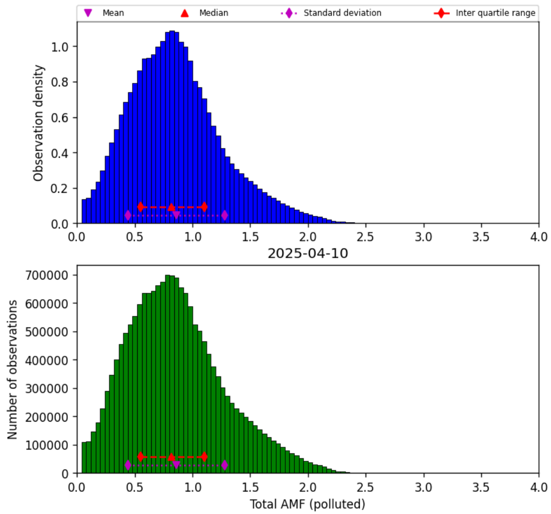
Figure 80: Histogram of “Total AMF (polluted)” for 2025-04-10 to 2025-04-11
