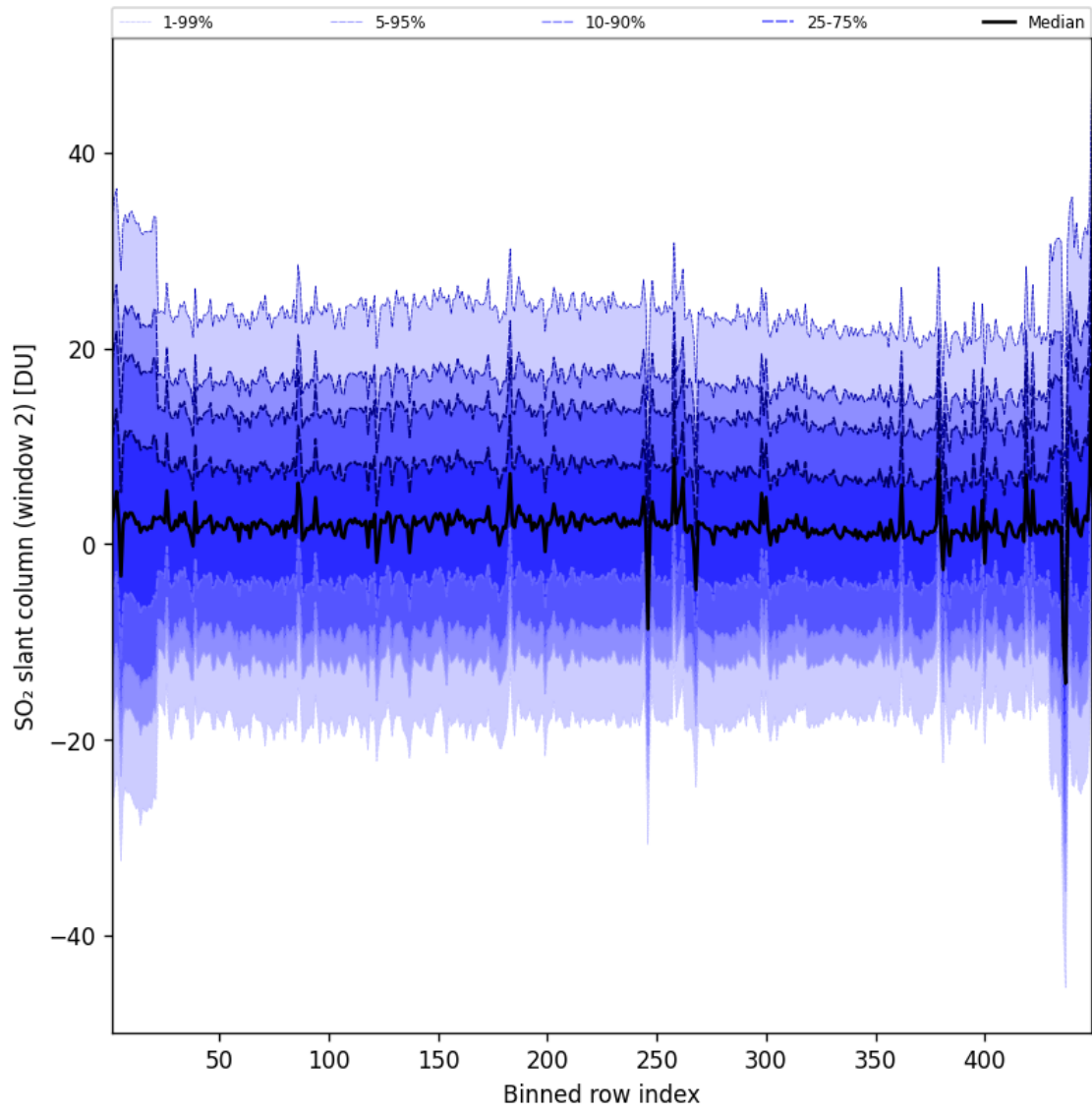
Figure 94: Along track statistics of “SO 2 slant column (window 2)” for 2025-04-10 to 2025-04-11
