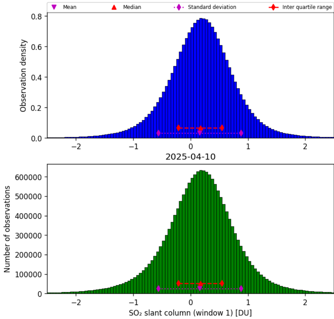
Figure 63: Histogram of “SO 2 slant column (window 1)” for 2025-04-10 to 2025-04-11
