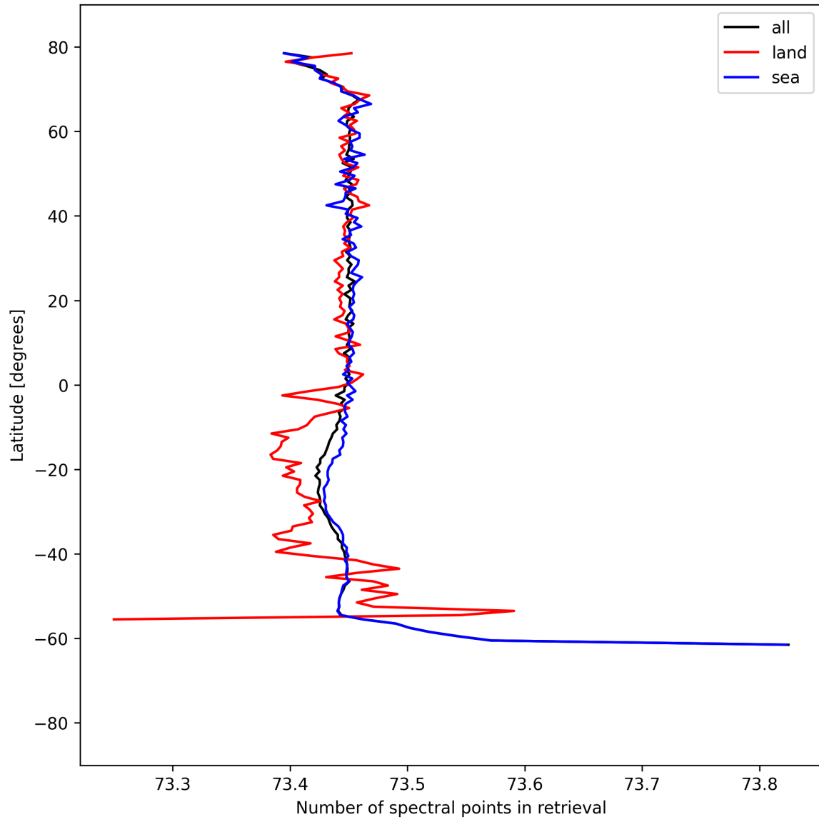
Figure 56: Zonal average of “Number of spectral points in retrieval” for 2025-04-10 to 2025-04-11.
