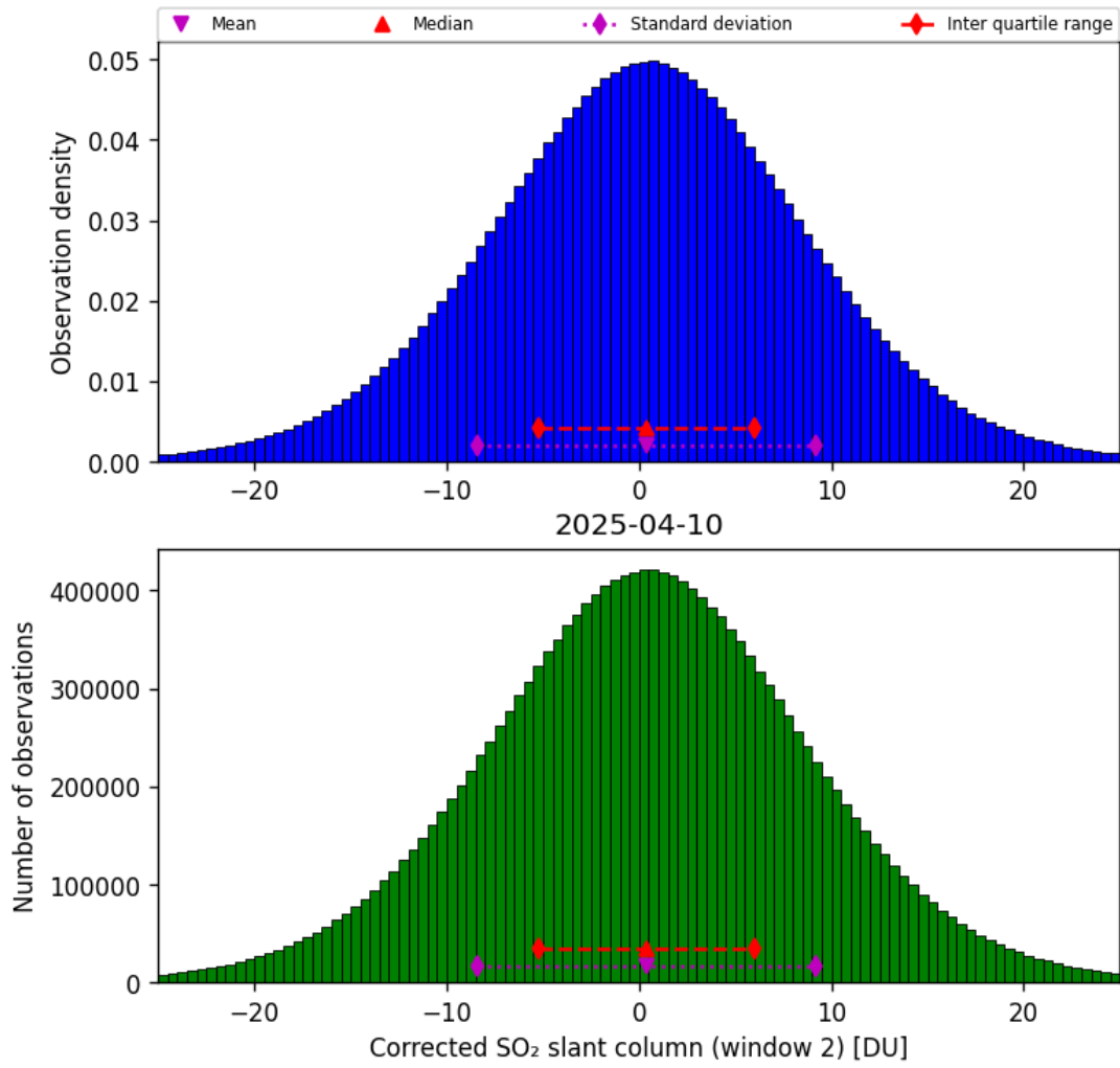
Figure 69: Histogram of “Corrected SO 2 slant column (window 2)” for 2025-04-10 to 2025-04-11
