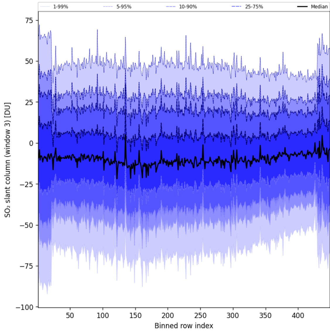
Figure 98: Along track statistics of “SO 2 slant column (window 3)” for 2025-04-10 to 2025-04-11
