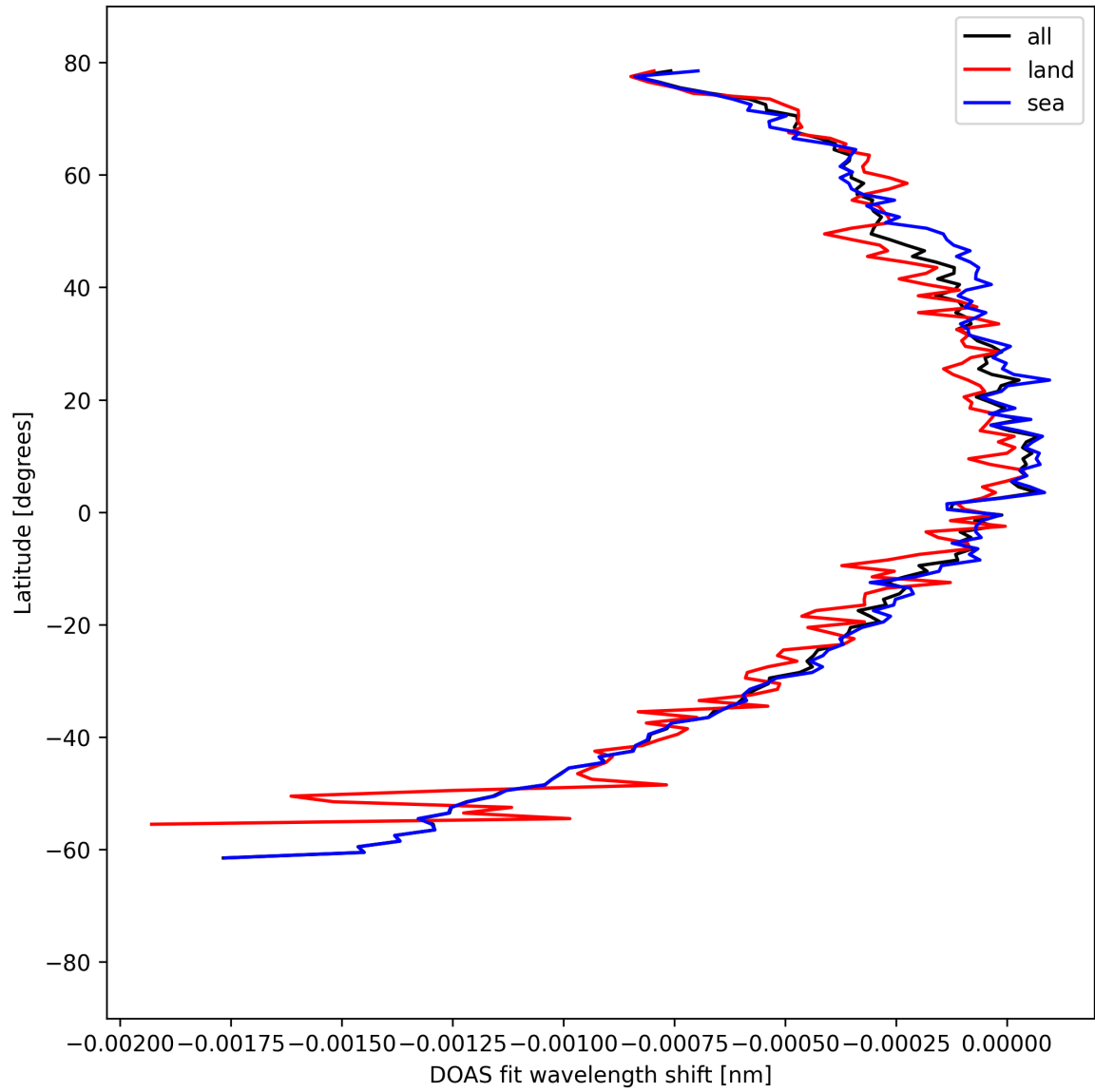
Figure 50: Zonal average of “DOAS fit wavelength shift” for 2025-04-10 to 2025-04-11.
