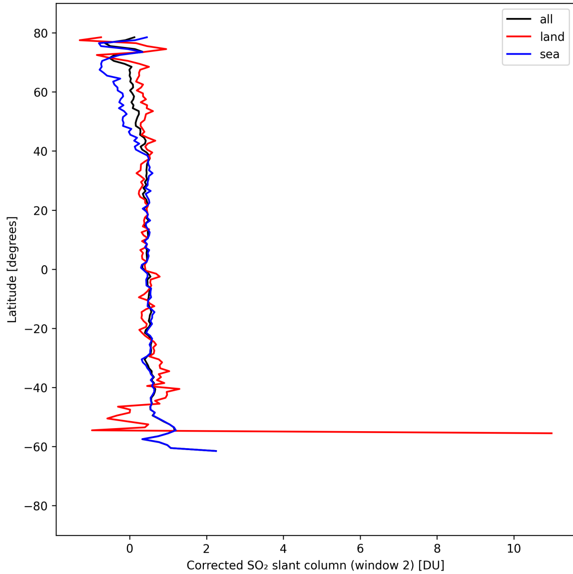
Figure 42: Zonal average of “Corrected SO 2 slant column (window 2)” for 2025-04-10 to 2025-04-11.
