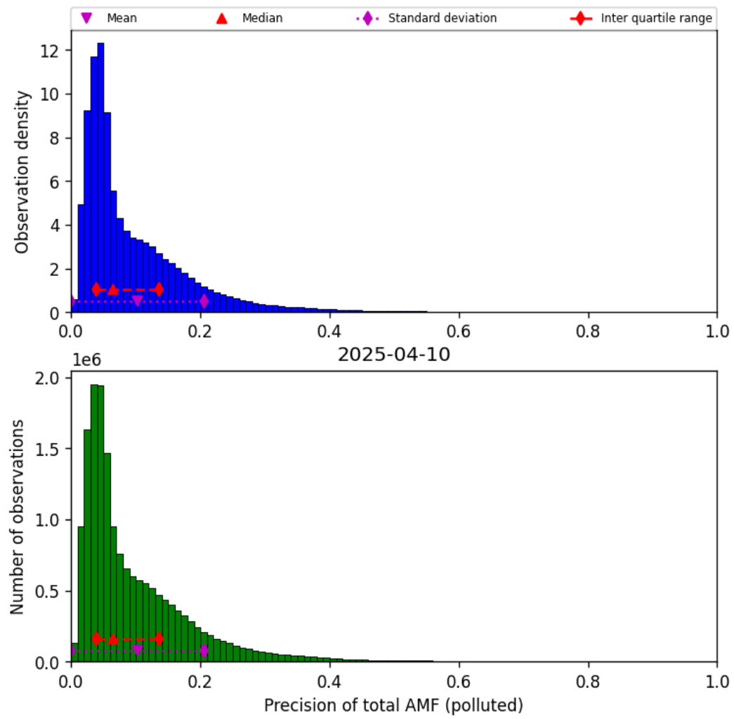
Figure 81: Histogram of “Precision of total AMF (polluted)” for 2025-04-10 to 2025-04-11
