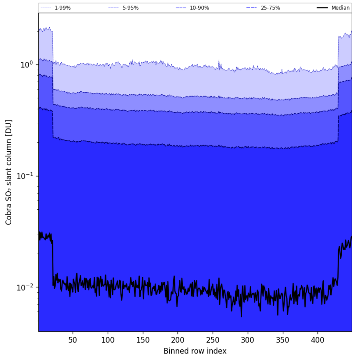
Figure 88: Along track statistics of “Cobra SO 2 slant column” for 2025-04-10 to 2025-04-11
