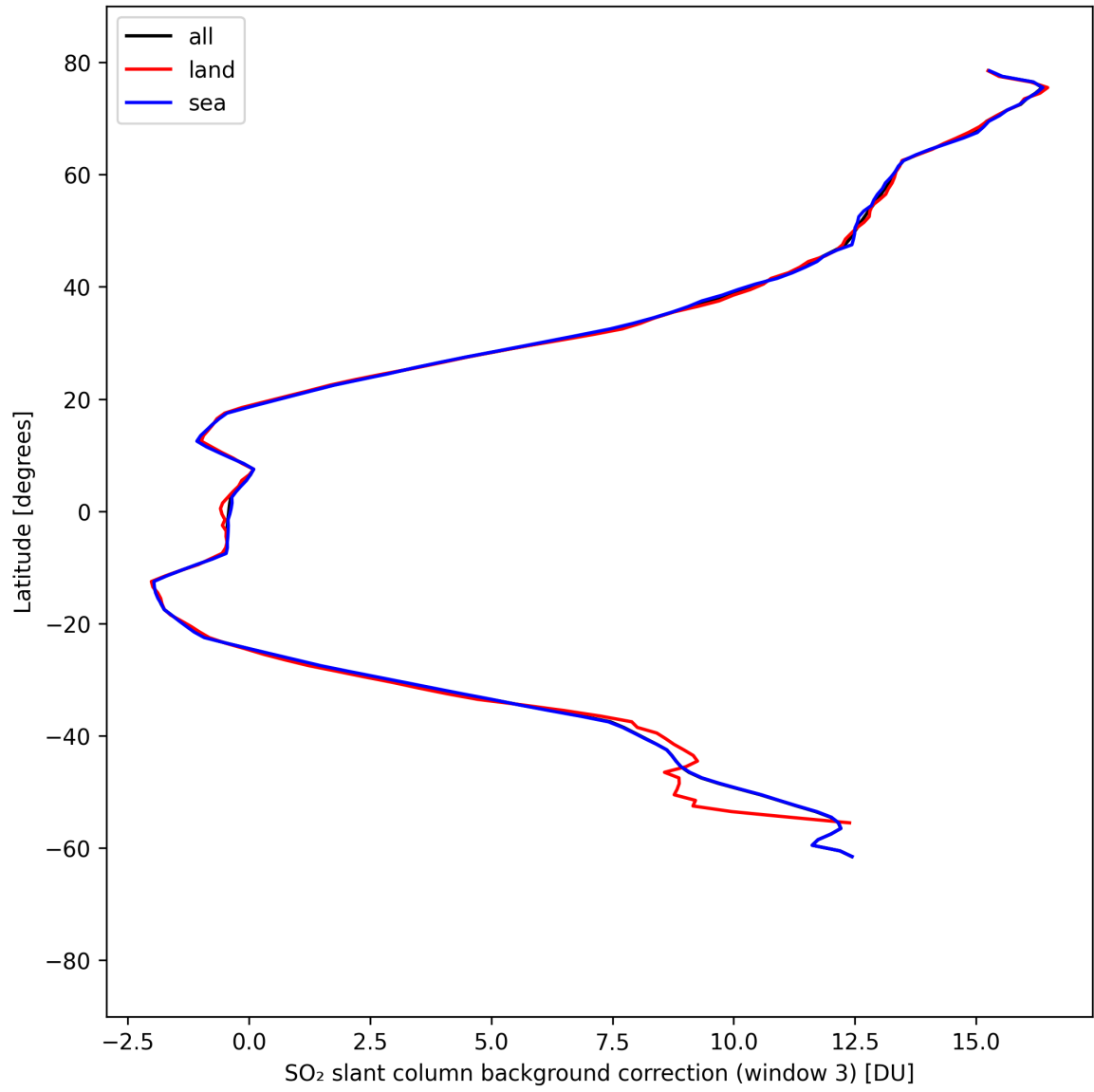
Figure 47: Zonal average of “SO 2 slant column background correction (window 3)” for 2025-04-10 to 2025-04-11.
