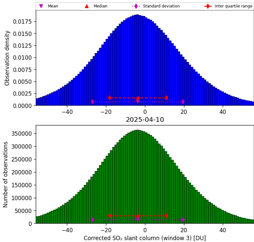
Figure 73: Histogram of “Corrected SO 2 slant column (window 3)” for 2025-04-10 to 2025-04-11
