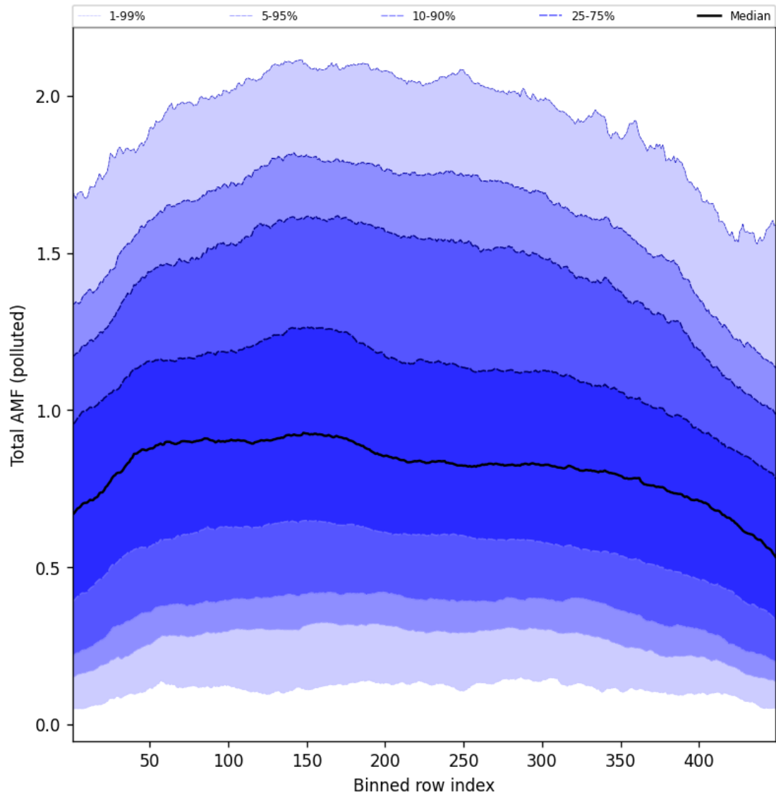
Figure 107: Along track statistics of “Total AMF (polluted)” for 2025-04-10 to 2025-04-11
