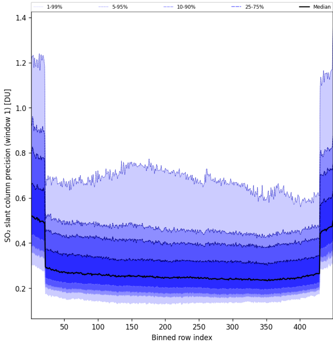
Figure 91: Along track statistics of “SO 2 slant column precision (window 1)” for 2025-04-10 to 2025-04-11
