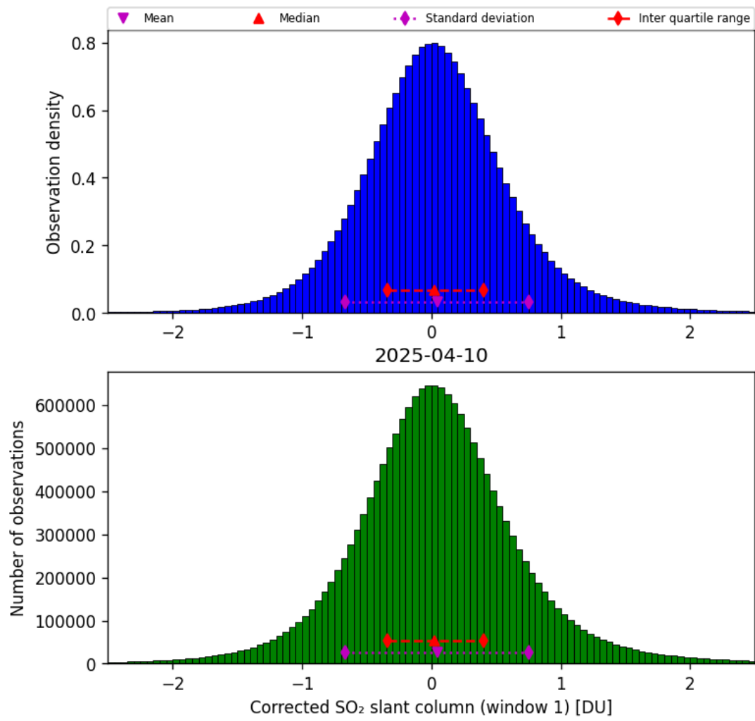
Figure 65: Histogram of “Corrected SO 2 slant column (window 1)” for 2025-04-10 to 2025-04-11
