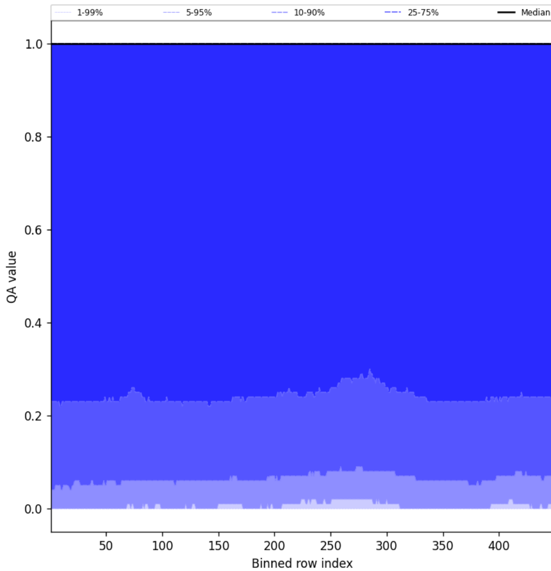
Figure 84: Along track statistics of “QA value” for 2025-04-10 to 2025-04-11
