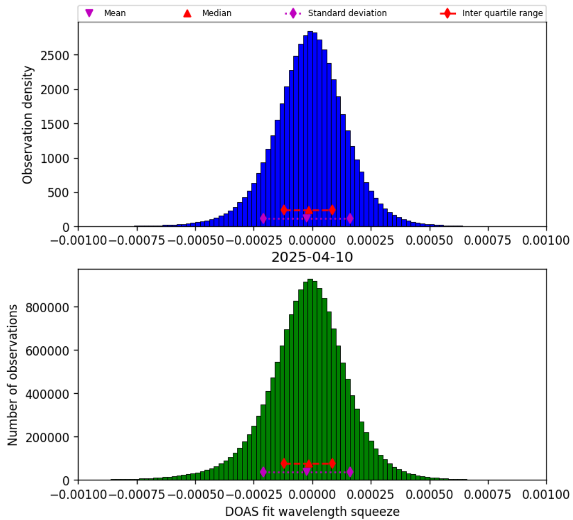
Figure 78: Histogram of “DOAS fit wavelength squeeze” for 2025-04-10 to 2025-04-11
