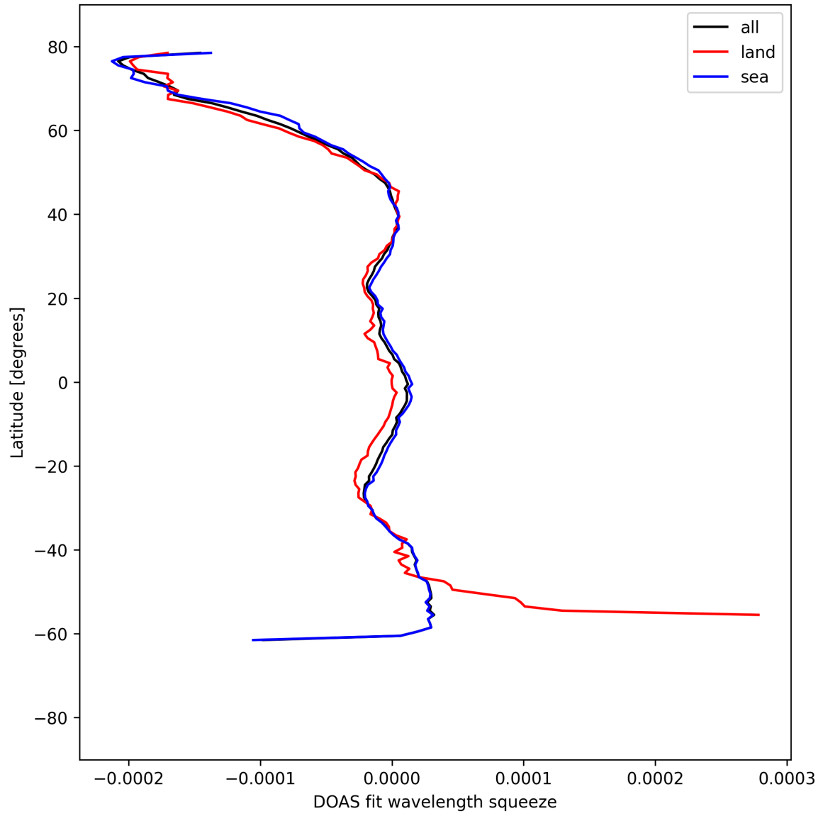
Figure 51: Zonal average of “DOAS fit wavelength squeeze” for 2025-04-10 to 2025-04-11.
