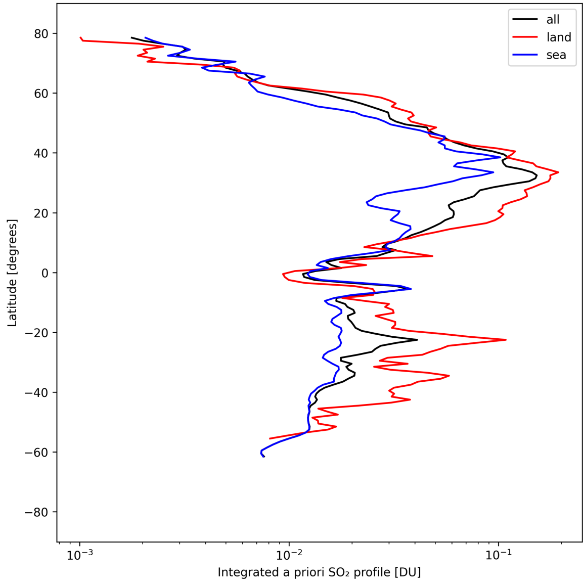
Figure 49: Zonal average of “Integrated a priori SO 2 profile” for 2025-04-10 to 2025-04-11.
