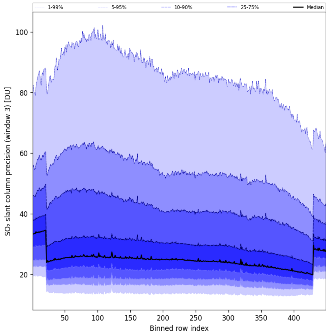
Figure 99: Along track statistics of “SO 2 slant column precision (window 3)” for 2025-04-10 to 2025-04-11
