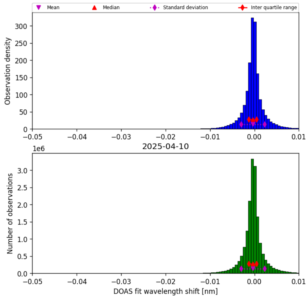
Figure 77: Histogram of “DOAS fit wavelength shift” for 2025-04-10 to 2025-04-11
