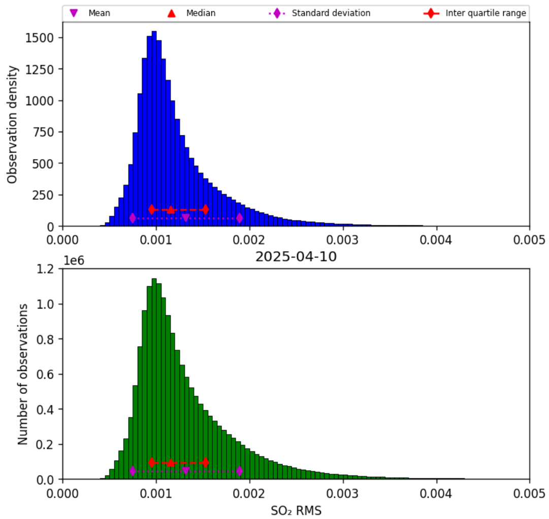
Figure 79: Histogram of “SO 2 RMS” for 2025-04-10 to 2025-04-11
