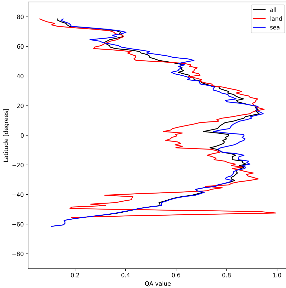
Figure 30: Zonal average of “QA value” for 2025-04-10 to 2025-04-11.
