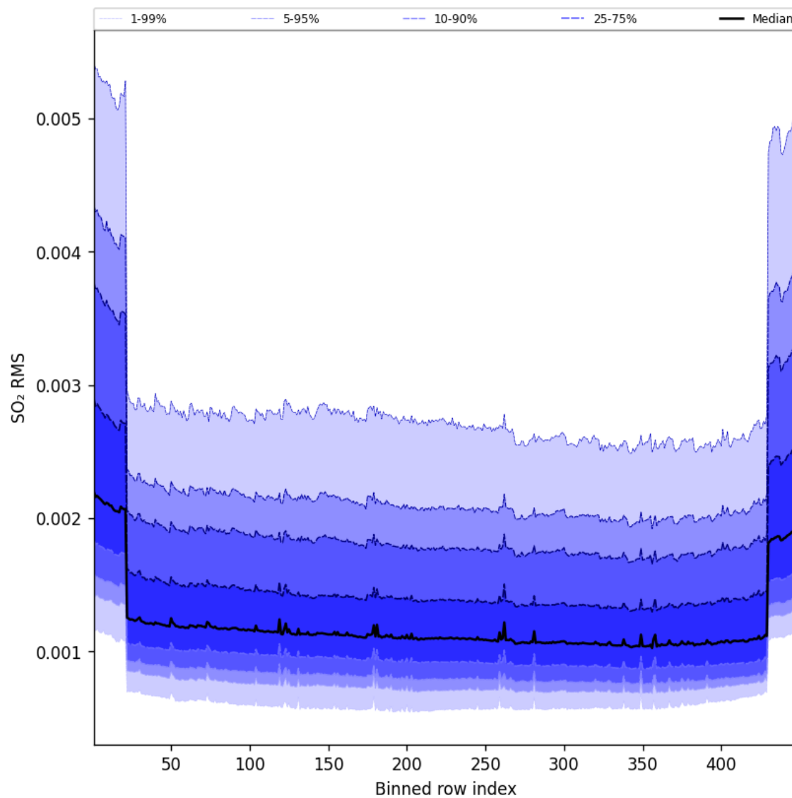
Figure 106: Along track statistics of “SO 2 RMS” for 2025-04-10 to 2025-04-11
