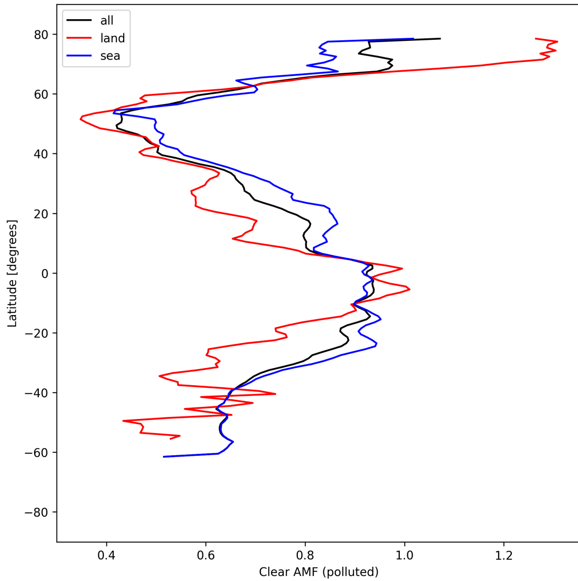
Figure 55: Zonal average of “Clear AMF (polluted)” for 2025-04-10 to 2025-04-11.
