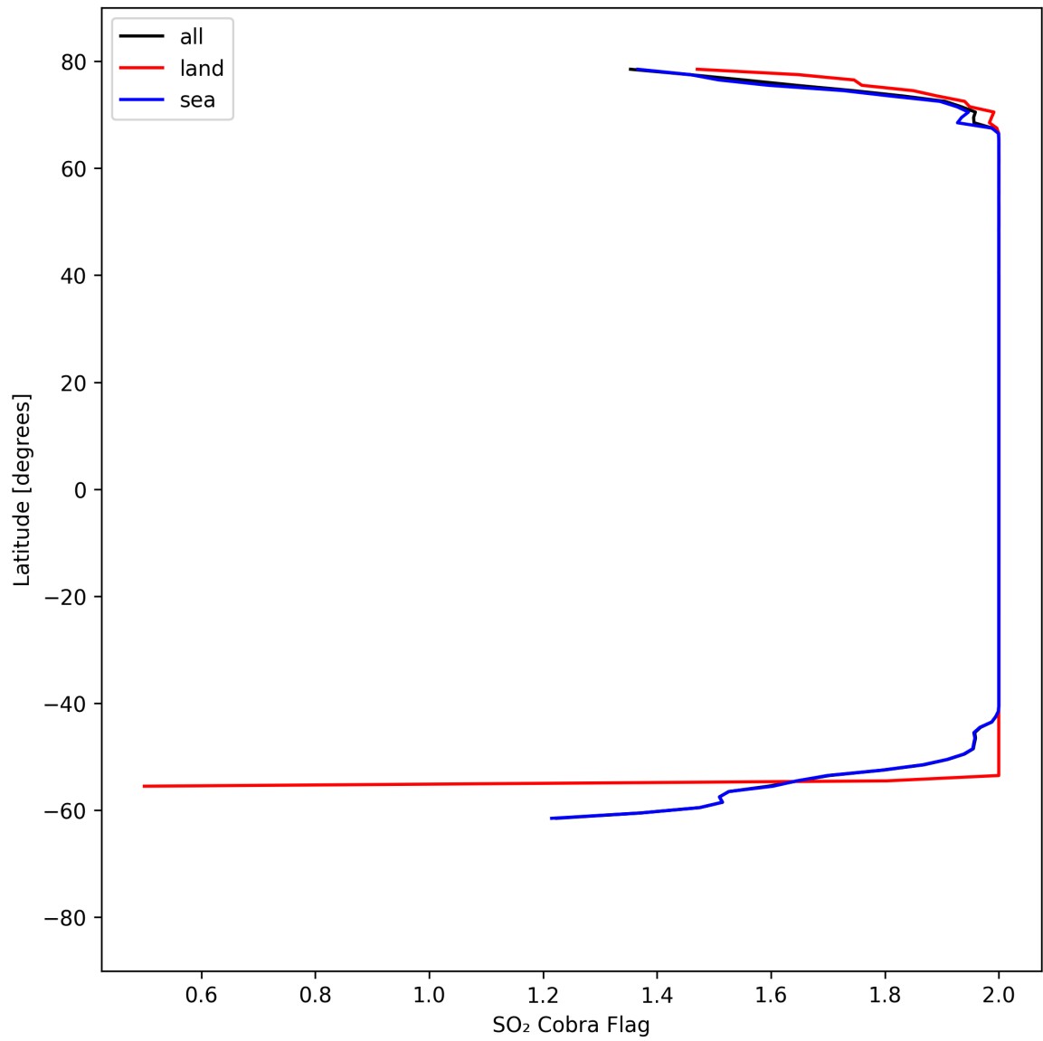
Figure 48: Zonal average of "SO 2 Cobra Flag" for 2025-04-10 to 2025-04-11.
