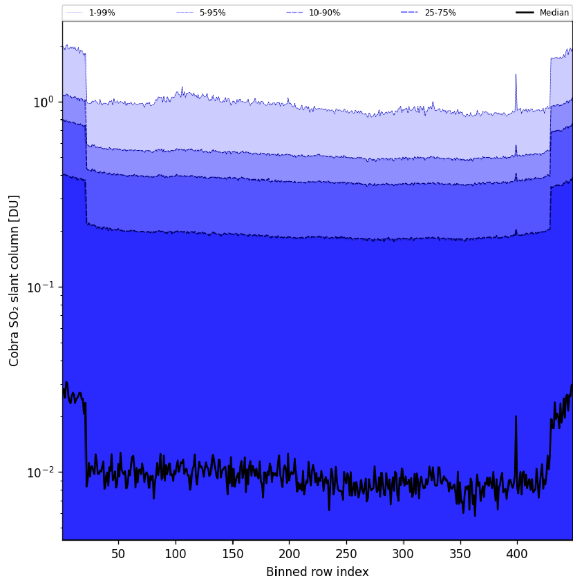
Figure 88: Along track statistics of “Cobra SO 2 slant column” for 2025-04-16 to 2025-04-16
