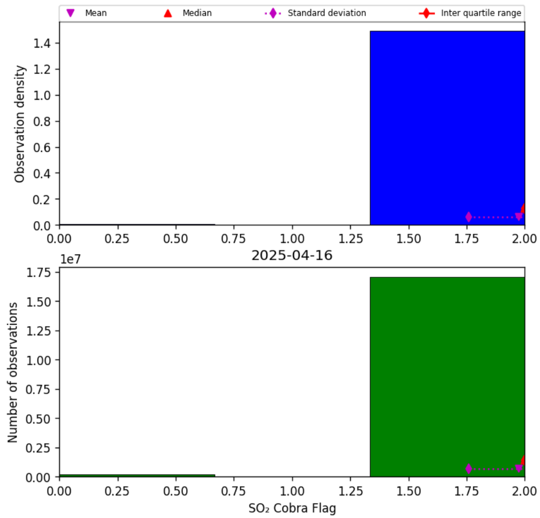
Figure 75: Histogram of “SO 2 Cobra Flag” for 2025-04-16 to 2025-04-16
