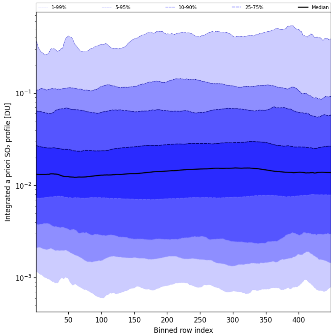
Figure 103: Along track statistics of “Integrated a priori SO 2 profile” for 2025-04-16 to 2025-04-16
