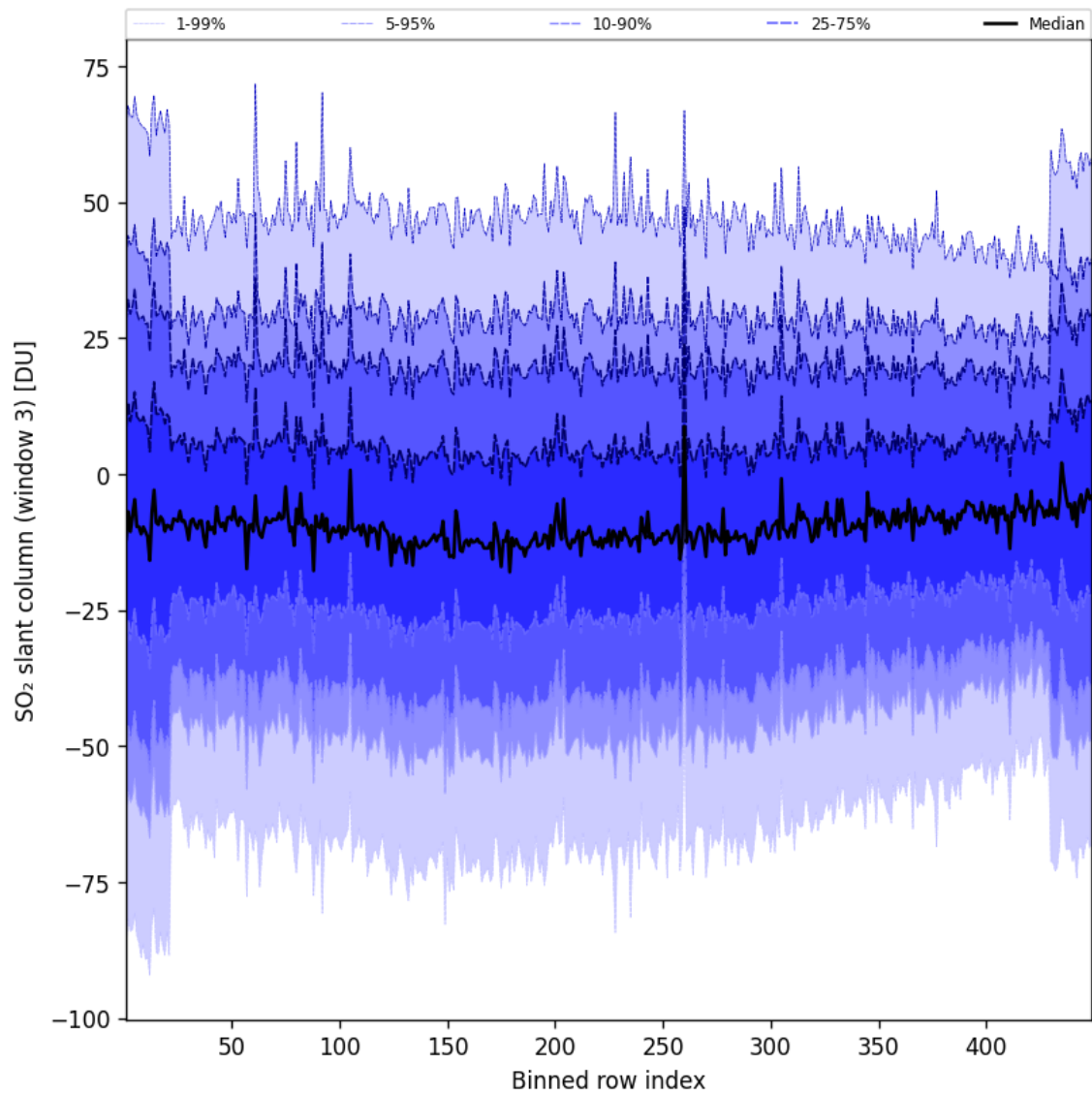
Figure 98: Along track statistics of “SO 2 slant column (window 3)” for 2025-04-16 to 2025-04-16
