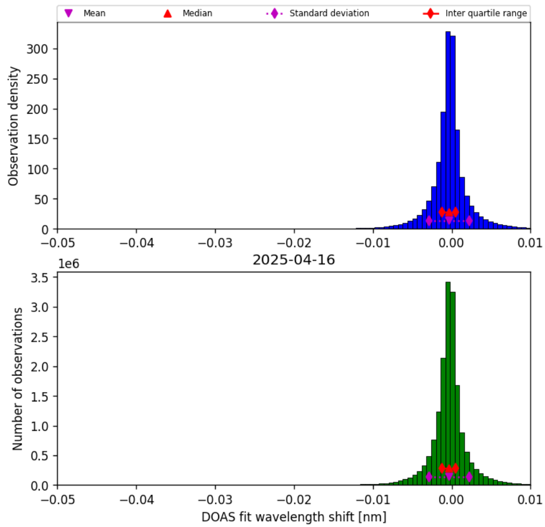
Figure 77: Histogram of “DOAS fit wavelength shift” for 2025-04-16 to 2025-04-16
