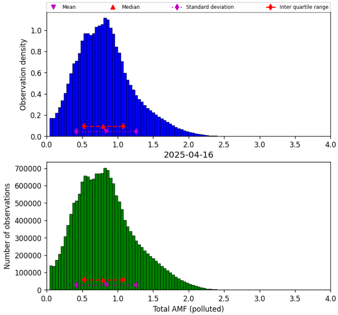
Figure 80: Histogram of “Total AMF (polluted)” for 2025-04-16 to 2025-04-16
