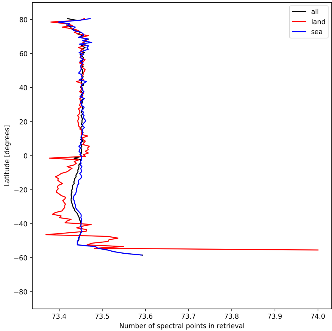
Figure 56: Zonal average of “Number of spectral points in retrieval” for 2025-04-16 to 2025-04-16.
