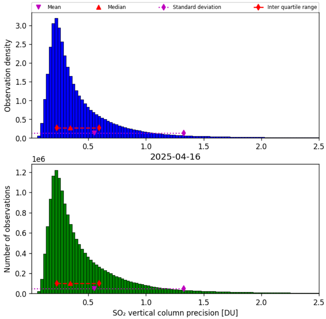
Figure 59: Histogram of “SO 2 vertical column precision” for 2025-04-16 to 2025-04-16
