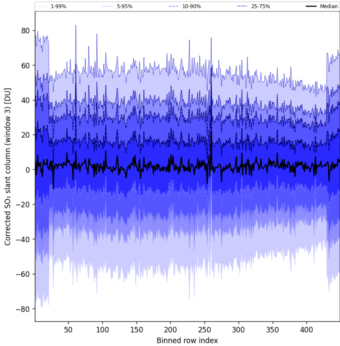
Figure 100: Along track statistics of “Corrected SO 2 slant column (window 3)” for 2025-04-16 to 2025-04-16
