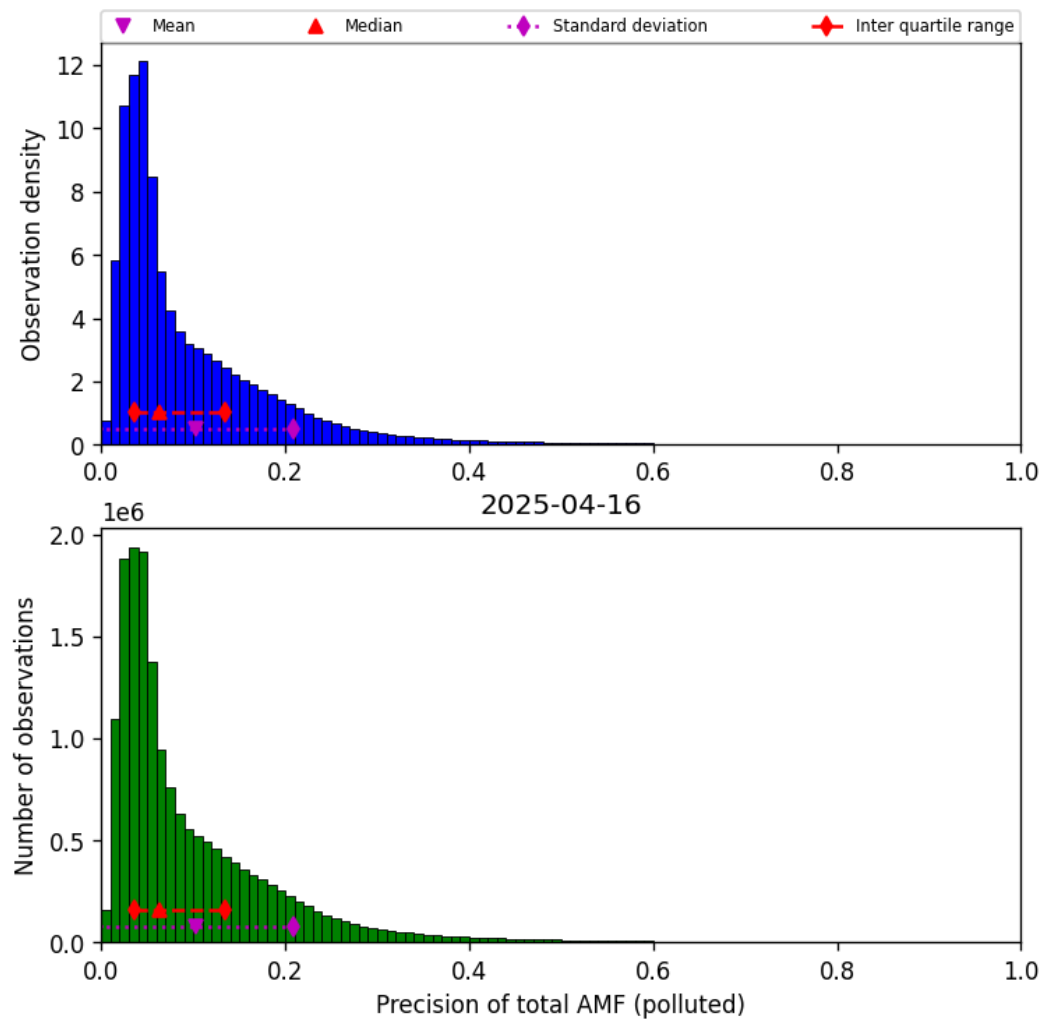
Figure 81: Histogram of “Precision of total AMF (polluted)” for 2025-04-16 to 2025-04-16
