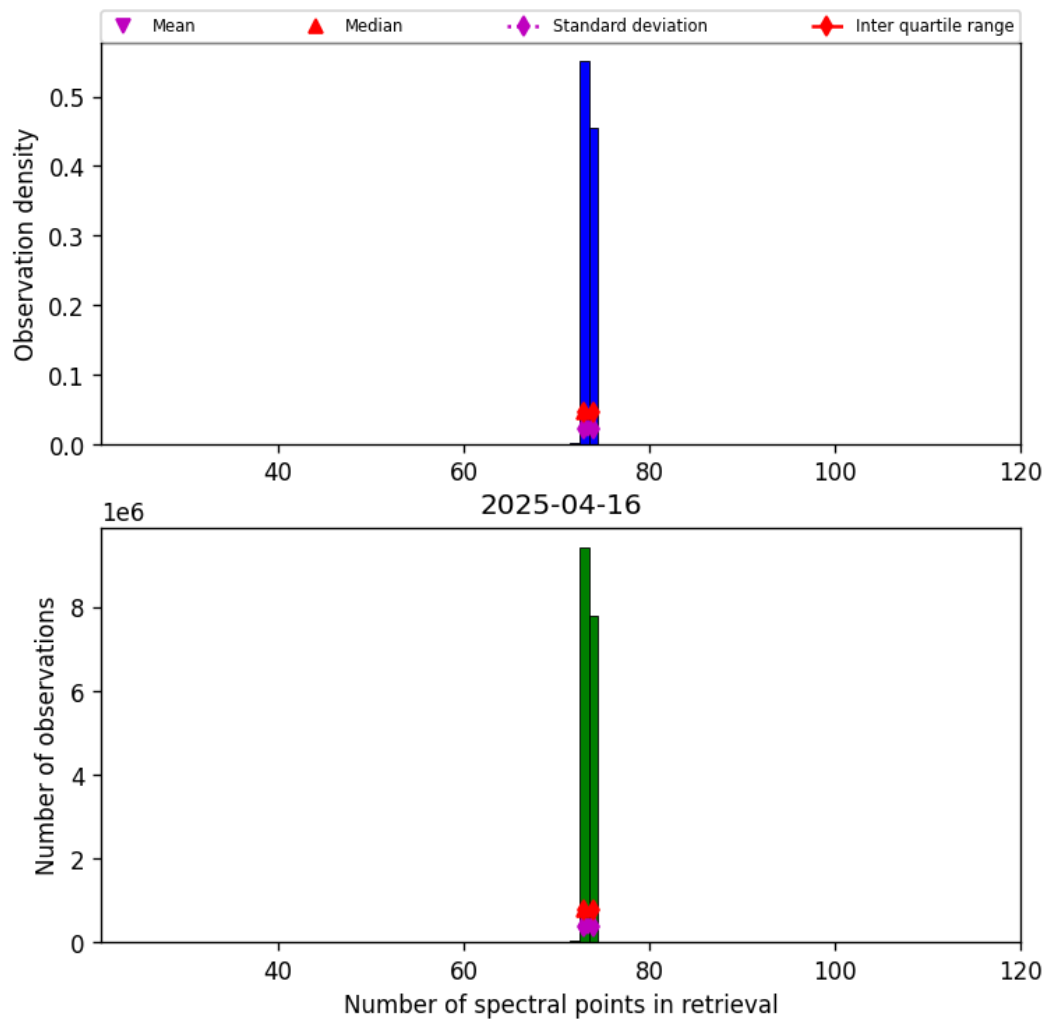
Figure 83: Histogram of "Number of spectral points in retrieval" for 2025-04-16 to 2025-04-16
