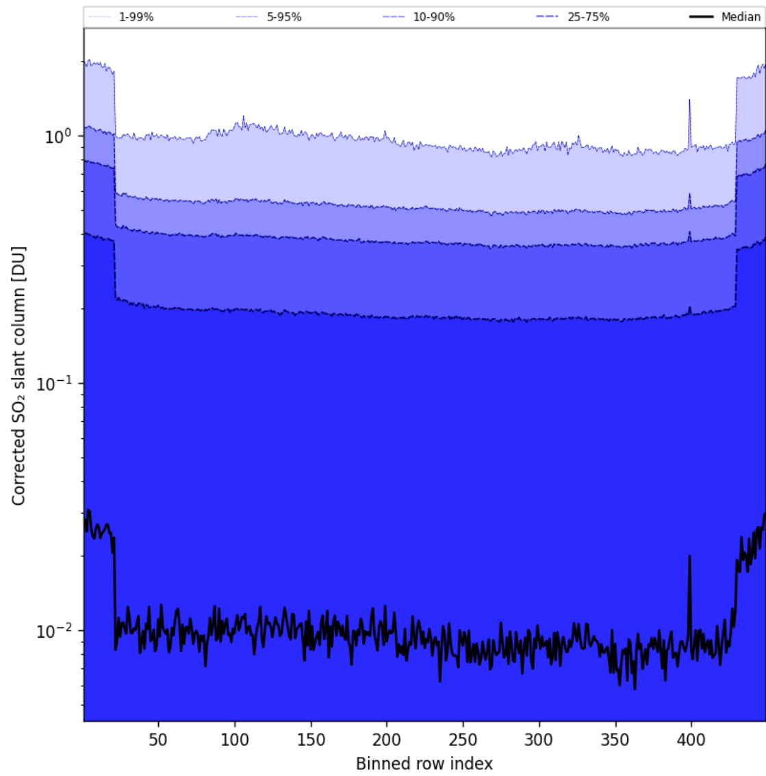
Figure 87: Along track statistics of "Corrected SO 2 slant column" for 2025-04-16 to 2025-04-16
