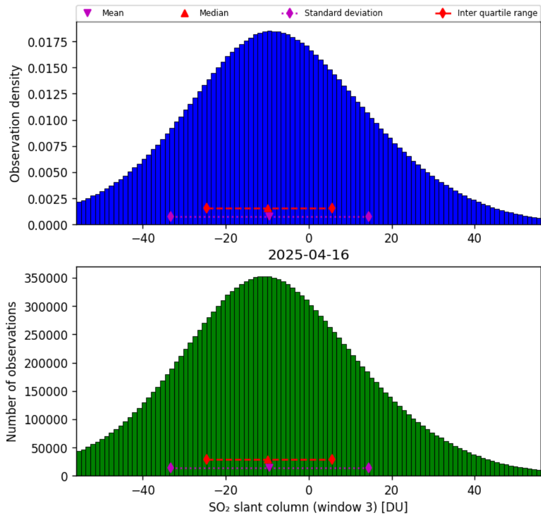
Figure 71: Histogram of “SO 2 slant column (window 3)” for 2025-04-16 to 2025-04-16
