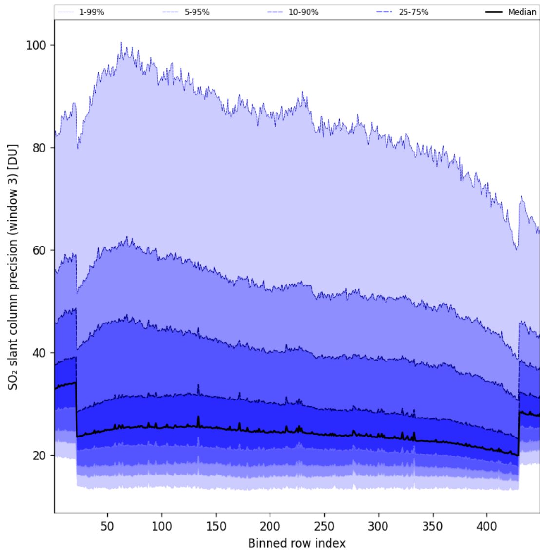
Figure 99: Along track statistics of “SO 2 slant column precision (window 3)” for 2025-04-16 to 2025-04-16
