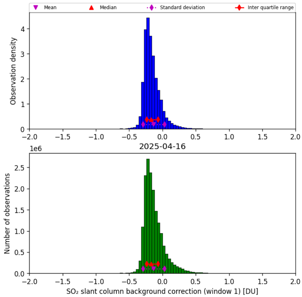
Figure 66: Histogram of “SO 2 slant column background correction (window 1)” for 2025-04-16 to 2025-04-16
