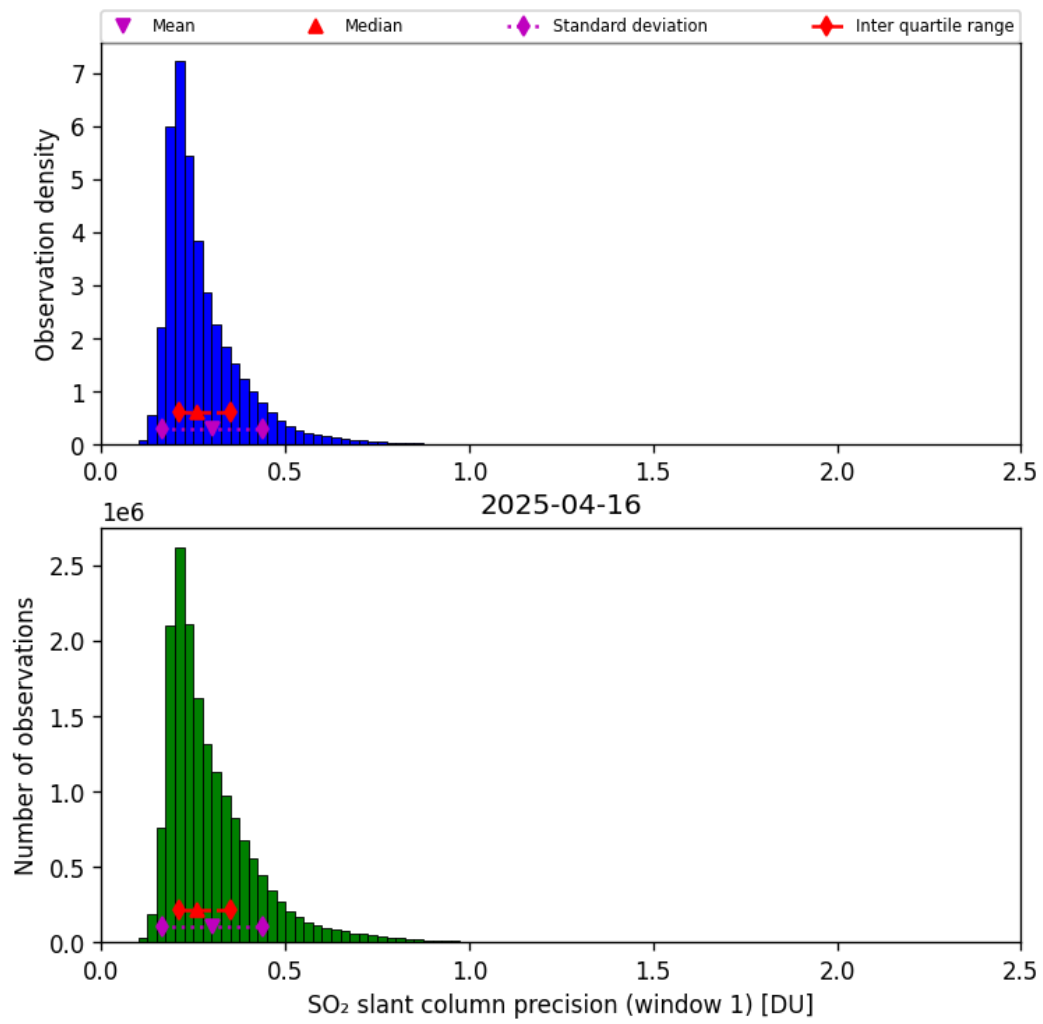
Figure 64: Histogram of “SO 2 slant column precision (window 1)” for 2025-04-16 to 2025-04-16
