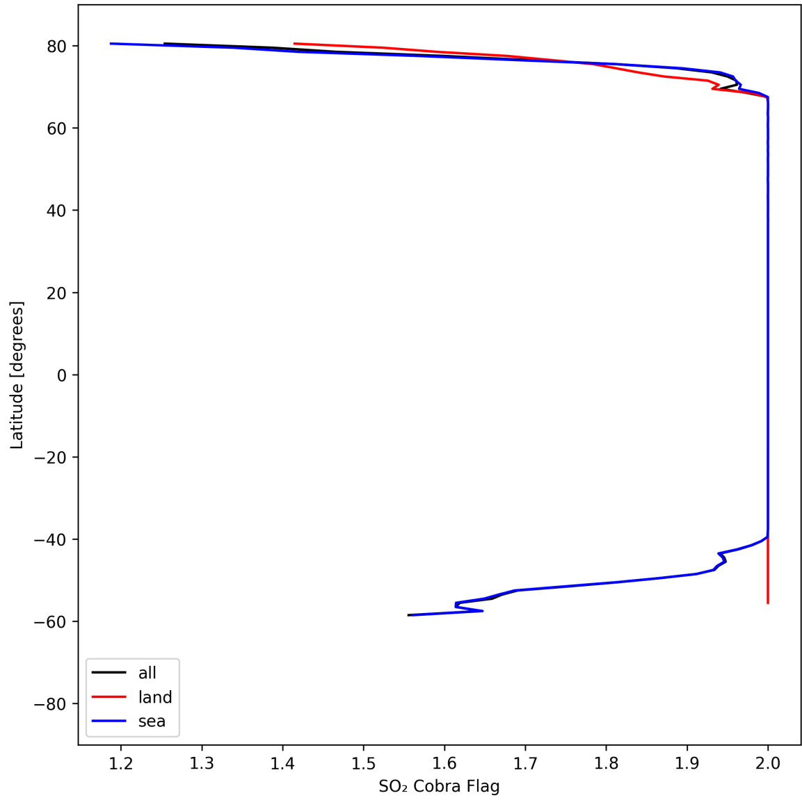
Figure 48: Zonal average of "SO 2 Cobra Flag" for 2025-04-16 to 2025-04-16.
