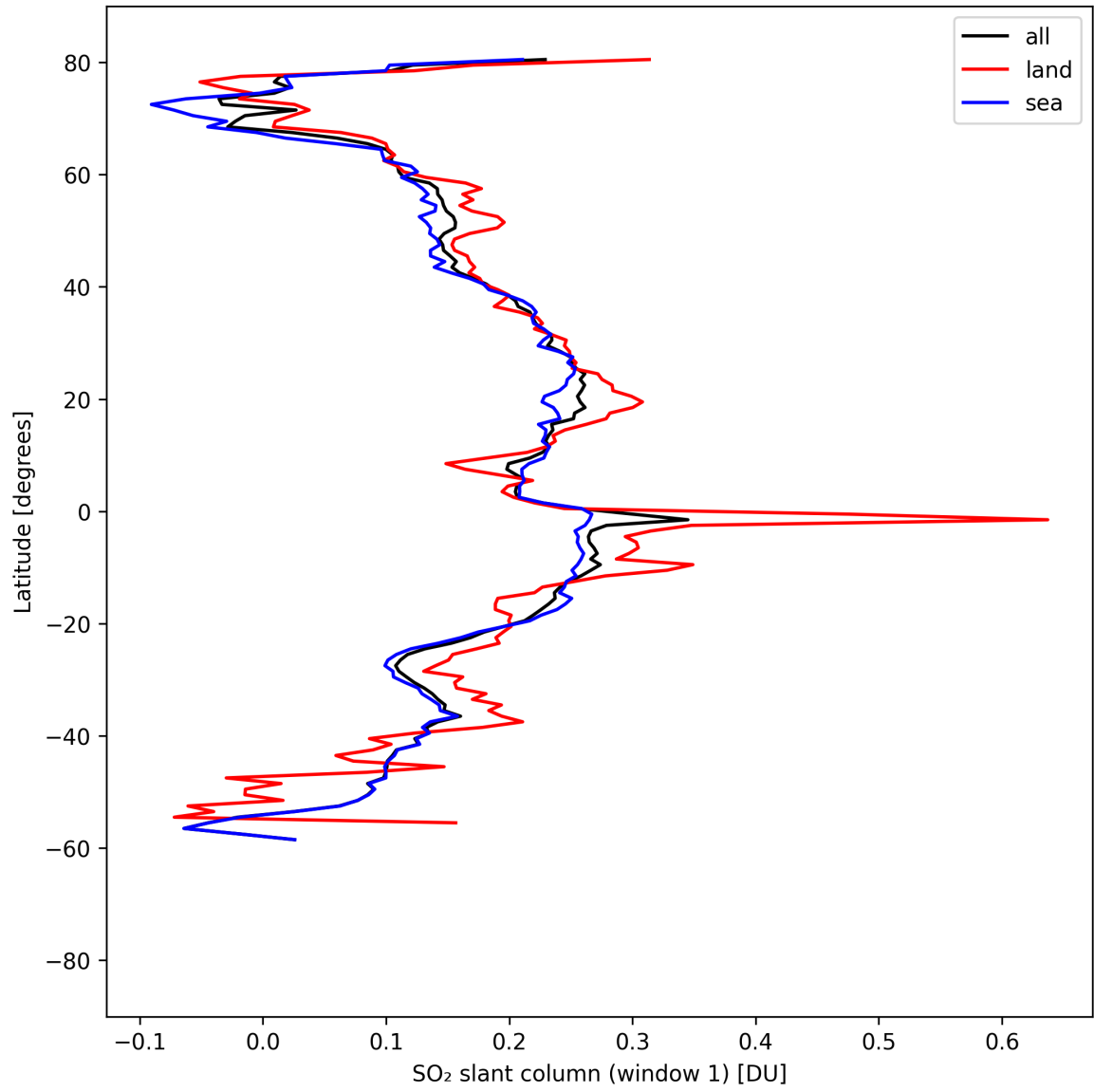
Figure 36: Zonal average of “SO 2 slant column (window 1)” for 2025-04-16 to 2025-04-16.
