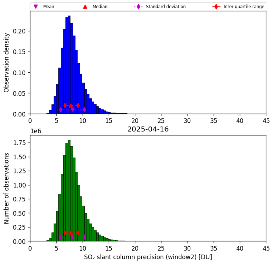
Figure 68: Histogram of “SO 2 slant column precision (window2)” for 2025-04-16 to 2025-04-16
