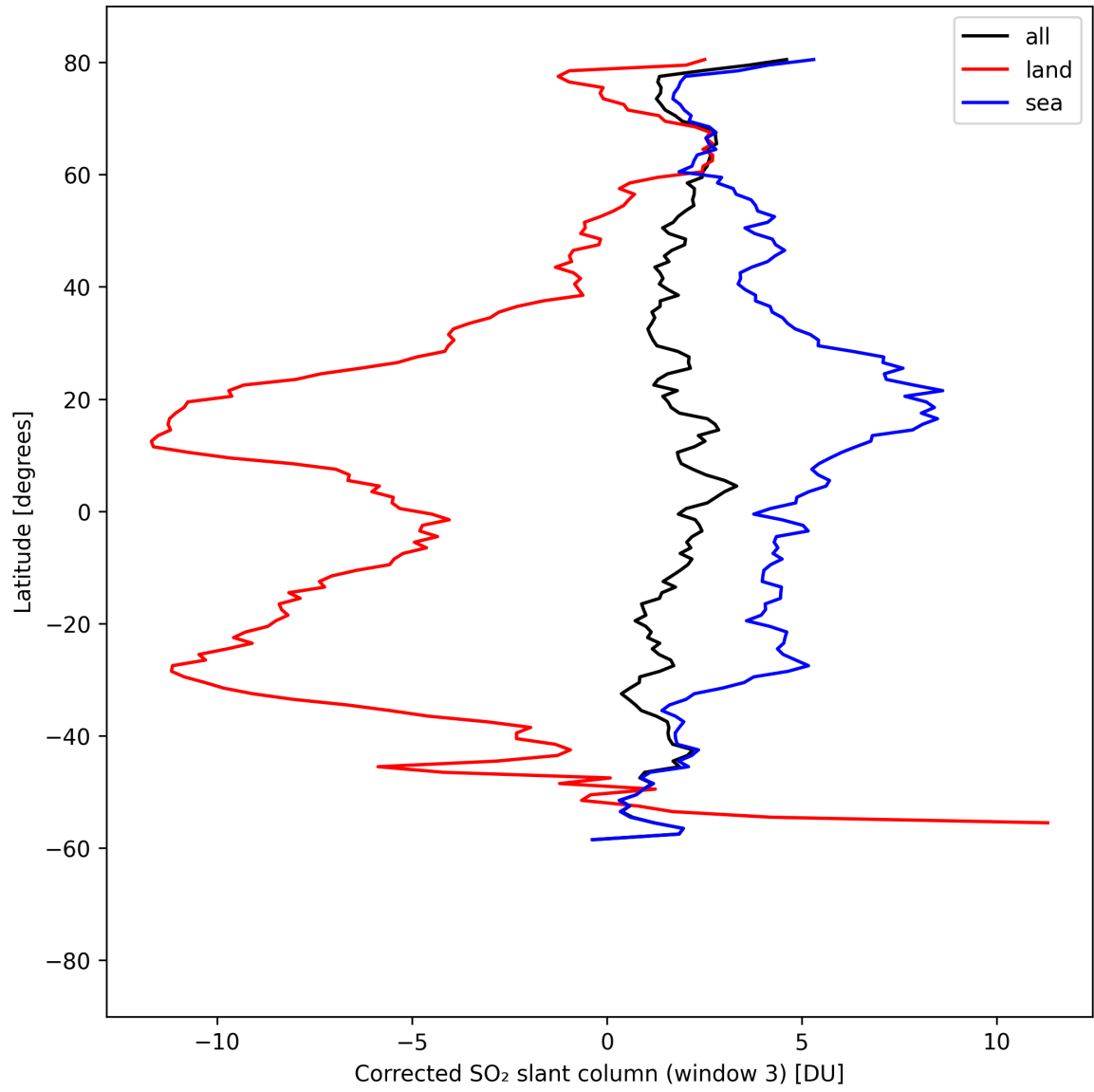
Figure 46: Zonal average of “Corrected SO 2 slant column (window 3)” for 2025-04-16 to 2025-04-16.
