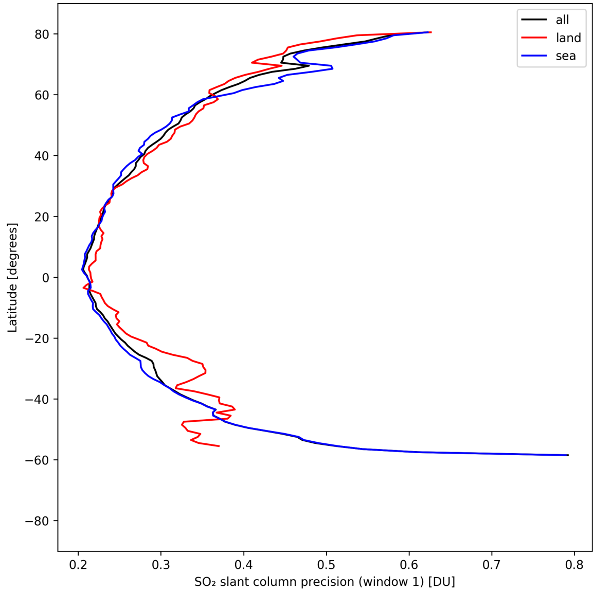
Figure 37: Zonal average of “SO 2 slant column precision (window 1)” for 2025-04-16 to 2025-04-16.
