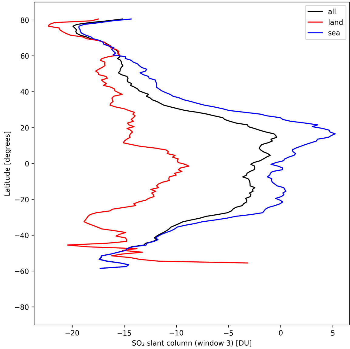
Figure 44: Zonal average of “SO 2 slant column (window 3)” for 2025-04-16 to 2025-04-16.
