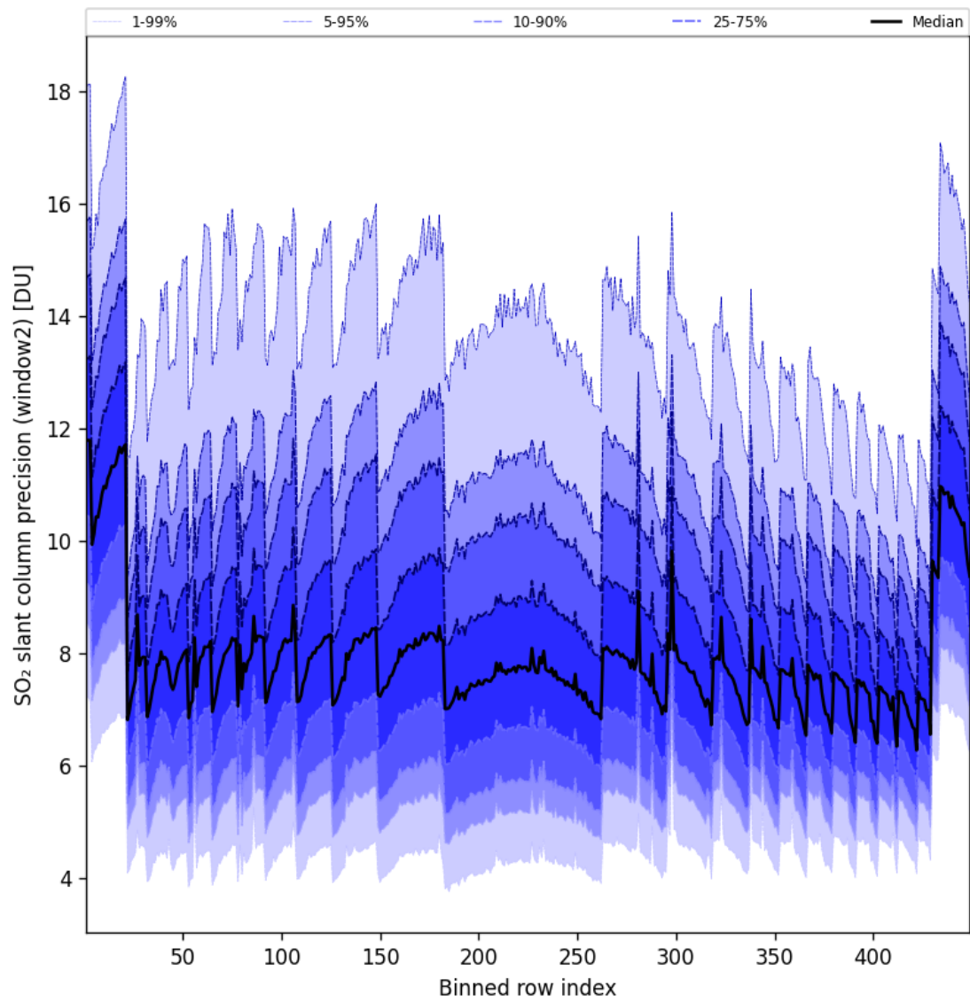
Figure 95: Along track statistics of “SO 2 slant column precision (window2)” for 2025-04-16 to 2025-04-16
