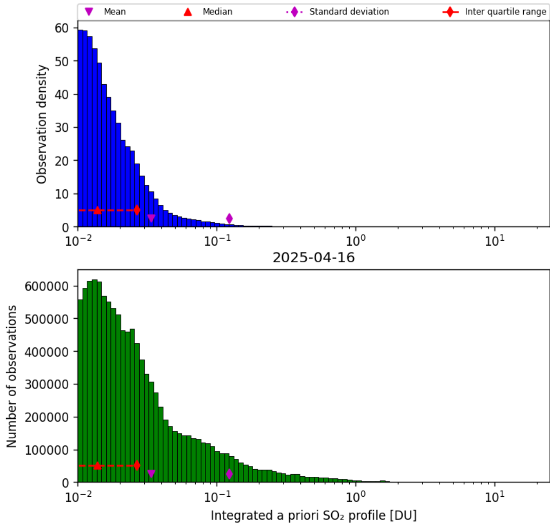
Figure 76: Histogram of “Integrated a priori SO 2 profile” for 2025-04-16 to 2025-04-16
