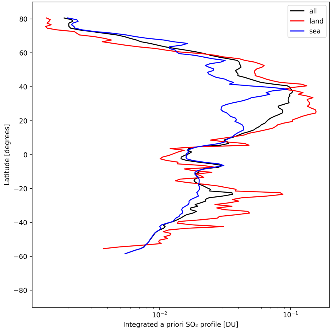
Figure 49: Zonal average of “Integrated a priori SO 2 profile” for 2025-04-16 to 2025-04-16.
