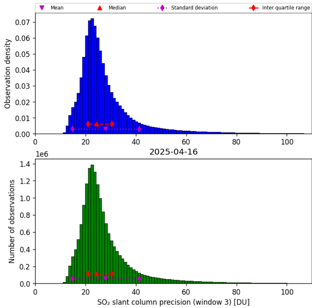
Figure 72: Histogram of “SO 2 slant column precision (window 3)” for 2025-04-16 to 2025-04-16
