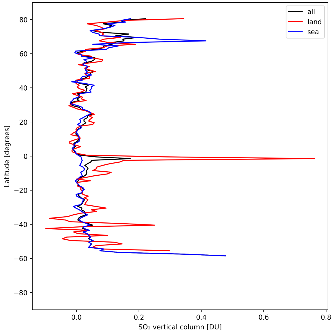
Figure 31: Zonal average of “SO 2 vertical column” for 2025-04-16 to 2025-04-16.
