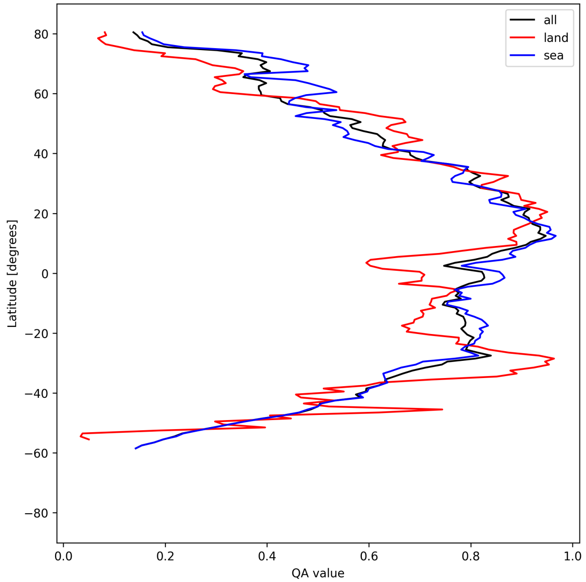
Figure 30: Zonal average of “QA value” for 2025-04-16 to 2025-04-16.
