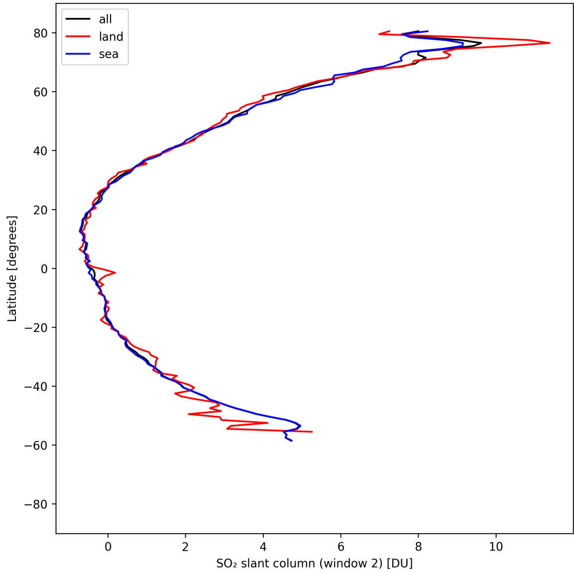
Figure 40: Zonal average of “SO 2 slant column (window 2)” for 2025-04-16 to 2025-04-16.
