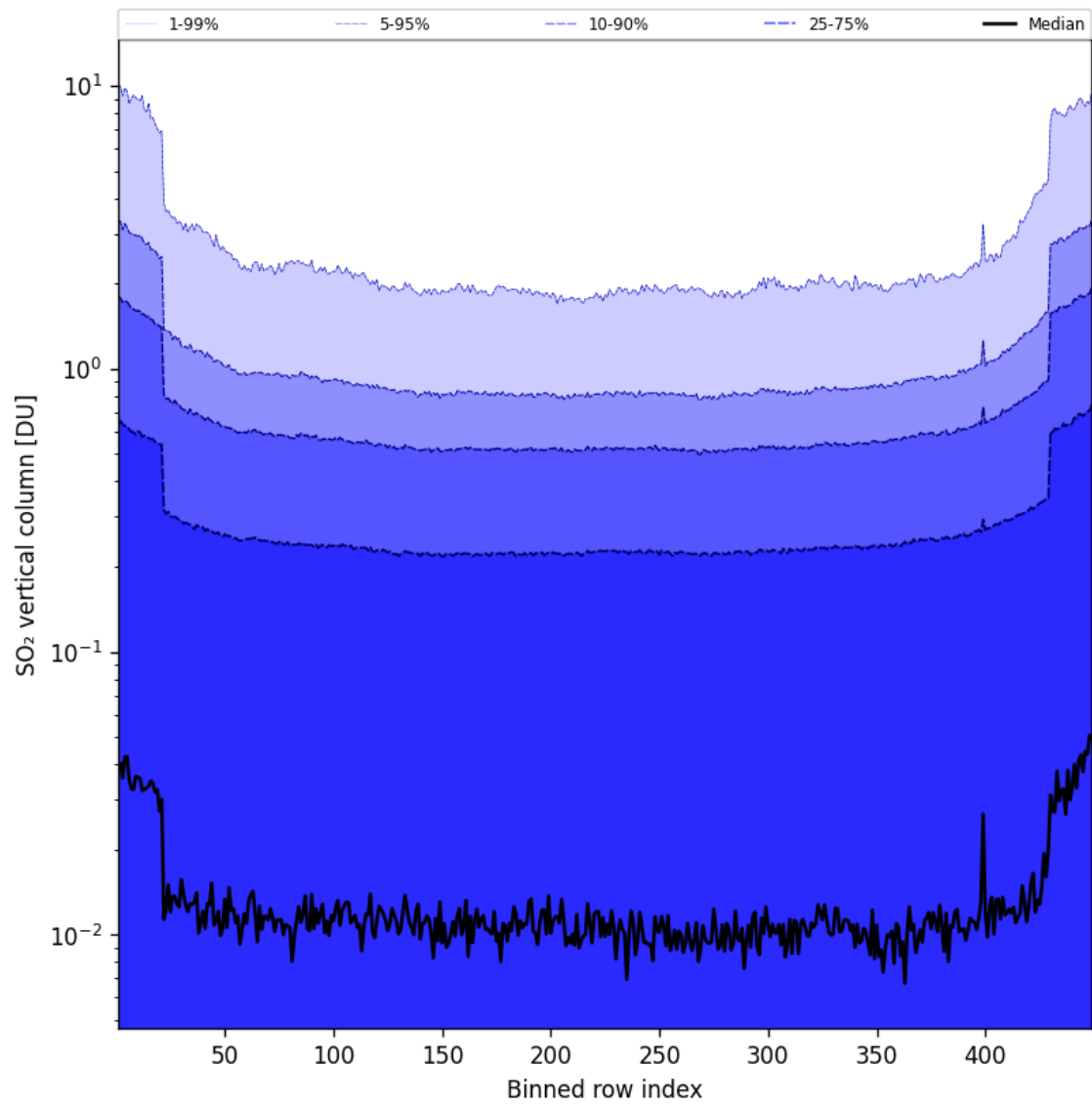
Figure 85: Along track statistics of “SO 2 vertical column” for 2025-04-16 to 2025-04-16
