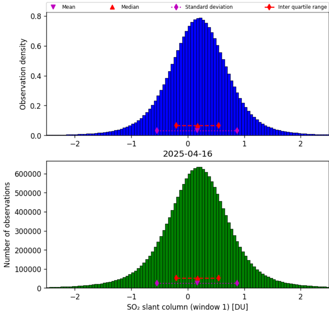
Figure 63: Histogram of “SO 2 slant column (window 1)” for 2025-04-16 to 2025-04-16
