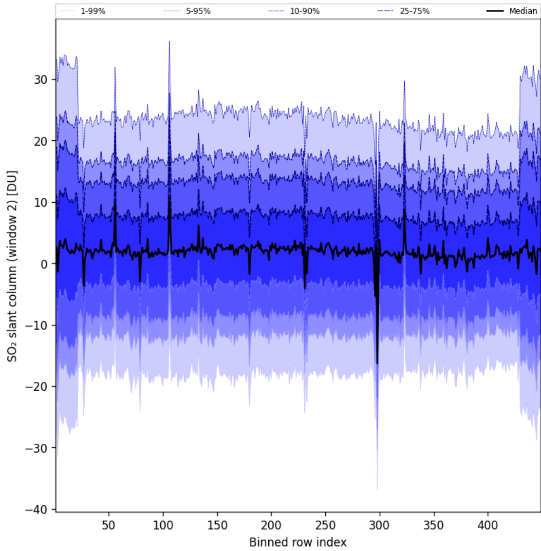
Figure 94: Along track statistics of “SO 2 slant column (window 2)” for 2025-04-16 to 2025-04-16
