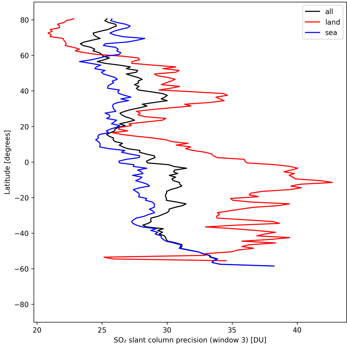
Figure 45: Zonal average of “SO 2 slant column precision (window 3)” for 2025-04-16 to 2025-04-16.
