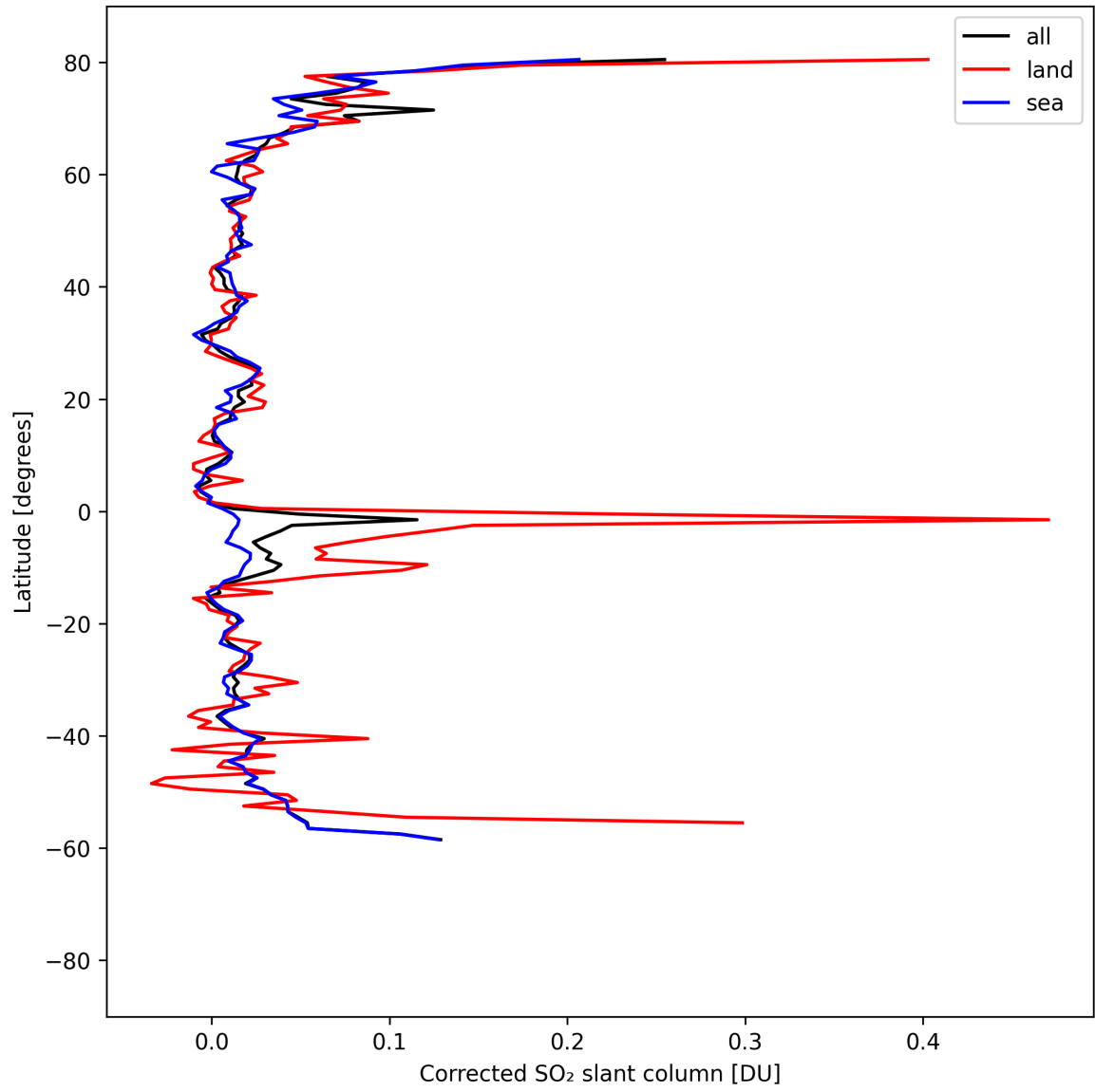
Figure 33: Zonal average of “Corrected SO 2 slant column” for 2025-04-16 to 2025-04-16.
