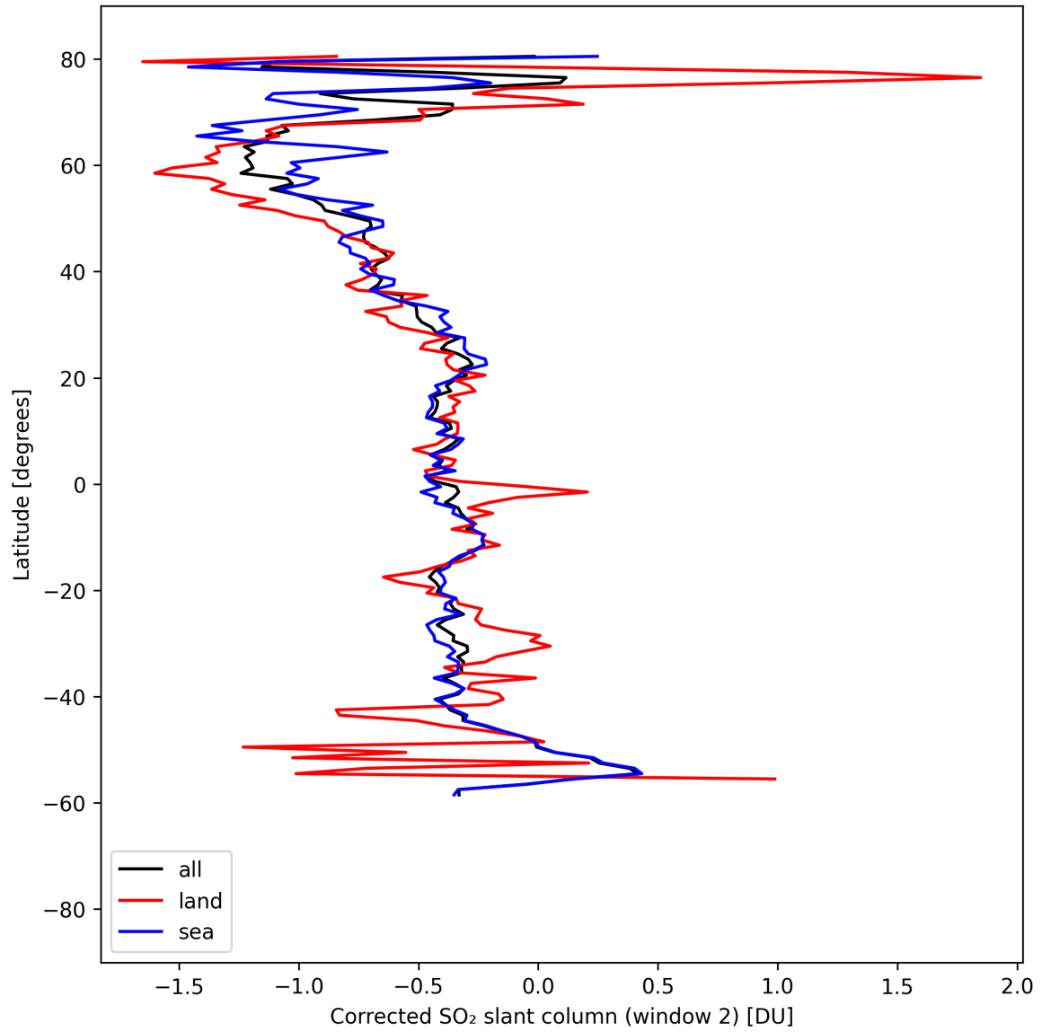
Figure 42: Zonal average of “Corrected SO 2 slant column (window 2)” for 2025-04-16 to 2025-04-16.
