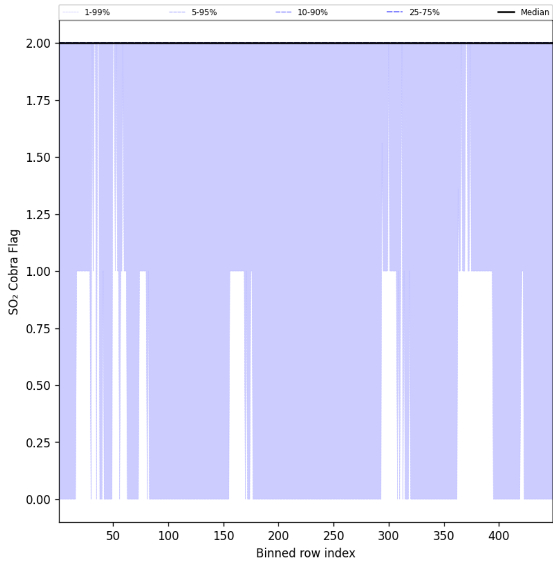
Figure 102: Along track statistics of “SO 2 Cobra Flag” for 2025-04-16 to 2025-04-16
