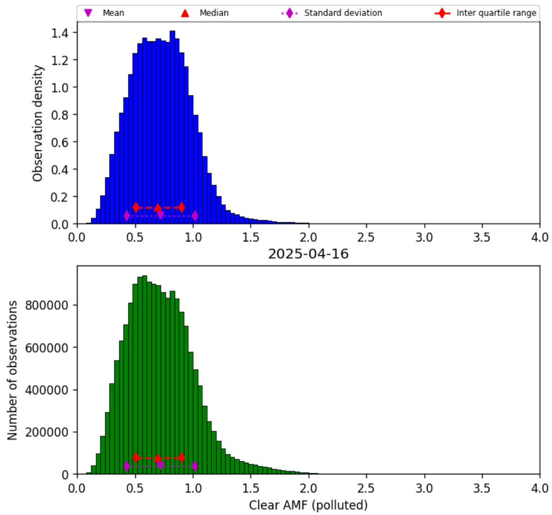
Figure 82: Histogram of “Clear AMF (polluted)” for 2025-04-16 to 2025-04-16
