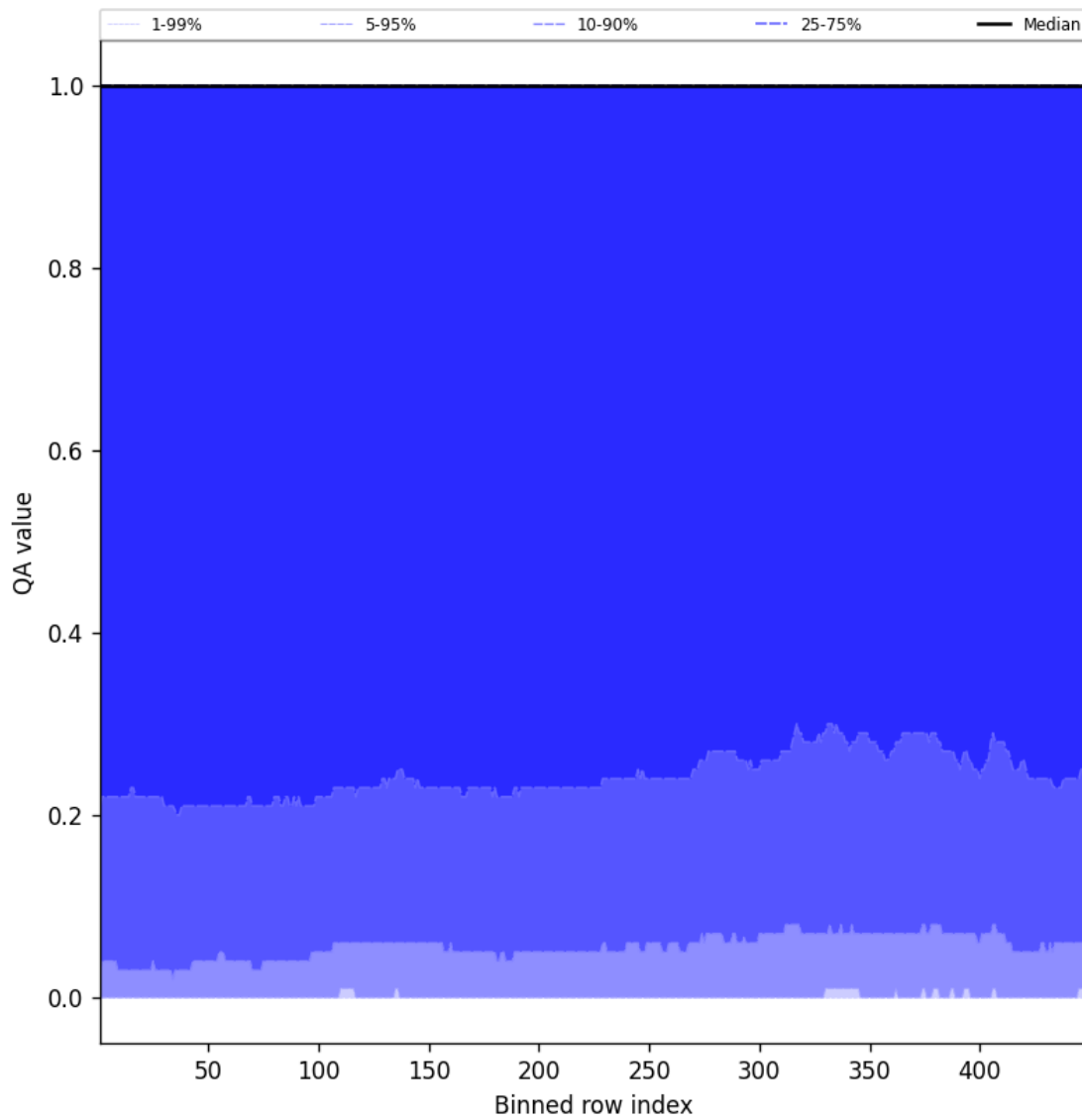
Figure 84: Along track statistics of “QA value” for 2025-04-16 to 2025-04-16
