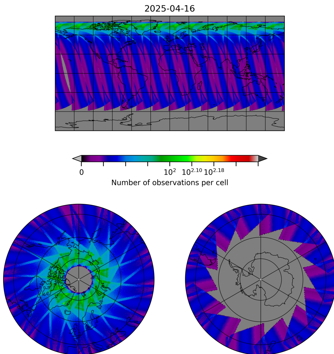
Figure 29: Map of the number of observations for 2025-04-16 to 2025-04-16
