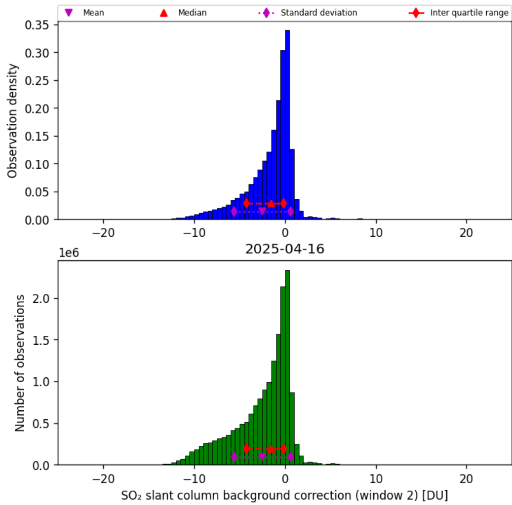
Figure 70: Histogram of “SO 2 slant column background correction (window 2)” for 2025-04-16 to 2025-04-16
