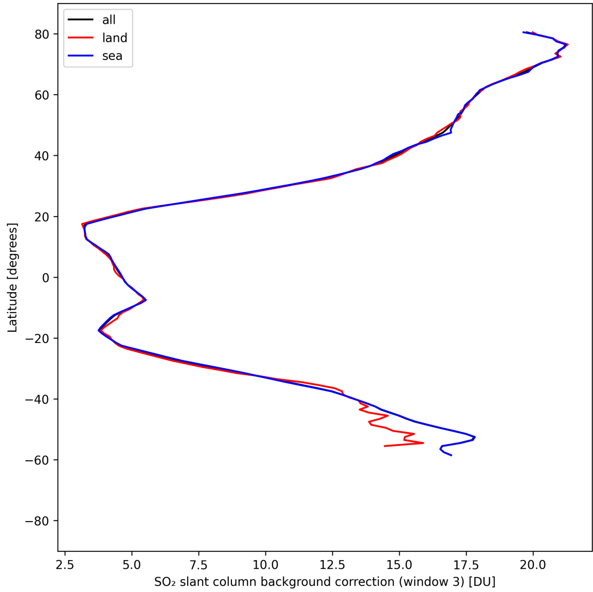
Figure 47: Zonal average of “SO 2 slant column background correction (window 3)” for 2025-04-16 to 2025-04-16.
