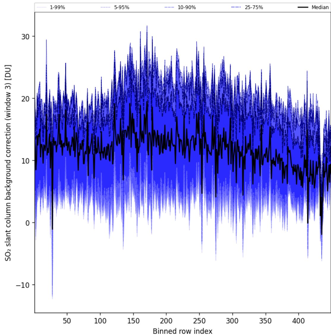
Figure 101: Along track statistics of “SO 2 slant column background correction (window 3)” for 2025-04-16 to 2025-04-16
