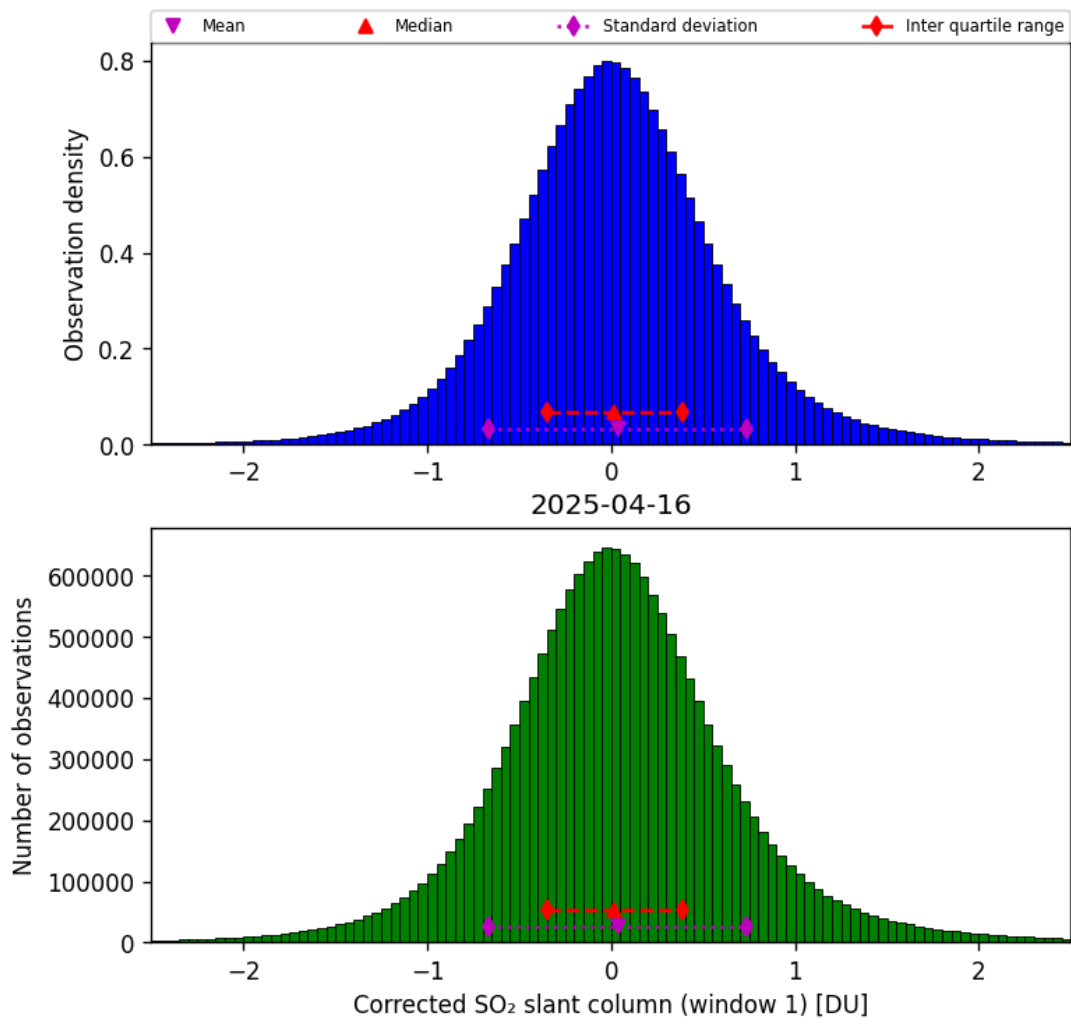
Figure 65: Histogram of “Corrected SO 2 slant column (window 1)” for 2025-04-16 to 2025-04-16
