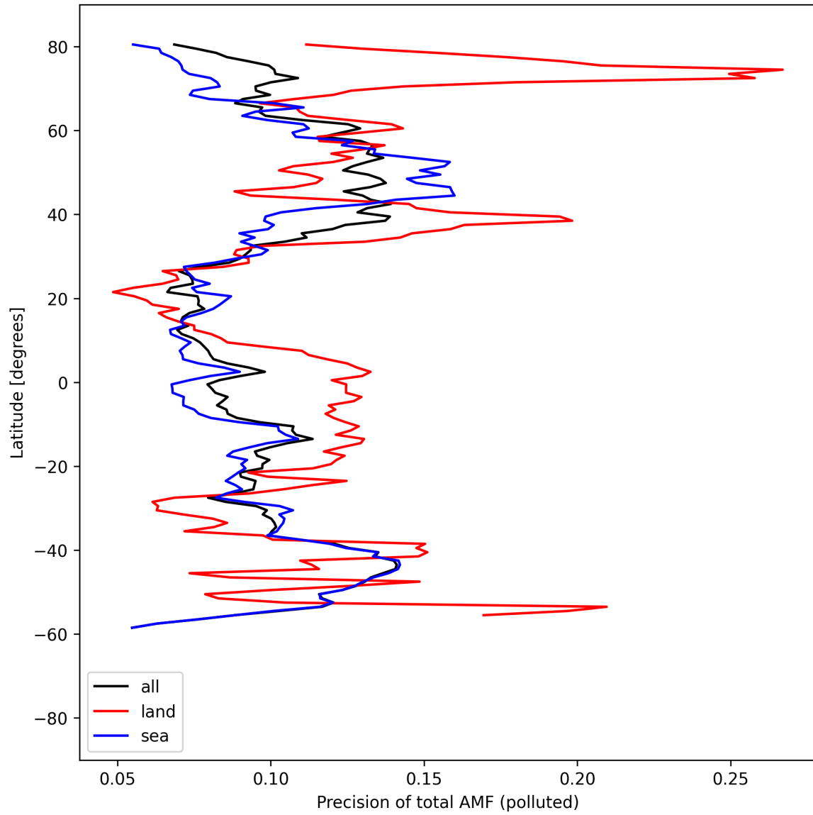
Figure 54: Zonal average of “Precision of total AMF (polluted)” for 2025-04-16 to 2025-04-16.
