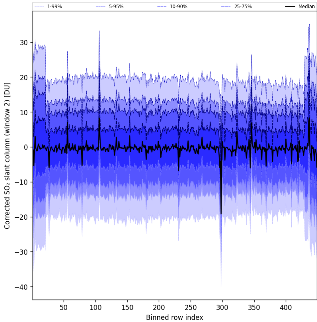
Figure 96: Along track statistics of “Corrected SO 2 slant column (window 2)” for 2025-04-16 to 2025-04-16
