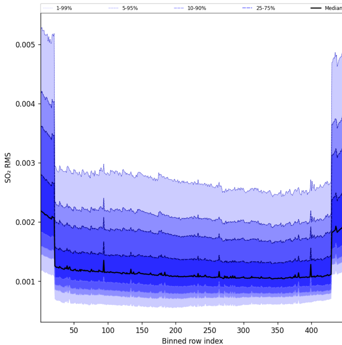
Figure 106: Along track statistics of “SO 2 RMS” for 2025-04-16 to 2025-04-16
