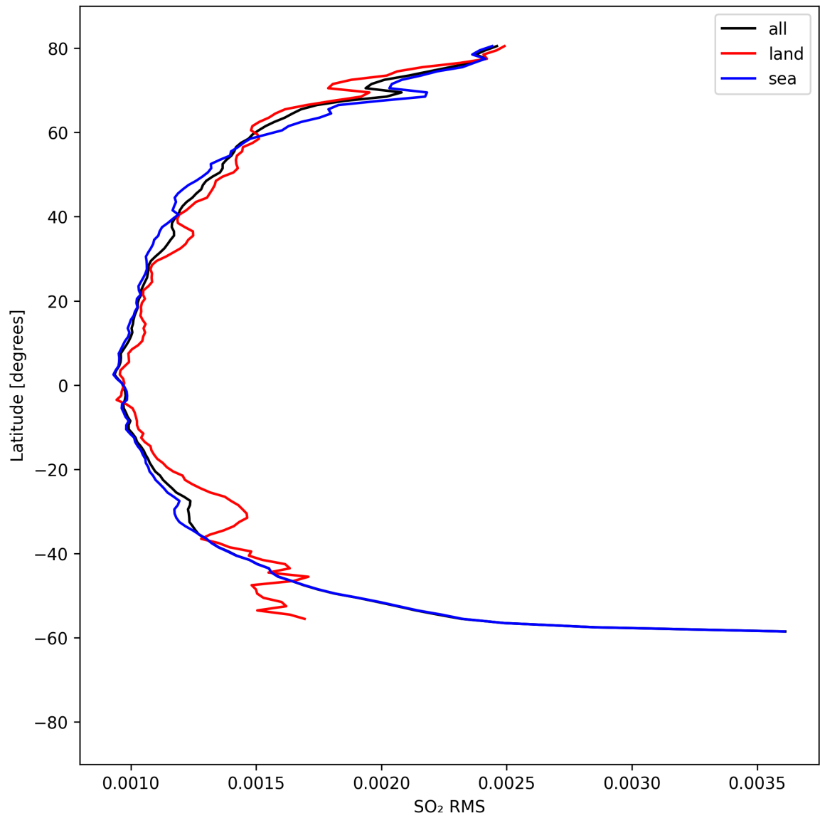
Figure 52: Zonal average of “SO 2 RMS” for 2025-04-16 to 2025-04-16.
