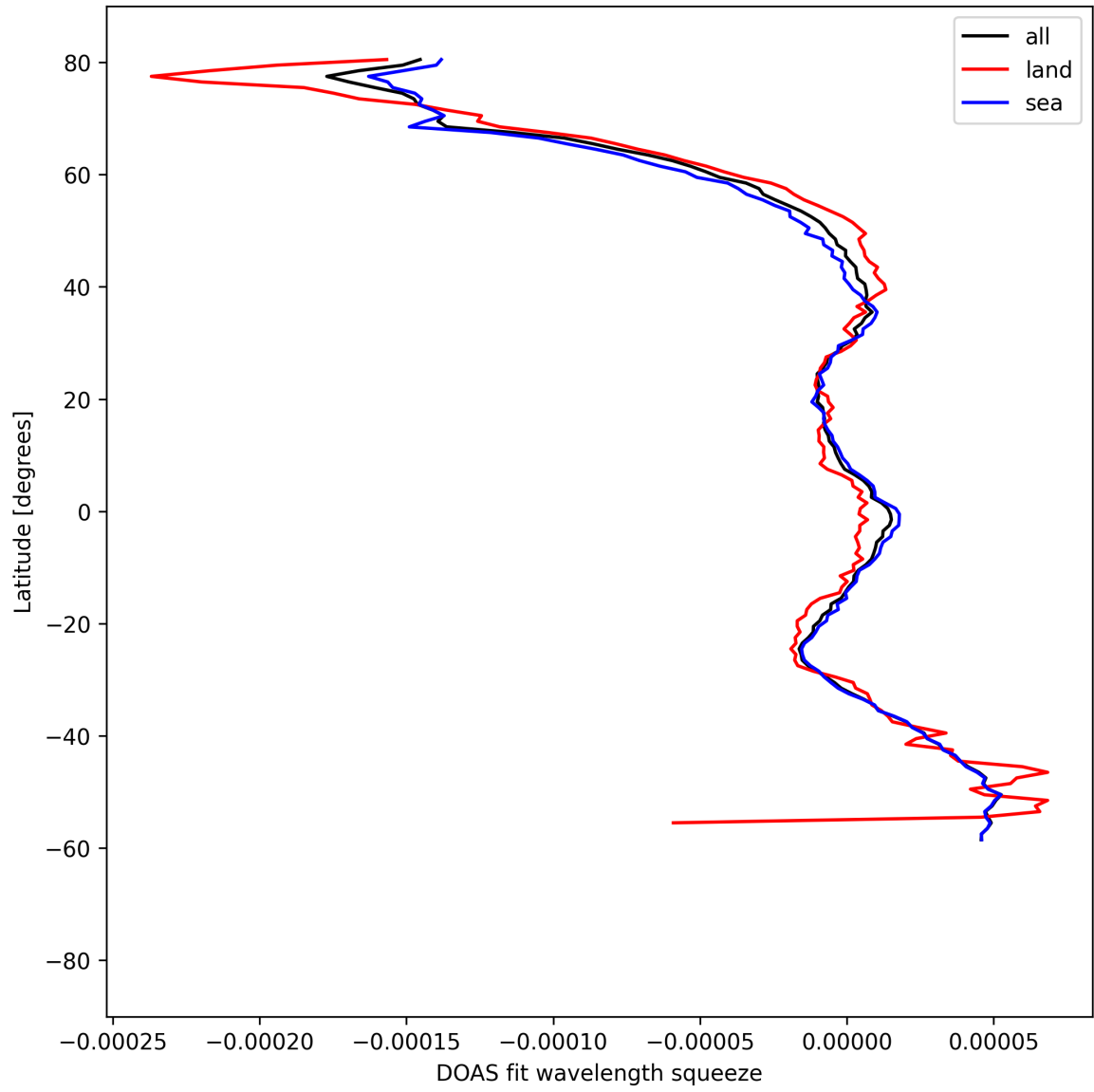
Figure 51: Zonal average of “DOAS fit wavelength squeeze” for 2025-04-16 to 2025-04-16.
