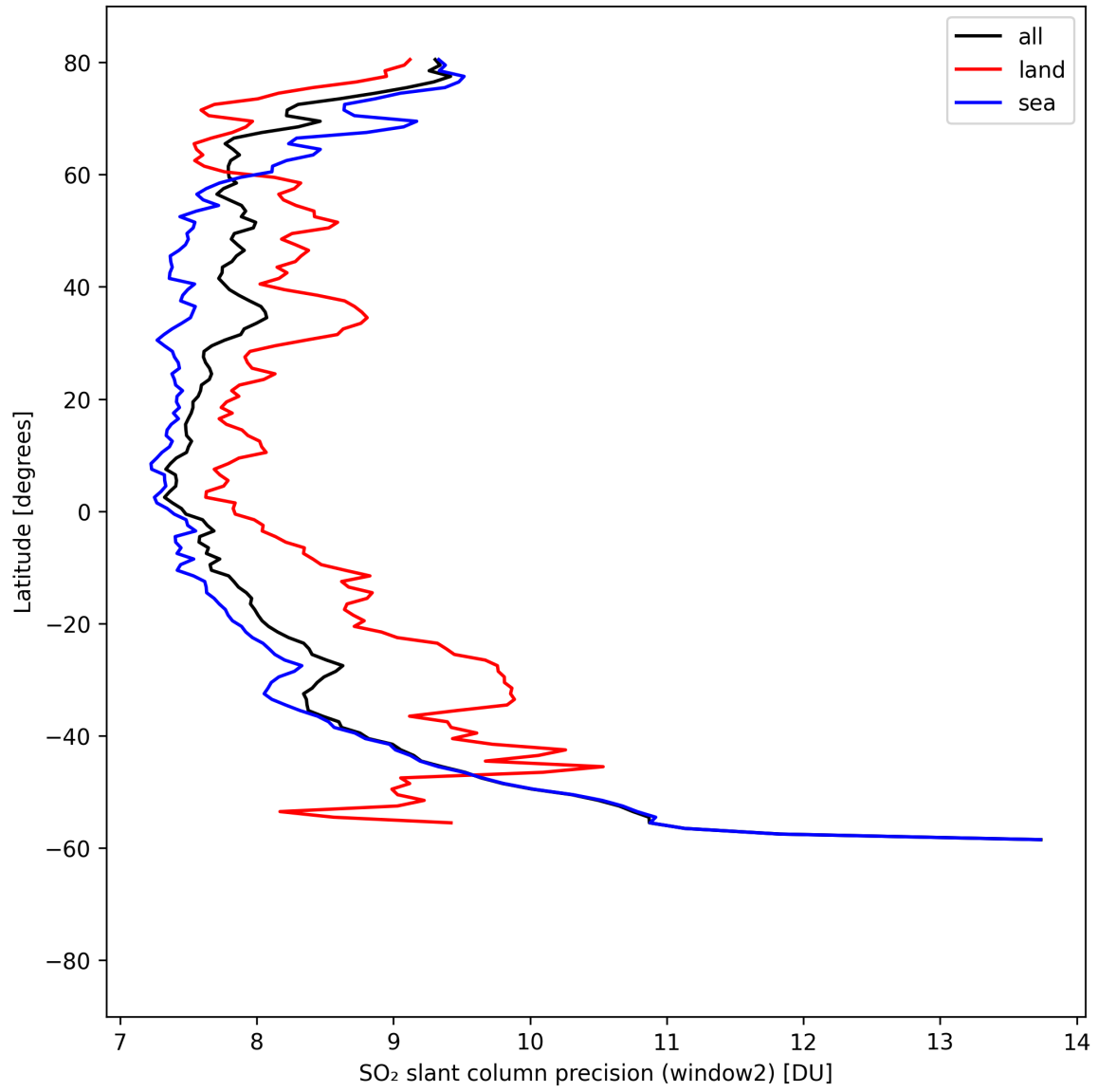
Figure 41: Zonal average of “SO 2 slant column precision (window2)” for 2025-04-16 to 2025-04-16.
