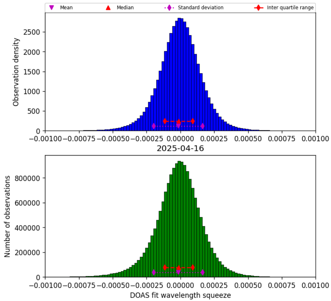
Figure 78: Histogram of “DOAS fit wavelength squeeze” for 2025-04-16 to 2025-04-16
