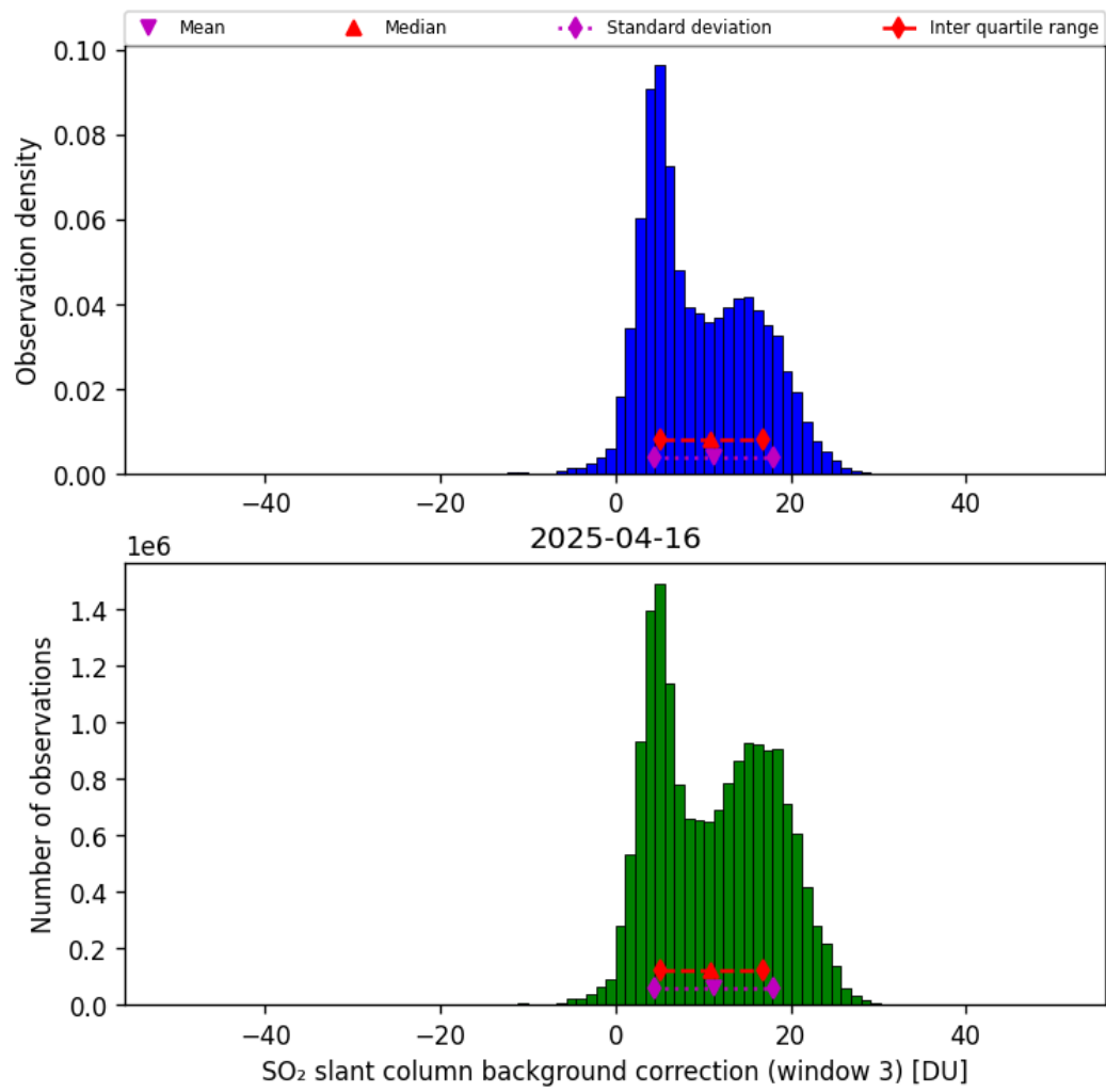
Figure 74: Histogram of “SO 2 slant column background correction (window 3)” for 2025-04-16 to 2025-04-16
