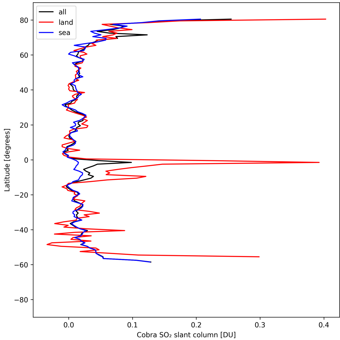
Figure 34: Zonal average of “Cobra SO 2 slant column” for 2025-04-16 to 2025-04-16.
