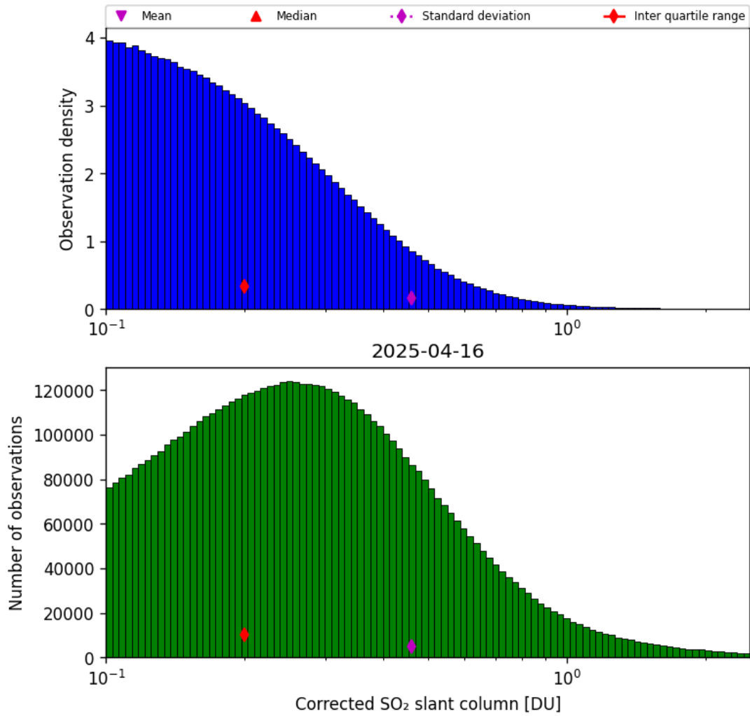
Figure 60: Histogram of “Corrected SO 2 slant column” for 2025-04-16 to 2025-04-16
