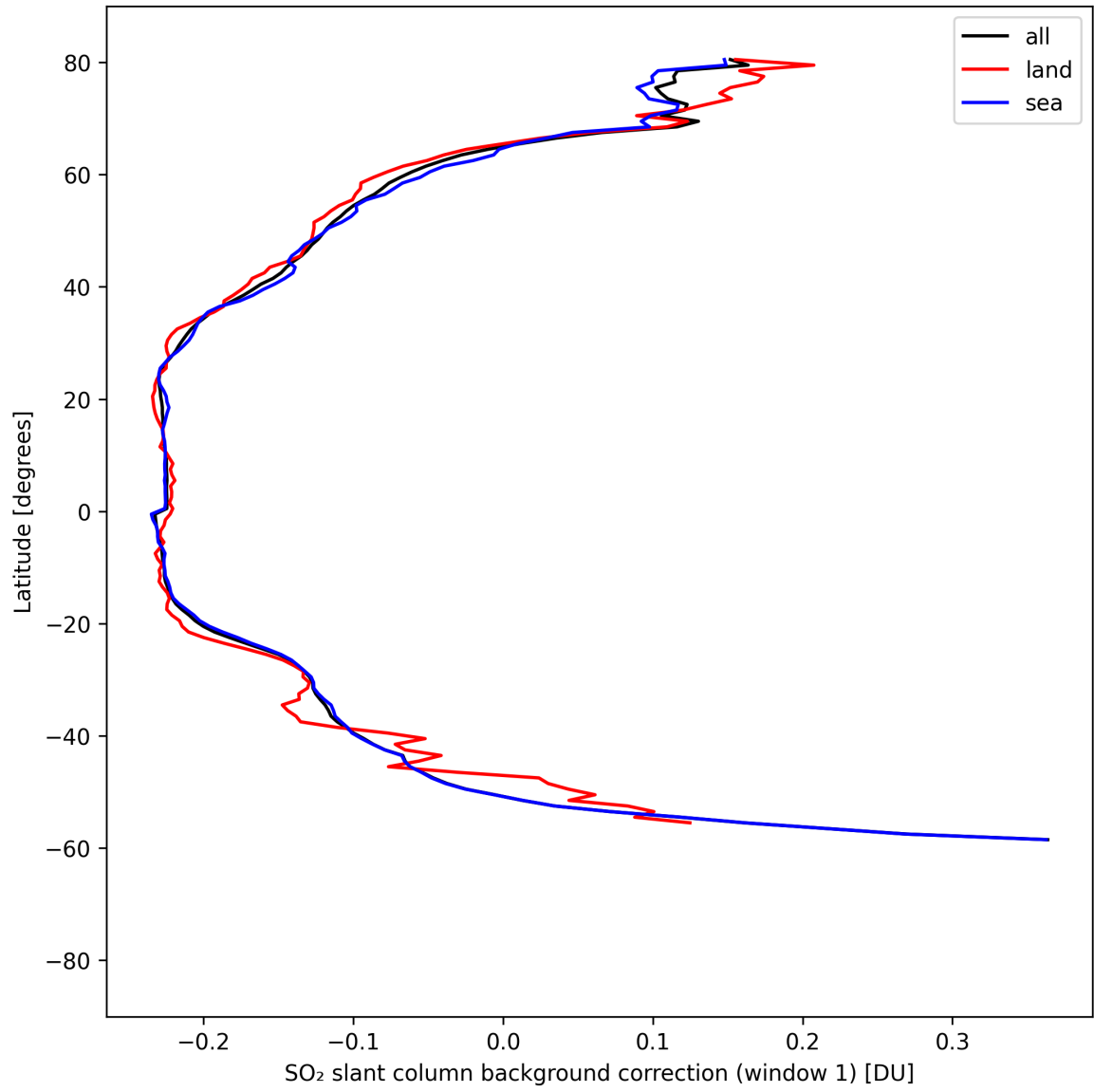
Figure 39: Zonal average of "SO 2 slant column background correction (window 1)" for 2025-04-16 to 2025-04-16.
