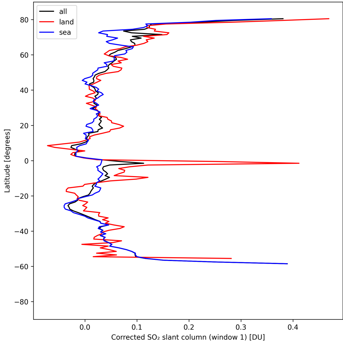
Figure 38: Zonal average of “Corrected SO 2 slant column (window 1)” for 2025-04-16 to 2025-04-16.
