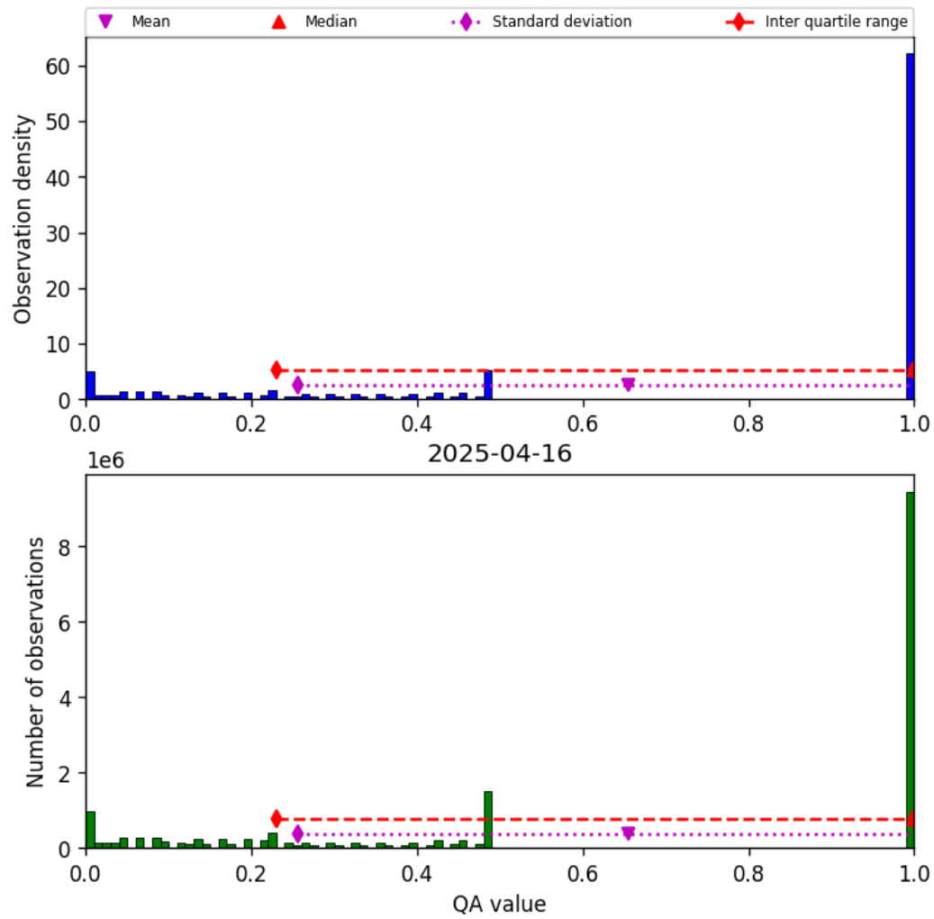
Figure 57: Histogram of “QA value” for 2025-04-16 to 2025-04-16
