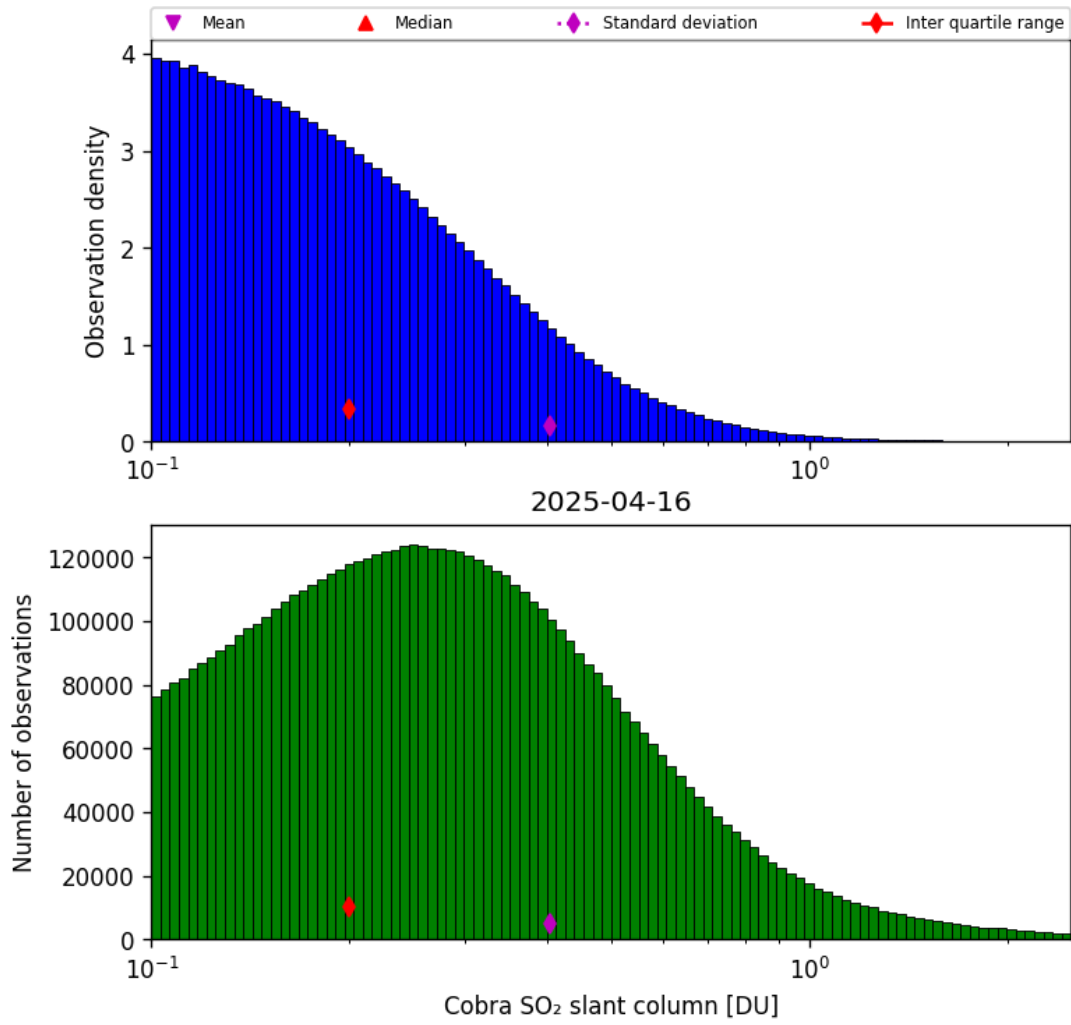
Figure 61: Histogram of “Cobra SO 2 slant column” for 2025-04-16 to 2025-04-16
