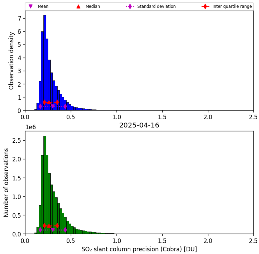
Figure 62: Histogram of “SO 2 slant column precision (Cobra)” for 2025-04-16 to 2025-04-16
