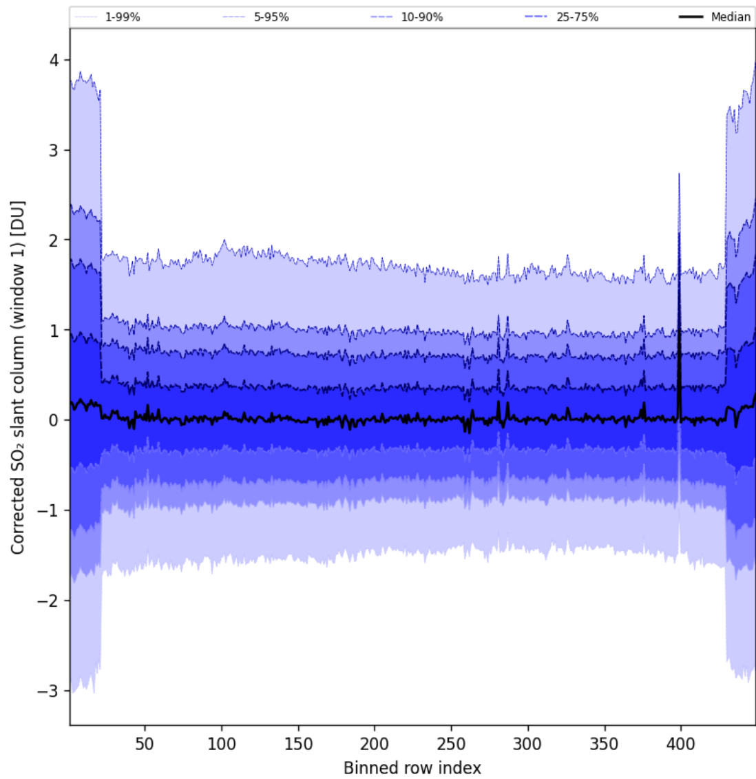
Figure 92: Along track statistics of “Corrected SO 2 slant column (window 1)” for 2025-04-16 to 2025-04-16
