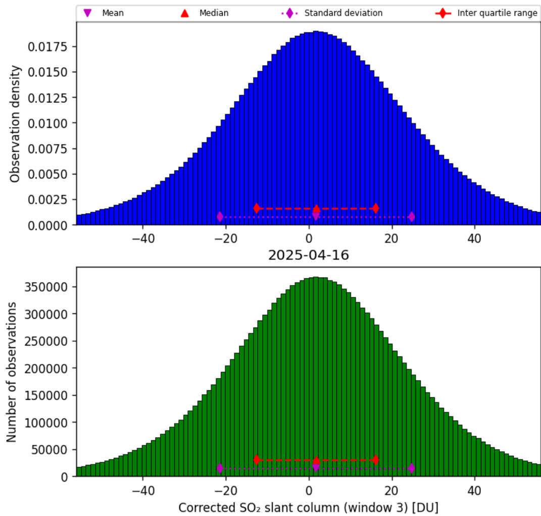
Figure 73: Histogram of “Corrected SO 2 slant column (window 3)” for 2025-04-16 to 2025-04-16
