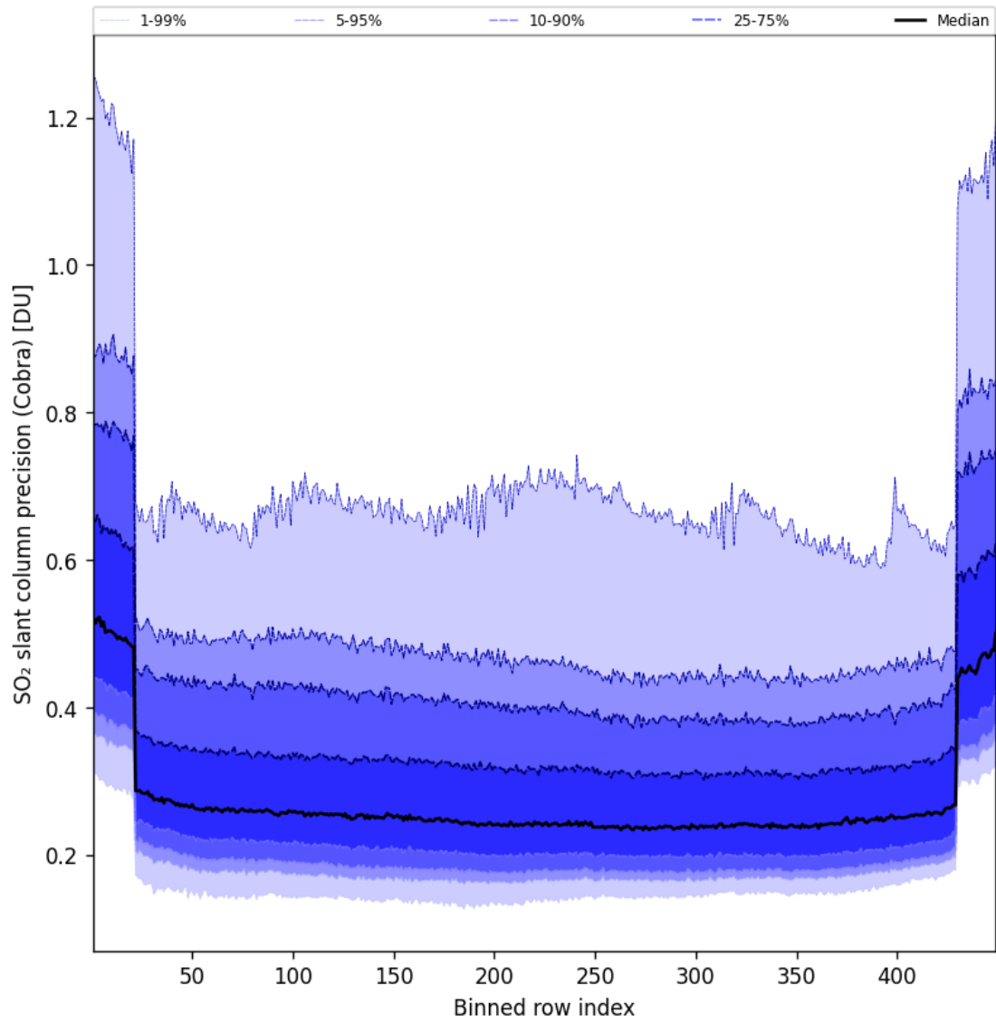
Figure 89: Along track statistics of “SO 2 slant column precision (Cobra)” for 2025-04-16 to 2025-04-16
