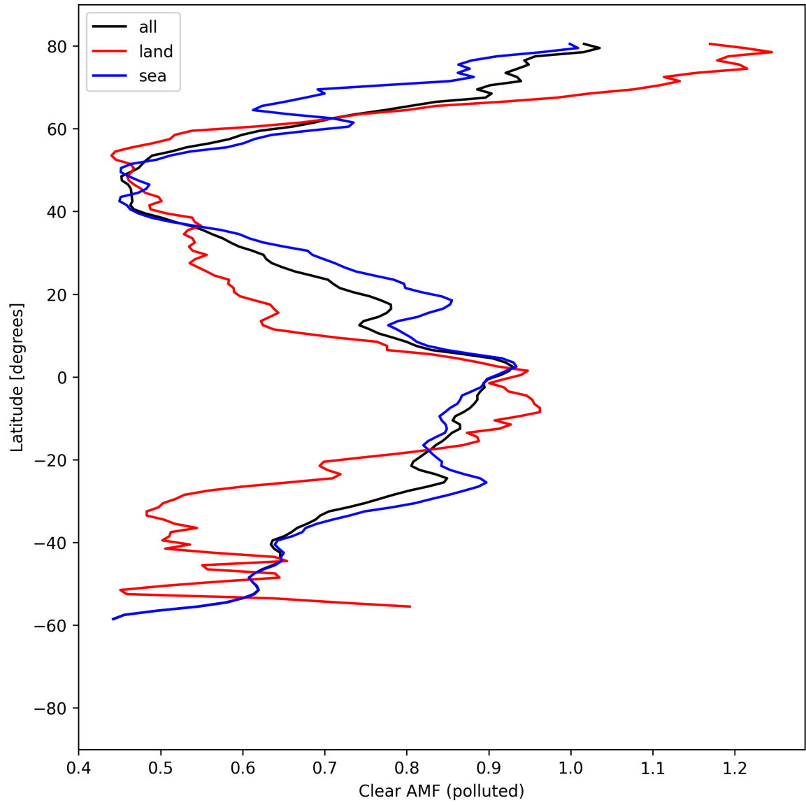
Figure 55: Zonal average of “Clear AMF (polluted)” for 2025-04-16 to 2025-04-16.
