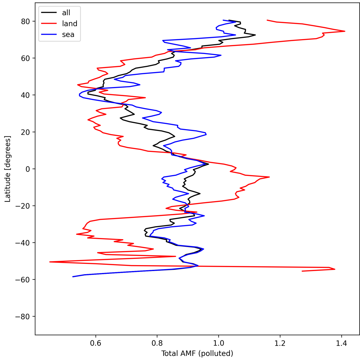
Figure 53: Zonal average of “Total AMF (polluted)” for 2025-04-16 to 2025-04-16.
