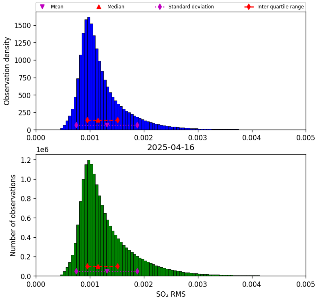
Figure 79: Histogram of “SO 2 RMS” for 2025-04-16 to 2025-04-16
