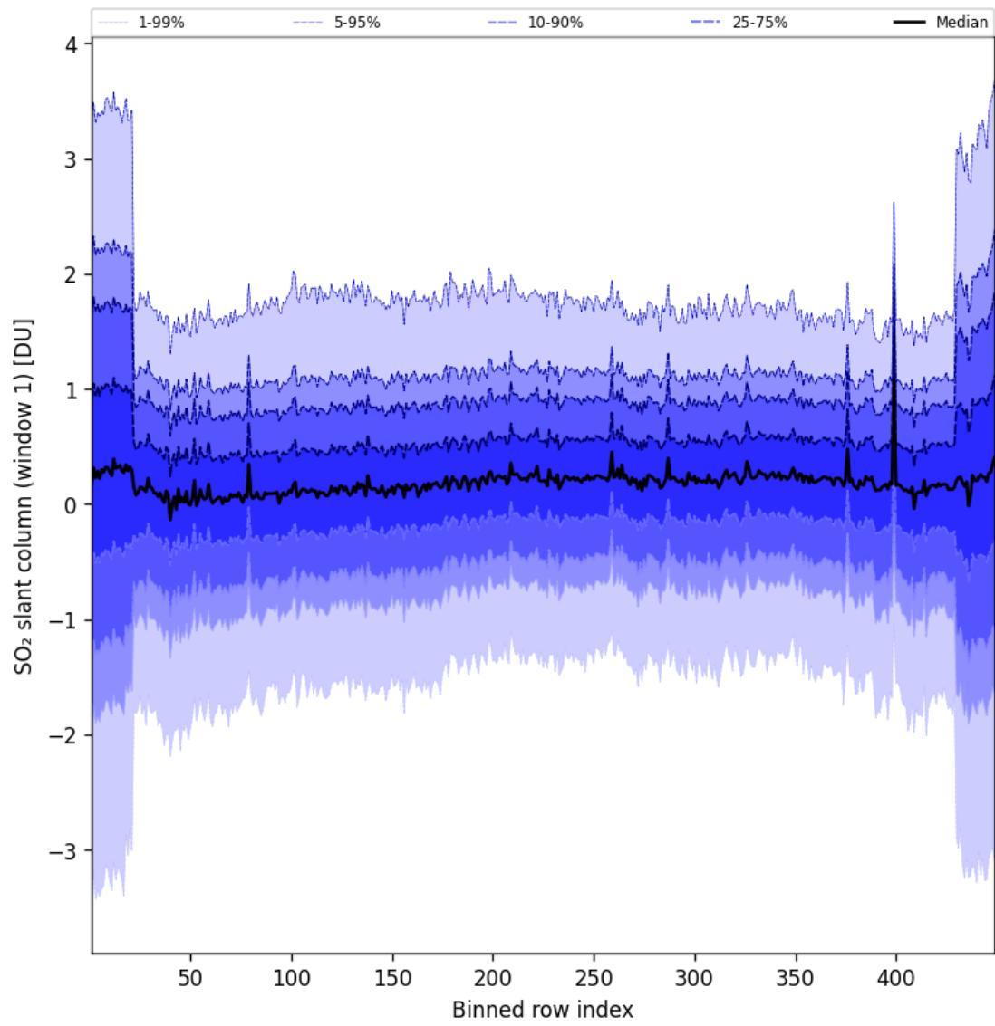
Figure 90: Along track statistics of “SO 2 slant column (window 1)” for 2025-04-16 to 2025-04-16
