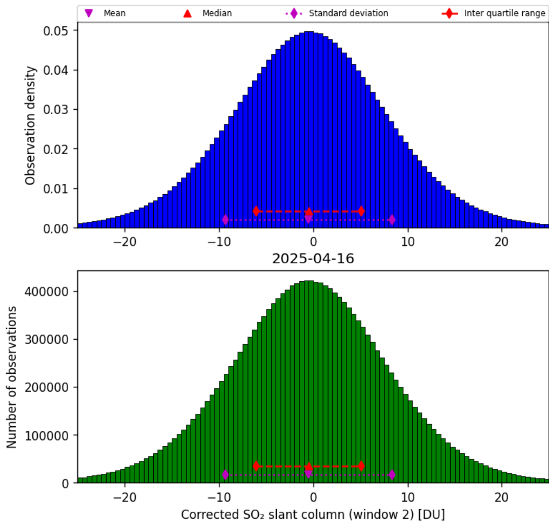
Figure 69: Histogram of “Corrected SO 2 slant column (window 2)” for 2025-04-16 to 2025-04-16
