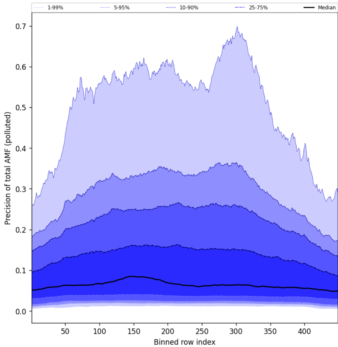
Figure 108: Along track statistics of “Precision of total AMF (polluted)” for 2025-04-16 to 2025-04-16
