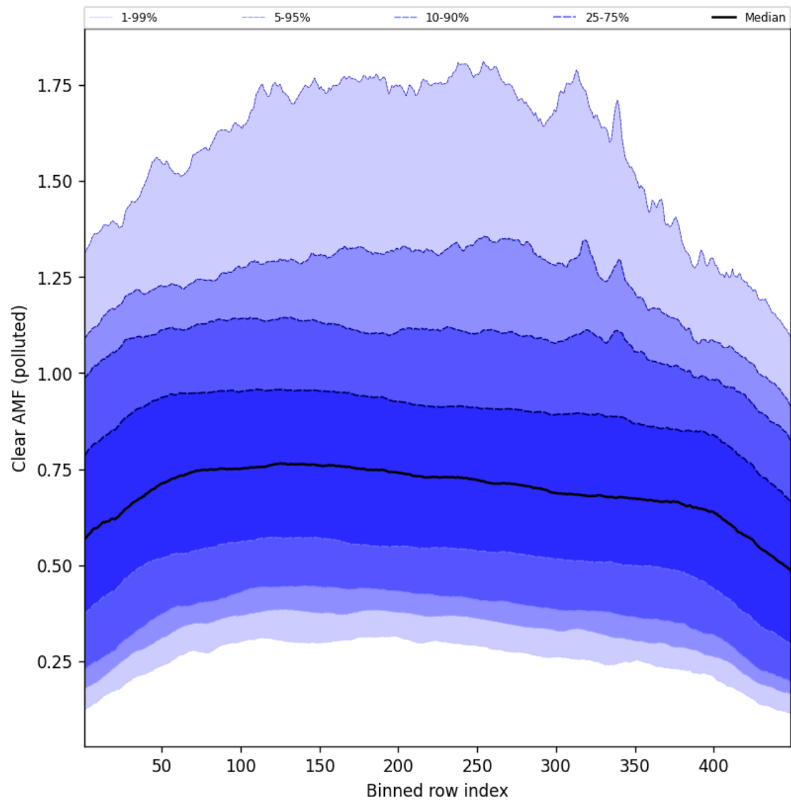
Figure 109: Along track statistics of “Clear AMF (polluted)” for 2025-04-16 to 2025-04-16
