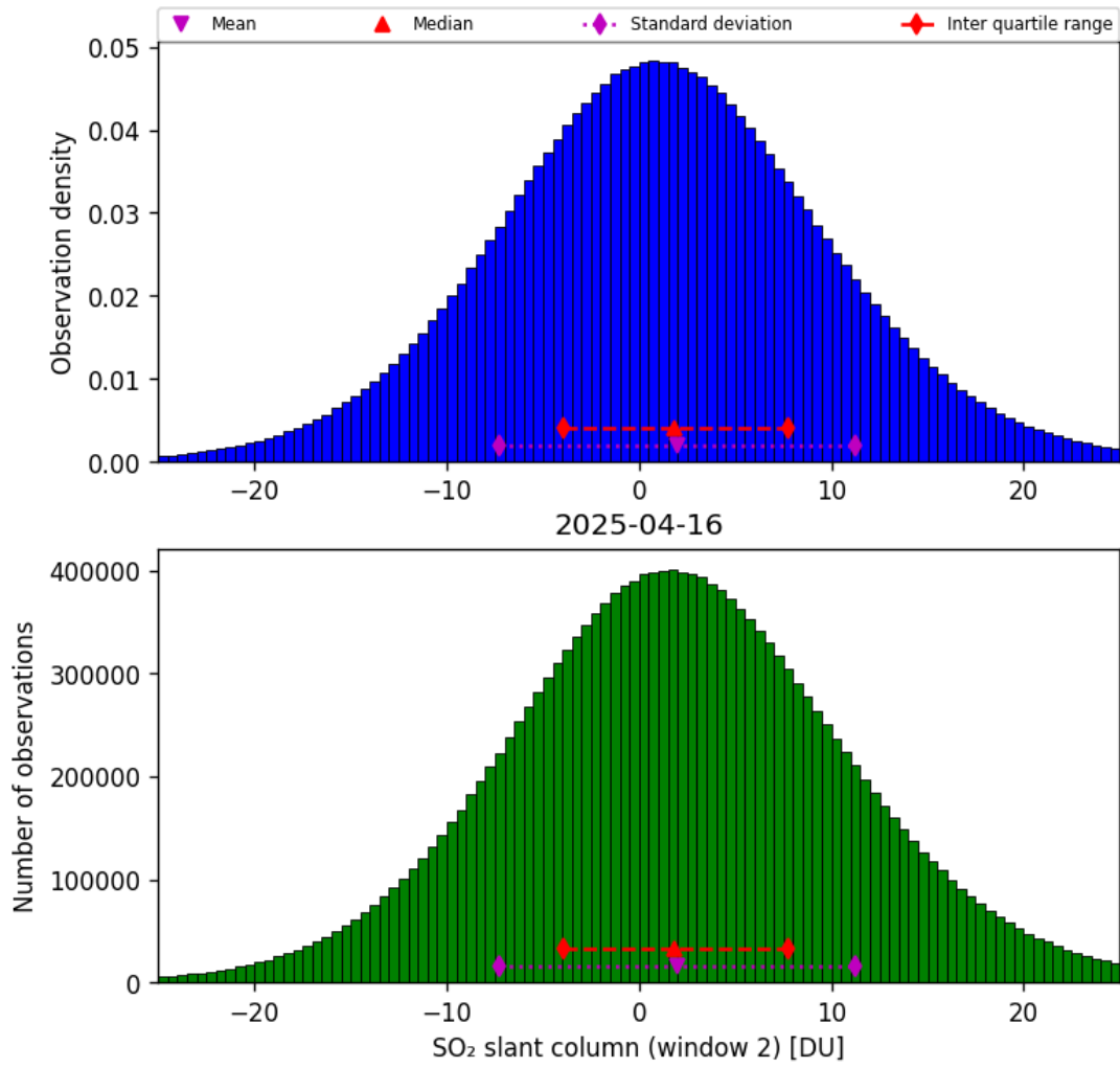
Figure 67: Histogram of “SO 2 slant column (window 2)” for 2025-04-16 to 2025-04-16
