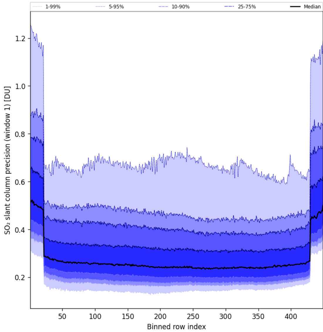
Figure 91: Along track statistics of “SO 2 slant column precision (window 1)” for 2025-04-16 to 2025-04-16
