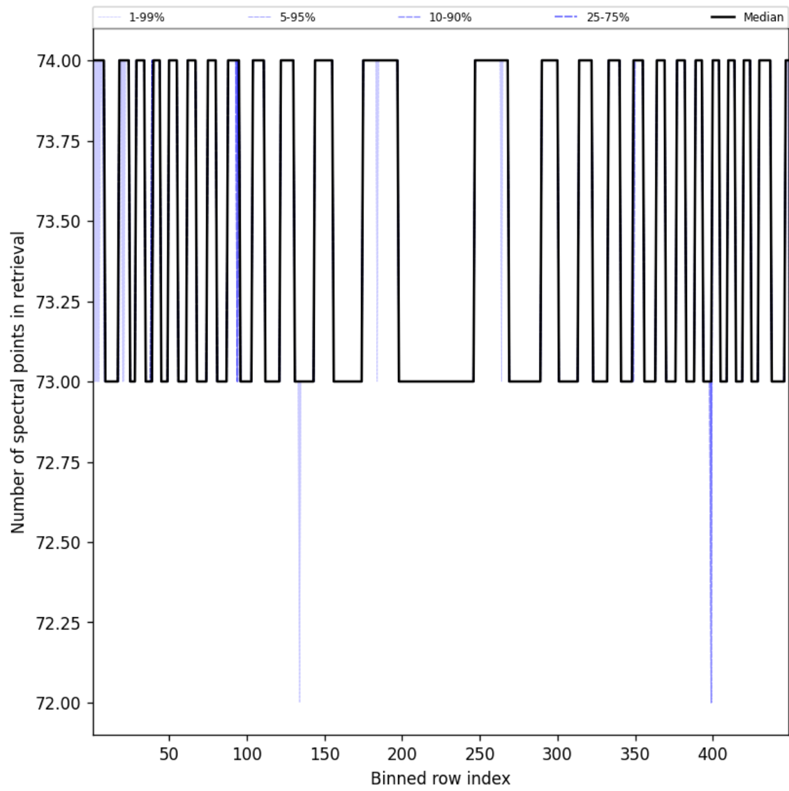
Figure 110: Along track statistics of “Number of spectral points in retrieval” for 2025-04-16 to 2025-04-16
