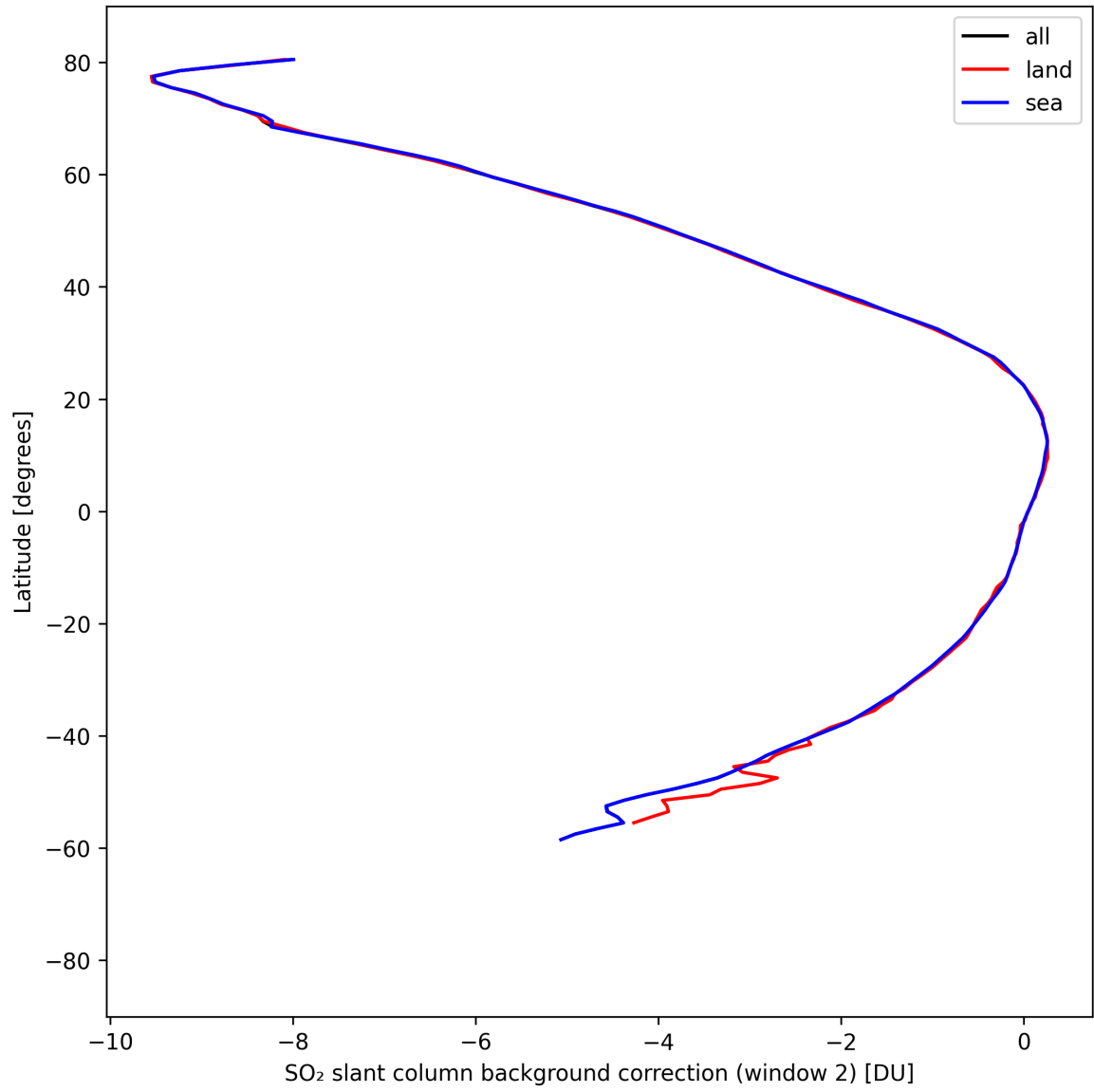
Figure 43: Zonal average of “SO 2 slant column background correction (window 2)” for 2025-04-16 to 2025-04-16.
