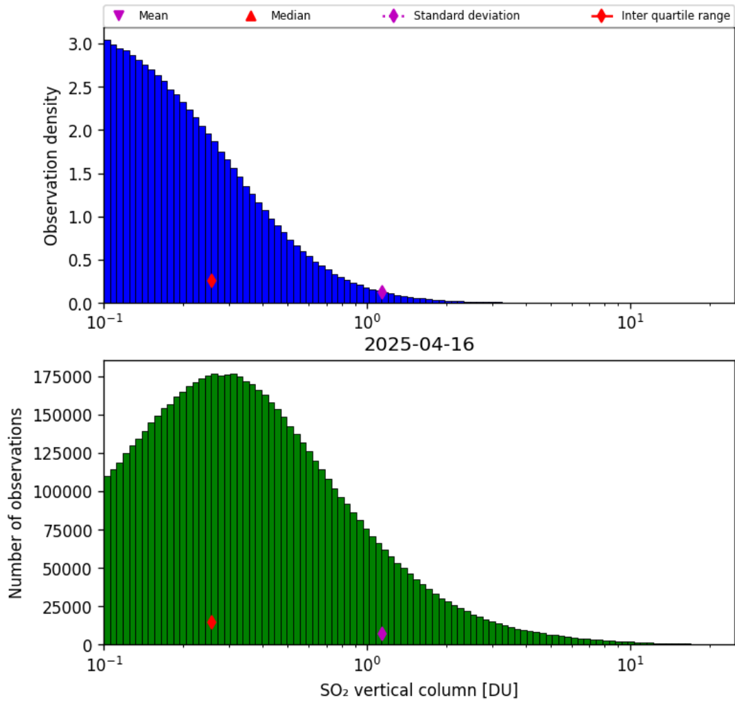
Figure 58: Histogram of “SO 2 vertical column” for 2025-04-16 to 2025-04-16
