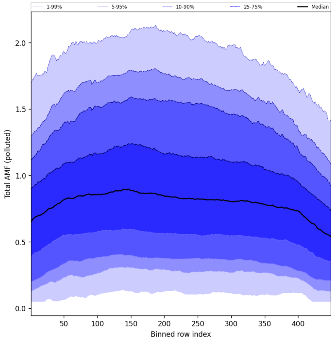
Figure 107: Along track statistics of “Total AMF (polluted)” for 2025-04-16 to 2025-04-16
