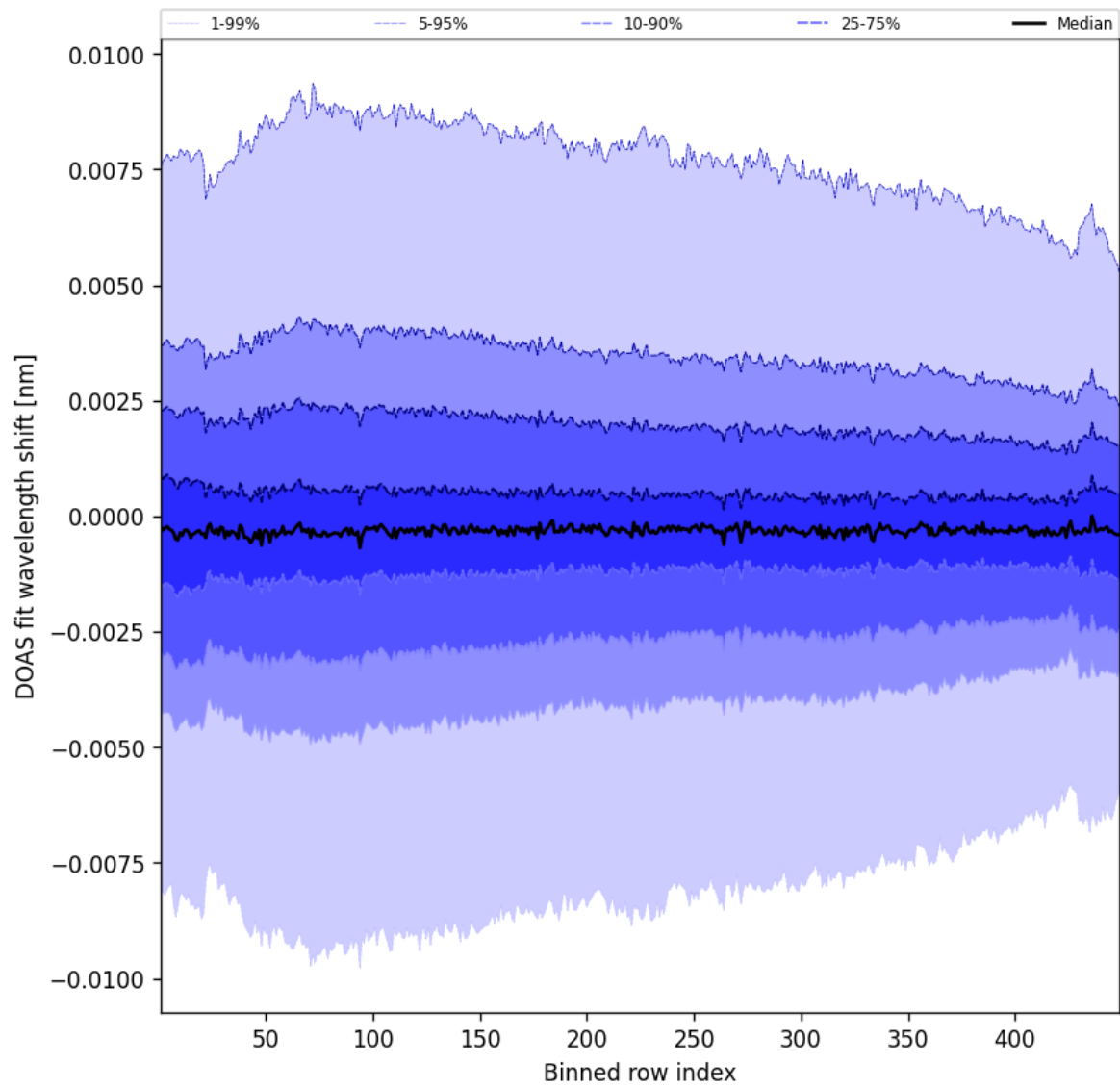
Figure 104: Along track statistics of “DOAS fit wavelength shift” for 2025-04-16 to 2025-04-16
