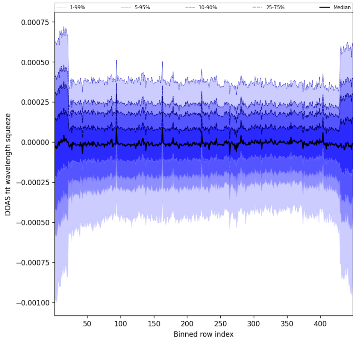
Figure 105: Along track statistics of “DOAS fit wavelength squeeze” for 2025-04-16 to 2025-04-16
