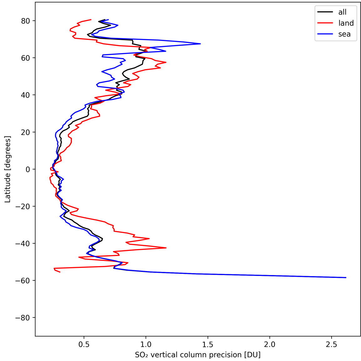
Figure 32: Zonal average of “SO 2 vertical column precision” for 2025-04-16 to 2025-04-16.
