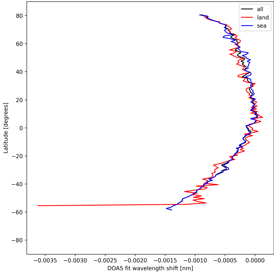
Figure 50: Zonal average of “DOAS fit wavelength shift” for 2025-04-16 to 2025-04-16.
