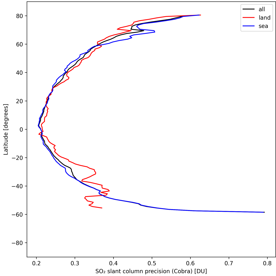
Figure 35: Zonal average of “SO 2 slant column precision (Cobra)” for 2025-04-16 to 2025-04-16.
