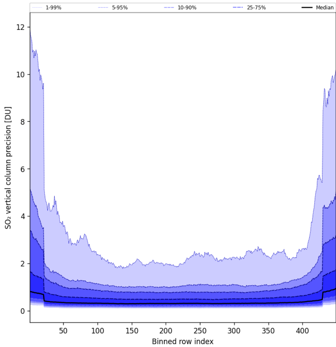
Figure 86: Along track statistics of “SO 2 vertical column precision” for 2025-04-16 to 2025-04-16
