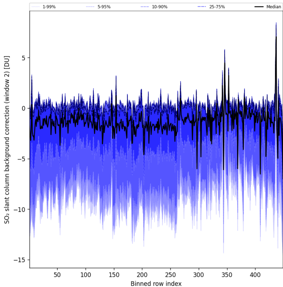
Figure 97: Along track statistics of “SO 2 slant column background correction (window 2)” for 2025-04-16 to 2025-04-16
