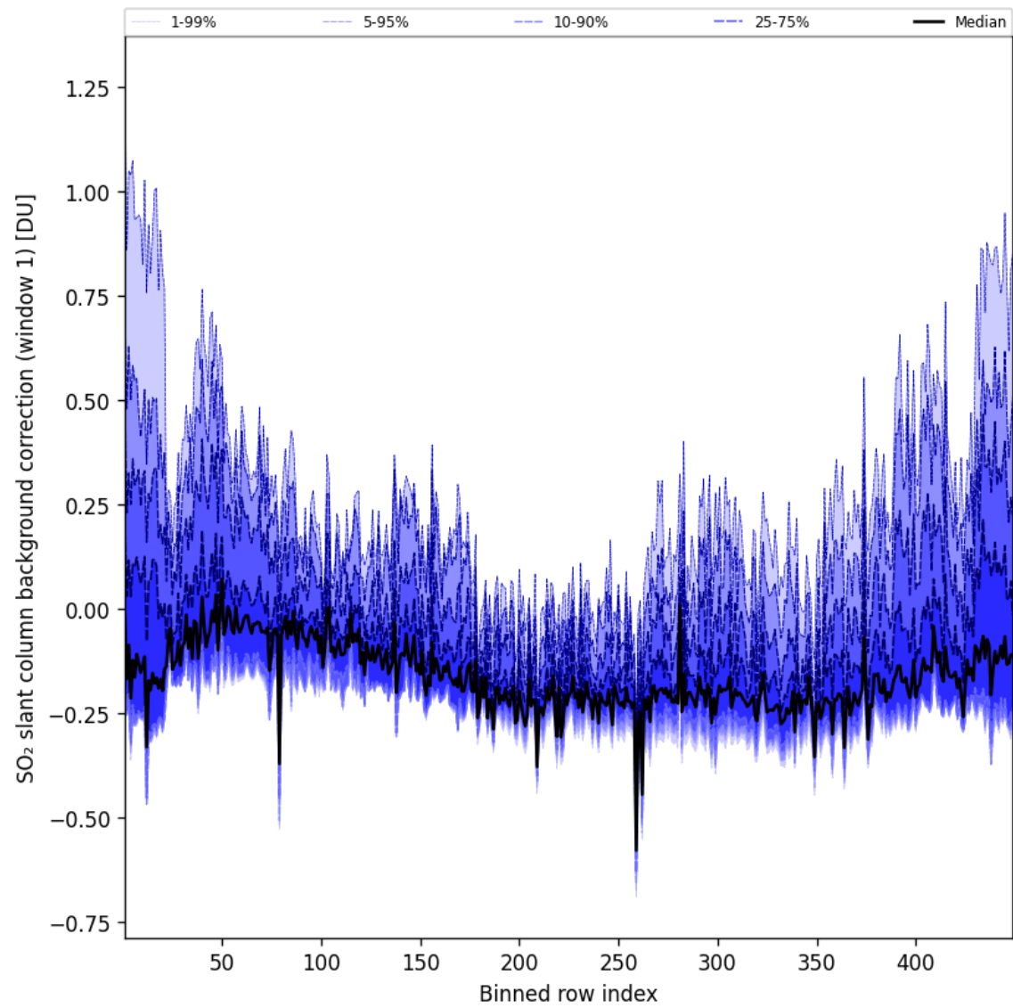
Figure 93: Along track statistics of “SO 2 slant column background correction (window 1)” for 2025-04-16 to 2025-04-16
