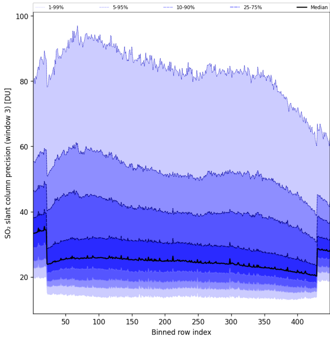
Figure 99: Along track statistics of “SO 2 slant column precision (window 3)” for 2025-04-28 to 2025-04-29
