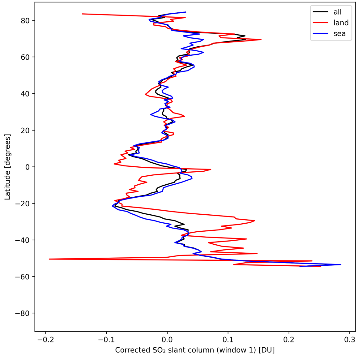
Figure 38: Zonal average of “Corrected SO 2 slant column (window 1)” for 2025-04-28 to 2025-04-29.
