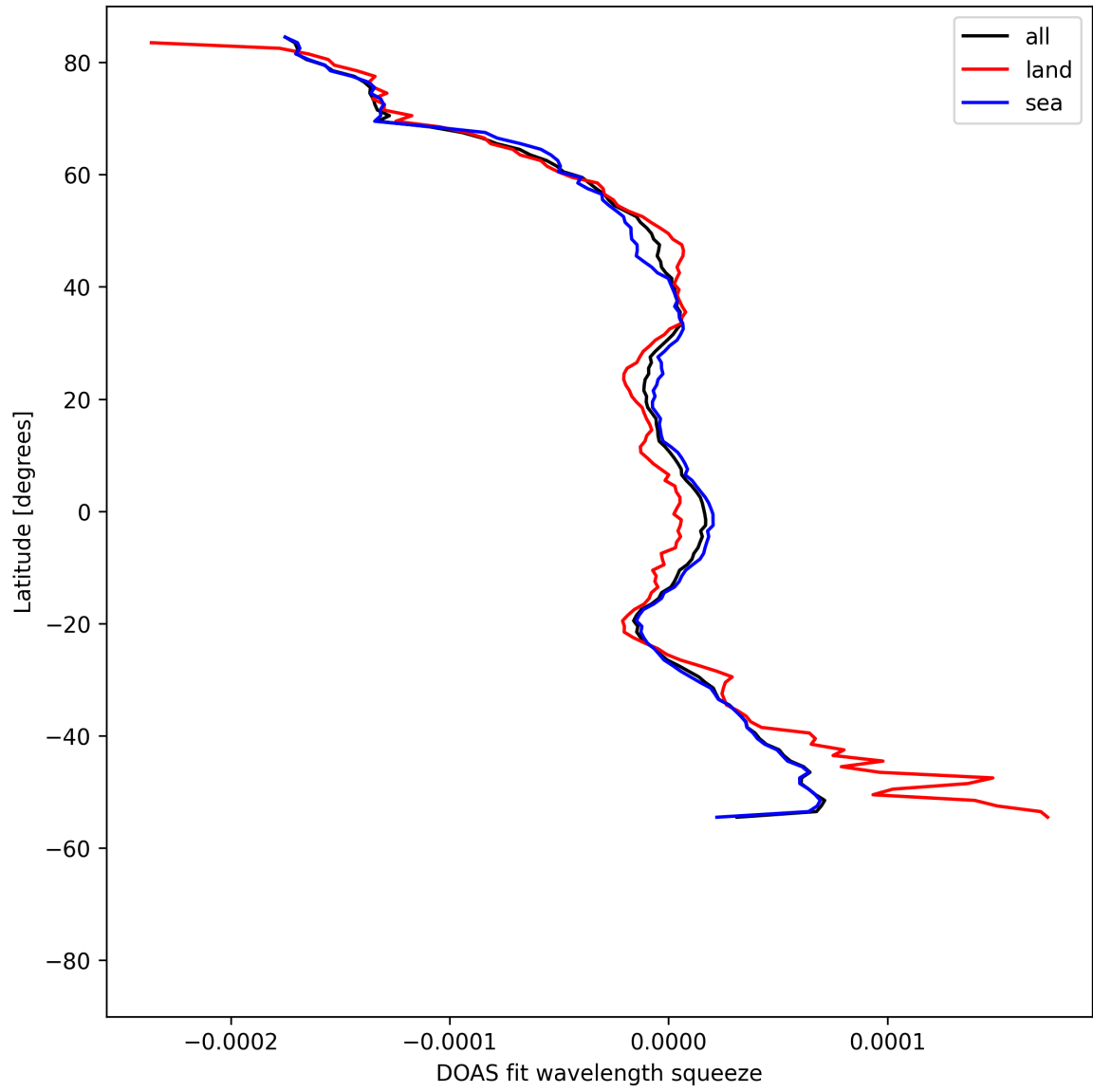
Figure 51: Zonal average of “DOAS fit wavelength squeeze” for 2025-04-28 to 2025-04-29.
