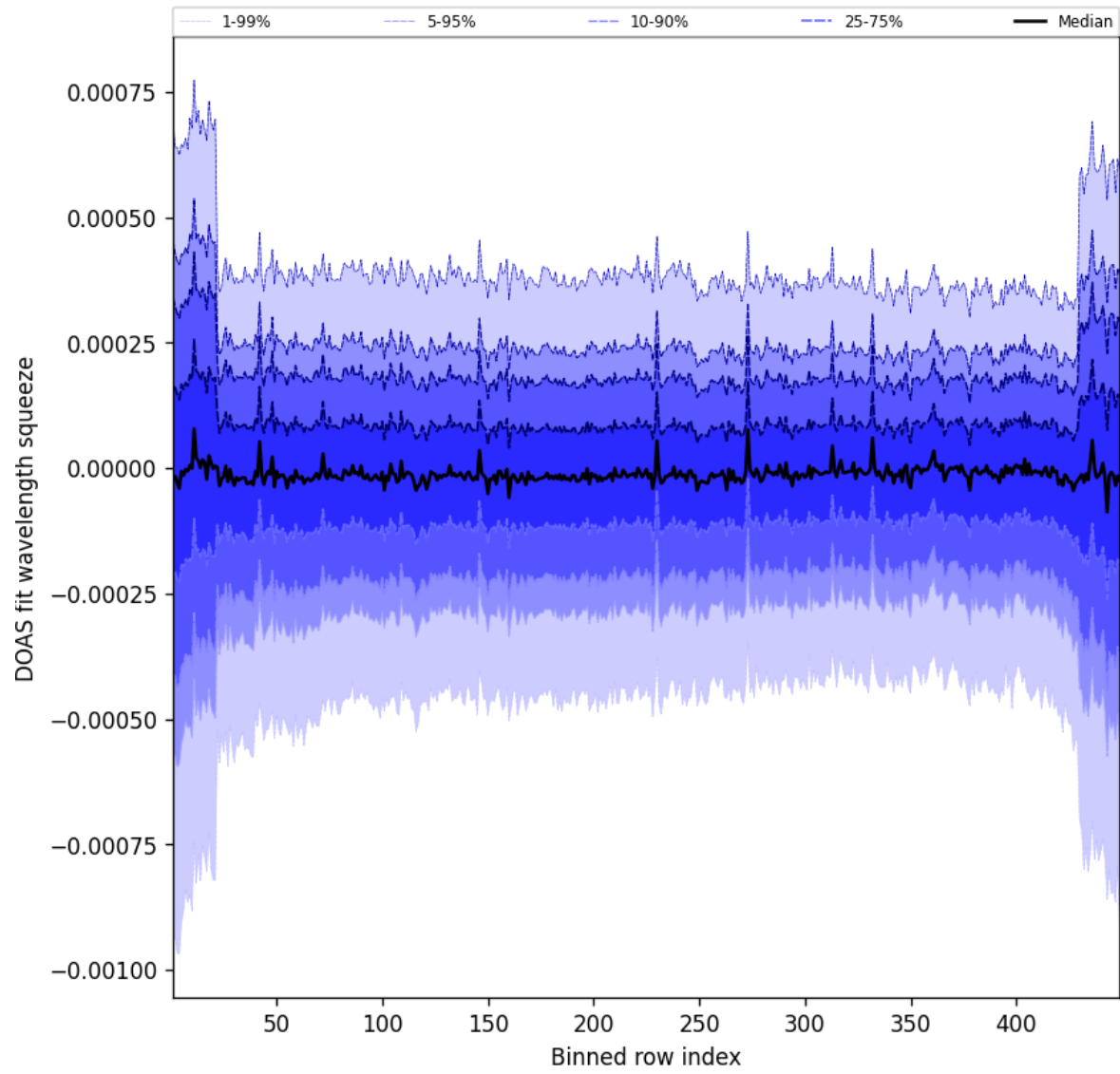
Figure 105: Along track statistics of “DOAS fit wavelength squeeze” for 2025-04-28 to 2025-04-29
