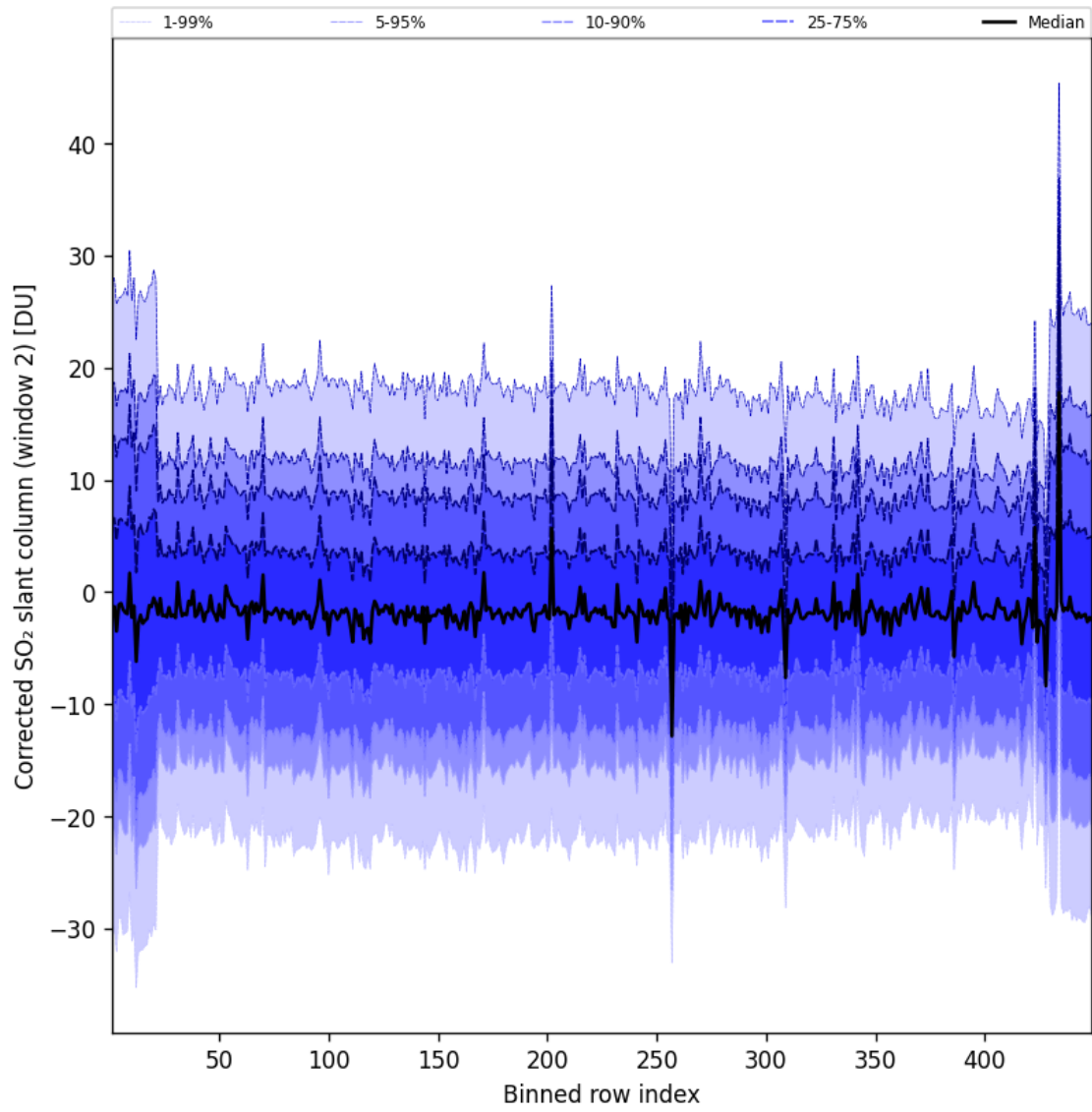
Figure 96: Along track statistics of “Corrected SO 2 slant column (window 2)” for 2025-04-28 to 2025-04-29
