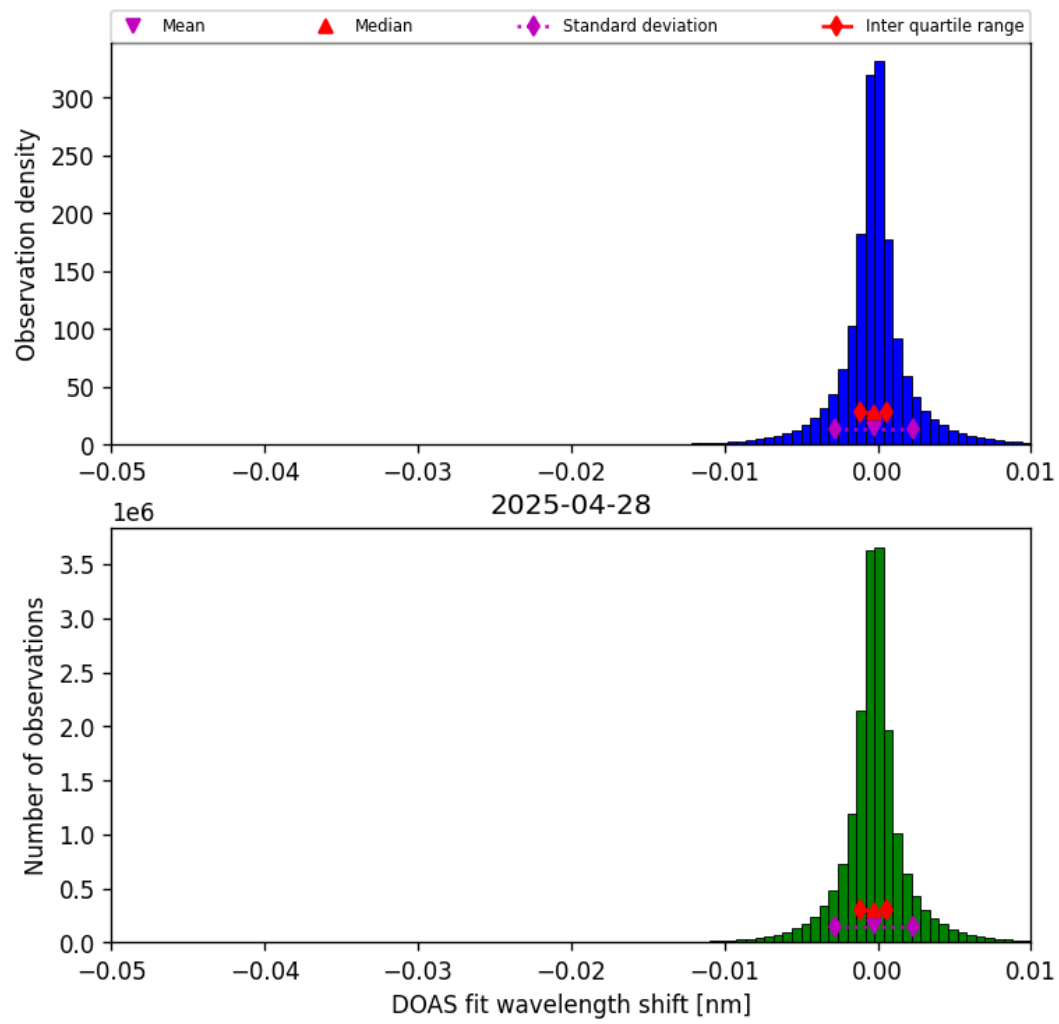
Figure 77: Histogram of “DOAS fit wavelength shift” for 2025-04-28 to 2025-04-29
