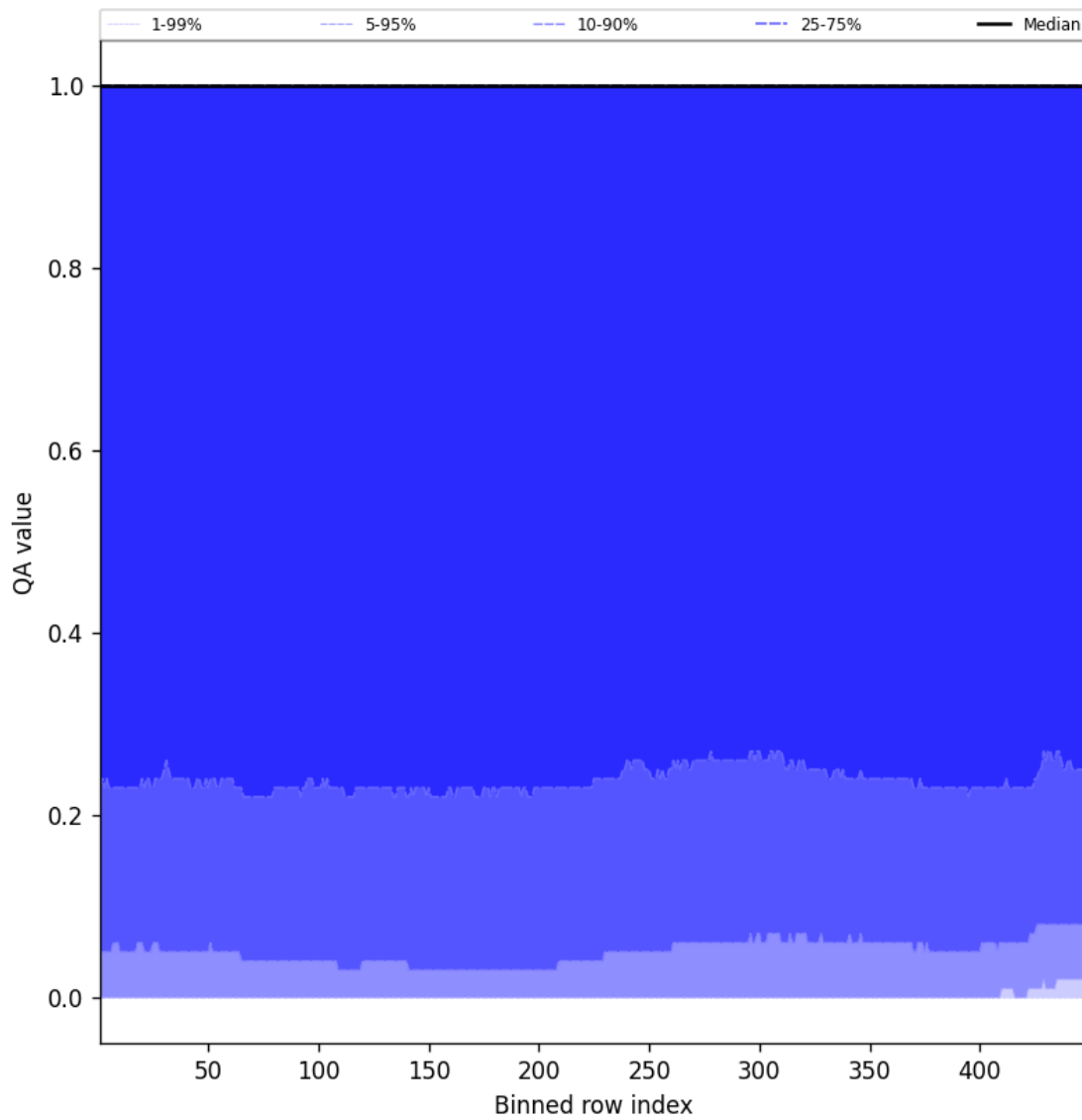
Figure 84: Along track statistics of “QA value” for 2025-04-28 to 2025-04-29
