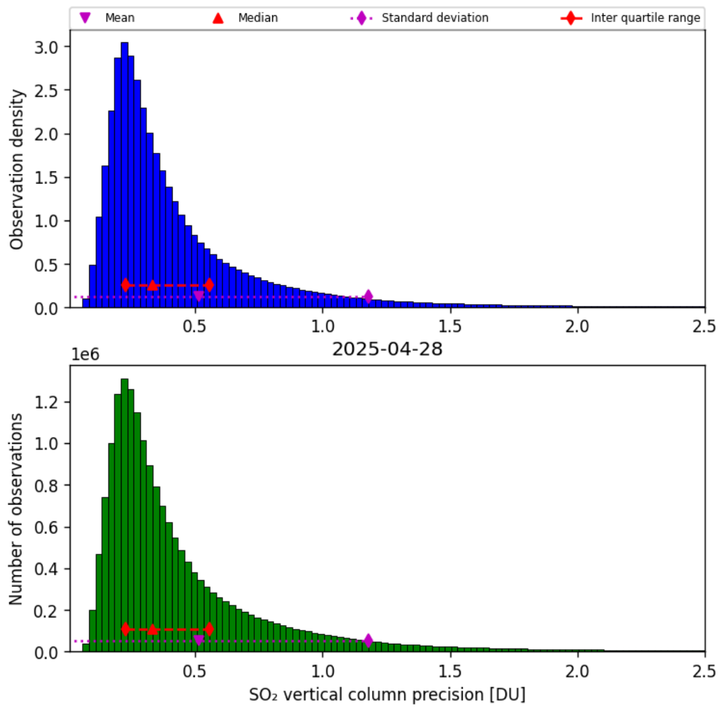
Figure 59: Histogram of “SO 2 vertical column precision” for 2025-04-28 to 2025-04-29
