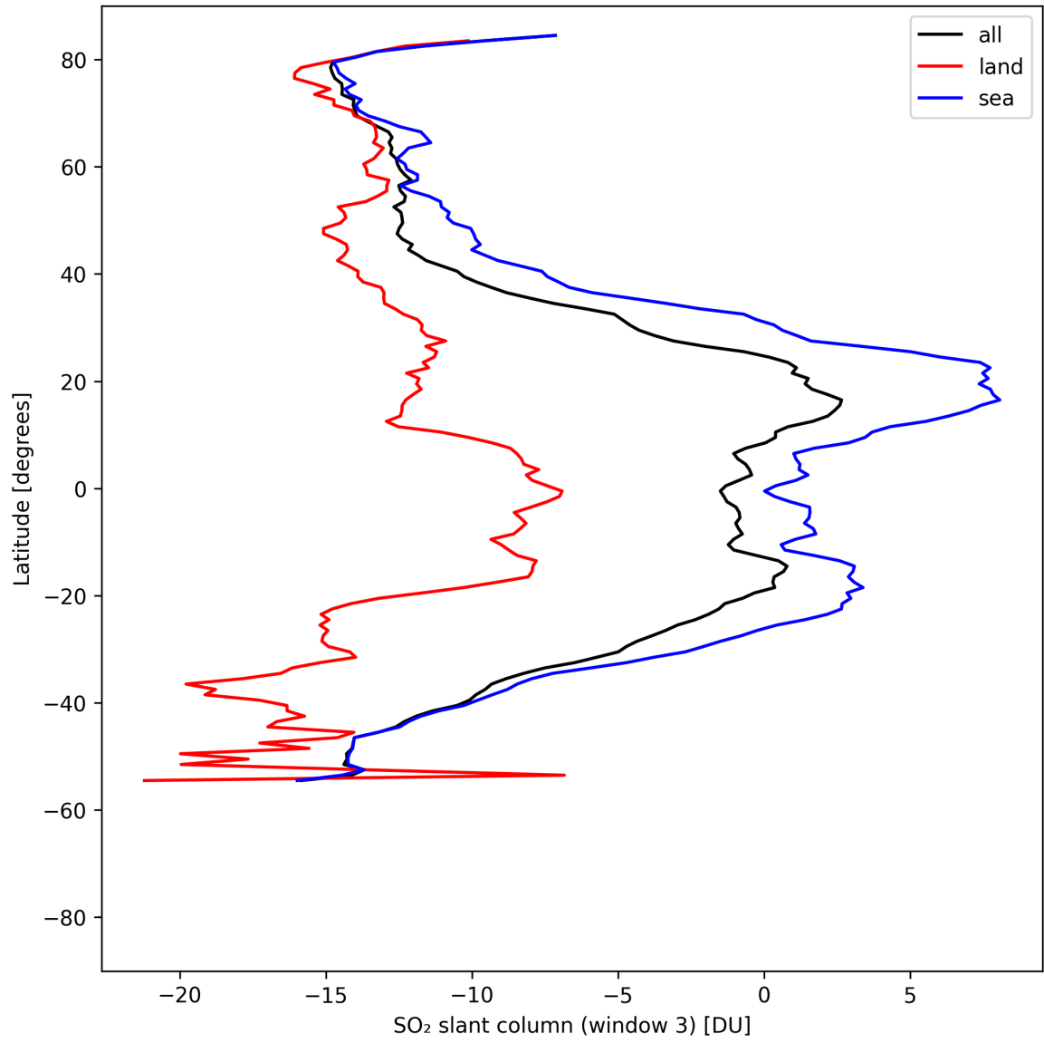
Figure 44: Zonal average of “SO 2 slant column (window 3)” for 2025-04-28 to 2025-04-29.
