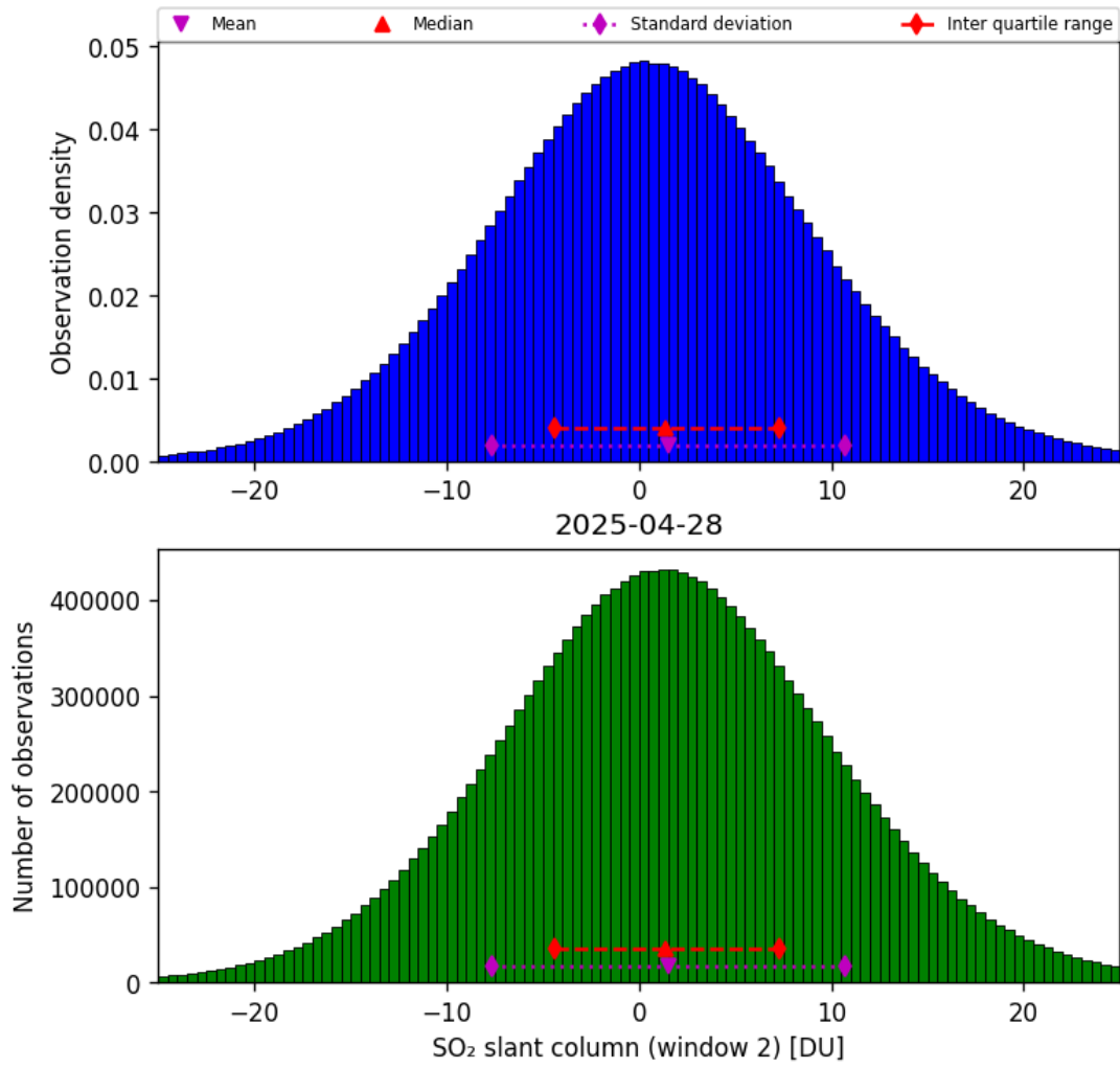
Figure 67: Histogram of “SO 2 slant column (window 2)” for 2025-04-28 to 2025-04-29
