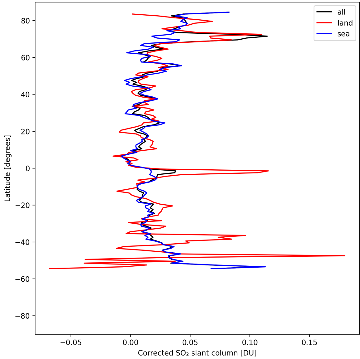
Figure 33: Zonal average of “Corrected SO 2 slant column” for 2025-04-28 to 2025-04-29.
