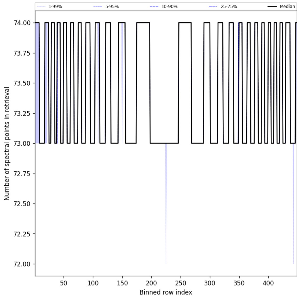
Figure 110: Along track statistics of “Number of spectral points in retrieval” for 2025-04-28 to 2025-04-29
