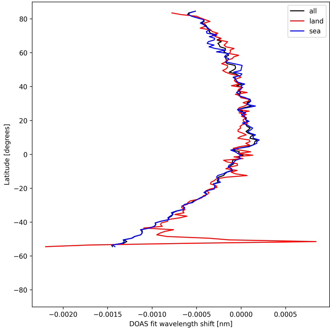
Figure 50: Zonal average of “DOAS fit wavelength shift” for 2025-04-28 to 2025-04-29.
