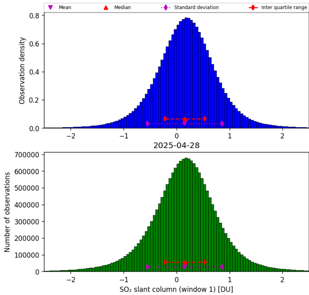
Figure 63: Histogram of “SO 2 slant column (window 1)” for 2025-04-28 to 2025-04-29
