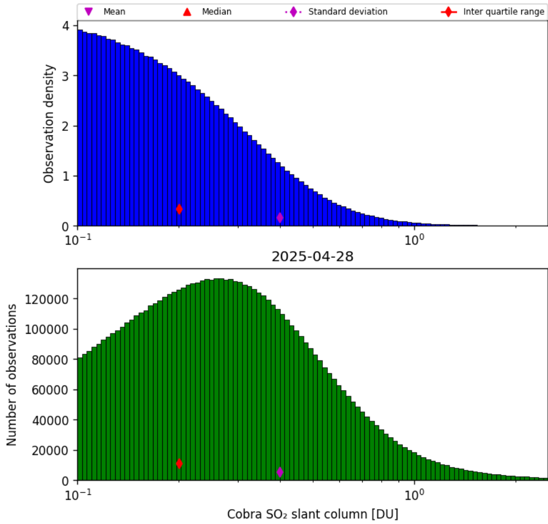
Figure 61: Histogram of “Cobra SO 2 slant column” for 2025-04-28 to 2025-04-29
