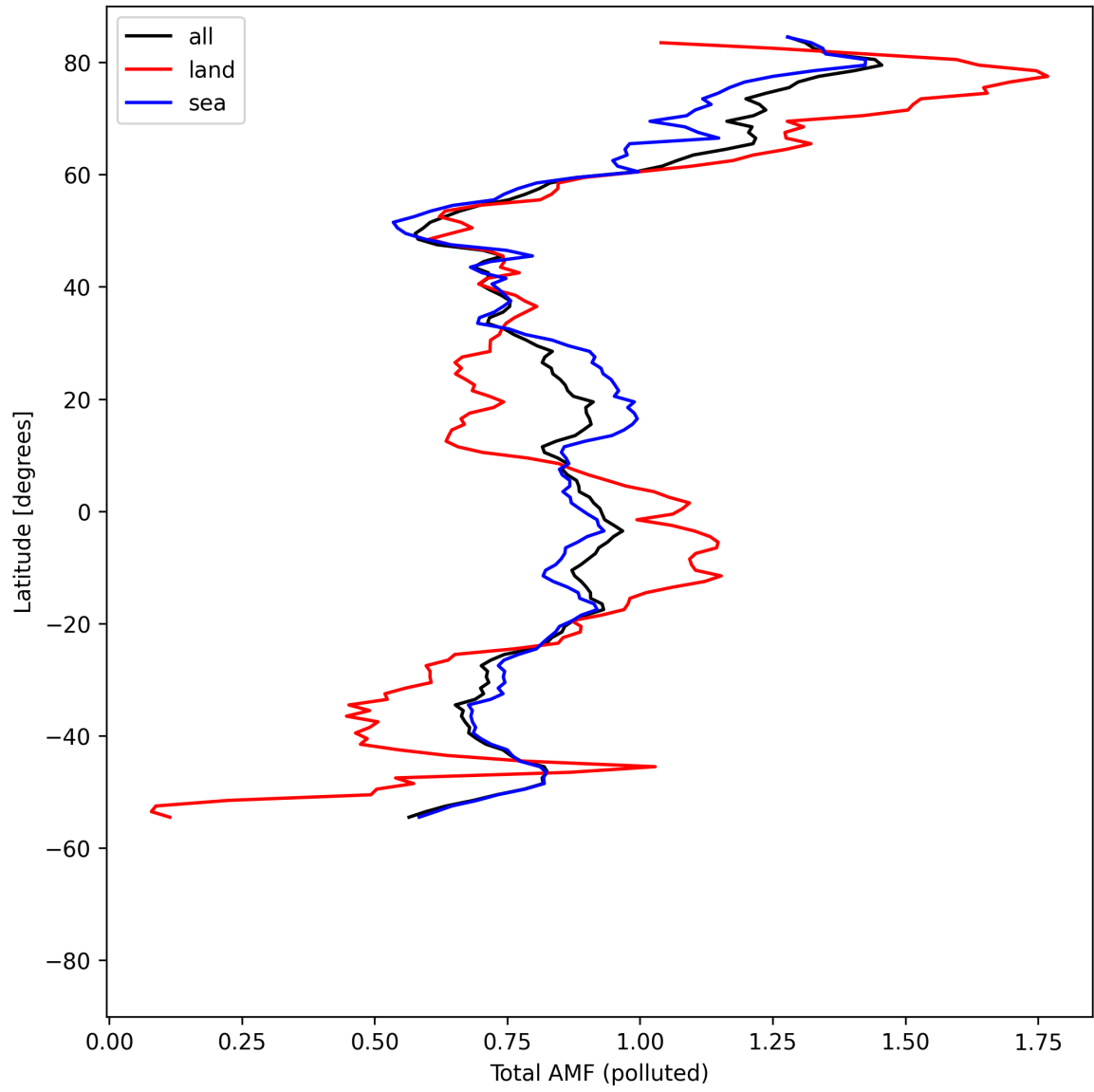
Figure 53: Zonal average of “Total AMF (polluted)” for 2025-04-28 to 2025-04-29.
