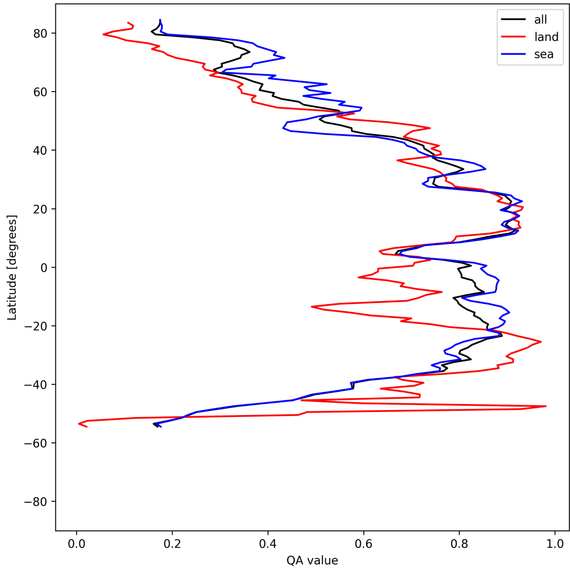
Figure 30: Zonal average of “QA value” for 2025-04-28 to 2025-04-29.
