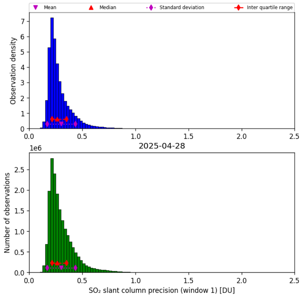
Figure 64: Histogram of “SO 2 slant column precision (window 1)” for 2025-04-28 to 2025-04-29
