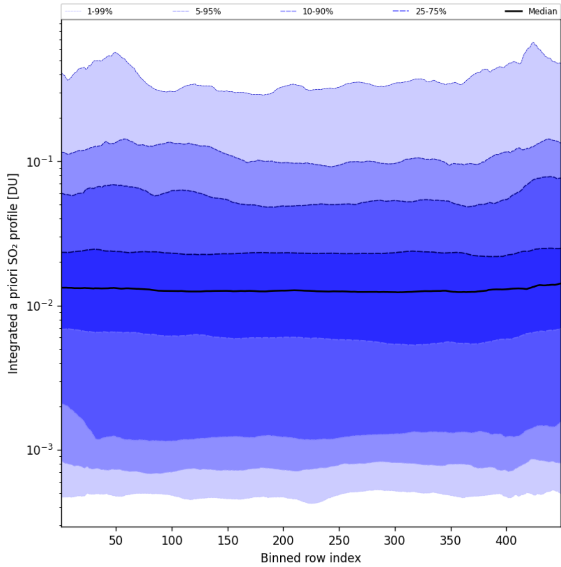
Figure 103: Along track statistics of “Integrated a priori SO 2 profile” for 2025-04-28 to 2025-04-29
