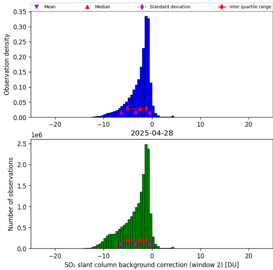
Figure 70: Histogram of “SO 2 slant column background correction (window 2)” for 2025-04-28 to 2025-04-29
