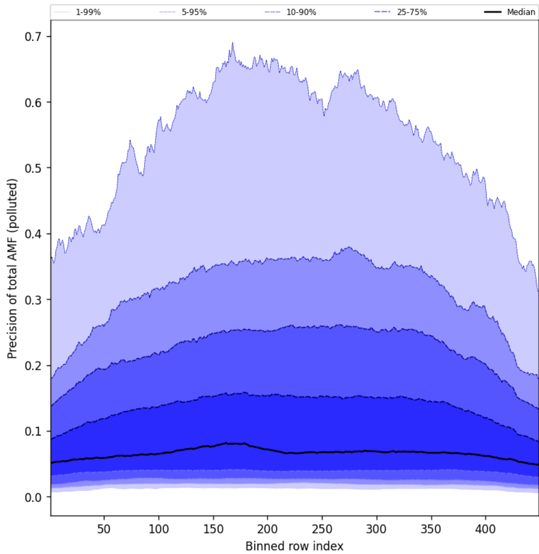
Figure 108: Along track statistics of “Precision of total AMF (polluted)” for 2025-04-28 to 2025-04-29
