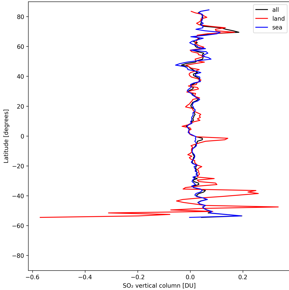
Figure 31: Zonal average of “SO 2 vertical column” for 2025-04-28 to 2025-04-29.
