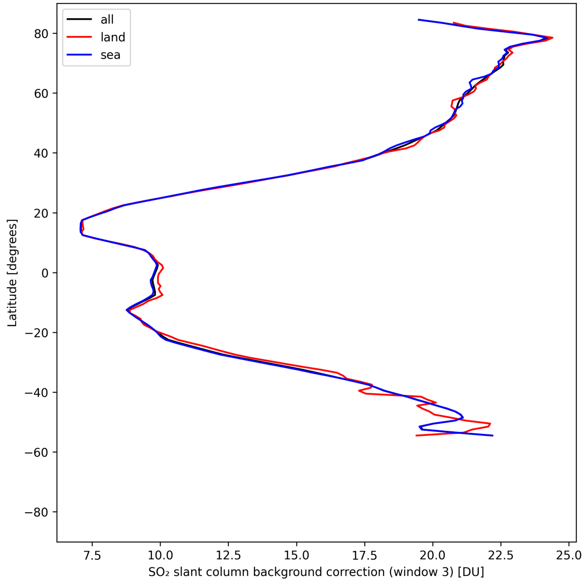
Figure 47: Zonal average of “SO 2 slant column background correction (window 3)” for 2025-04-28 to 2025-04-29.
