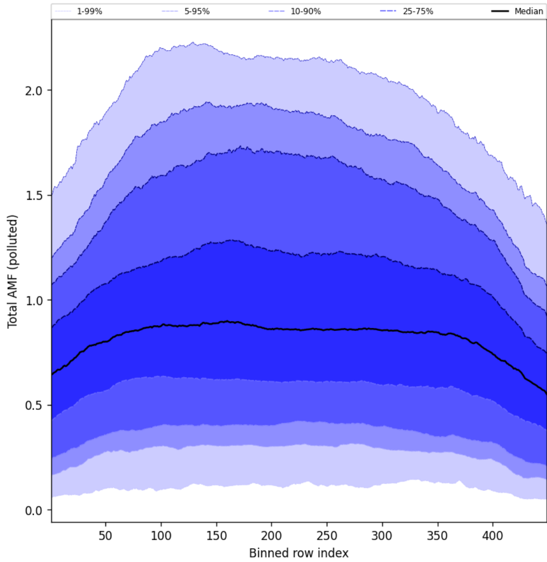
Figure 107: Along track statistics of “Total AMF (polluted)” for 2025-04-28 to 2025-04-29
