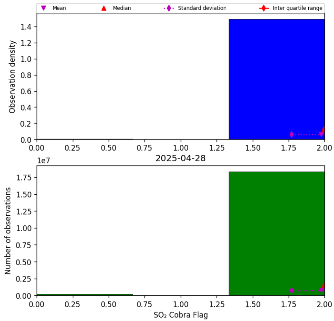
Figure 75: Histogram of "SO 2 Cobra Flag" for 2025-04-28 to 2025-04-29
