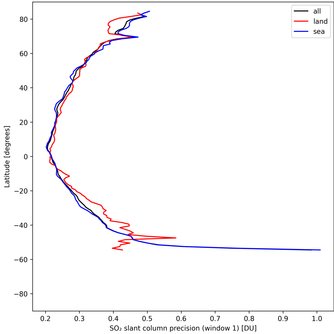
Figure 37: Zonal average of “SO 2 slant column precision (window 1)” for 2025-04-28 to 2025-04-29.
