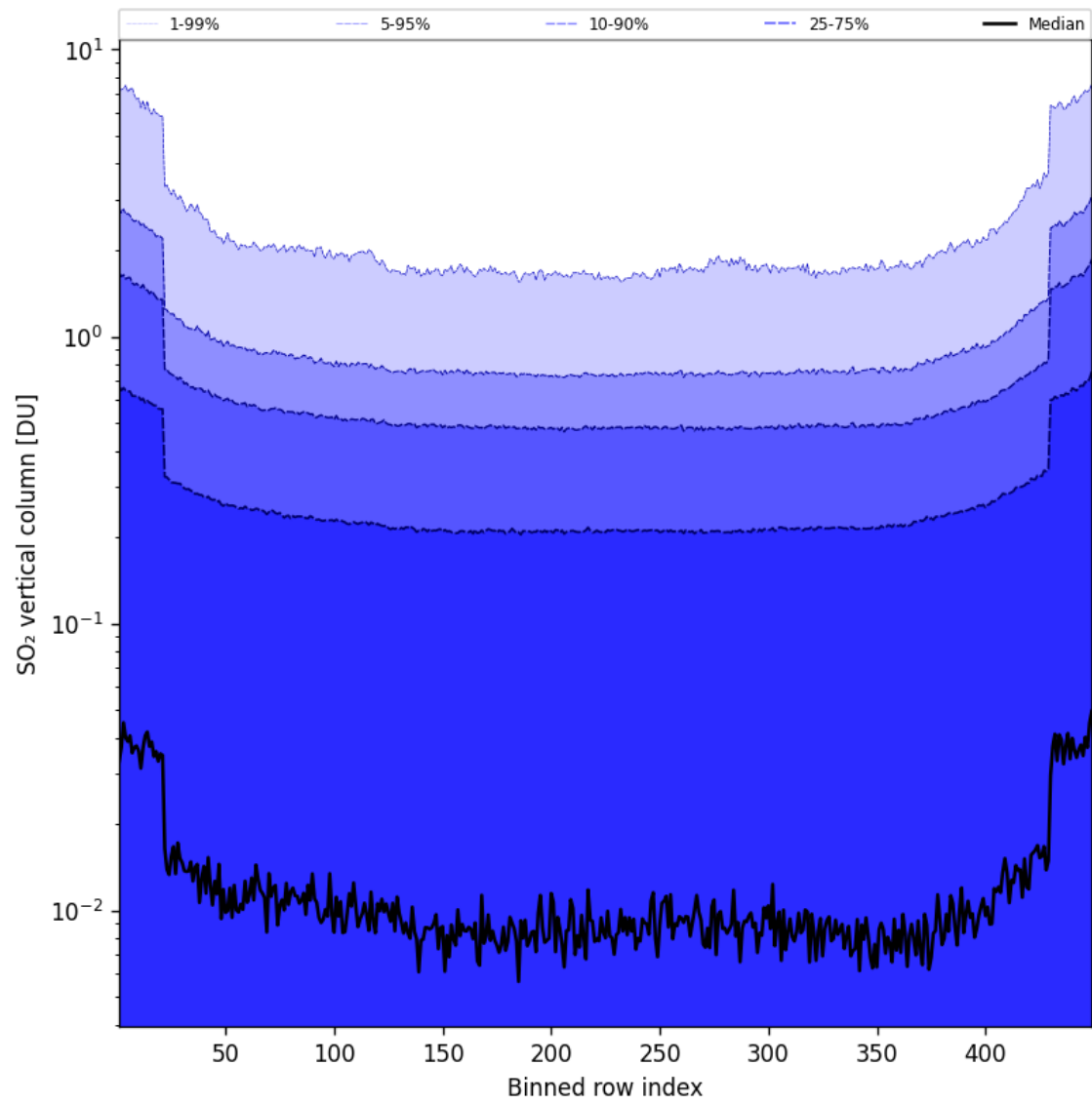
Figure 85: Along track statistics of “SO 2 vertical column” for 2025-04-28 to 2025-04-29
