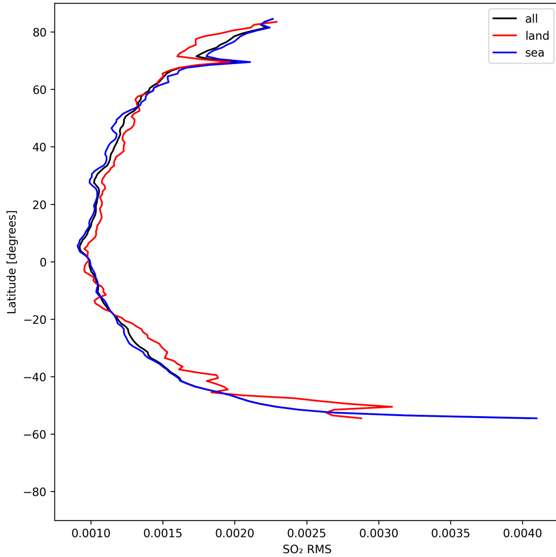
Figure 52: Zonal average of “SO 2 RMS” for 2025-04-28 to 2025-04-29.
