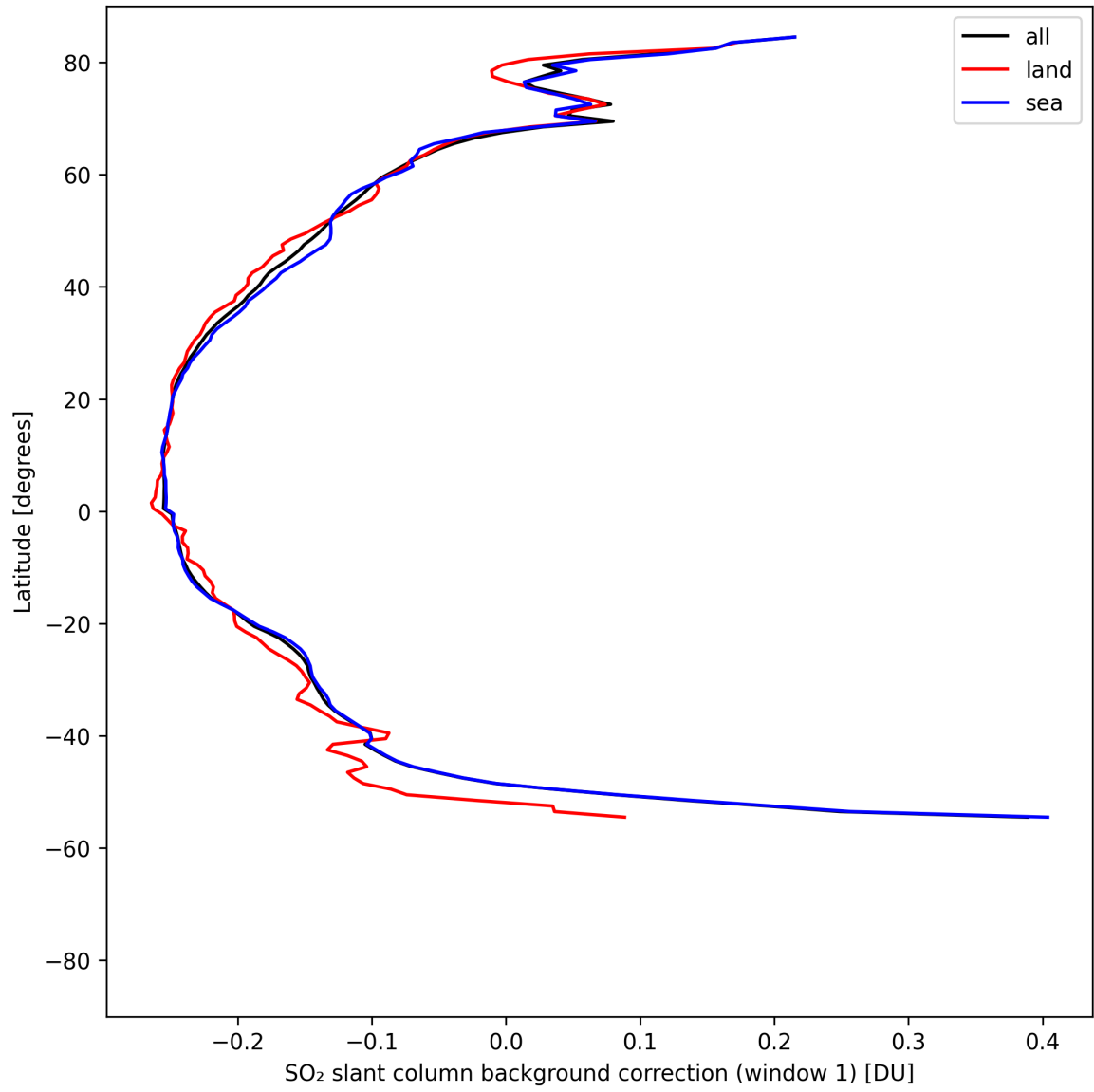
Figure 39: Zonal average of “SO 2 slant column background correction (window 1)” for 2025-04-28 to 2025-04-29.
