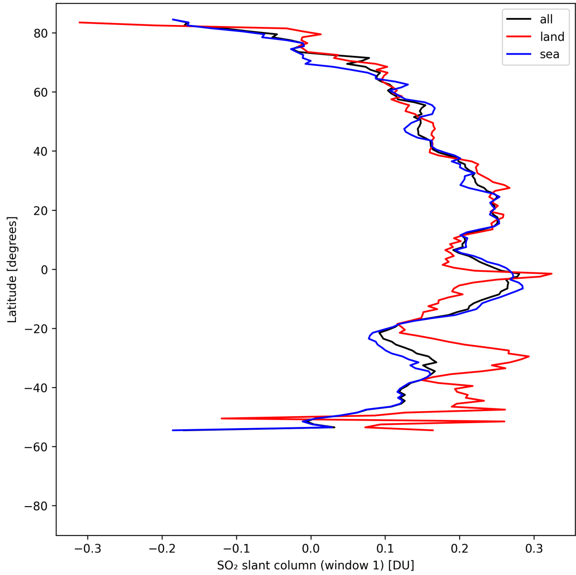
Figure 36: Zonal average of “SO 2 slant column (window 1)” for 2025-04-28 to 2025-04-29.
