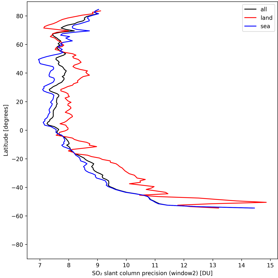
Figure 41: Zonal average of “SO 2 slant column precision (window2)” for 2025-04-28 to 2025-04-29.
