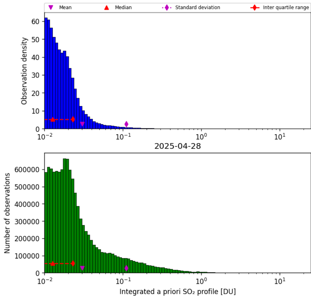
Figure 76: Histogram of “Integrated a priori SO 2 profile” for 2025-04-28 to 2025-04-29
