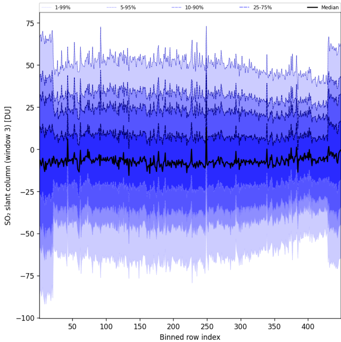
Figure 98: Along track statistics of “SO 2 slant column (window 3)” for 2025-04-28 to 2025-04-29
