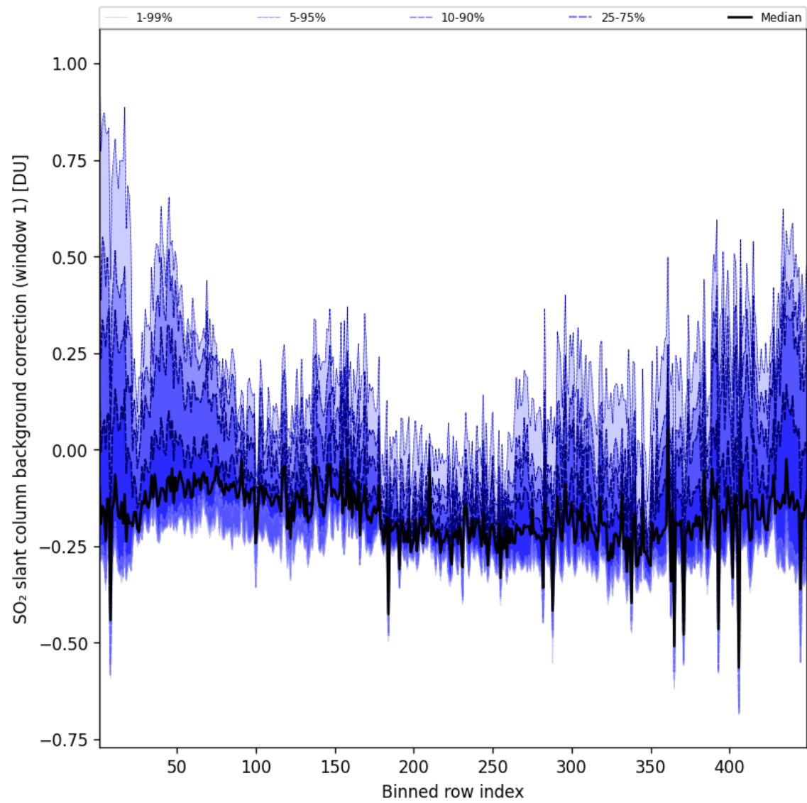
Figure 93: Along track statistics of "SO 2 slant column background correction (window 1)" for 2025-04-28 to 2025-04-29
