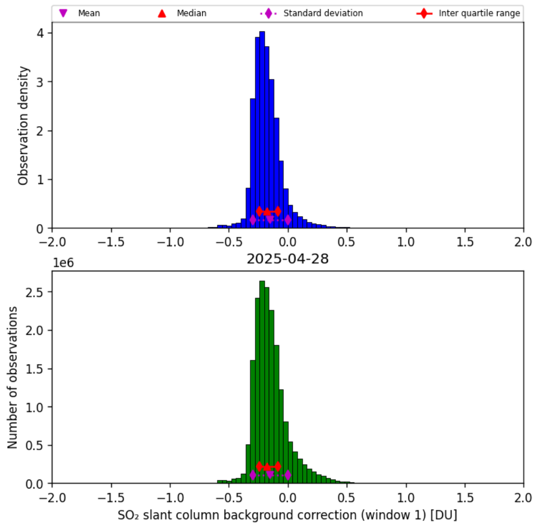
Figure 66: Histogram of “SO 2 slant column background correction (window 1)” for 2025-04-28 to 2025-04-29
