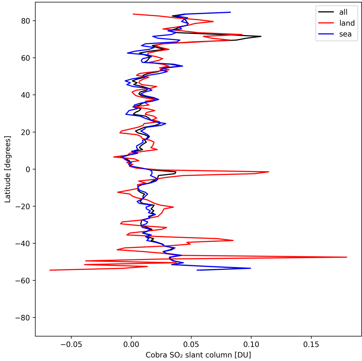
Figure 34: Zonal average of “Cobra SO 2 slant column” for 2025-04-28 to 2025-04-29.
