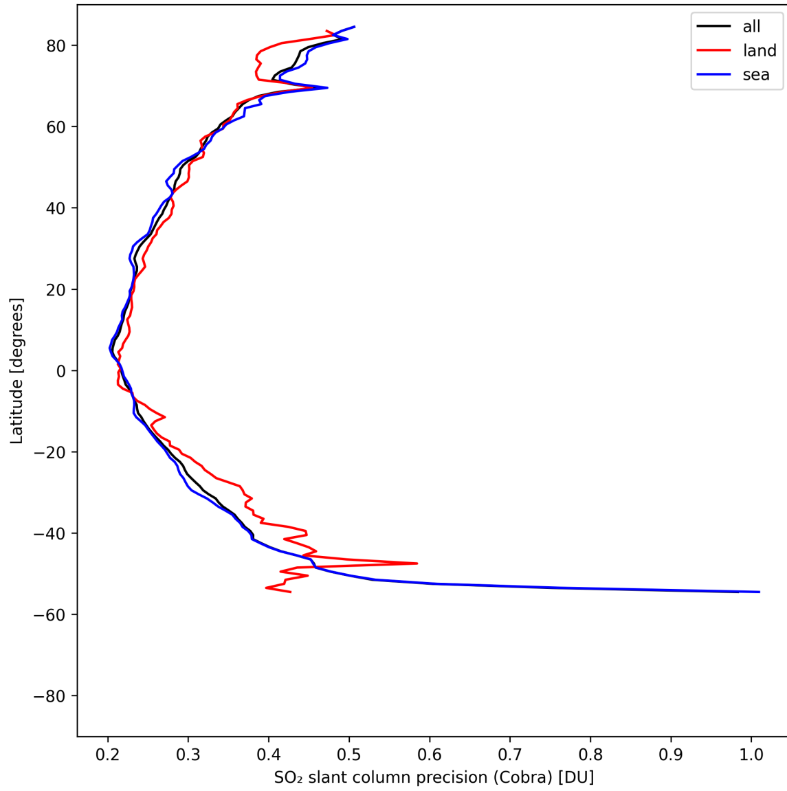
Figure 35: Zonal average of “SO 2 slant column precision (Cobra)” for 2025-04-28 to 2025-04-29.
