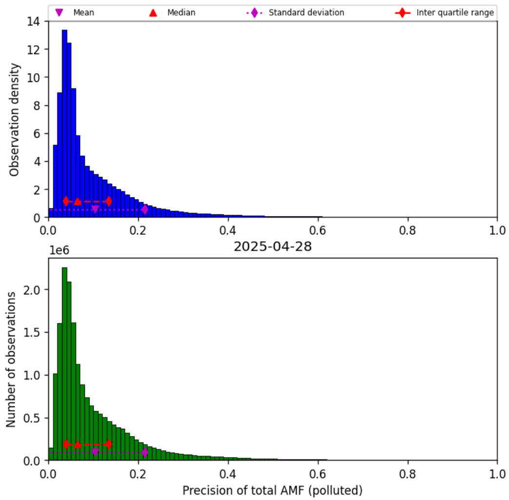
Figure 81: Histogram of “Precision of total AMF (polluted)” for 2025-04-28 to 2025-04-29
