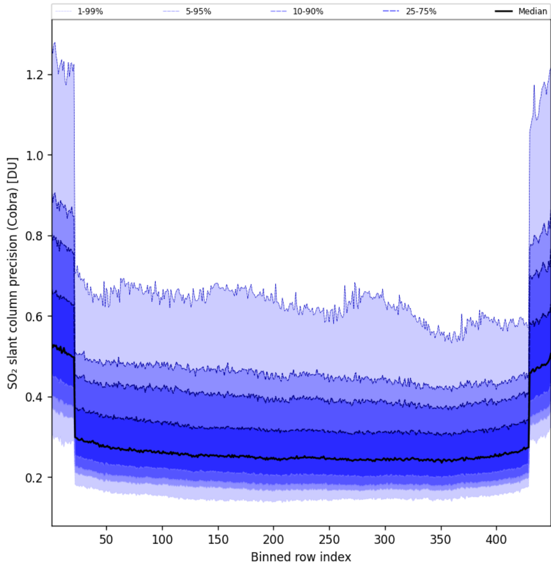
Figure 89: Along track statistics of “SO 2 slant column precision (Cobra)” for 2025-04-28 to 2025-04-29
