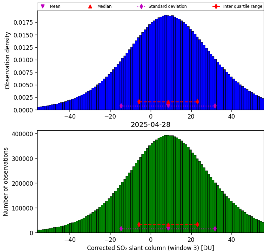
Figure 73: Histogram of “Corrected SO 2 slant column (window 3)” for 2025-04-28 to 2025-04-29
