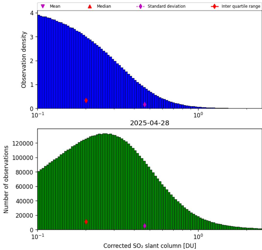
Figure 60: Histogram of “Corrected SO 2 slant column” for 2025-04-28 to 2025-04-29
