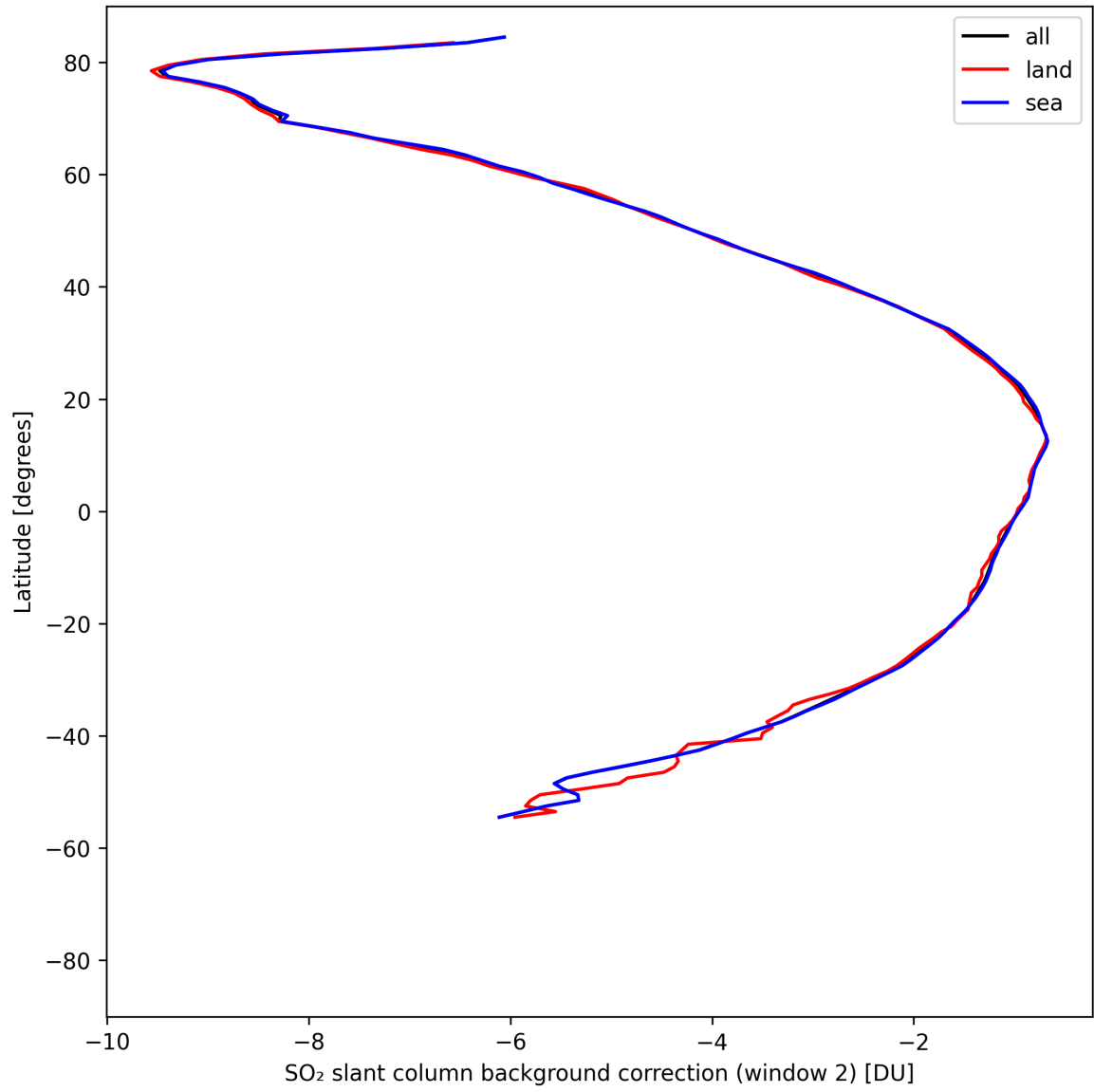
Figure 43: Zonal average of “SO 2 slant column background correction (window 2)” for 2025-04-28 to 2025-04-29.
