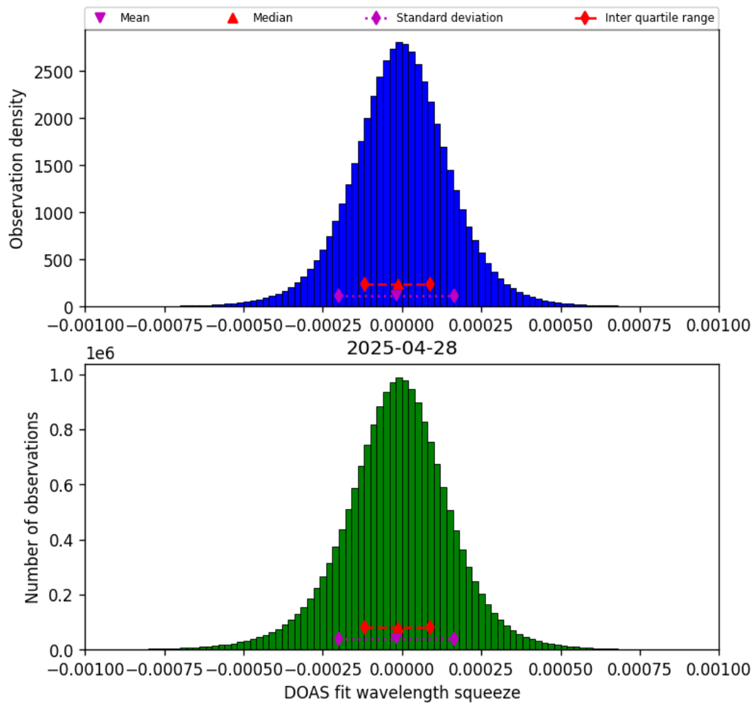
Figure 78: Histogram of “DOAS fit wavelength squeeze” for 2025-04-28 to 2025-04-29
