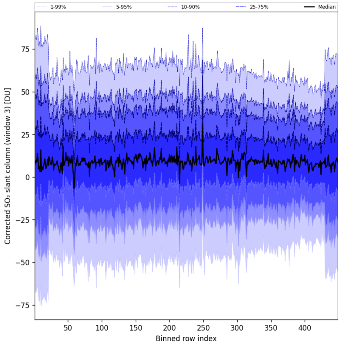
Figure 100: Along track statistics of "Corrected SO 2 slant column (window 3)" for 2025-04-28 to 2025-04-29
