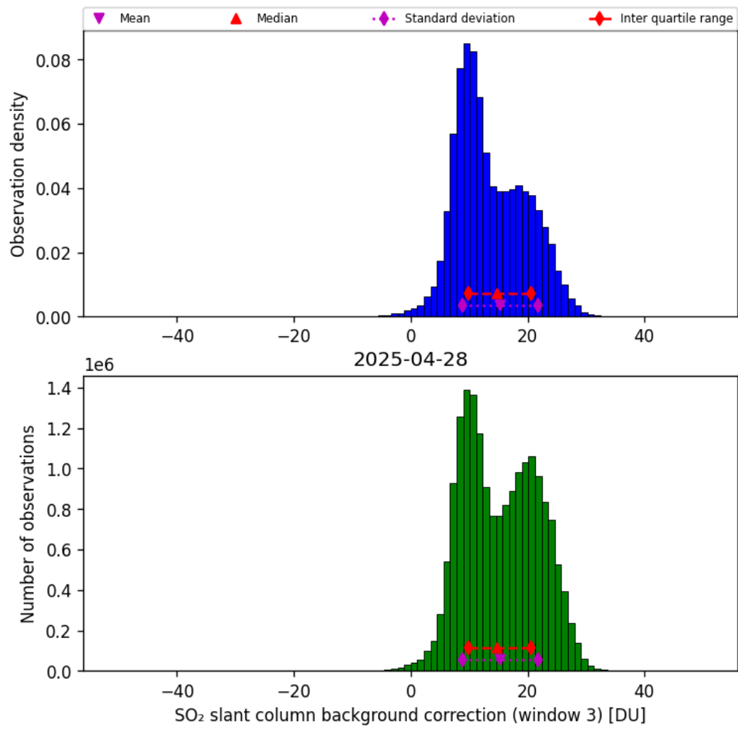
Figure 74: Histogram of “SO 2 slant column background correction (window 3)” for 2025-04-28 to 2025-04-29
