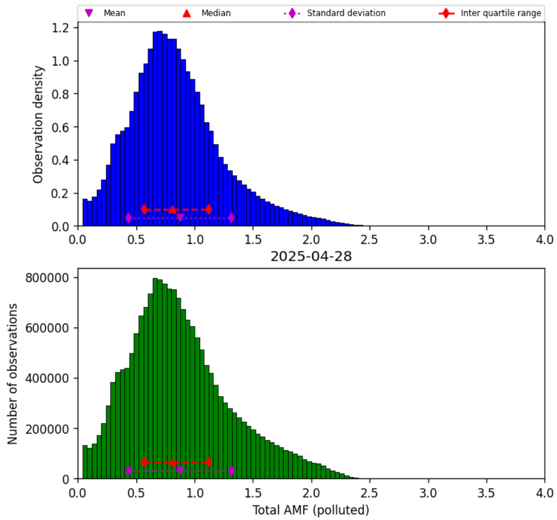
Figure 80: Histogram of “Total AMF (polluted)” for 2025-04-28 to 2025-04-29
