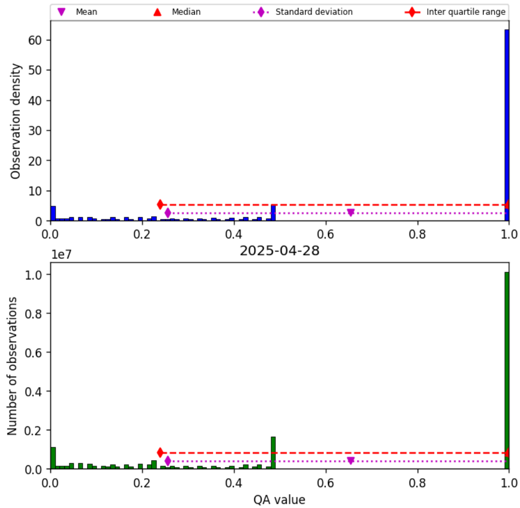
Figure 57: Histogram of “QA value” for 2025-04-28 to 2025-04-29
