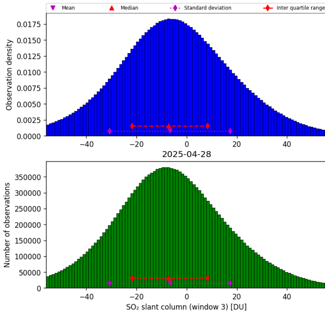
Figure 71: Histogram of “SO 2 slant column (window 3)” for 2025-04-28 to 2025-04-29
