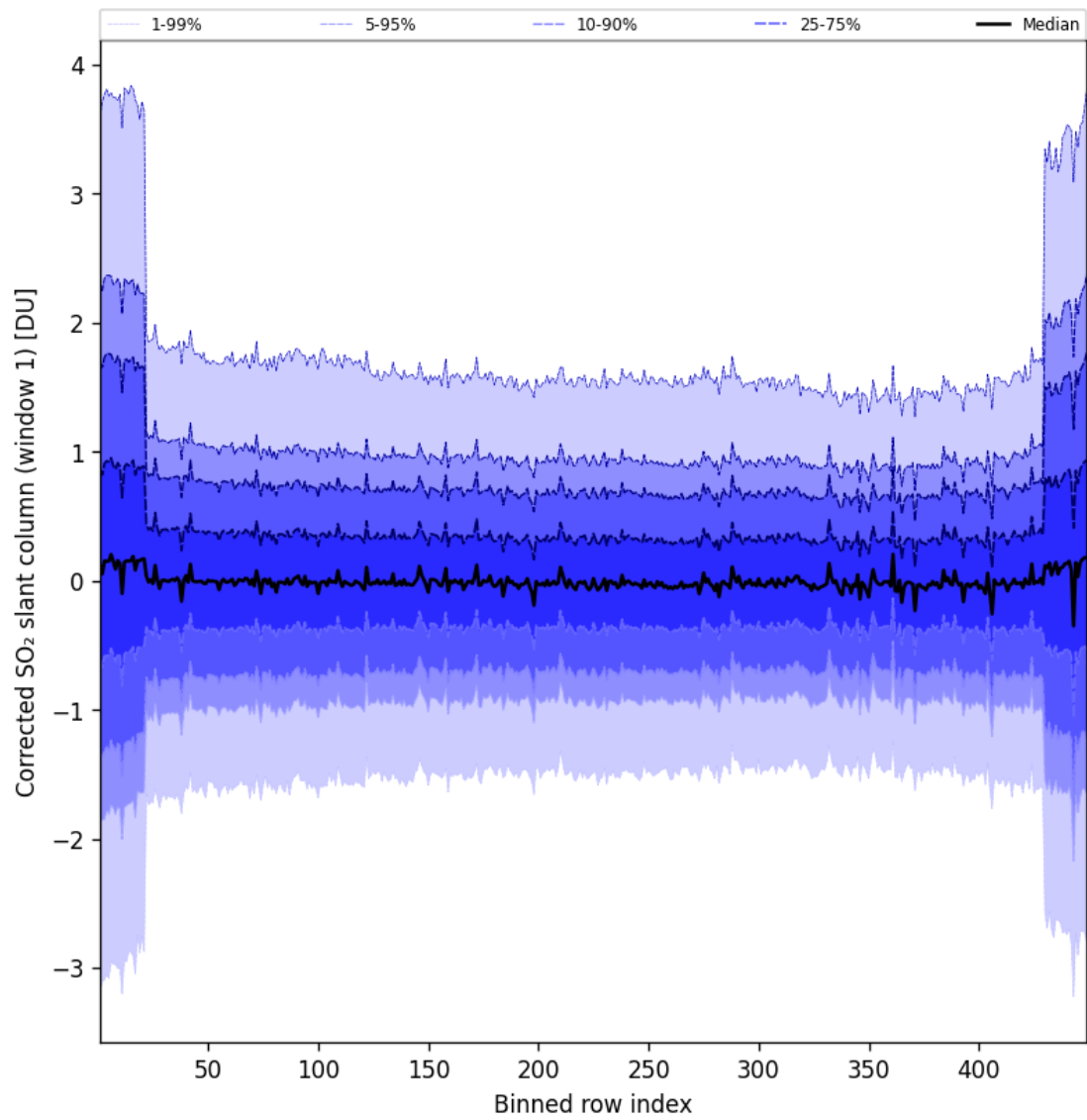
Figure 92: Along track statistics of “Corrected SO 2 slant column (window 1)” for 2025-04-28 to 2025-04-29
