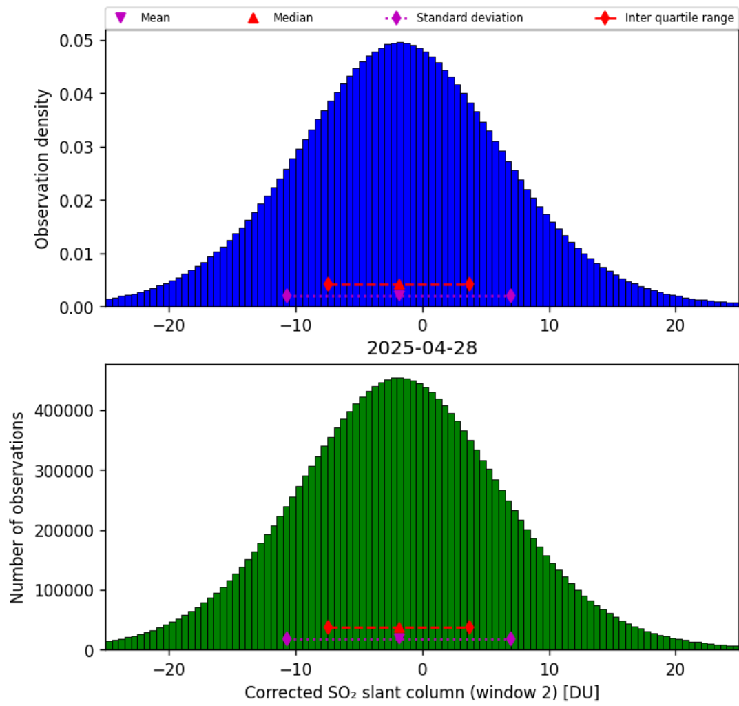
Figure 69: Histogram of “Corrected SO 2 slant column (window 2)” for 2025-04-28 to 2025-04-29
