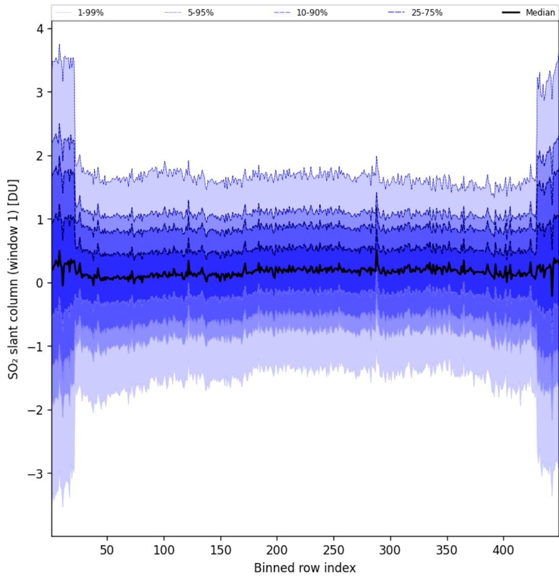
Figure 90: Along track statistics of "SO 2 slant column (window 1)" for 2025-04-28 to 2025-04-29
