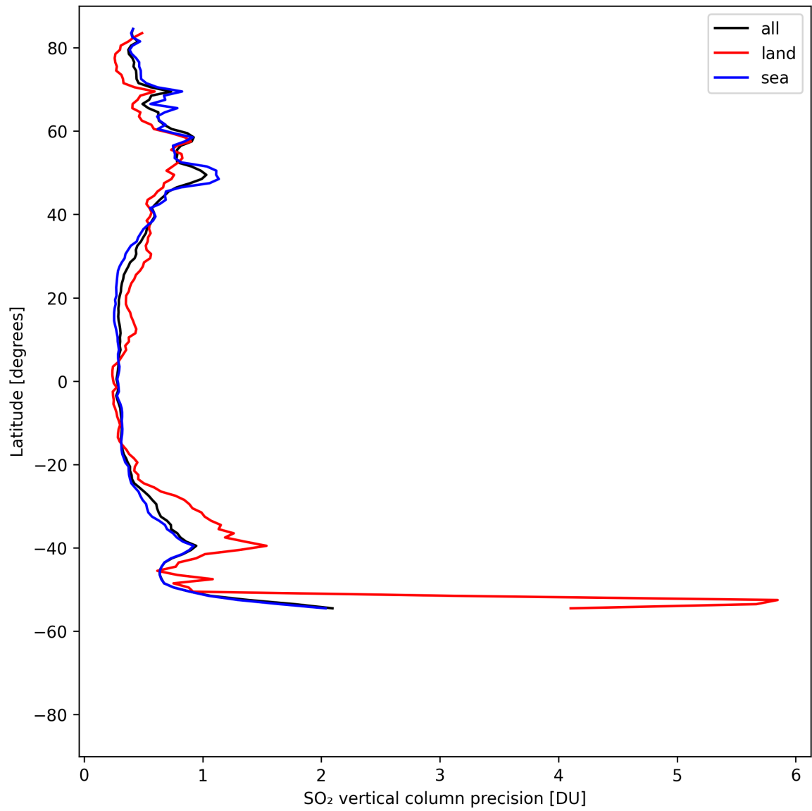
Figure 32: Zonal average of “SO 2 vertical column precision” for 2025-04-28 to 2025-04-29.
