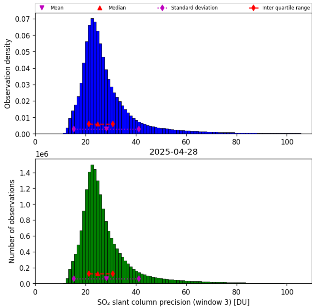
Figure 72: Histogram of “SO 2 slant column precision (window 3)” for 2025-04-28 to 2025-04-29
