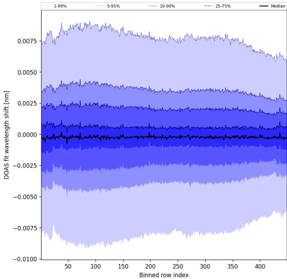
Figure 104: Along track statistics of “DOAS fit wavelength shift” for 2025-04-28 to 2025-04-29
