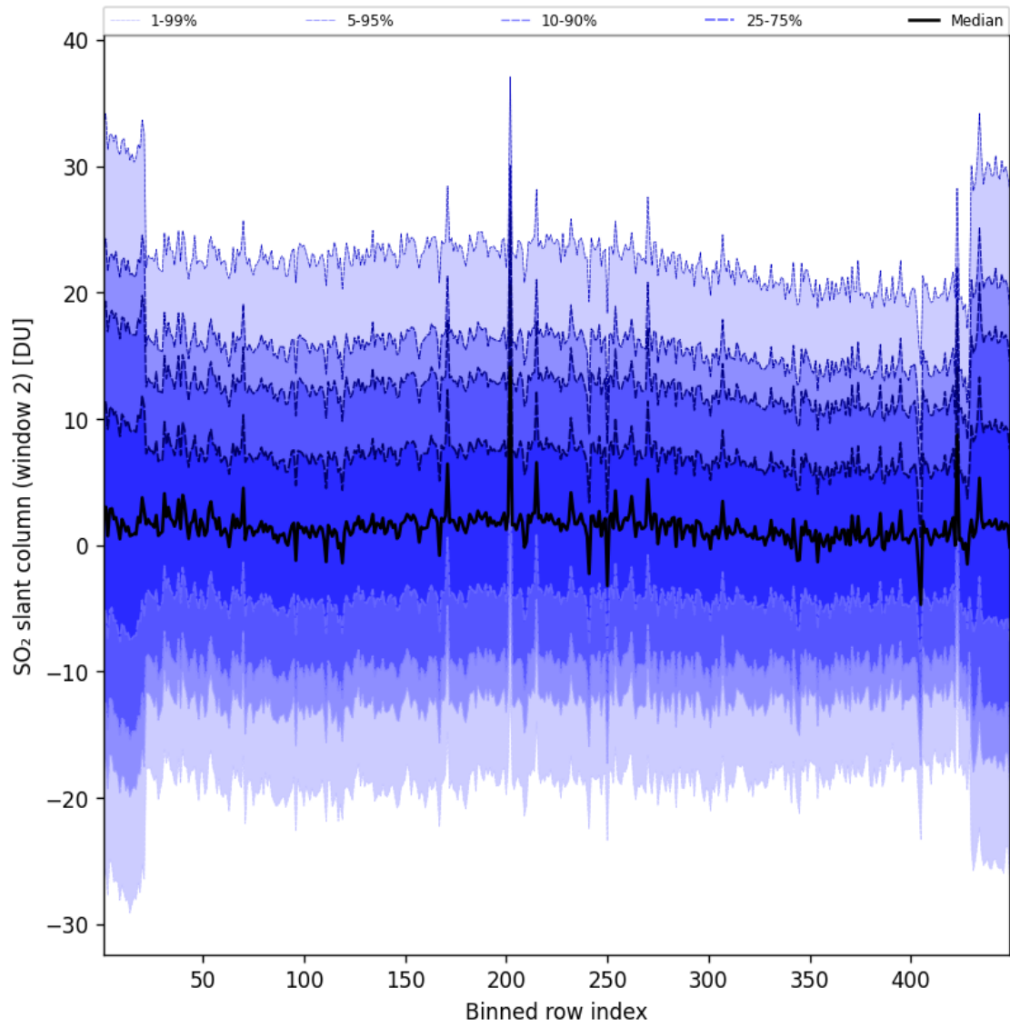
Figure 94: Along track statistics of “SO 2 slant column (window 2)” for 2025-04-28 to 2025-04-29
