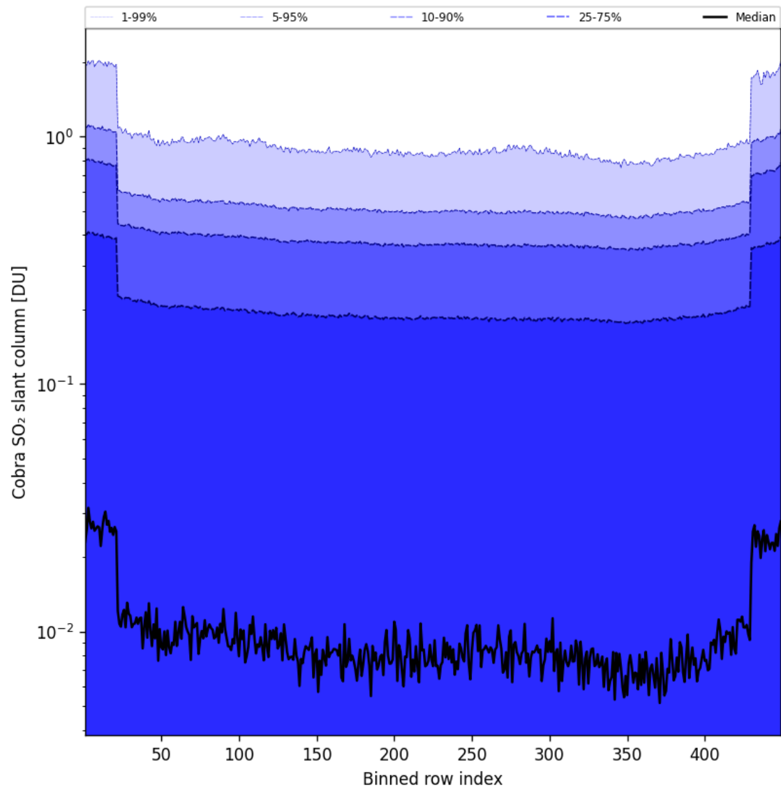
Figure 88: Along track statistics of "Cobra SO 2 slant column" for 2025-04-28 to 2025-04-29
