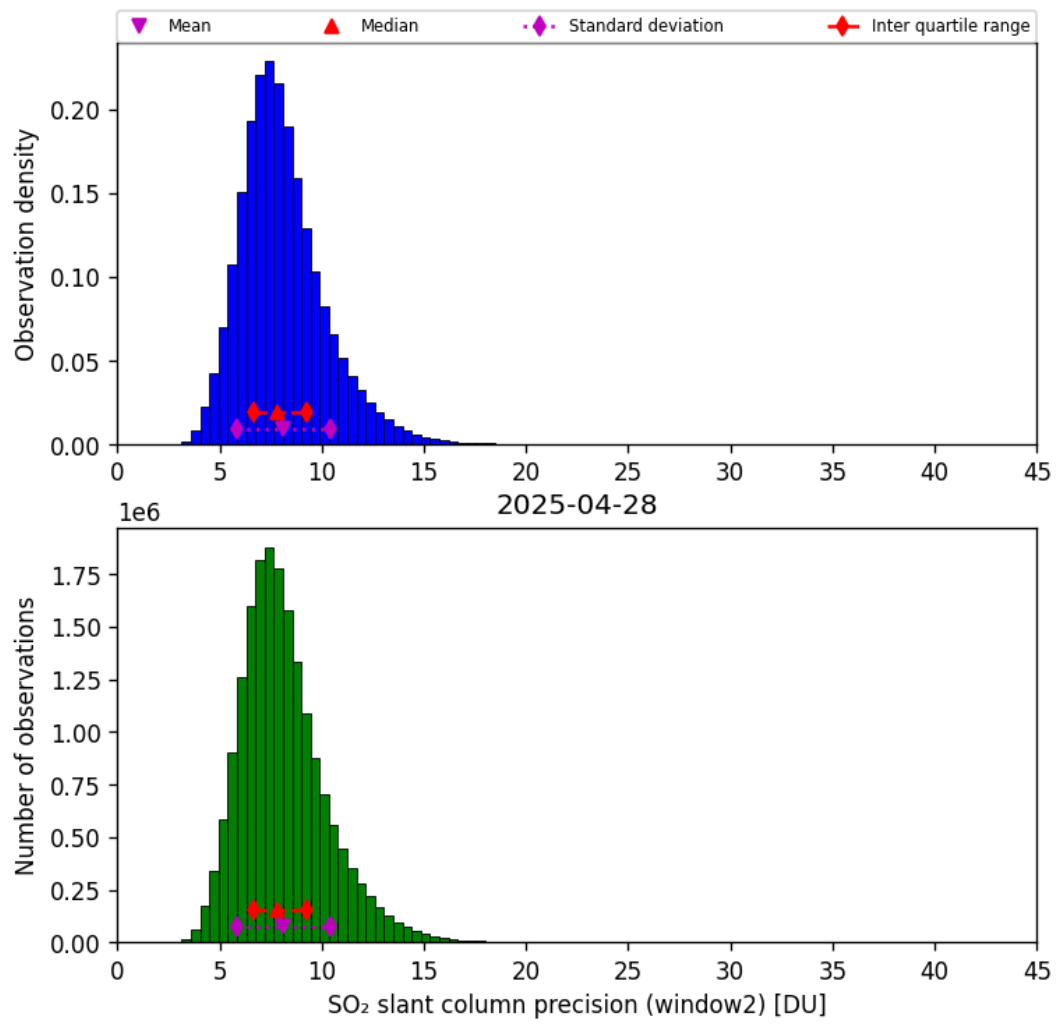
Figure 68: Histogram of “SO 2 slant column precision (window2)” for 2025-04-28 to 2025-04-29
