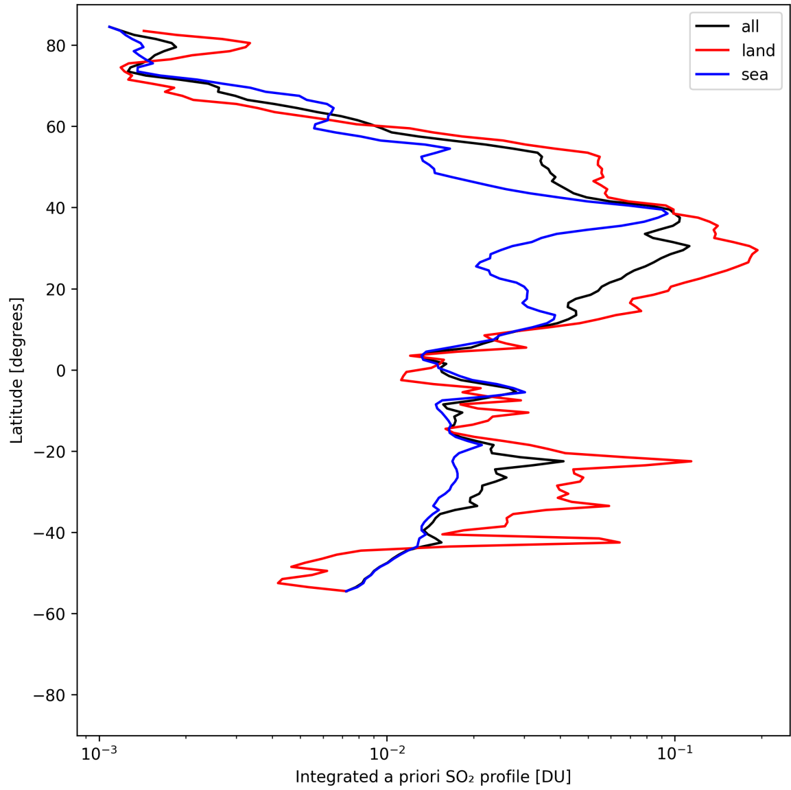
Figure 49: Zonal average of “Integrated a priori SO 2 profile” for 2025-04-28 to 2025-04-29.
