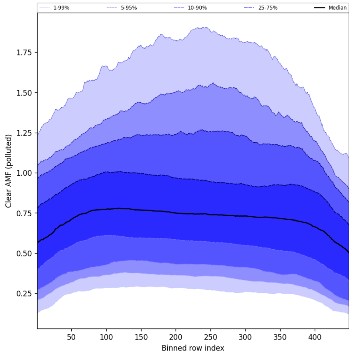
Figure 109: Along track statistics of “Clear AMF (polluted)” for 2025-04-28 to 2025-04-29
