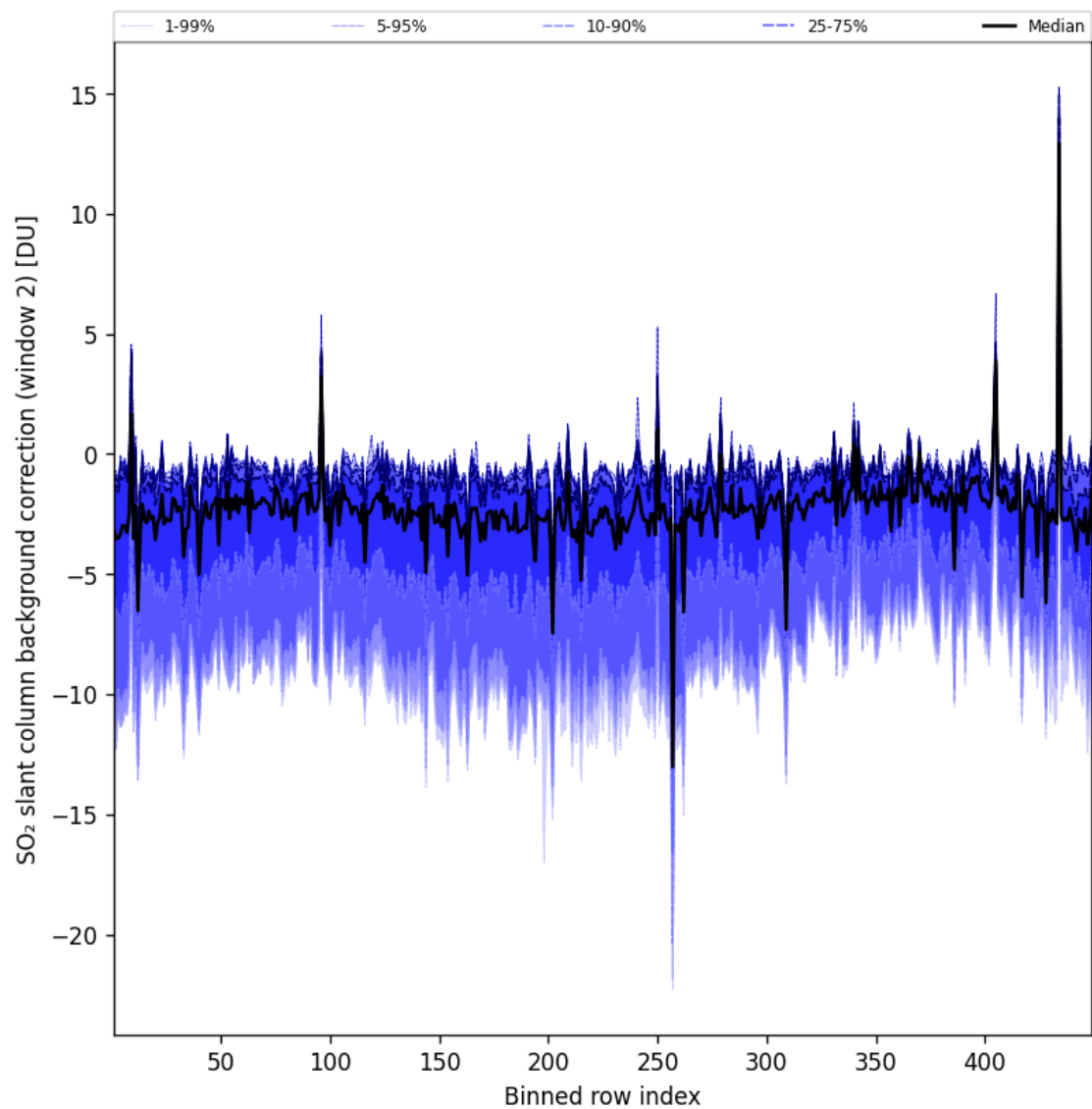
Figure 97: Along track statistics of “SO 2 slant column background correction (window 2)” for 2025-04-28 to 2025-04-29
