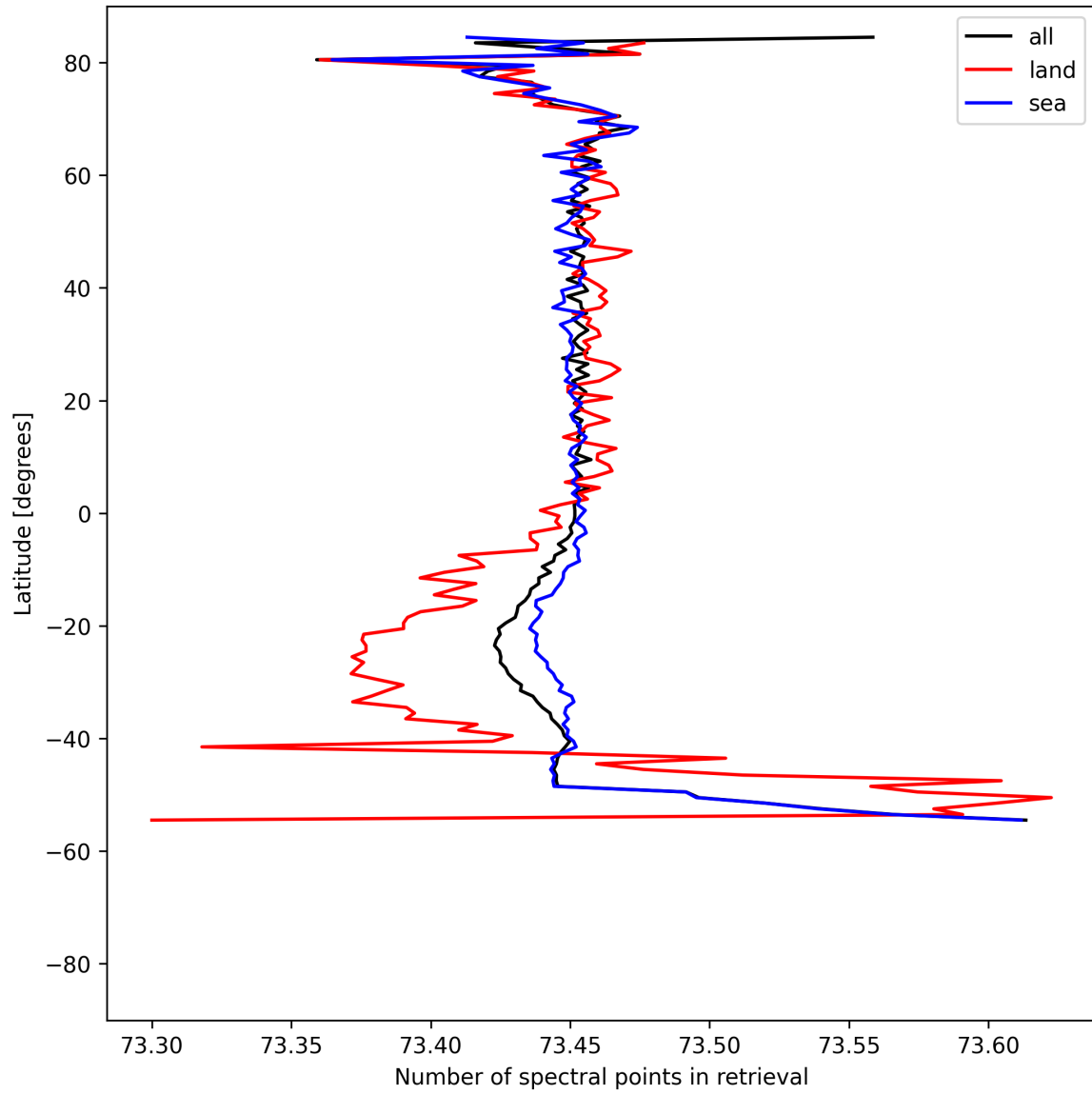
Figure 56: Zonal average of “Number of spectral points in retrieval” for 2025-04-28 to 2025-04-29.
