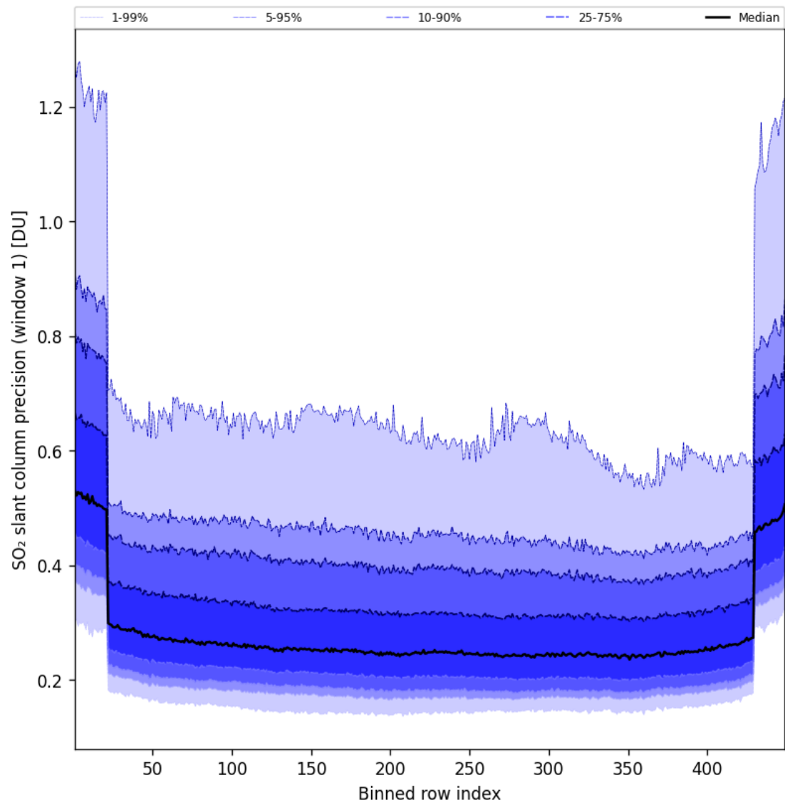
Figure 91: Along track statistics of “SO 2 slant column precision (window 1)” for 2025-04-28 to 2025-04-29
