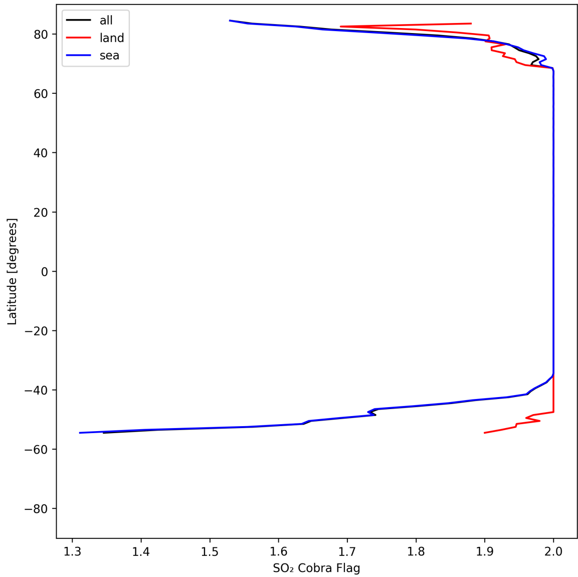
Figure 48: Zonal average of "SO 2 Cobra Flag" for 2025-04-28 to 2025-04-29.
