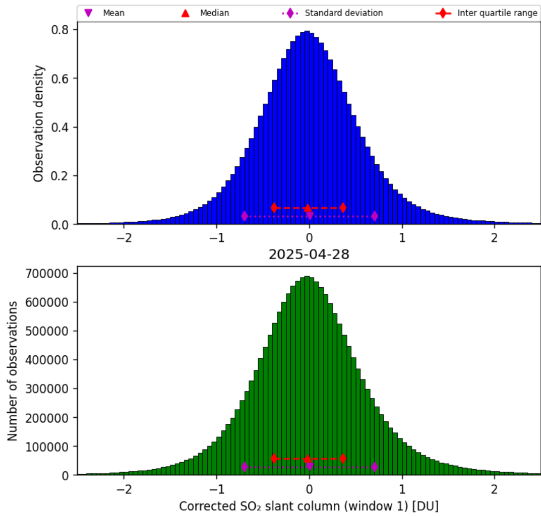
Figure 65: Histogram of “Corrected SO 2 slant column (window 1)” for 2025-04-28 to 2025-04-29
