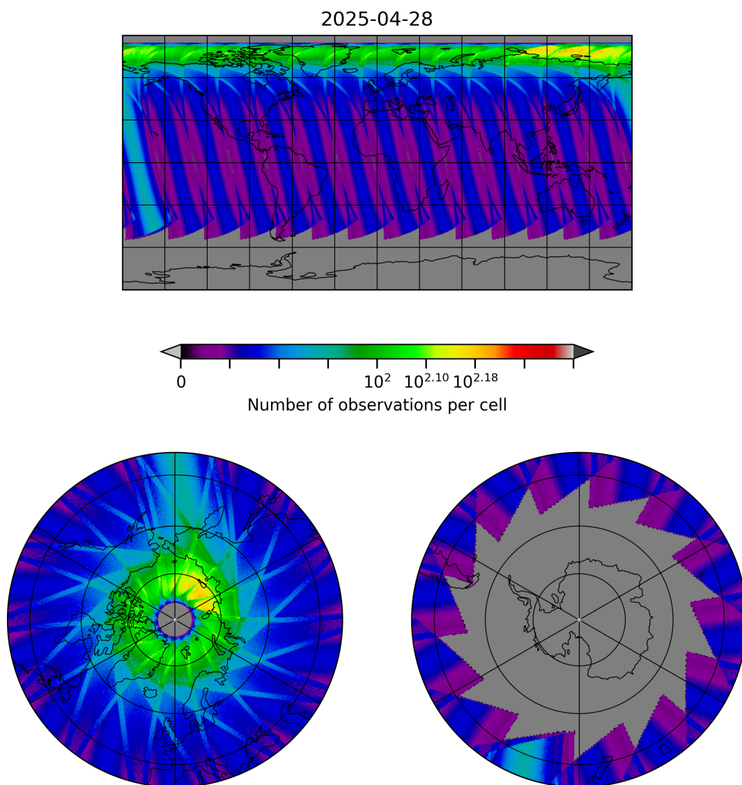
Figure 29: Map of the number of observations for 2025-04-28 to 2025-04-29
