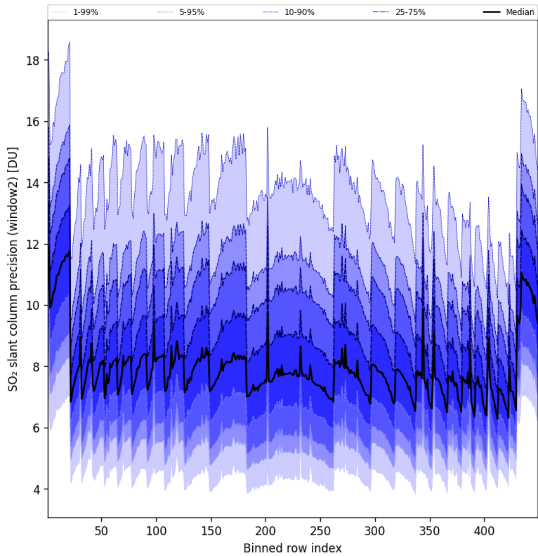
Figure 95: Along track statistics of “SO 2 slant column precision (window2)” for 2025-04-28 to 2025-04-29
