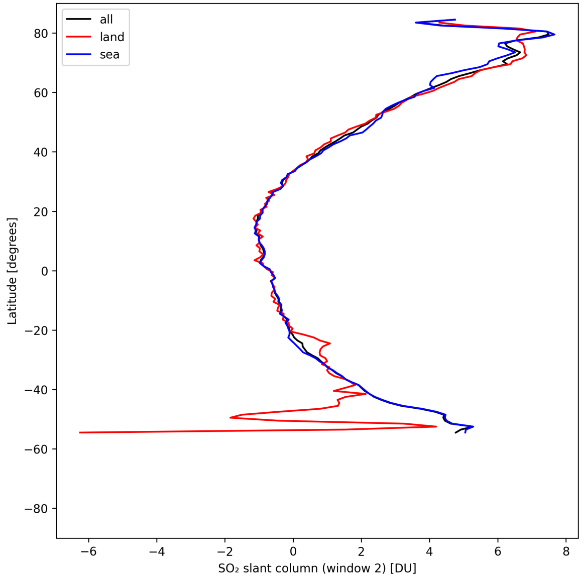
Figure 40: Zonal average of “SO 2 slant column (window 2)” for 2025-04-28 to 2025-04-29.
