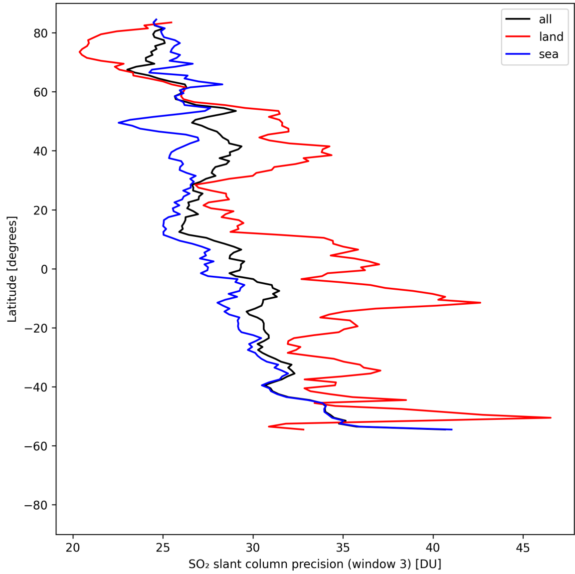
Figure 45: Zonal average of “SO 2 slant column precision (window 3)” for 2025-04-28 to 2025-04-29.
