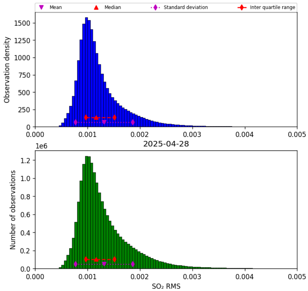
Figure 79: Histogram of “SO 2 RMS” for 2025-04-28 to 2025-04-29
