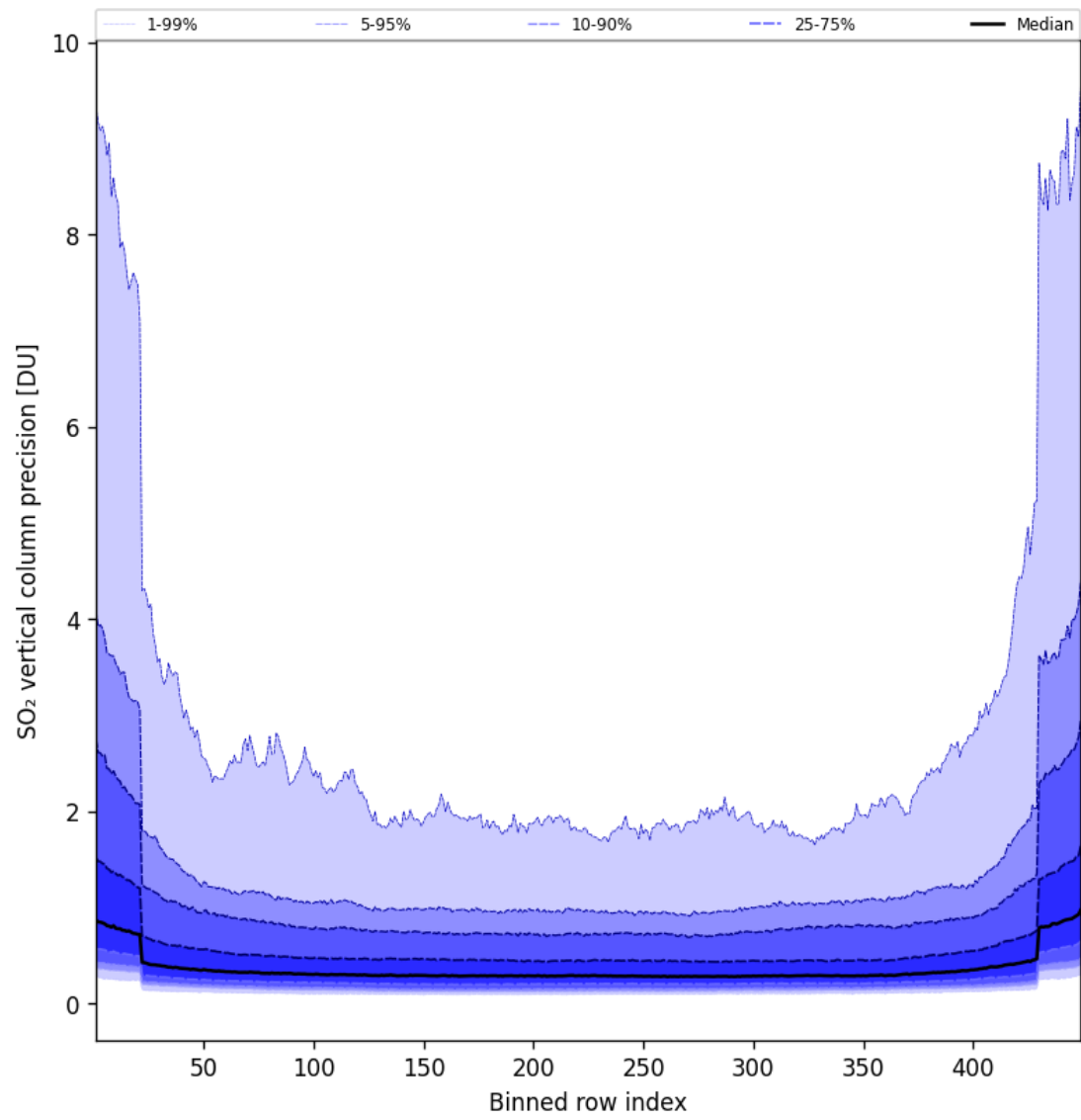
Figure 86: Along track statistics of “SO 2 vertical column precision” for 2025-04-28 to 2025-04-29
