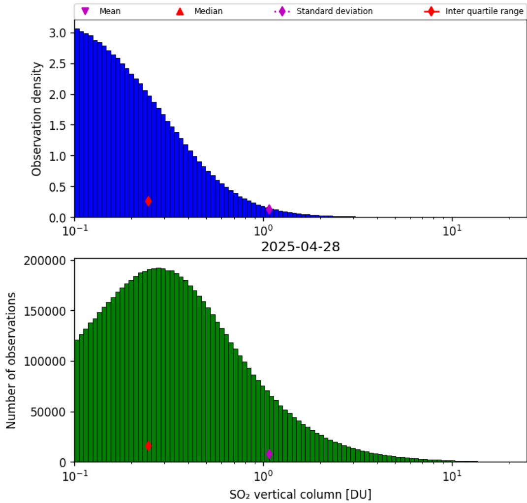
Figure 58: Histogram of “SO 2 vertical column” for 2025-04-28 to 2025-04-29
