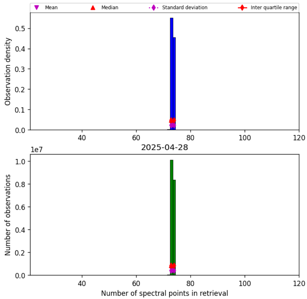
Figure 83: Histogram of “Number of spectral points in retrieval” for 2025-04-28 to 2025-04-29
