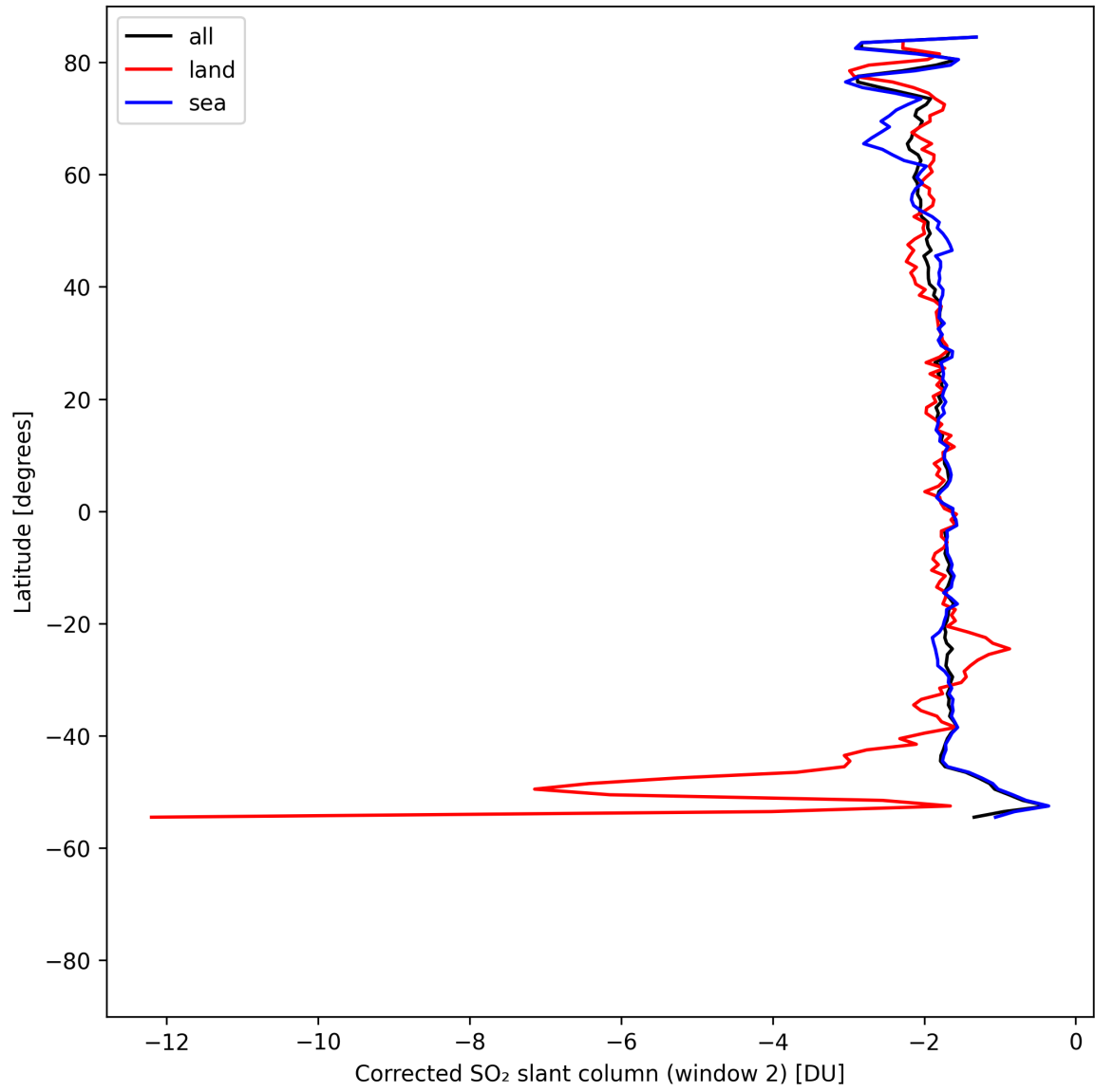
Figure 42: Zonal average of “Corrected SO 2 slant column (window 2)” for 2025-04-28 to 2025-04-29.
