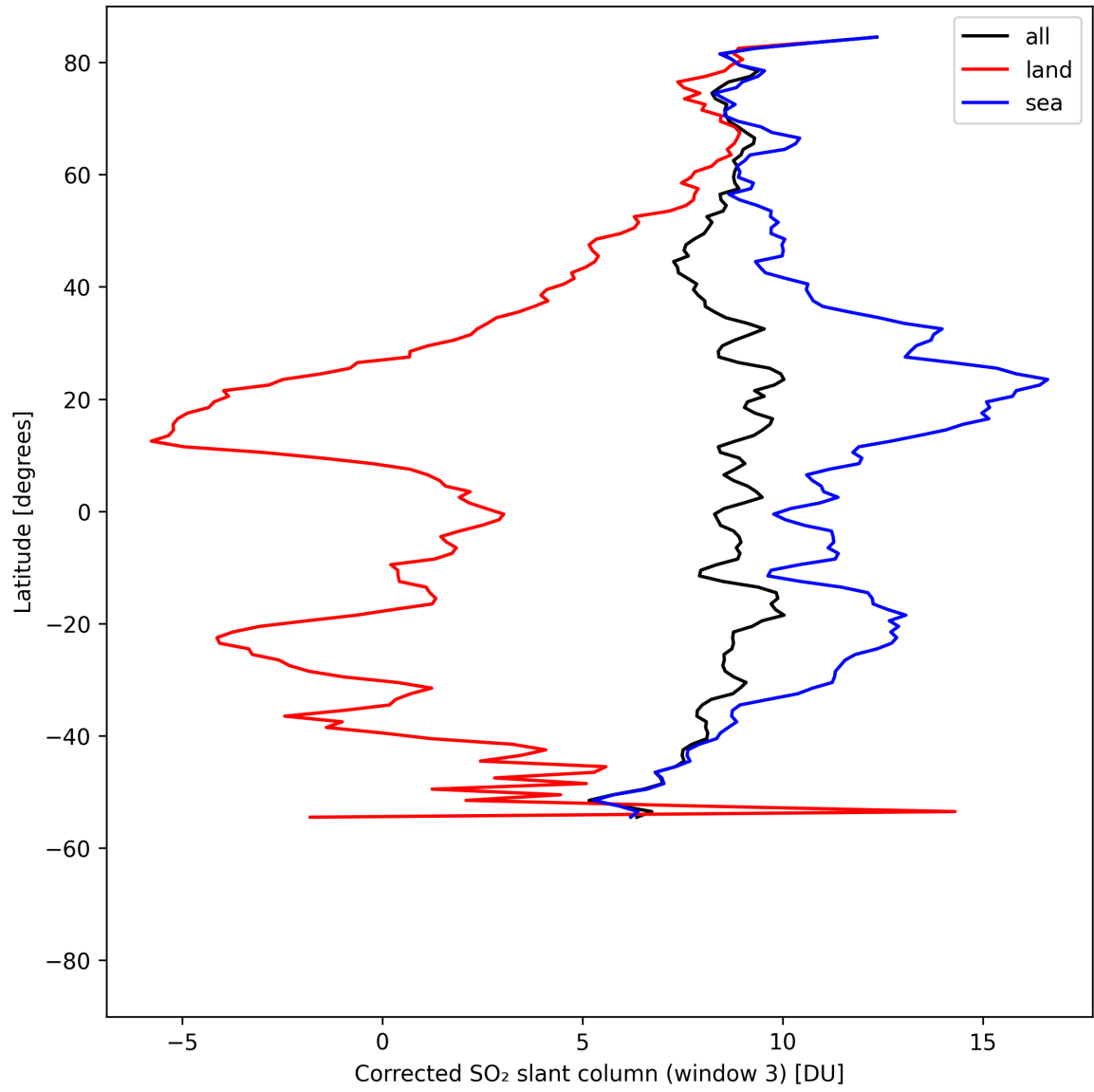
Figure 46: Zonal average of “Corrected SO 2 slant column (window 3)” for 2025-04-28 to 2025-04-29.
