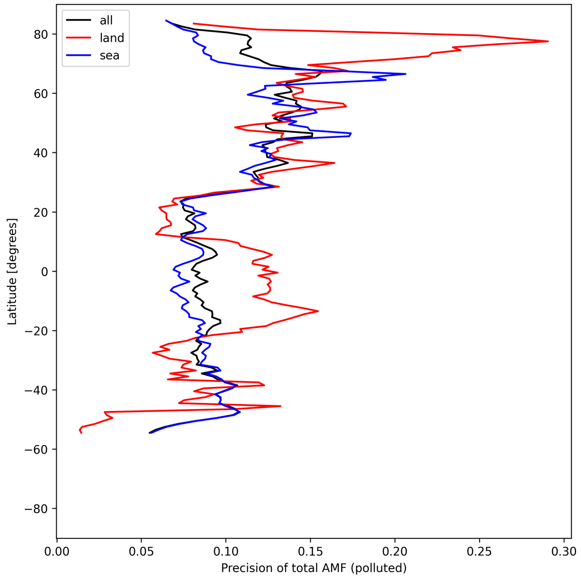
Figure 54: Zonal average of “Precision of total AMF (polluted)” for 2025-04-28 to 2025-04-29.
