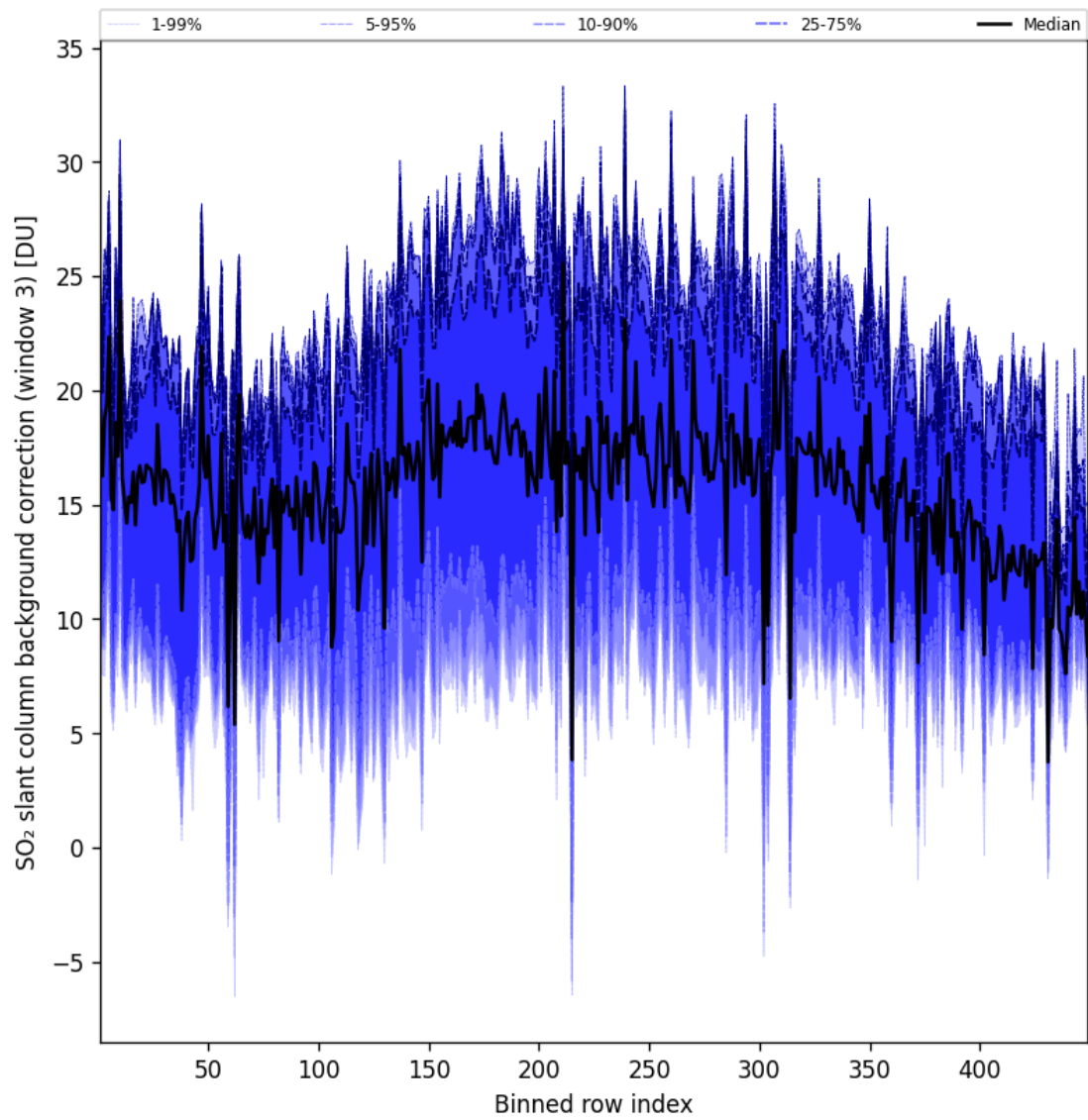
Figure 101: Along track statistics of “SO 2 slant column background correction (window 3)” for 2025-04-28 to 2025-04-29
