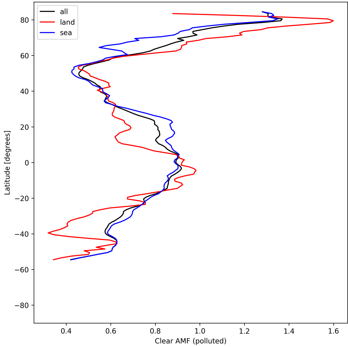
Figure 55: Zonal average of “Clear AMF (polluted)” for 2025-04-28 to 2025-04-29.
