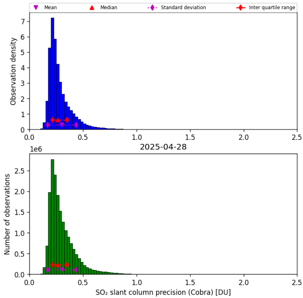
Figure 62: Histogram of “SO 2 slant column precision (Cobra)” for 2025-04-28 to 2025-04-29
