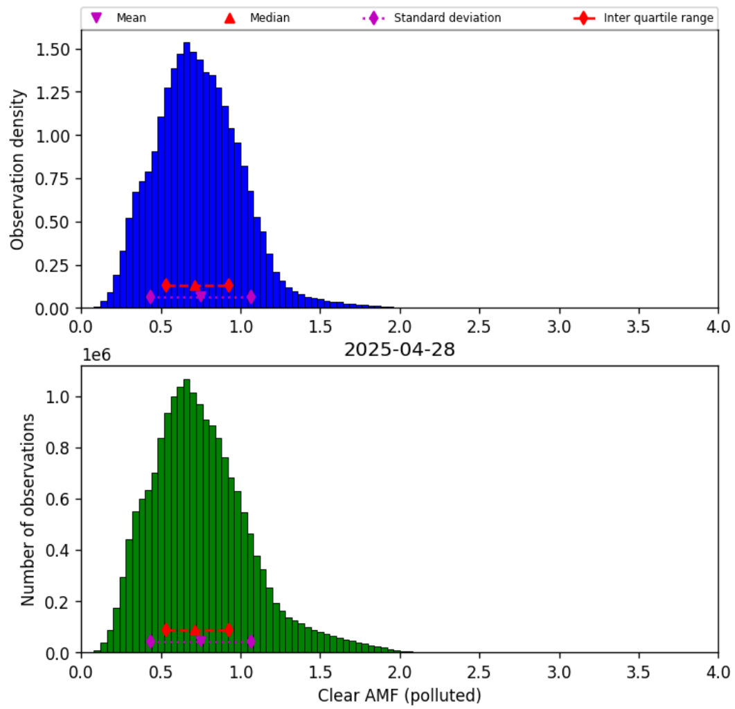
Figure 82: Histogram of “Clear AMF (polluted)” for 2025-04-28 to 2025-04-29
