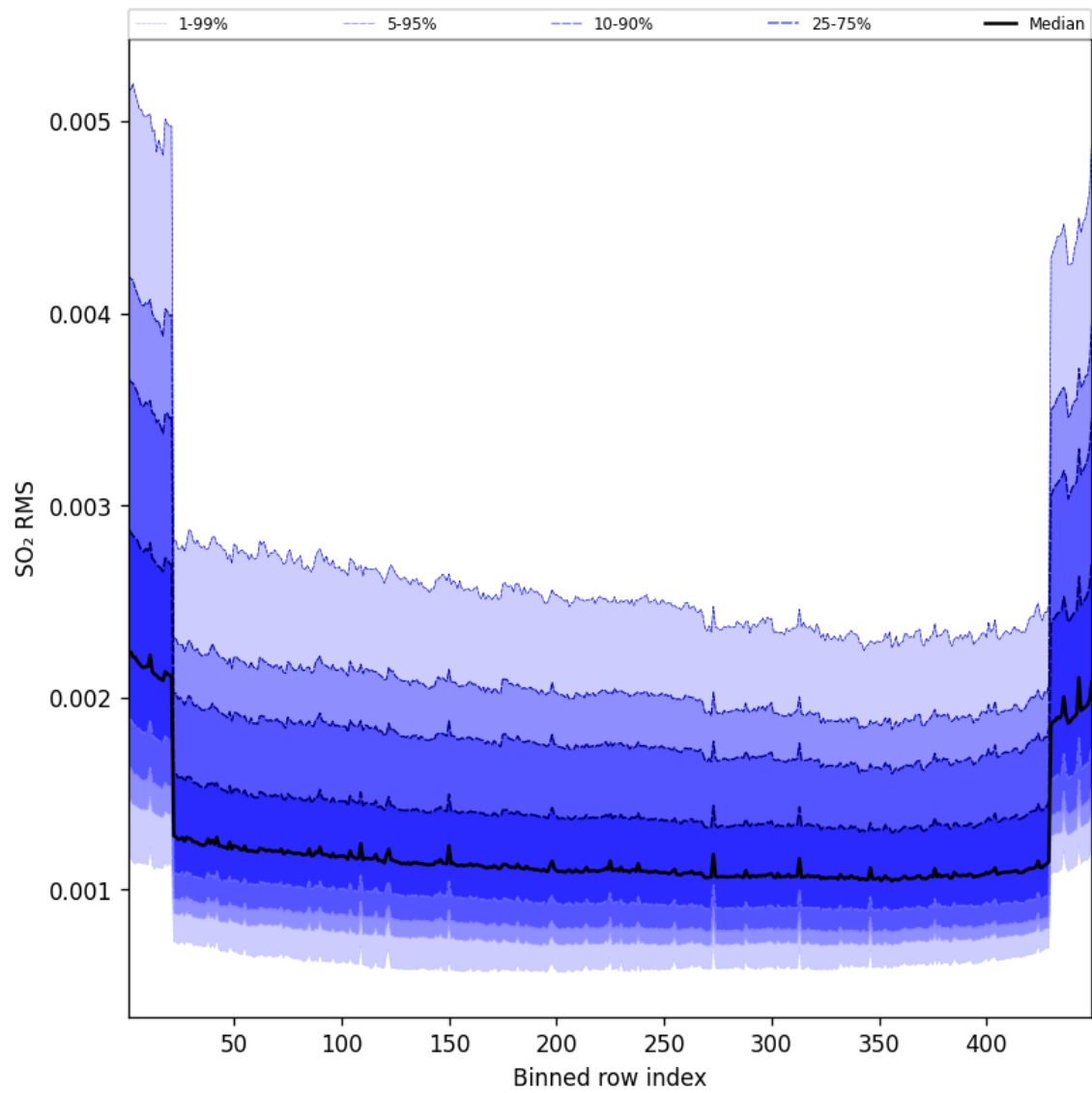
Figure 106: Along track statistics of “SO 2 RMS” for 2025-04-28 to 2025-04-29
