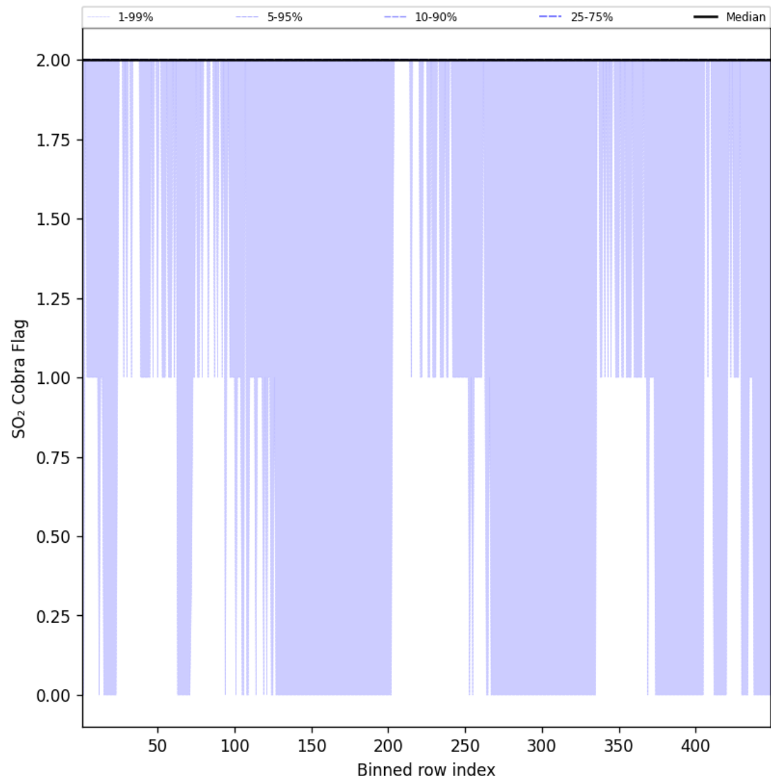
Figure 102: Along track statistics of “SO 2 Cobra Flag” for 2025-04-28 to 2025-04-29
