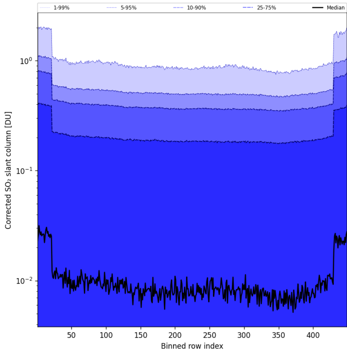
Figure 87: Along track statistics of “Corrected SO 2 slant column” for 2025-04-28 to 2025-04-29
