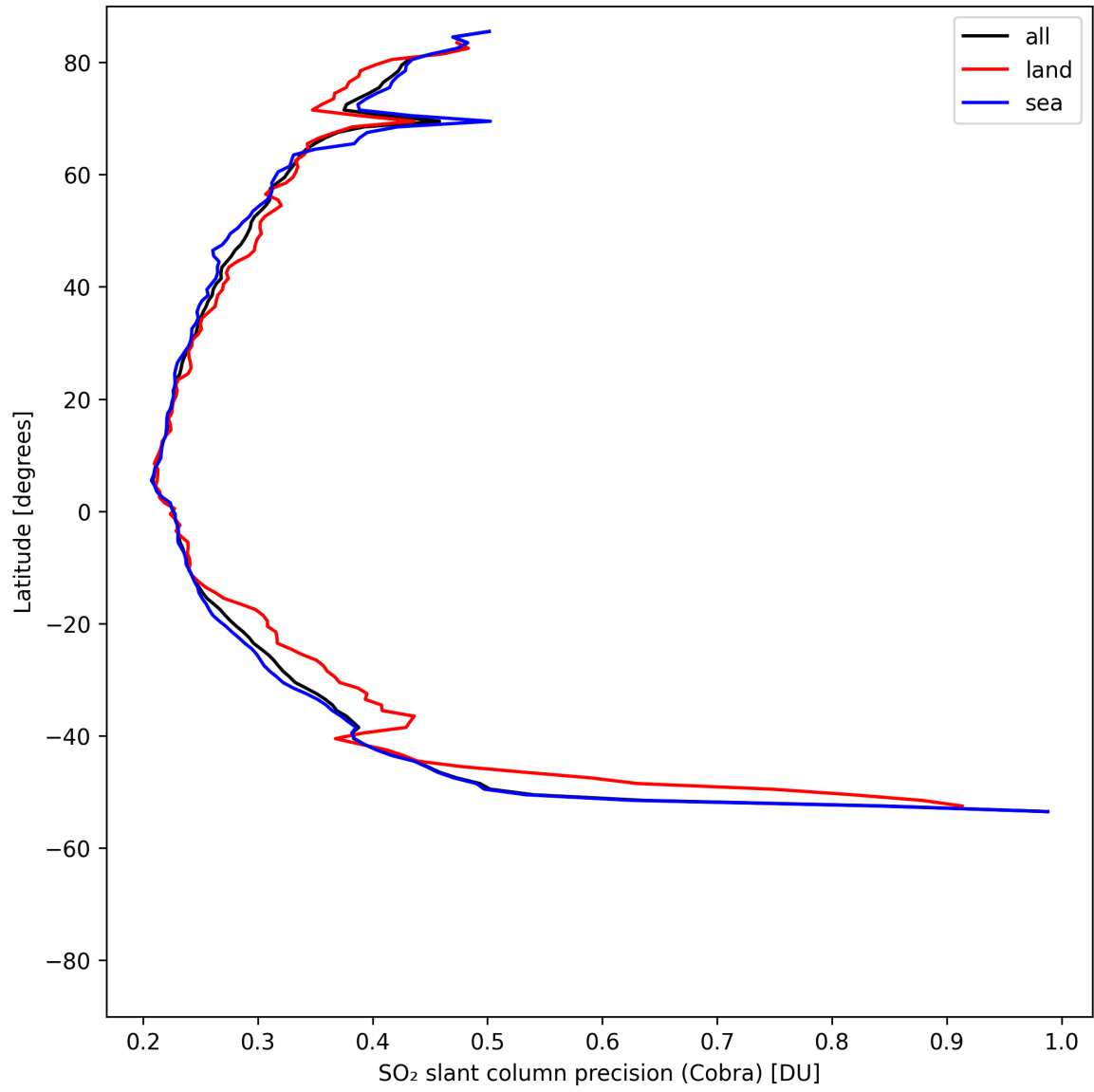
Figure 35: Zonal average of “SO 2 slant column precision (Cobra)” for 2025-05-03 to 2025-05-03.
