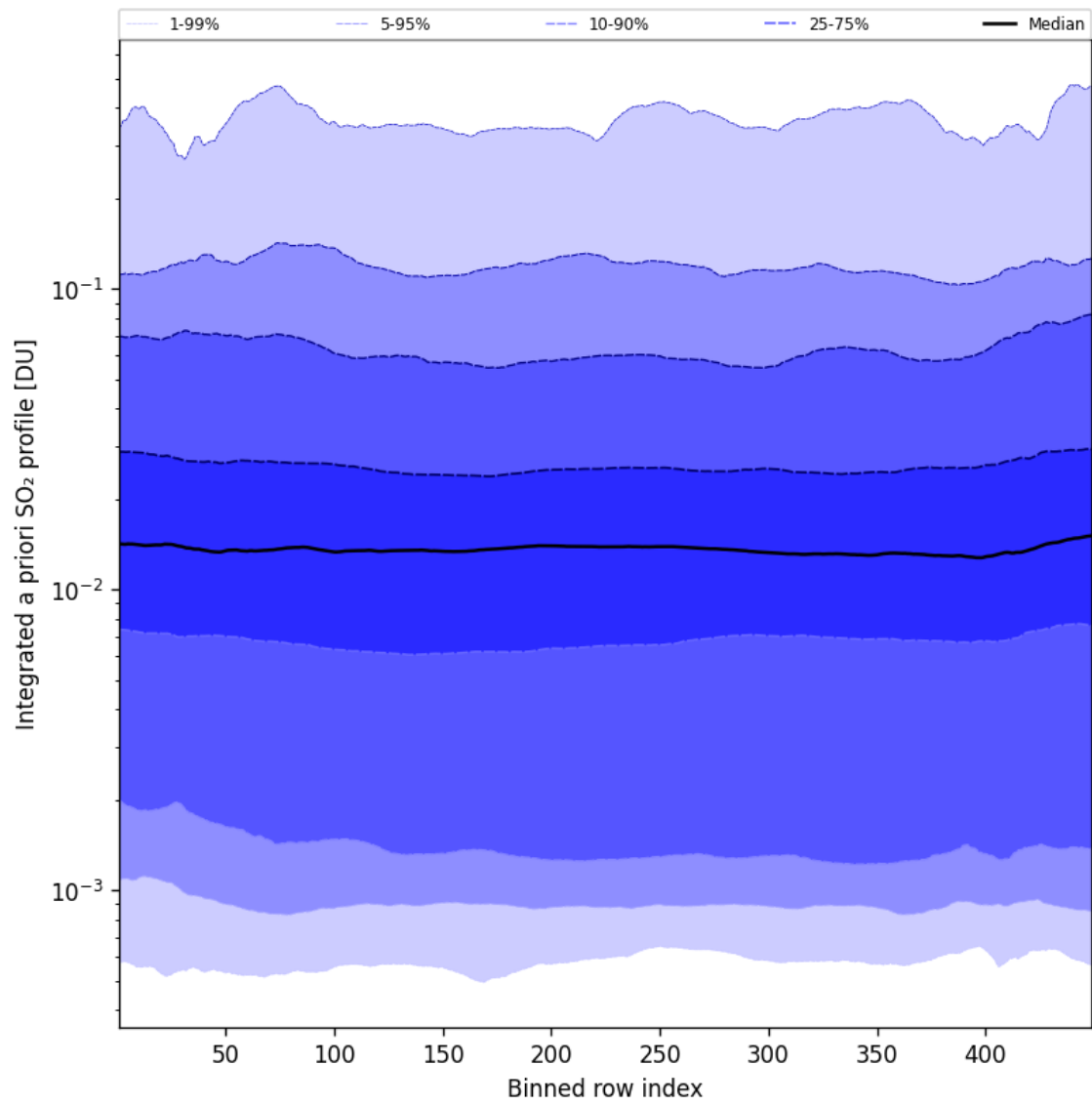
Figure 103: Along track statistics of “Integrated a priori SO 2 profile” for 2025-05-03 to 2025-05-03
