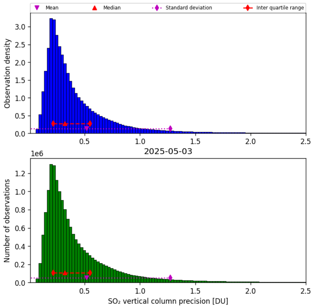
Figure 59: Histogram of “SO 2 vertical column precision” for 2025-05-03 to 2025-05-03
