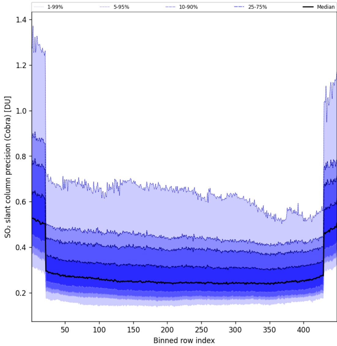
Figure 89: Along track statistics of “SO 2 slant column precision (Cobra)” for 2025-05-03 to 2025-05-03
