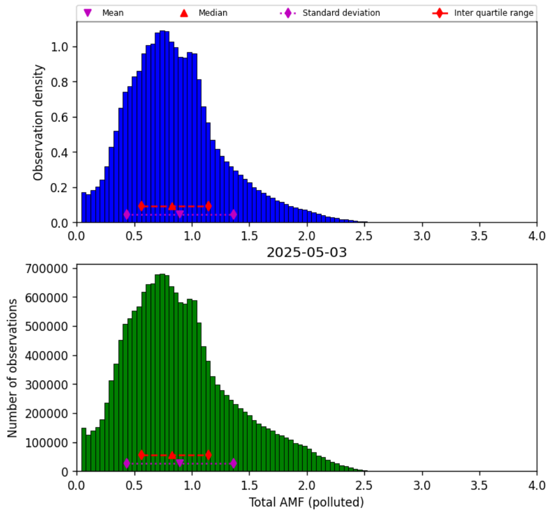
Figure 80: Histogram of “Total AMF (polluted)” for 2025-05-03 to 2025-05-03
