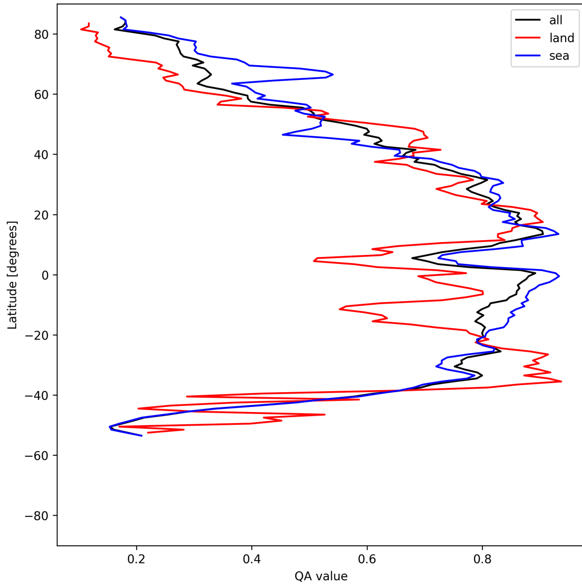
Figure 30: Zonal average of “QA value” for 2025-05-03 to 2025-05-03.
