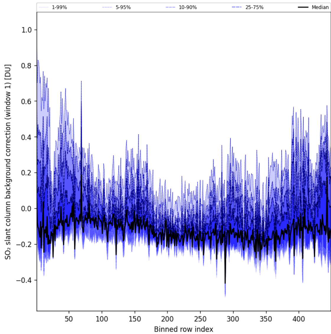
Figure 93: Along track statistics of “SO 2 slant column background correction (window 1)” for 2025-05-03 to 2025-05-03
