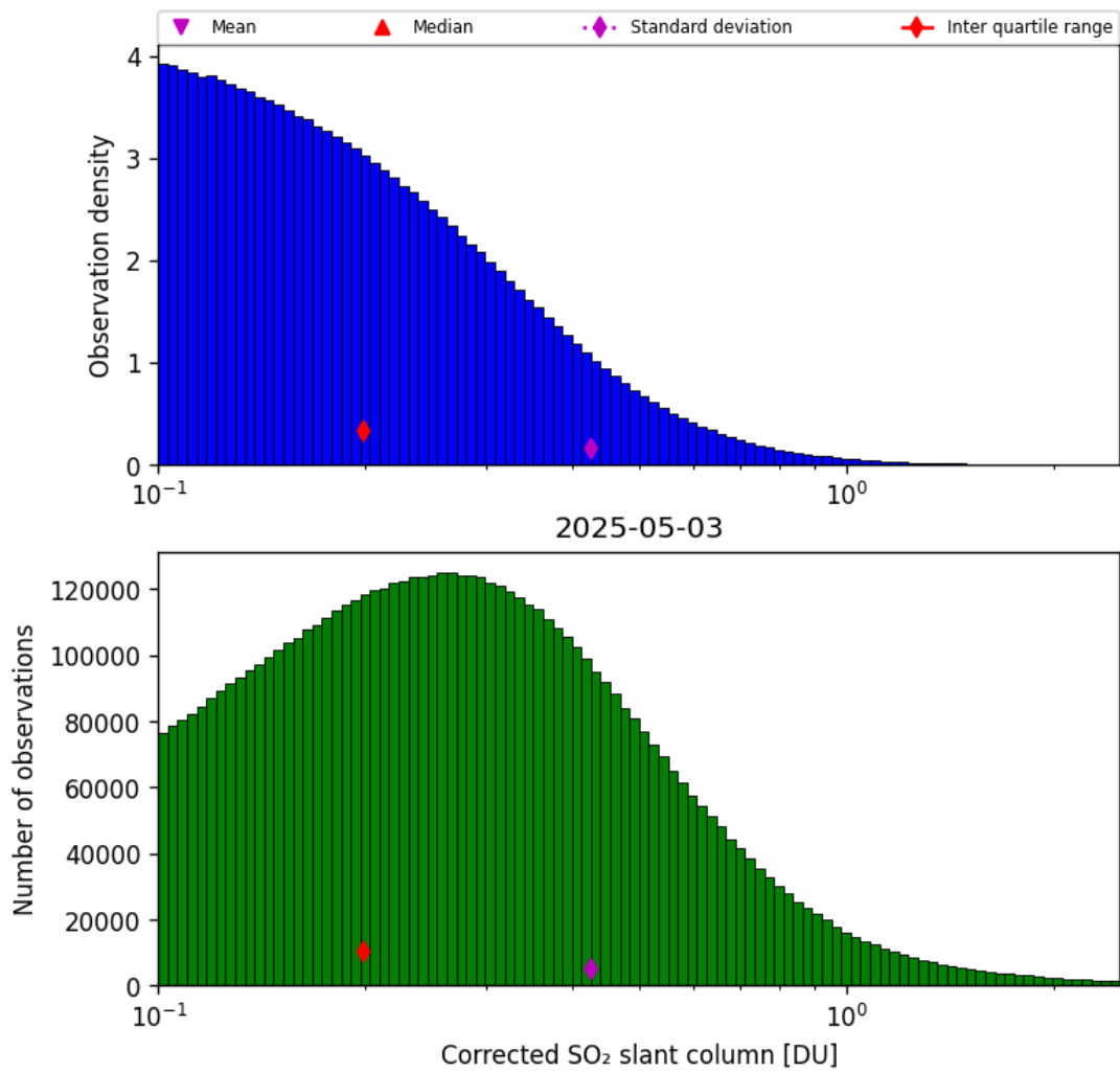
Figure 60: Histogram of “Corrected SO 2 slant column” for 2025-05-03 to 2025-05-03
