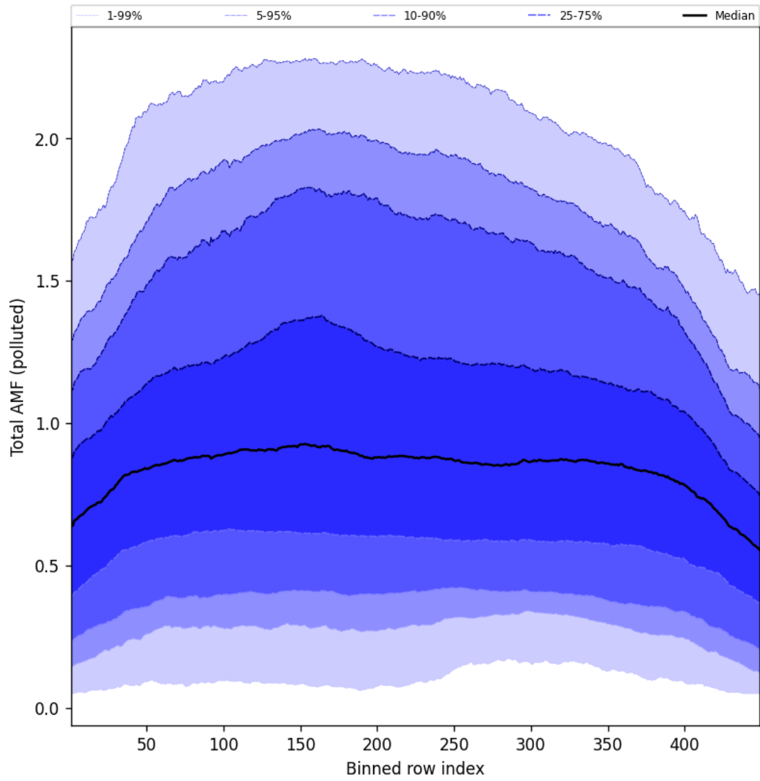
Figure 107: Along track statistics of “Total AMF (polluted)” for 2025-05-03 to 2025-05-03
