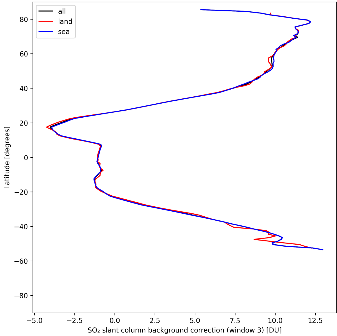
Figure 47: Zonal average of “SO 2 slant column background correction (window 3)” for 2025-05-03 to 2025-05-03.
