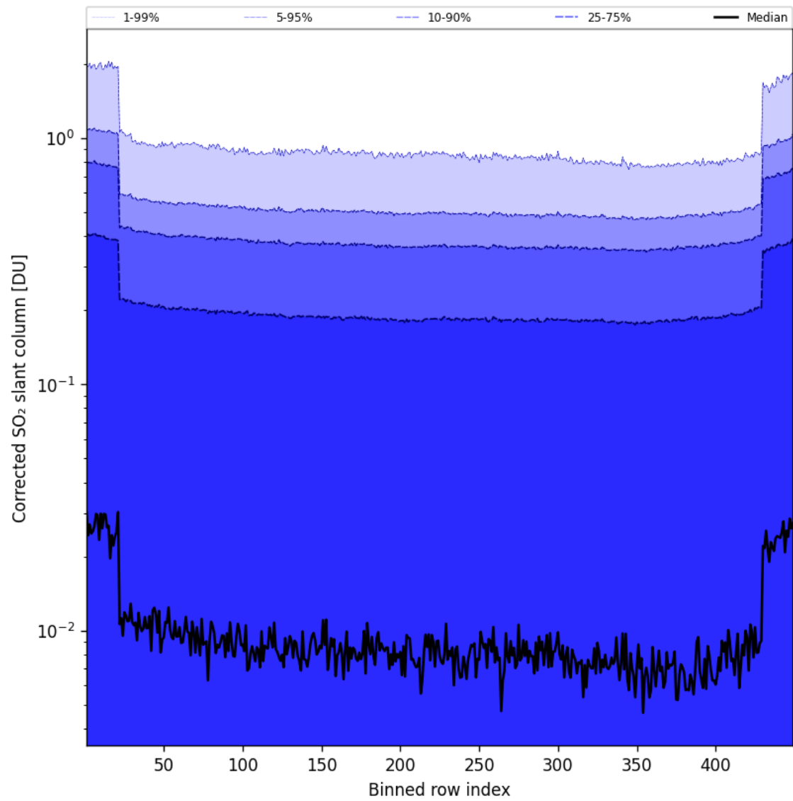
Figure 87: Along track statistics of “Corrected SO 2 slant column” for 2025-05-03 to 2025-05-03
