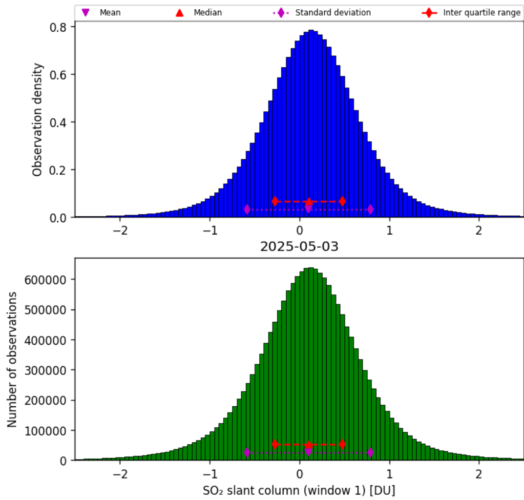
Figure 63: Histogram of “SO 2 slant column (window 1)” for 2025-05-03 to 2025-05-03
