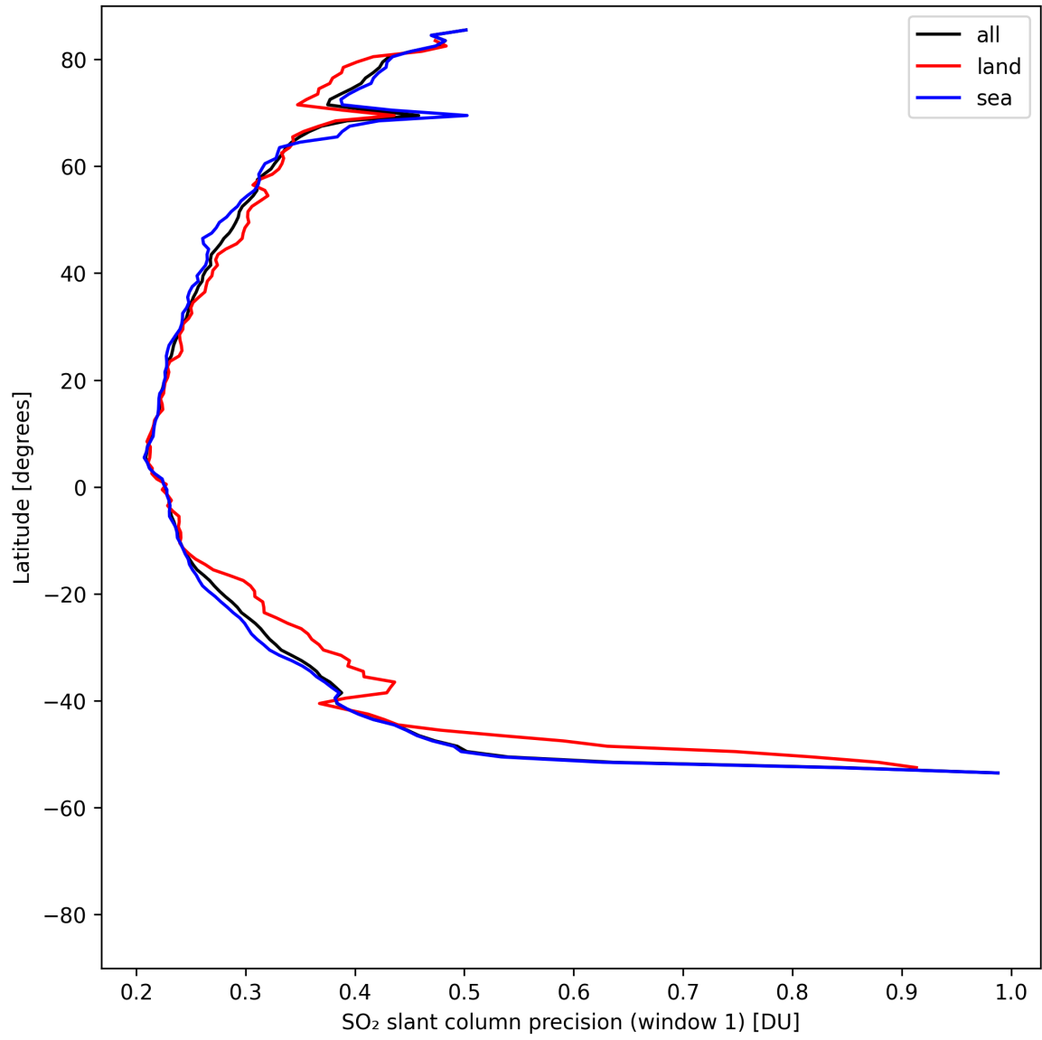
Figure 37: Zonal average of “SO 2 slant column precision (window 1)” for 2025-05-03 to 2025-05-03.
