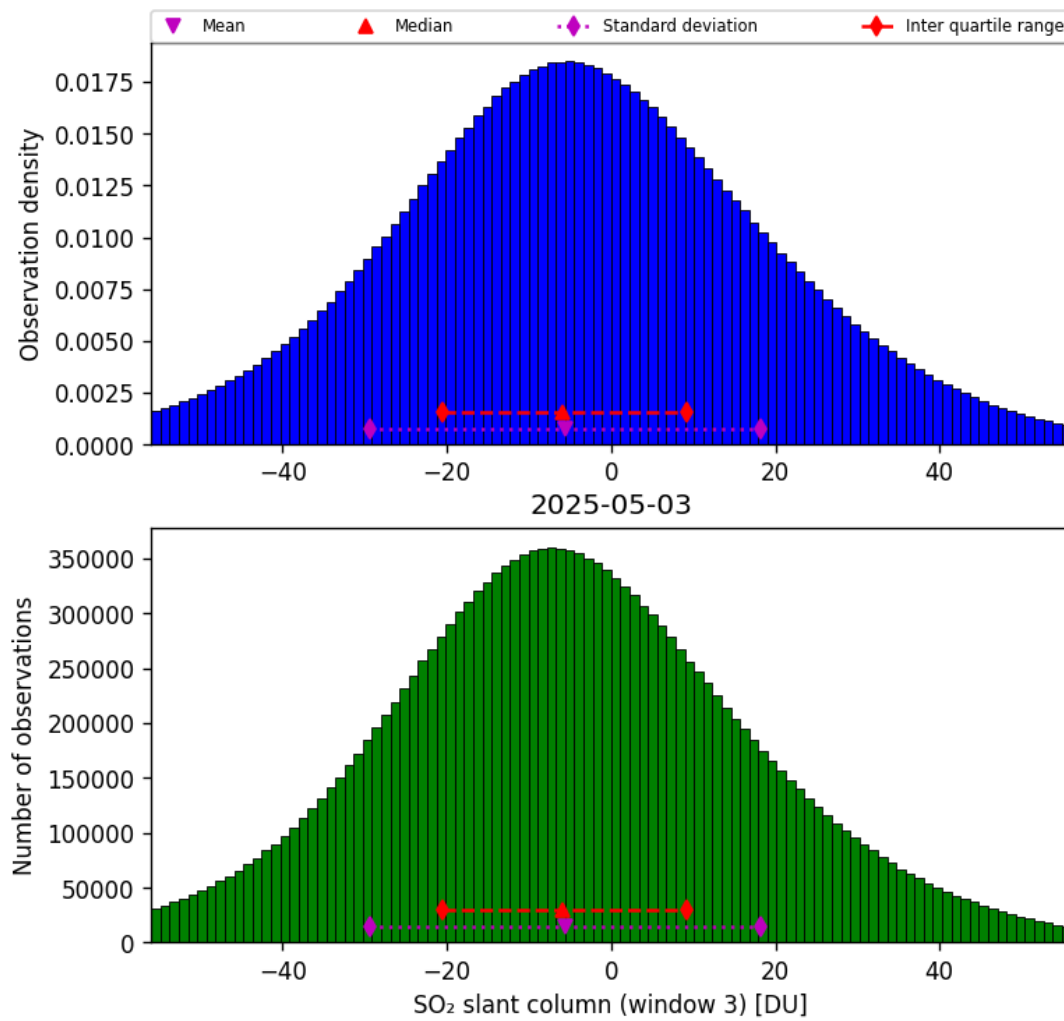
Figure 71: Histogram of “SO 2 slant column (window 3)” for 2025-05-03 to 2025-05-03
