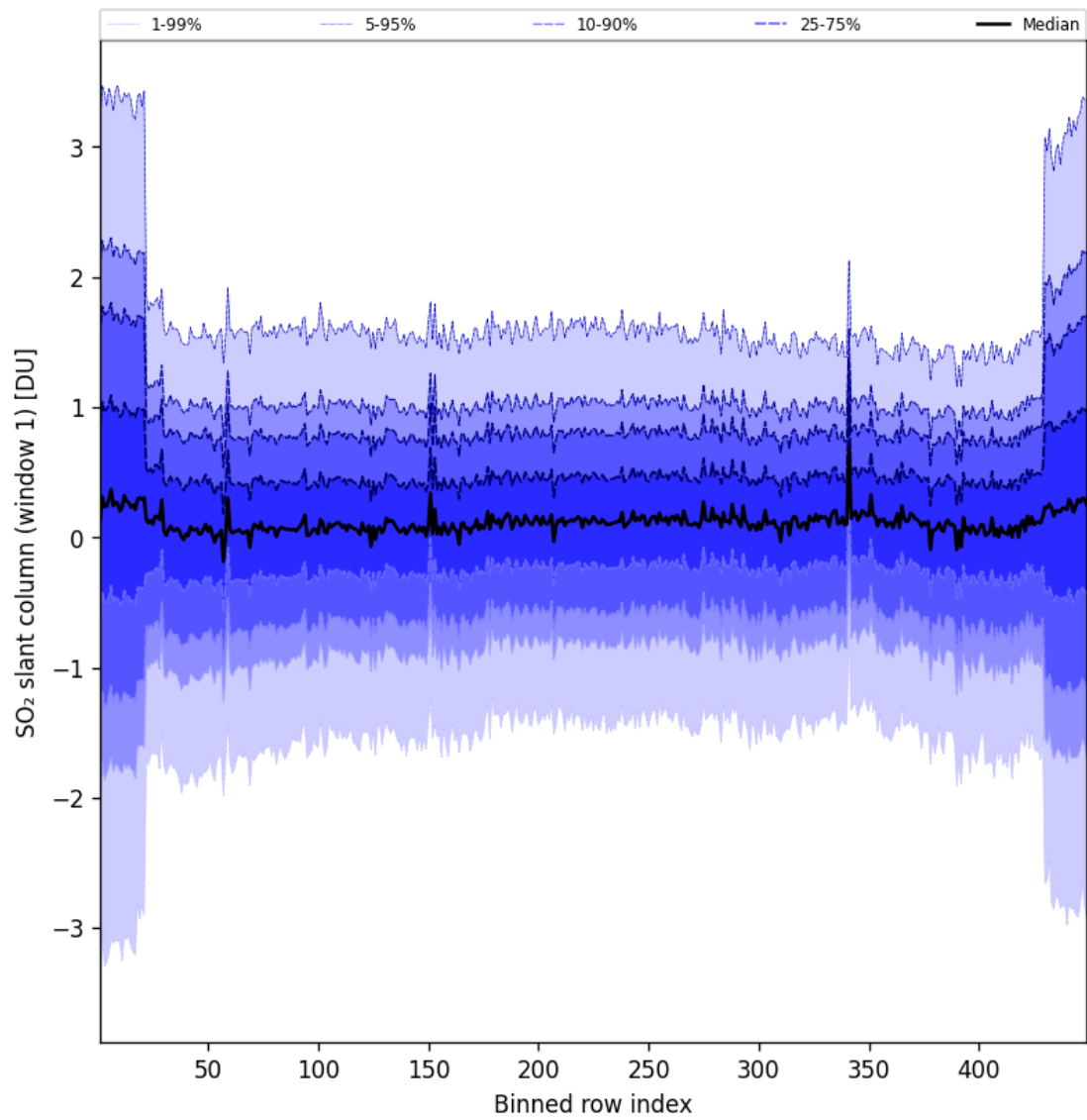
Figure 90: Along track statistics of “SO 2 slant column (window 1)” for 2025-05-03 to 2025-05-03
