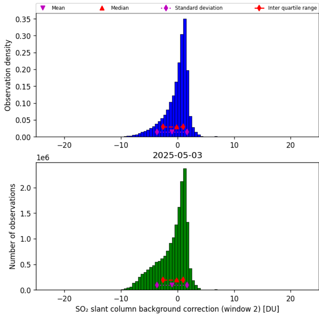
Figure 70: Histogram of “SO 2 slant column background correction (window 2)” for 2025-05-03 to 2025-05-03
