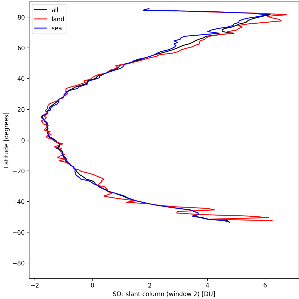
Figure 40: Zonal average of “SO 2 slant column (window 2)” for 2025-05-03 to 2025-05-03.
