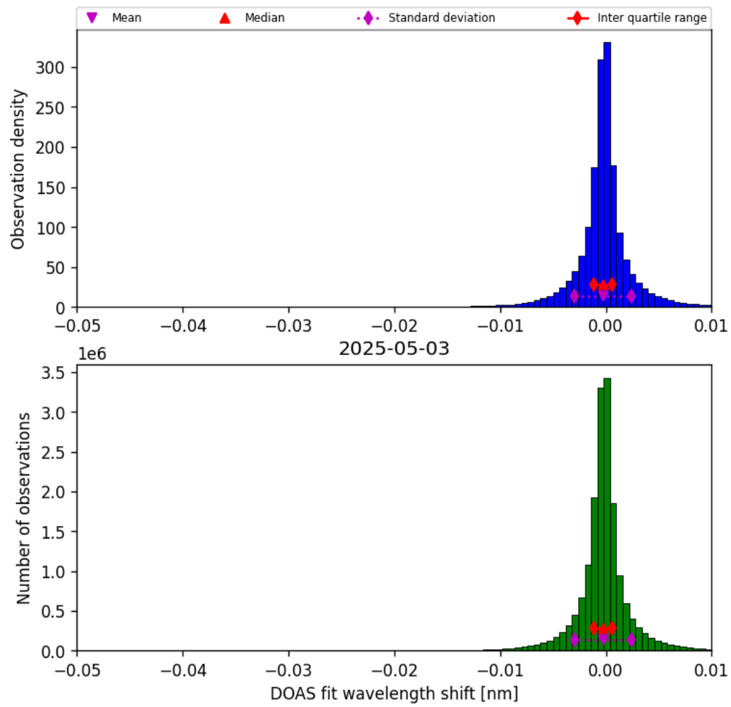
Figure 77: Histogram of “DOAS fit wavelength shift” for 2025-05-03 to 2025-05-03
