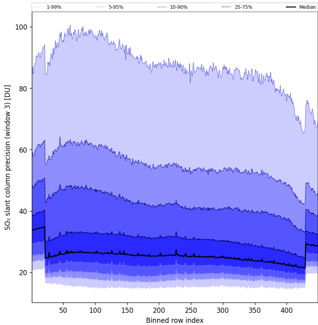
Figure 99: Along track statistics of “SO 2 slant column precision (window 3)” for 2025-05-03 to 2025-05-03
