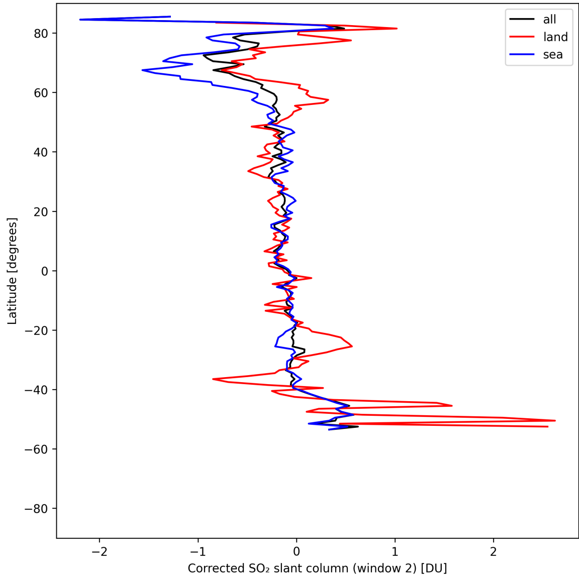
Figure 42: Zonal average of “Corrected SO 2 slant column (window 2)” for 2025-05-03 to 2025-05-03.
