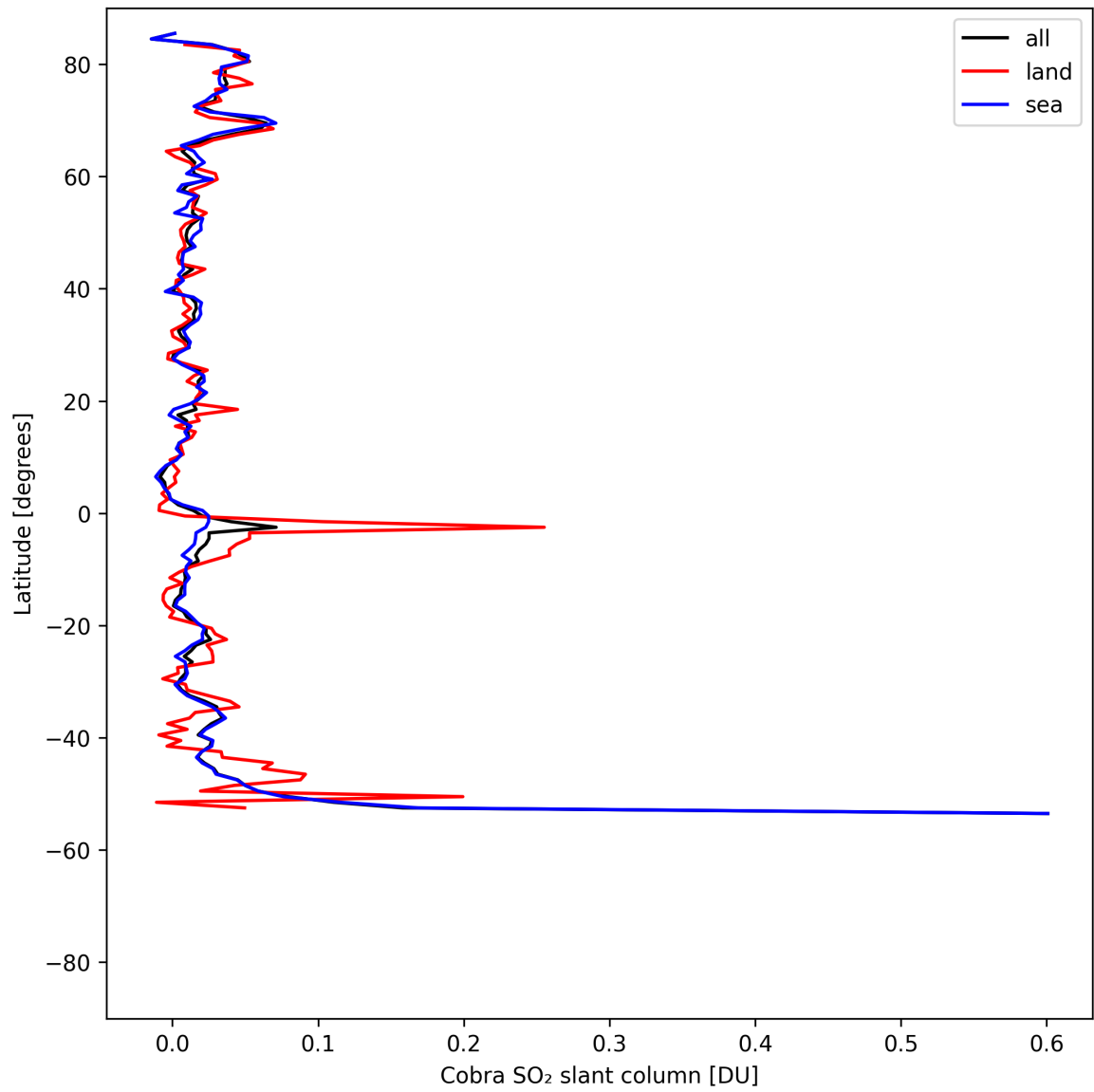
Figure 34: Zonal average of “Cobra SO 2 slant column” for 2025-05-03 to 2025-05-03.
