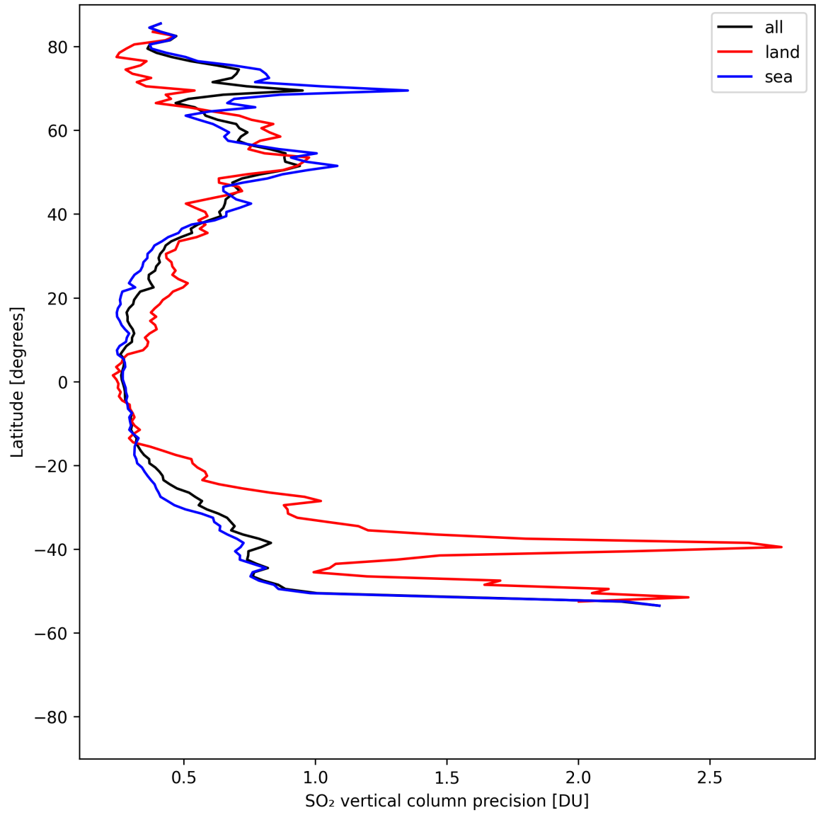
Figure 32: Zonal average of “SO 2 vertical column precision” for 2025-05-03 to 2025-05-03.
