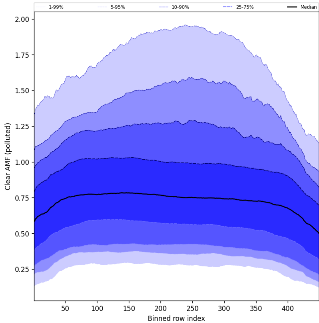
Figure 109: Along track statistics of “Clear AMF (polluted)” for 2025-05-03 to 2025-05-03
