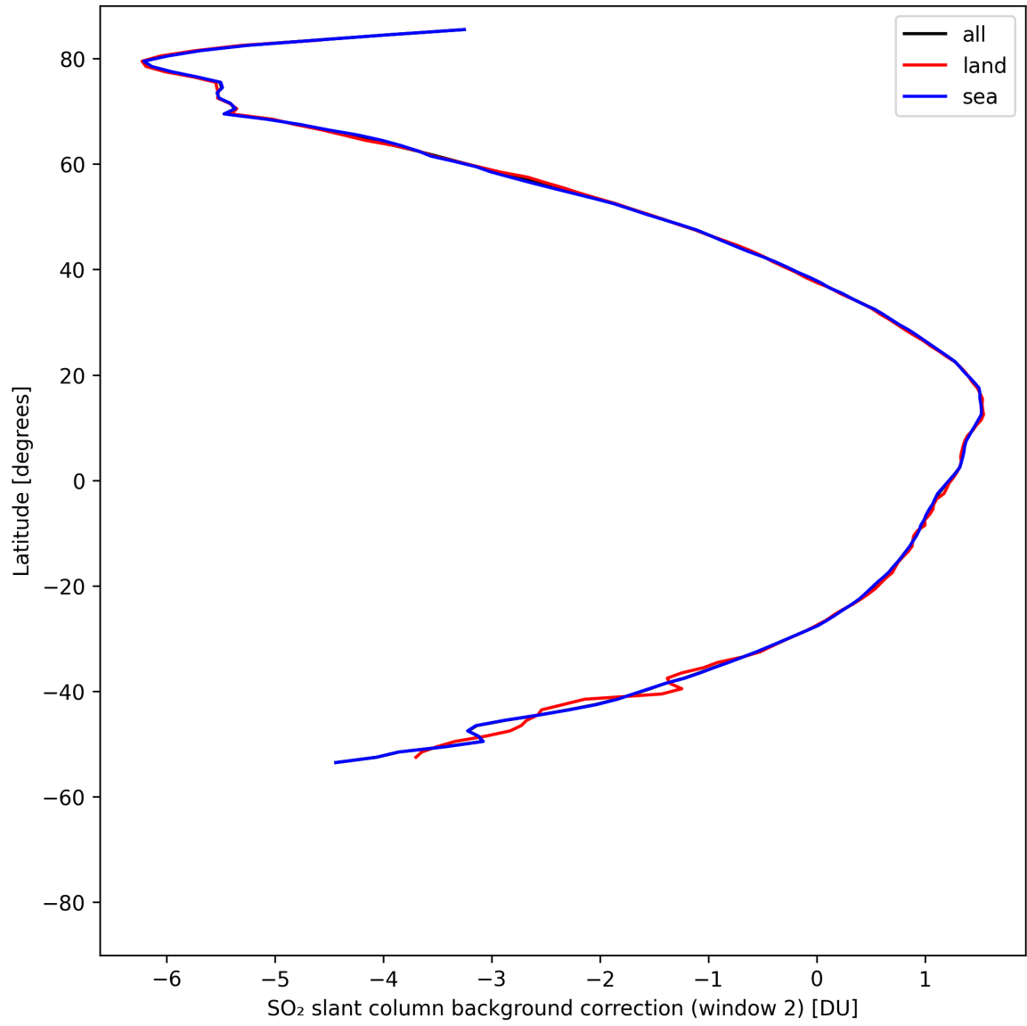
Figure 43: Zonal average of “SO 2 slant column background correction (window 2)” for 2025-05-03 to 2025-05-03.
