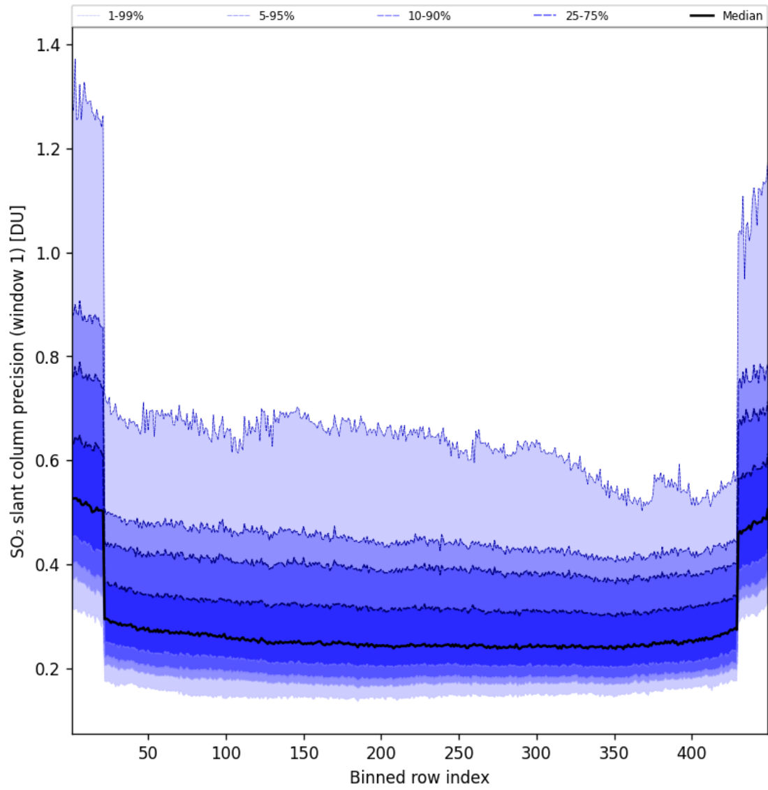
Figure 91: Along track statistics of “SO 2 slant column precision (window 1)” for 2025-05-03 to 2025-05-03
