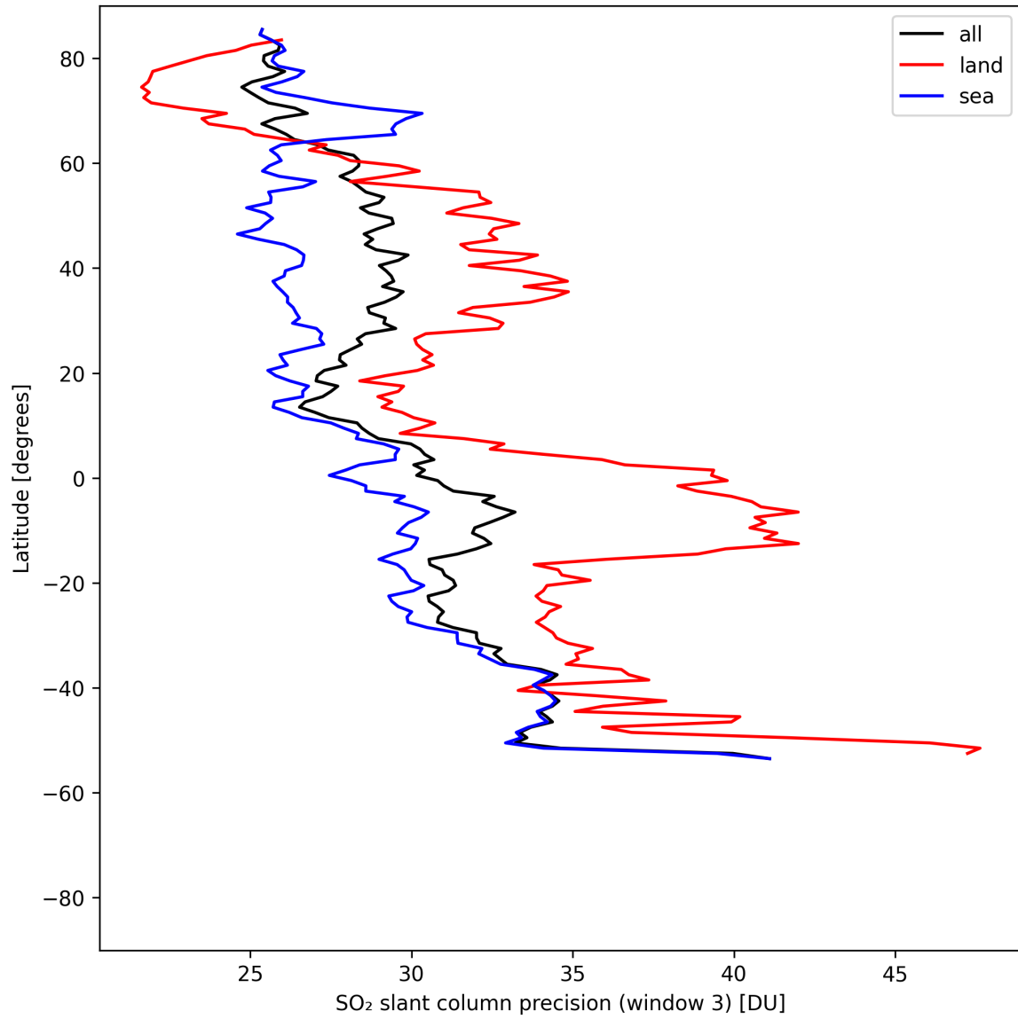
Figure 45: Zonal average of “SO 2 slant column precision (window 3)” for 2025-05-03 to 2025-05-03.
