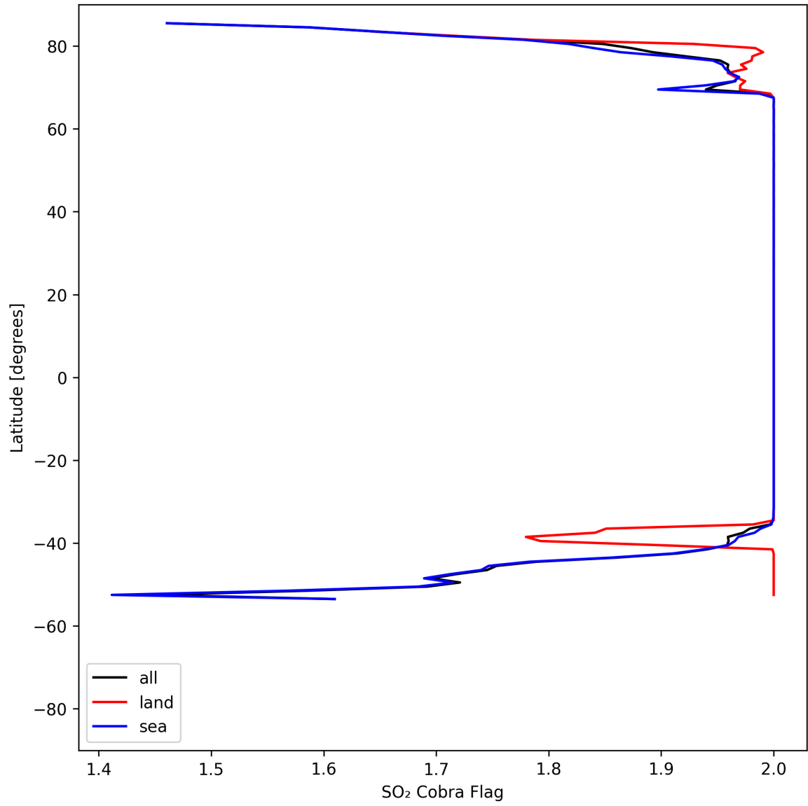
Figure 48: Zonal average of "SO 2 Cobra Flag" for 2025-05-03 to 2025-05-03.
