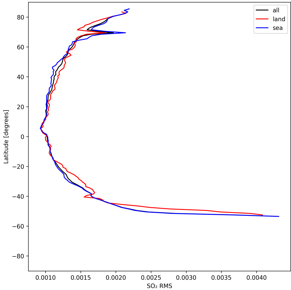
Figure 52: Zonal average of “SO 2 RMS” for 2025-05-03 to 2025-05-03.
