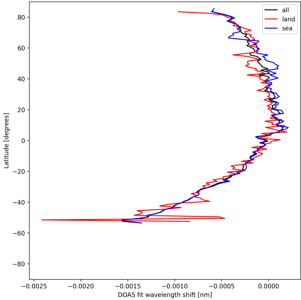
Figure 50: Zonal average of “DOAS fit wavelength shift” for 2025-05-03 to 2025-05-03.
