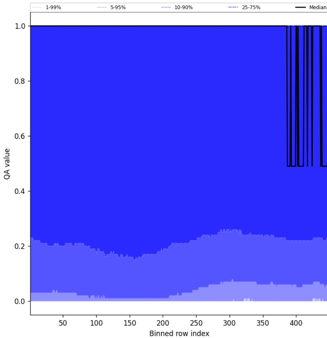
Figure 84: Along track statistics of “QA value” for 2025-05-03 to 2025-05-03
