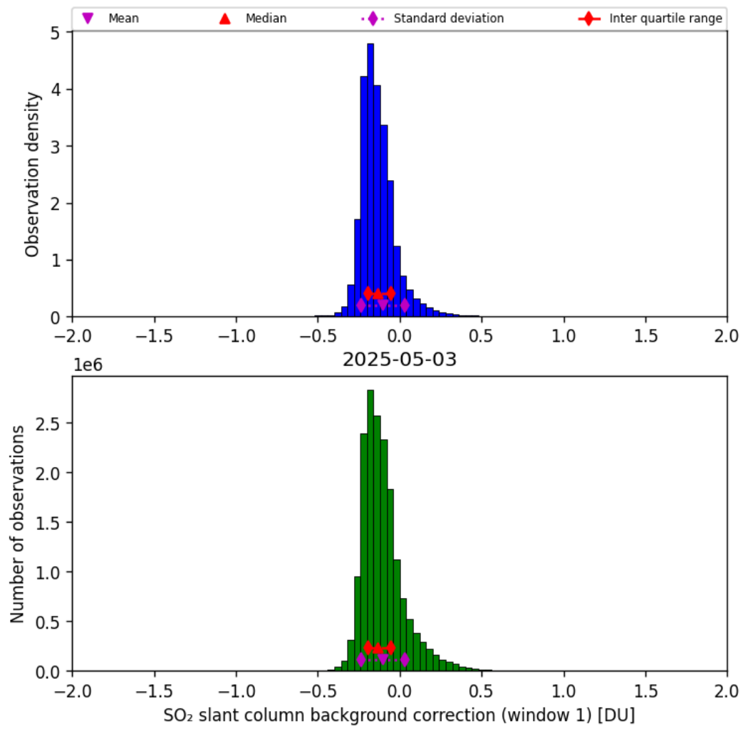
Figure 66: Histogram of “SO 2 slant column background correction (window 1)” for 2025-05-03 to 2025-05-03
