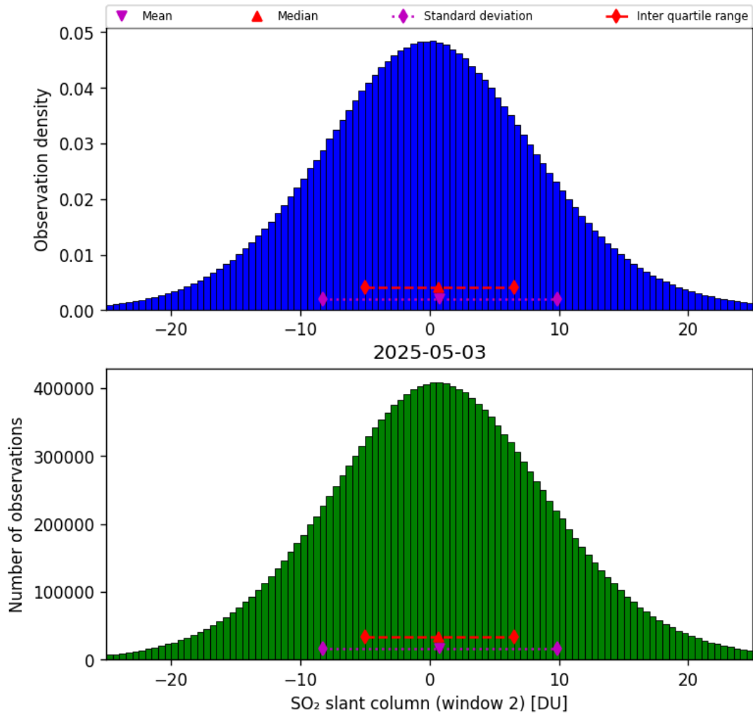
Figure 67: Histogram of “SO 2 slant column (window 2)” for 2025-05-03 to 2025-05-03
