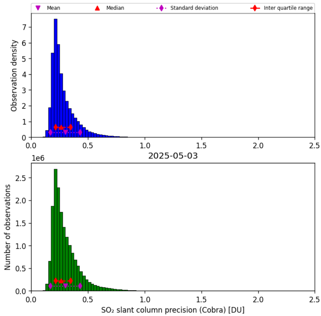
Figure 62: Histogram of “SO 2 slant column precision (Cobra)” for 2025-05-03 to 2025-05-03
