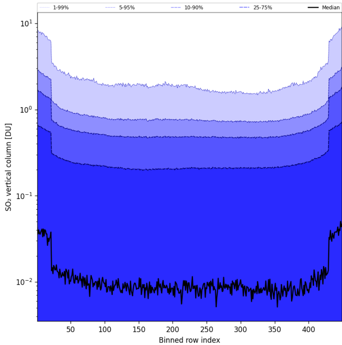
Figure 85: Along track statistics of “SO 2 vertical column” for 2025-05-03 to 2025-05-03
