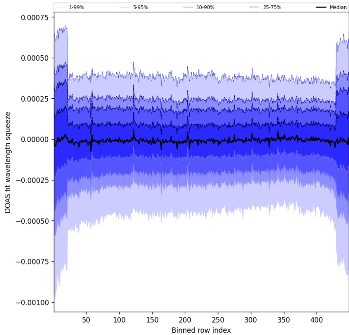
Figure 105: Along track statistics of “DOAS fit wavelength squeeze” for 2025-05-03 to 2025-05-03
