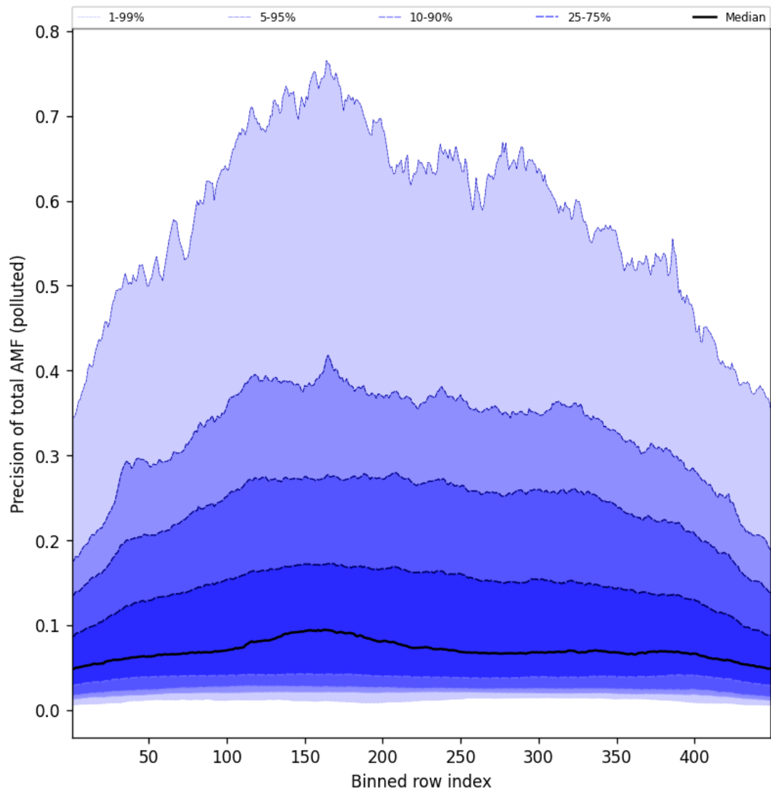
Figure 108: Along track statistics of “Precision of total AMF (polluted)” for 2025-05-03 to 2025-05-03
