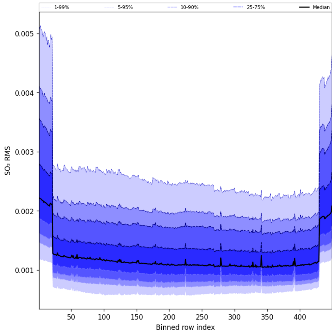
Figure 106: Along track statistics of “SO 2 RMS” for 2025-05-03 to 2025-05-03
