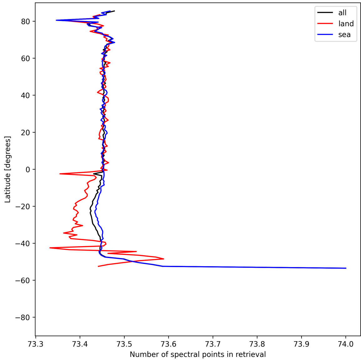
Figure 56: Zonal average of “Number of spectral points in retrieval” for 2025-05-03 to 2025-05-03.
