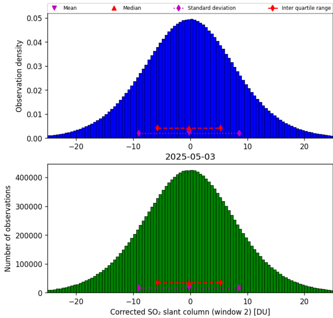
Figure 69: Histogram of “Corrected SO 2 slant column (window 2)” for 2025-05-03 to 2025-05-03
