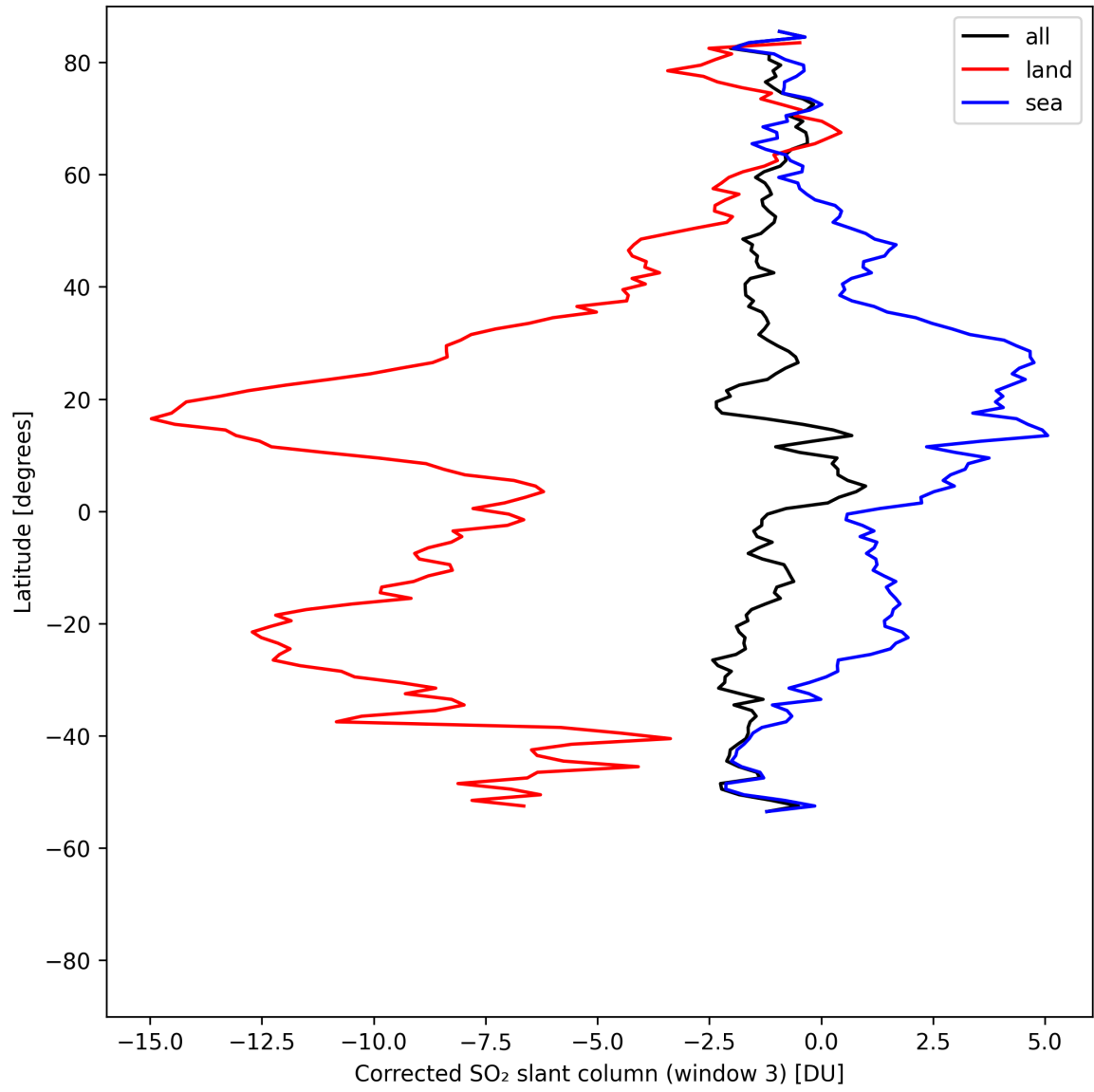
Figure 46: Zonal average of “Corrected SO 2 slant column (window 3)” for 2025-05-03 to 2025-05-03.
