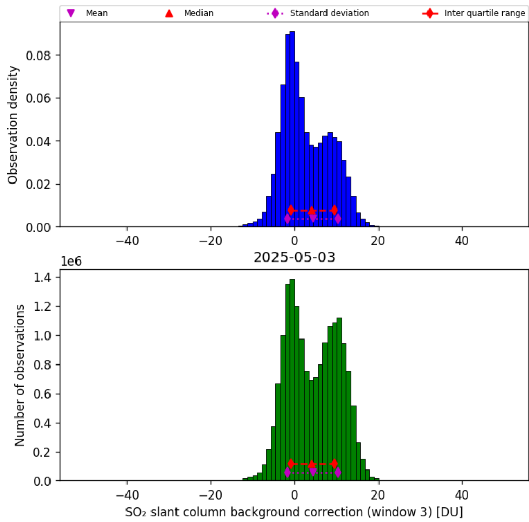
Figure 74: Histogram of “SO 2 slant column background correction (window 3)” for 2025-05-03 to 2025-05-03
