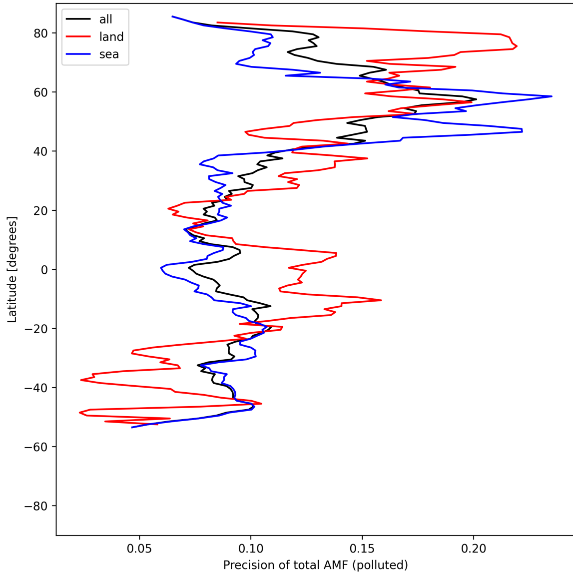
Figure 54: Zonal average of “Precision of total AMF (polluted)” for 2025-05-03 to 2025-05-03.
