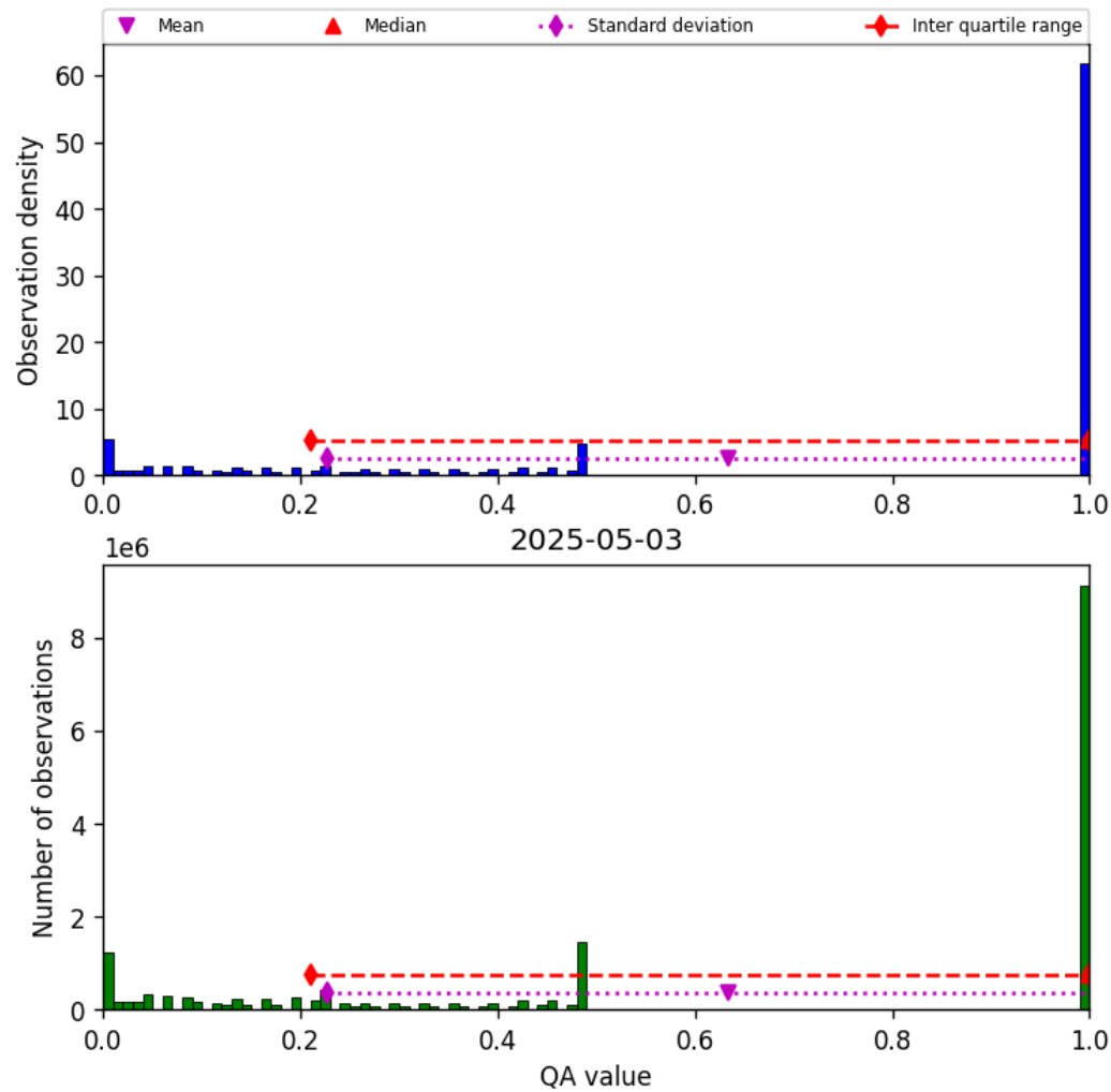
Figure 57: Histogram of “QA value” for 2025-05-03 to 2025-05-03
