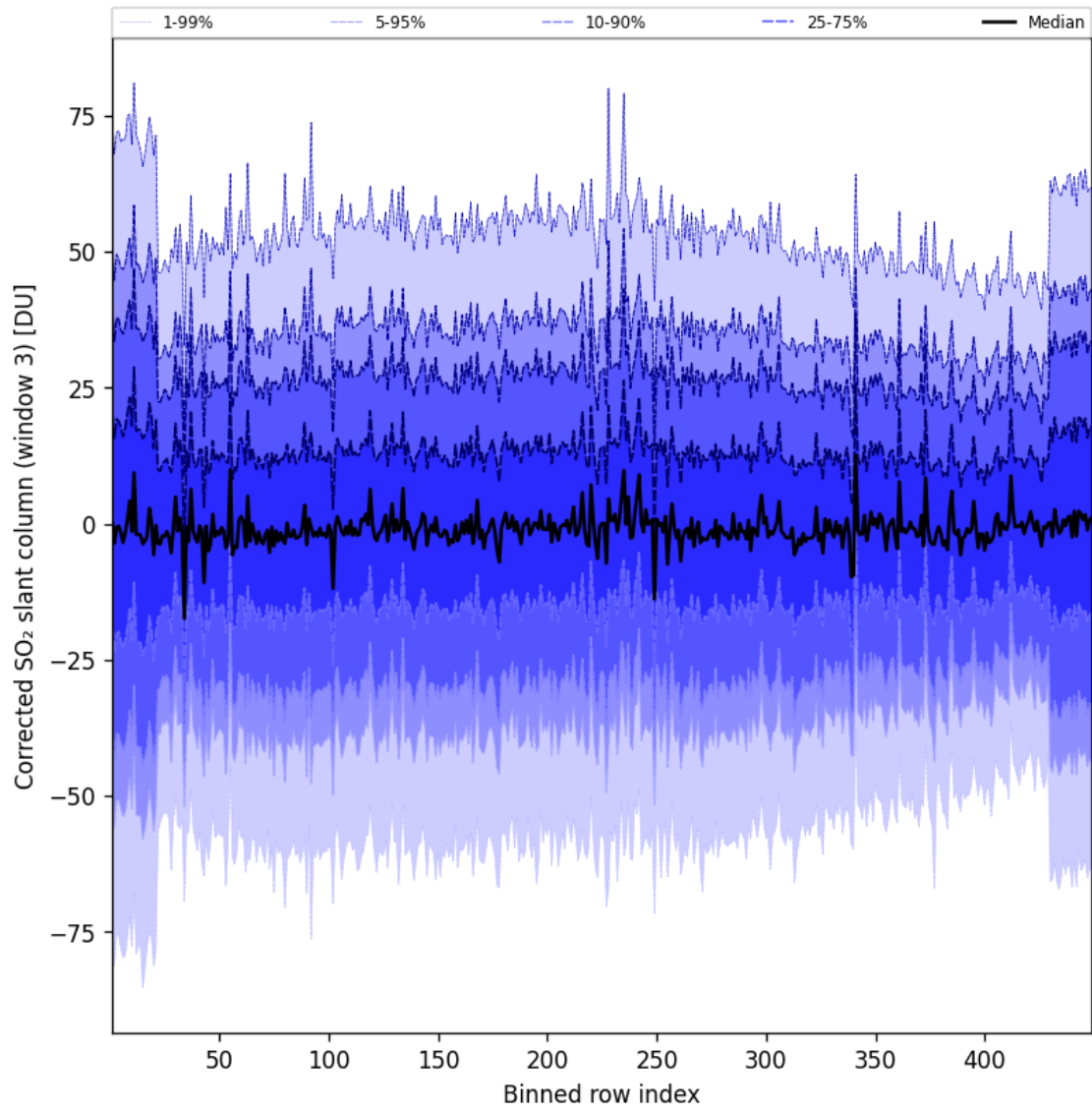
Figure 100: Along track statistics of “Corrected SO 2 slant column (window 3)” for 2025-05-03 to 2025-05-03
