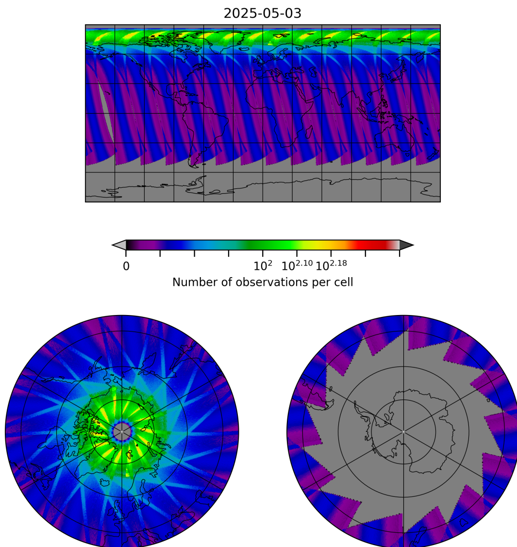
Figure 29: Map of the number of observations for 2025-05-03 to 2025-05-03
