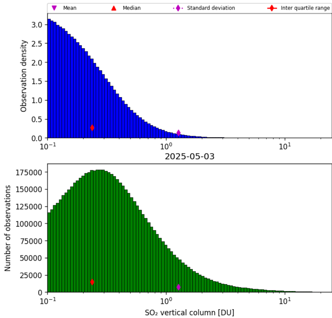
Figure 58: Histogram of “SO 2 vertical column” for 2025-05-03 to 2025-05-03
