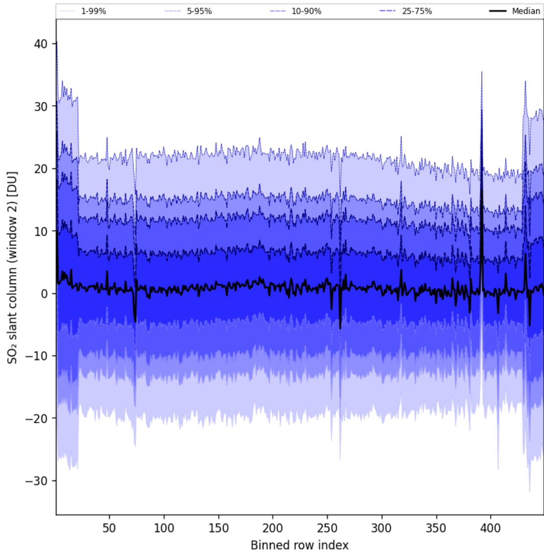
Figure 94: Along track statistics of “SO 2 slant column (window 2)” for 2025-05-03 to 2025-05-03
