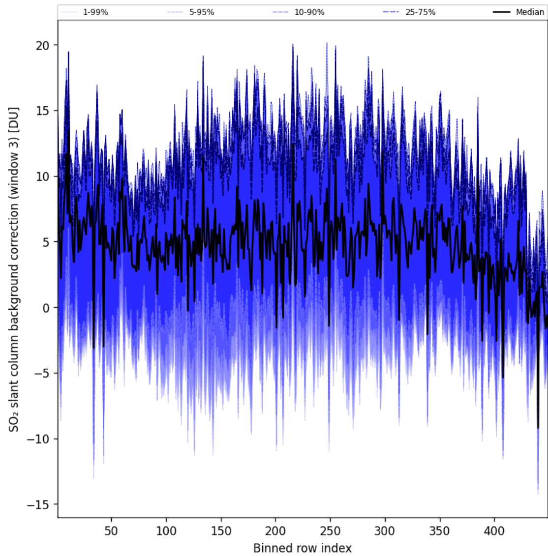
Figure 101: Along track statistics of “SO 2 slant column background correction (window 3)” for 2025-05-03 to 2025-05-03
