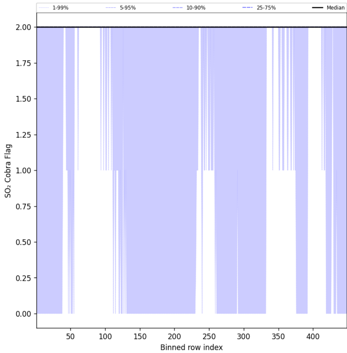
Figure 102: Along track statistics of “SO 2 Cobra Flag” for 2025-05-03 to 2025-05-03
