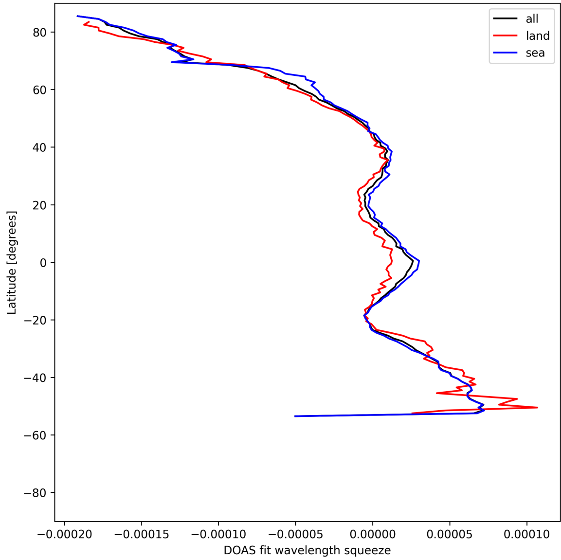
Figure 51: Zonal average of “DOAS fit wavelength squeeze” for 2025-05-03 to 2025-05-03.
