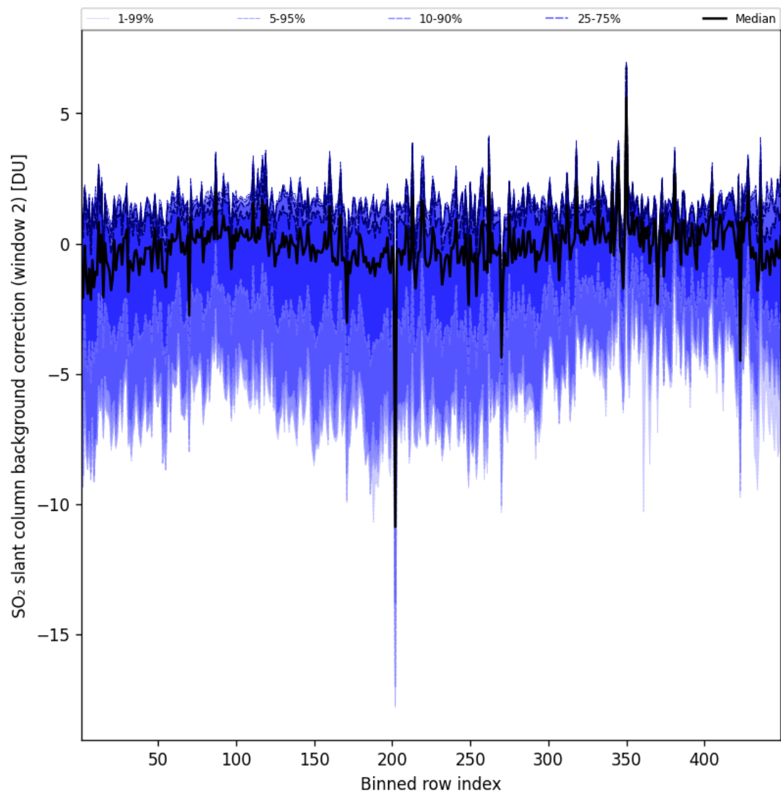
Figure 97: Along track statistics of “SO 2 slant column background correction (window 2)” for 2025-05-03 to 2025-05-03
