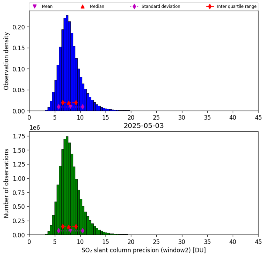
Figure 68: Histogram of “SO 2 slant column precision (window2)” for 2025-05-03 to 2025-05-03
