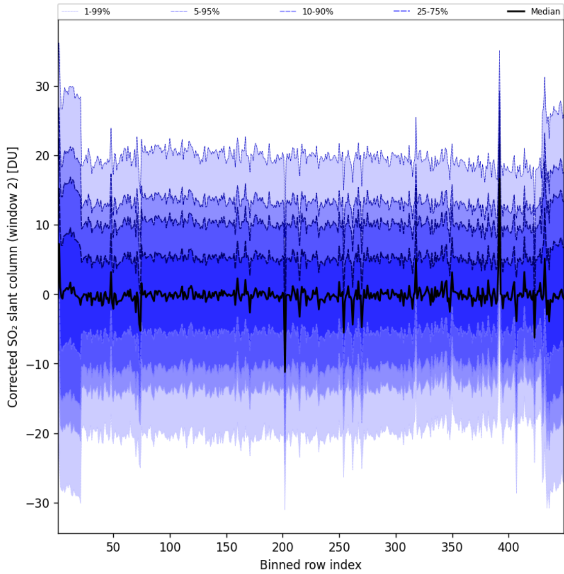
Figure 96: Along track statistics of “Corrected SO 2 slant column (window 2)” for 2025-05-03 to 2025-05-03
