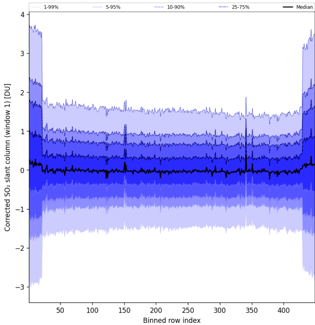
Figure 92: Along track statistics of “Corrected SO 2 slant column (window 1)” for 2025-05-03 to 2025-05-03
