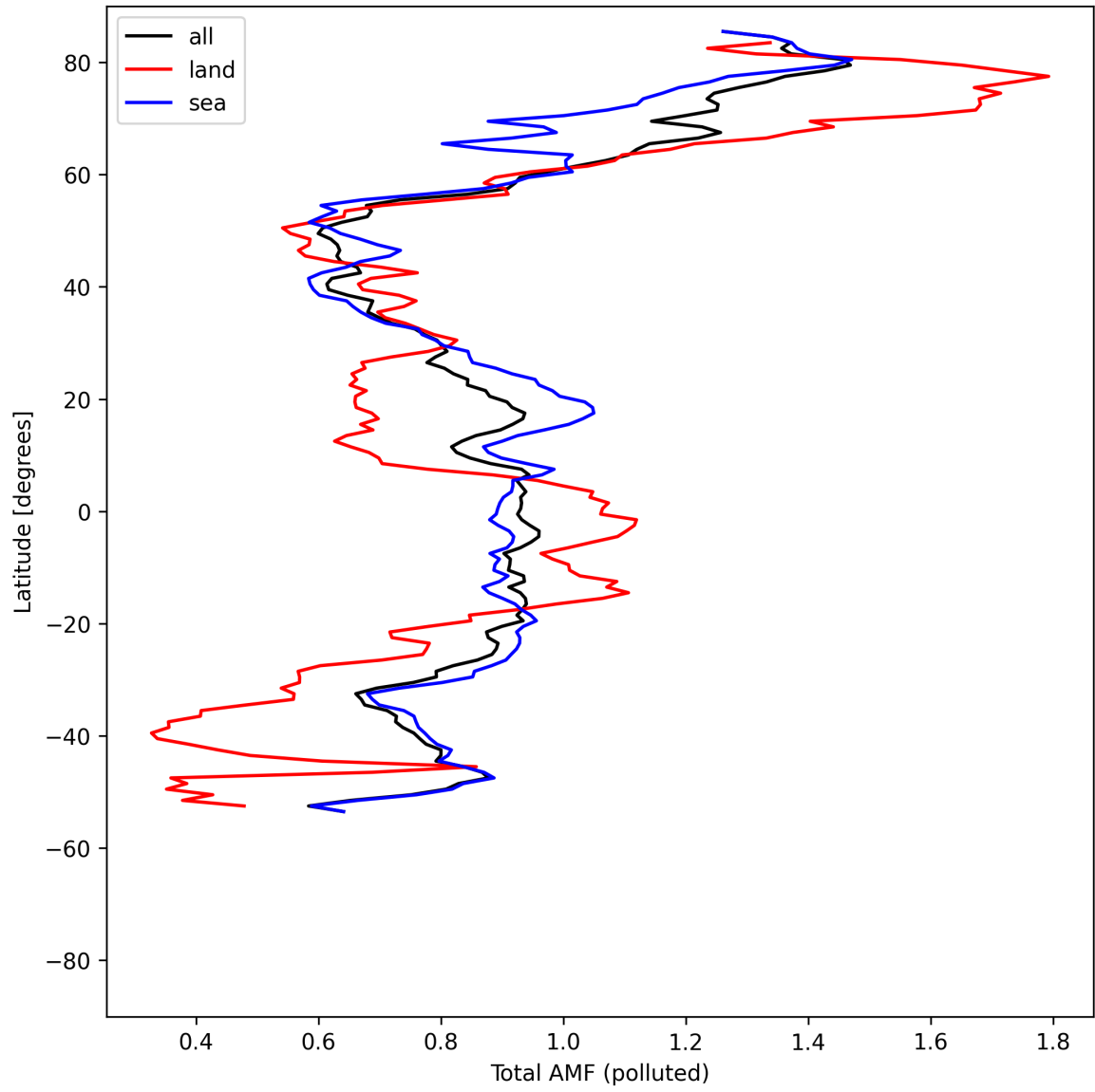
Figure 53: Zonal average of “Total AMF (polluted)” for 2025-05-03 to 2025-05-03.
