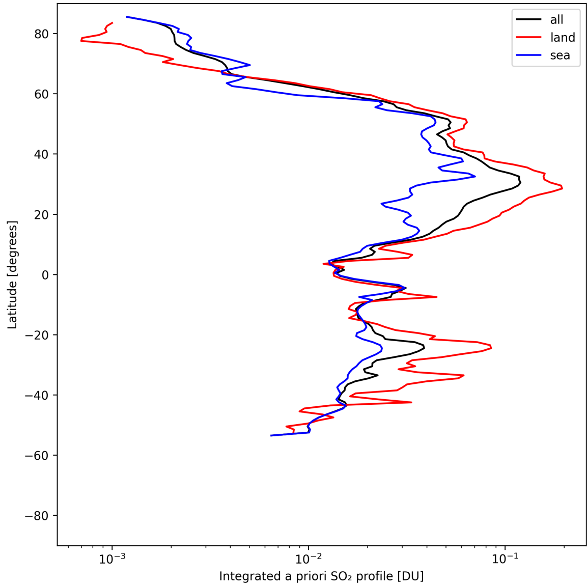
Figure 49: Zonal average of “Integrated a priori SO 2 profile” for 2025-05-03 to 2025-05-03.
