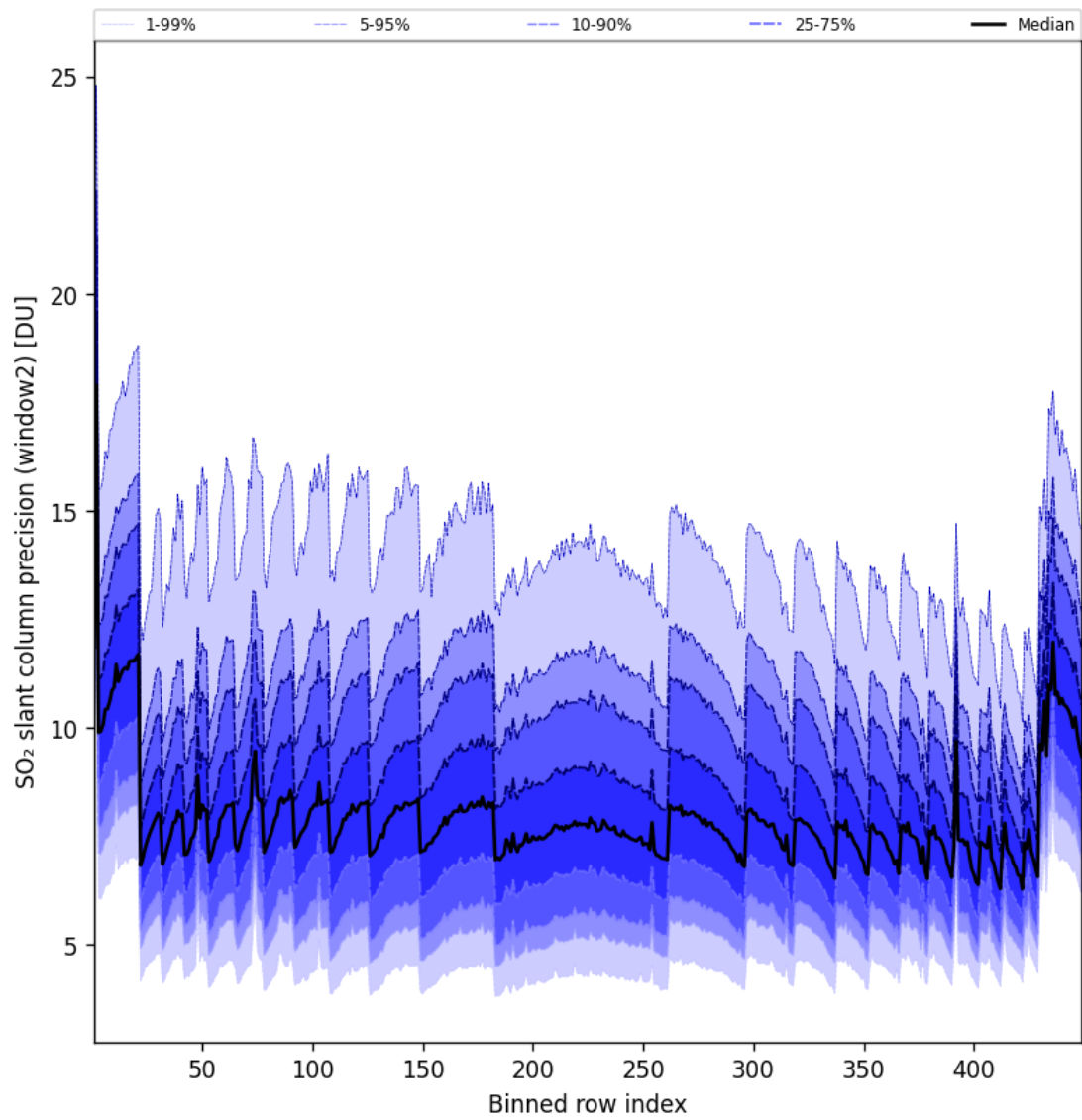
Figure 95: Along track statistics of “SO 2 slant column precision (window2)” for 2025-05-03 to 2025-05-03
