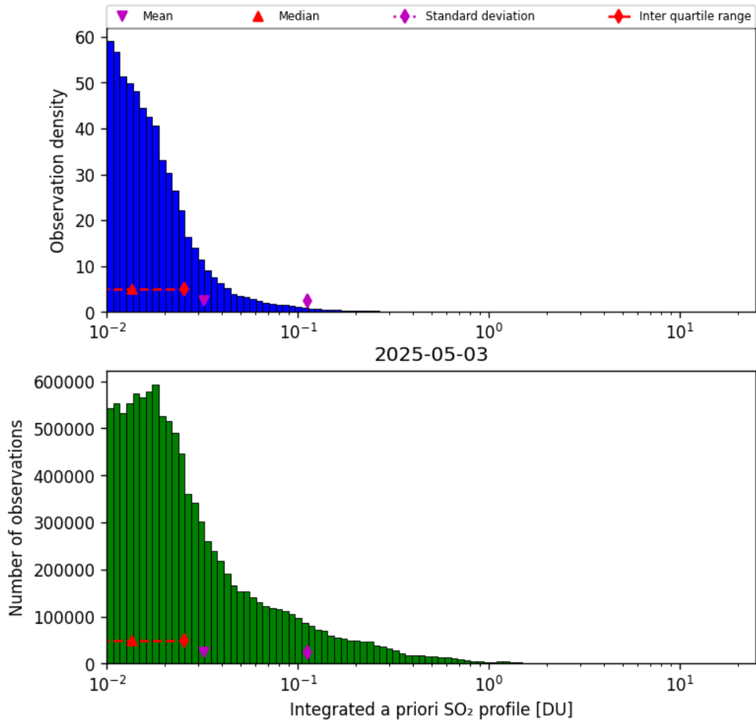
Figure 76: Histogram of “Integrated a priori SO 2 profile” for 2025-05-03 to 2025-05-03
