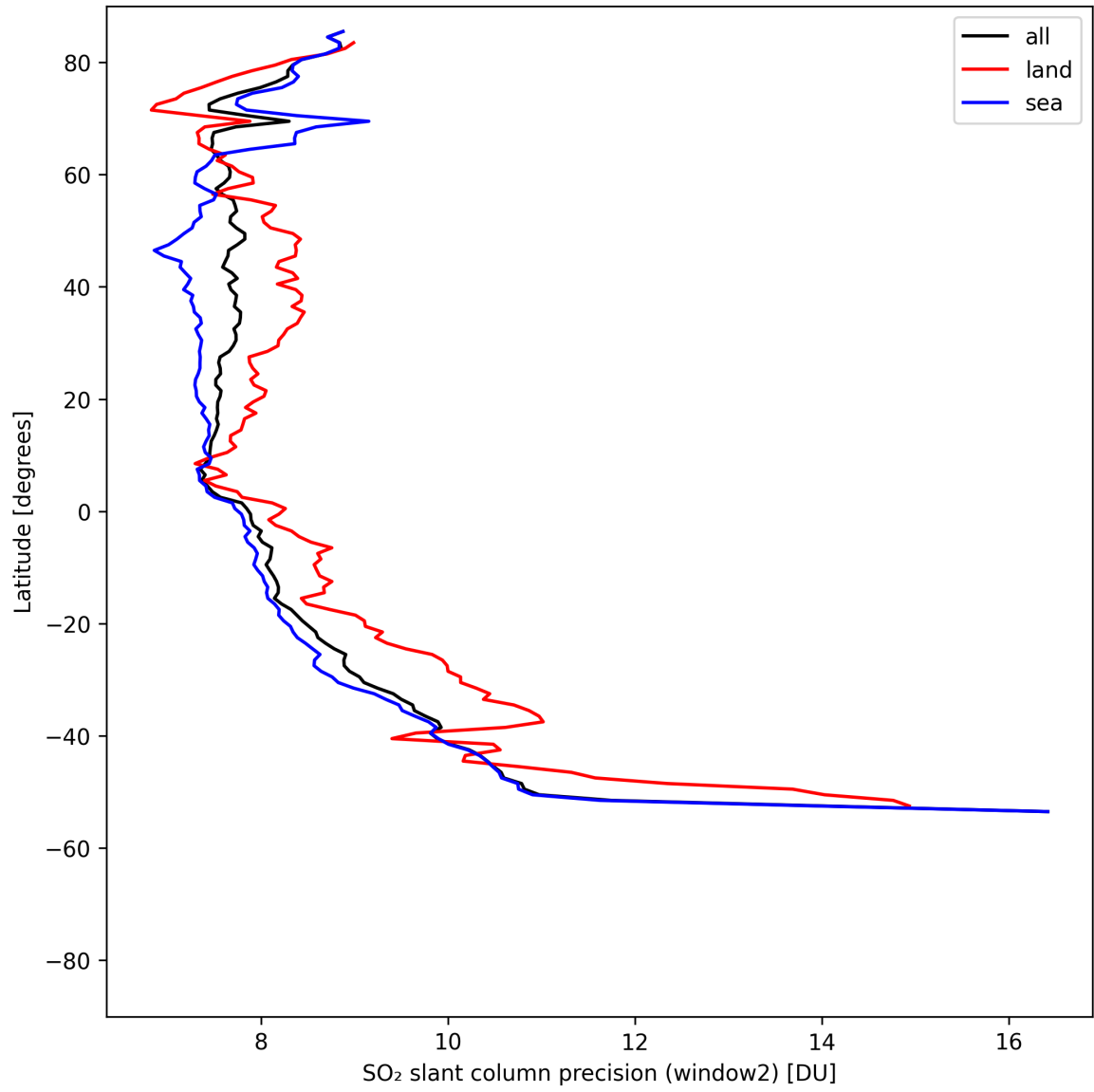
Figure 41: Zonal average of “SO 2 slant column precision (window2)” for 2025-05-03 to 2025-05-03.
