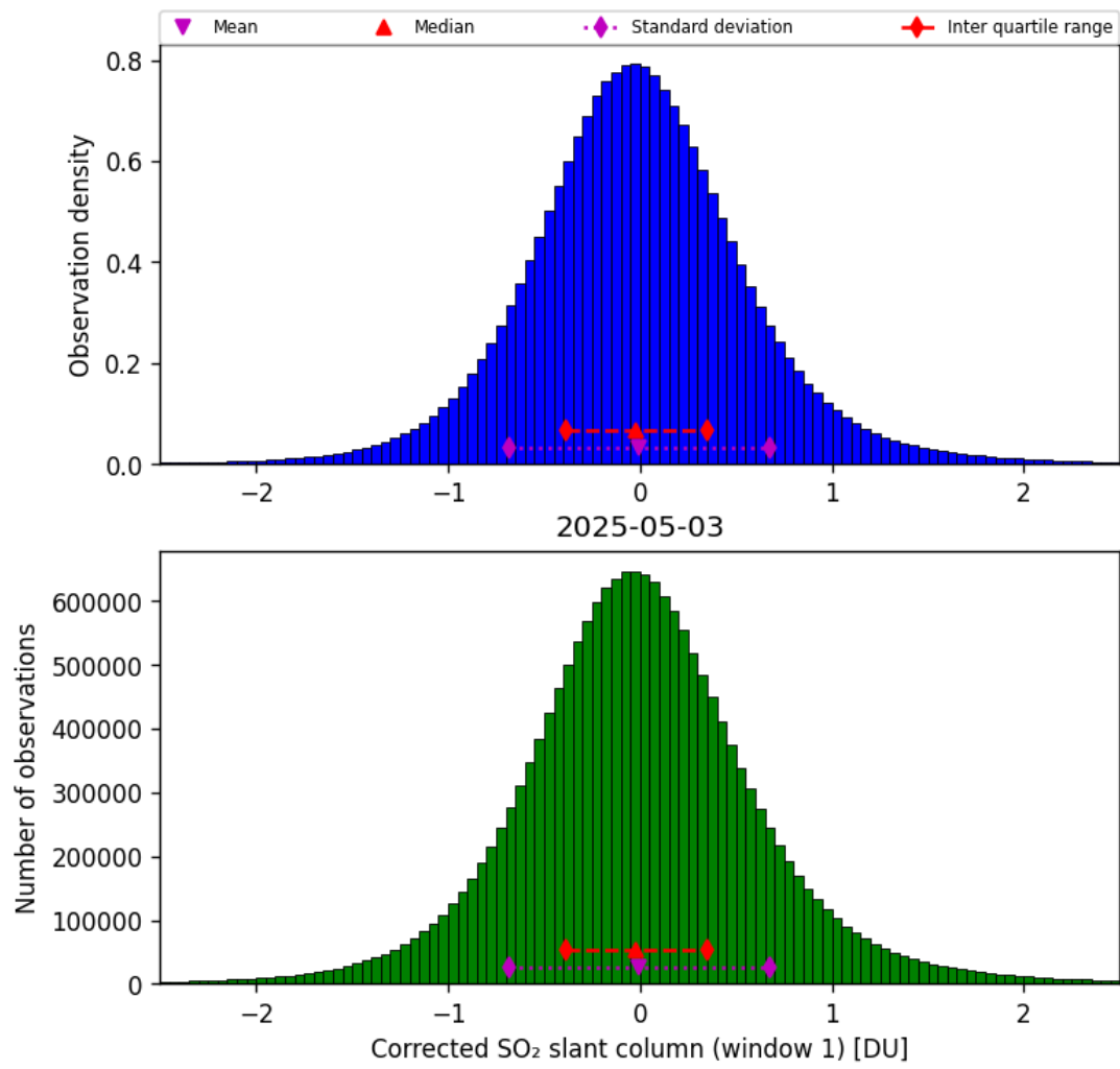
Figure 65: Histogram of “Corrected SO 2 slant column (window 1)” for 2025-05-03 to 2025-05-03
