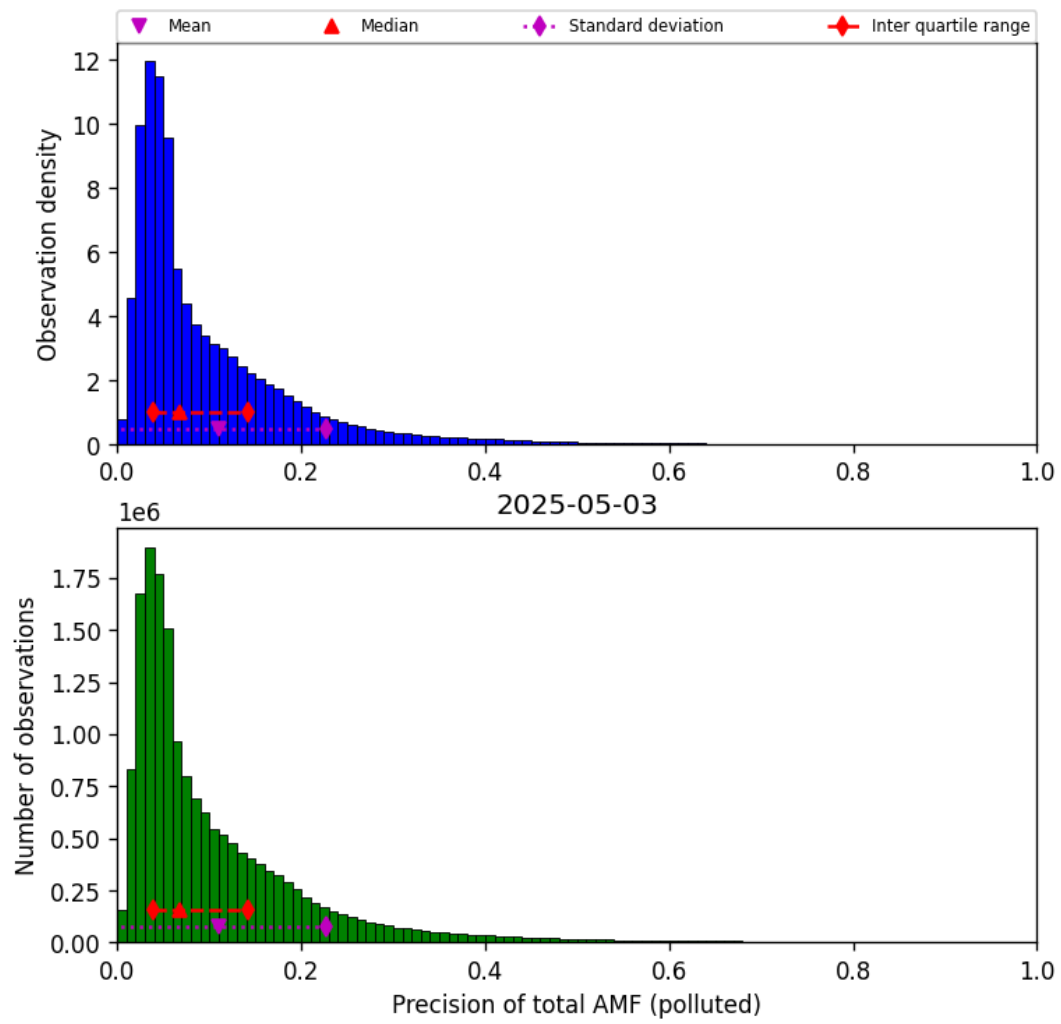
Figure 81: Histogram of “Precision of total AMF (polluted)” for 2025-05-03 to 2025-05-03
