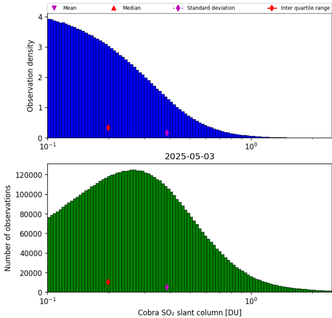
Figure 61: Histogram of “Cobra SO 2 slant column” for 2025-05-03 to 2025-05-03
