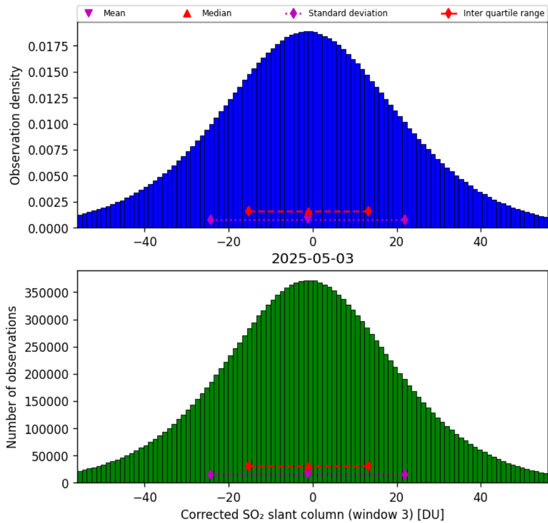
Figure 73: Histogram of “Corrected SO 2 slant column (window 3)” for 2025-05-03 to 2025-05-03
