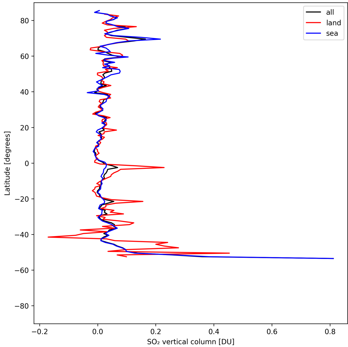
Figure 31: Zonal average of “SO 2 vertical column” for 2025-05-03 to 2025-05-03.
