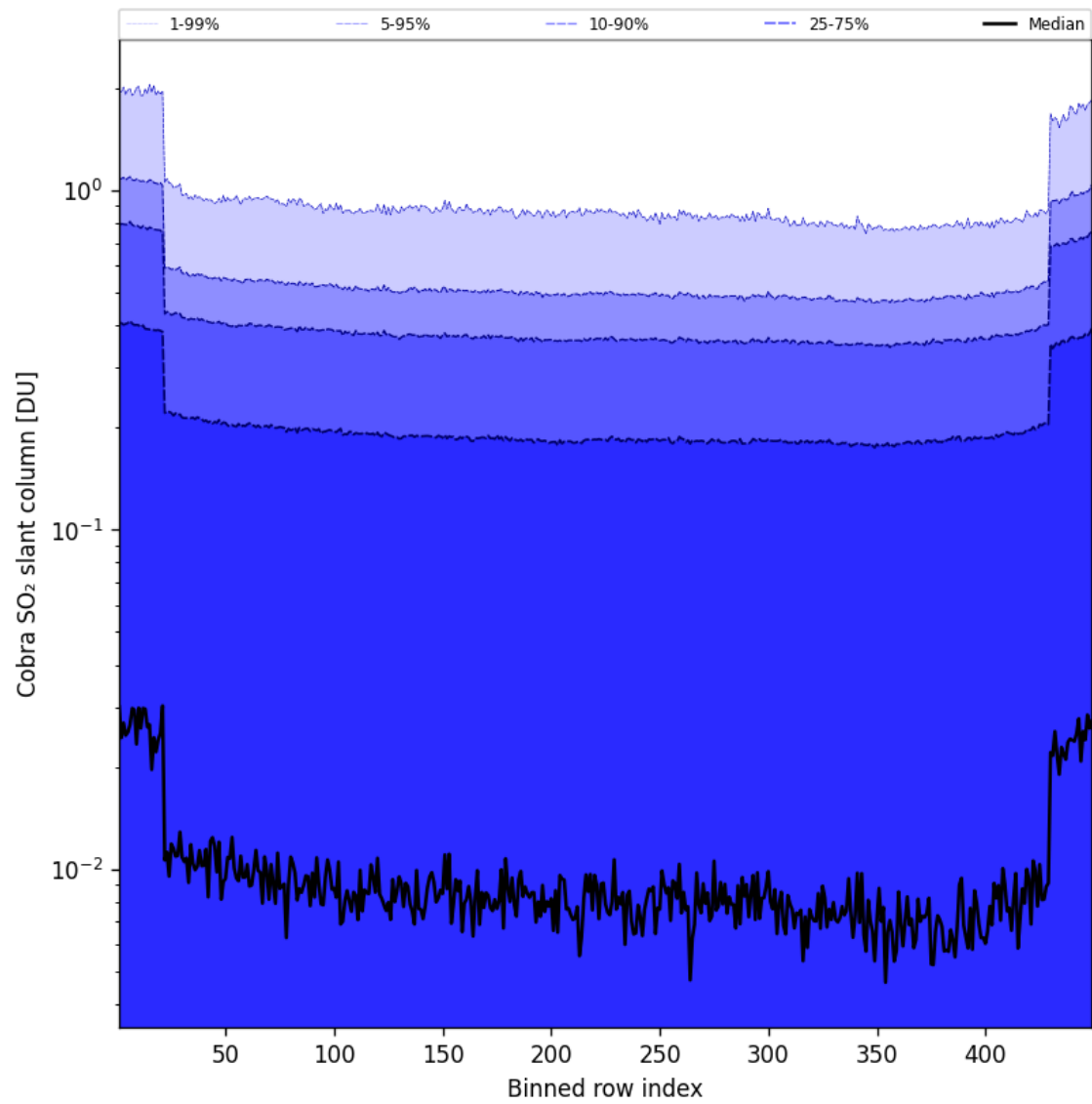
Figure 88: Along track statistics of "Cobra SO 2 slant column" for 2025-05-03 to 2025-05-03
