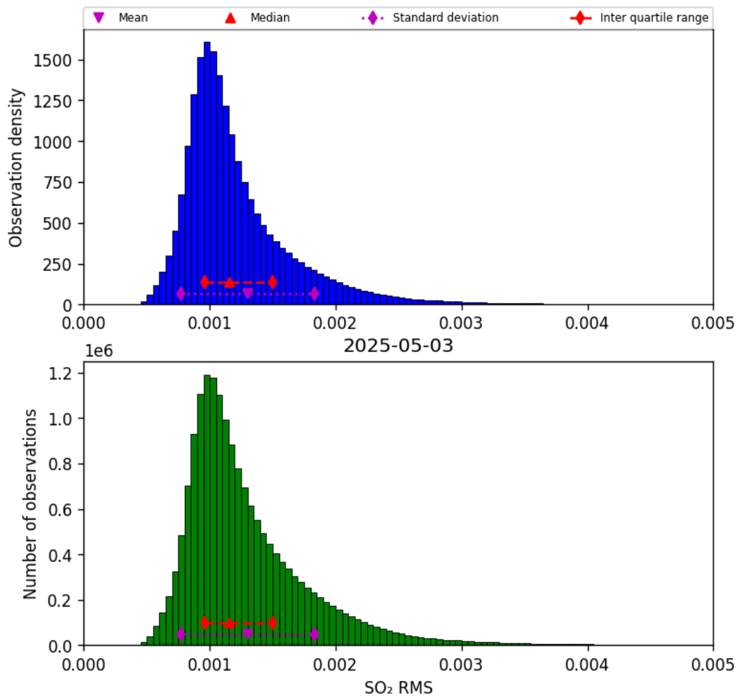
Figure 79: Histogram of “SO 2 RMS” for 2025-05-03 to 2025-05-03
