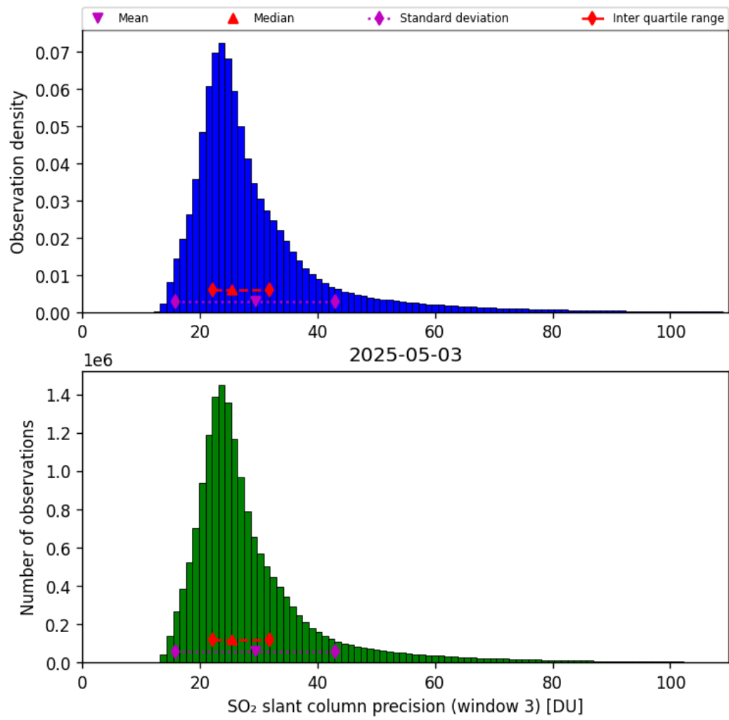
Figure 72: Histogram of “SO 2 slant column precision (window 3)” for 2025-05-03 to 2025-05-03
