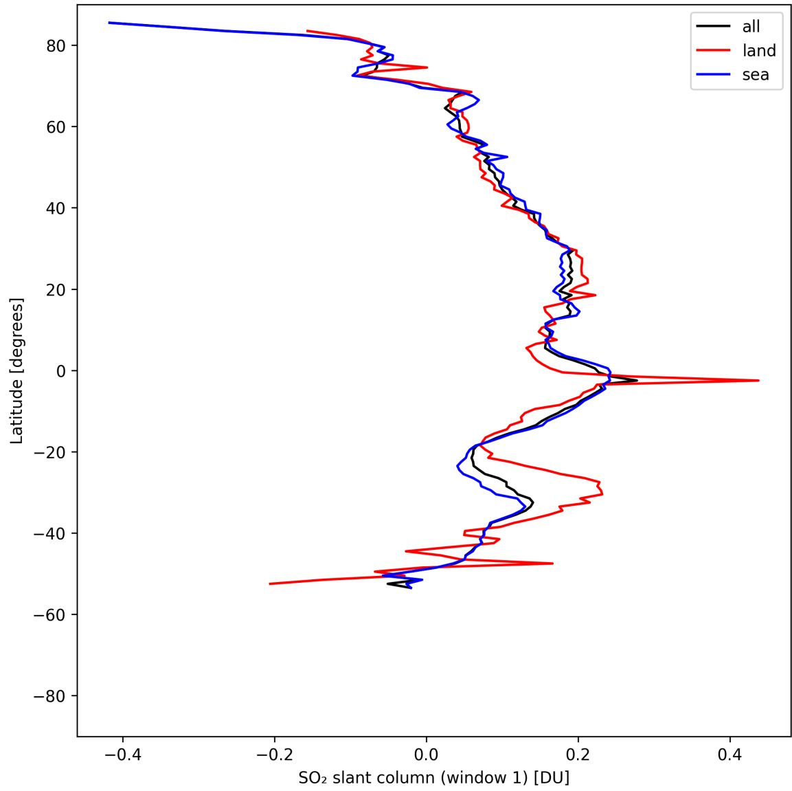
Figure 36: Zonal average of “SO 2 slant column (window 1)” for 2025-05-03 to 2025-05-03.
