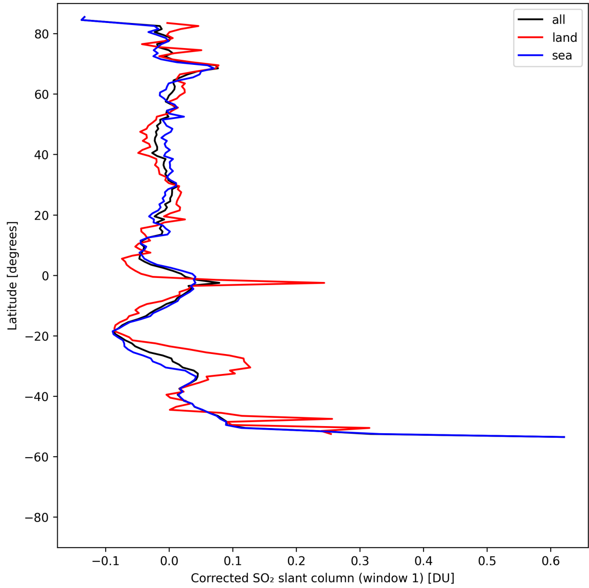
Figure 38: Zonal average of “Corrected SO 2 slant column (window 1)” for 2025-05-03 to 2025-05-03.
