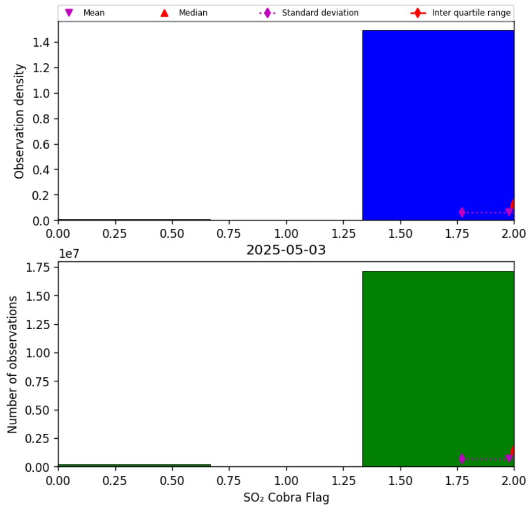
Figure 75: Histogram of “SO 2 Cobra Flag” for 2025-05-03 to 2025-05-03
