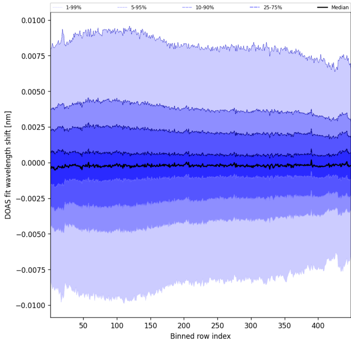
Figure 104: Along track statistics of “DOAS fit wavelength shift” for 2025-05-03 to 2025-05-03
