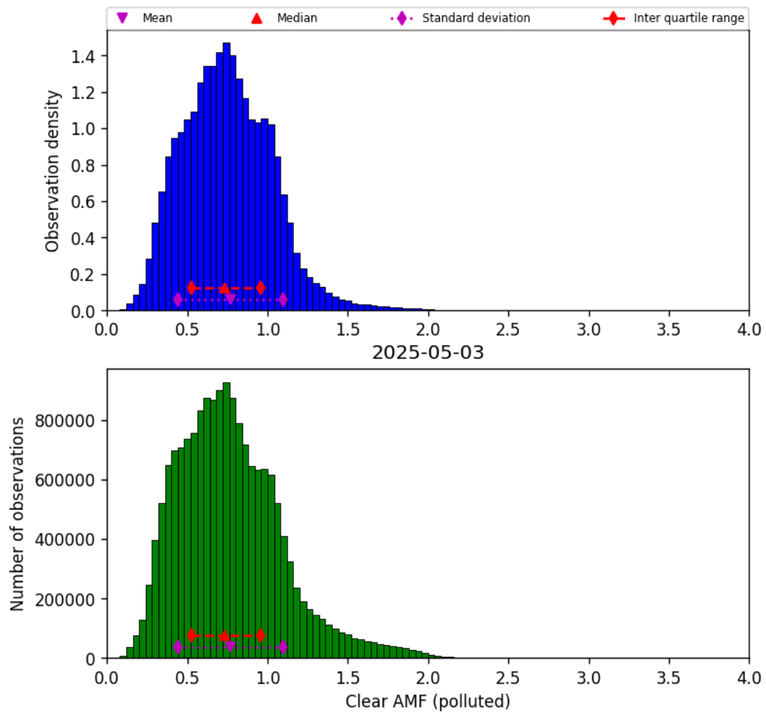
Figure 82: Histogram of “Clear AMF (polluted)” for 2025-05-03 to 2025-05-03
