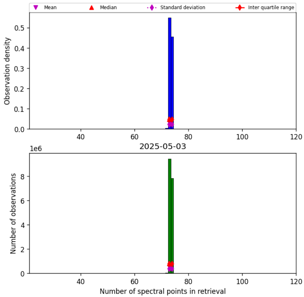
Figure 83: Histogram of “Number of spectral points in retrieval” for 2025-05-03 to 2025-05-03
