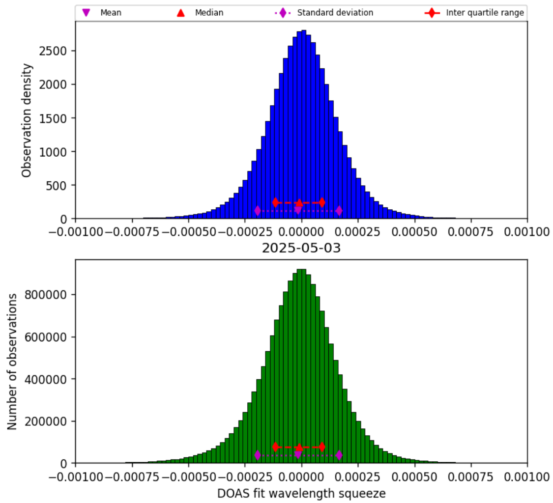
Figure 78: Histogram of “DOAS fit wavelength squeeze” for 2025-05-03 to 2025-05-03
