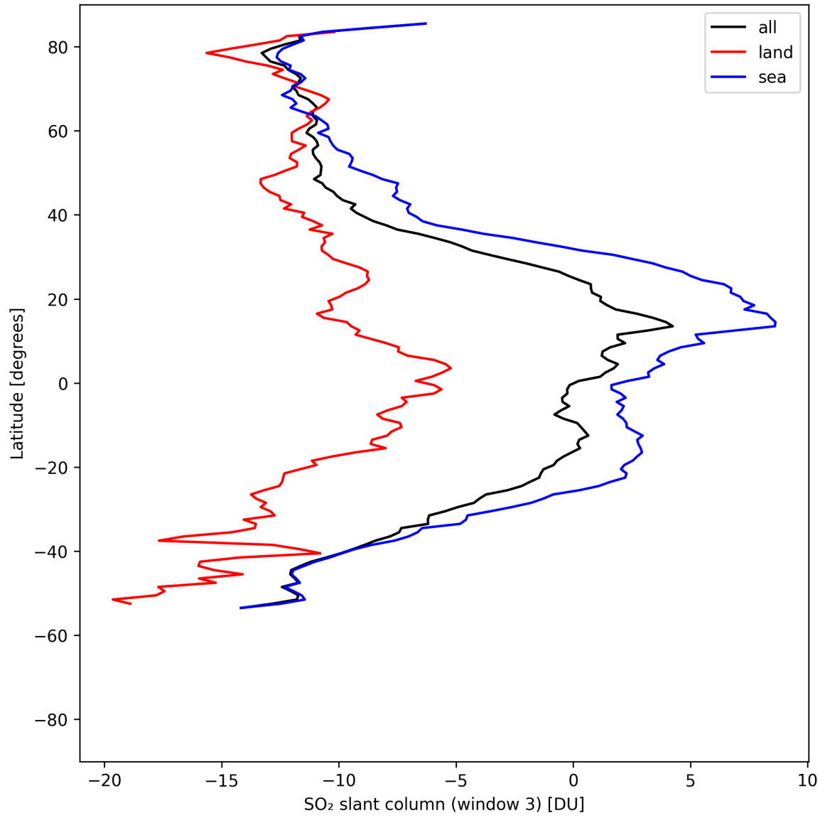
Figure 44: Zonal average of “SO 2 slant column (window 3)” for 2025-05-03 to 2025-05-03.
