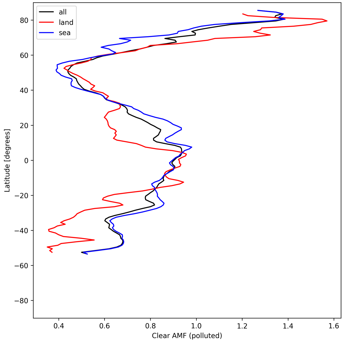
Figure 55: Zonal average of “Clear AMF (polluted)” for 2025-05-03 to 2025-05-03.
