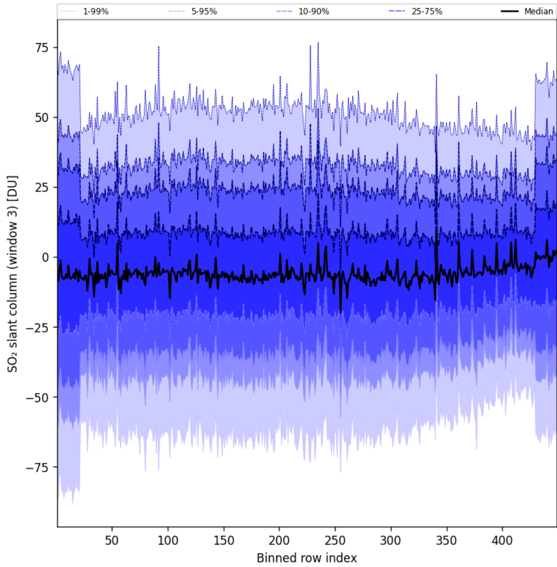
Figure 98: Along track statistics of “SO 2 slant column (window 3)” for 2025-05-03 to 2025-05-03
