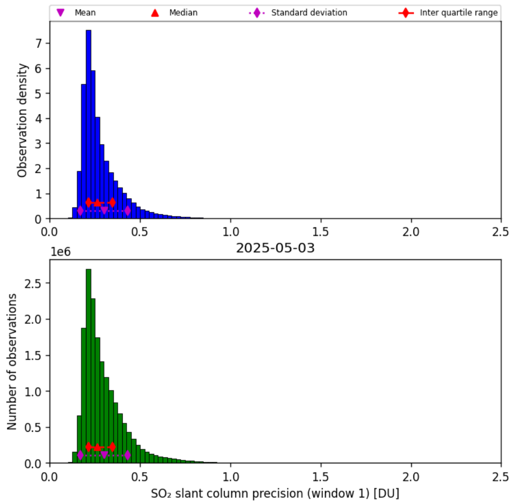
Figure 64: Histogram of “SO 2 slant column precision (window 1)” for 2025-05-03 to 2025-05-03
