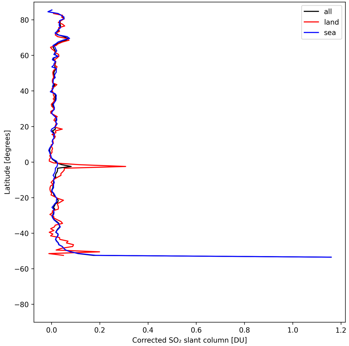
Figure 33: Zonal average of “Corrected SO 2 slant column” for 2025-05-03 to 2025-05-03.
