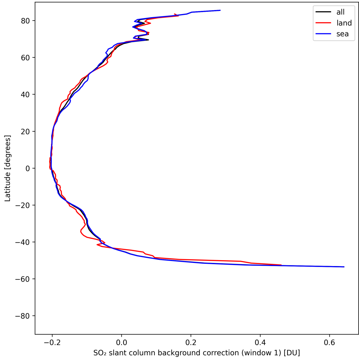
Figure 39: Zonal average of "SO 2 slant column background correction (window 1)" for 2025-05-03 to 2025-05-03.
