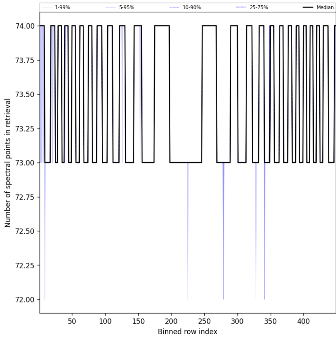
Figure 110: Along track statistics of “Number of spectral points in retrieval” for 2025-05-03 to 2025-05-03
