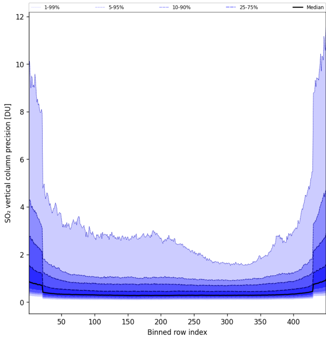
Figure 86: Along track statistics of “SO 2 vertical column precision” for 2025-05-03 to 2025-05-03
