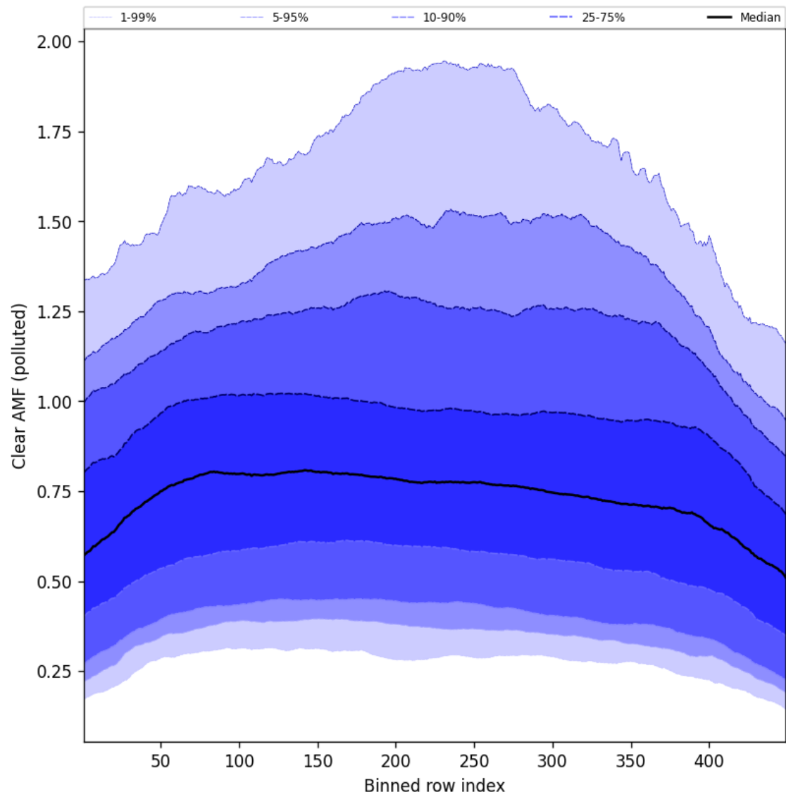
Figure 109: Along track statistics of “Clear AMF (polluted)” for 2025-05-06 to 2025-05-07
