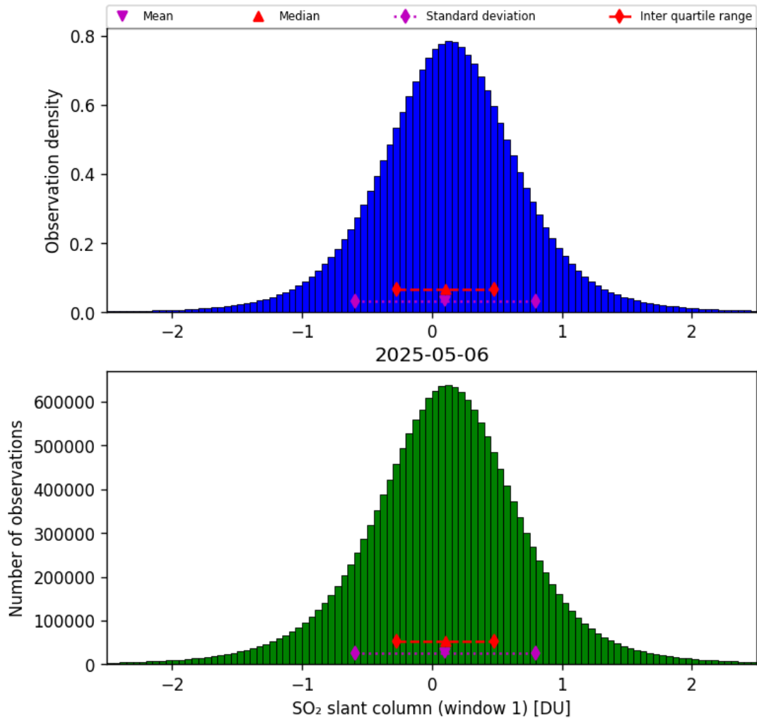
Figure 63: Histogram of “SO 2 slant column (window 1)” for 2025-05-06 to 2025-05-07
