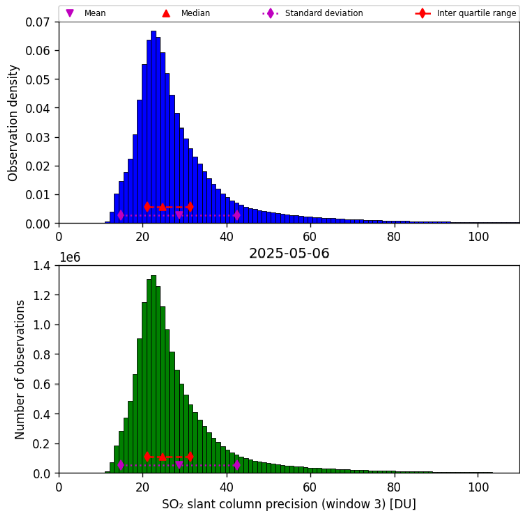
Figure 72: Histogram of “SO 2 slant column precision (window 3)” for 2025-05-06 to 2025-05-07
