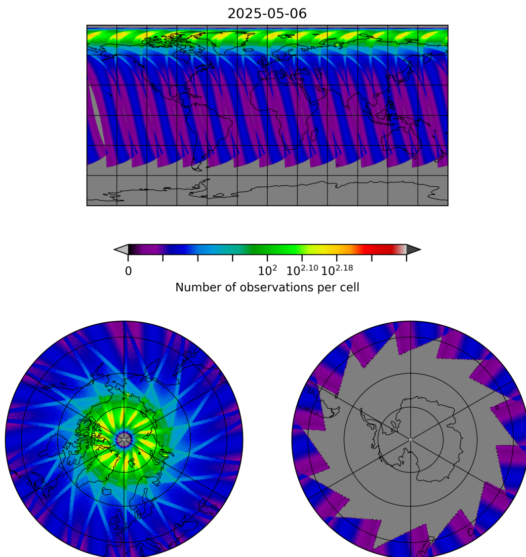
Figure 29: Map of the number of observations for 2025-05-06 to 2025-05-07
