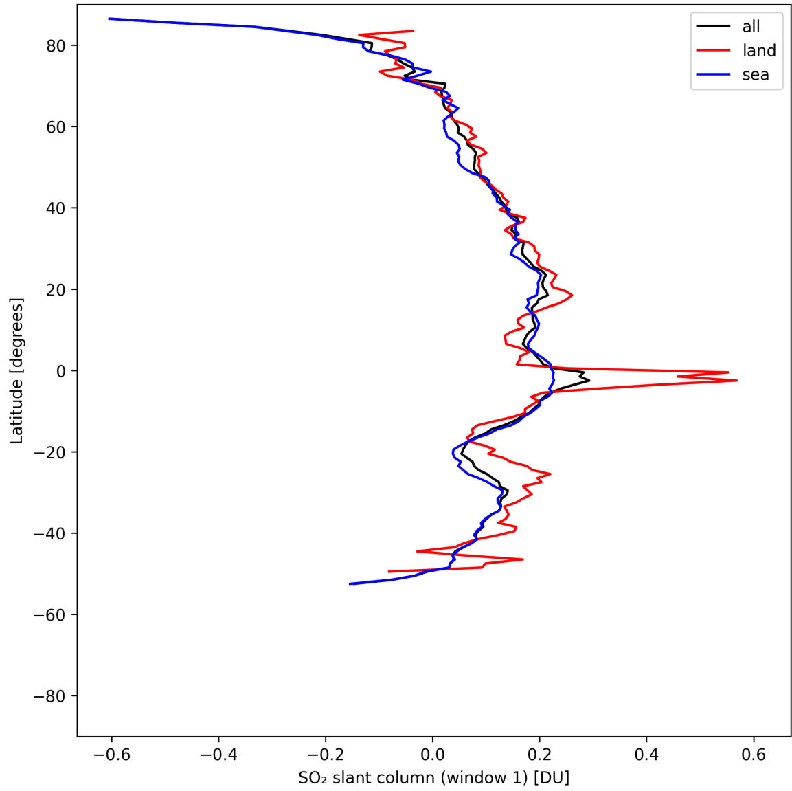
Figure 36: Zonal average of “SO 2 slant column (window 1)” for 2025-05-06 to 2025-05-07.
