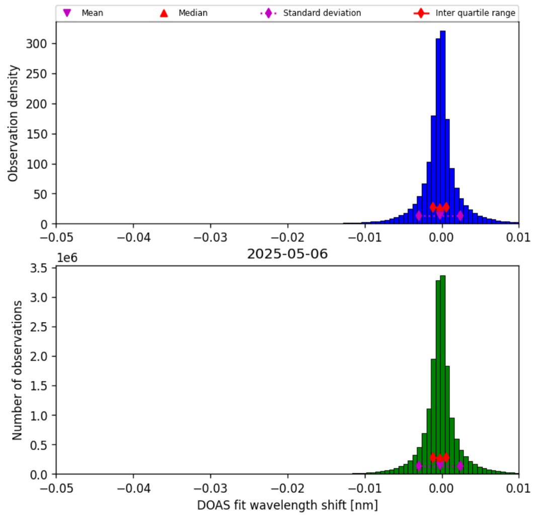
Figure 77: Histogram of “DOAS fit wavelength shift” for 2025-05-06 to 2025-05-07
