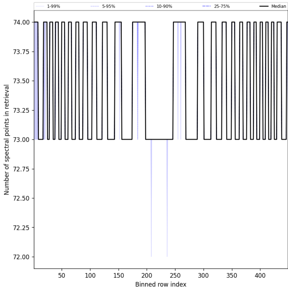
Figure 110: Along track statistics of “Number of spectral points in retrieval” for 2025-05-06 to 2025-05-07
