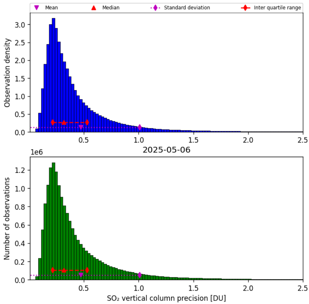
Figure 59: Histogram of “SO 2 vertical column precision” for 2025-05-06 to 2025-05-07
