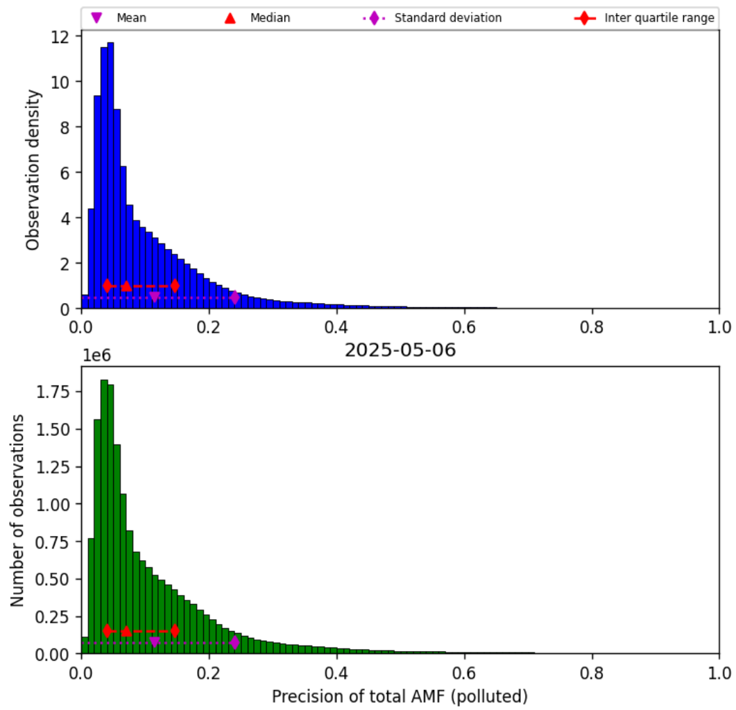
Figure 81: Histogram of “Precision of total AMF (polluted)” for 2025-05-06 to 2025-05-07
