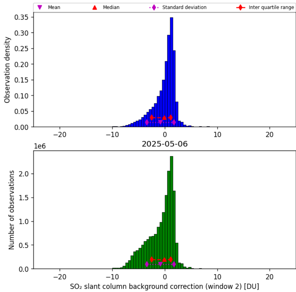
Figure 70: Histogram of “SO 2 slant column background correction (window 2)” for 2025-05-06 to 2025-05-07
