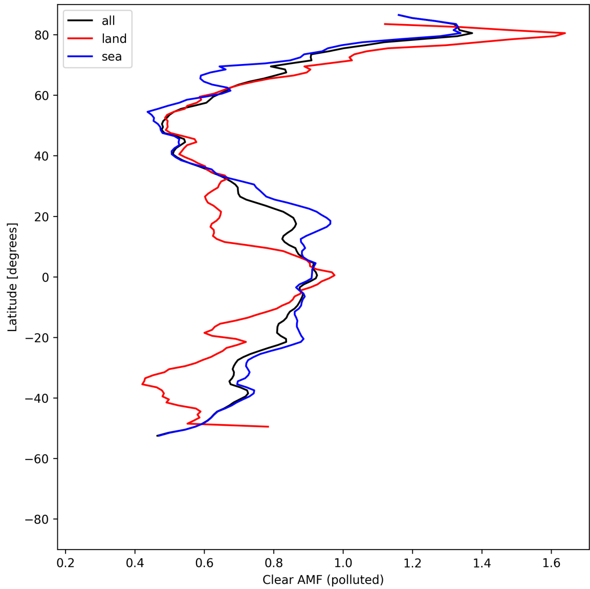
Figure 55: Zonal average of “Clear AMF (polluted)” for 2025-05-06 to 2025-05-07.
