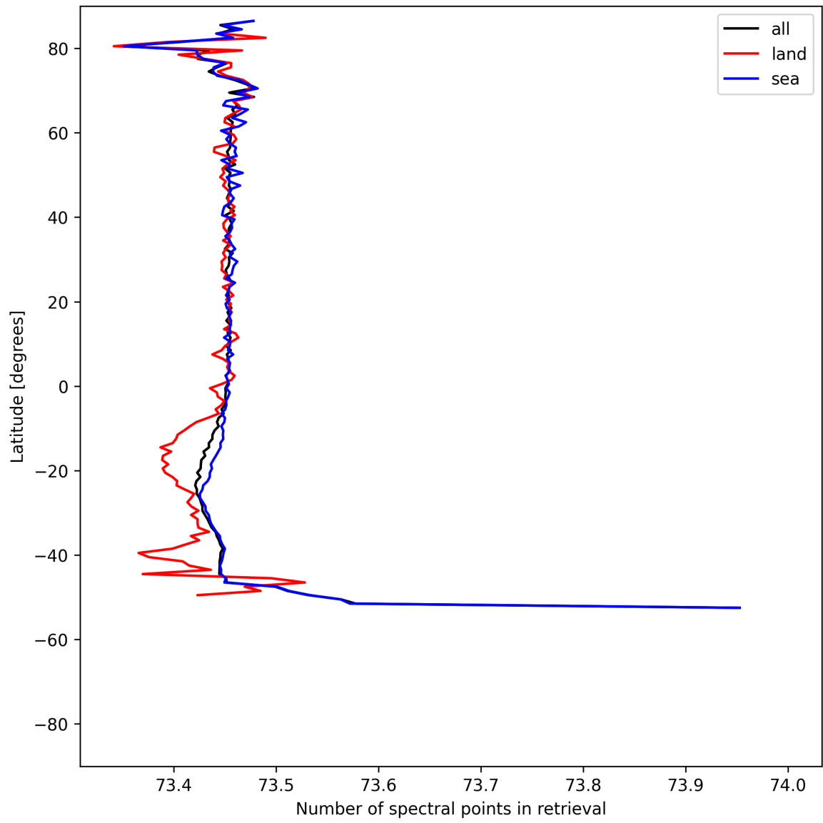
Figure 56: Zonal average of “Number of spectral points in retrieval” for 2025-05-06 to 2025-05-07.
