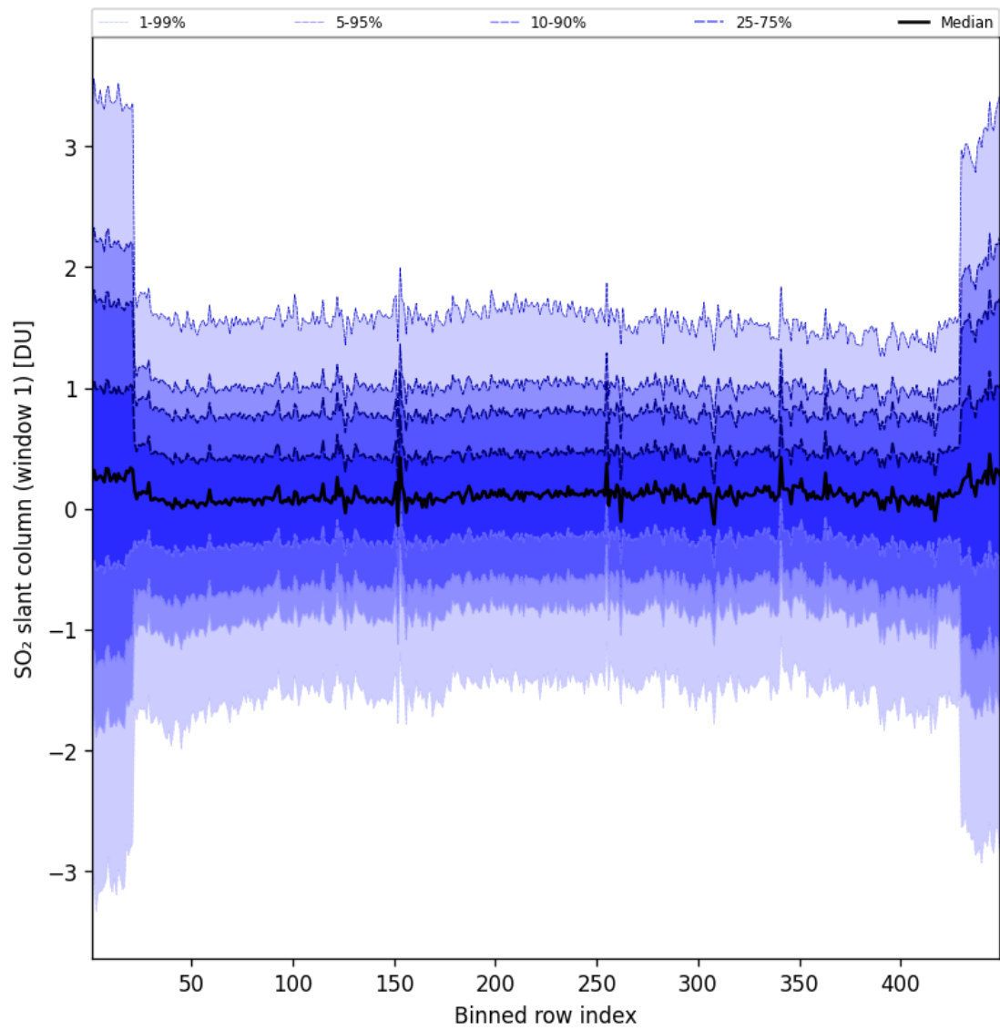
Figure 90: Along track statistics of “SO 2 slant column (window 1)” for 2025-05-06 to 2025-05-07
