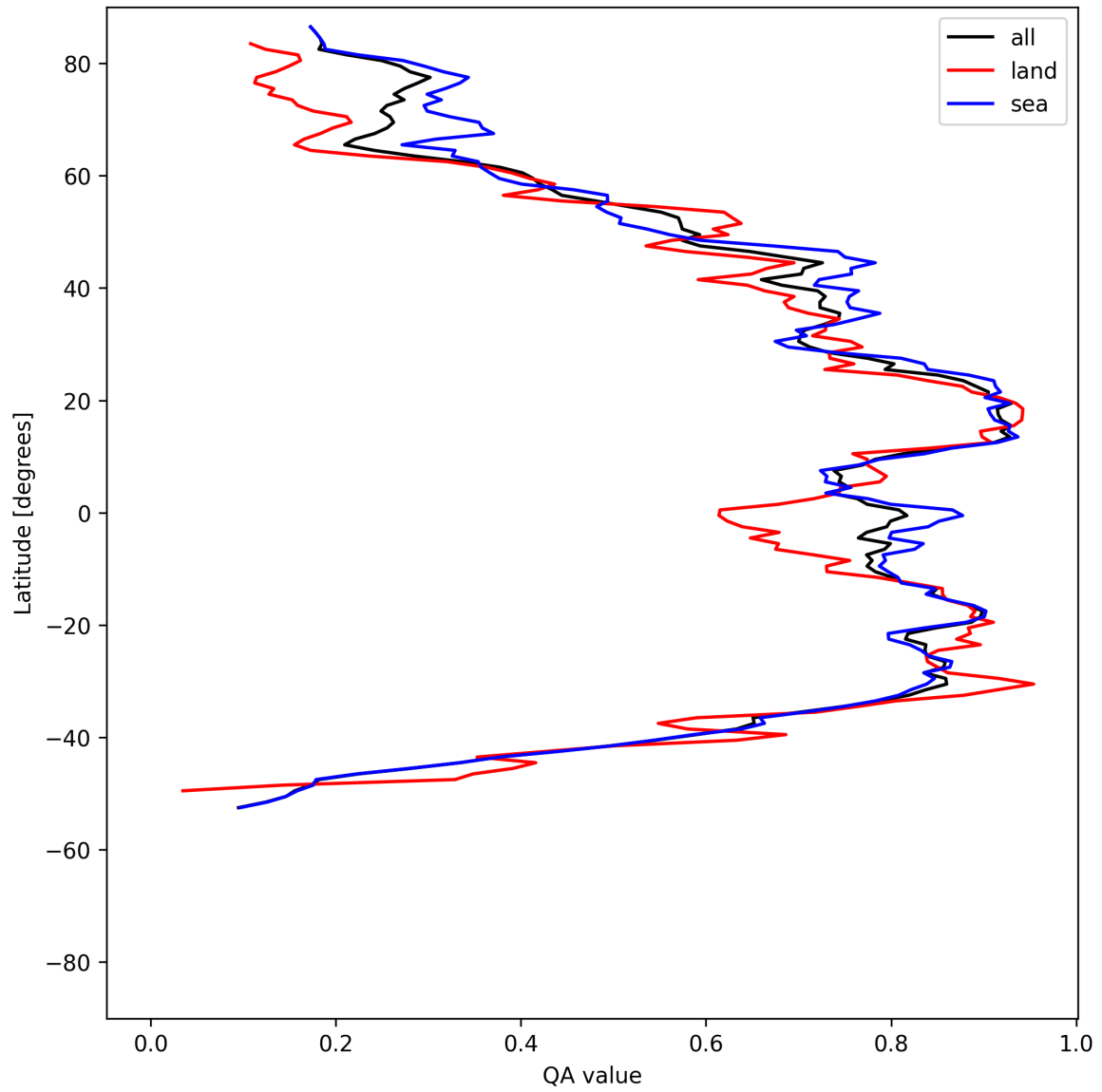
Figure 30: Zonal average of “QA value” for 2025-05-06 to 2025-05-07.
