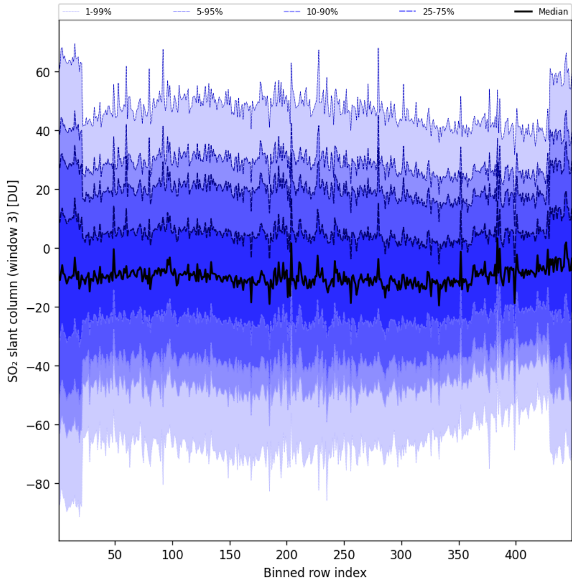
Figure 98: Along track statistics of “SO 2 slant column (window 3)” for 2025-05-06 to 2025-05-07
