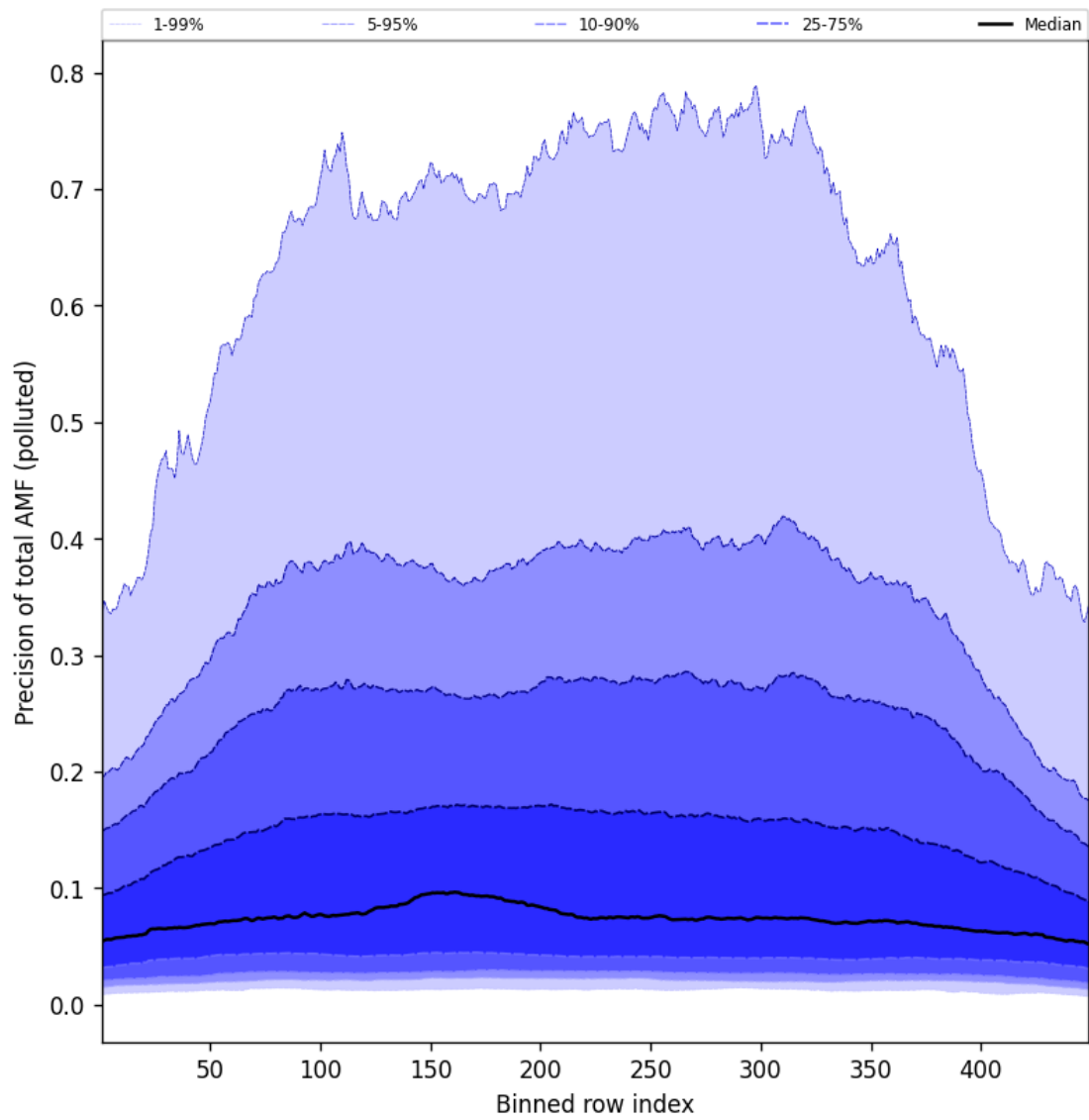
Figure 108: Along track statistics of “Precision of total AMF (polluted)” for 2025-05-06 to 2025-05-07
