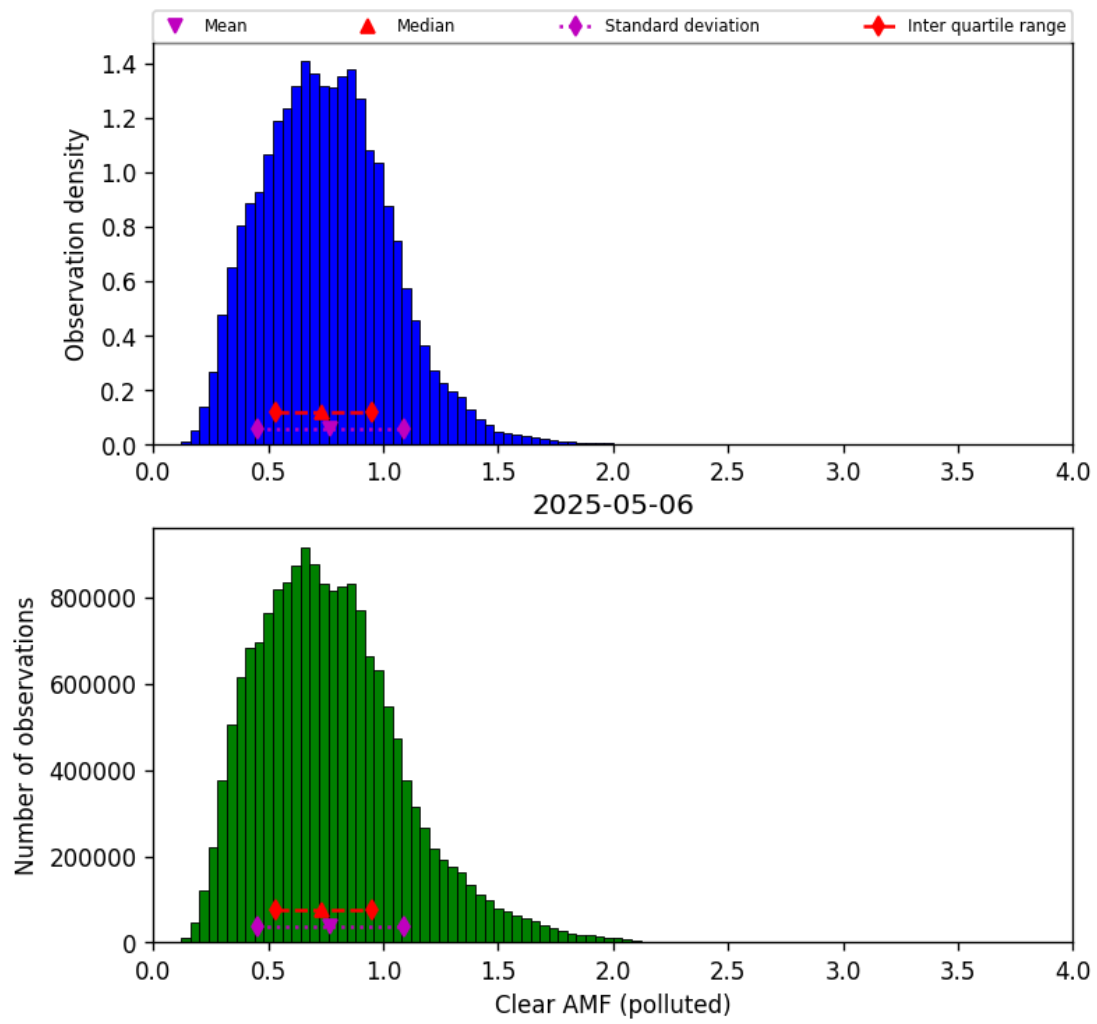
Figure 82: Histogram of “Clear AMF (polluted)” for 2025-05-06 to 2025-05-07
