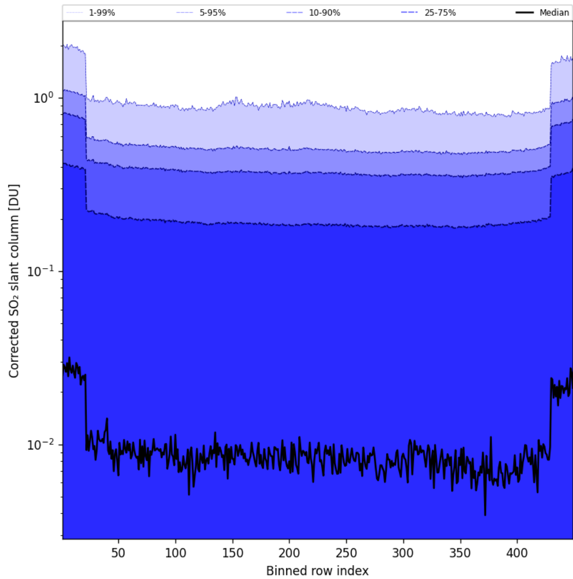
Figure 87: Along track statistics of “Corrected SO 2 slant column” for 2025-05-06 to 2025-05-07
