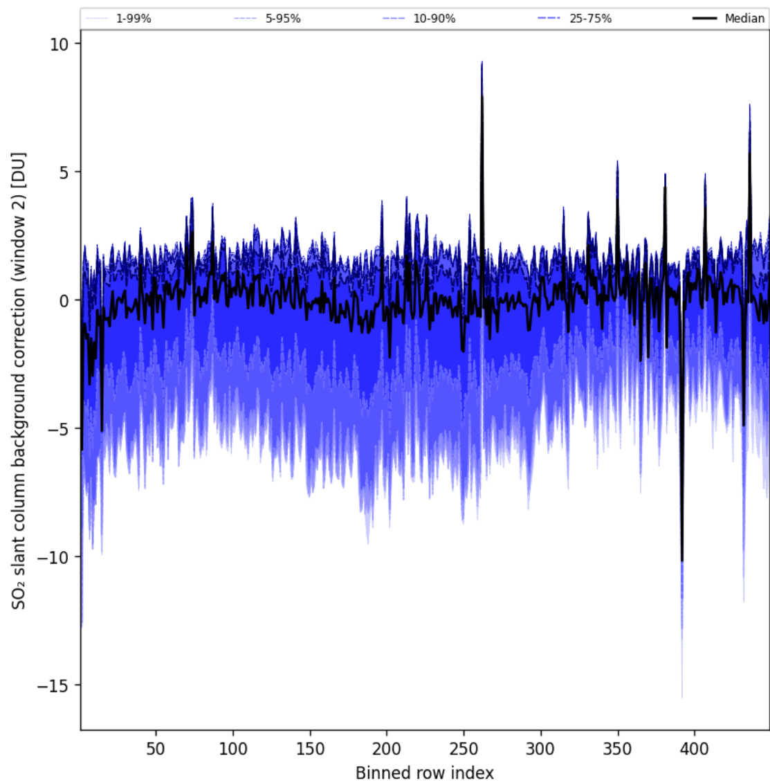
Figure 97: Along track statistics of “SO 2 slant column background correction (window 2)” for 2025-05-06 to 2025-05-07
