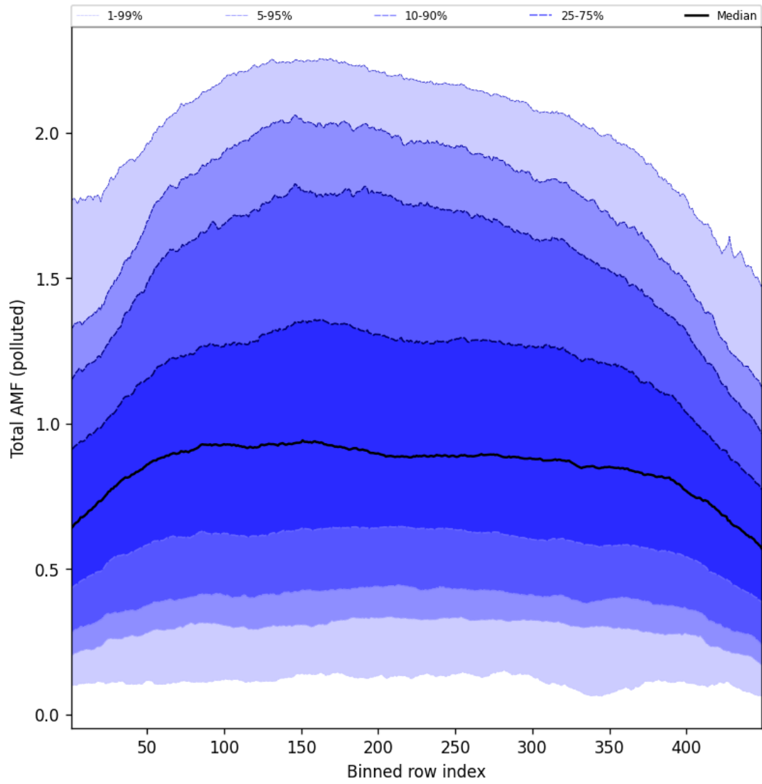
Figure 107: Along track statistics of “Total AMF (polluted)” for 2025-05-06 to 2025-05-07
