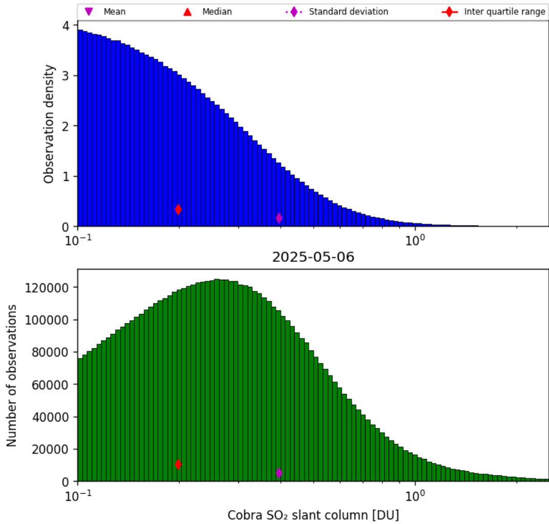
Figure 61: Histogram of “Cobra SO 2 slant column” for 2025-05-06 to 2025-05-07
