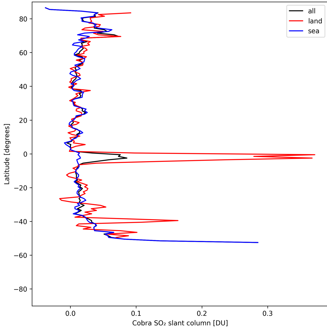
Figure 34: Zonal average of “Cobra SO 2 slant column” for 2025-05-06 to 2025-05-07.
