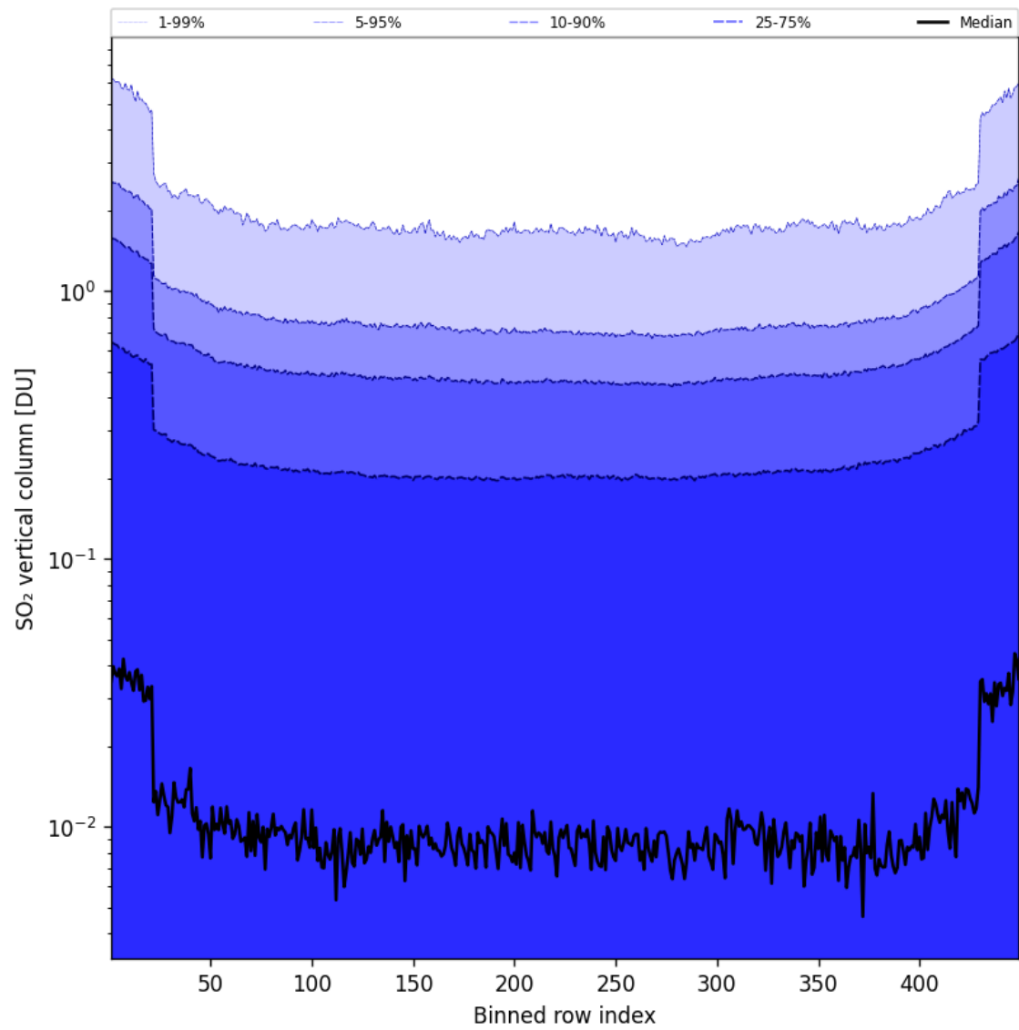
Figure 85: Along track statistics of “SO 2 vertical column” for 2025-05-06 to 2025-05-07
