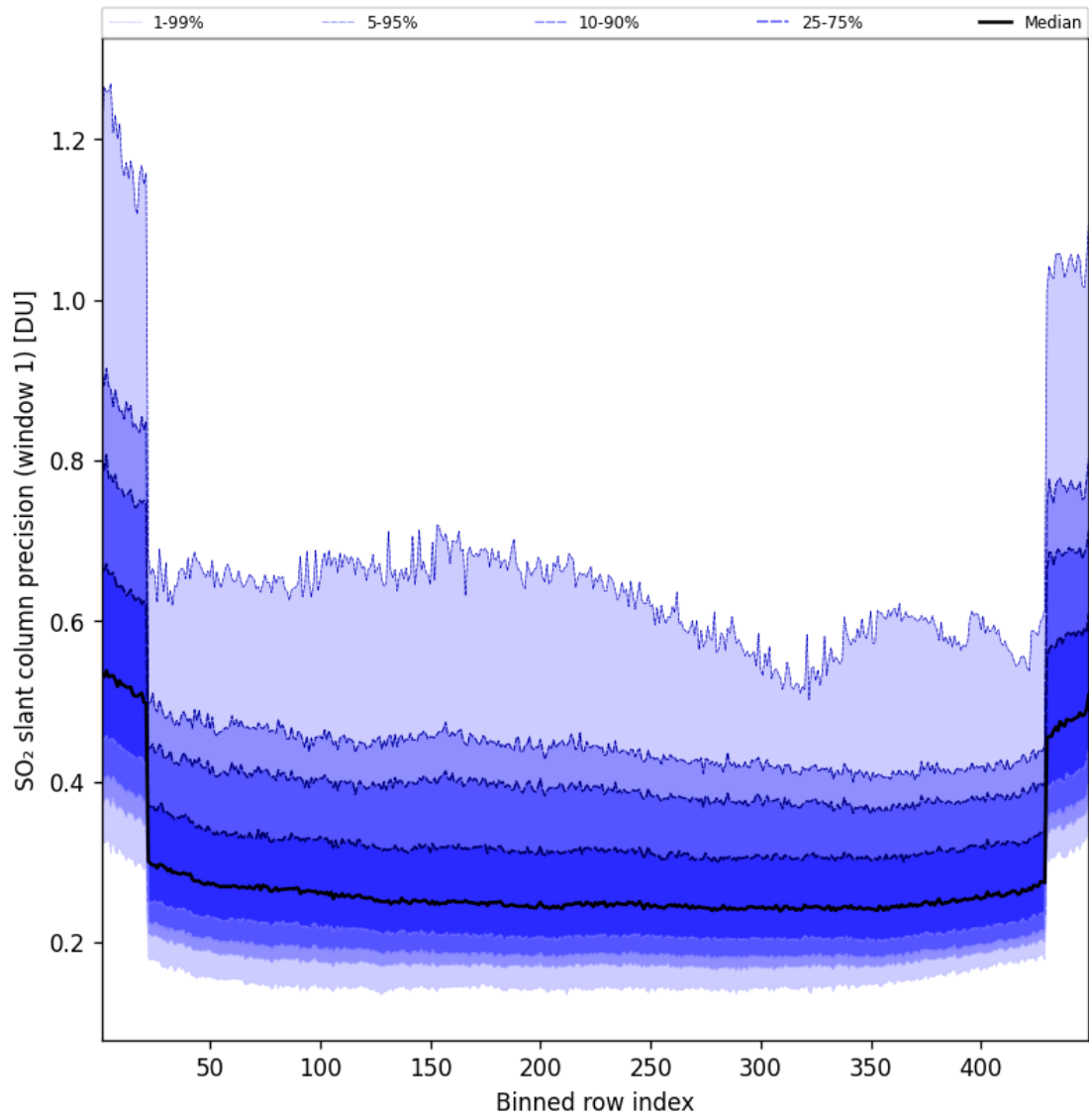
Figure 91: Along track statistics of “SO 2 slant column precision (window 1)” for 2025-05-06 to 2025-05-07
