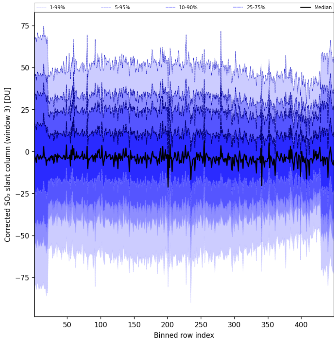
Figure 100: Along track statistics of “Corrected SO 2 slant column (window 3)” for 2025-05-06 to 2025-05-07
