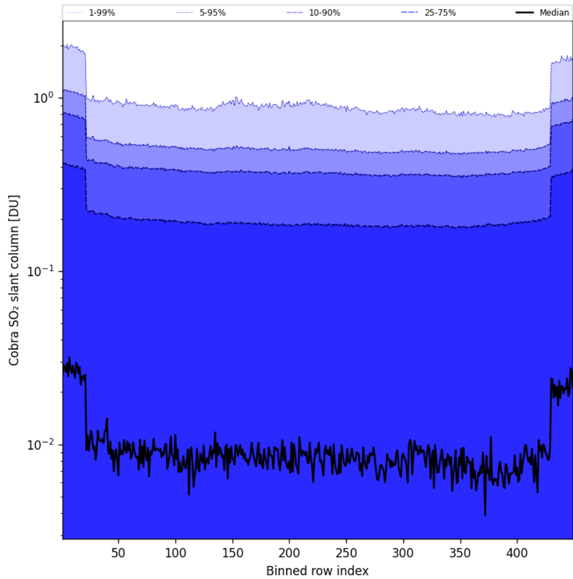
Figure 88: Along track statistics of “Cobra SO 2 slant column” for 2025-05-06 to 2025-05-07
