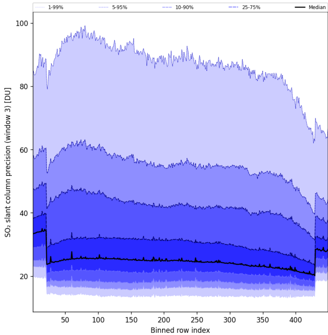
Figure 99: Along track statistics of “SO 2 slant column precision (window 3)” for 2025-05-06 to 2025-05-07
