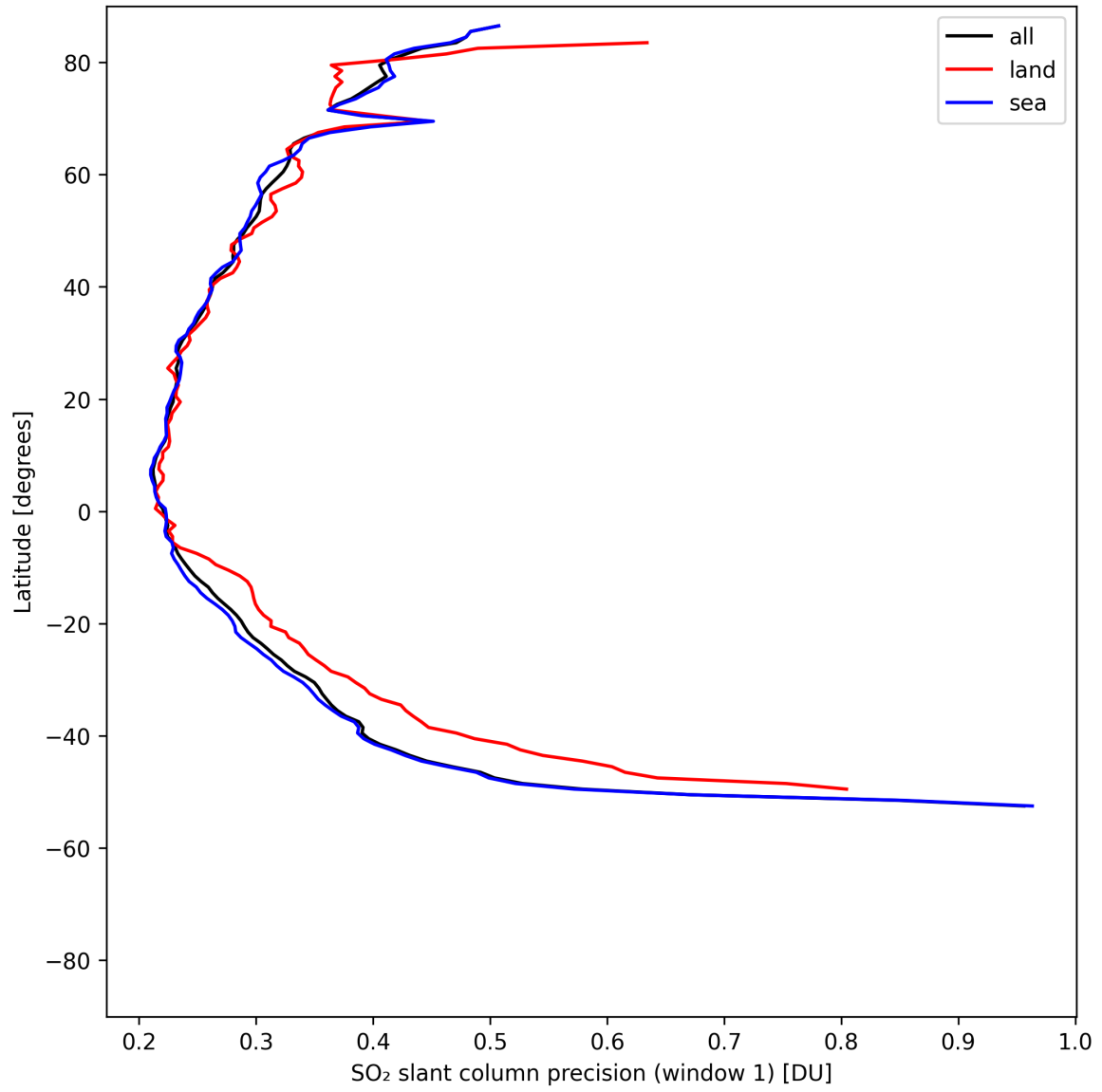
Figure 37: Zonal average of “SO 2 slant column precision (window 1)” for 2025-05-06 to 2025-05-07.
