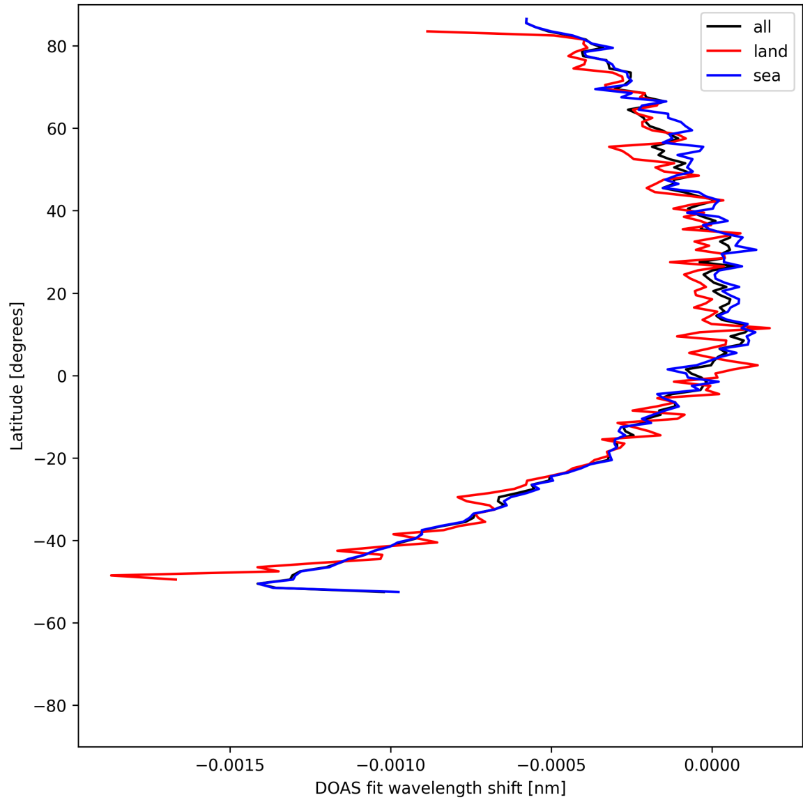
Figure 50: Zonal average of “DOAS fit wavelength shift” for 2025-05-06 to 2025-05-07.
