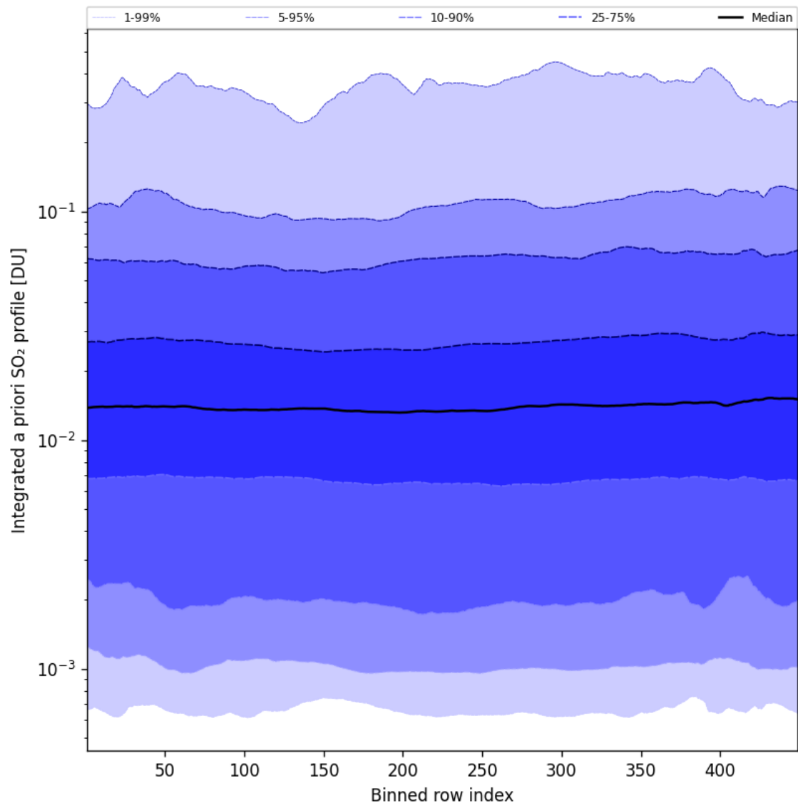
Figure 103: Along track statistics of “Integrated a priori SO 2 profile” for 2025-05-06 to 2025-05-07
