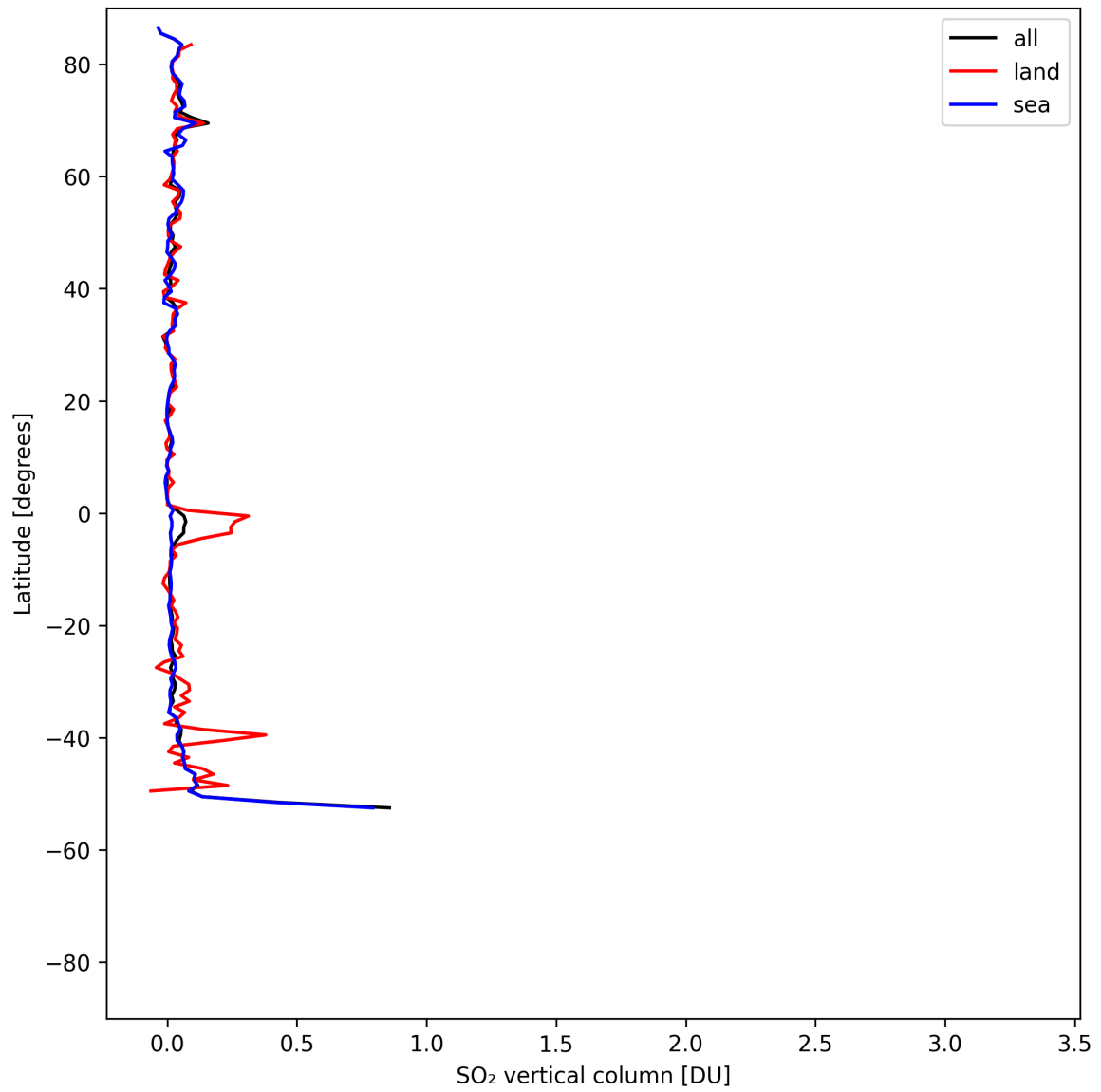
Figure 31: Zonal average of “SO 2 vertical column” for 2025-05-06 to 2025-05-07.
