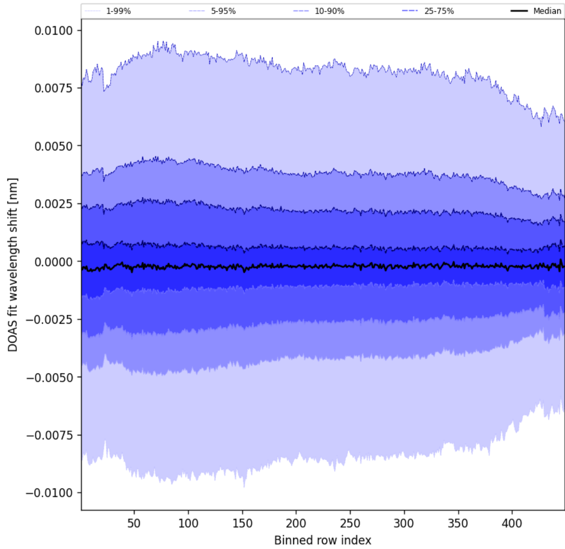
Figure 104: Along track statistics of “DOAS fit wavelength shift” for 2025-05-06 to 2025-05-07
