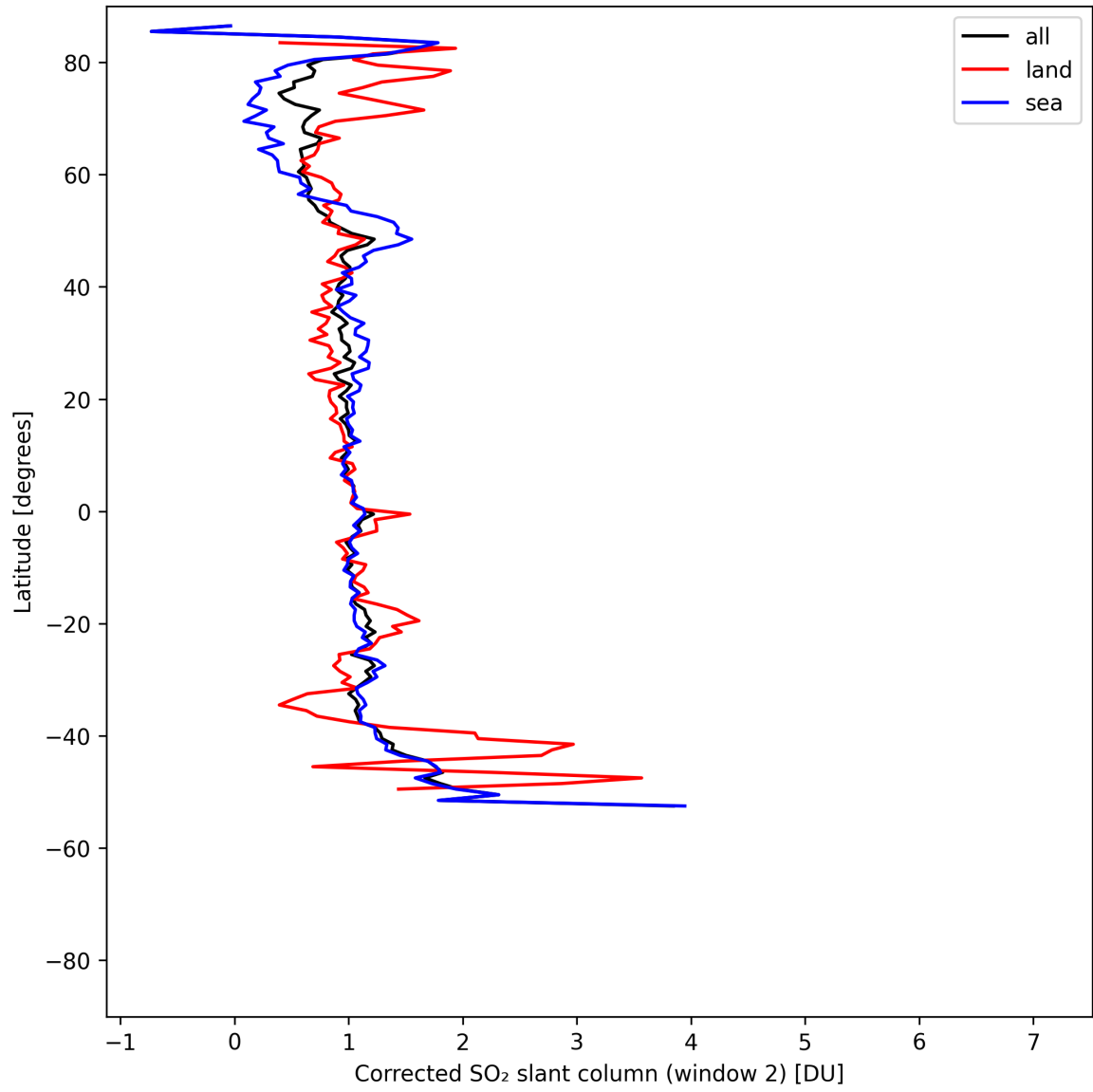
Figure 42: Zonal average of “Corrected SO 2 slant column (window 2)” for 2025-05-06 to 2025-05-07.
