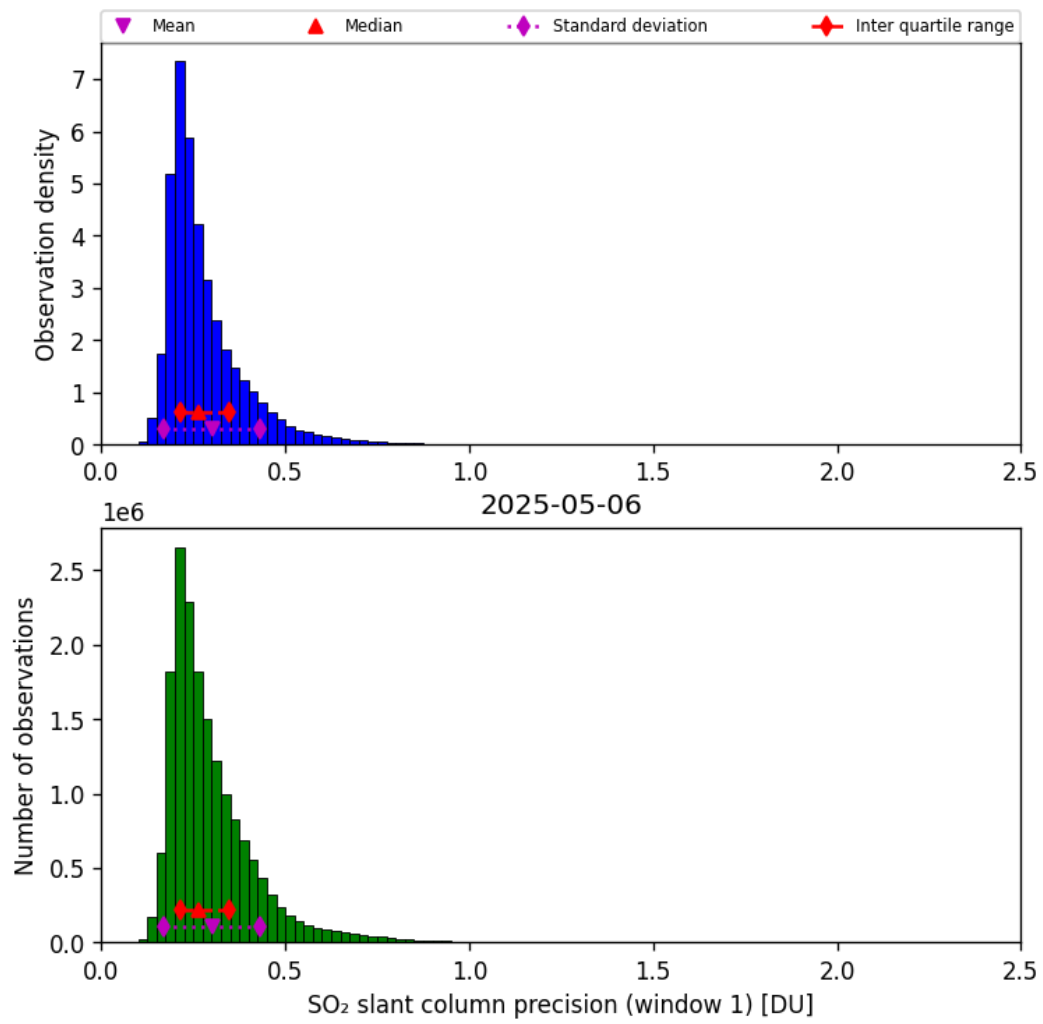
Figure 64: Histogram of “SO 2 slant column precision (window 1)” for 2025-05-06 to 2025-05-07
