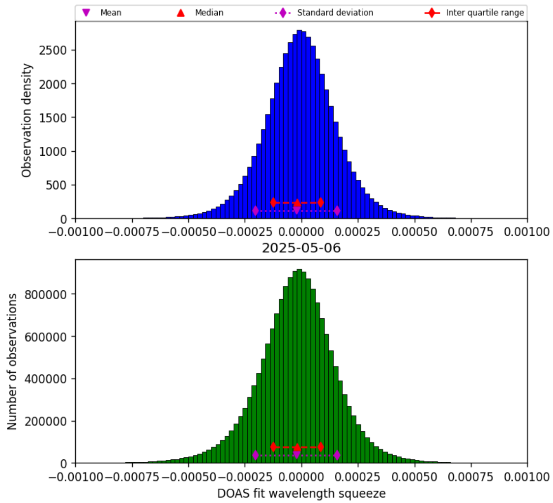
Figure 78: Histogram of “DOAS fit wavelength squeeze” for 2025-05-06 to 2025-05-07
