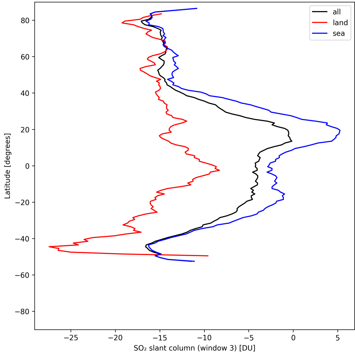
Figure 44: Zonal average of “SO 2 slant column (window 3)” for 2025-05-06 to 2025-05-07.
