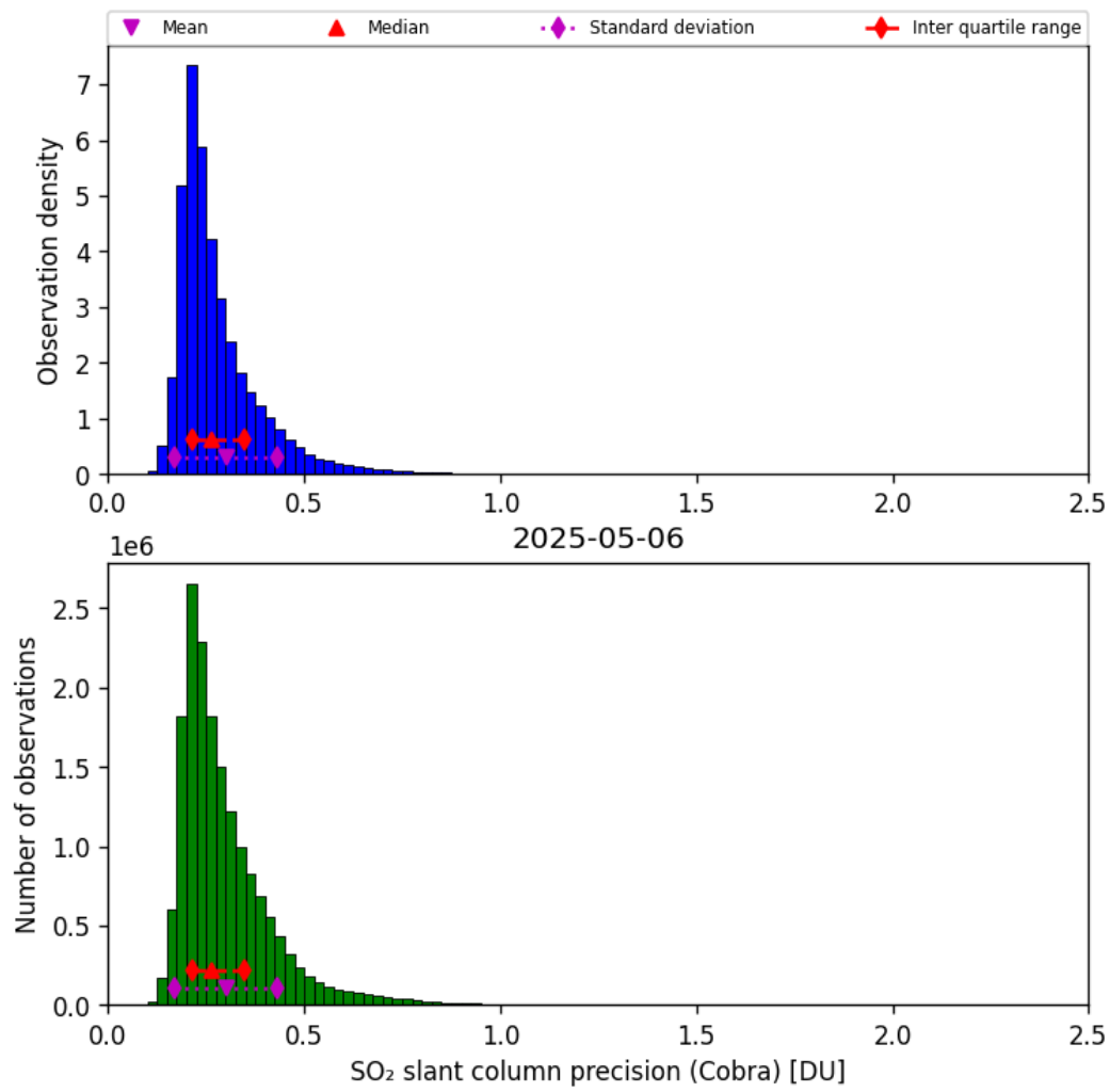
Figure 62: Histogram of “SO 2 slant column precision (Cobra)” for 2025-05-06 to 2025-05-07
