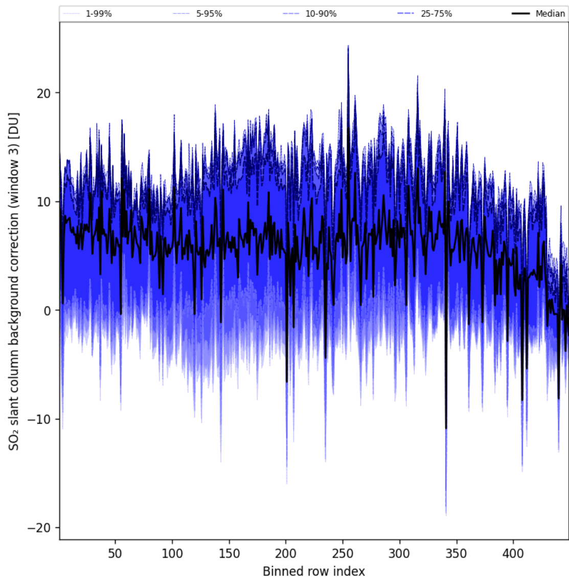
Figure 101: Along track statistics of “SO 2 slant column background correction (window 3)” for 2025-05-06 to 2025-05-07
