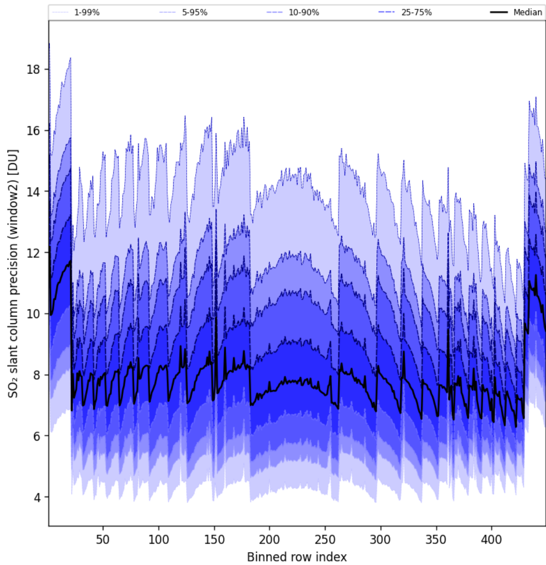
Figure 95: Along track statistics of “SO 2 slant column precision (window2)” for 2025-05-06 to 2025-05-07
