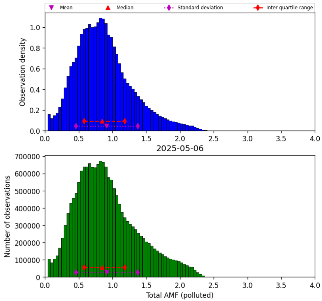
Figure 80: Histogram of “Total AMF (polluted)” for 2025-05-06 to 2025-05-07
