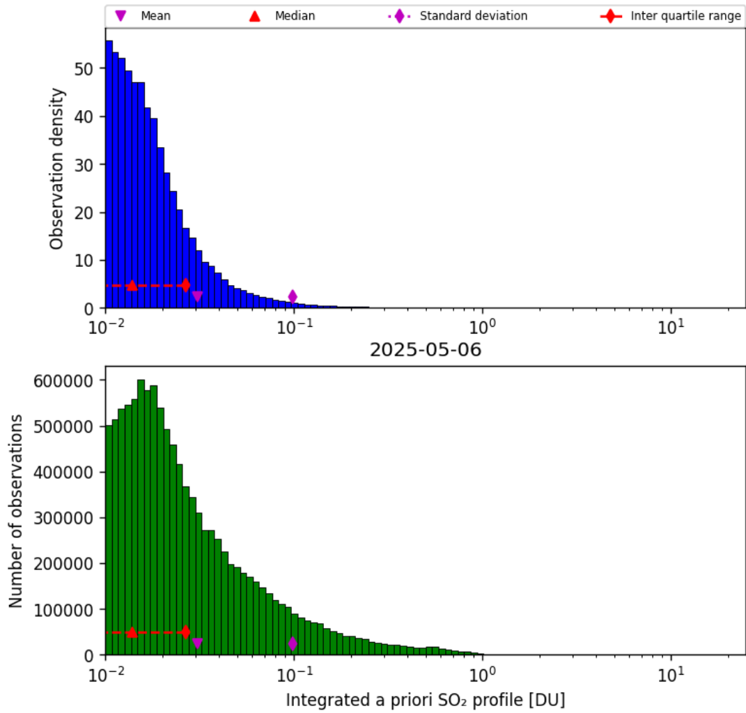
Figure 76: Histogram of “Integrated a priori SO 2 profile” for 2025-05-06 to 2025-05-07
