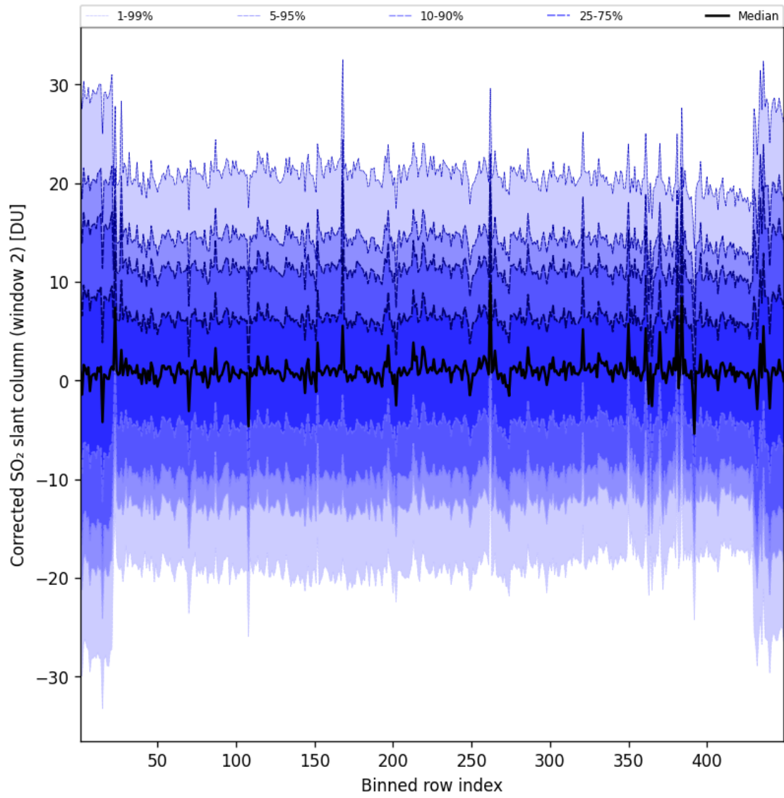
Figure 96: Along track statistics of “Corrected SO 2 slant column (window 2)” for 2025-05-06 to 2025-05-07
