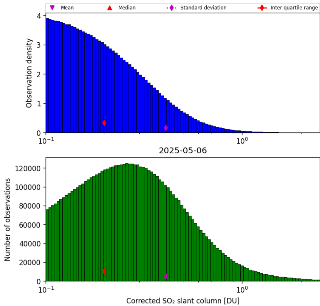
Figure 60: Histogram of “Corrected SO 2 slant column” for 2025-05-06 to 2025-05-07
