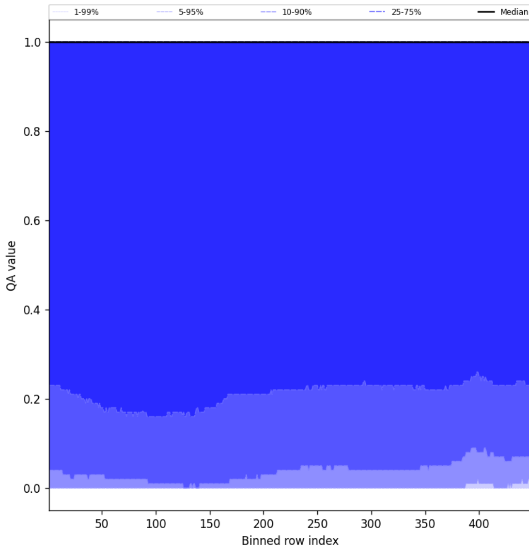
Figure 84: Along track statistics of “QA value” for 2025-05-06 to 2025-05-07
