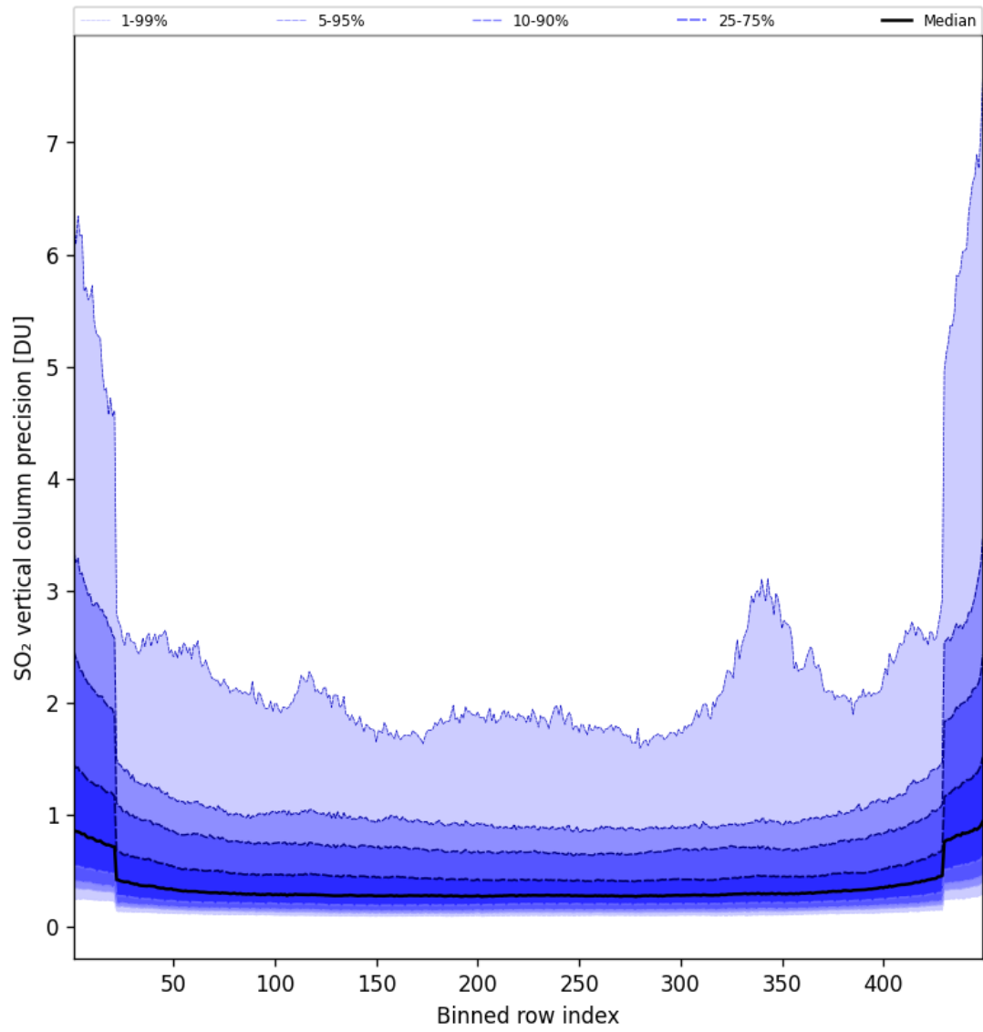
Figure 86: Along track statistics of “SO 2 vertical column precision” for 2025-05-06 to 2025-05-07
