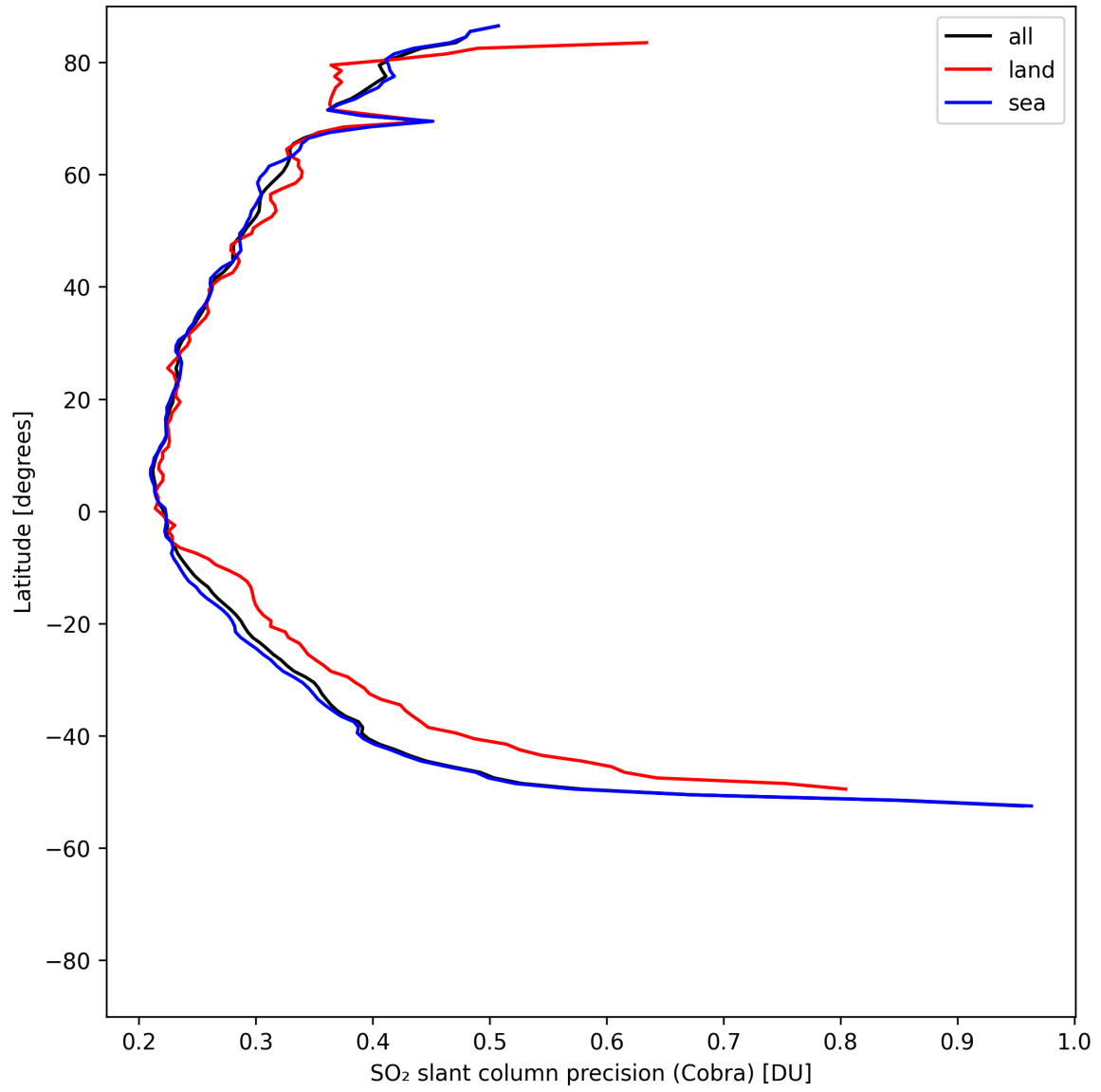
Figure 35: Zonal average of “SO 2 slant column precision (Cobra)” for 2025-05-06 to 2025-05-07.
