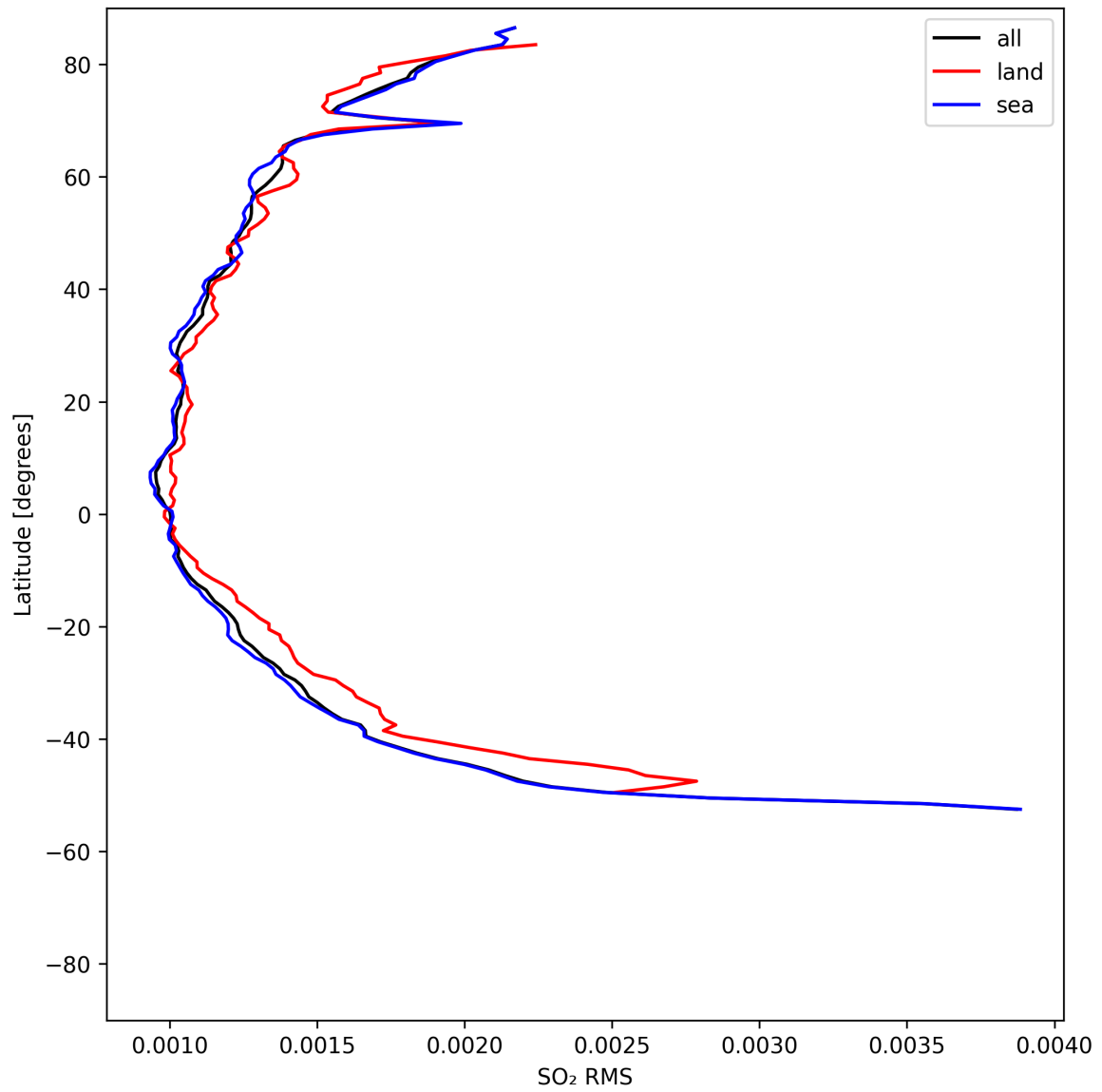
Figure 52: Zonal average of “SO 2 RMS” for 2025-05-06 to 2025-05-07.
