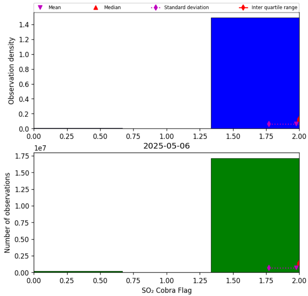
Figure 75: Histogram of “SO 2 Cobra Flag” for 2025-05-06 to 2025-05-07
