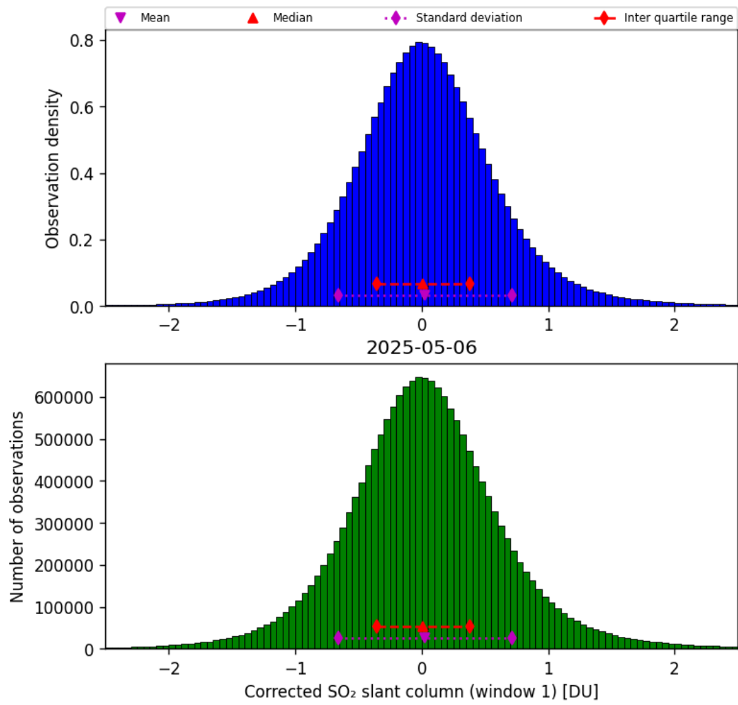
Figure 65: Histogram of “Corrected SO 2 slant column (window 1)” for 2025-05-06 to 2025-05-07
