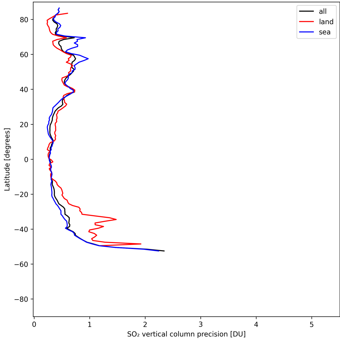
Figure 32: Zonal average of “SO 2 vertical column precision” for 2025-05-06 to 2025-05-07.
