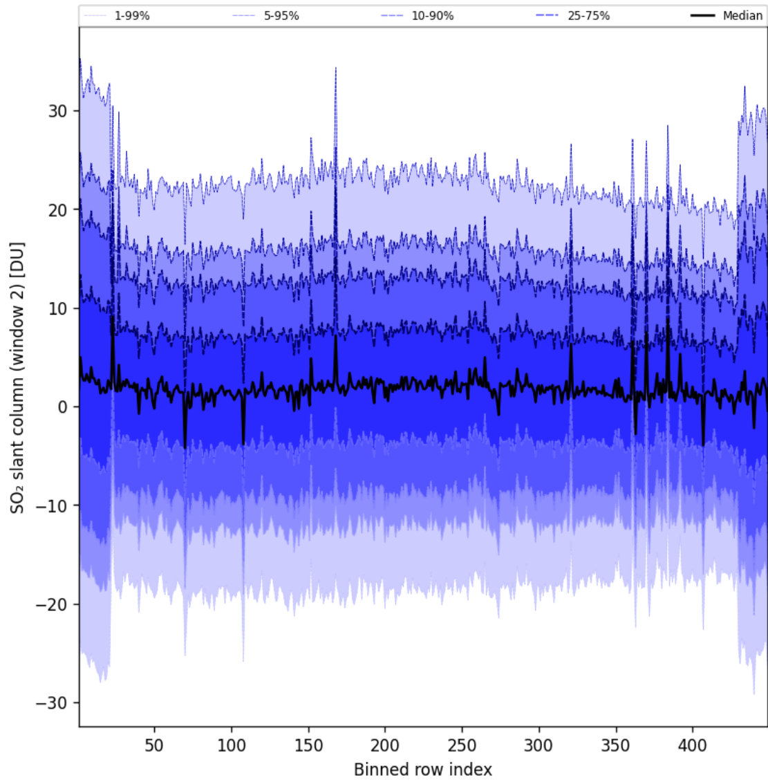
Figure 94: Along track statistics of “SO 2 slant column (window 2)” for 2025-05-06 to 2025-05-07
