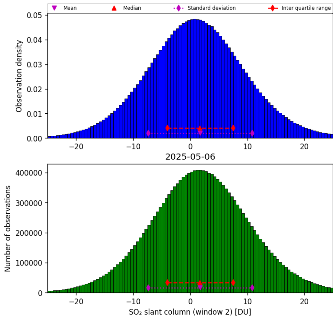
Figure 67: Histogram of “SO 2 slant column (window 2)” for 2025-05-06 to 2025-05-07
