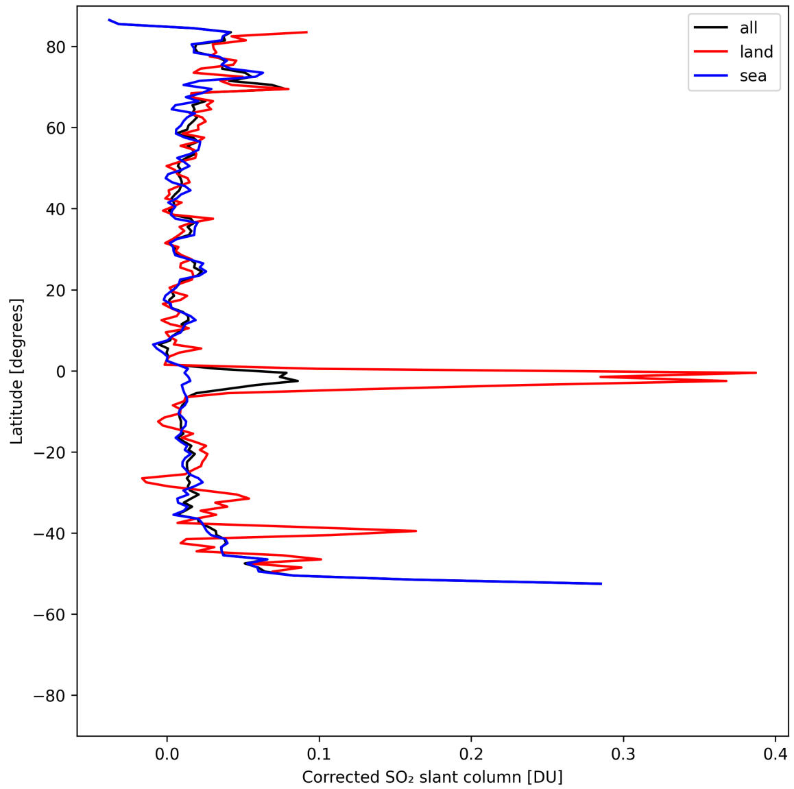
Figure 33: Zonal average of "Corrected SO 2 slant column" for 2025-05-06 to 2025-05-07.
