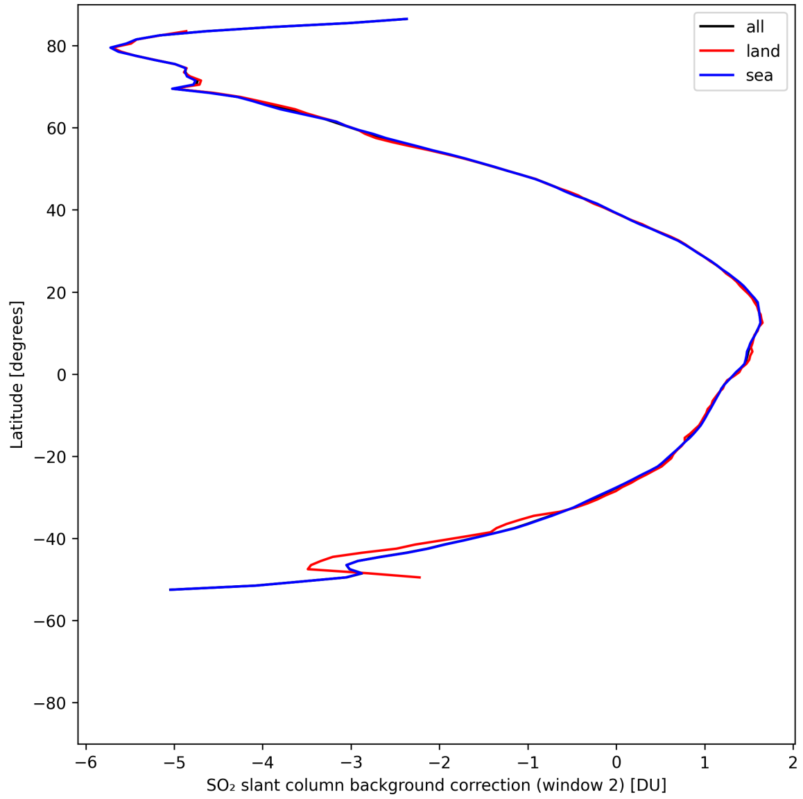
Figure 43: Zonal average of “SO 2 slant column background correction (window 2)” for 2025-05-06 to 2025-05-07.
