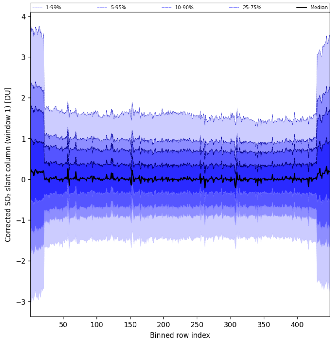
Figure 92: Along track statistics of “Corrected SO 2 slant column (window 1)” for 2025-05-06 to 2025-05-07
