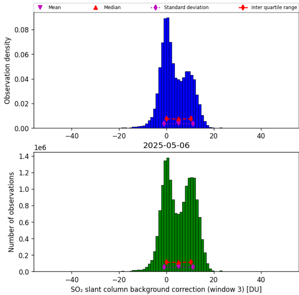
Figure 74: Histogram of “SO 2 slant column background correction (window 3)” for 2025-05-06 to 2025-05-07
