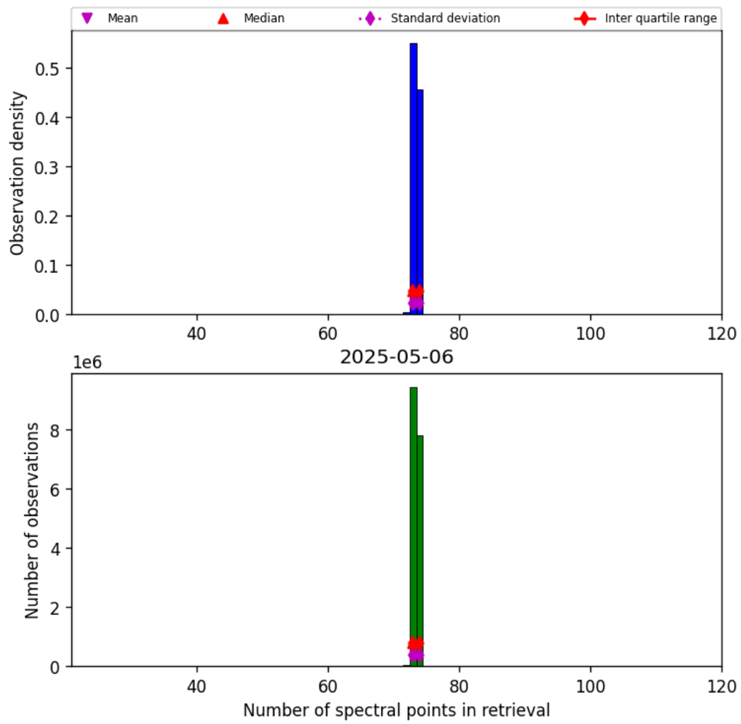
Figure 83: Histogram of “Number of spectral points in retrieval” for 2025-05-06 to 2025-05-07
