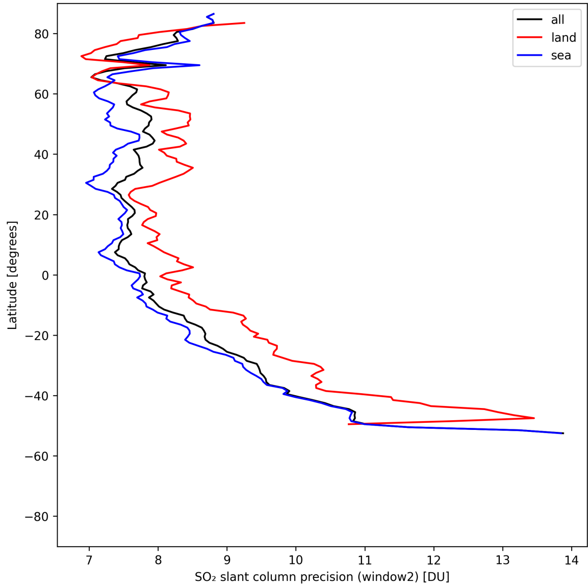
Figure 41: Zonal average of “SO 2 slant column precision (window2)” for 2025-05-06 to 2025-05-07.
