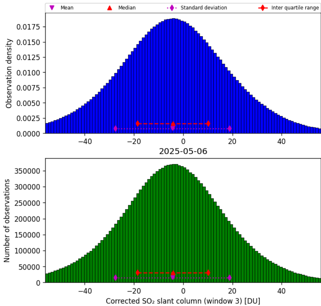
Figure 73: Histogram of “Corrected SO 2 slant column (window 3)” for 2025-05-06 to 2025-05-07
