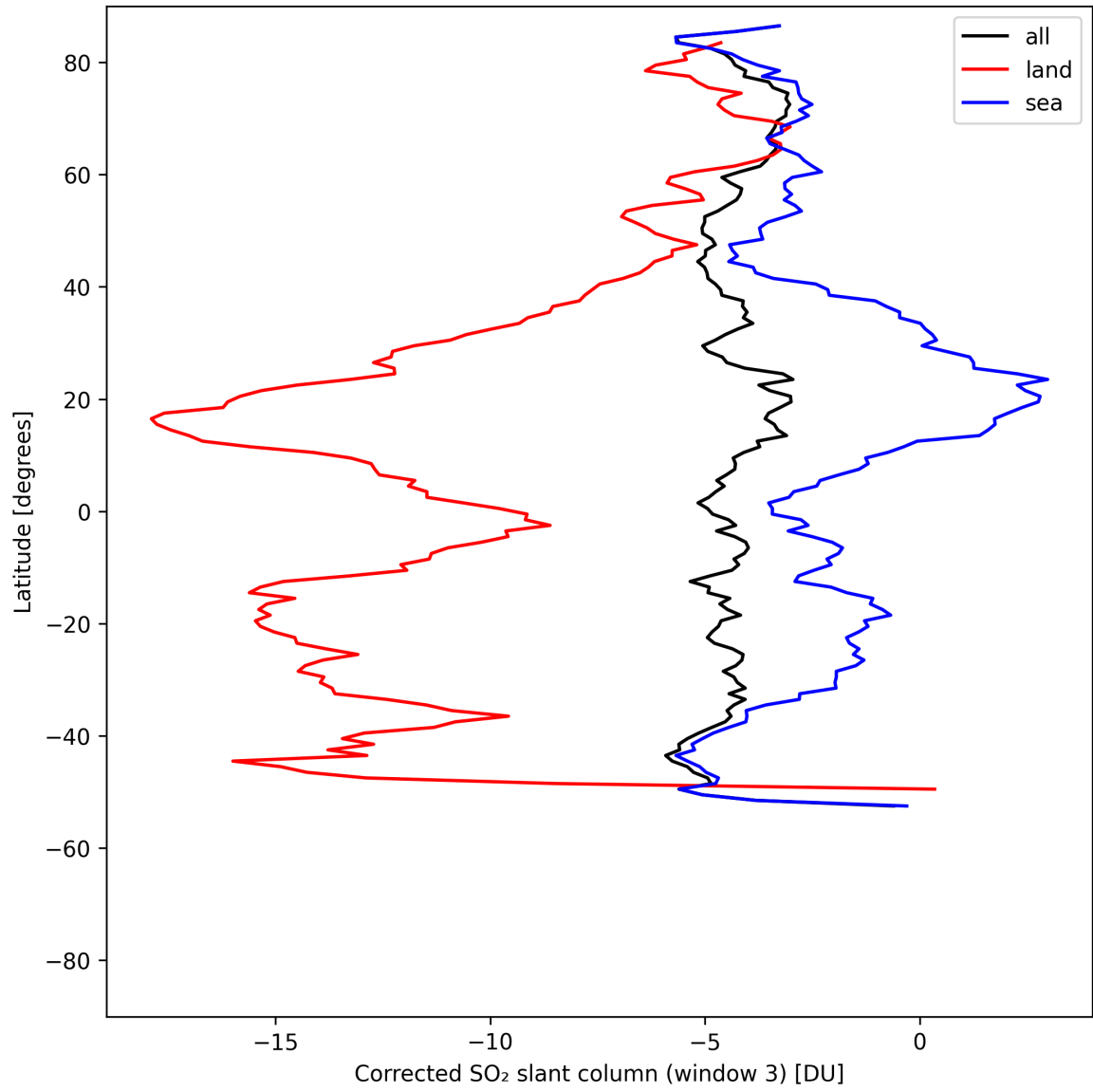
Figure 46: Zonal average of “Corrected SO 2 slant column (window 3)” for 2025-05-06 to 2025-05-07.
