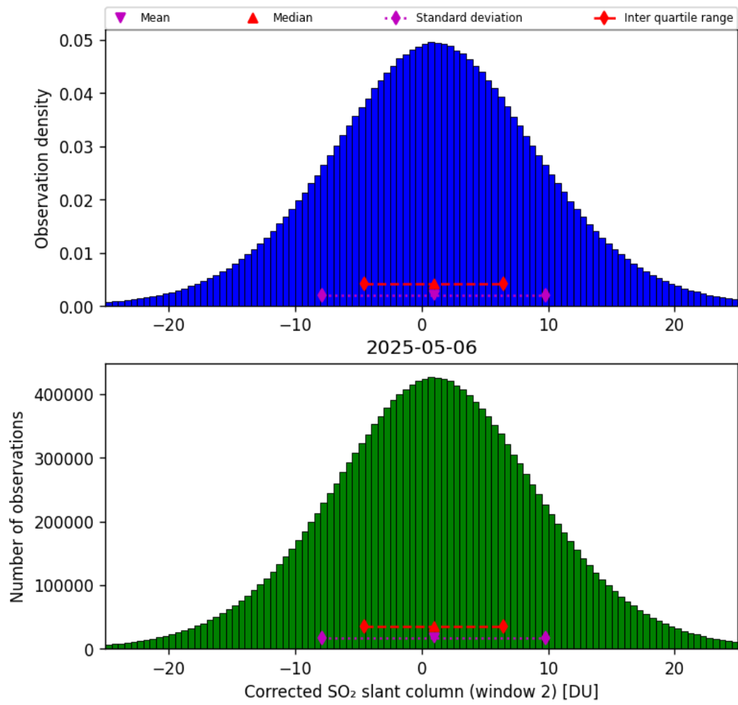
Figure 69: Histogram of “Corrected SO 2 slant column (window 2)” for 2025-05-06 to 2025-05-07
