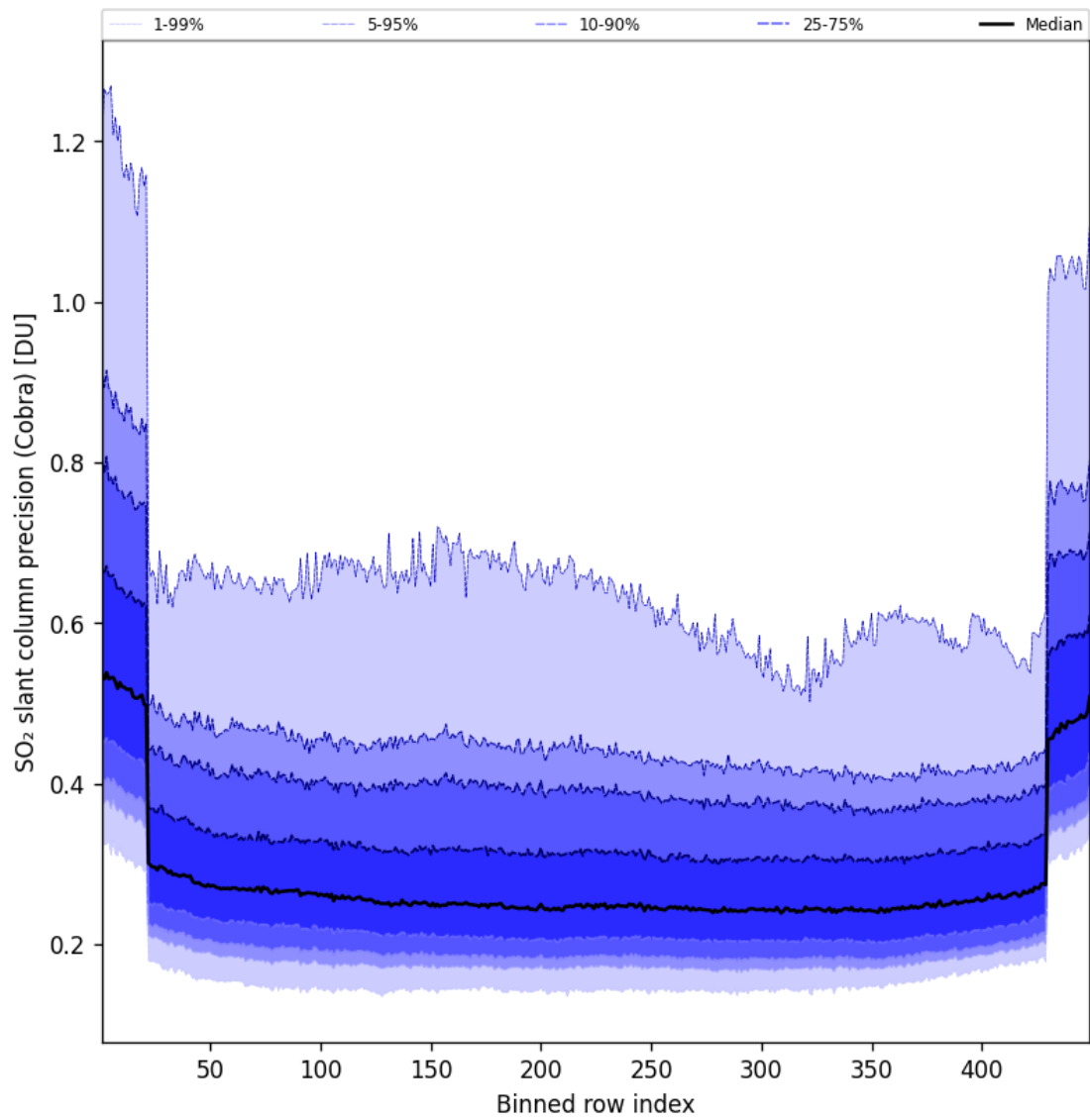
Figure 89: Along track statistics of “SO 2 slant column precision (Cobra)” for 2025-05-06 to 2025-05-07
