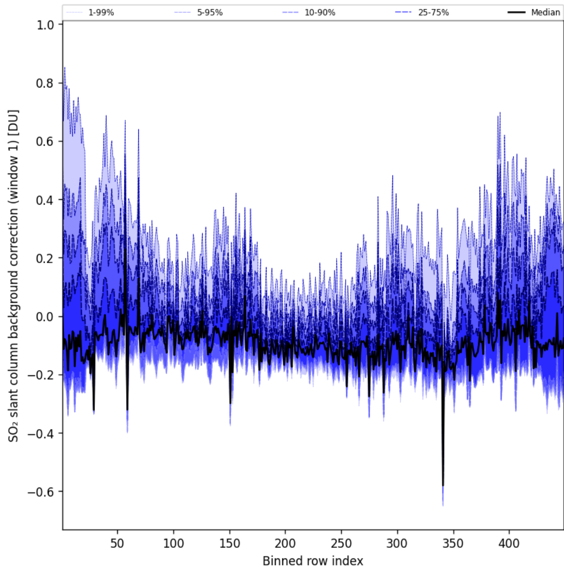
Figure 93: Along track statistics of “SO 2 slant column background correction (window 1)” for 2025-05-06 to 2025-05-07
