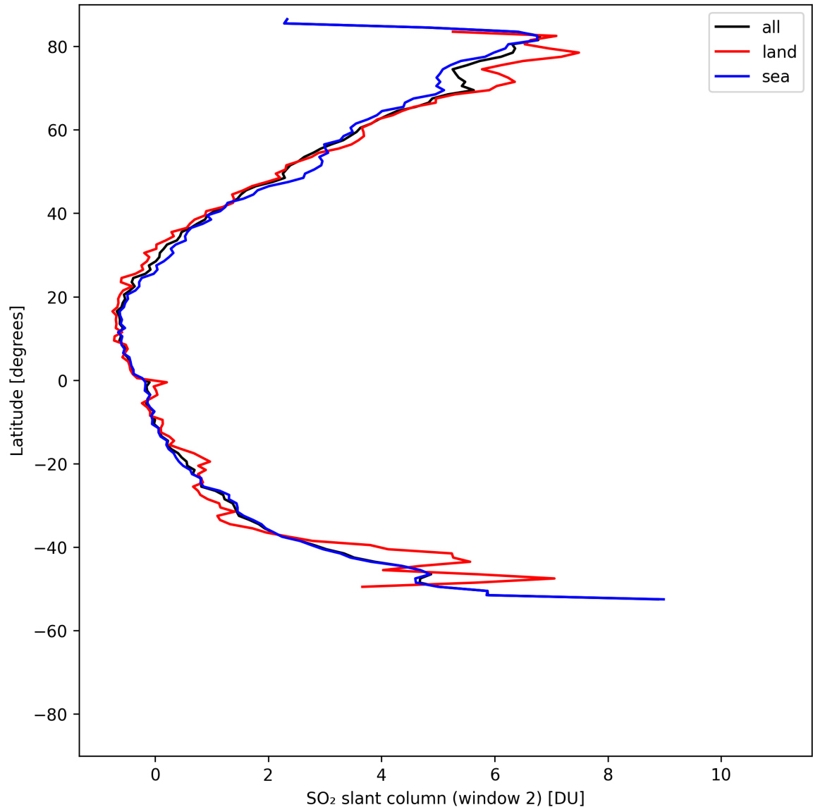
Figure 40: Zonal average of “SO 2 slant column (window 2)” for 2025-05-06 to 2025-05-07.
