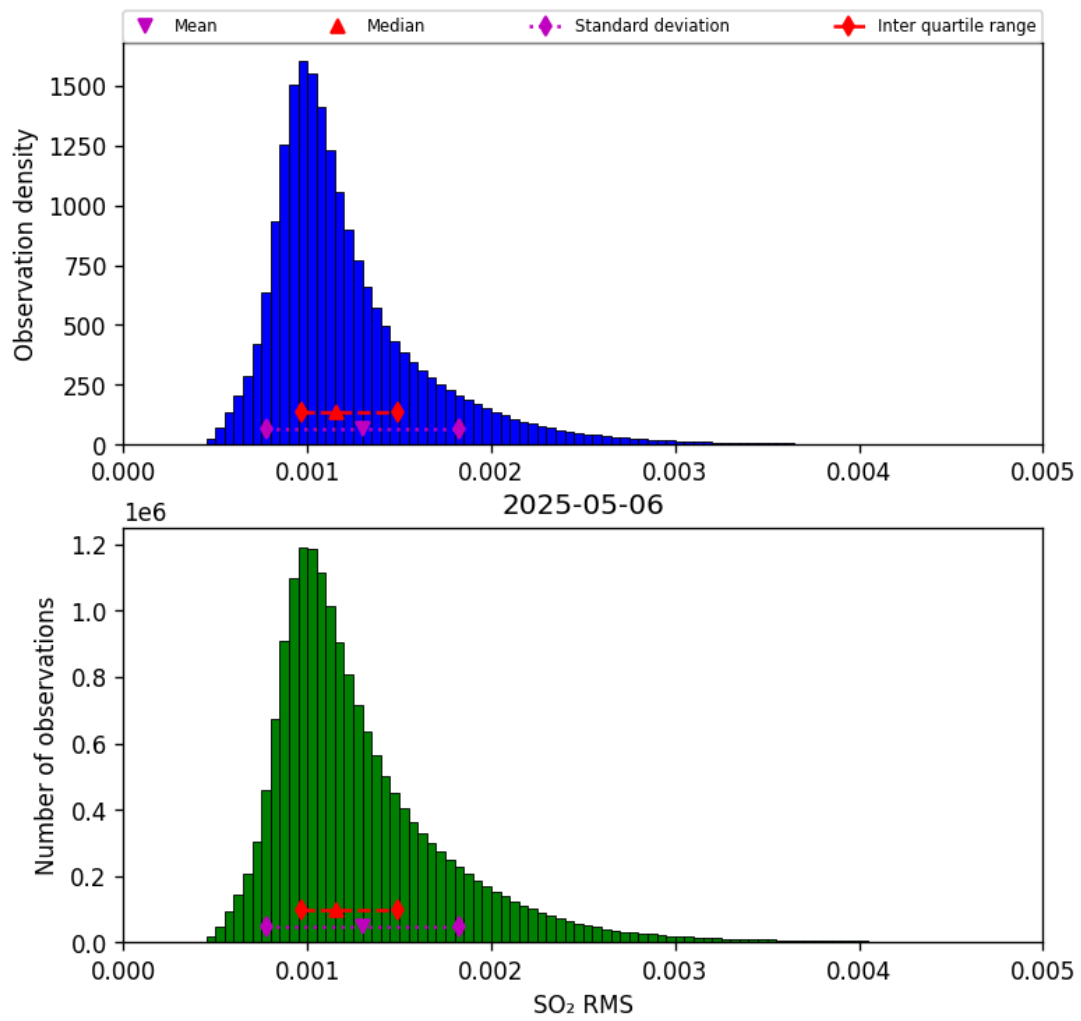
Figure 79: Histogram of “SO 2 RMS” for 2025-05-06 to 2025-05-07
