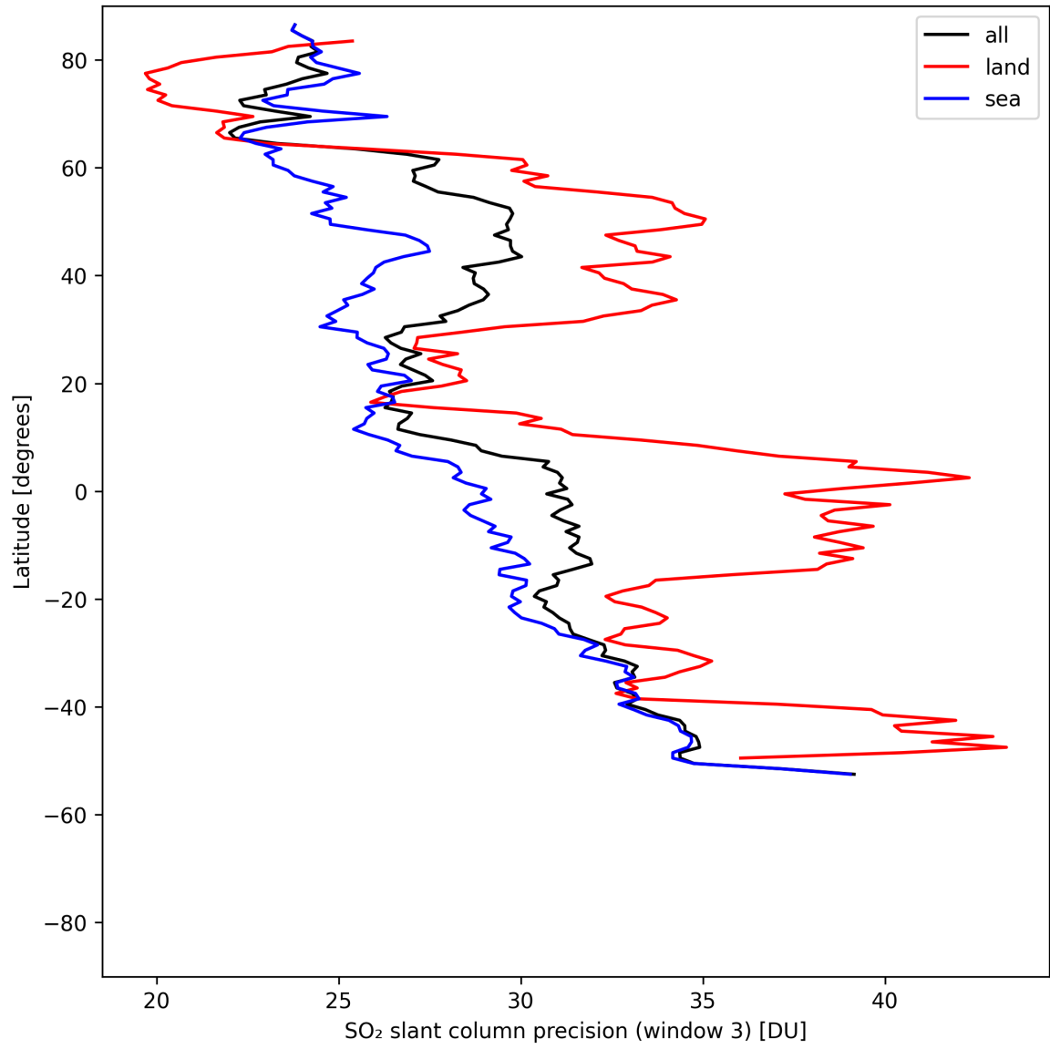
Figure 45: Zonal average of “SO 2 slant column precision (window 3)” for 2025-05-06 to 2025-05-07.
