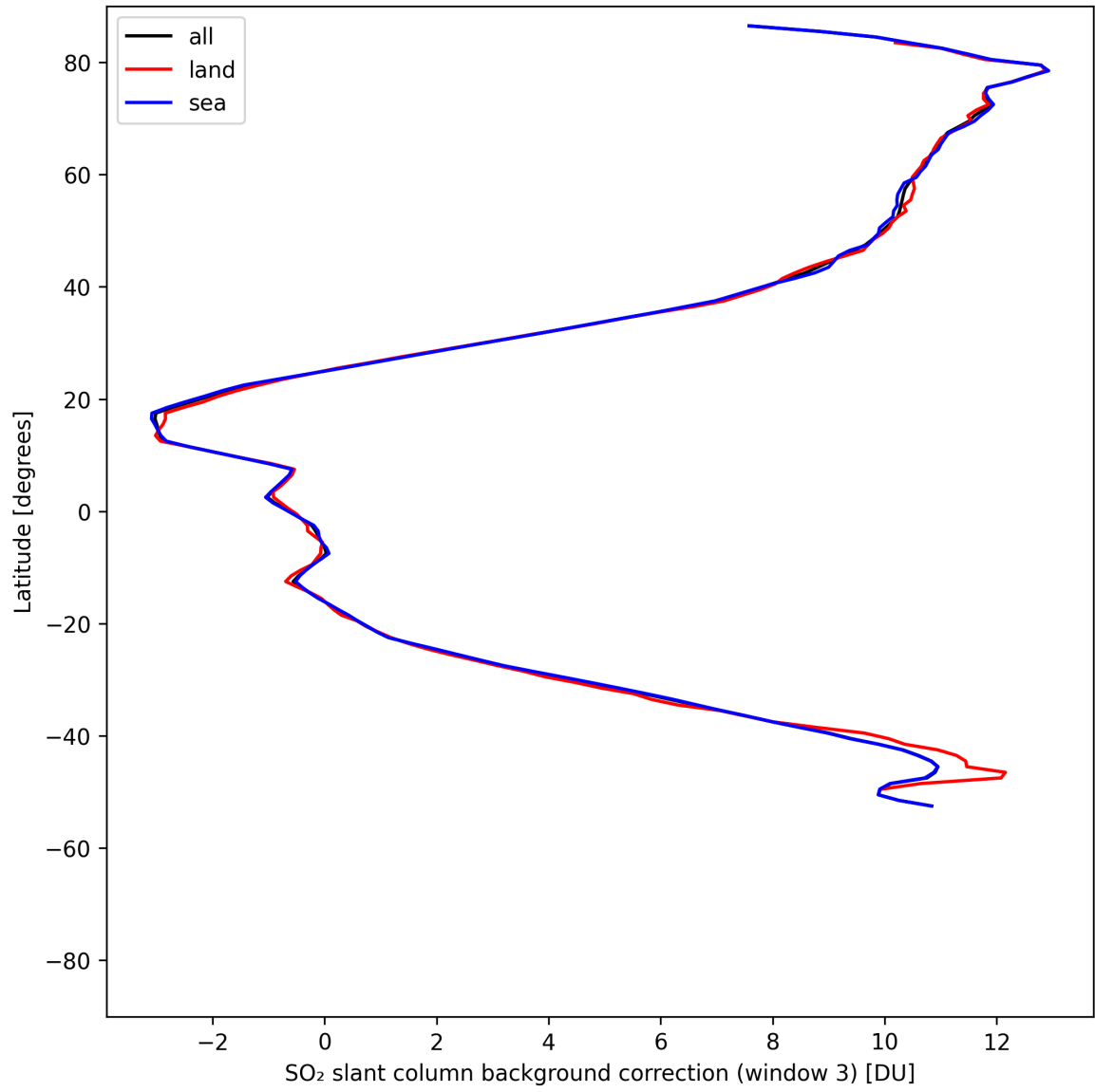
Figure 47: Zonal average of “SO 2 slant column background correction (window 3)” for 2025-05-06 to 2025-05-07.
