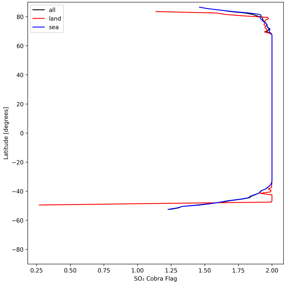
Figure 48: Zonal average of "SO 2 Cobra Flag" for 2025-05-06 to 2025-05-07.
