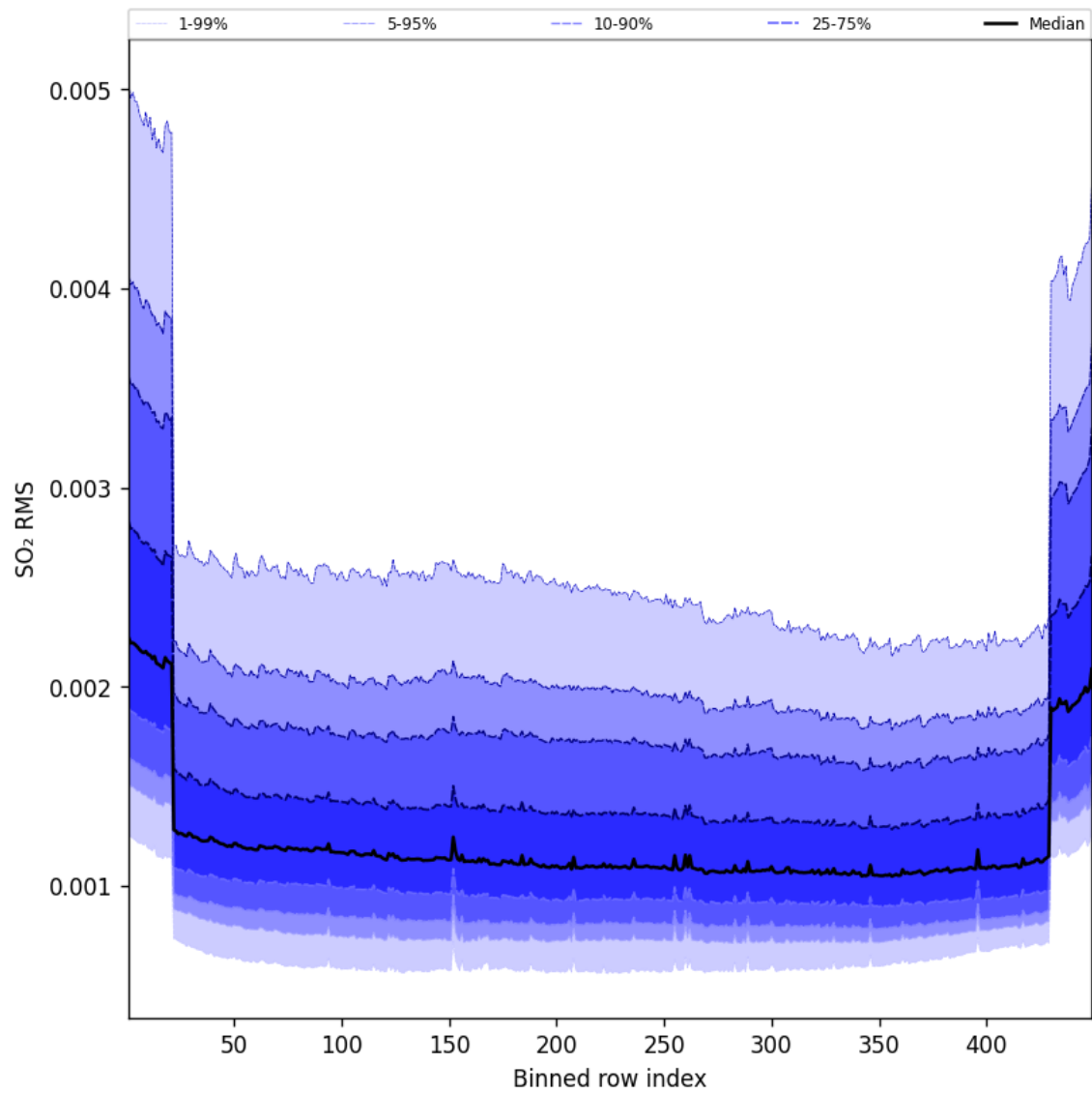
Figure 106: Along track statistics of “SO 2 RMS” for 2025-05-06 to 2025-05-07
