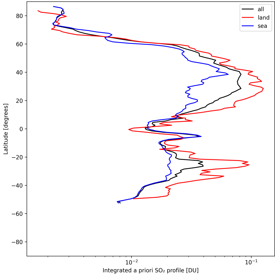
Figure 49: Zonal average of “Integrated a priori SO 2 profile” for 2025-05-06 to 2025-05-07.
