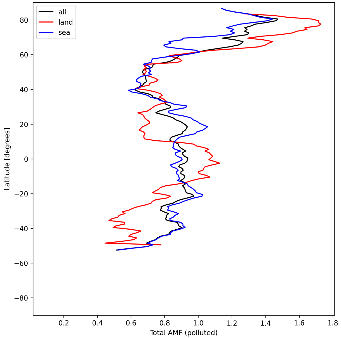
Figure 53: Zonal average of “Total AMF (polluted)” for 2025-05-06 to 2025-05-07.
