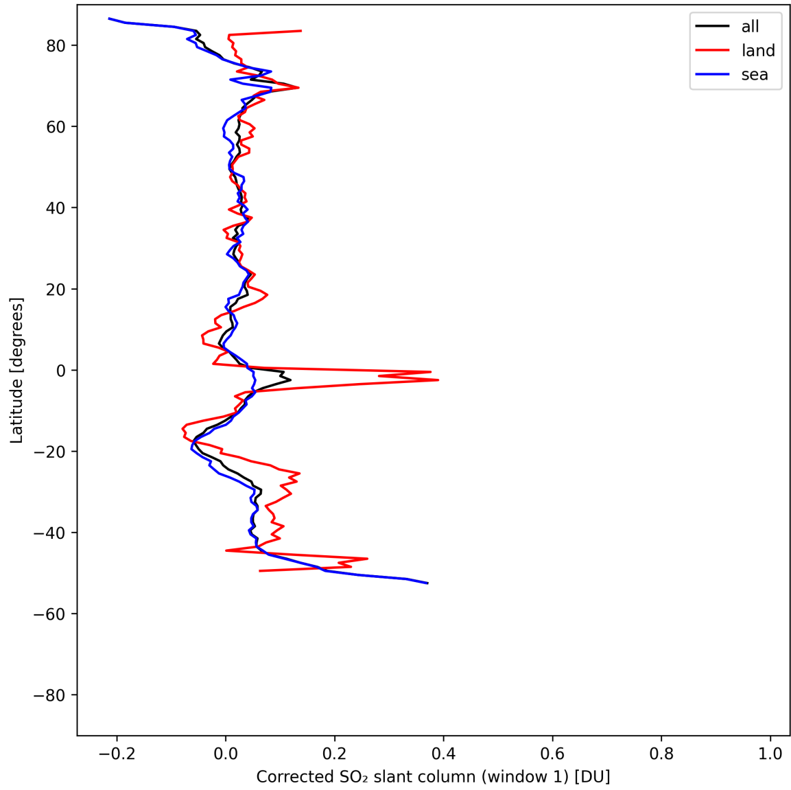
Figure 38: Zonal average of “Corrected SO 2 slant column (window 1)” for 2025-05-06 to 2025-05-07.
