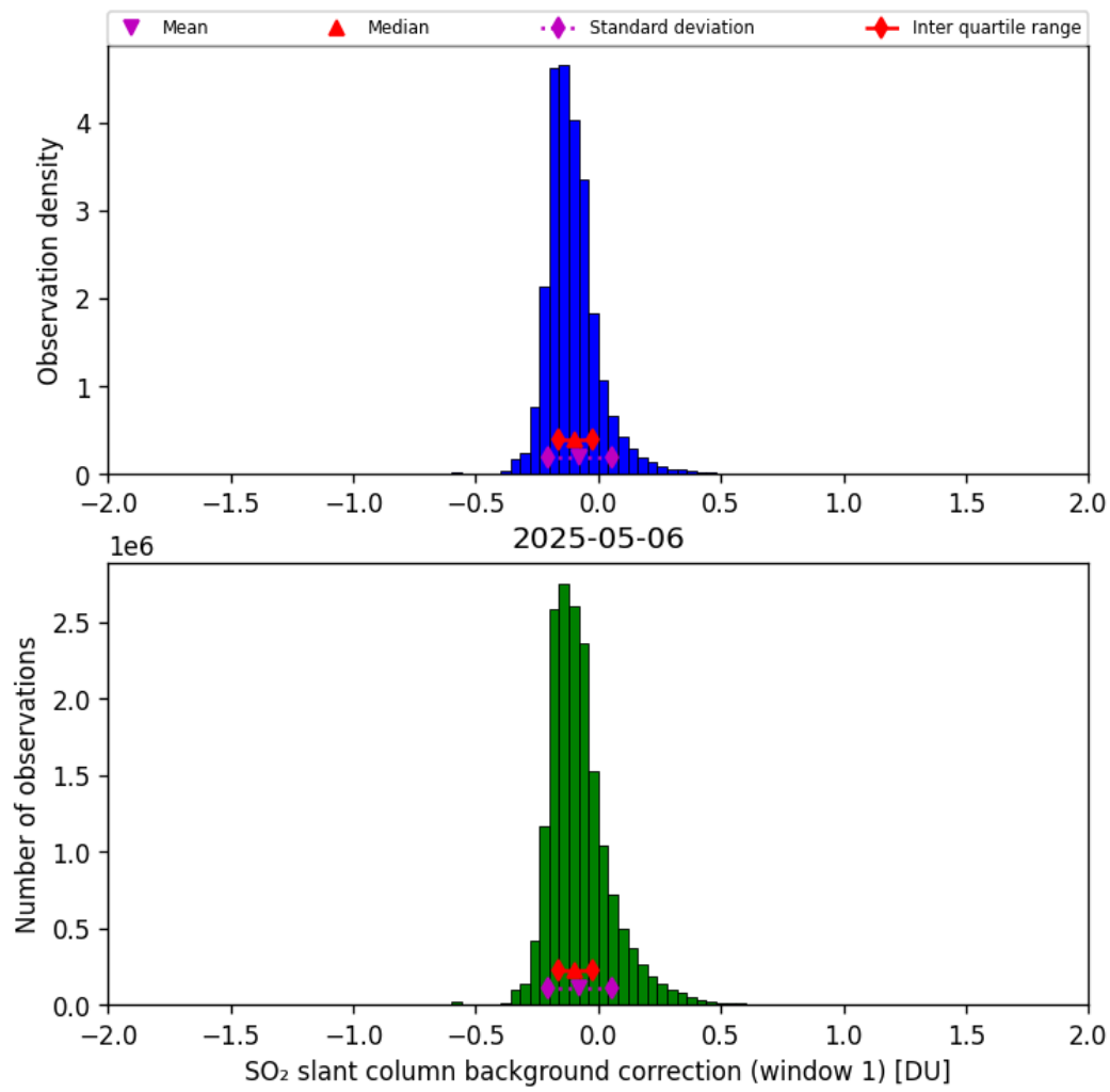
Figure 66: Histogram of “SO 2 slant column background correction (window 1)” for 2025-05-06 to 2025-05-07
