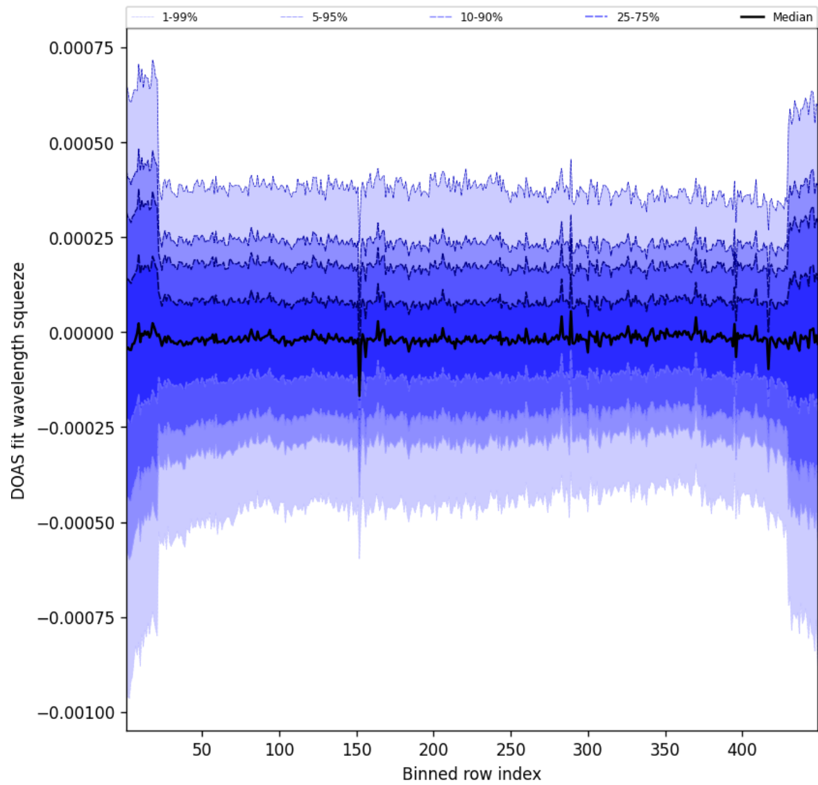
Figure 105: Along track statistics of “DOAS fit wavelength squeeze” for 2025-05-06 to 2025-05-07
