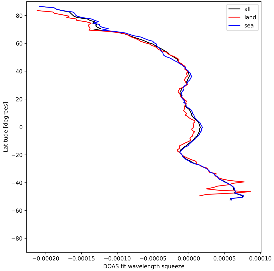
Figure 51: Zonal average of “DOAS fit wavelength squeeze” for 2025-05-06 to 2025-05-07.
