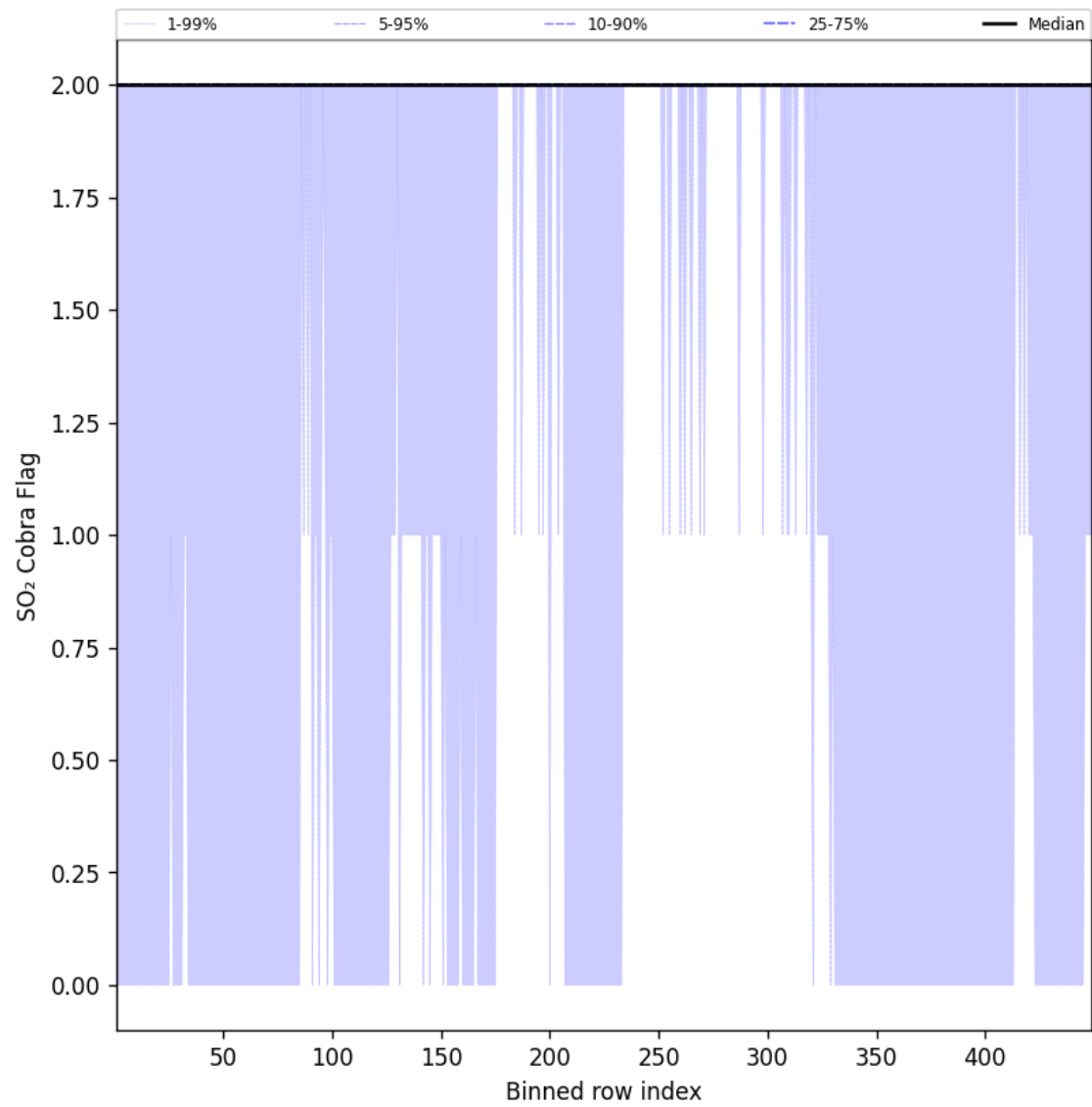
Figure 102: Along track statistics of “SO 2 Cobra Flag” for 2025-05-06 to 2025-05-07
