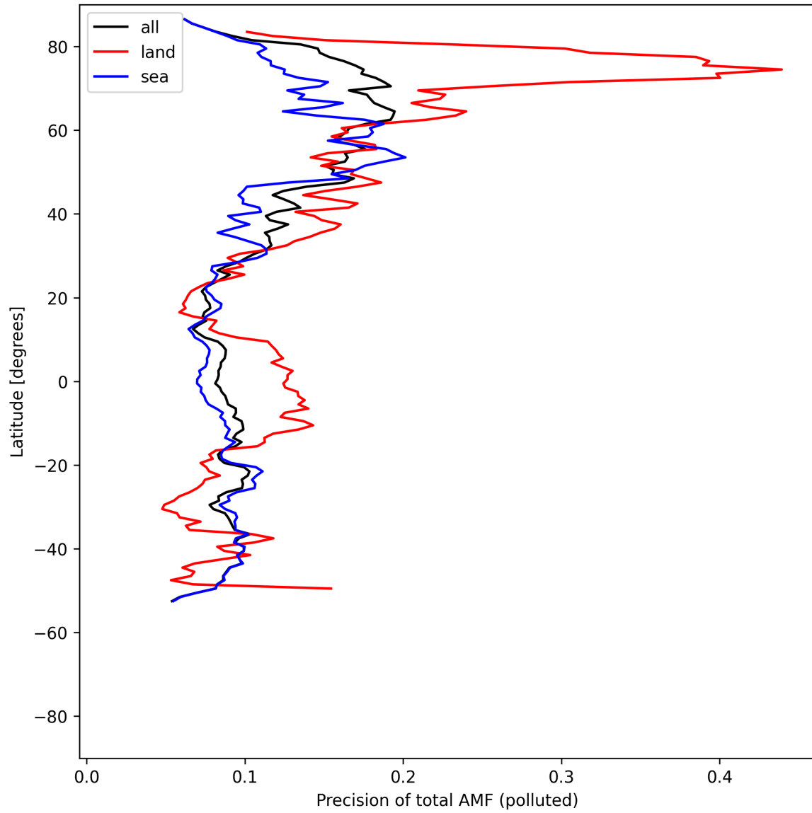
Figure 54: Zonal average of “Precision of total AMF (polluted)” for 2025-05-06 to 2025-05-07.
