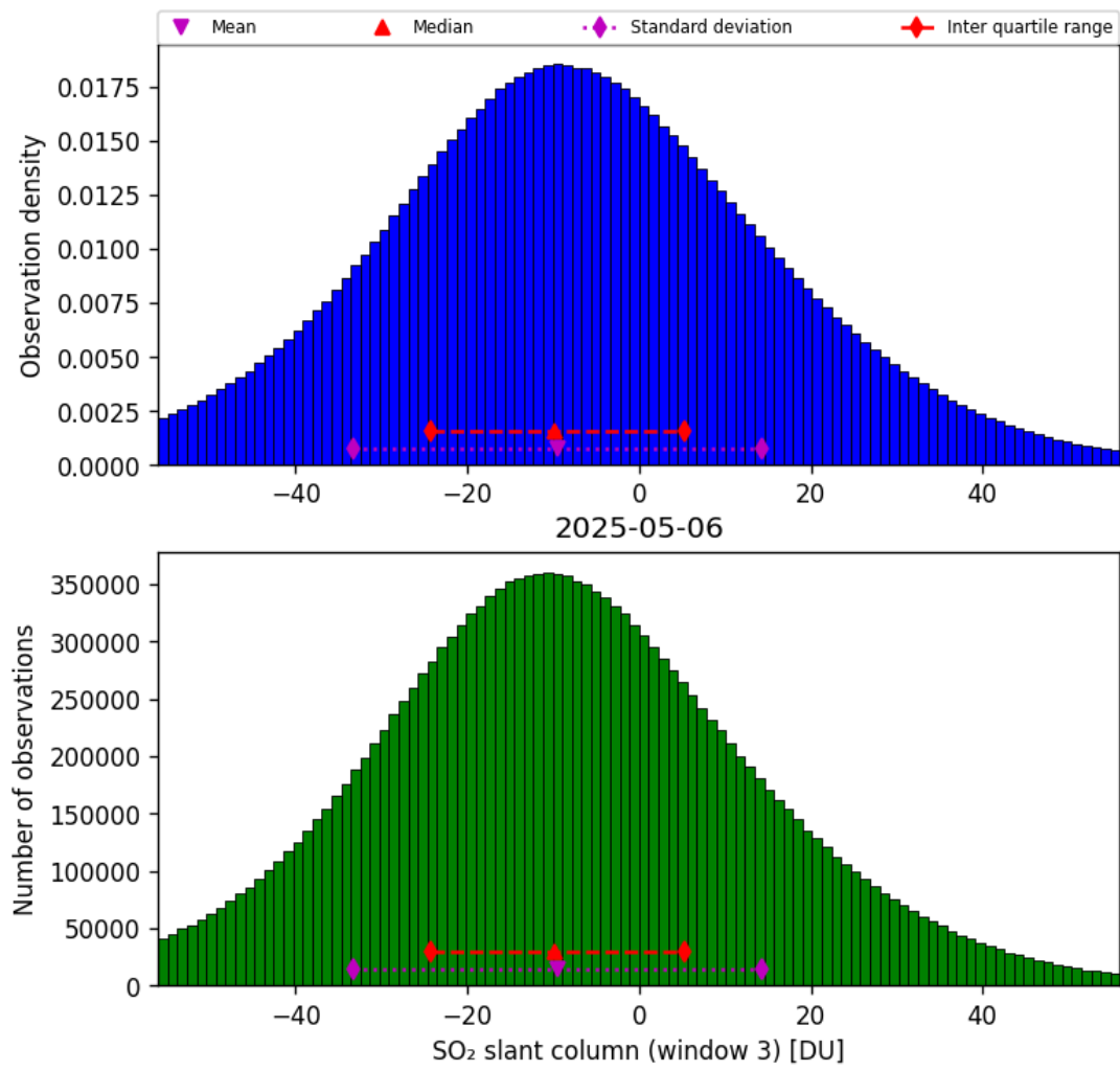
Figure 71: Histogram of “SO 2 slant column (window 3)” for 2025-05-06 to 2025-05-07
