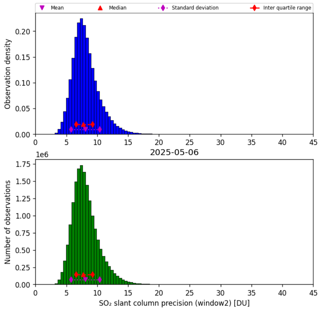
Figure 68: Histogram of “SO 2 slant column precision (window2)” for 2025-05-06 to 2025-05-07
