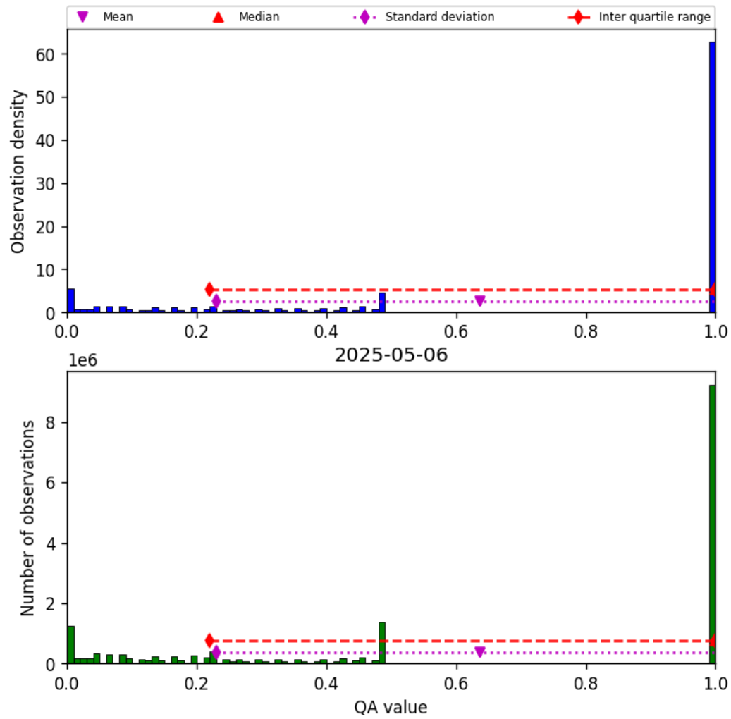
Figure 57: Histogram of “QA value” for 2025-05-06 to 2025-05-07
