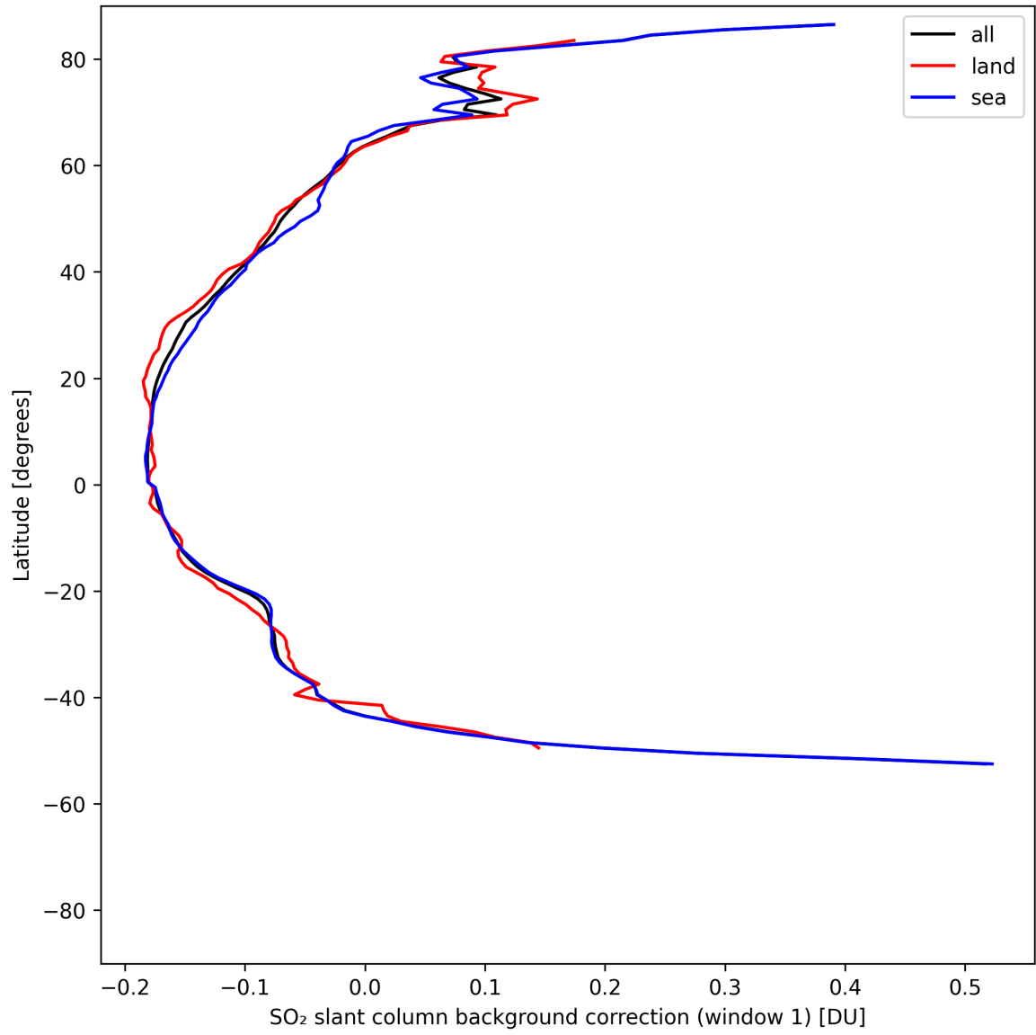
Figure 39: Zonal average of “SO 2 slant column background correction (window 1)” for 2025-05-06 to 2025-05-07.
