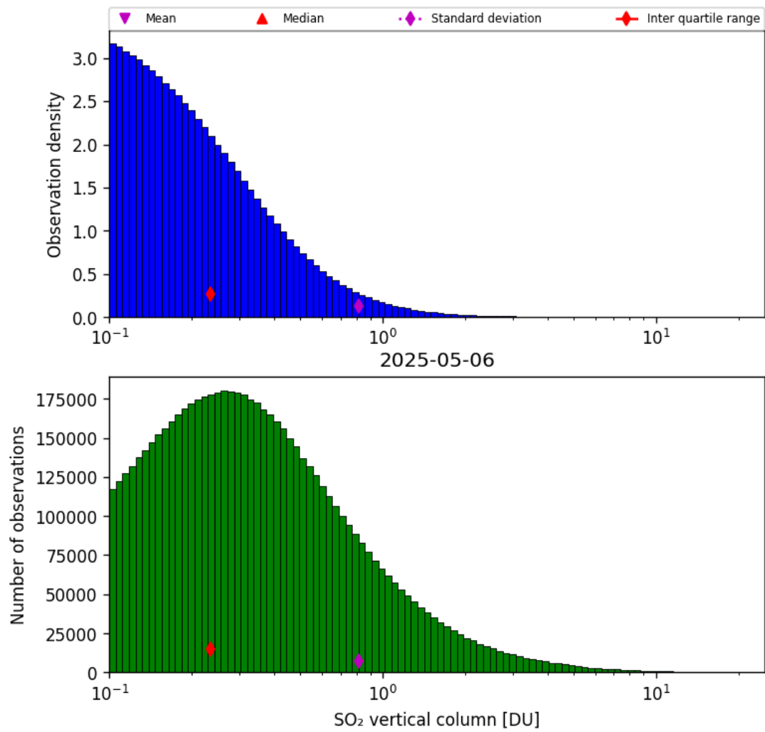
Figure 58: Histogram of “SO 2 vertical column” for 2025-05-06 to 2025-05-07
