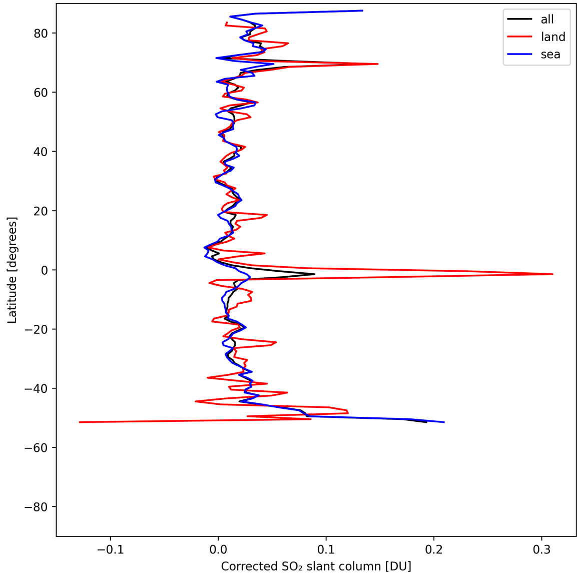
Figure 33: Zonal average of “Corrected SO 2 slant column” for 2025-05-08 to 2025-05-08.
