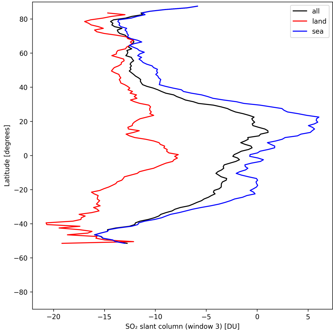
Figure 44: Zonal average of “SO 2 slant column (window 3)” for 2025-05-08 to 2025-05-08.
