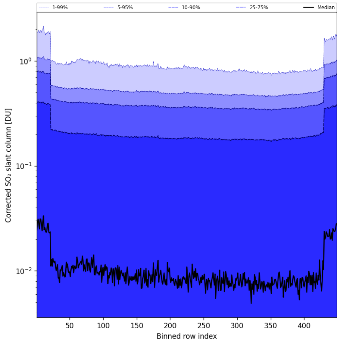
Figure 87: Along track statistics of “Corrected SO 2 slant column” for 2025-05-08 to 2025-05-08
