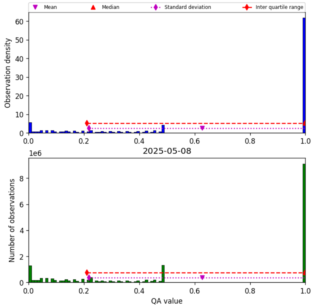
Figure 57: Histogram of “QA value” for 2025-05-08 to 2025-05-08
