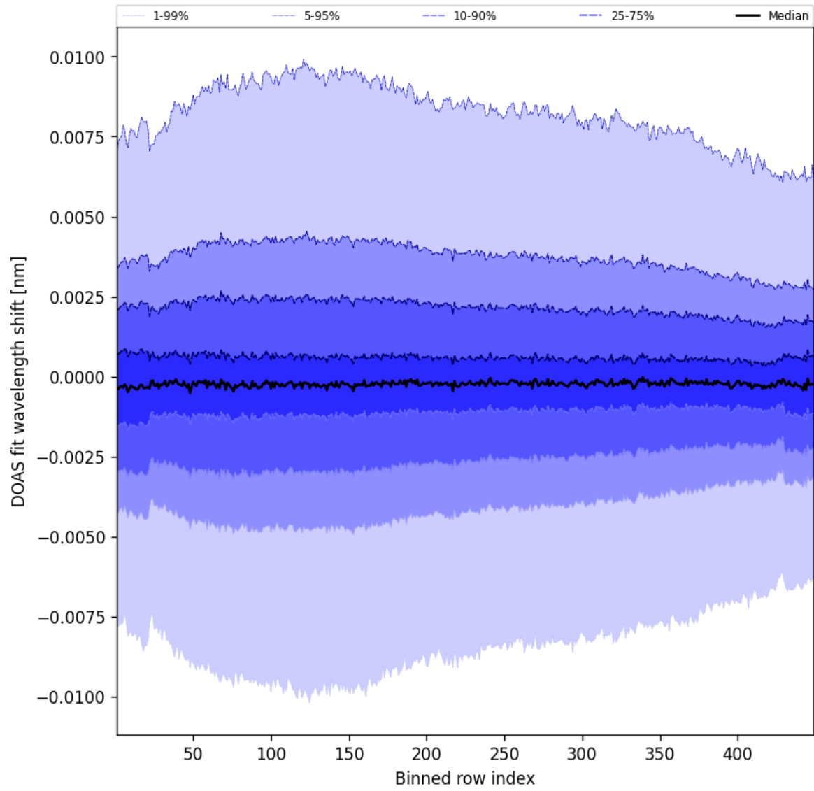
Figure 104: Along track statistics of “DOAS fit wavelength shift” for 2025-05-08 to 2025-05-08
