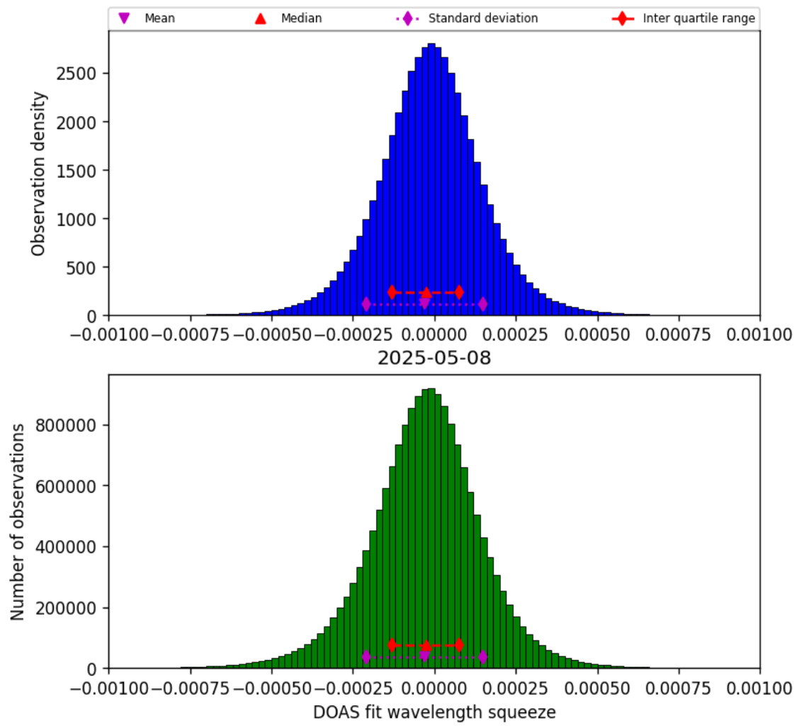
Figure 78: Histogram of “DOAS fit wavelength squeeze” for 2025-05-08 to 2025-05-08
