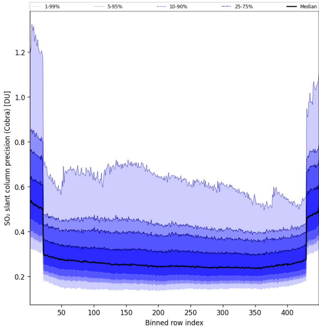
Figure 89: Along track statistics of “SO 2 slant column precision (Cobra)” for 2025-05-08 to 2025-05-08
