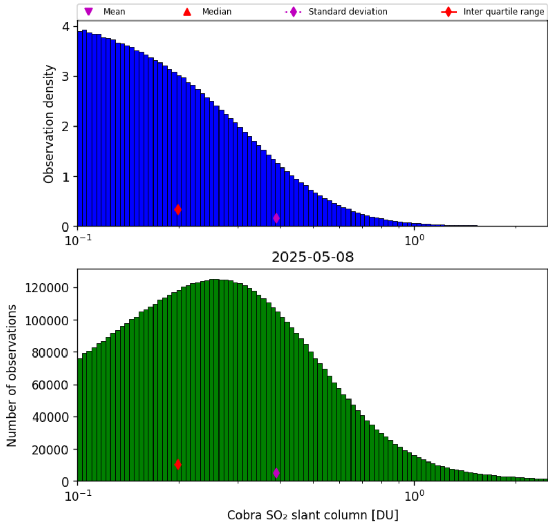
Figure 61: Histogram of “Cobra SO 2 slant column” for 2025-05-08 to 2025-05-08
