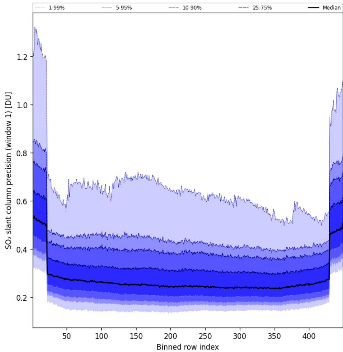
Figure 91: Along track statistics of “SO 2 slant column precision (window 1)” for 2025-05-08 to 2025-05-08
