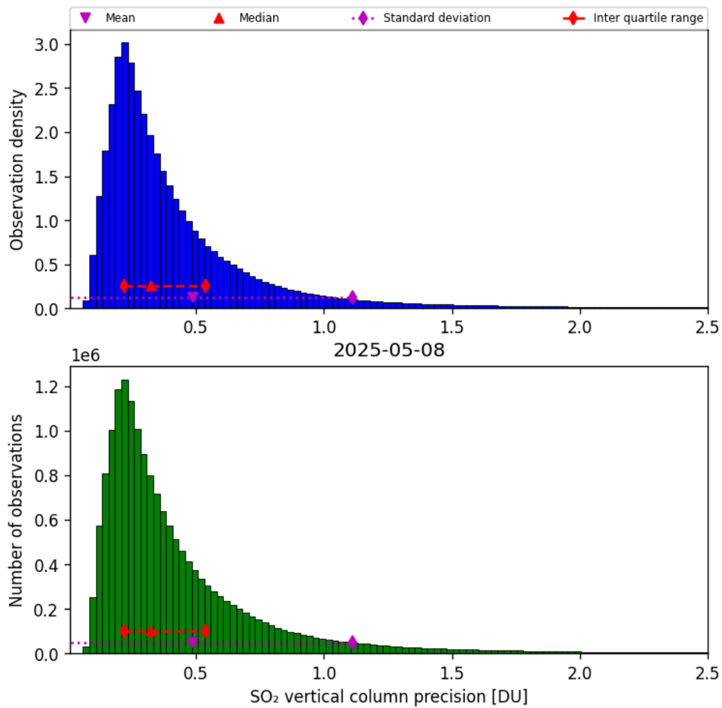
Figure 59: Histogram of “SO 2 vertical column precision” for 2025-05-08 to 2025-05-08
