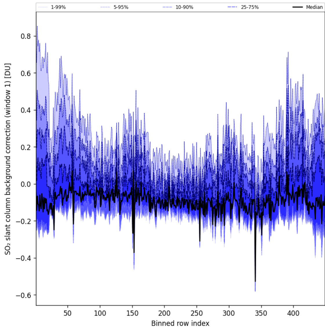
Figure 93: Along track statistics of “SO 2 slant column background correction (window 1)” for 2025-05-08 to 2025-05-08
