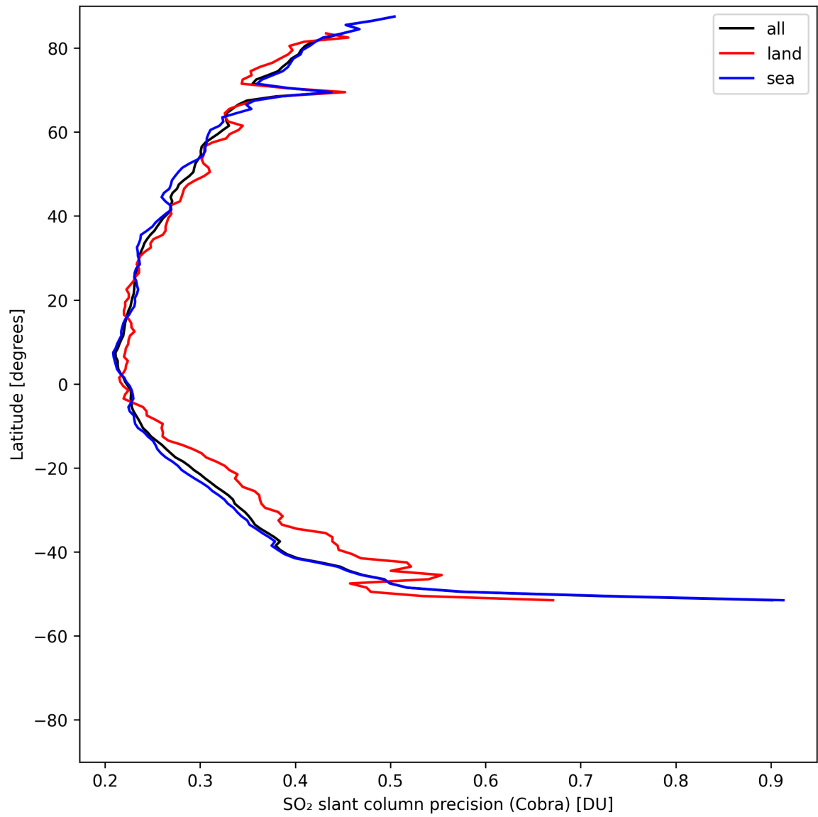
Figure 35: Zonal average of “SO 2 slant column precision (Cobra)” for 2025-05-08 to 2025-05-08.
