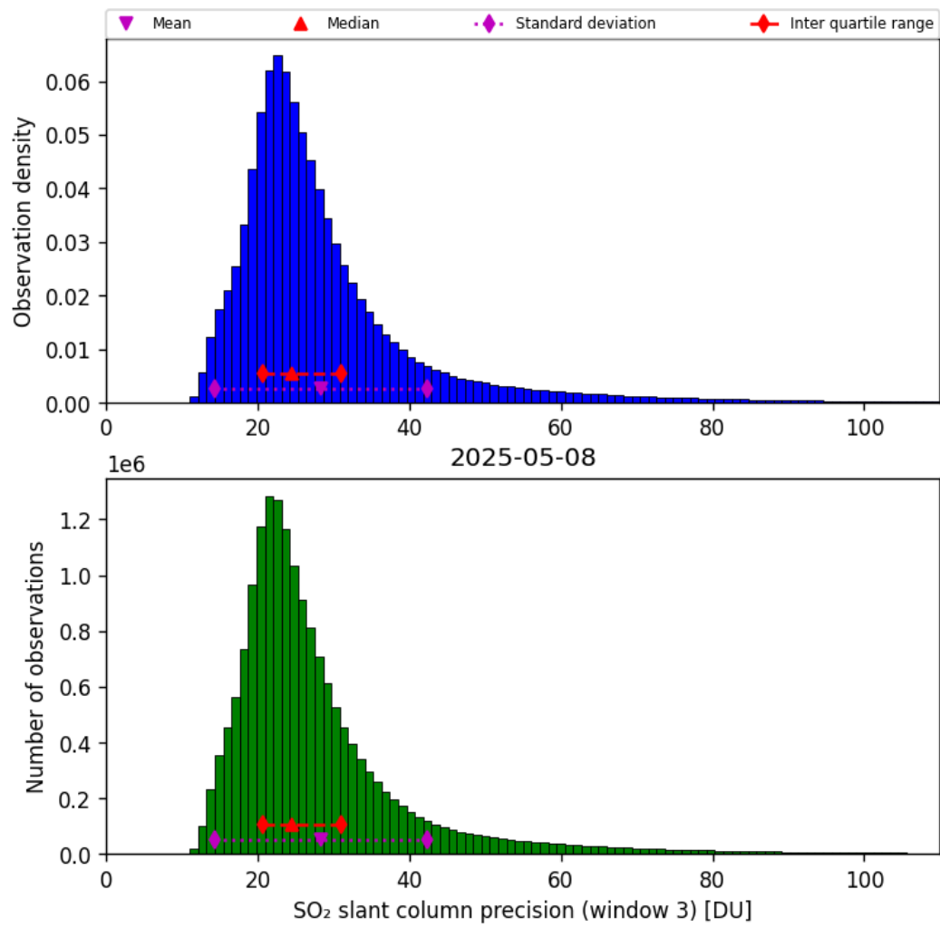
Figure 72: Histogram of “SO 2 slant column precision (window 3)” for 2025-05-08 to 2025-05-08
