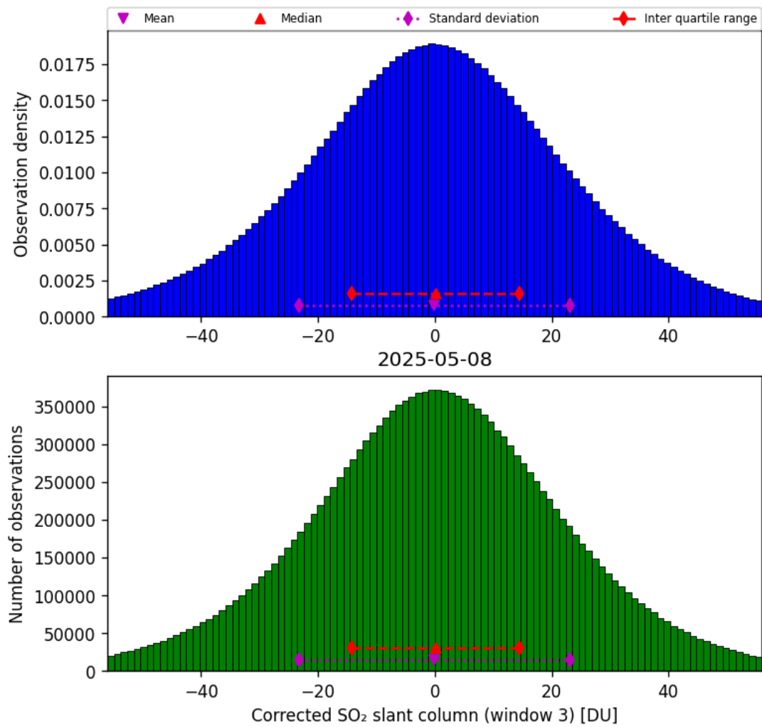
Figure 73: Histogram of “Corrected SO 2 slant column (window 3)” for 2025-05-08 to 2025-05-08
