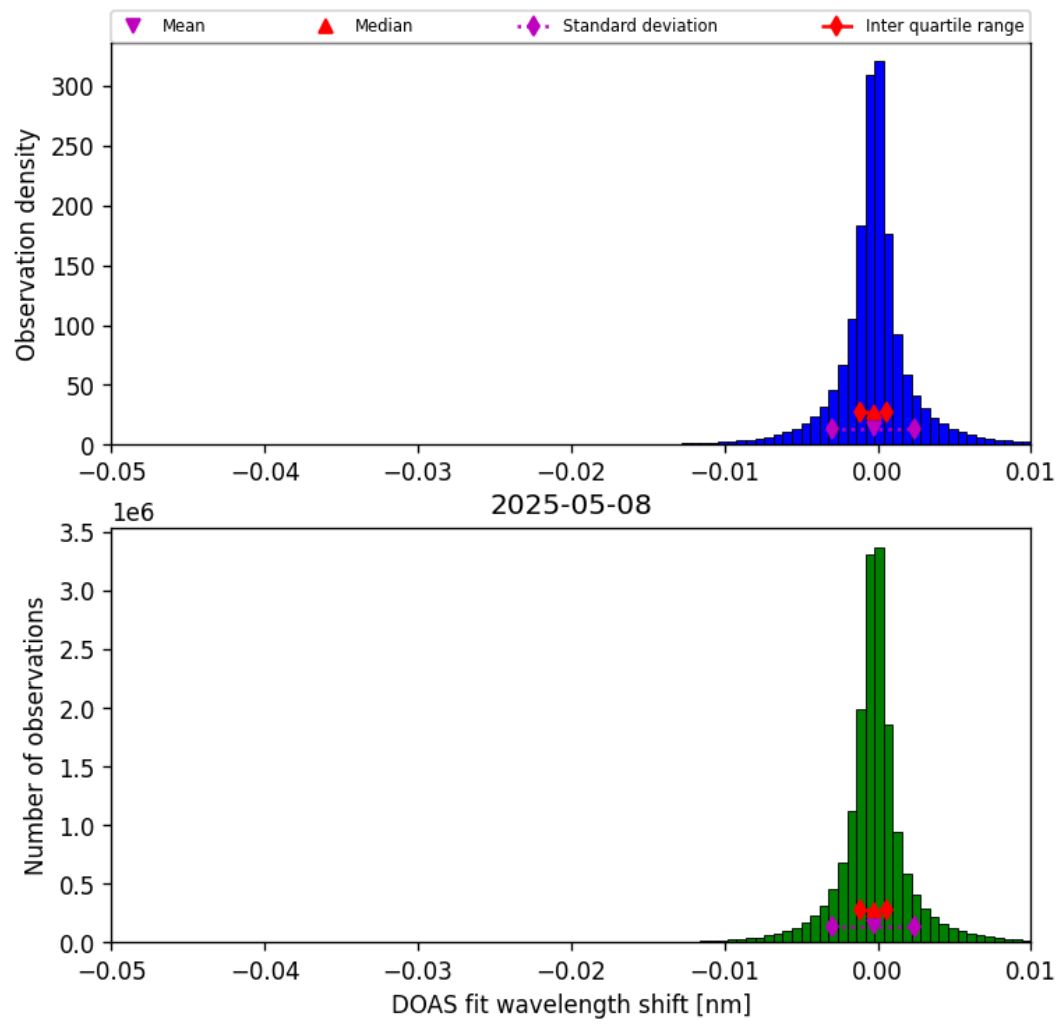
Figure 77: Histogram of “DOAS fit wavelength shift” for 2025-05-08 to 2025-05-08
