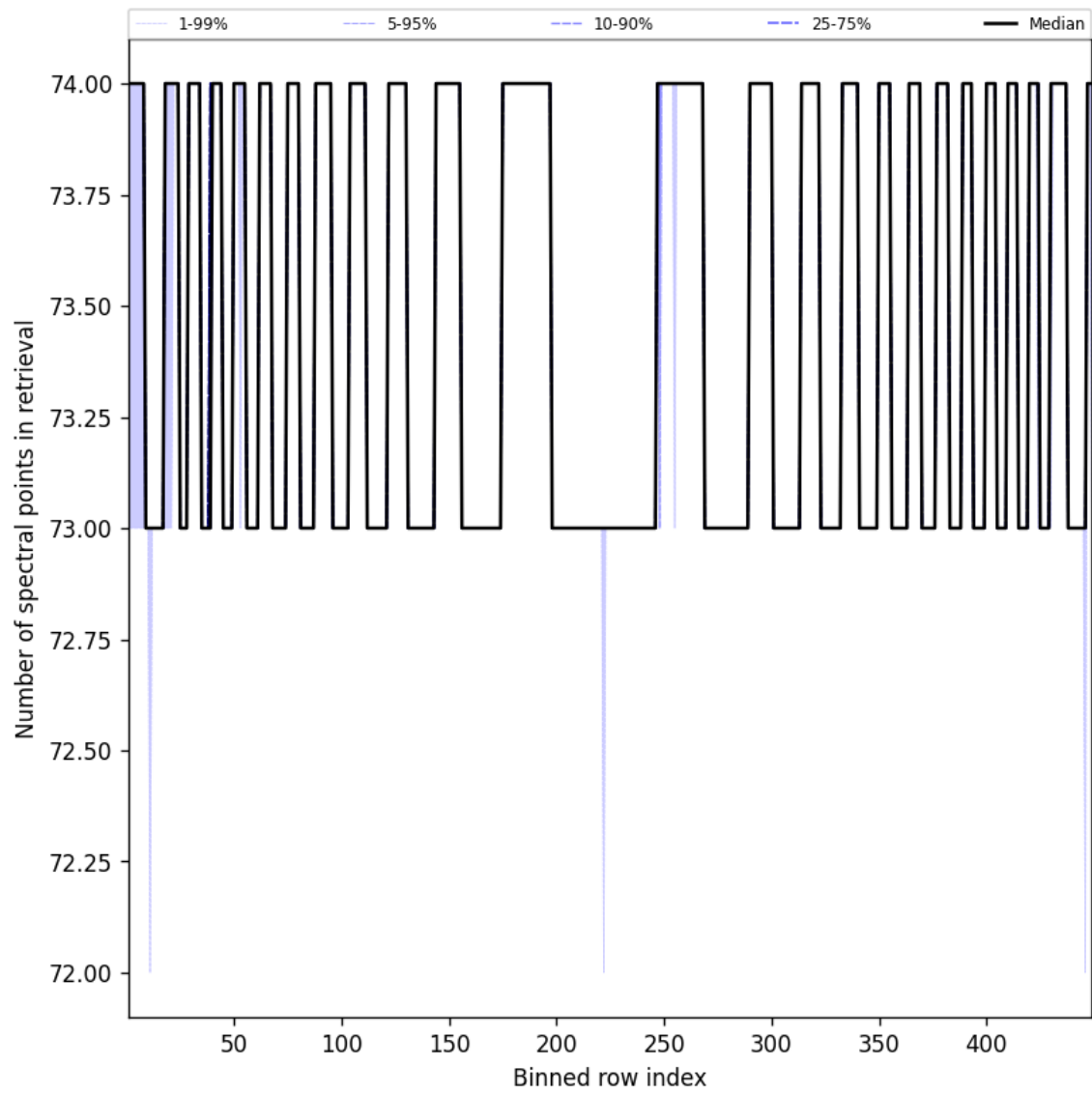
Figure 110: Along track statistics of “Number of spectral points in retrieval” for 2025-05-08 to 2025-05-08
