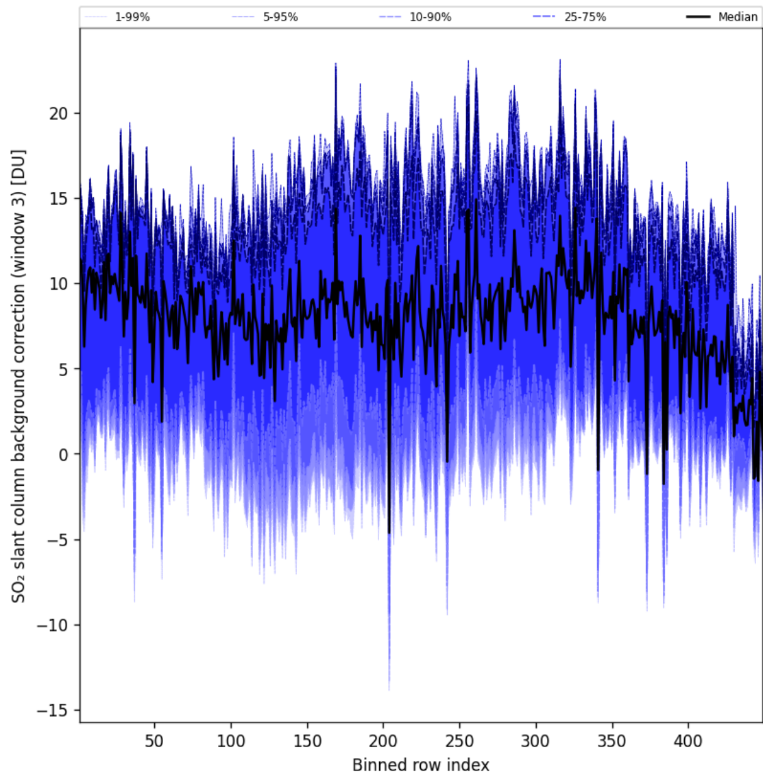
Figure 101: Along track statistics of “SO 2 slant column background correction (window 3)” for 2025-05-08 to 2025-05-08
