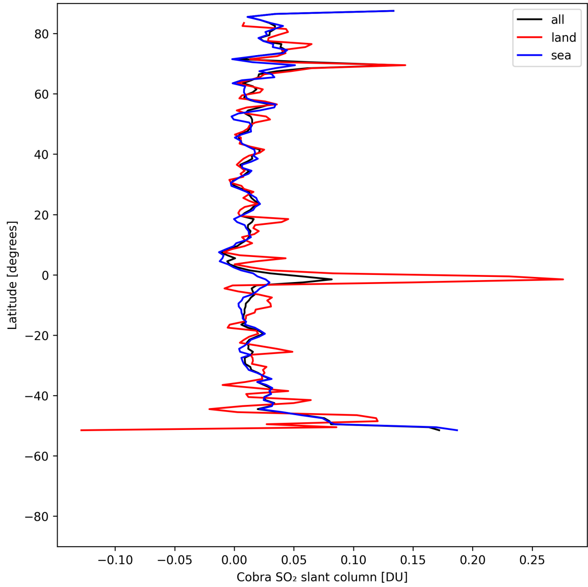
Figure 34: Zonal average of “Cobra SO 2 slant column” for 2025-05-08 to 2025-05-08.
