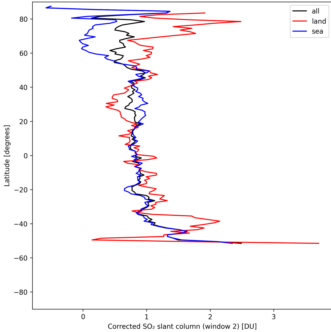
Figure 42: Zonal average of “Corrected SO 2 slant column (window 2)” for 2025-05-08 to 2025-05-08.
