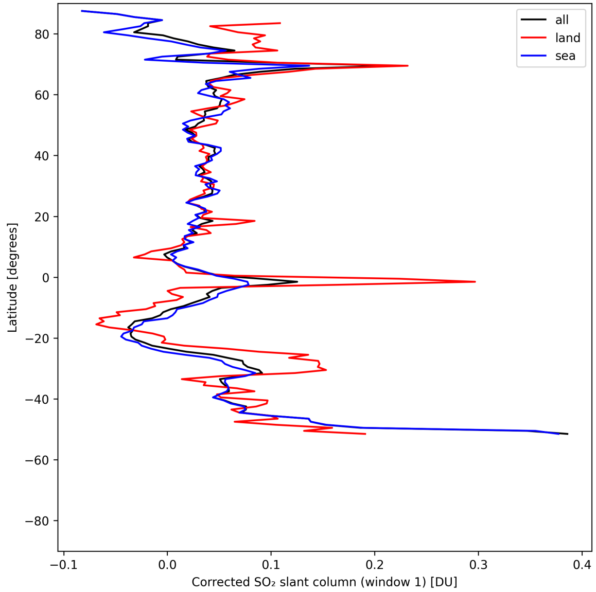
Figure 38: Zonal average of “Corrected SO 2 slant column (window 1)” for 2025-05-08 to 2025-05-08.
