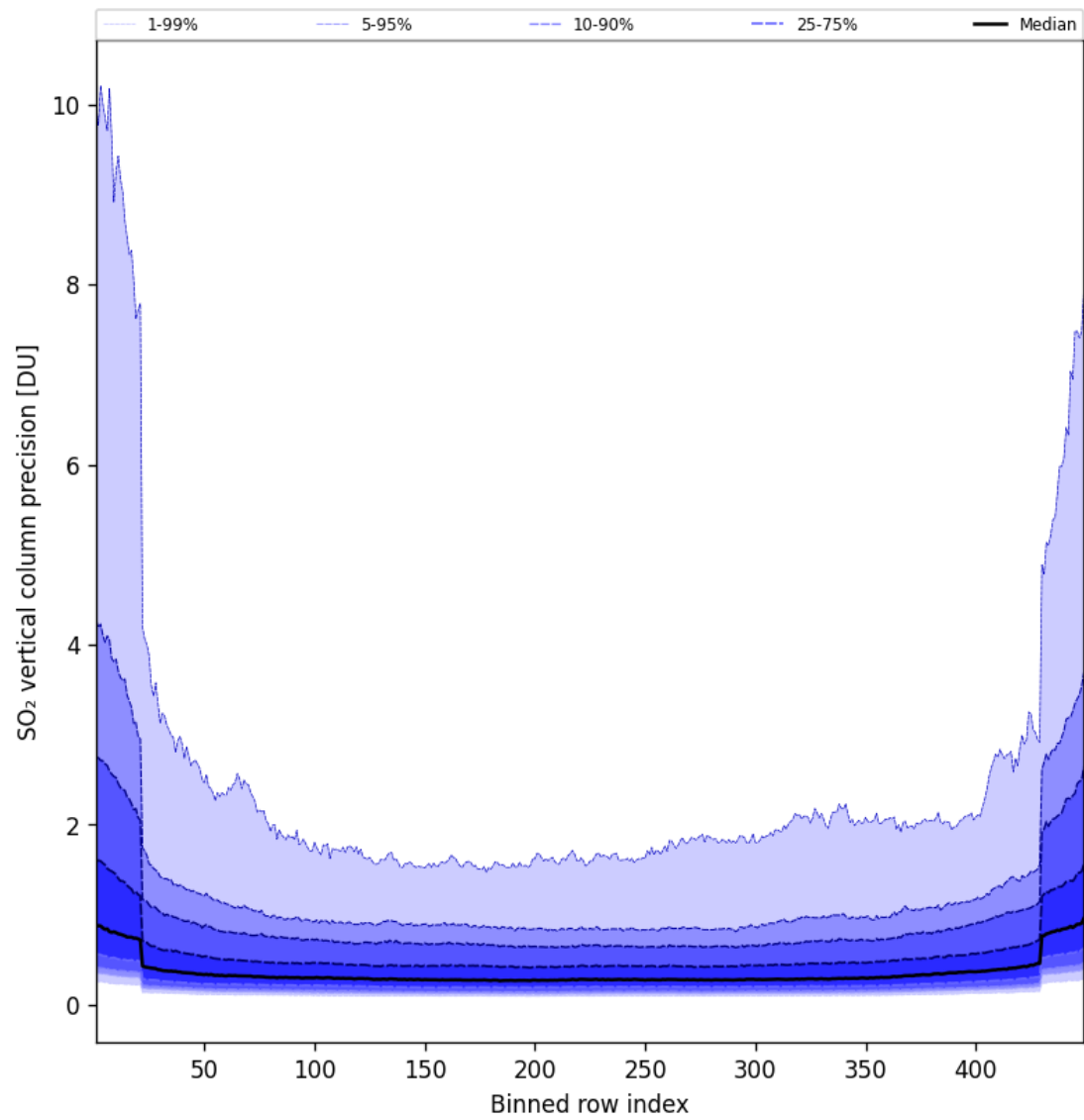
Figure 86: Along track statistics of “SO 2 vertical column precision” for 2025-05-08 to 2025-05-08
