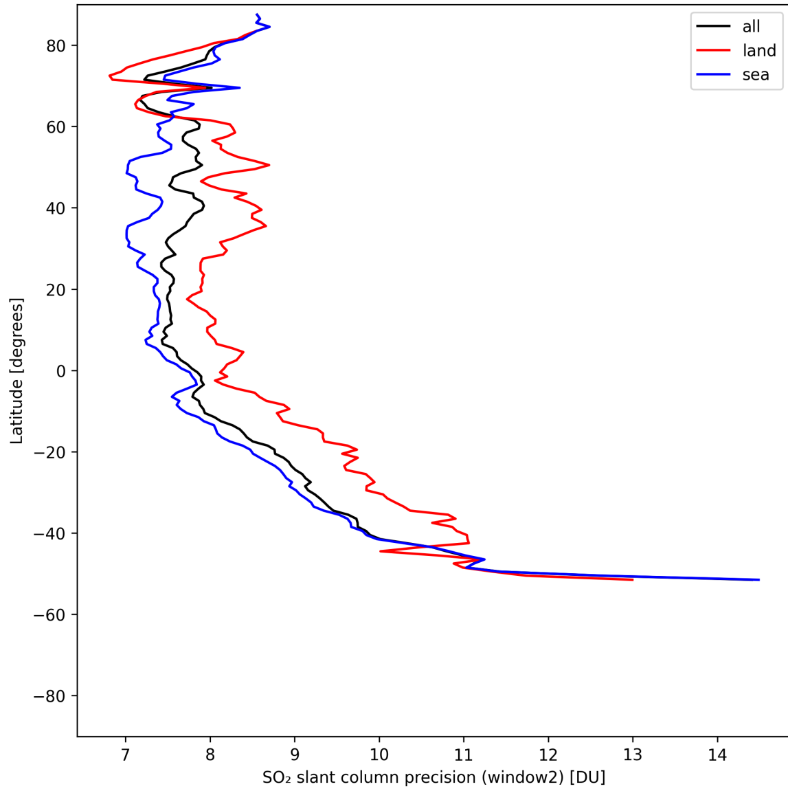
Figure 41: Zonal average of “SO 2 slant column precision (window2)” for 2025-05-08 to 2025-05-08.
