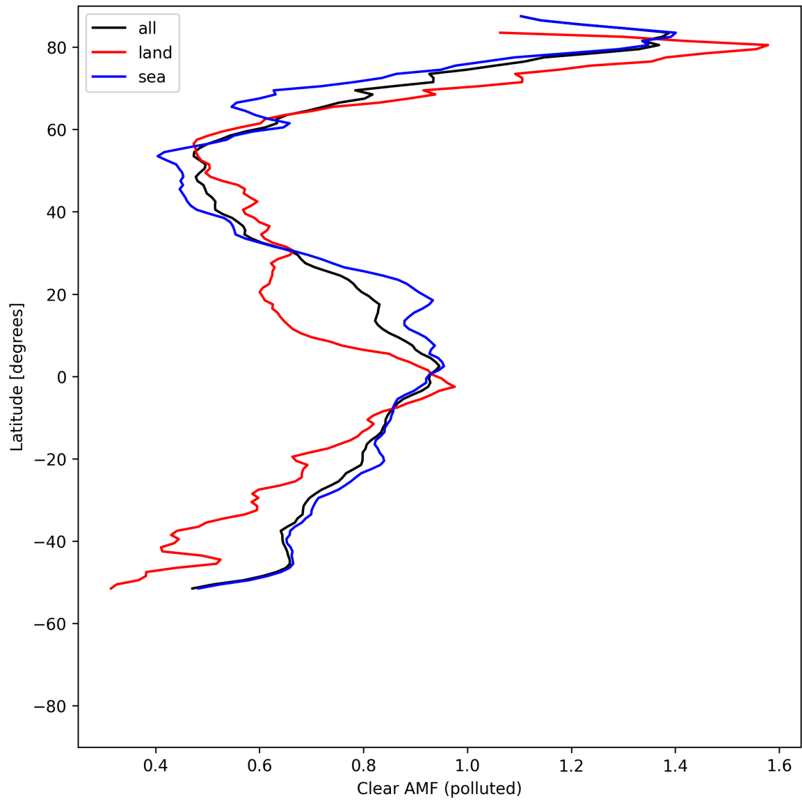
Figure 55: Zonal average of “Clear AMF (polluted)” for 2025-05-08 to 2025-05-08.
