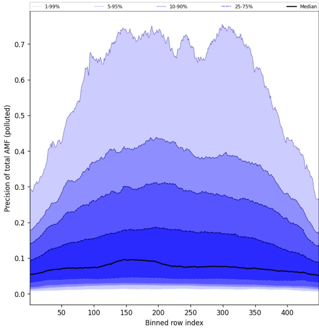
Figure 108: Along track statistics of “Precision of total AMF (polluted)” for 2025-05-08 to 2025-05-08
