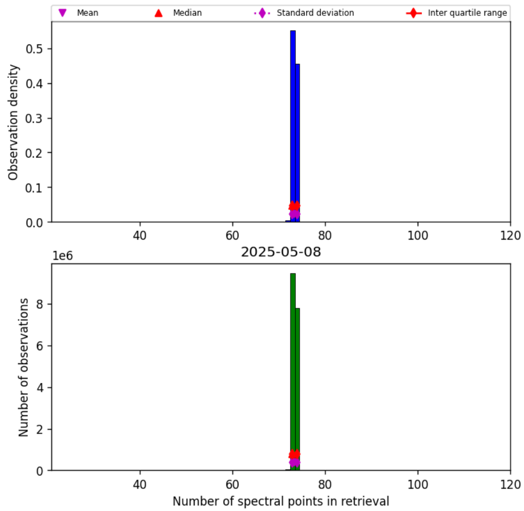
Figure 83: Histogram of “Number of spectral points in retrieval” for 2025-05-08 to 2025-05-08
