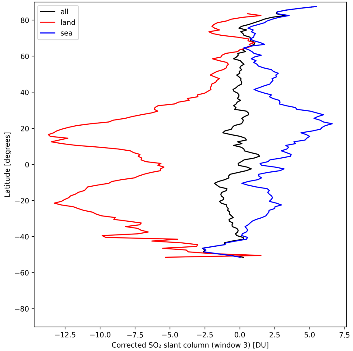
Figure 46: Zonal average of “Corrected SO 2 slant column (window 3)” for 2025-05-08 to 2025-05-08.
