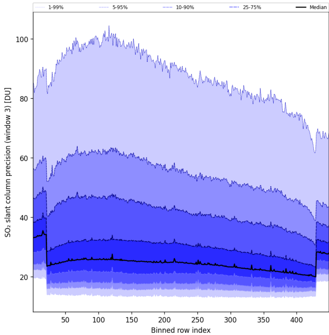
Figure 99: Along track statistics of “SO 2 slant column precision (window 3)” for 2025-05-08 to 2025-05-08
