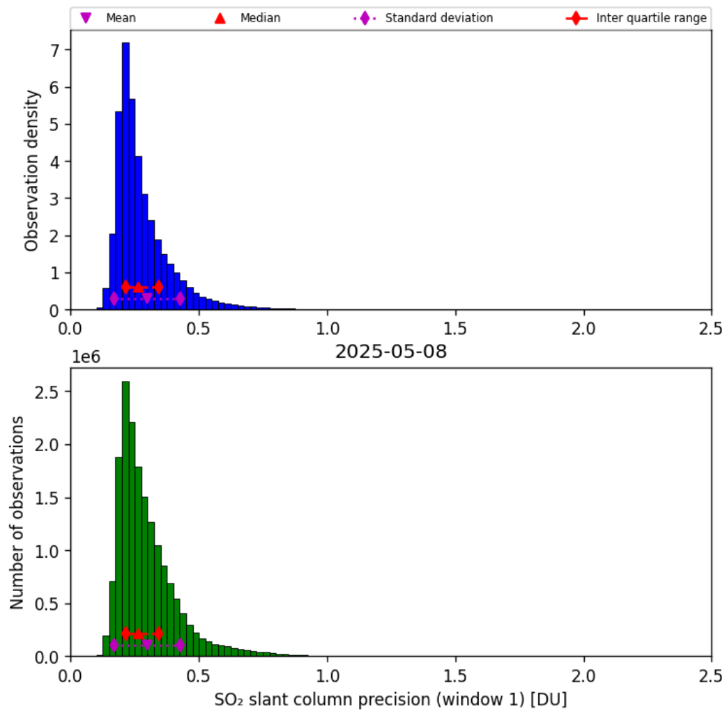
Figure 64: Histogram of “SO 2 slant column precision (window 1)” for 2025-05-08 to 2025-05-08
