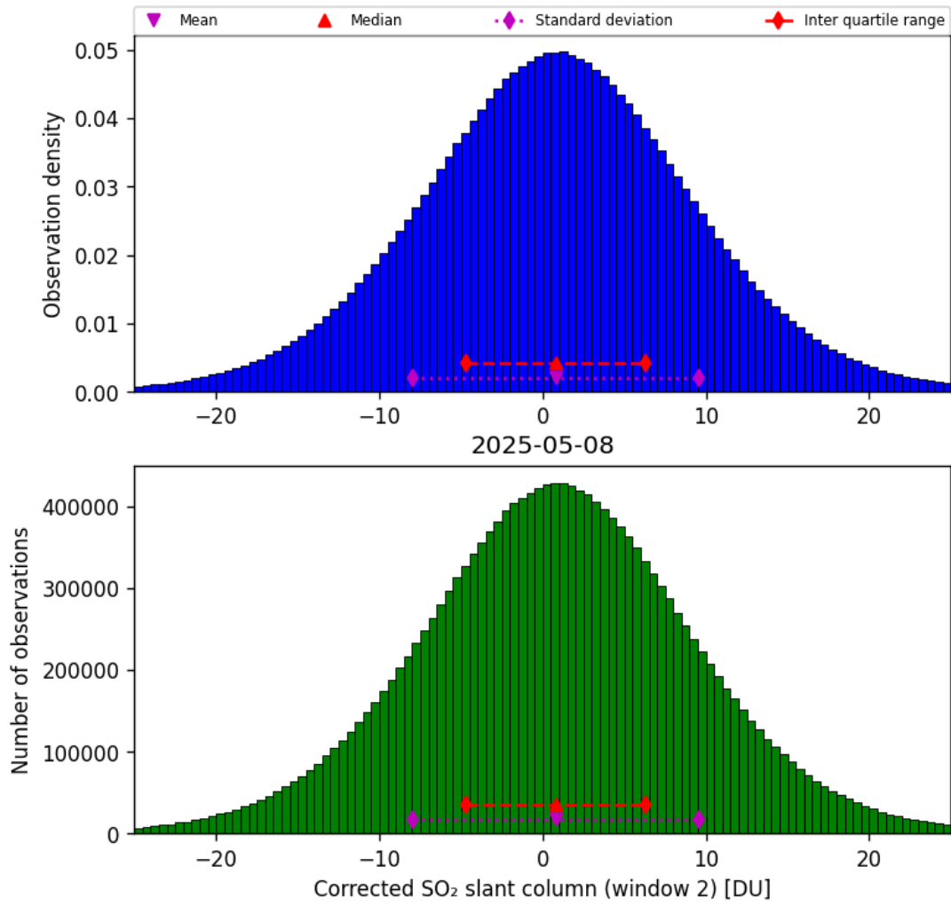
Figure 69: Histogram of “Corrected SO 2 slant column (window 2)” for 2025-05-08 to 2025-05-08
