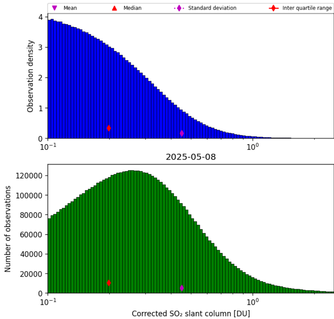
Figure 60: Histogram of “Corrected SO 2 slant column” for 2025-05-08 to 2025-05-08
