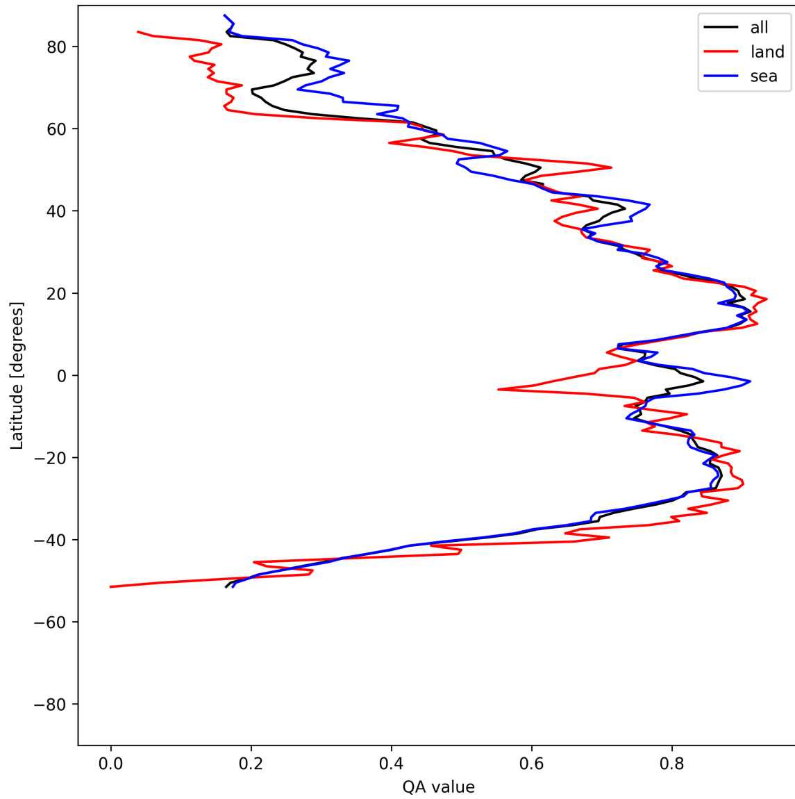
Figure 30: Zonal average of “QA value” for 2025-05-08 to 2025-05-08.
