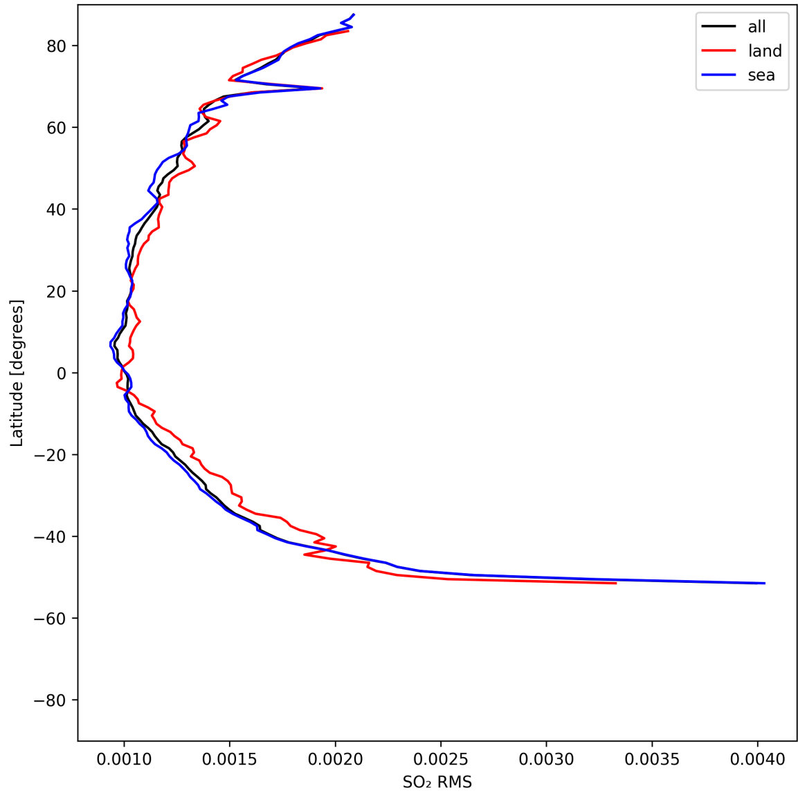
Figure 52: Zonal average of “SO 2 RMS” for 2025-05-08 to 2025-05-08.
