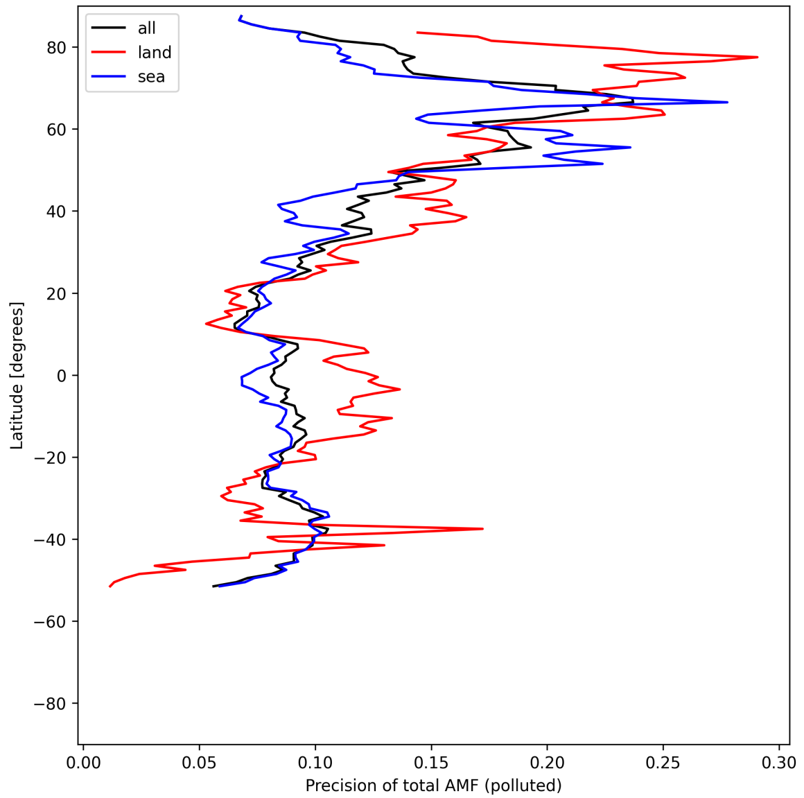
Figure 54: Zonal average of “Precision of total AMF (polluted)” for 2025-05-08 to 2025-05-08.
