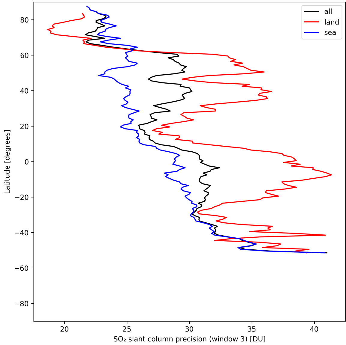
Figure 45: Zonal average of “SO 2 slant column precision (window 3)” for 2025-05-08 to 2025-05-08.
