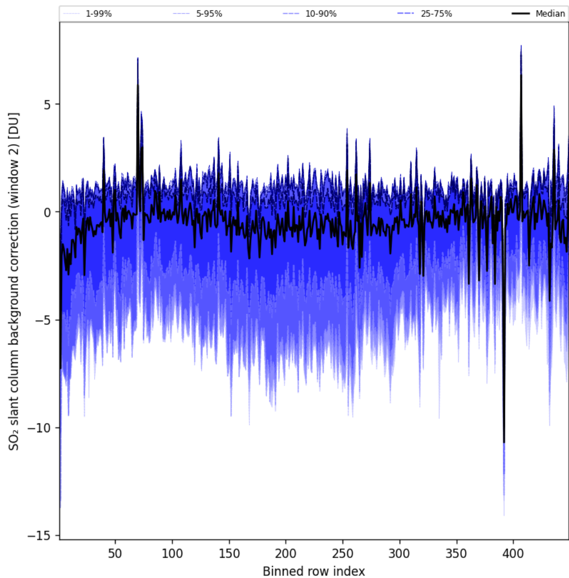
Figure 97: Along track statistics of “SO 2 slant column background correction (window 2)” for 2025-05-08 to 2025-05-08
