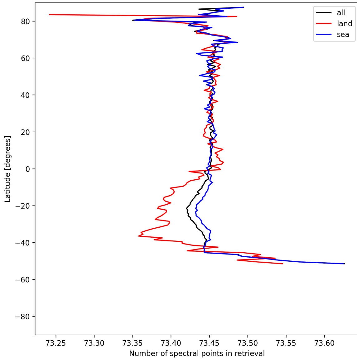
Figure 56: Zonal average of “Number of spectral points in retrieval” for 2025-05-08 to 2025-05-08.
