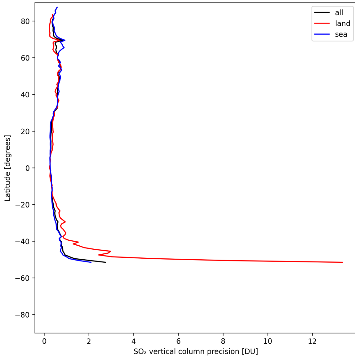
Figure 32: Zonal average of “SO 2 vertical column precision” for 2025-05-08 to 2025-05-08.
