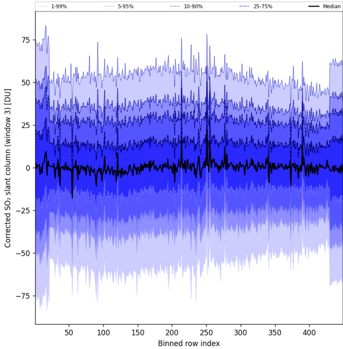
Figure 100: Along track statistics of “Corrected SO 2 slant column (window 3)” for 2025-05-08 to 2025-05-08
