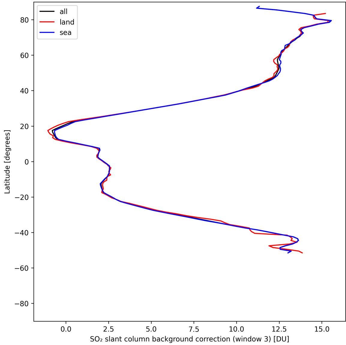
Figure 47: Zonal average of “SO 2 slant column background correction (window 3)” for 2025-05-08 to 2025-05-08.
