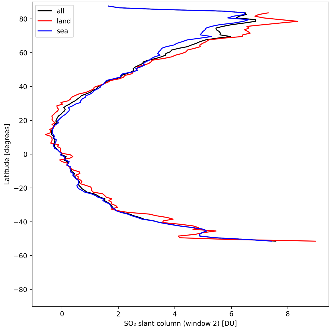
Figure 40: Zonal average of “SO 2 slant column (window 2)” for 2025-05-08 to 2025-05-08.
