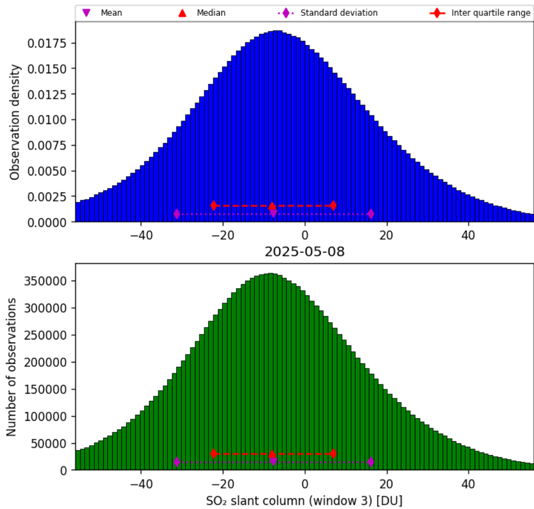
Figure 71: Histogram of “SO 2 slant column (window 3)” for 2025-05-08 to 2025-05-08
