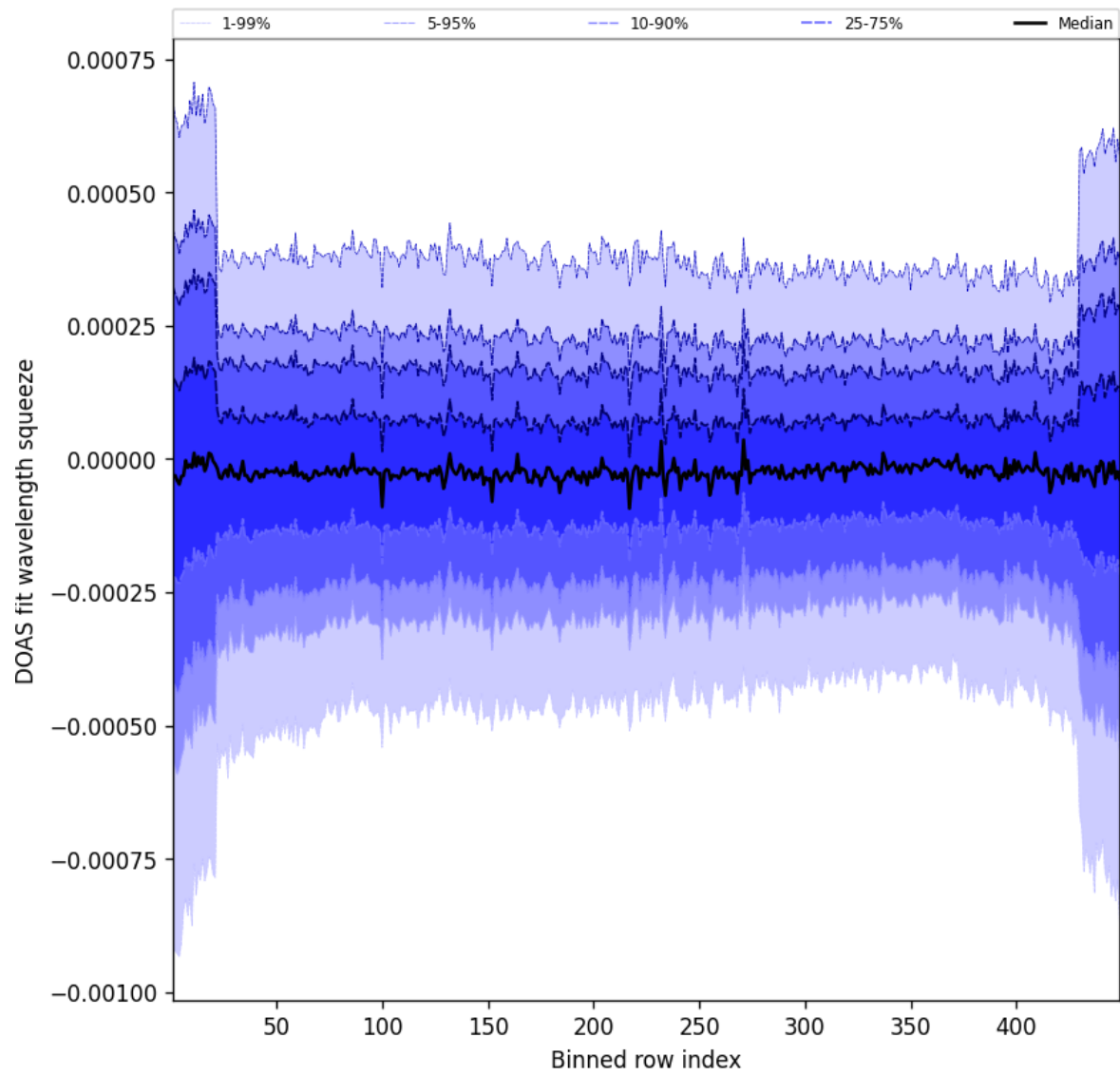
Figure 105: Along track statistics of “DOAS fit wavelength squeeze” for 2025-05-08 to 2025-05-08
