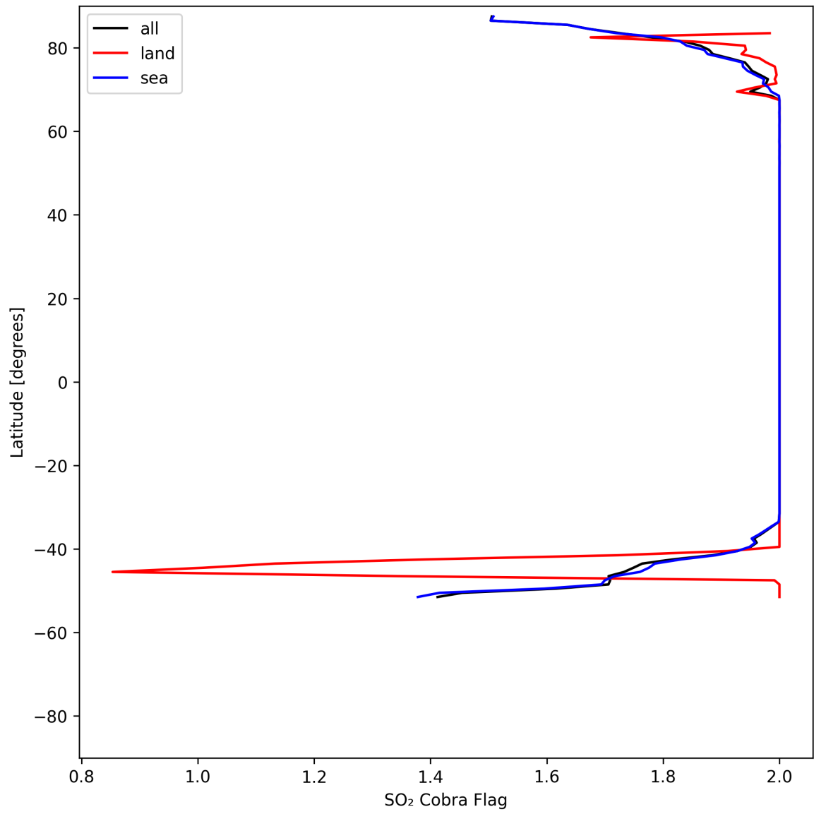
Figure 48: Zonal average of “SO 2 Cobra Flag” for 2025-05-08 to 2025-05-08.
