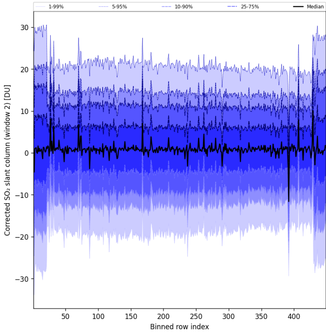
Figure 96: Along track statistics of “Corrected SO 2 slant column (window 2)” for 2025-05-08 to 2025-05-08
