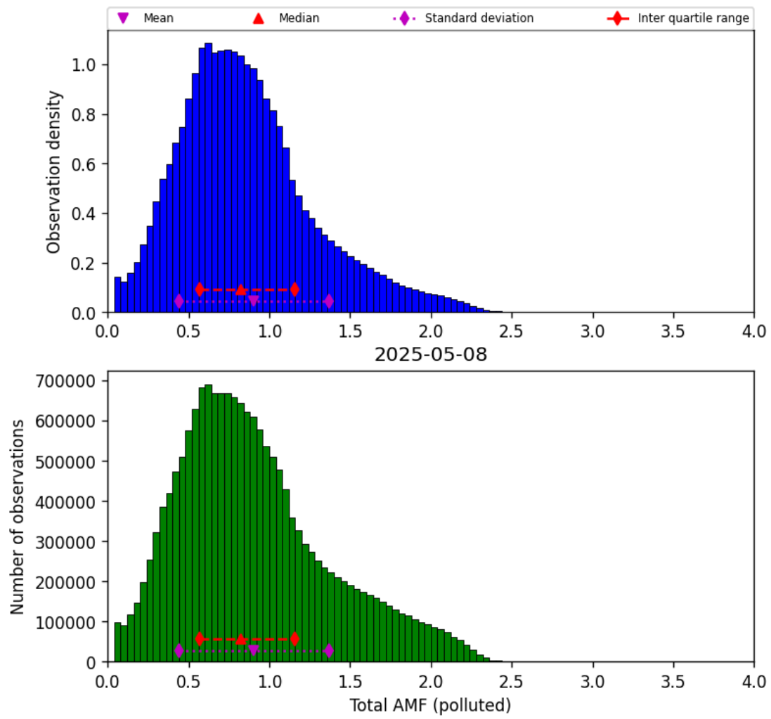
Figure 80: Histogram of “Total AMF (polluted)” for 2025-05-08 to 2025-05-08
