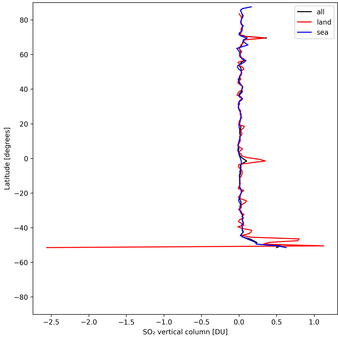
Figure 31: Zonal average of “SO 2 vertical column” for 2025-05-08 to 2025-05-08.
