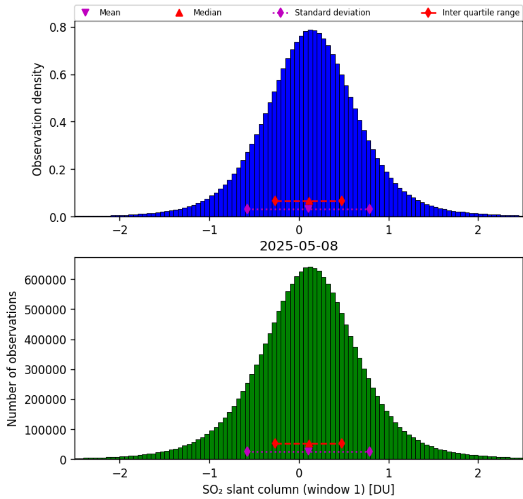
Figure 63: Histogram of “SO 2 slant column (window 1)” for 2025-05-08 to 2025-05-08
