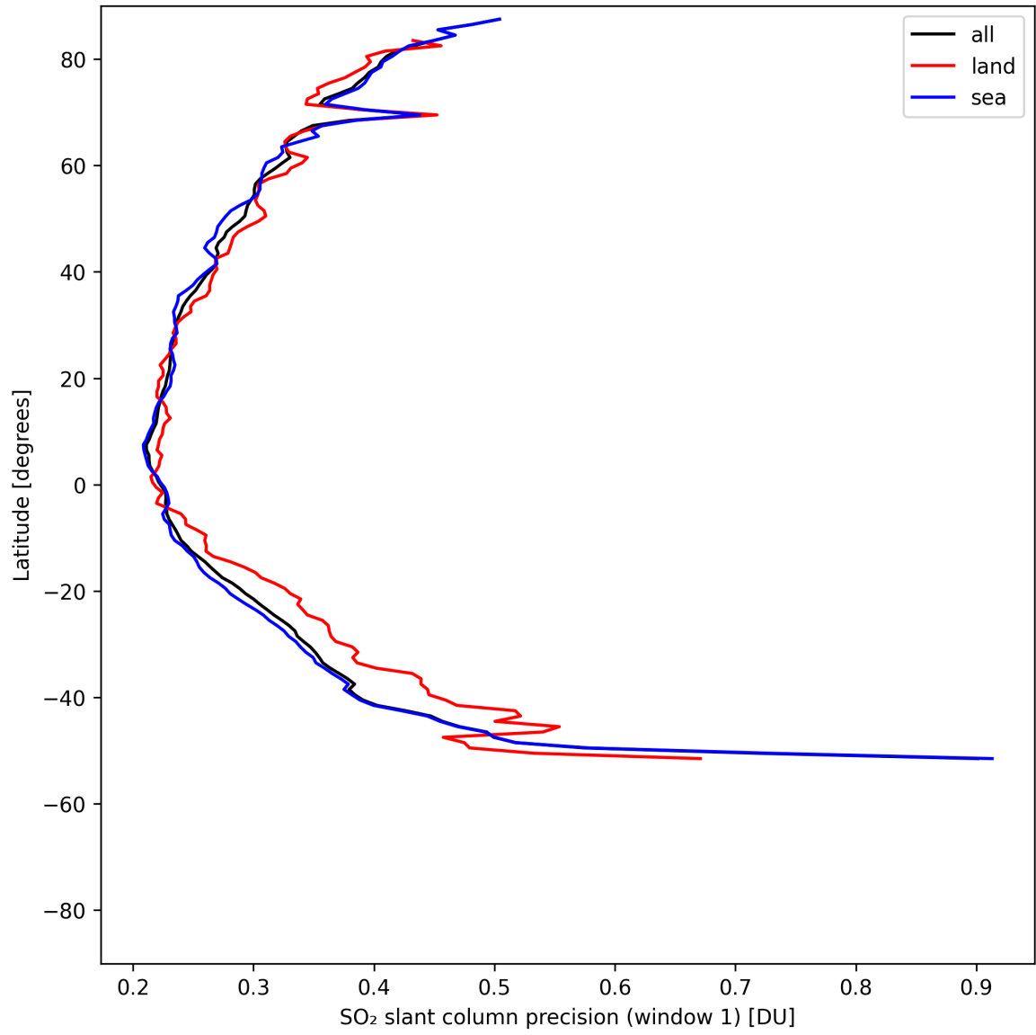
Figure 37: Zonal average of “SO 2 slant column precision (window 1)” for 2025-05-08 to 2025-05-08.
