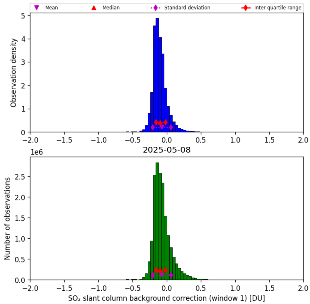
Figure 66: Histogram of “SO 2 slant column background correction (window 1)” for 2025-05-08 to 2025-05-08
