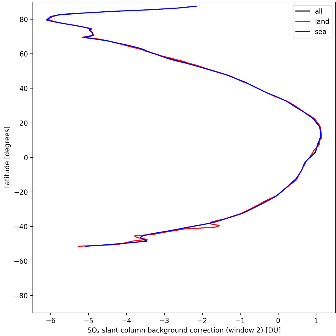
Figure 43: Zonal average of “SO 2 slant column background correction (window 2)” for 2025-05-08 to 2025-05-08.
