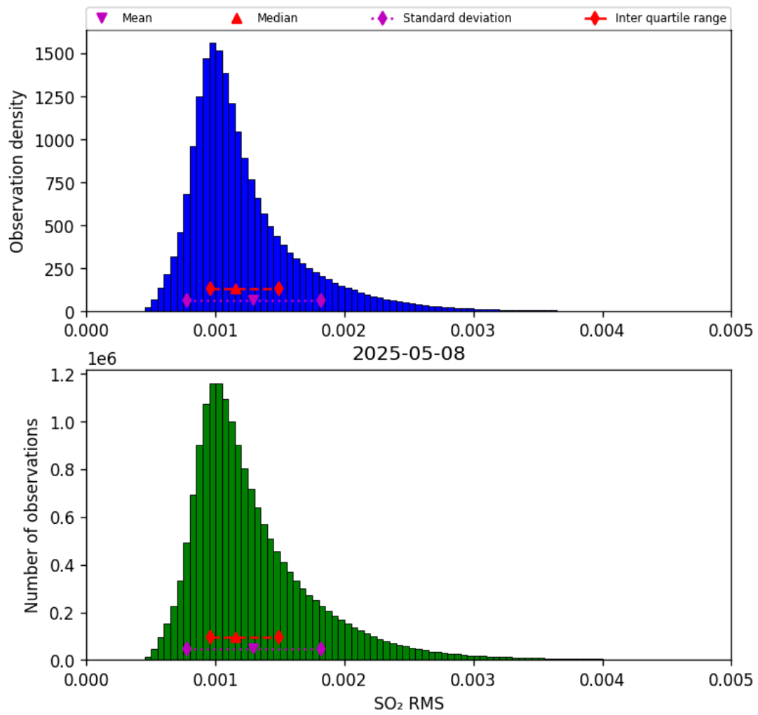
Figure 79: Histogram of “SO 2 RMS” for 2025-05-08 to 2025-05-08
