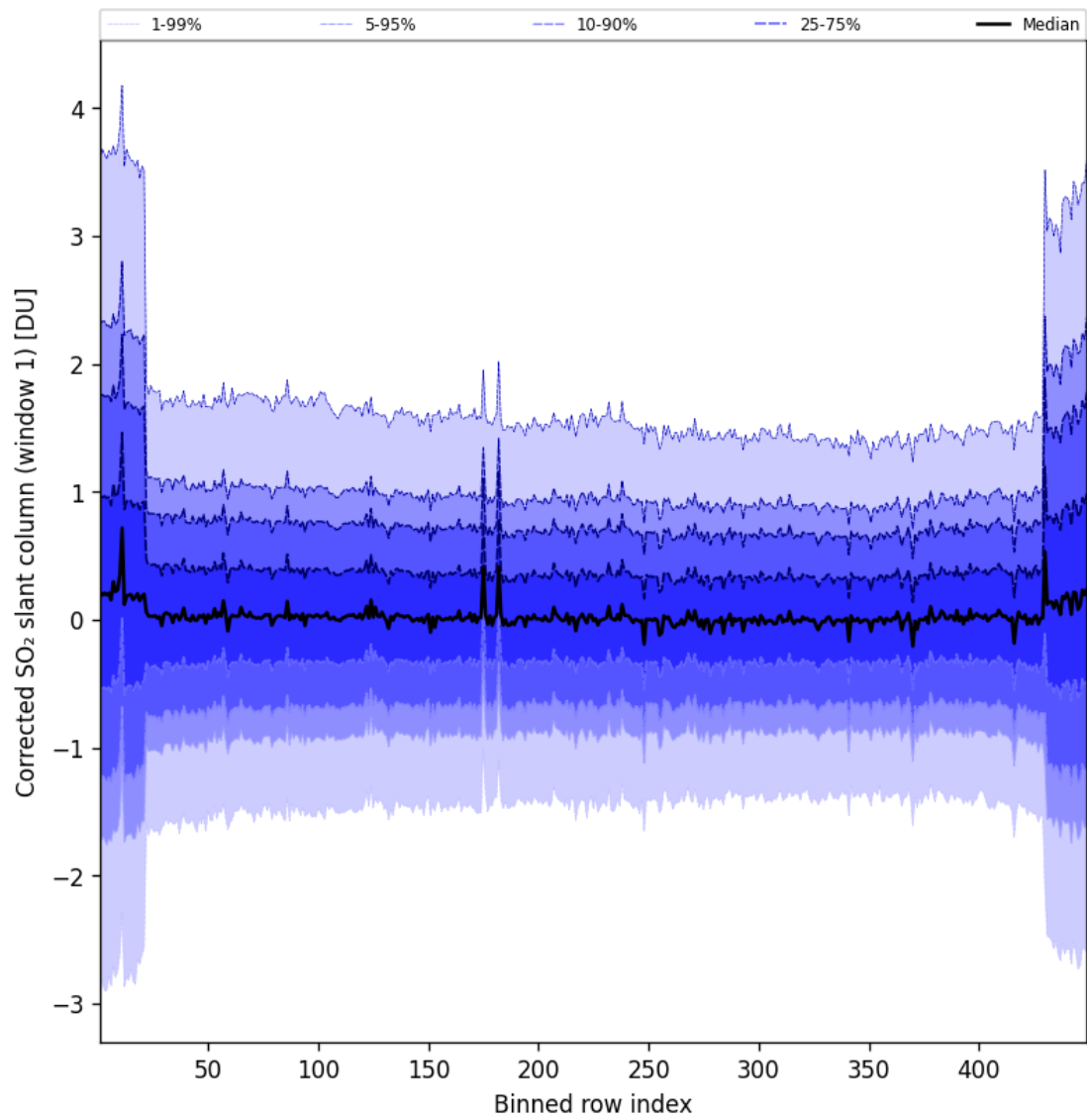
Figure 92: Along track statistics of “Corrected SO 2 slant column (window 1)” for 2025-05-08 to 2025-05-08
