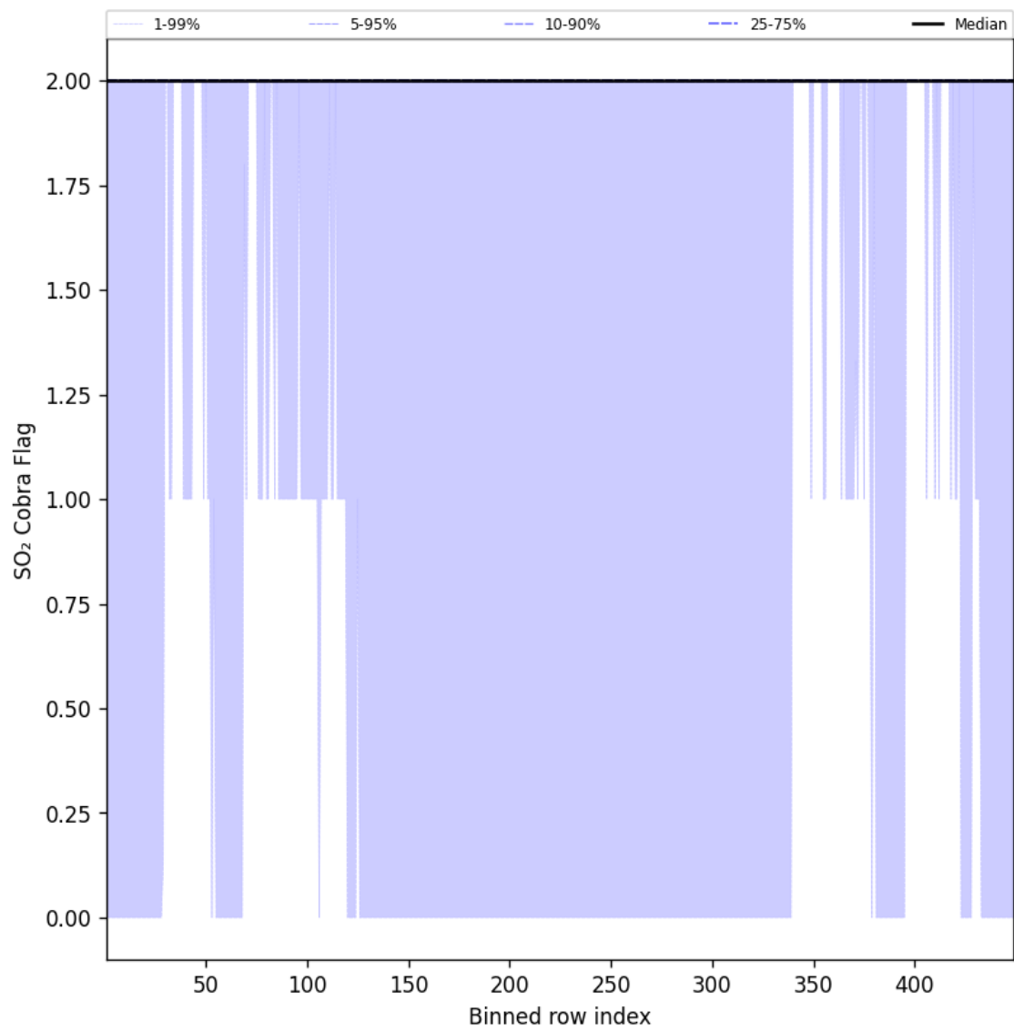
Figure 102: Along track statistics of "SO 2 Cobra Flag" for 2025-05-08 to 2025-05-08
