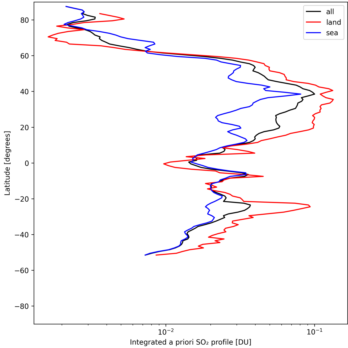
Figure 49: Zonal average of “Integrated a priori SO 2 profile” for 2025-05-08 to 2025-05-08.
