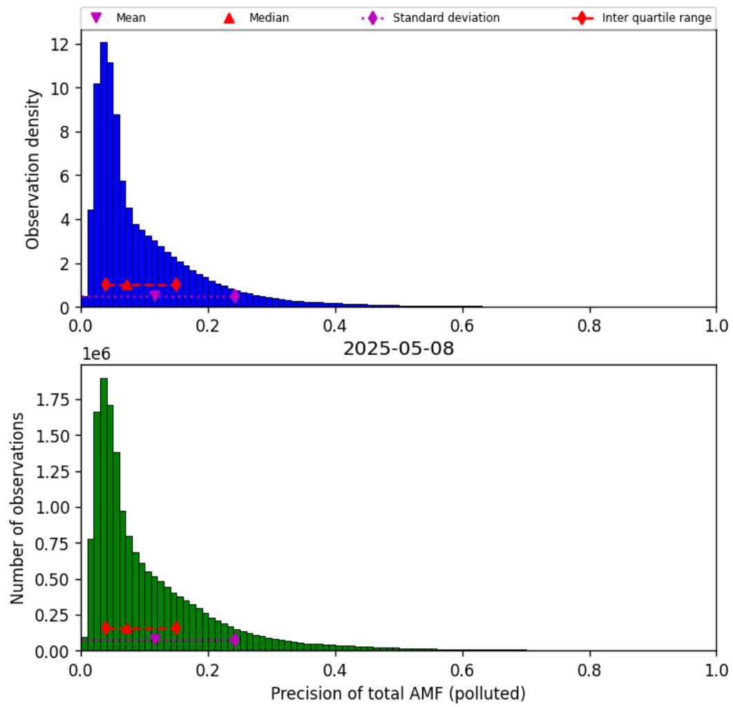
Figure 81: Histogram of “Precision of total AMF (polluted)” for 2025-05-08 to 2025-05-08
