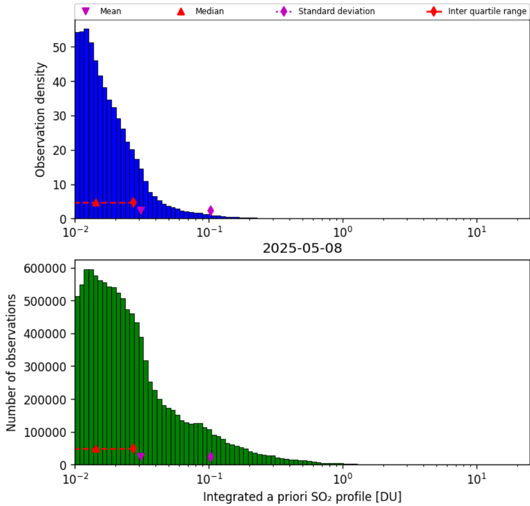
Figure 76: Histogram of “Integrated a priori SO 2 profile” for 2025-05-08 to 2025-05-08
