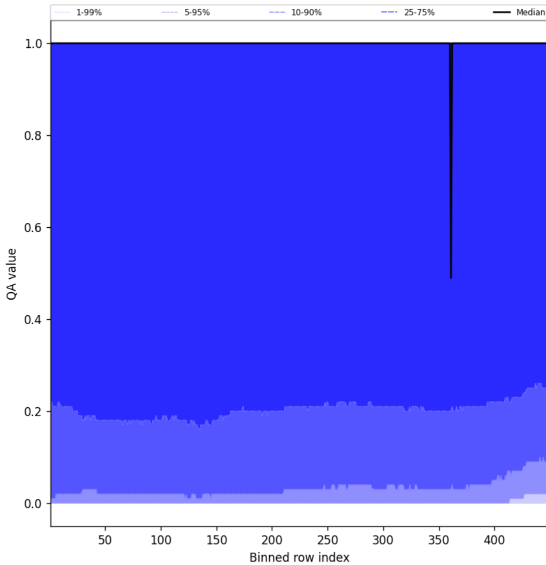
Figure 84: Along track statistics of “QA value” for 2025-05-08 to 2025-05-08
