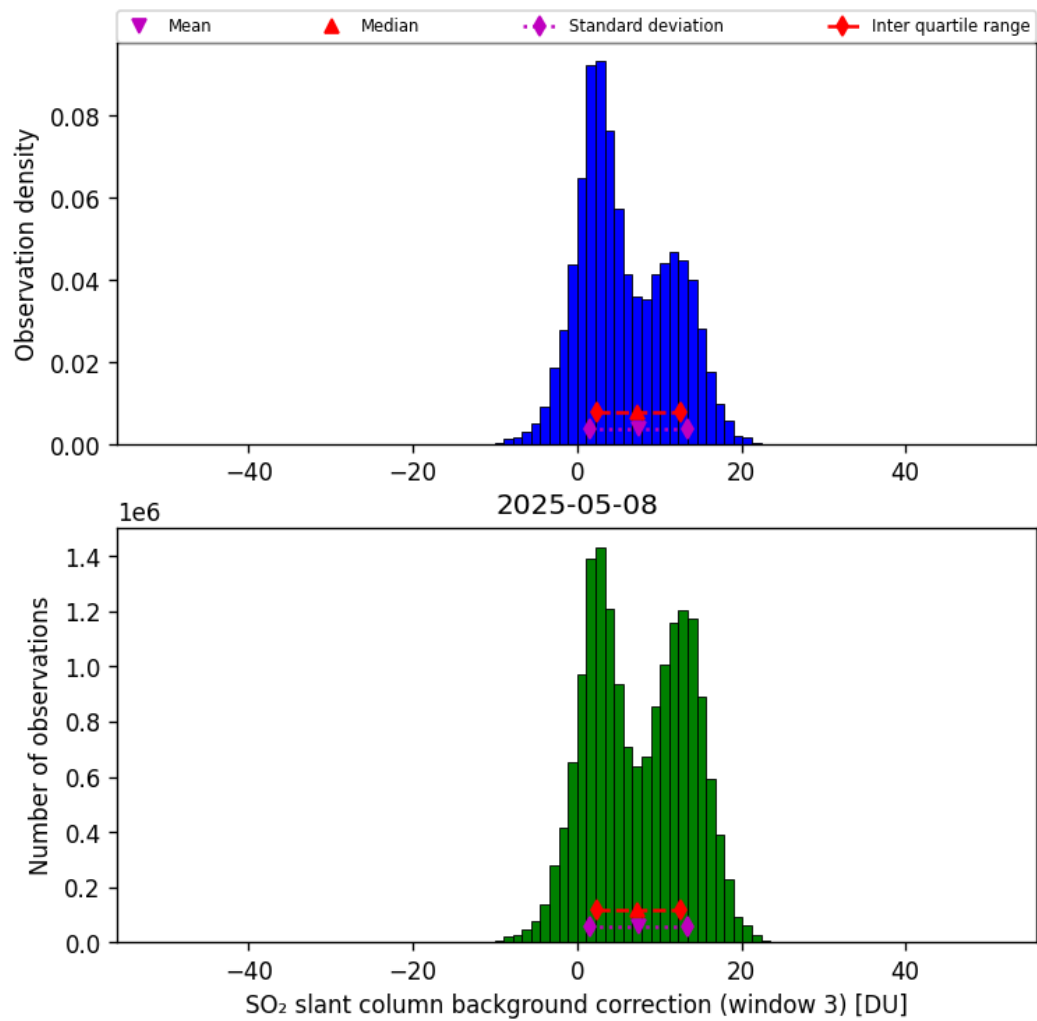
Figure 74: Histogram of “SO 2 slant column background correction (window 3)” for 2025-05-08 to 2025-05-08
