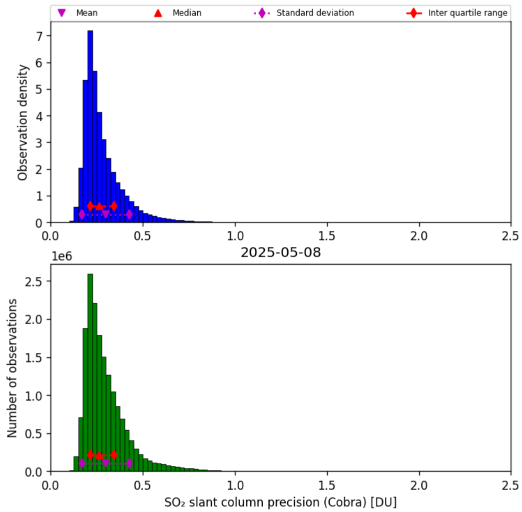
Figure 62: Histogram of “SO 2 slant column precision (Cobra)” for 2025-05-08 to 2025-05-08
