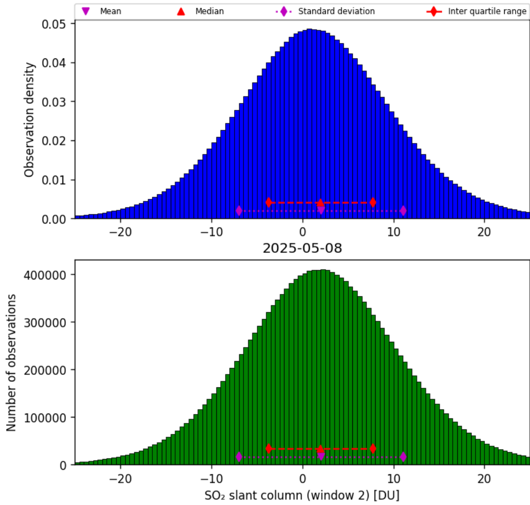
Figure 67: Histogram of “SO 2 slant column (window 2)” for 2025-05-08 to 2025-05-08
