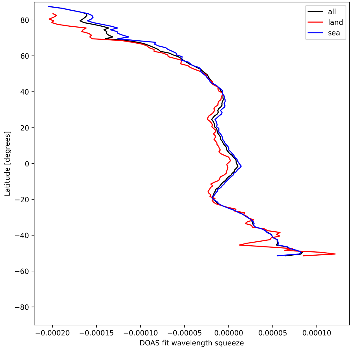
Figure 51: Zonal average of “DOAS fit wavelength squeeze” for 2025-05-08 to 2025-05-08.
