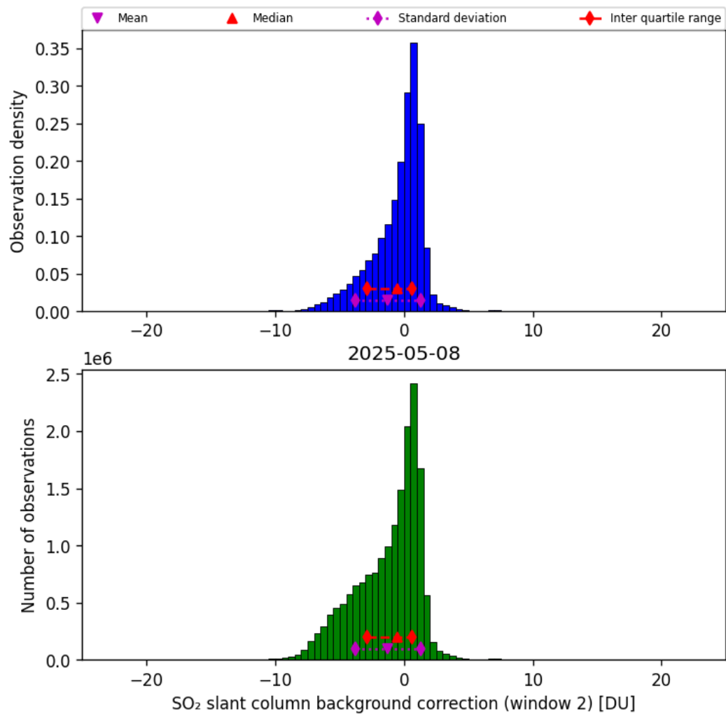
Figure 70: Histogram of “SO 2 slant column background correction (window 2)” for 2025-05-08 to 2025-05-08
