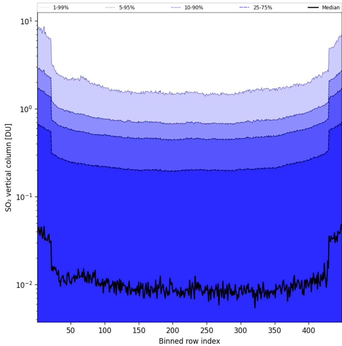
Figure 85: Along track statistics of “SO 2 vertical column” for 2025-05-08 to 2025-05-08
