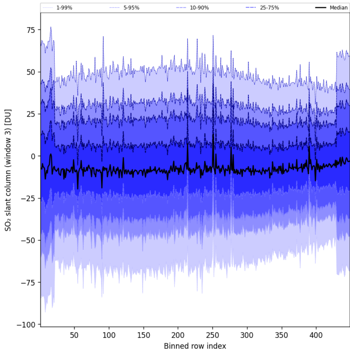
Figure 98: Along track statistics of “SO 2 slant column (window 3)” for 2025-05-08 to 2025-05-08
