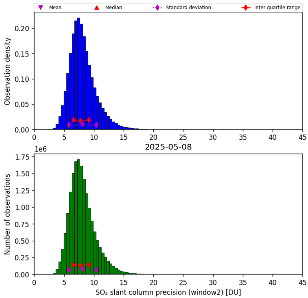
Figure 68: Histogram of “SO 2 slant column precision (window2)” for 2025-05-08 to 2025-05-08
