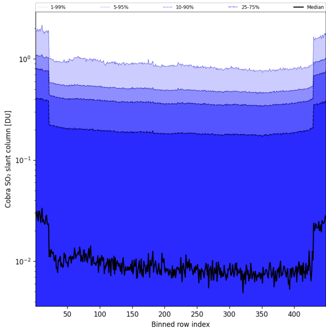
Figure 88: Along track statistics of “Cobra SO 2 slant column” for 2025-05-08 to 2025-05-08
