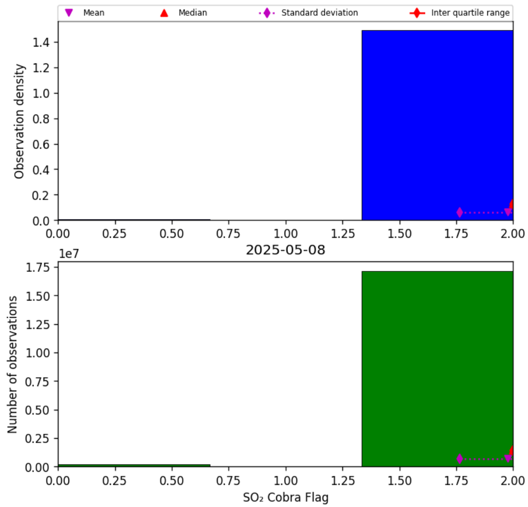
Figure 75: Histogram of “SO 2 Cobra Flag” for 2025-05-08 to 2025-05-08
