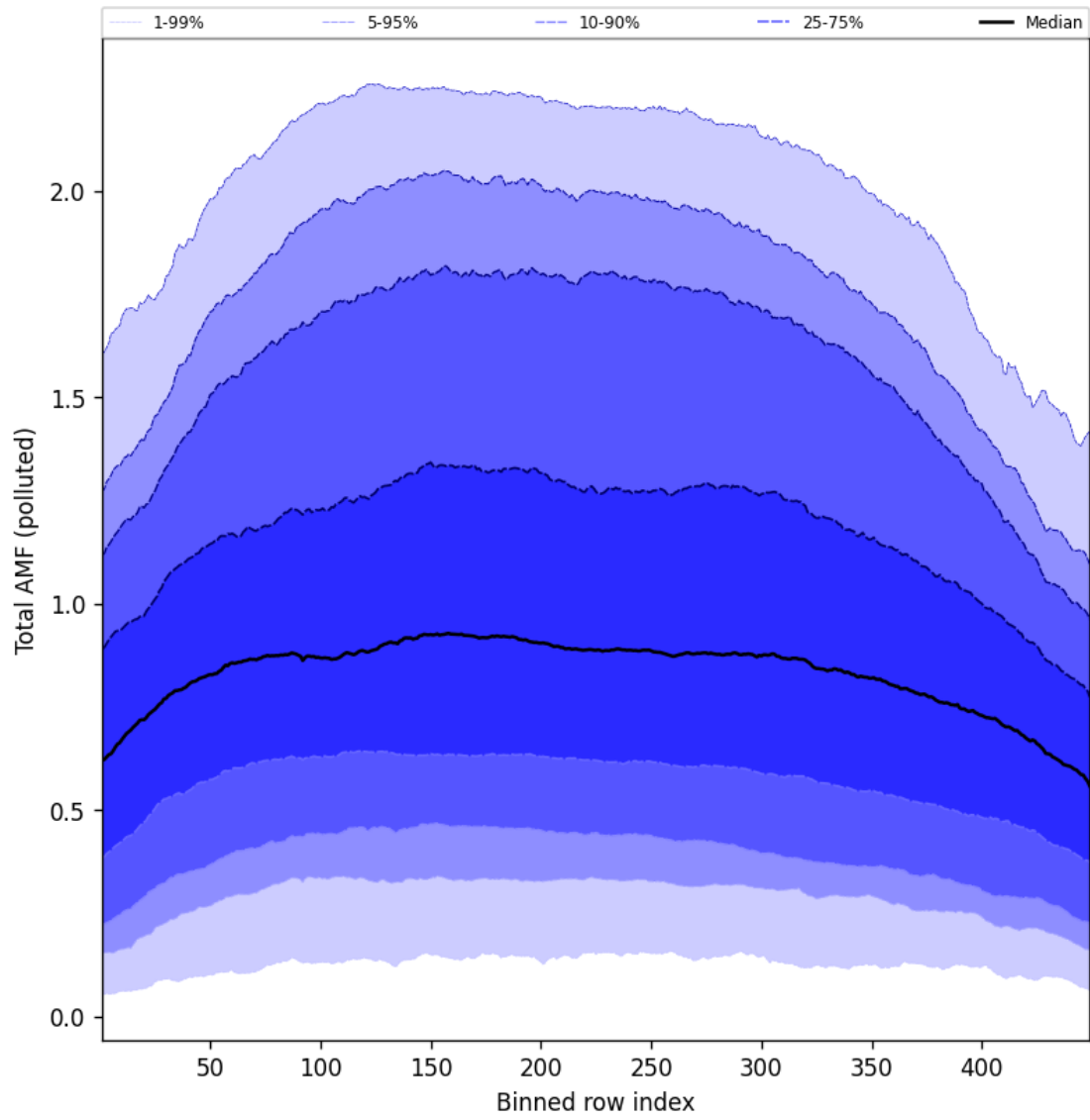
Figure 107: Along track statistics of “Total AMF (polluted)” for 2025-05-08 to 2025-05-08
