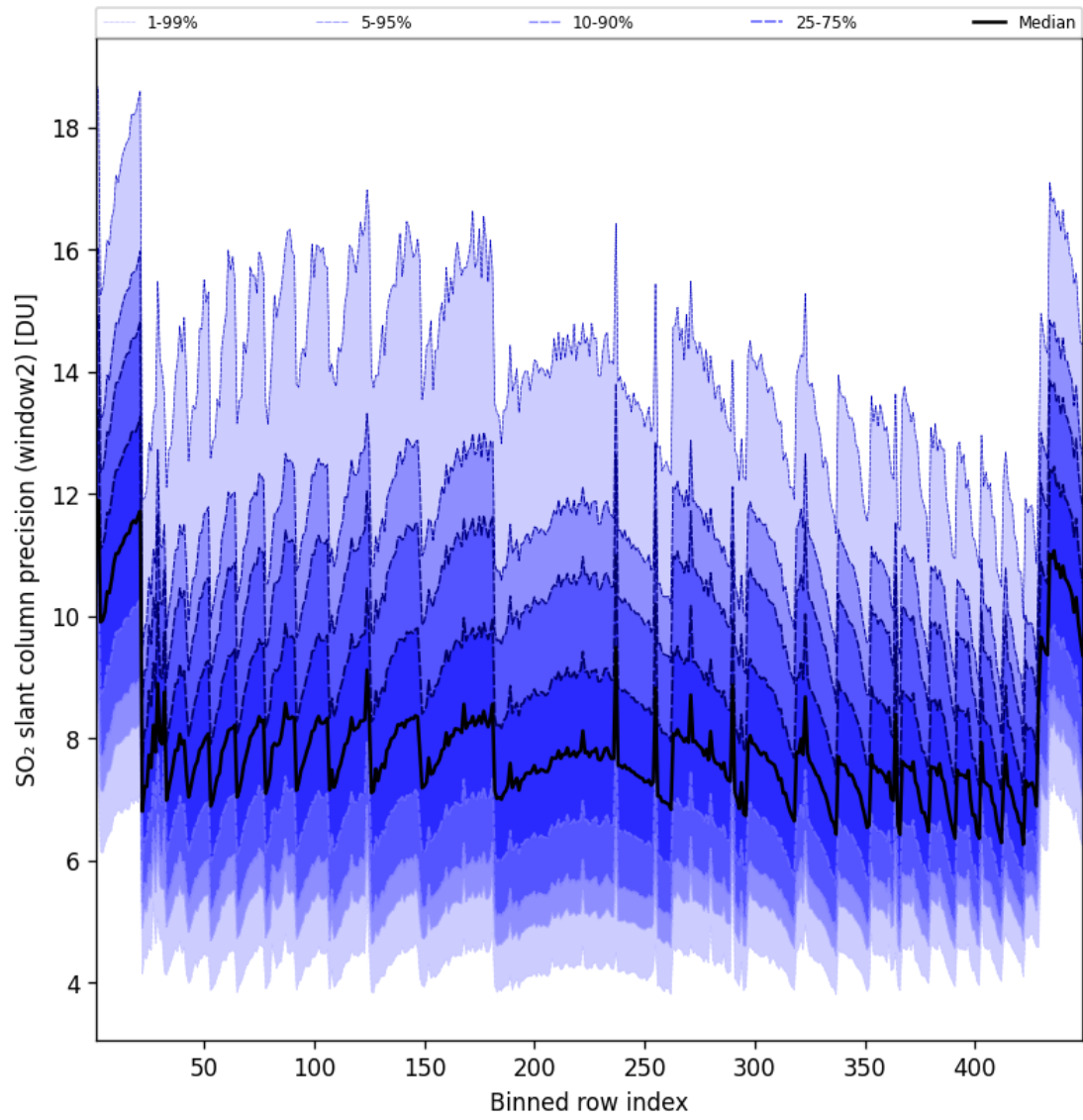
Figure 95: Along track statistics of “SO 2 slant column precision (window2)” for 2025-05-08 to 2025-05-08
