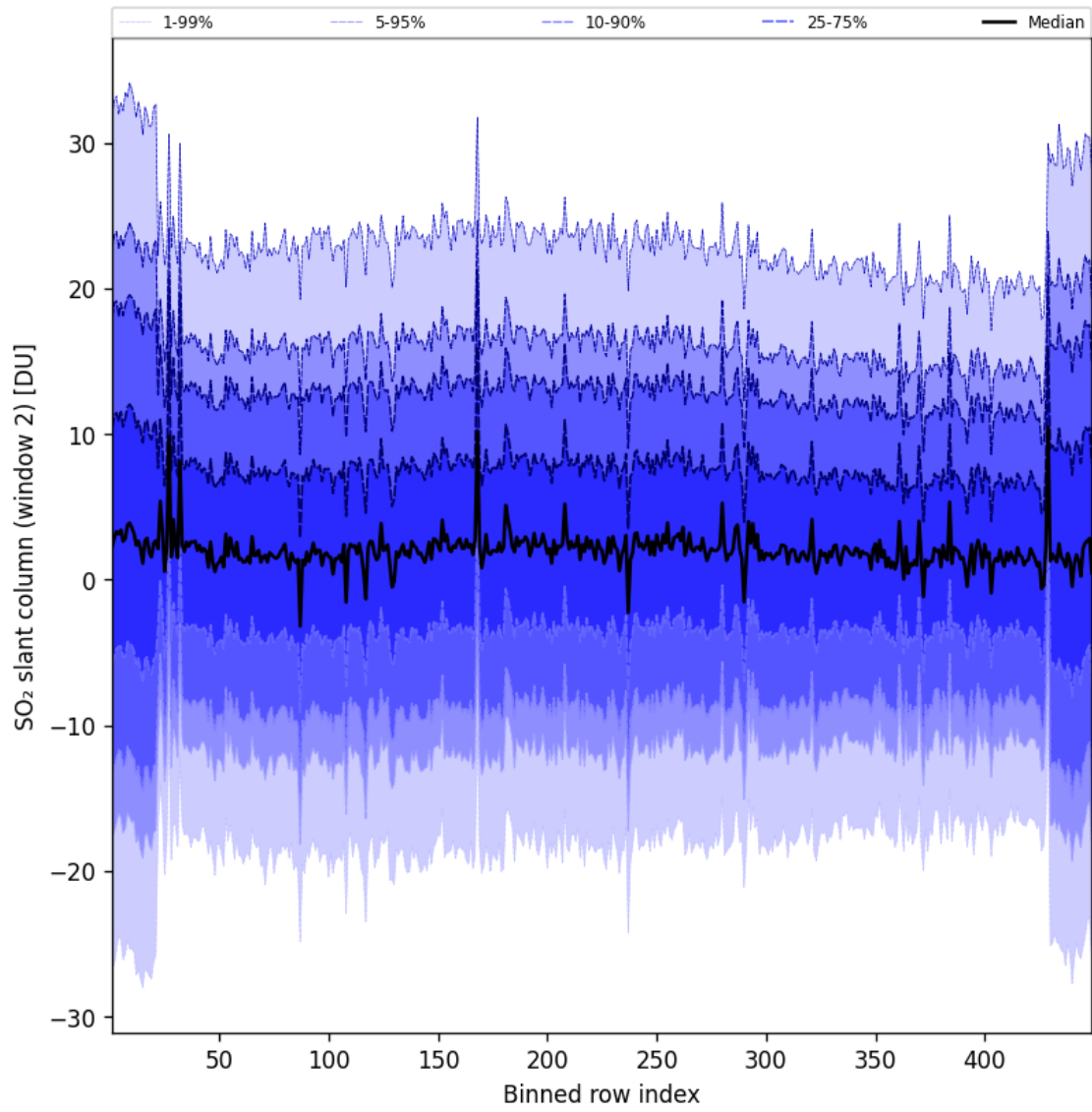
Figure 94: Along track statistics of “SO 2 slant column (window 2)” for 2025-05-08 to 2025-05-08
