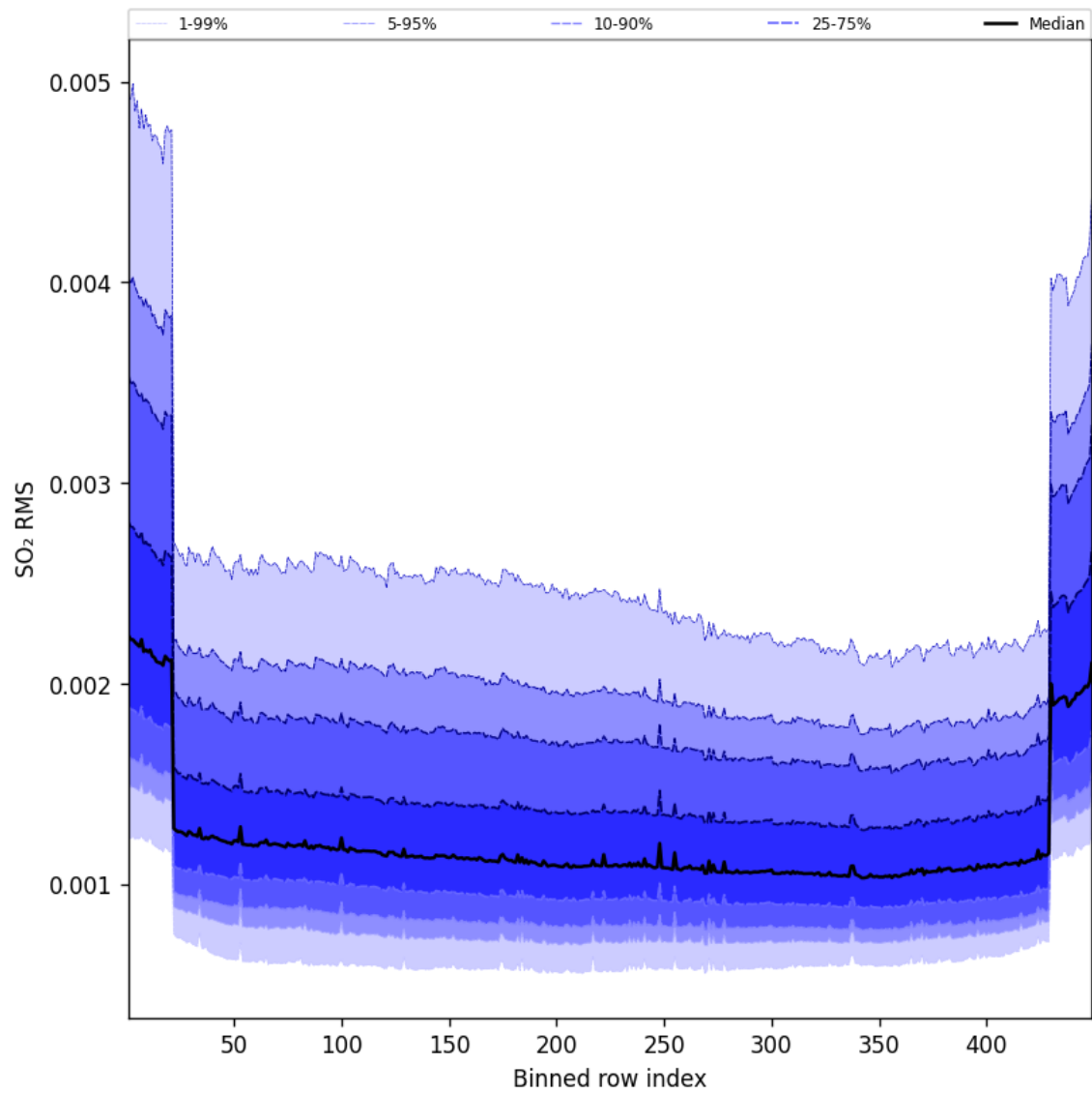
Figure 106: Along track statistics of “SO 2 RMS” for 2025-05-08 to 2025-05-08
