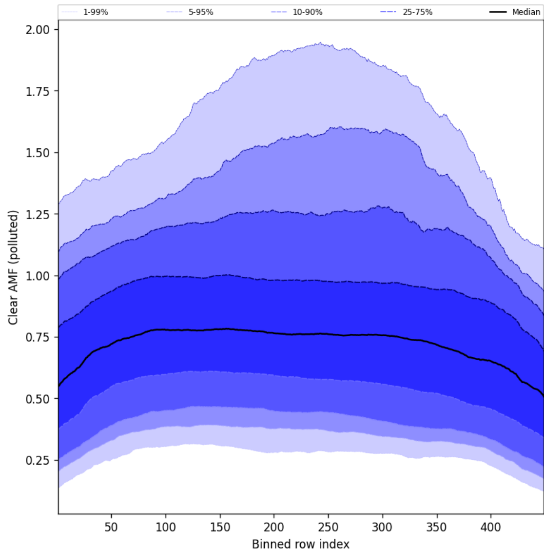
Figure 109: Along track statistics of “Clear AMF (polluted)” for 2025-05-08 to 2025-05-08
