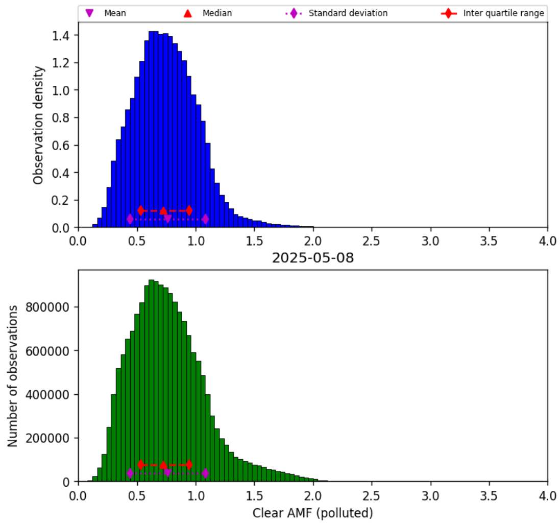
Figure 82: Histogram of “Clear AMF (polluted)” for 2025-05-08 to 2025-05-08
