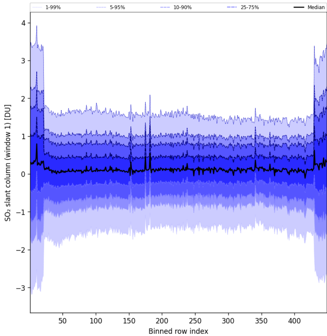
Figure 90: Along track statistics of “SO 2 slant column (window 1)” for 2025-05-08 to 2025-05-08
