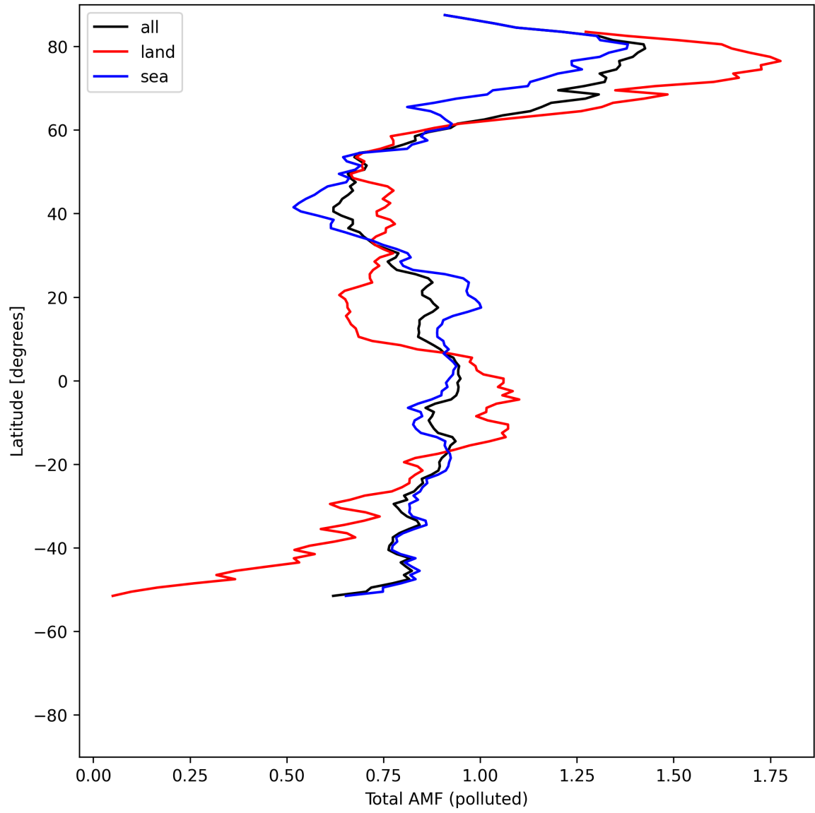
Figure 53: Zonal average of “Total AMF (polluted)” for 2025-05-08 to 2025-05-08.
