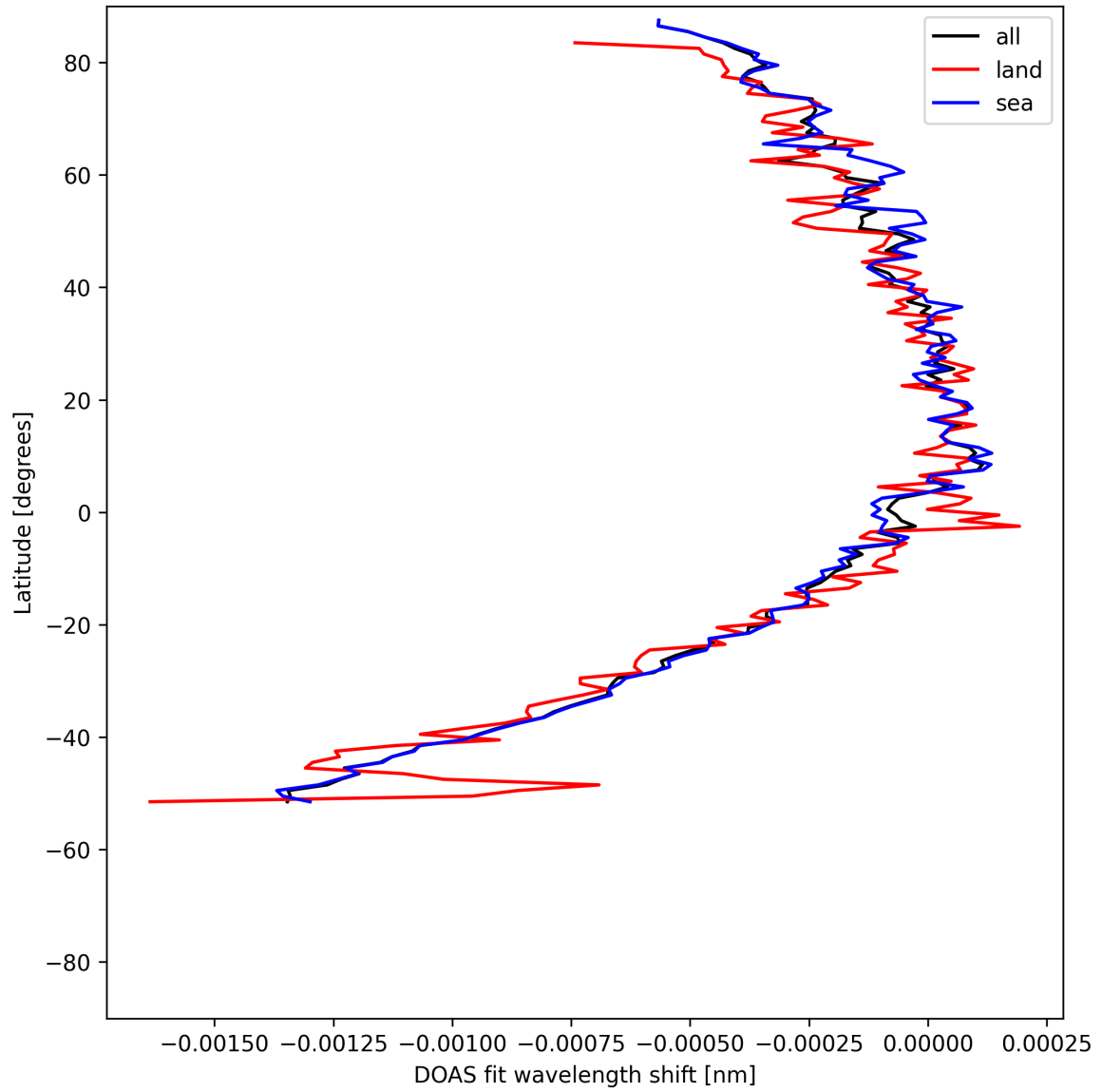
Figure 50: Zonal average of "DOAS fit wavelength shift" for 2025-05-08 to 2025-05-08.
