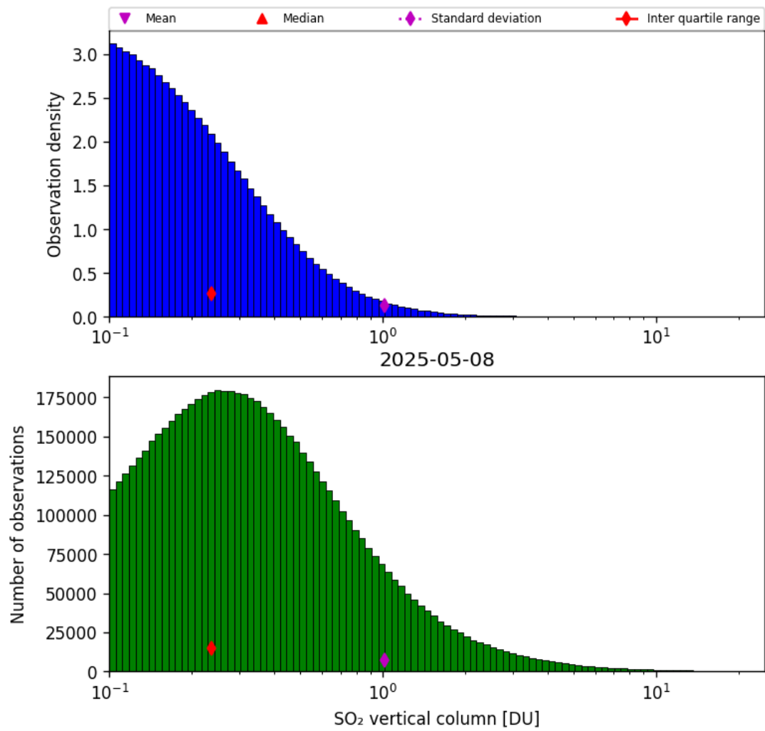
Figure 58: Histogram of “SO 2 vertical column” for 2025-05-08 to 2025-05-08
