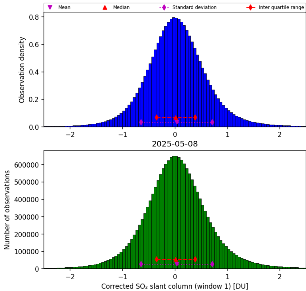
Figure 65: Histogram of “Corrected SO 2 slant column (window 1)” for 2025-05-08 to 2025-05-08
