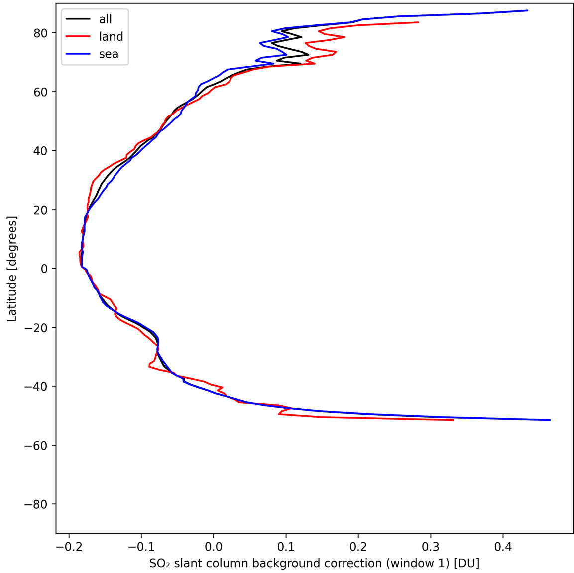
Figure 39: Zonal average of "SO 2 slant column background correction (window 1)" for 2025-05-08 to 2025-05-08.
