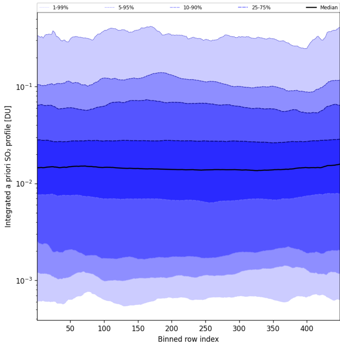
Figure 103: Along track statistics of “Integrated a priori SO 2 profile” for 2025-05-08 to 2025-05-08
