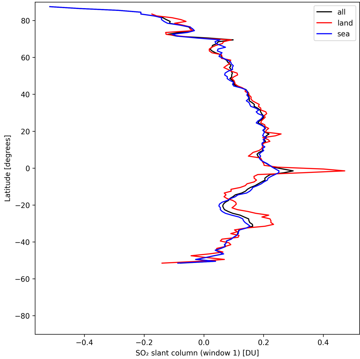
Figure 36: Zonal average of “SO 2 slant column (window 1)” for 2025-05-08 to 2025-05-08.
