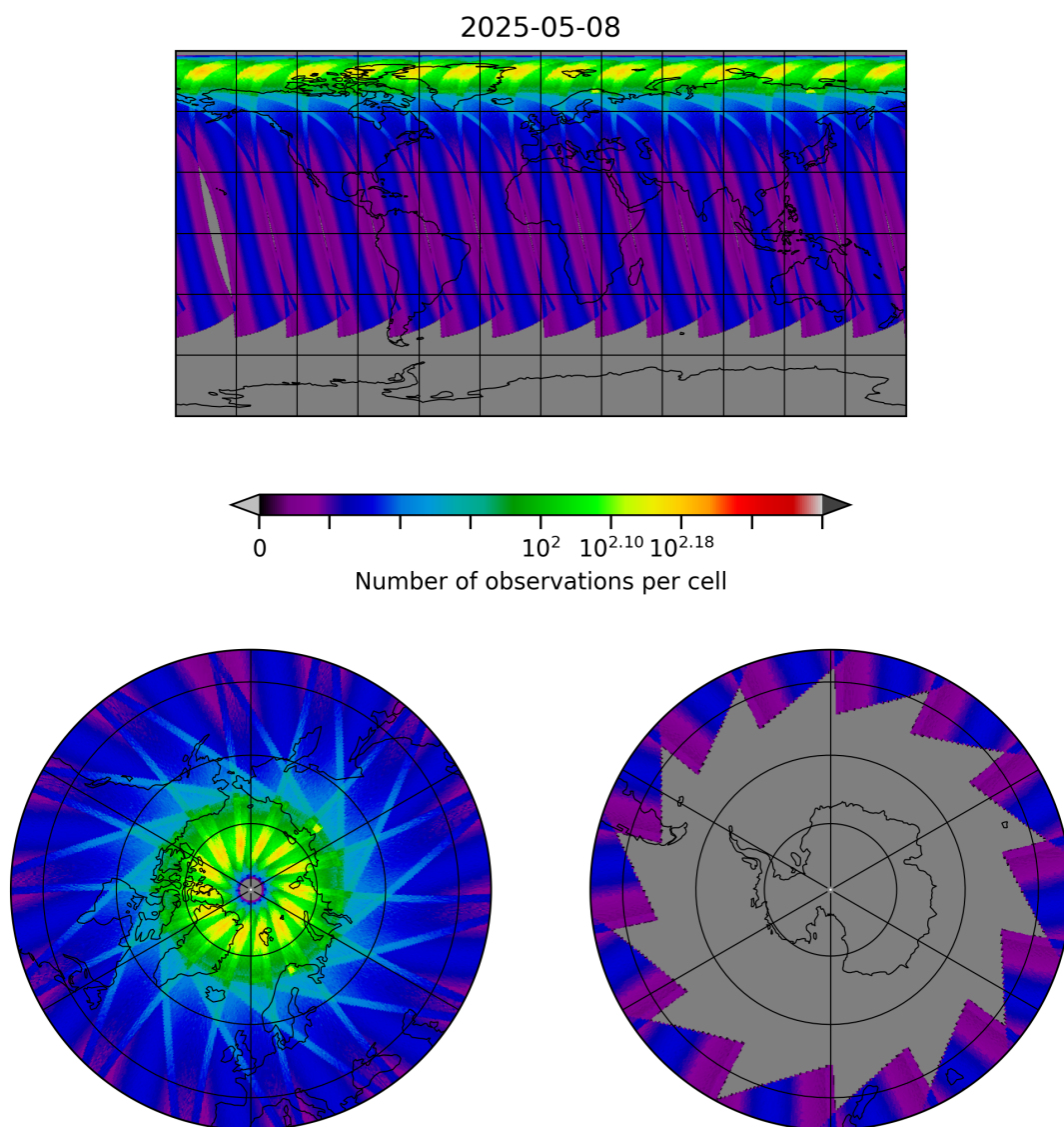
Figure 29: Map of the number of observations for 2025-05-08 to 2025-05-08
