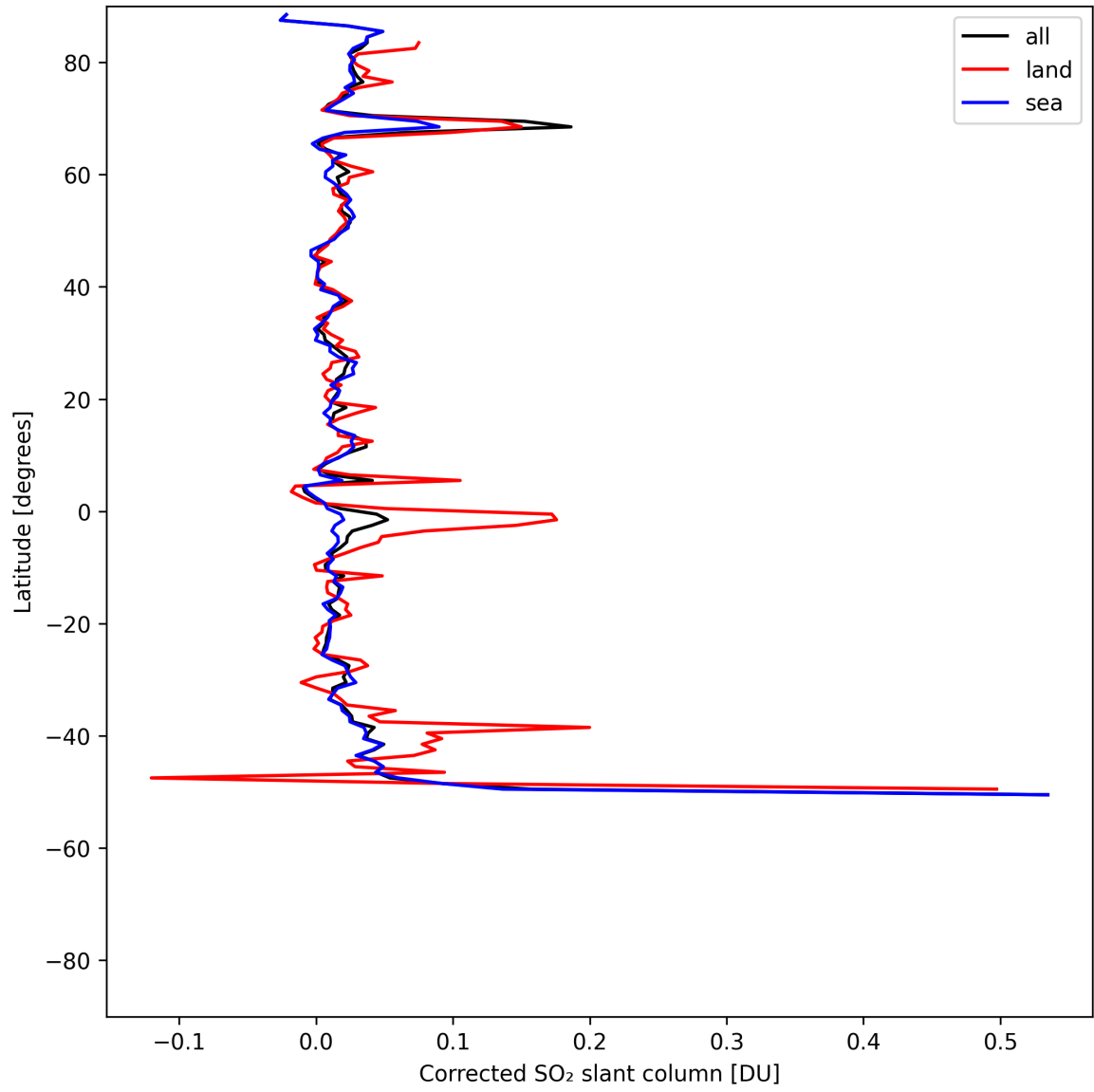
Figure 33: Zonal average of “Corrected SO 2 slant column” for 2025-05-14 to 2025-05-15.
