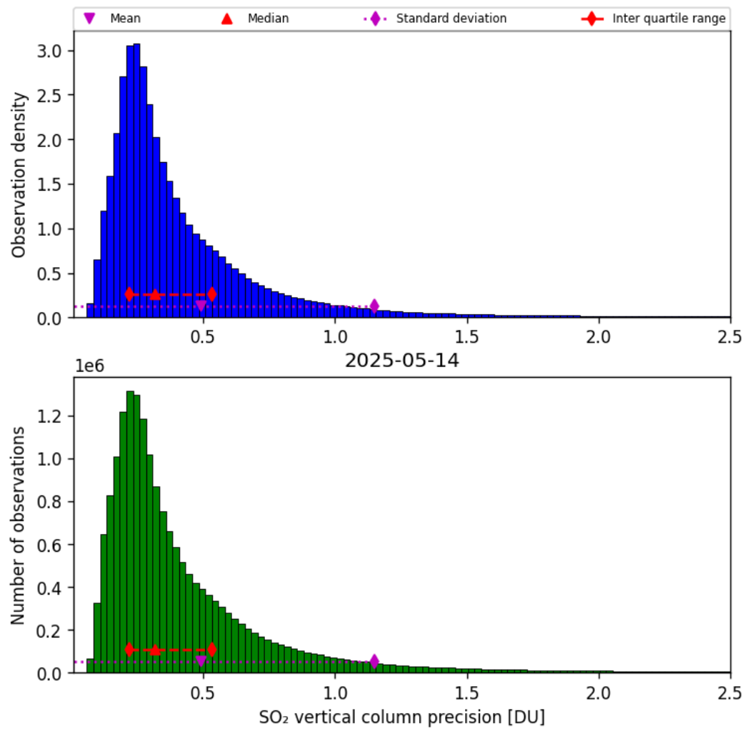
Figure 59: Histogram of “SO 2 vertical column precision” for 2025-05-14 to 2025-05-15
