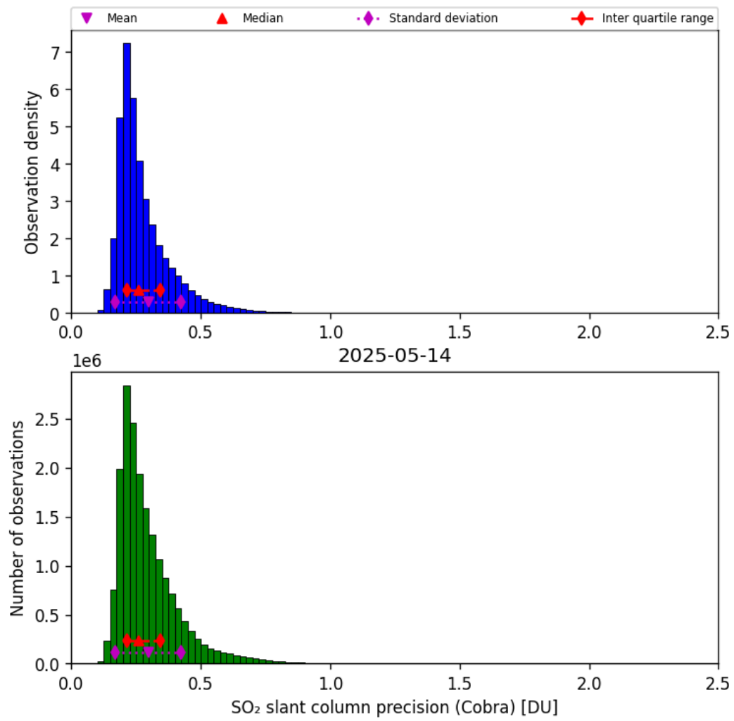
Figure 62: Histogram of “SO 2 slant column precision (Cobra)” for 2025-05-14 to 2025-05-15
