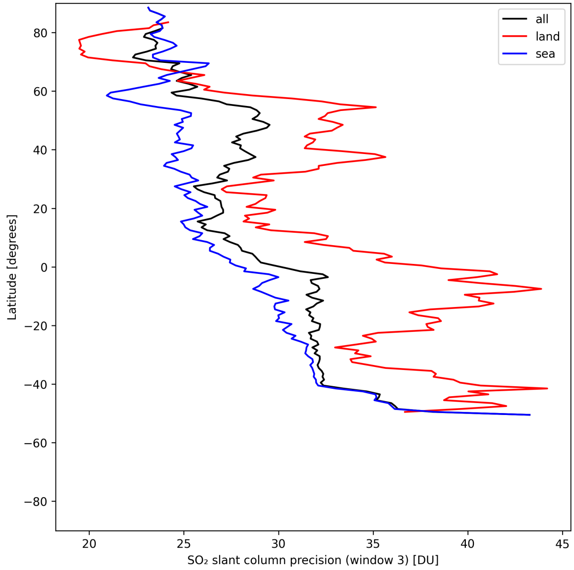
Figure 45: Zonal average of "SO 2 slant column precision (window 3)" for 2025-05-14 to 2025-05-15.
