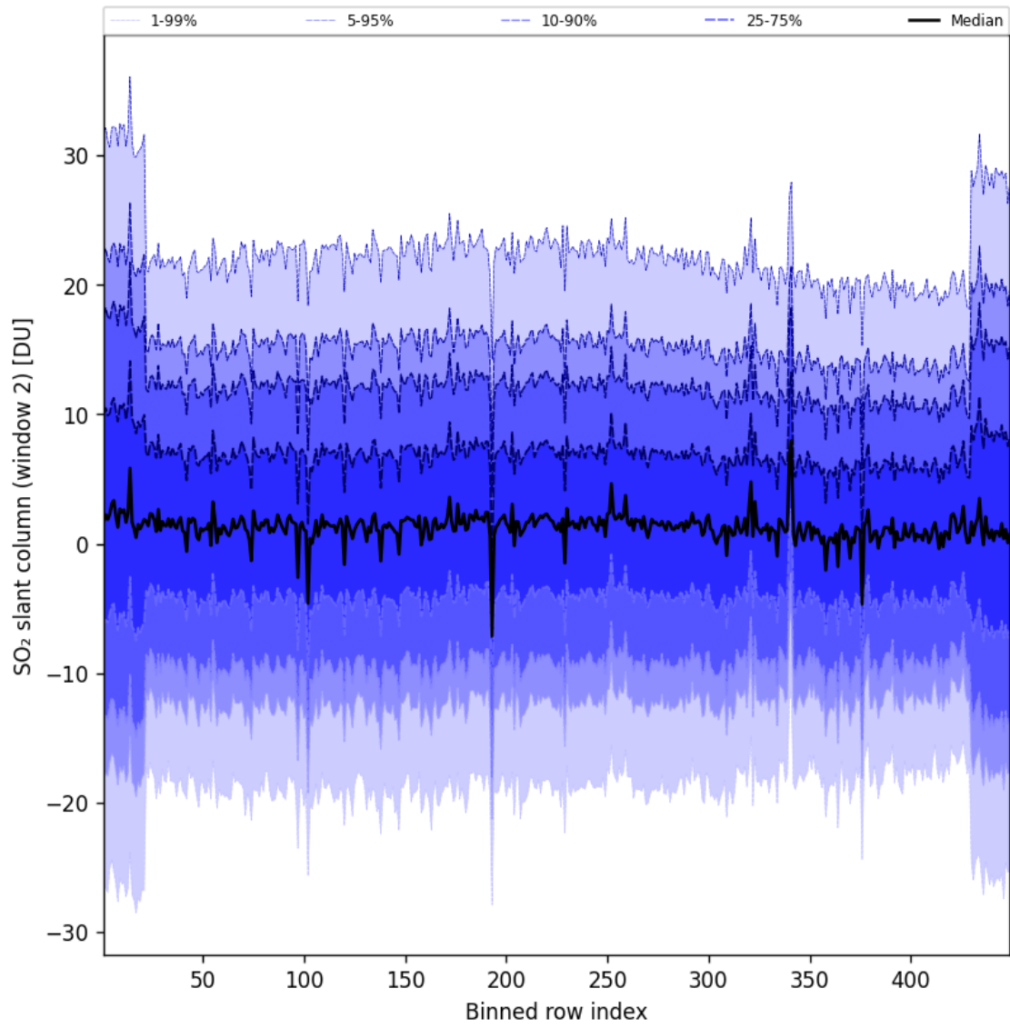
Figure 94: Along track statistics of “SO 2 slant column (window 2)” for 2025-05-14 to 2025-05-15
