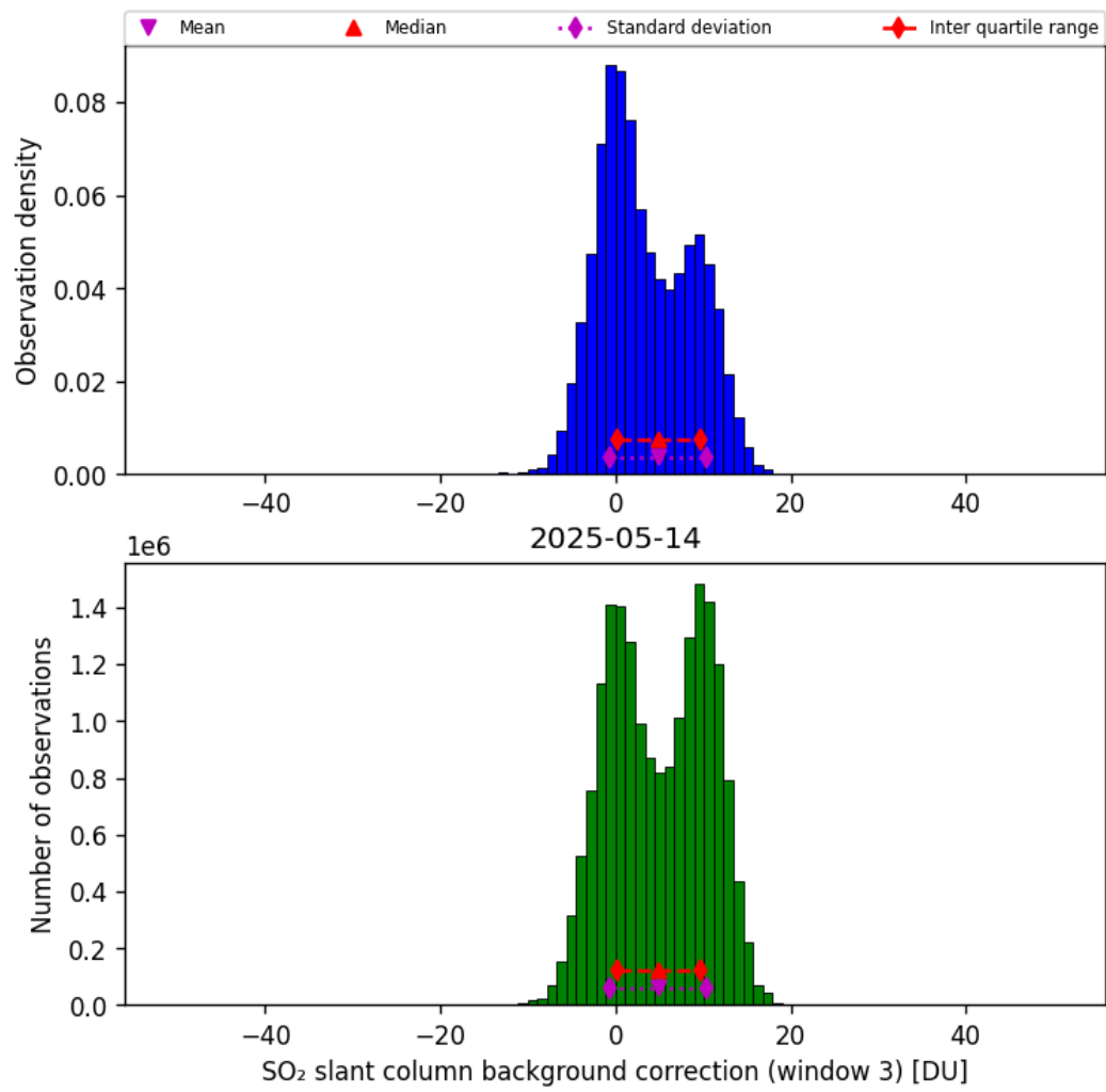
Figure 74: Histogram of “SO 2 slant column background correction (window 3)” for 2025-05-14 to 2025-05-15
