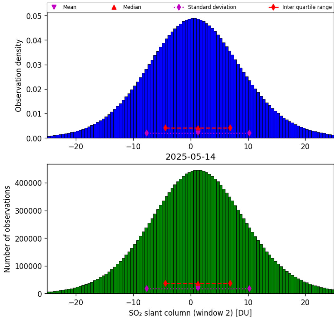
Figure 67: Histogram of “SO 2 slant column (window 2)” for 2025-05-14 to 2025-05-15
