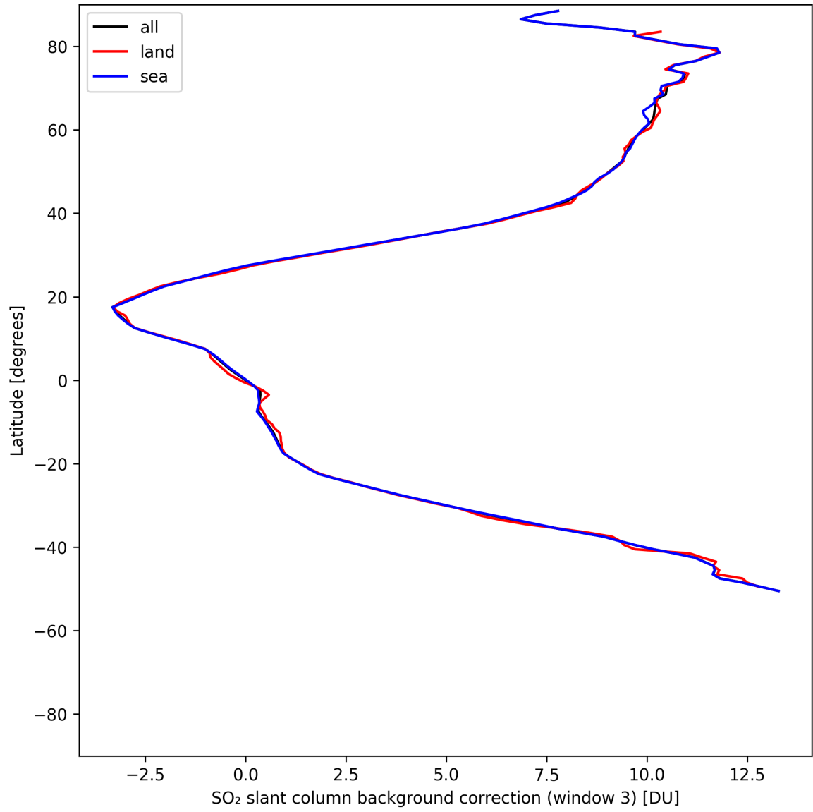
Figure 47: Zonal average of “SO 2 slant column background correction (window 3)” for 2025-05-14 to 2025-05-15.
