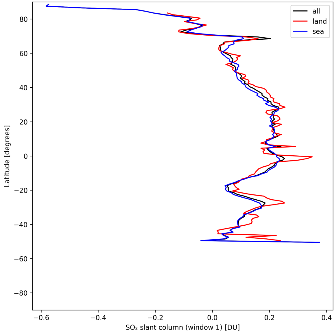
Figure 36: Zonal average of “SO 2 slant column (window 1)” for 2025-05-14 to 2025-05-15.
