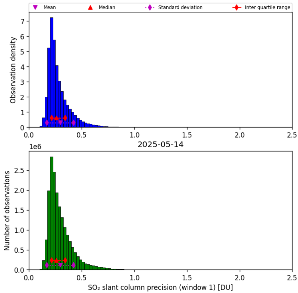
Figure 64: Histogram of “SO 2 slant column precision (window 1)” for 2025-05-14 to 2025-05-15
