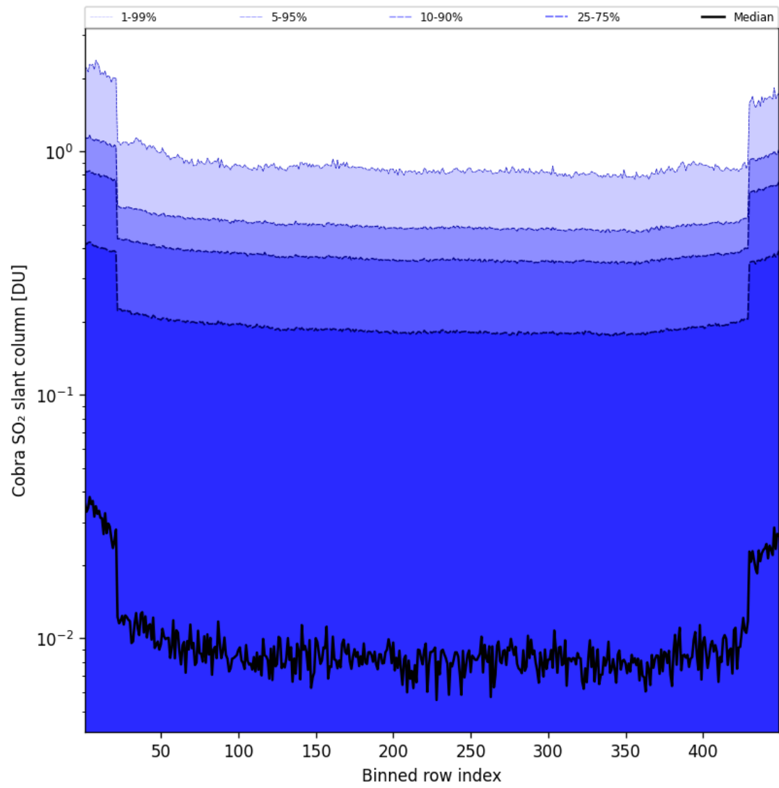
Figure 88: Along track statistics of “Cobra SO 2 slant column” for 2025-05-14 to 2025-05-15
