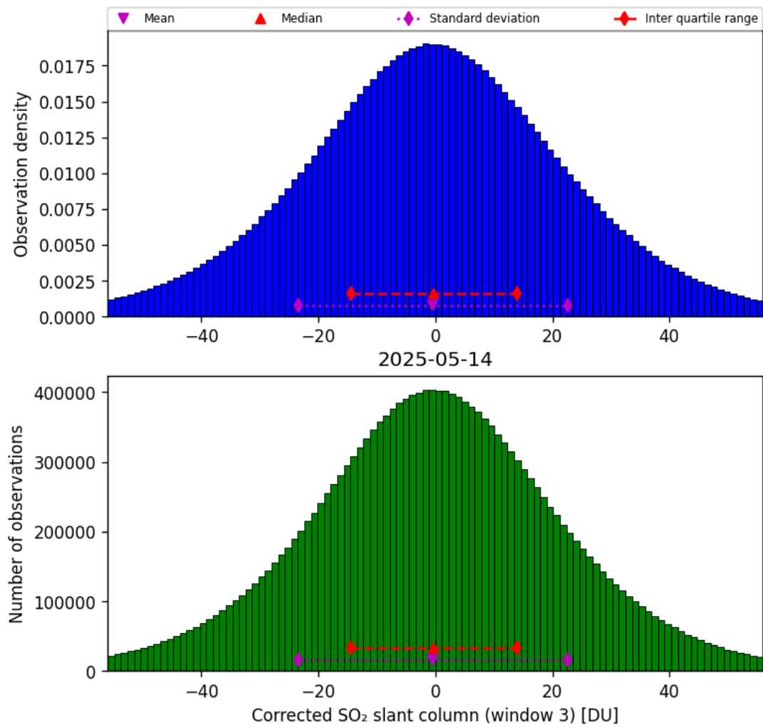
Figure 73: Histogram of “Corrected SO 2 slant column (window 3)” for 2025-05-14 to 2025-05-15
