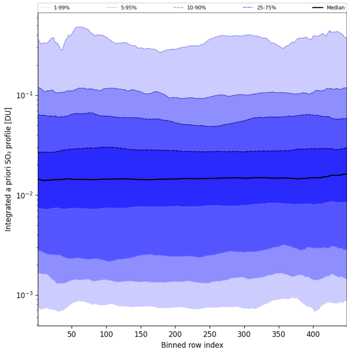
Figure 103: Along track statistics of “Integrated a priori SO 2 profile” for 2025-05-14 to 2025-05-15
