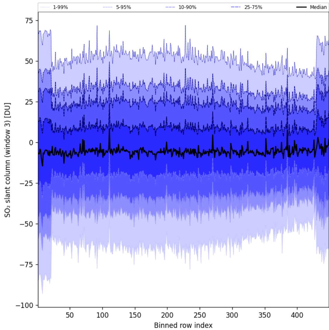
Figure 98: Along track statistics of “SO 2 slant column (window 3)” for 2025-05-14 to 2025-05-15
