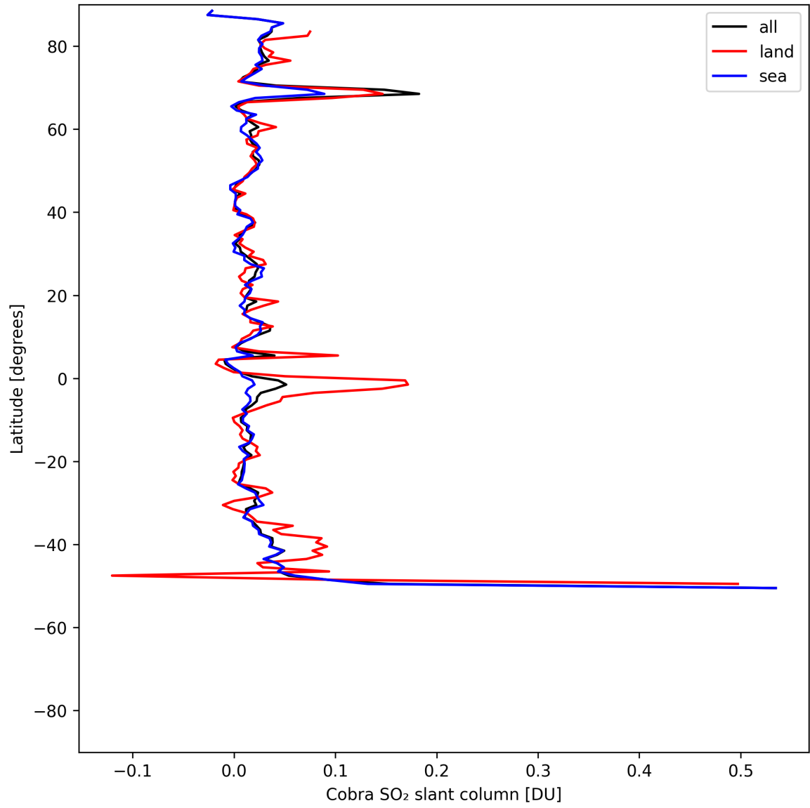
Figure 34: Zonal average of “Cobra SO 2 slant column” for 2025-05-14 to 2025-05-15.
