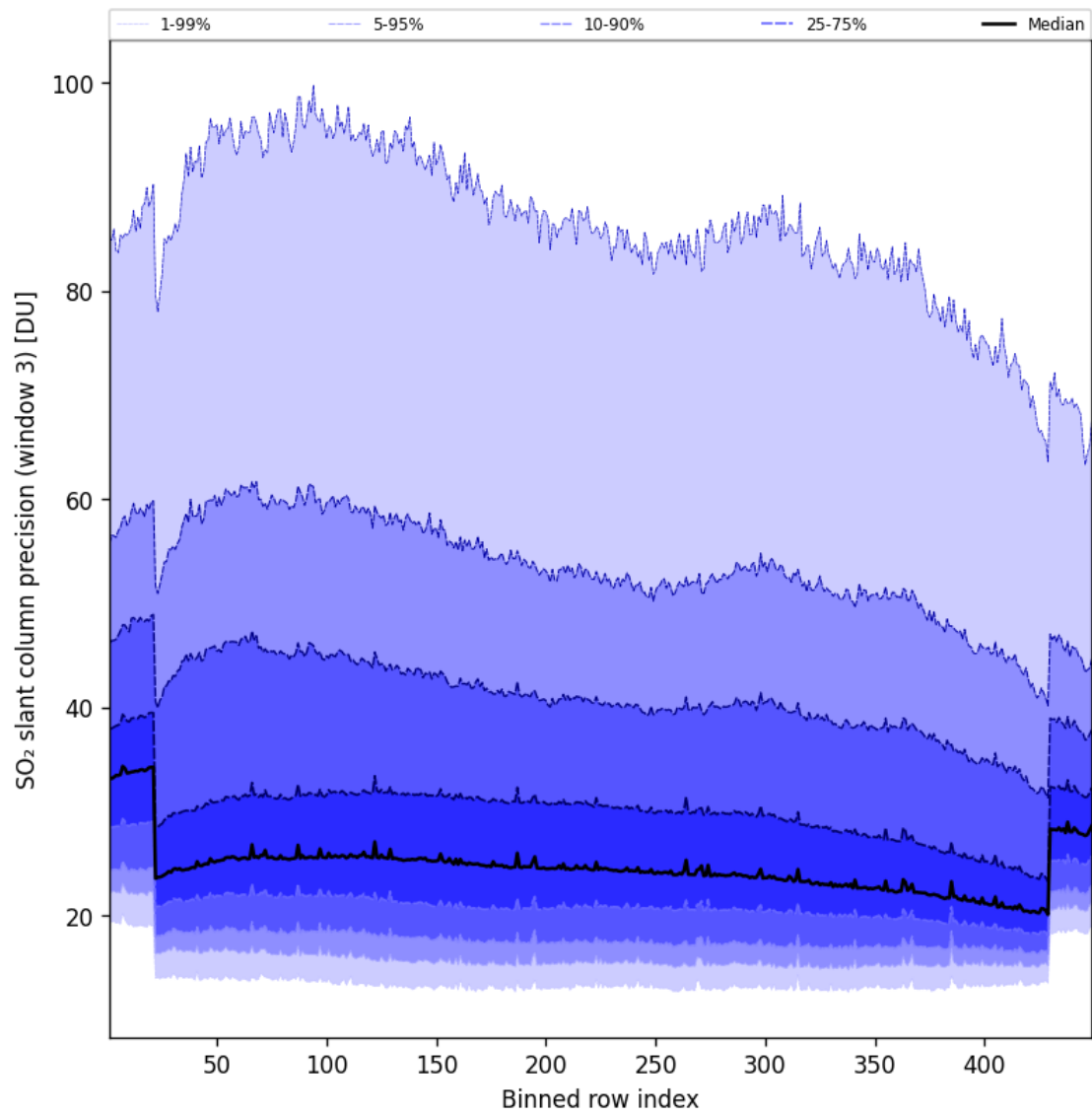
Figure 99: Along track statistics of “SO 2 slant column precision (window 3)” for 2025-05-14 to 2025-05-15
