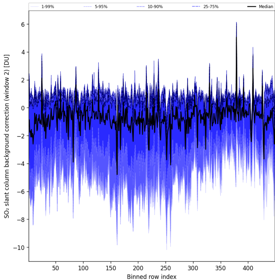
Figure 97: Along track statistics of “SO 2 slant column background correction (window 2)” for 2025-05-14 to 2025-05-15
