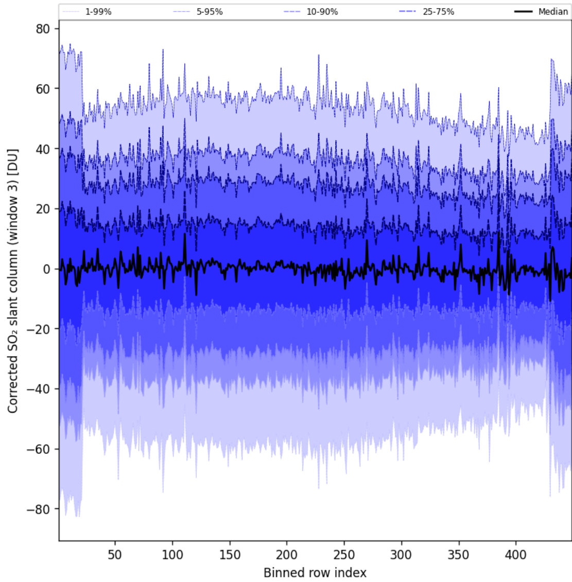
Figure 100: Along track statistics of “Corrected SO 2 slant column (window 3)” for 2025-05-14 to 2025-05-15
