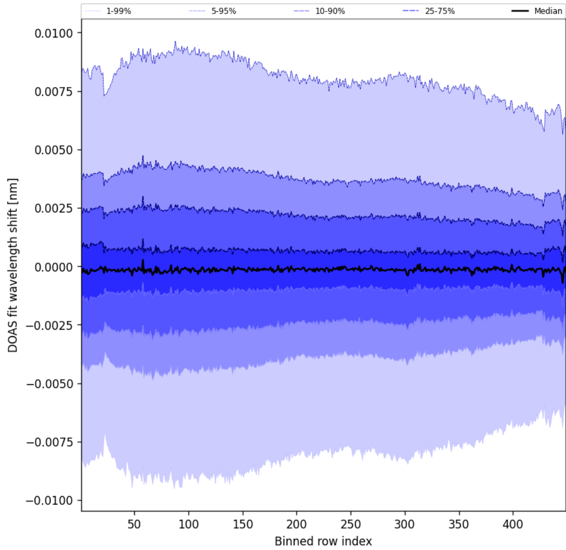
Figure 104: Along track statistics of “DOAS fit wavelength shift” for 2025-05-14 to 2025-05-15
