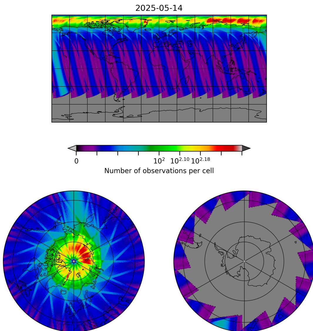
Figure 29: Map of the number of observations for 2025-05-14 to 2025-05-15
