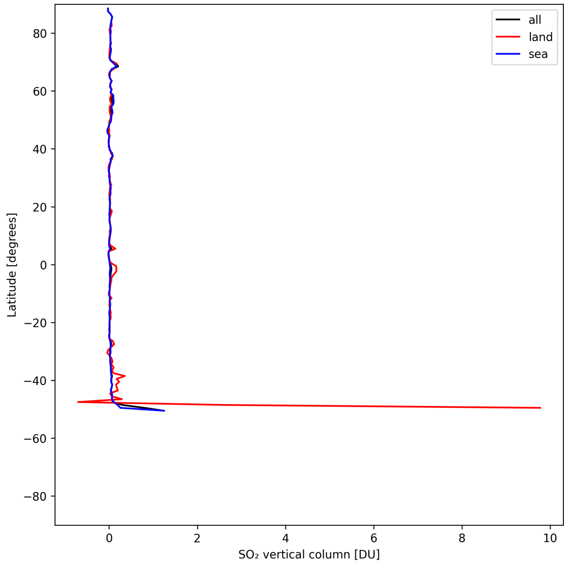
Figure 31: Zonal average of “SO 2 vertical column” for 2025-05-14 to 2025-05-15.
