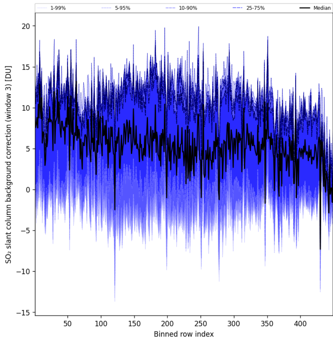
Figure 101: Along track statistics of “SO 2 slant column background correction (window 3)” for 2025-05-14 to 2025-05-15
