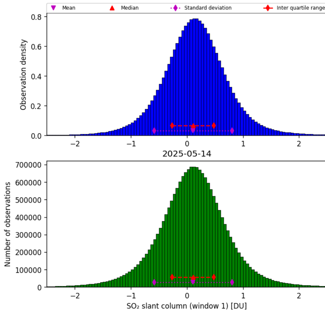
Figure 63: Histogram of “SO 2 slant column (window 1)” for 2025-05-14 to 2025-05-15
