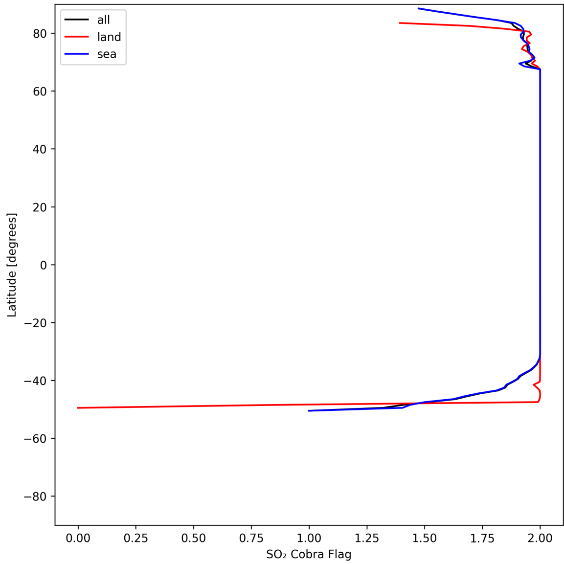
Figure 48: Zonal average of "SO 2 Cobra Flag" for 2025-05-14 to 2025-05-15.
