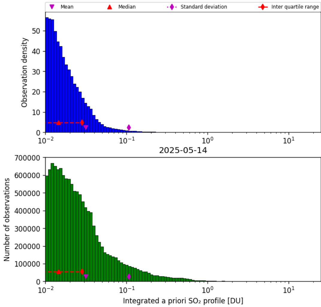
Figure 76: Histogram of “Integrated a priori SO 2 profile” for 2025-05-14 to 2025-05-15
