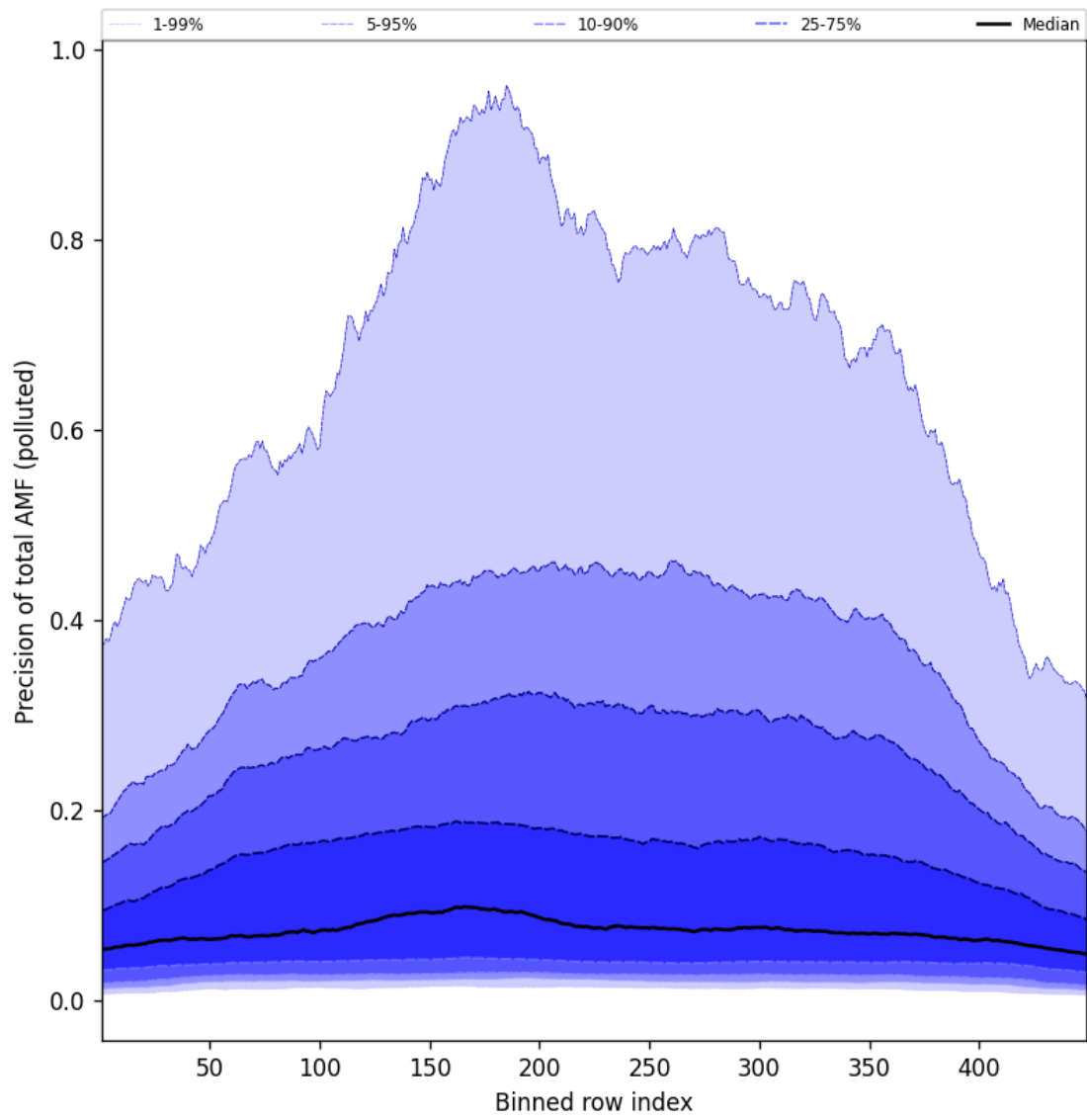
Figure 108: Along track statistics of “Precision of total AMF (polluted)” for 2025-05-14 to 2025-05-15
