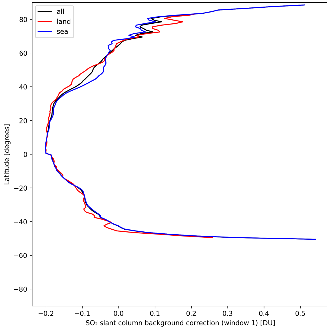
Figure 39: Zonal average of "SO 2 slant column background correction (window 1)" for 2025-05-14 to 2025-05-15.
