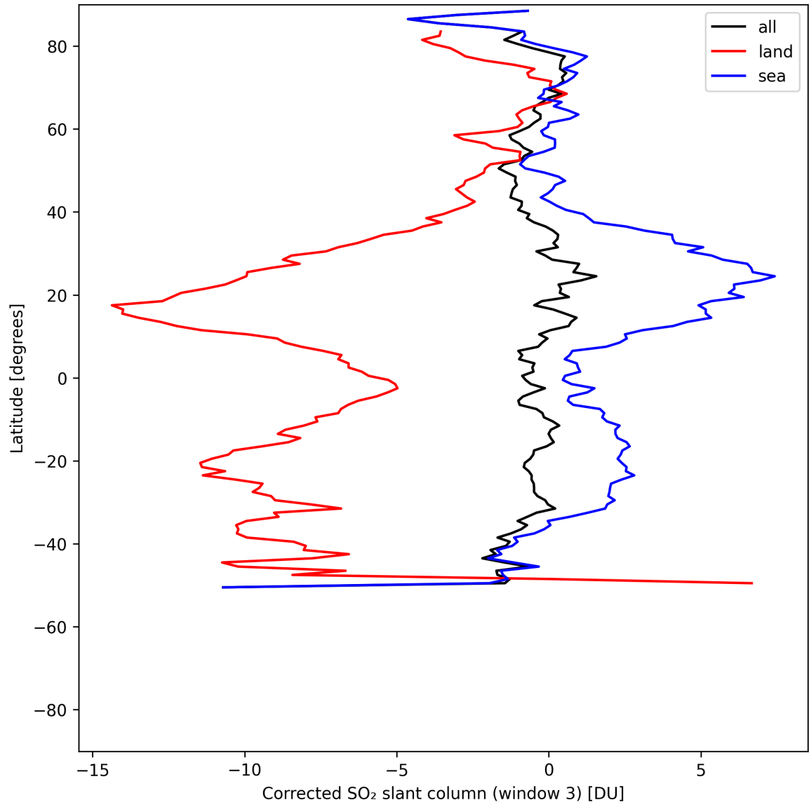
Figure 46: Zonal average of “Corrected SO 2 slant column (window 3)” for 2025-05-14 to 2025-05-15.
