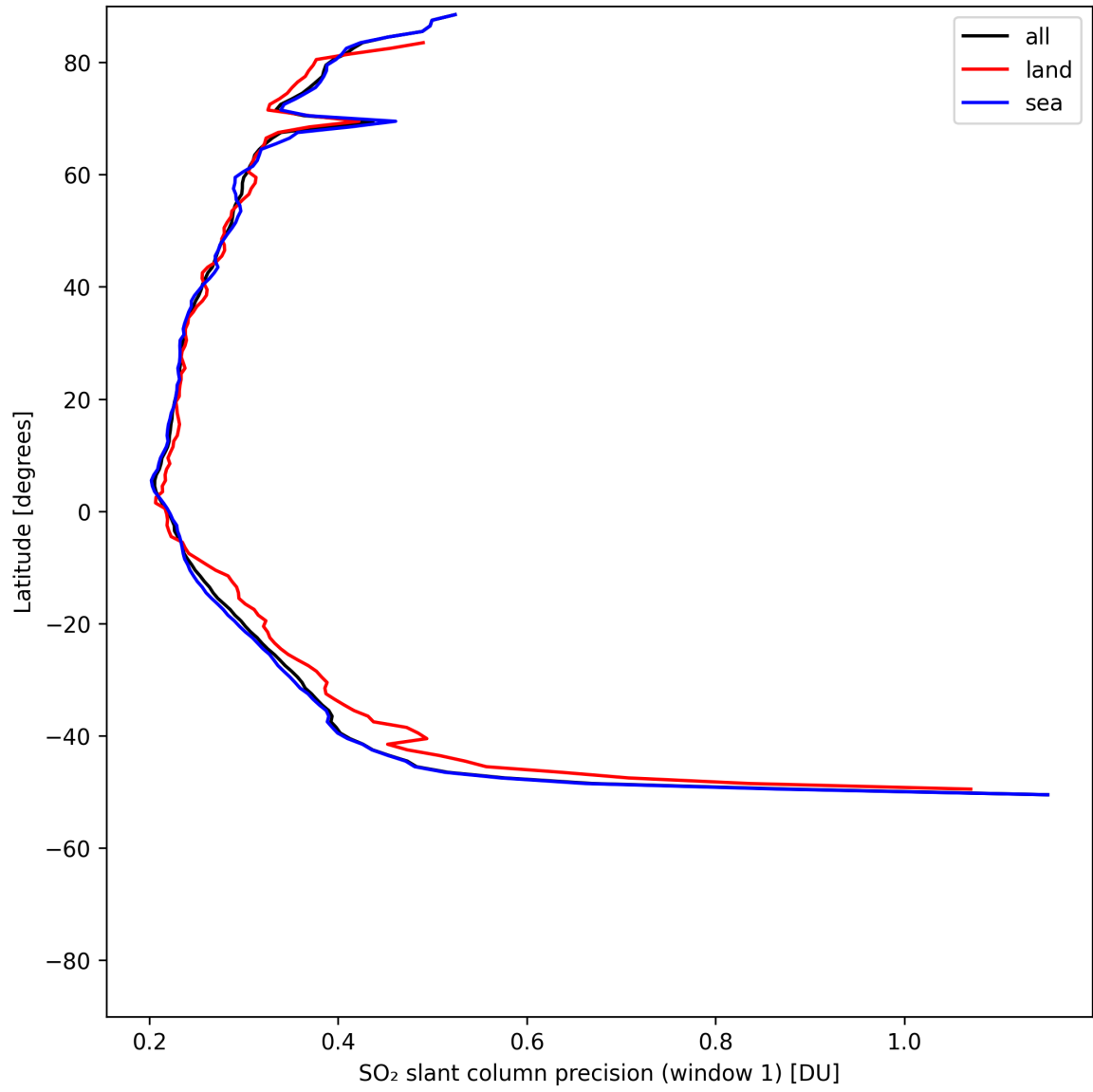
Figure 37: Zonal average of “SO 2 slant column precision (window 1)” for 2025-05-14 to 2025-05-15.
