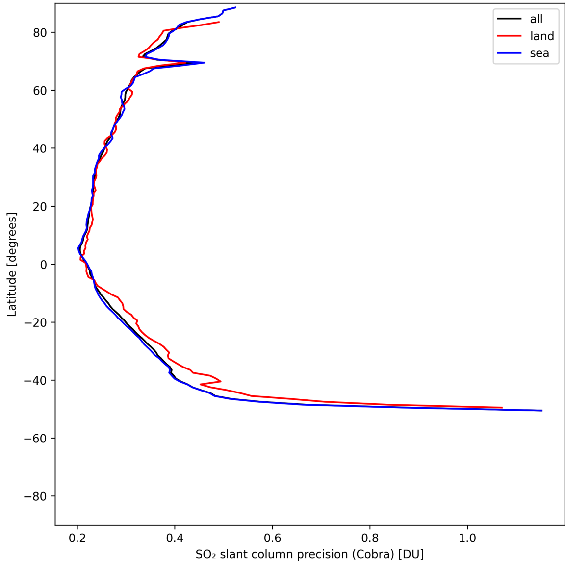
Figure 35: Zonal average of “SO 2 slant column precision (Cobra)” for 2025-05-14 to 2025-05-15.
