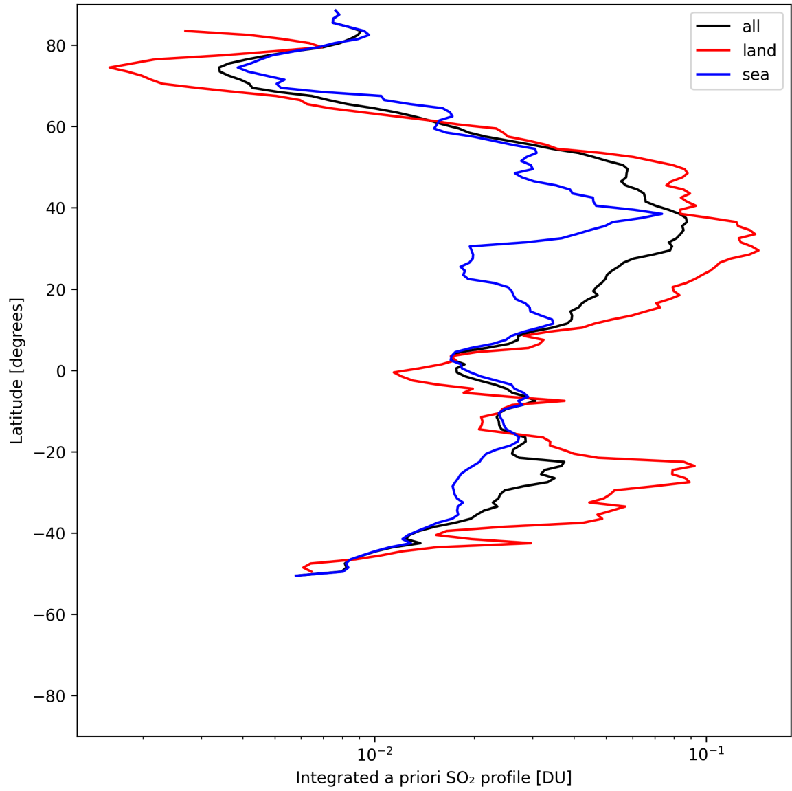
Figure 49: Zonal average of “Integrated a priori SO 2 profile” for 2025-05-14 to 2025-05-15.
