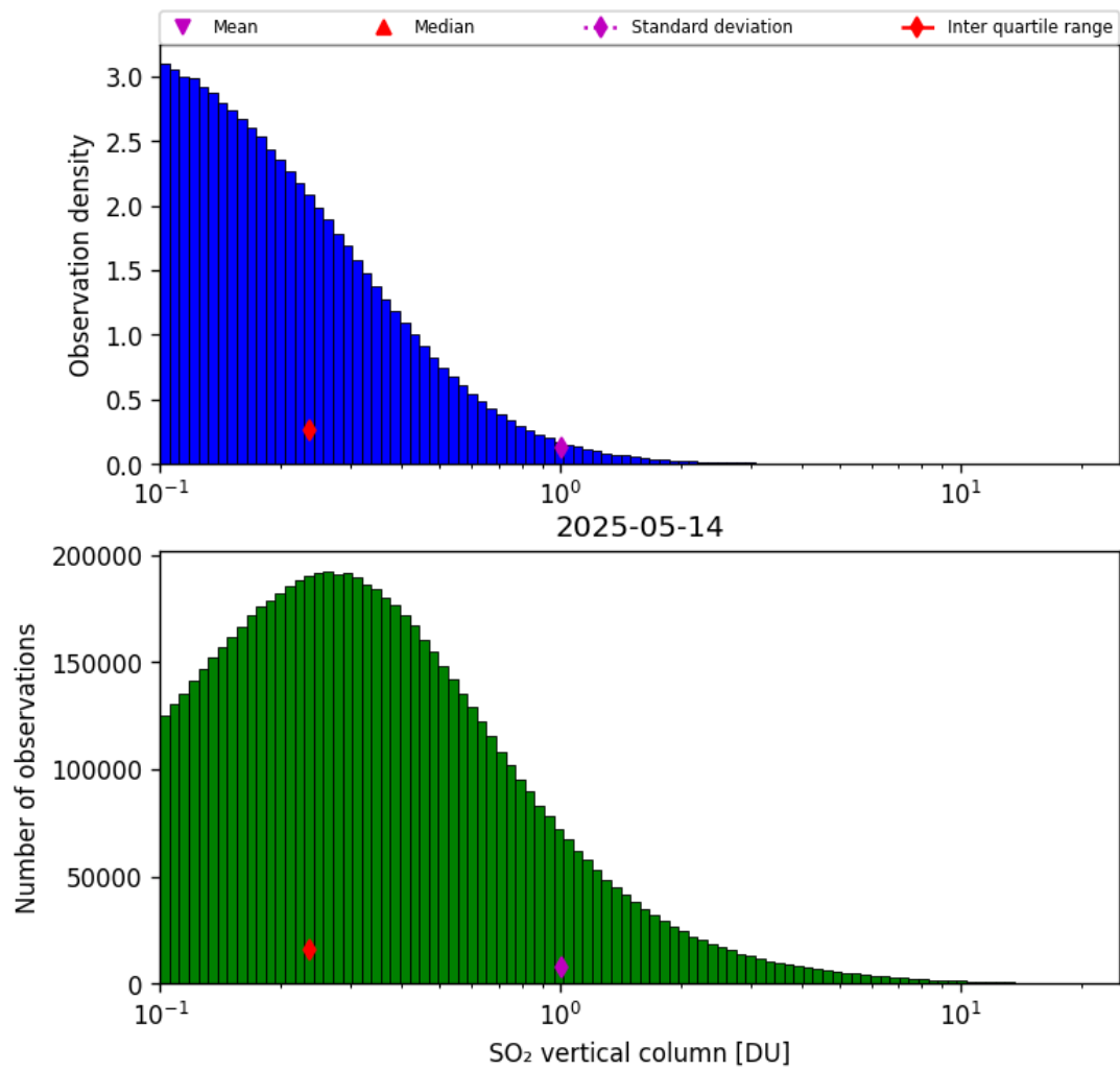
Figure 58: Histogram of “SO 2 vertical column” for 2025-05-14 to 2025-05-15
