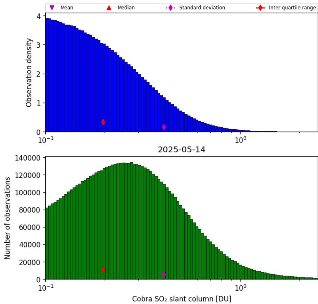
Figure 61: Histogram of “Cobra SO 2 slant column” for 2025-05-14 to 2025-05-15
