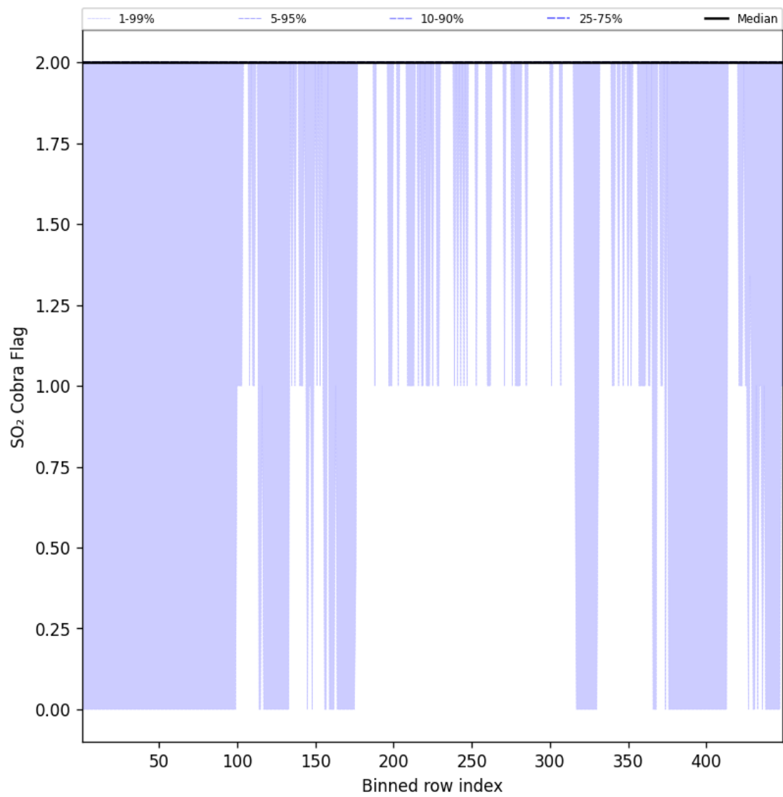
Figure 102: Along track statistics of “SO 2 Cobra Flag” for 2025-05-14 to 2025-05-15
