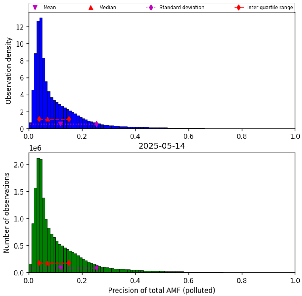
Figure 81: Histogram of “Precision of total AMF (polluted)” for 2025-05-14 to 2025-05-15
