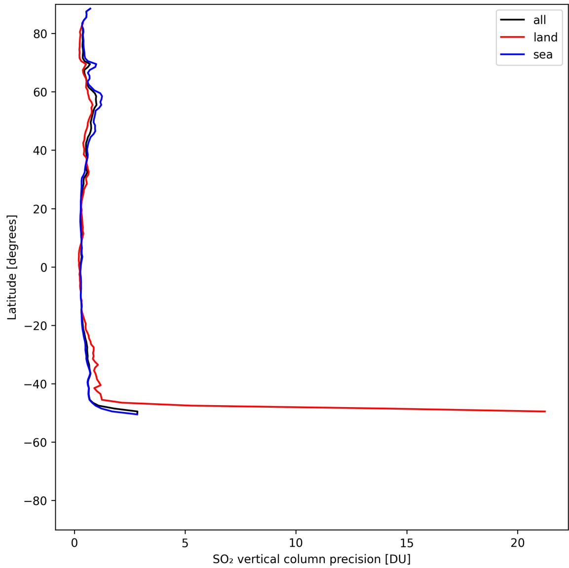
Figure 32: Zonal average of “SO 2 vertical column precision” for 2025-05-14 to 2025-05-15.
