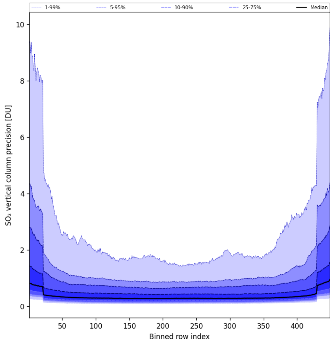
Figure 86: Along track statistics of “SO 2 vertical column precision” for 2025-05-14 to 2025-05-15
