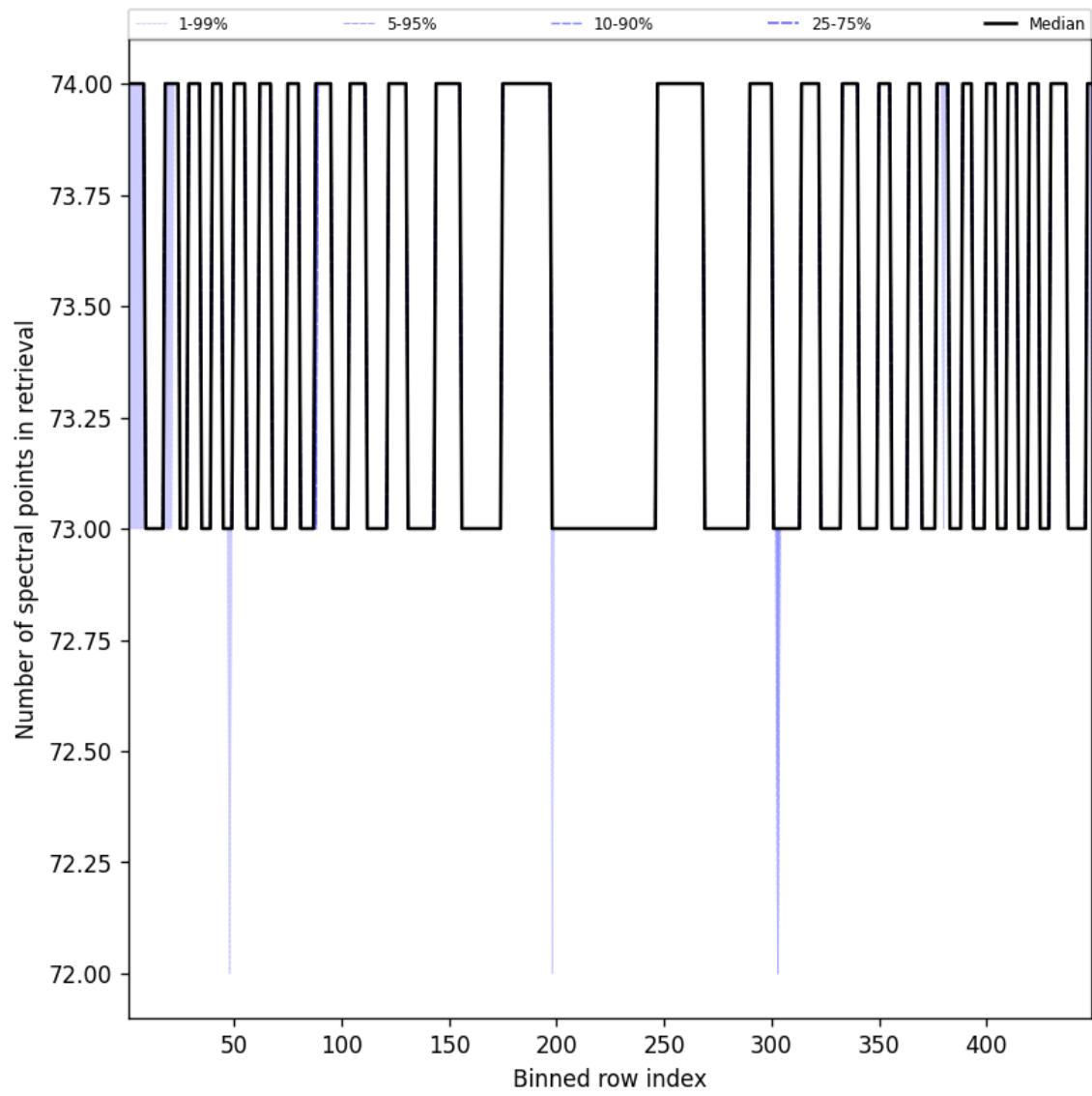
Figure 110: Along track statistics of “Number of spectral points in retrieval” for 2025-05-14 to 2025-05-15
