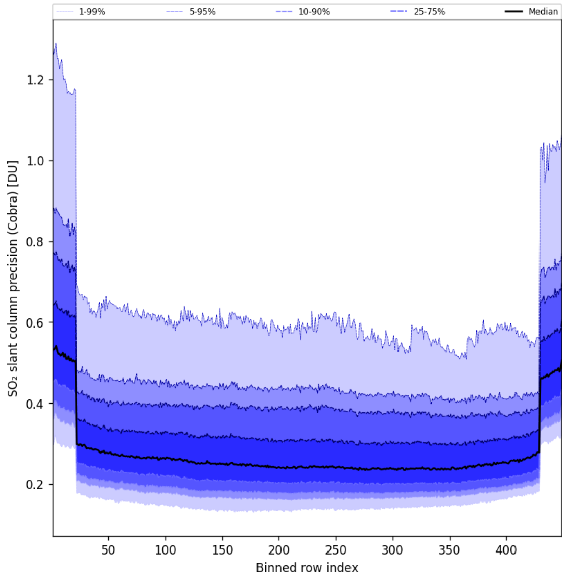
Figure 89: Along track statistics of “SO 2 slant column precision (Cobra)” for 2025-05-14 to 2025-05-15
