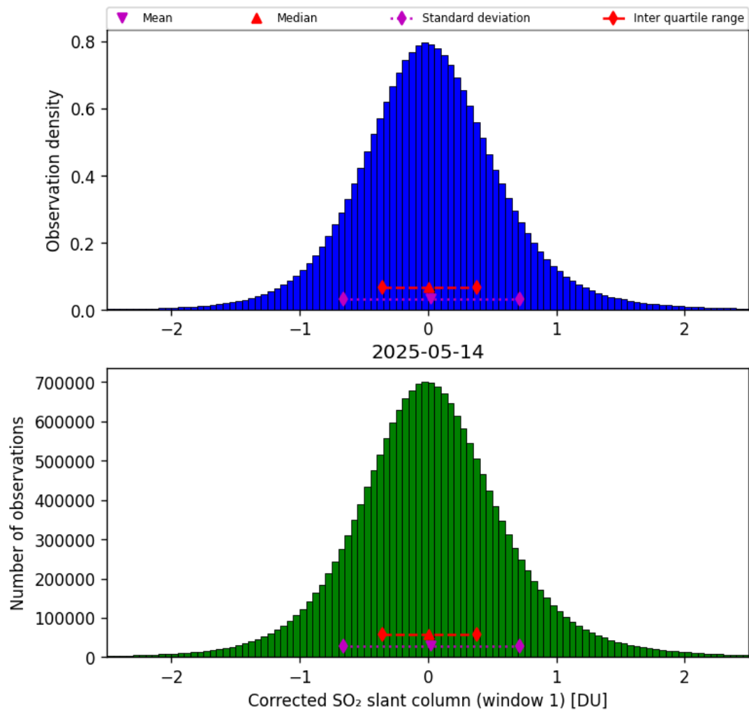
Figure 65: Histogram of “Corrected SO 2 slant column (window 1)” for 2025-05-14 to 2025-05-15
