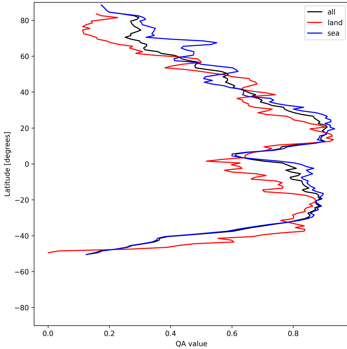
Figure 30: Zonal average of “QA value” for 2025-05-14 to 2025-05-15.
