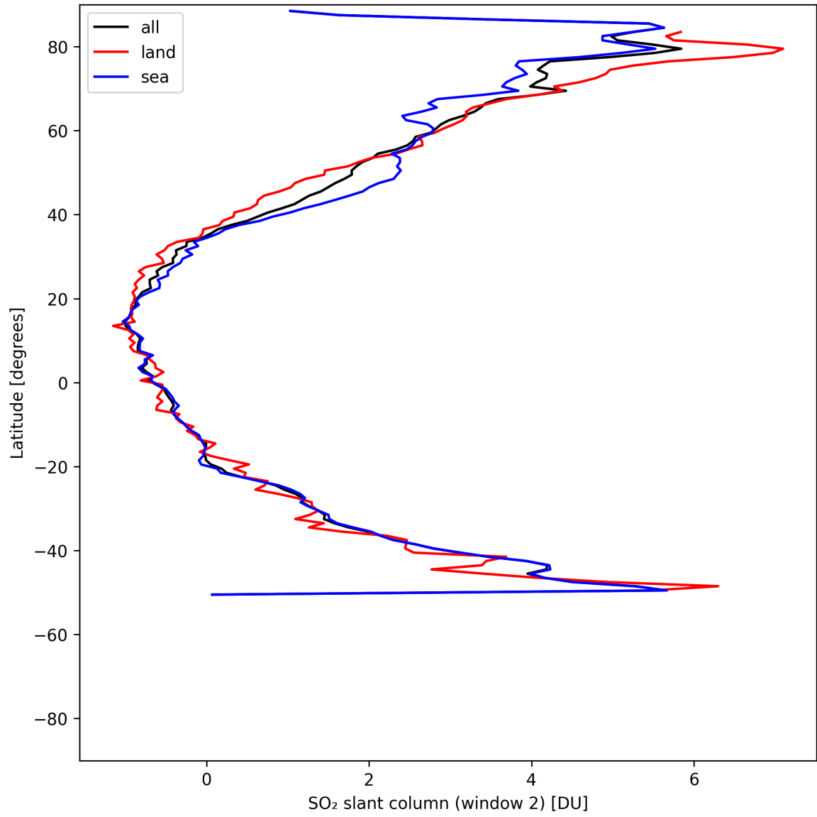
Figure 40: Zonal average of “SO 2 slant column (window 2)” for 2025-05-14 to 2025-05-15.
