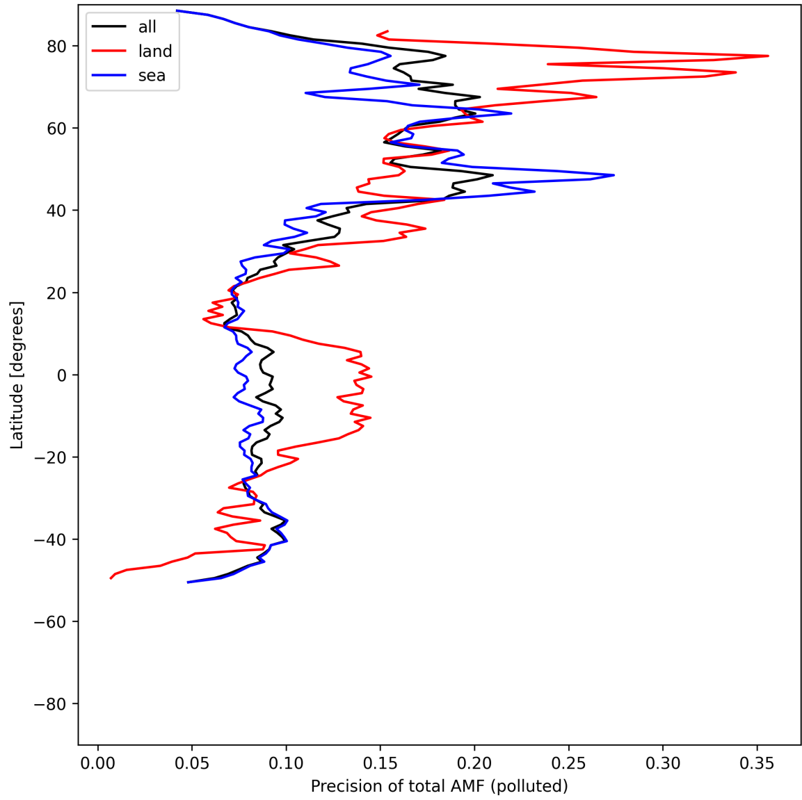
Figure 54: Zonal average of “Precision of total AMF (polluted)” for 2025-05-14 to 2025-05-15.
