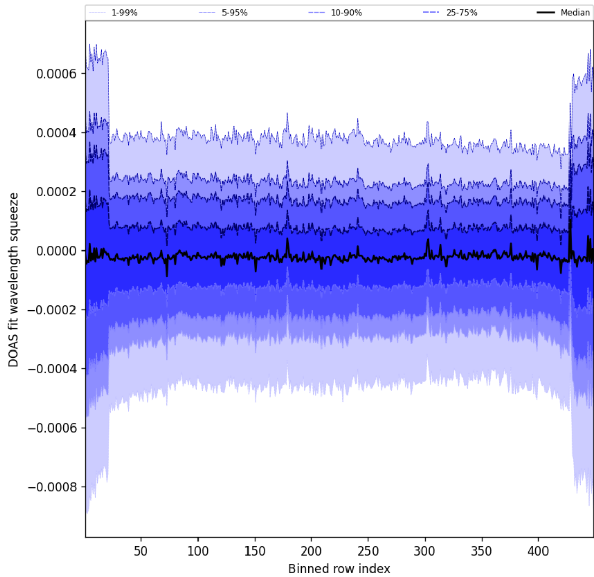
Figure 105: Along track statistics of “DOAS fit wavelength squeeze” for 2025-05-14 to 2025-05-15
