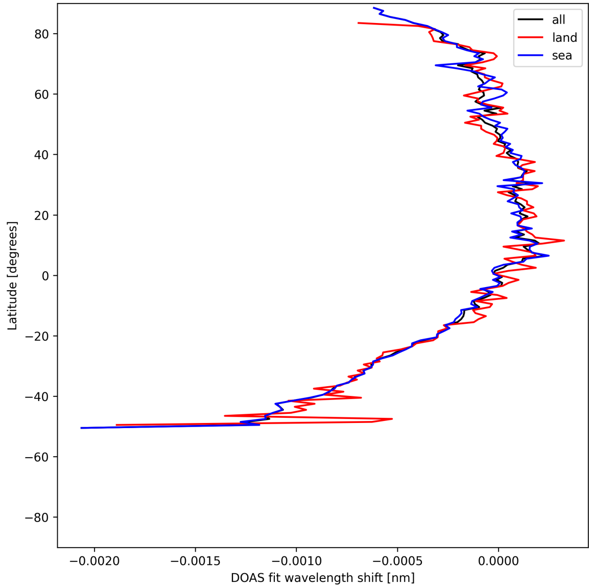
Figure 50: Zonal average of “DOAS fit wavelength shift” for 2025-05-14 to 2025-05-15.
