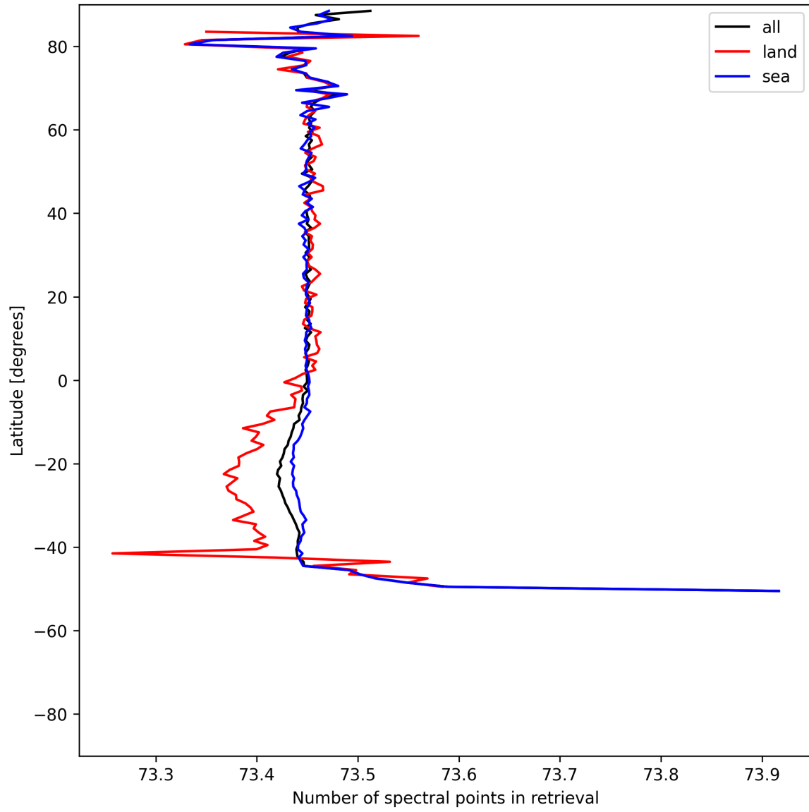
Figure 56: Zonal average of “Number of spectral points in retrieval” for 2025-05-14 to 2025-05-15.
