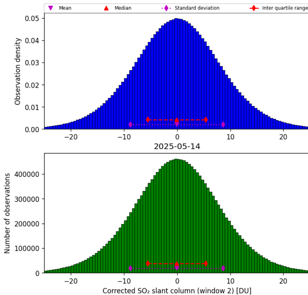
Figure 69: Histogram of “Corrected SO 2 slant column (window 2)” for 2025-05-14 to 2025-05-15
