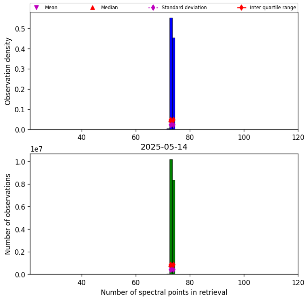
Figure 83: Histogram of “Number of spectral points in retrieval” for 2025-05-14 to 2025-05-15
