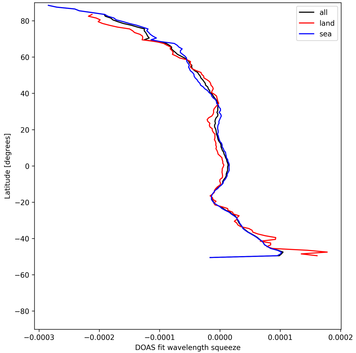
Figure 51: Zonal average of “DOAS fit wavelength squeeze” for 2025-05-14 to 2025-05-15.
