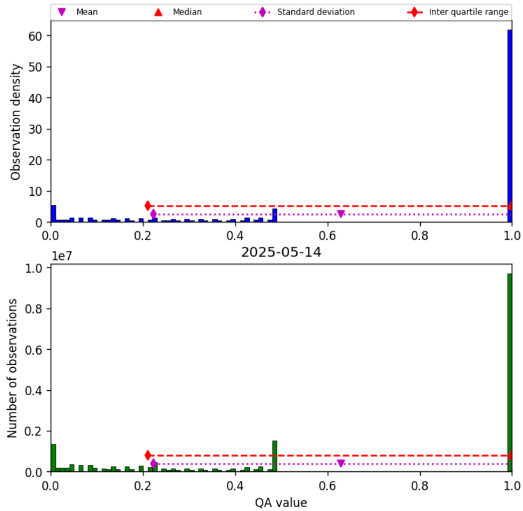
Figure 57: Histogram of “QA value” for 2025-05-14 to 2025-05-15
