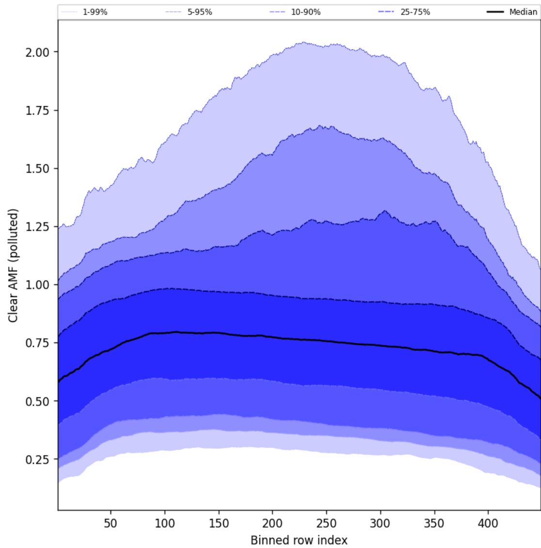
Figure 109: Along track statistics of “Clear AMF (polluted)” for 2025-05-14 to 2025-05-15
