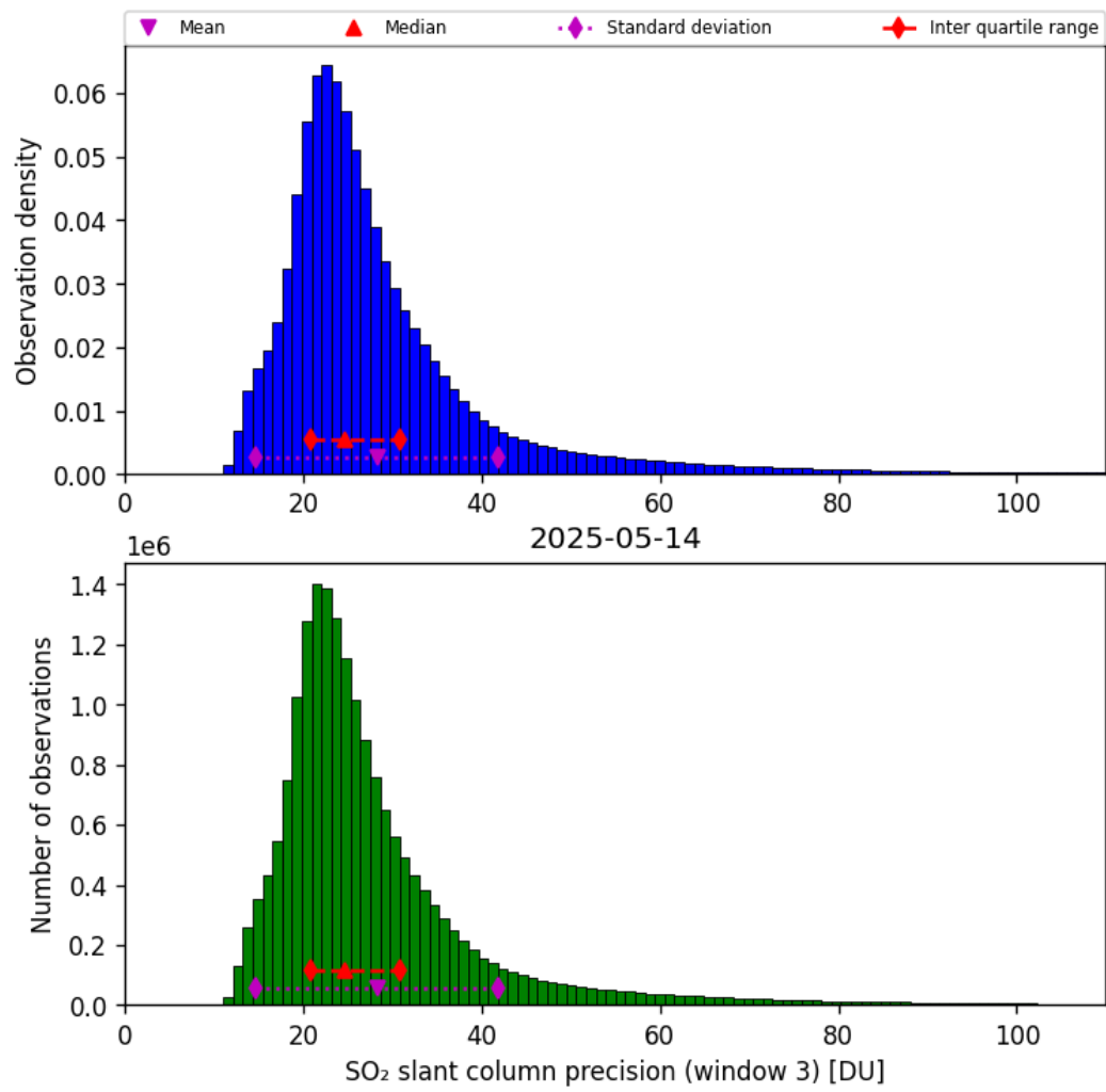
Figure 72: Histogram of “SO 2 slant column precision (window 3)” for 2025-05-14 to 2025-05-15
