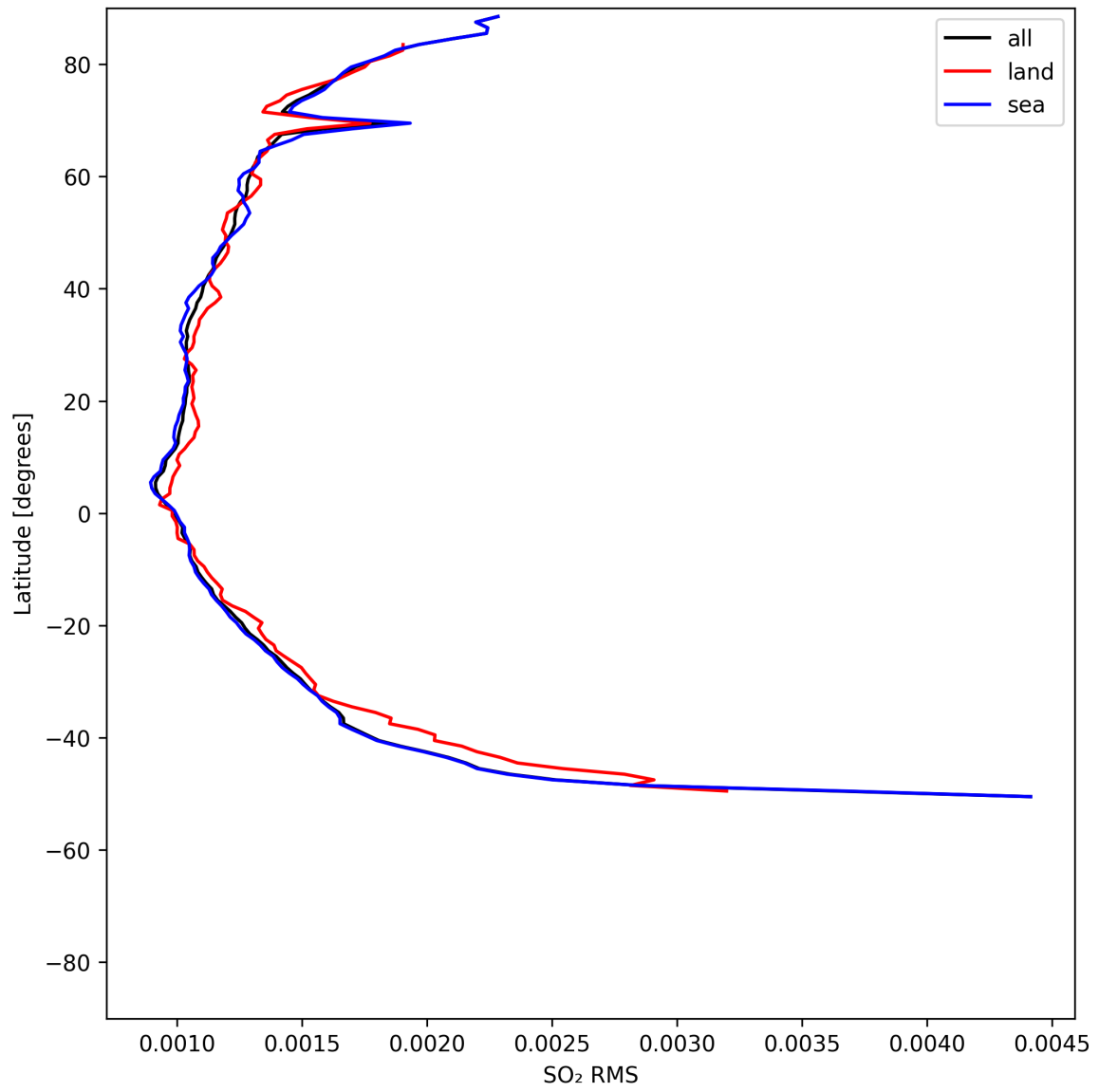
Figure 52: Zonal average of “SO 2 RMS” for 2025-05-14 to 2025-05-15.
