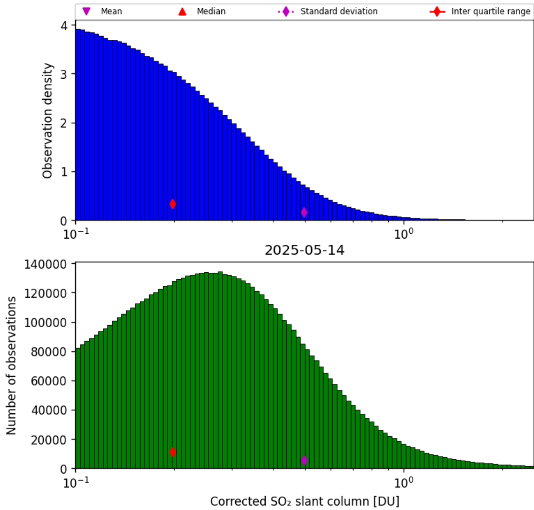
Figure 60: Histogram of “Corrected SO 2 slant column” for 2025-05-14 to 2025-05-15
