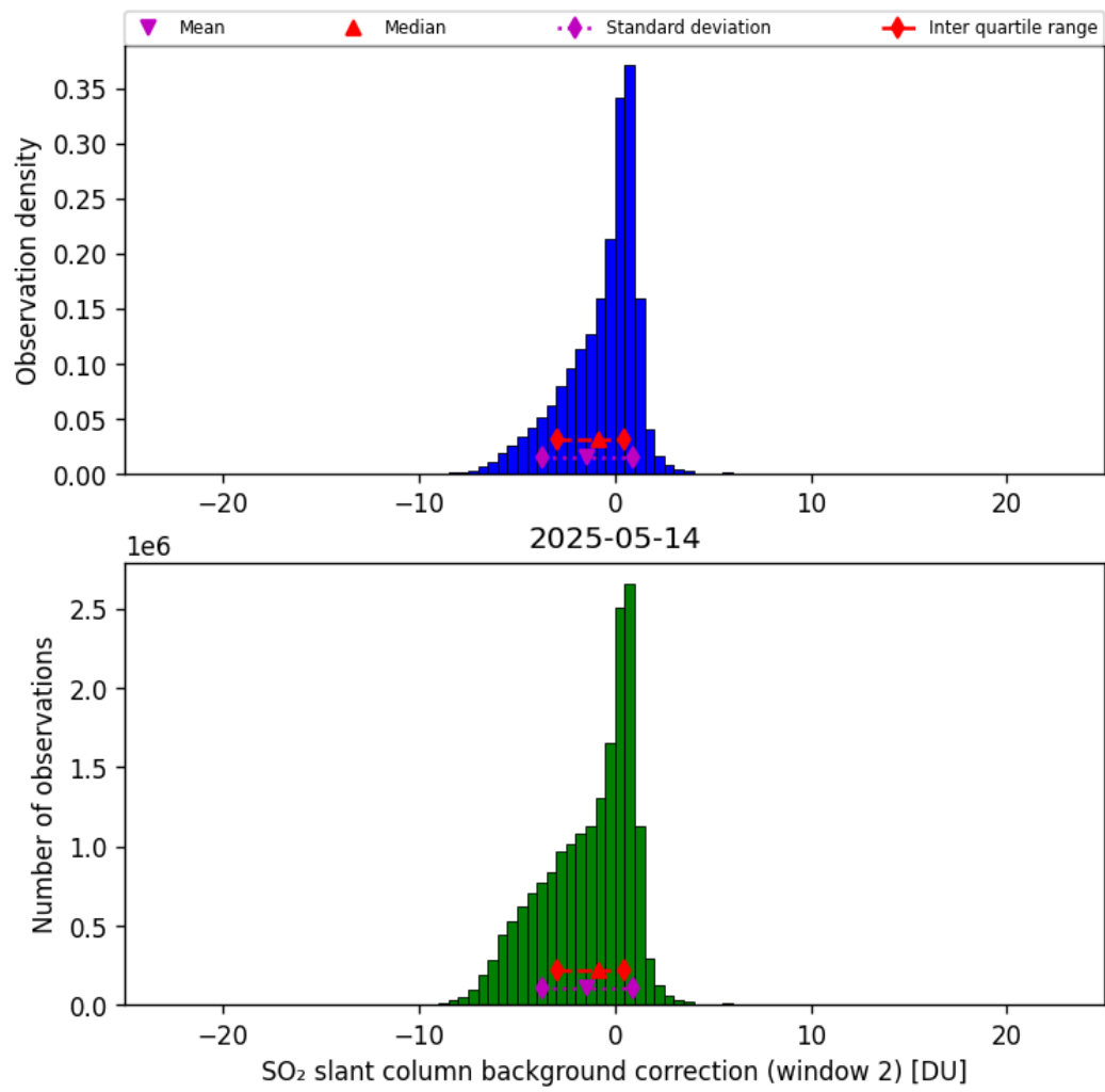
Figure 70: Histogram of “SO 2 slant column background correction (window 2)” for 2025-05-14 to 2025-05-15
