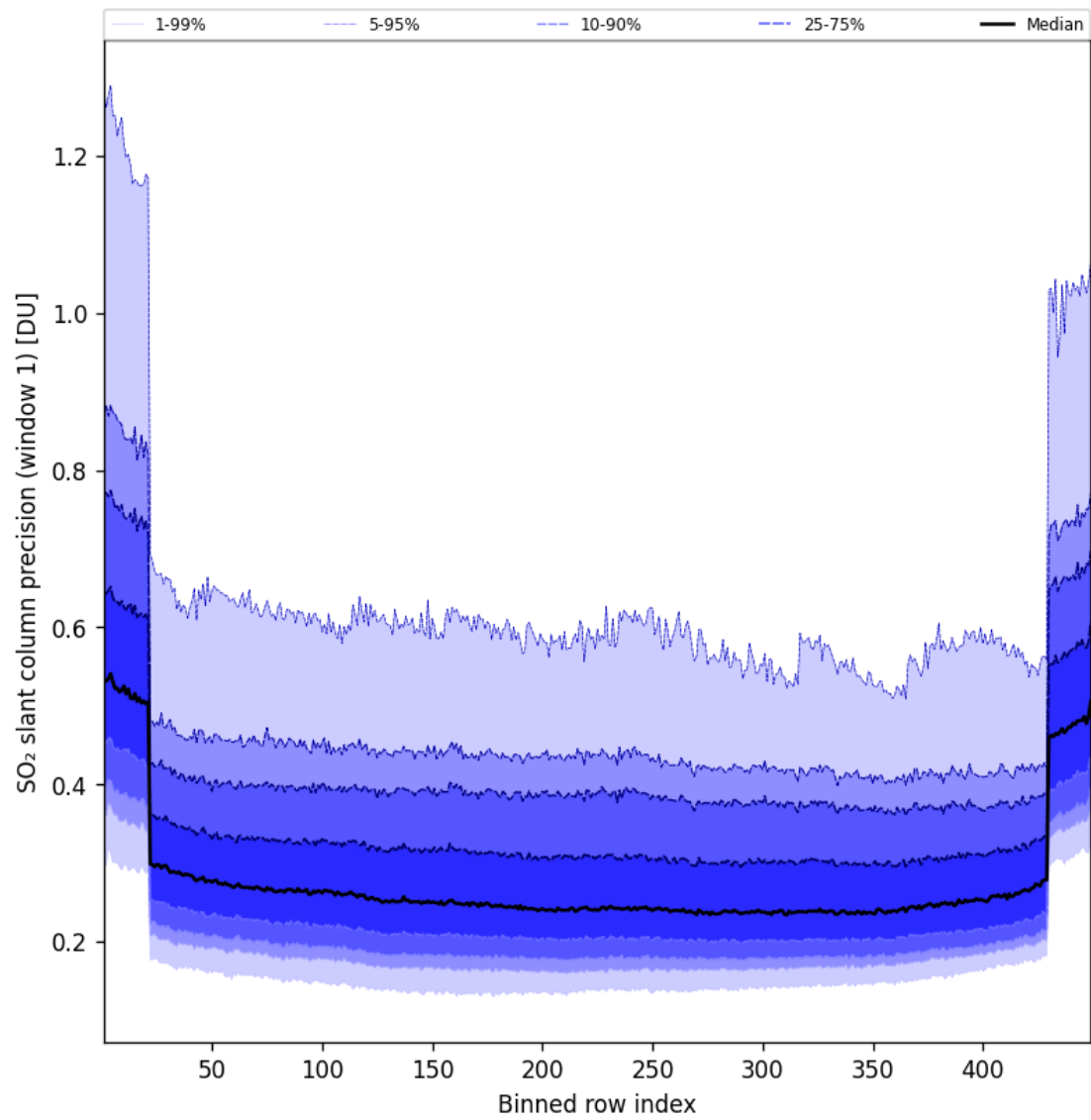
Figure 91: Along track statistics of “SO 2 slant column precision (window 1)” for 2025-05-14 to 2025-05-15
