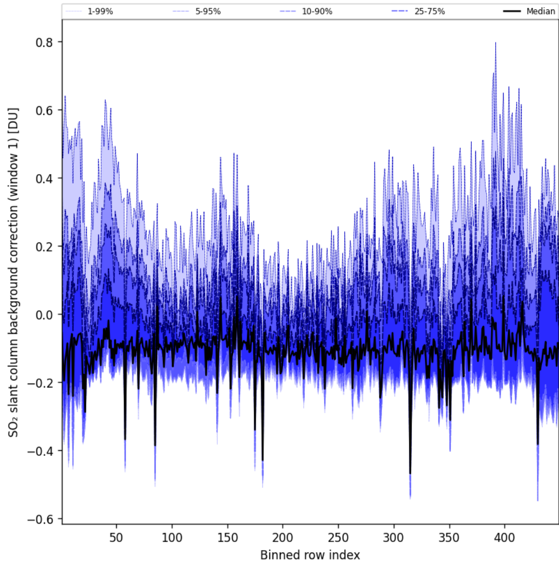
Figure 93: Along track statistics of “SO 2 slant column background correction (window 1)” for 2025-05-14 to 2025-05-15
