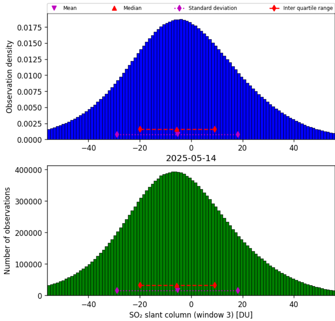
Figure 71: Histogram of “SO 2 slant column (window 3)” for 2025-05-14 to 2025-05-15
