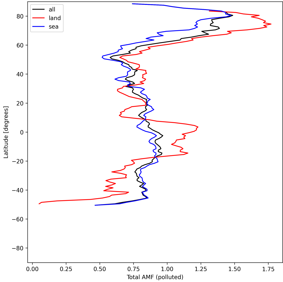
Figure 53: Zonal average of “Total AMF (polluted)” for 2025-05-14 to 2025-05-15.
