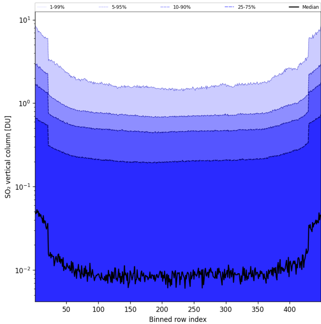
Figure 85: Along track statistics of “SO 2 vertical column” for 2025-05-14 to 2025-05-15
