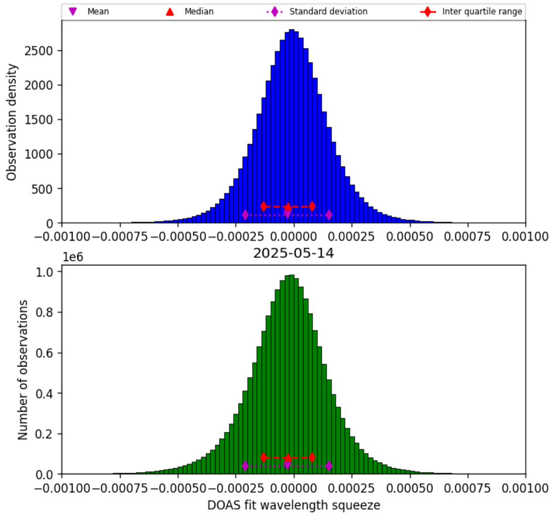
Figure 78: Histogram of “DOAS fit wavelength squeeze” for 2025-05-14 to 2025-05-15
