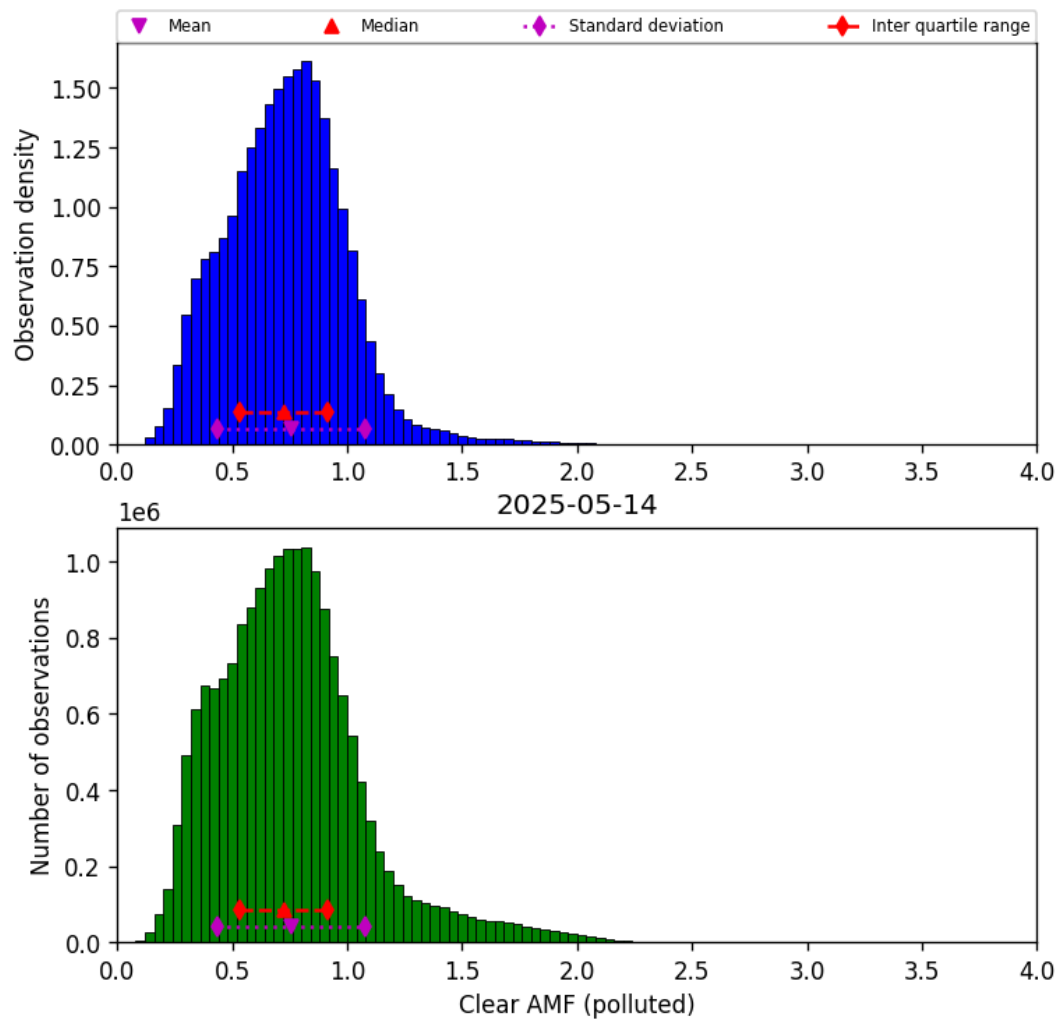
Figure 82: Histogram of “Clear AMF (polluted)” for 2025-05-14 to 2025-05-15
