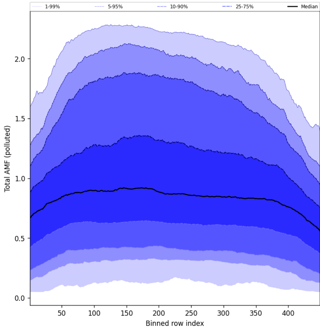
Figure 107: Along track statistics of “Total AMF (polluted)” for 2025-05-14 to 2025-05-15
