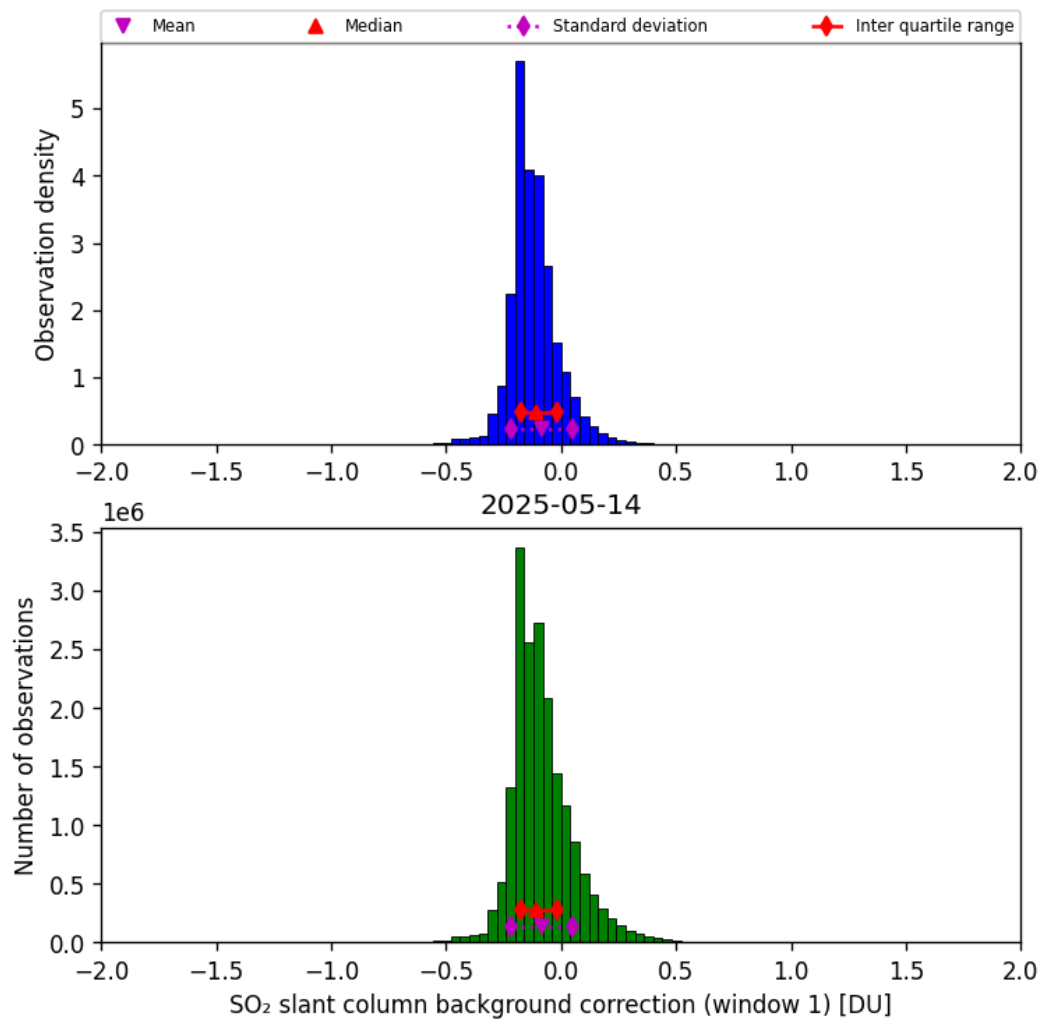
Figure 66: Histogram of “SO 2 slant column background correction (window 1)” for 2025-05-14 to 2025-05-15
