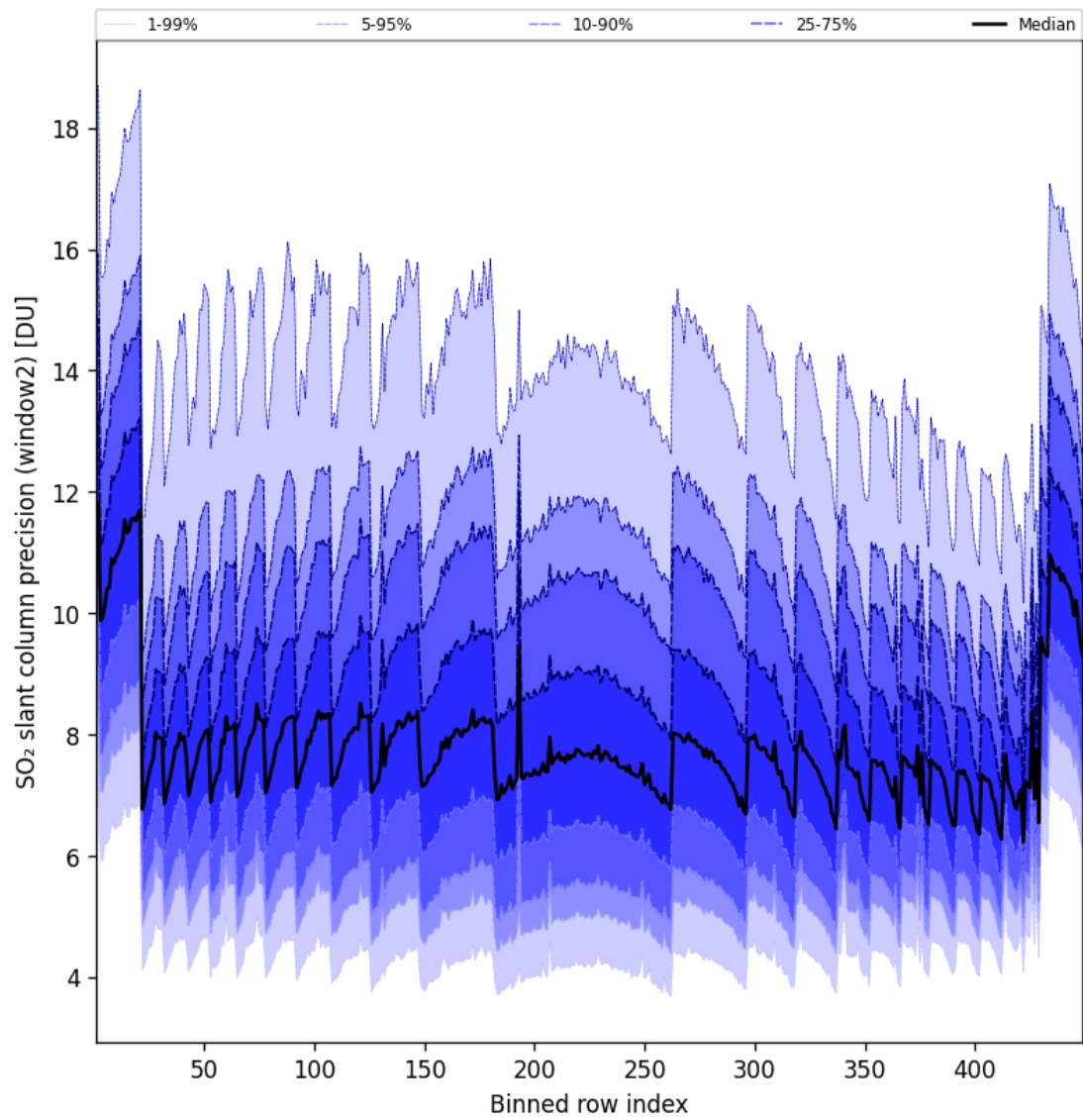
Figure 95: Along track statistics of “SO 2 slant column precision (window2)” for 2025-05-14 to 2025-05-15
