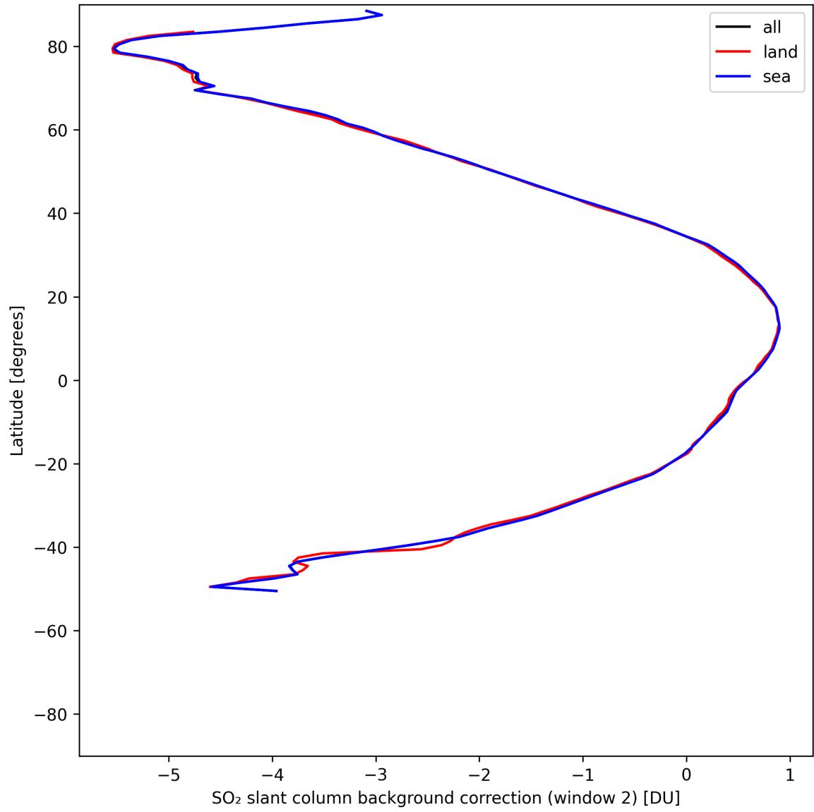
Figure 43: Zonal average of “SO 2 slant column background correction (window 2)” for 2025-05-14 to 2025-05-15.
