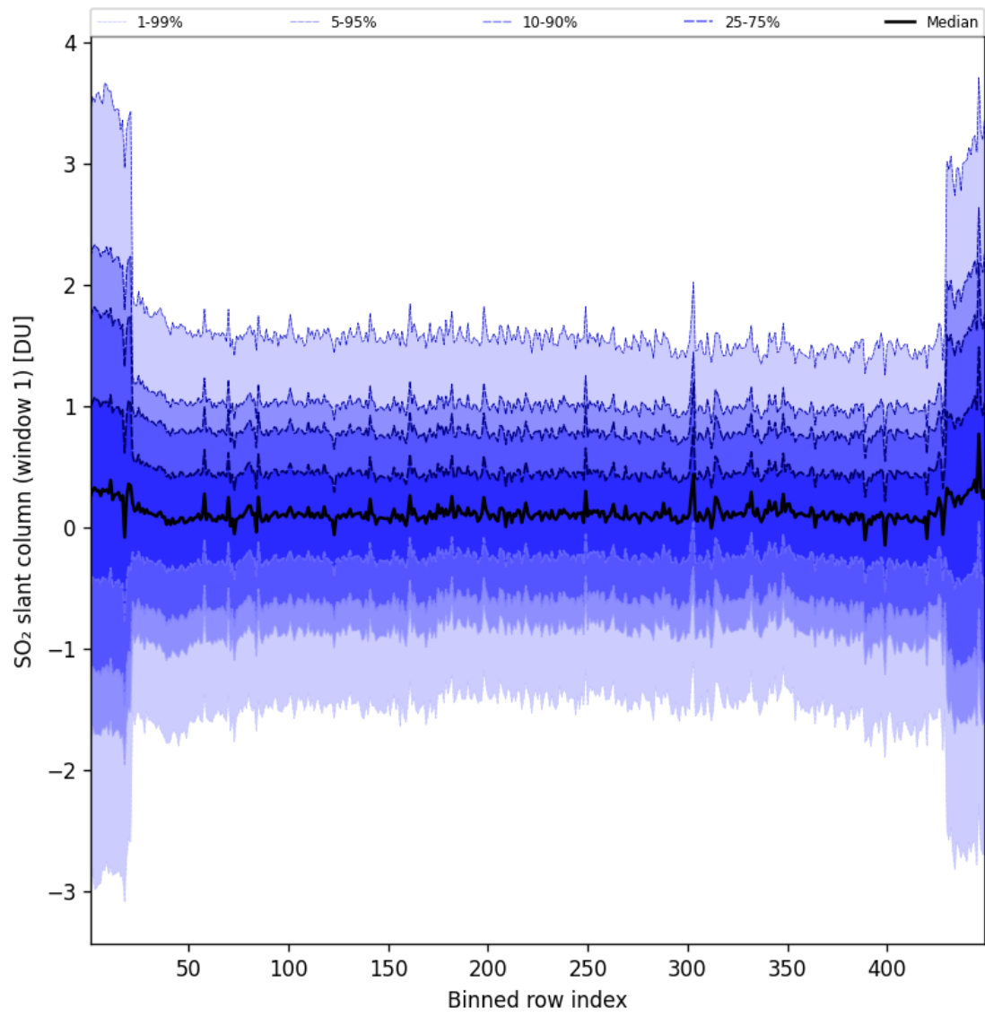
Figure 90: Along track statistics of “SO 2 slant column (window 1)” for 2025-05-14 to 2025-05-15
