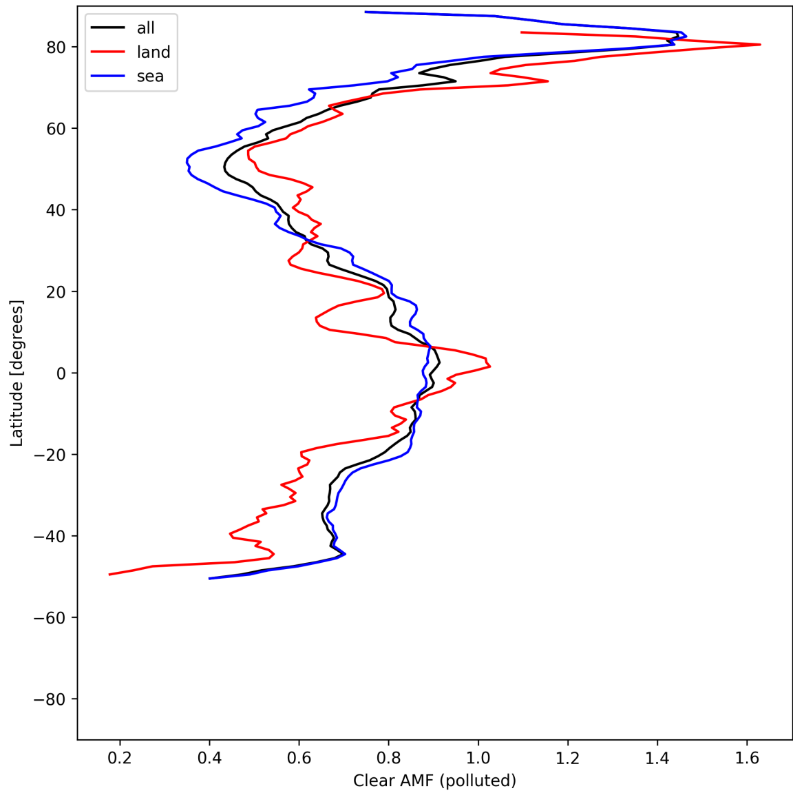
Figure 55: Zonal average of “Clear AMF (polluted)” for 2025-05-14 to 2025-05-15.
