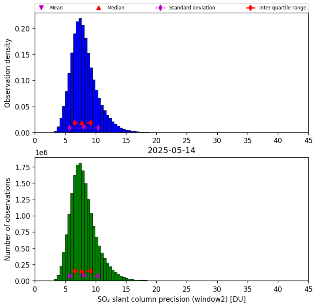
Figure 68: Histogram of “SO 2 slant column precision (window2)” for 2025-05-14 to 2025-05-15
