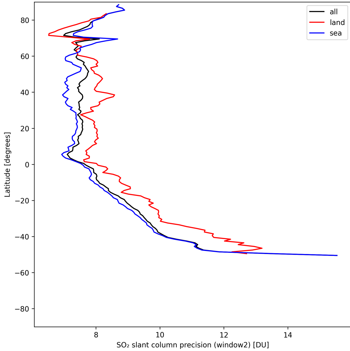
Figure 41: Zonal average of “SO 2 slant column precision (window2)” for 2025-05-14 to 2025-05-15.
