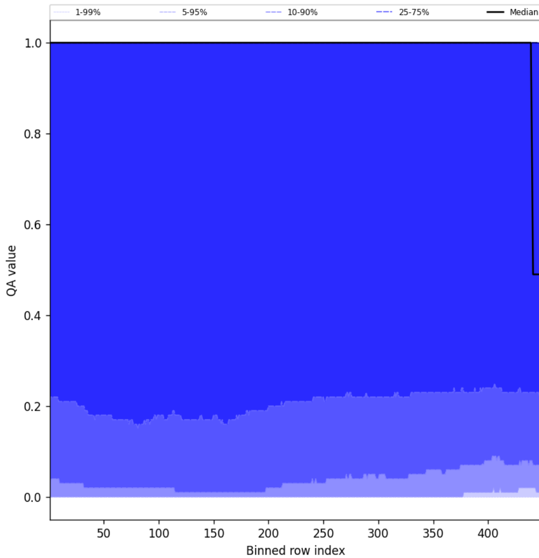
Figure 84: Along track statistics of “QA value” for 2025-05-14 to 2025-05-15
