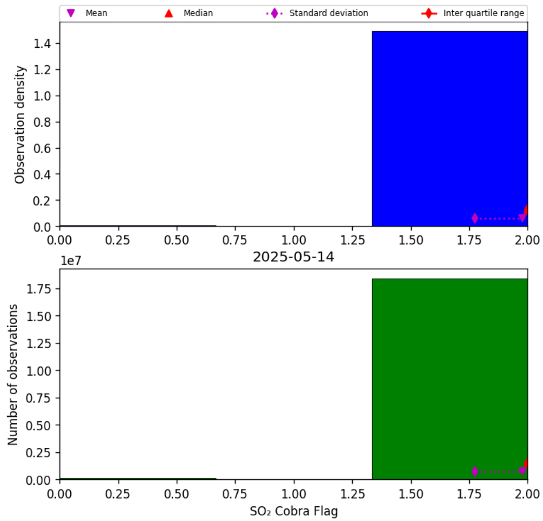
Figure 75: Histogram of “SO 2 Cobra Flag” for 2025-05-14 to 2025-05-15
