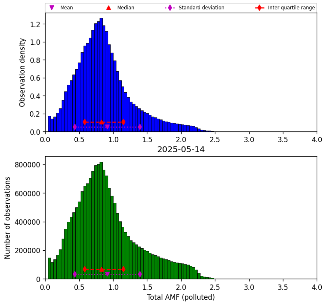
Figure 80: Histogram of “Total AMF (polluted)” for 2025-05-14 to 2025-05-15
