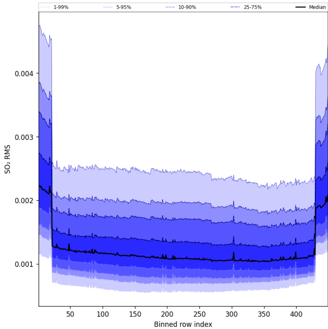
Figure 106: Along track statistics of “SO 2 RMS” for 2025-05-14 to 2025-05-15
