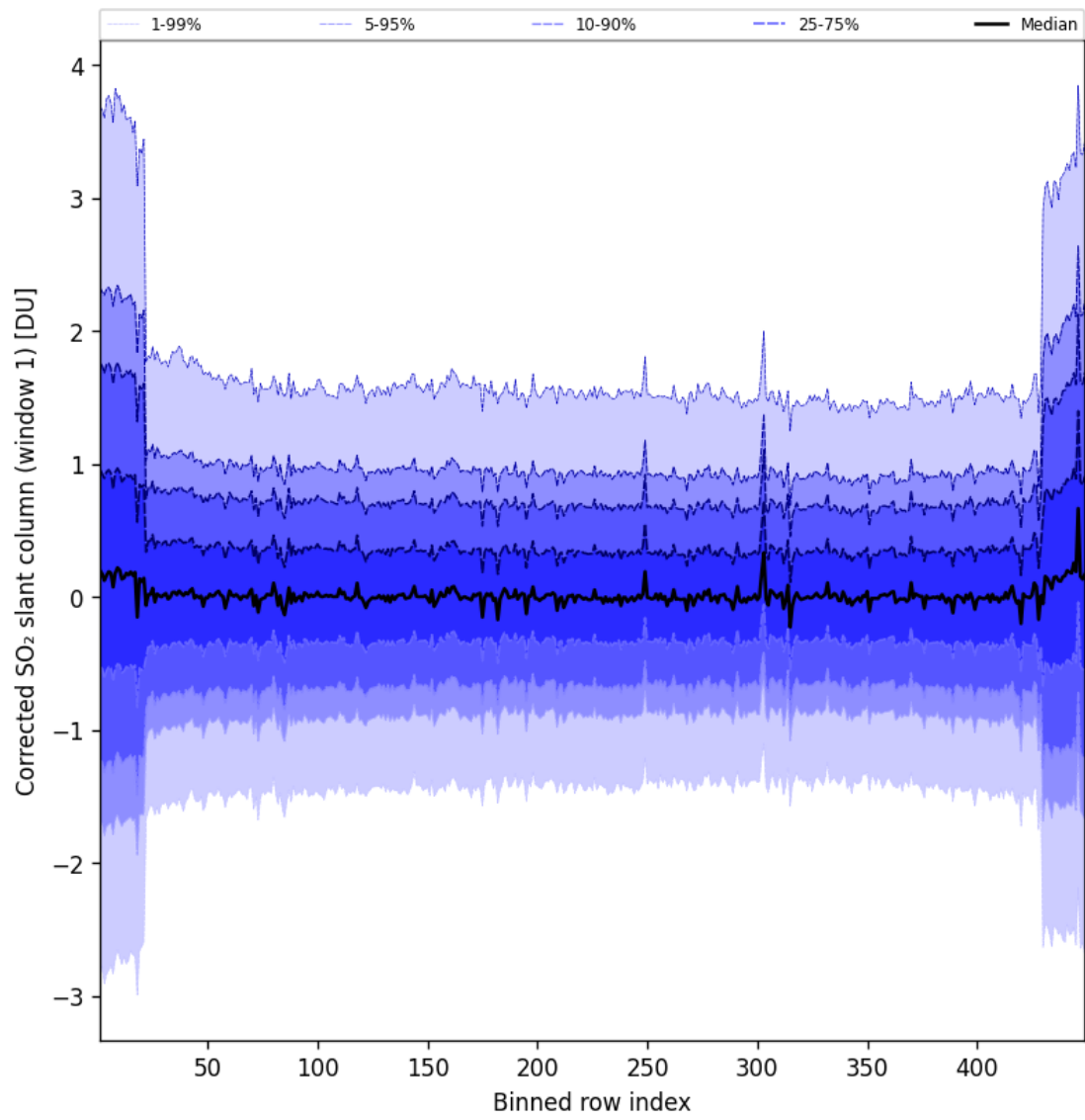
Figure 92: Along track statistics of “Corrected SO 2 slant column (window 1)” for 2025-05-14 to 2025-05-15
