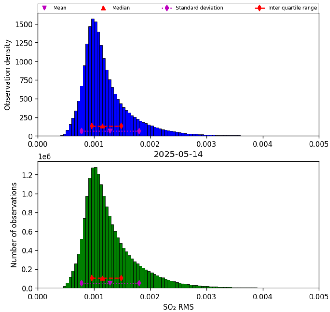
Figure 79: Histogram of “SO 2 RMS” for 2025-05-14 to 2025-05-15
