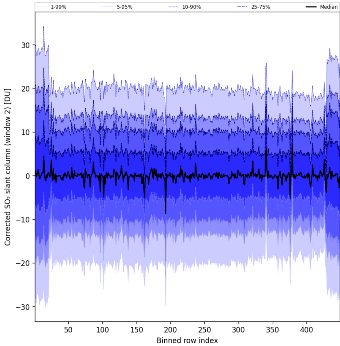
Figure 96: Along track statistics of “Corrected SO 2 slant column (window 2)” for 2025-05-14 to 2025-05-15
