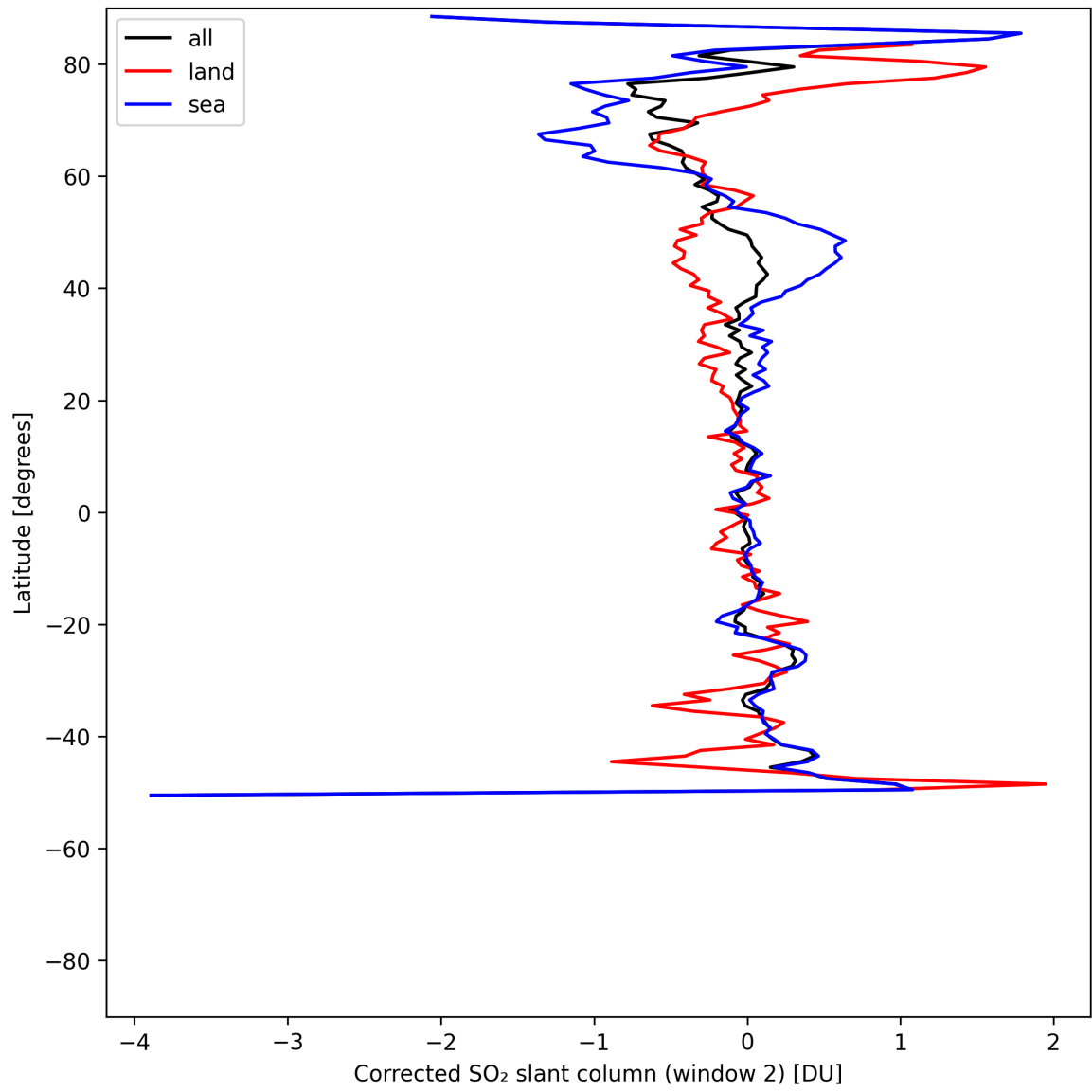
Figure 42: Zonal average of “Corrected SO 2 slant column (window 2)” for 2025-05-14 to 2025-05-15.
