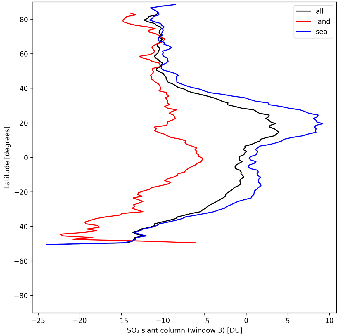
Figure 44: Zonal average of “SO 2 slant column (window 3)” for 2025-05-14 to 2025-05-15.
