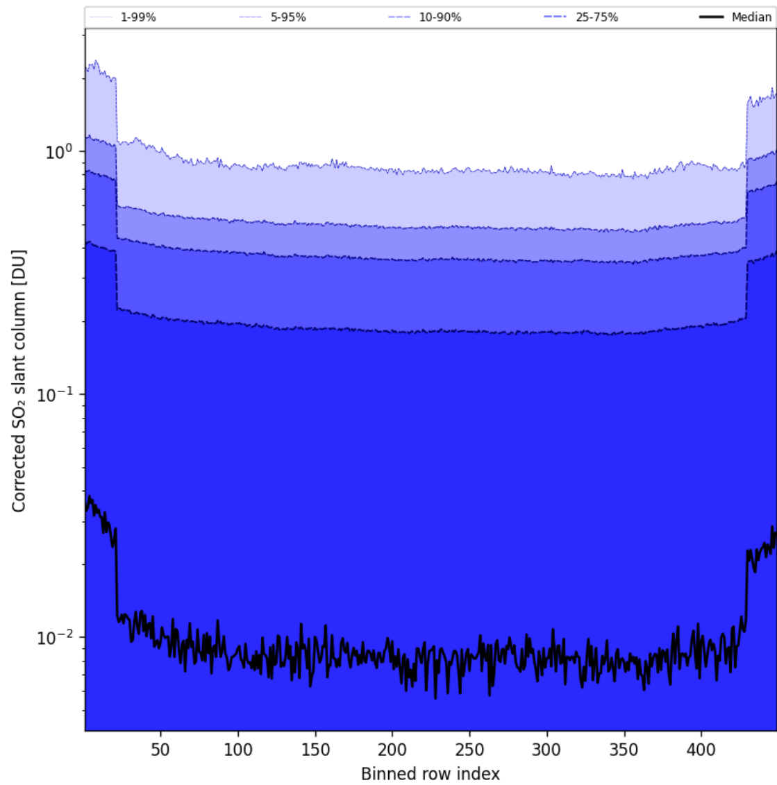
Figure 87: Along track statistics of “Corrected SO 2 slant column” for 2025-05-14 to 2025-05-15
