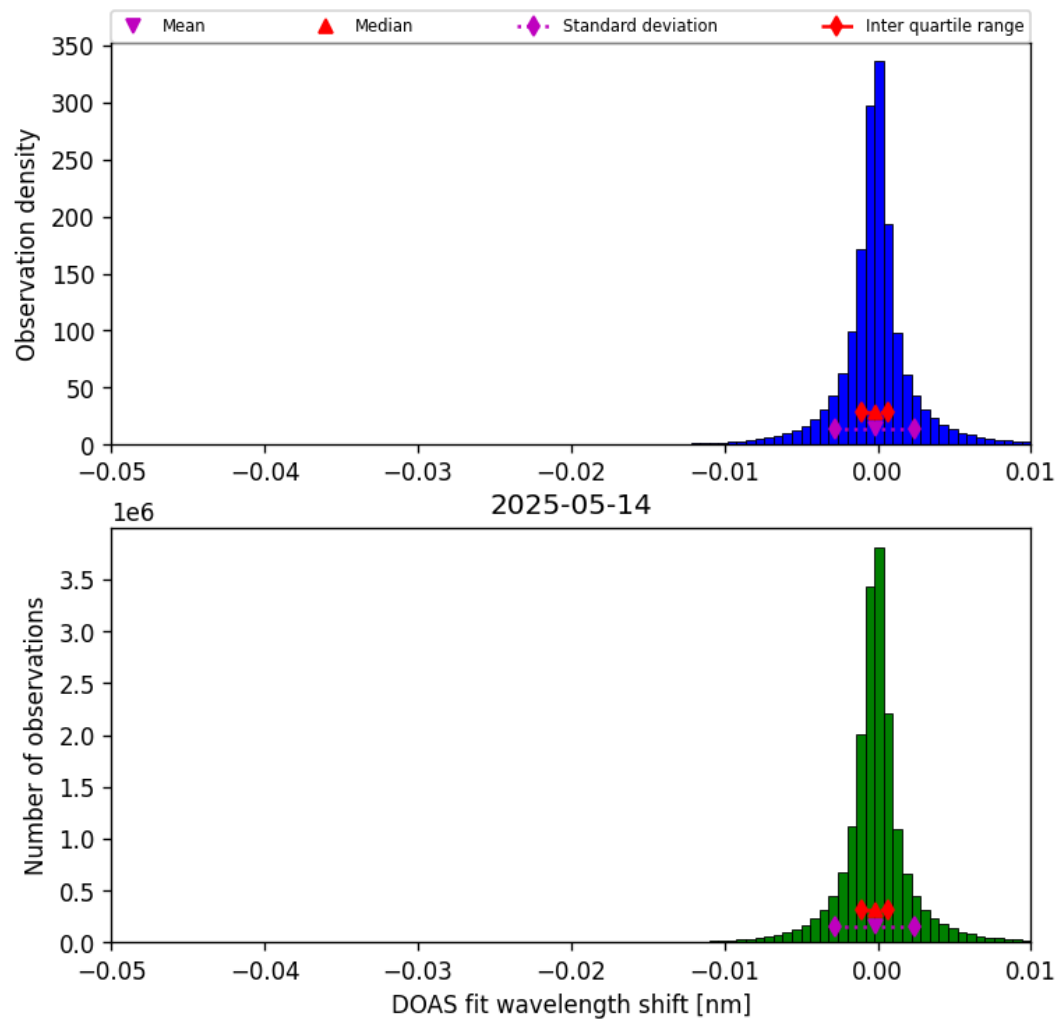
Figure 77: Histogram of “DOAS fit wavelength shift” for 2025-05-14 to 2025-05-15
