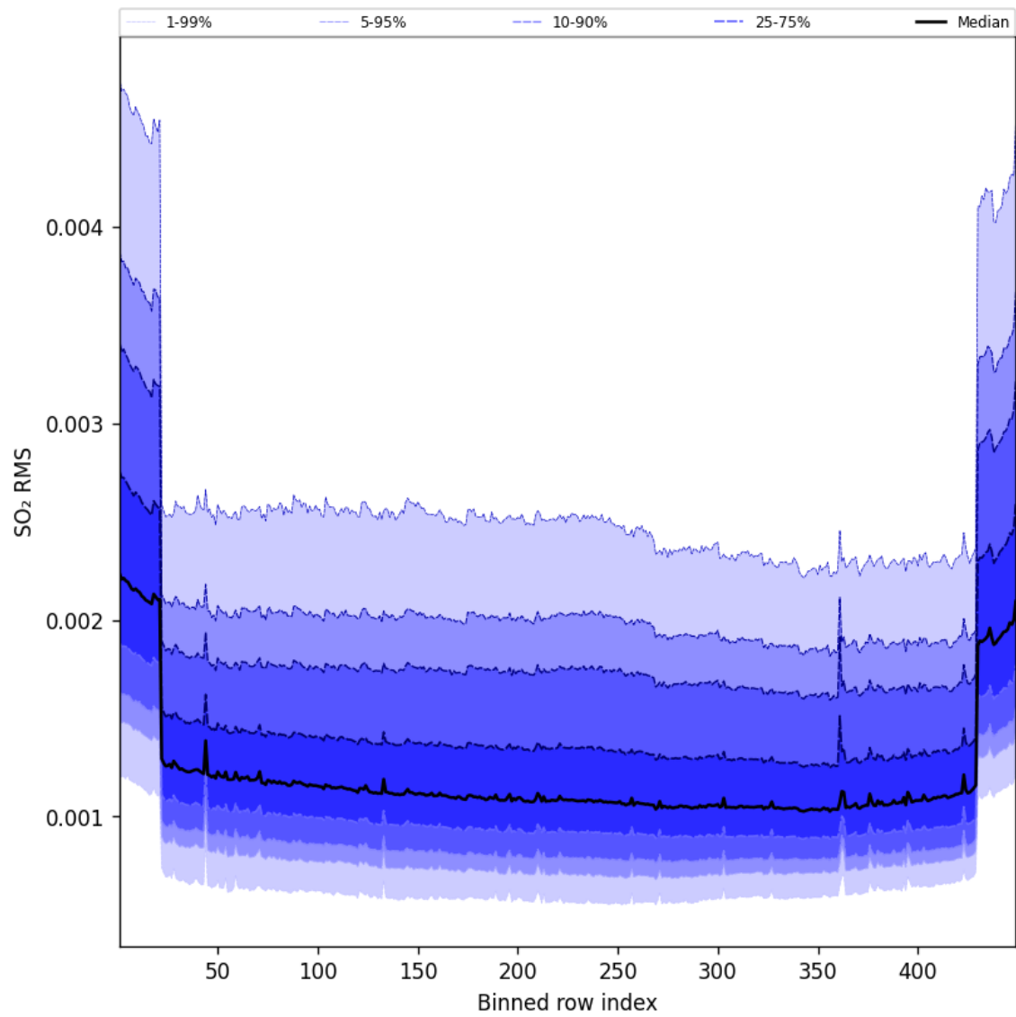
Figure 106: Along track statistics of “SO 2 RMS” for 2025-05-17 to 2025-05-18
