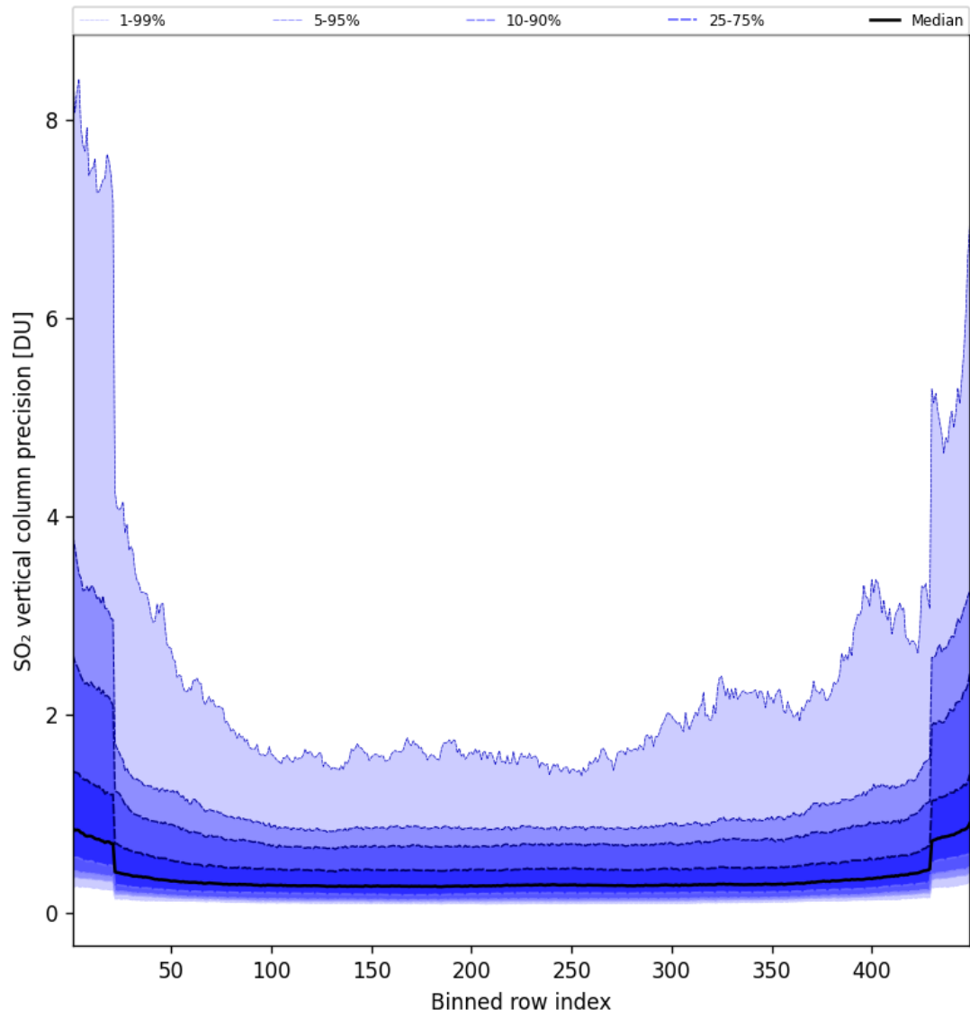
Figure 86: Along track statistics of “SO 2 vertical column precision” for 2025-05-17 to 2025-05-18
