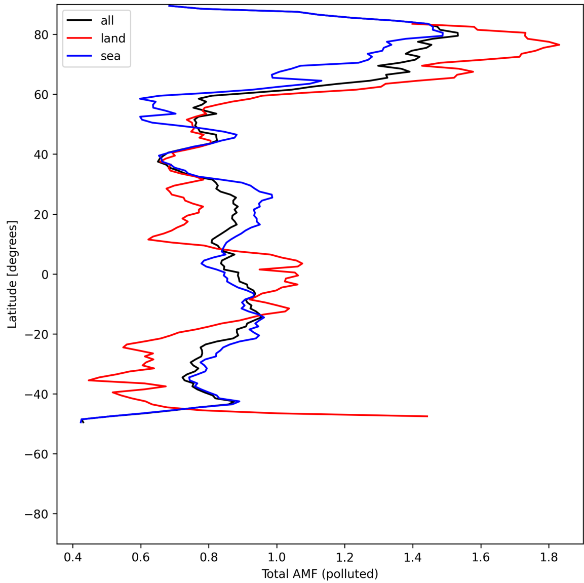
Figure 53: Zonal average of “Total AMF (polluted)” for 2025-05-17 to 2025-05-18.
