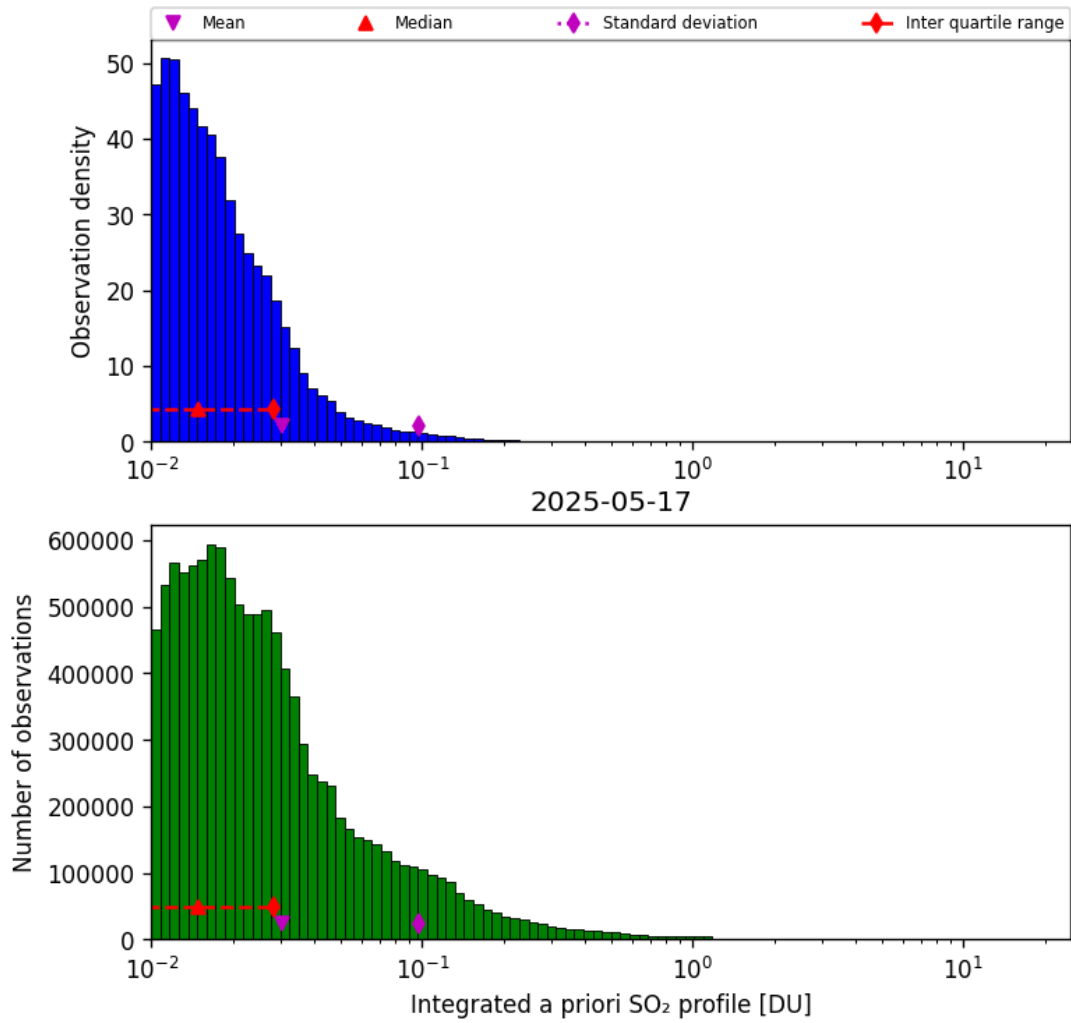
Figure 76: Histogram of “Integrated a priori SO 2 profile” for 2025-05-17 to 2025-05-18
