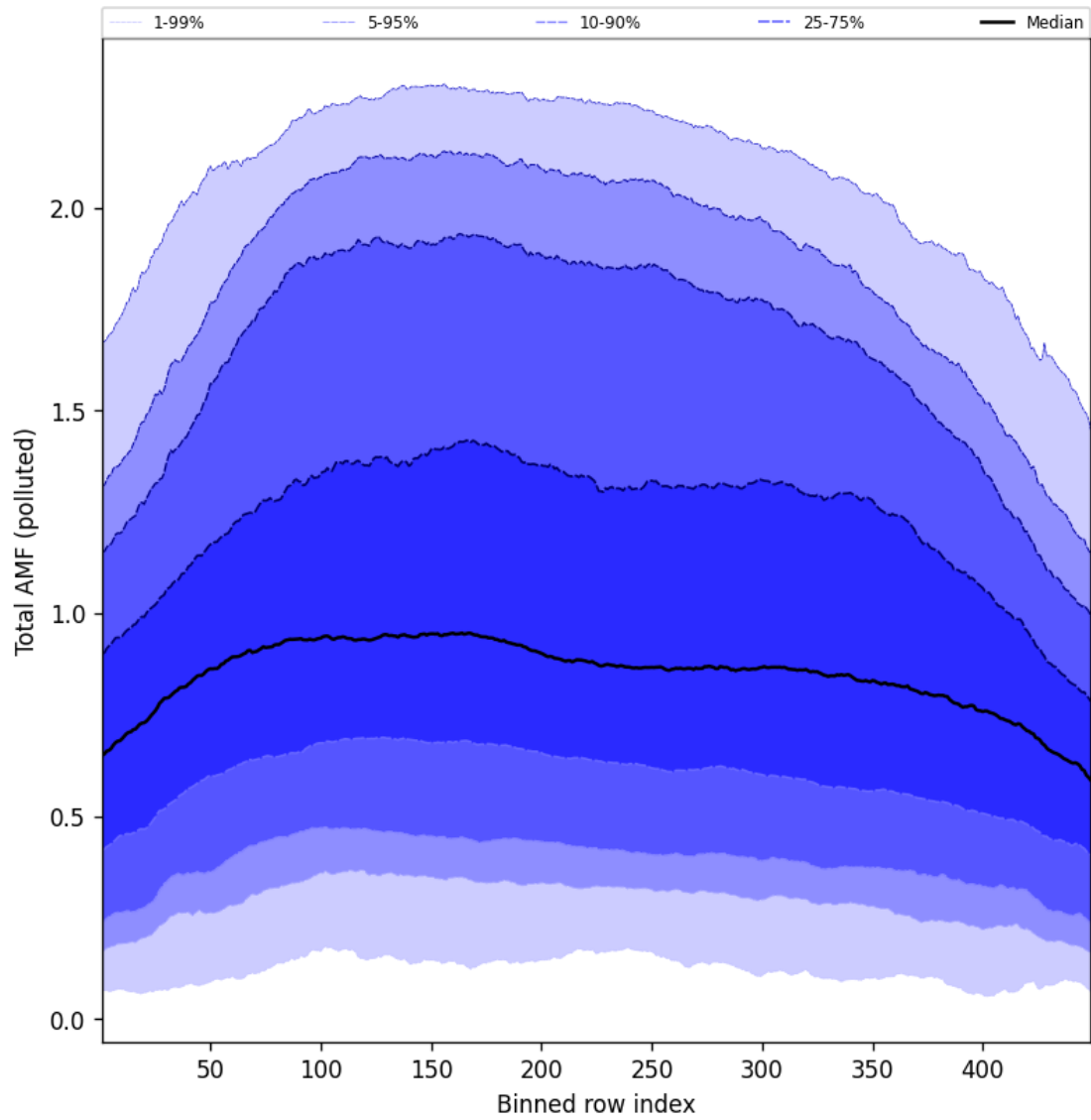
Figure 107: Along track statistics of “Total AMF (polluted)” for 2025-05-17 to 2025-05-18
