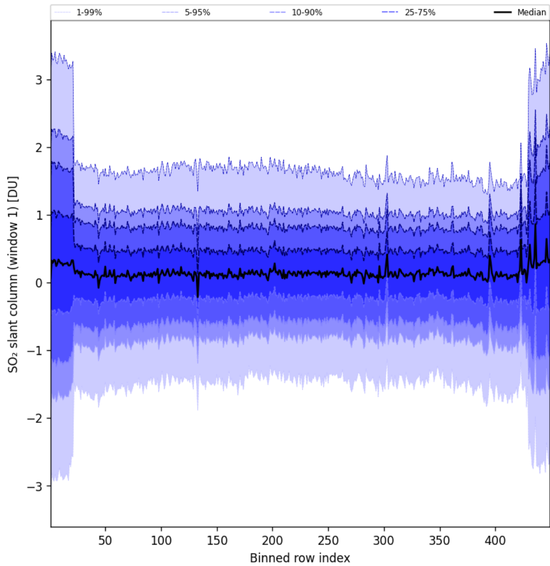
Figure 90: Along track statistics of “SO 2 slant column (window 1)” for 2025-05-17 to 2025-05-18
