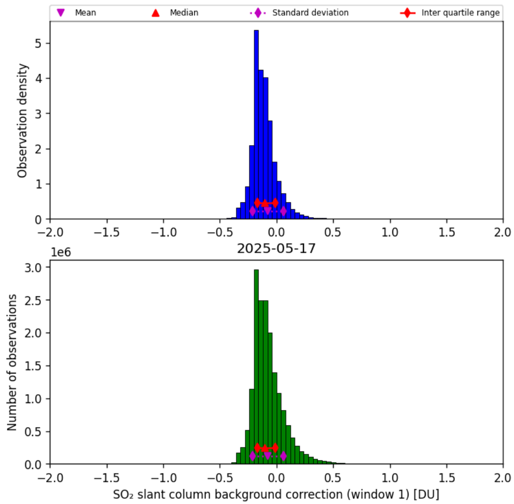
Figure 66: Histogram of “SO 2 slant column background correction (window 1)” for 2025-05-17 to 2025-05-18
