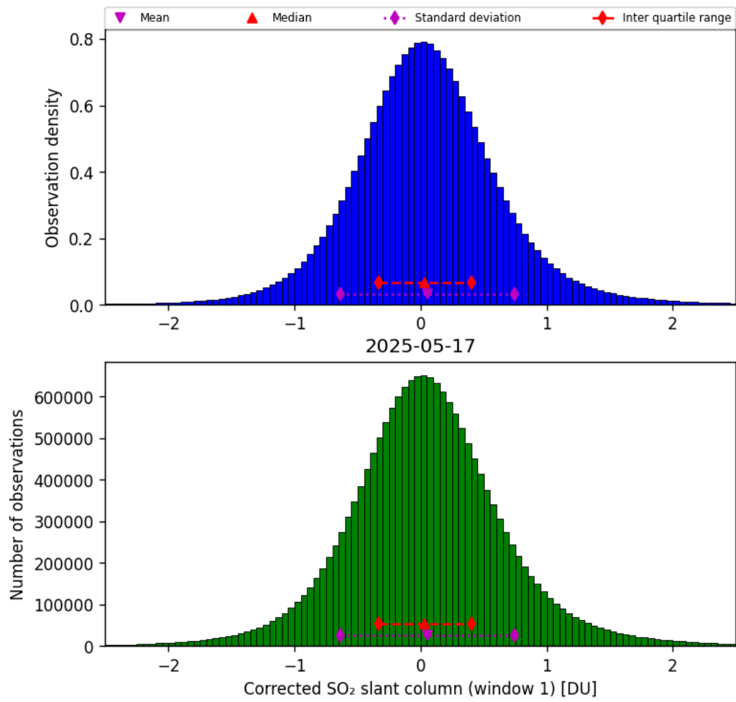
Figure 65: Histogram of “Corrected SO 2 slant column (window 1)” for 2025-05-17 to 2025-05-18
