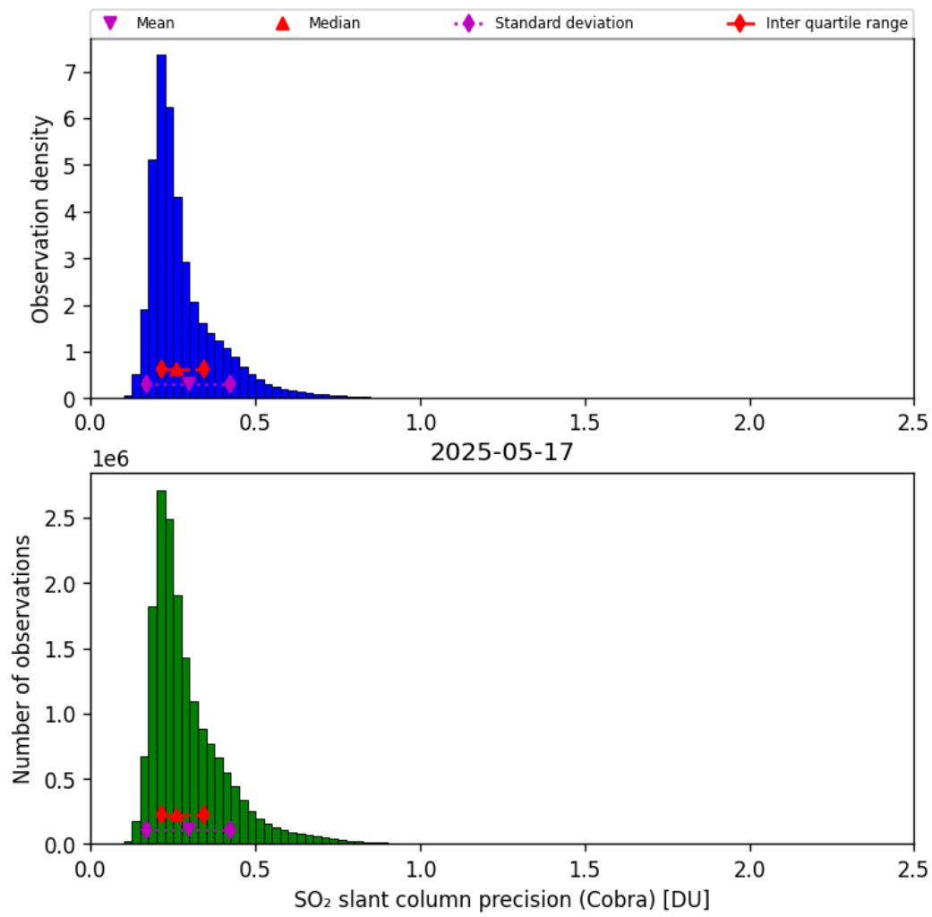
Figure 62: Histogram of “SO 2 slant column precision (Cobra)” for 2025-05-17 to 2025-05-18
