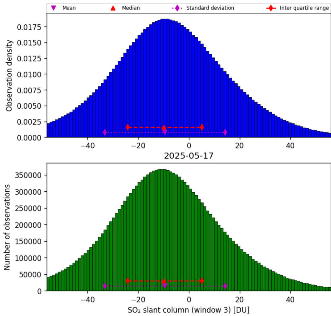
Figure 71: Histogram of “SO 2 slant column (window 3)” for 2025-05-17 to 2025-05-18
