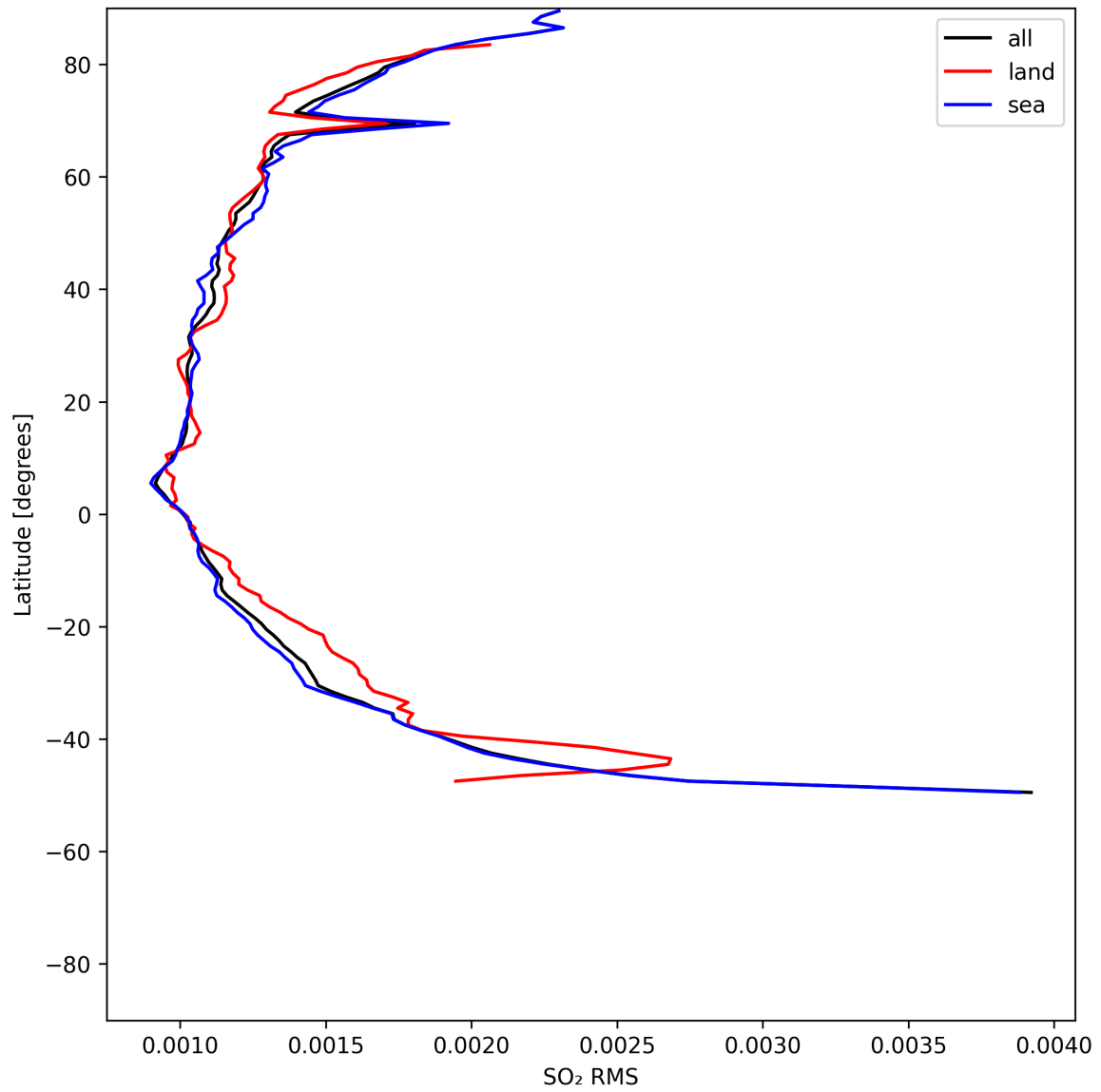
Figure 52: Zonal average of “SO 2 RMS” for 2025-05-17 to 2025-05-18.
