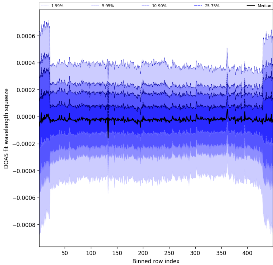
Figure 105: Along track statistics of “DOAS fit wavelength squeeze” for 2025-05-17 to 2025-05-18
