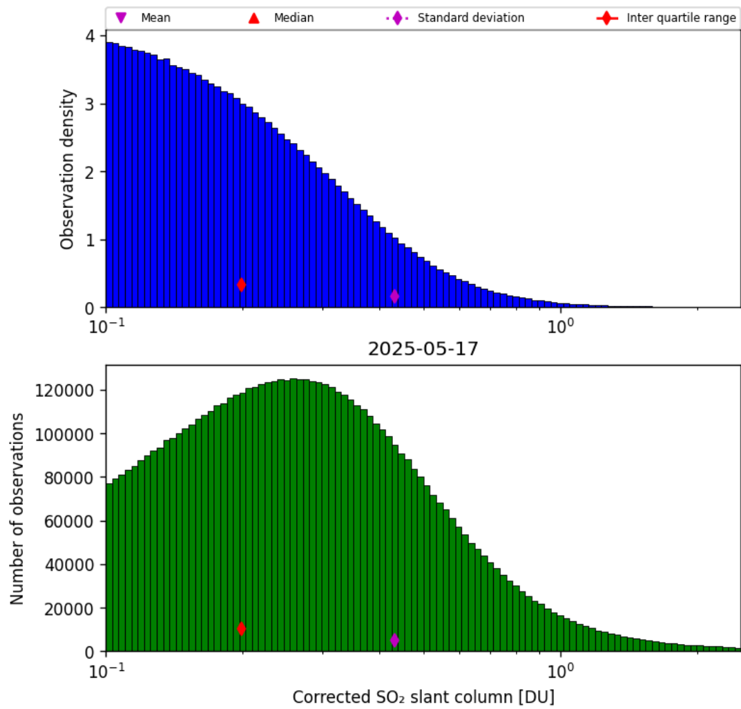
Figure 60: Histogram of “Corrected SO 2 slant column” for 2025-05-17 to 2025-05-18
