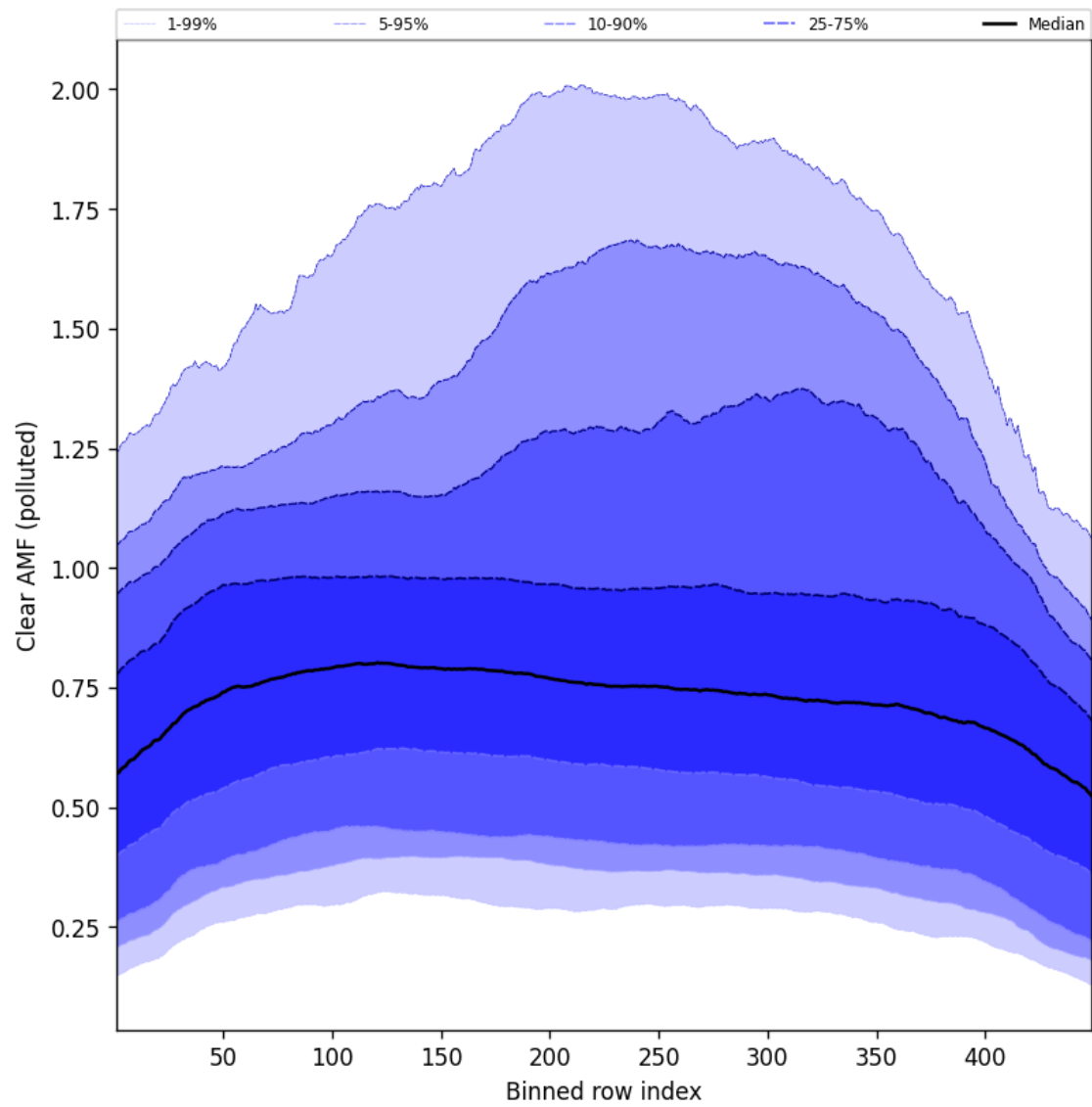
Figure 109: Along track statistics of “Clear AMF (polluted)” for 2025-05-17 to 2025-05-18
