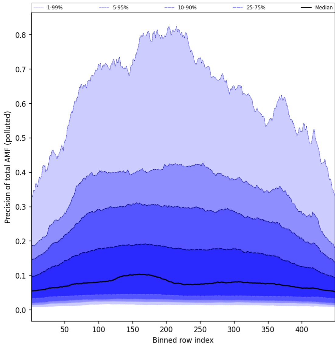
Figure 108: Along track statistics of “Precision of total AMF (polluted)” for 2025-05-17 to 2025-05-18
