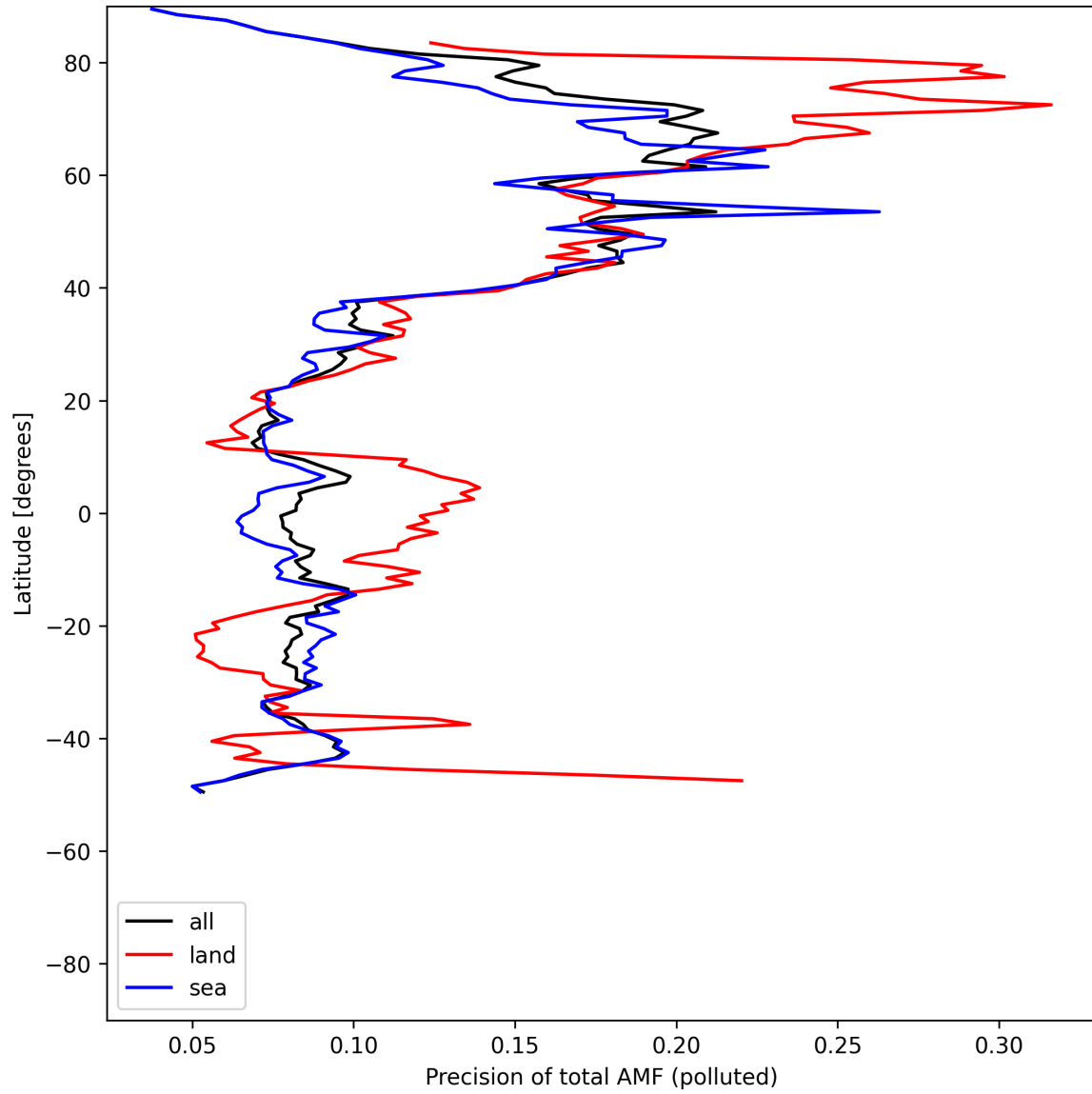
Figure 54: Zonal average of “Precision of total AMF (polluted)” for 2025-05-17 to 2025-05-18.
