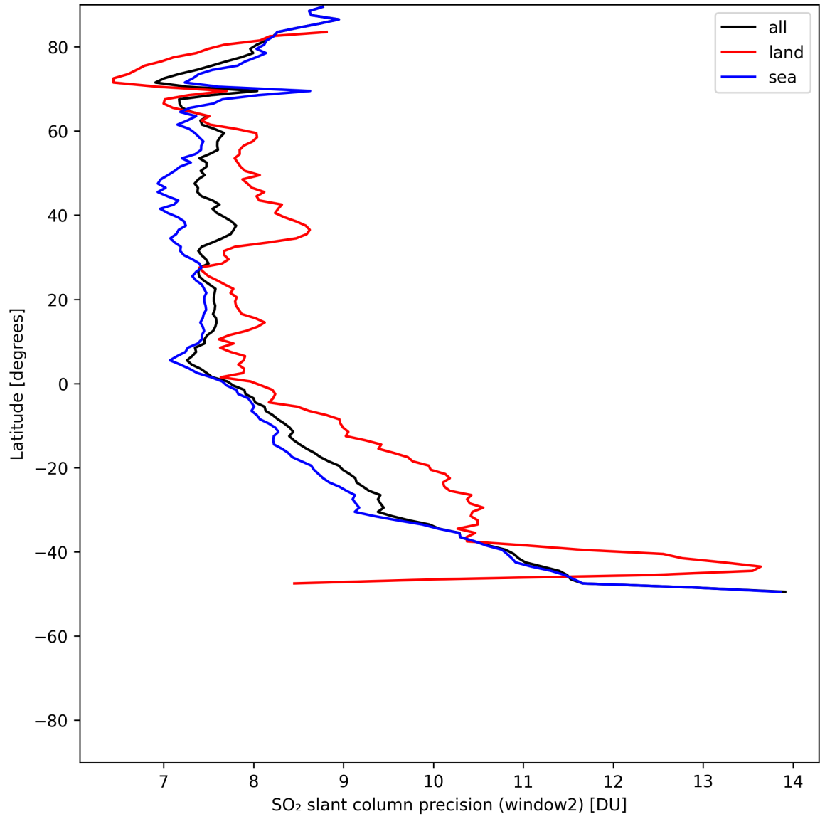
Figure 41: Zonal average of “SO 2 slant column precision (window2)” for 2025-05-17 to 2025-05-18.
