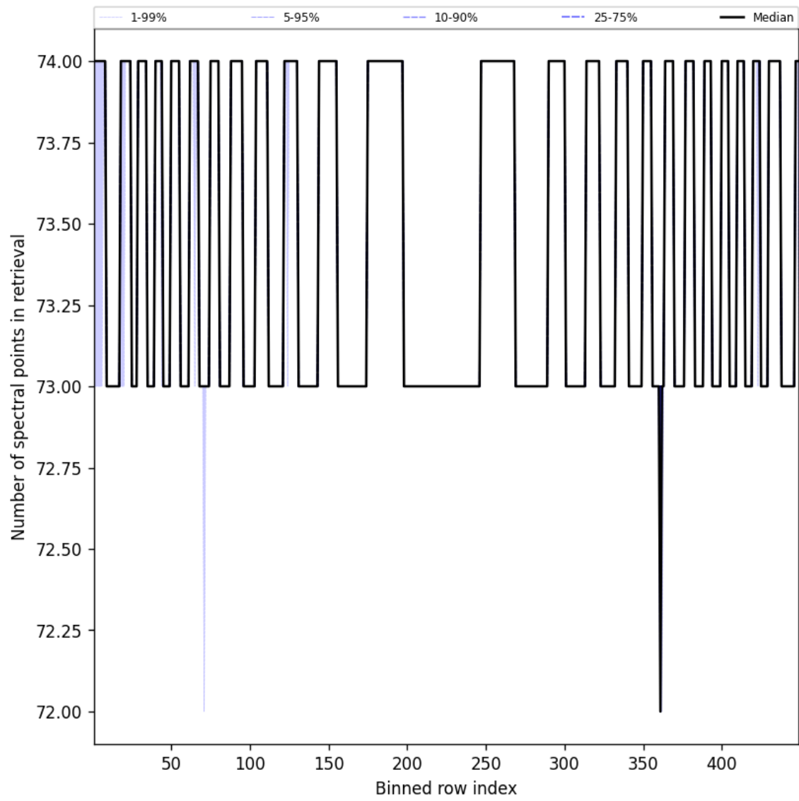
Figure 110: Along track statistics of “Number of spectral points in retrieval” for 2025-05-17 to 2025-05-18
