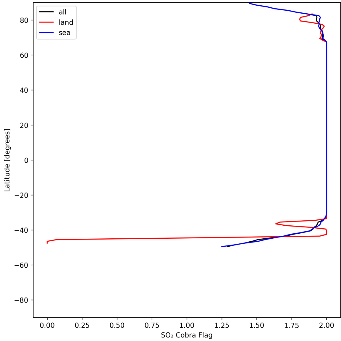
Figure 48: Zonal average of "SO 2 Cobra Flag" for 2025-05-17 to 2025-05-18.
