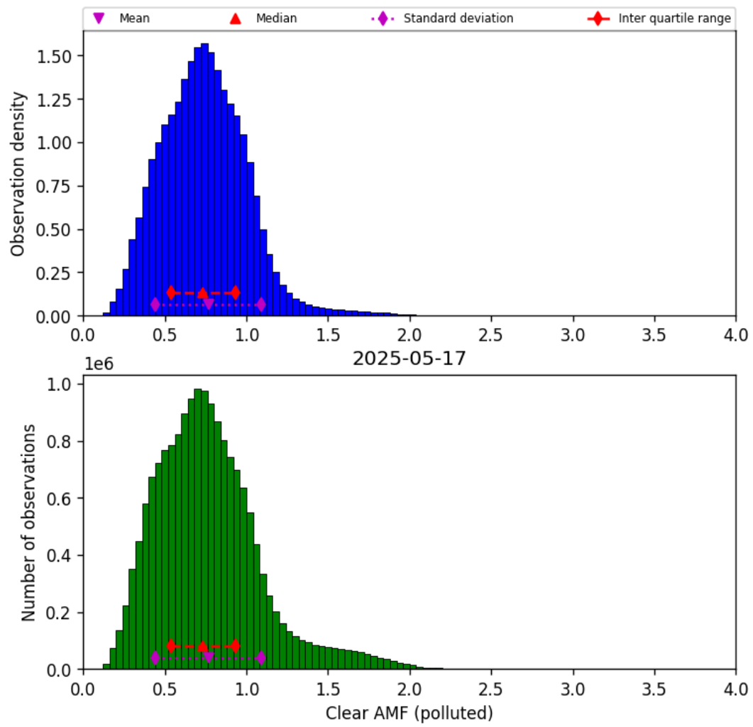
Figure 82: Histogram of "Clear AMF (polluted)" for 2025-05-17 to 2025-05-18
