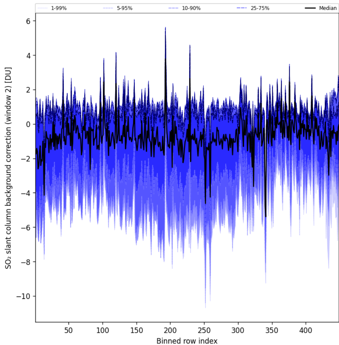
Figure 97: Along track statistics of “SO 2 slant column background correction (window 2)” for 2025-05-17 to 2025-05-18
