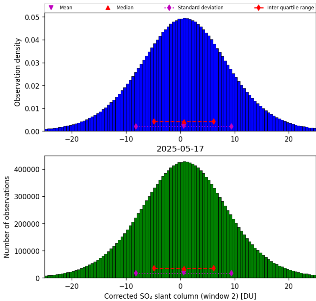
Figure 69: Histogram of “Corrected SO 2 slant column (window 2)” for 2025-05-17 to 2025-05-18
