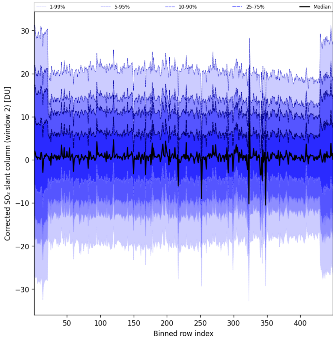
Figure 96: Along track statistics of “Corrected SO 2 slant column (window 2)” for 2025-05-17 to 2025-05-18
