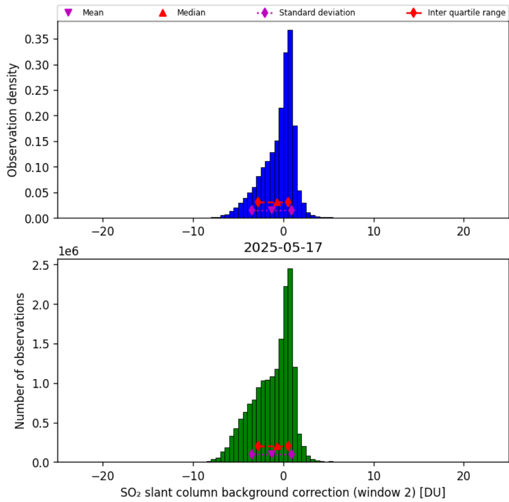
Figure 70: Histogram of “SO 2 slant column background correction (window 2)” for 2025-05-17 to 2025-05-18
