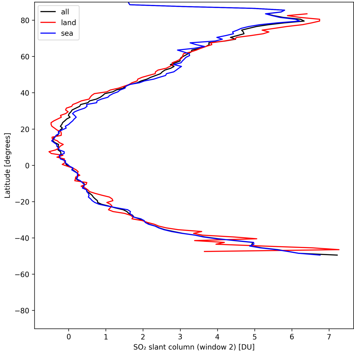
Figure 40: Zonal average of “SO 2 slant column (window 2)” for 2025-05-17 to 2025-05-18.
