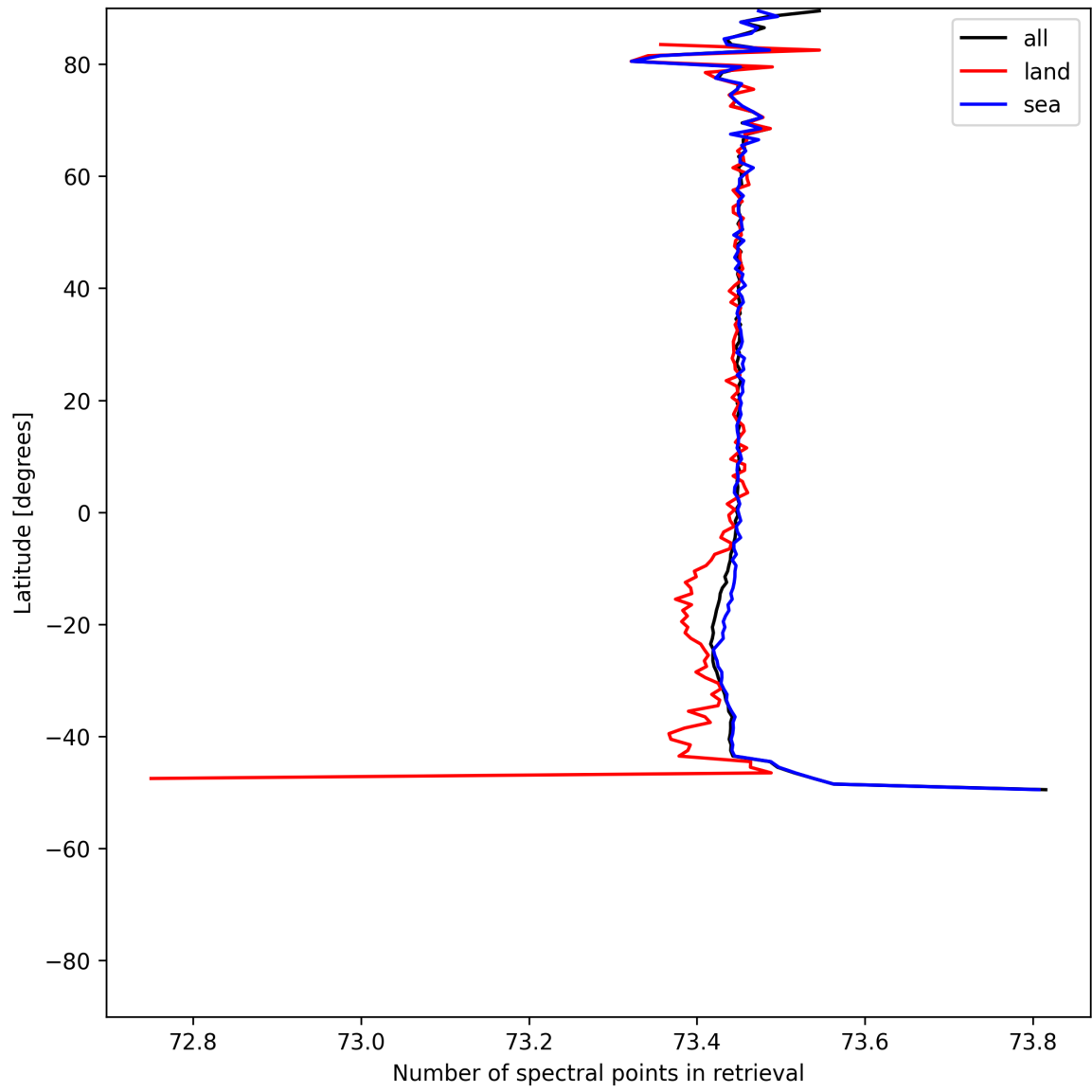
Figure 56: Zonal average of “Number of spectral points in retrieval” for 2025-05-17 to 2025-05-18.
