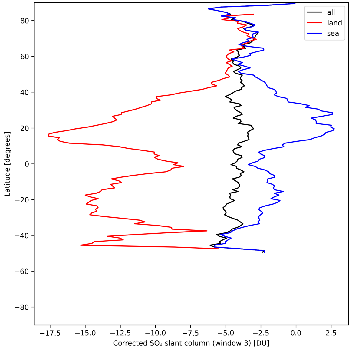
Figure 46: Zonal average of “Corrected SO 2 slant column (window 3)” for 2025-05-17 to 2025-05-18.
