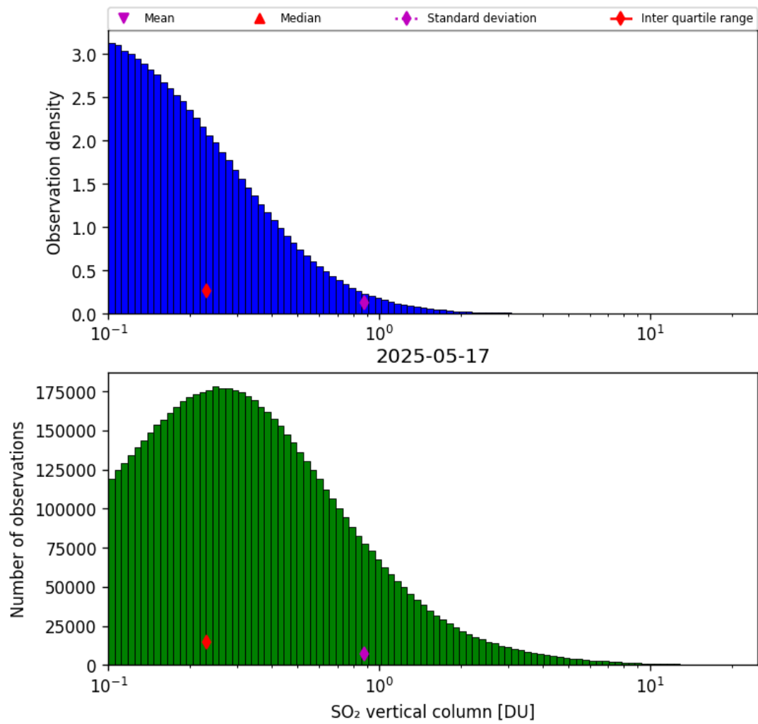
Figure 58: Histogram of “SO 2 vertical column” for 2025-05-17 to 2025-05-18
