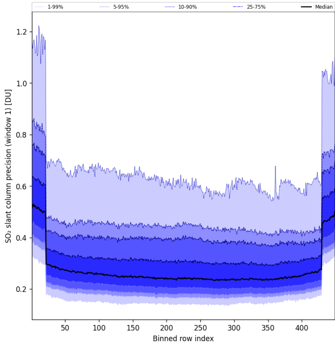
Figure 91: Along track statistics of “SO 2 slant column precision (window 1)” for 2025-05-17 to 2025-05-18
