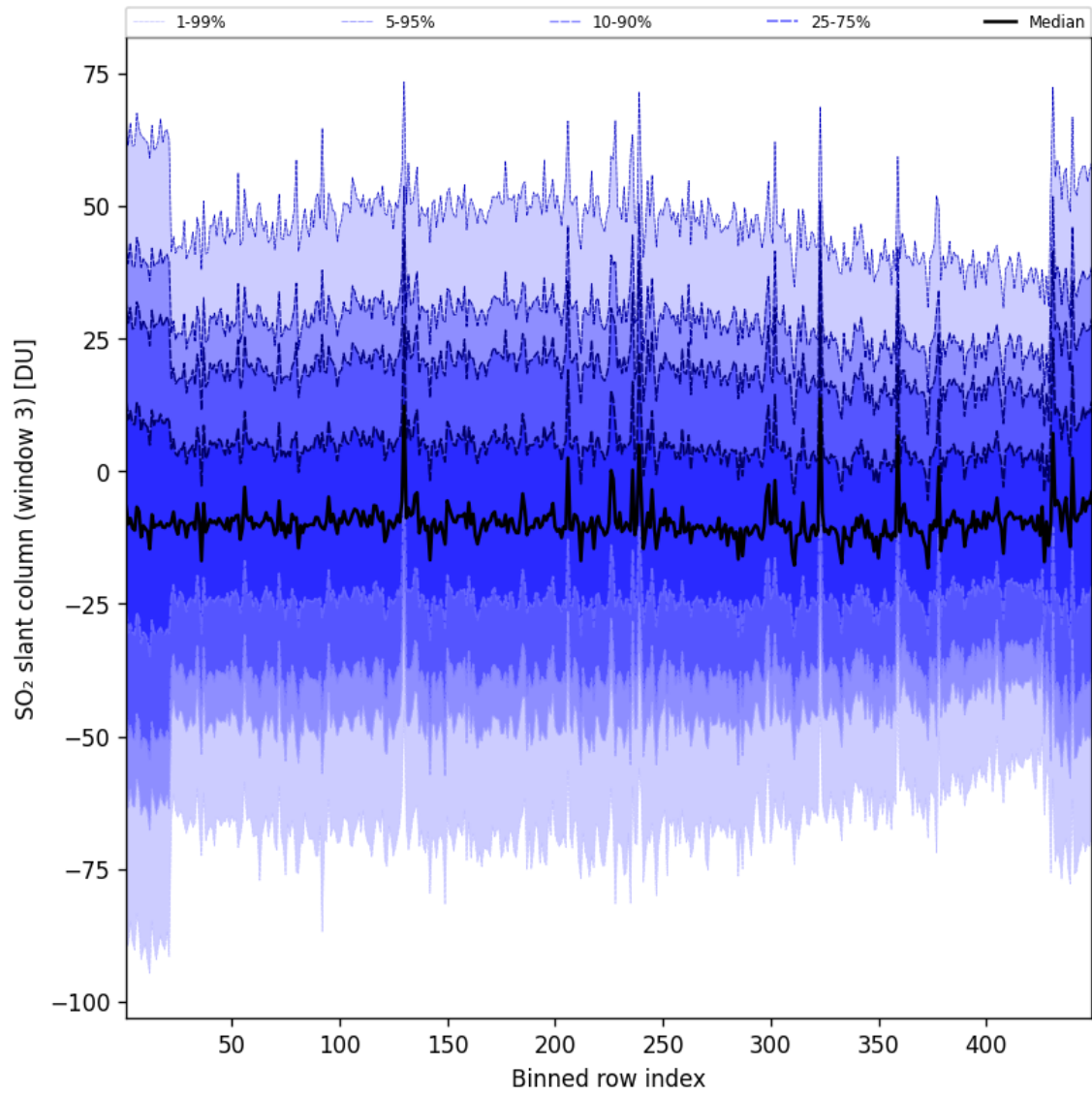
Figure 98: Along track statistics of “SO 2 slant column (window 3)” for 2025-05-17 to 2025-05-18
