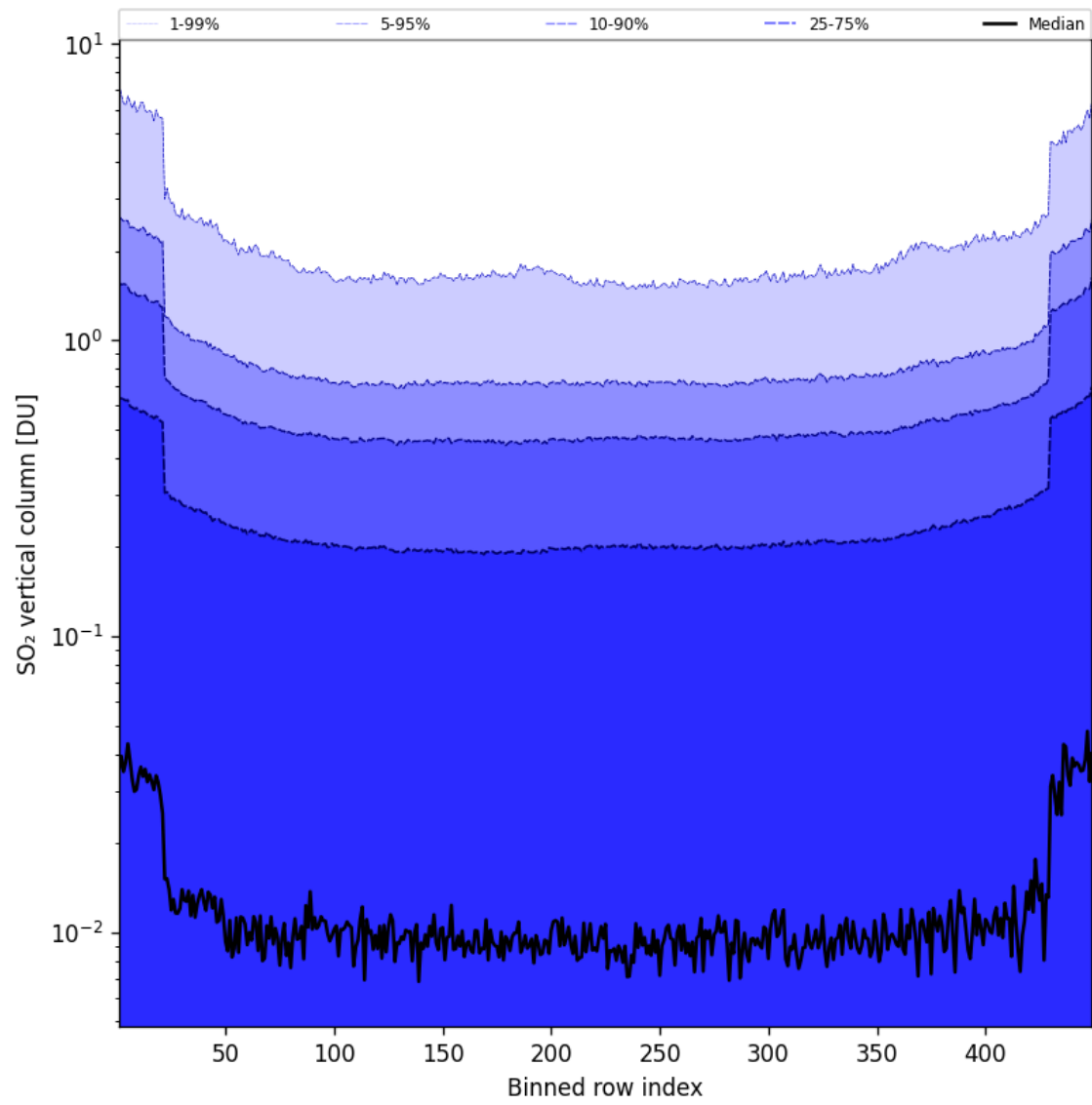
Figure 85: Along track statistics of “SO 2 vertical column” for 2025-05-17 to 2025-05-18
