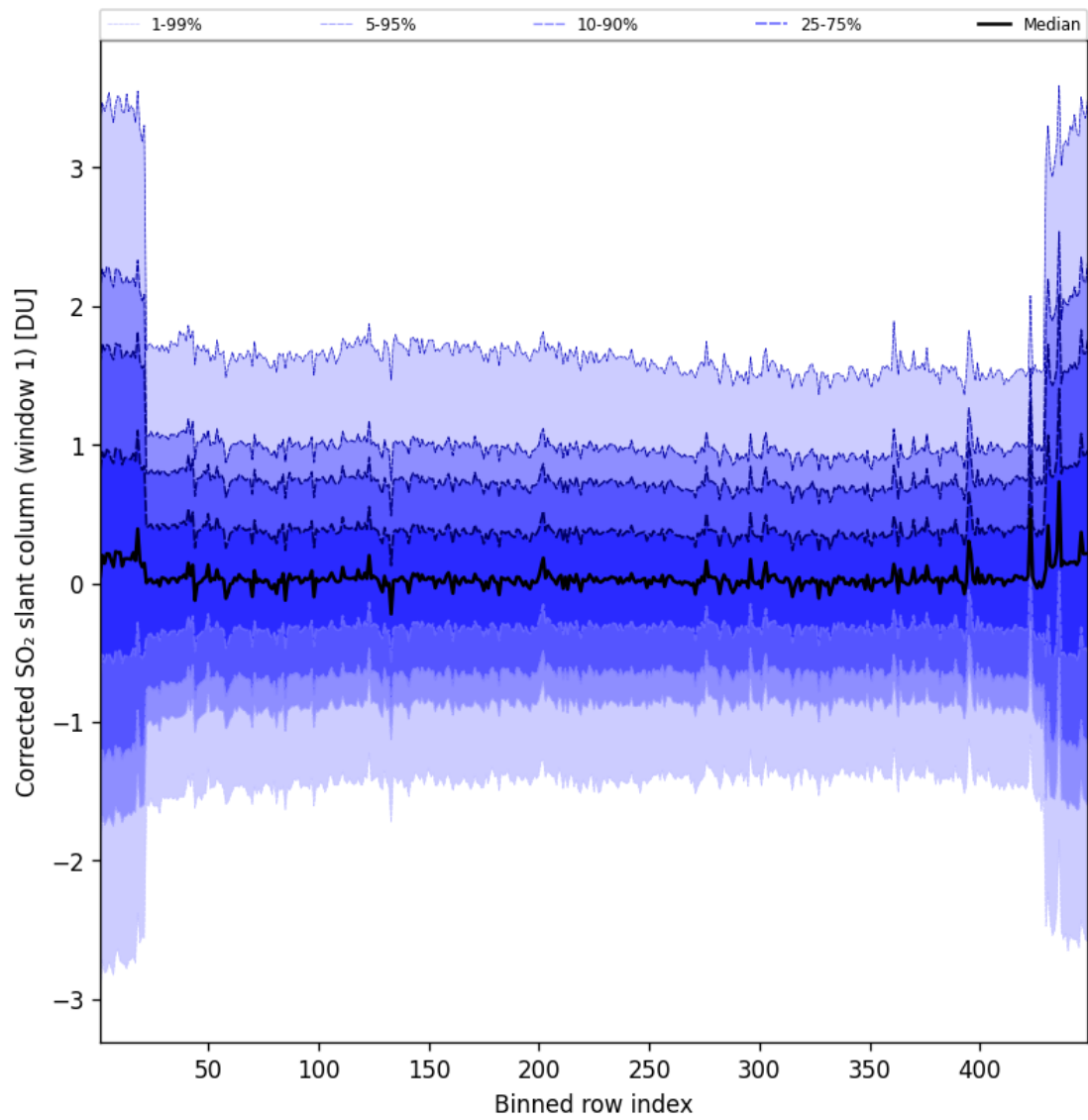
Figure 92: Along track statistics of “Corrected SO 2 slant column (window 1)” for 2025-05-17 to 2025-05-18
