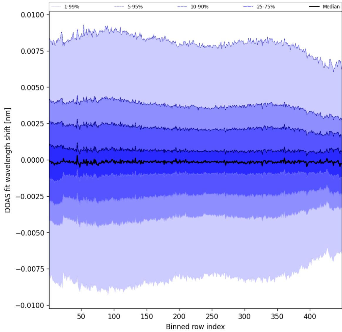
Figure 104: Along track statistics of “DOAS fit wavelength shift” for 2025-05-17 to 2025-05-18
