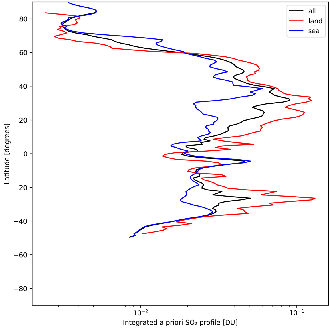
Figure 49: Zonal average of “Integrated a priori SO 2 profile” for 2025-05-17 to 2025-05-18.
