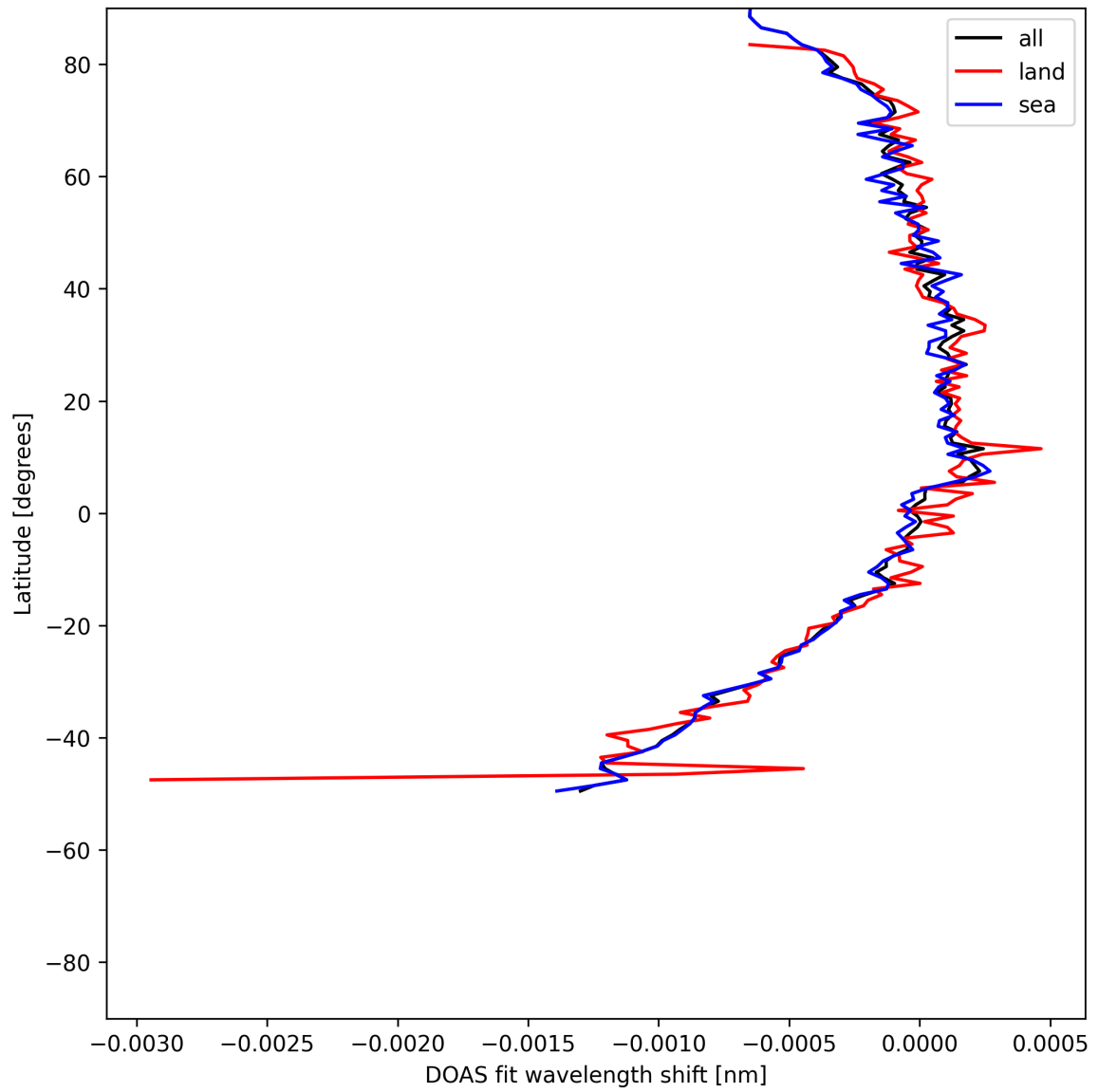
Figure 50: Zonal average of “DOAS fit wavelength shift” for 2025-05-17 to 2025-05-18.
