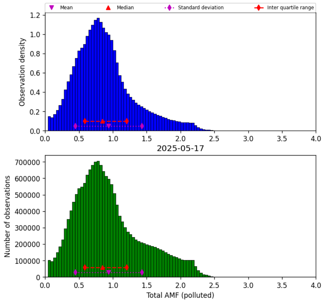
Figure 80: Histogram of “Total AMF (polluted)” for 2025-05-17 to 2025-05-18
