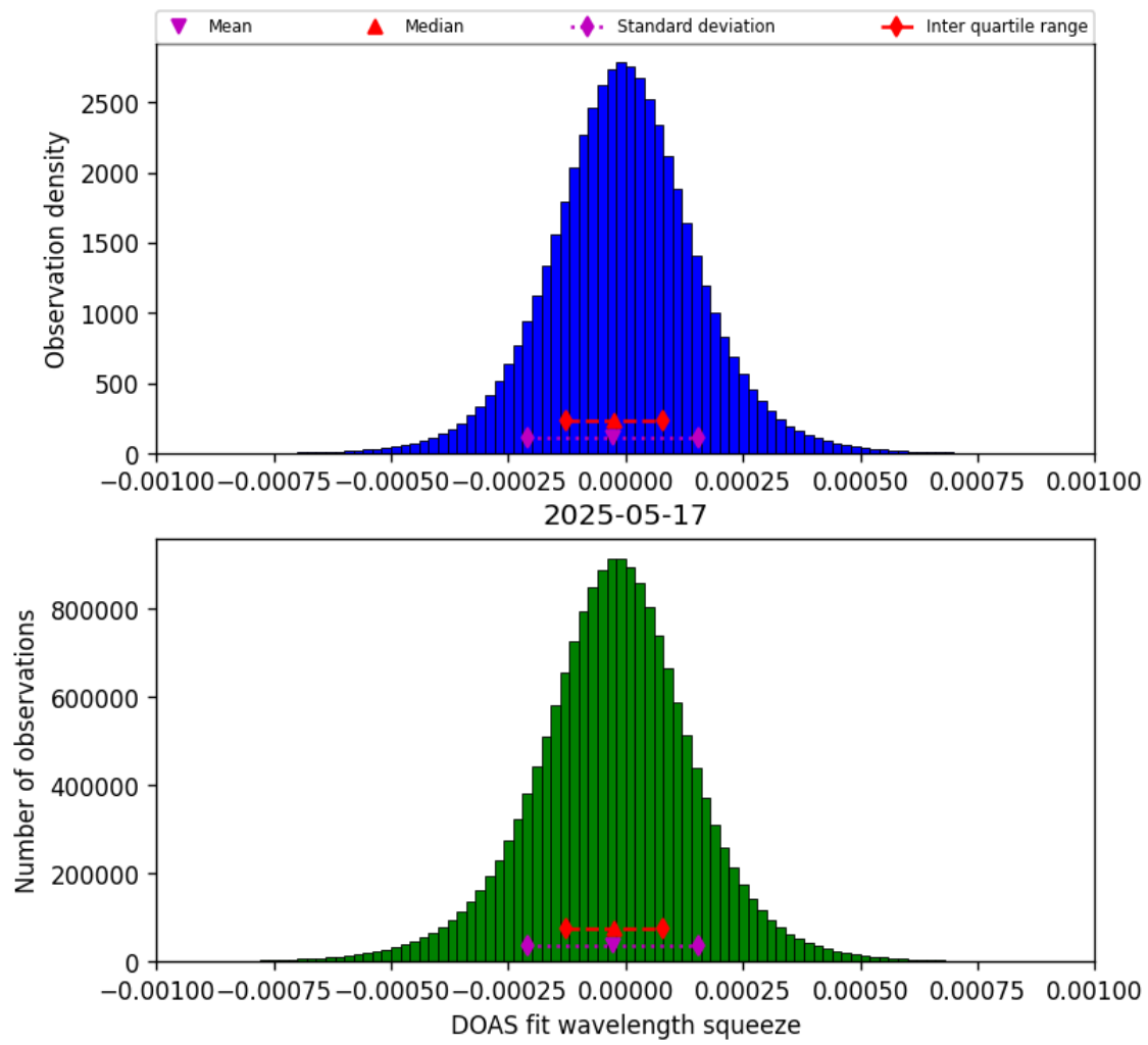
Figure 78: Histogram of “DOAS fit wavelength squeeze” for 2025-05-17 to 2025-05-18
