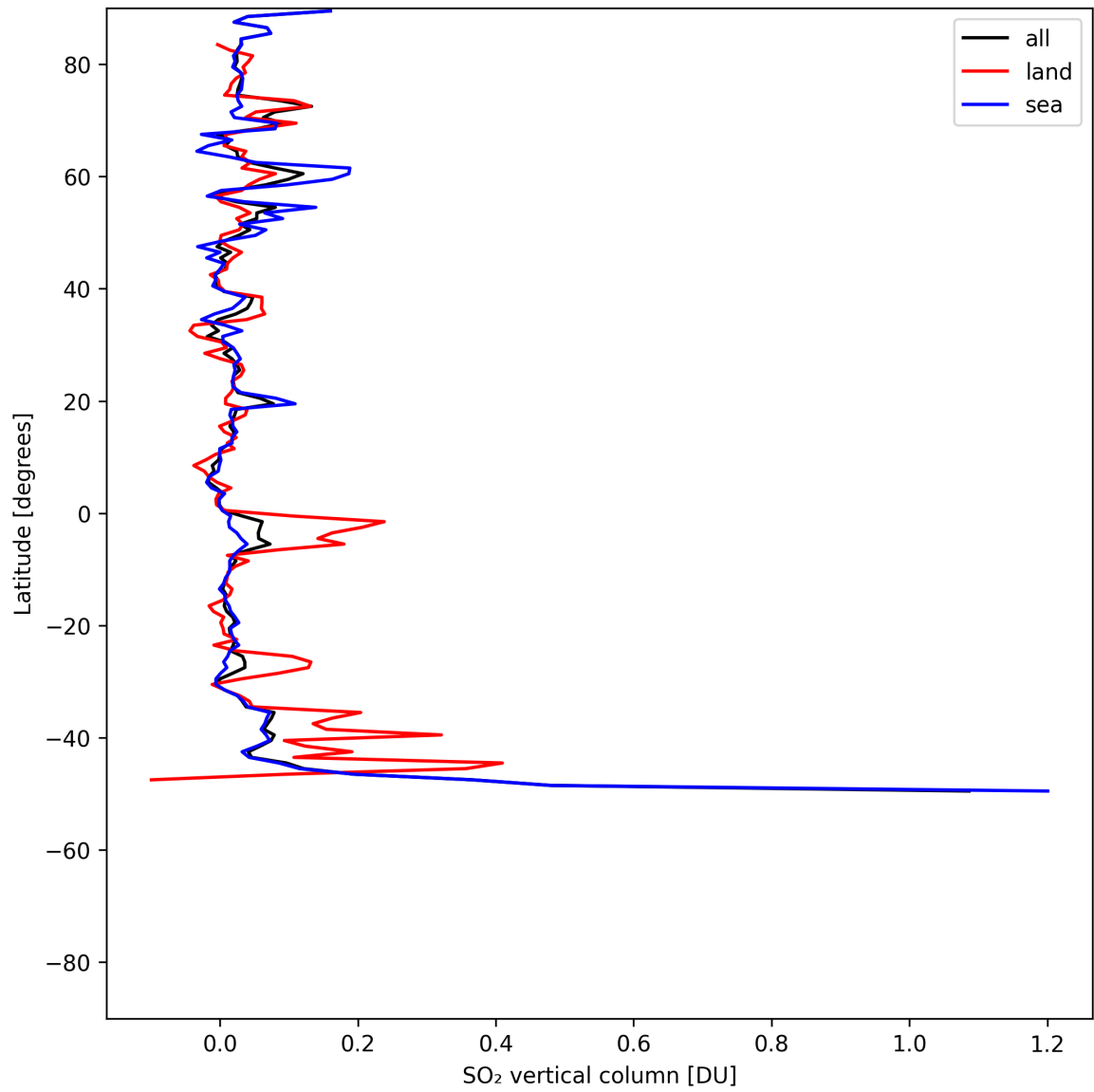
Figure 31: Zonal average of “SO 2 vertical column” for 2025-05-17 to 2025-05-18.
