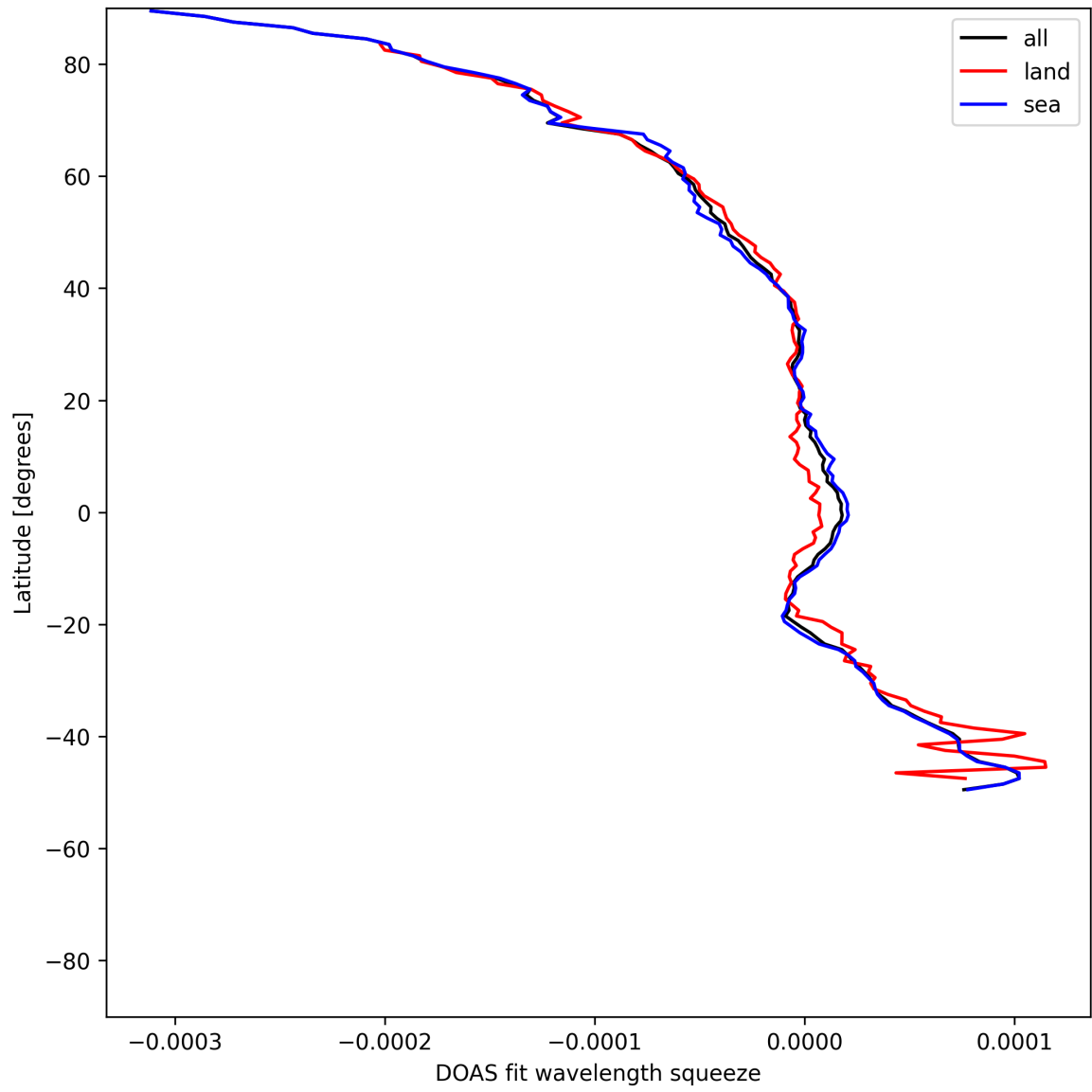
Figure 51: Zonal average of “DOAS fit wavelength squeeze” for 2025-05-17 to 2025-05-18.
