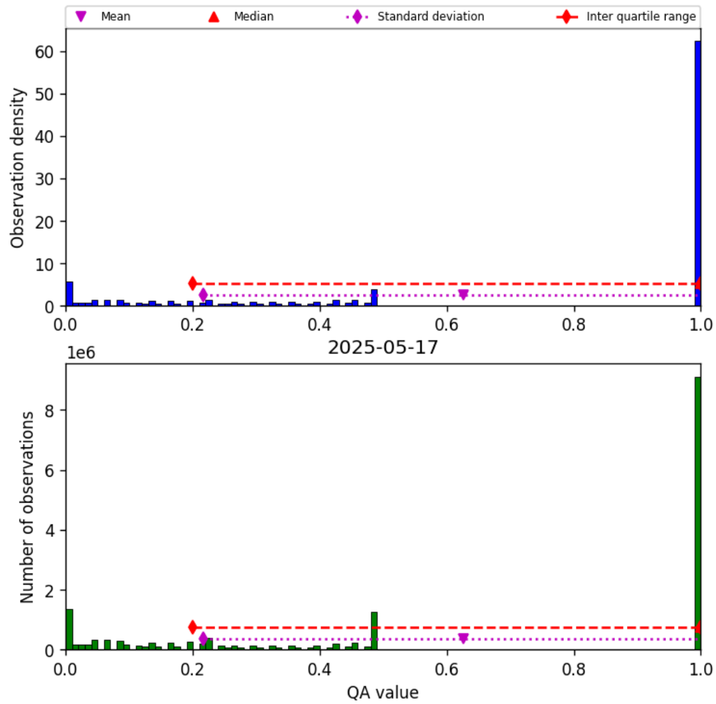
Figure 57: Histogram of “QA value” for 2025-05-17 to 2025-05-18
