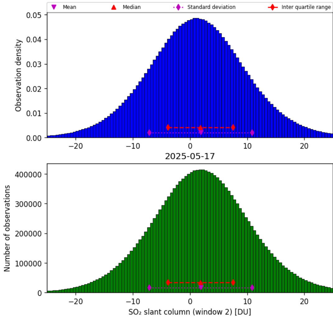
Figure 67: Histogram of “SO 2 slant column (window 2)” for 2025-05-17 to 2025-05-18
