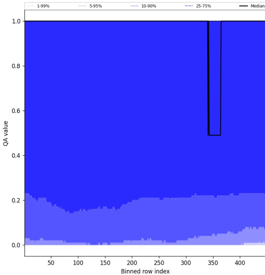
Figure 84: Along track statistics of “QA value” for 2025-05-17 to 2025-05-18
