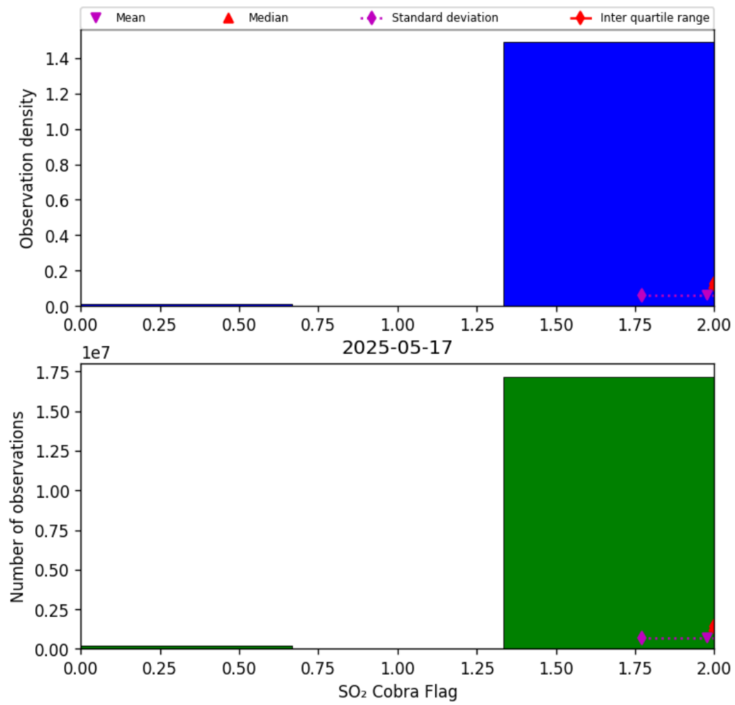
Figure 75: Histogram of “SO 2 Cobra Flag” for 2025-05-17 to 2025-05-18
