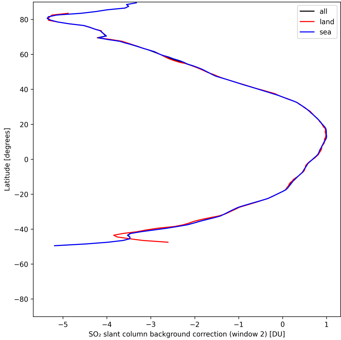
Figure 43: Zonal average of “SO 2 slant column background correction (window 2)” for 2025-05-17 to 2025-05-18.
