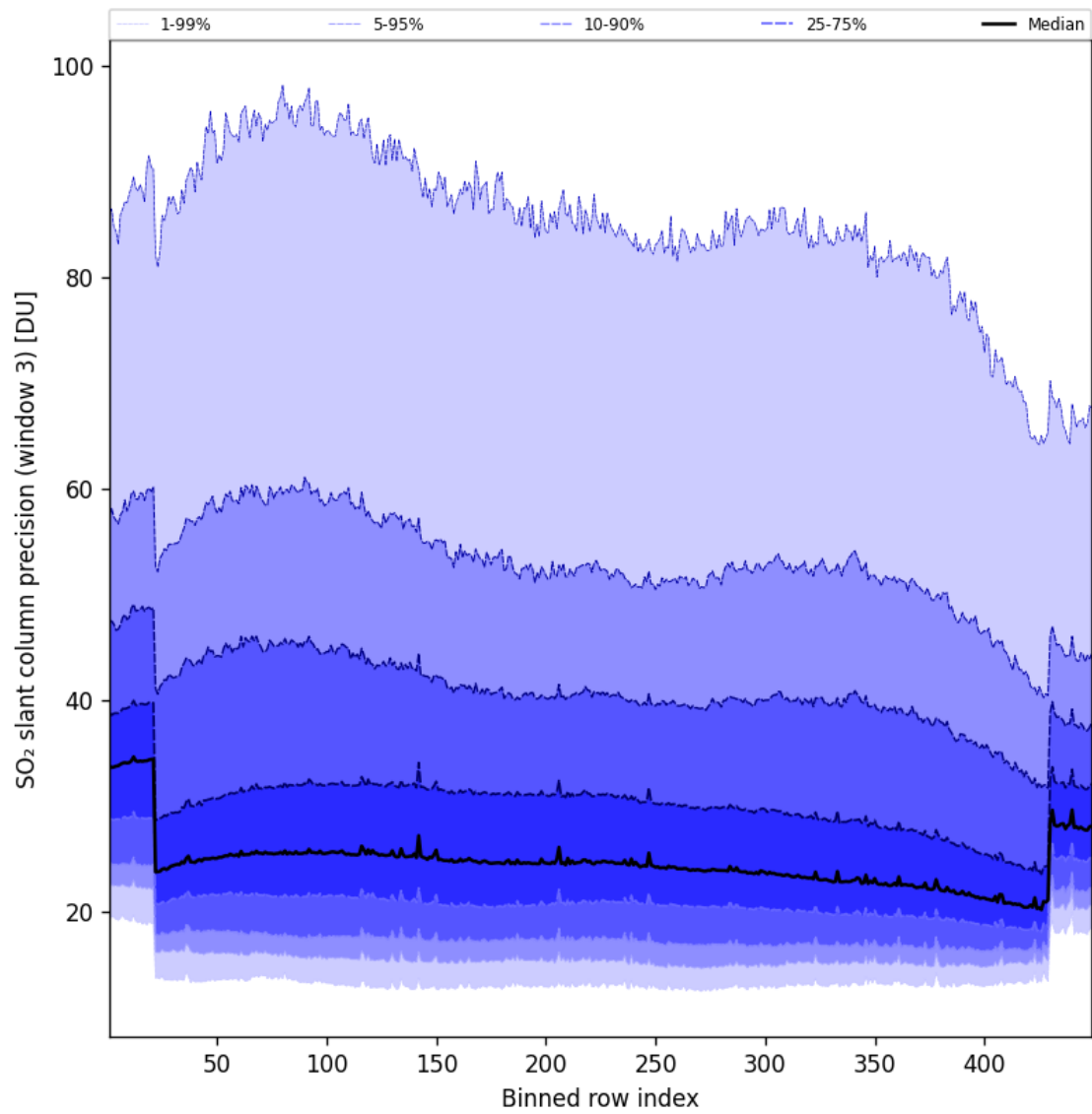
Figure 99: Along track statistics of “SO 2 slant column precision (window 3)” for 2025-05-17 to 2025-05-18
