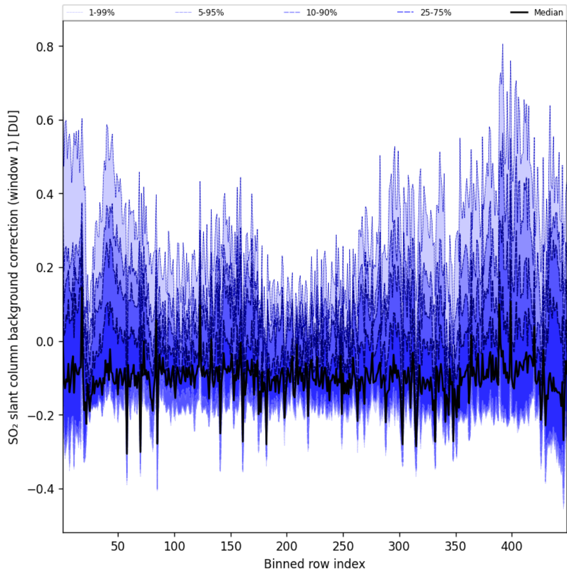
Figure 93: Along track statistics of “SO 2 slant column background correction (window 1)” for 2025-05-17 to 2025-05-18
