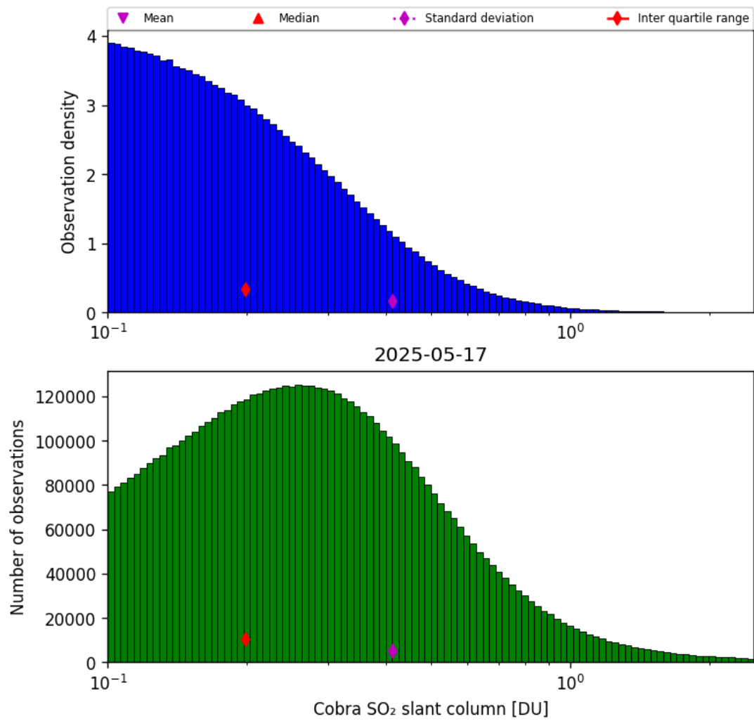
Figure 61: Histogram of “Cobra SO 2 slant column” for 2025-05-17 to 2025-05-18
