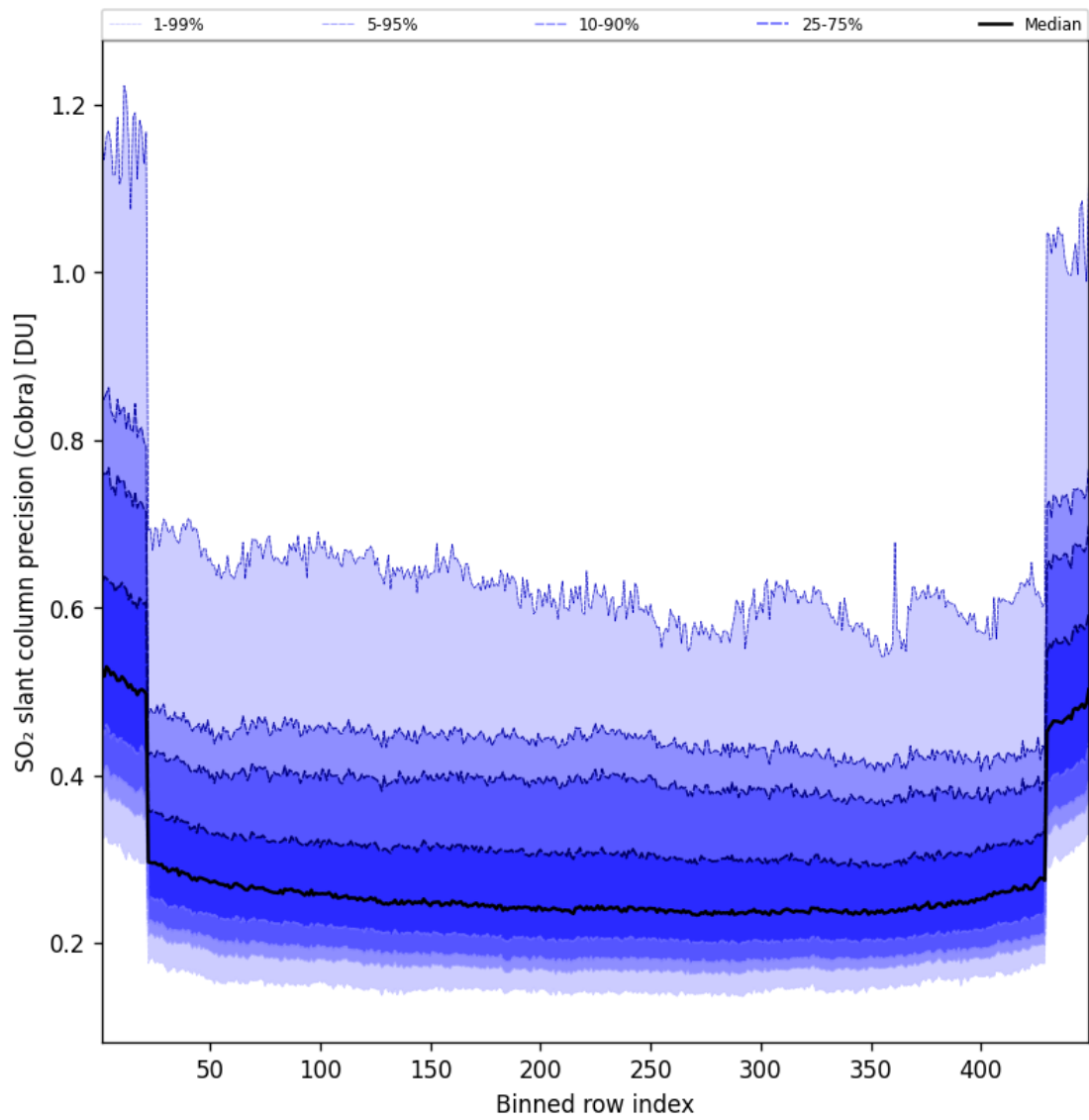
Figure 89: Along track statistics of “SO 2 slant column precision (Cobra)” for 2025-05-17 to 2025-05-18
