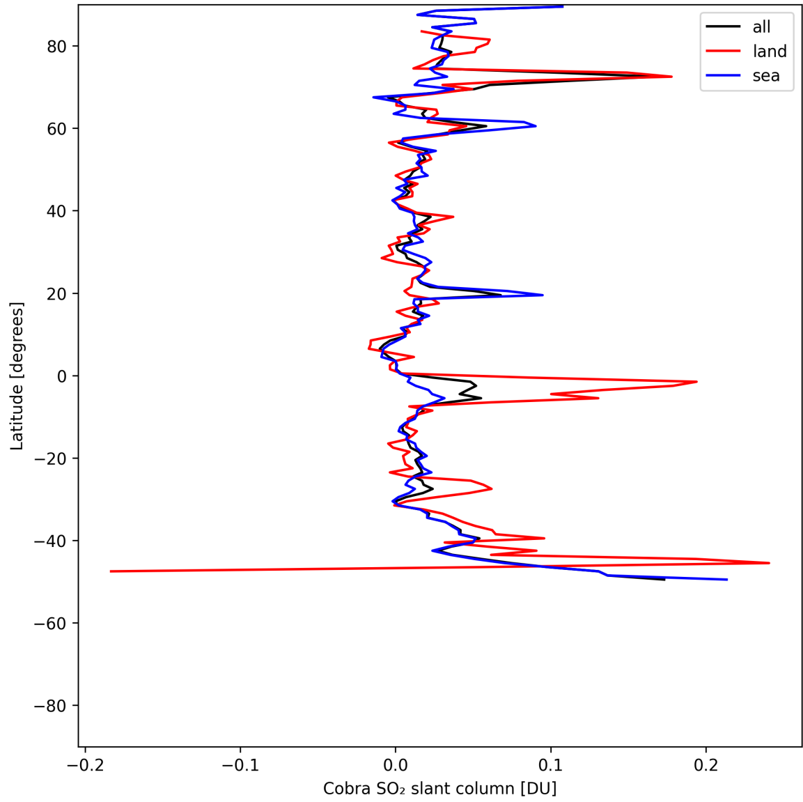
Figure 34: Zonal average of “Cobra SO 2 slant column” for 2025-05-17 to 2025-05-18.
