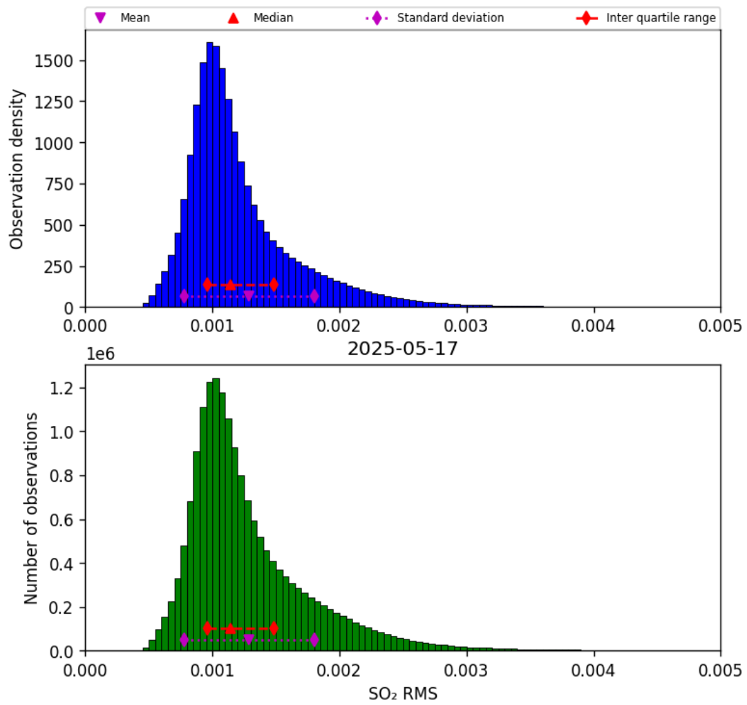
Figure 79: Histogram of “SO 2 RMS” for 2025-05-17 to 2025-05-18
