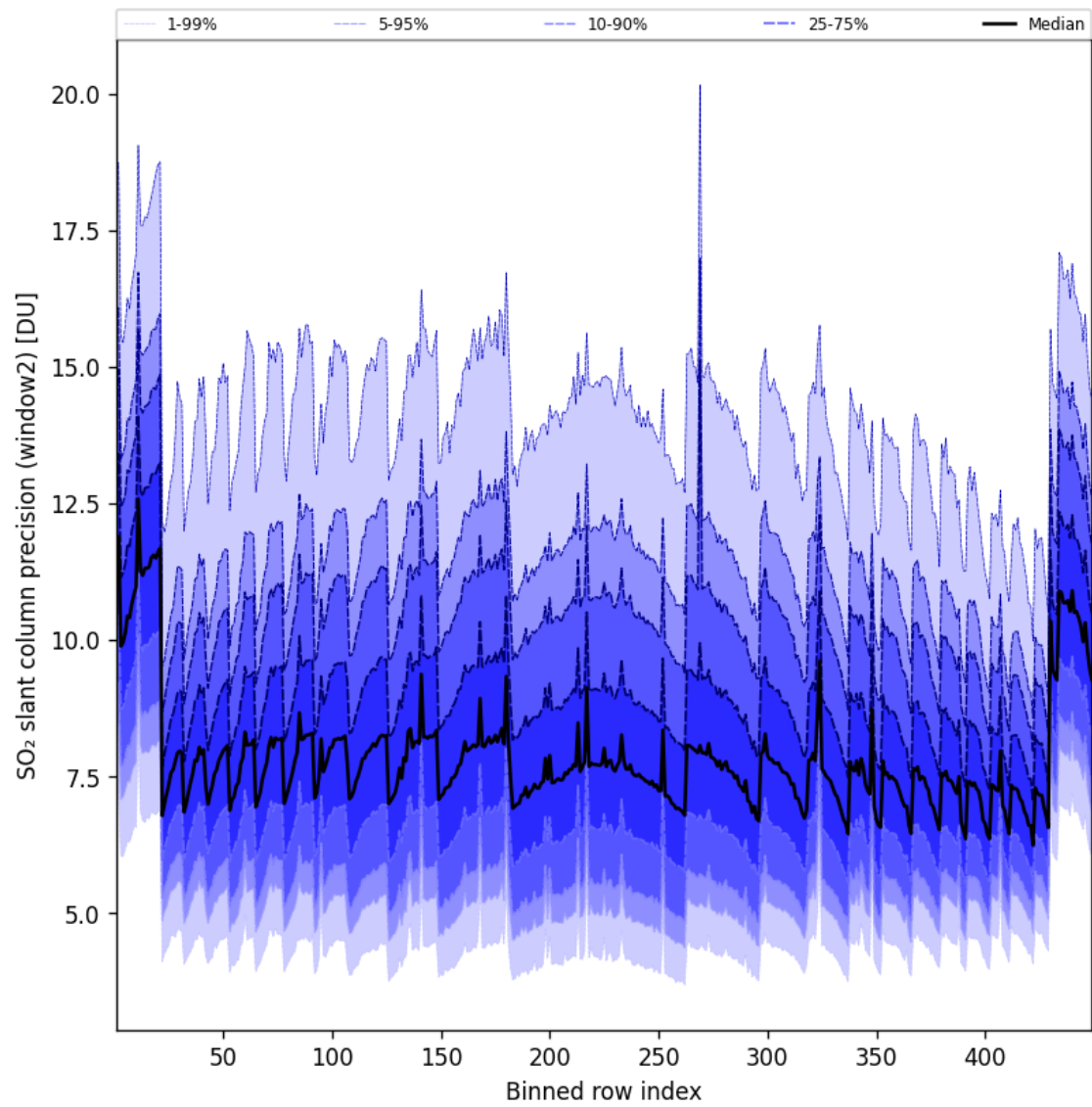
Figure 95: Along track statistics of “SO 2 slant column precision (window2)” for 2025-05-17 to 2025-05-18
