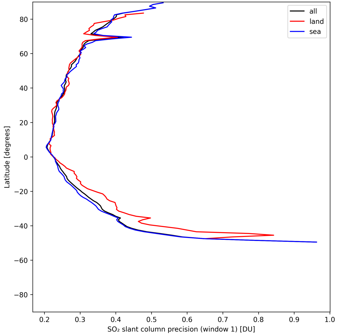
Figure 37: Zonal average of “SO 2 slant column precision (window 1)” for 2025-05-17 to 2025-05-18.
