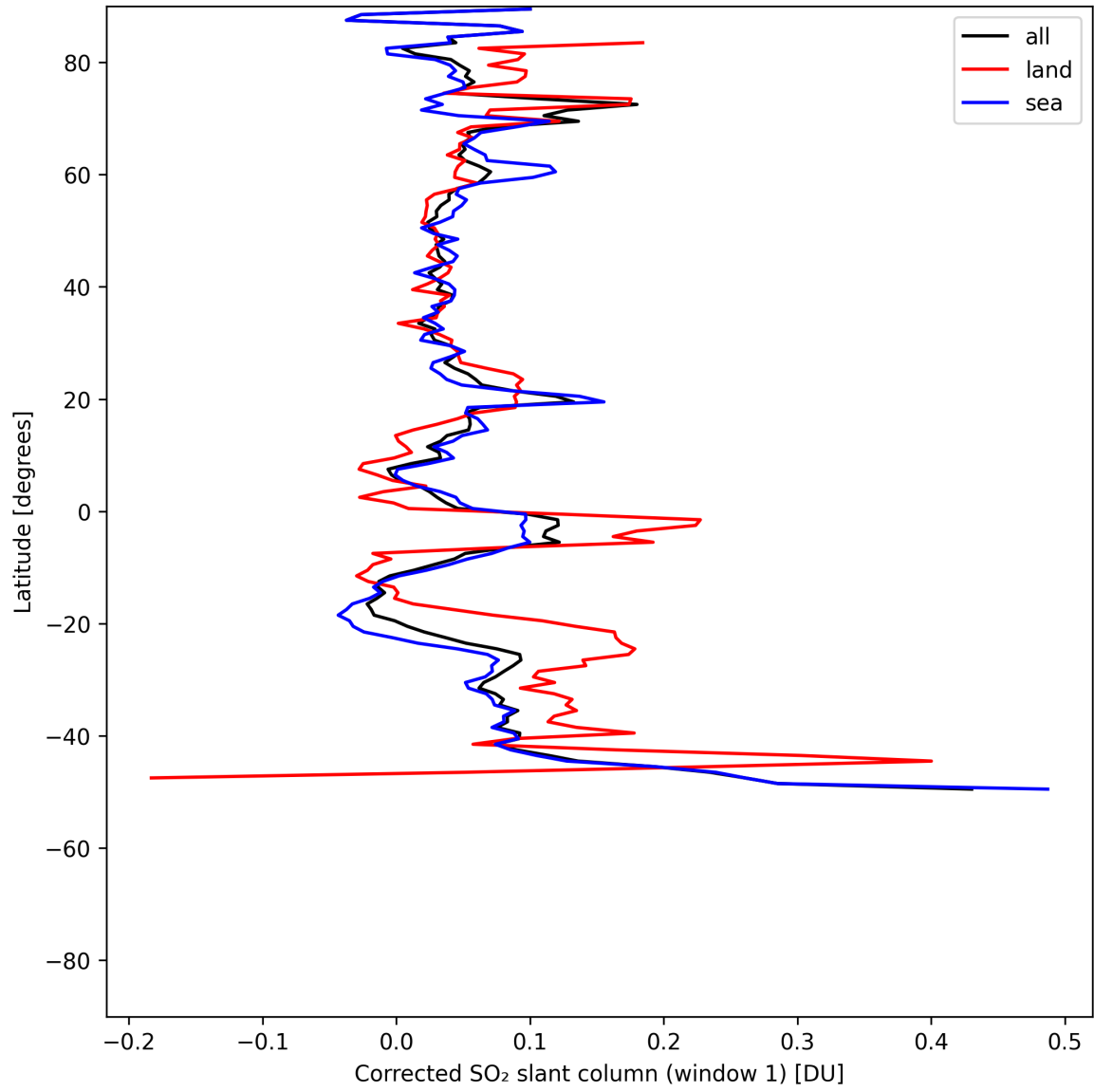
Figure 38: Zonal average of “Corrected SO 2 slant column (window 1)” for 2025-05-17 to 2025-05-18.
