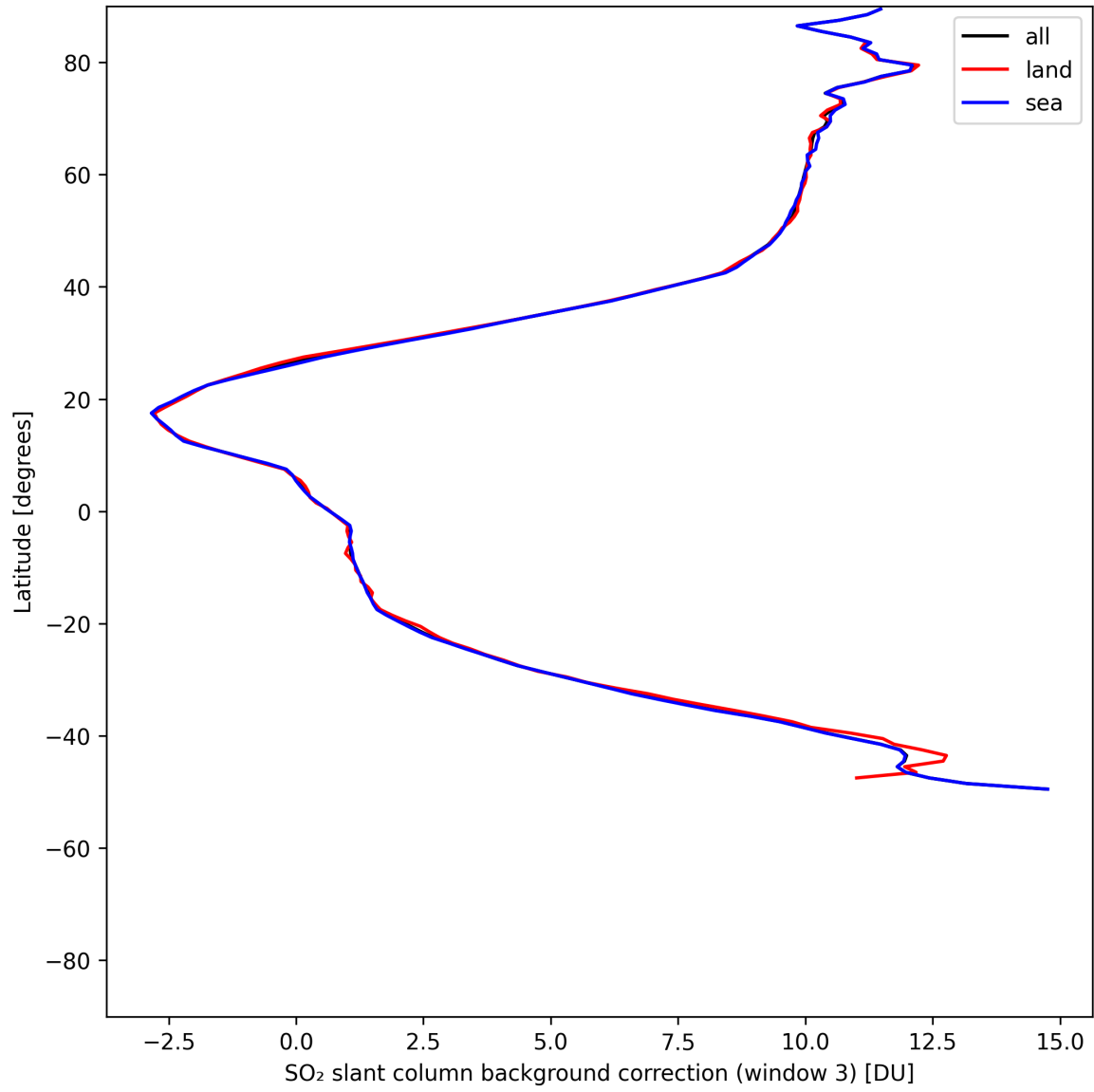
Figure 47: Zonal average of “SO 2 slant column background correction (window 3)” for 2025-05-17 to 2025-05-18.
