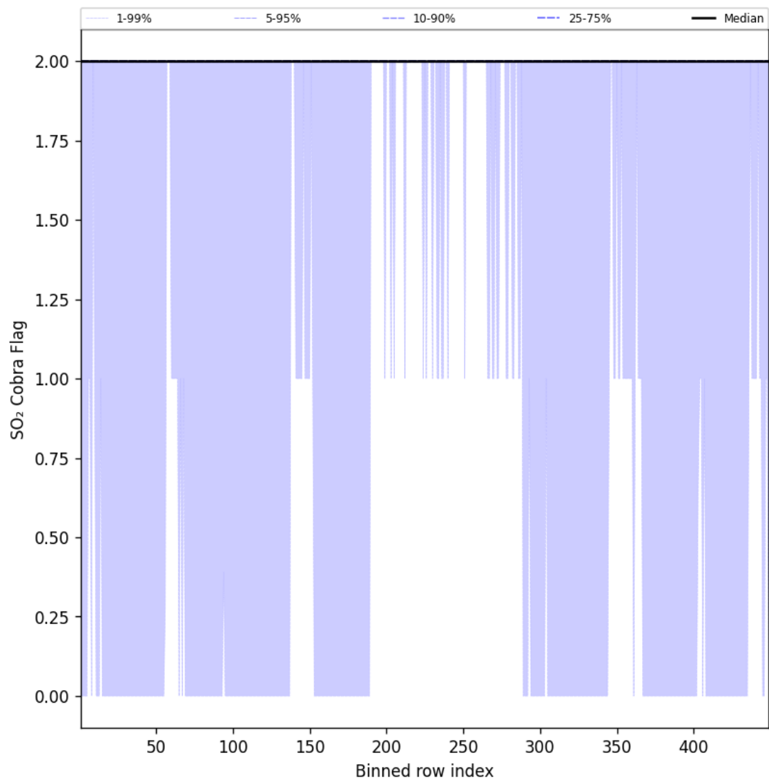
Figure 102: Along track statistics of “SO 2 Cobra Flag” for 2025-05-17 to 2025-05-18
