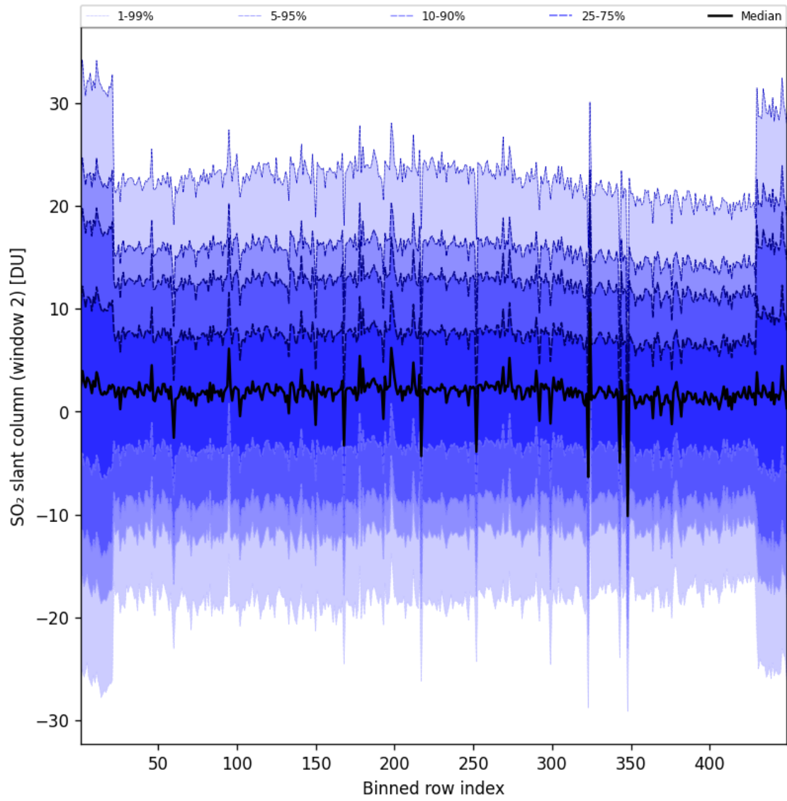
Figure 94: Along track statistics of “SO 2 slant column (window 2)” for 2025-05-17 to 2025-05-18
