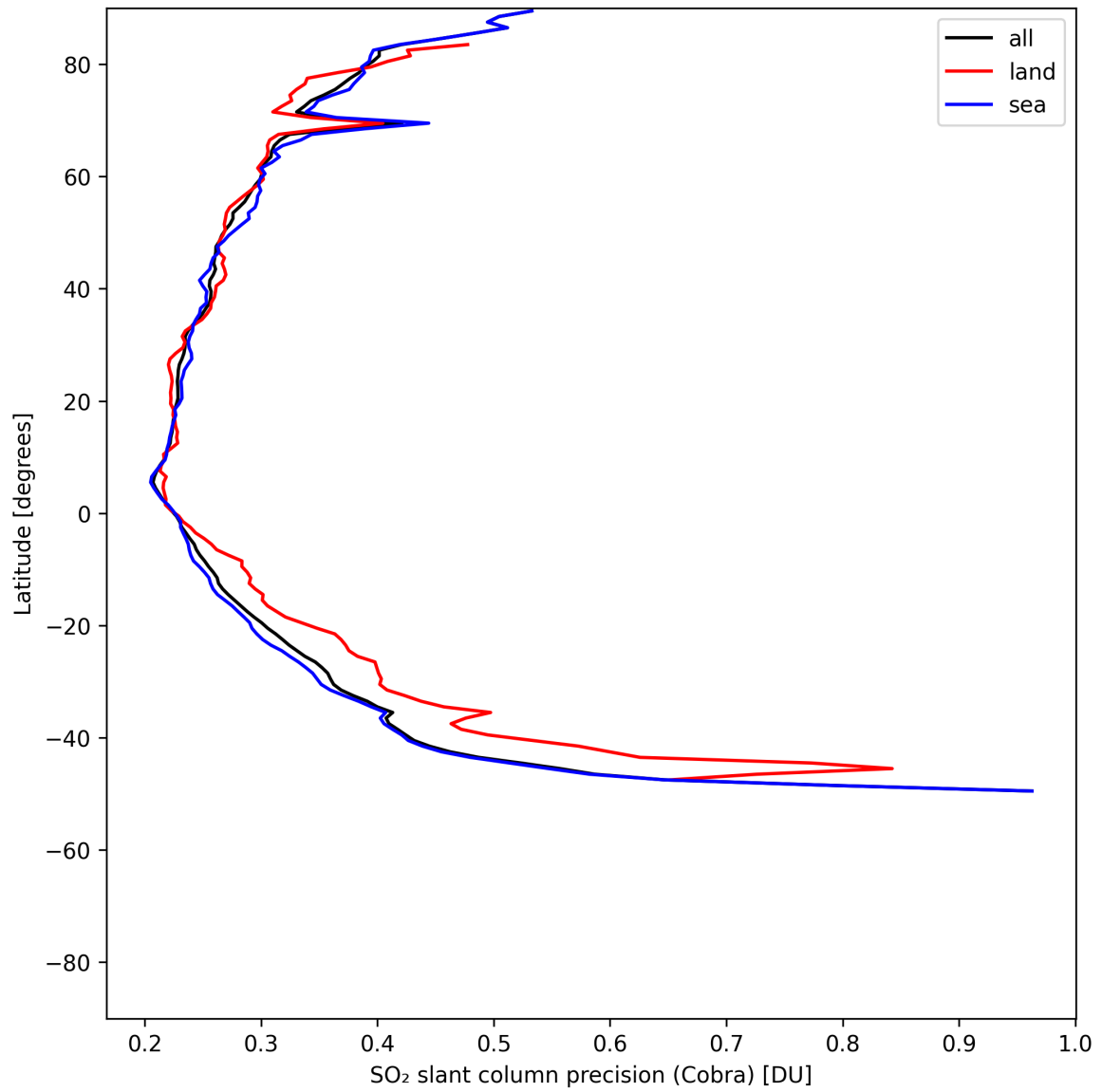
Figure 35: Zonal average of “SO 2 slant column precision (Cobra)” for 2025-05-17 to 2025-05-18.
