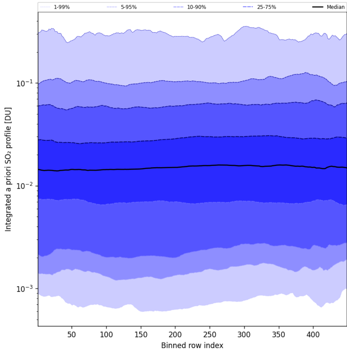
Figure 103: Along track statistics of “Integrated a priori SO 2 profile” for 2025-05-17 to 2025-05-18
