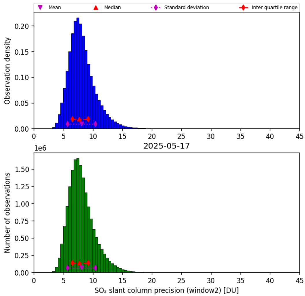
Figure 68: Histogram of “SO 2 slant column precision (window2)” for 2025-05-17 to 2025-05-18
