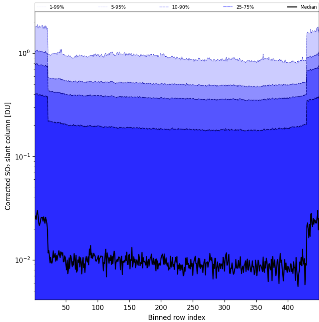
Figure 87: Along track statistics of "Corrected SO 2 slant column" for 2025-05-17 to 2025-05-18
