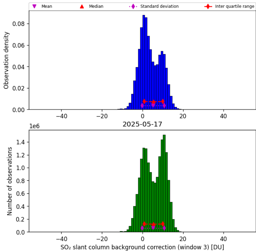
Figure 74: Histogram of “SO 2 slant column background correction (window 3)” for 2025-05-17 to 2025-05-18
