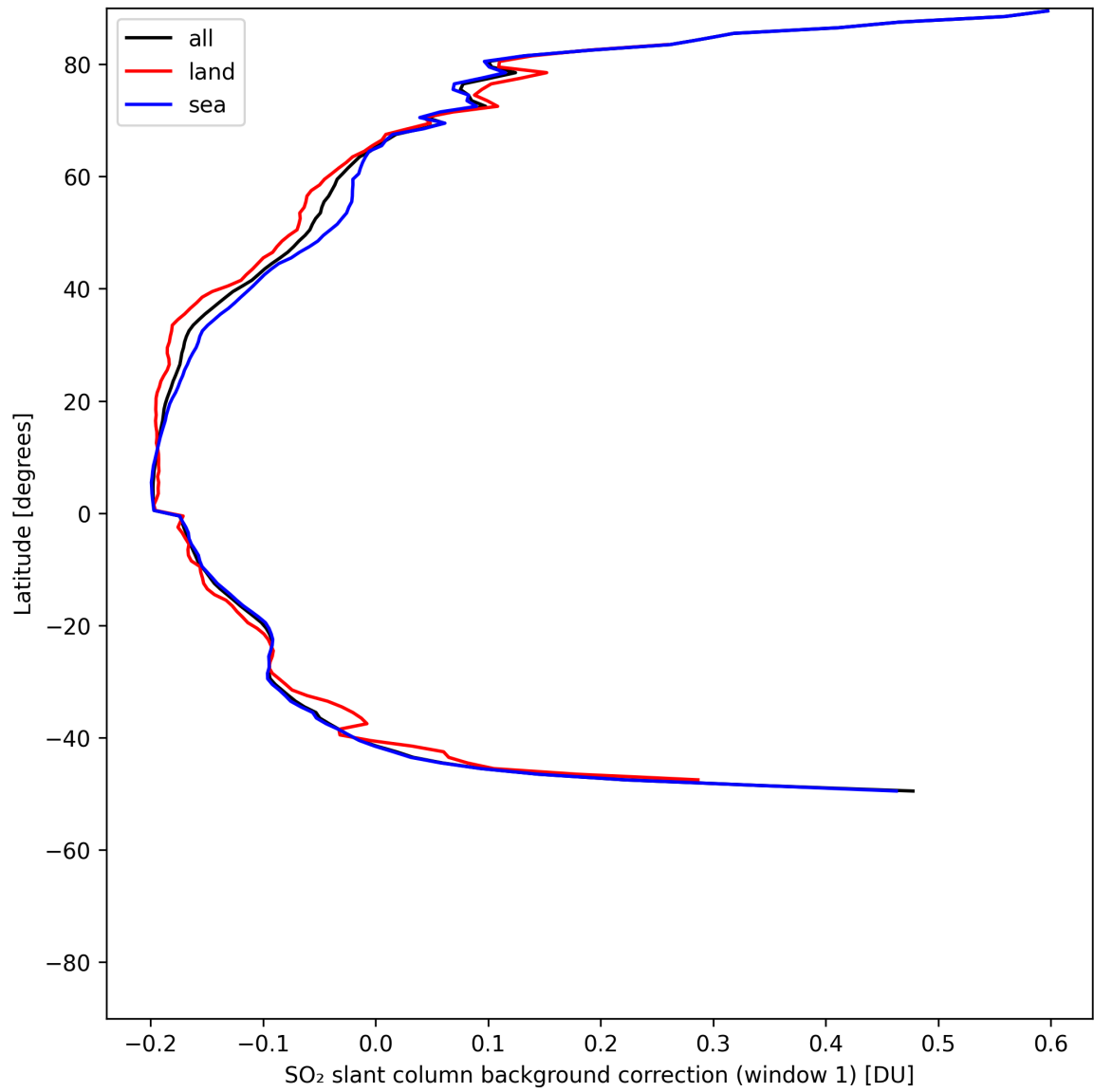
Figure 39: Zonal average of “SO 2 slant column background correction (window 1)” for 2025-05-17 to 2025-05-18.
