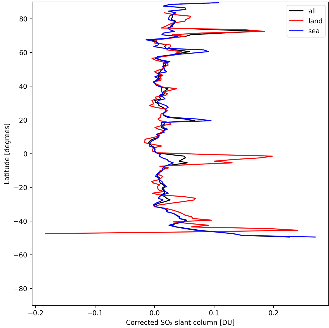
Figure 33: Zonal average of “Corrected SO 2 slant column” for 2025-05-17 to 2025-05-18.
