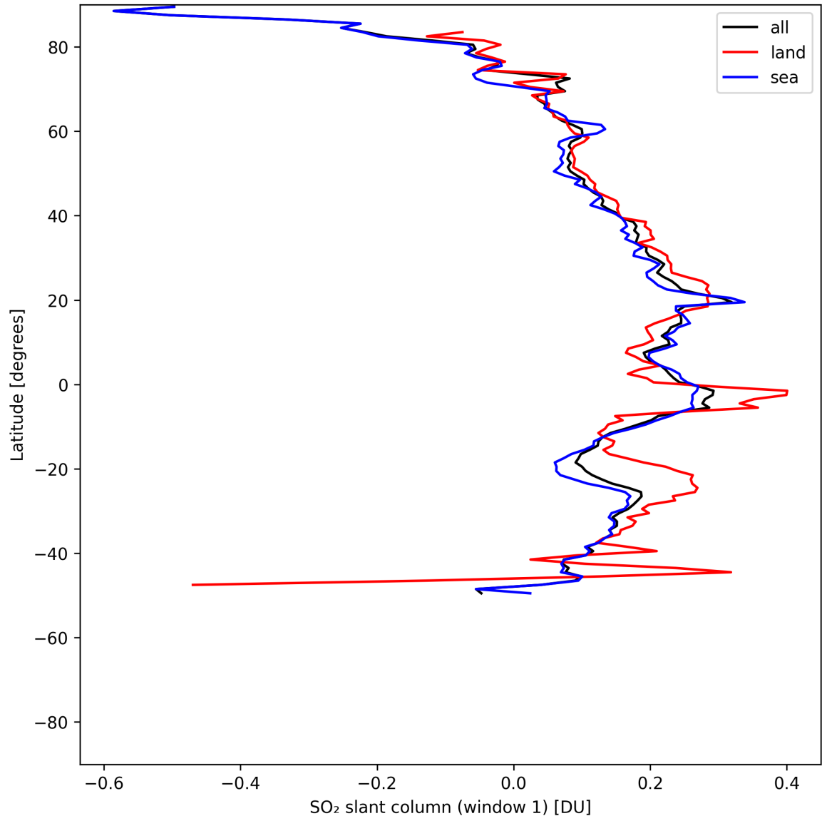
Figure 36: Zonal average of “SO 2 slant column (window 1)” for 2025-05-17 to 2025-05-18.
