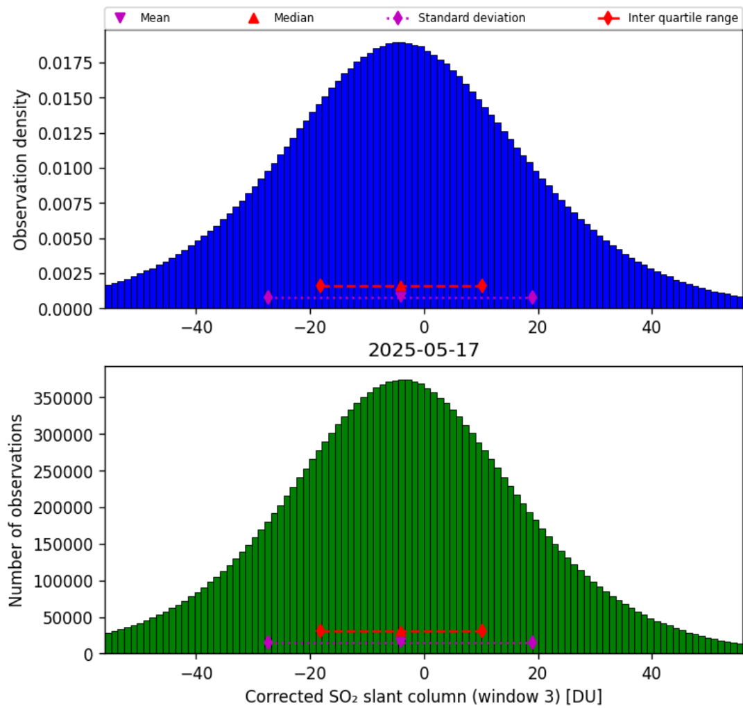
Figure 73: Histogram of “Corrected SO 2 slant column (window 3)” for 2025-05-17 to 2025-05-18
