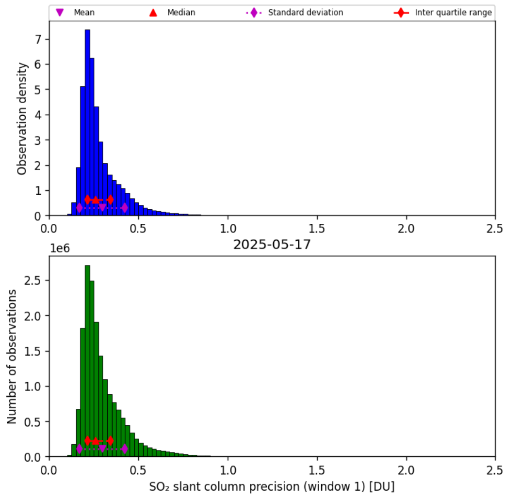
Figure 64: Histogram of “SO 2 slant column precision (window 1)” for 2025-05-17 to 2025-05-18
