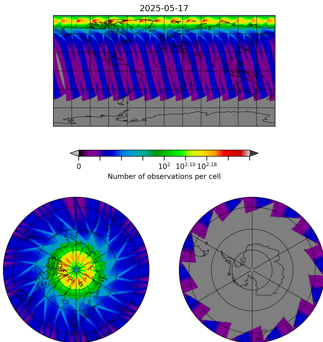
Figure 29: Map of the number of observations for 2025-05-17 to 2025-05-18
