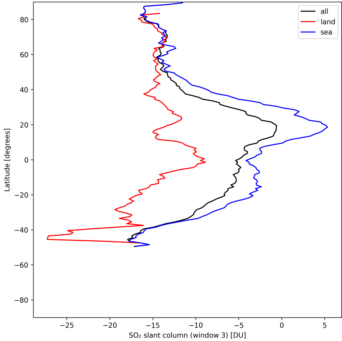
Figure 44: Zonal average of “SO 2 slant column (window 3)” for 2025-05-17 to 2025-05-18.
