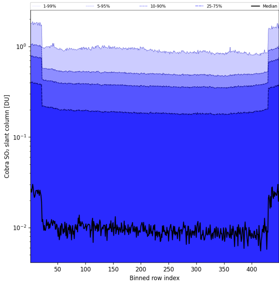
Figure 88: Along track statistics of “Cobra SO 2 slant column” for 2025-05-17 to 2025-05-18
