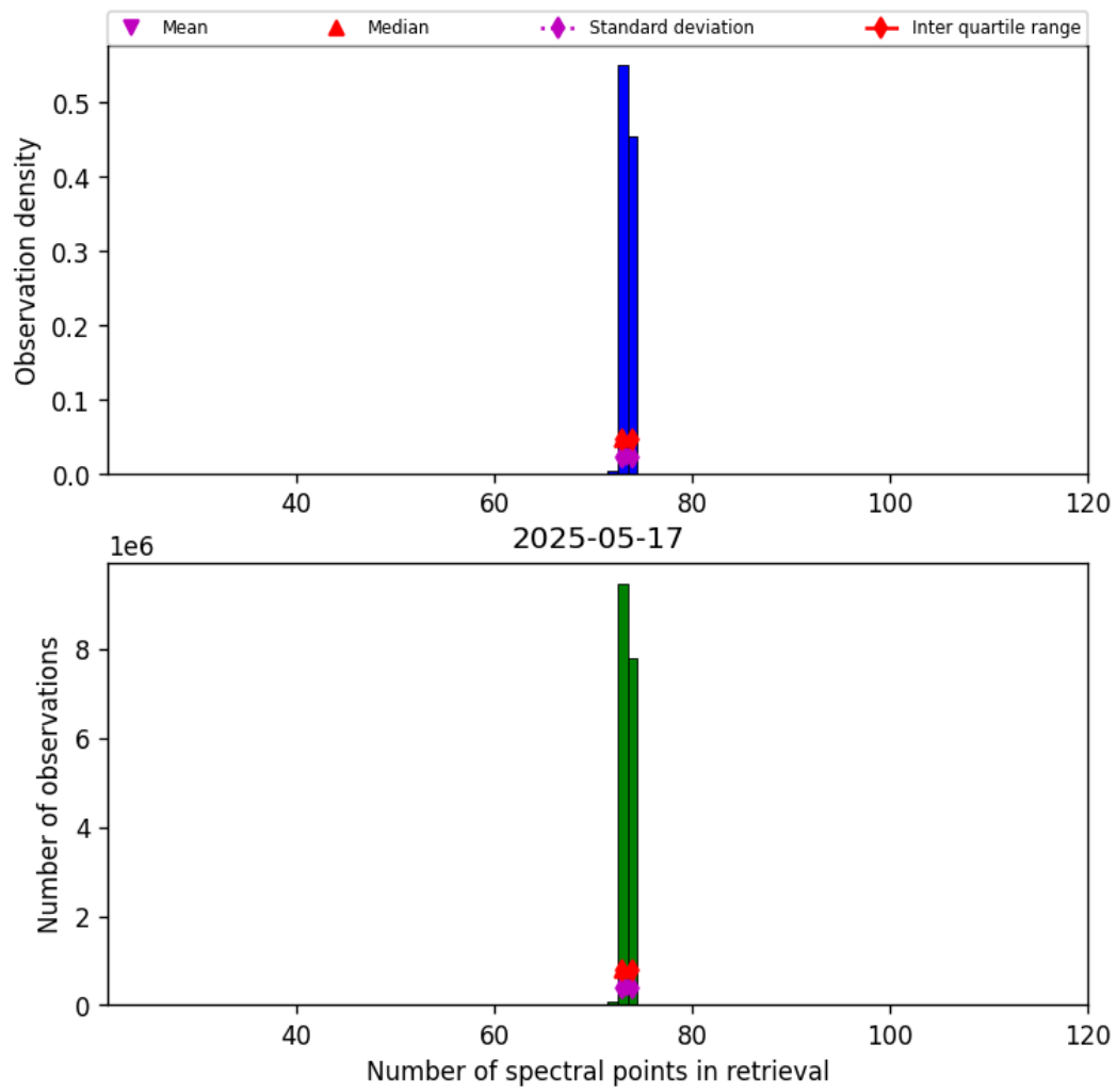
Figure 83: Histogram of “Number of spectral points in retrieval” for 2025-05-17 to 2025-05-18
