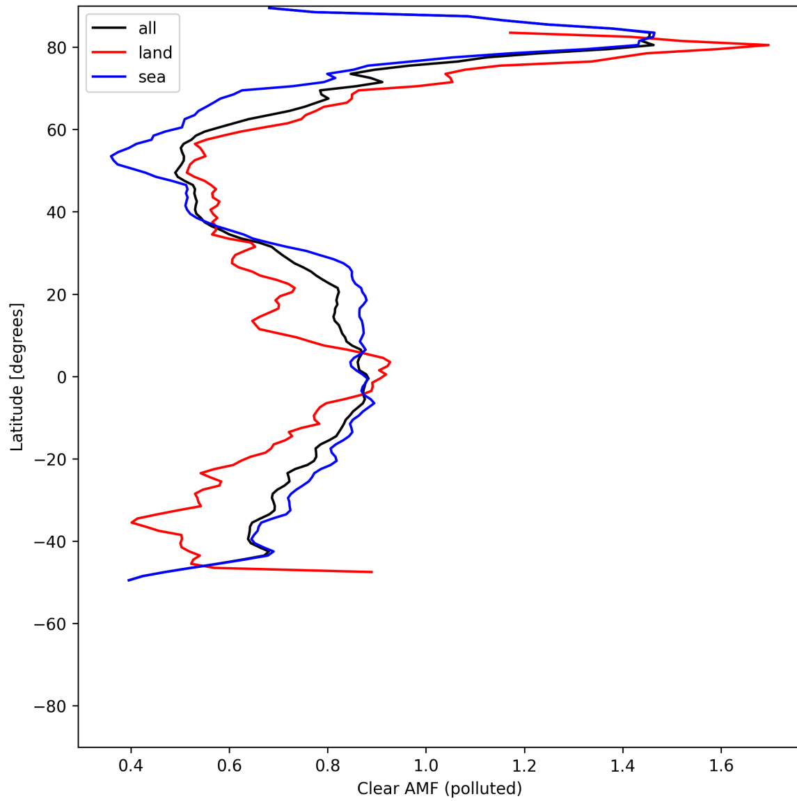
Figure 55: Zonal average of “Clear AMF (polluted)” for 2025-05-17 to 2025-05-18.
