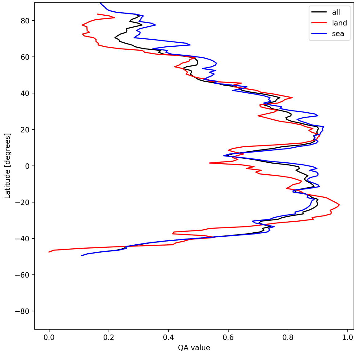
Figure 30: Zonal average of “QA value” for 2025-05-17 to 2025-05-18.
