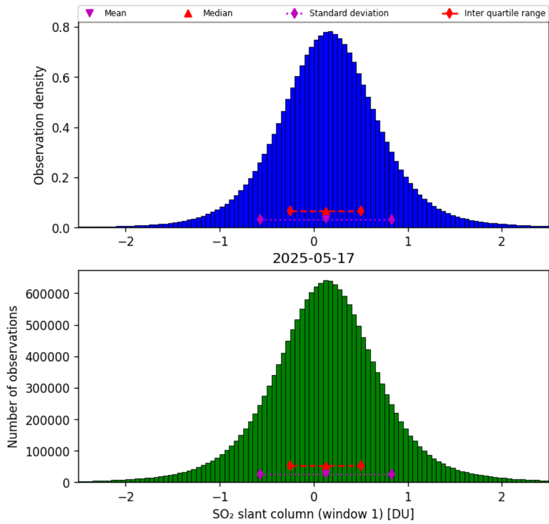
Figure 63: Histogram of “SO 2 slant column (window 1)” for 2025-05-17 to 2025-05-18
