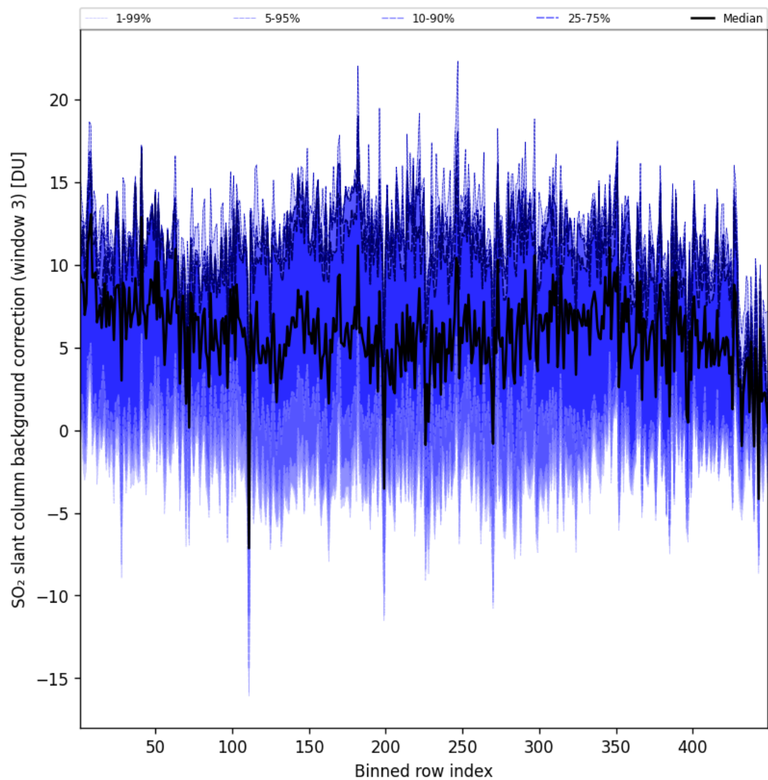
Figure 101: Along track statistics of “SO 2 slant column background correction (window 3)” for 2025-05-17 to 2025-05-18
