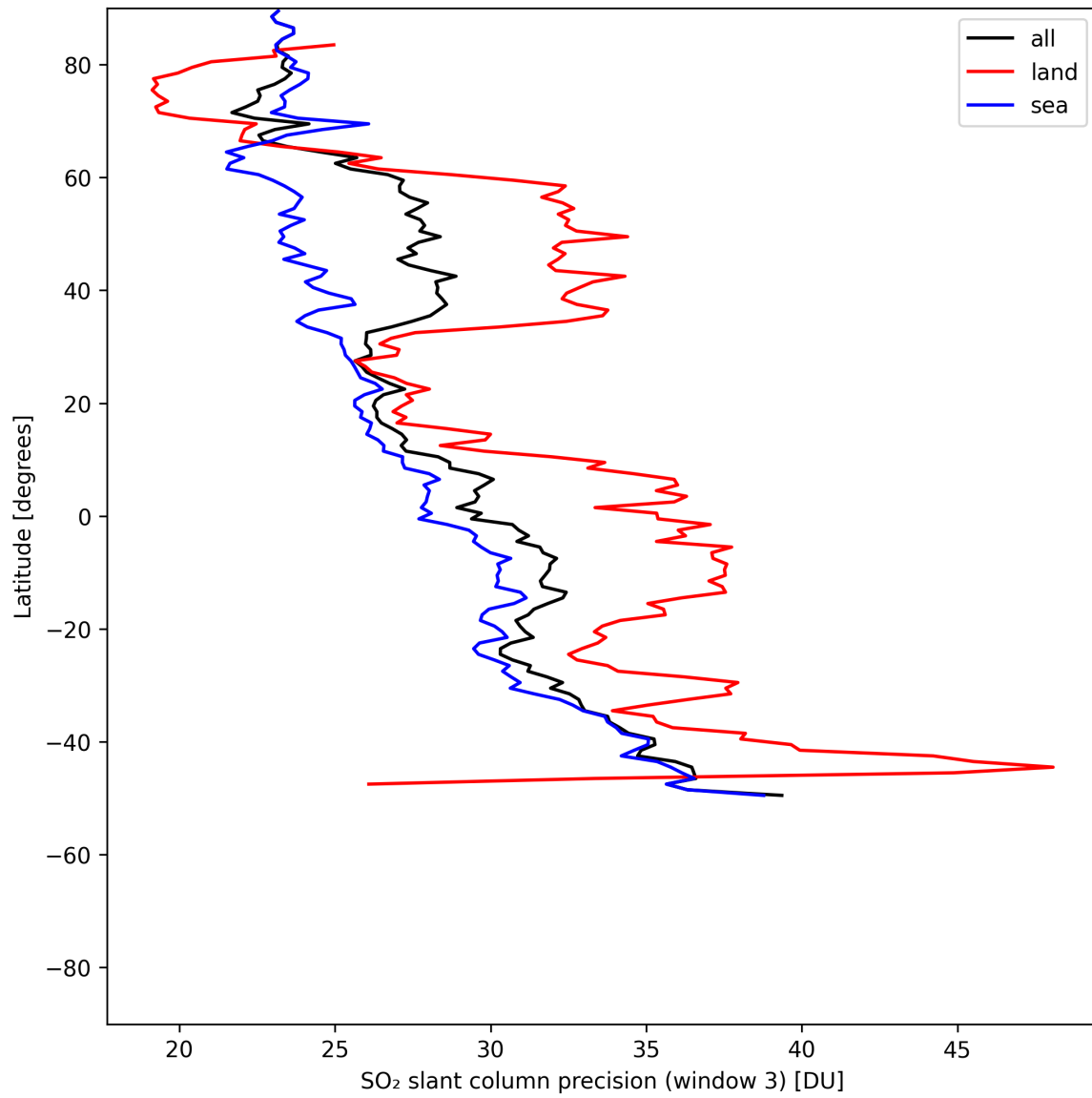
Figure 45: Zonal average of “SO 2 slant column precision (window 3)” for 2025-05-17 to 2025-05-18.
