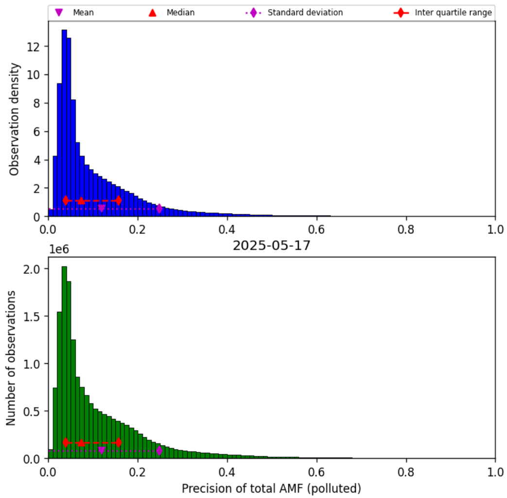
Figure 81: Histogram of “Precision of total AMF (polluted)” for 2025-05-17 to 2025-05-18
