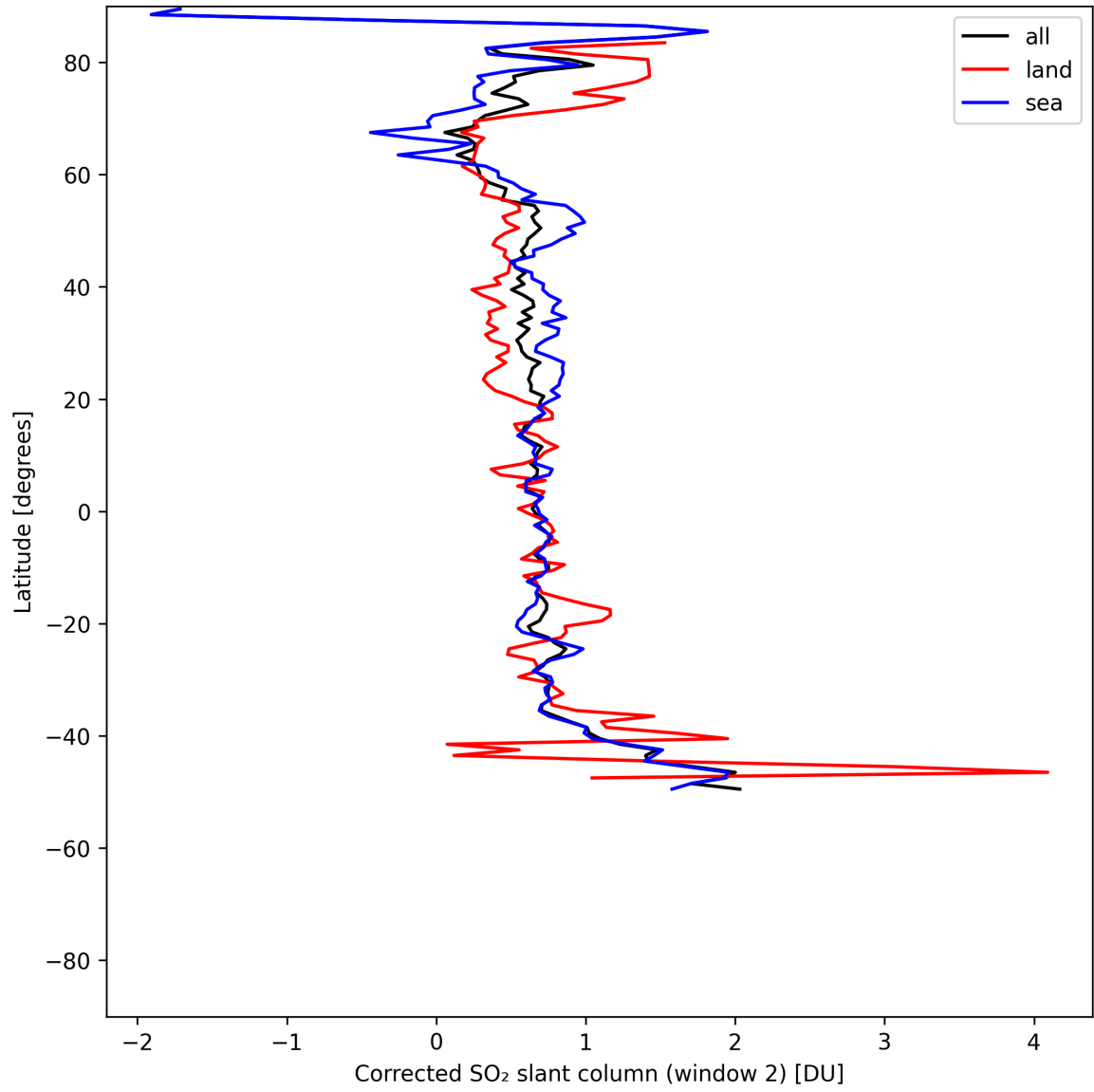
Figure 42: Zonal average of “Corrected SO 2 slant column (window 2)” for 2025-05-17 to 2025-05-18.
