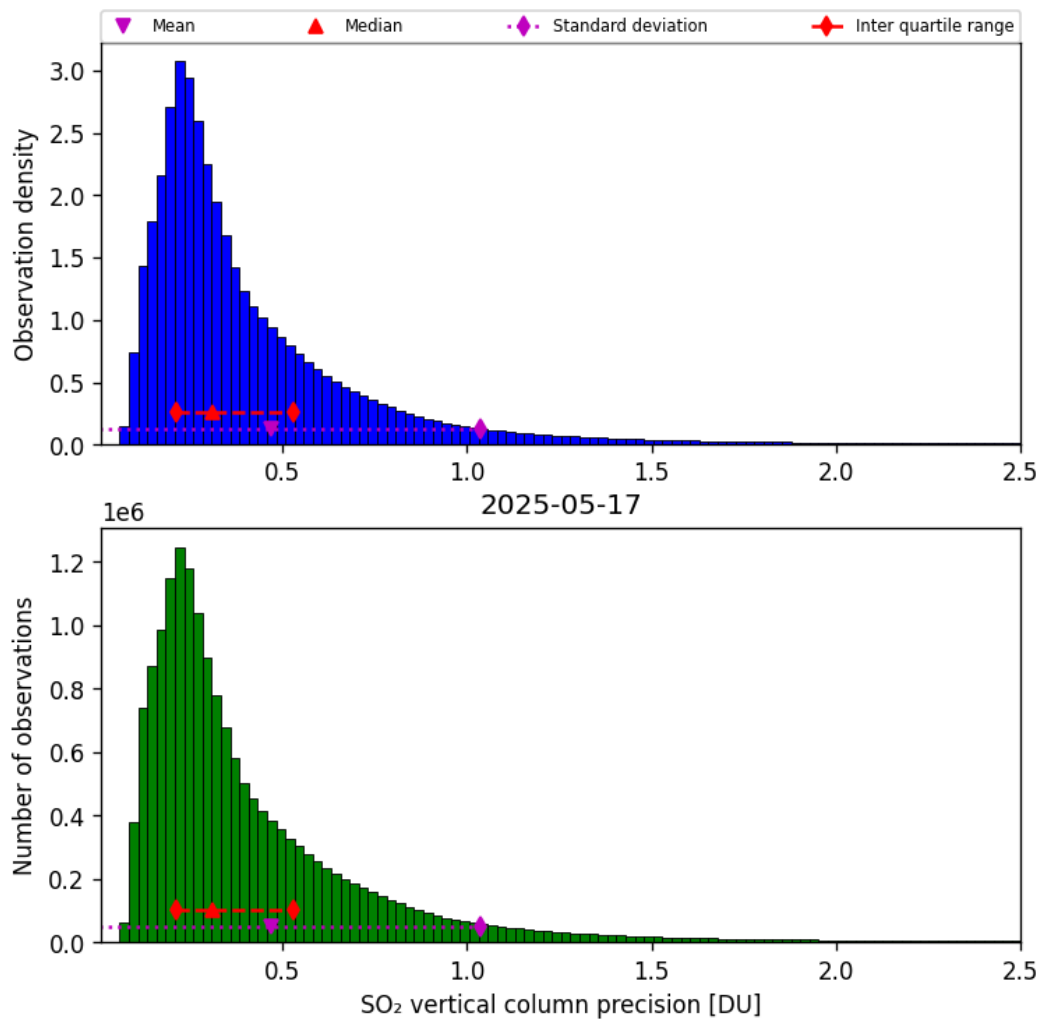
Figure 59: Histogram of “SO 2 vertical column precision” for 2025-05-17 to 2025-05-18
