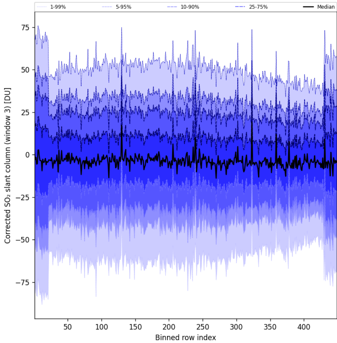
Figure 100: Along track statistics of “Corrected SO 2 slant column (window 3)” for 2025-05-17 to 2025-05-18
