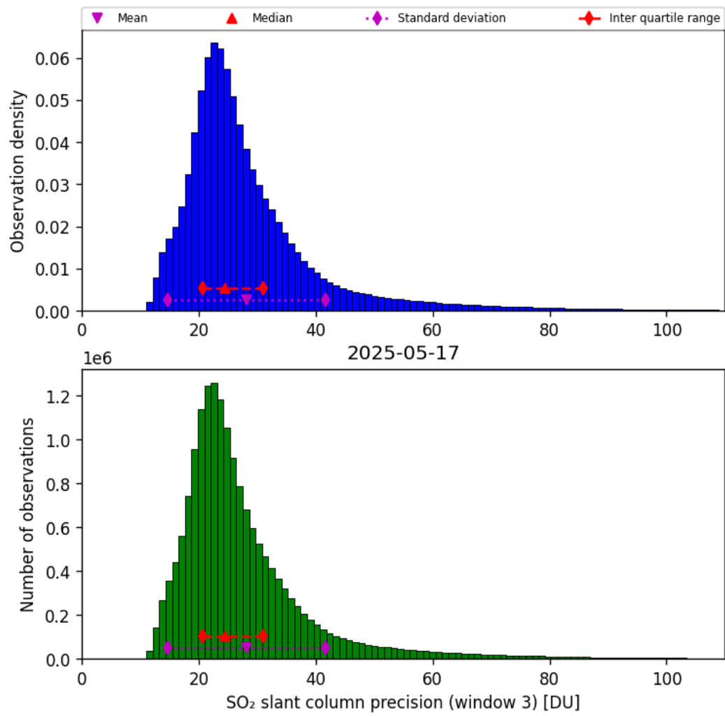
Figure 72: Histogram of “SO 2 slant column precision (window 3)” for 2025-05-17 to 2025-05-18
