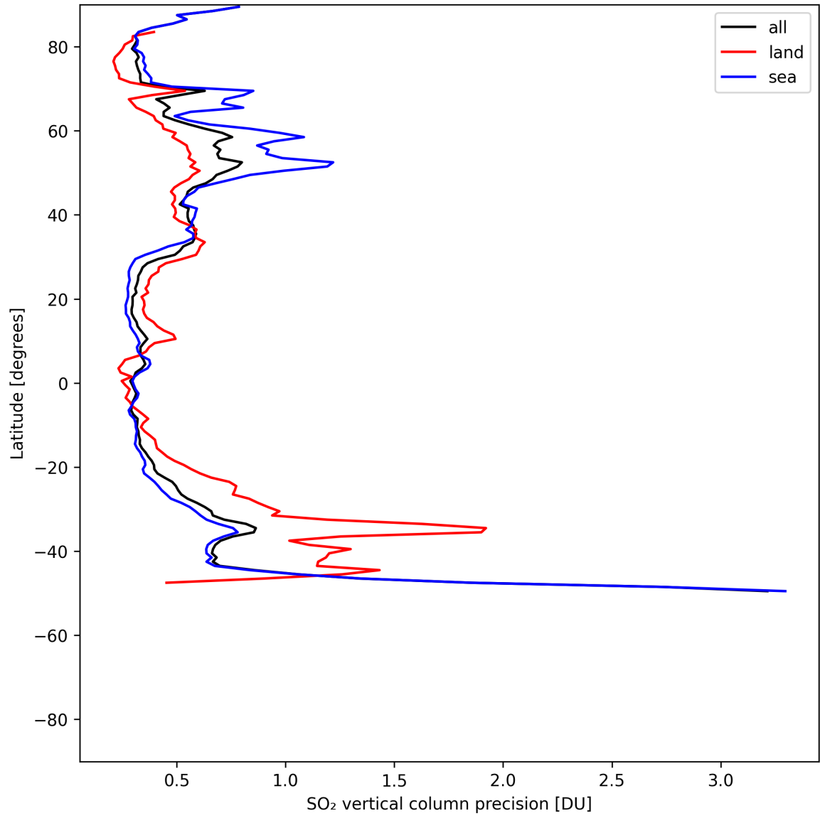
Figure 32: Zonal average of “SO 2 vertical column precision” for 2025-05-17 to 2025-05-18.
