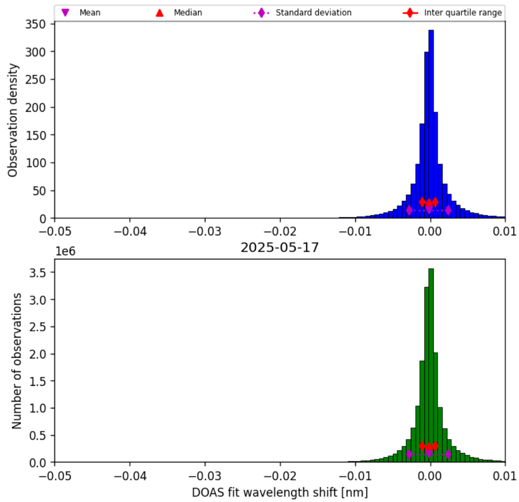
Figure 77: Histogram of “DOAS fit wavelength shift” for 2025-05-17 to 2025-05-18
