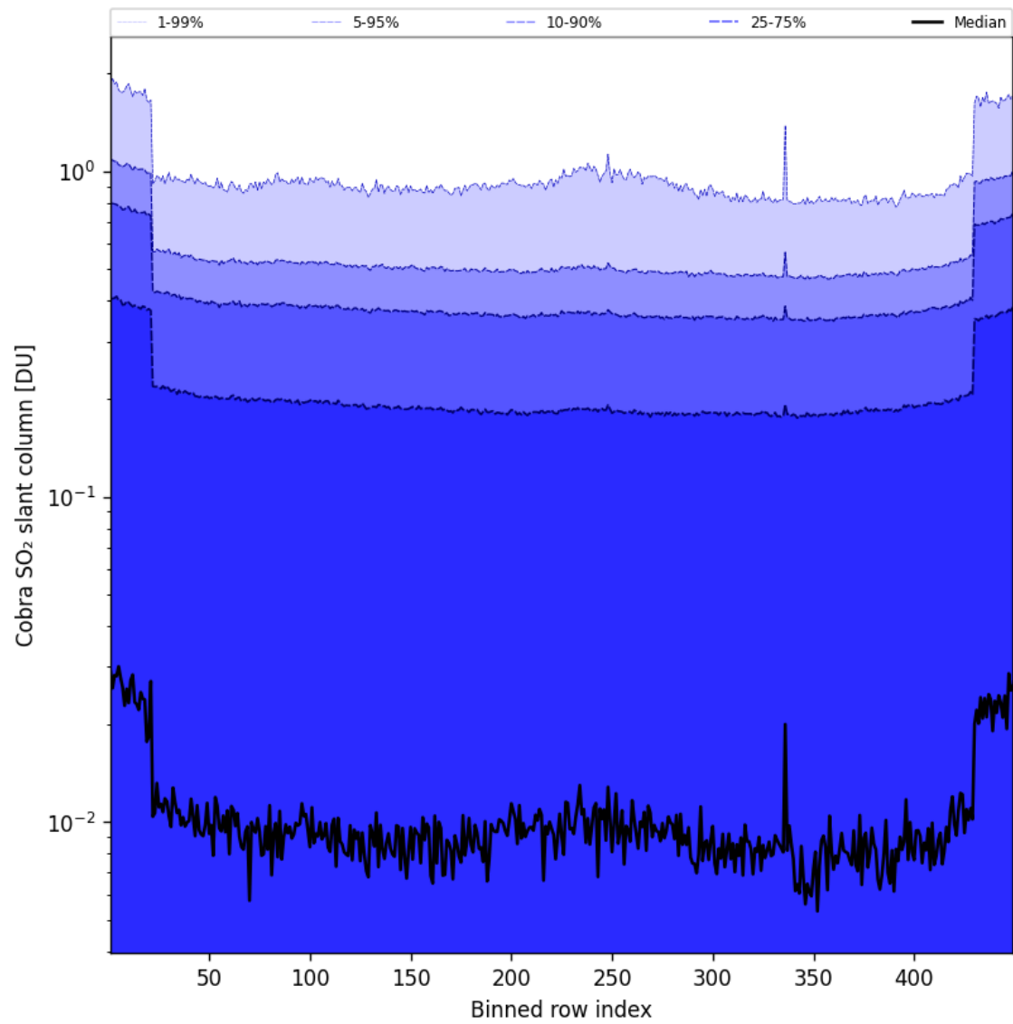
Figure 88: Along track statistics of “Cobra SO 2 slant column” for 2025-05-19 to 2025-05-19
