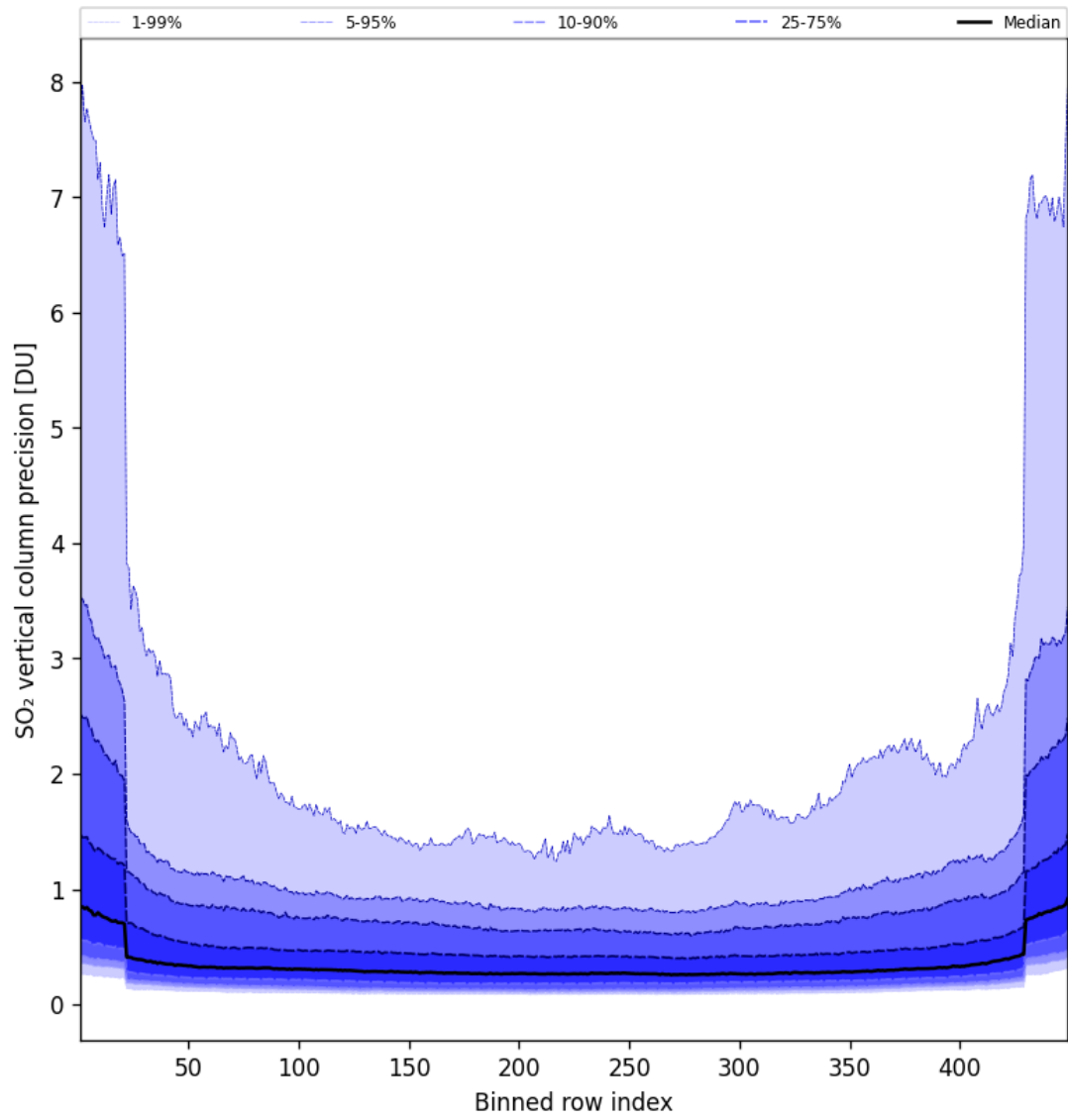
Figure 86: Along track statistics of “SO 2 vertical column precision” for 2025-05-19 to 2025-05-19
