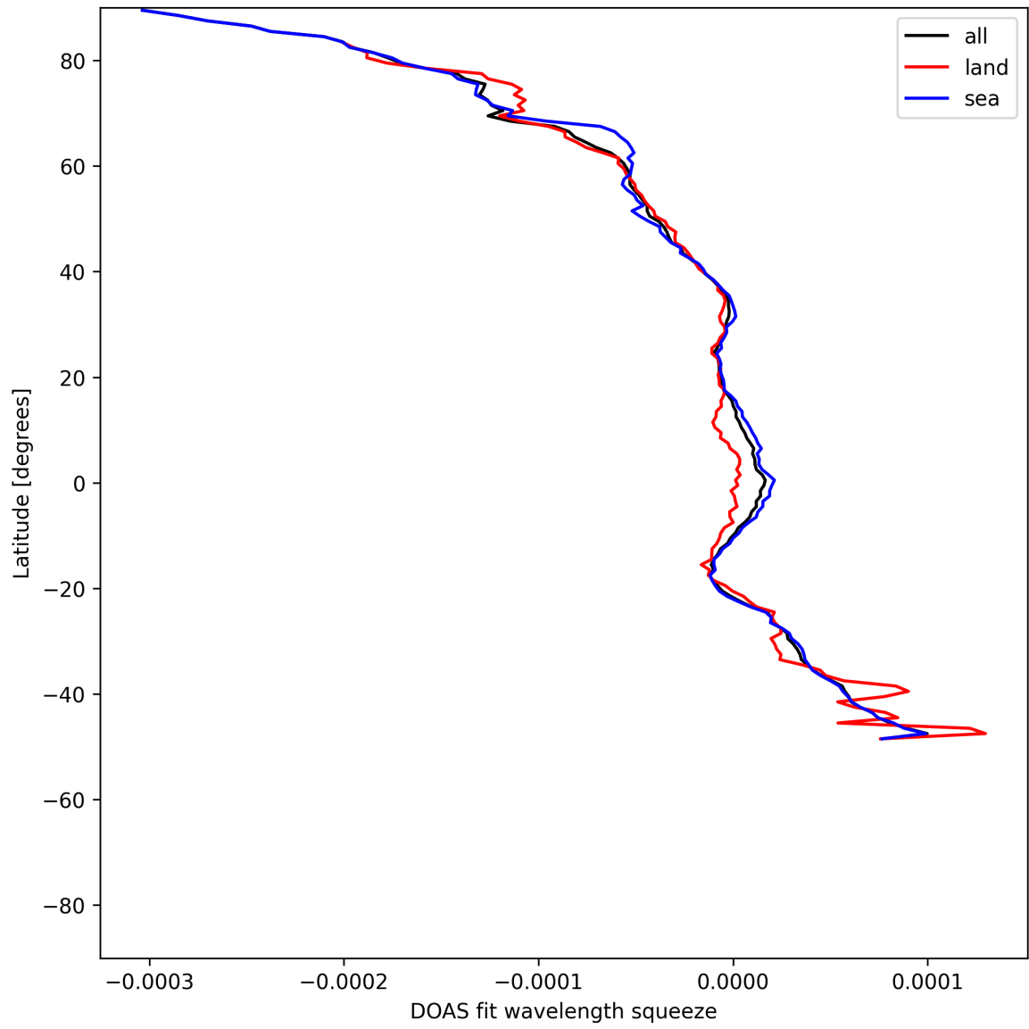
Figure 51: Zonal average of “DOAS fit wavelength squeeze” for 2025-05-19 to 2025-05-19.
