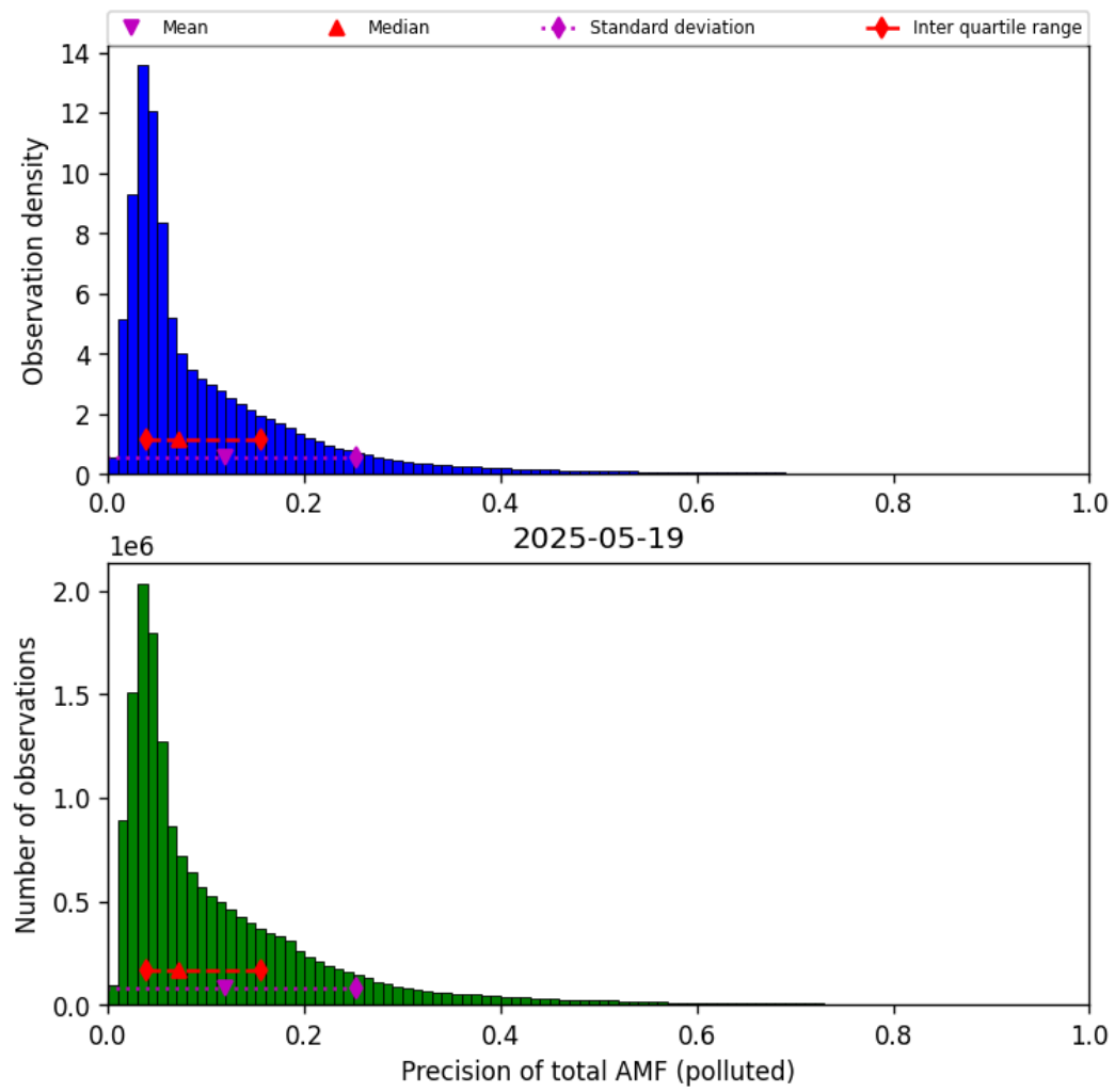
Figure 81: Histogram of “Precision of total AMF (polluted)” for 2025-05-19 to 2025-05-19
