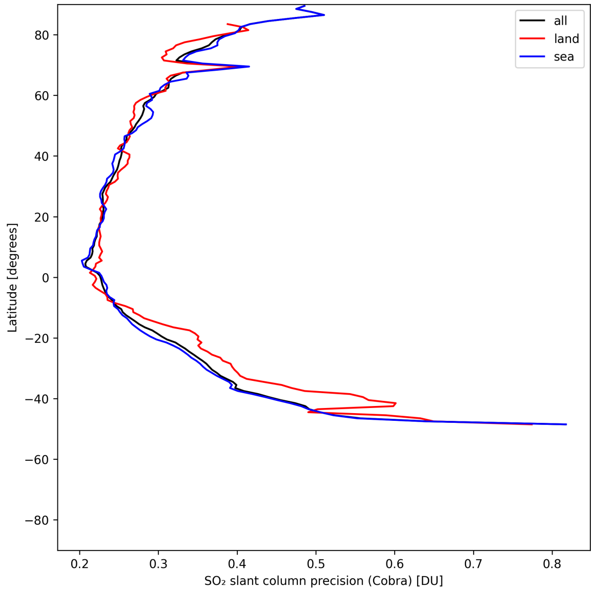
Figure 35: Zonal average of “SO 2 slant column precision (Cobra)” for 2025-05-19 to 2025-05-19.
