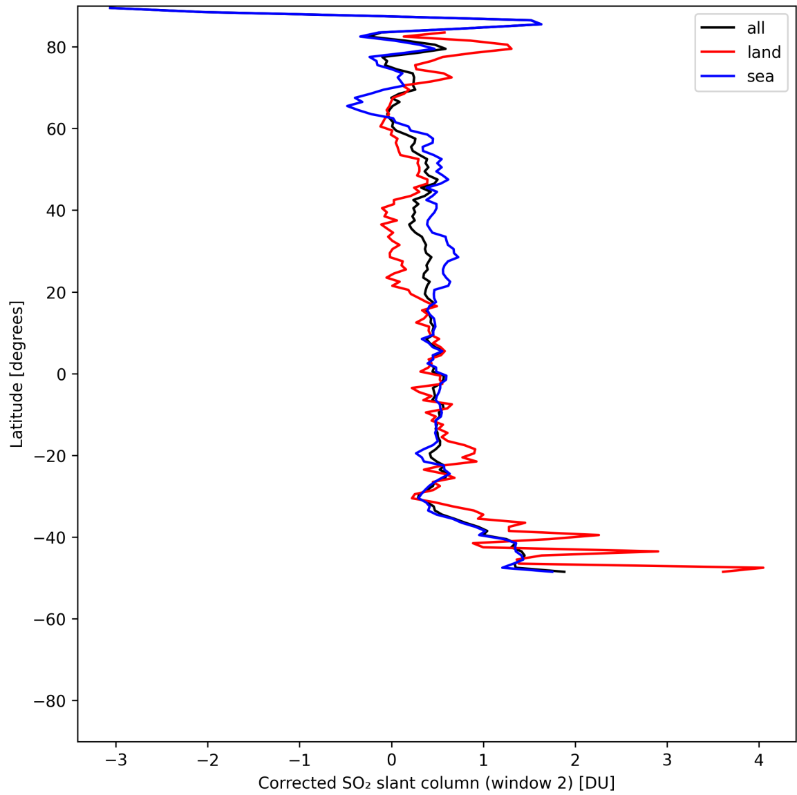
Figure 42: Zonal average of “Corrected SO 2 slant column (window 2)” for 2025-05-19 to 2025-05-19.
