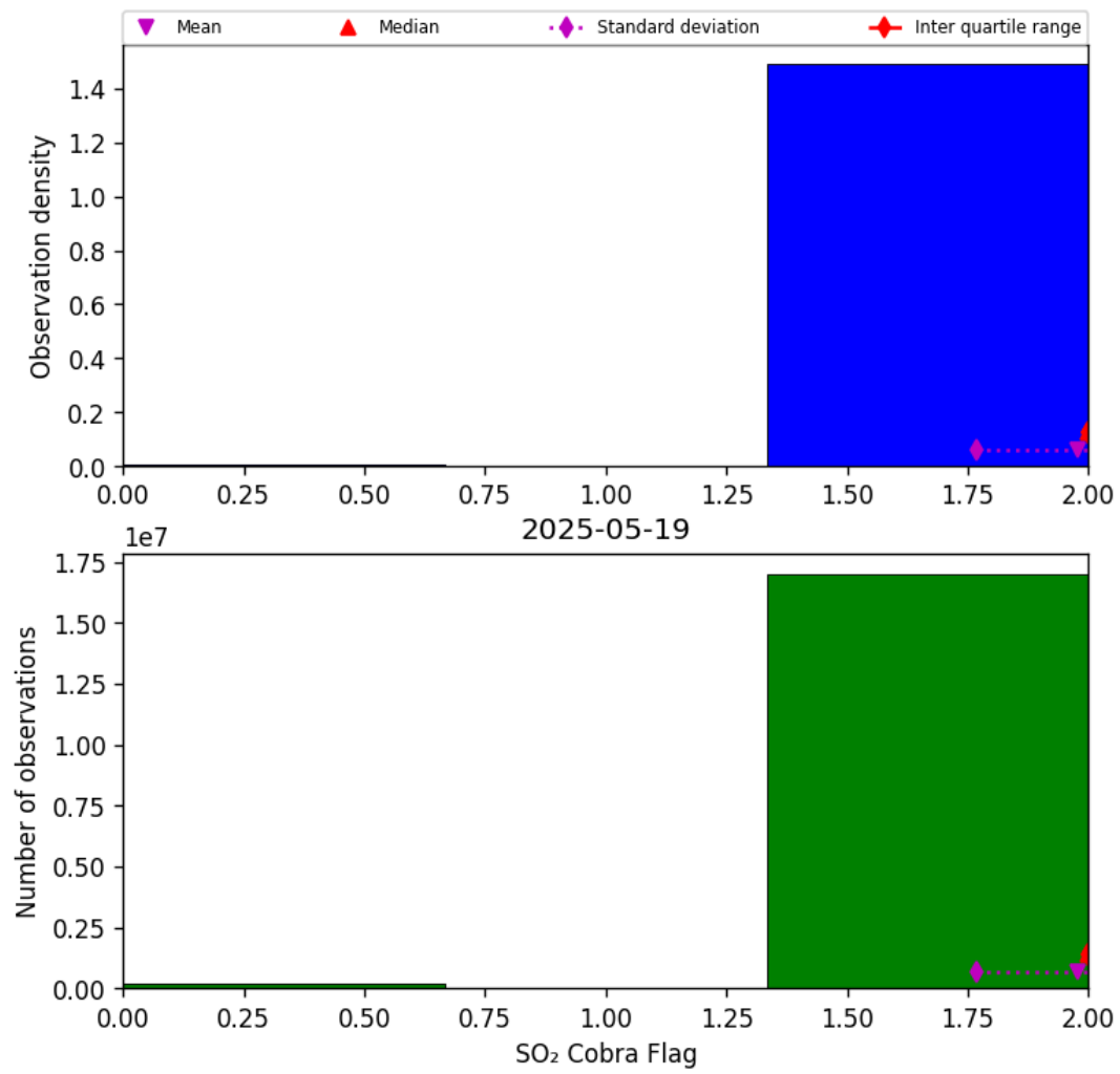
Figure 75: Histogram of “SO 2 Cobra Flag” for 2025-05-19 to 2025-05-19
