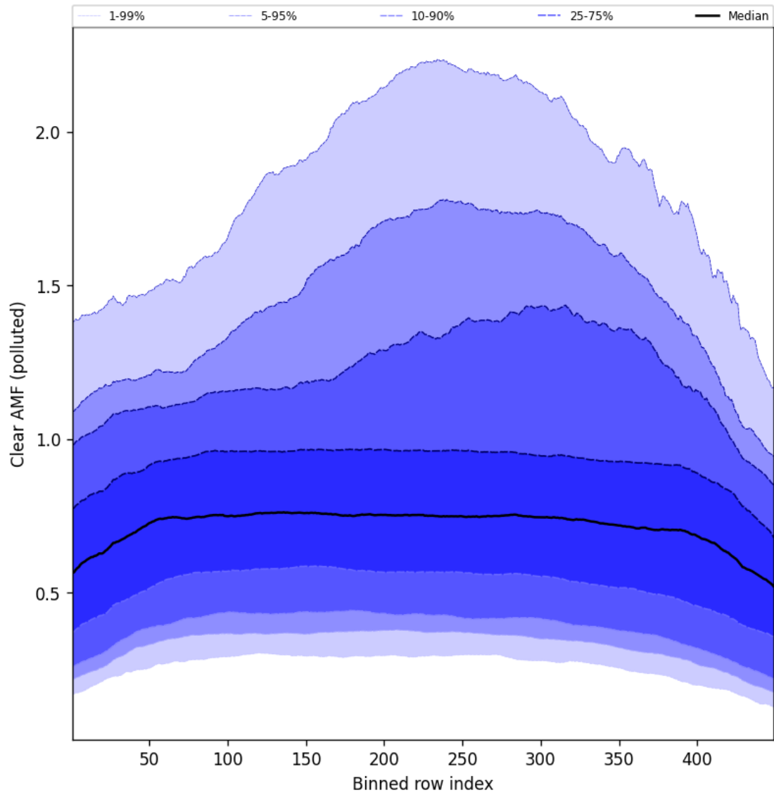
Figure 109: Along track statistics of “Clear AMF (polluted)” for 2025-05-19 to 2025-05-19
