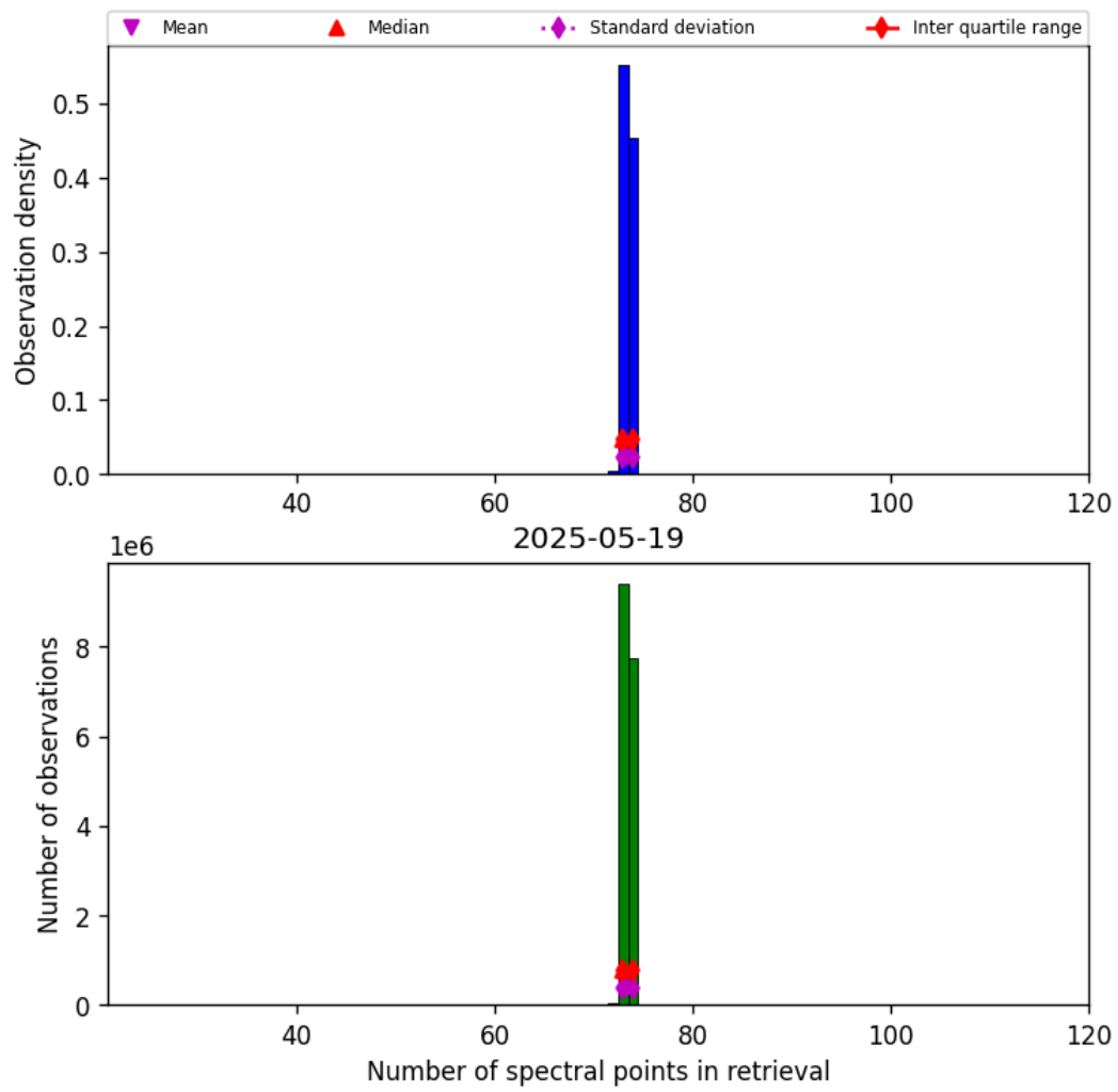
Figure 83: Histogram of “Number of spectral points in retrieval” for 2025-05-19 to 2025-05-19
