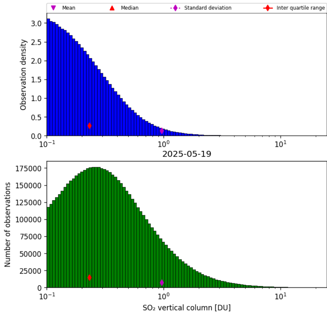
Figure 58: Histogram of “SO 2 vertical column” for 2025-05-19 to 2025-05-19
