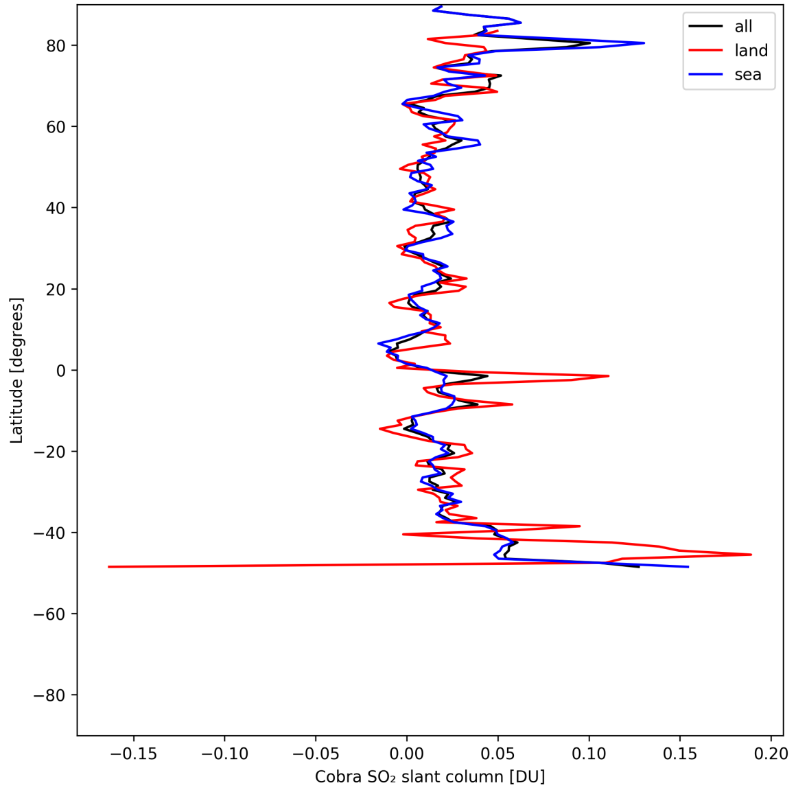
Figure 34: Zonal average of “Cobra SO 2 slant column” for 2025-05-19 to 2025-05-19.
