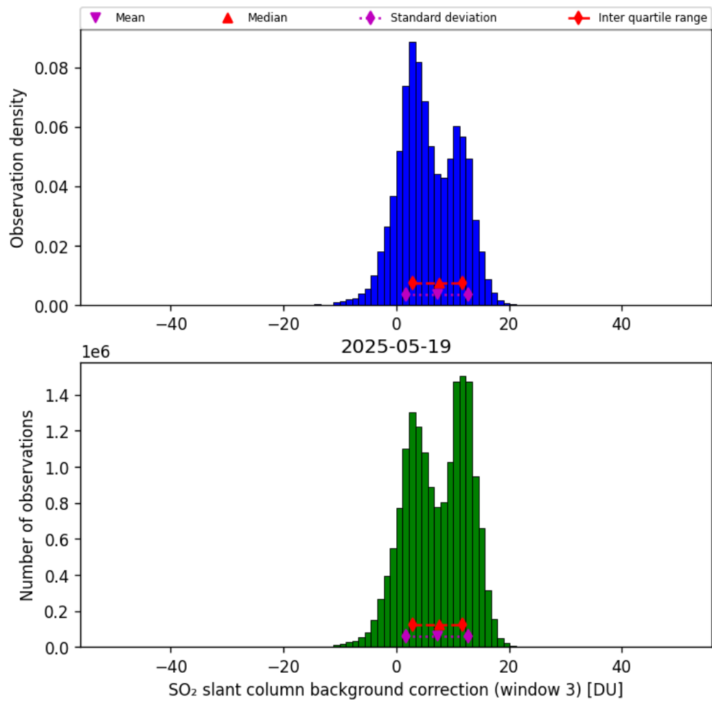
Figure 74: Histogram of “SO 2 slant column background correction (window 3)” for 2025-05-19 to 2025-05-19
