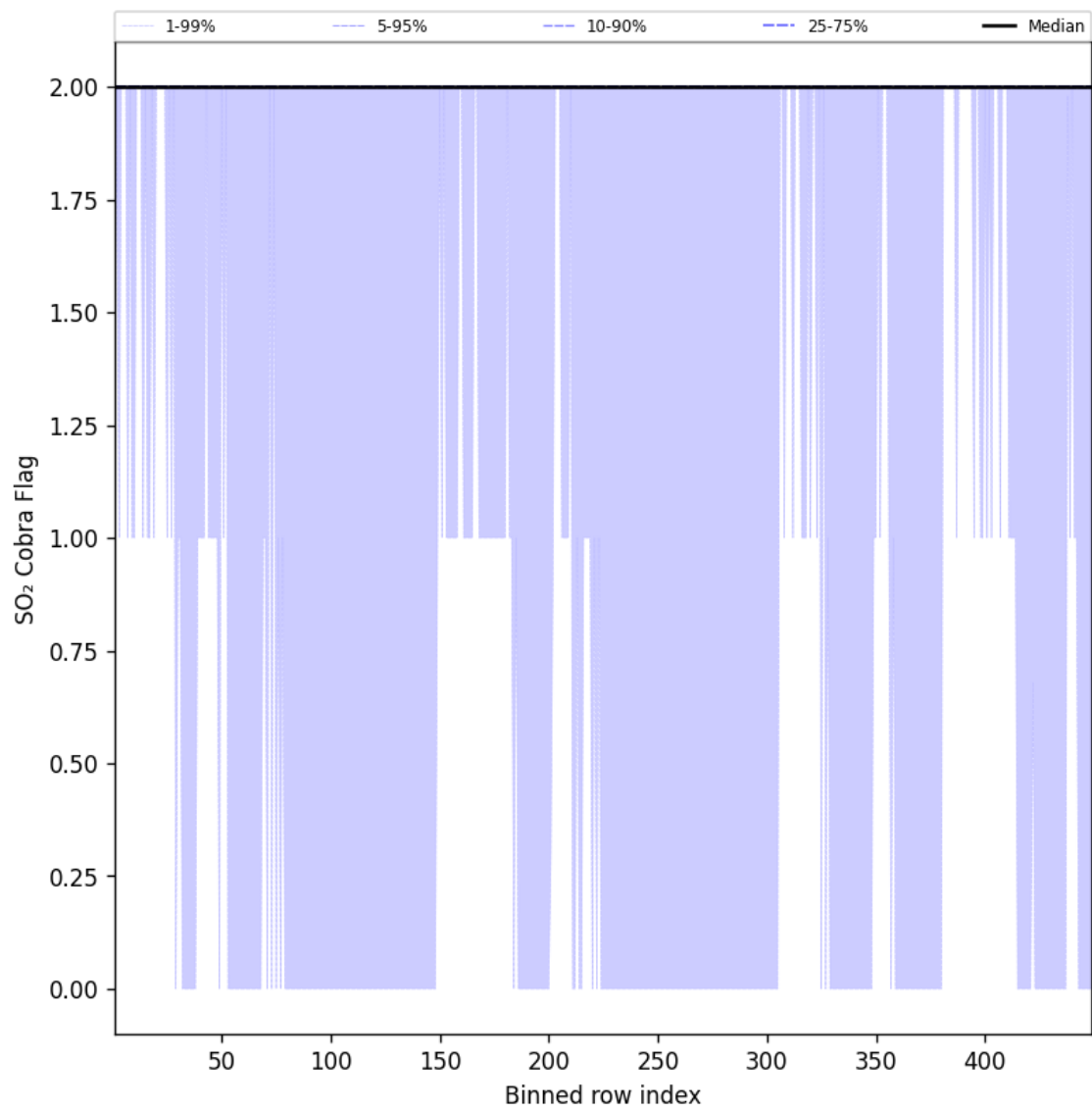
Figure 102: Along track statistics of "SO 2 Cobra Flag" for 2025-05-19 to 2025-05-19
