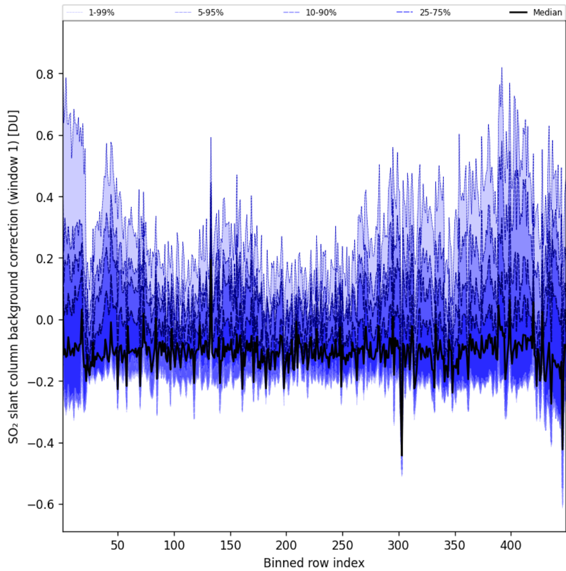
Figure 93: Along track statistics of “SO 2 slant column background correction (window 1)” for 2025-05-19 to 2025-05-19
