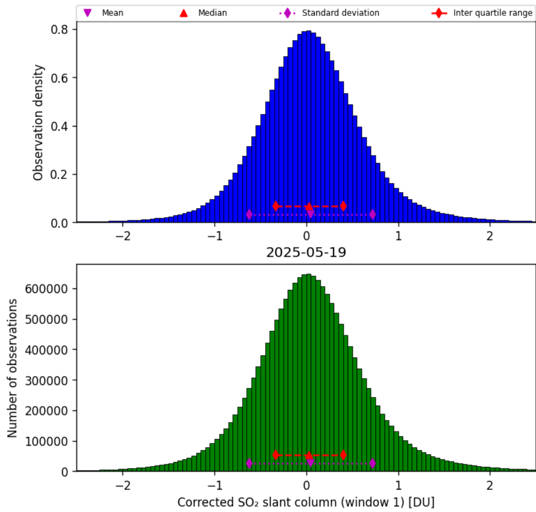
Figure 65: Histogram of “Corrected SO 2 slant column (window 1)” for 2025-05-19 to 2025-05-19
