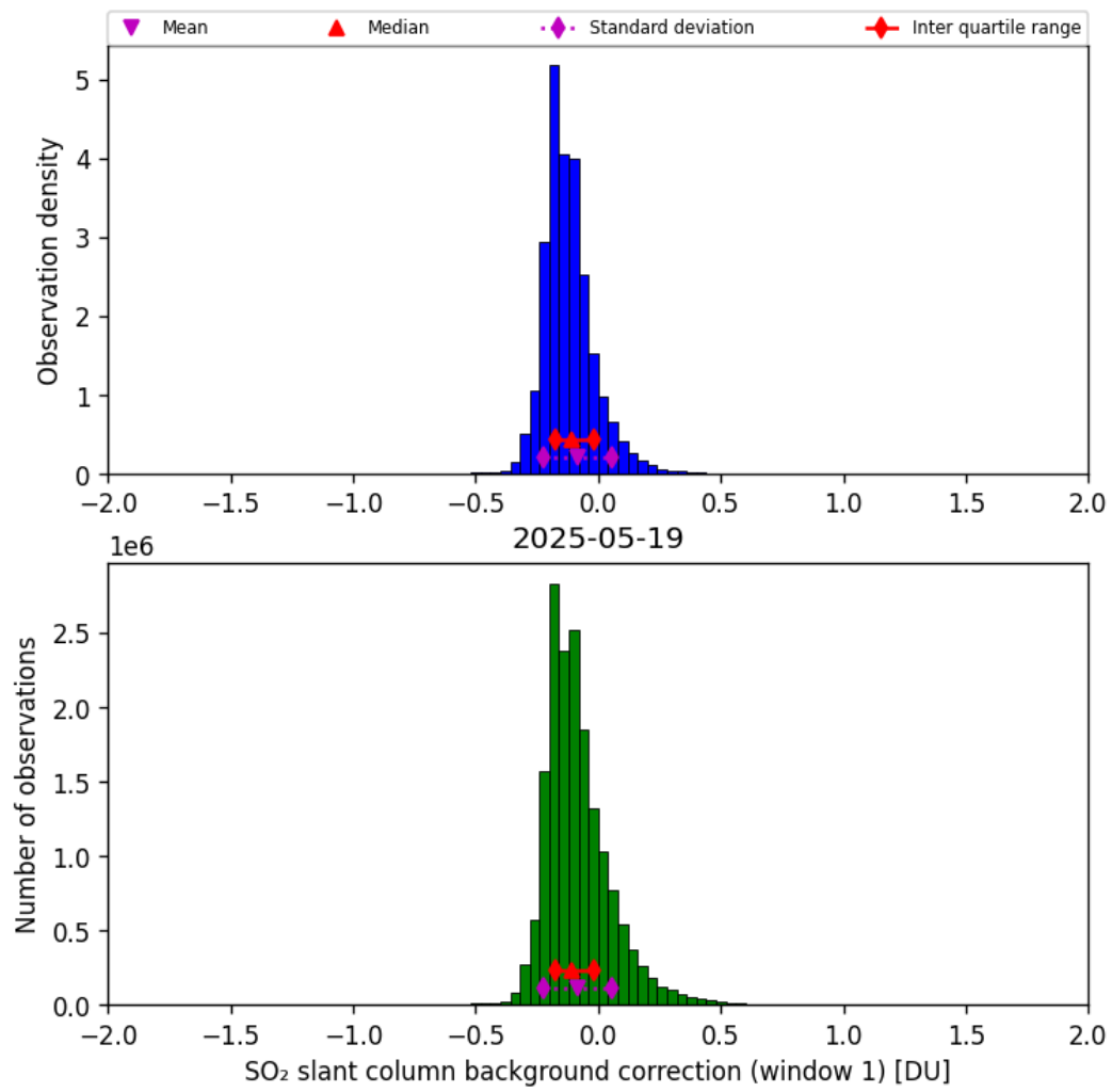
Figure 66: Histogram of “SO 2 slant column background correction (window 1)” for 2025-05-19 to 2025-05-19
