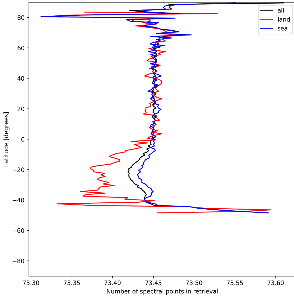
Figure 56: Zonal average of “Number of spectral points in retrieval” for 2025-05-19 to 2025-05-19.
