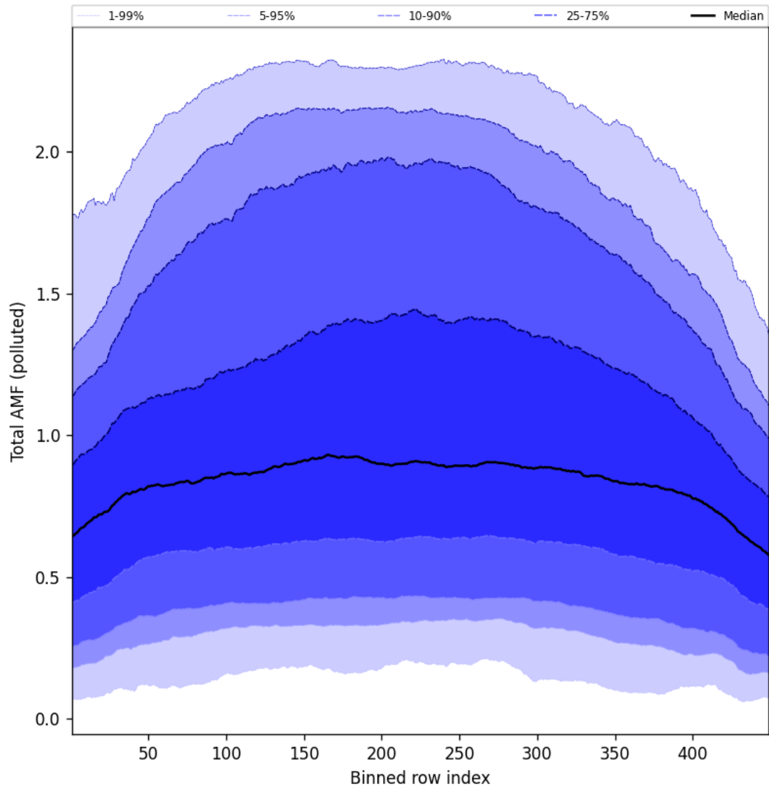
Figure 107: Along track statistics of “Total AMF (polluted)” for 2025-05-19 to 2025-05-19
