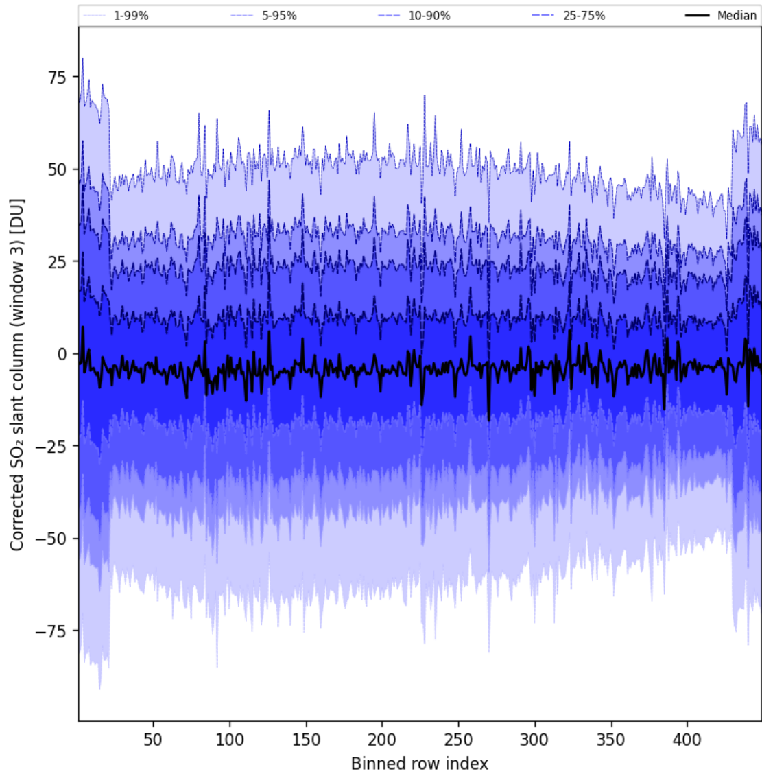
Figure 100: Along track statistics of “Corrected SO 2 slant column (window 3)” for 2025-05-19 to 2025-05-19
