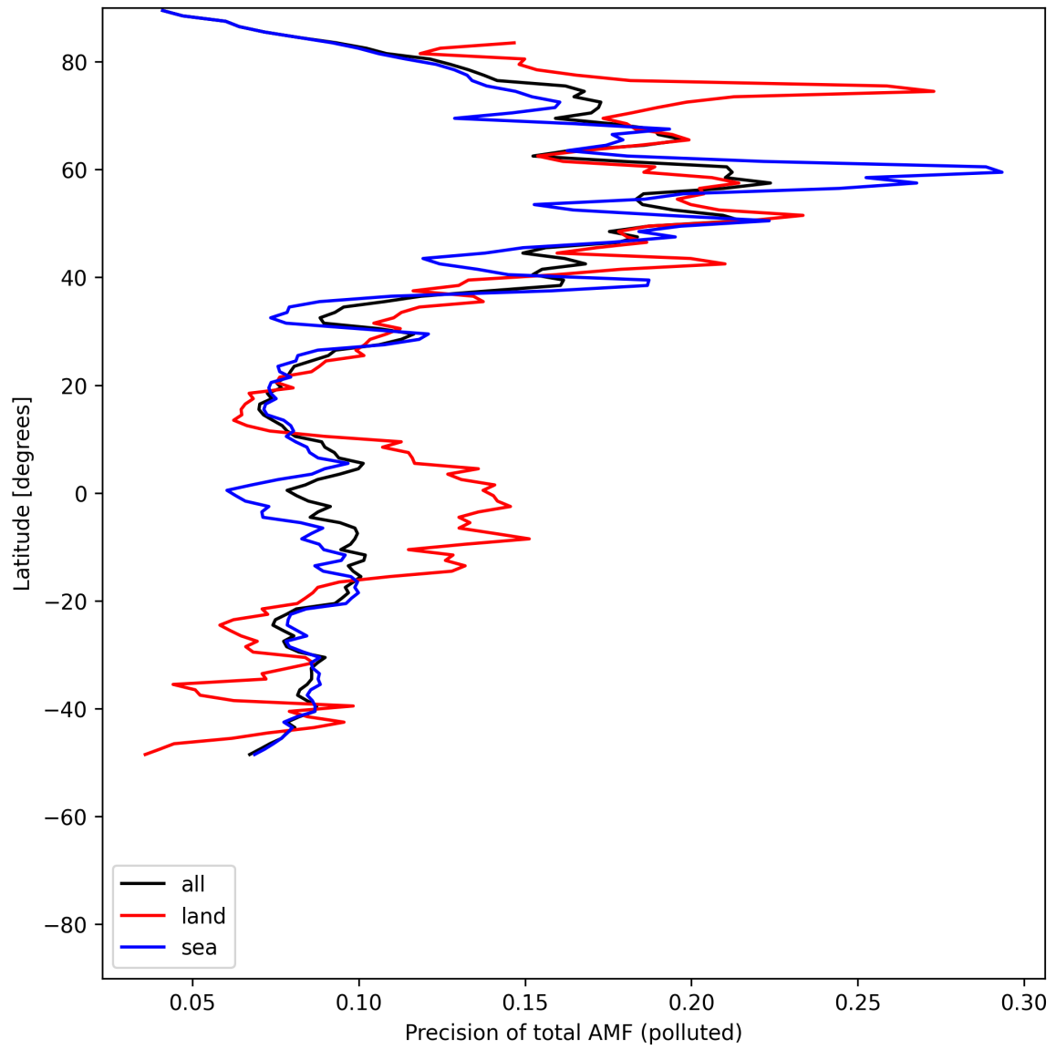
Figure 54: Zonal average of “Precision of total AMF (polluted)” for 2025-05-19 to 2025-05-19.
