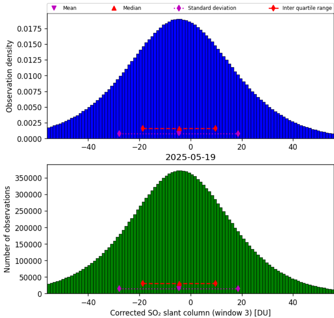
Figure 73: Histogram of “Corrected SO 2 slant column (window 3)” for 2025-05-19 to 2025-05-19
