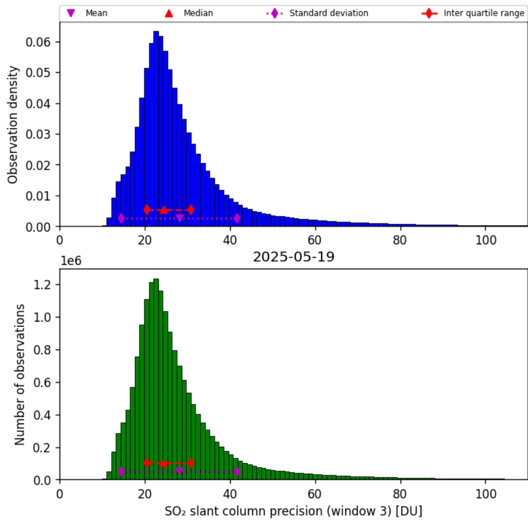
Figure 72: Histogram of “SO 2 slant column precision (window 3)” for 2025-05-19 to 2025-05-19
