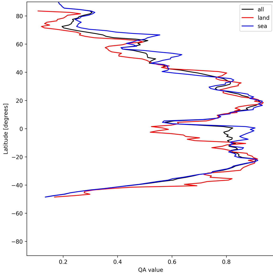
Figure 30: Zonal average of “QA value” for 2025-05-19 to 2025-05-19.
