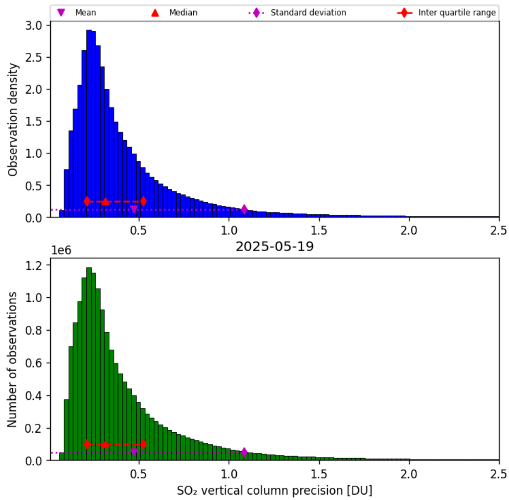
Figure 59: Histogram of “SO 2 vertical column precision” for 2025-05-19 to 2025-05-19
