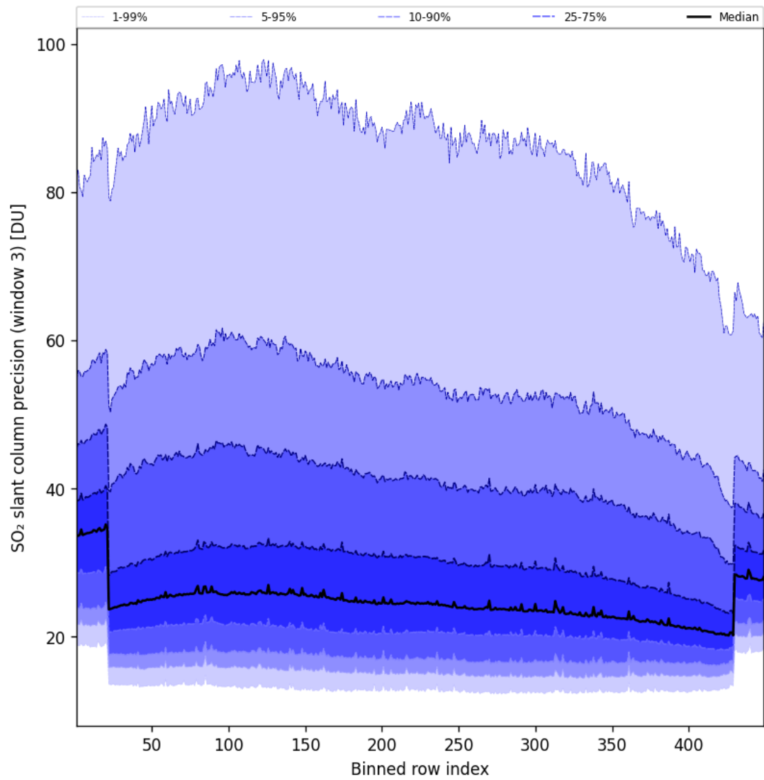
Figure 99: Along track statistics of “SO 2 slant column precision (window 3)” for 2025-05-19 to 2025-05-19
