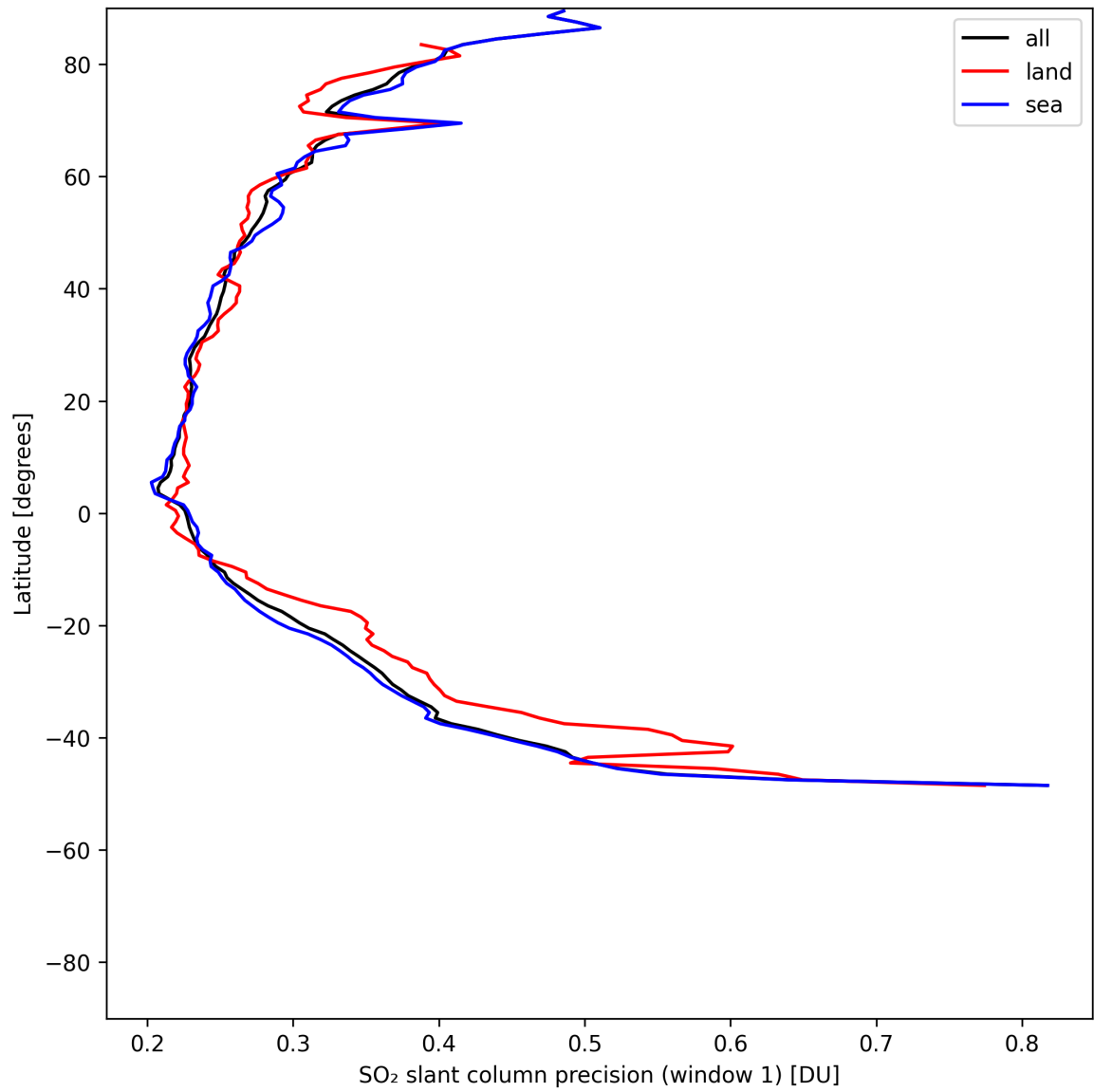
Figure 37: Zonal average of “SO 2 slant column precision (window 1)” for 2025-05-19 to 2025-05-19.
