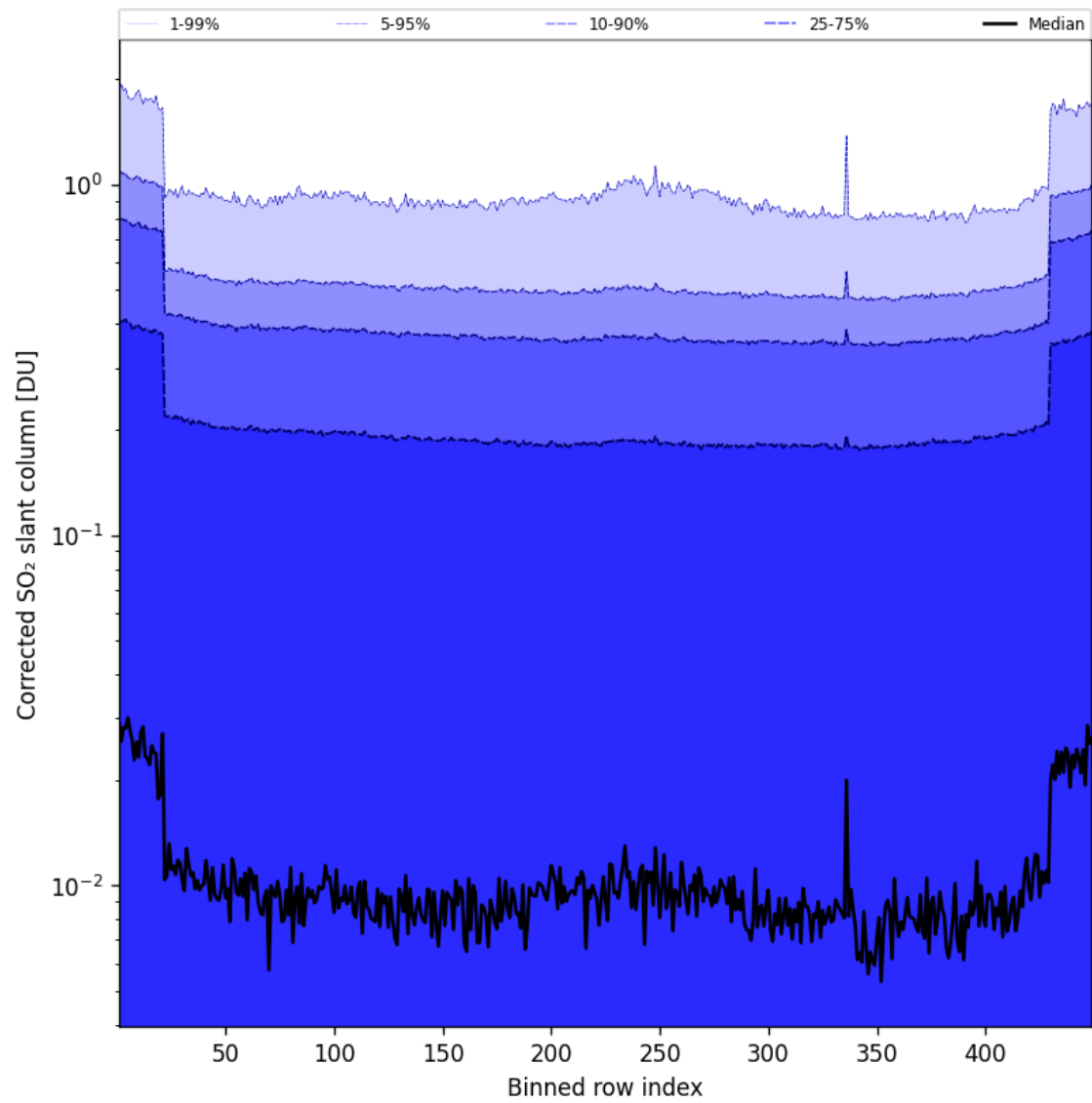
Figure 87: Along track statistics of “Corrected SO 2 slant column” for 2025-05-19 to 2025-05-19
