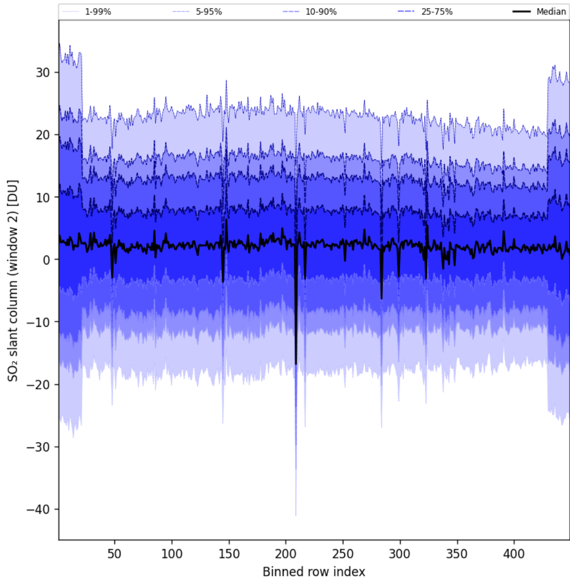
Figure 94: Along track statistics of “SO 2 slant column (window 2)” for 2025-05-19 to 2025-05-19
