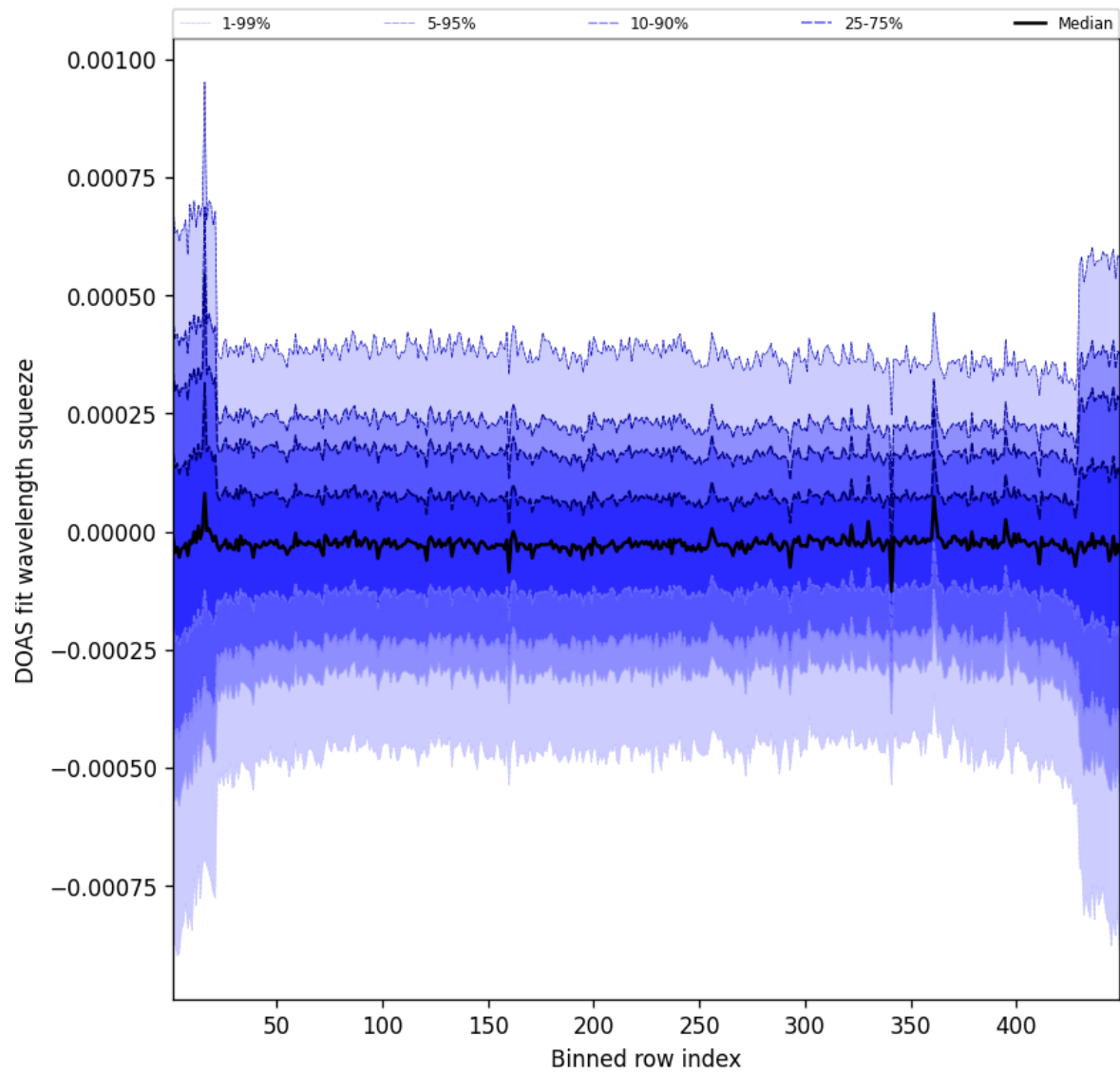
Figure 105: Along track statistics of “DOAS fit wavelength squeeze” for 2025-05-19 to 2025-05-19
