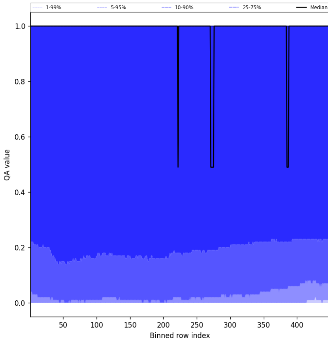
Figure 84: Along track statistics of “QA value” for 2025-05-19 to 2025-05-19
