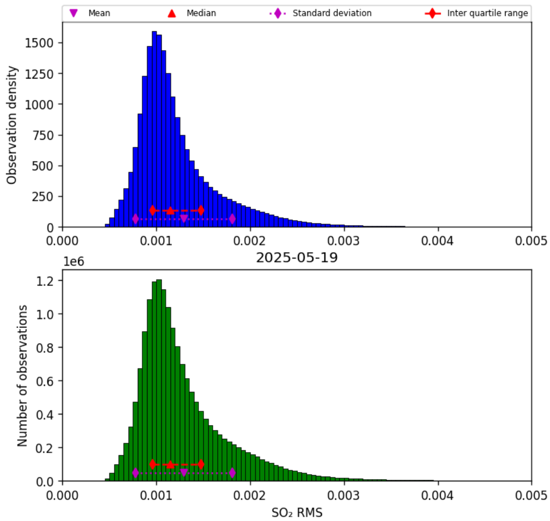
Figure 79: Histogram of “SO 2 RMS” for 2025-05-19 to 2025-05-19
