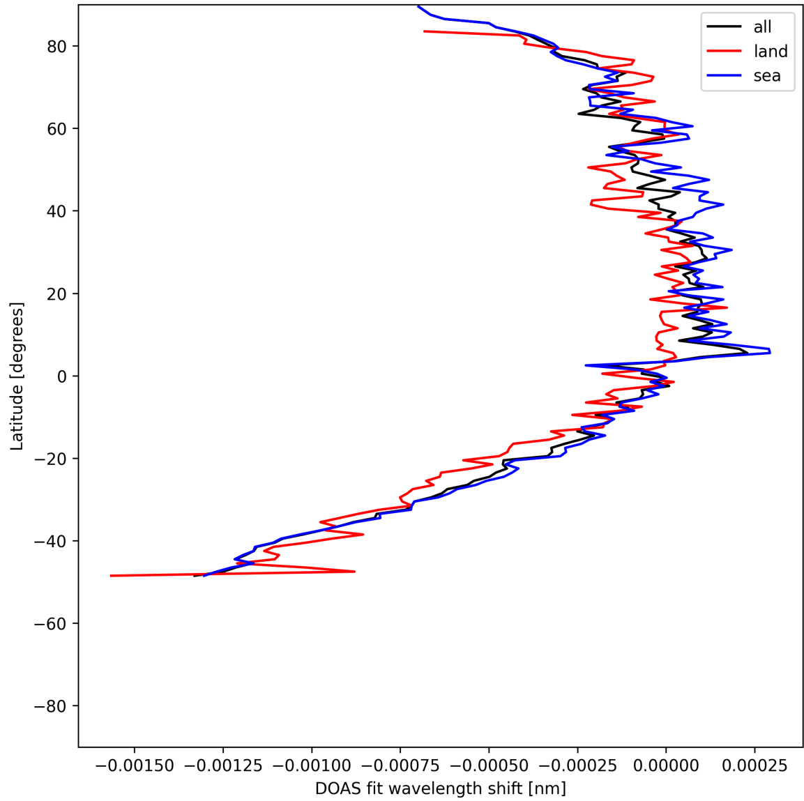
Figure 50: Zonal average of “DOAS fit wavelength shift” for 2025-05-19 to 2025-05-19.
