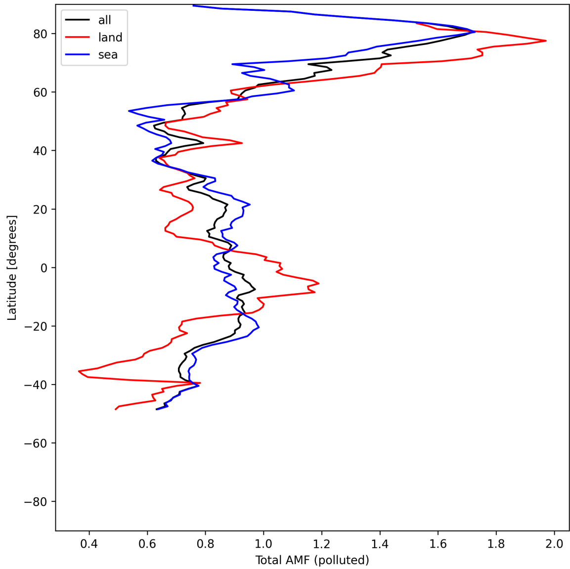
Figure 53: Zonal average of “Total AMF (polluted)” for 2025-05-19 to 2025-05-19.
