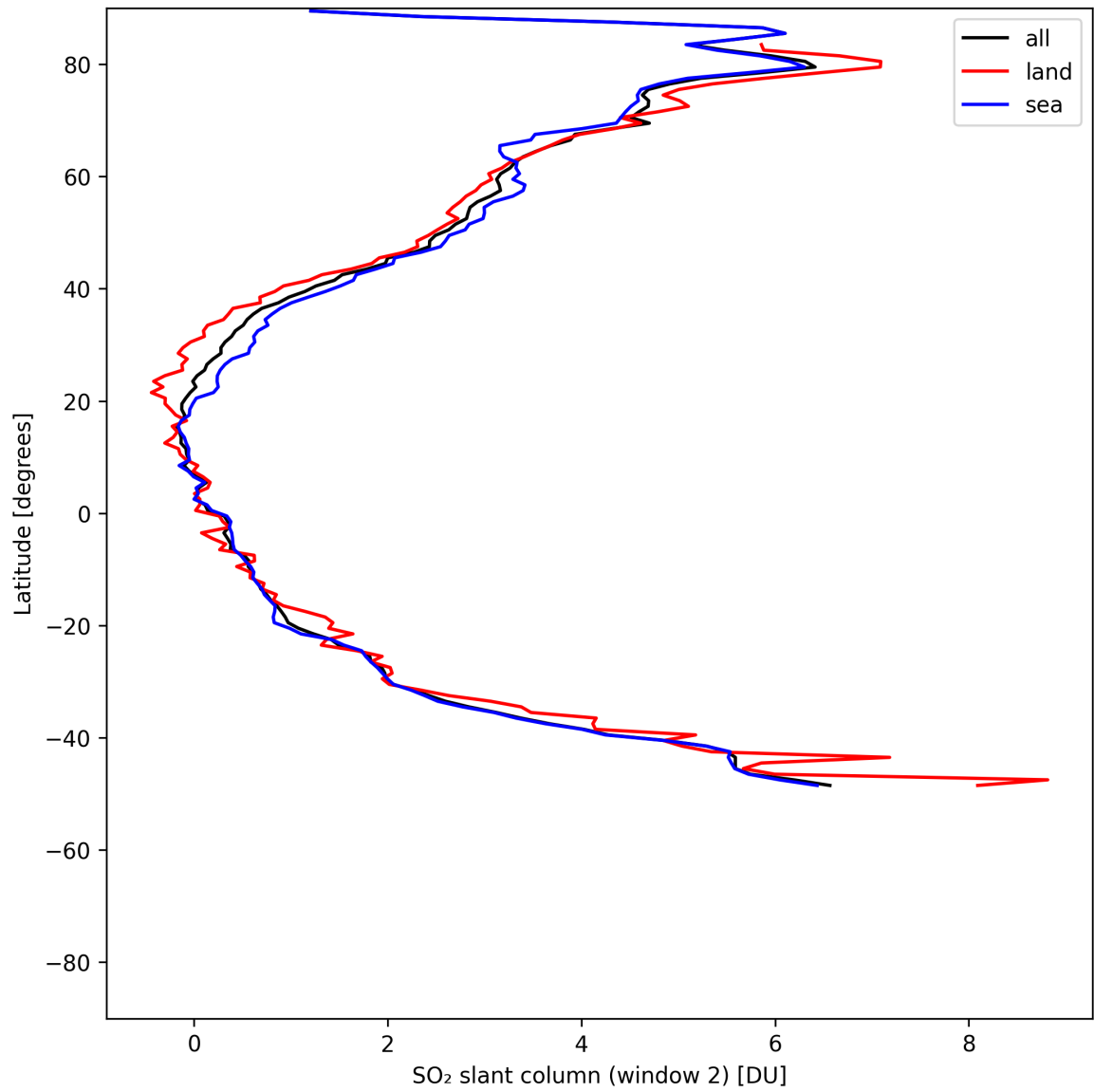
Figure 40: Zonal average of “SO 2 slant column (window 2)” for 2025-05-19 to 2025-05-19.
