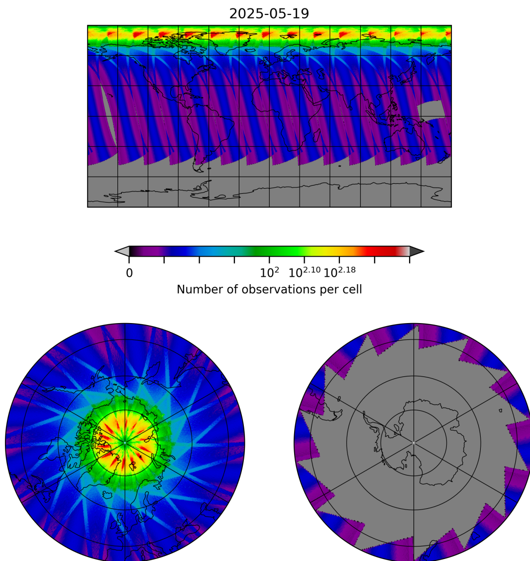
Figure 29: Map of the number of observations for 2025-05-19 to 2025-05-19
