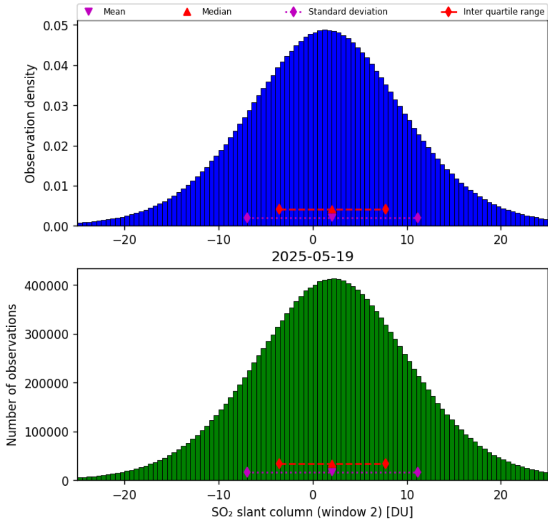
Figure 67: Histogram of “SO 2 slant column (window 2)” for 2025-05-19 to 2025-05-19
