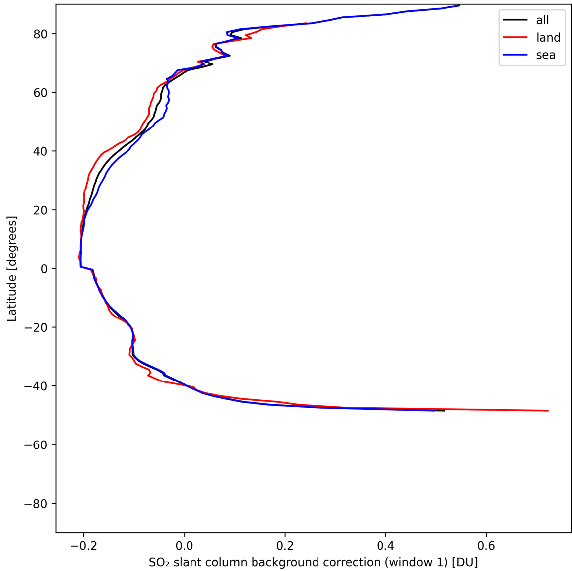
Figure 39: Zonal average of “SO 2 slant column background correction (window 1)” for 2025-05-19 to 2025-05-19.
