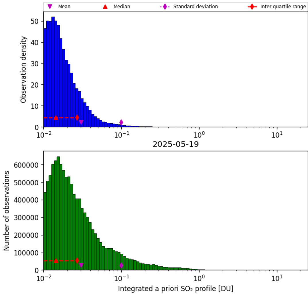
Figure 76: Histogram of “Integrated a priori SO 2 profile” for 2025-05-19 to 2025-05-19
