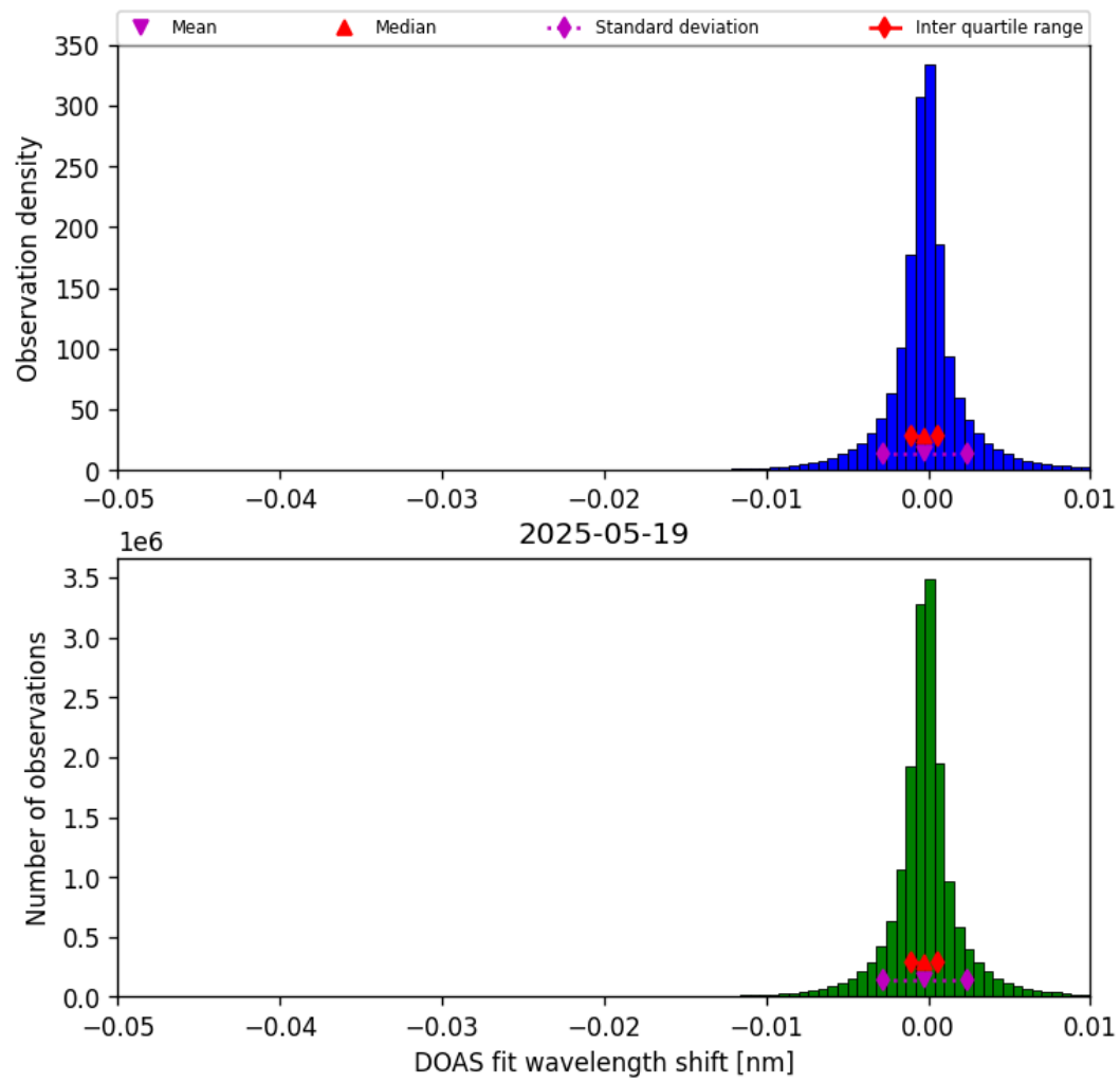
Figure 77: Histogram of “DOAS fit wavelength shift” for 2025-05-19 to 2025-05-19
