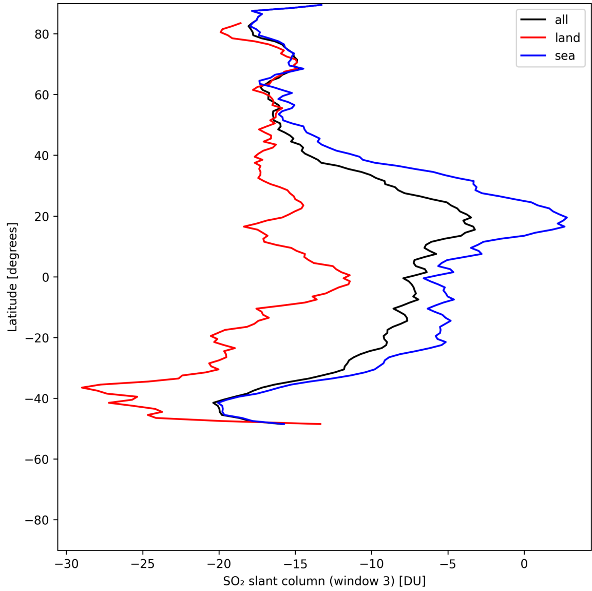
Figure 44: Zonal average of “SO 2 slant column (window 3)” for 2025-05-19 to 2025-05-19.
