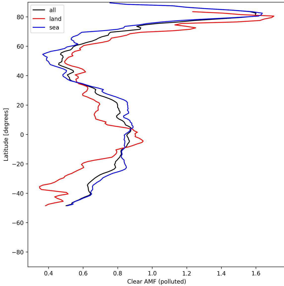
Figure 55: Zonal average of “Clear AMF (polluted)” for 2025-05-19 to 2025-05-19.
