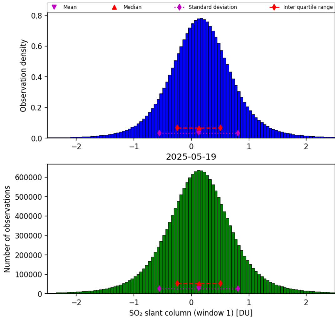
Figure 63: Histogram of “SO 2 slant column (window 1)” for 2025-05-19 to 2025-05-19
