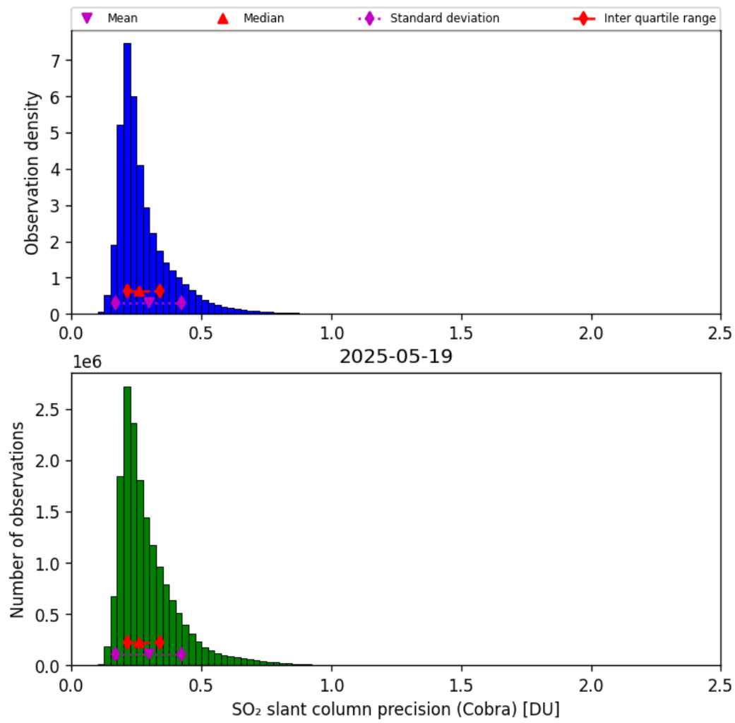
Figure 62: Histogram of “SO 2 slant column precision (Cobra)” for 2025-05-19 to 2025-05-19
