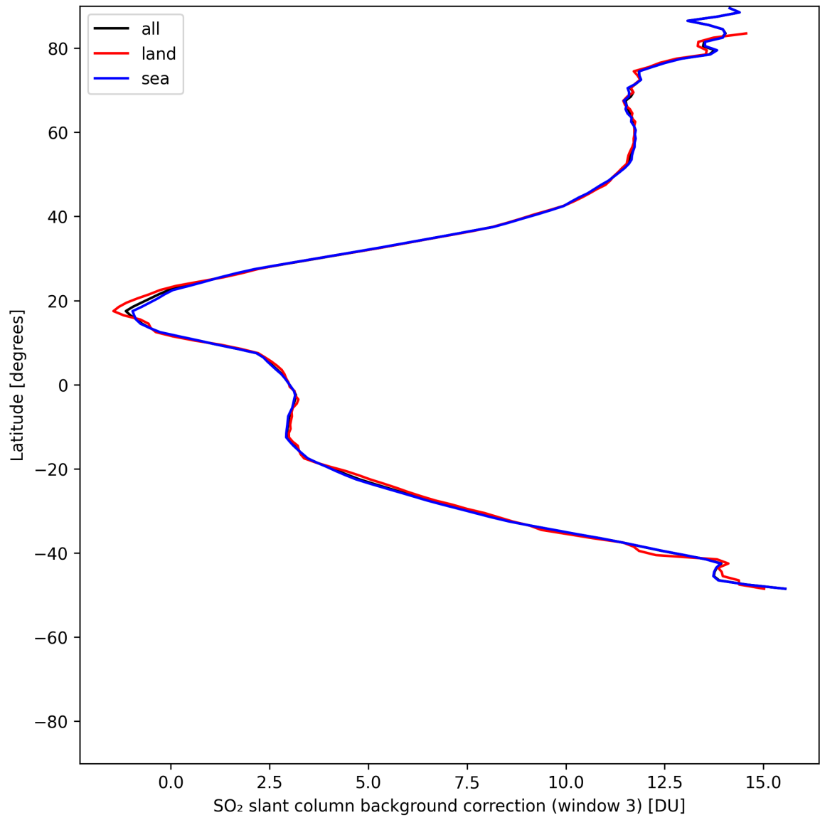
Figure 47: Zonal average of “SO 2 slant column background correction (window 3)” for 2025-05-19 to 2025-05-19.
