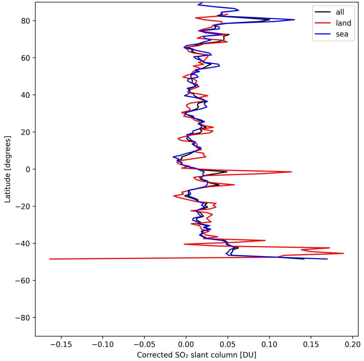
Figure 33: Zonal average of "Corrected SO 2 slant column" for 2025-05-19 to 2025-05-19.
