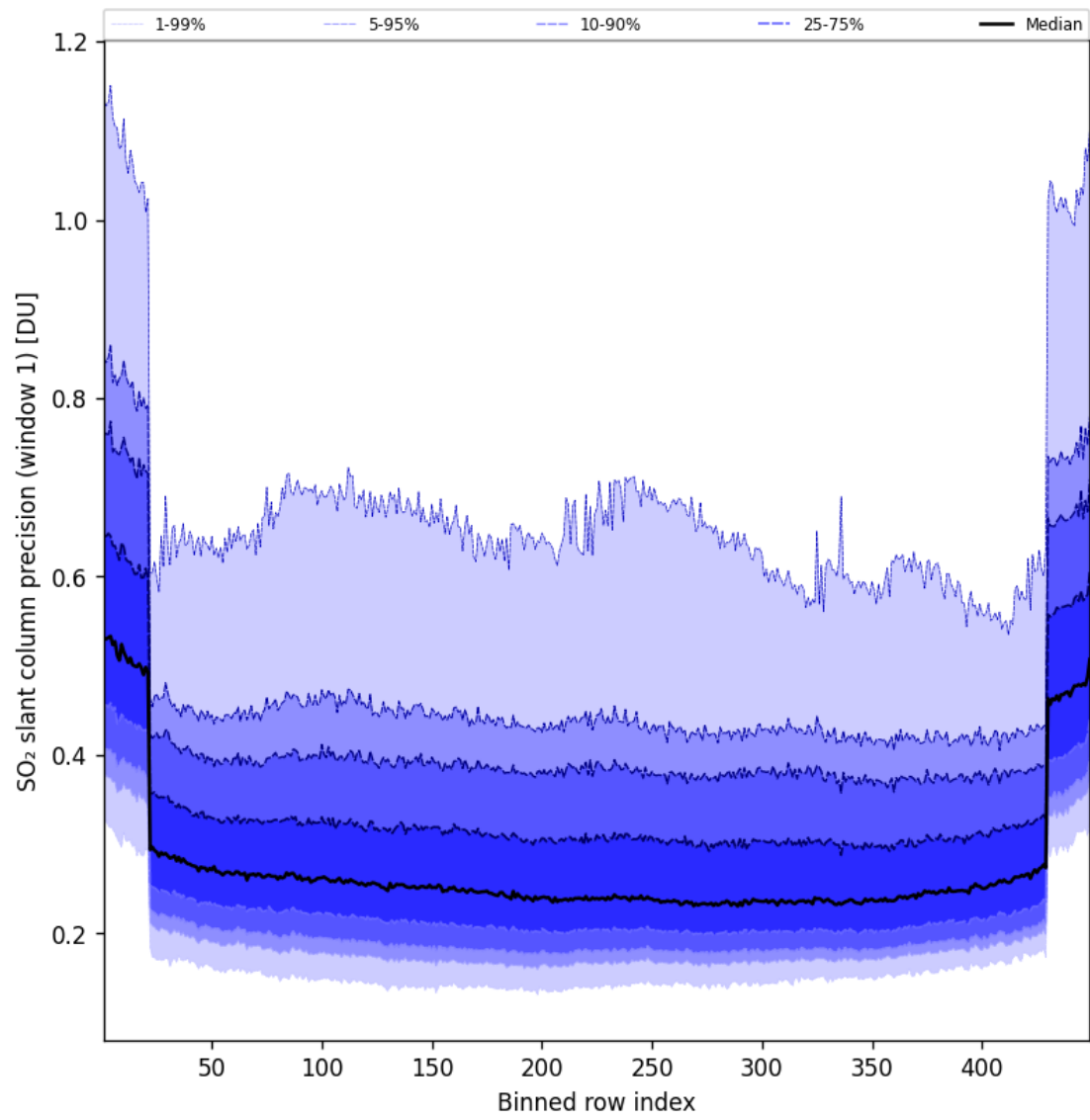
Figure 91: Along track statistics of “SO 2 slant column precision (window 1)” for 2025-05-19 to 2025-05-19
