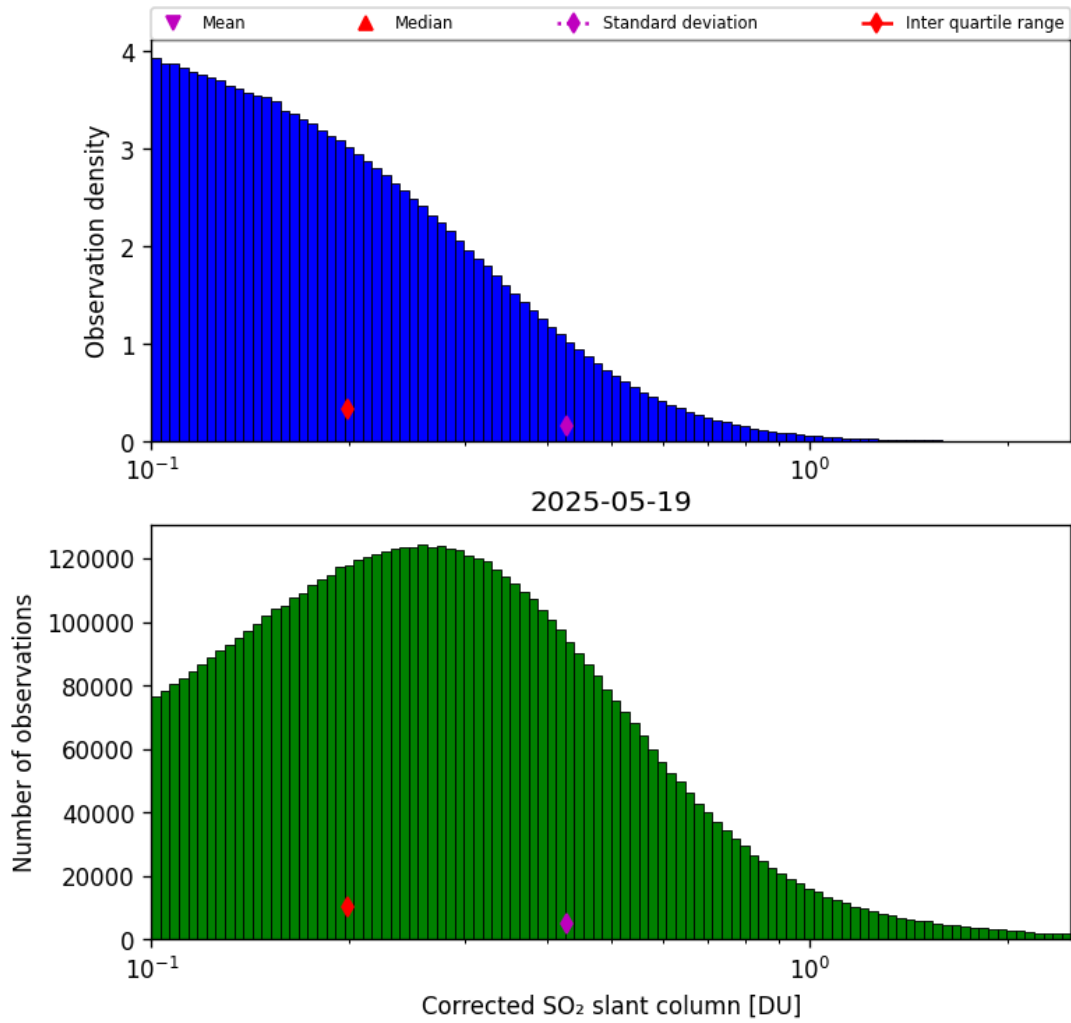
Figure 60: Histogram of “Corrected SO 2 slant column” for 2025-05-19 to 2025-05-19
