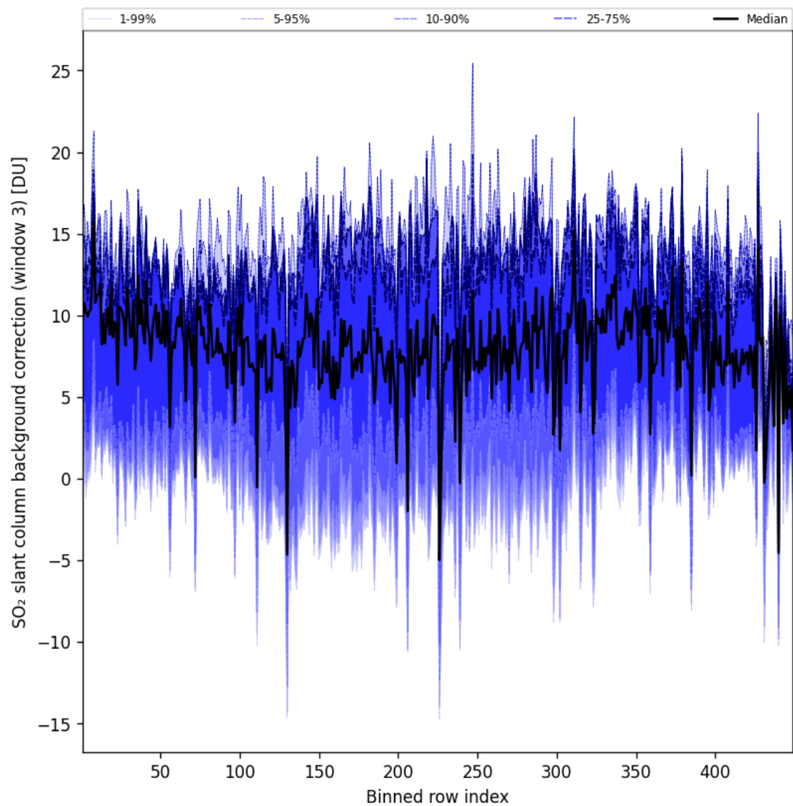
Figure 101: Along track statistics of “SO 2 slant column background correction (window 3)” for 2025-05-19 to 2025-05-19
