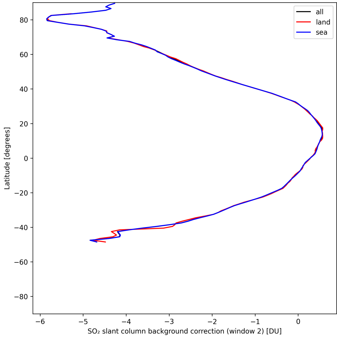
Figure 43: Zonal average of “SO 2 slant column background correction (window 2)” for 2025-05-19 to 2025-05-19.
