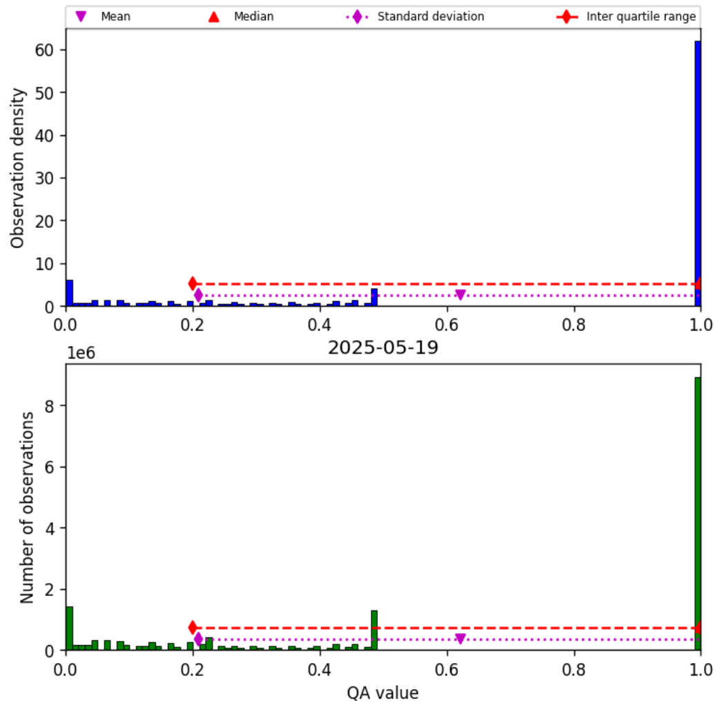
Figure 57: Histogram of “QA value” for 2025-05-19 to 2025-05-19
