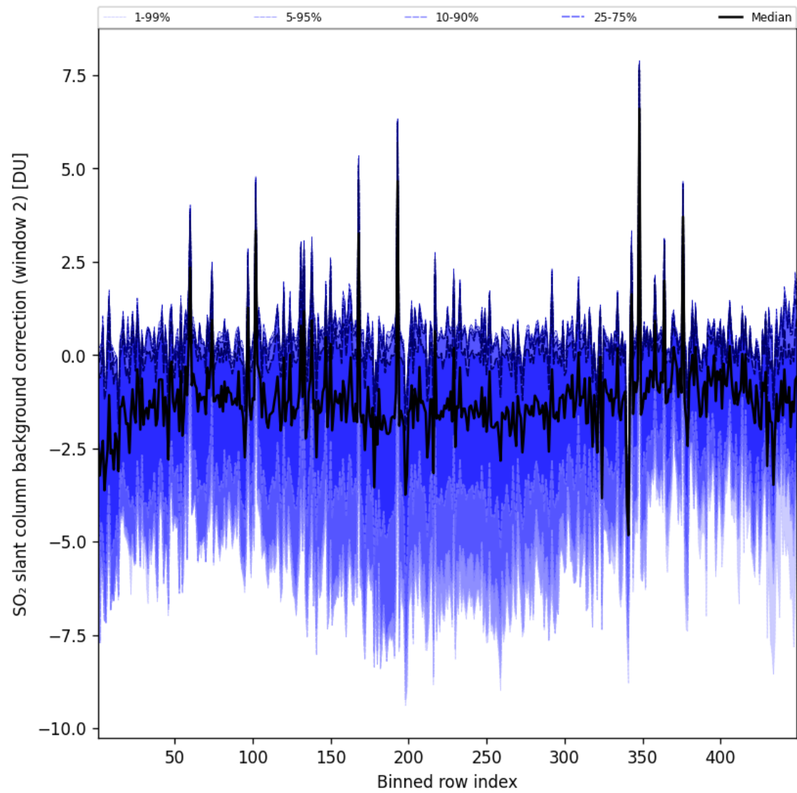
Figure 97: Along track statistics of “SO 2 slant column background correction (window 2)” for 2025-05-19 to 2025-05-19
