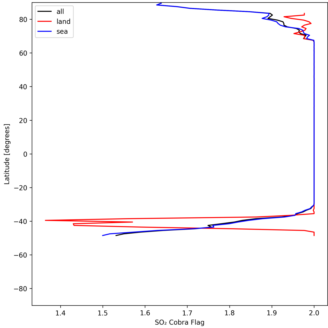
Figure 48: Zonal average of "SO 2 Cobra Flag" for 2025-05-19 to 2025-05-19.
