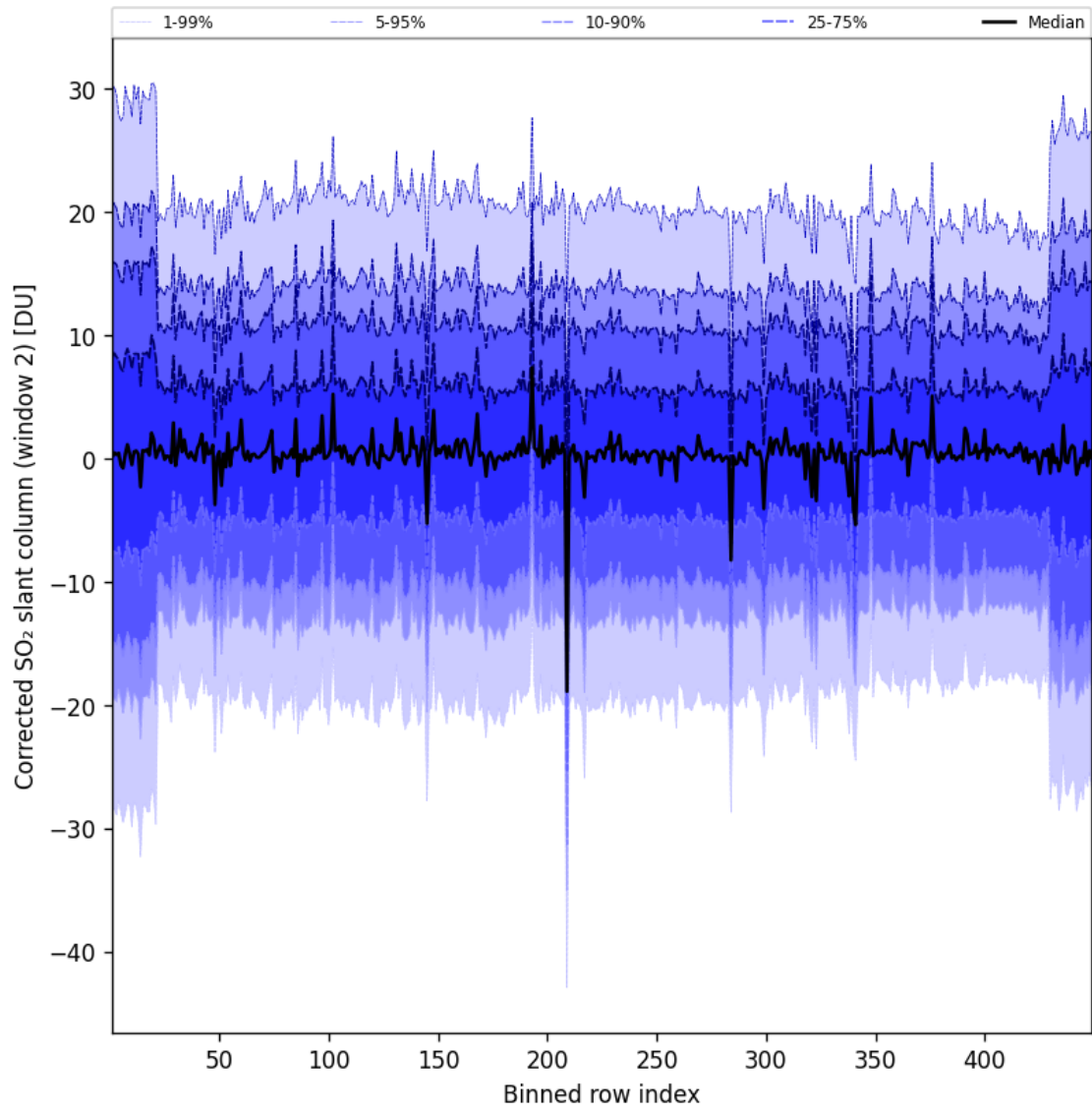
Figure 96: Along track statistics of “Corrected SO 2 slant column (window 2)” for 2025-05-19 to 2025-05-19
