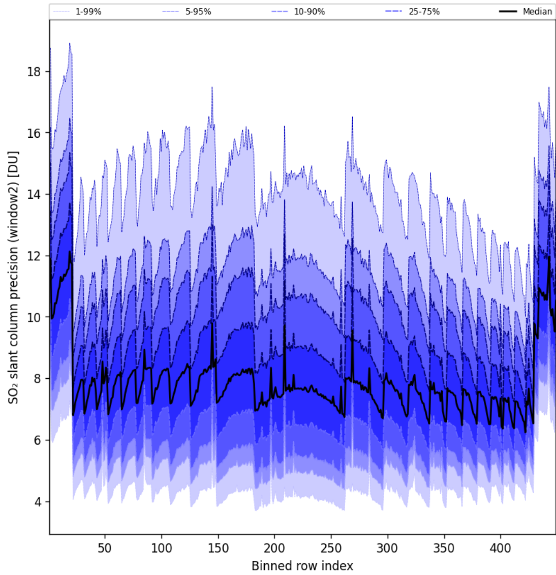
Figure 95: Along track statistics of “SO 2 slant column precision (window2)” for 2025-05-19 to 2025-05-19
