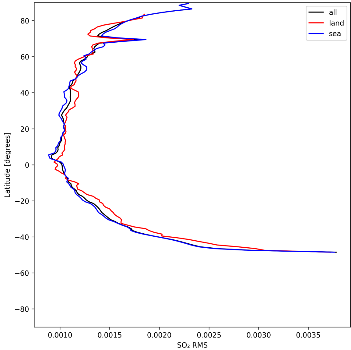
Figure 52: Zonal average of “SO 2 RMS” for 2025-05-19 to 2025-05-19.
