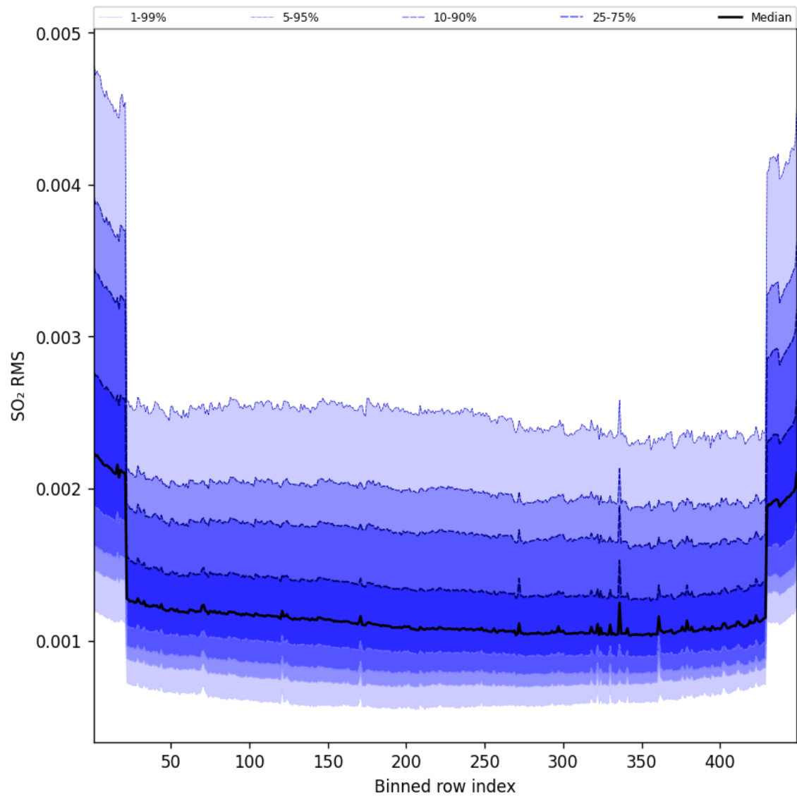
Figure 106: Along track statistics of “SO 2 RMS” for 2025-05-19 to 2025-05-19
