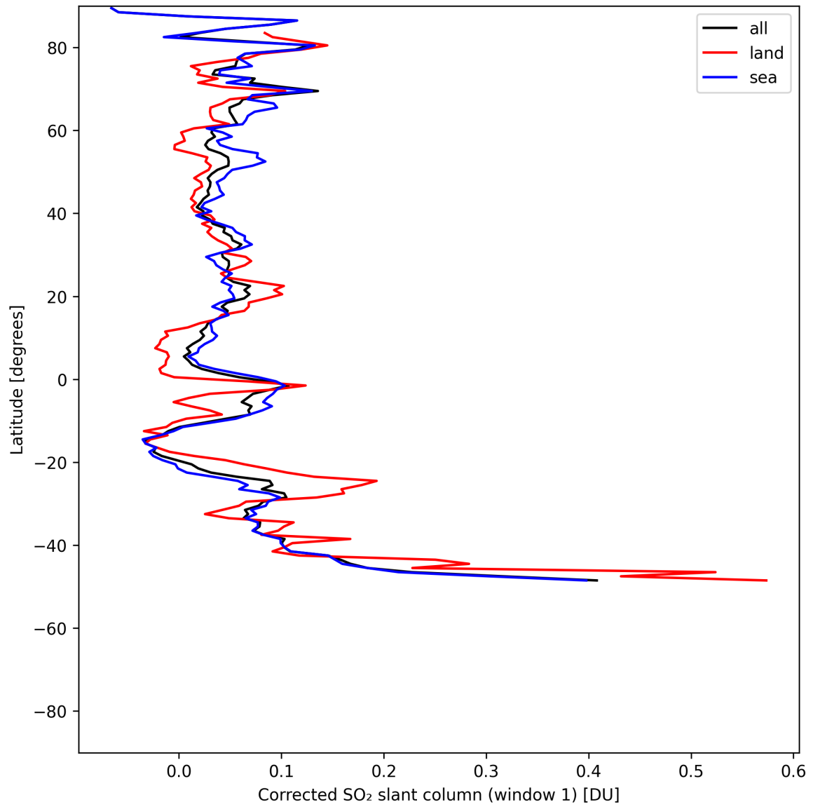
Figure 38: Zonal average of “Corrected SO 2 slant column (window 1)” for 2025-05-19 to 2025-05-19.
