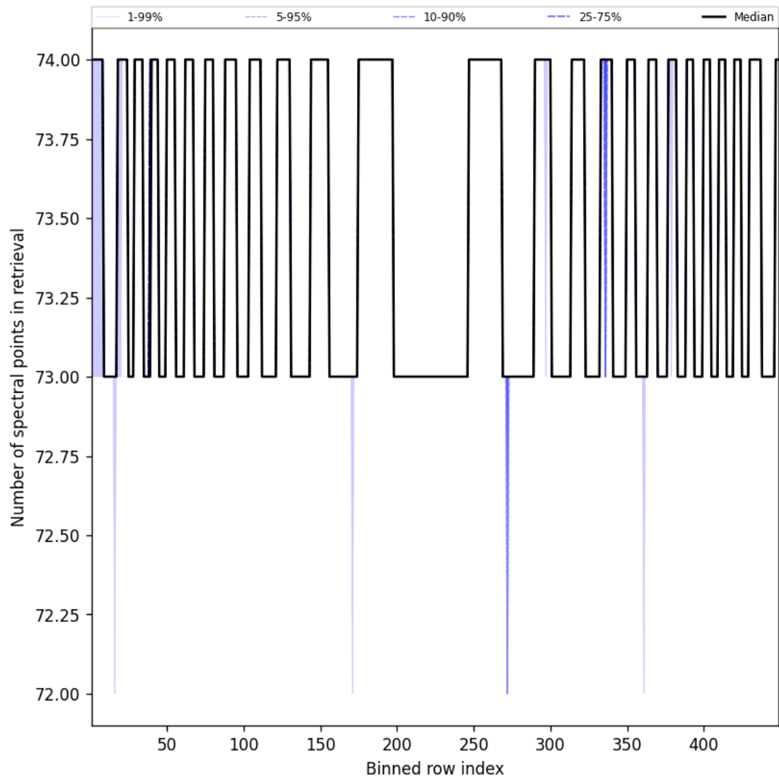
Figure 110: Along track statistics of “Number of spectral points in retrieval” for 2025-05-19 to 2025-05-19
