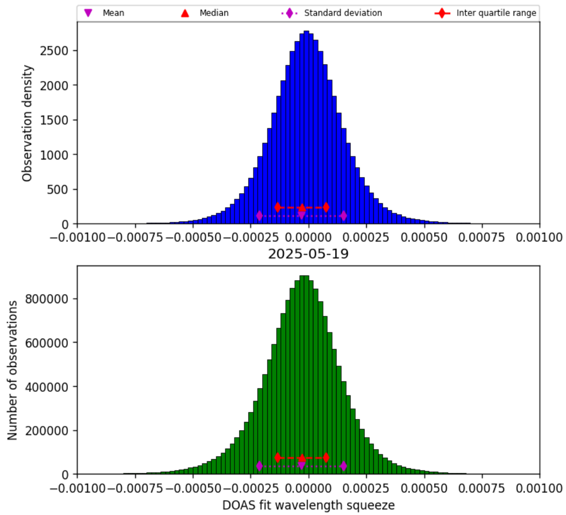
Figure 78: Histogram of “DOAS fit wavelength squeeze” for 2025-05-19 to 2025-05-19
