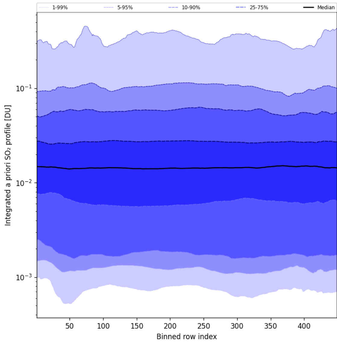
Figure 103: Along track statistics of “Integrated a priori SO 2 profile” for 2025-05-19 to 2025-05-19
