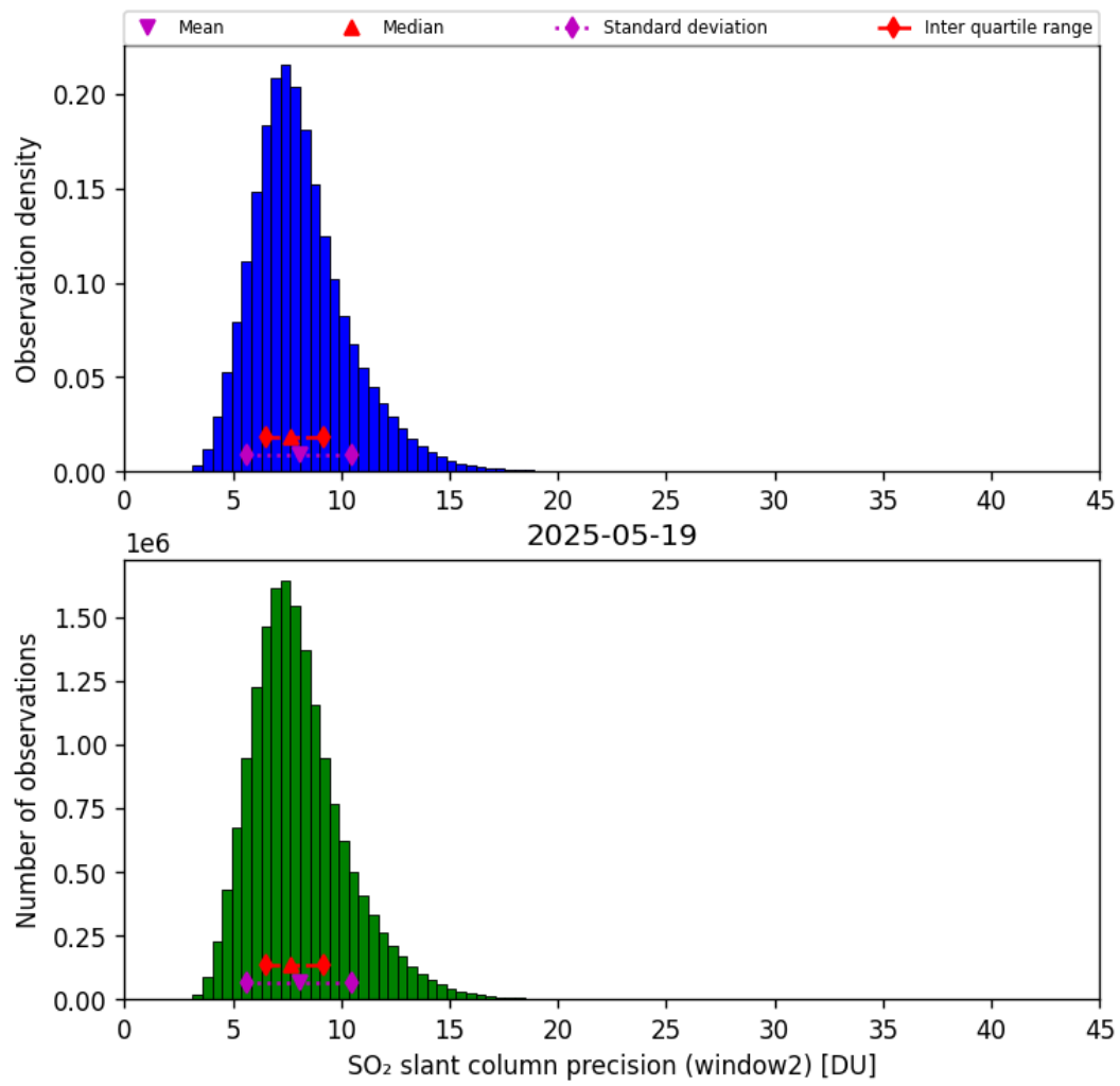
Figure 68: Histogram of “SO 2 slant column precision (window2)” for 2025-05-19 to 2025-05-19
