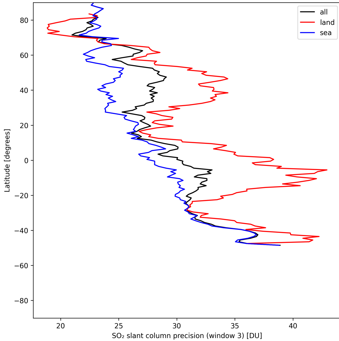
Figure 45: Zonal average of “SO 2 slant column precision (window 3)” for 2025-05-19 to 2025-05-19.
