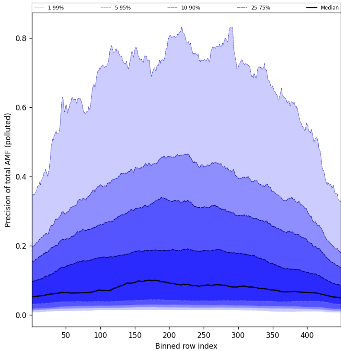
Figure 108: Along track statistics of “Precision of total AMF (polluted)” for 2025-05-19 to 2025-05-19
