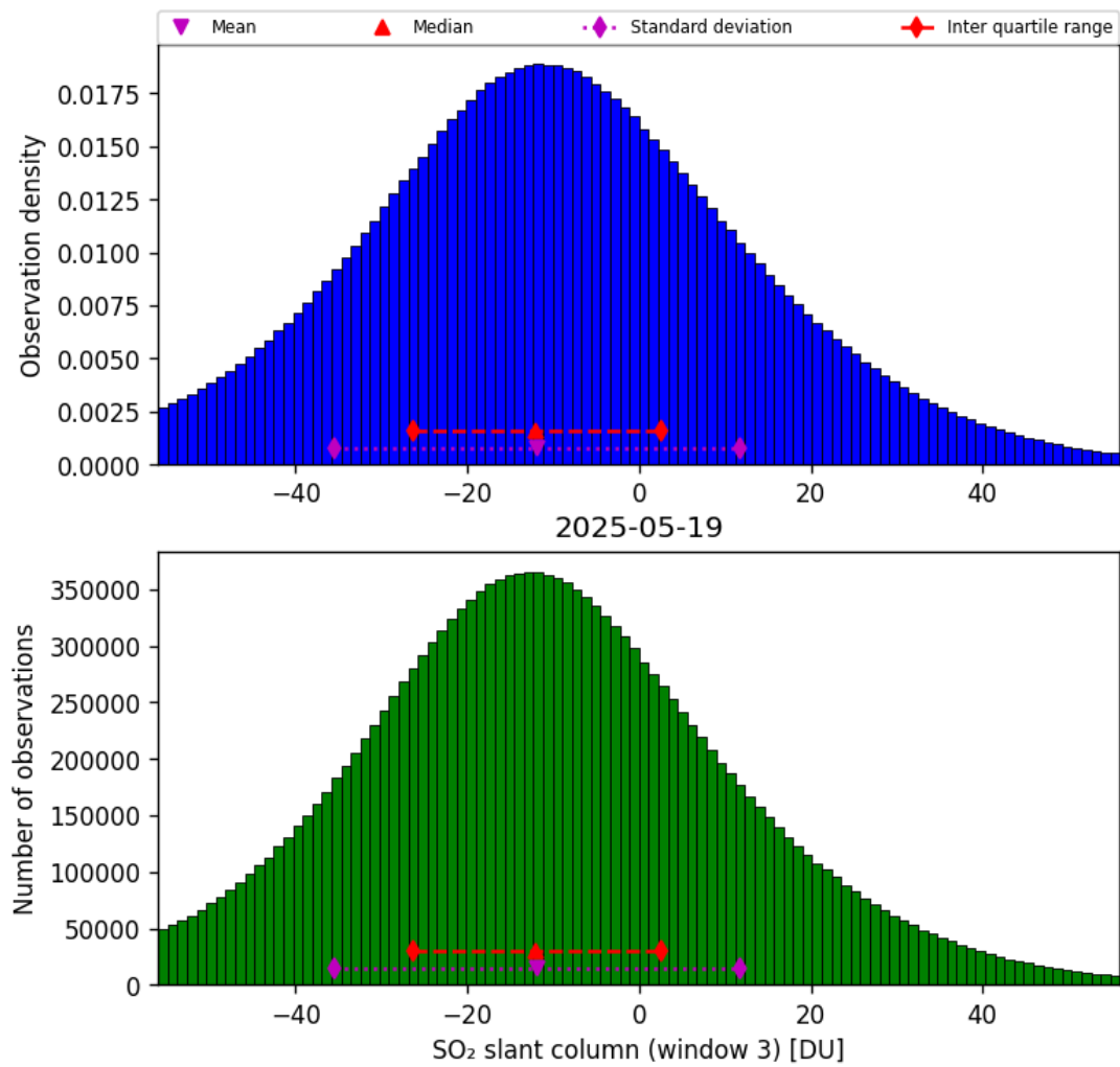
Figure 71: Histogram of “SO 2 slant column (window 3)” for 2025-05-19 to 2025-05-19
