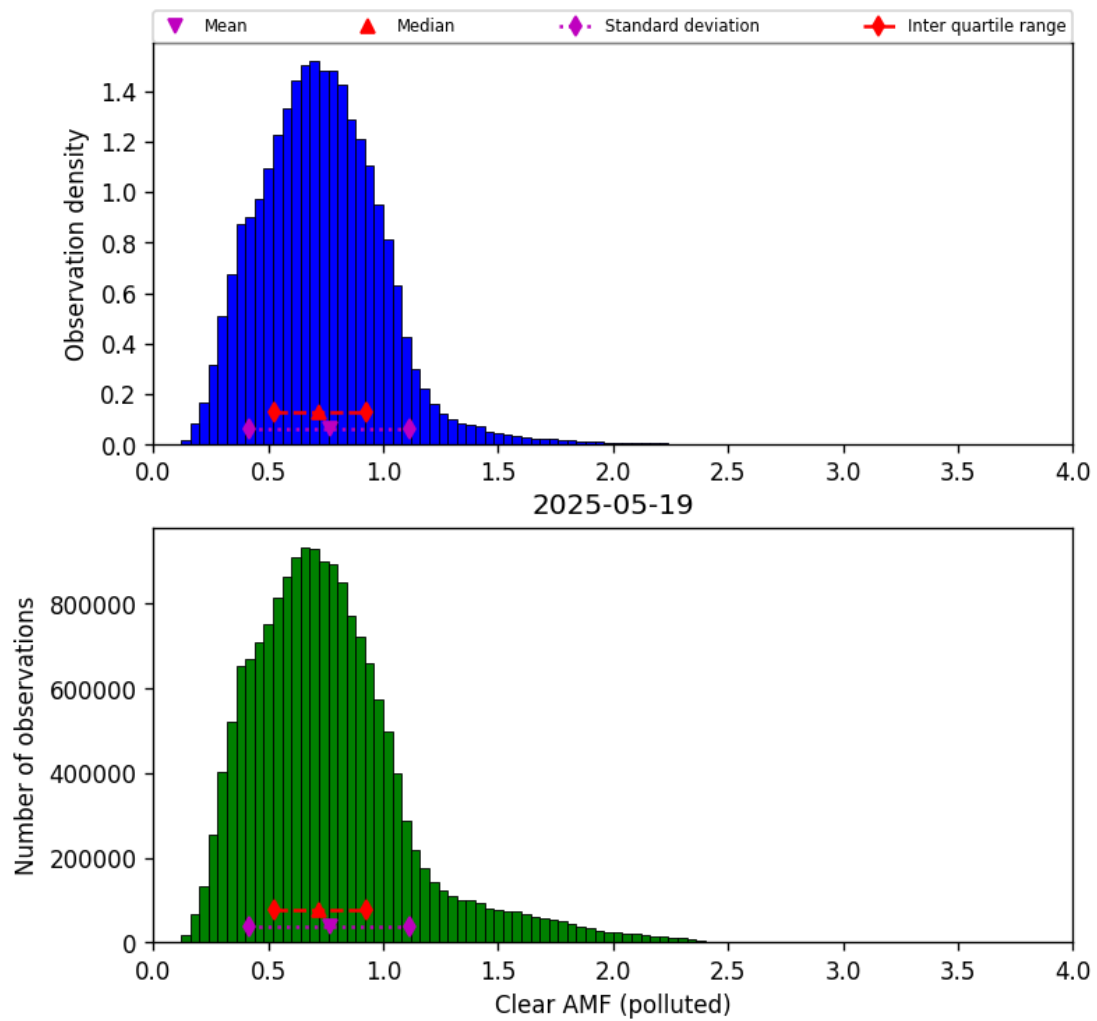
Figure 82: Histogram of “Clear AMF (polluted)” for 2025-05-19 to 2025-05-19
