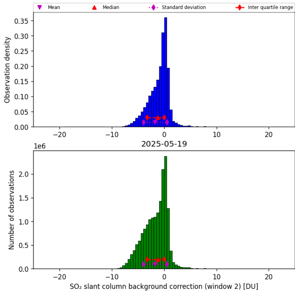
Figure 70: Histogram of “SO 2 slant column background correction (window 2)” for 2025-05-19 to 2025-05-19
