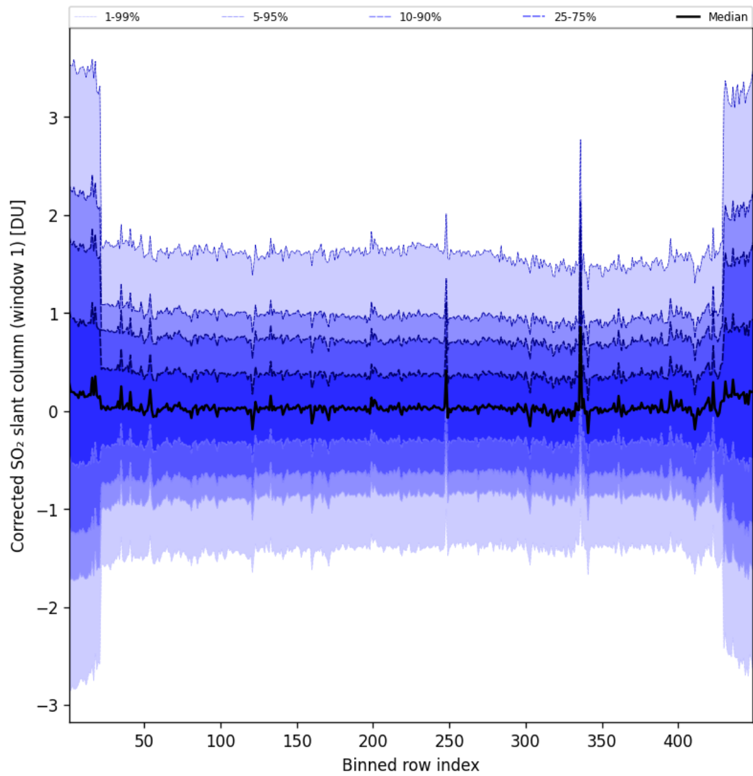
Figure 92: Along track statistics of “Corrected SO 2 slant column (window 1)” for 2025-05-19 to 2025-05-19
