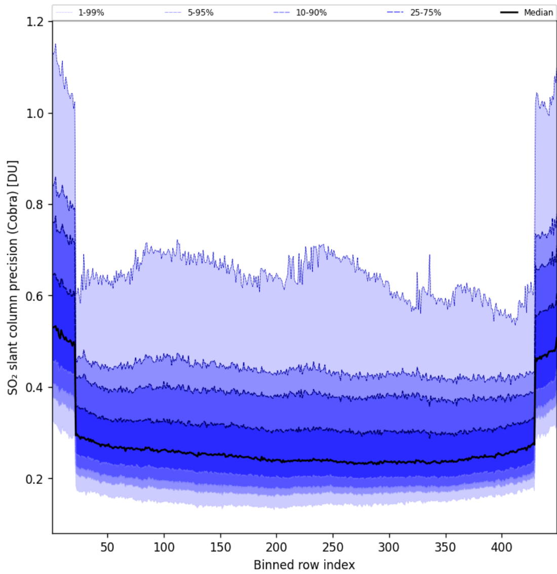
Figure 89: Along track statistics of “SO 2 slant column precision (Cobra)” for 2025-05-19 to 2025-05-19
