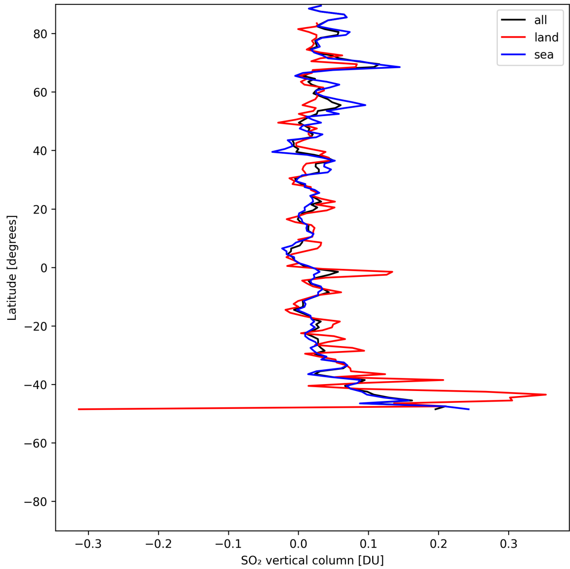
Figure 31: Zonal average of “SO 2 vertical column” for 2025-05-19 to 2025-05-19.
