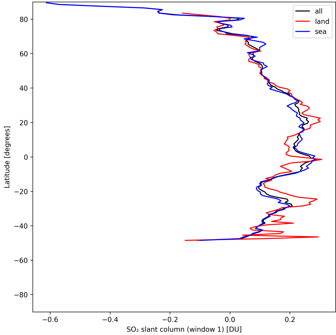
Figure 36: Zonal average of “SO 2 slant column (window 1)” for 2025-05-19 to 2025-05-19.
