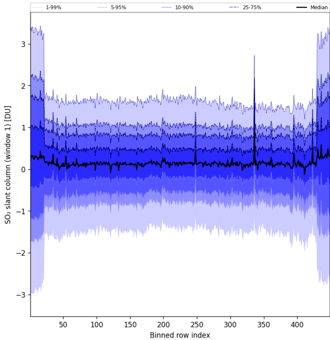
Figure 90: Along track statistics of “SO 2 slant column (window 1)” for 2025-05-19 to 2025-05-19
