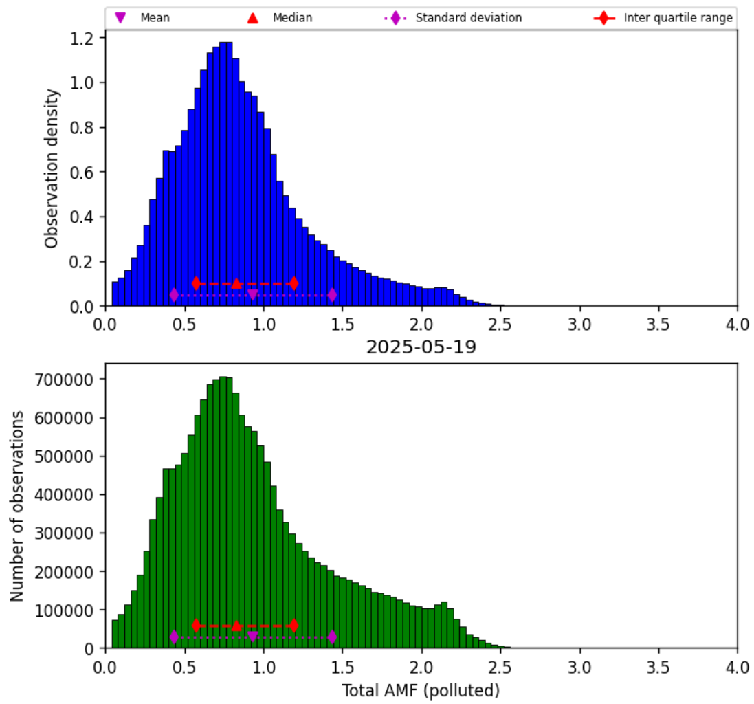
Figure 80: Histogram of “Total AMF (polluted)” for 2025-05-19 to 2025-05-19
