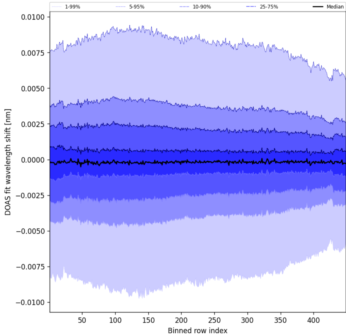
Figure 104: Along track statistics of “DOAS fit wavelength shift” for 2025-05-19 to 2025-05-19
