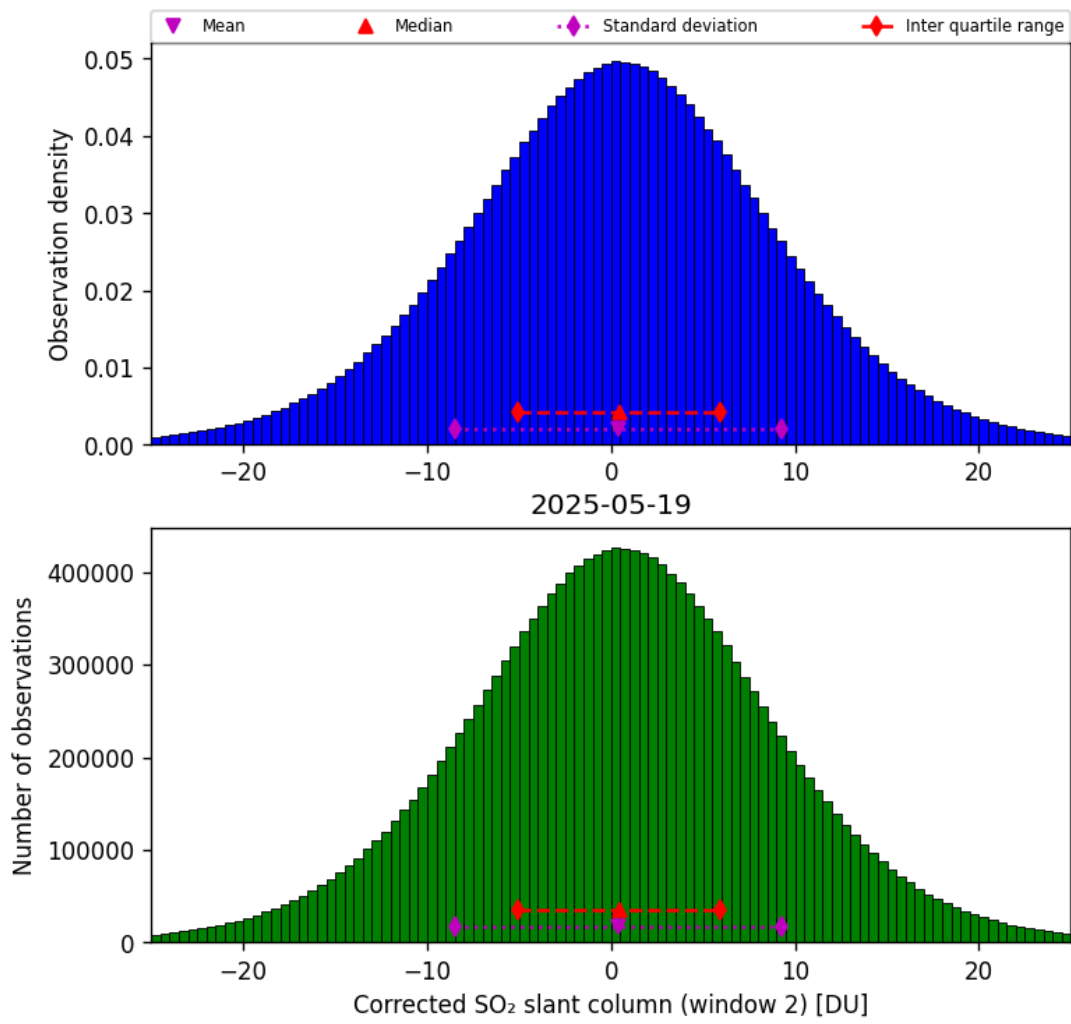
Figure 69: Histogram of “Corrected SO 2 slant column (window 2)” for 2025-05-19 to 2025-05-19
