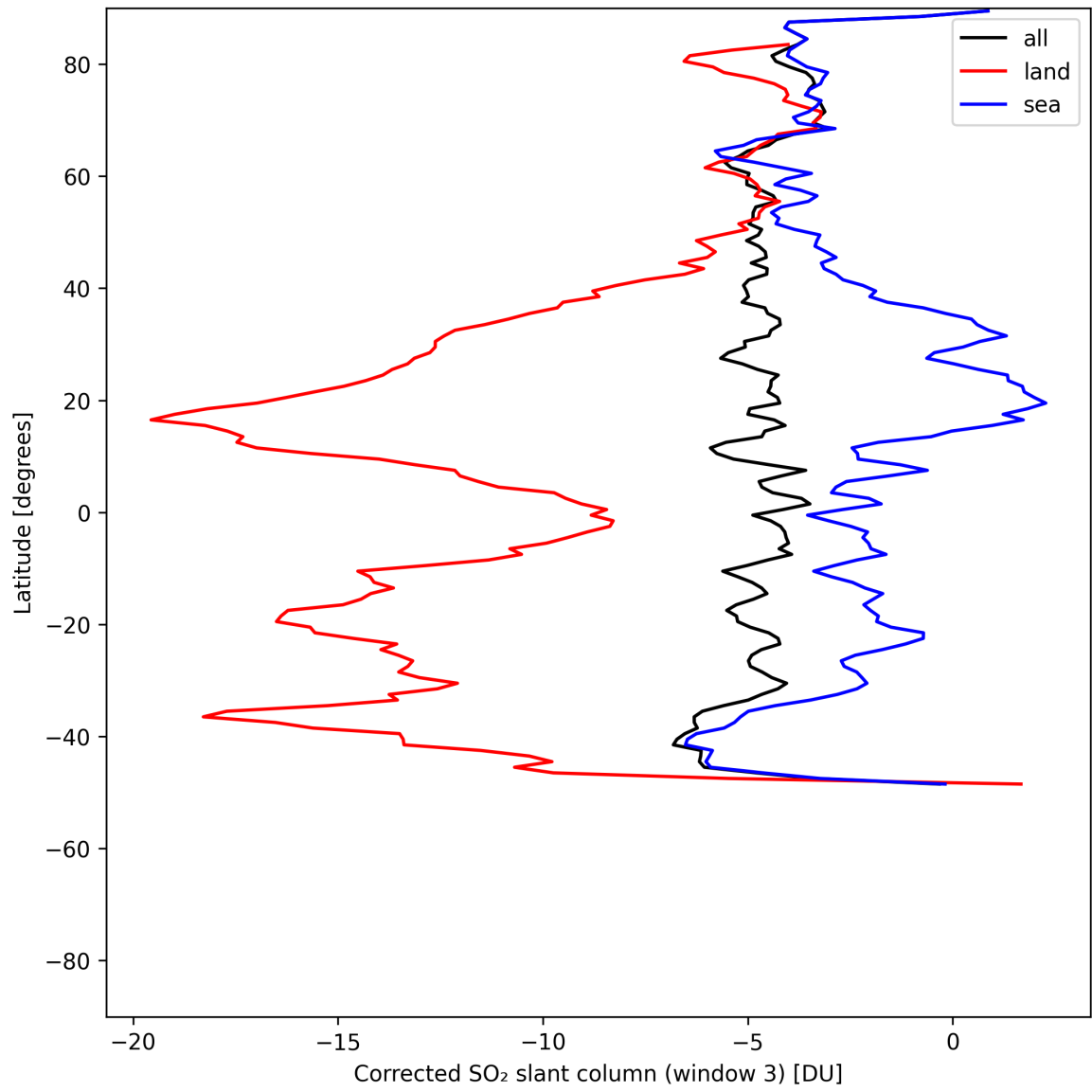
Figure 46: Zonal average of “Corrected SO 2 slant column (window 3)” for 2025-05-19 to 2025-05-19.
