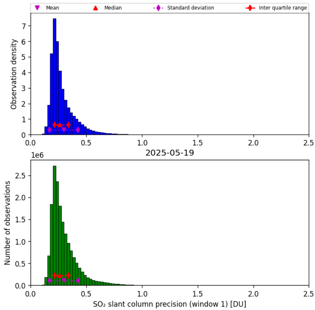
Figure 64: Histogram of “SO 2 slant column precision (window 1)” for 2025-05-19 to 2025-05-19
