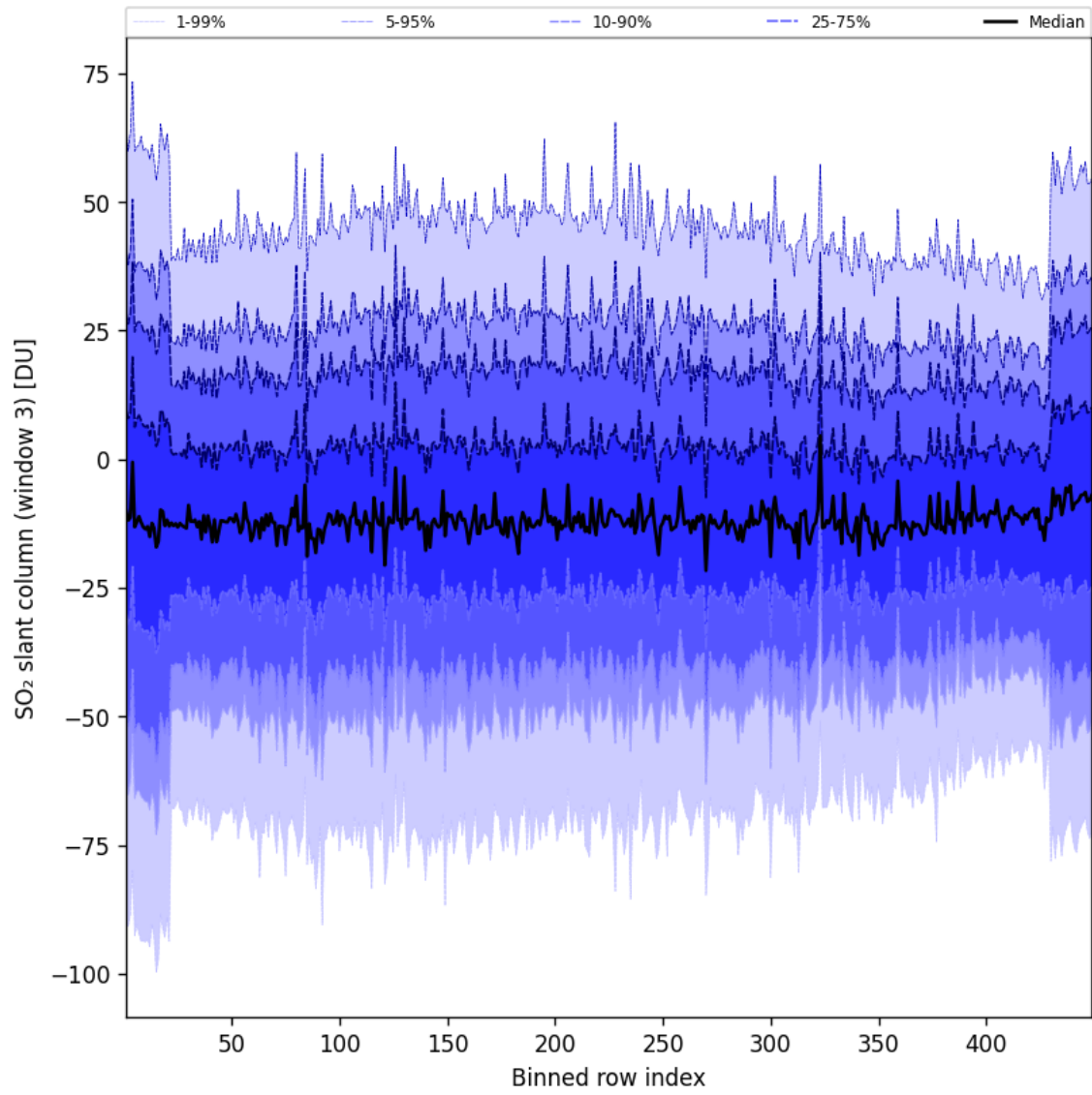
Figure 98: Along track statistics of “SO 2 slant column (window 3)” for 2025-05-19 to 2025-05-19
