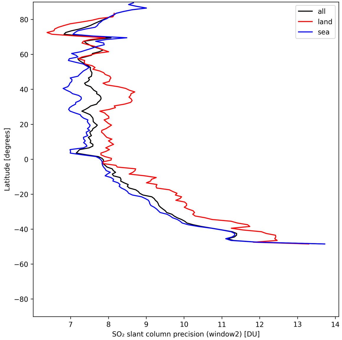
Figure 41: Zonal average of “SO 2 slant column precision (window2)” for 2025-05-19 to 2025-05-19.
