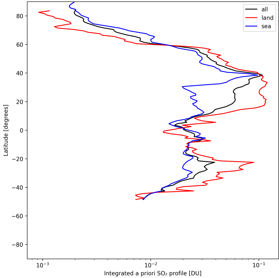
Figure 49: Zonal average of “Integrated a priori SO 2 profile” for 2025-05-19 to 2025-05-19.
