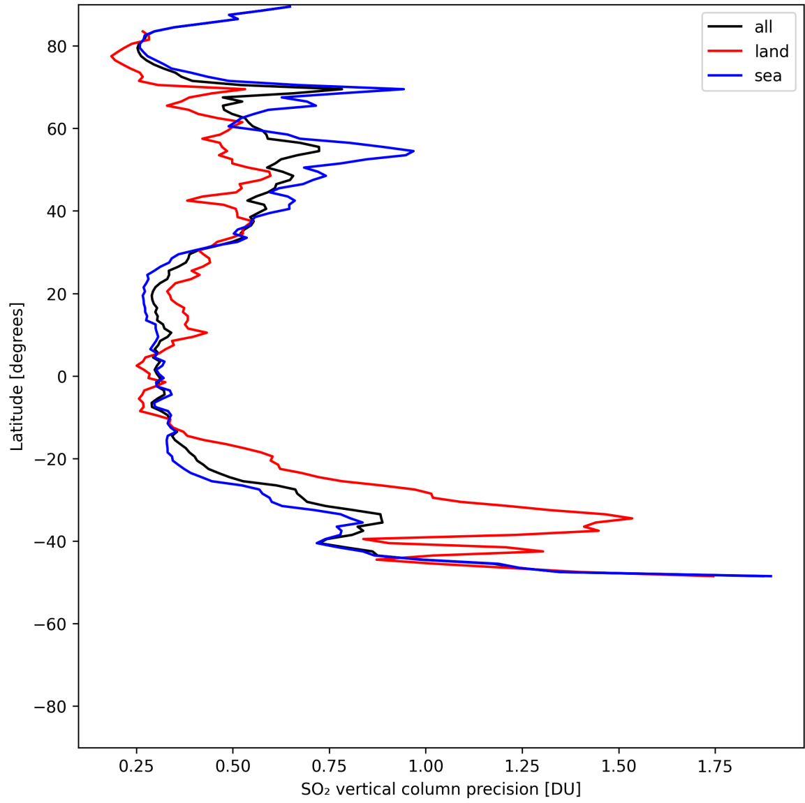
Figure 32: Zonal average of “SO 2 vertical column precision” for 2025-05-19 to 2025-05-19.
