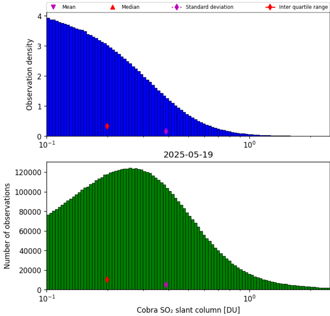
Figure 61: Histogram of “Cobra SO 2 slant column” for 2025-05-19 to 2025-05-19
