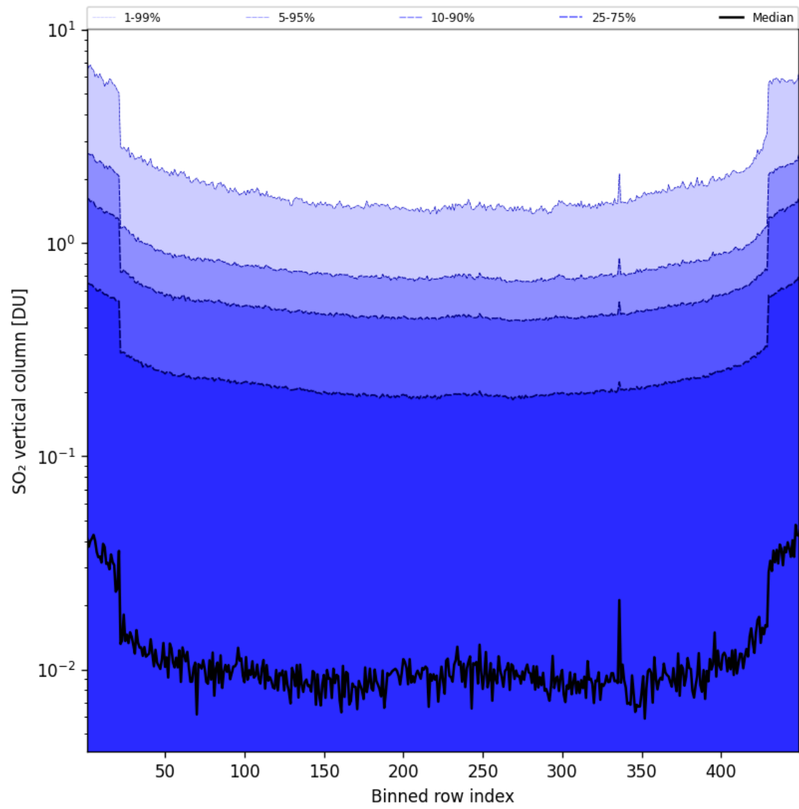
Figure 85: Along track statistics of “SO 2 vertical column” for 2025-05-19 to 2025-05-19
