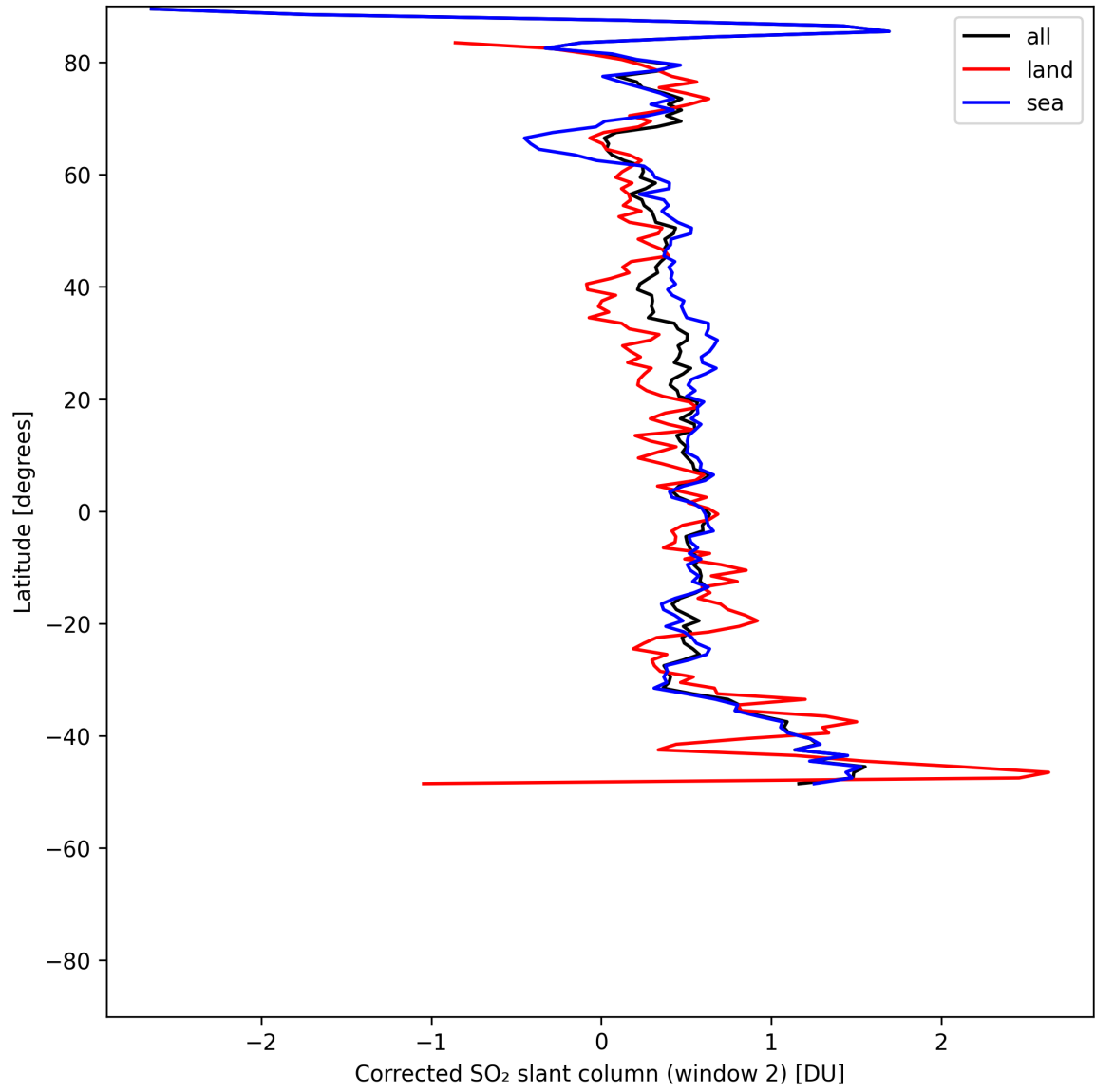
Figure 42: Zonal average of “Corrected SO 2 slant column (window 2)” for 2025-05-20 to 2025-05-21.
