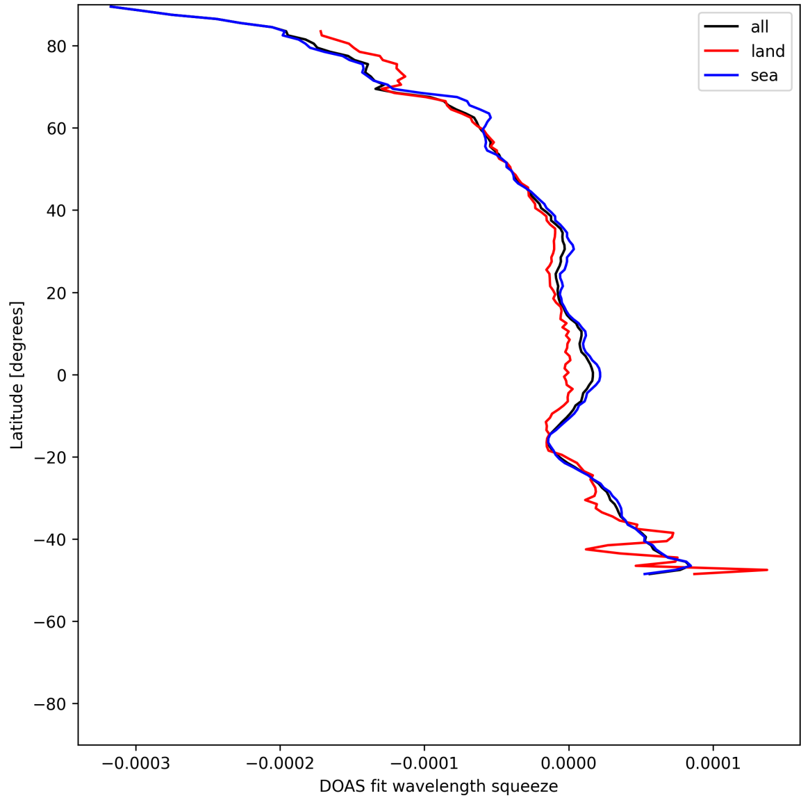
Figure 51: Zonal average of “DOAS fit wavelength squeeze” for 2025-05-20 to 2025-05-21.
