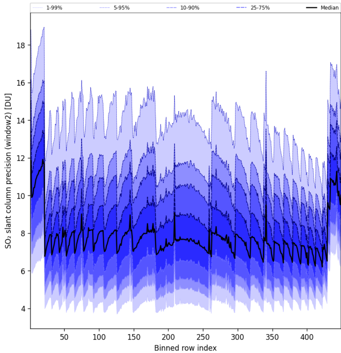
Figure 95: Along track statistics of “SO 2 slant column precision (window2)” for 2025-05-20 to 2025-05-21
