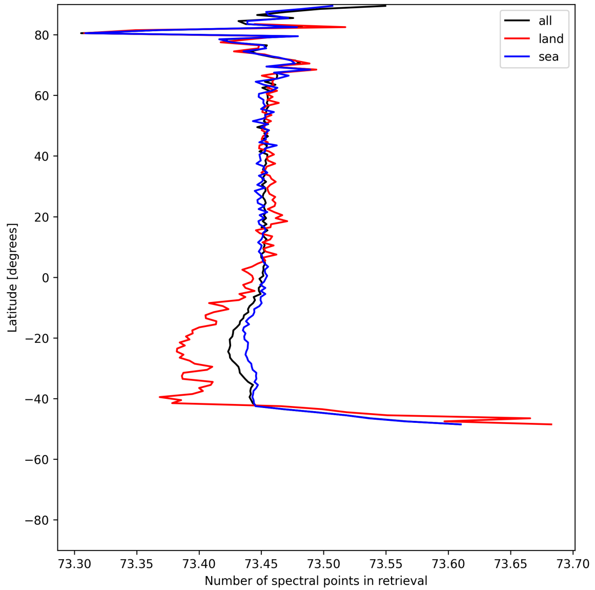
Figure 56: Zonal average of “Number of spectral points in retrieval” for 2025-05-20 to 2025-05-21.
