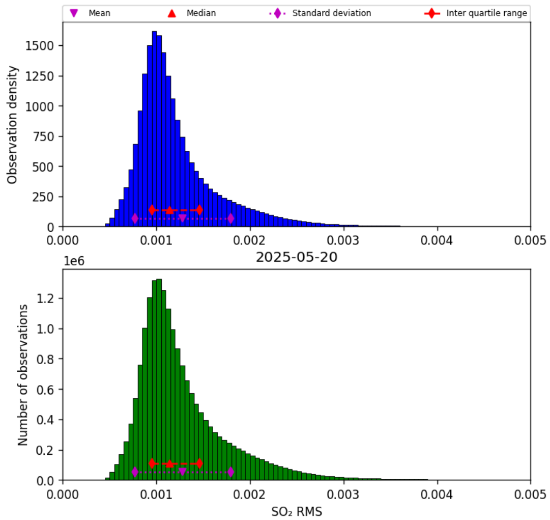
Figure 79: Histogram of “SO 2 RMS” for 2025-05-20 to 2025-05-21
