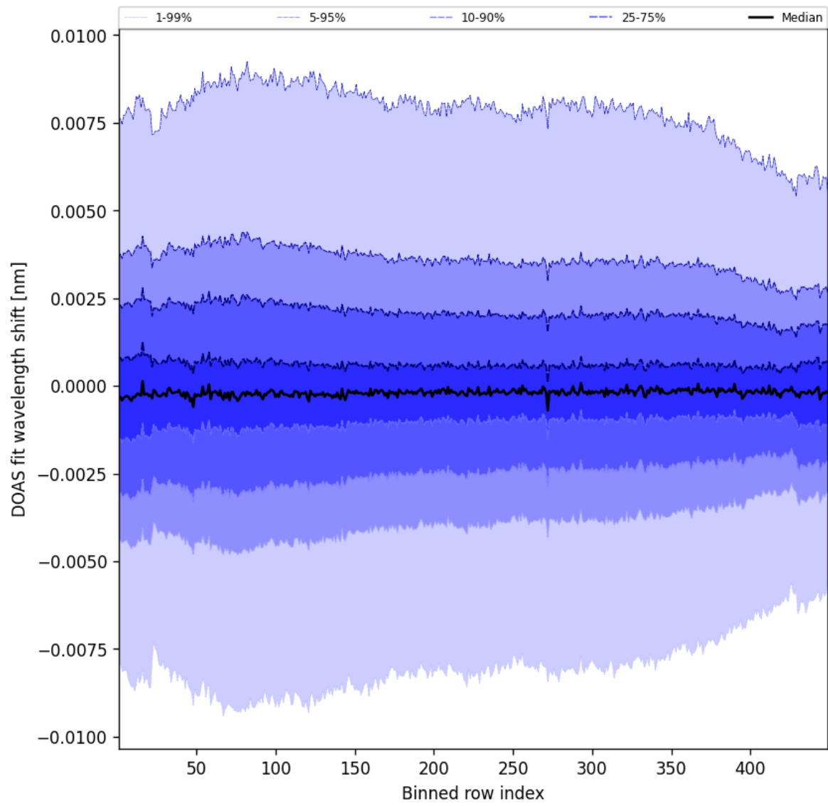
Figure 104: Along track statistics of “DOAS fit wavelength shift” for 2025-05-20 to 2025-05-21
