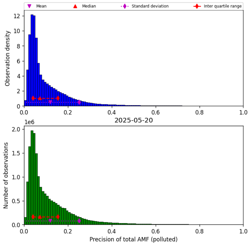
Figure 81: Histogram of “Precision of total AMF (polluted)” for 2025-05-20 to 2025-05-21
