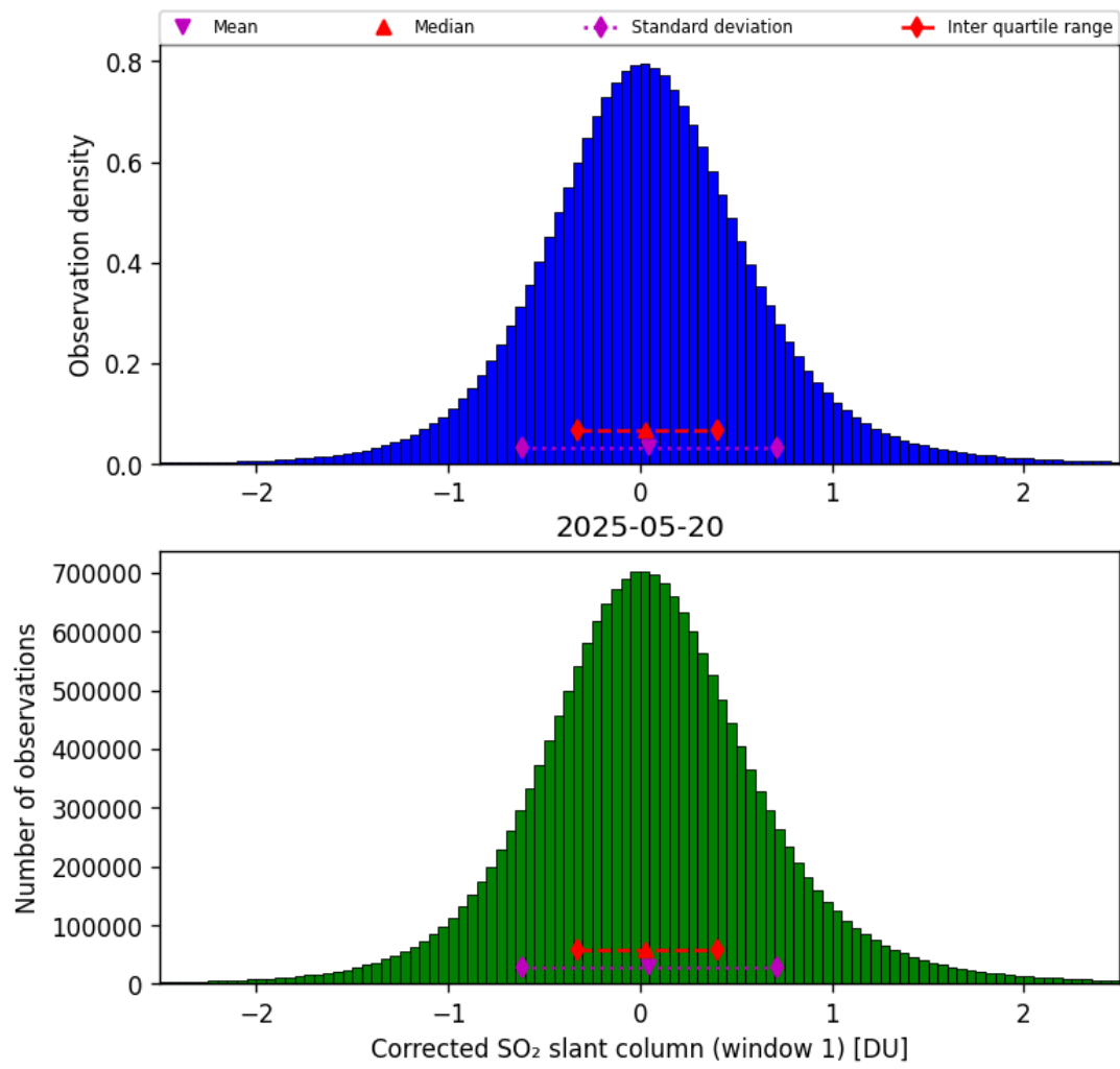
Figure 65: Histogram of “Corrected SO 2 slant column (window 1)” for 2025-05-20 to 2025-05-21
