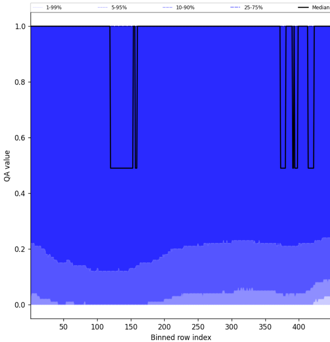
Figure 84: Along track statistics of “QA value” for 2025-05-20 to 2025-05-21
