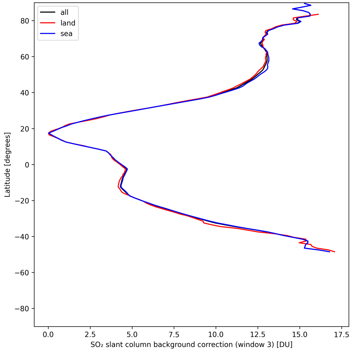
Figure 47: Zonal average of “SO 2 slant column background correction (window 3)” for 2025-05-20 to 2025-05-21.
