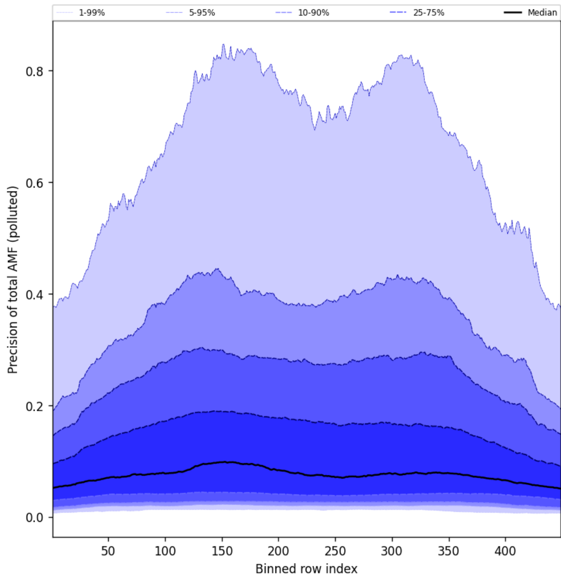
Figure 108: Along track statistics of “Precision of total AMF (polluted)” for 2025-05-20 to 2025-05-21
