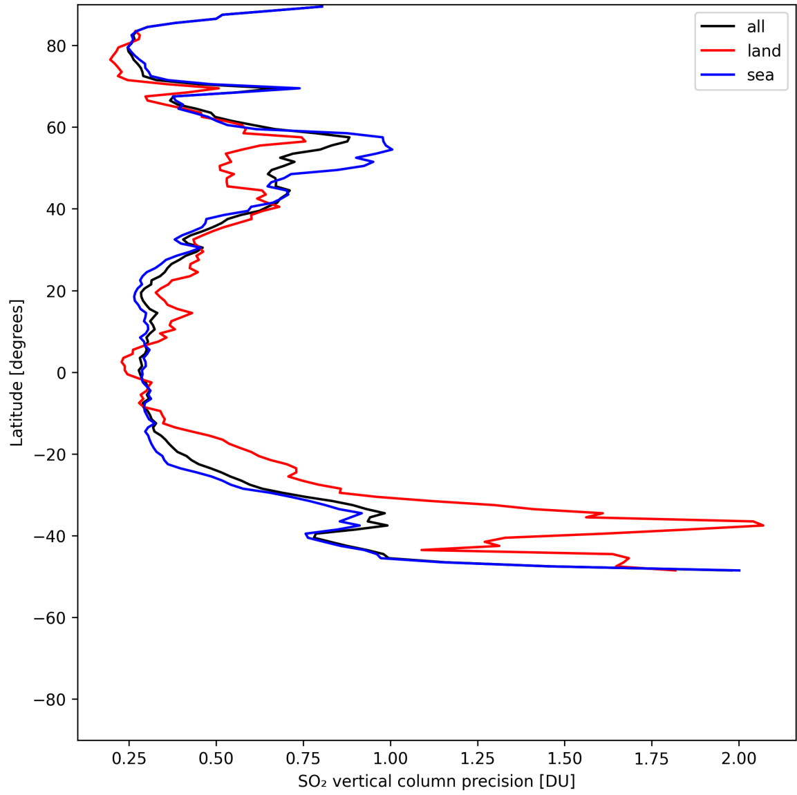
Figure 32: Zonal average of “SO 2 vertical column precision” for 2025-05-20 to 2025-05-21.
