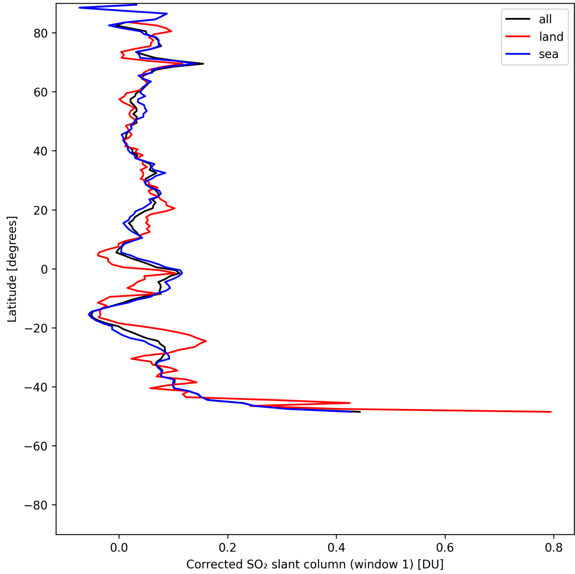
Figure 38: Zonal average of “Corrected SO 2 slant column (window 1)” for 2025-05-20 to 2025-05-21.
