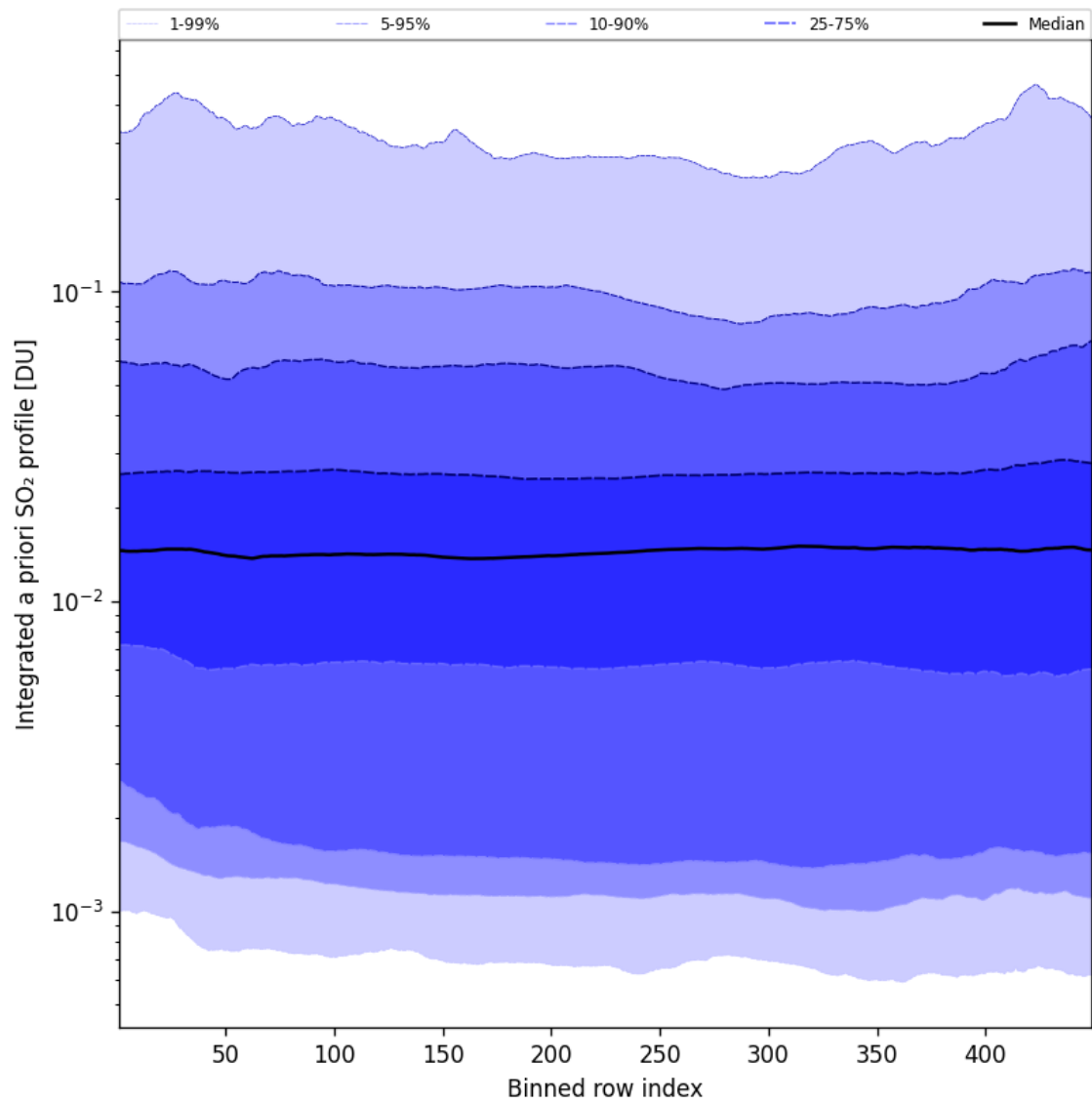
Figure 103: Along track statistics of “Integrated a priori SO 2 profile” for 2025-05-20 to 2025-05-21
