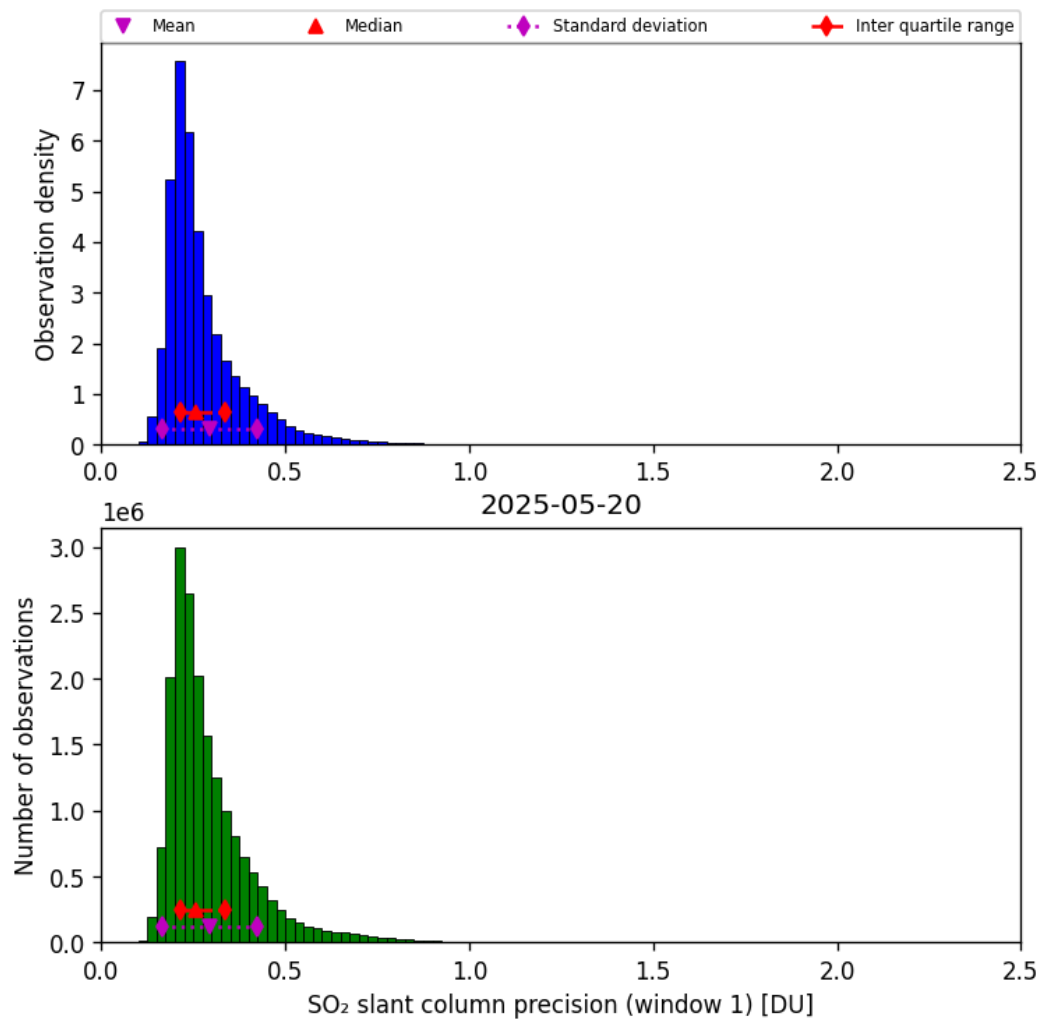
Figure 64: Histogram of “SO 2 slant column precision (window 1)” for 2025-05-20 to 2025-05-21
