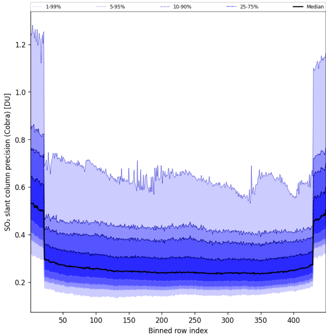
Figure 89: Along track statistics of “SO 2 slant column precision (Cobra)” for 2025-05-20 to 2025-05-21
