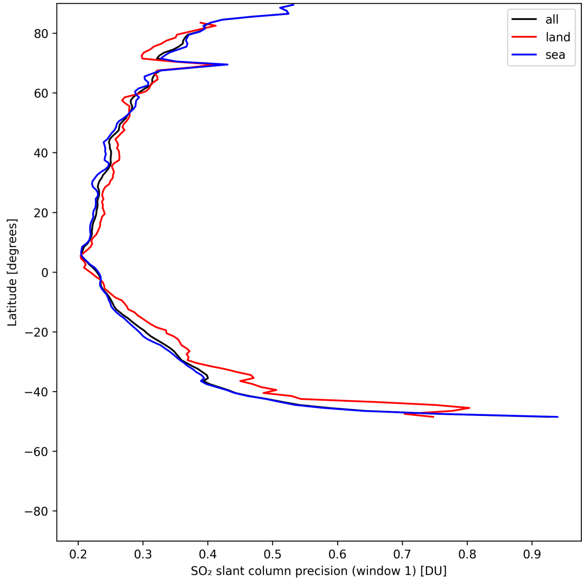
Figure 37: Zonal average of “SO 2 slant column precision (window 1)” for 2025-05-20 to 2025-05-21.
