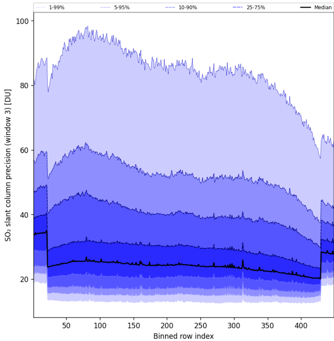
Figure 99: Along track statistics of “SO 2 slant column precision (window 3)” for 2025-05-20 to 2025-05-21
