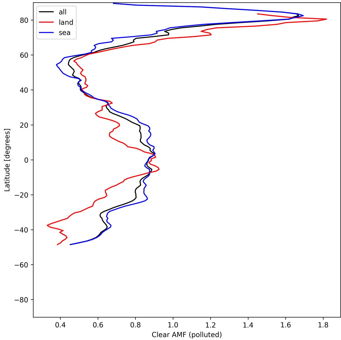
Figure 55: Zonal average of “Clear AMF (polluted)” for 2025-05-20 to 2025-05-21.
