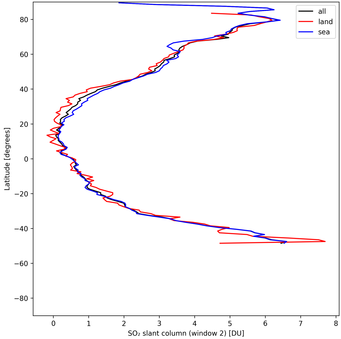
Figure 40: Zonal average of “SO 2 slant column (window 2)” for 2025-05-20 to 2025-05-21.
