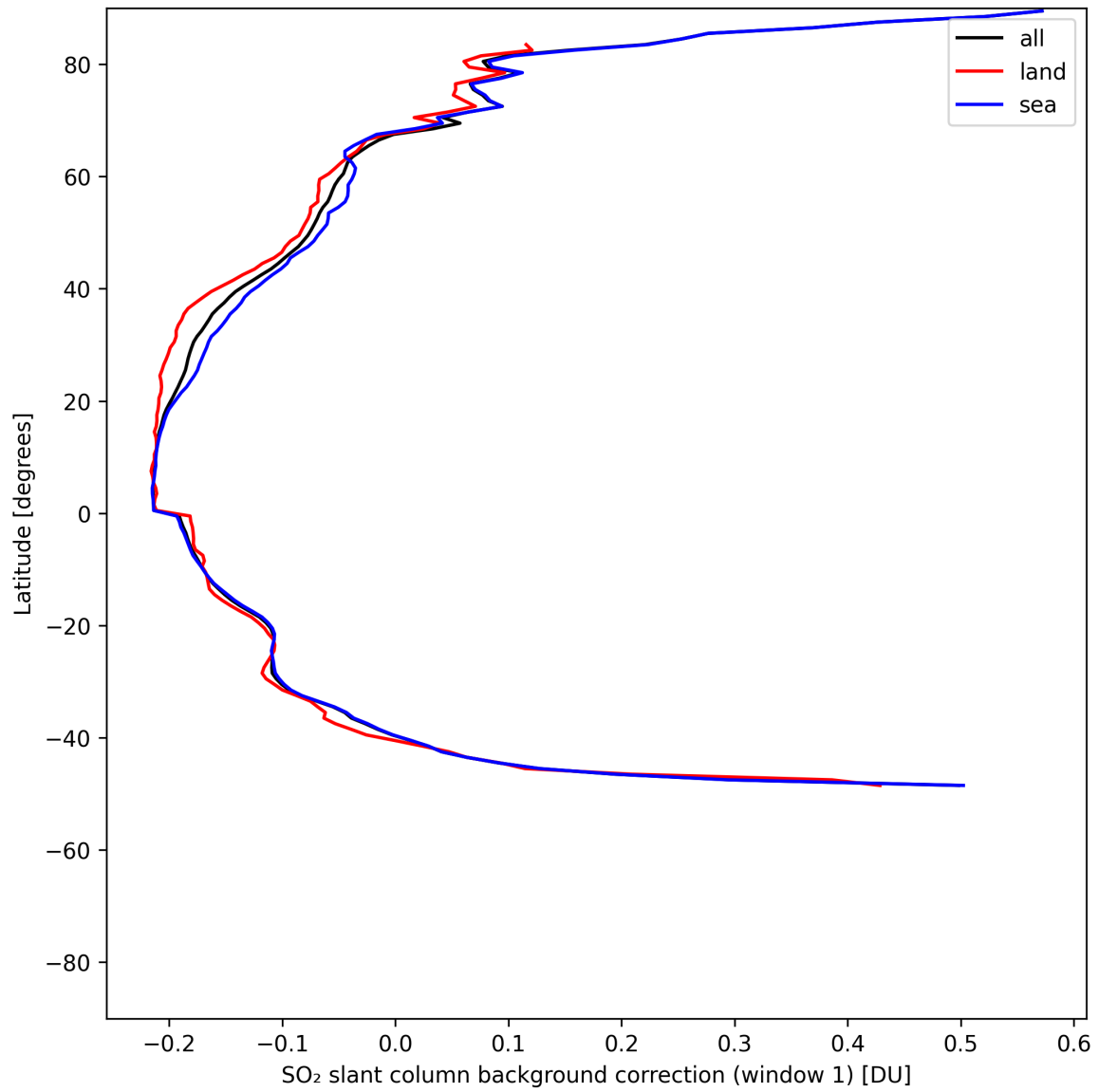
Figure 39: Zonal average of "SO 2 slant column background correction (window 1)" for 2025-05-20 to 2025-05-21.
