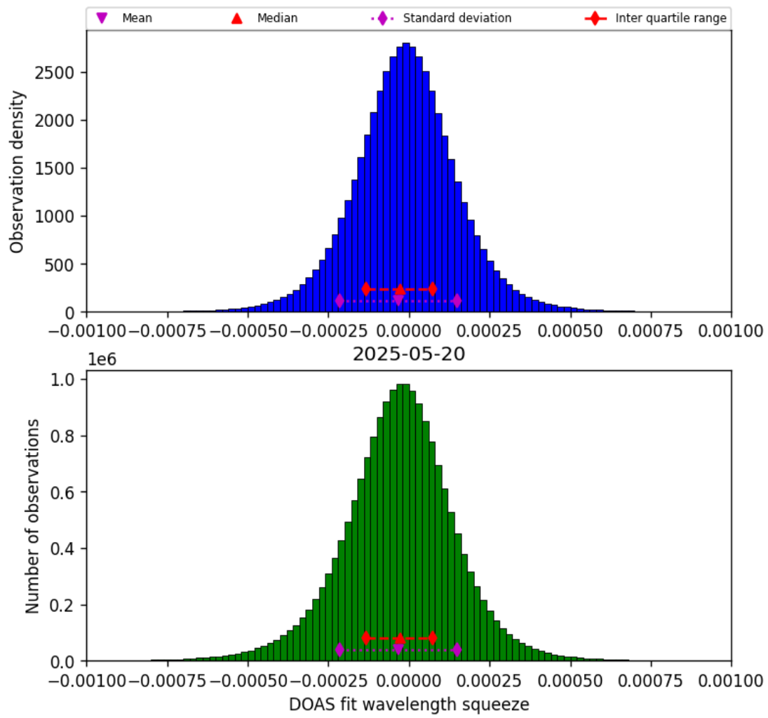
Figure 78: Histogram of "DOAS fit wavelength squeeze" for 2025-05-20 to 2025-05-21
