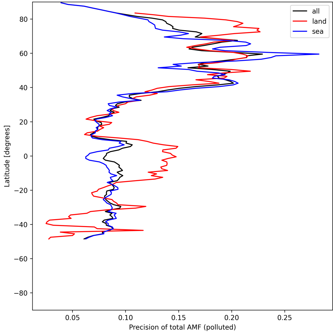
Figure 54: Zonal average of “Precision of total AMF (polluted)” for 2025-05-20 to 2025-05-21.
