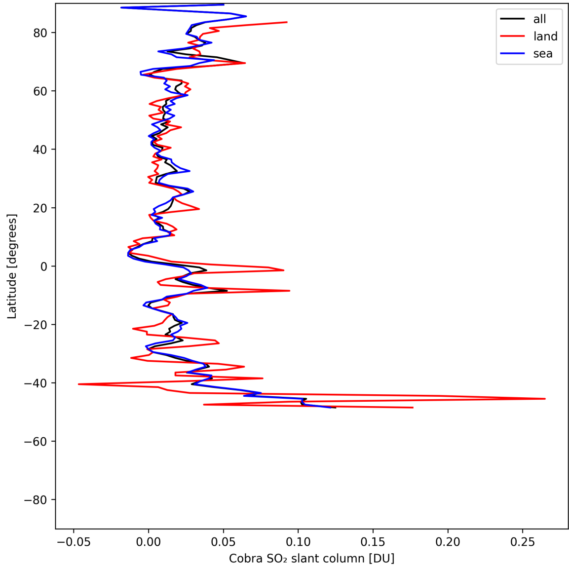
Figure 34: Zonal average of “Cobra SO 2 slant column” for 2025-05-20 to 2025-05-21.
