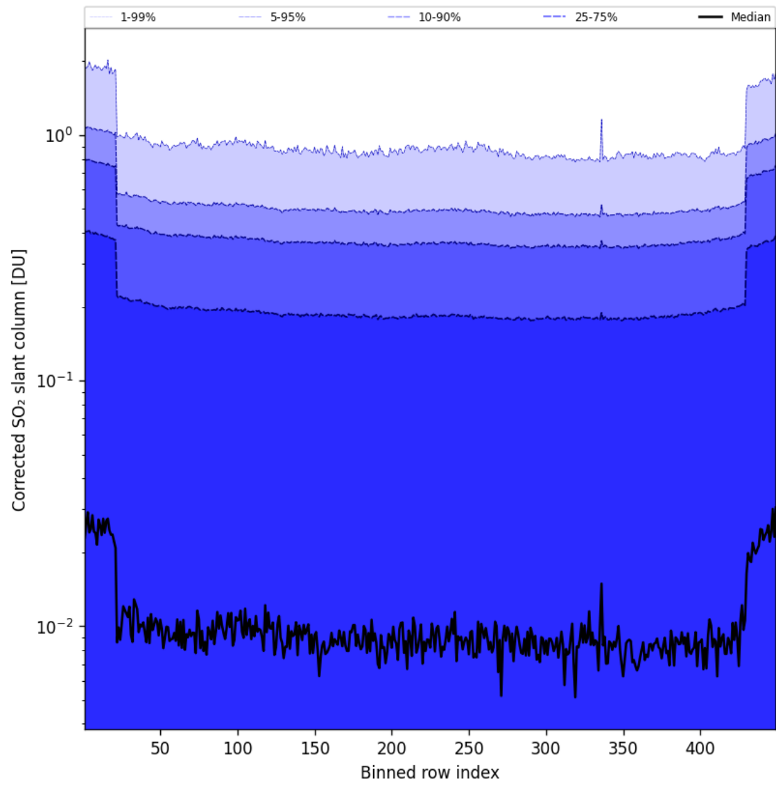
Figure 87: Along track statistics of “Corrected SO 2 slant column” for 2025-05-20 to 2025-05-21
