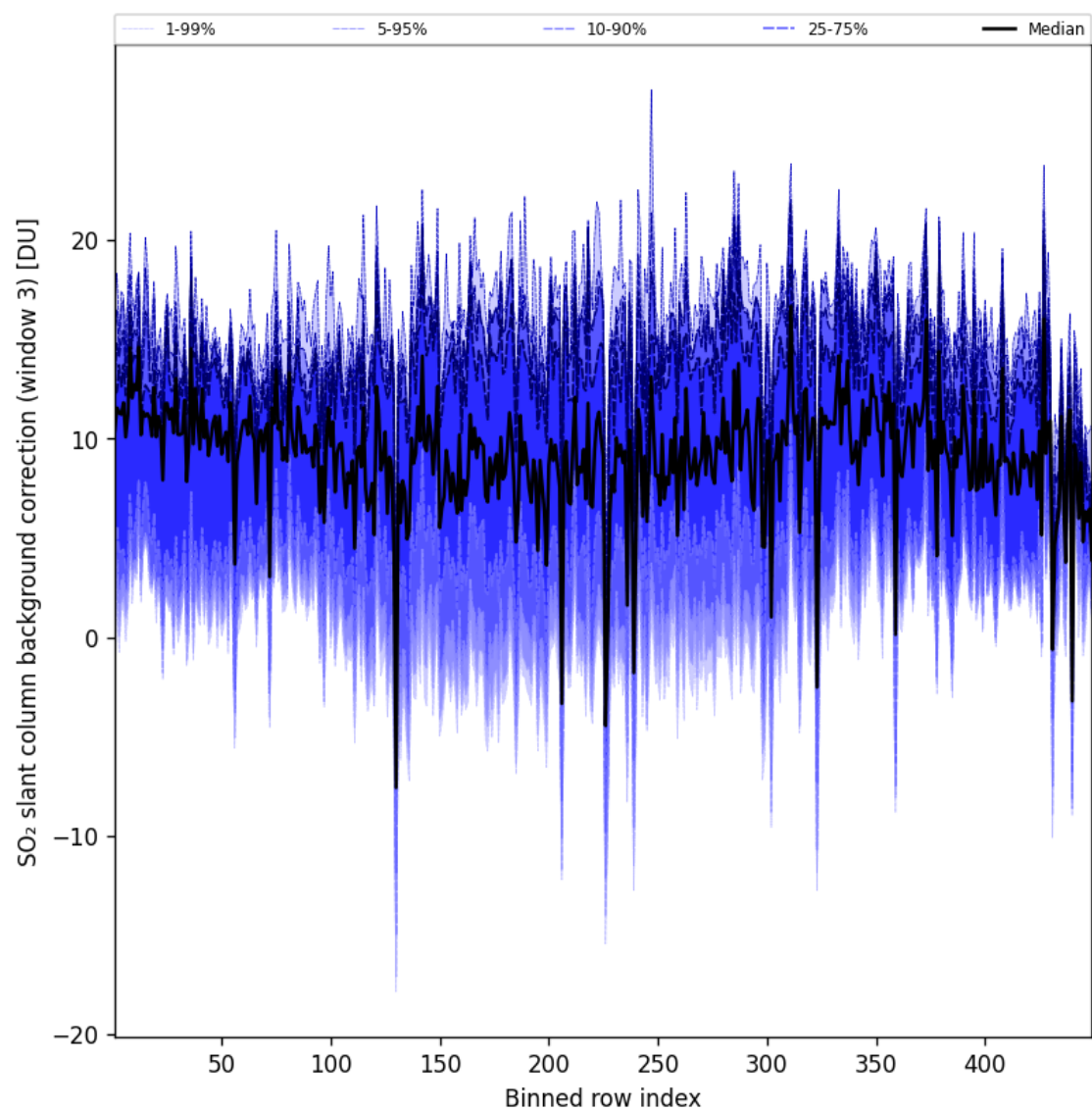
Figure 101: Along track statistics of "SO 2 slant column background correction (window 3)" for 2025-05-20 to 2025-05-21
