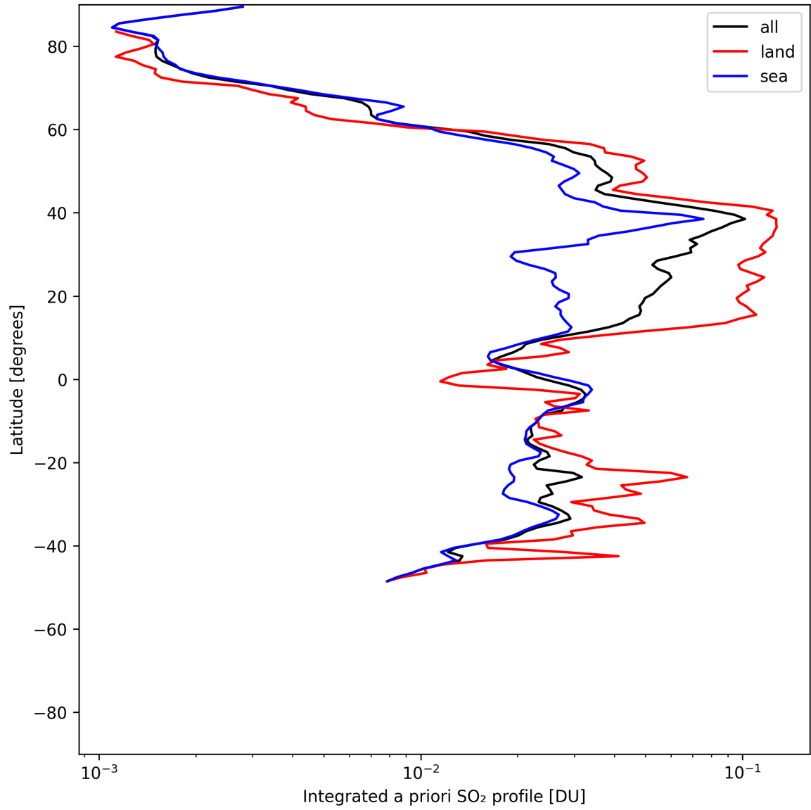
Figure 49: Zonal average of “Integrated a priori SO 2 profile” for 2025-05-20 to 2025-05-21.
