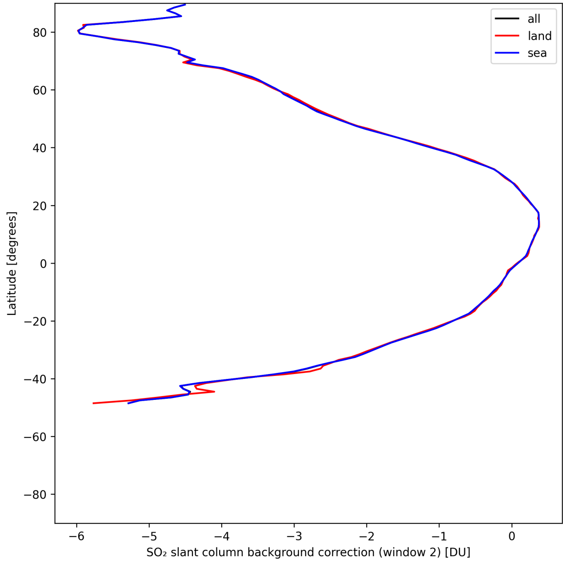
Figure 43: Zonal average of “SO 2 slant column background correction (window 2)” for 2025-05-20 to 2025-05-21.
