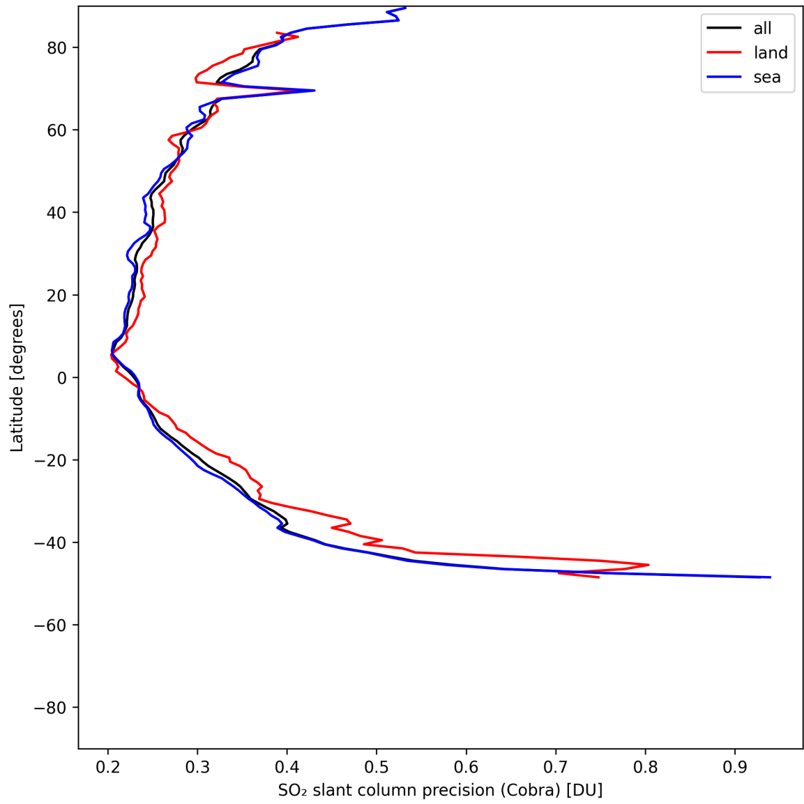
Figure 35: Zonal average of “SO 2 slant column precision (Cobra)” for 2025-05-20 to 2025-05-21.
