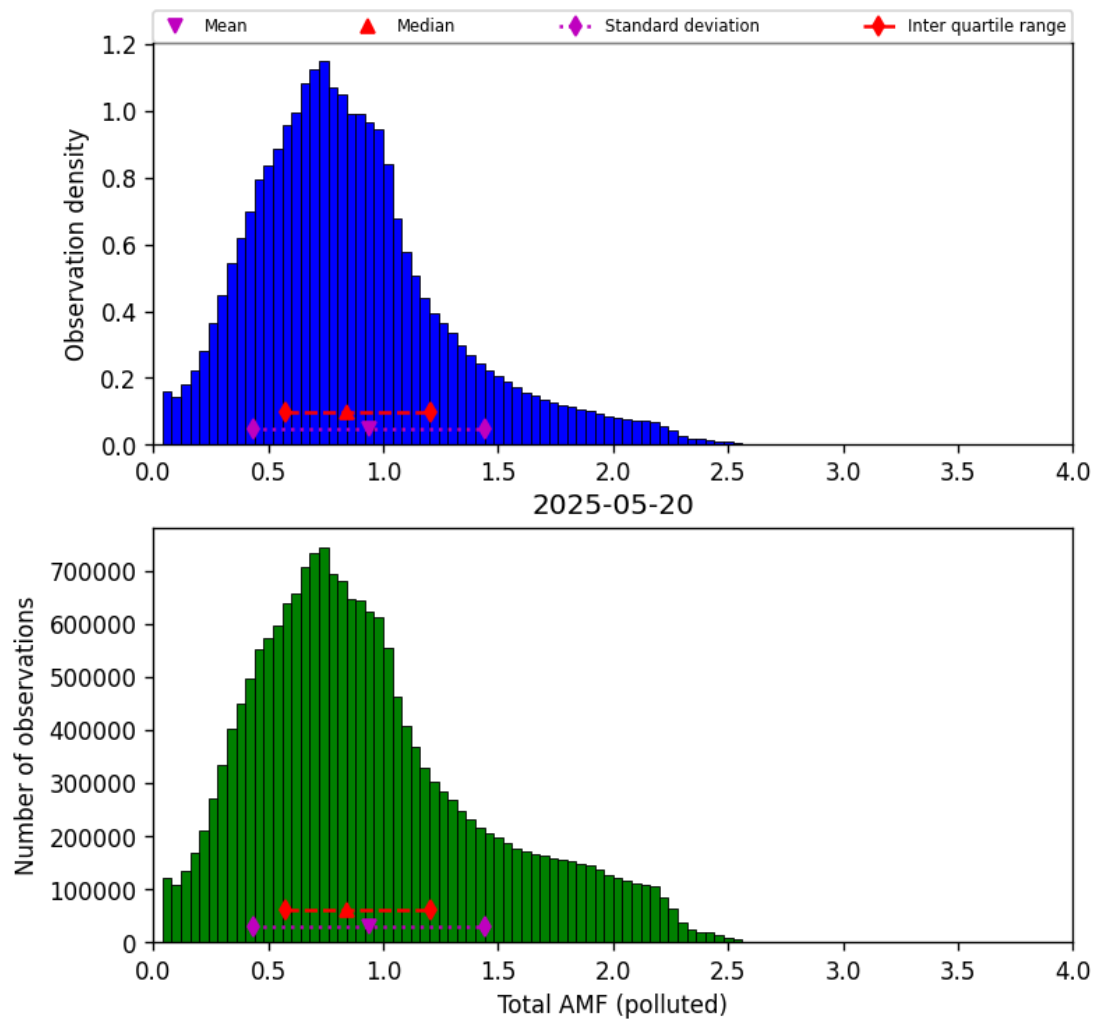
Figure 80: Histogram of “Total AMF (polluted)” for 2025-05-20 to 2025-05-21
