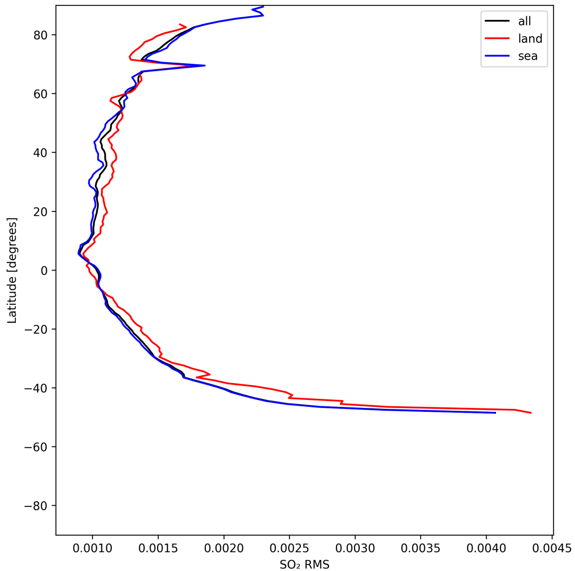
Figure 52: Zonal average of “SO 2 RMS” for 2025-05-20 to 2025-05-21.
