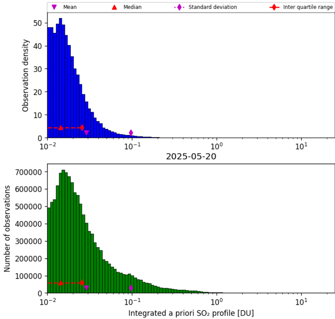
Figure 76: Histogram of “Integrated a priori SO 2 profile” for 2025-05-20 to 2025-05-21
