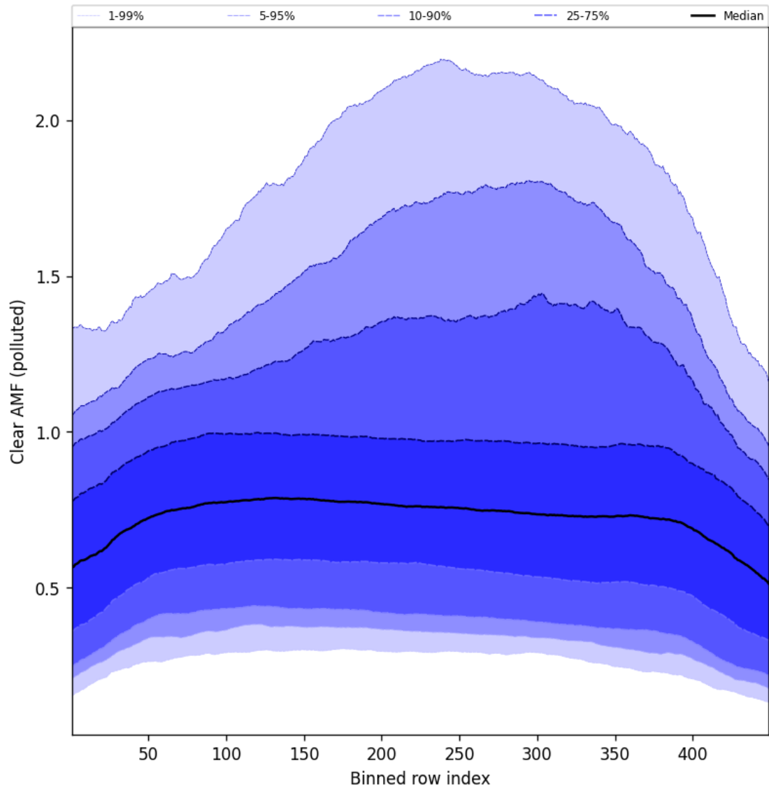
Figure 109: Along track statistics of “Clear AMF (polluted)” for 2025-05-20 to 2025-05-21
