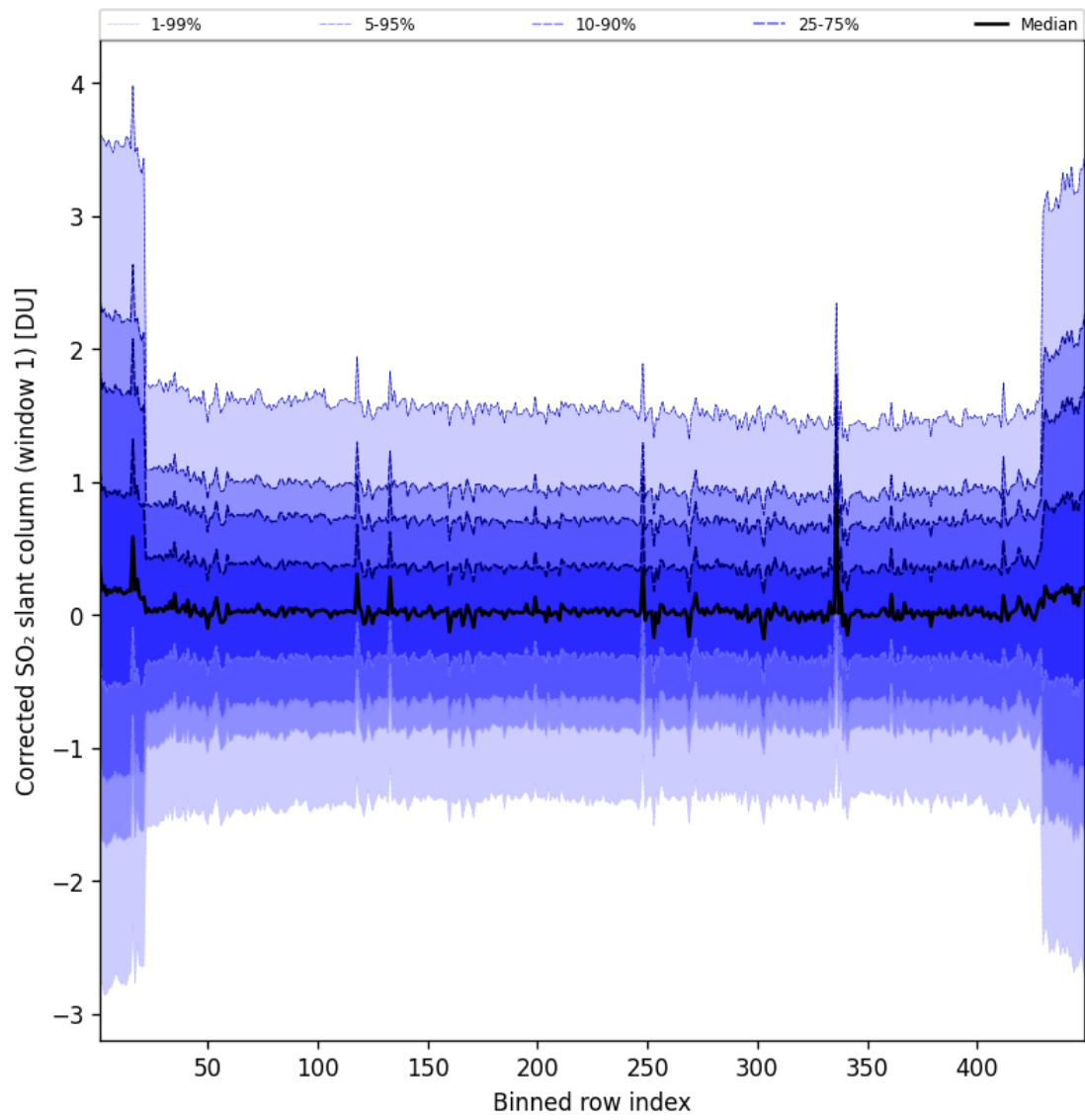
Figure 92: Along track statistics of “Corrected SO 2 slant column (window 1)” for 2025-05-20 to 2025-05-21
