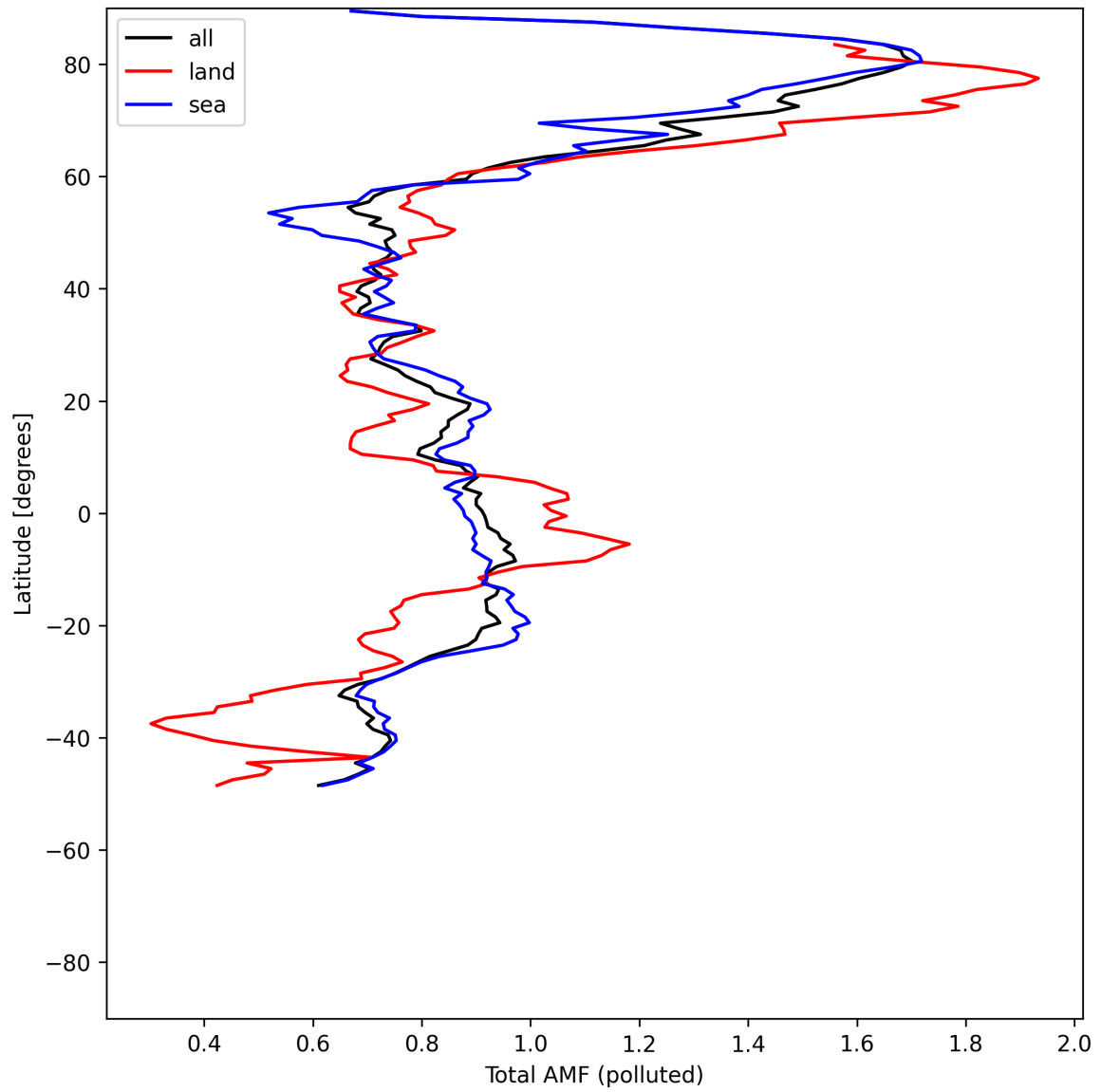
Figure 53: Zonal average of “Total AMF (polluted)” for 2025-05-20 to 2025-05-21.
