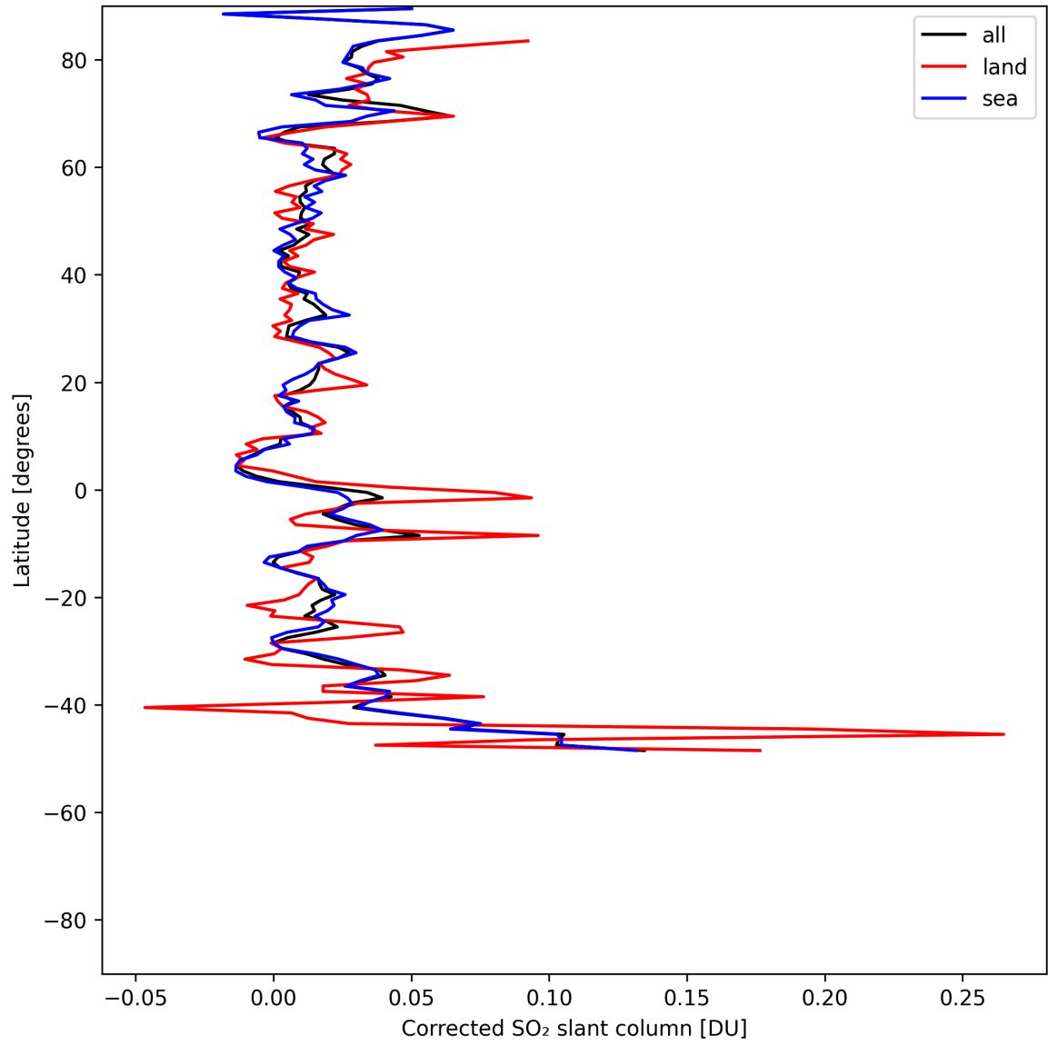
Figure 33: Zonal average of “Corrected SO 2 slant column” for 2025-05-20 to 2025-05-21.
