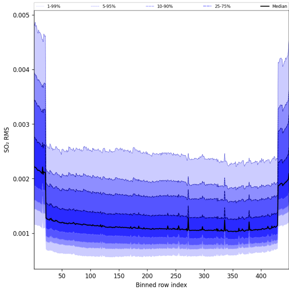
Figure 106: Along track statistics of “SO 2 RMS” for 2025-05-20 to 2025-05-21
