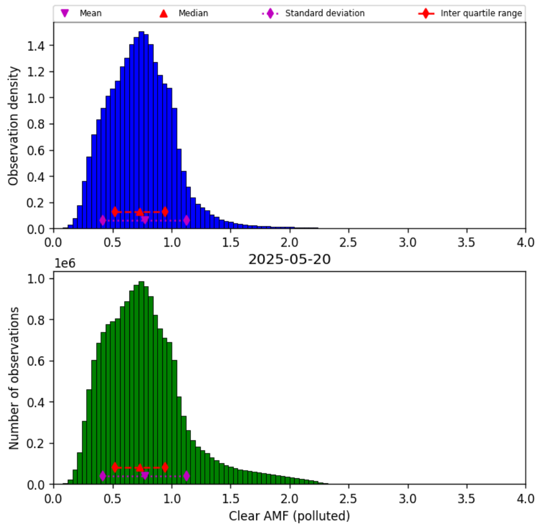
Figure 82: Histogram of “Clear AMF (polluted)” for 2025-05-20 to 2025-05-21
