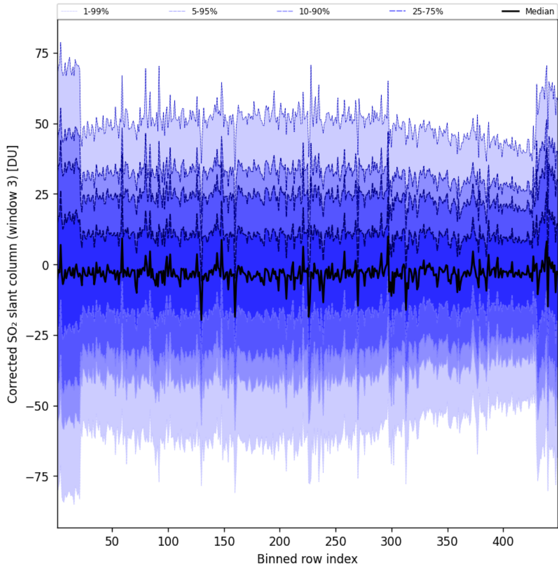
Figure 100: Along track statistics of “Corrected SO 2 slant column (window 3)” for 2025-05-20 to 2025-05-21
