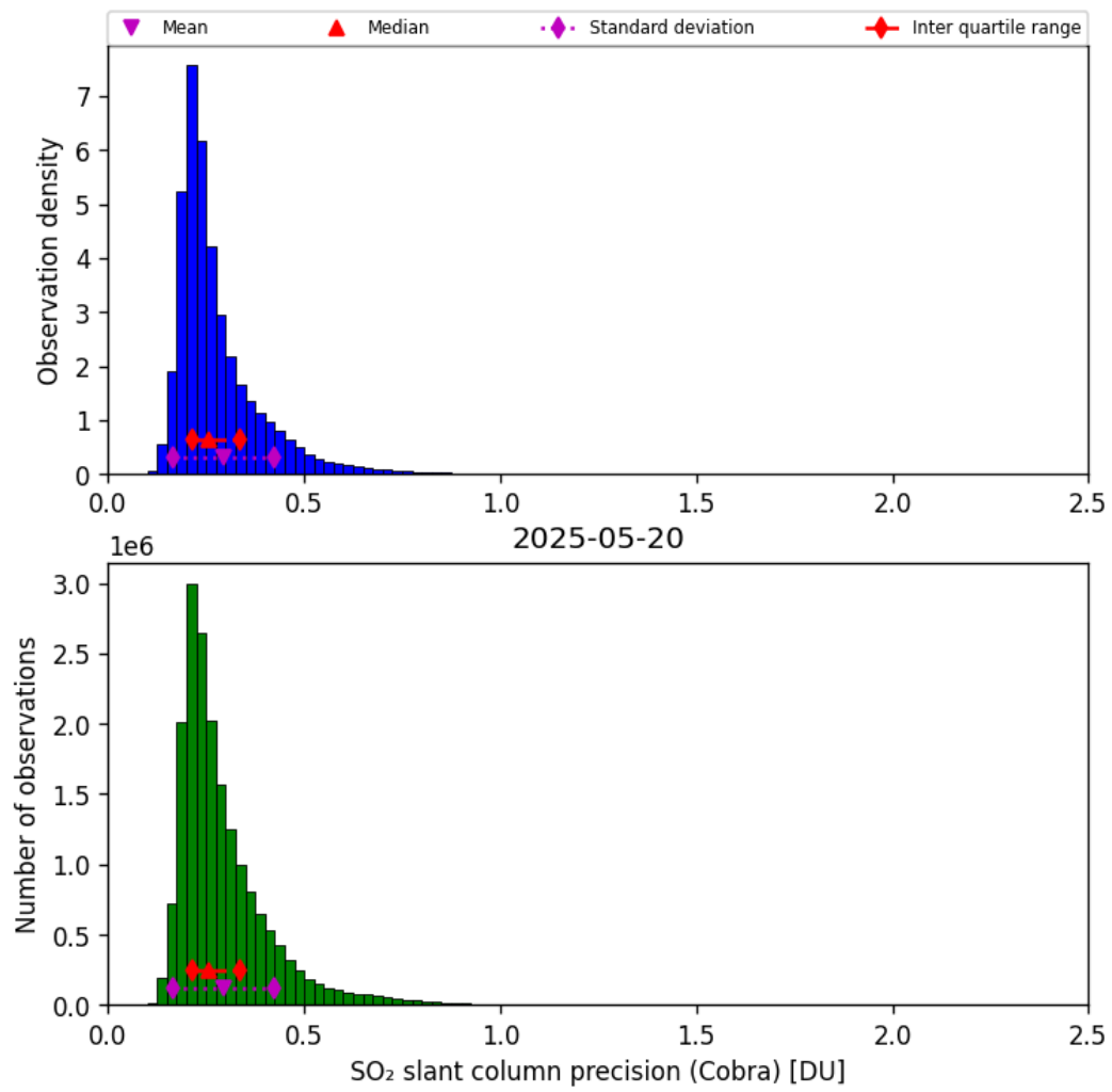
Figure 62: Histogram of “SO 2 slant column precision (Cobra)” for 2025-05-20 to 2025-05-21
