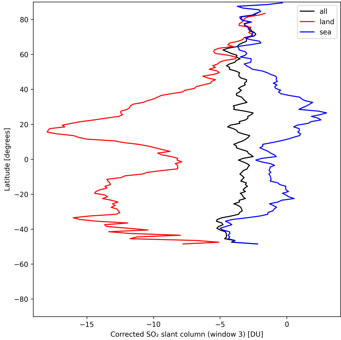
Figure 46: Zonal average of “Corrected SO 2 slant column (window 3)” for 2025-05-20 to 2025-05-21.
