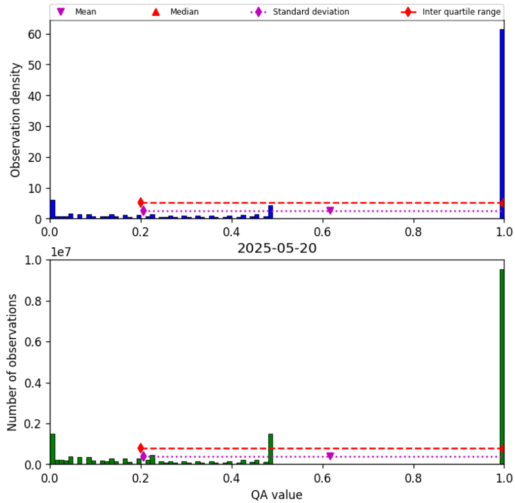
Figure 57: Histogram of “QA value” for 2025-05-20 to 2025-05-21
