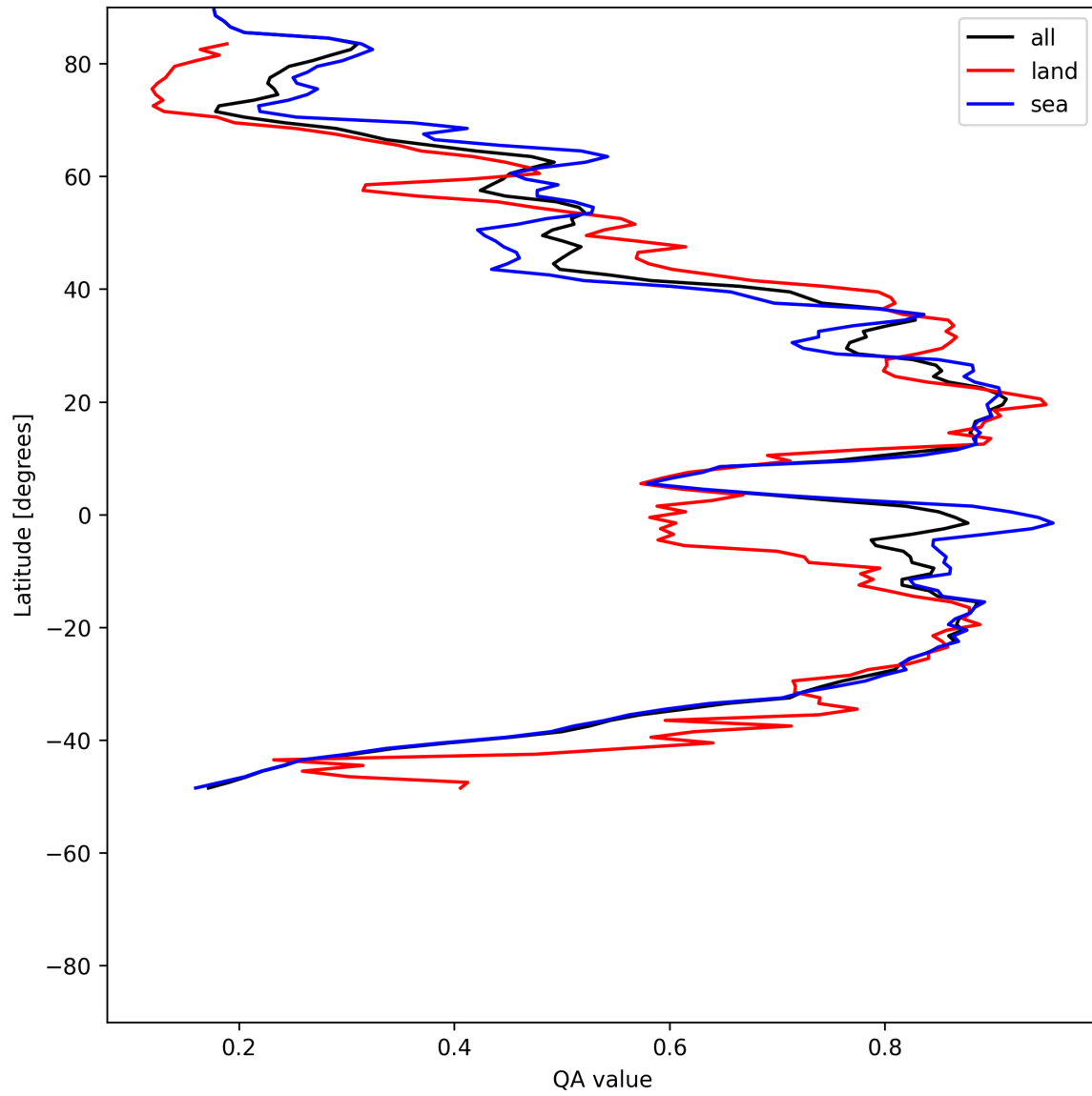
Figure 30: Zonal average of “QA value” for 2025-05-20 to 2025-05-21.
