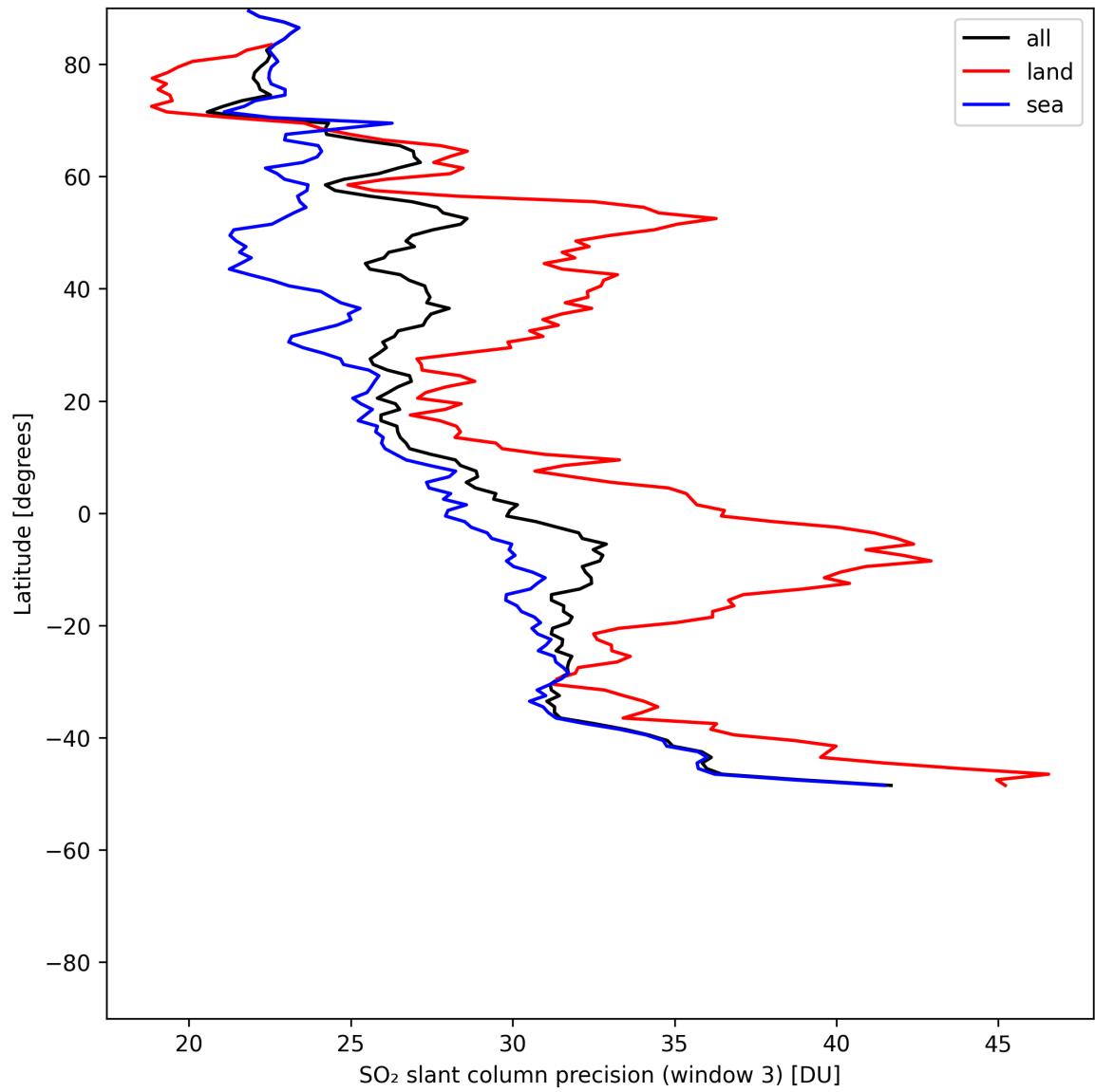
Figure 45: Zonal average of “SO 2 slant column precision (window 3)” for 2025-05-20 to 2025-05-21.
