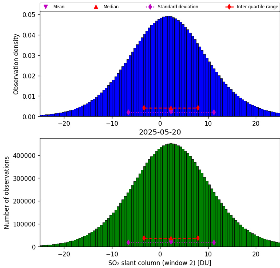
Figure 67: Histogram of “SO 2 slant column (window 2)” for 2025-05-20 to 2025-05-21
