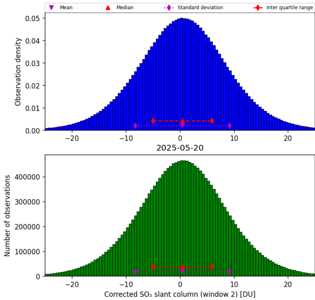
Figure 69: Histogram of “Corrected SO 2 slant column (window 2)” for 2025-05-20 to 2025-05-21
