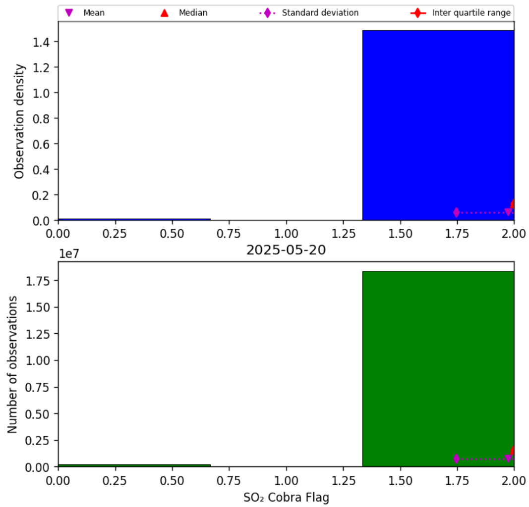
Figure 75: Histogram of “SO 2 Cobra Flag” for 2025-05-20 to 2025-05-21
