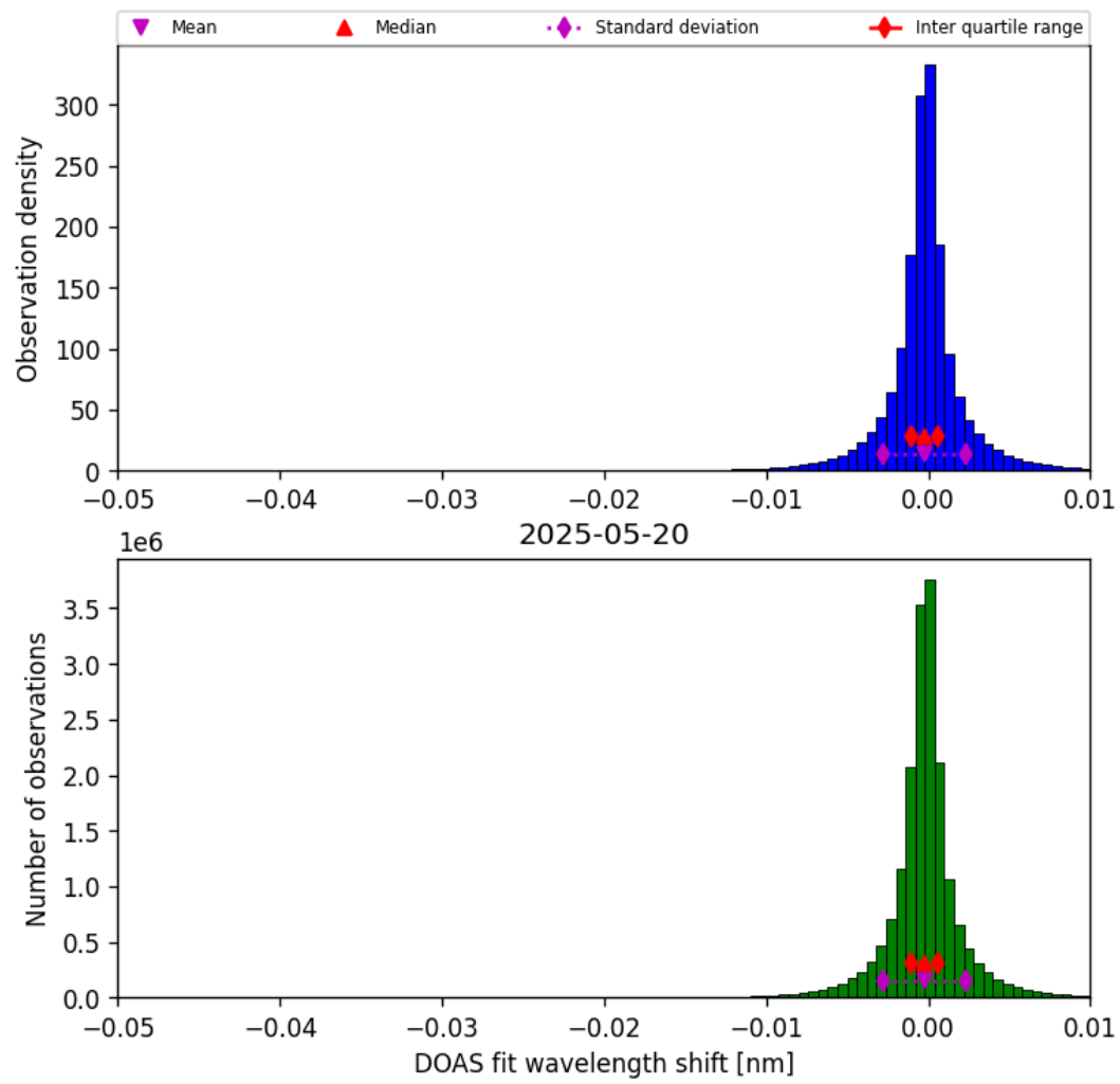
Figure 77: Histogram of “DOAS fit wavelength shift” for 2025-05-20 to 2025-05-21
