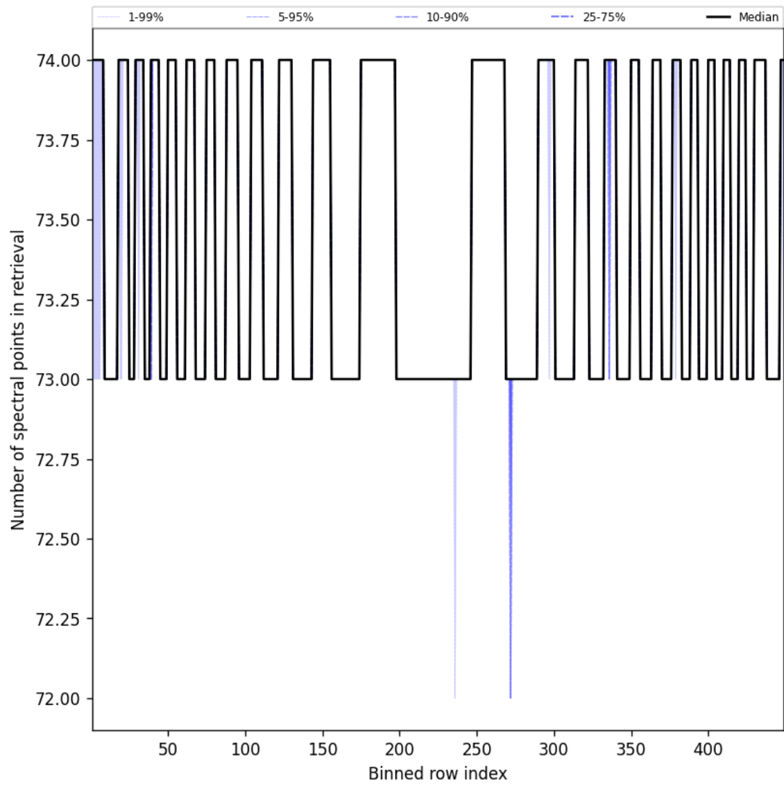
Figure 110: Along track statistics of “Number of spectral points in retrieval” for 2025-05-20 to 2025-05-21
