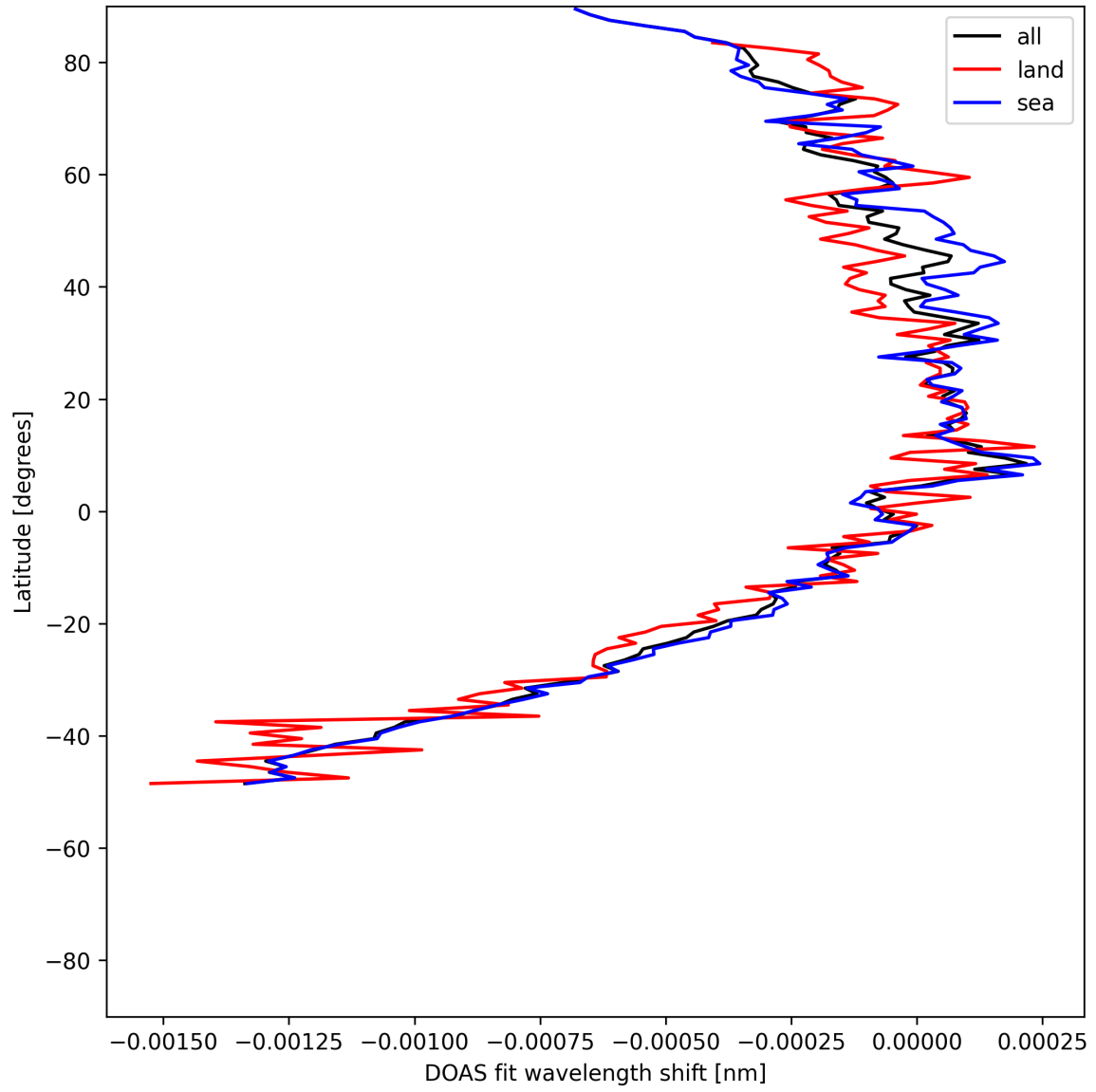
Figure 50: Zonal average of “DOAS fit wavelength shift” for 2025-05-20 to 2025-05-21.
