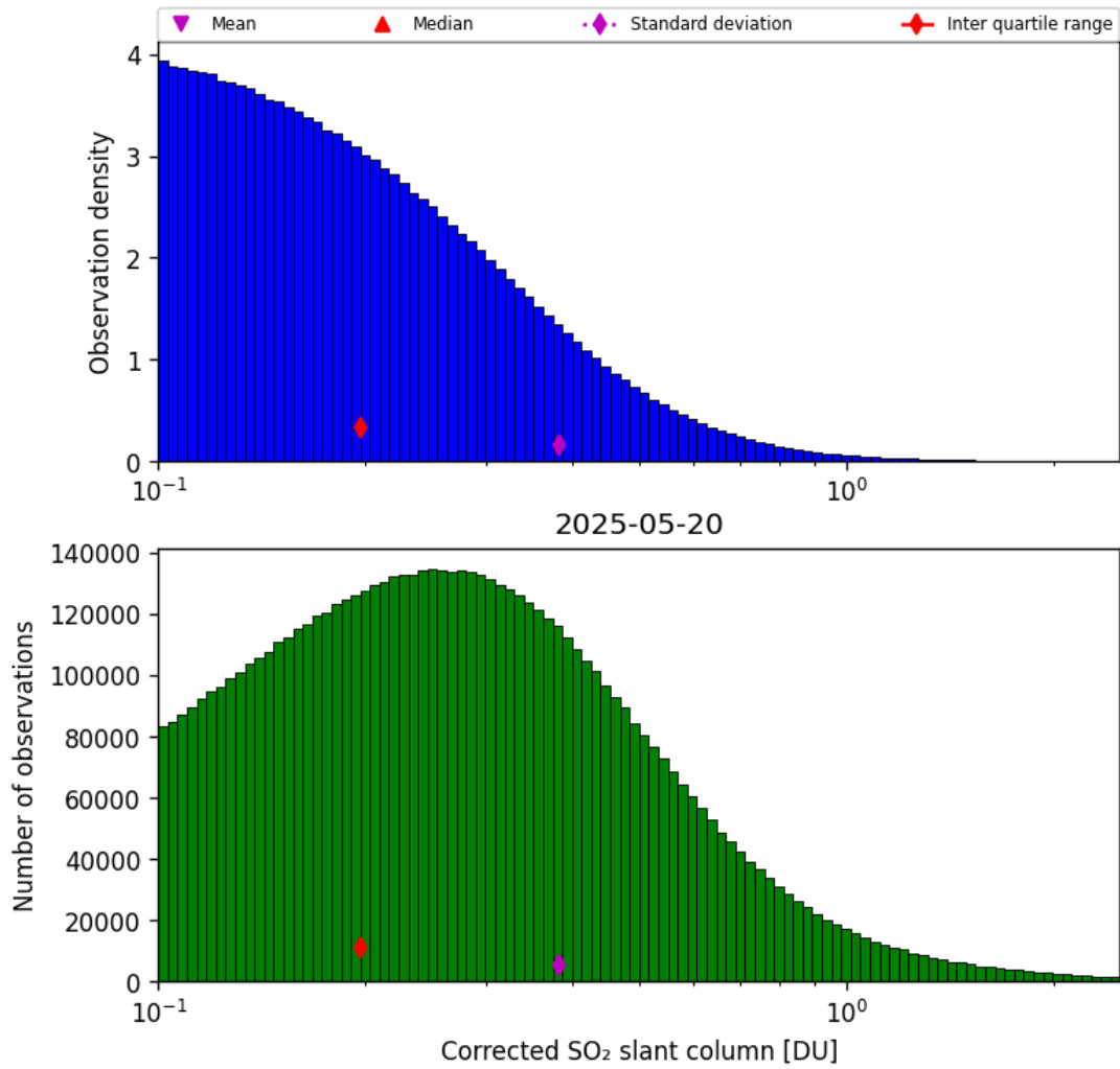
Figure 60: Histogram of “Corrected SO 2 slant column” for 2025-05-20 to 2025-05-21
