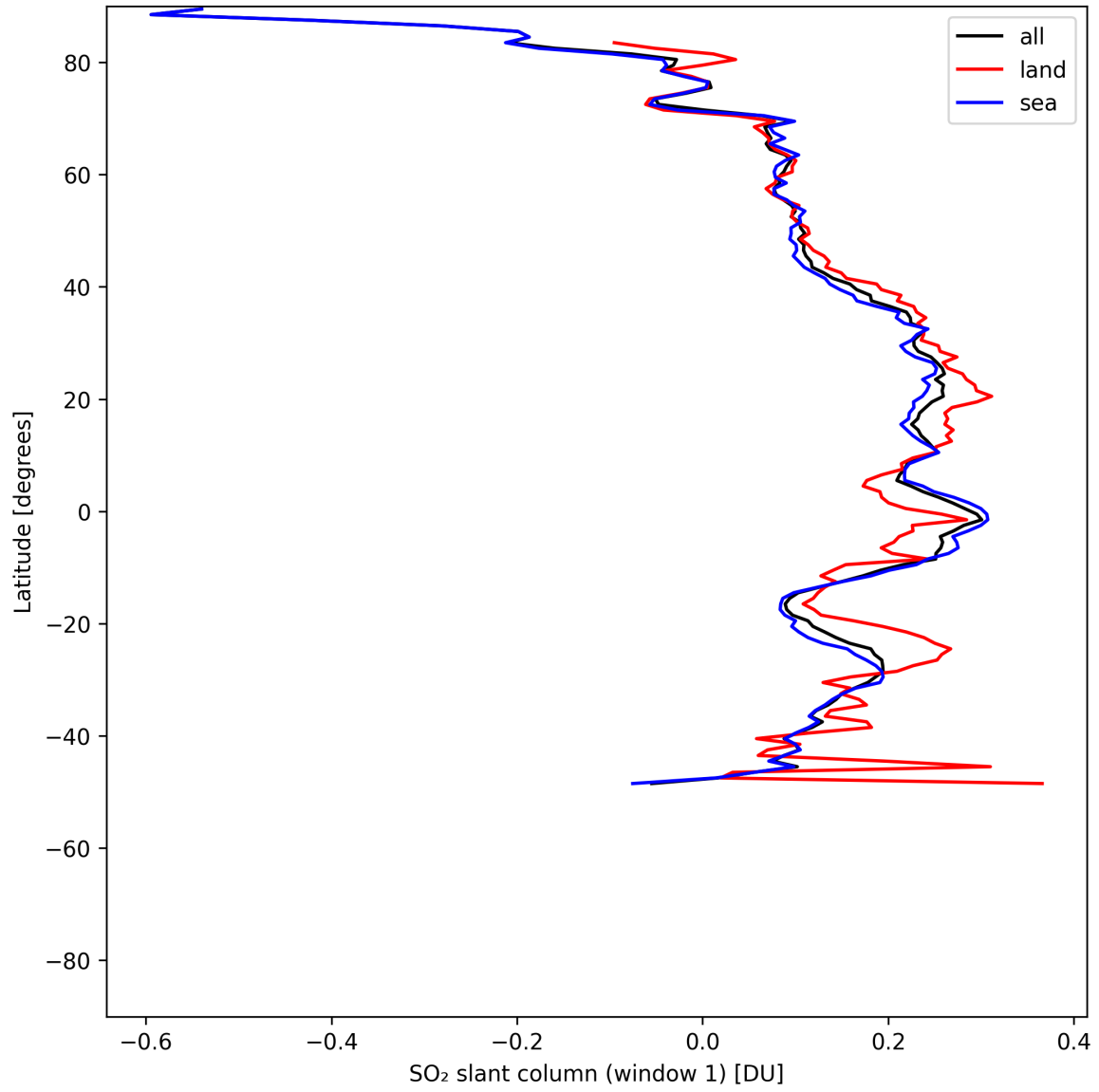
Figure 36: Zonal average of “SO 2 slant column (window 1)” for 2025-05-20 to 2025-05-21.
