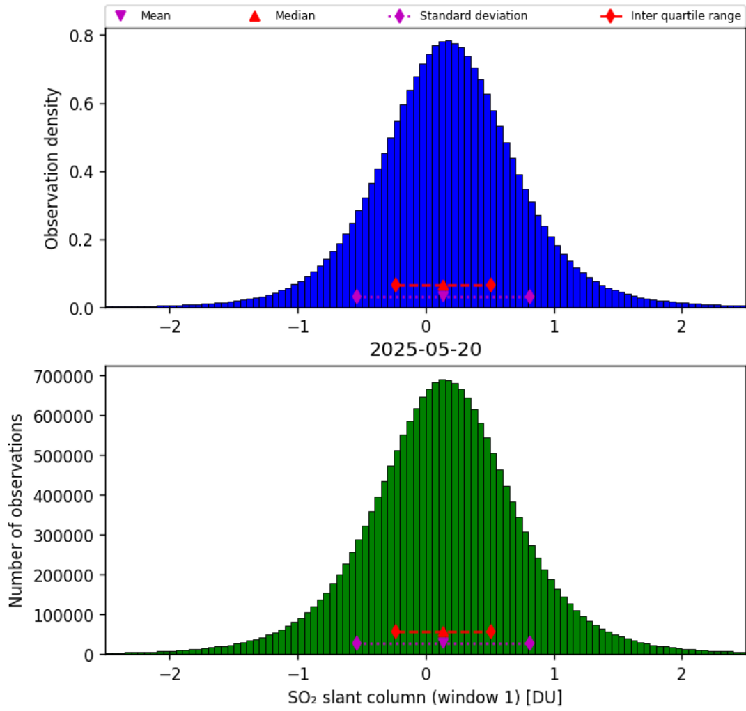
Figure 63: Histogram of “SO 2 slant column (window 1)” for 2025-05-20 to 2025-05-21
