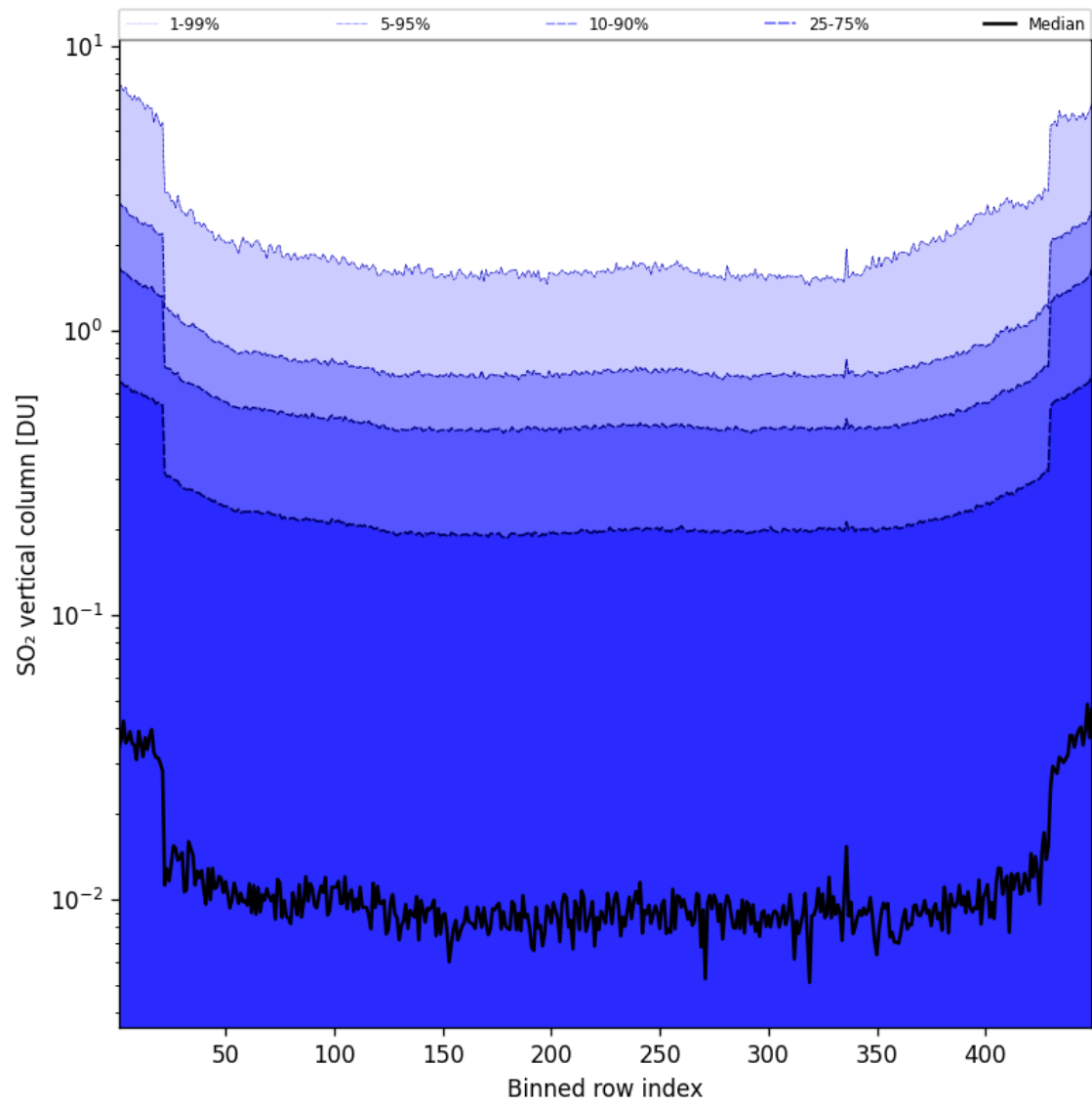
Figure 85: Along track statistics of “SO 2 vertical column” for 2025-05-20 to 2025-05-21
