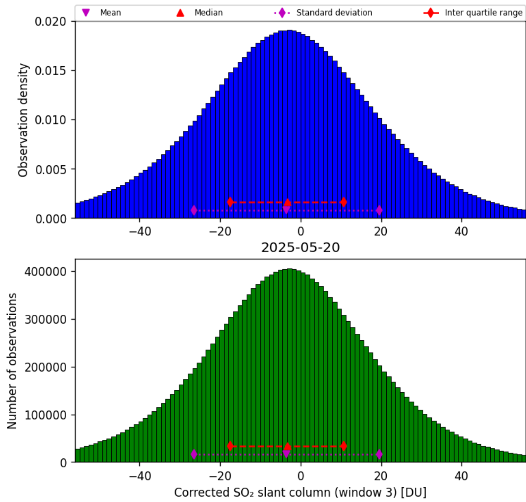
Figure 73: Histogram of “Corrected SO 2 slant column (window 3)” for 2025-05-20 to 2025-05-21
