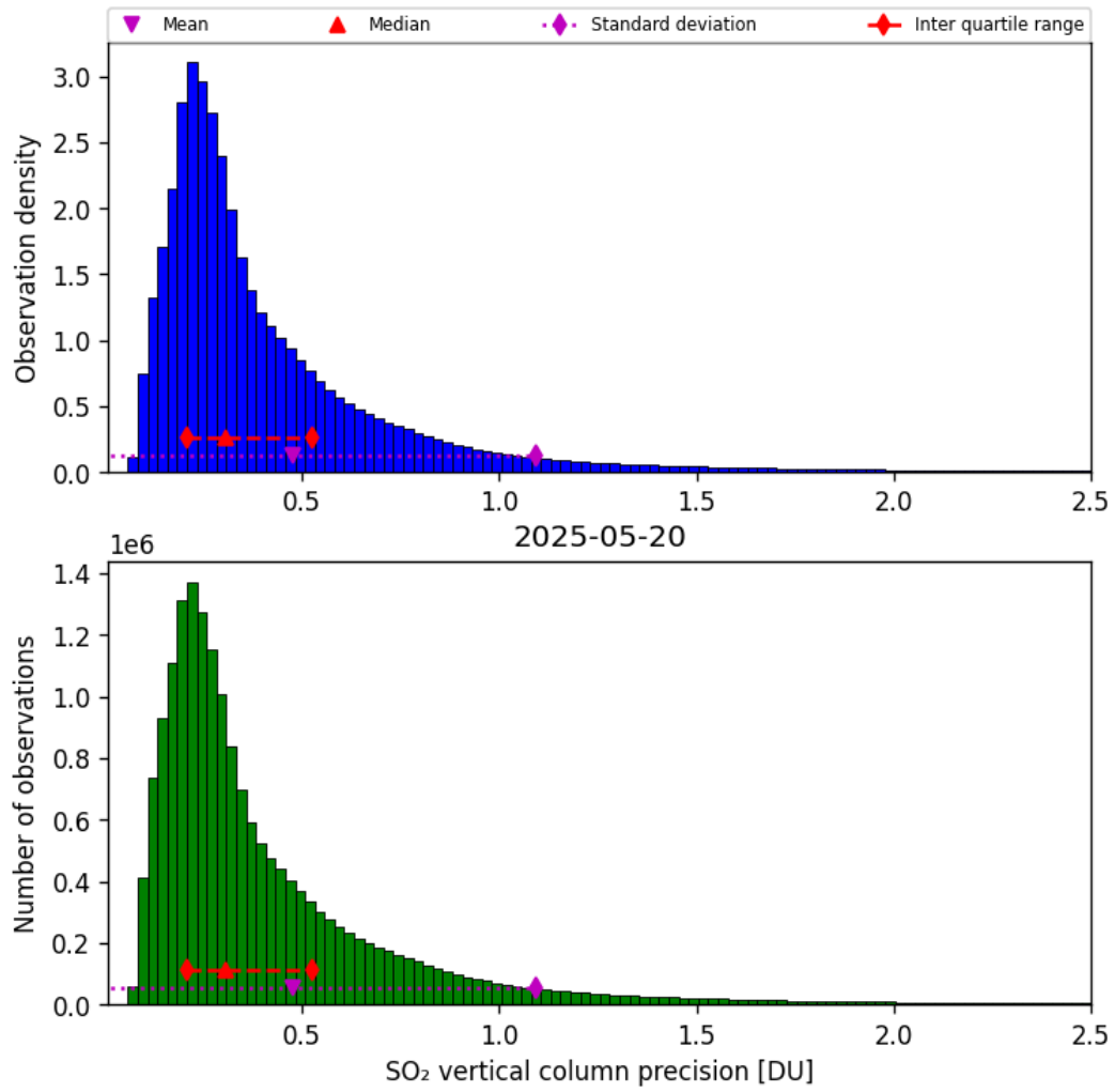
Figure 59: Histogram of “SO 2 vertical column precision” for 2025-05-20 to 2025-05-21
