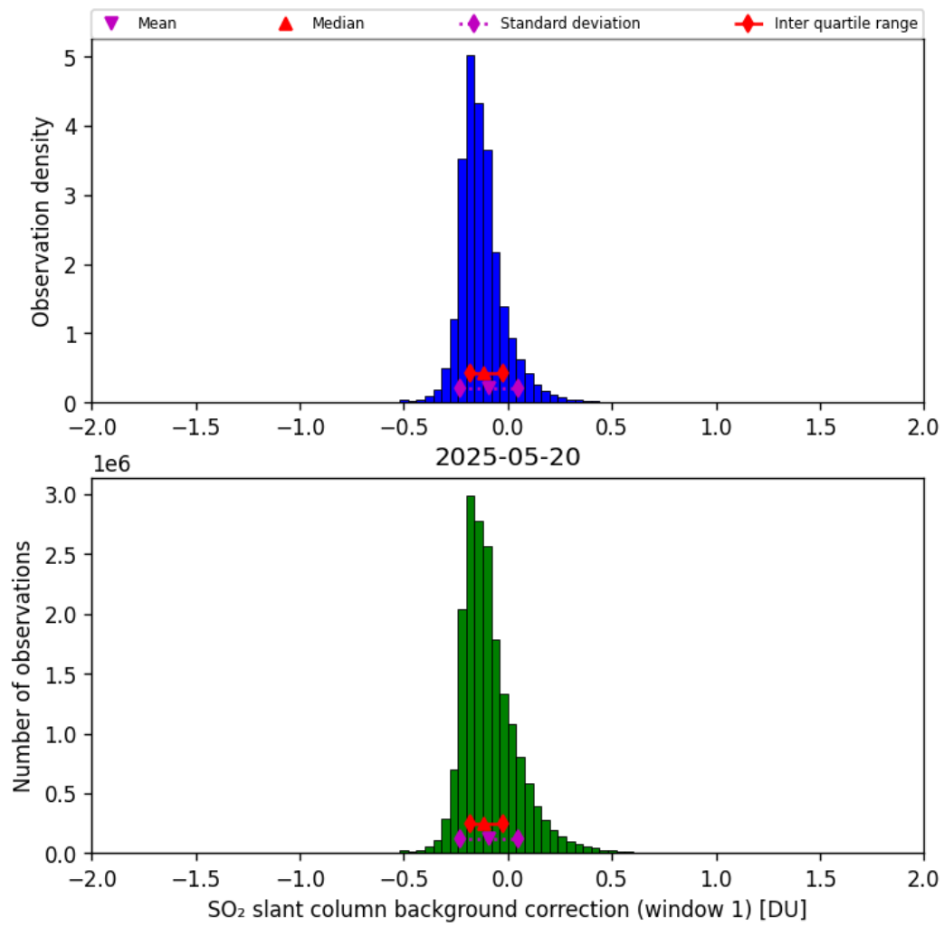
Figure 66: Histogram of “SO 2 slant column background correction (window 1)” for 2025-05-20 to 2025-05-21
