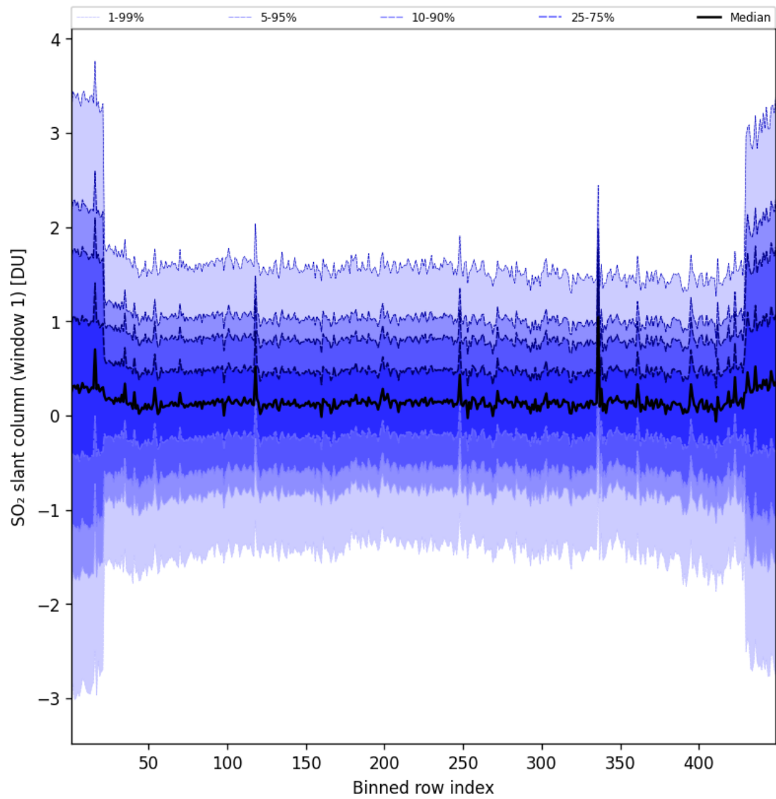
Figure 90: Along track statistics of “SO 2 slant column (window 1)” for 2025-05-20 to 2025-05-21
