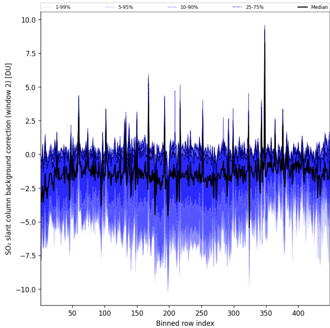
Figure 97: Along track statistics of “SO 2 slant column background correction (window 2)” for 2025-05-20 to 2025-05-21
