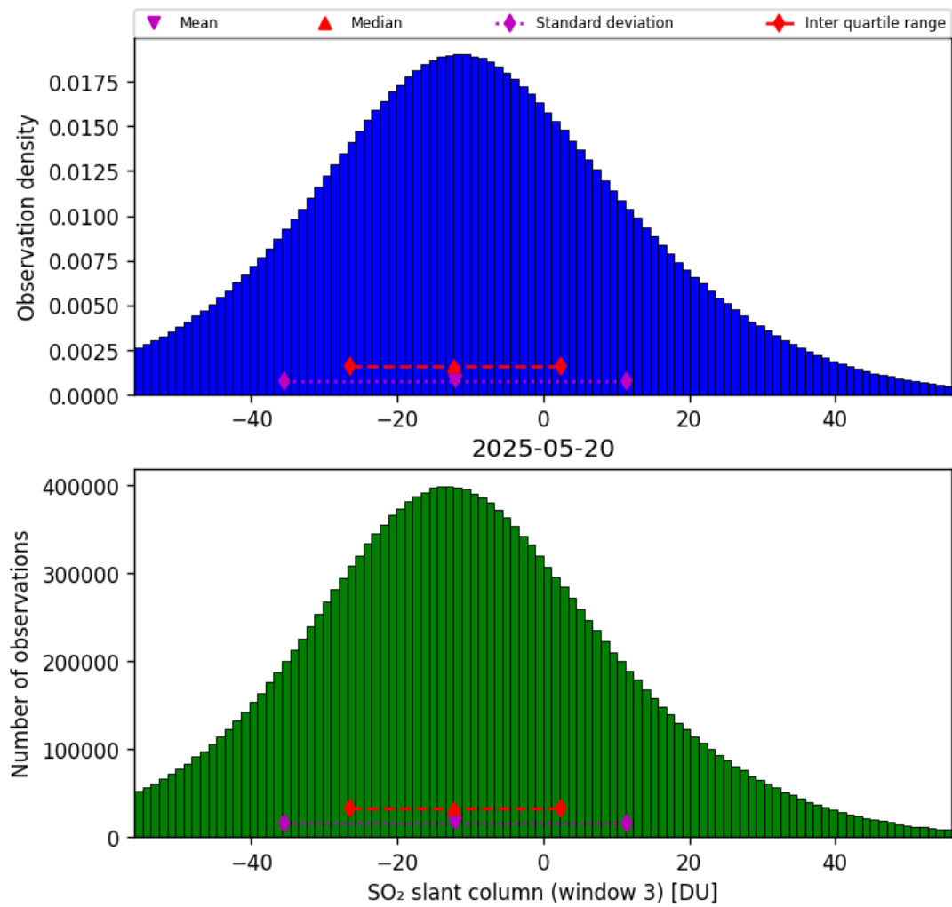
Figure 71: Histogram of “SO 2 slant column (window 3)” for 2025-05-20 to 2025-05-21
