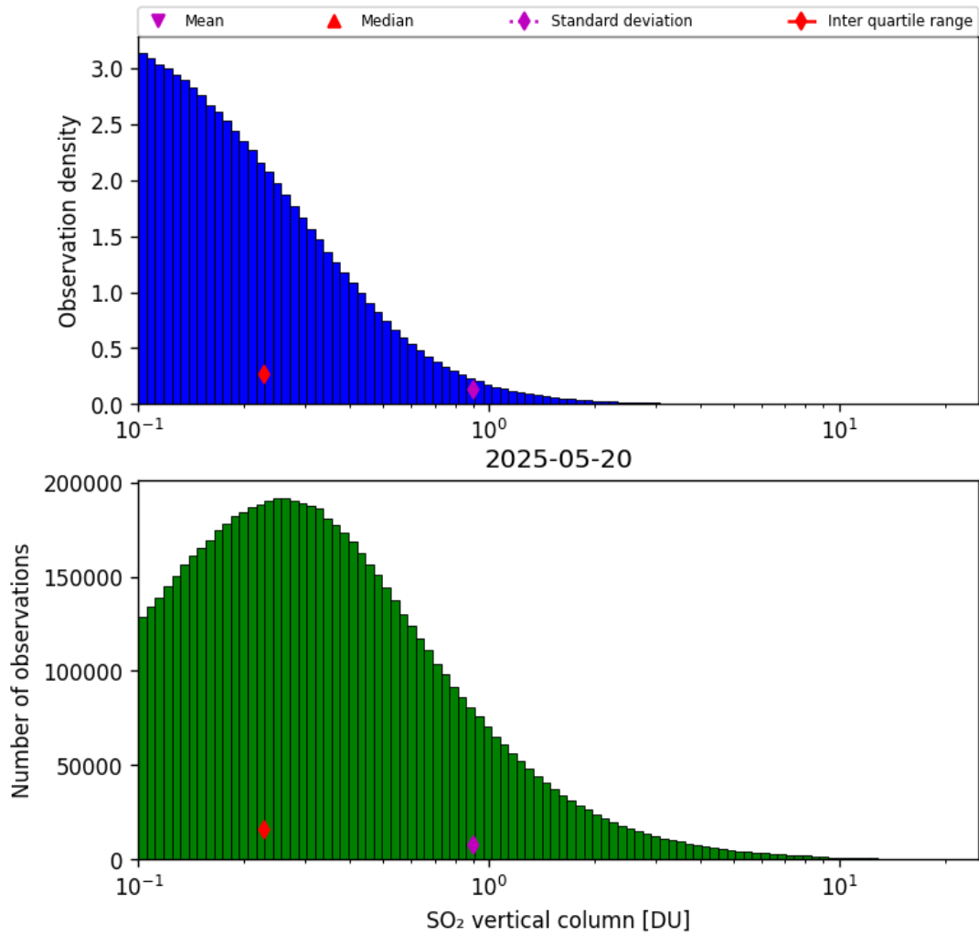
Figure 58: Histogram of “SO 2 vertical column” for 2025-05-20 to 2025-05-21
