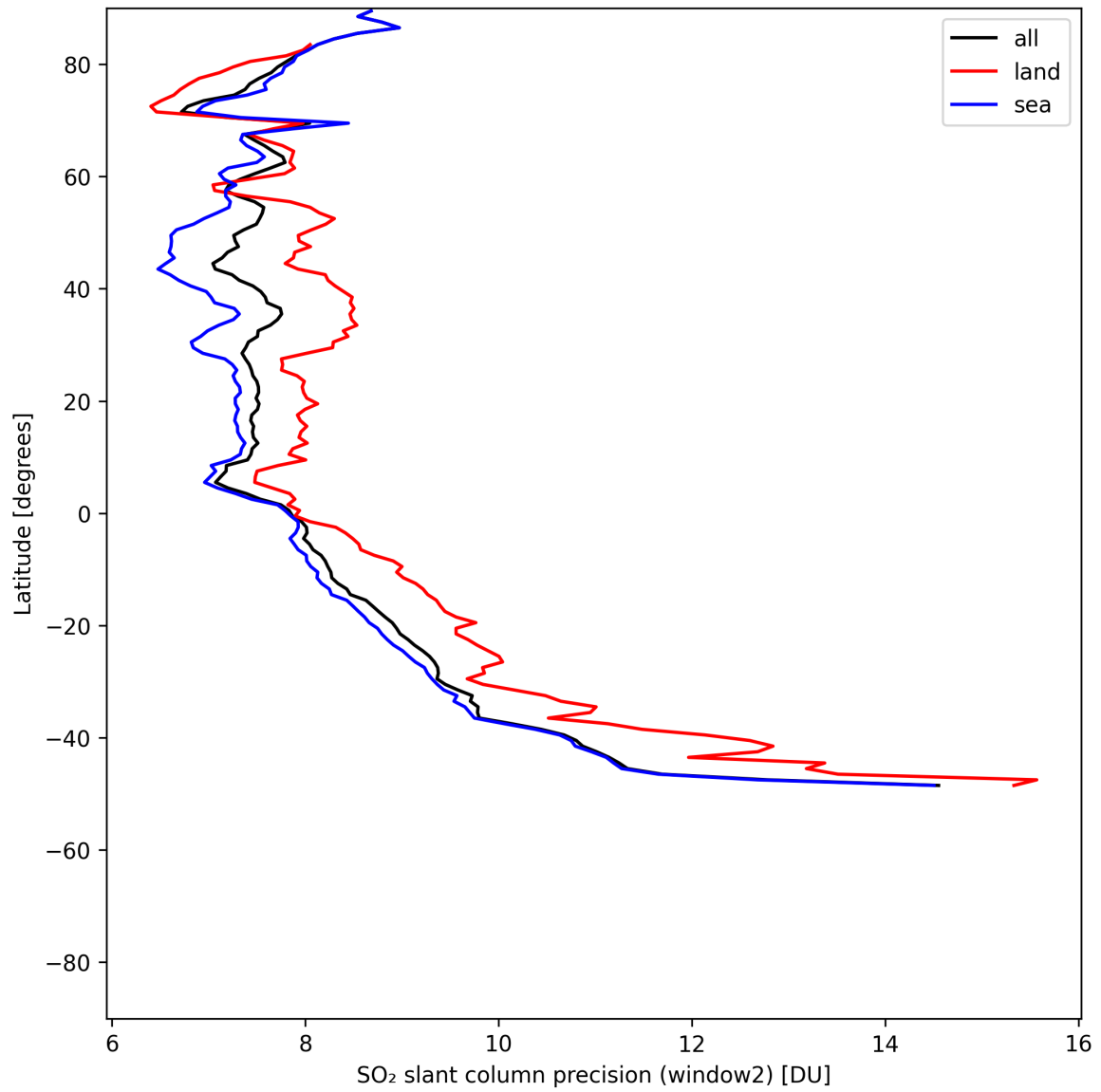
Figure 41: Zonal average of “SO 2 slant column precision (window2)” for 2025-05-20 to 2025-05-21.
