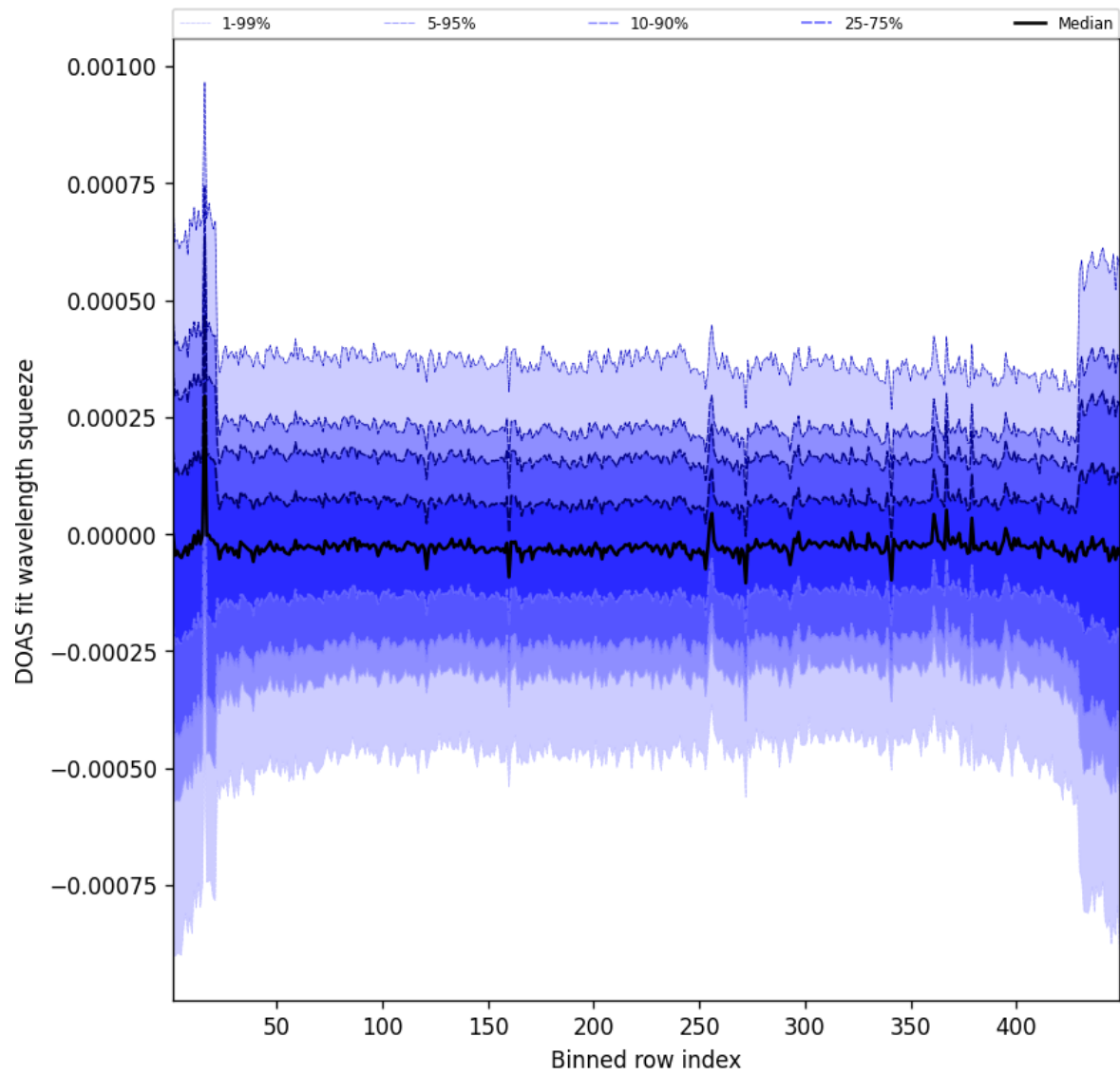
Figure 105: Along track statistics of “DOAS fit wavelength squeeze” for 2025-05-20 to 2025-05-21
