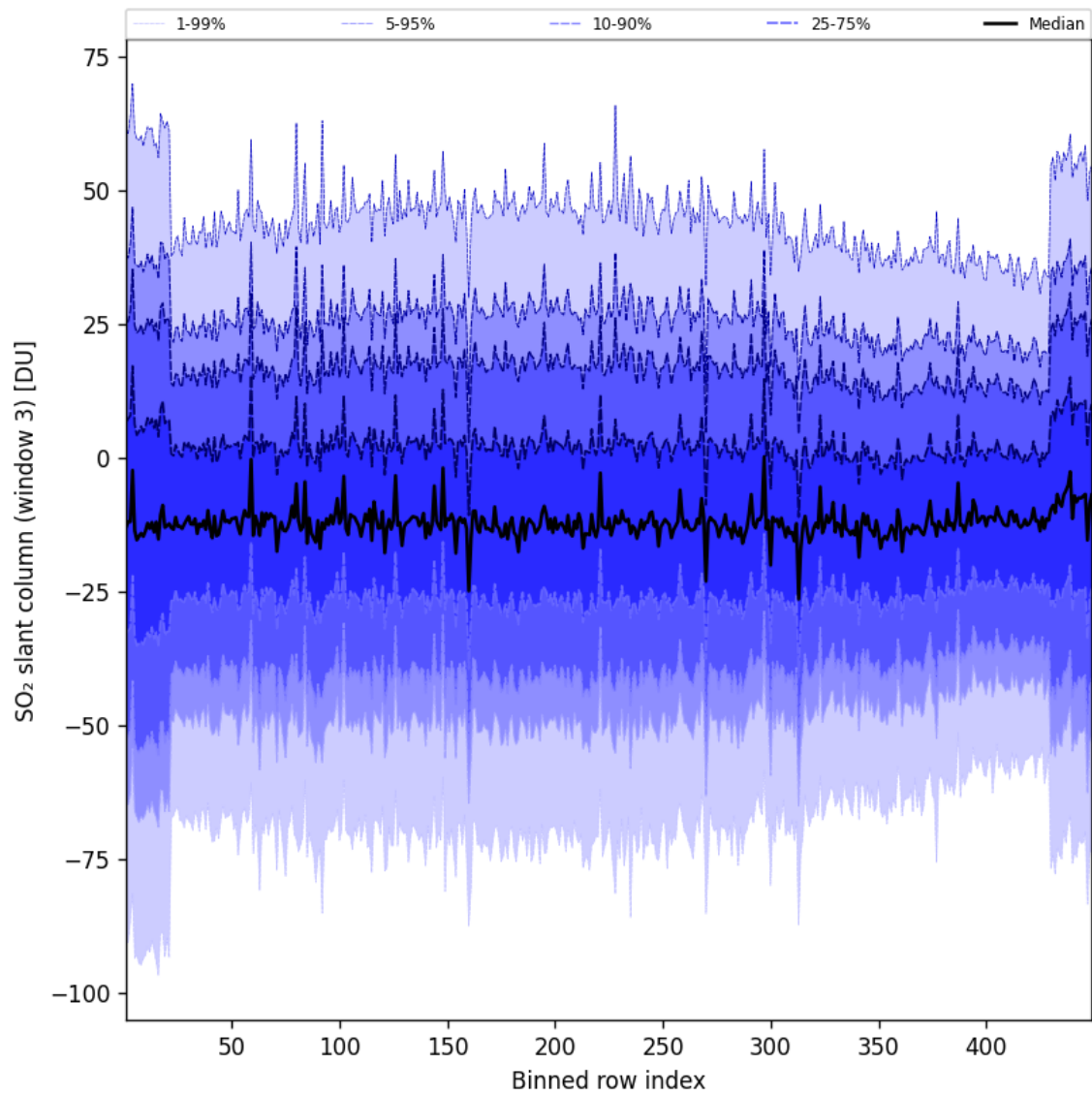
Figure 98: Along track statistics of “SO 2 slant column (window 3)” for 2025-05-20 to 2025-05-21
