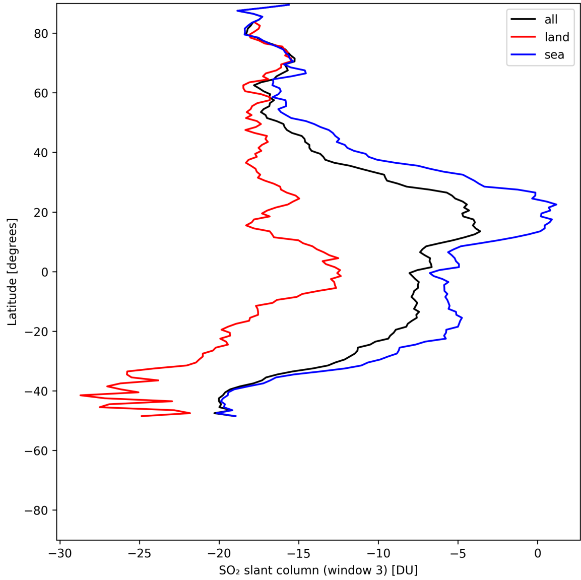
Figure 44: Zonal average of “SO 2 slant column (window 3)” for 2025-05-20 to 2025-05-21.
