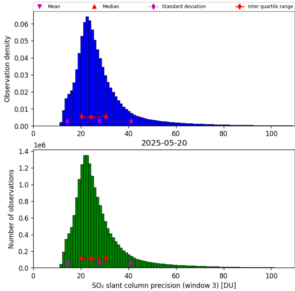
Figure 72: Histogram of “SO 2 slant column precision (window 3)” for 2025-05-20 to 2025-05-21
