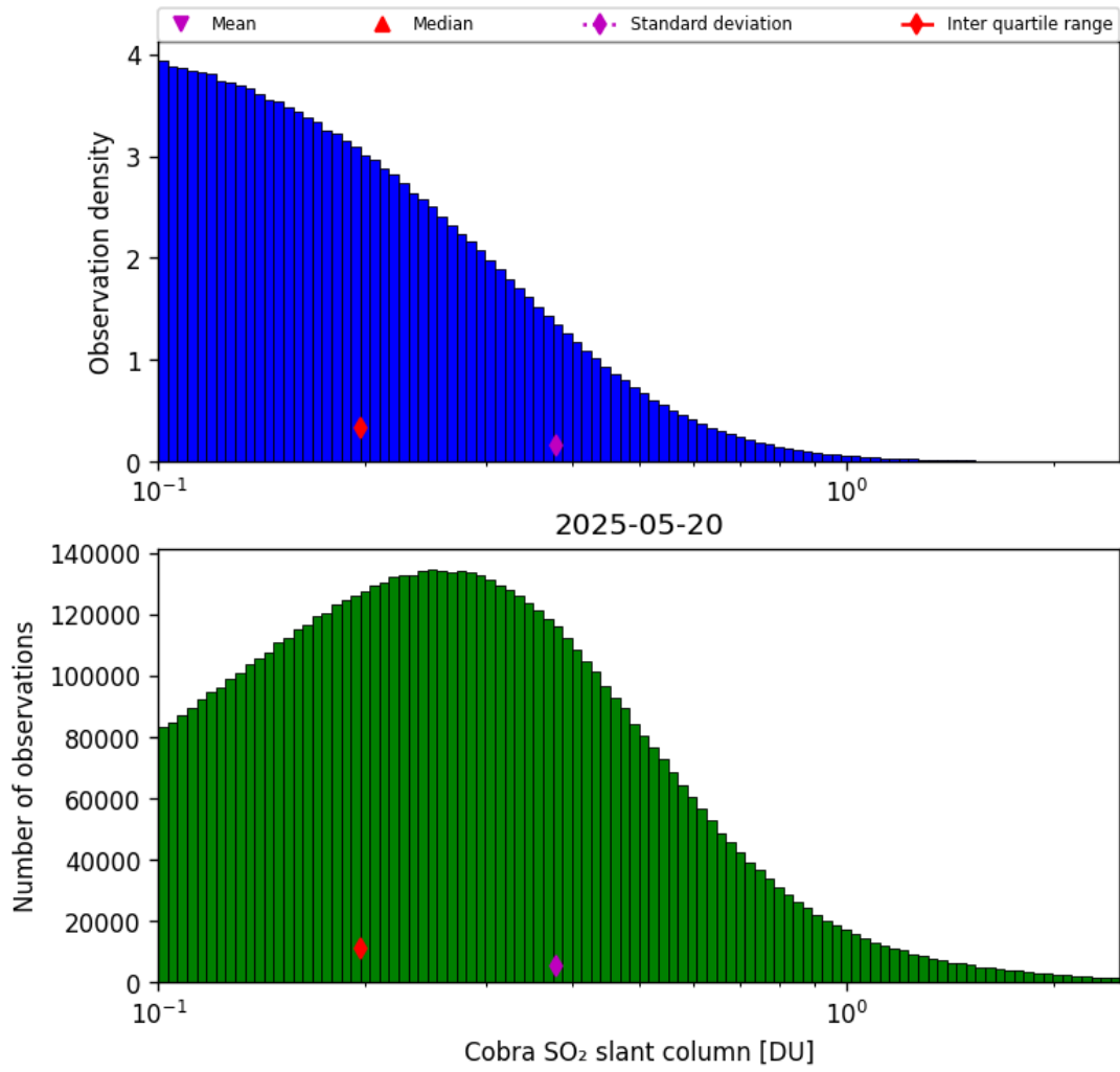
Figure 61: Histogram of “Cobra SO 2 slant column” for 2025-05-20 to 2025-05-21
