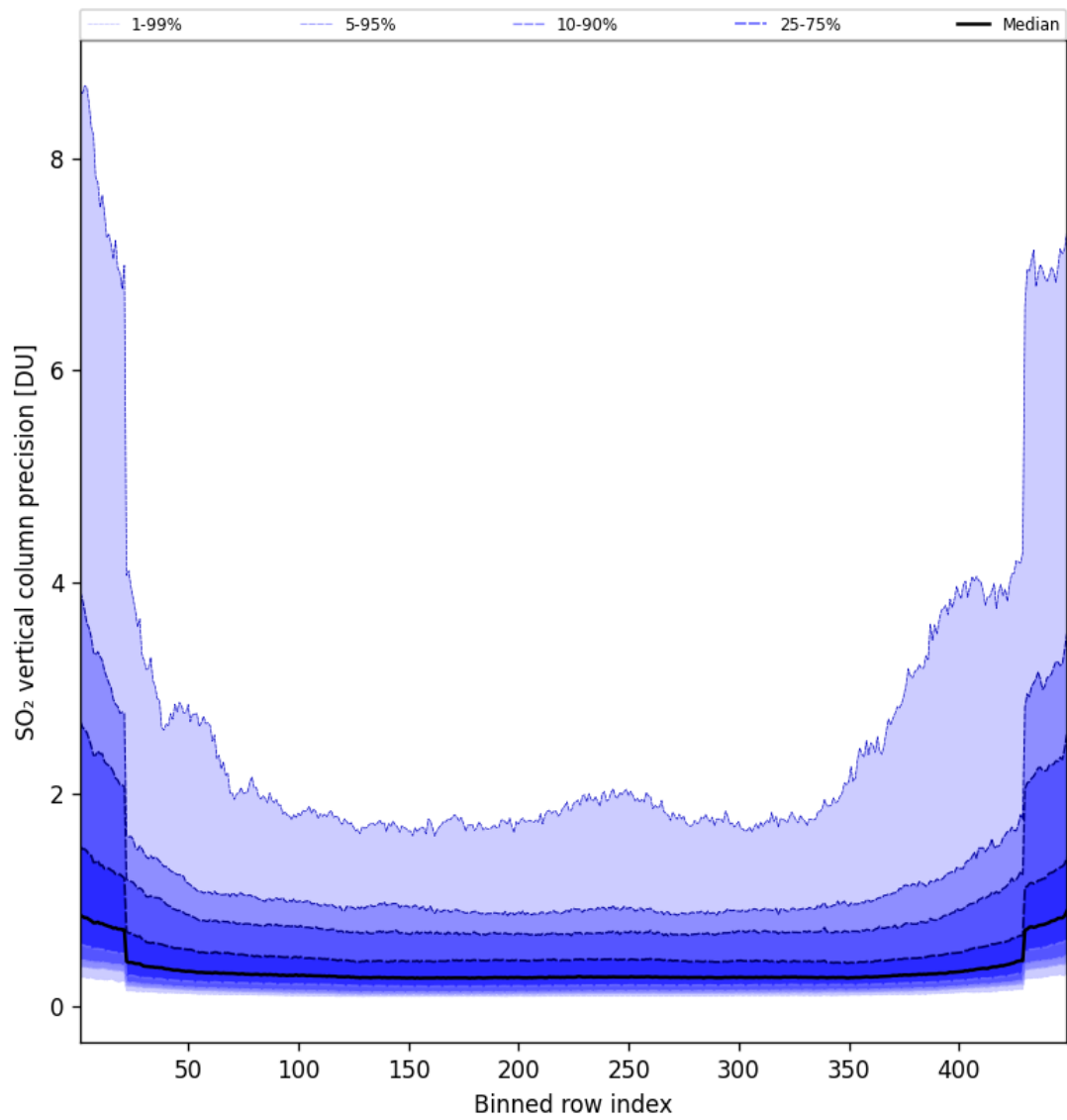
Figure 86: Along track statistics of “SO 2 vertical column precision” for 2025-05-20 to 2025-05-21
