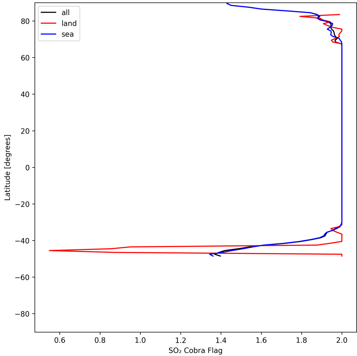
Figure 48: Zonal average of "SO 2 Cobra Flag" for 2025-05-20 to 2025-05-21.
