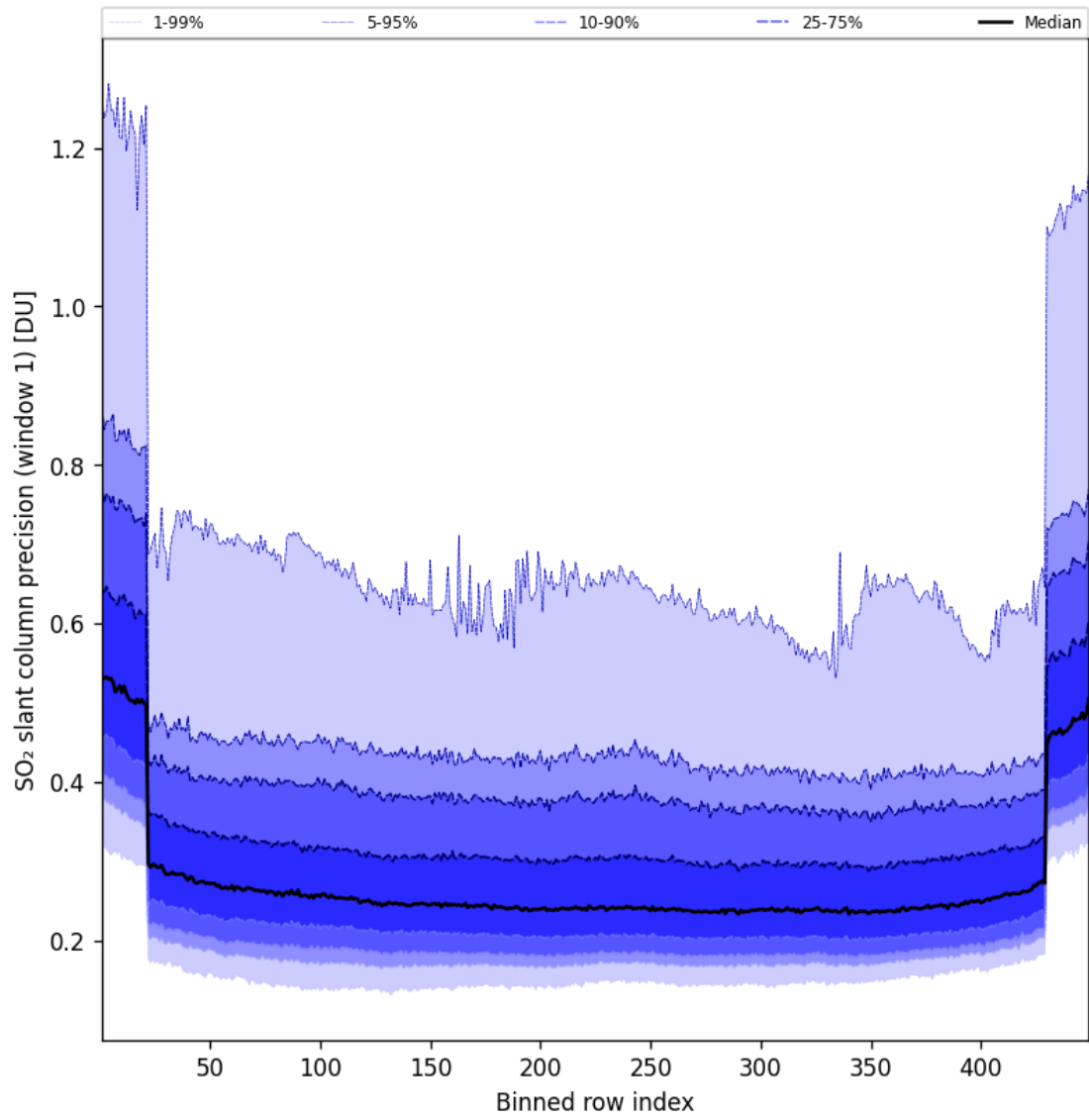
Figure 91: Along track statistics of “SO 2 slant column precision (window 1)” for 2025-05-20 to 2025-05-21
