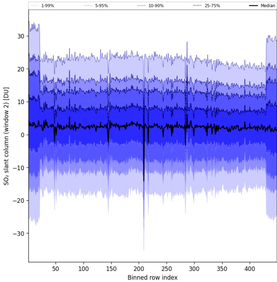
Figure 94: Along track statistics of “SO 2 slant column (window 2)” for 2025-05-20 to 2025-05-21
