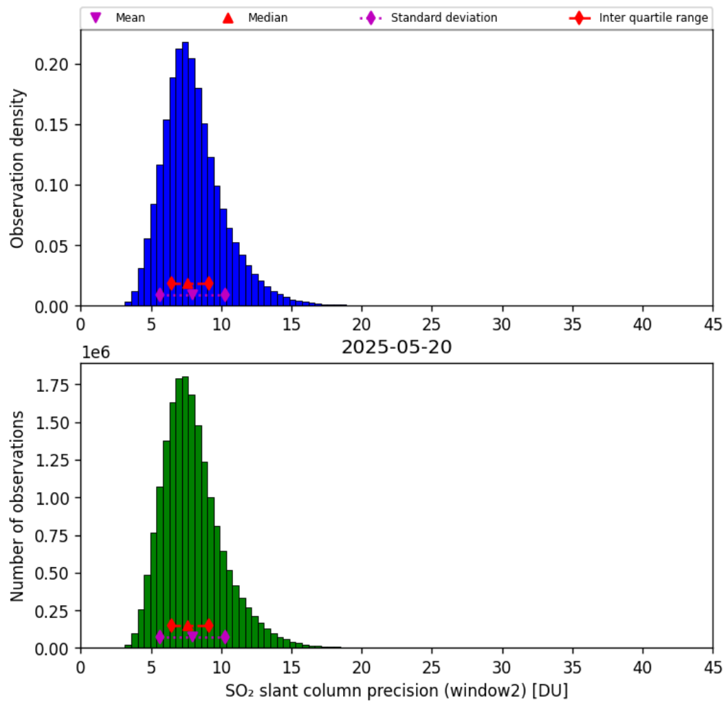
Figure 68: Histogram of “SO 2 slant column precision (window2)” for 2025-05-20 to 2025-05-21
