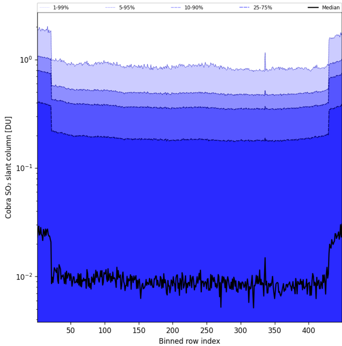
Figure 88: Along track statistics of “Cobra SO 2 slant column” for 2025-05-20 to 2025-05-21
