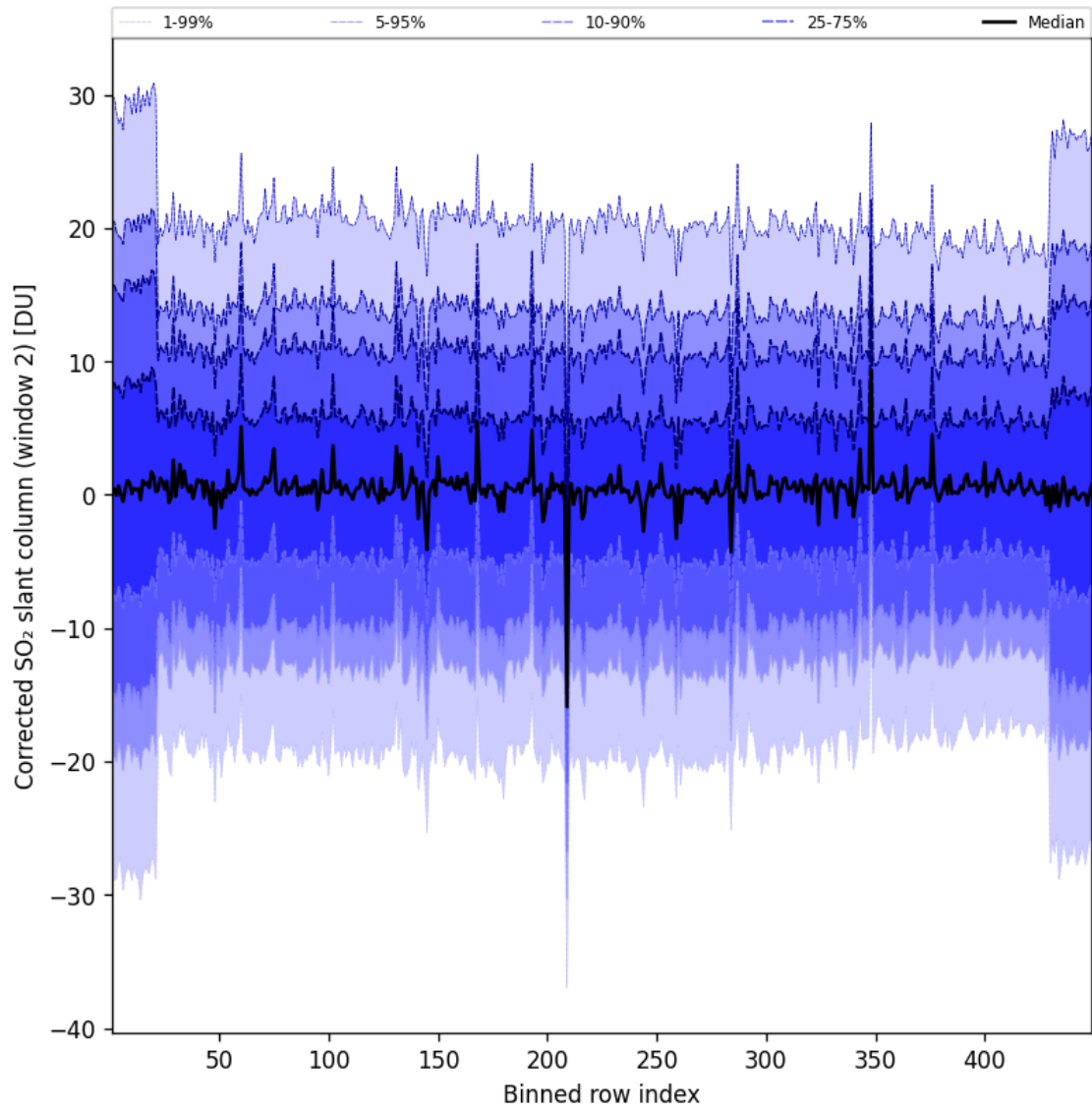
Figure 96: Along track statistics of “Corrected SO 2 slant column (window 2)” for 2025-05-20 to 2025-05-21
