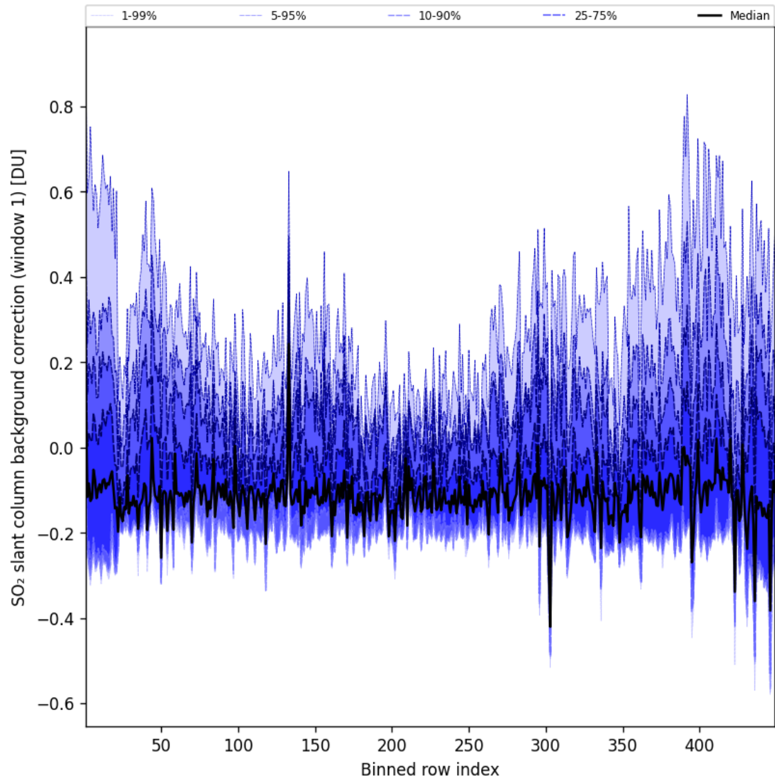
Figure 93: Along track statistics of “SO 2 slant column background correction (window 1)” for 2025-05-20 to 2025-05-21
