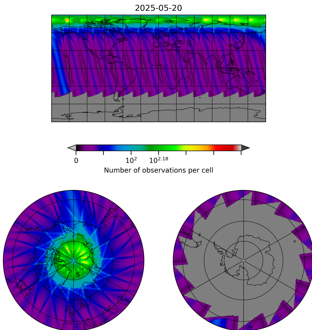
Figure 29: Map of the number of observations for 2025-05-20 to 2025-05-21
