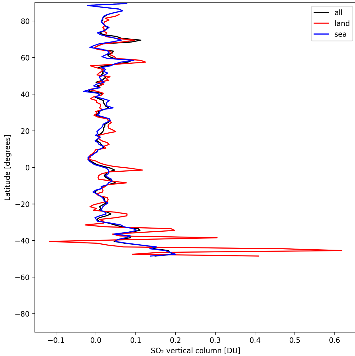
Figure 31: Zonal average of “SO 2 vertical column” for 2025-05-20 to 2025-05-21.
