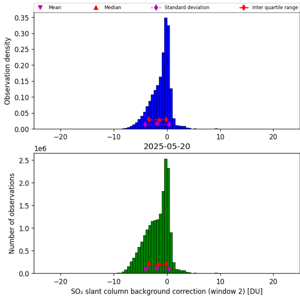
Figure 70: Histogram of “SO 2 slant column background correction (window 2)” for 2025-05-20 to 2025-05-21
