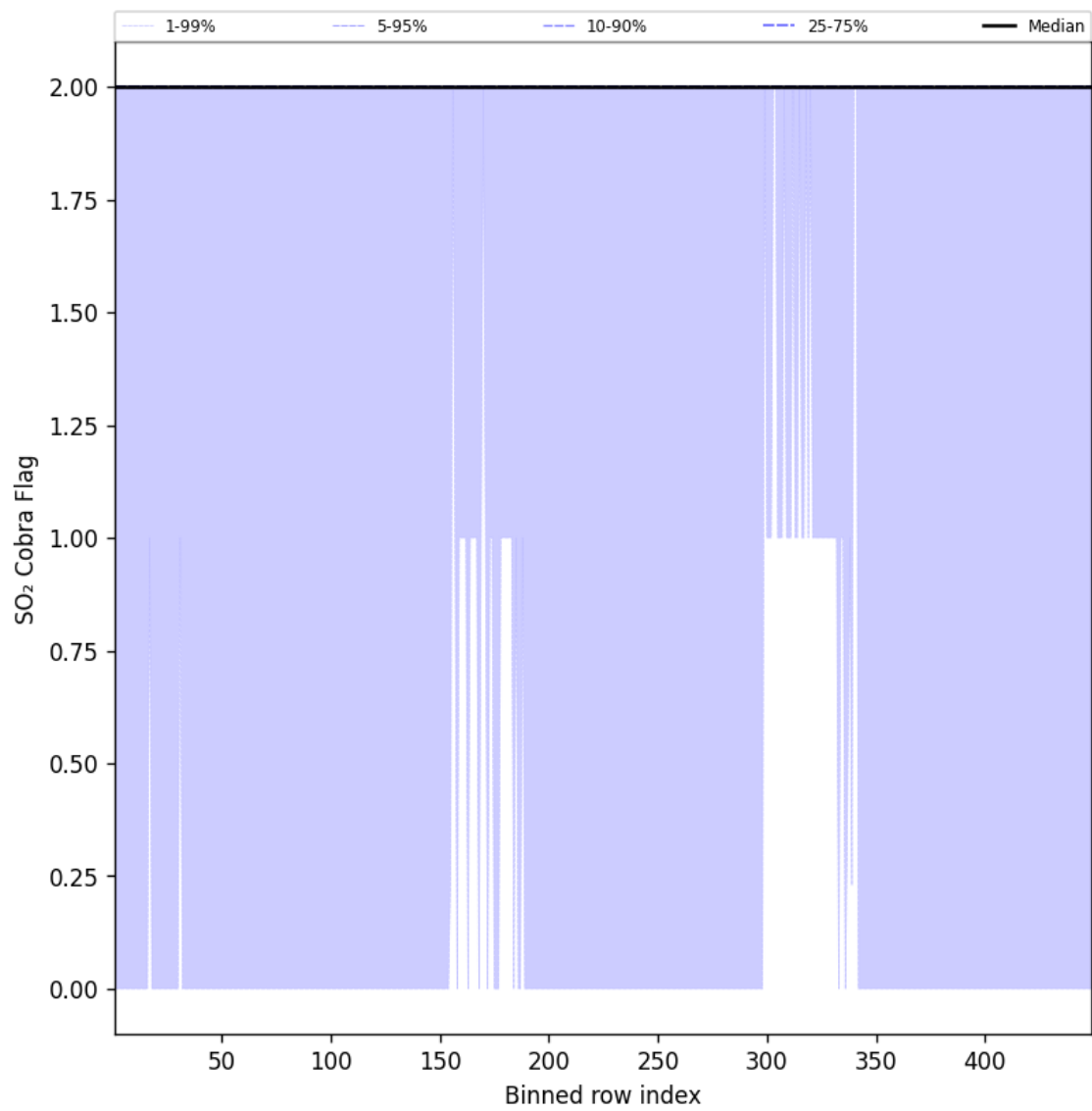
Figure 102: Along track statistics of “SO 2 Cobra Flag” for 2025-05-20 to 2025-05-21
