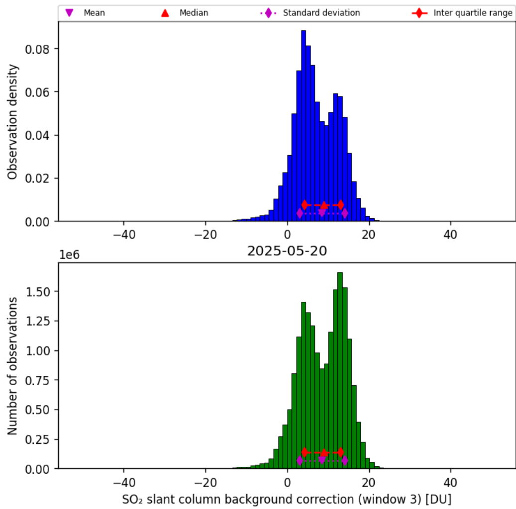
Figure 74: Histogram of “SO 2 slant column background correction (window 3)” for 2025-05-20 to 2025-05-21
