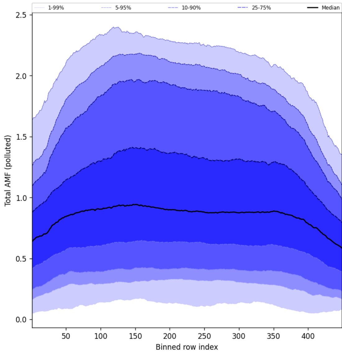
Figure 107: Along track statistics of “Total AMF (polluted)” for 2025-05-20 to 2025-05-21
