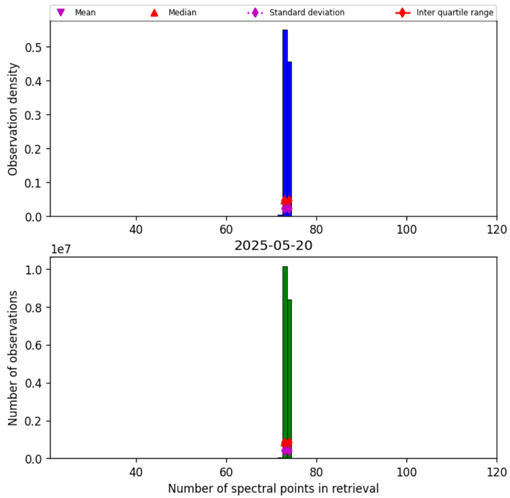
Figure 83: Histogram of "Number of spectral points in retrieval" for 2025-05-20 to 2025-05-21
