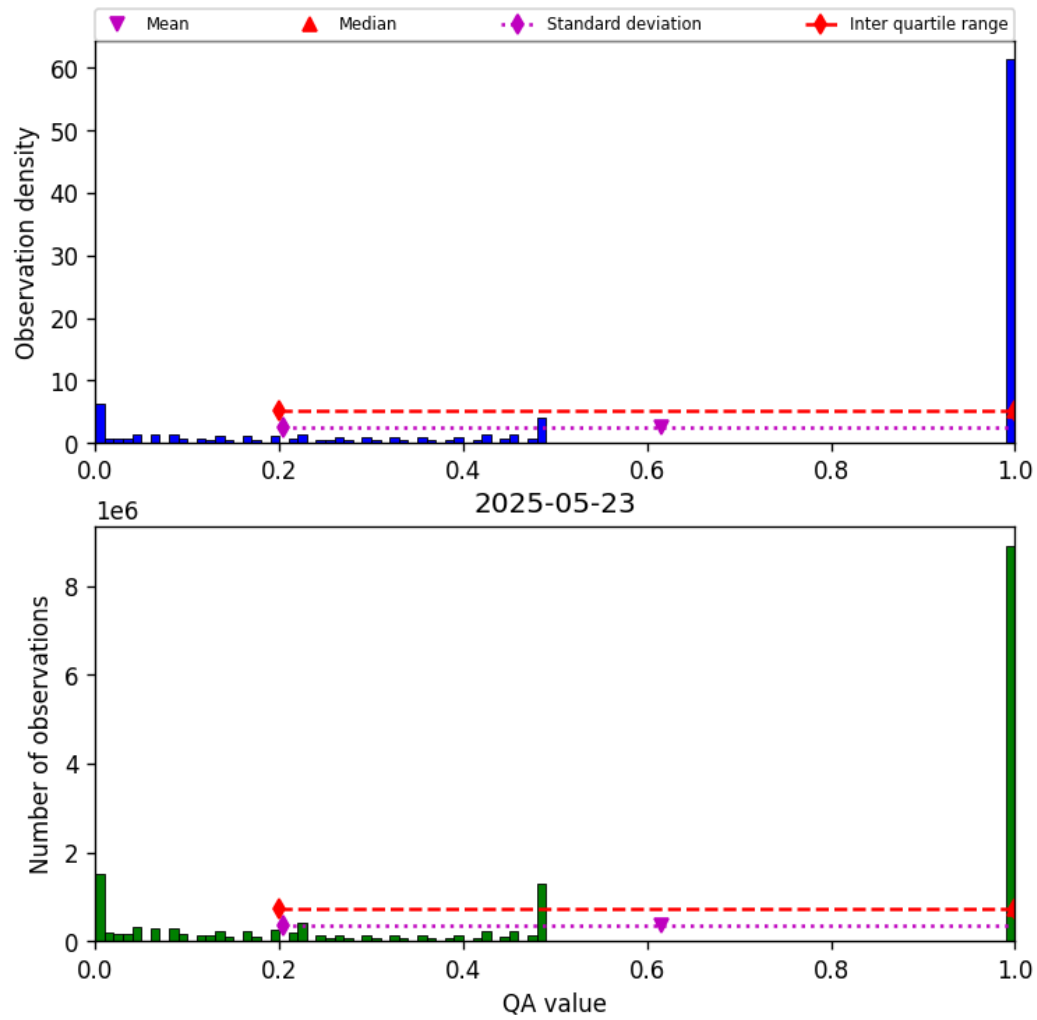
Figure 57: Histogram of “QA value” for 2025-05-23 to 2025-05-24
