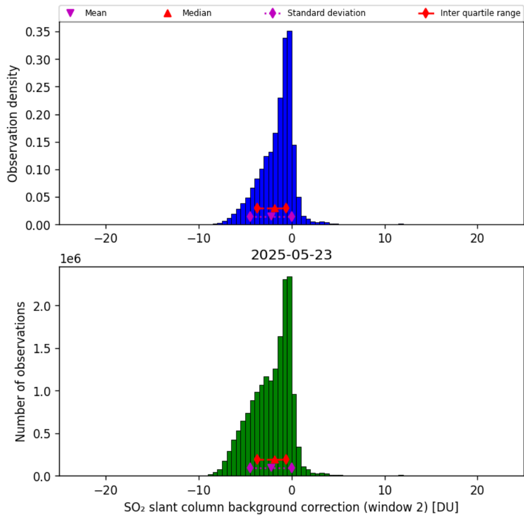
Figure 70: Histogram of “SO 2 slant column background correction (window 2)” for 2025-05-23 to 2025-05-24
