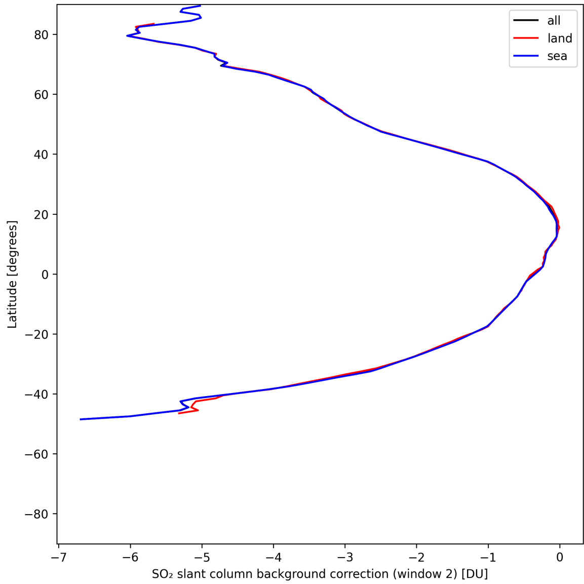
Figure 43: Zonal average of “SO 2 slant column background correction (window 2)” for 2025-05-23 to 2025-05-24.
