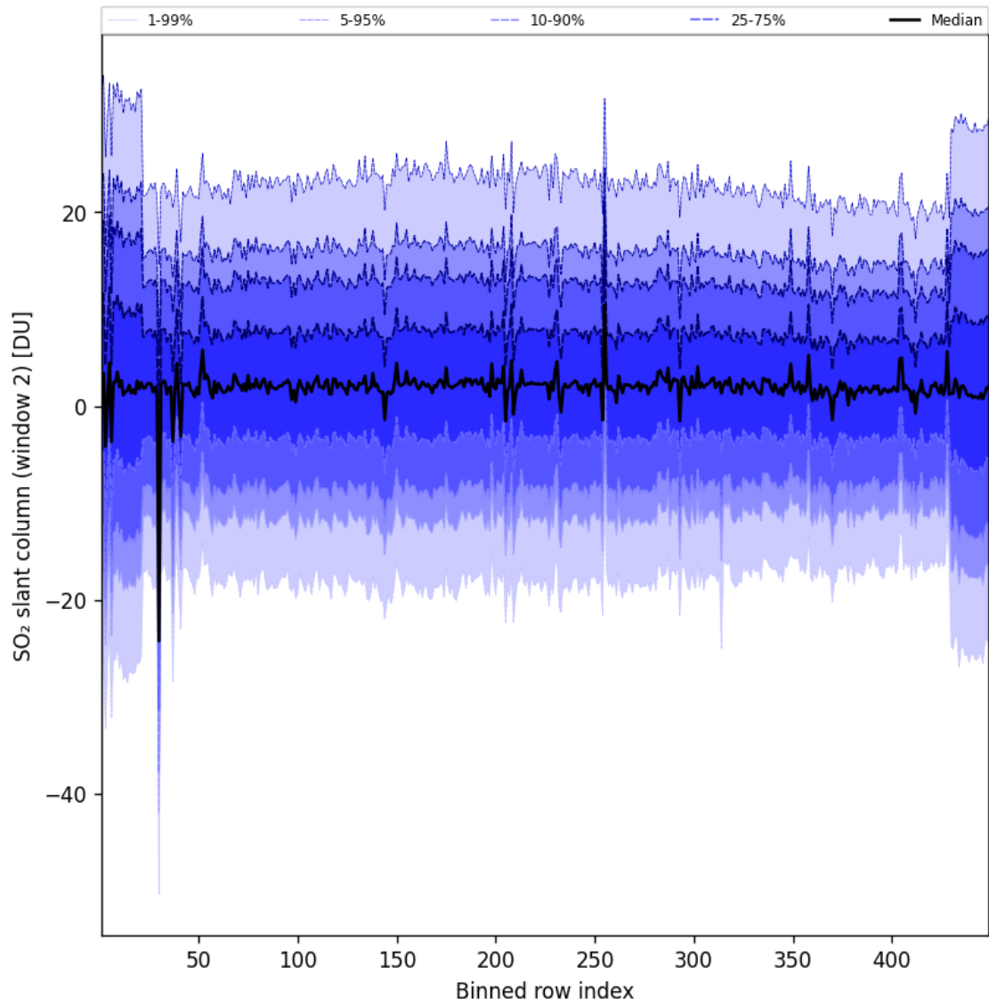
Figure 94: Along track statistics of “SO 2 slant column (window 2)” for 2025-05-23 to 2025-05-24
