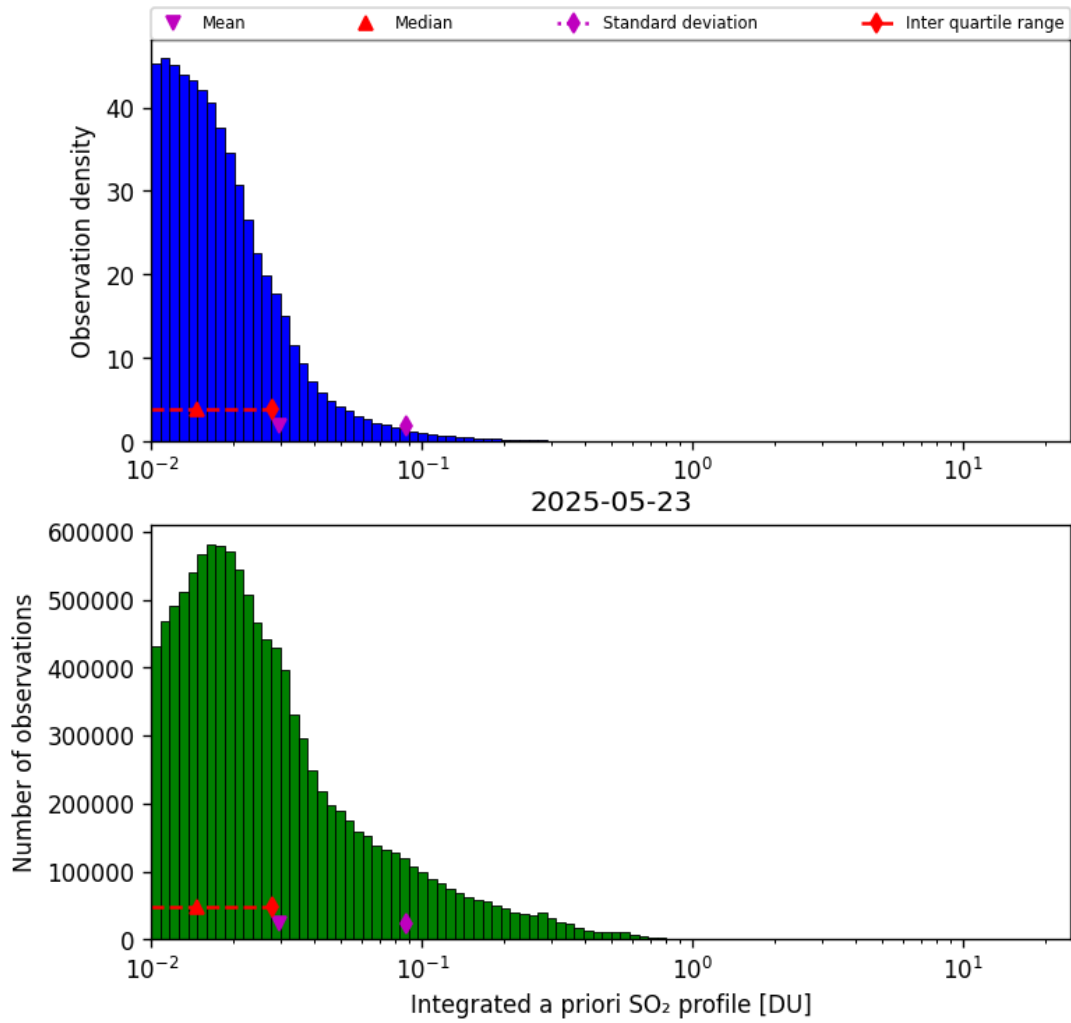
Figure 76: Histogram of “Integrated a priori SO 2 profile” for 2025-05-23 to 2025-05-24
