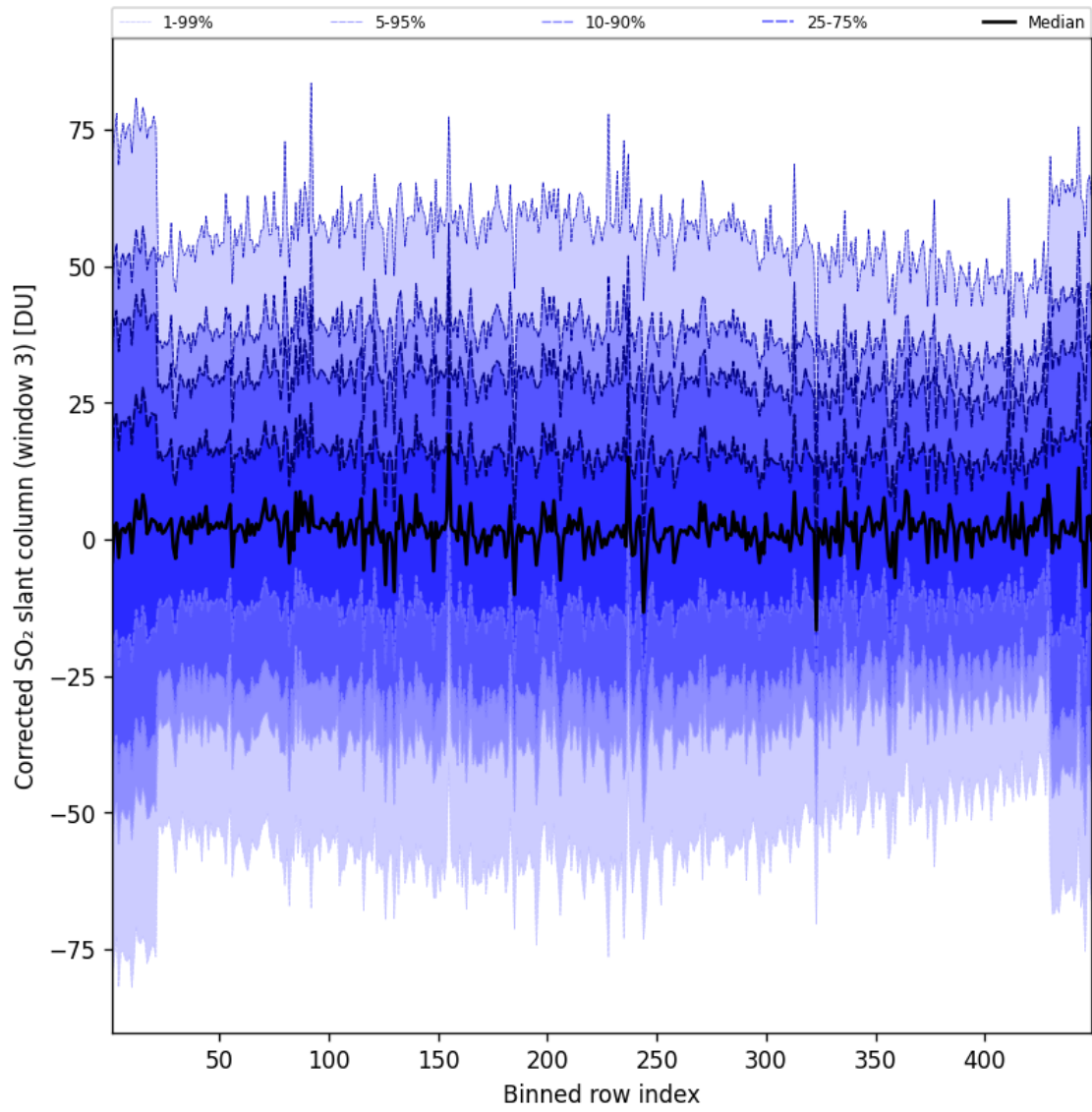
Figure 100: Along track statistics of “Corrected SO 2 slant column (window 3)” for 2025-05-23 to 2025-05-24
