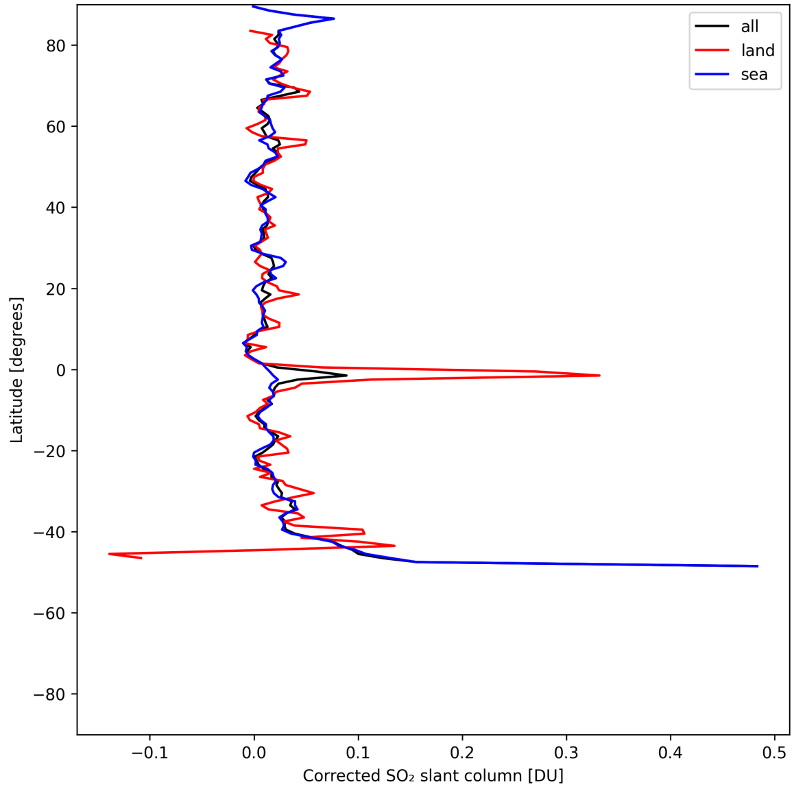
Figure 33: Zonal average of “Corrected SO 2 slant column” for 2025-05-23 to 2025-05-24.
