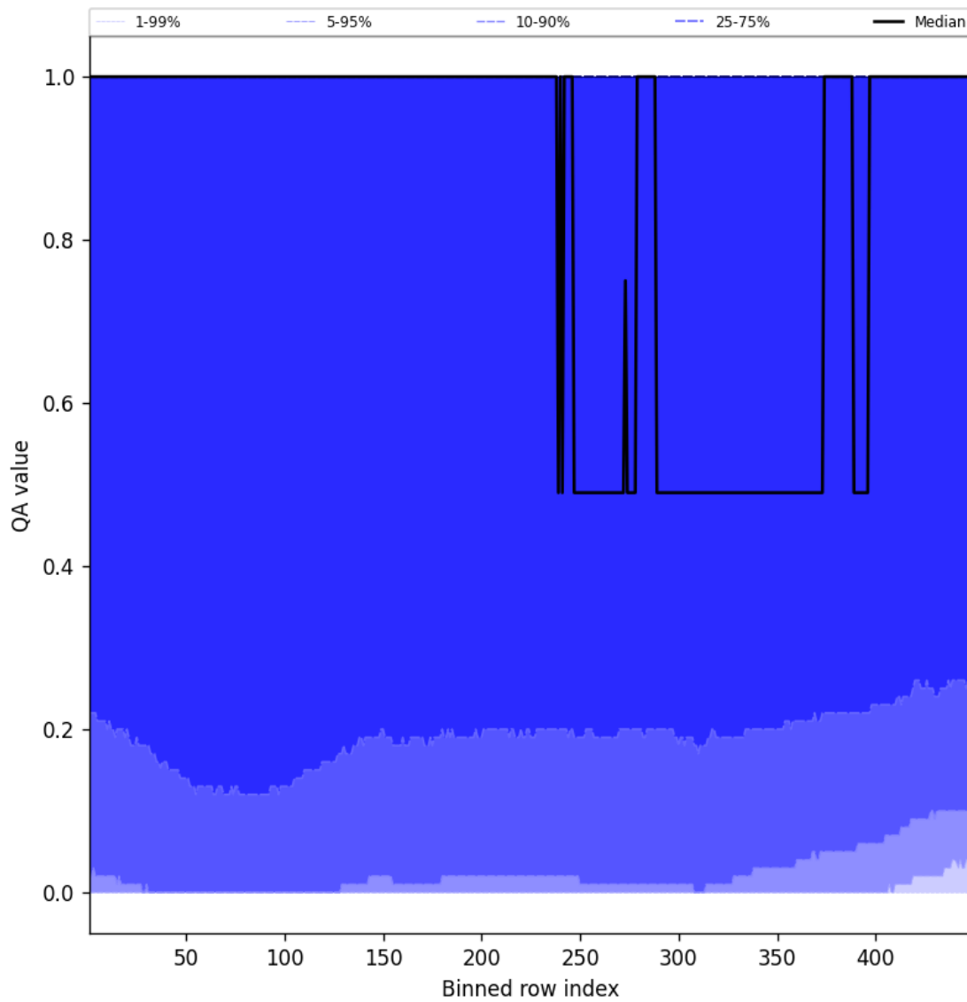
Figure 84: Along track statistics of “QA value” for 2025-05-23 to 2025-05-24
