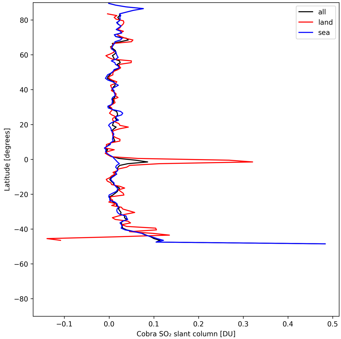
Figure 34: Zonal average of “Cobra SO 2 slant column” for 2025-05-23 to 2025-05-24.
