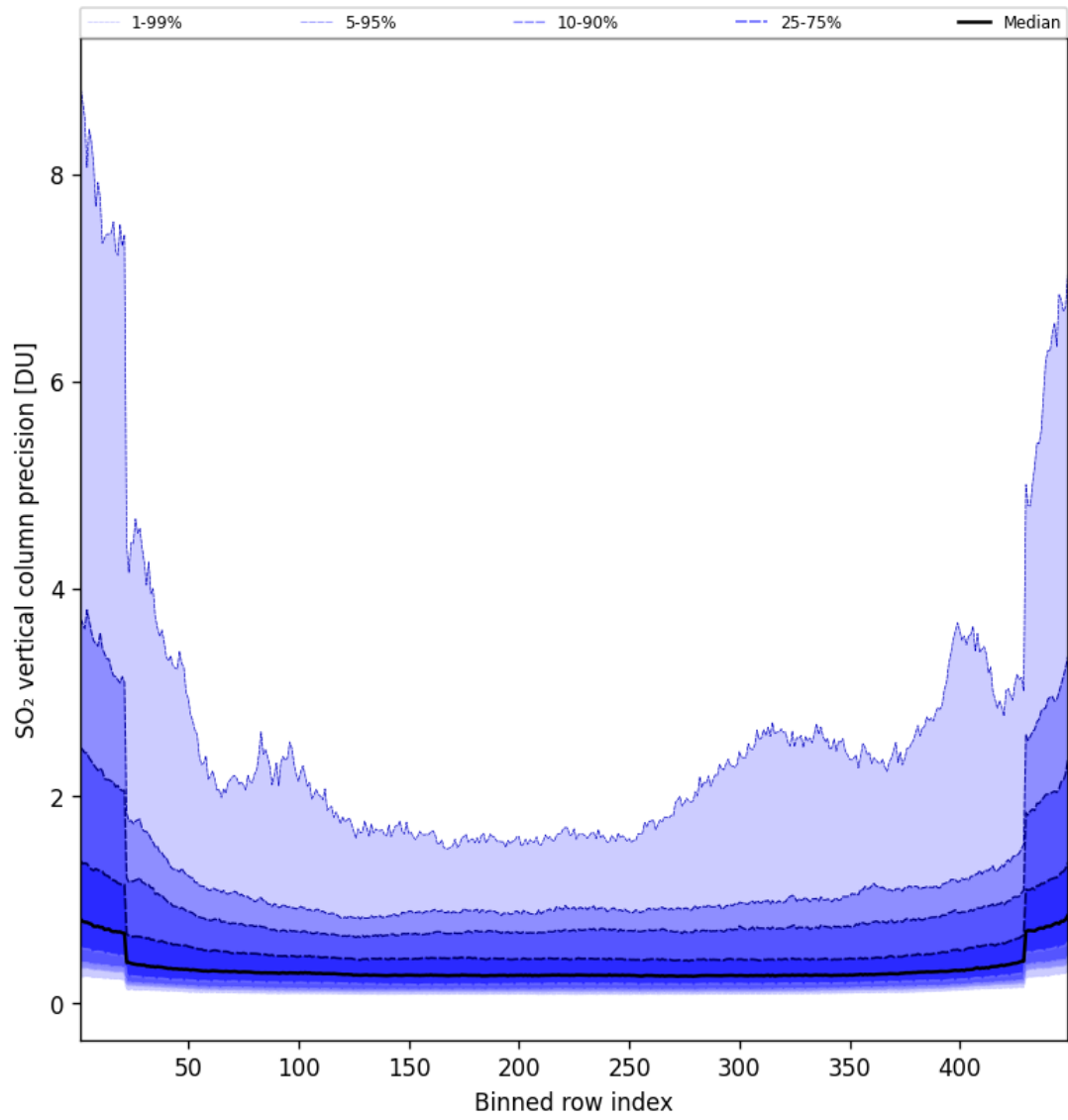
Figure 86: Along track statistics of “SO 2 vertical column precision” for 2025-05-23 to 2025-05-24
