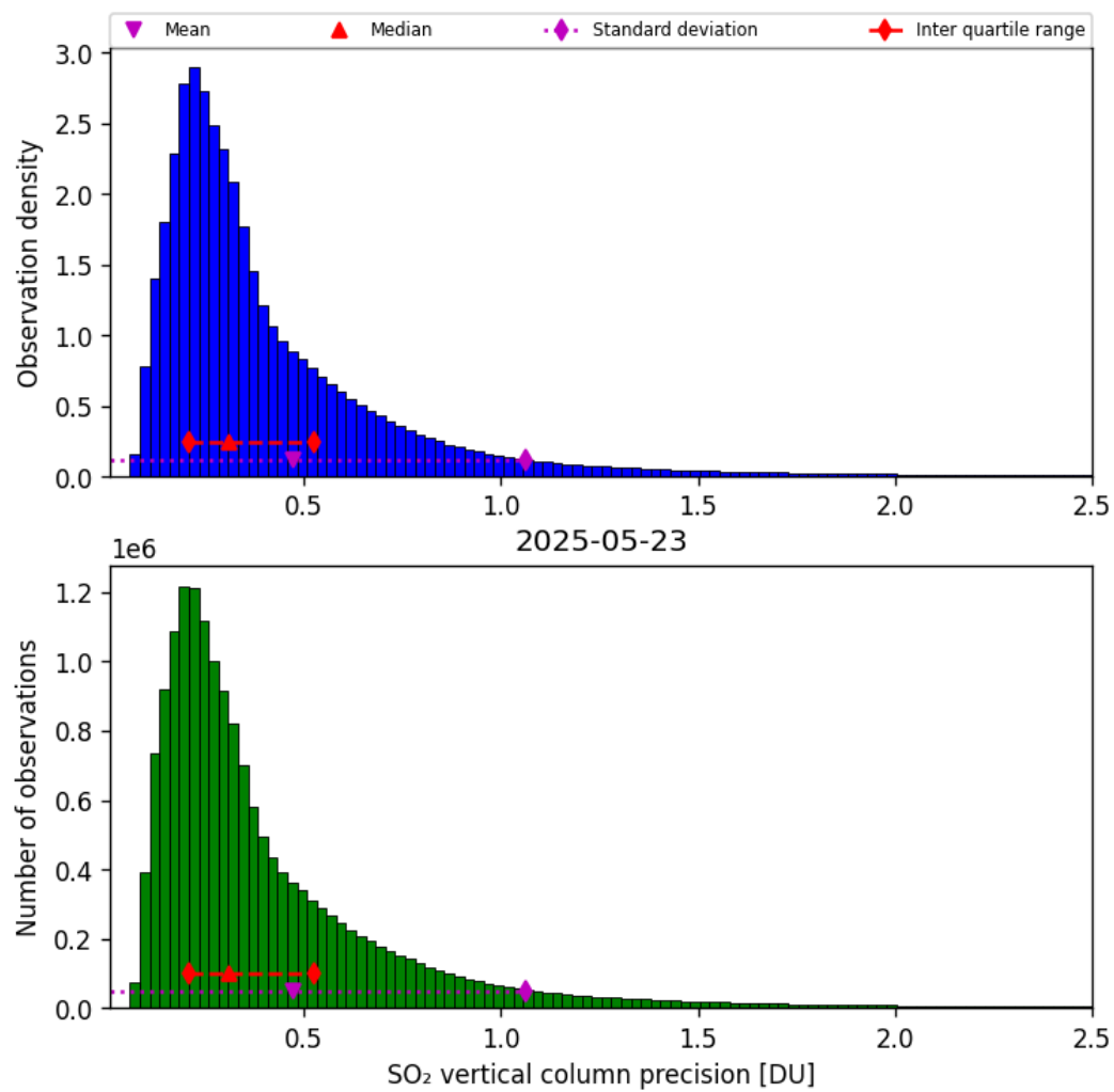
Figure 59: Histogram of “SO 2 vertical column precision” for 2025-05-23 to 2025-05-24
