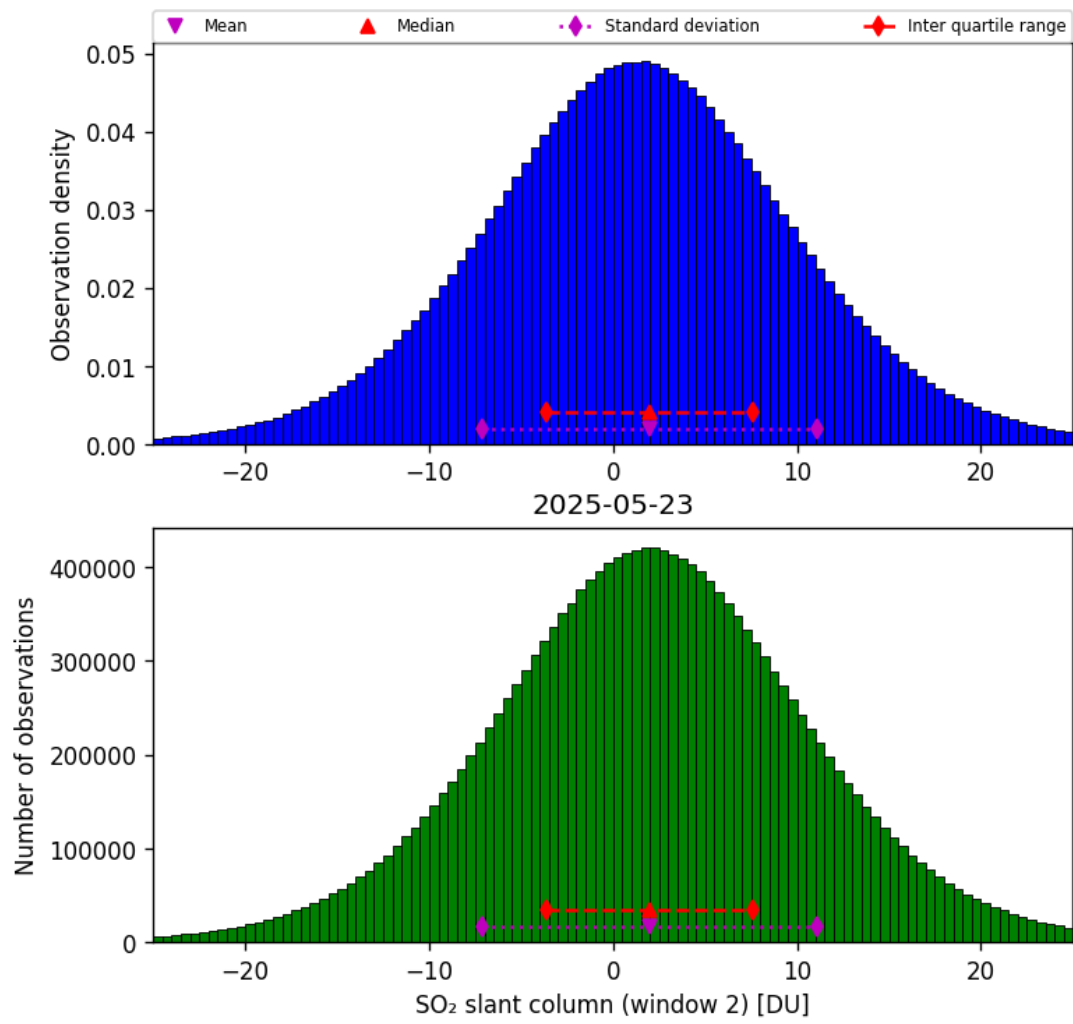
Figure 67: Histogram of “SO 2 slant column (window 2)” for 2025-05-23 to 2025-05-24
