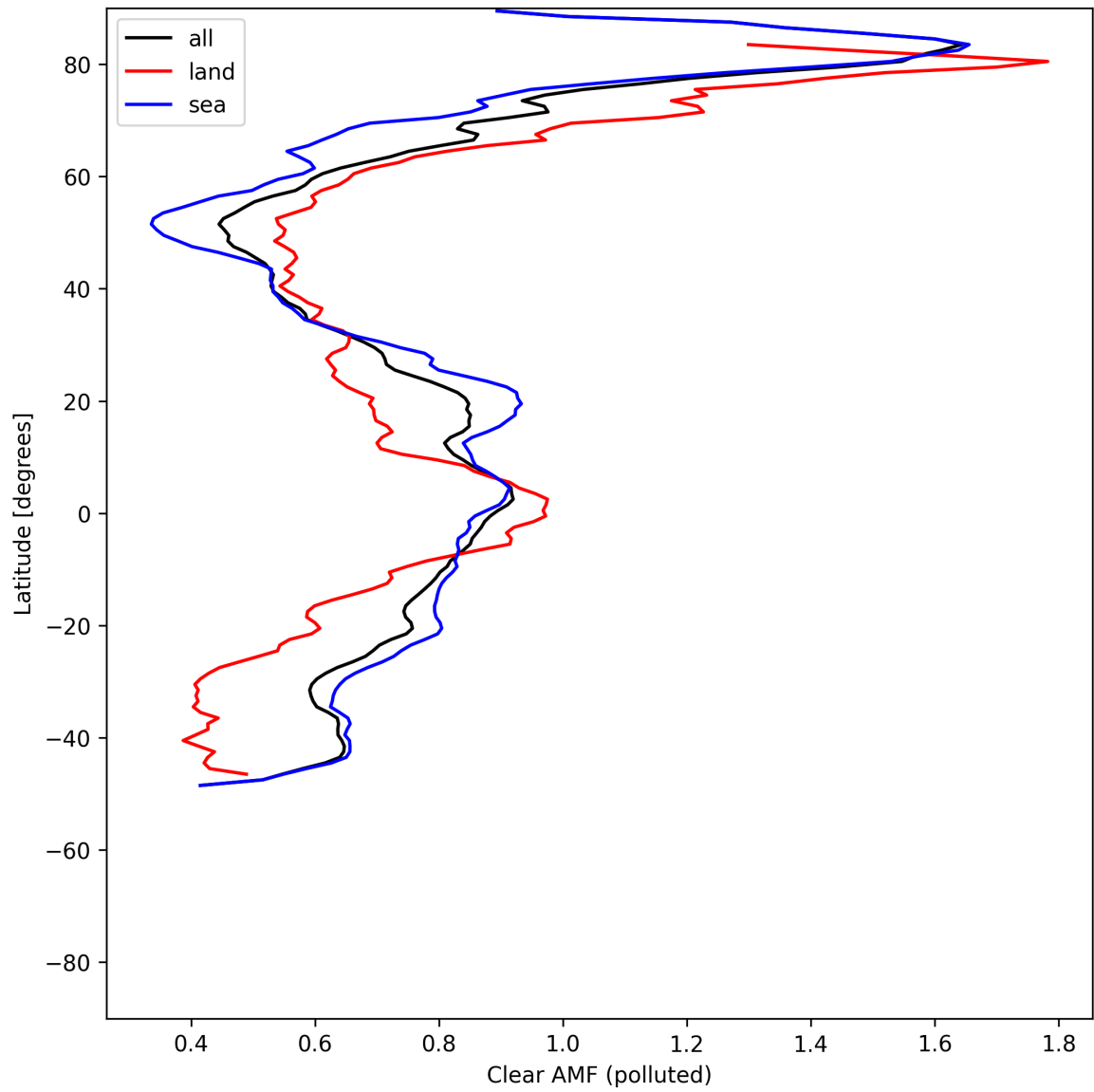
Figure 55: Zonal average of “Clear AMF (polluted)” for 2025-05-23 to 2025-05-24.
