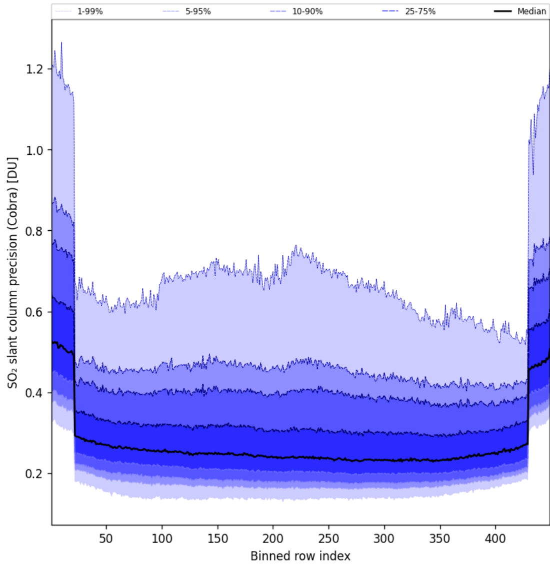
Figure 89: Along track statistics of “SO 2 slant column precision (Cobra)” for 2025-05-23 to 2025-05-24
