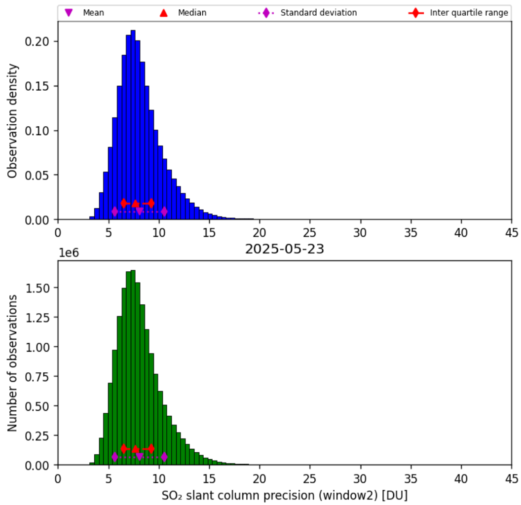
Figure 68: Histogram of “SO 2 slant column precision (window2)” for 2025-05-23 to 2025-05-24
