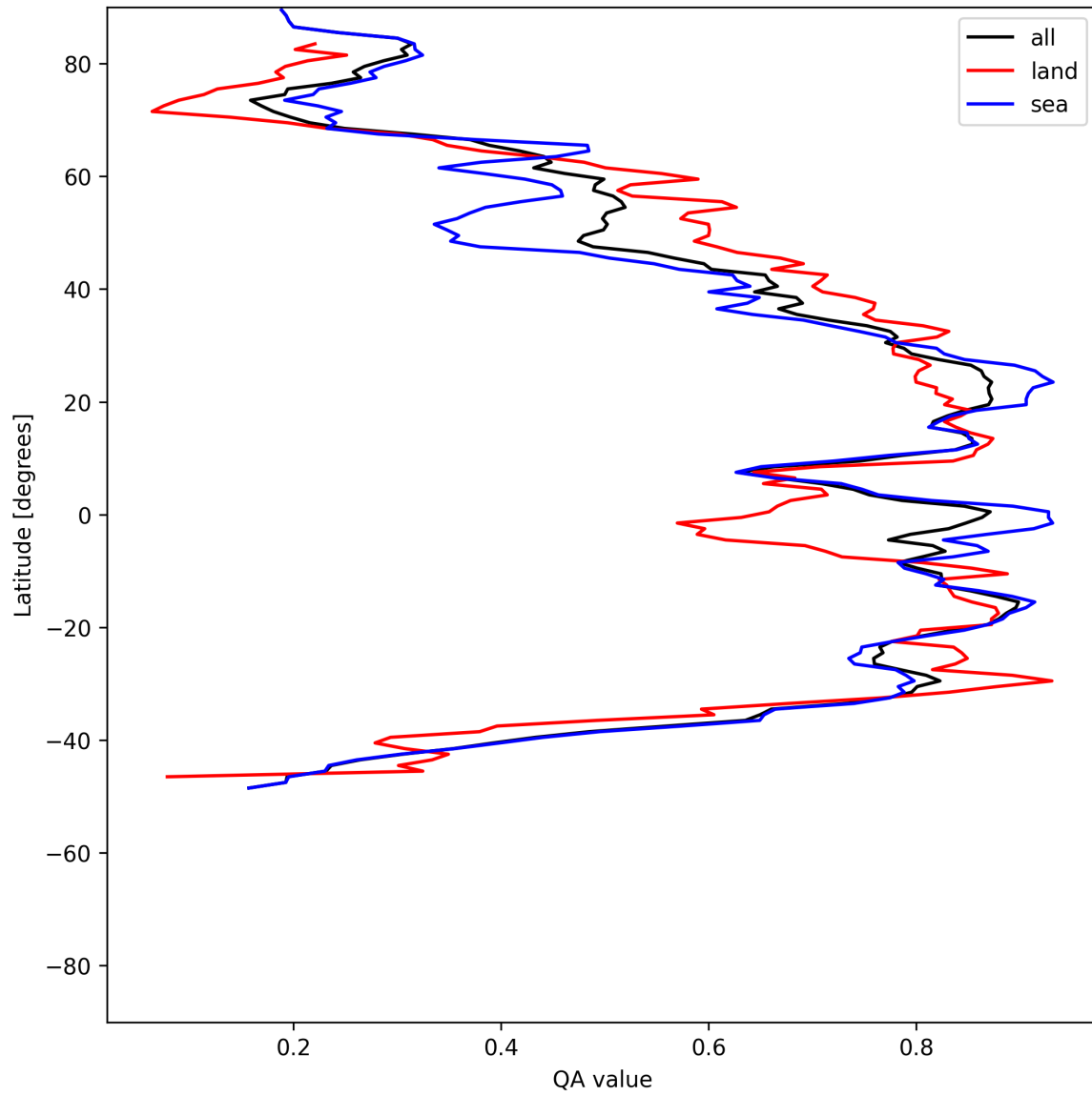
Figure 30: Zonal average of “QA value” for 2025-05-23 to 2025-05-24.
