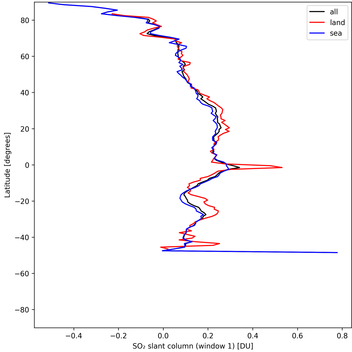
Figure 36: Zonal average of “SO 2 slant column (window 1)” for 2025-05-23 to 2025-05-24.
