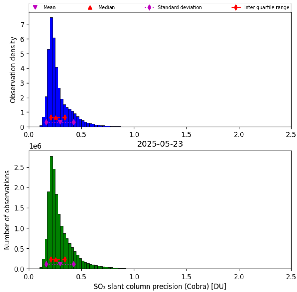
Figure 62: Histogram of “SO 2 slant column precision (Cobra)” for 2025-05-23 to 2025-05-24
