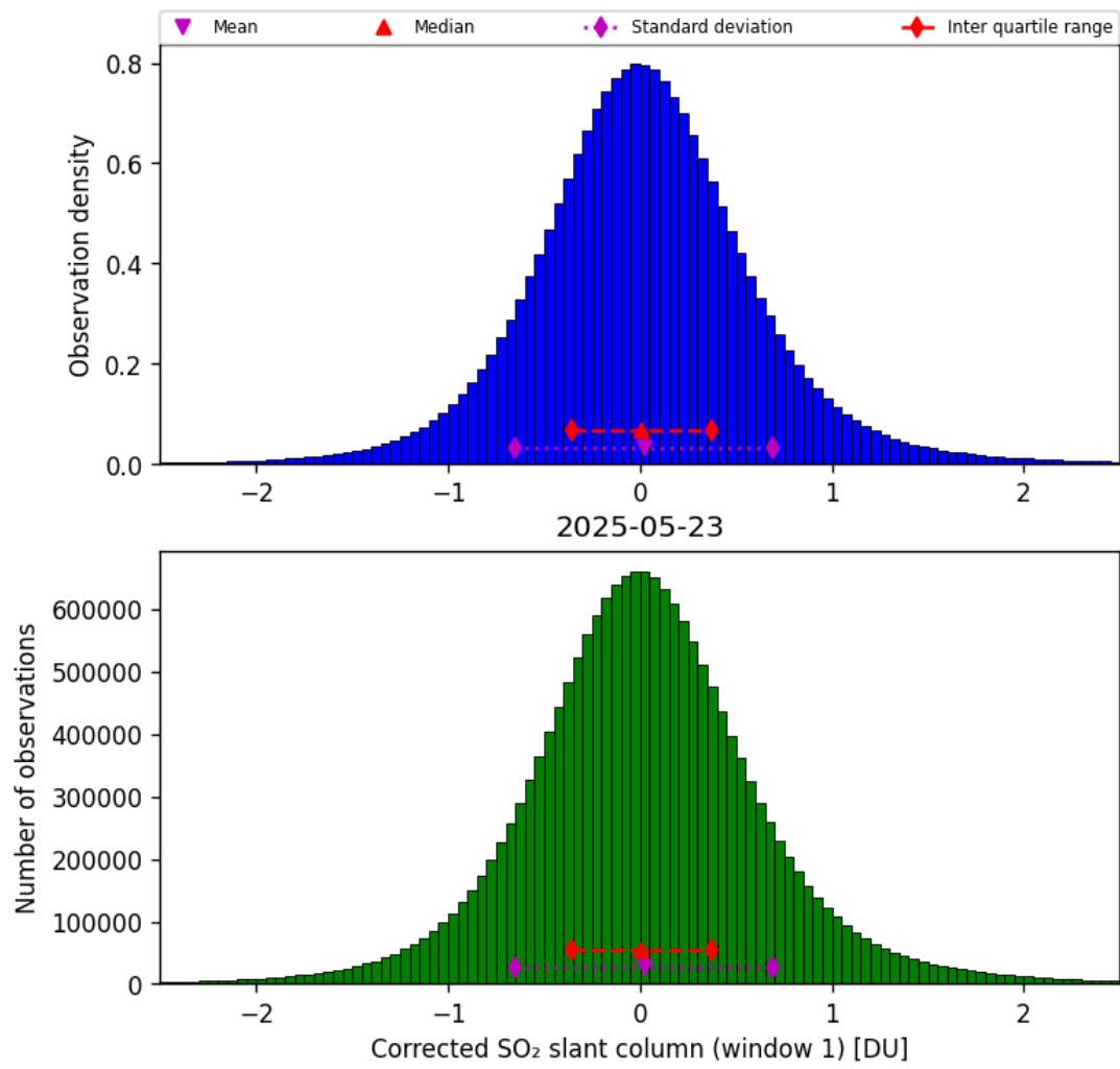
Figure 65: Histogram of “Corrected SO 2 slant column (window 1)” for 2025-05-23 to 2025-05-24
