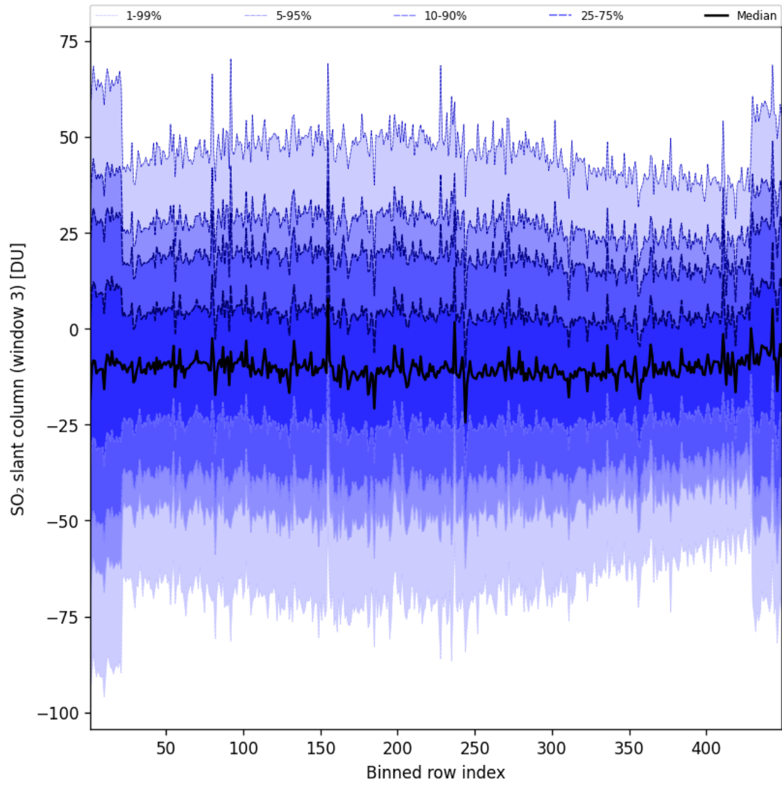
Figure 98: Along track statistics of “SO 2 slant column (window 3)” for 2025-05-23 to 2025-05-24
