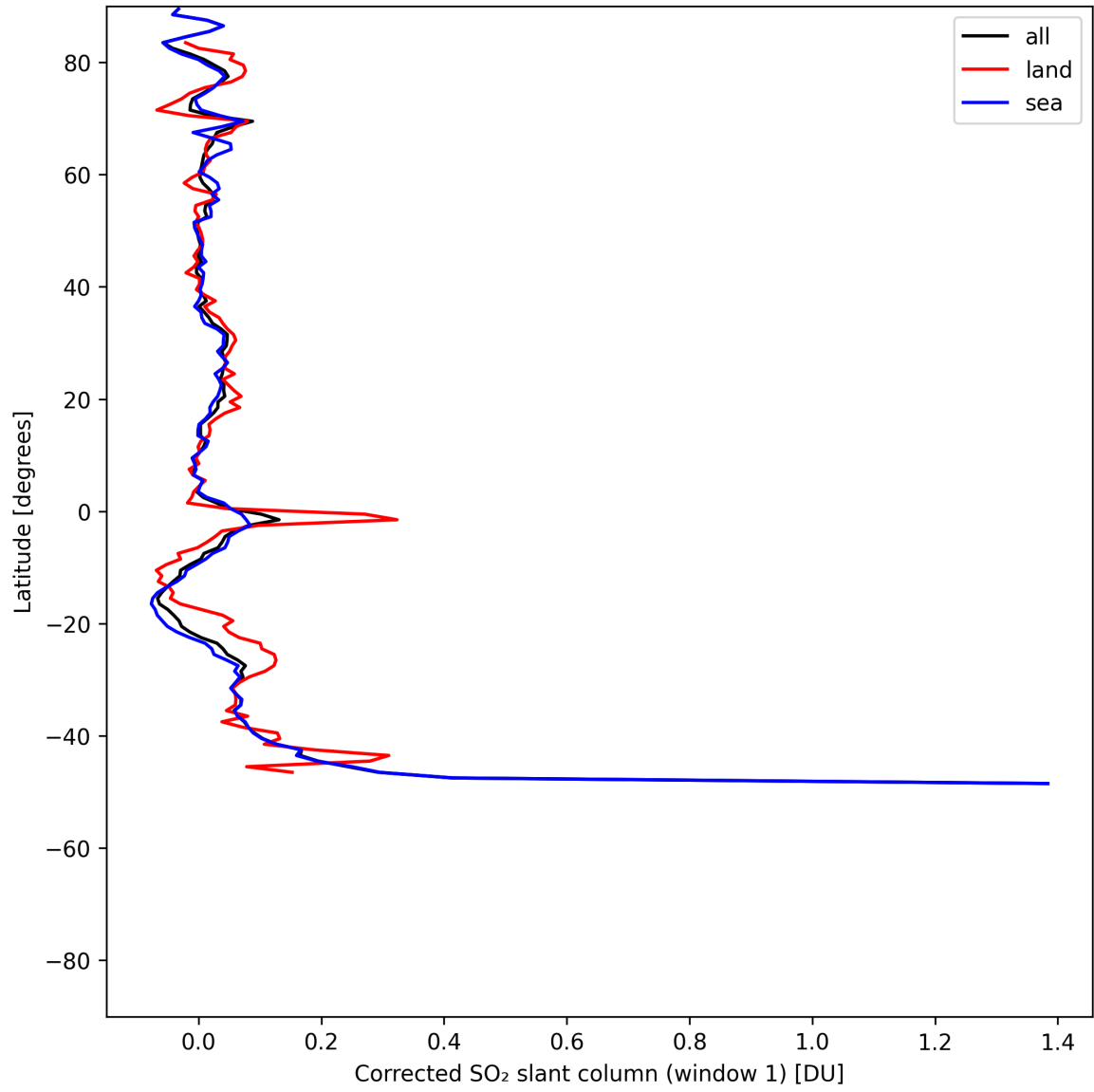
Figure 38: Zonal average of “Corrected SO 2 slant column (window 1)” for 2025-05-23 to 2025-05-24.
