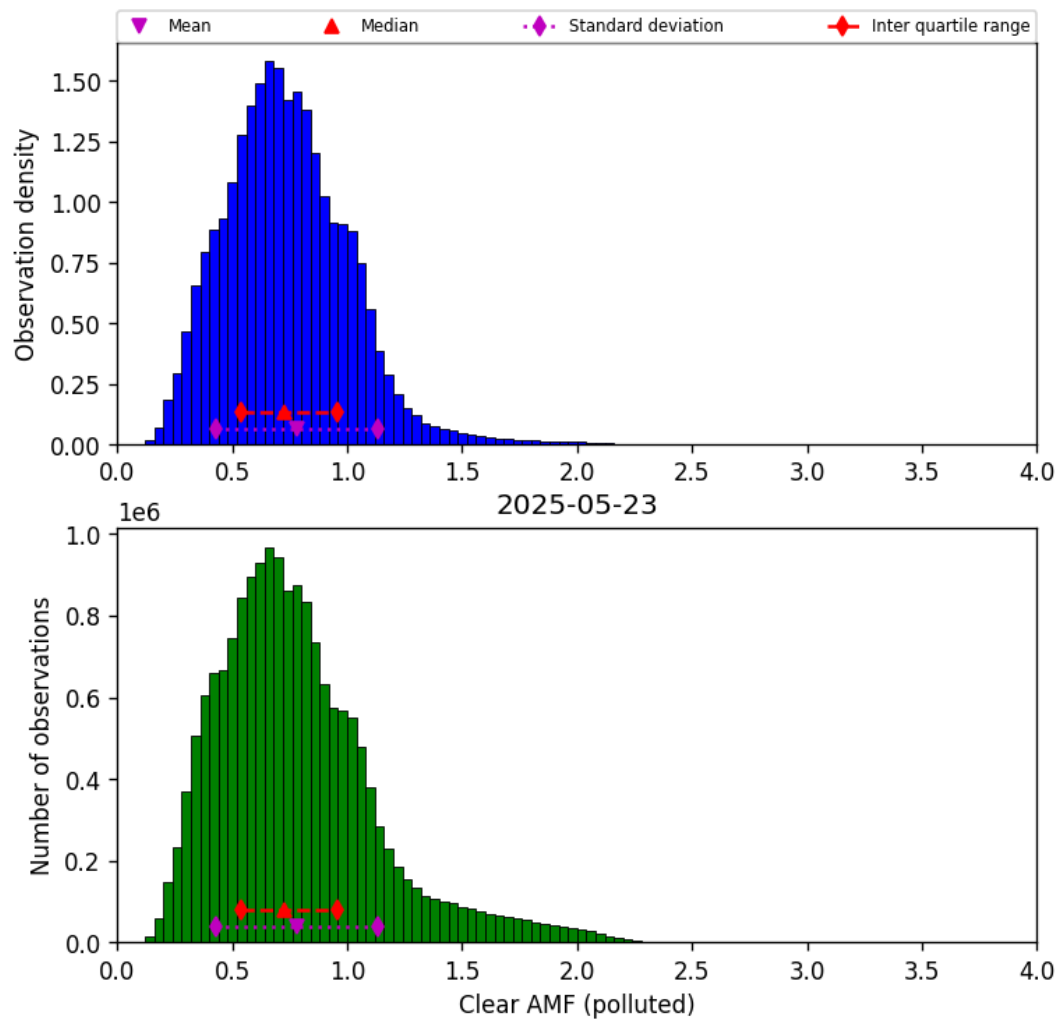
Figure 82: Histogram of “Clear AMF (polluted)” for 2025-05-23 to 2025-05-24
