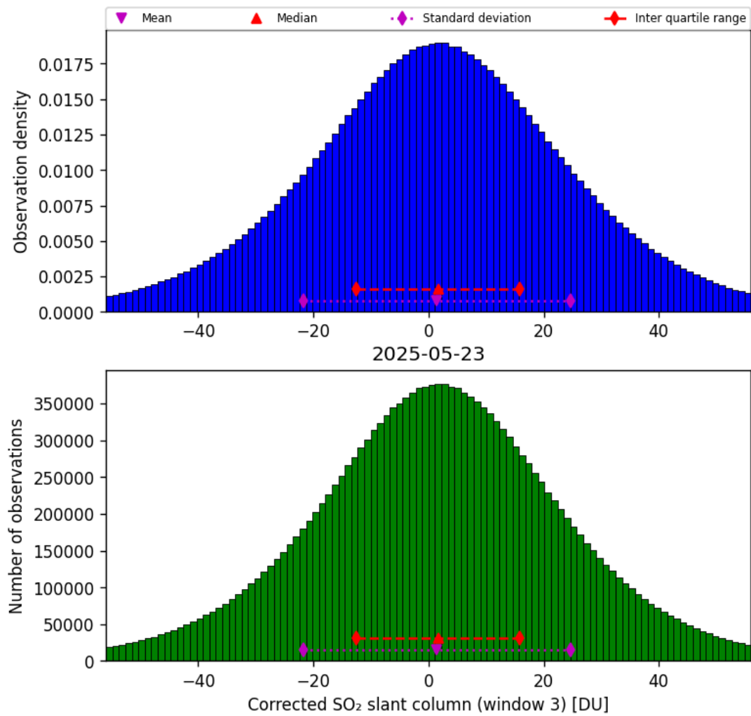
Figure 73: Histogram of “Corrected SO 2 slant column (window 3)” for 2025-05-23 to 2025-05-24
