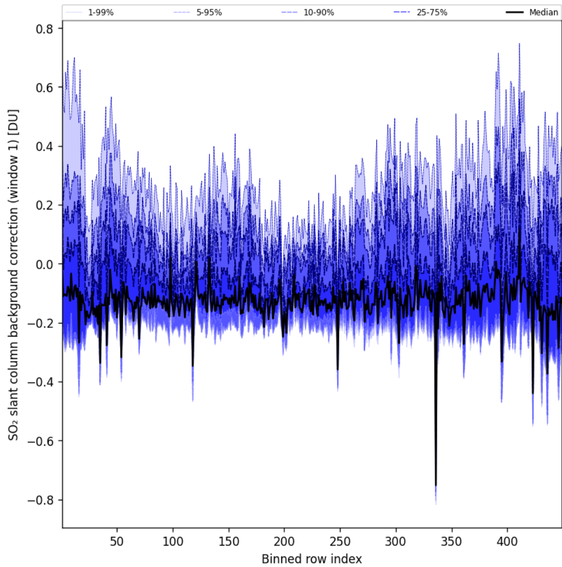
Figure 93: Along track statistics of “SO 2 slant column background correction (window 1)” for 2025-05-23 to 2025-05-24
