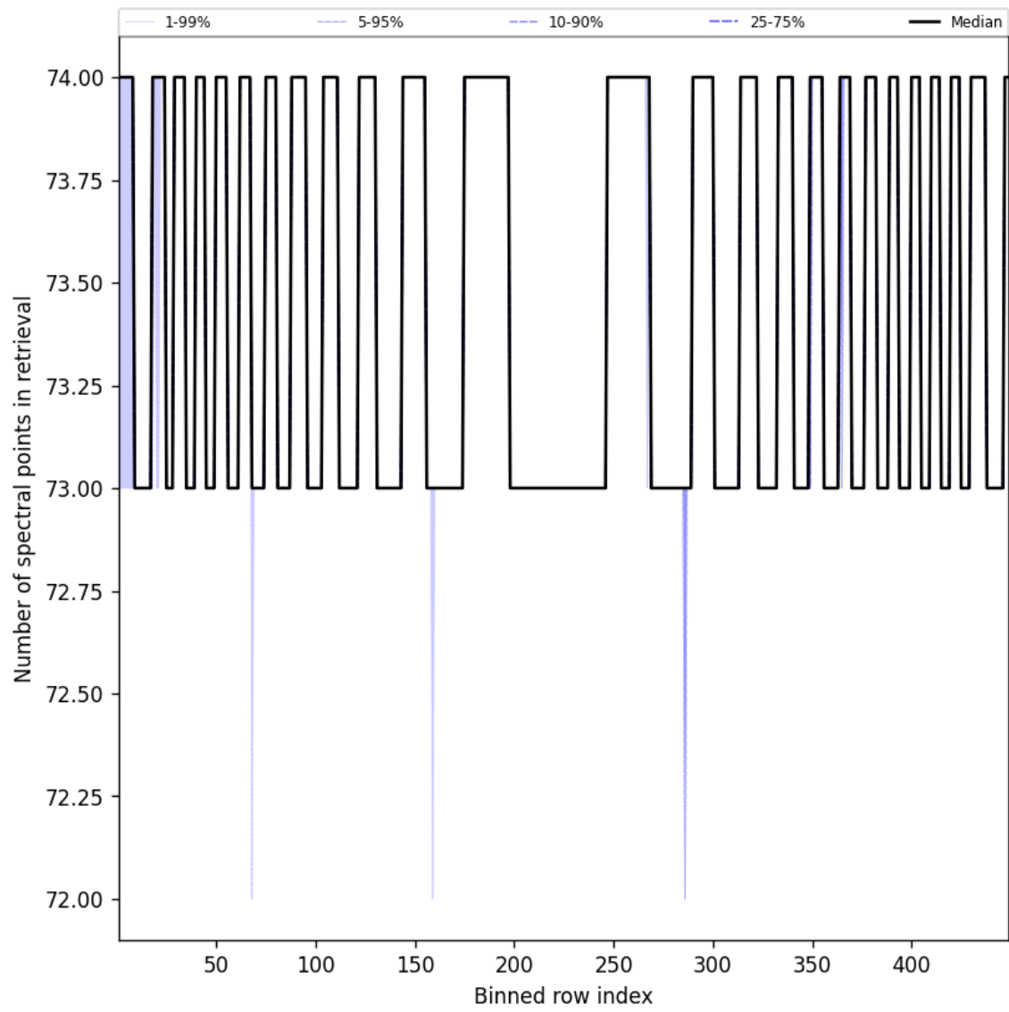
Figure 110: Along track statistics of “Number of spectral points in retrieval” for 2025-05-23 to 2025-05-24
