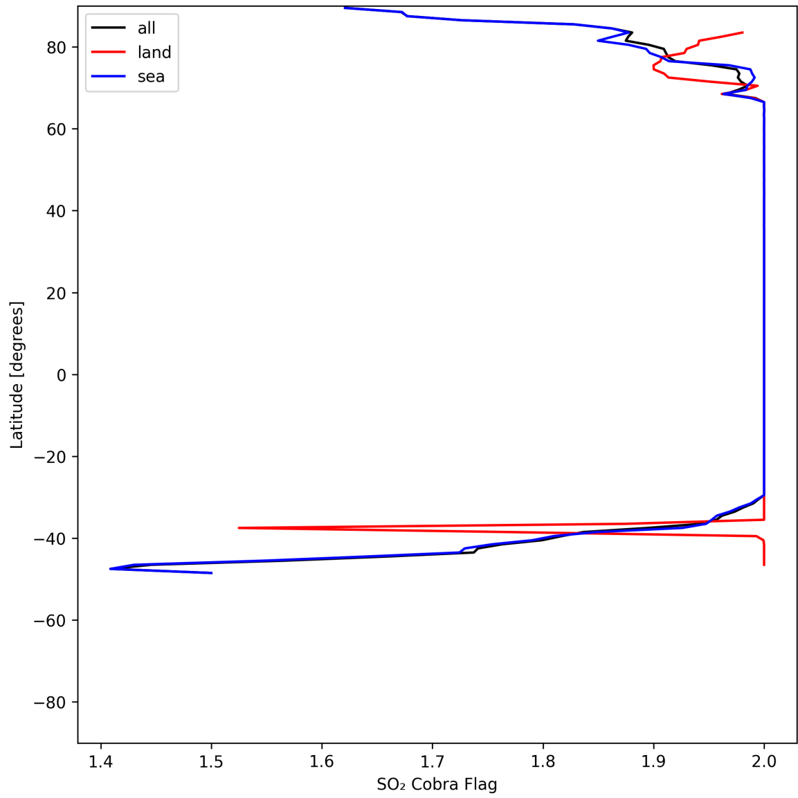
Figure 48: Zonal average of “SO 2 Cobra Flag” for 2025-05-23 to 2025-05-24.
