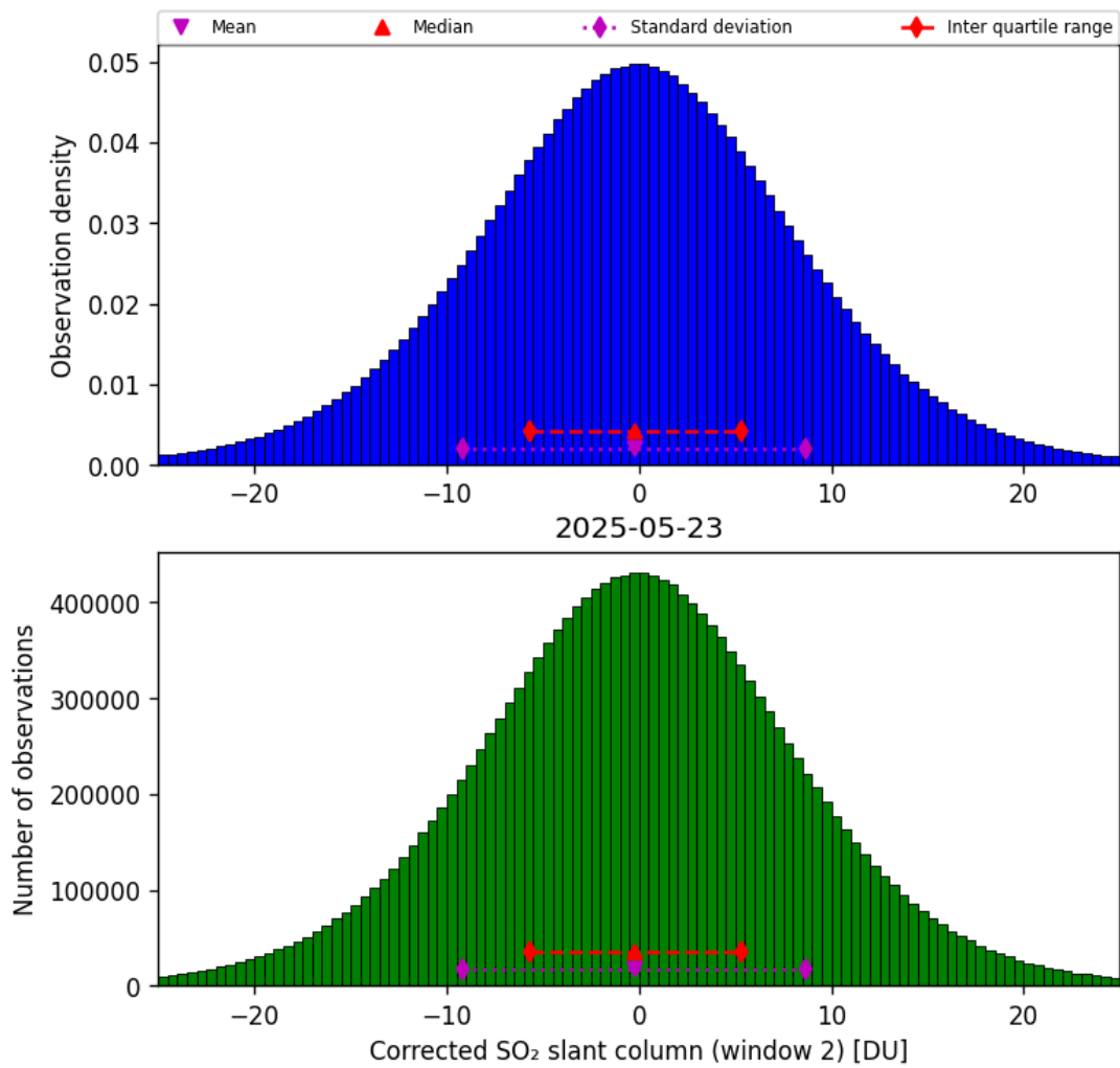
Figure 69: Histogram of “Corrected SO 2 slant column (window 2)” for 2025-05-23 to 2025-05-24
