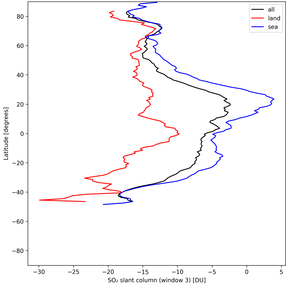
Figure 44: Zonal average of “SO 2 slant column (window 3)” for 2025-05-23 to 2025-05-24.
