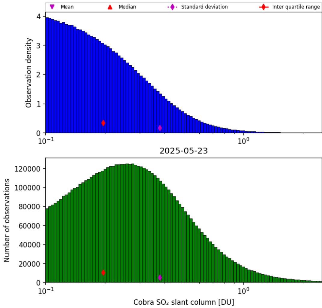
Figure 61: Histogram of “Cobra SO 2 slant column” for 2025-05-23 to 2025-05-24
