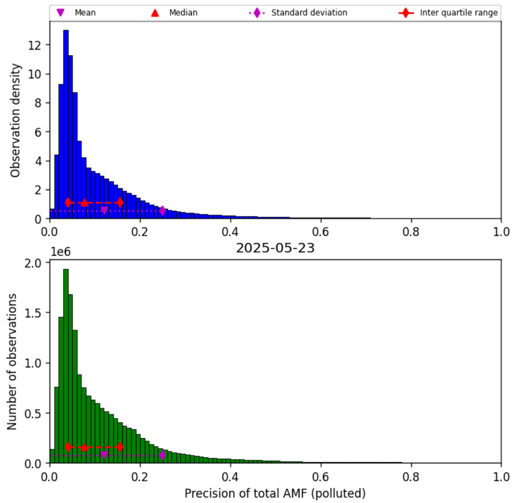
Figure 81: Histogram of “Precision of total AMF (polluted)” for 2025-05-23 to 2025-05-24
