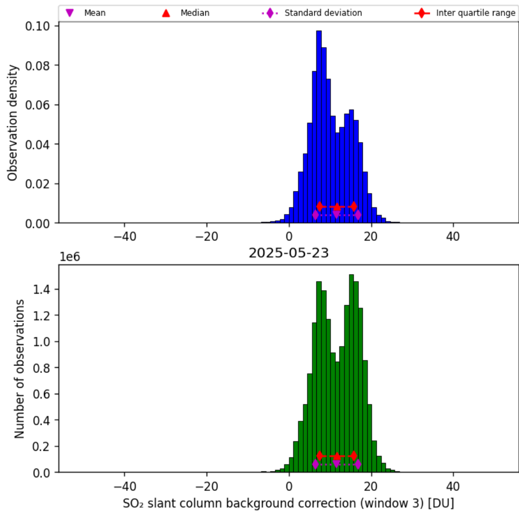
Figure 74: Histogram of “SO 2 slant column background correction (window 3)” for 2025-05-23 to 2025-05-24
