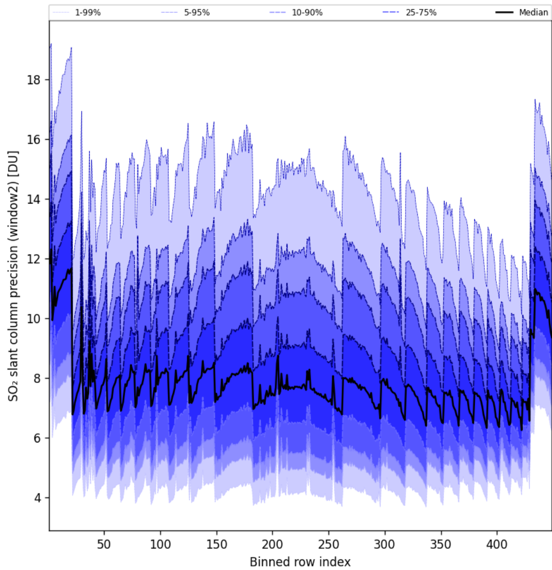
Figure 95: Along track statistics of “SO 2 slant column precision (window2)” for 2025-05-23 to 2025-05-24
