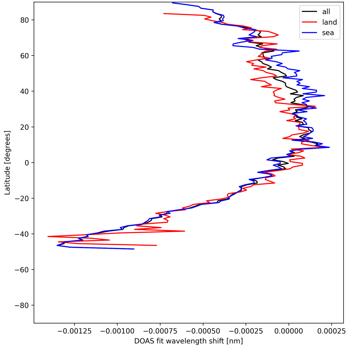
Figure 50: Zonal average of “DOAS fit wavelength shift” for 2025-05-23 to 2025-05-24.
