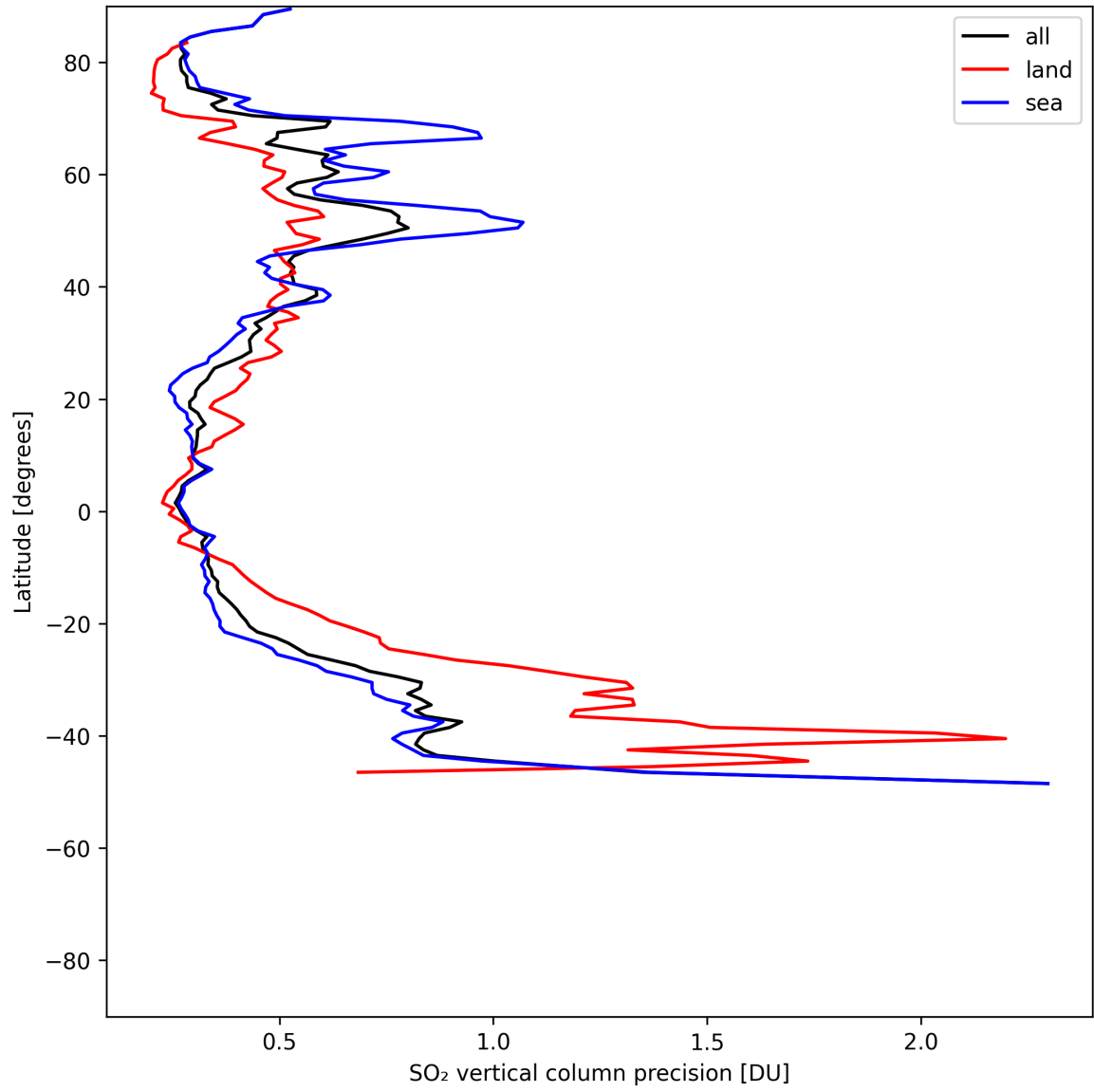
Figure 32: Zonal average of “SO 2 vertical column precision” for 2025-05-23 to 2025-05-24.
