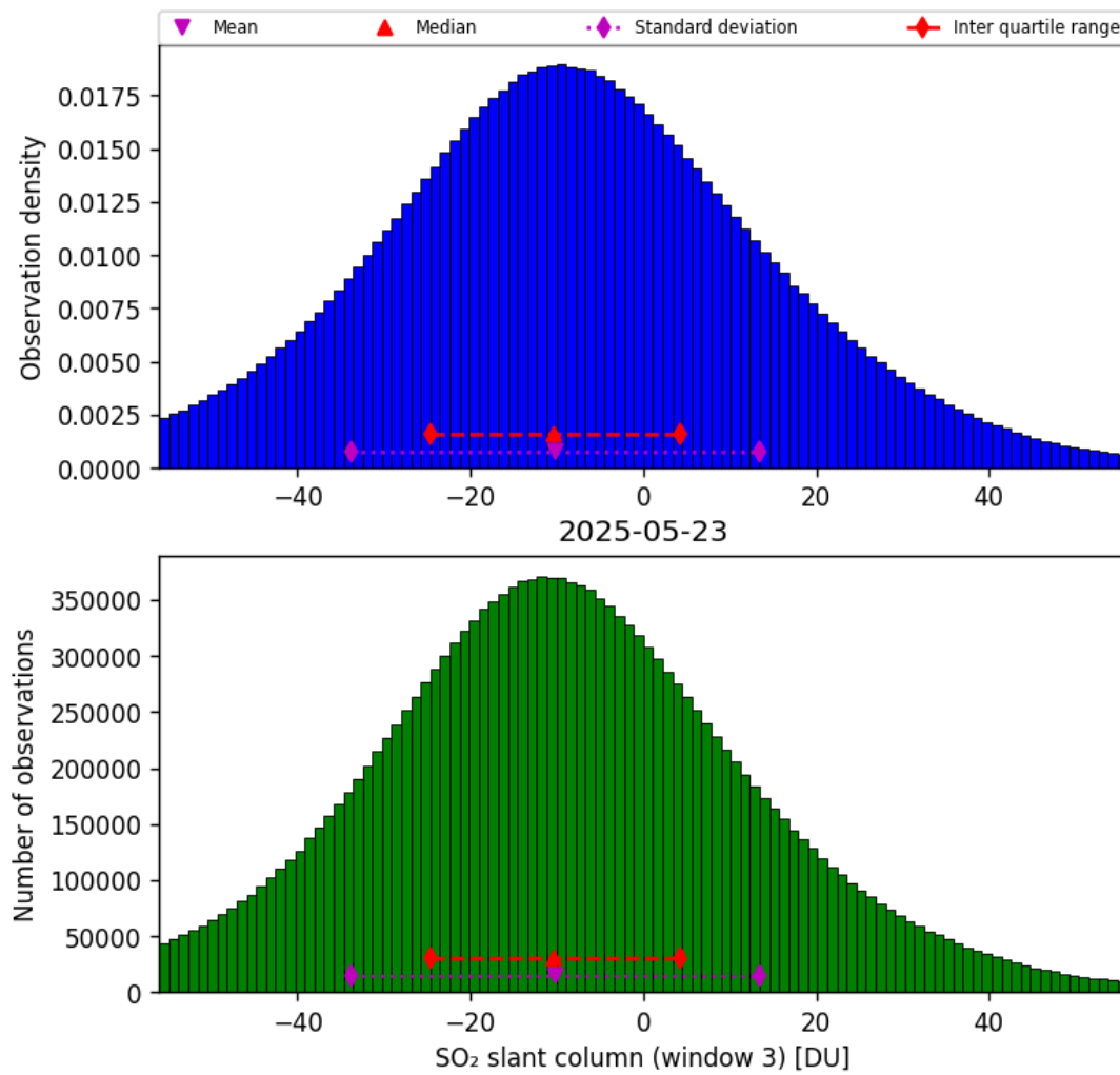
Figure 71: Histogram of “SO 2 slant column (window 3)” for 2025-05-23 to 2025-05-24
