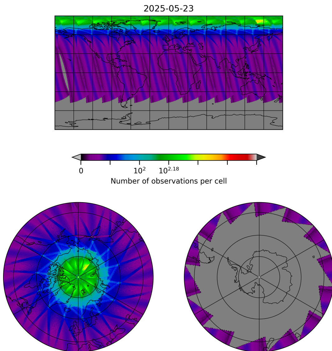
Figure 29: Map of the number of observations for 2025-05-23 to 2025-05-24
