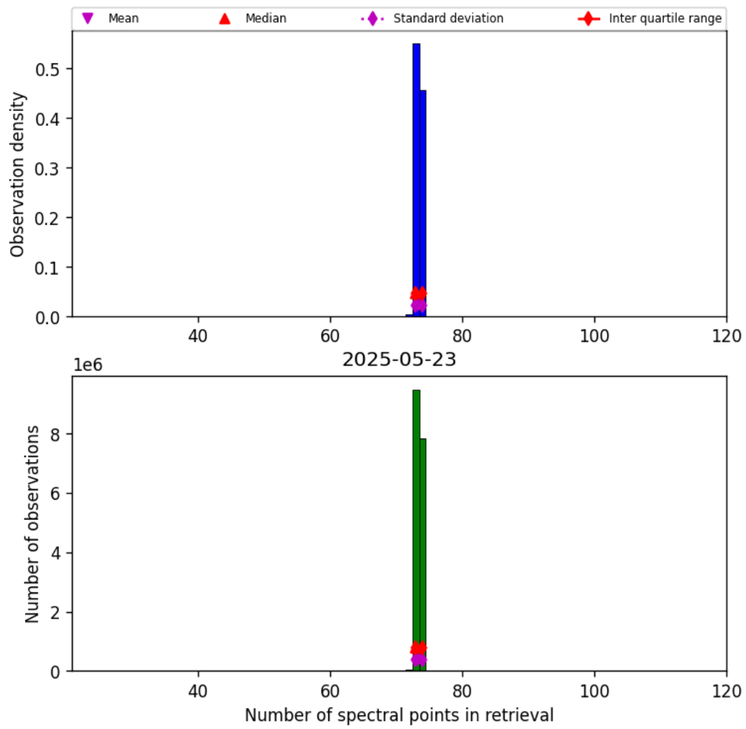
Figure 83: Histogram of “Number of spectral points in retrieval” for 2025-05-23 to 2025-05-24
