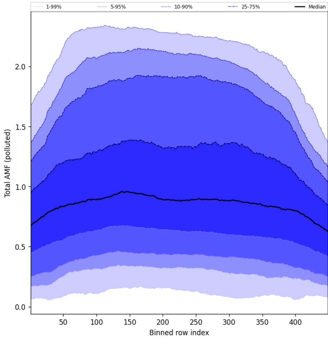
Figure 107: Along track statistics of “Total AMF (polluted)” for 2025-05-23 to 2025-05-24
