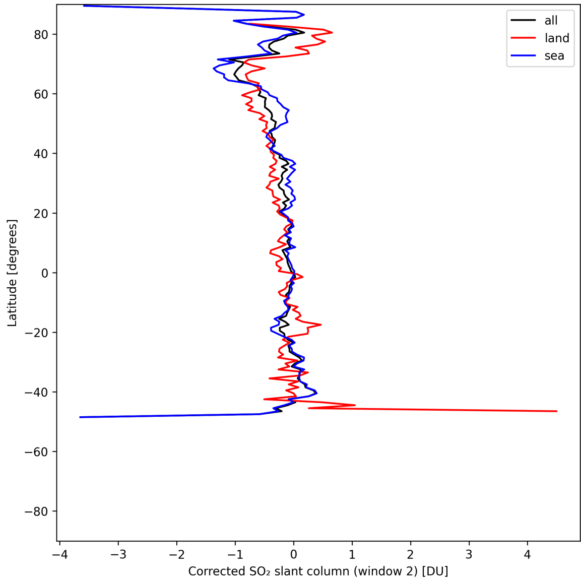
Figure 42: Zonal average of “Corrected SO 2 slant column (window 2)” for 2025-05-23 to 2025-05-24.
