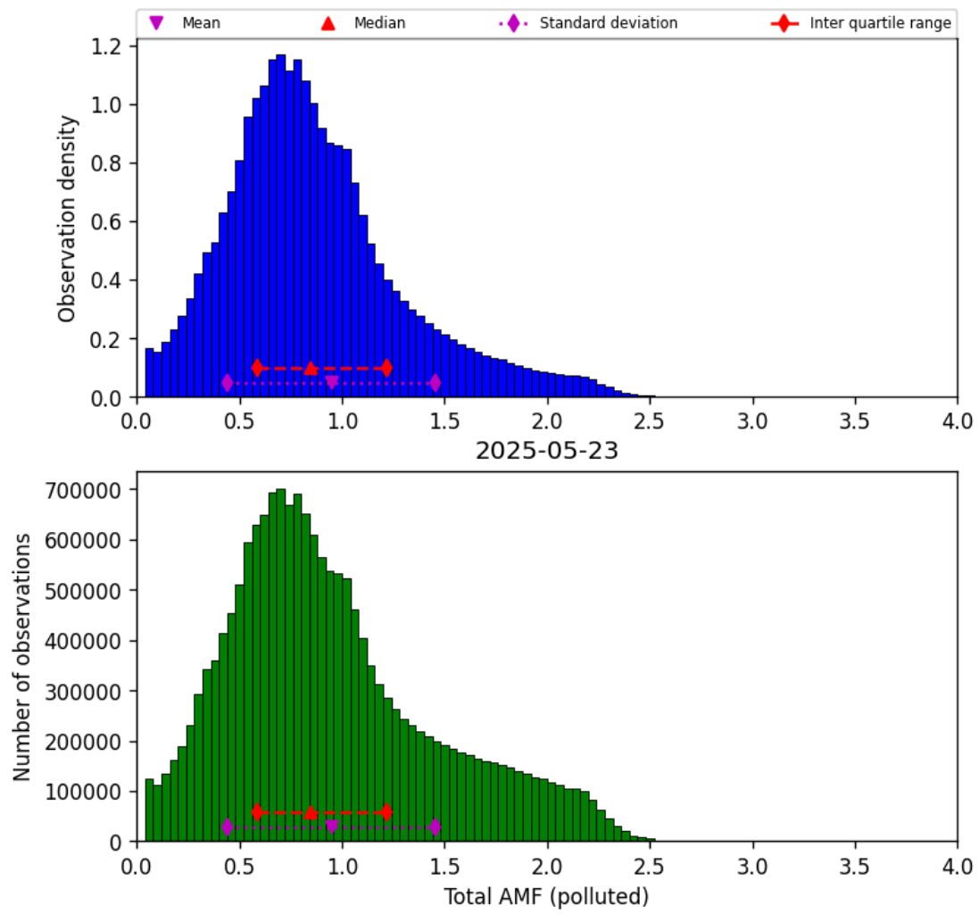
Figure 80: Histogram of “Total AMF (polluted)” for 2025-05-23 to 2025-05-24
