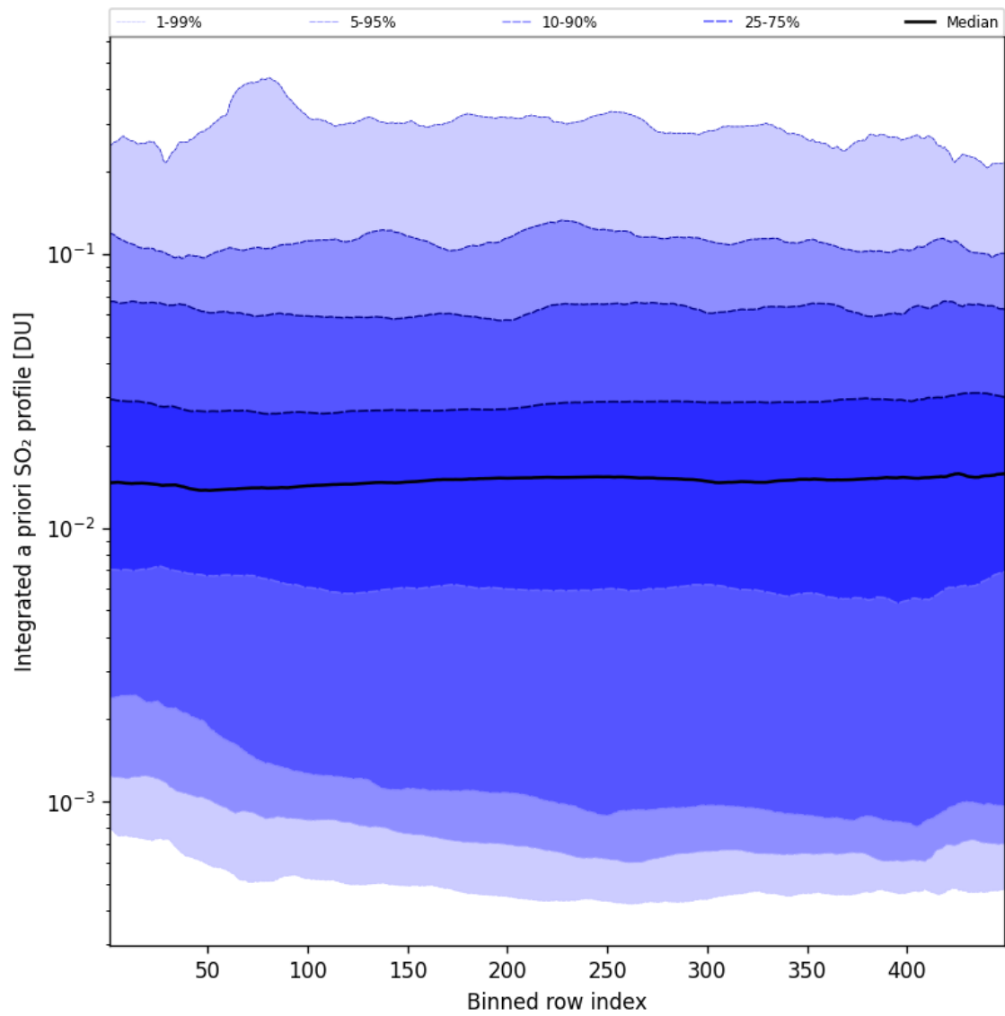
Figure 103: Along track statistics of “Integrated a priori SO 2 profile” for 2025-05-23 to 2025-05-24
