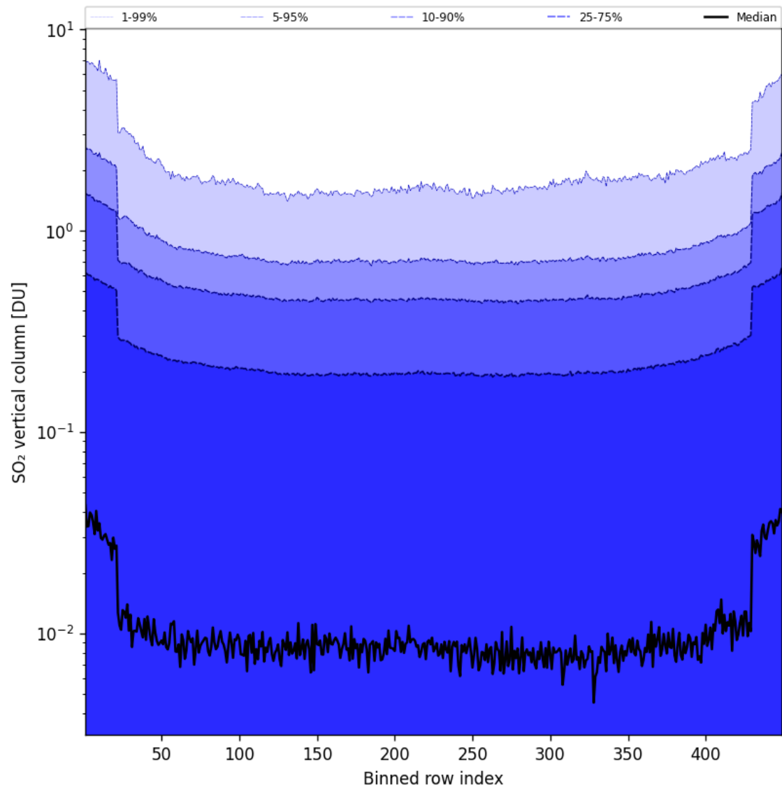
Figure 85: Along track statistics of “SO 2 vertical column” for 2025-05-23 to 2025-05-24
