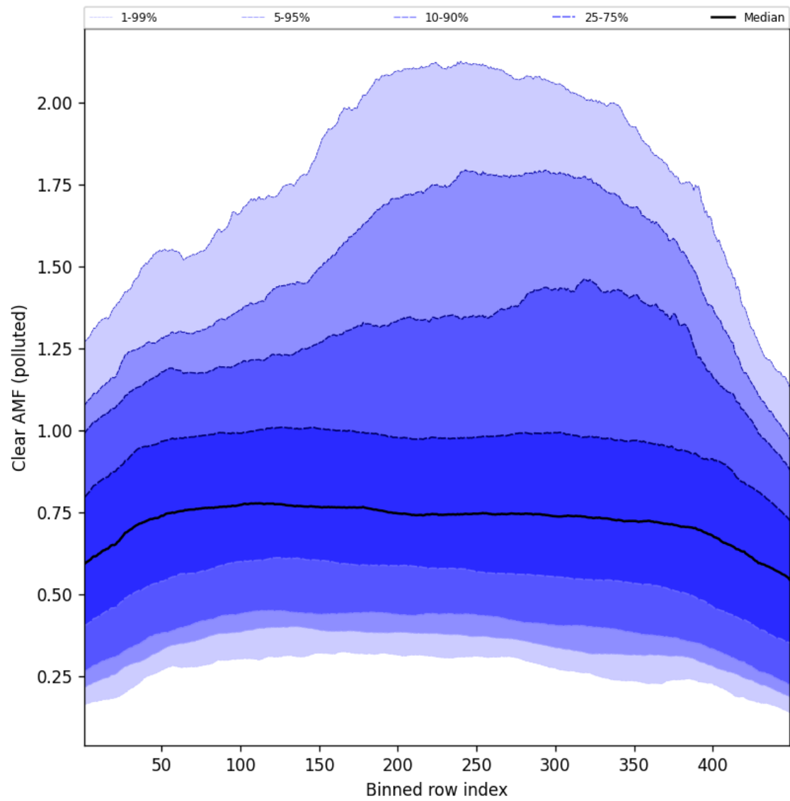
Figure 109: Along track statistics of “Clear AMF (polluted)” for 2025-05-23 to 2025-05-24
