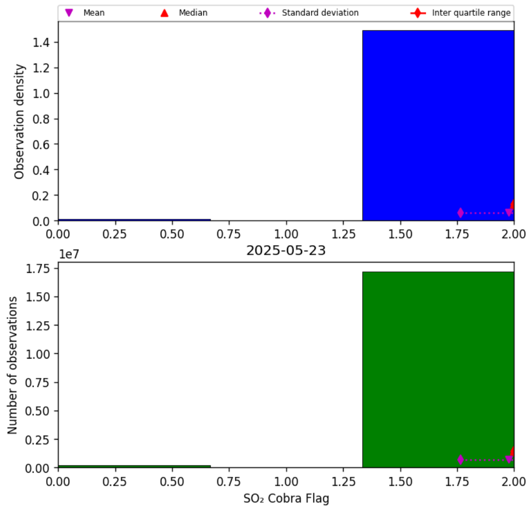
Figure 75: Histogram of “SO 2 Cobra Flag” for 2025-05-23 to 2025-05-24
