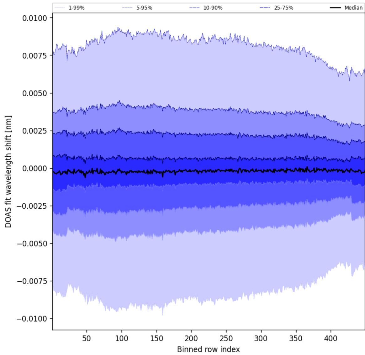
Figure 104: Along track statistics of “DOAS fit wavelength shift” for 2025-05-23 to 2025-05-24
