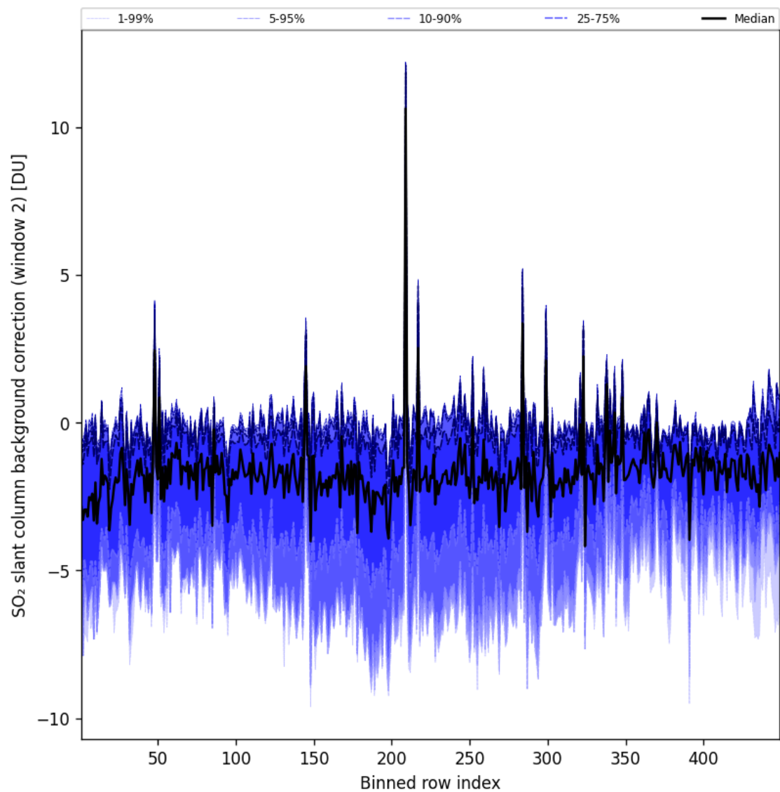
Figure 97: Along track statistics of “SO 2 slant column background correction (window 2)” for 2025-05-23 to 2025-05-24
