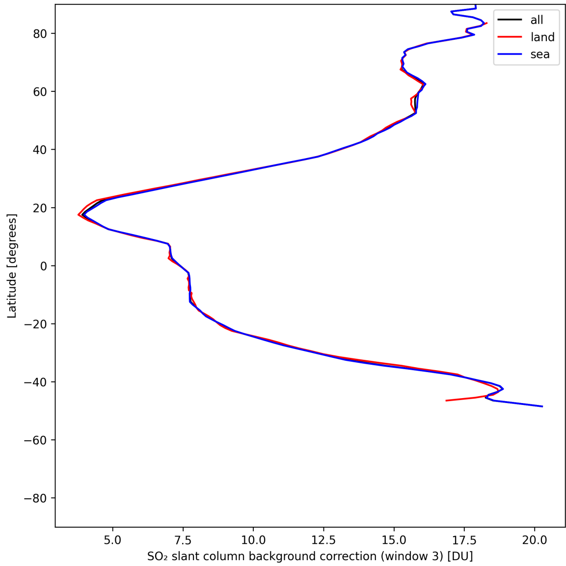
Figure 47: Zonal average of “SO 2 slant column background correction (window 3)” for 2025-05-23 to 2025-05-24.
