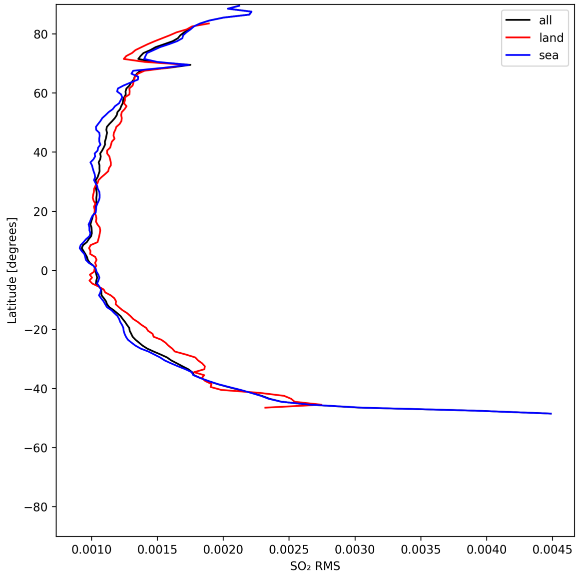
Figure 52: Zonal average of “SO 2 RMS” for 2025-05-23 to 2025-05-24.
