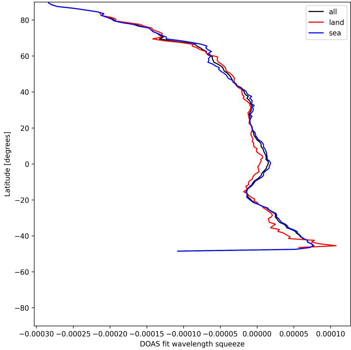
Figure 51: Zonal average of “DOAS fit wavelength squeeze” for 2025-05-23 to 2025-05-24.
