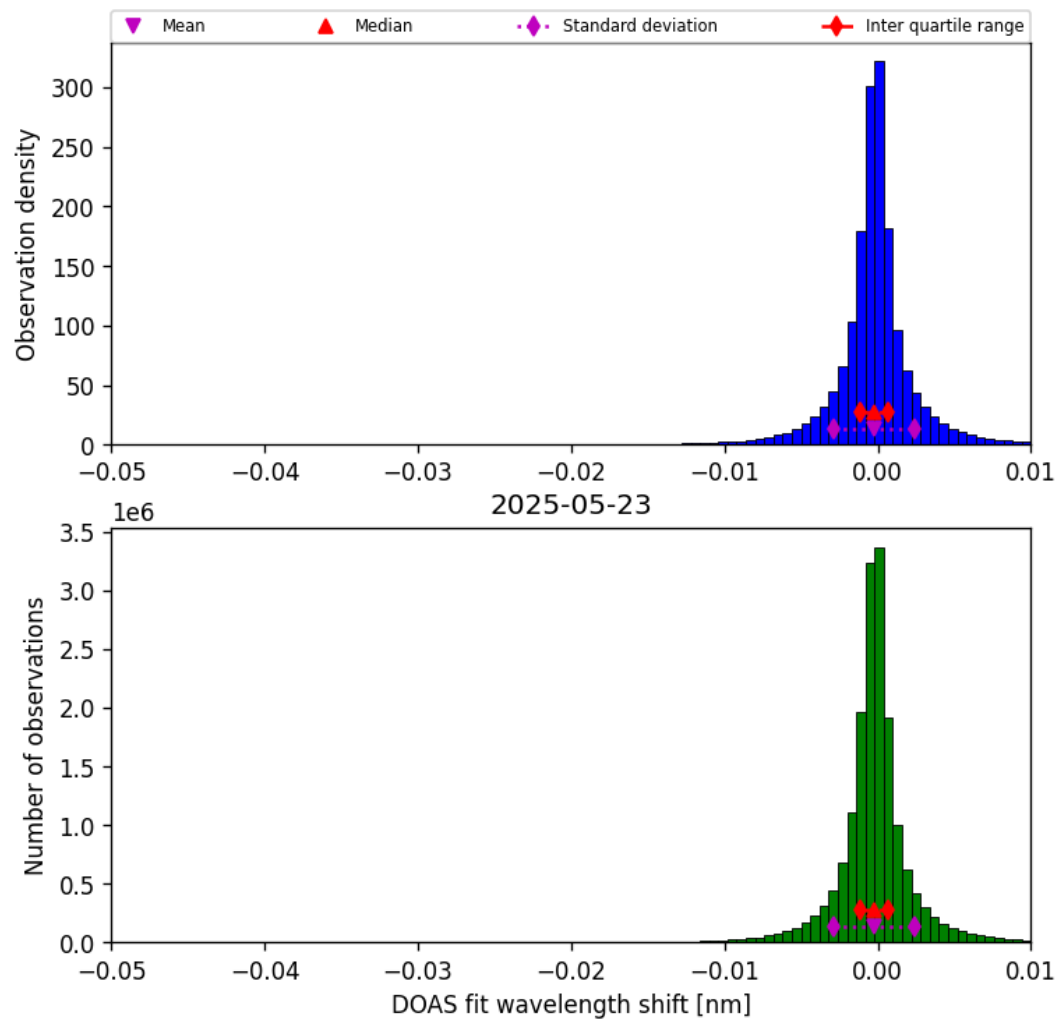
Figure 77: Histogram of “DOAS fit wavelength shift” for 2025-05-23 to 2025-05-24
