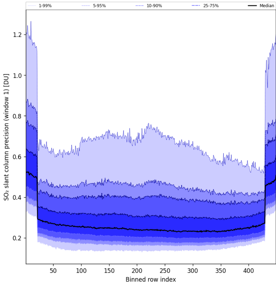
Figure 91: Along track statistics of “SO 2 slant column precision (window 1)” for 2025-05-23 to 2025-05-24
