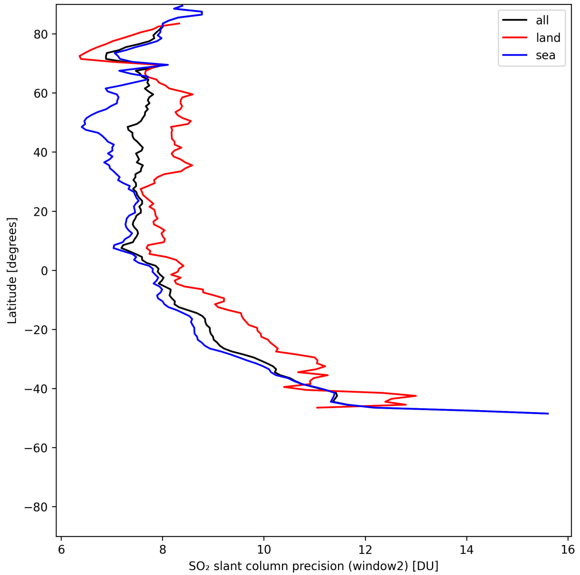
Figure 41: Zonal average of “SO 2 slant column precision (window2)” for 2025-05-23 to 2025-05-24.
