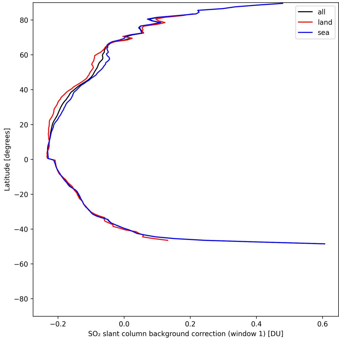
Figure 39: Zonal average of "SO 2 slant column background correction (window 1)" for 2025-05-23 to 2025-05-24.
