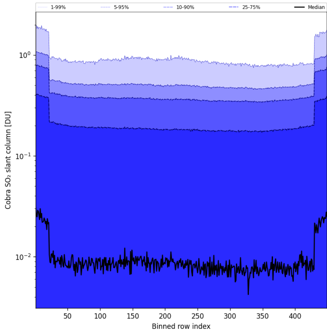
Figure 88: Along track statistics of “Cobra SO 2 slant column” for 2025-05-23 to 2025-05-24
