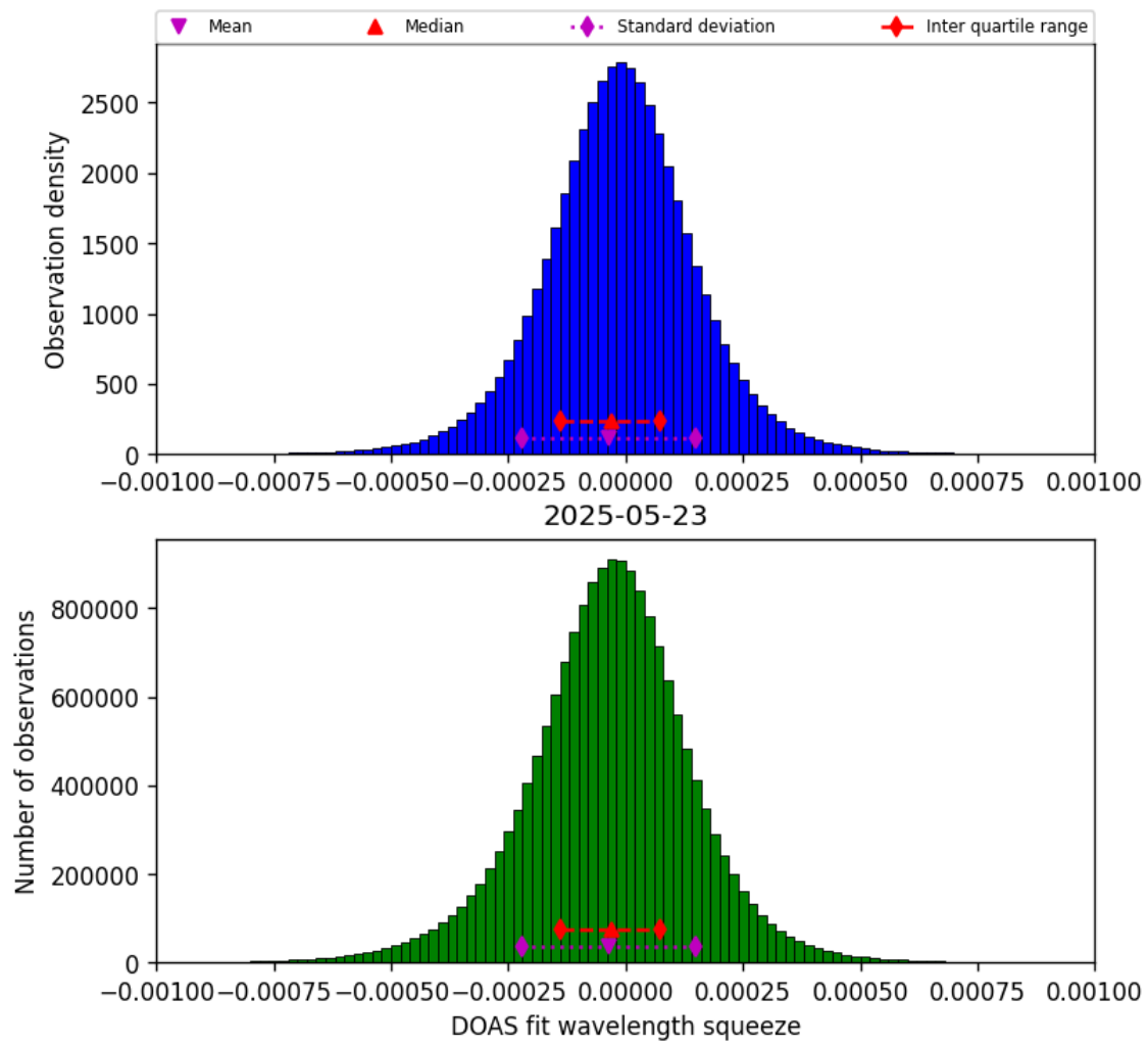
Figure 78: Histogram of “DOAS fit wavelength squeeze” for 2025-05-23 to 2025-05-24
