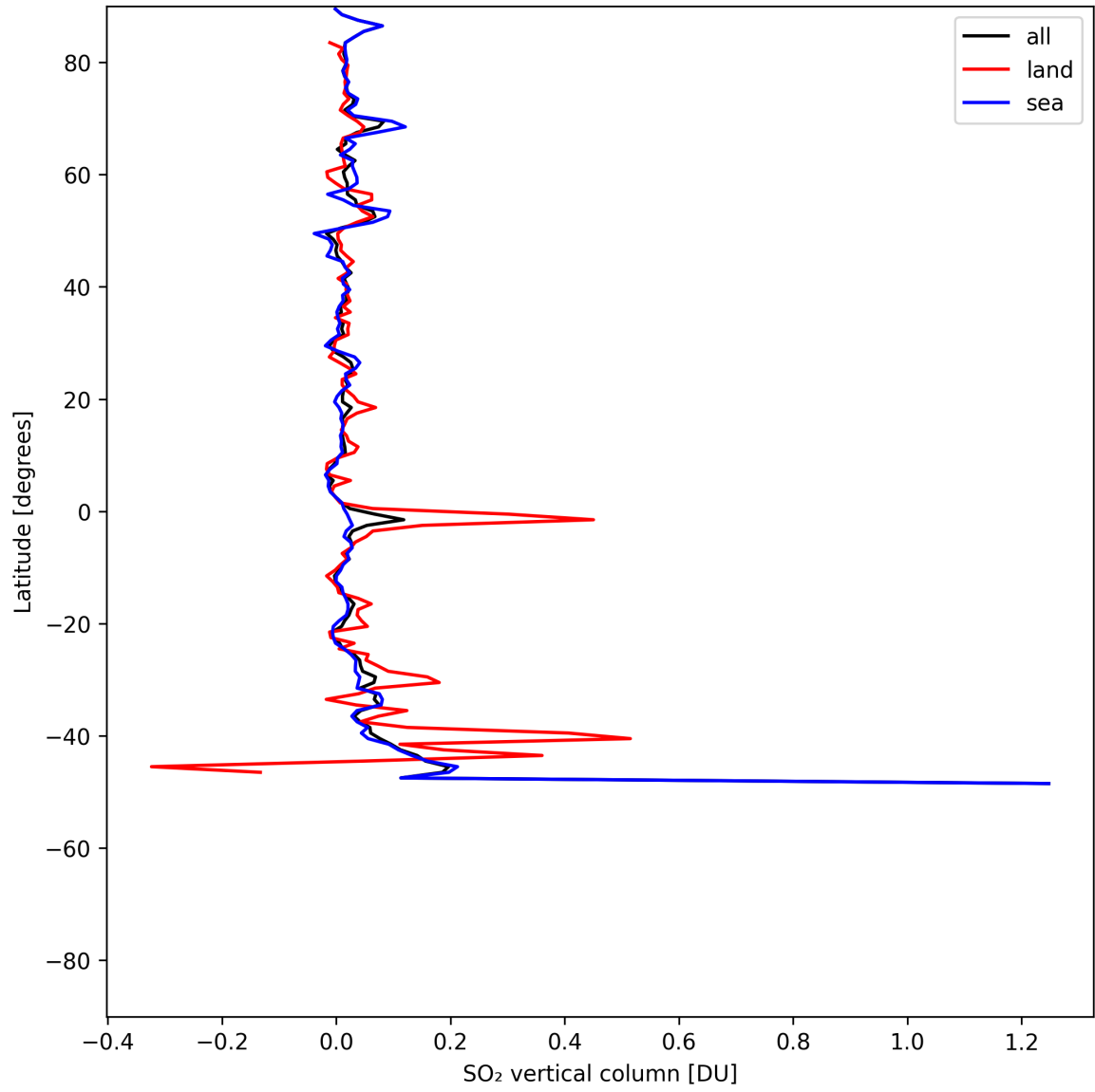
Figure 31: Zonal average of “SO 2 vertical column” for 2025-05-23 to 2025-05-24.
