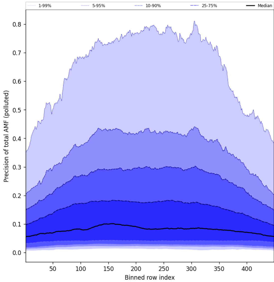
Figure 108: Along track statistics of “Precision of total AMF (polluted)” for 2025-05-23 to 2025-05-24
