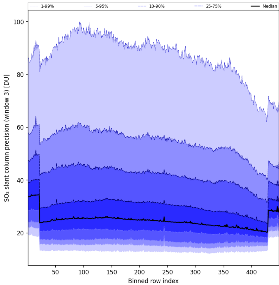
Figure 99: Along track statistics of “SO 2 slant column precision (window 3)” for 2025-05-23 to 2025-05-24
