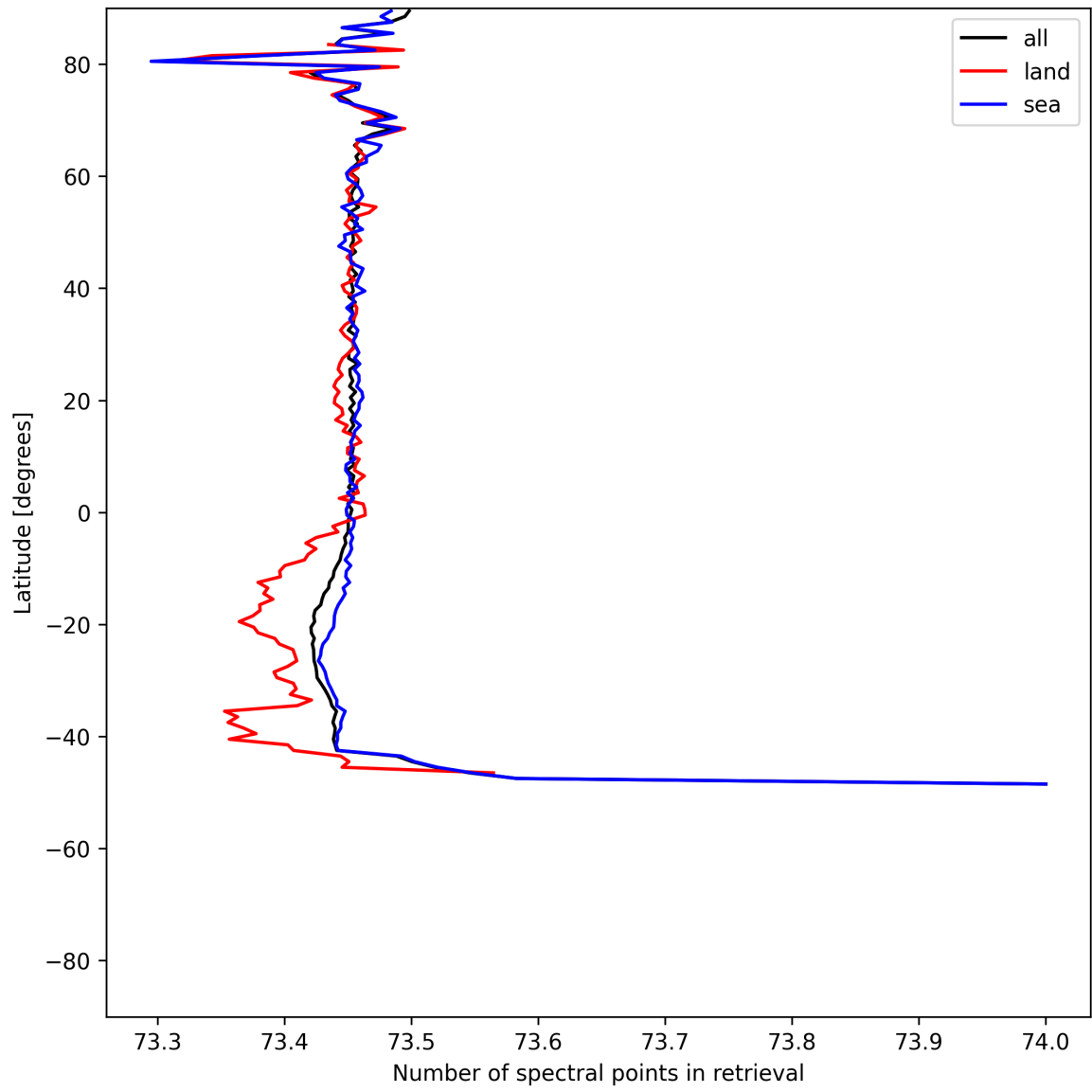
Figure 56: Zonal average of “Number of spectral points in retrieval” for 2025-05-23 to 2025-05-24.
