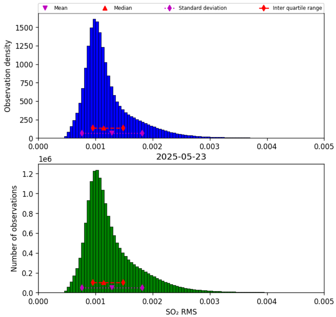
Figure 79: Histogram of “SO 2 RMS” for 2025-05-23 to 2025-05-24
