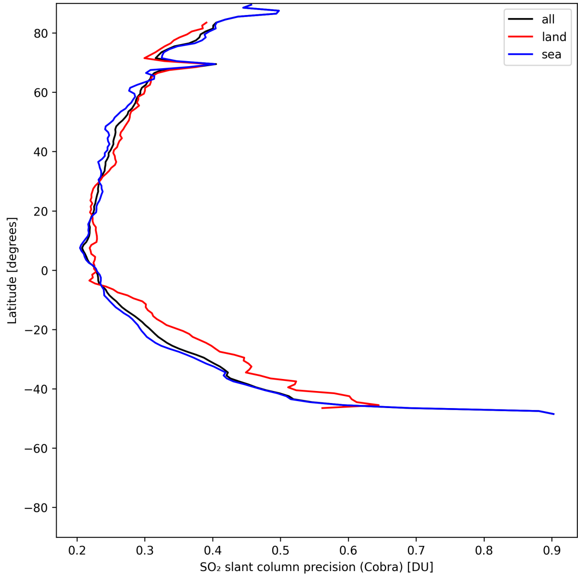
Figure 35: Zonal average of "SO 2 slant column precision (Cobra)" for 2025-05-23 to 2025-05-24.
