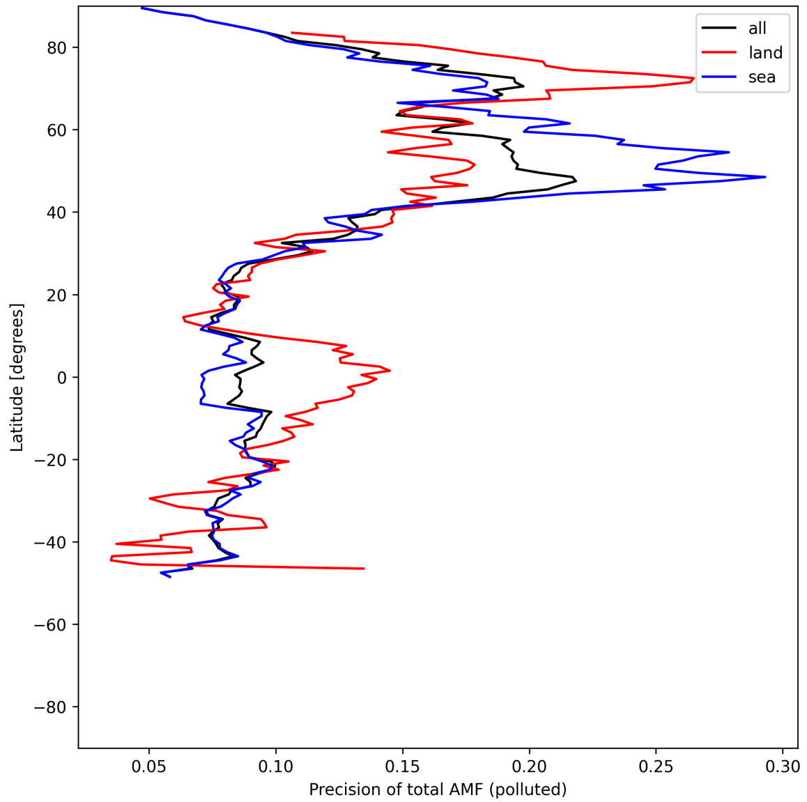
Figure 54: Zonal average of “Precision of total AMF (polluted)” for 2025-05-23 to 2025-05-24.
