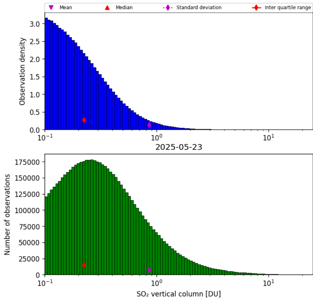
Figure 58: Histogram of “SO 2 vertical column” for 2025-05-23 to 2025-05-24
