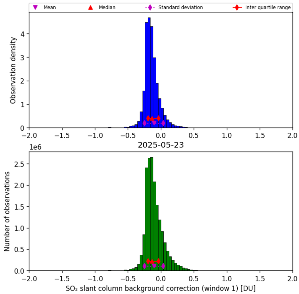
Figure 66: Histogram of “SO 2 slant column background correction (window 1)” for 2025-05-23 to 2025-05-24
