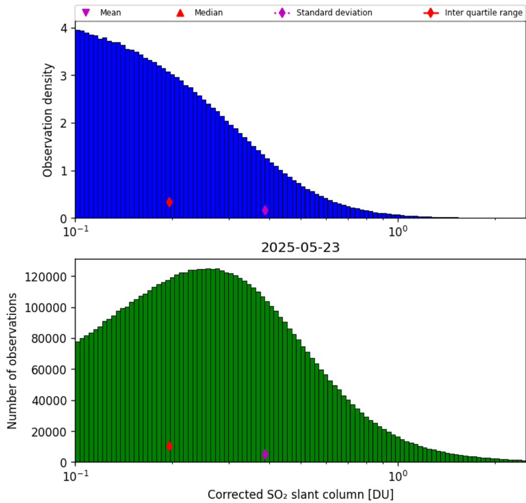
Figure 60: Histogram of “Corrected SO 2 slant column” for 2025-05-23 to 2025-05-24
