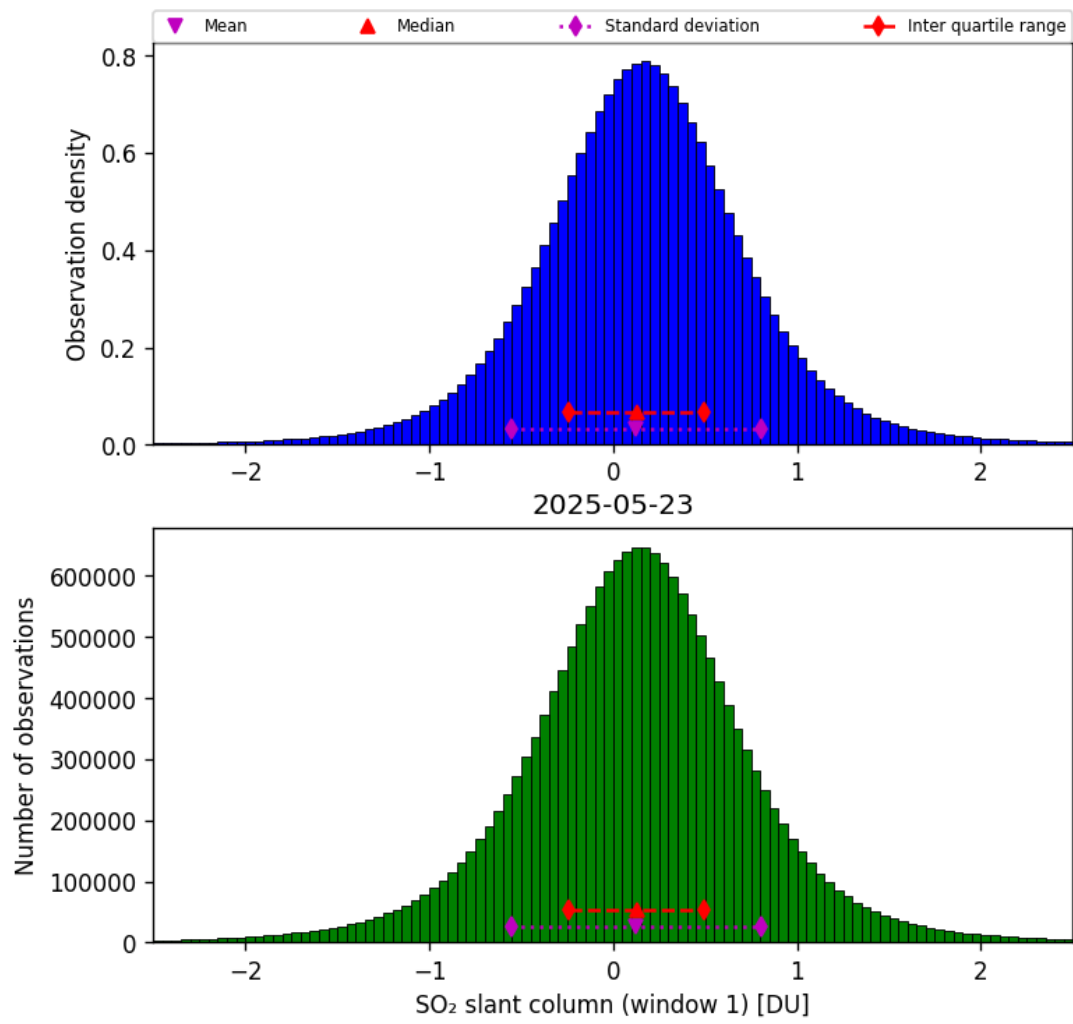
Figure 63: Histogram of “SO 2 slant column (window 1)” for 2025-05-23 to 2025-05-24
