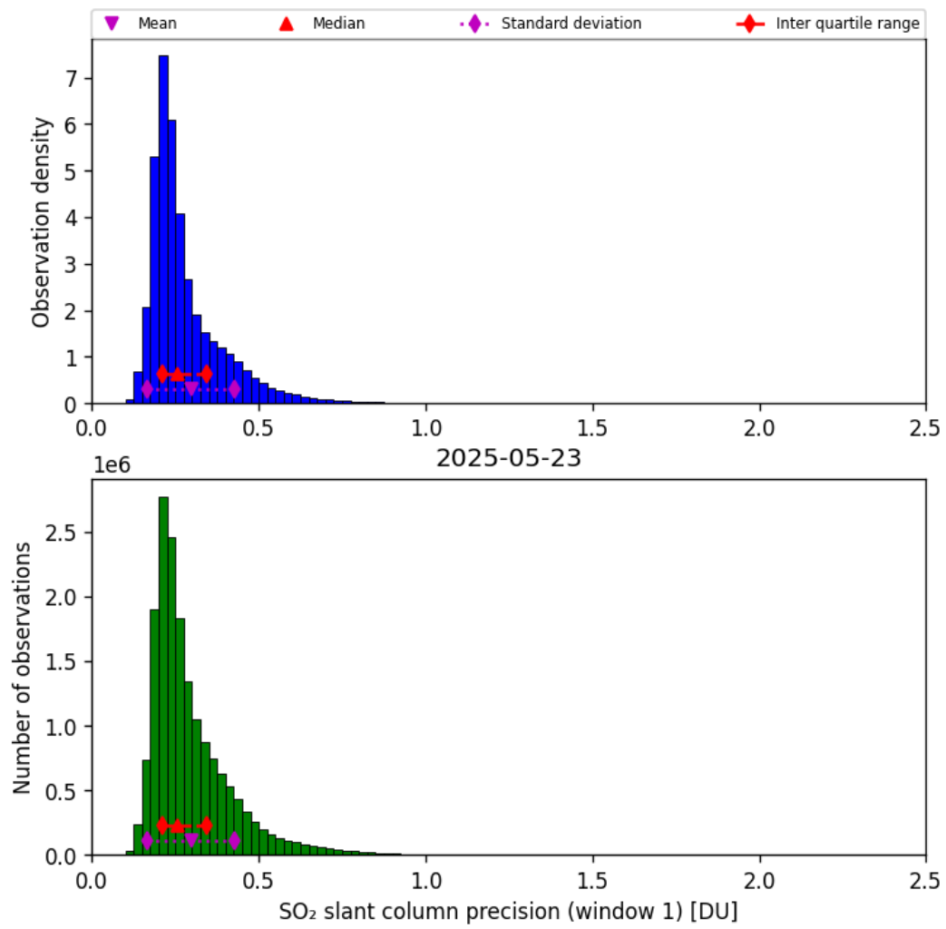
Figure 64: Histogram of “SO 2 slant column precision (window 1)” for 2025-05-23 to 2025-05-24
