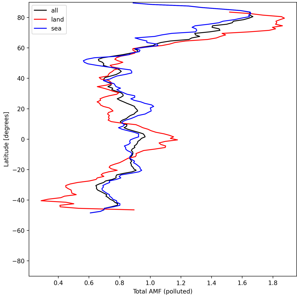
Figure 53: Zonal average of “Total AMF (polluted)” for 2025-05-23 to 2025-05-24.
