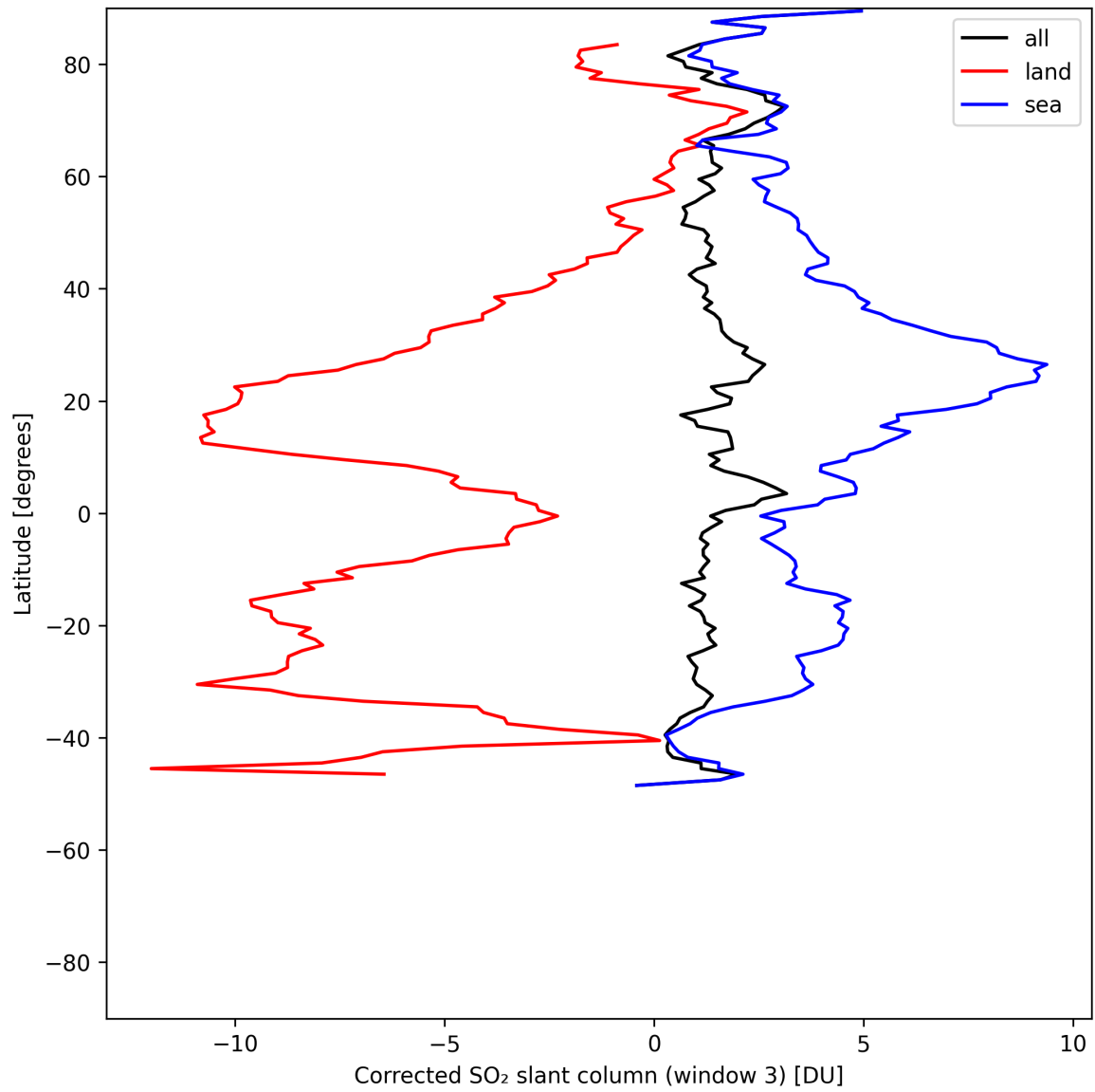
Figure 46: Zonal average of “Corrected SO 2 slant column (window 3)” for 2025-05-23 to 2025-05-24.
