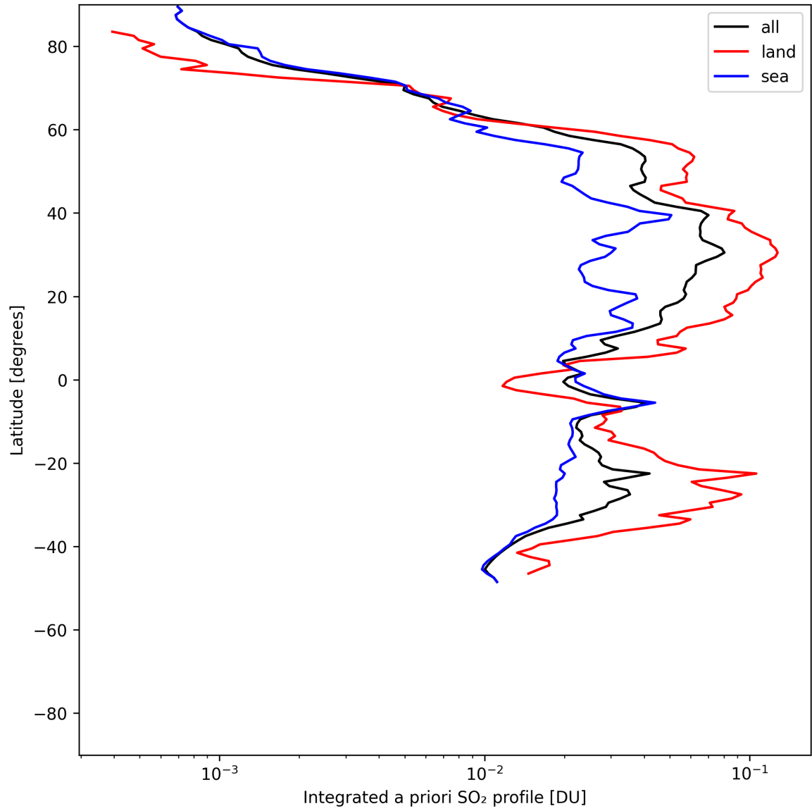
Figure 49: Zonal average of “Integrated a priori SO 2 profile” for 2025-05-23 to 2025-05-24.
