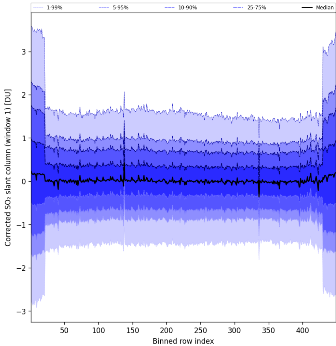
Figure 92: Along track statistics of “Corrected SO 2 slant column (window 1)” for 2025-05-23 to 2025-05-24
