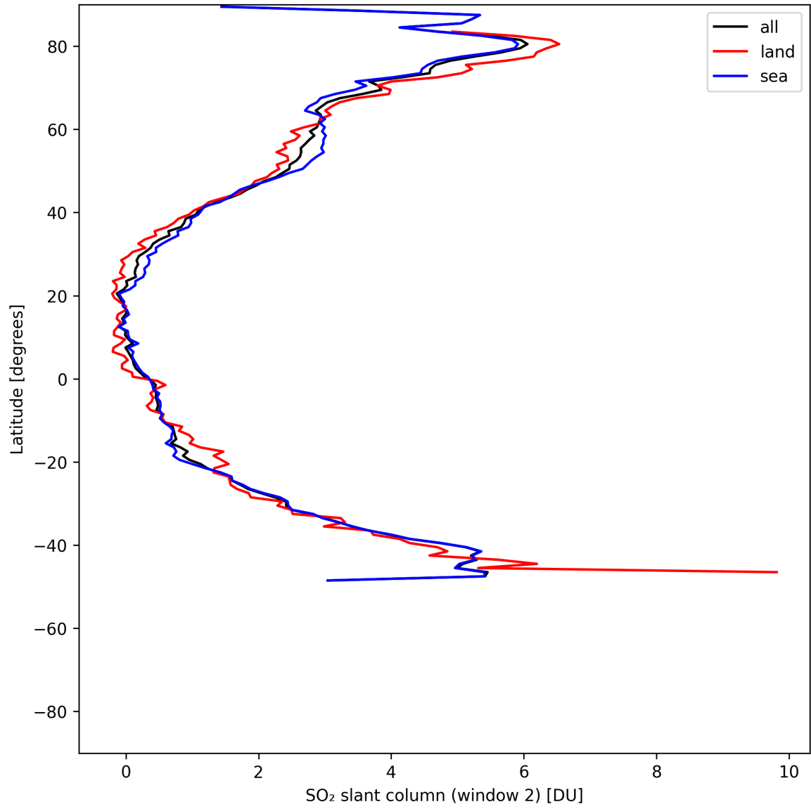
Figure 40: Zonal average of “SO 2 slant column (window 2)” for 2025-05-23 to 2025-05-24.
