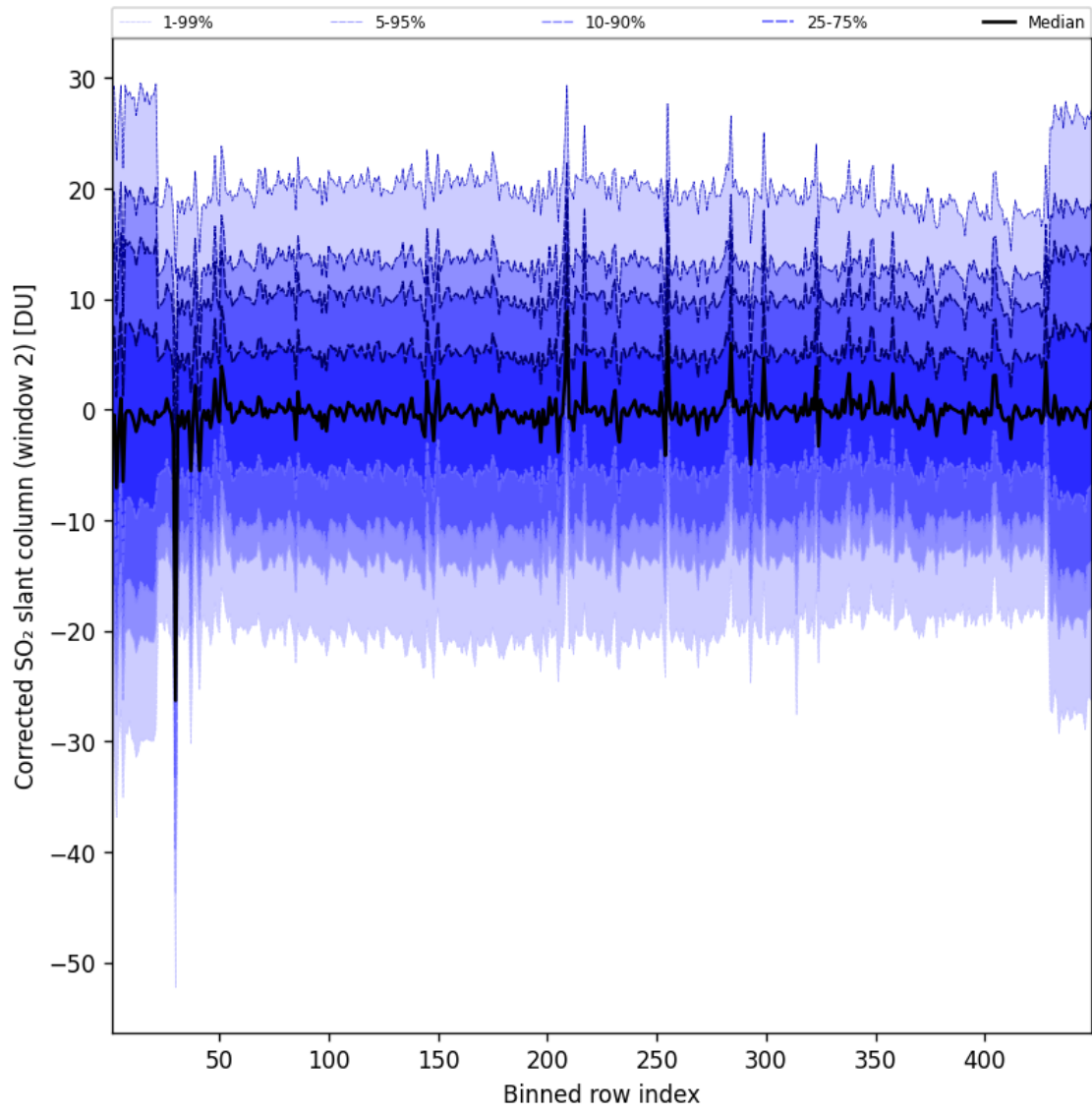
Figure 96: Along track statistics of “Corrected SO 2 slant column (window 2)” for 2025-05-23 to 2025-05-24
