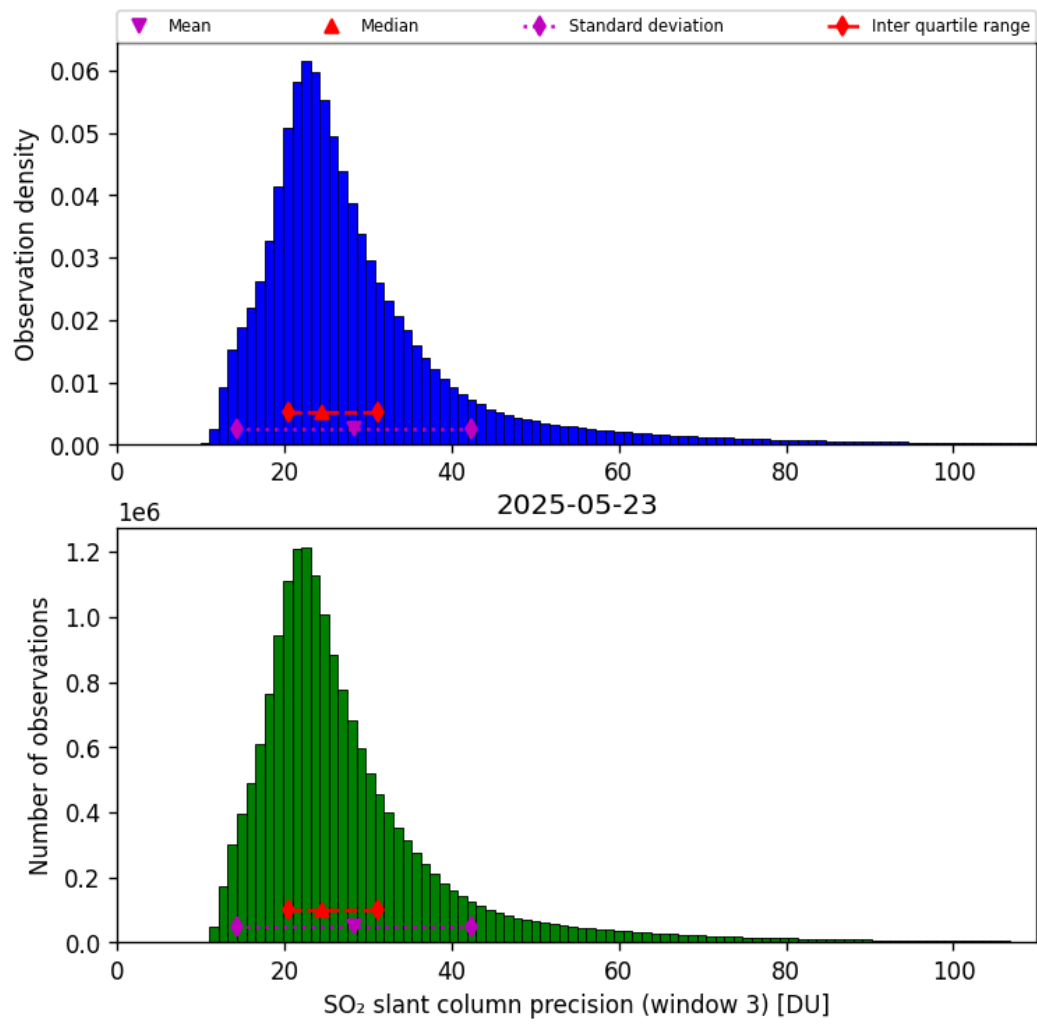
Figure 72: Histogram of “SO 2 slant column precision (window 3)” for 2025-05-23 to 2025-05-24
