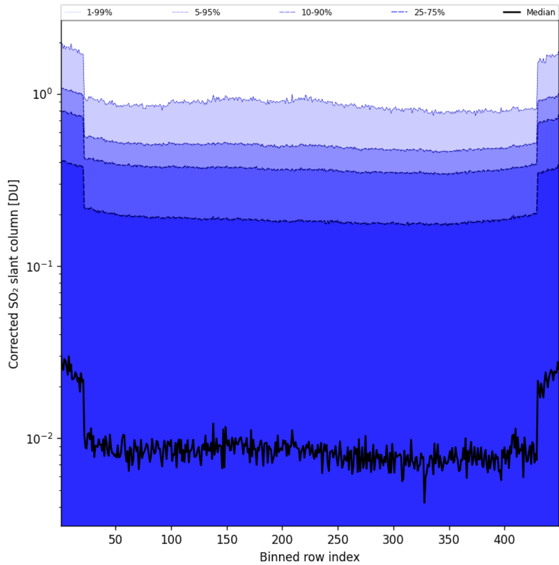
Figure 87: Along track statistics of “Corrected SO 2 slant column” for 2025-05-23 to 2025-05-24
