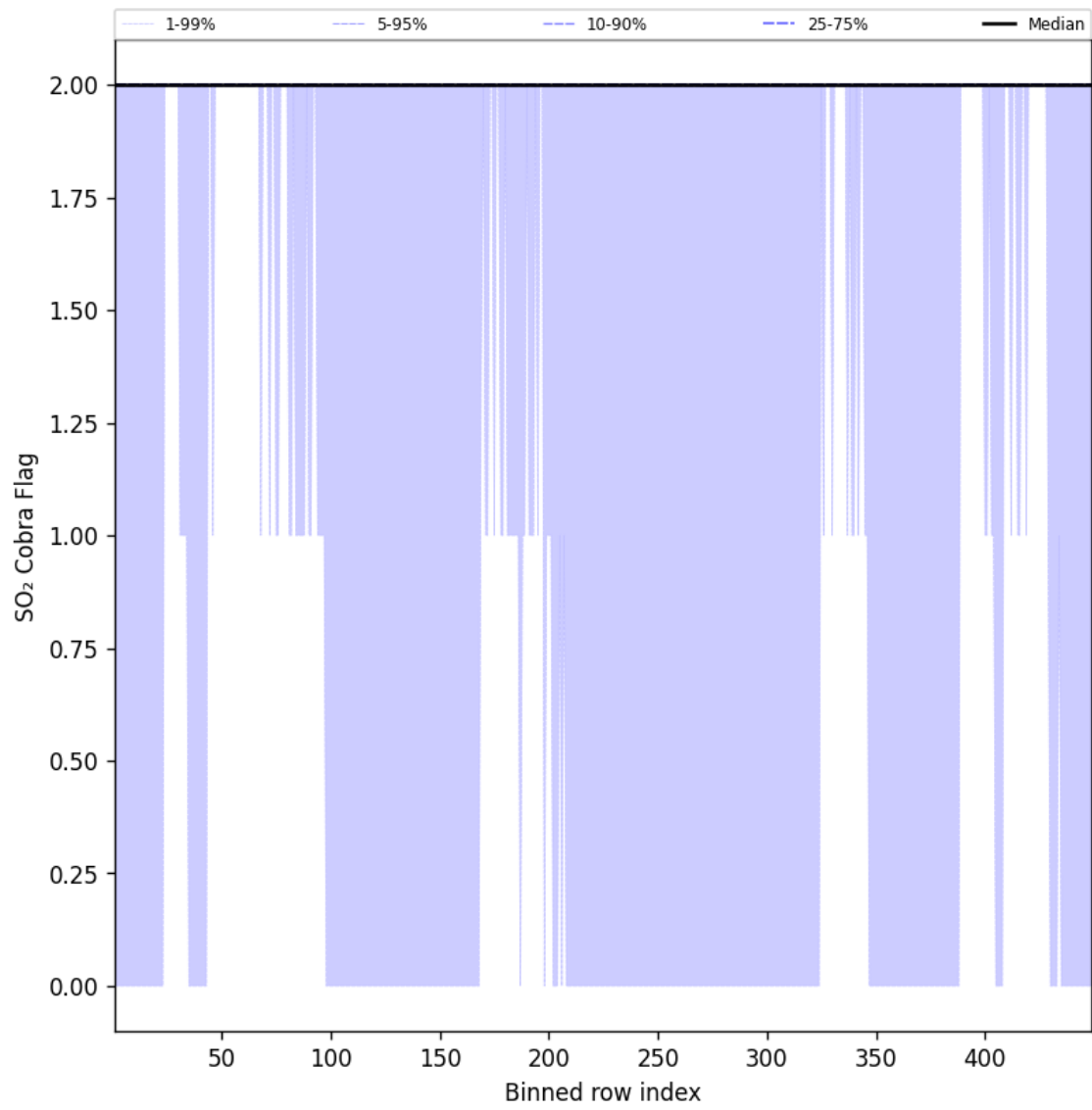
Figure 102: Along track statistics of "SO 2 Cobra Flag" for 2025-05-23 to 2025-05-24
