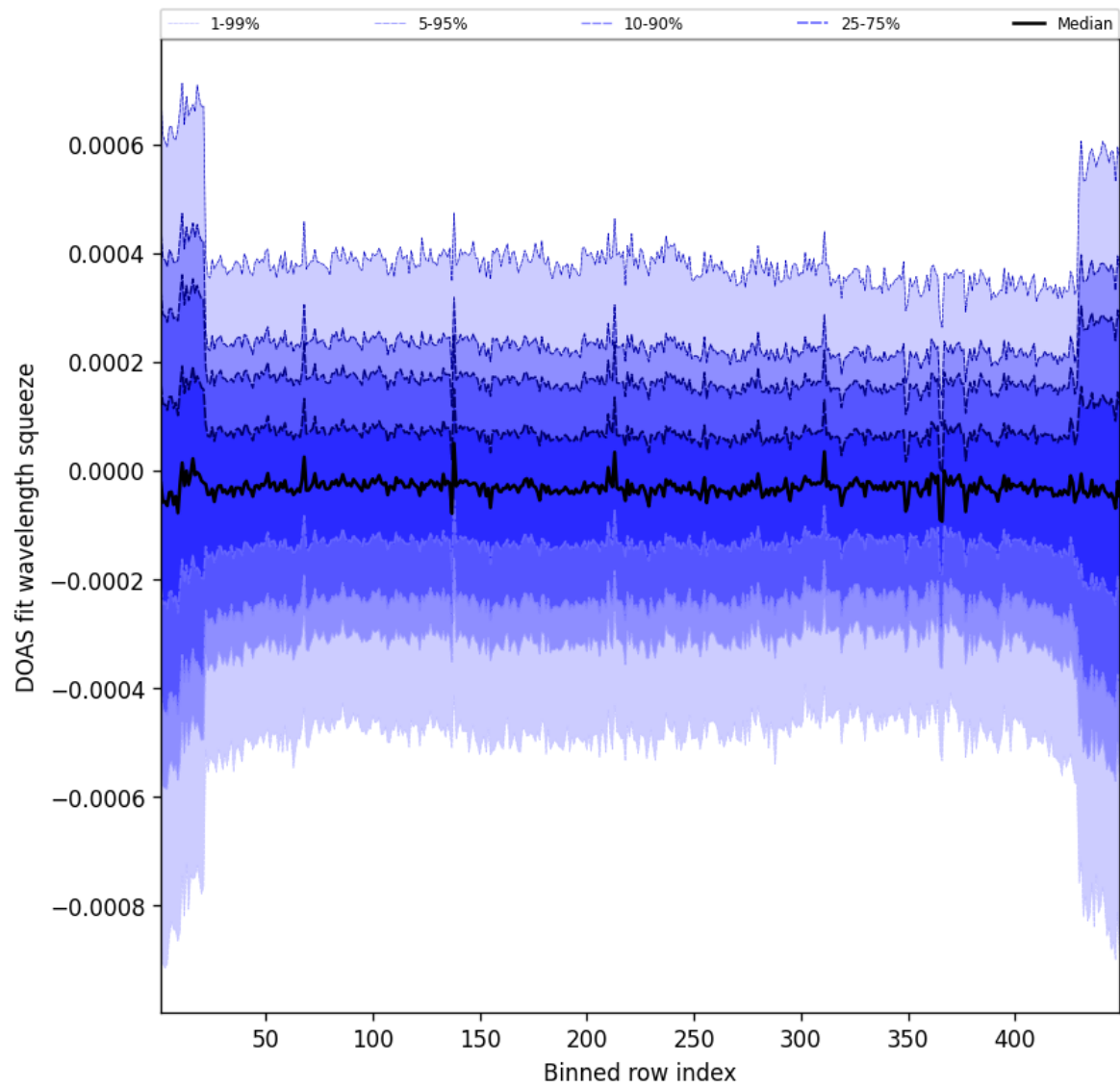
Figure 105: Along track statistics of “DOAS fit wavelength squeeze” for 2025-05-23 to 2025-05-24
