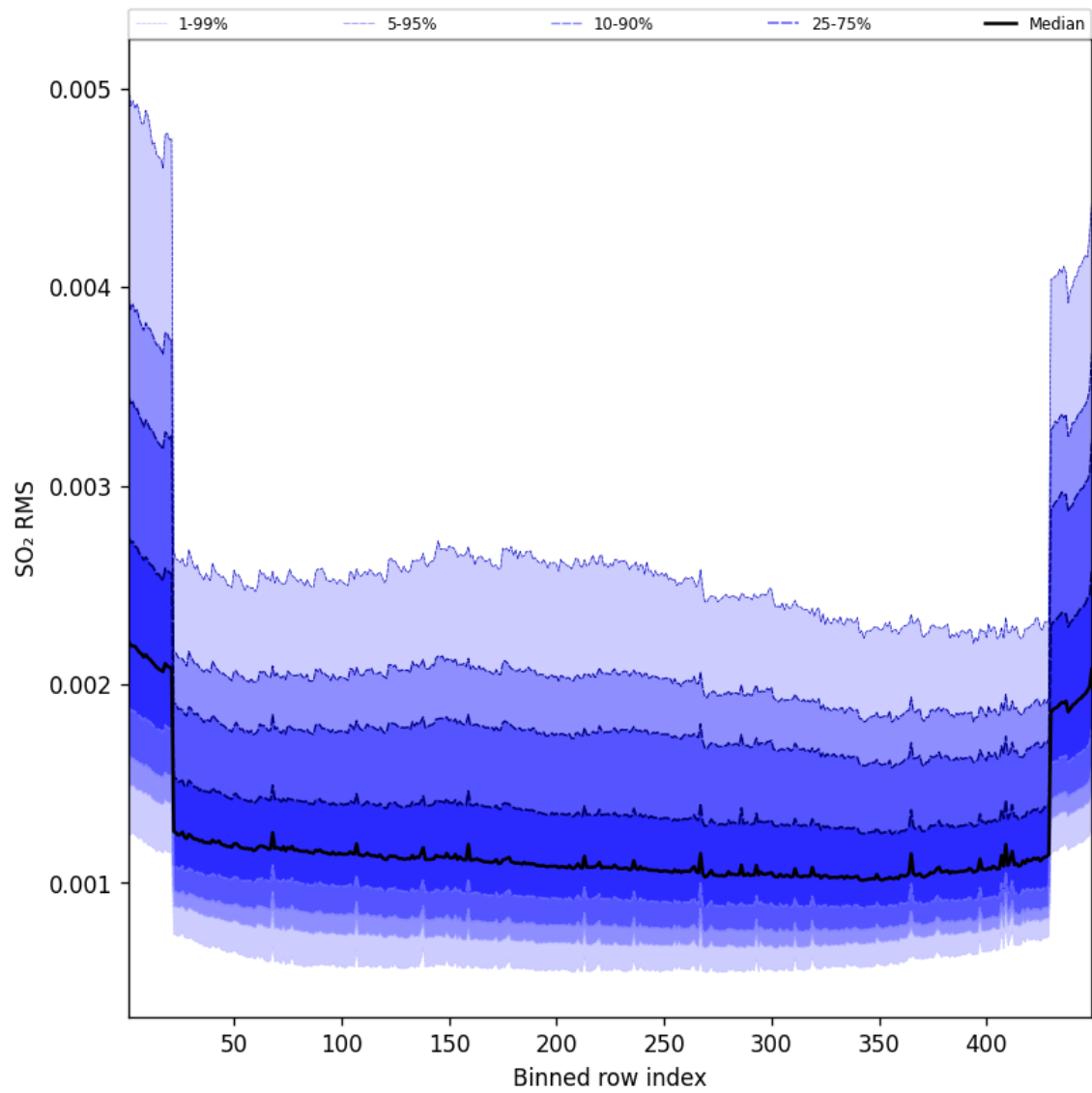
Figure 106: Along track statistics of “SO 2 RMS” for 2025-05-23 to 2025-05-24
