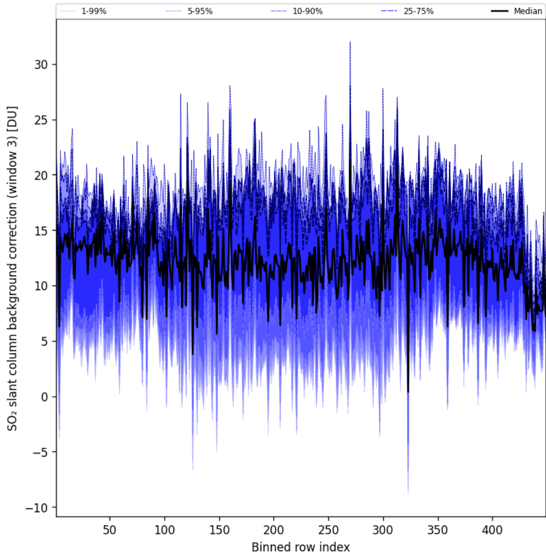
Figure 101: Along track statistics of “SO 2 slant column background correction (window 3)” for 2025-05-23 to 2025-05-24
