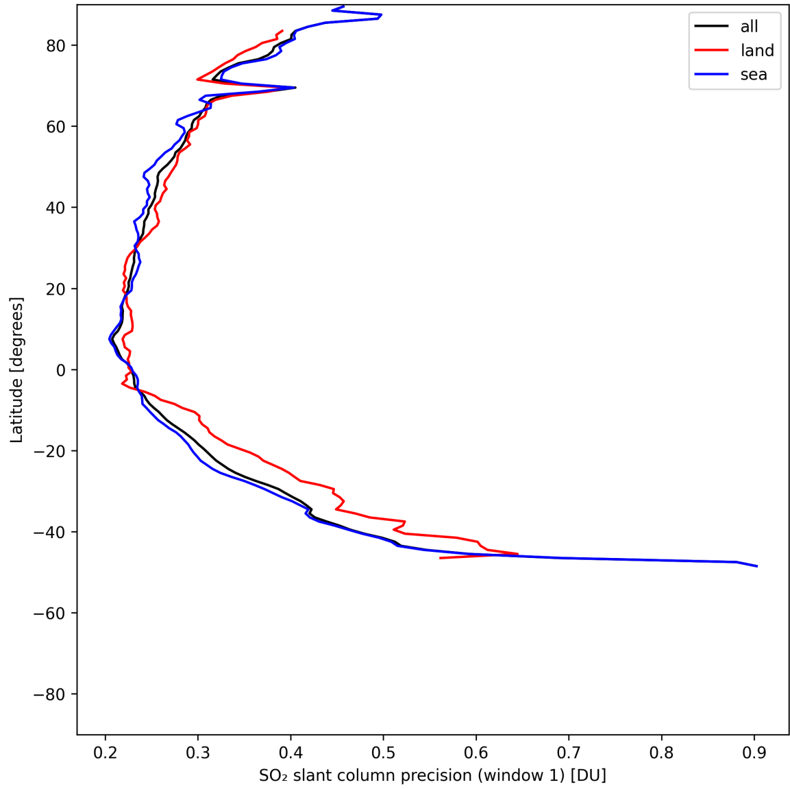
Figure 37: Zonal average of “SO 2 slant column precision (window 1)” for 2025-05-23 to 2025-05-24.
