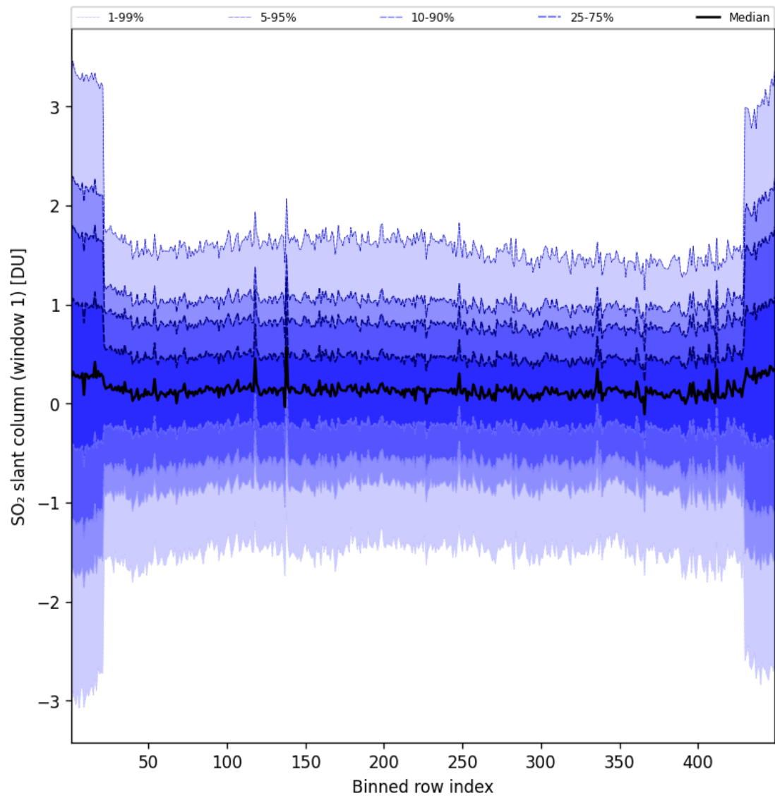
Figure 90: Along track statistics of “SO 2 slant column (window 1)” for 2025-05-23 to 2025-05-24
