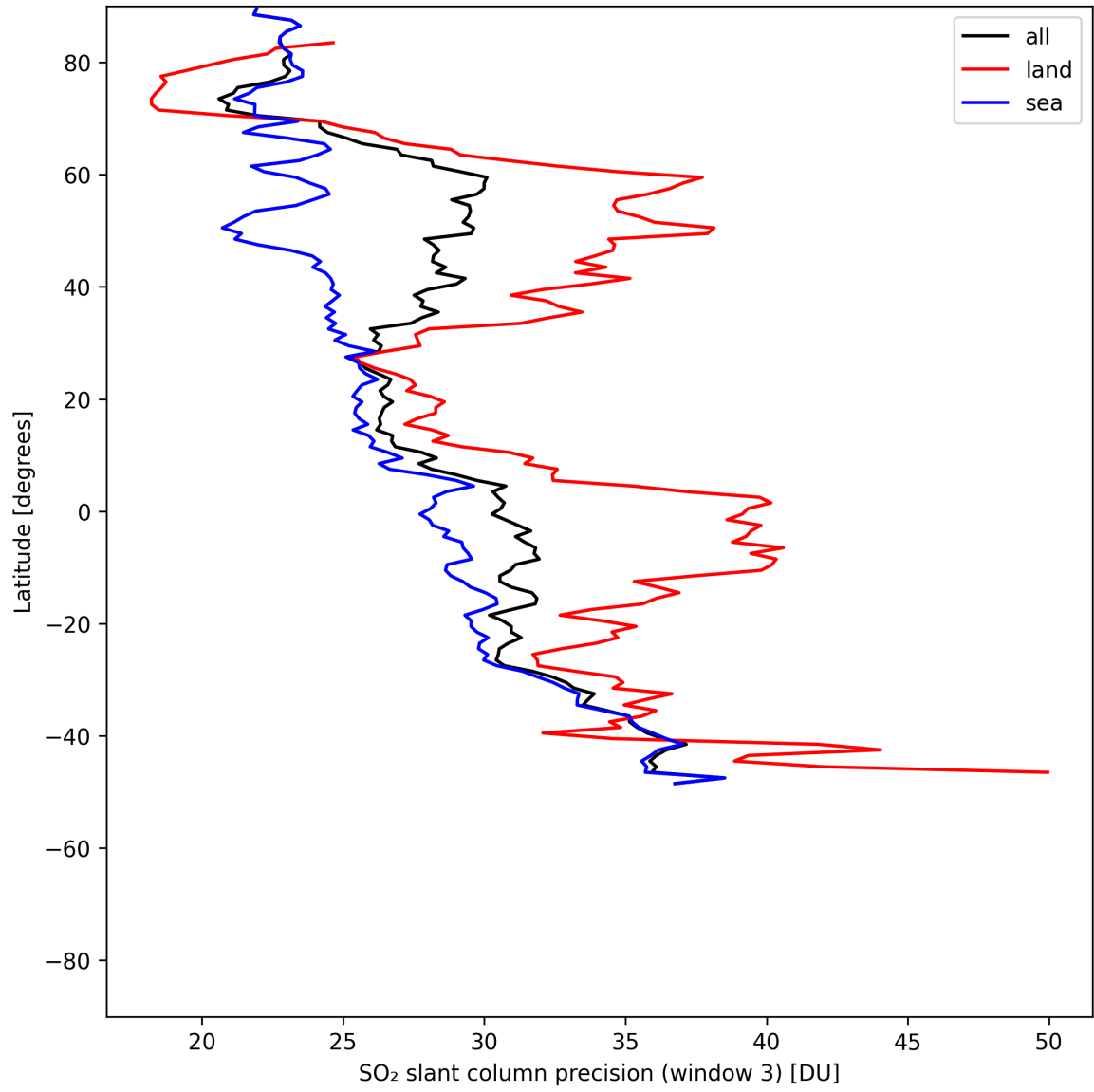
Figure 45: Zonal average of “SO 2 slant column precision (window 3)” for 2025-05-23 to 2025-05-24.
