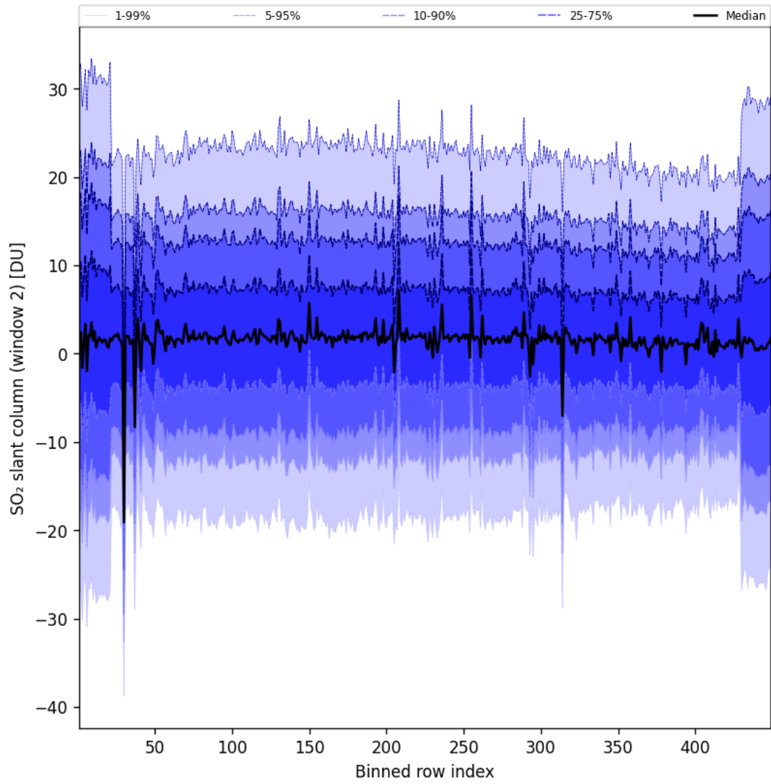
Figure 94: Along track statistics of “SO 2 slant column (window 2)” for 2025-05-24 to 2025-05-24
