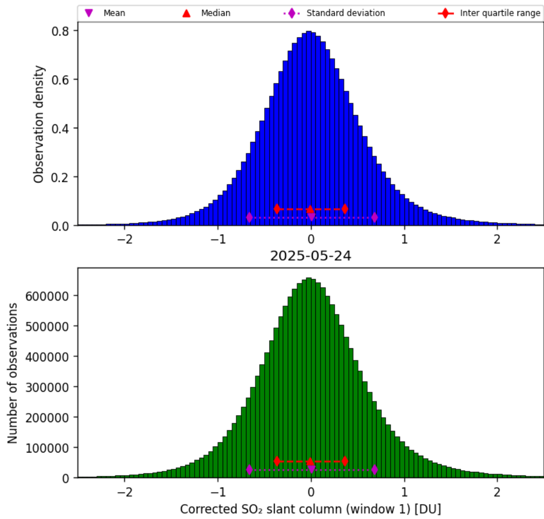
Figure 65: Histogram of “Corrected SO 2 slant column (window 1)” for 2025-05-24 to 2025-05-24
