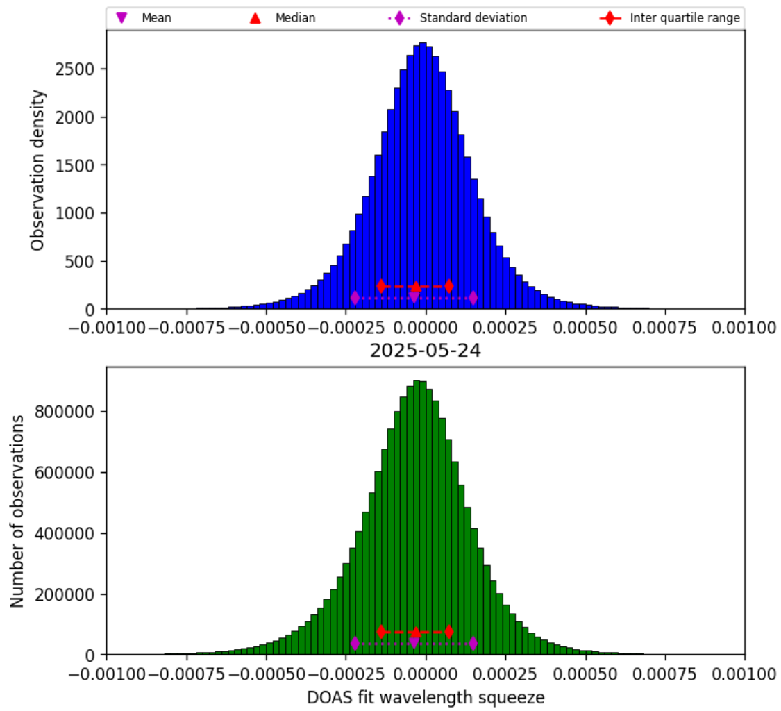
Figure 78: Histogram of "DOAS fit wavelength squeeze" for 2025-05-24 to 2025-05-24
