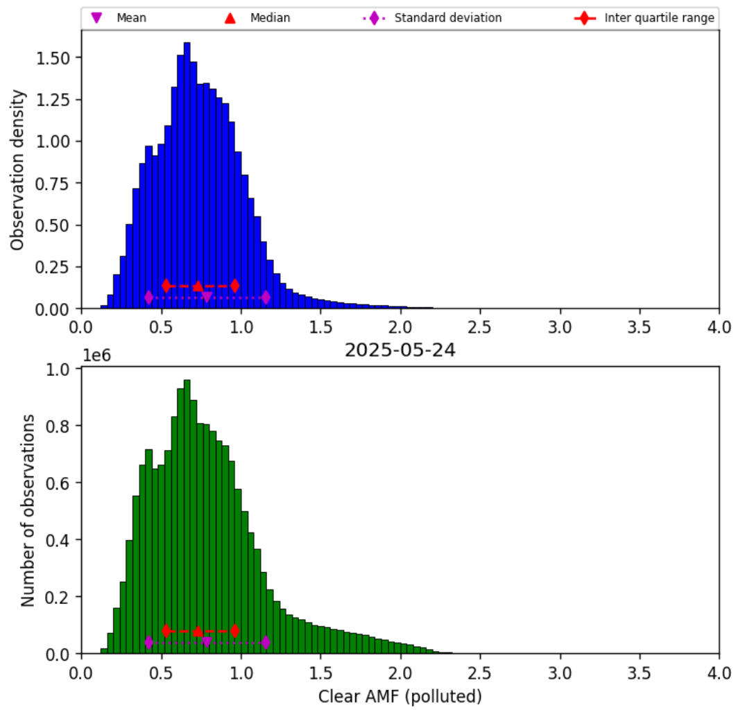
Figure 82: Histogram of “Clear AMF (polluted)” for 2025-05-24 to 2025-05-24
