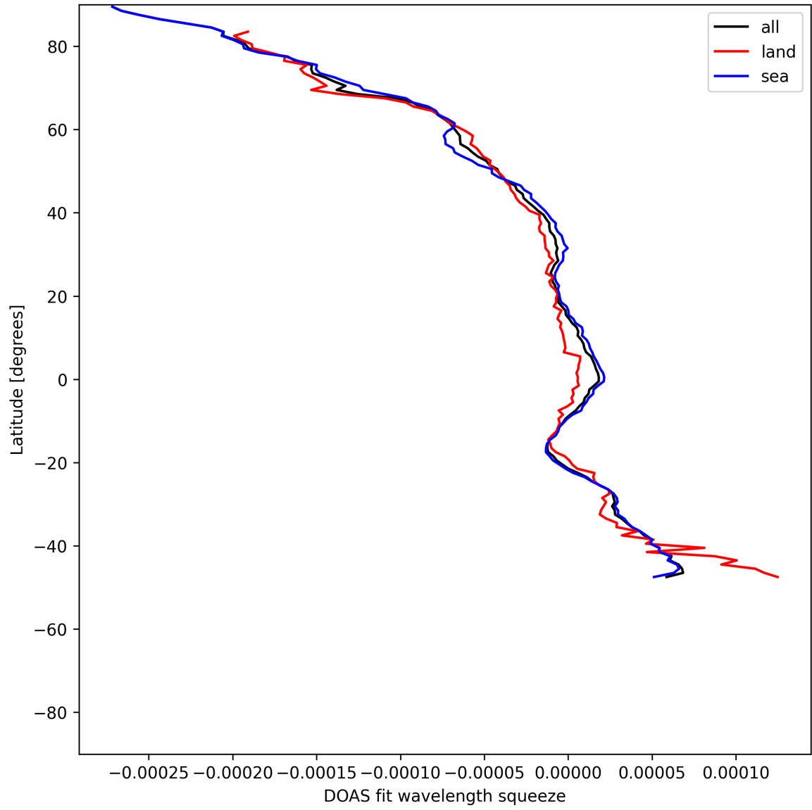
Figure 51: Zonal average of “DOAS fit wavelength squeeze” for 2025-05-24 to 2025-05-24.
