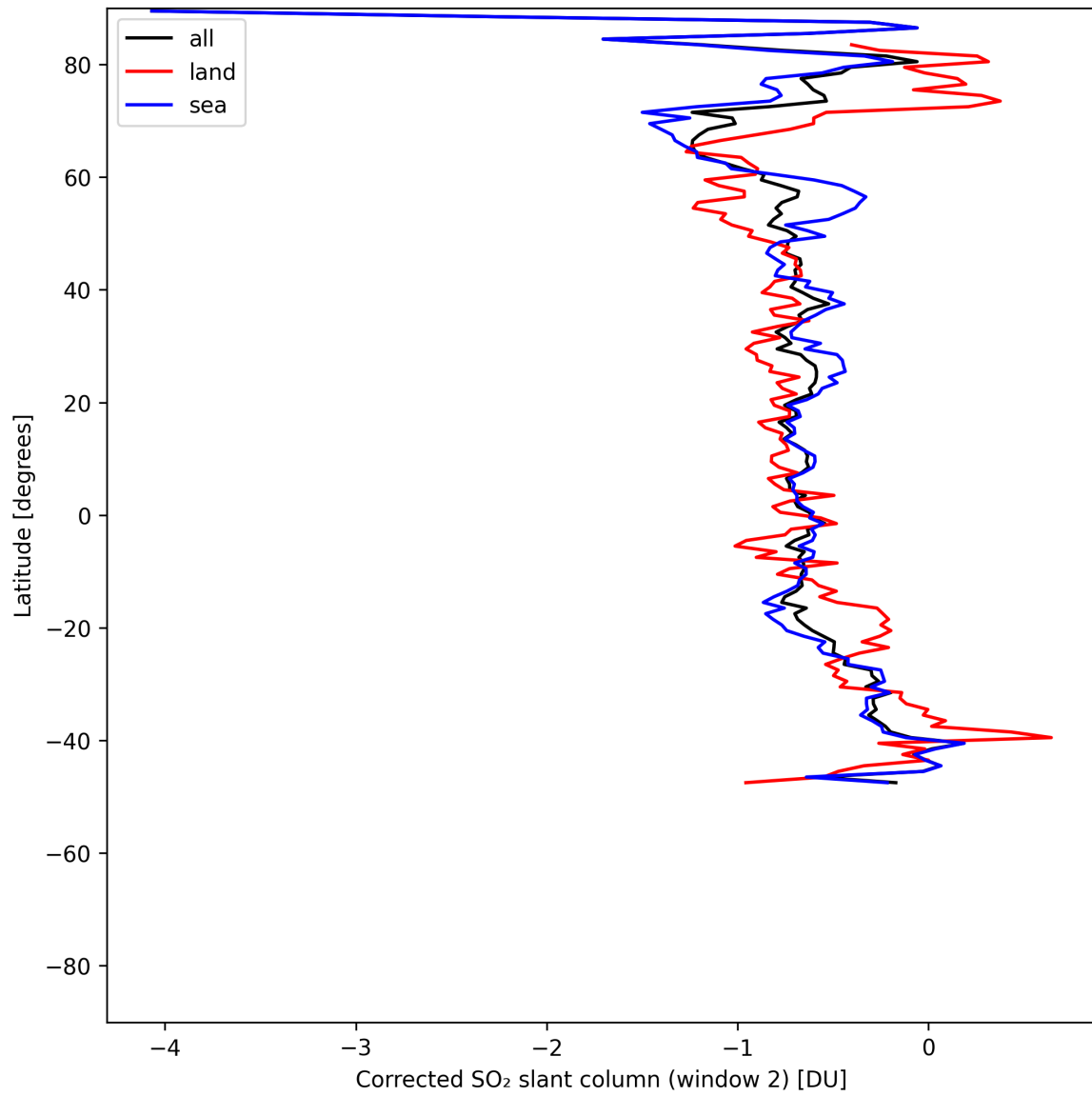
Figure 42: Zonal average of “Corrected SO 2 slant column (window 2)” for 2025-05-24 to 2025-05-24.
