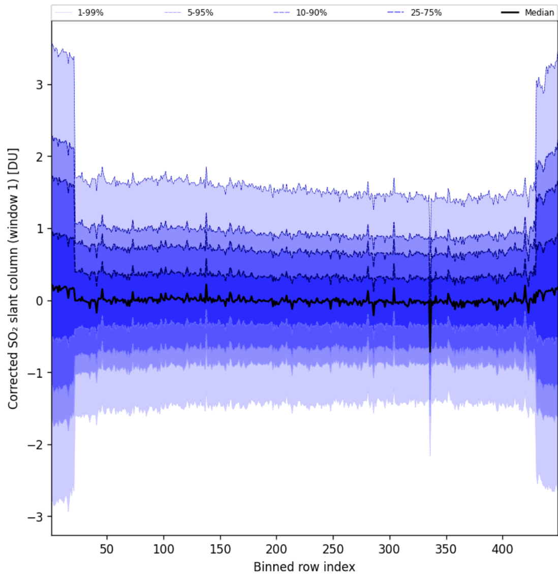
Figure 92: Along track statistics of “Corrected SO 2 slant column (window 1)” for 2025-05-24 to 2025-05-24
