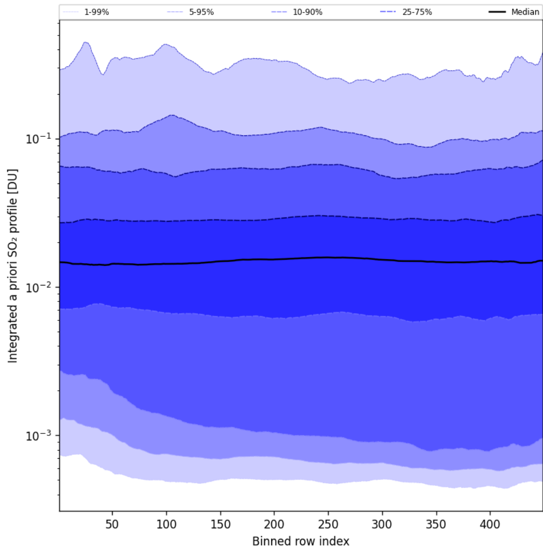
Figure 103: Along track statistics of “Integrated a priori SO 2 profile” for 2025-05-24 to 2025-05-24
