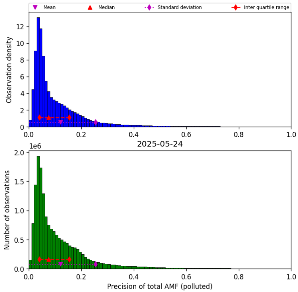
Figure 81: Histogram of “Precision of total AMF (polluted)” for 2025-05-24 to 2025-05-24
