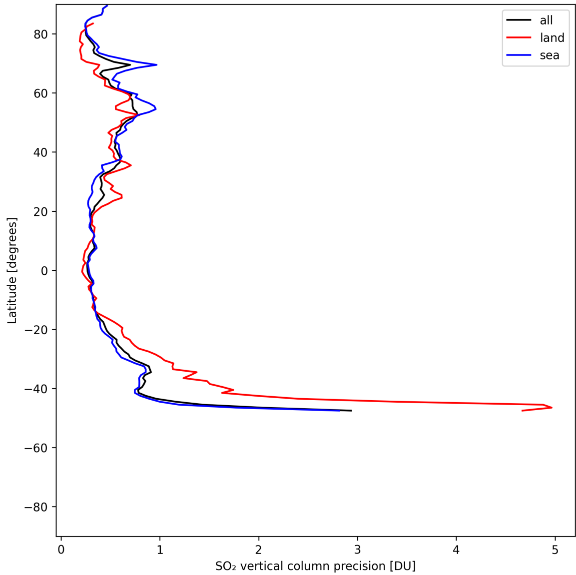
Figure 32: Zonal average of “SO 2 vertical column precision” for 2025-05-24 to 2025-05-24.
