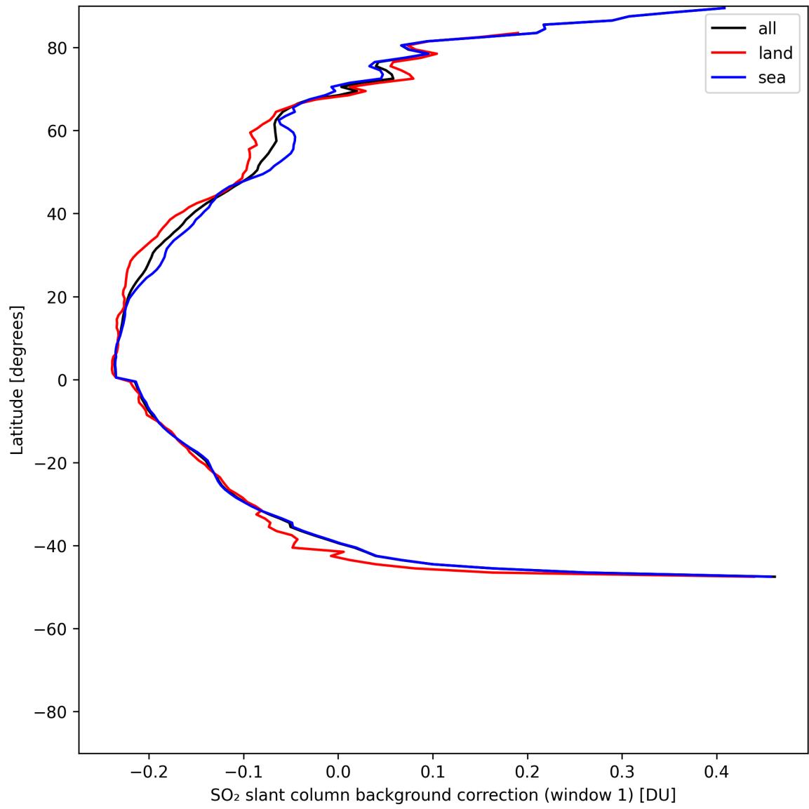
Figure 39: Zonal average of “SO 2 slant column background correction (window 1)” for 2025-05-24 to 2025-05-24.
