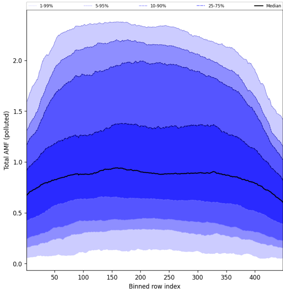
Figure 107: Along track statistics of “Total AMF (polluted)” for 2025-05-24 to 2025-05-24
