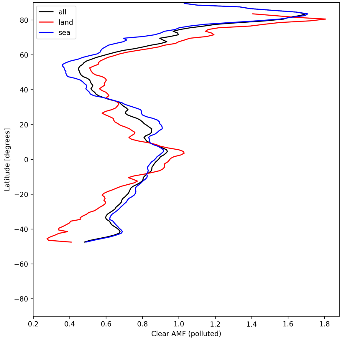
Figure 55: Zonal average of “Clear AMF (polluted)” for 2025-05-24 to 2025-05-24.
