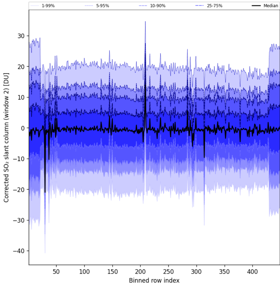
Figure 96: Along track statistics of “Corrected SO 2 slant column (window 2)” for 2025-05-24 to 2025-05-24
