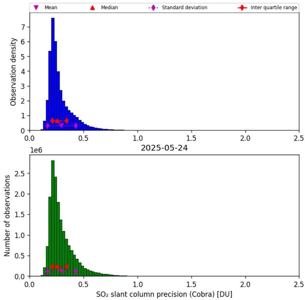
Figure 62: Histogram of “SO 2 slant column precision (Cobra)” for 2025-05-24 to 2025-05-24
