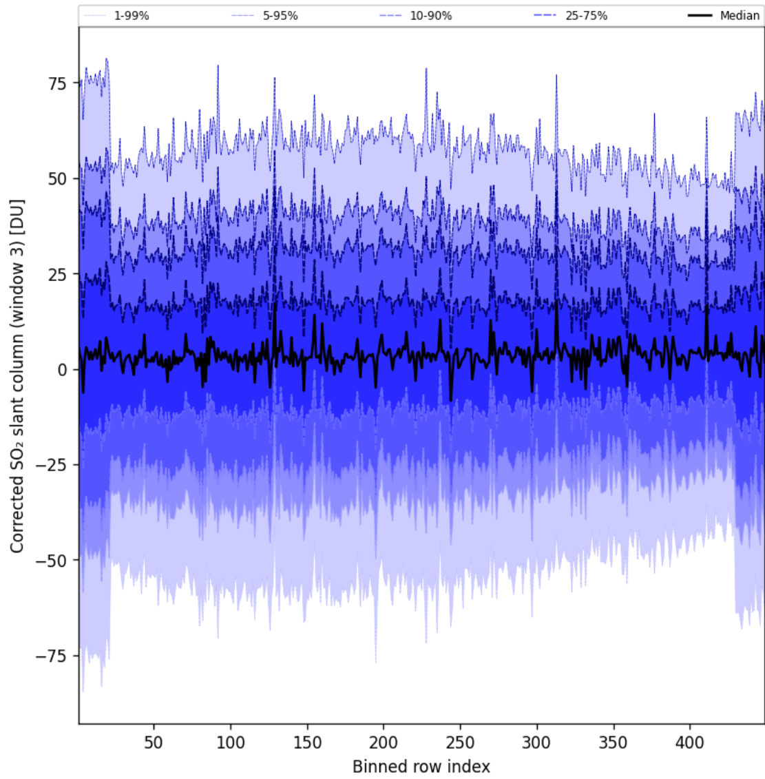
Figure 100: Along track statistics of “Corrected SO 2 slant column (window 3)” for 2025-05-24 to 2025-05-24
