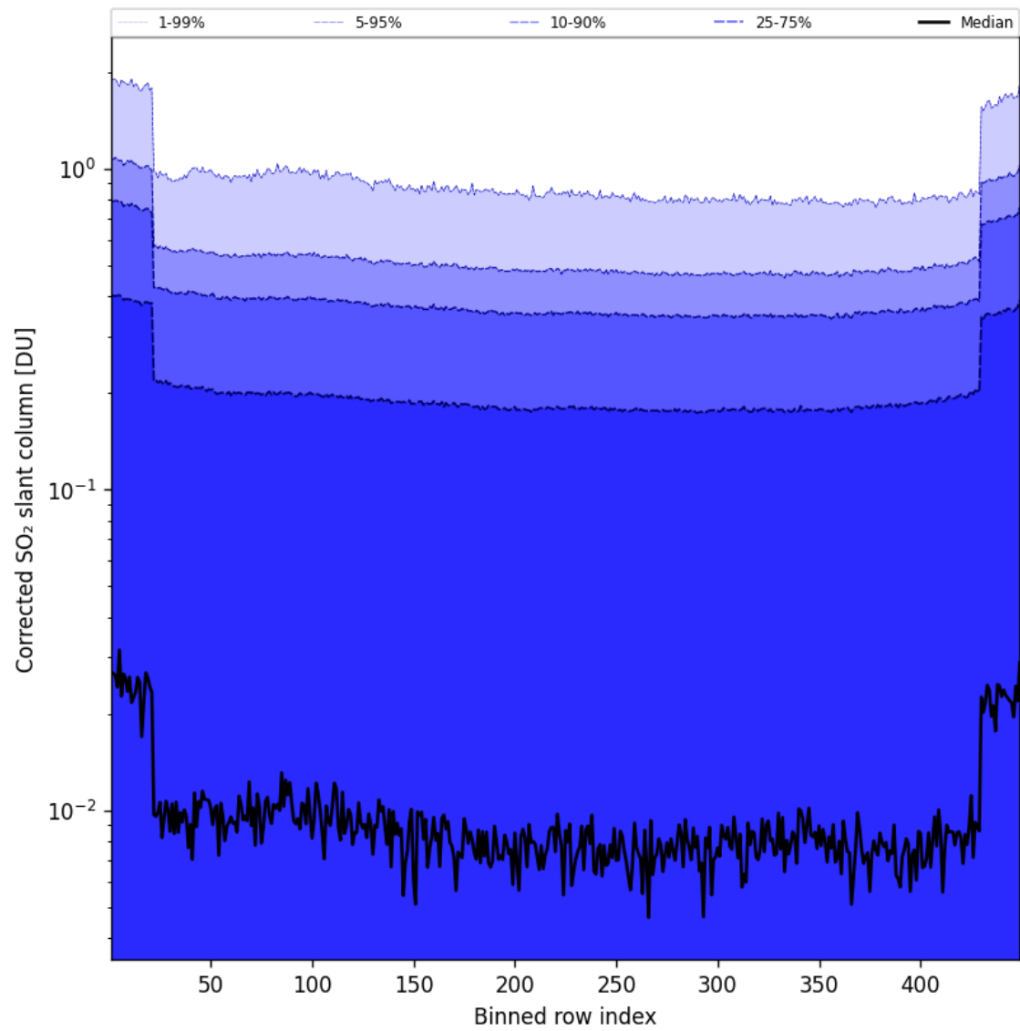
Figure 87: Along track statistics of “Corrected SO 2 slant column” for 2025-05-24 to 2025-05-24
