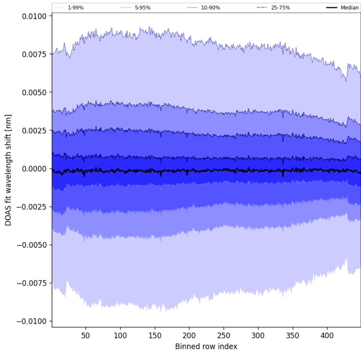
Figure 104: Along track statistics of “DOAS fit wavelength shift” for 2025-05-24 to 2025-05-24
