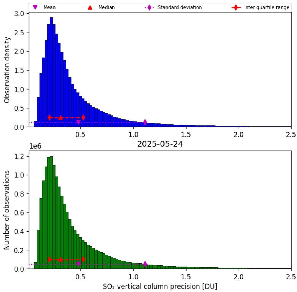
Figure 59: Histogram of "SO 2 vertical column precision" for 2025-05-24 to 2025-05-24
