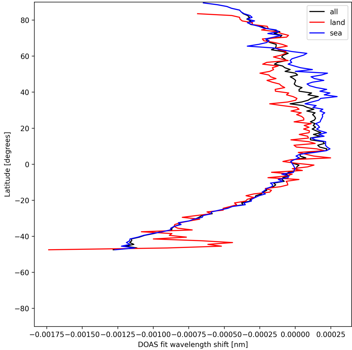
Figure 50: Zonal average of “DOAS fit wavelength shift” for 2025-05-24 to 2025-05-24.
