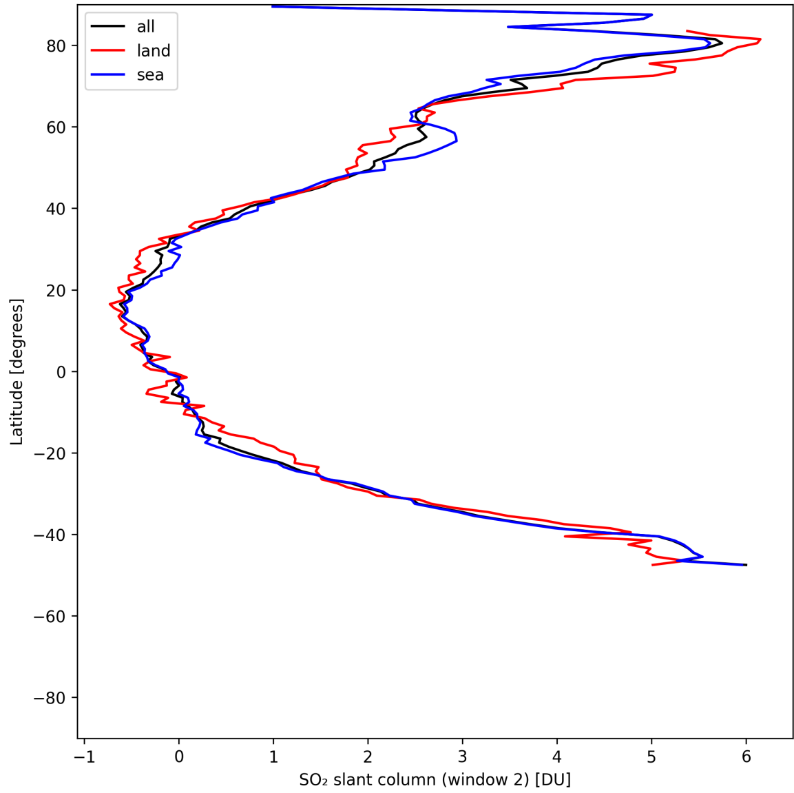
Figure 40: Zonal average of “SO 2 slant column (window 2)” for 2025-05-24 to 2025-05-24.
