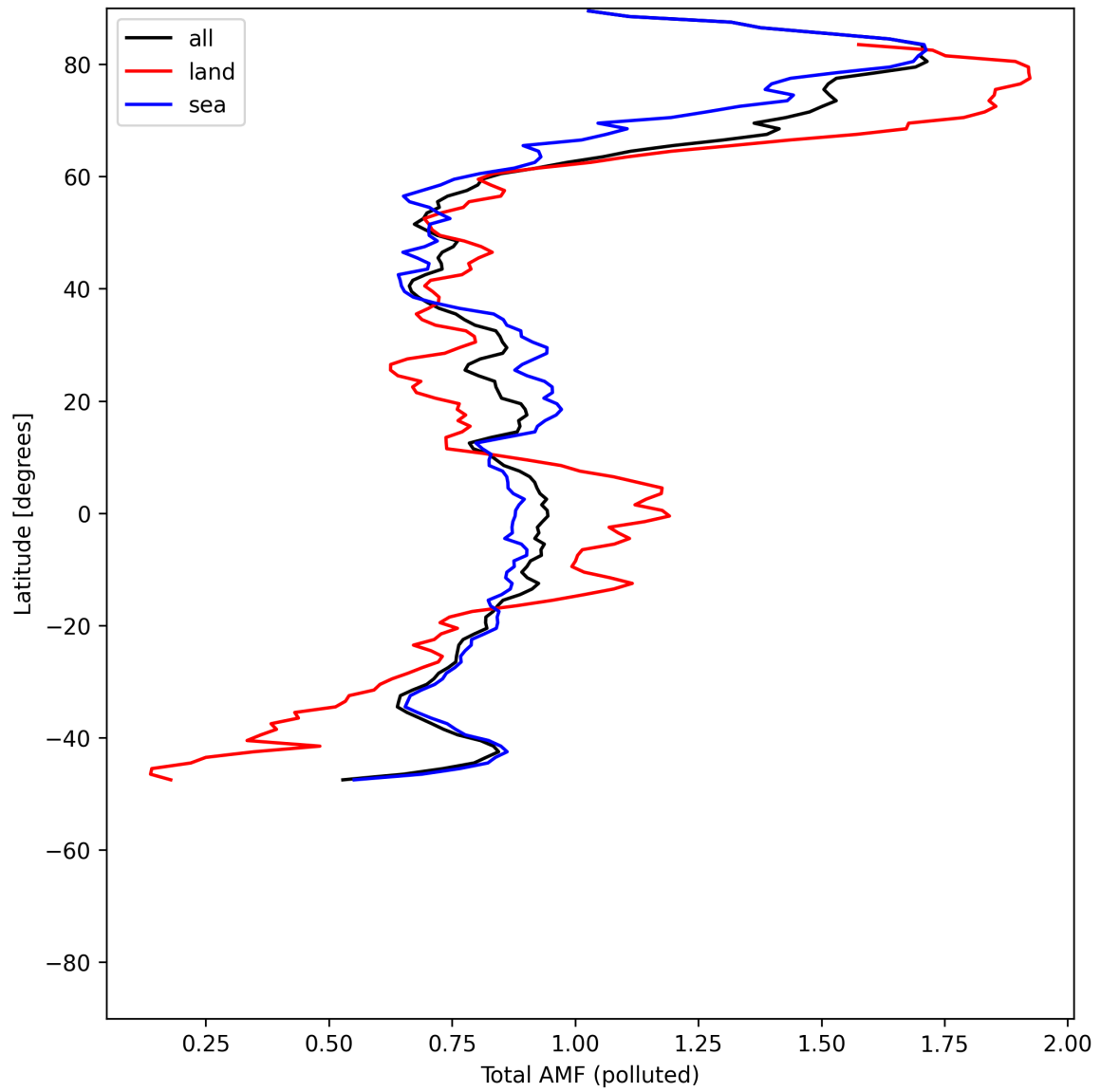
Figure 53: Zonal average of “Total AMF (polluted)” for 2025-05-24 to 2025-05-24.
