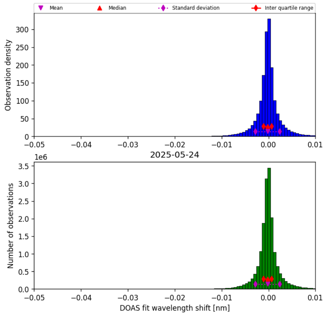
Figure 77: Histogram of “DOAS fit wavelength shift” for 2025-05-24 to 2025-05-24
