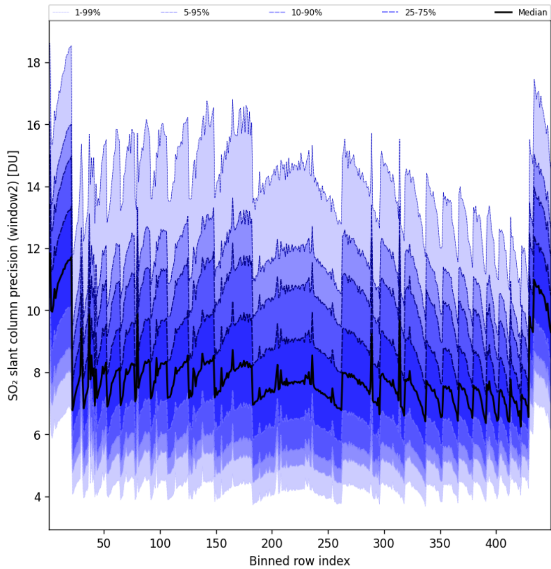
Figure 95: Along track statistics of “SO 2 slant column precision (window2)” for 2025-05-24 to 2025-05-24
