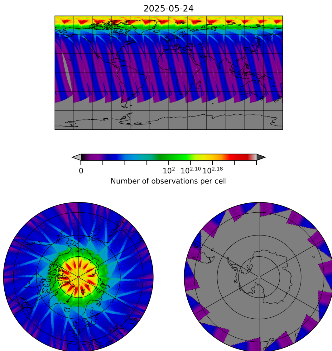
Figure 29: Map of the number of observations for 2025-05-24 to 2025-05-24
