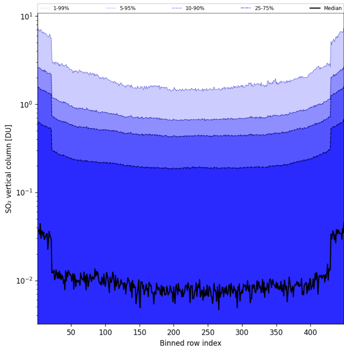
Figure 85: Along track statistics of “SO 2 vertical column” for 2025-05-24 to 2025-05-24
