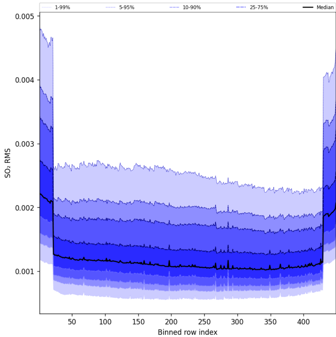
Figure 106: Along track statistics of “SO 2 RMS” for 2025-05-24 to 2025-05-24
