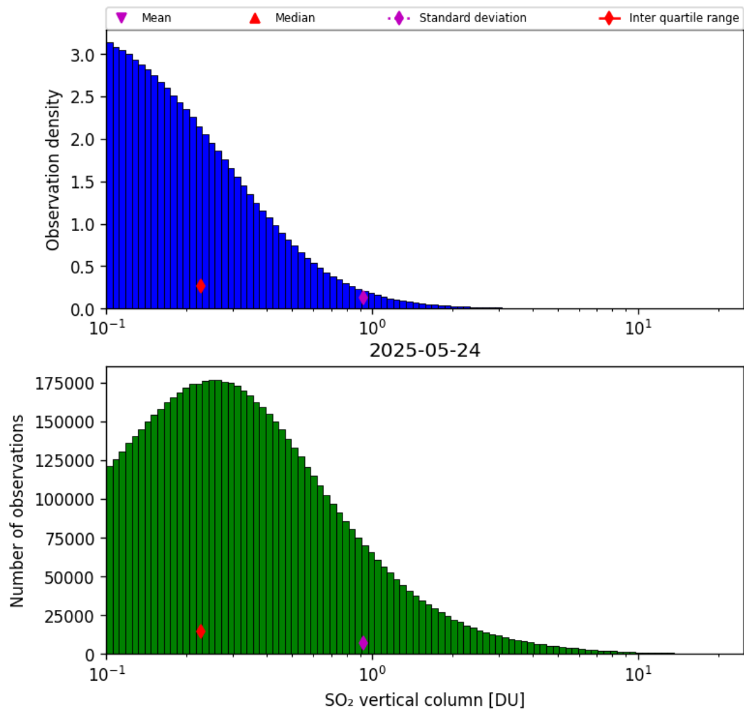
Figure 58: Histogram of “SO 2 vertical column” for 2025-05-24 to 2025-05-24
