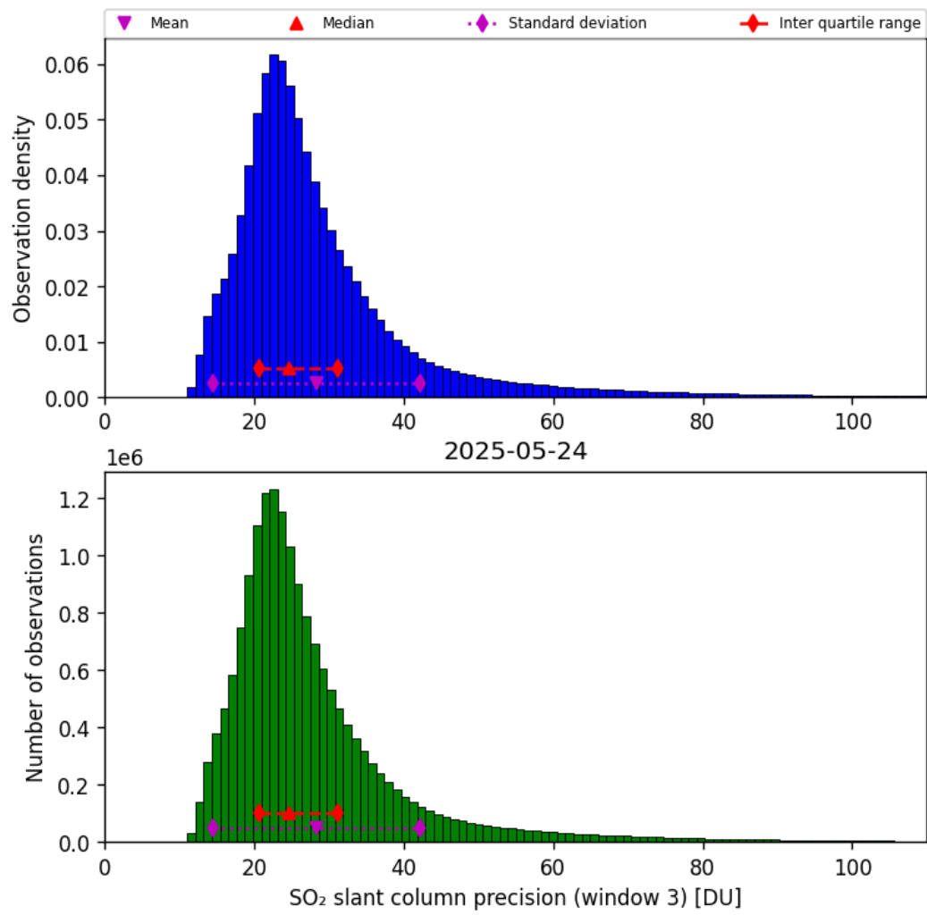
Figure 72: Histogram of “SO 2 slant column precision (window 3)” for 2025-05-24 to 2025-05-24
