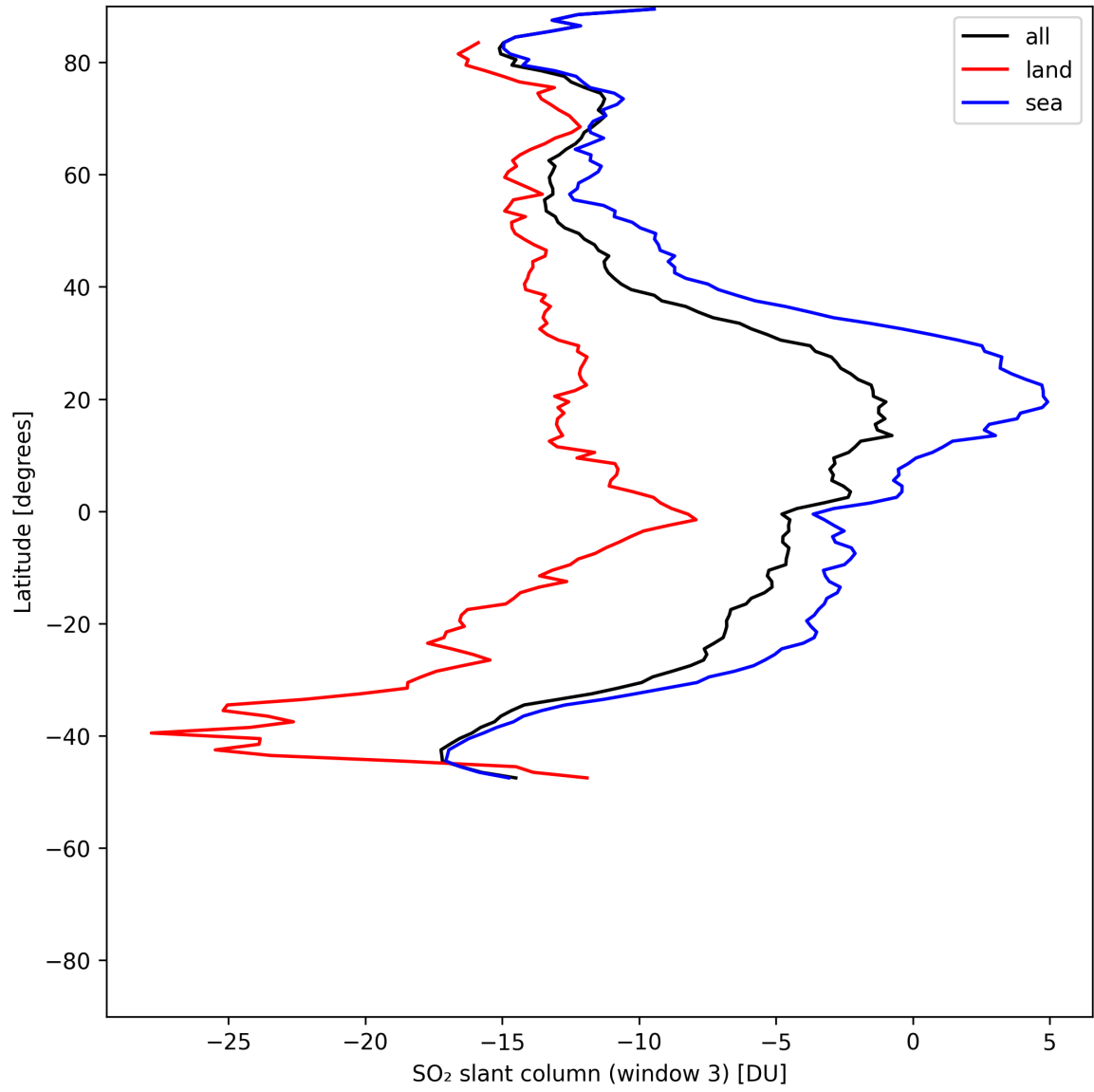
Figure 44: Zonal average of “SO 2 slant column (window 3)” for 2025-05-24 to 2025-05-24.
