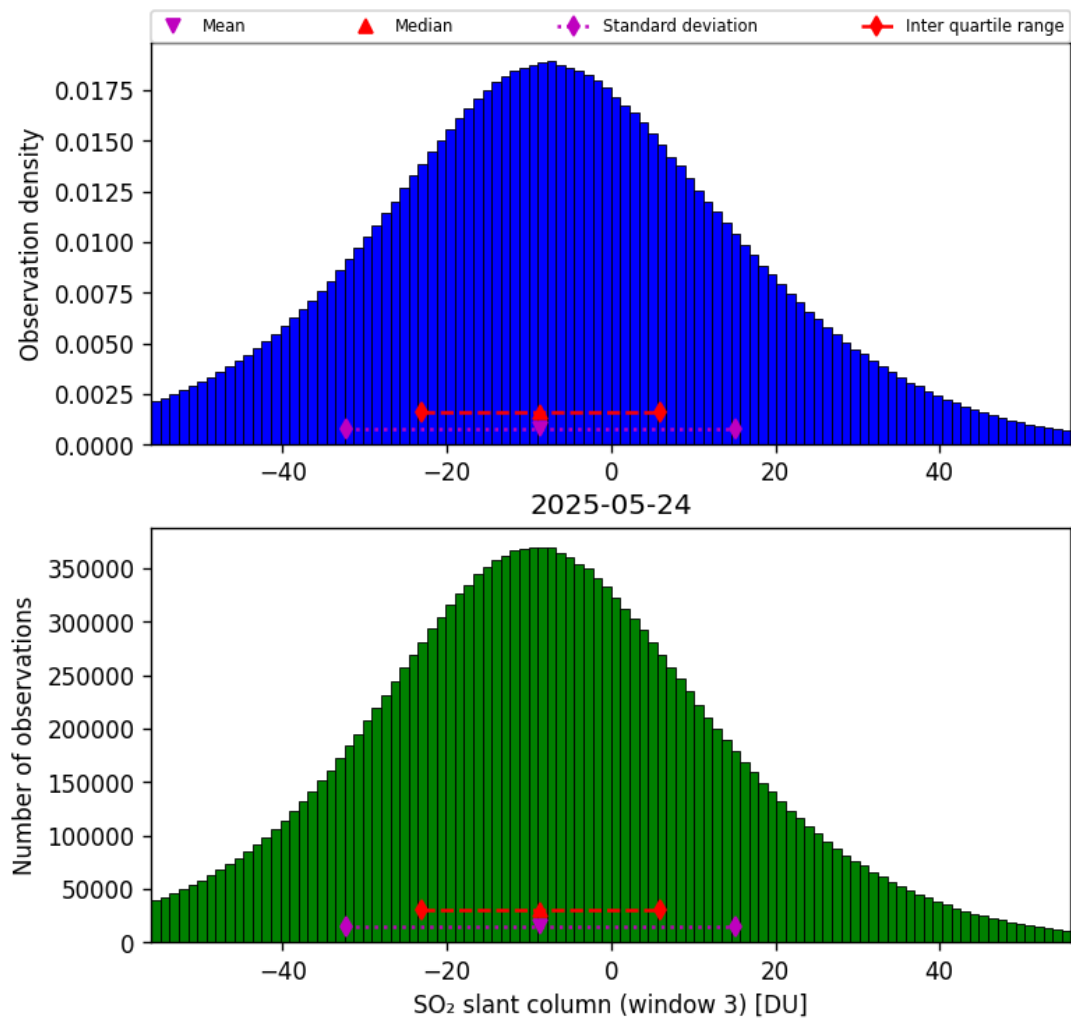
Figure 71: Histogram of “SO 2 slant column (window 3)” for 2025-05-24 to 2025-05-24
