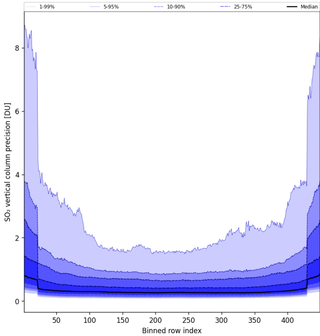
Figure 86: Along track statistics of “SO 2 vertical column precision” for 2025-05-24 to 2025-05-24
