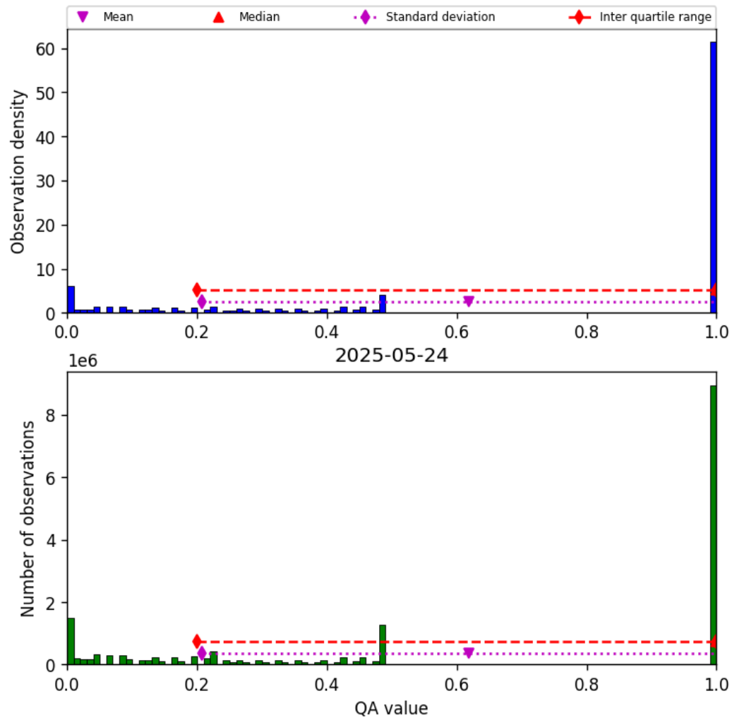
Figure 57: Histogram of “QA value” for 2025-05-24 to 2025-05-24
