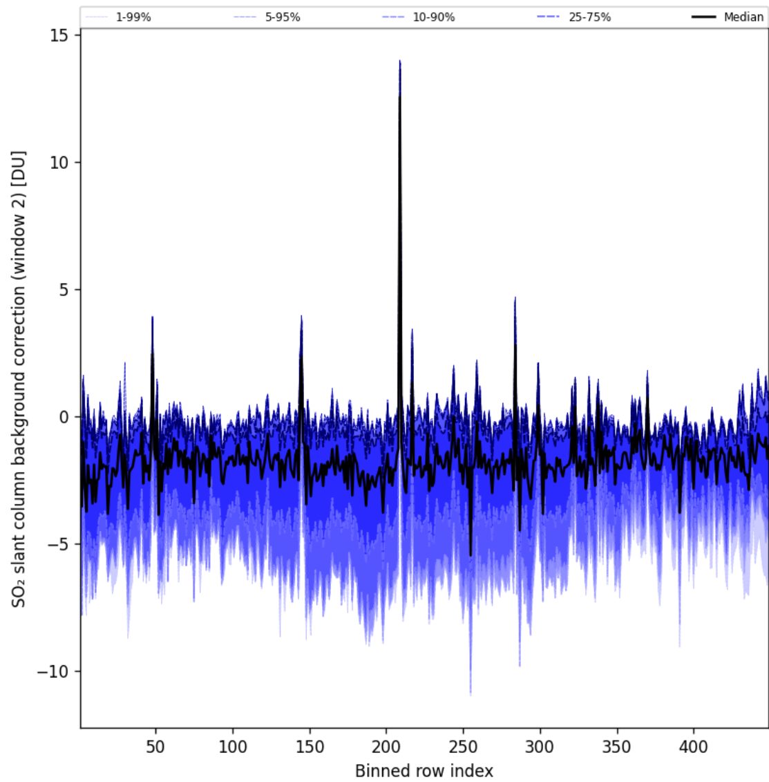
Figure 97: Along track statistics of “SO 2 slant column background correction (window 2)” for 2025-05-24 to 2025-05-24
