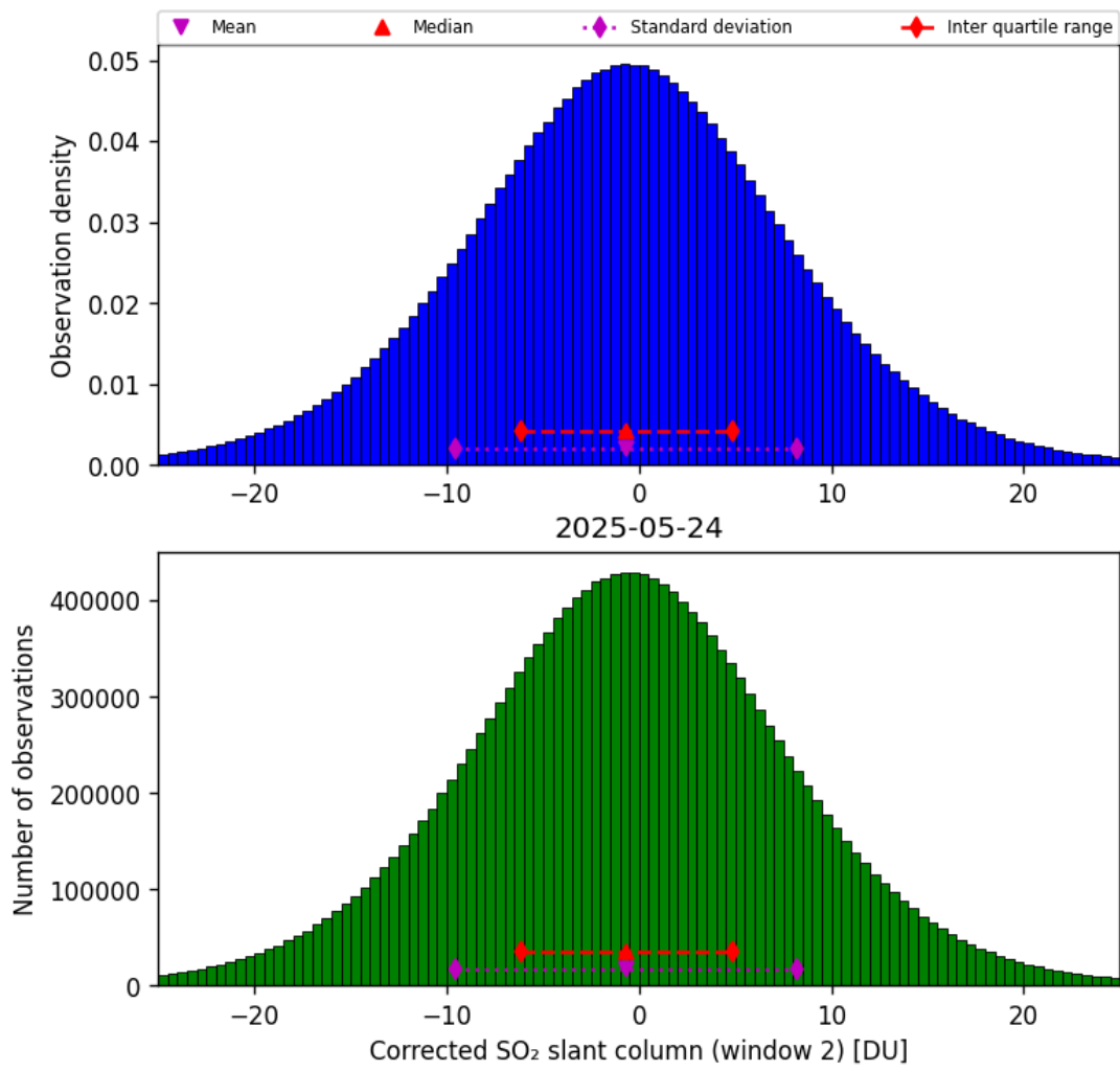
Figure 69: Histogram of “Corrected SO 2 slant column (window 2)” for 2025-05-24 to 2025-05-24
