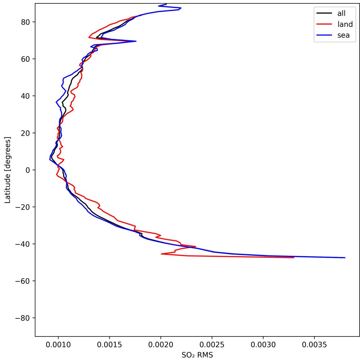
Figure 52: Zonal average of “SO 2 RMS” for 2025-05-24 to 2025-05-24.
