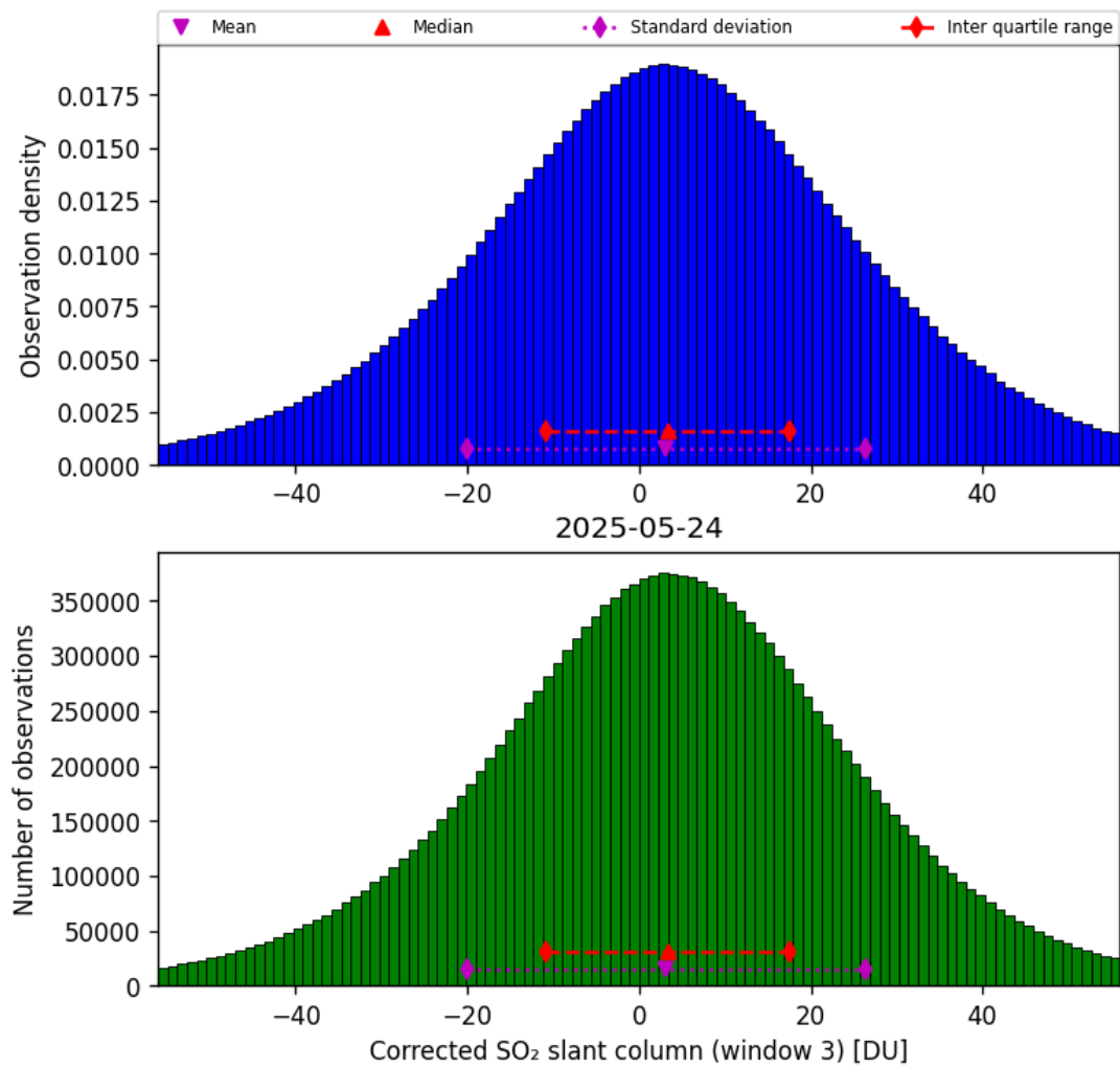
Figure 73: Histogram of “Corrected SO 2 slant column (window 3)” for 2025-05-24 to 2025-05-24
