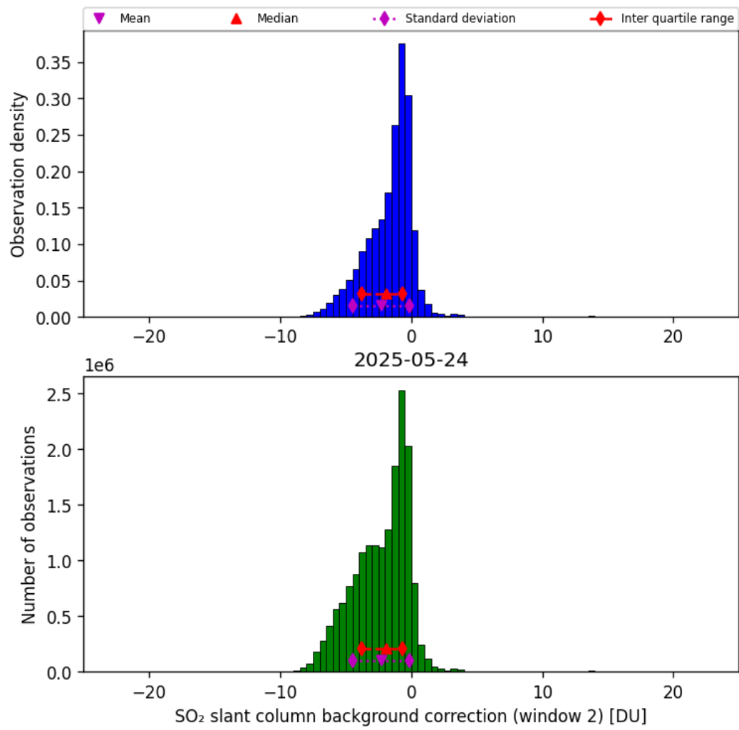
Figure 70: Histogram of “SO 2 slant column background correction (window 2)” for 2025-05-24 to 2025-05-24
