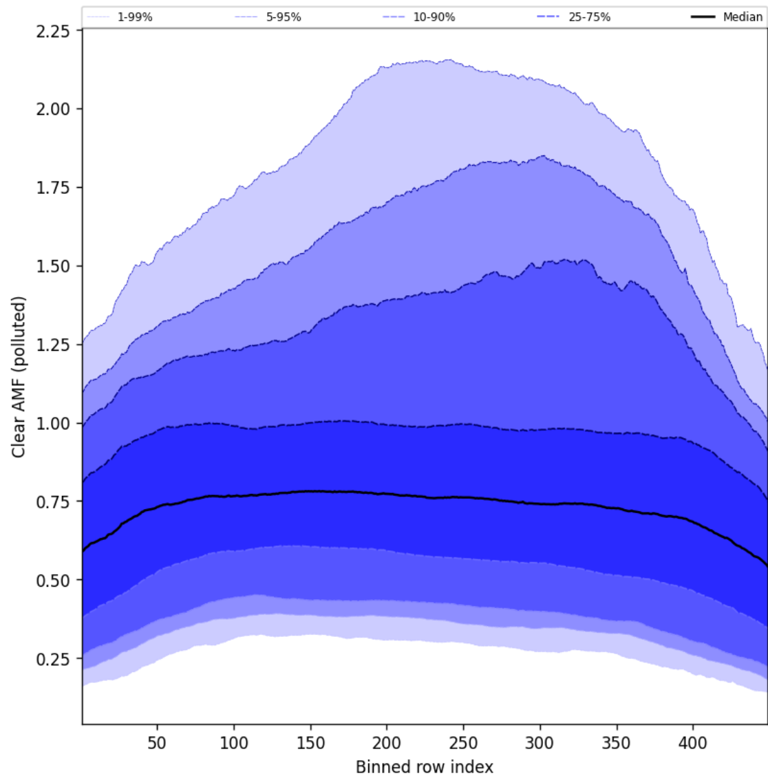
Figure 109: Along track statistics of “Clear AMF (polluted)” for 2025-05-24 to 2025-05-24
