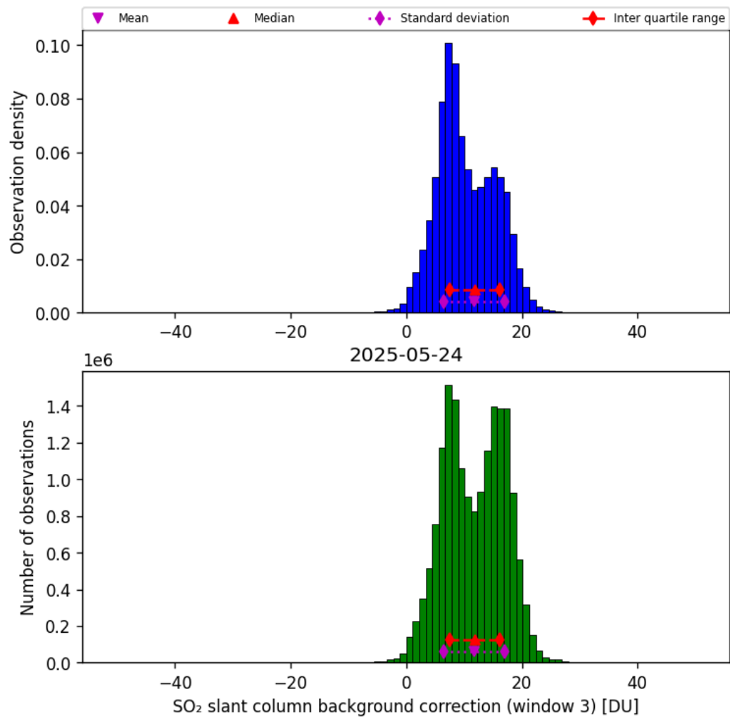
Figure 74: Histogram of “SO 2 slant column background correction (window 3)” for 2025-05-24 to 2025-05-24
