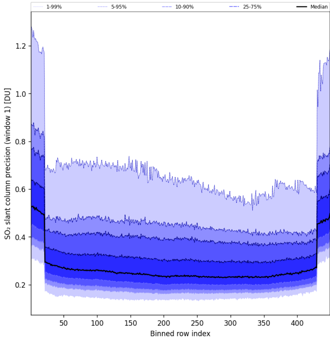
Figure 91: Along track statistics of “SO 2 slant column precision (window 1)” for 2025-05-24 to 2025-05-24
