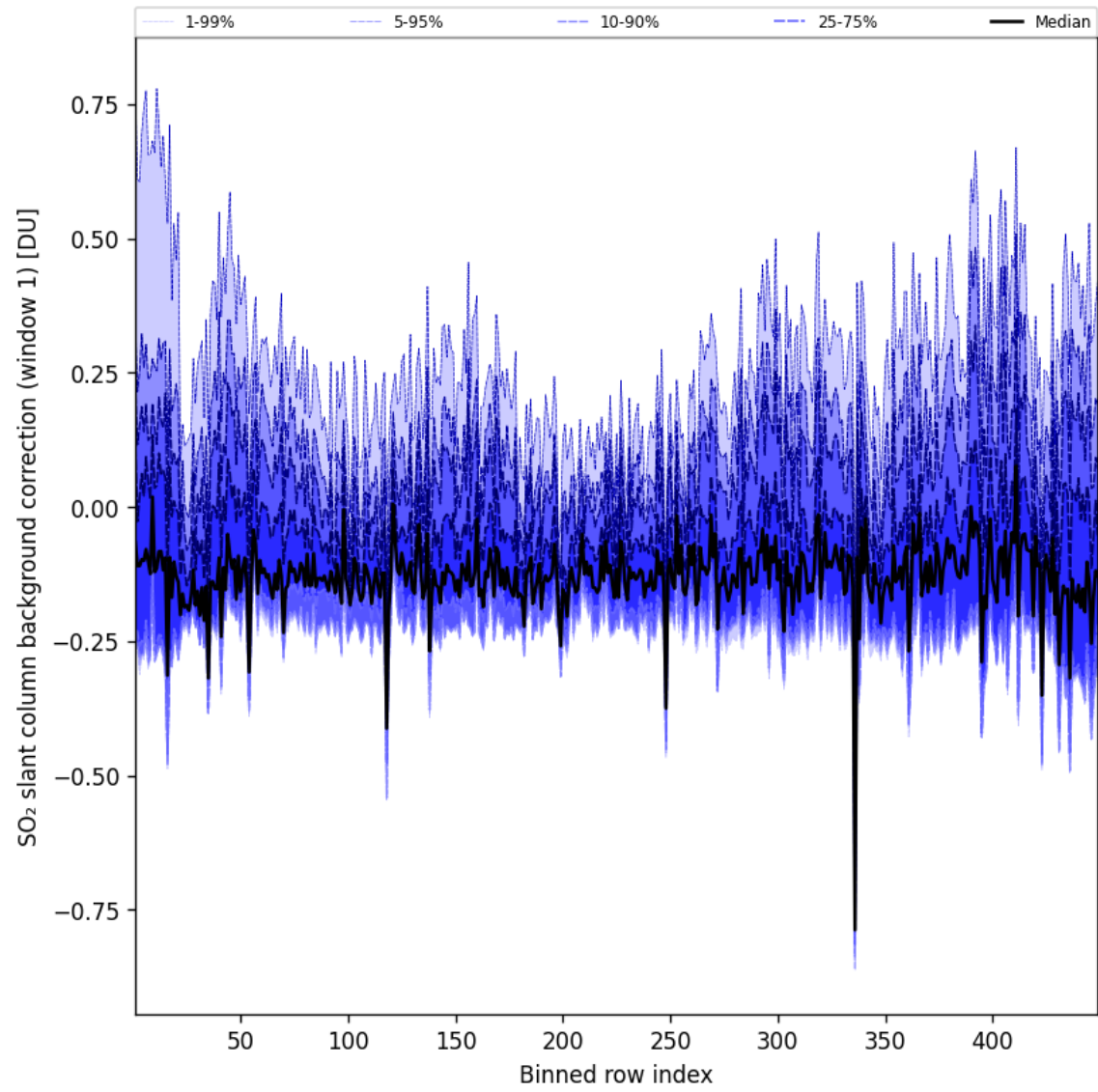
Figure 93: Along track statistics of “SO 2 slant column background correction (window 1)” for 2025-05-24 to 2025-05-24
