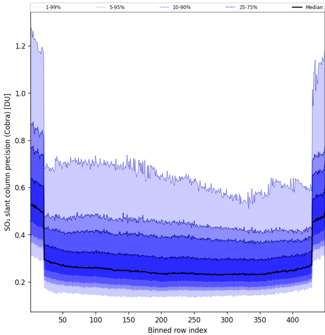
Figure 89: Along track statistics of “SO 2 slant column precision (Cobra)” for 2025-05-24 to 2025-05-24
