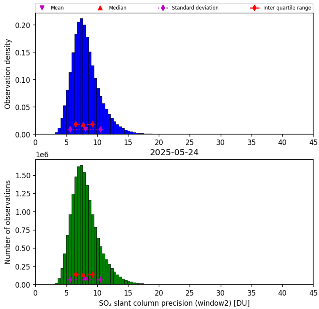
Figure 68: Histogram of “SO 2 slant column precision (window2)” for 2025-05-24 to 2025-05-24
