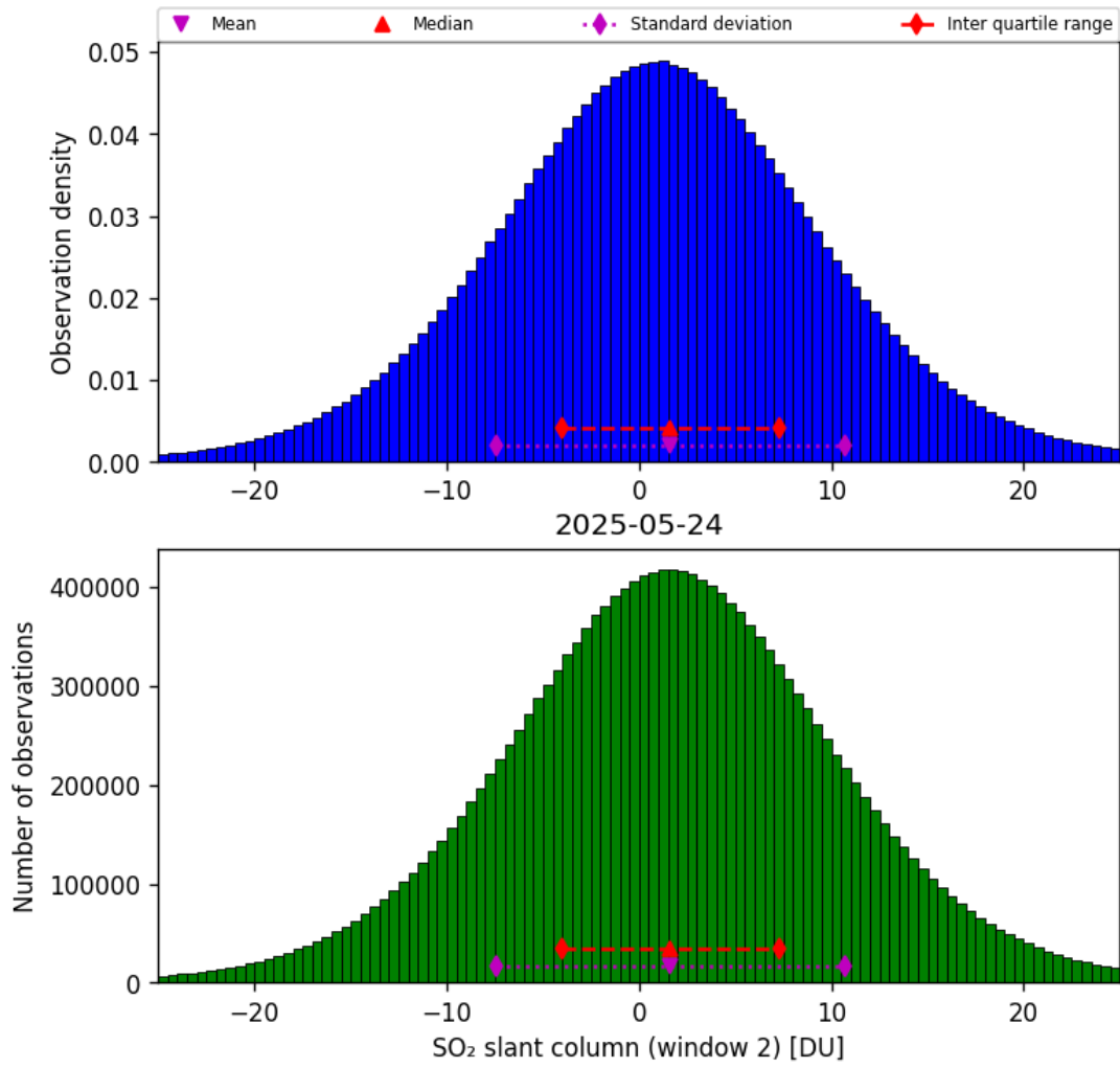
Figure 67: Histogram of “SO 2 slant column (window 2)” for 2025-05-24 to 2025-05-24
