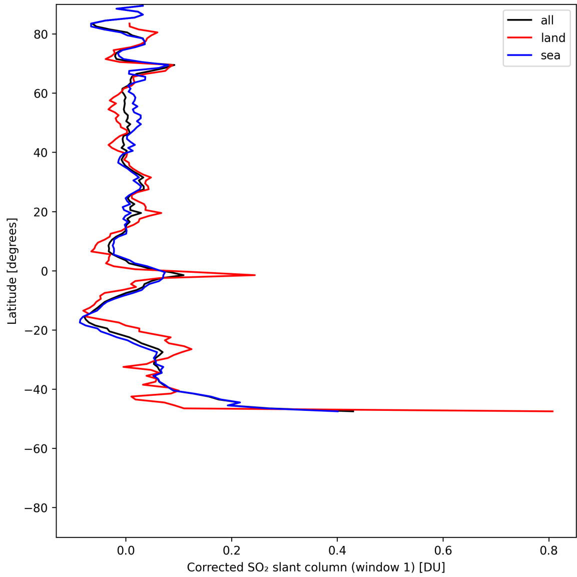
Figure 38: Zonal average of “Corrected SO 2 slant column (window 1)” for 2025-05-24 to 2025-05-24.
