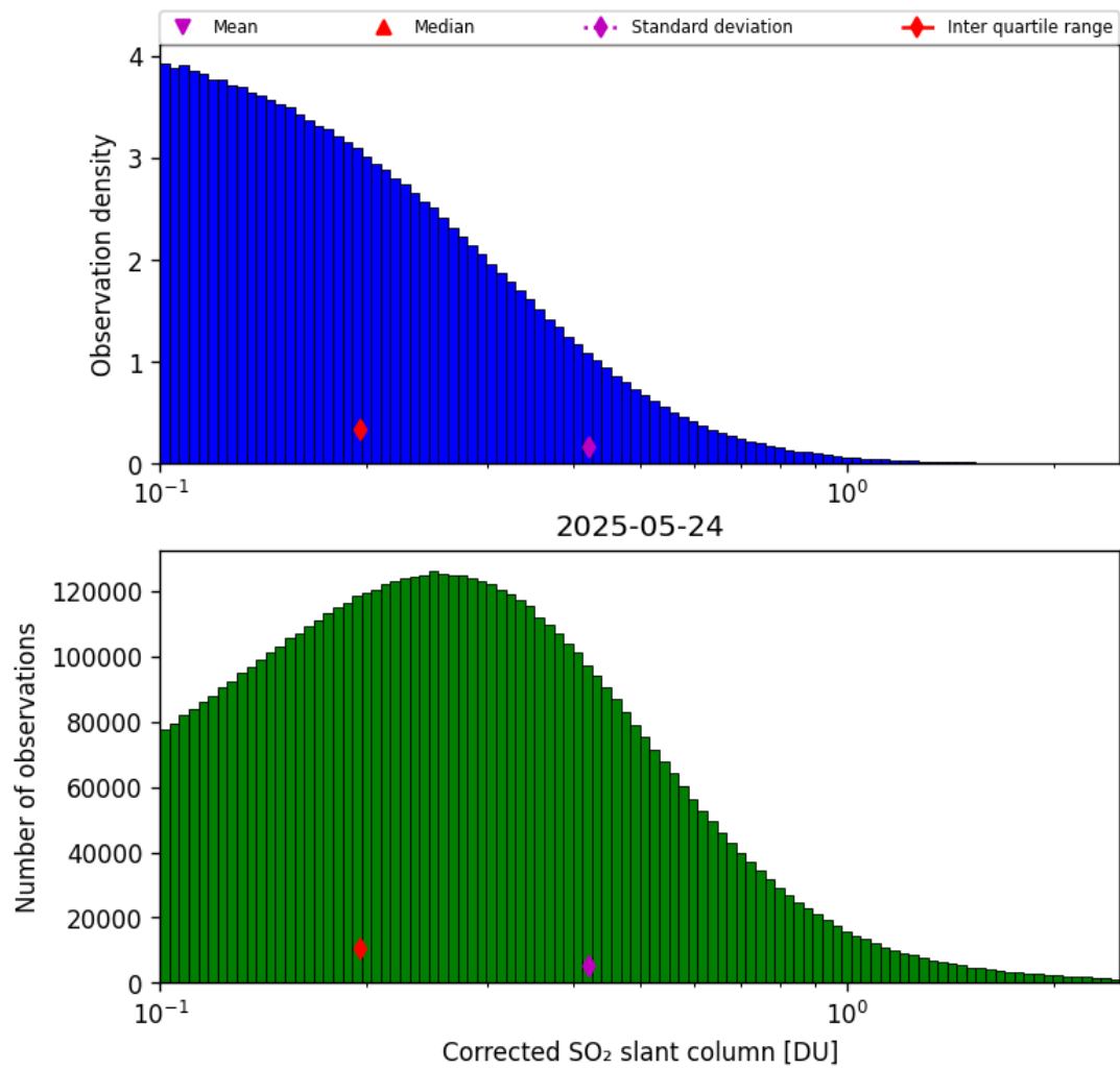
Figure 60: Histogram of “Corrected SO 2 slant column” for 2025-05-24 to 2025-05-24
