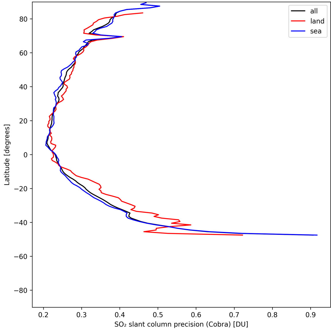
Figure 35: Zonal average of “SO 2 slant column precision (Cobra)” for 2025-05-24 to 2025-05-24.
