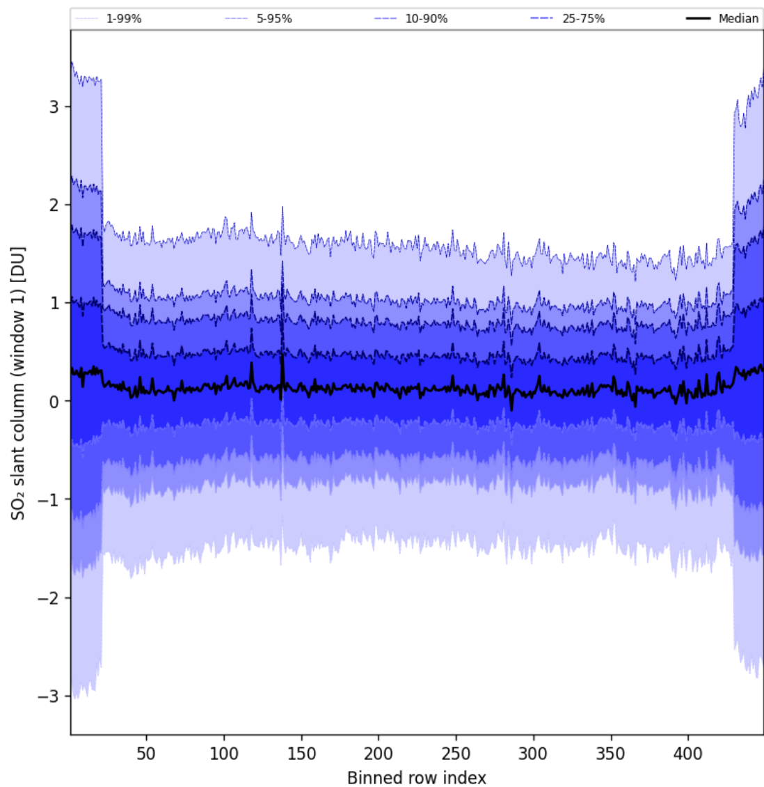
Figure 90: Along track statistics of “SO 2 slant column (window 1)” for 2025-05-24 to 2025-05-24
