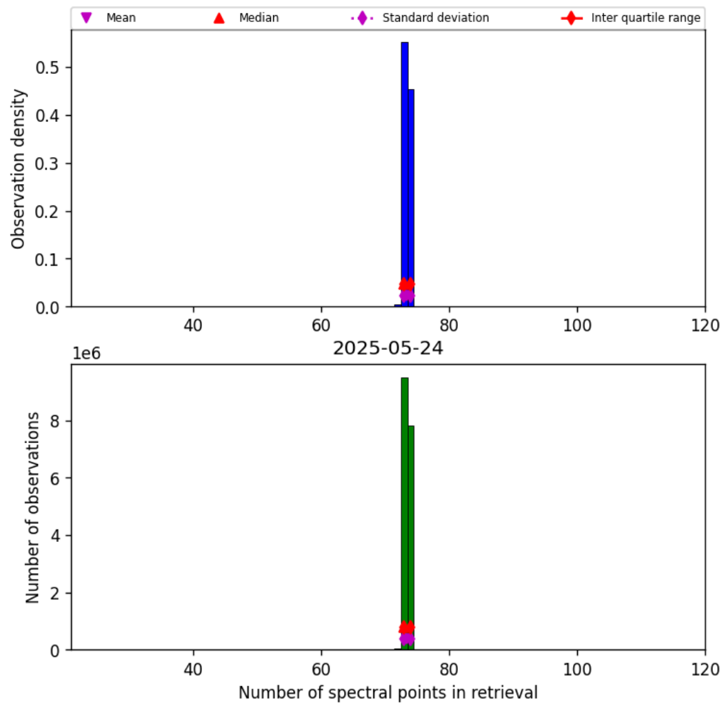
Figure 83: Histogram of “Number of spectral points in retrieval” for 2025-05-24 to 2025-05-24
