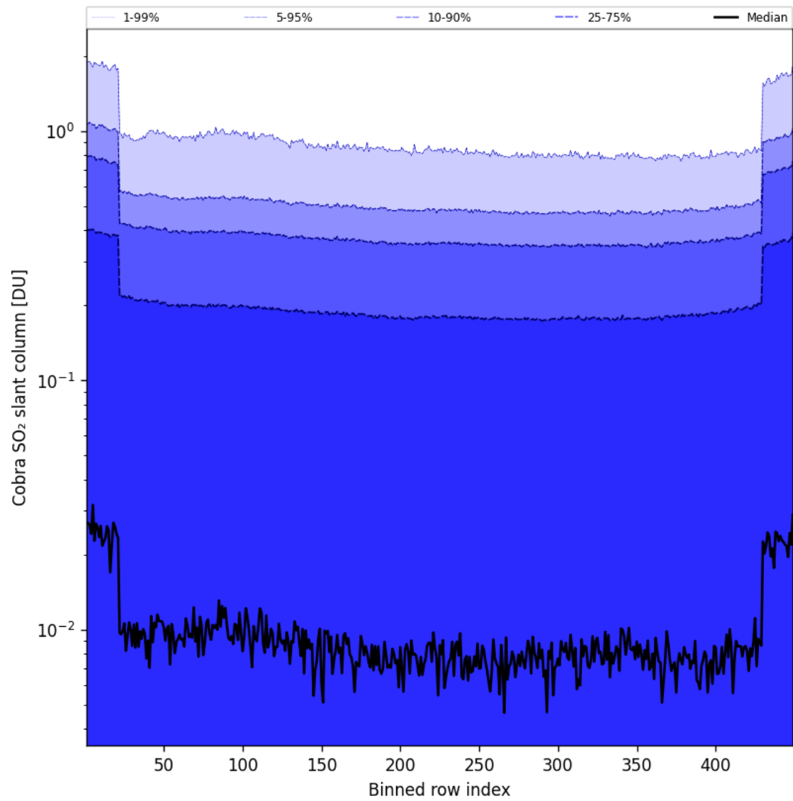
Figure 88: Along track statistics of “Cobra SO 2 slant column” for 2025-05-24 to 2025-05-24
