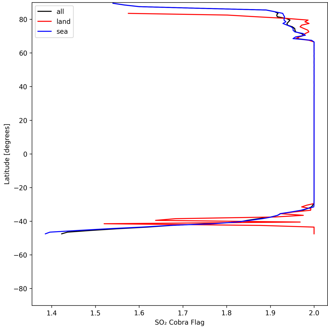
Figure 48: Zonal average of “SO 2 Cobra Flag” for 2025-05-24 to 2025-05-24.
