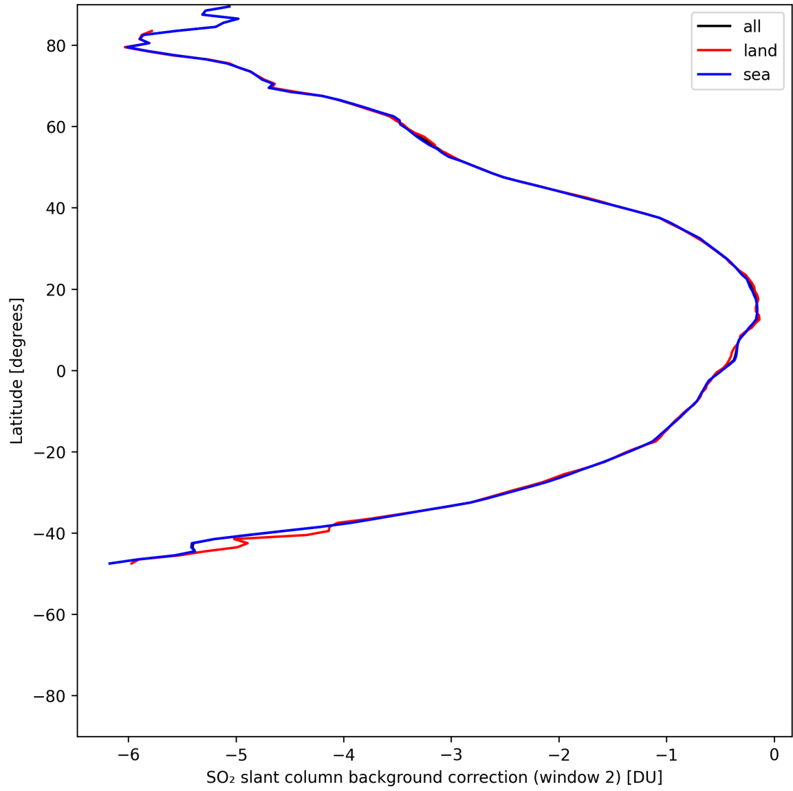
Figure 43: Zonal average of “SO 2 slant column background correction (window 2)” for 2025-05-24 to 2025-05-24.
