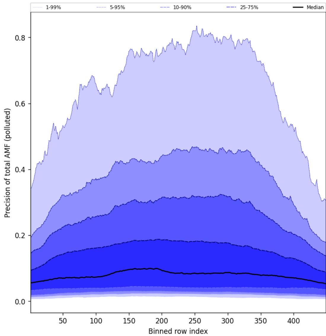
Figure 108: Along track statistics of “Precision of total AMF (polluted)” for 2025-05-24 to 2025-05-24
