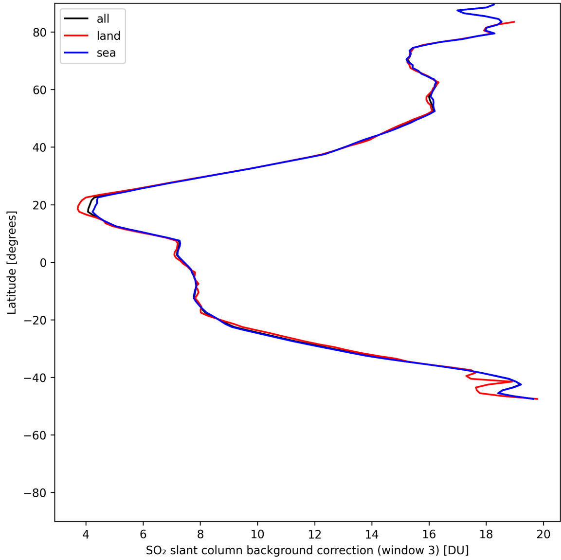
Figure 47: Zonal average of “SO 2 slant column background correction (window 3)” for 2025-05-24 to 2025-05-24.
