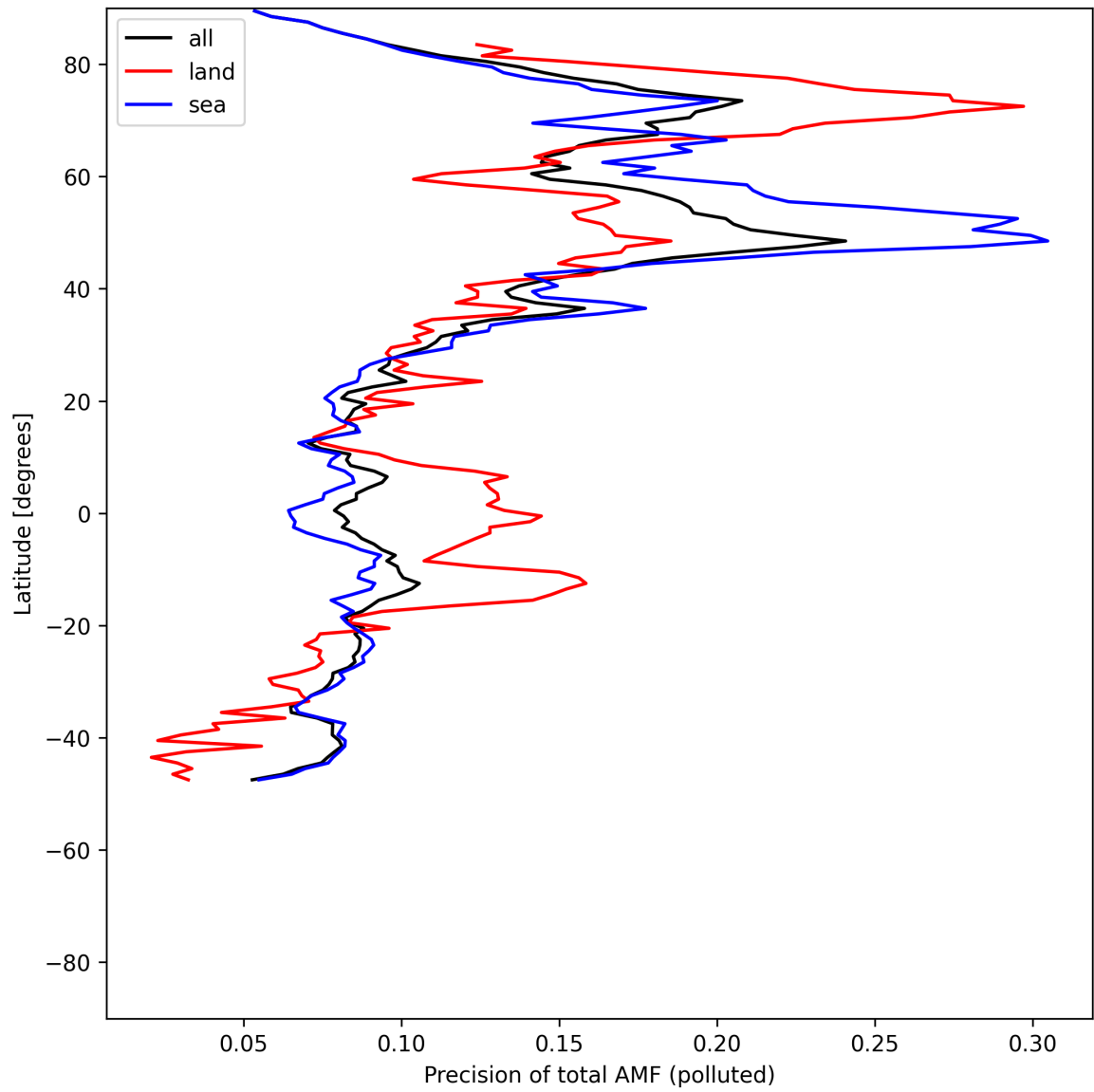
Figure 54: Zonal average of “Precision of total AMF (polluted)” for 2025-05-24 to 2025-05-24.
