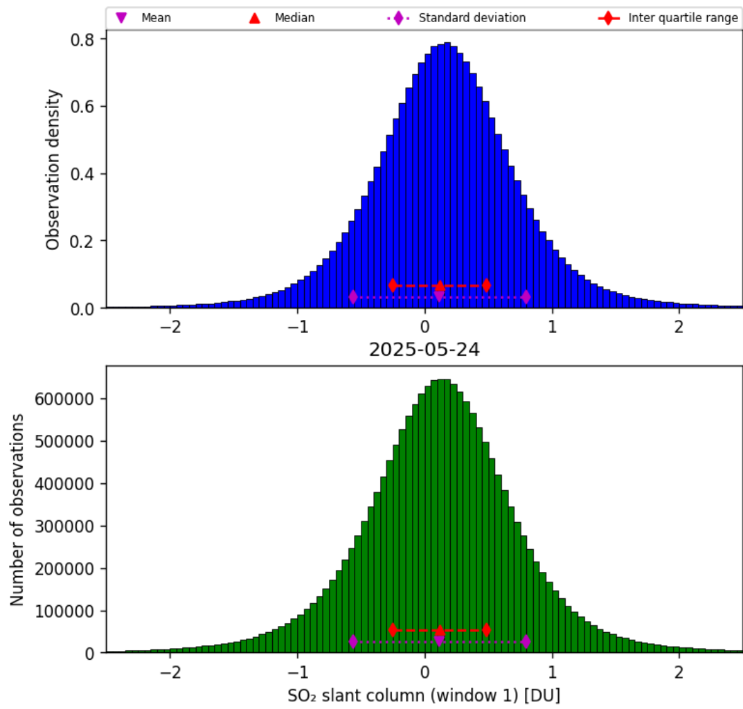
Figure 63: Histogram of “SO 2 slant column (window 1)” for 2025-05-24 to 2025-05-24
