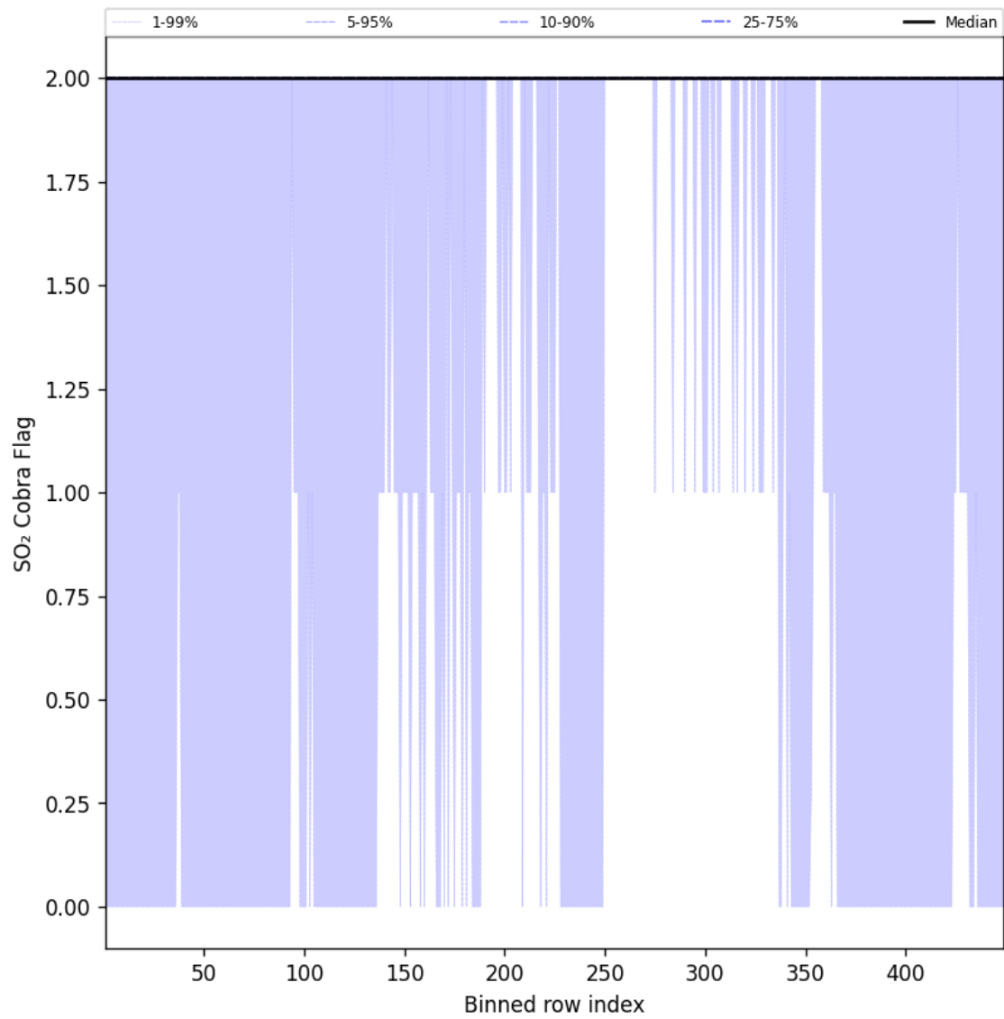
Figure 102: Along track statistics of “SO 2 Cobra Flag” for 2025-05-24 to 2025-05-24
