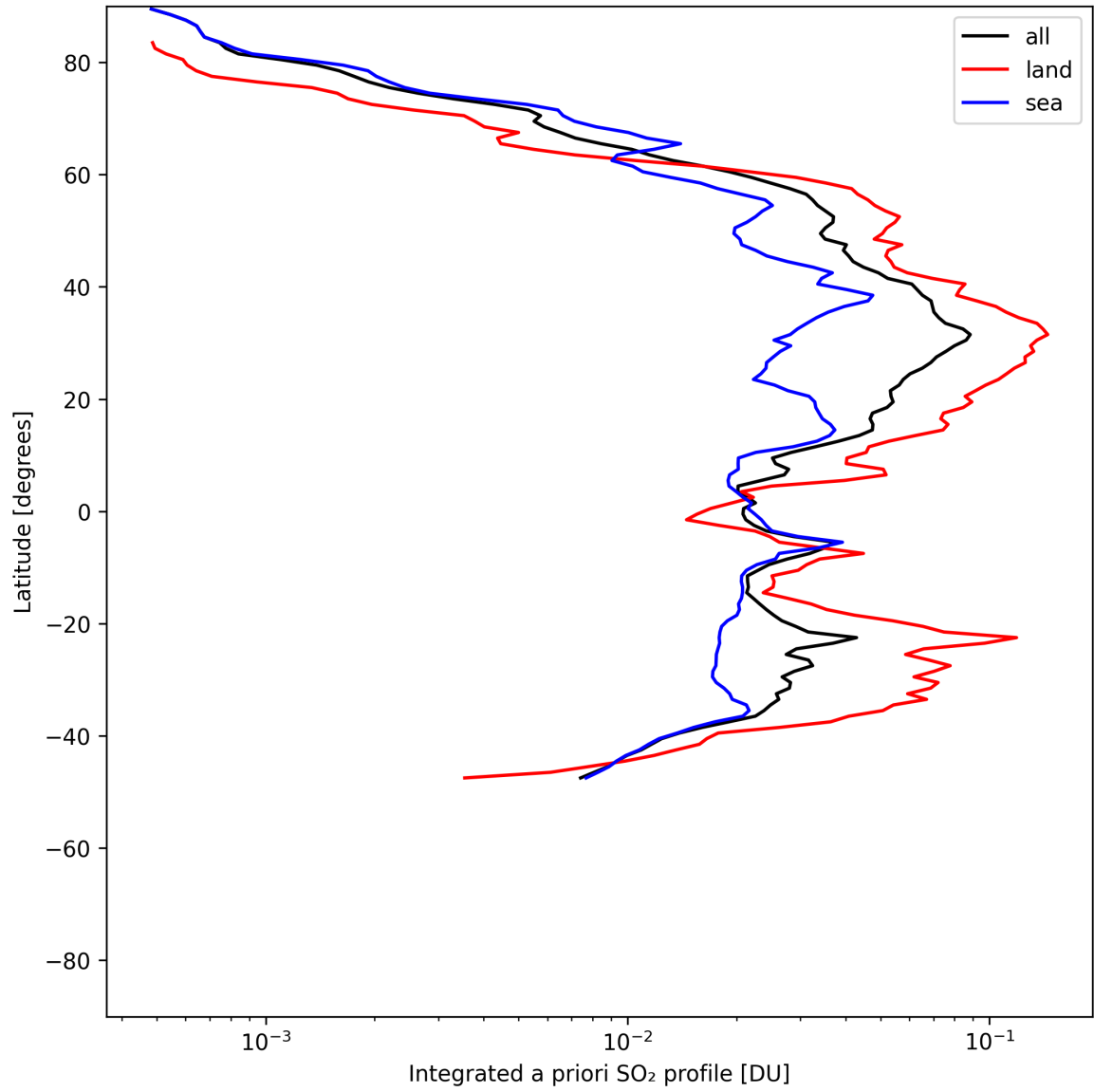
Figure 49: Zonal average of “Integrated a priori SO 2 profile” for 2025-05-24 to 2025-05-24.
