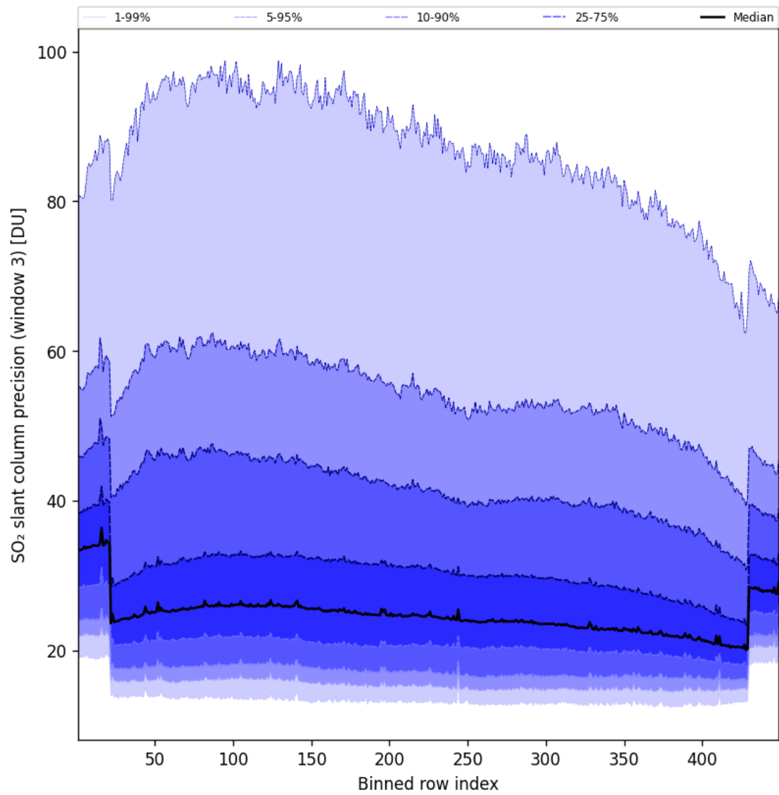
Figure 99: Along track statistics of “SO 2 slant column precision (window 3)” for 2025-05-24 to 2025-05-24
