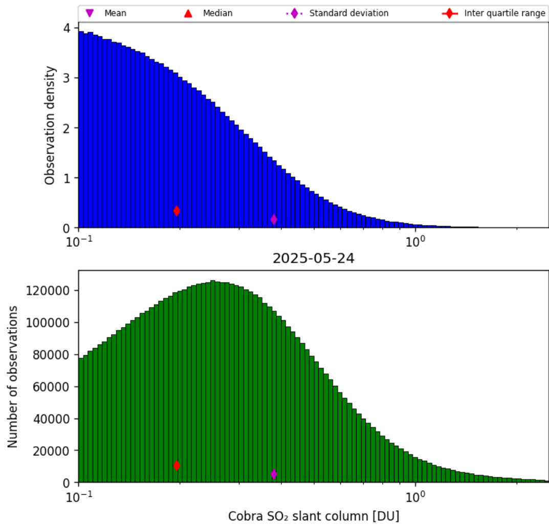
Figure 61: Histogram of “Cobra SO 2 slant column” for 2025-05-24 to 2025-05-24
