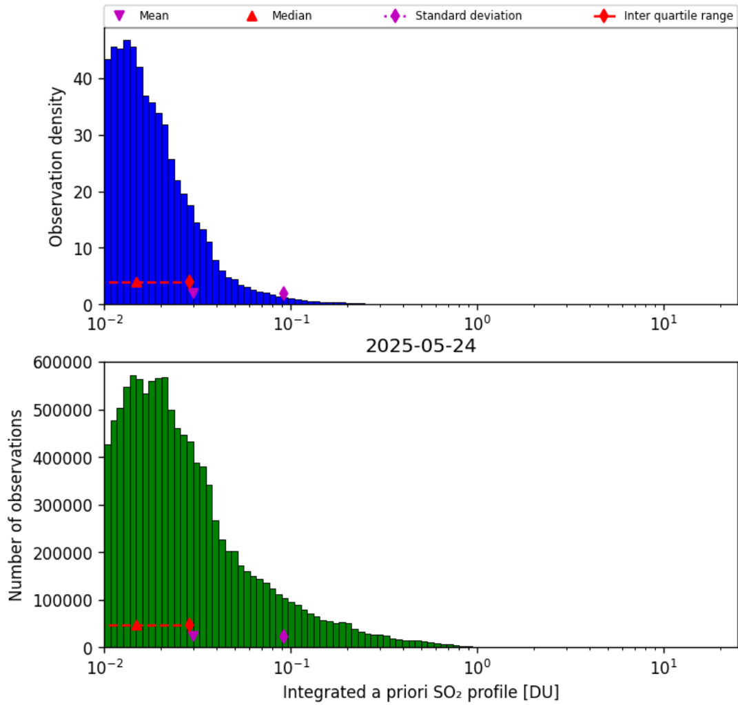
Figure 76: Histogram of “Integrated a priori SO 2 profile” for 2025-05-24 to 2025-05-24
