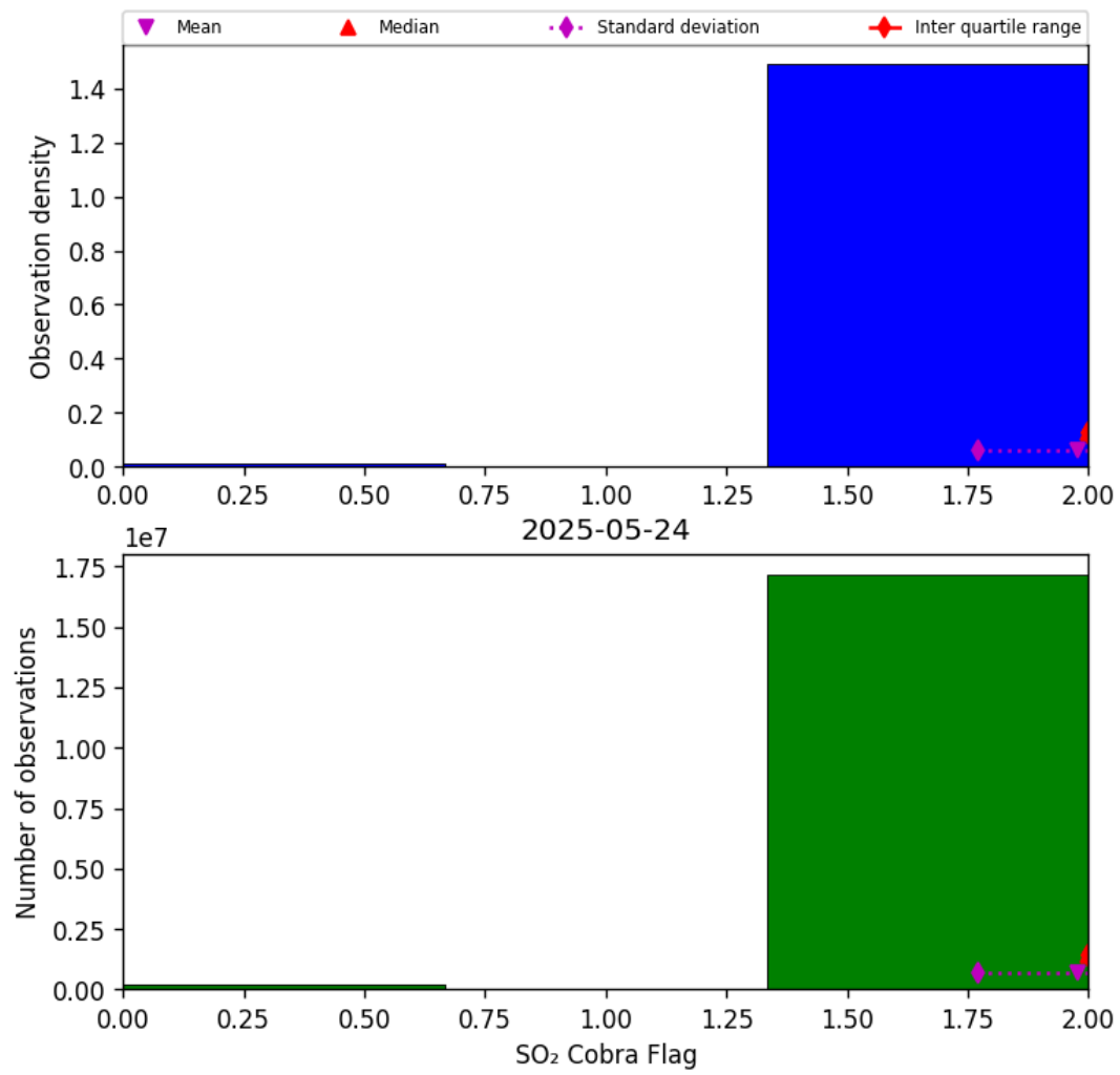
Figure 75: Histogram of "SO 2 Cobra Flag" for 2025-05-24 to 2025-05-24
