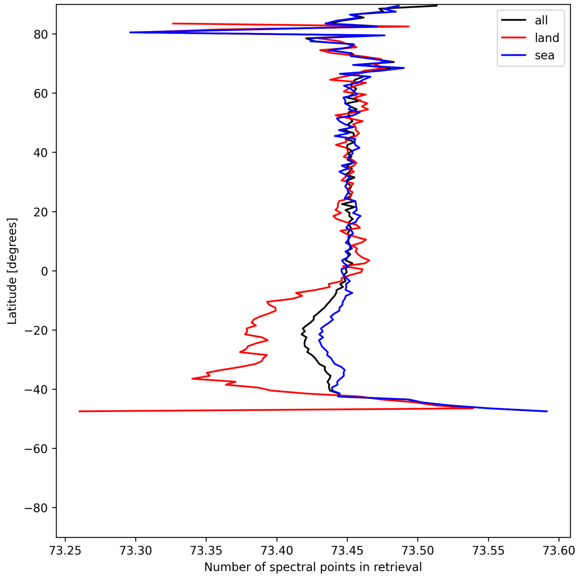
Figure 56: Zonal average of “Number of spectral points in retrieval” for 2025-05-24 to 2025-05-24.
