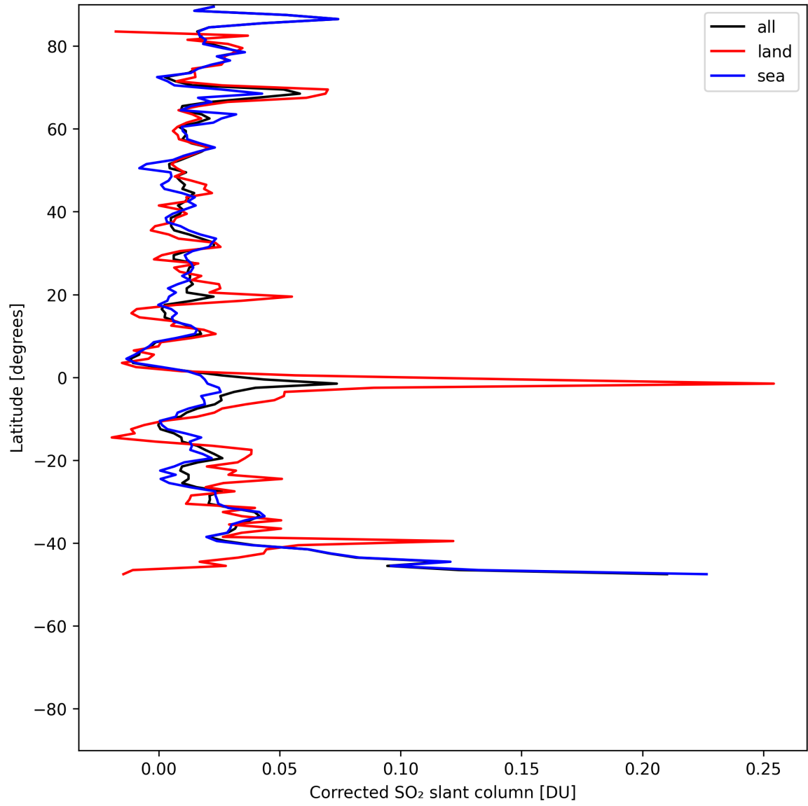
Figure 33: Zonal average of “Corrected SO 2 slant column” for 2025-05-24 to 2025-05-24.
