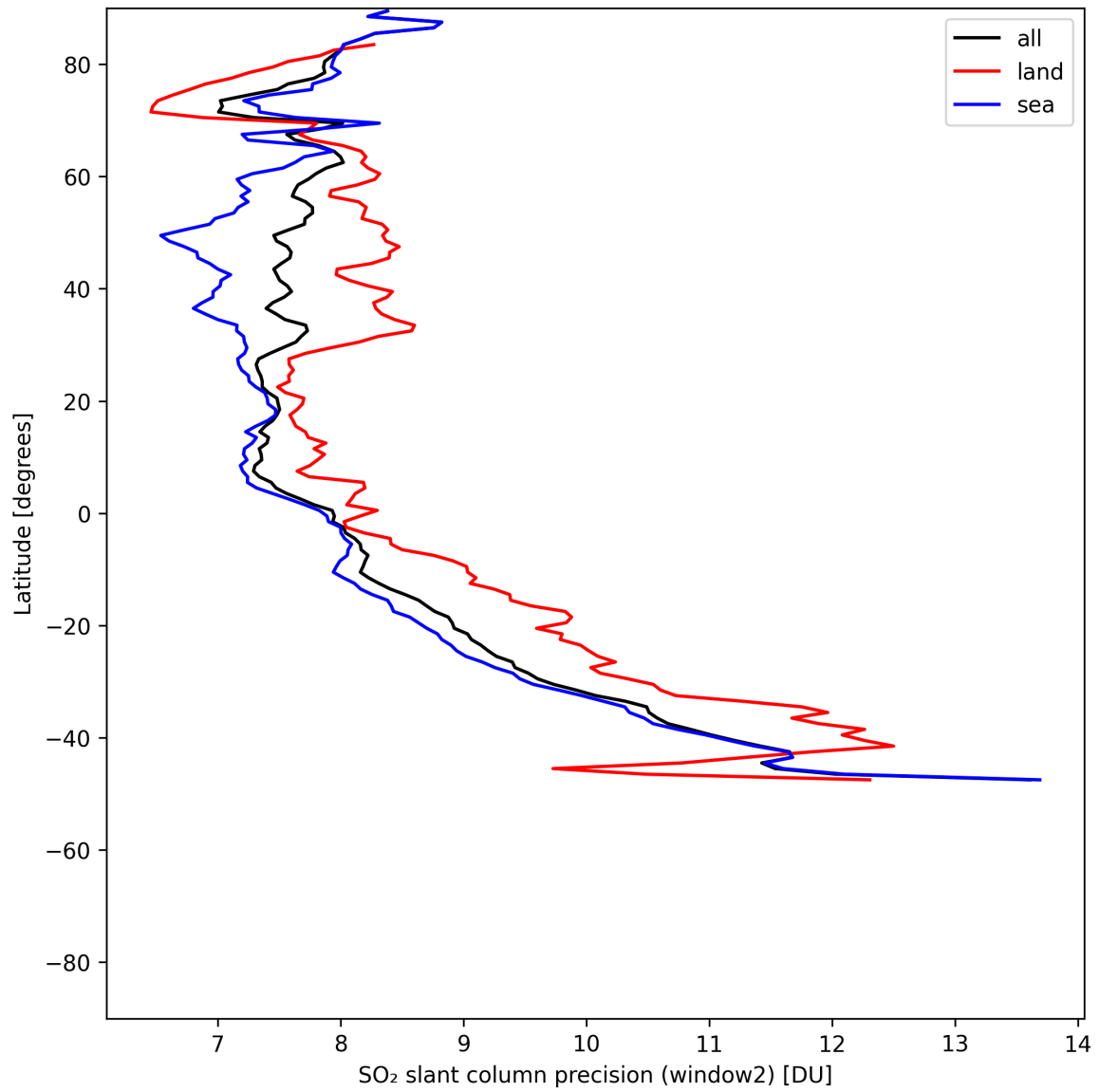
Figure 41: Zonal average of “SO 2 slant column precision (window2)” for 2025-05-24 to 2025-05-24.
