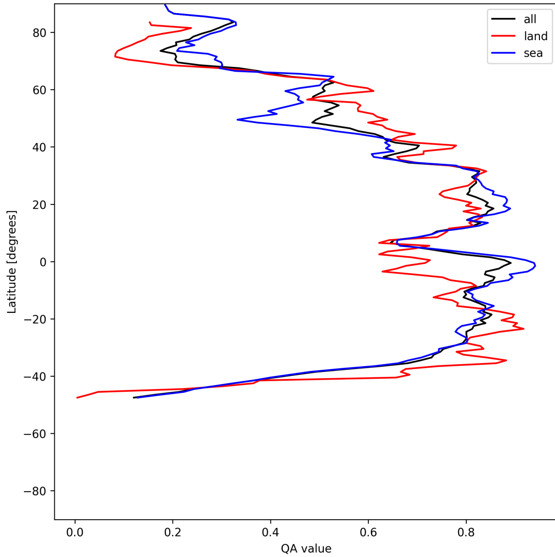
Figure 30: Zonal average of “QA value” for 2025-05-24 to 2025-05-24.
