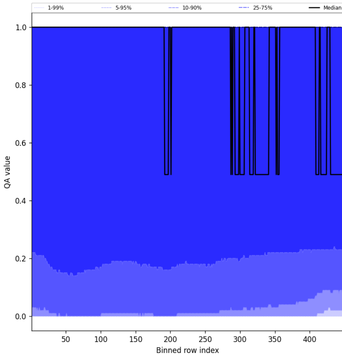
Figure 84: Along track statistics of “QA value” for 2025-05-24 to 2025-05-24
