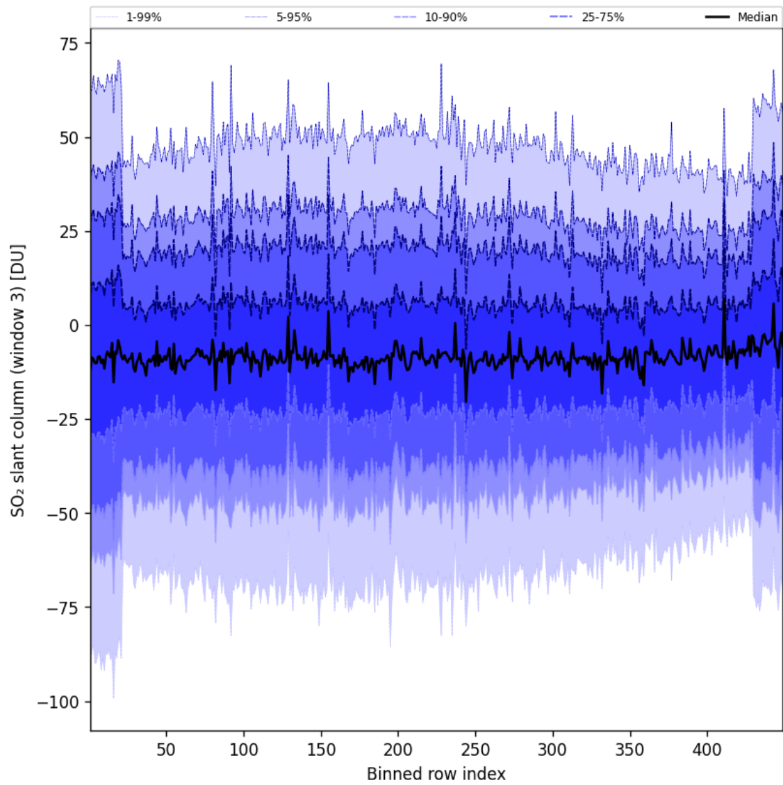
Figure 98: Along track statistics of “SO 2 slant column (window 3)” for 2025-05-24 to 2025-05-24
