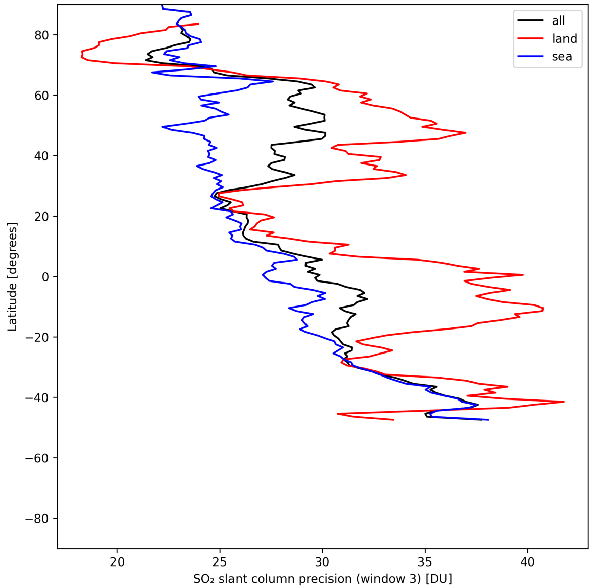
Figure 45: Zonal average of “SO 2 slant column precision (window 3)” for 2025-05-24 to 2025-05-24.
