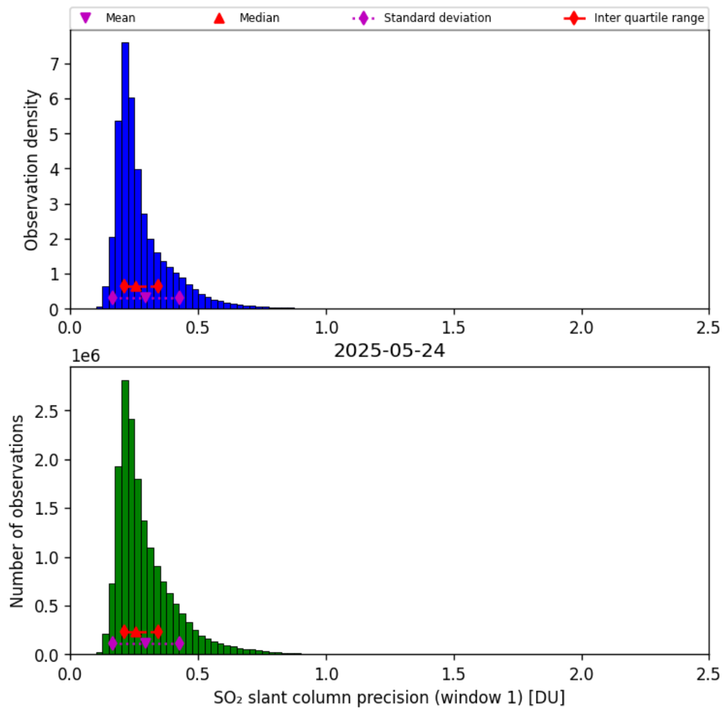
Figure 64: Histogram of “SO 2 slant column precision (window 1)” for 2025-05-24 to 2025-05-24
