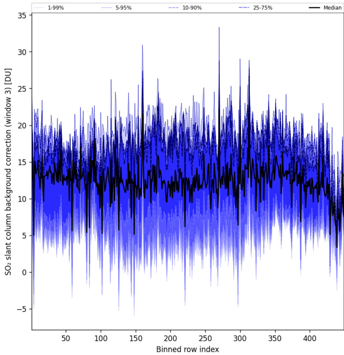
Figure 101: Along track statistics of "SO 2 slant column background correction (window 3)" for 2025-05-24 to 2025-05-24
