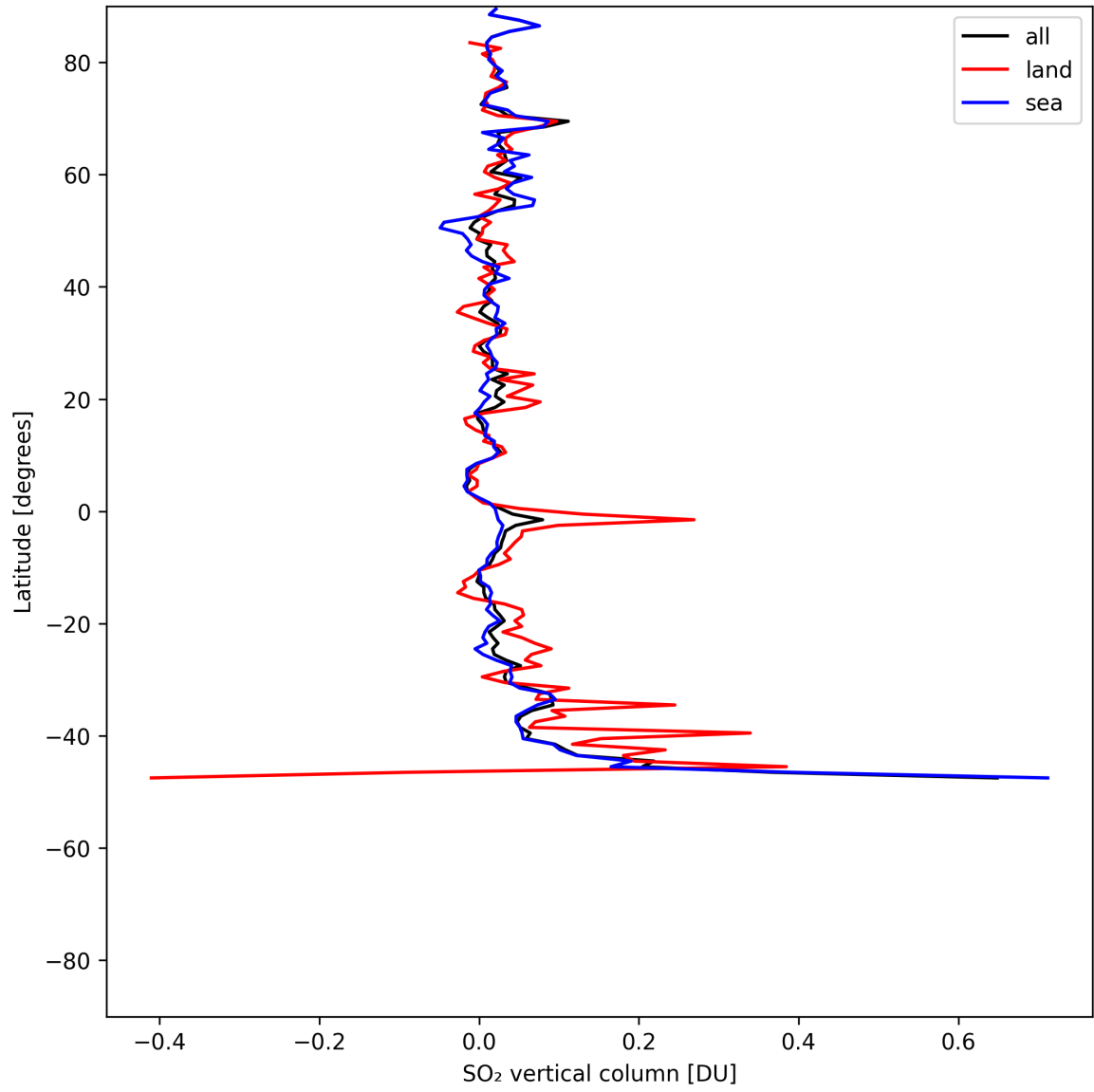
Figure 31: Zonal average of “SO 2 vertical column” for 2025-05-24 to 2025-05-24.
