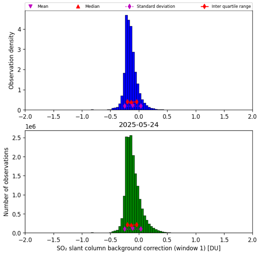
Figure 66: Histogram of “SO 2 slant column background correction (window 1)” for 2025-05-24 to 2025-05-24
