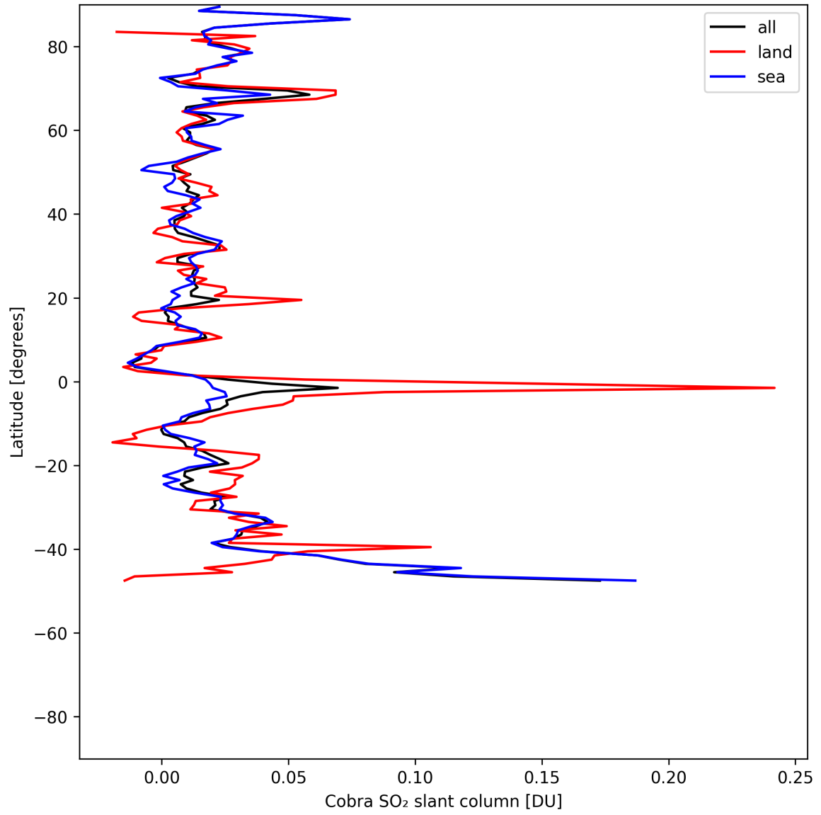
Figure 34: Zonal average of “Cobra SO 2 slant column” for 2025-05-24 to 2025-05-24.
