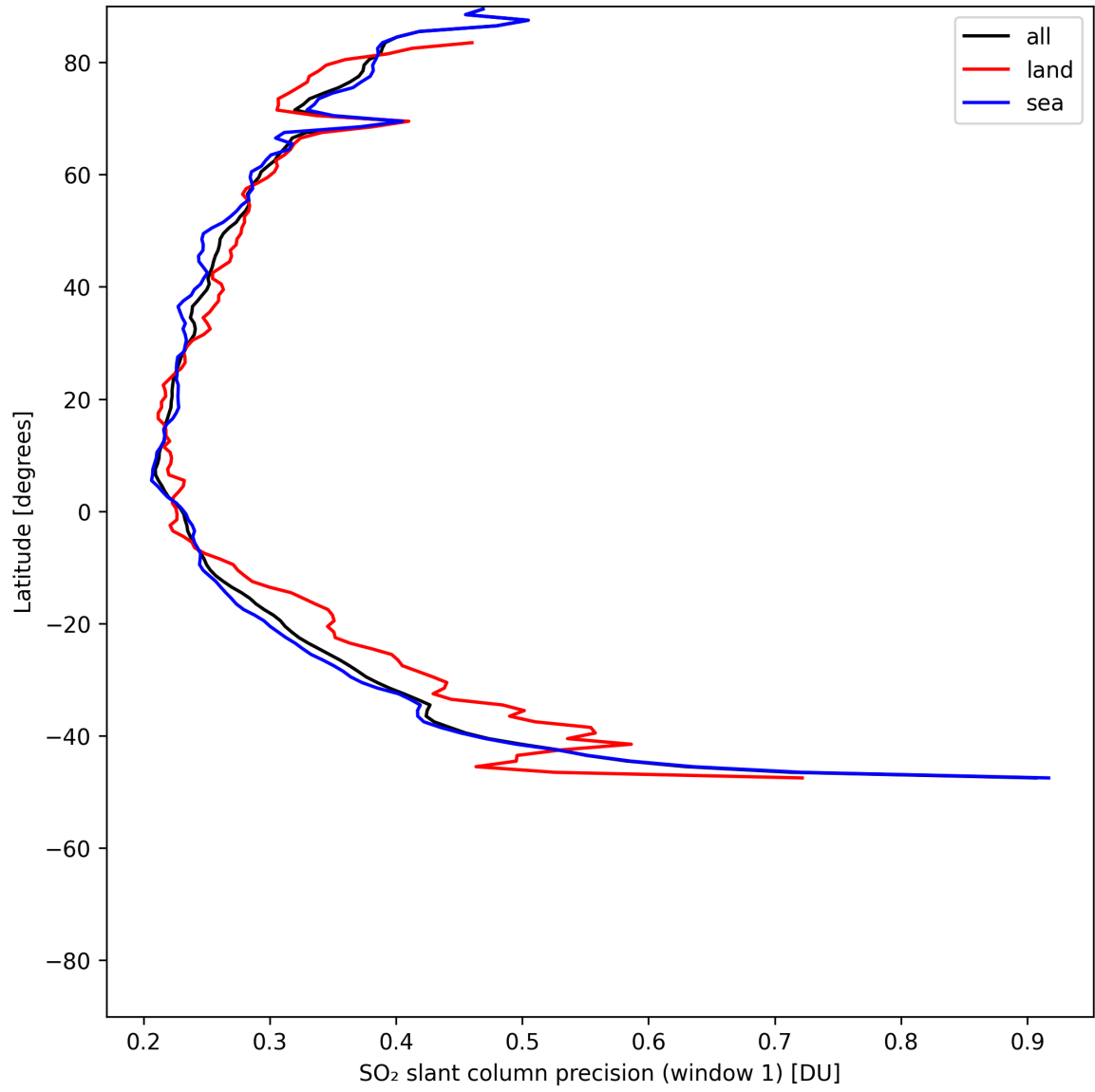
Figure 37: Zonal average of “SO 2 slant column precision (window 1)” for 2025-05-24 to 2025-05-24.
