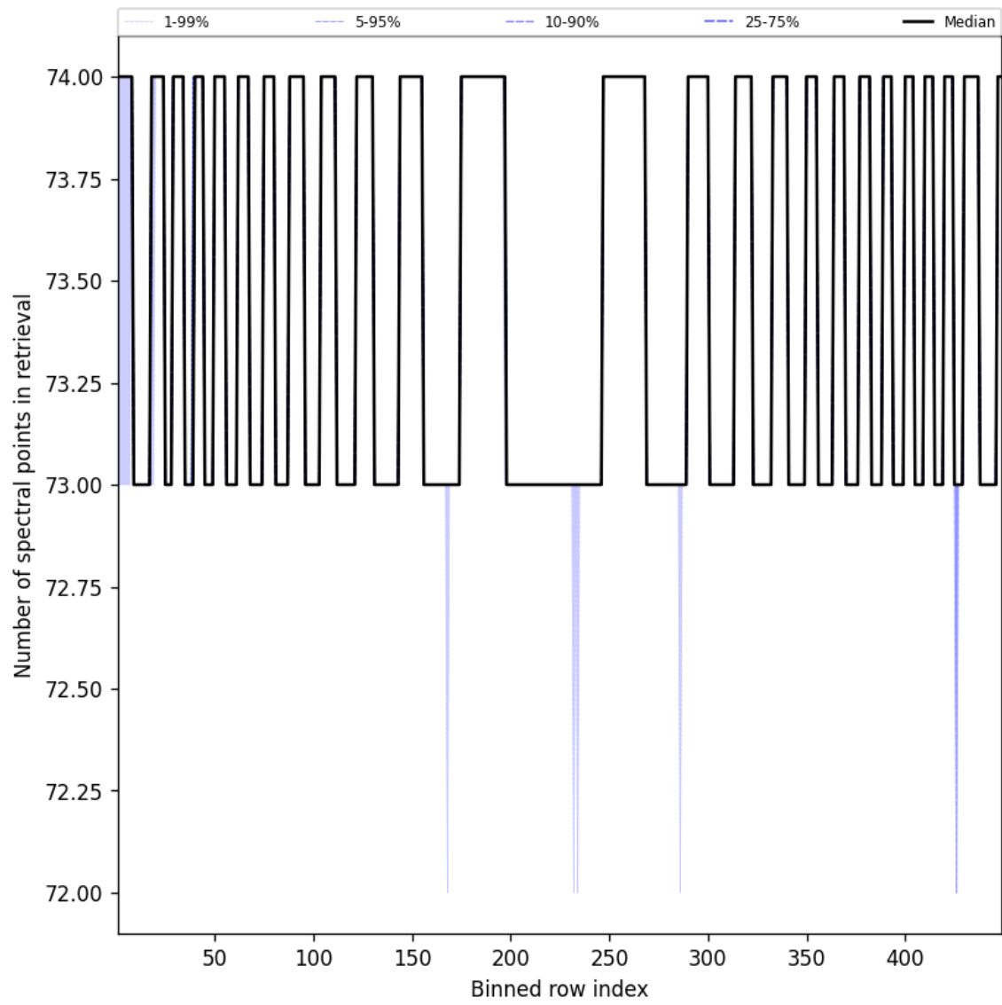
Figure 110: Along track statistics of “Number of spectral points in retrieval” for 2025-05-24 to 2025-05-24
