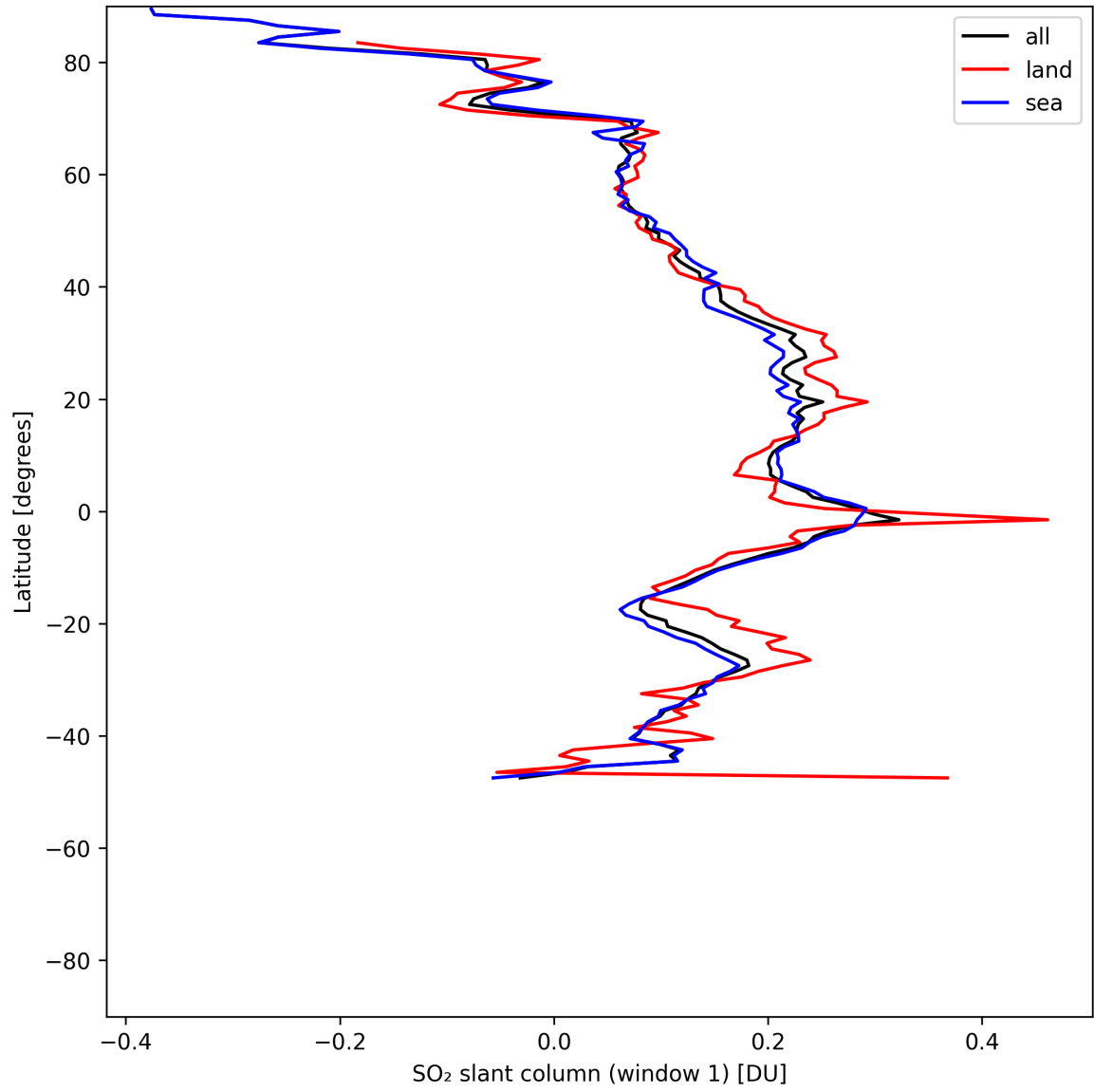
Figure 36: Zonal average of “SO 2 slant column (window 1)” for 2025-05-24 to 2025-05-24.
