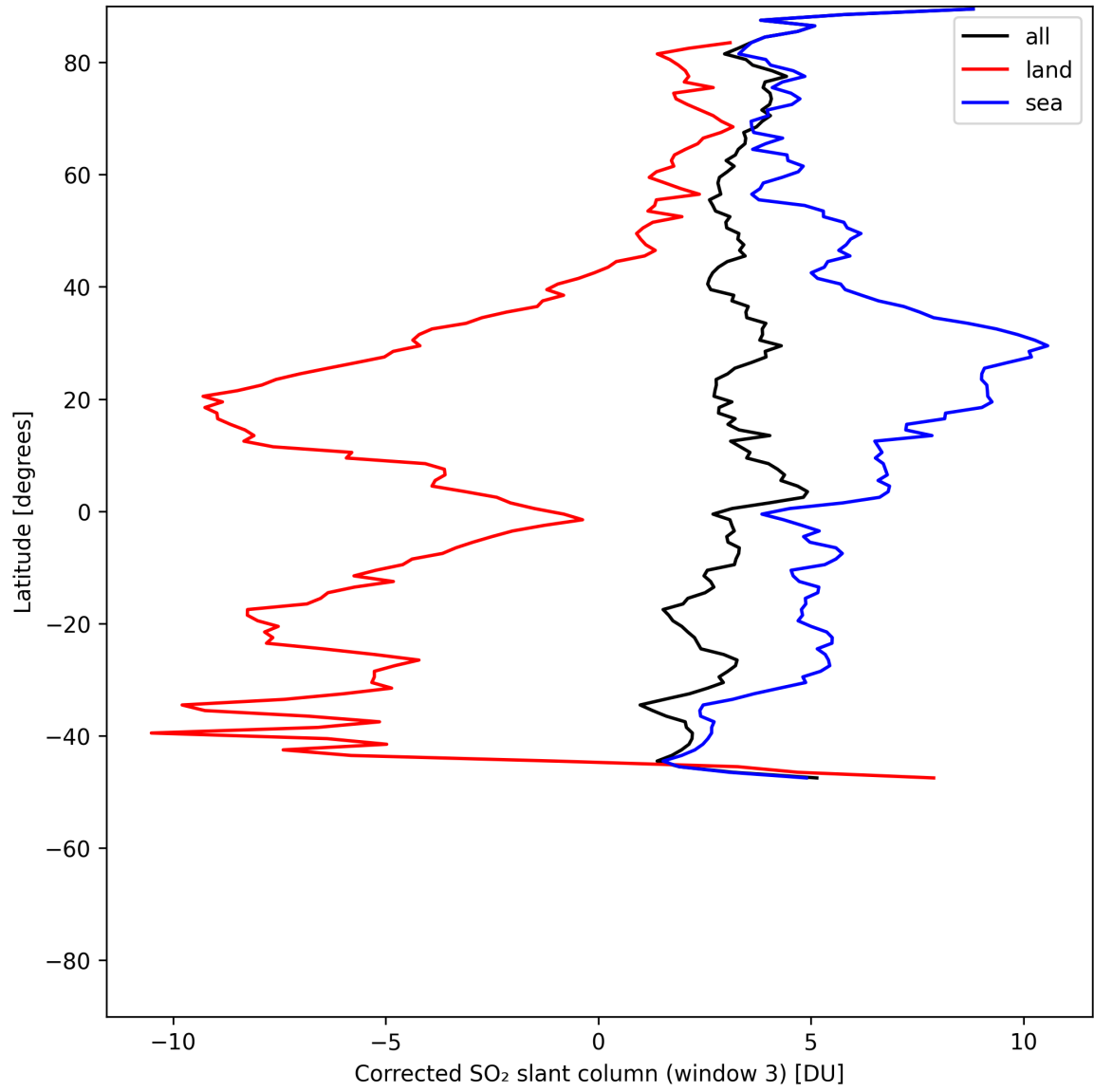
Figure 46: Zonal average of “Corrected SO 2 slant column (window 3)” for 2025-05-24 to 2025-05-24.
