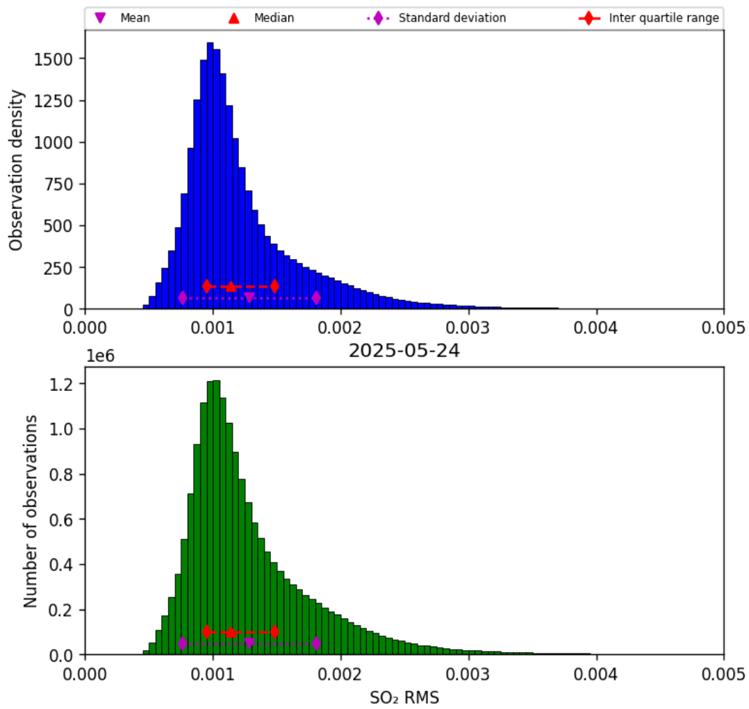
Figure 79: Histogram of “SO 2 RMS” for 2025-05-24 to 2025-05-24
