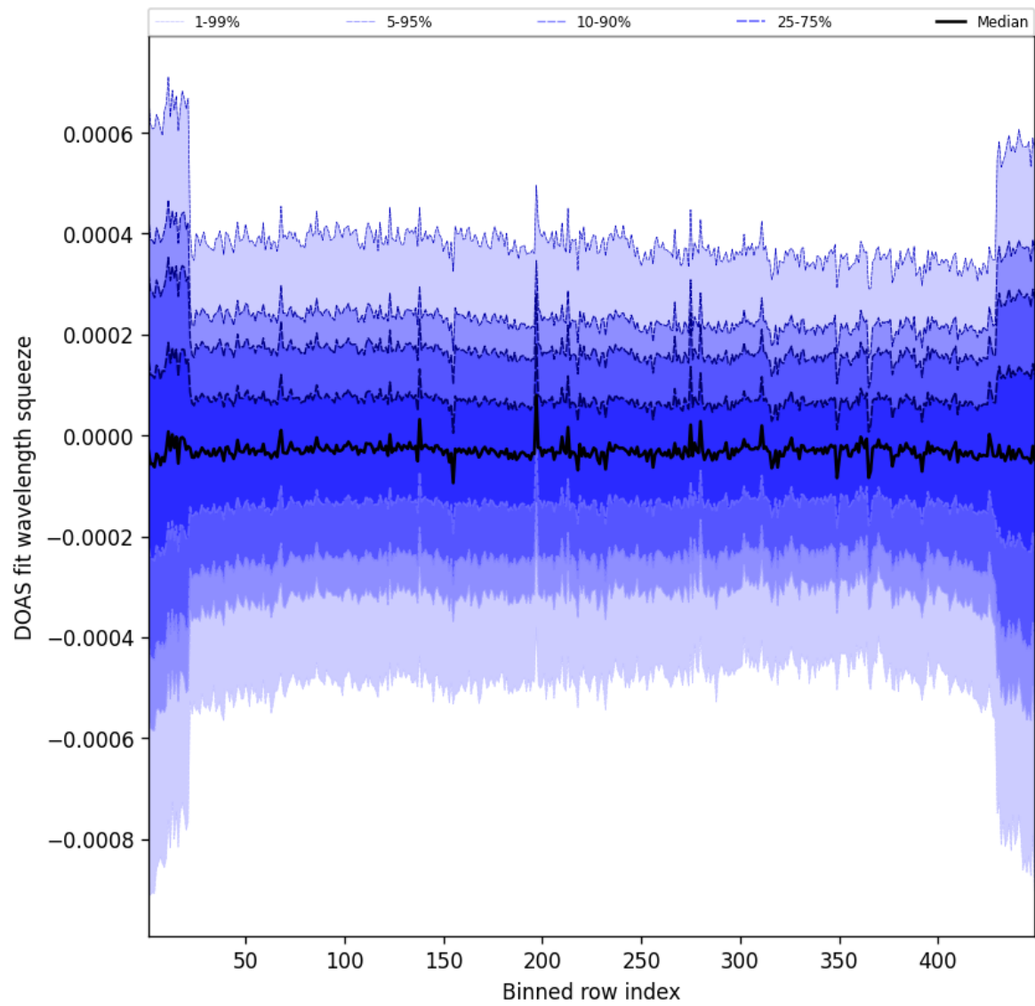
Figure 105: Along track statistics of “DOAS fit wavelength squeeze” for 2025-05-24 to 2025-05-24
