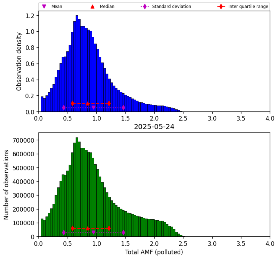
Figure 80: Histogram of “Total AMF (polluted)” for 2025-05-24 to 2025-05-24
