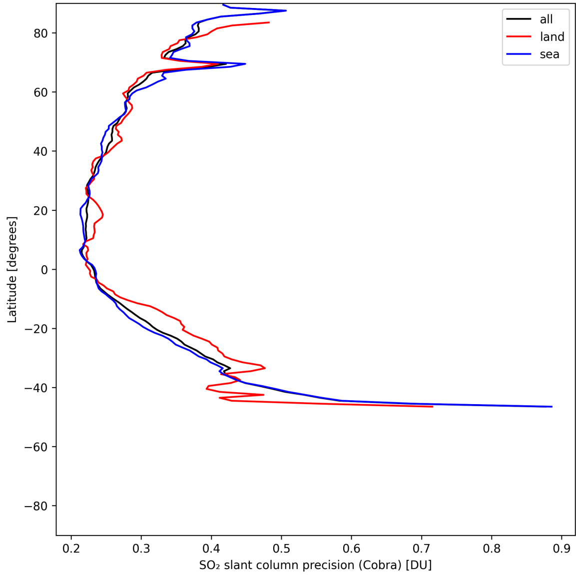
Figure 35: Zonal average of “SO 2 slant column precision (Cobra)” for 2025-06-01 to 2025-06-02.
