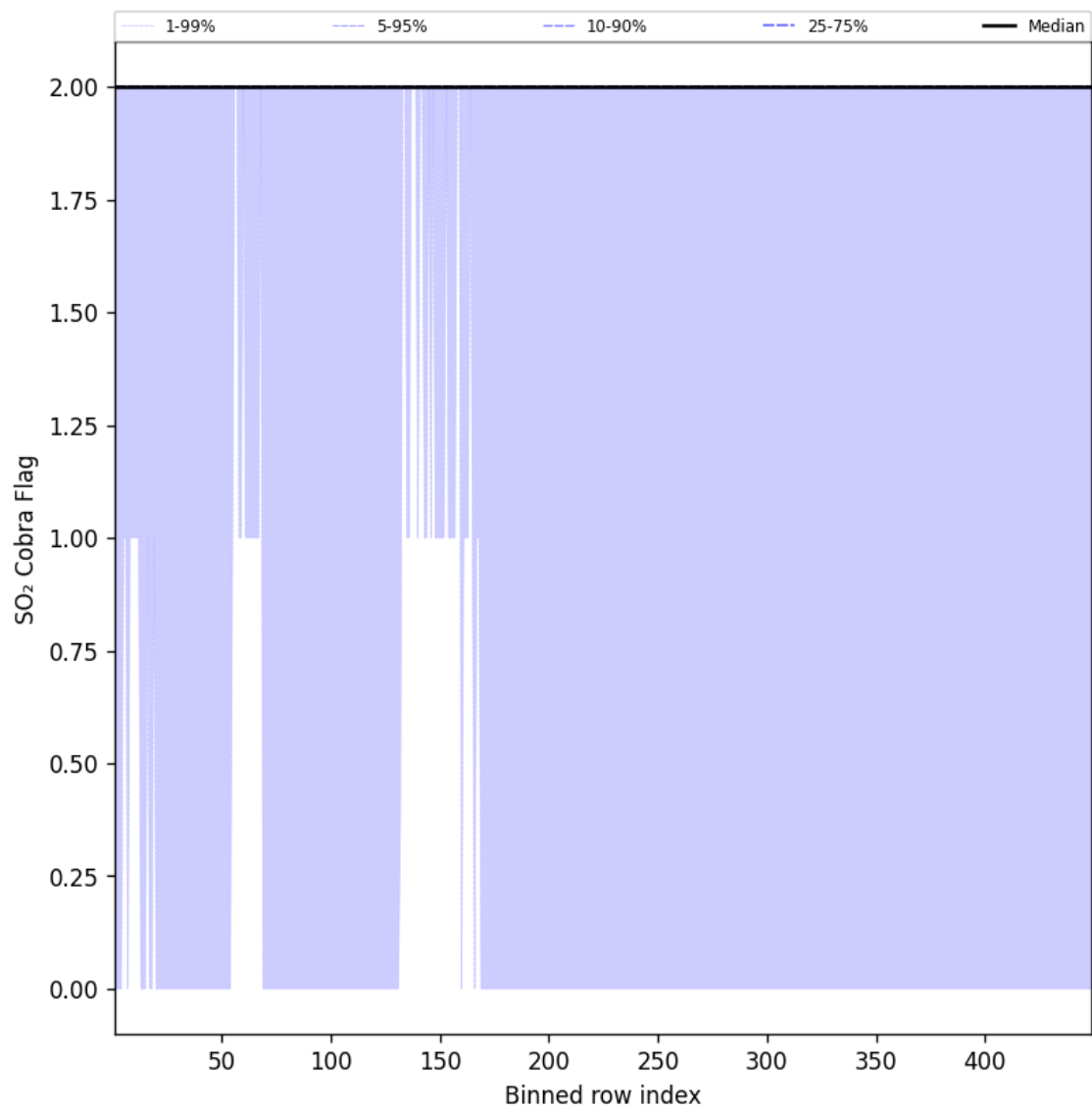
Figure 102: Along track statistics of “SO 2 Cobra Flag” for 2025-06-01 to 2025-06-02
