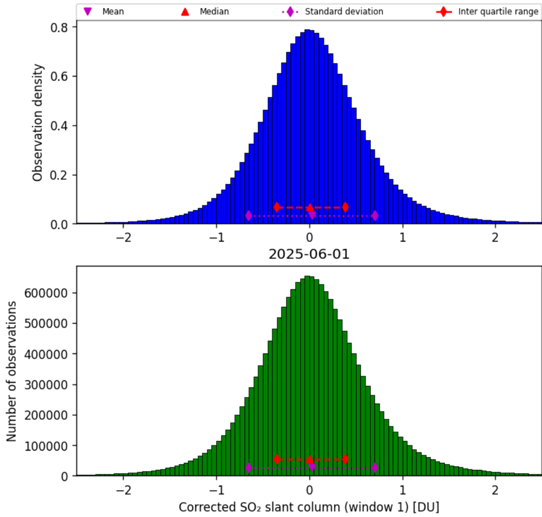
Figure 65: Histogram of “Corrected SO 2 slant column (window 1)” for 2025-06-01 to 2025-06-02
