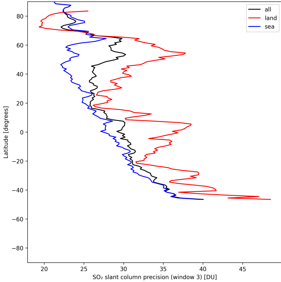
Figure 45: Zonal average of “SO 2 slant column precision (window 3)” for 2025-06-01 to 2025-06-02.
