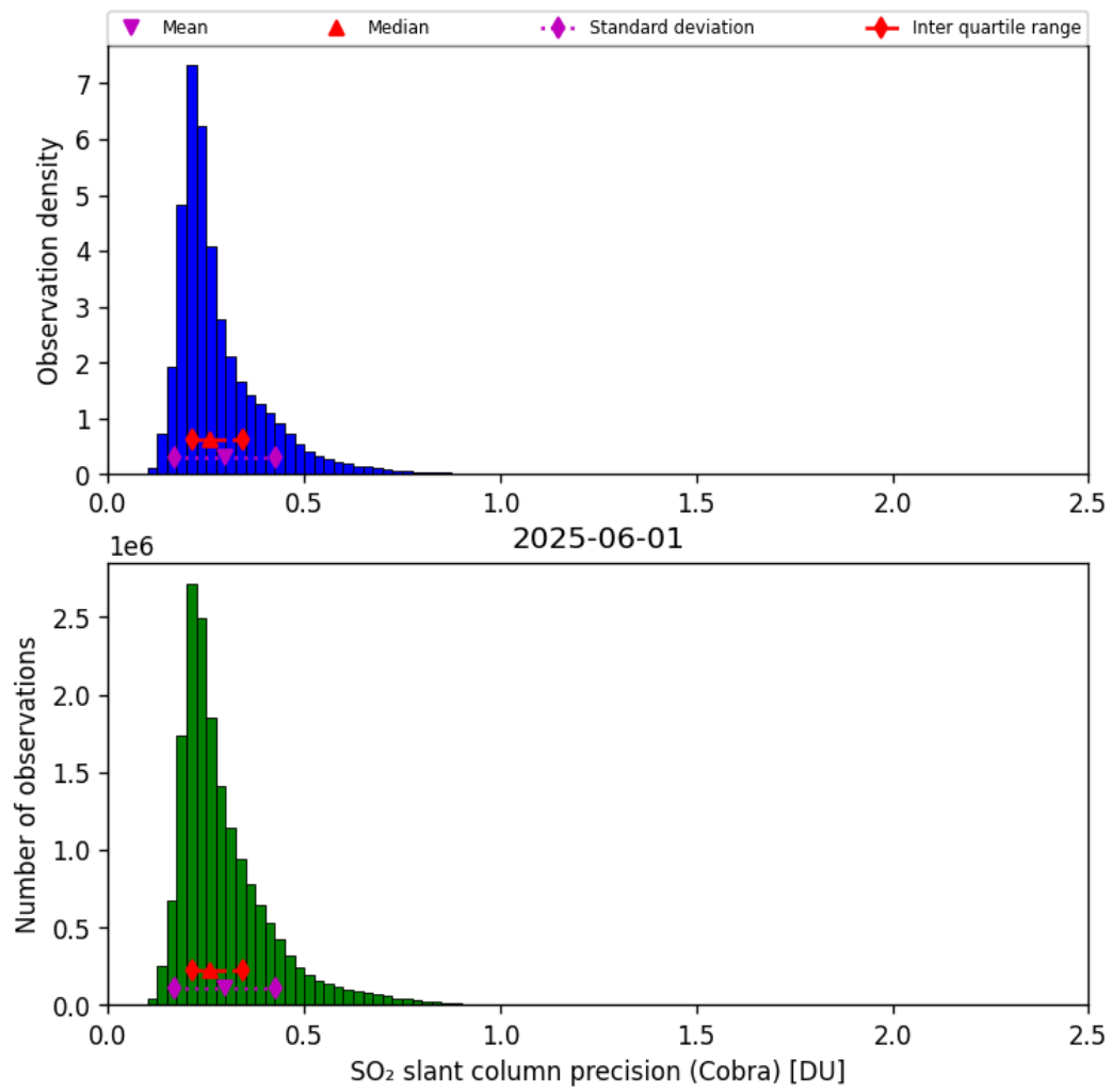
Figure 62: Histogram of “SO 2 slant column precision (Cobra)” for 2025-06-01 to 2025-06-02
