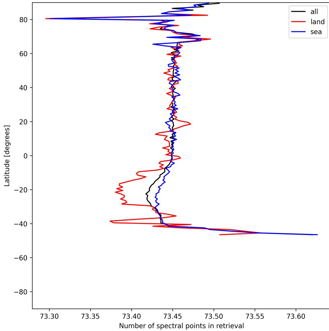
Figure 56: Zonal average of “Number of spectral points in retrieval” for 2025-06-01 to 2025-06-02.
