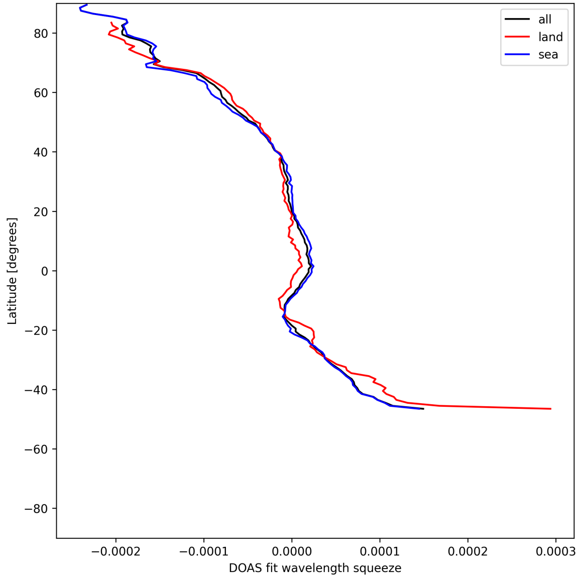
Figure 51: Zonal average of “DOAS fit wavelength squeeze” for 2025-06-01 to 2025-06-02.
