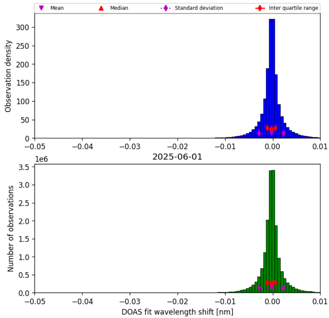
Figure 77: Histogram of “DOAS fit wavelength shift” for 2025-06-01 to 2025-06-02
