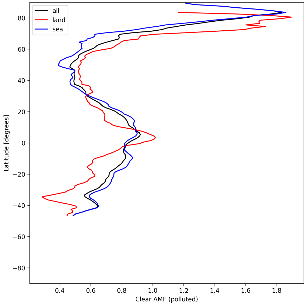
Figure 55: Zonal average of “Clear AMF (polluted)” for 2025-06-01 to 2025-06-02.
