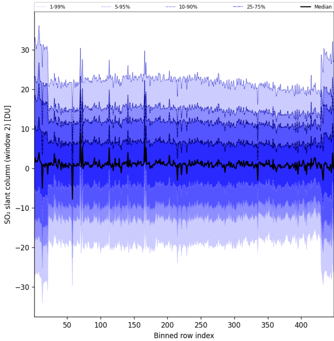
Figure 94: Along track statistics of “SO 2 slant column (window 2)” for 2025-06-01 to 2025-06-02
