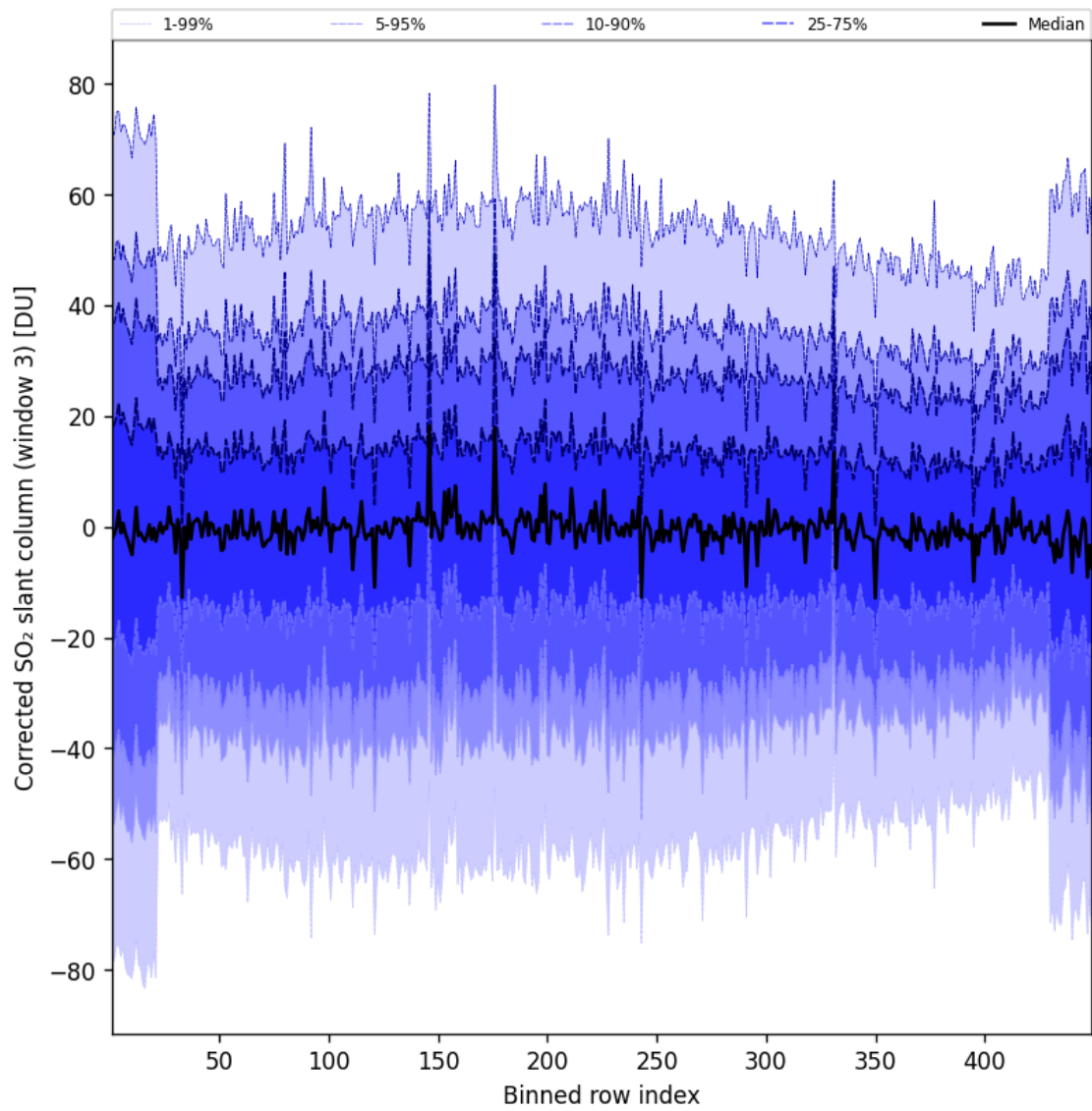
Figure 100: Along track statistics of "Corrected SO 2 slant column (window 3)" for 2025-06-01 to 2025-06-02
