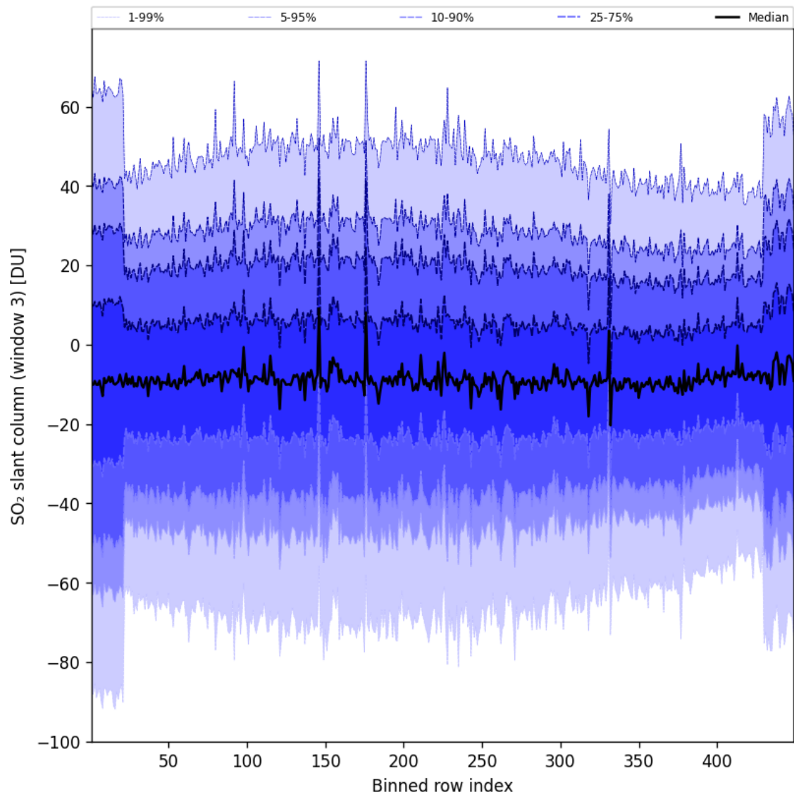
Figure 98: Along track statistics of “SO 2 slant column (window 3)” for 2025-06-01 to 2025-06-02
