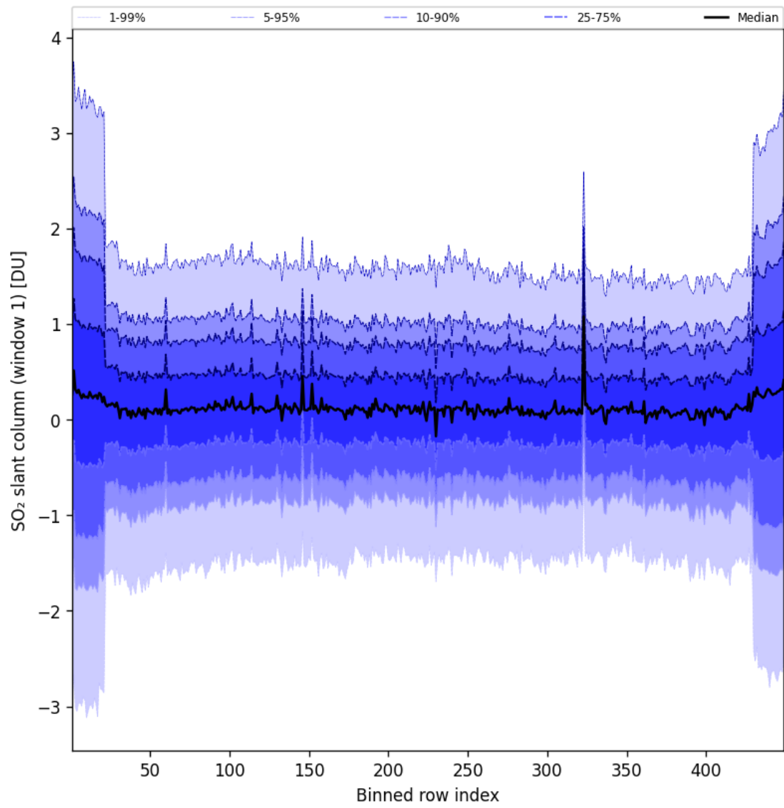
Figure 90: Along track statistics of “SO 2 slant column (window 1)” for 2025-06-01 to 2025-06-02
