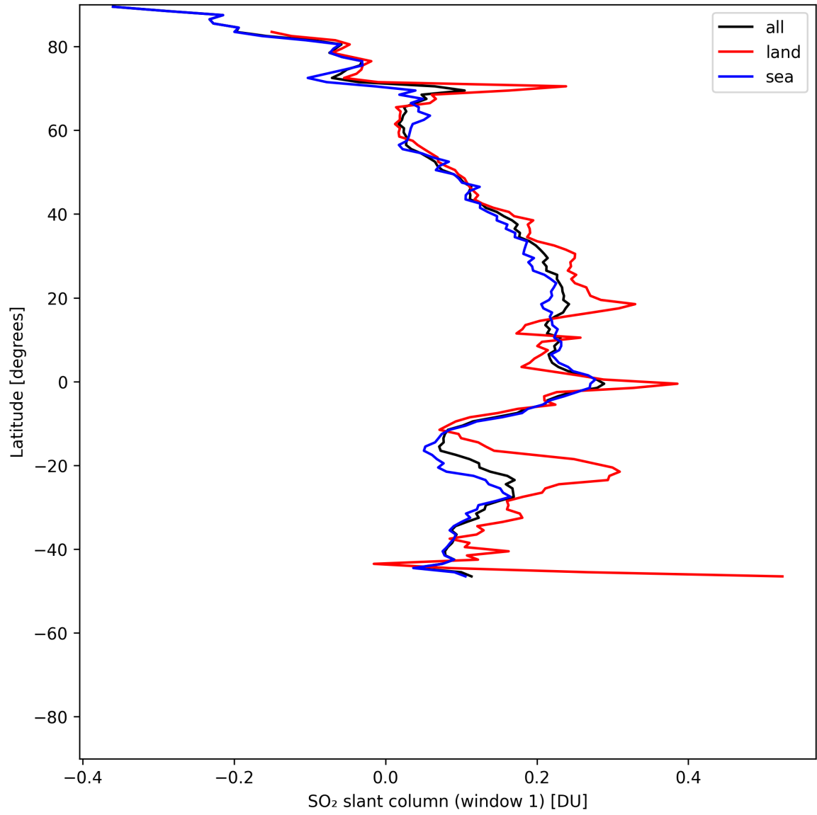
Figure 36: Zonal average of “SO 2 slant column (window 1)” for 2025-06-01 to 2025-06-02.
