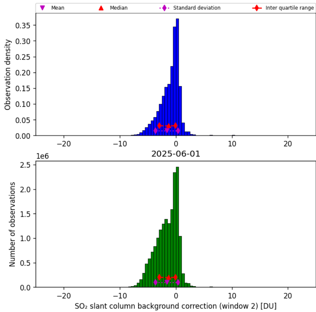
Figure 70: Histogram of “SO 2 slant column background correction (window 2)” for 2025-06-01 to 2025-06-02
