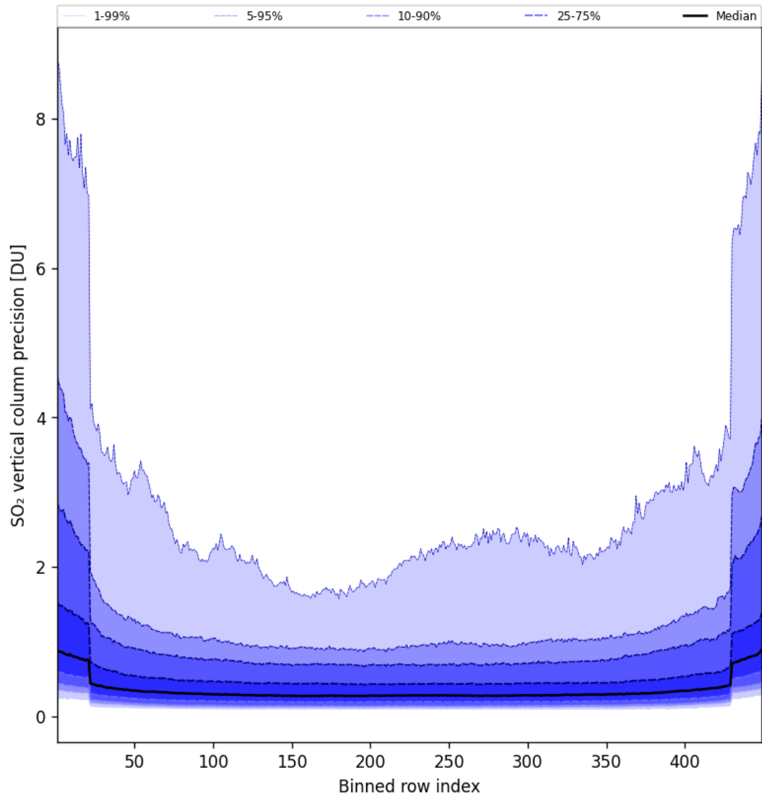
Figure 86: Along track statistics of “SO 2 vertical column precision” for 2025-06-01 to 2025-06-02
