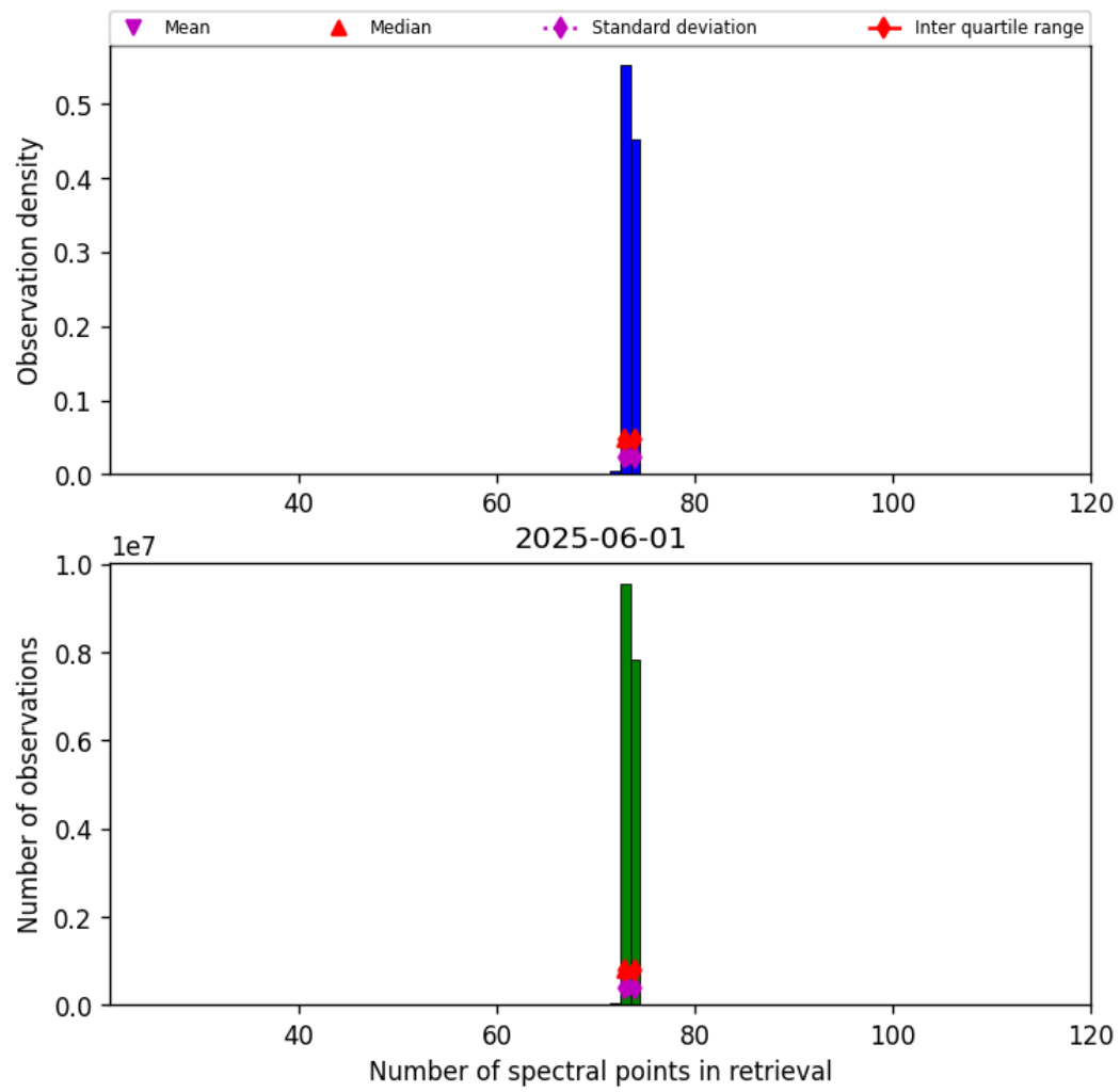
Figure 83: Histogram of “Number of spectral points in retrieval” for 2025-06-01 to 2025-06-02
