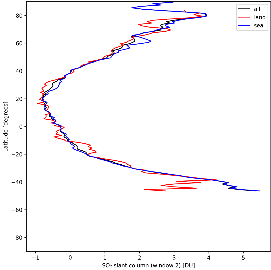
Figure 40: Zonal average of “SO 2 slant column (window 2)” for 2025-06-01 to 2025-06-02.
