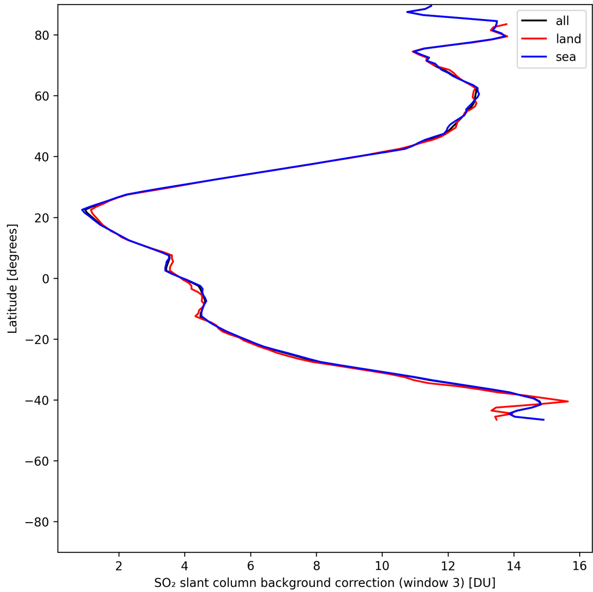
Figure 47: Zonal average of “SO 2 slant column background correction (window 3)” for 2025-06-01 to 2025-06-02.
