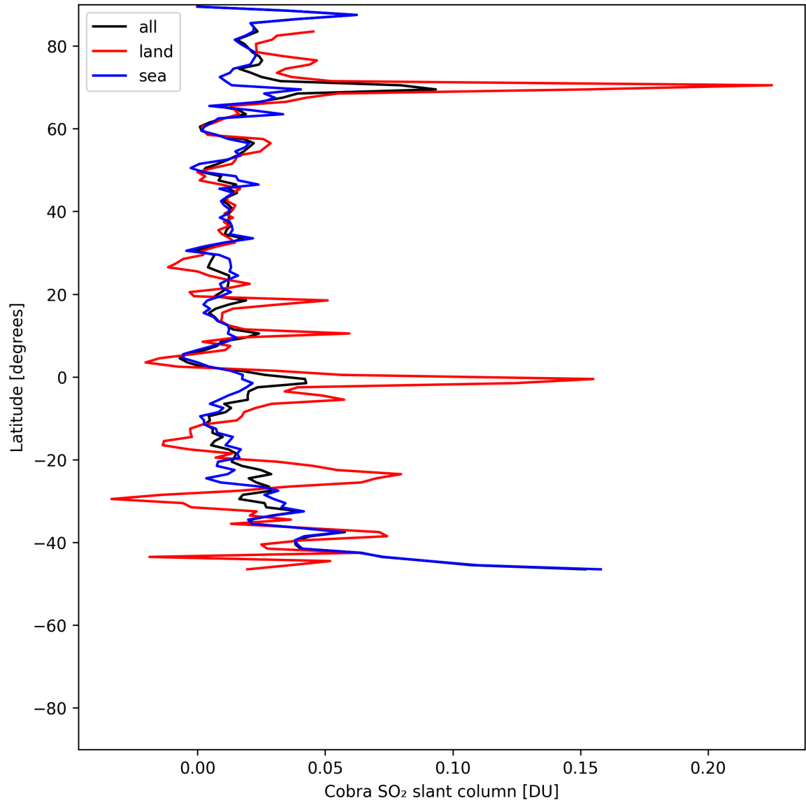
Figure 34: Zonal average of “Cobra SO 2 slant column” for 2025-06-01 to 2025-06-02.
