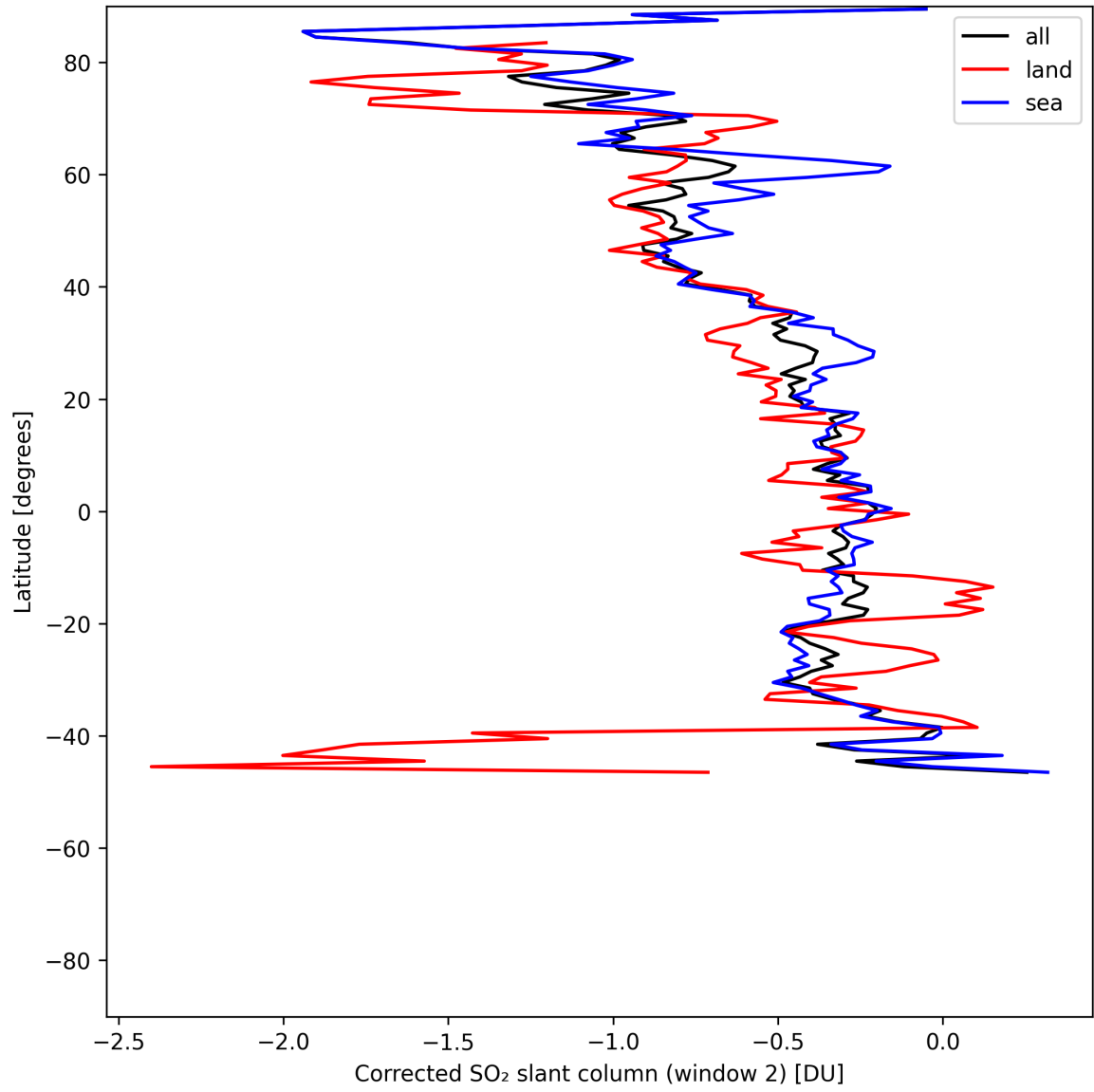
Figure 42: Zonal average of “Corrected SO 2 slant column (window 2)” for 2025-06-01 to 2025-06-02.
