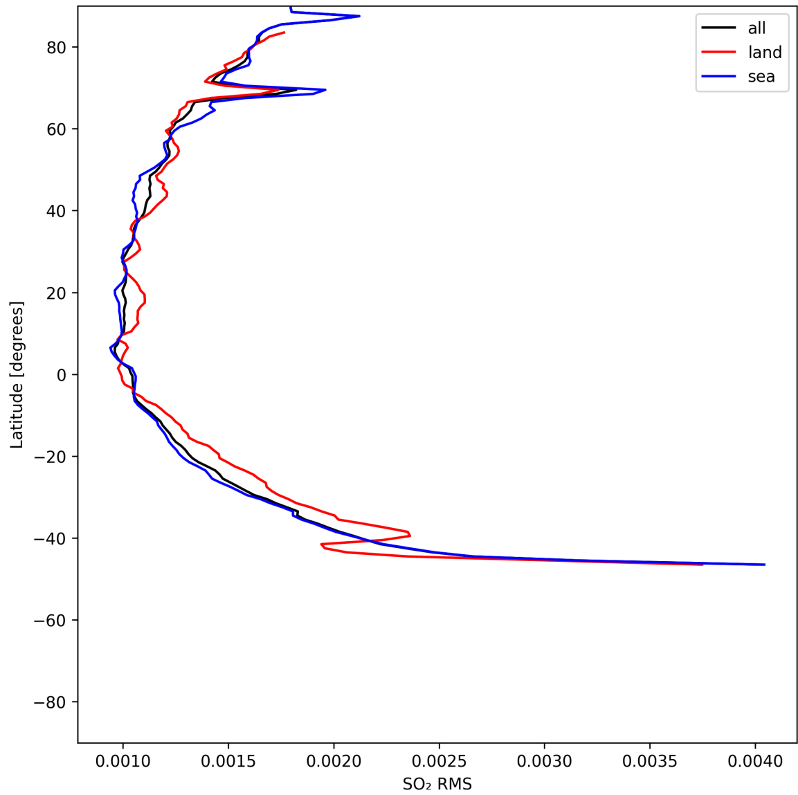
Figure 52: Zonal average of “SO 2 RMS” for 2025-06-01 to 2025-06-02.
