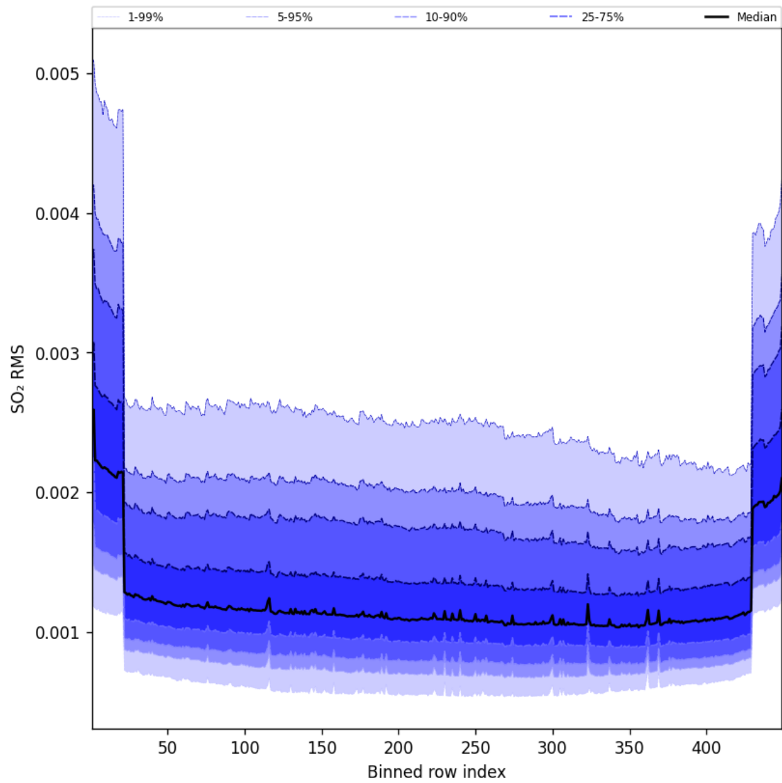
Figure 106: Along track statistics of “SO 2 RMS” for 2025-06-01 to 2025-06-02
