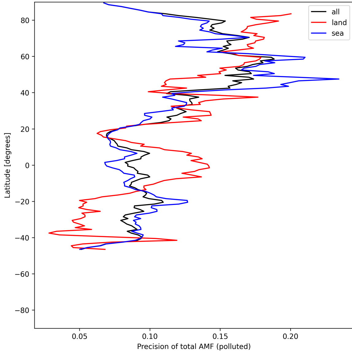
Figure 54: Zonal average of “Precision of total AMF (polluted)” for 2025-06-01 to 2025-06-02.
