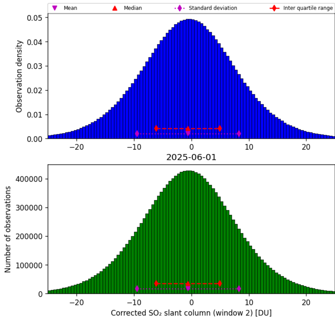
Figure 69: Histogram of “Corrected SO 2 slant column (window 2)” for 2025-06-01 to 2025-06-02
