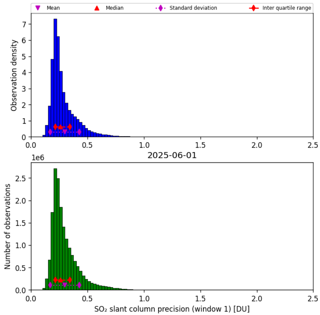
Figure 64: Histogram of “SO 2 slant column precision (window 1)” for 2025-06-01 to 2025-06-02
