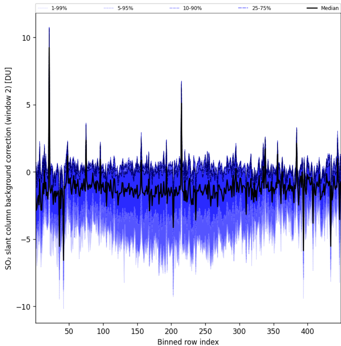
Figure 97: Along track statistics of “SO 2 slant column background correction (window 2)” for 2025-06-01 to 2025-06-02
