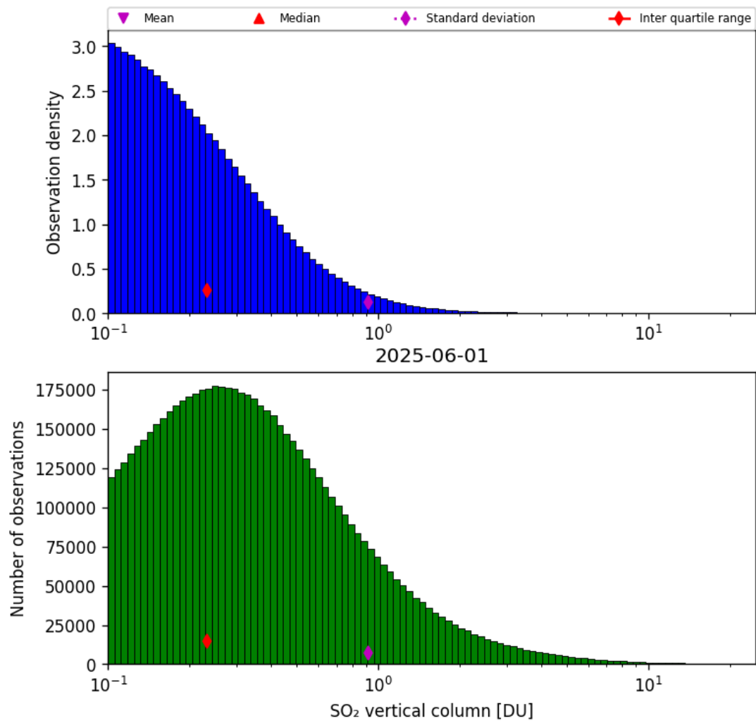
Figure 58: Histogram of “SO 2 vertical column” for 2025-06-01 to 2025-06-02
