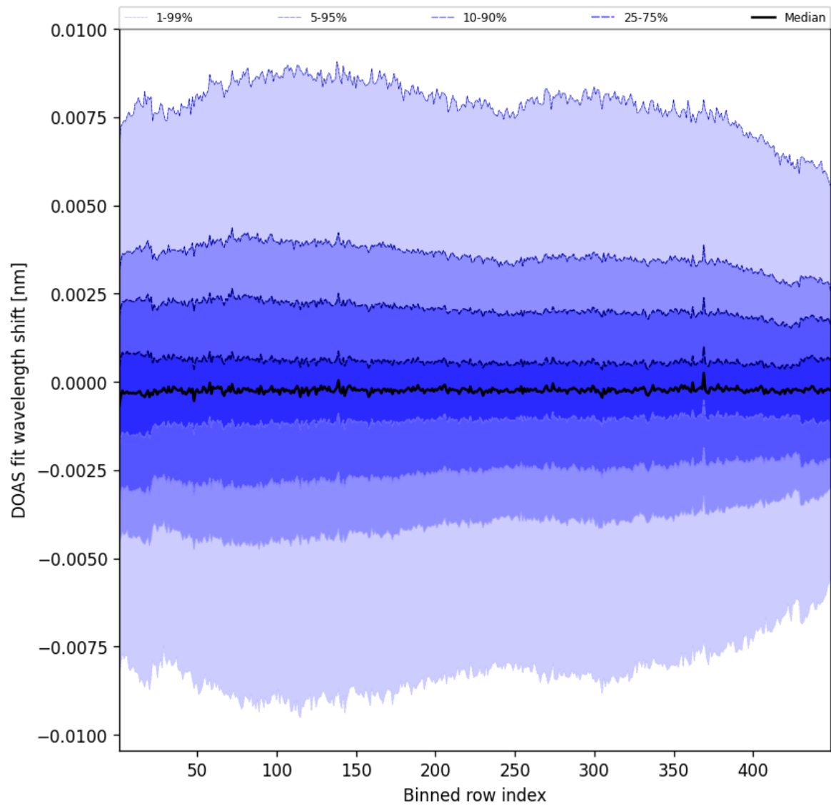
Figure 104: Along track statistics of “DOAS fit wavelength shift” for 2025-06-01 to 2025-06-02
