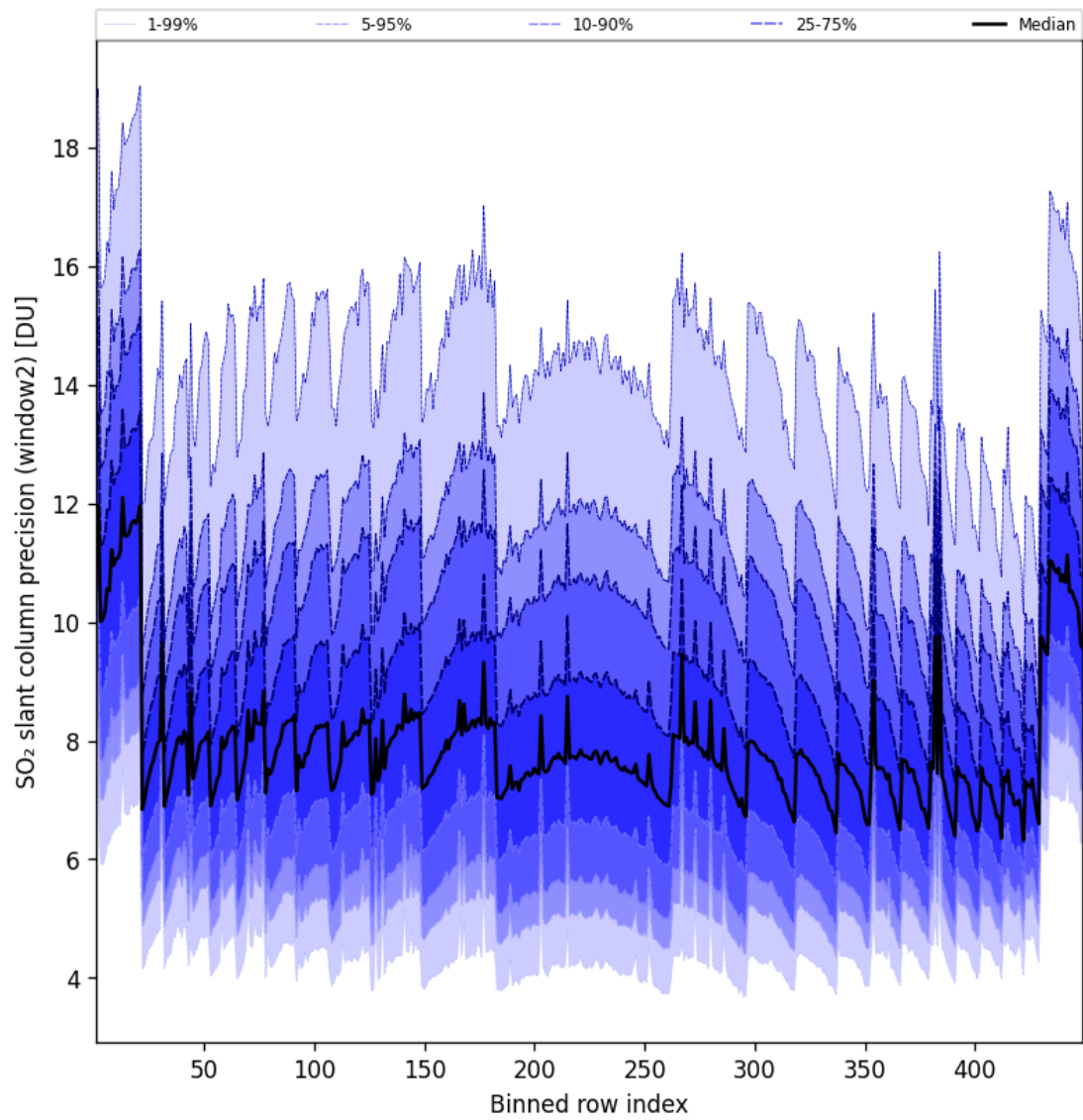
Figure 95: Along track statistics of “SO 2 slant column precision (window2)” for 2025-06-01 to 2025-06-02
