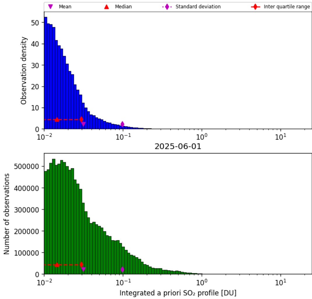
Figure 76: Histogram of “Integrated a priori SO 2 profile” for 2025-06-01 to 2025-06-02
