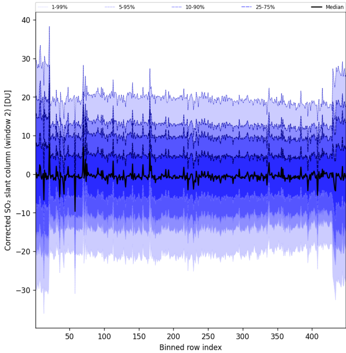
Figure 96: Along track statistics of “Corrected SO 2 slant column (window 2)” for 2025-06-01 to 2025-06-02
