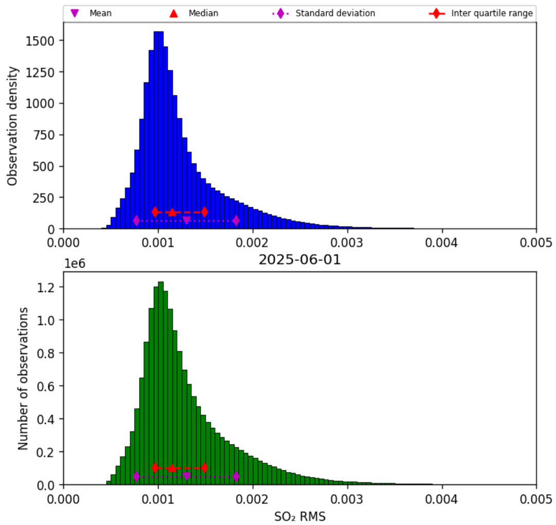
Figure 79: Histogram of “SO 2 RMS” for 2025-06-01 to 2025-06-02
