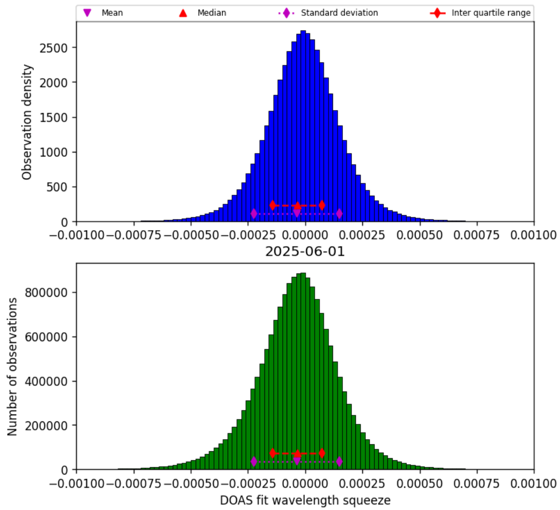
Figure 78: Histogram of “DOAS fit wavelength squeeze” for 2025-06-01 to 2025-06-02
