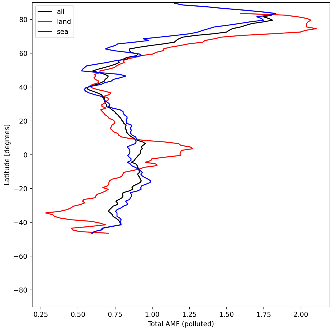
Figure 53: Zonal average of “Total AMF (polluted)” for 2025-06-01 to 2025-06-02.
