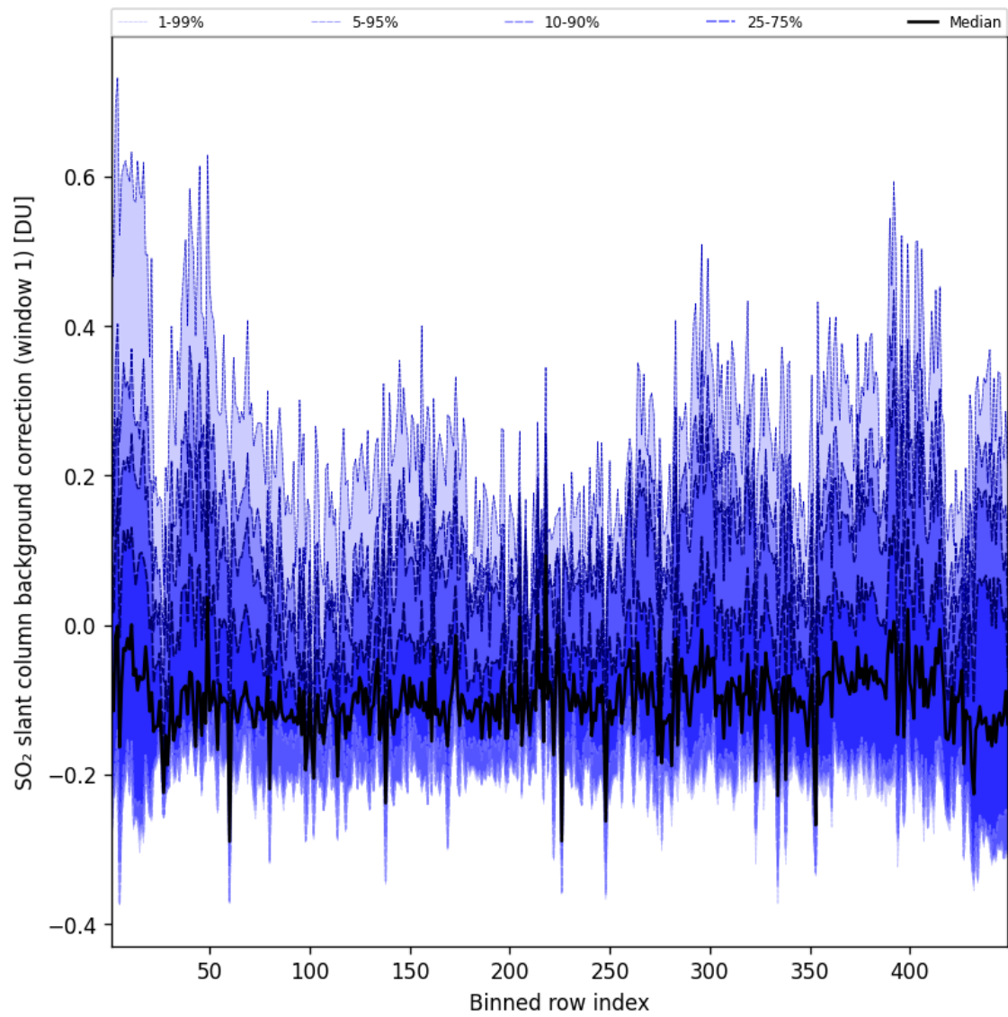
Figure 93: Along track statistics of “SO 2 slant column background correction (window 1)” for 2025-06-01 to 2025-06-02
