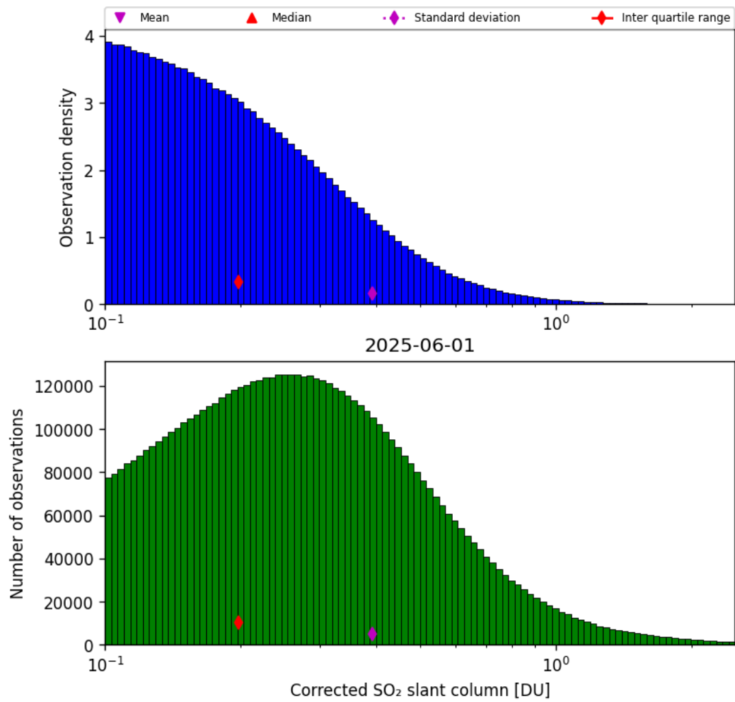
Figure 60: Histogram of “Corrected SO 2 slant column” for 2025-06-01 to 2025-06-02
