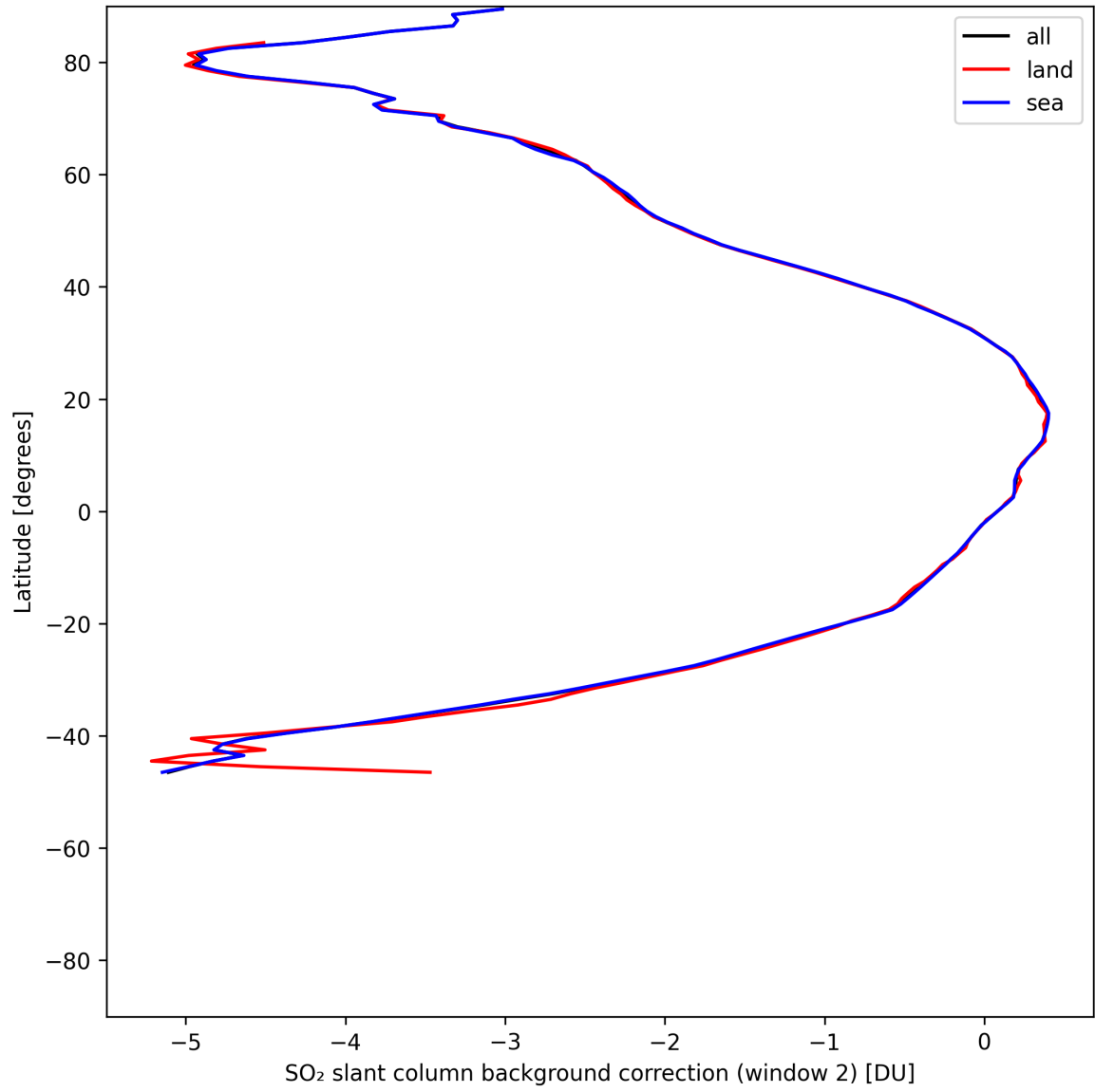
Figure 43: Zonal average of “SO 2 slant column background correction (window 2)” for 2025-06-01 to 2025-06-02.
