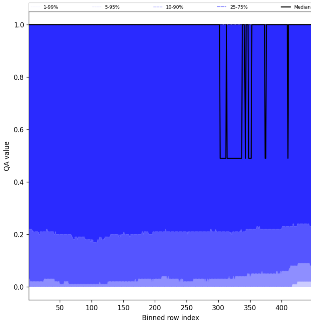
Figure 84: Along track statistics of “QA value” for 2025-06-01 to 2025-06-02
