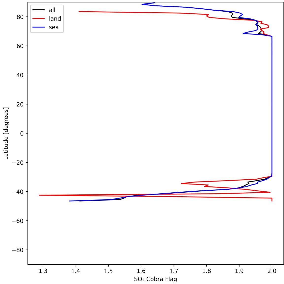
Figure 48: Zonal average of "SO 2 Cobra Flag" for 2025-06-01 to 2025-06-02.
