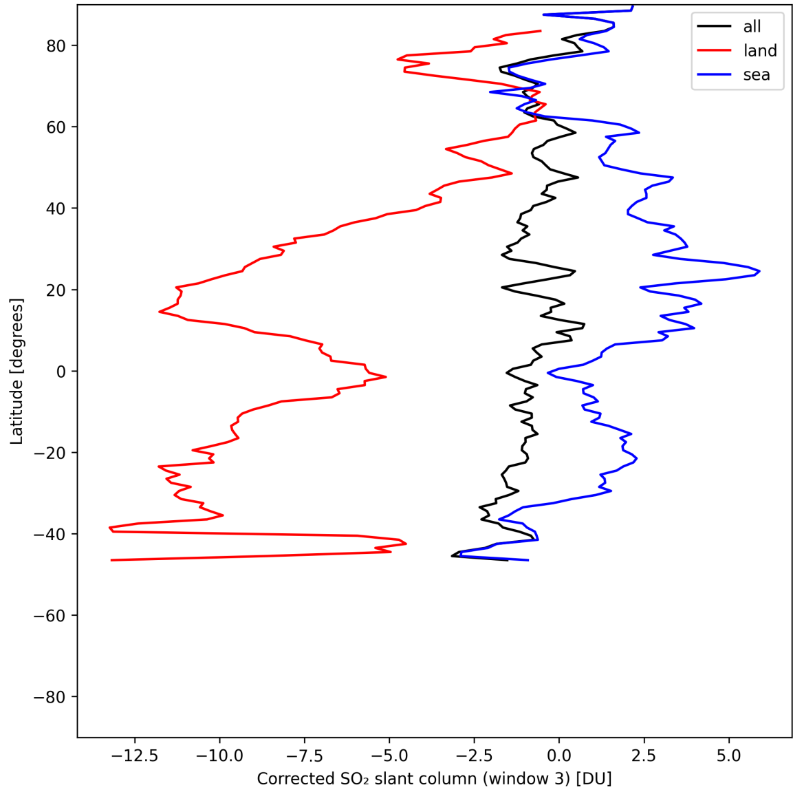
Figure 46: Zonal average of “Corrected SO 2 slant column (window 3)” for 2025-06-01 to 2025-06-02.
