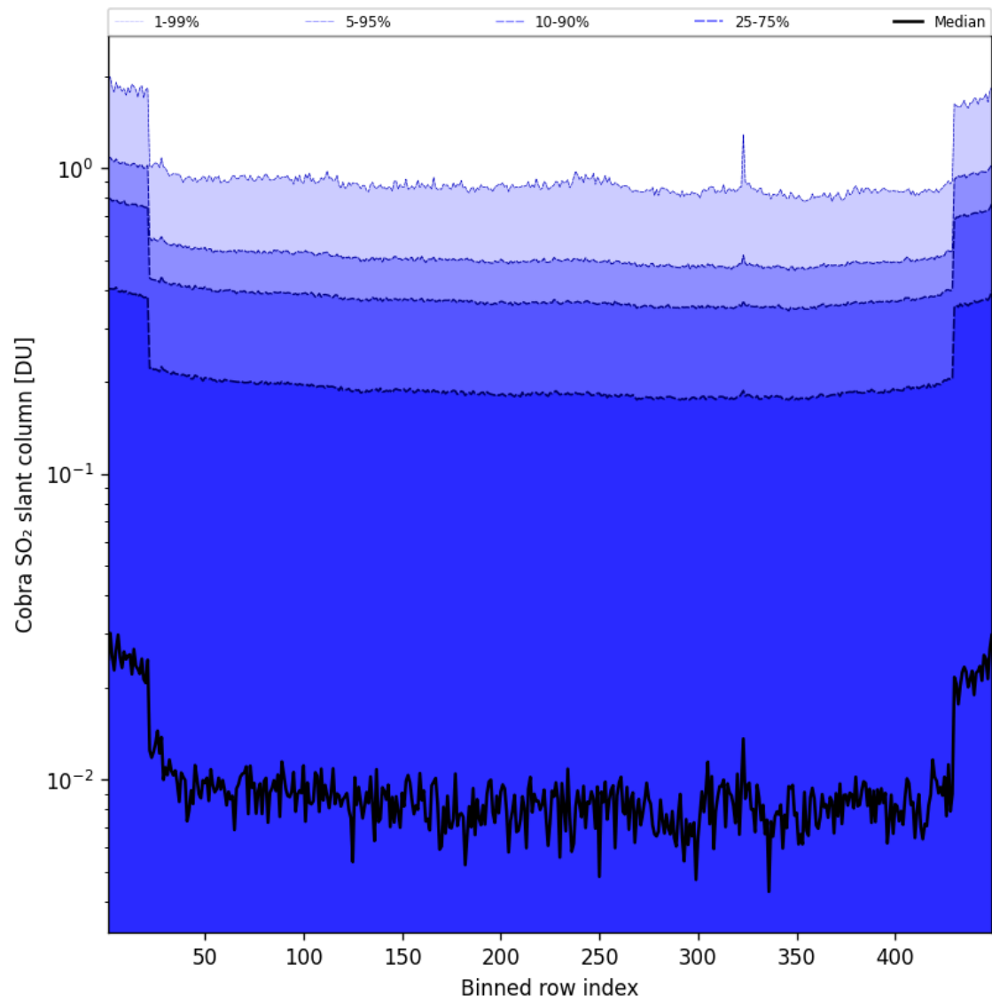
Figure 88: Along track statistics of “Cobra SO 2 slant column” for 2025-06-01 to 2025-06-02
