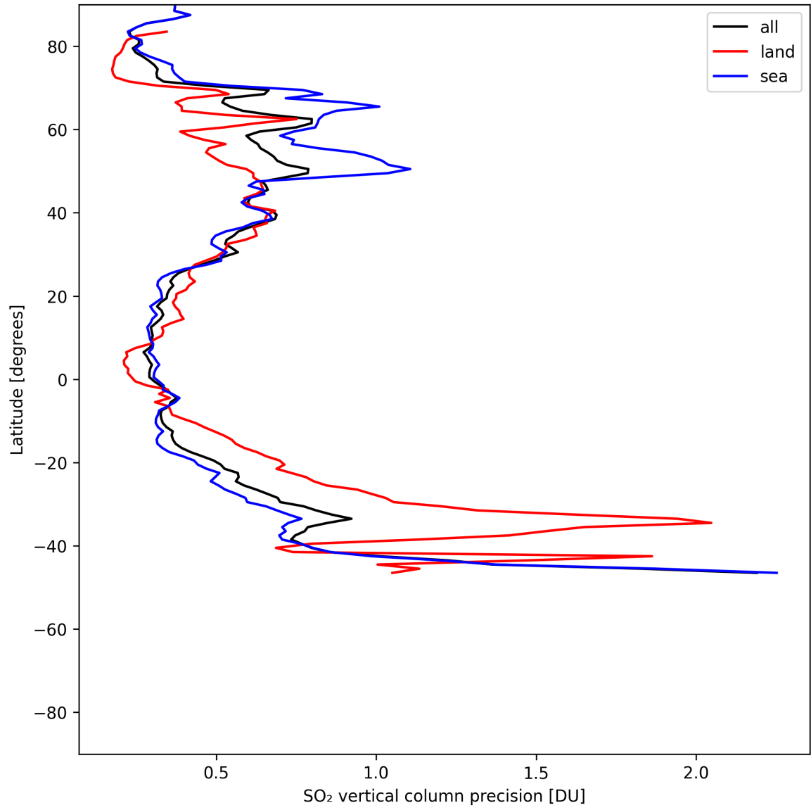
Figure 32: Zonal average of “SO 2 vertical column precision” for 2025-06-01 to 2025-06-02.
