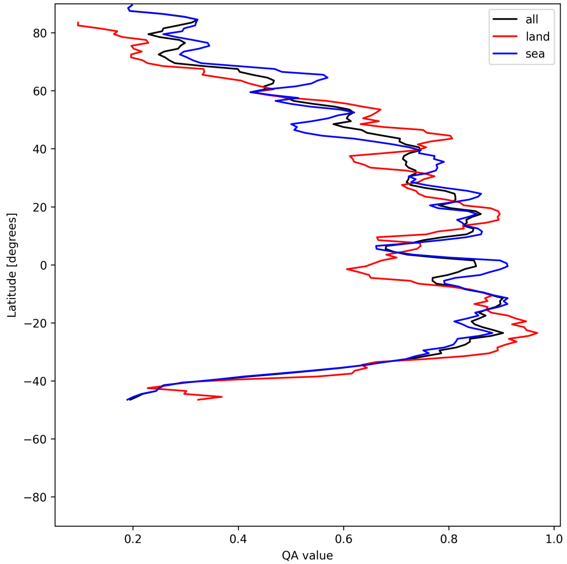
Figure 30: Zonal average of “QA value” for 2025-06-01 to 2025-06-02.
