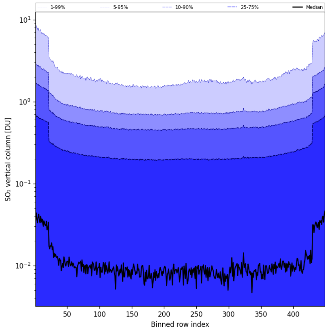
Figure 85: Along track statistics of “SO 2 vertical column” for 2025-06-01 to 2025-06-02
