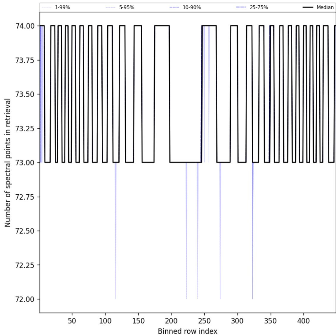
Figure 110: Along track statistics of “Number of spectral points in retrieval” for 2025-06-01 to 2025-06-02
