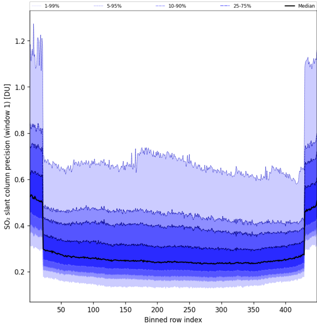
Figure 91: Along track statistics of “SO 2 slant column precision (window 1)” for 2025-06-01 to 2025-06-02
