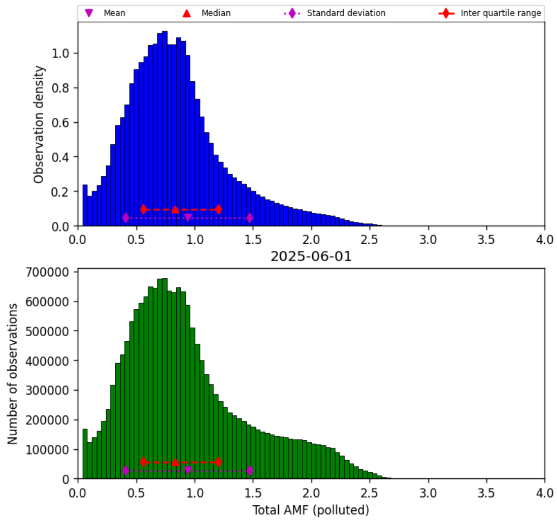
Figure 80: Histogram of “Total AMF (polluted)” for 2025-06-01 to 2025-06-02
