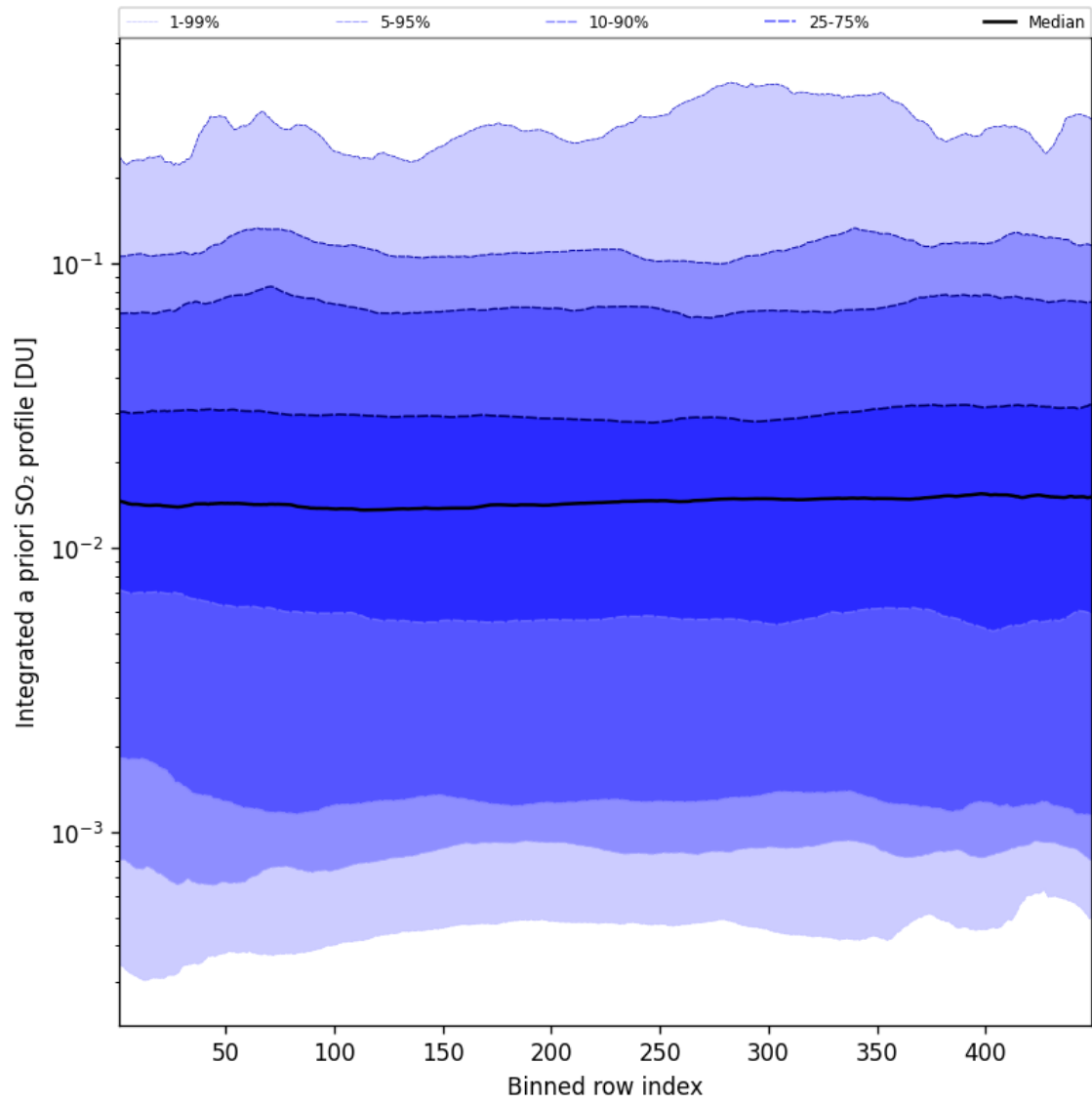
Figure 103: Along track statistics of “Integrated a priori SO 2 profile” for 2025-06-01 to 2025-06-02
