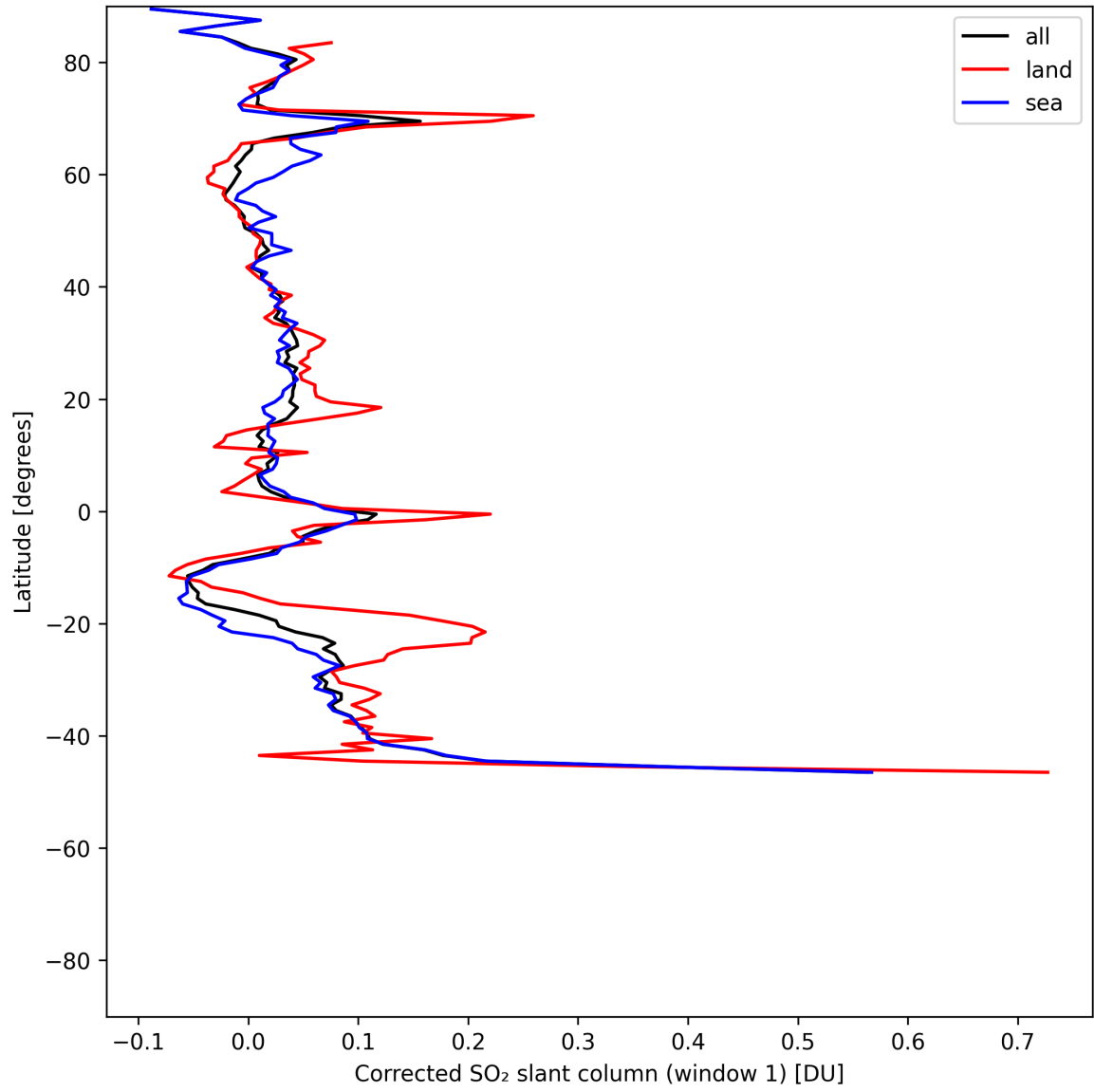
Figure 38: Zonal average of “Corrected SO 2 slant column (window 1)” for 2025-06-01 to 2025-06-02.
