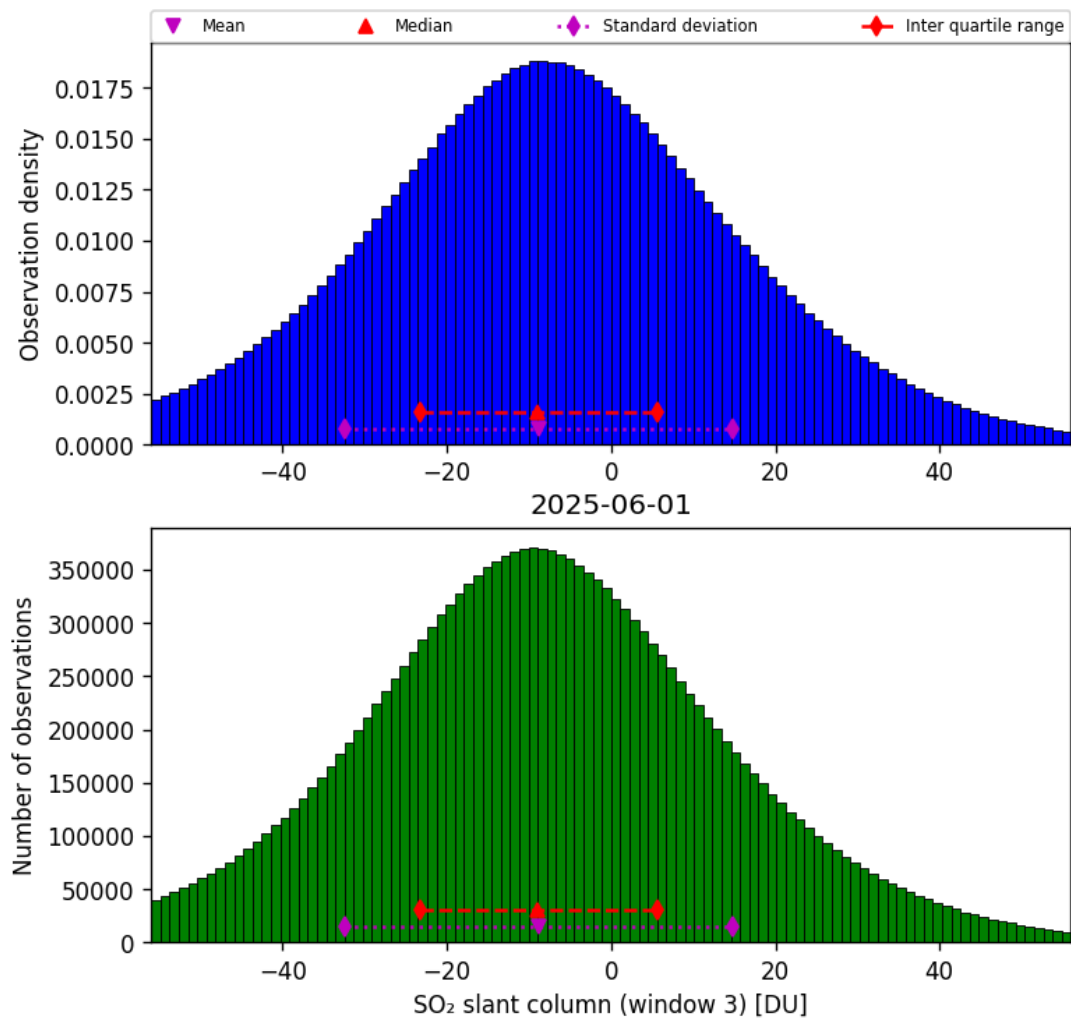
Figure 71: Histogram of “SO 2 slant column (window 3)” for 2025-06-01 to 2025-06-02
