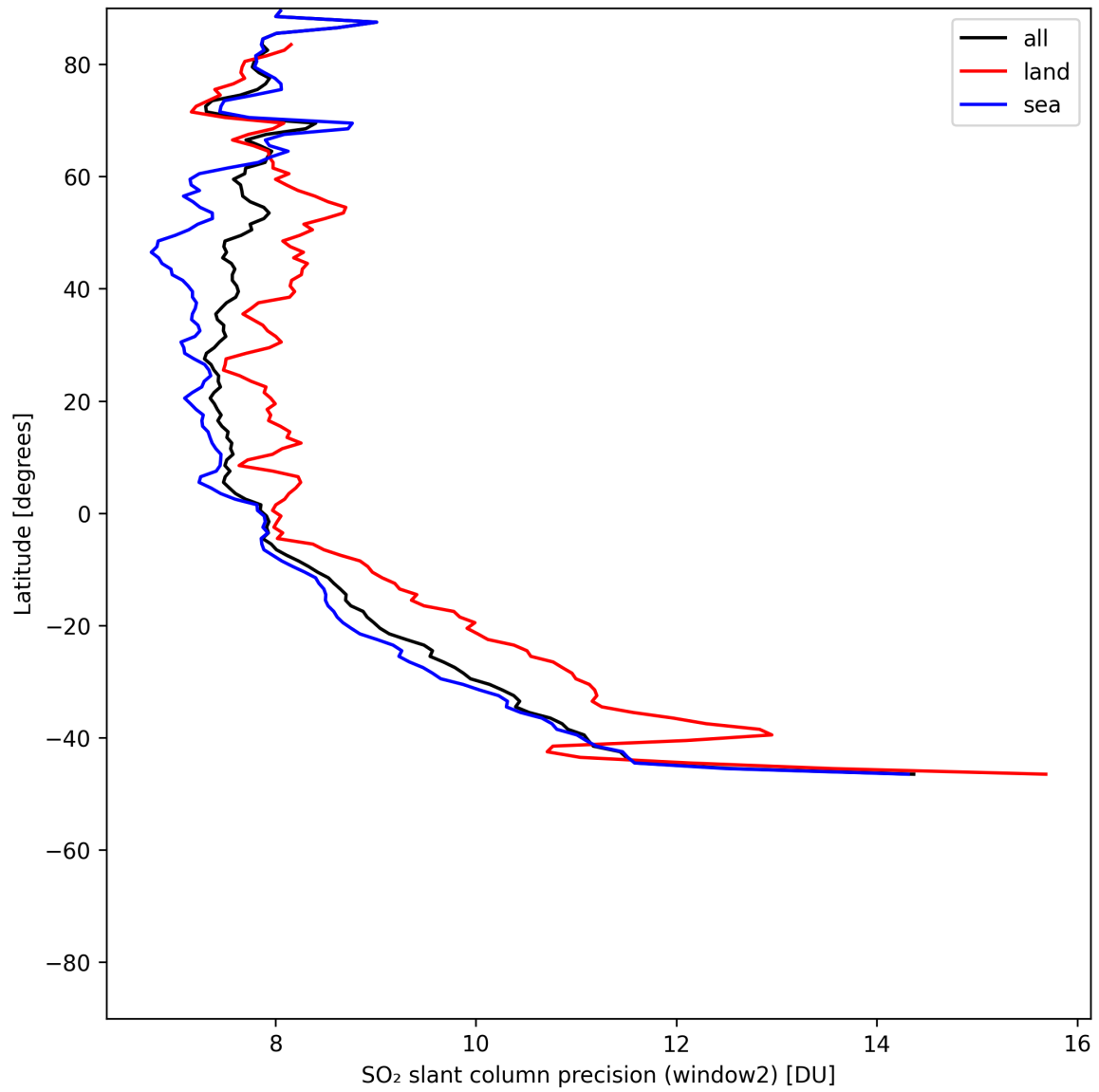
Figure 41: Zonal average of “SO 2 slant column precision (window2)” for 2025-06-01 to 2025-06-02.
