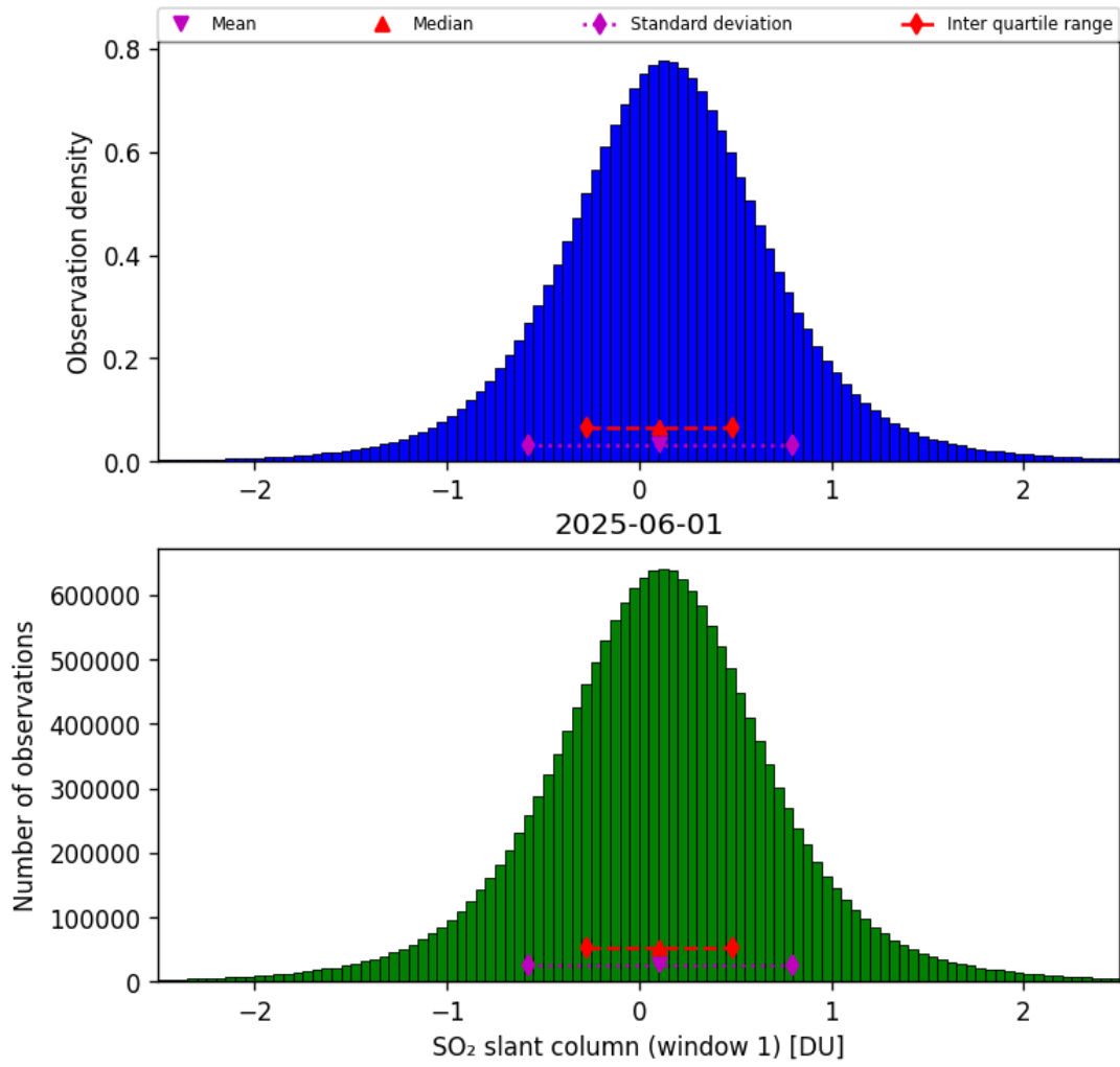
Figure 63: Histogram of “SO 2 slant column (window 1)” for 2025-06-01 to 2025-06-02
