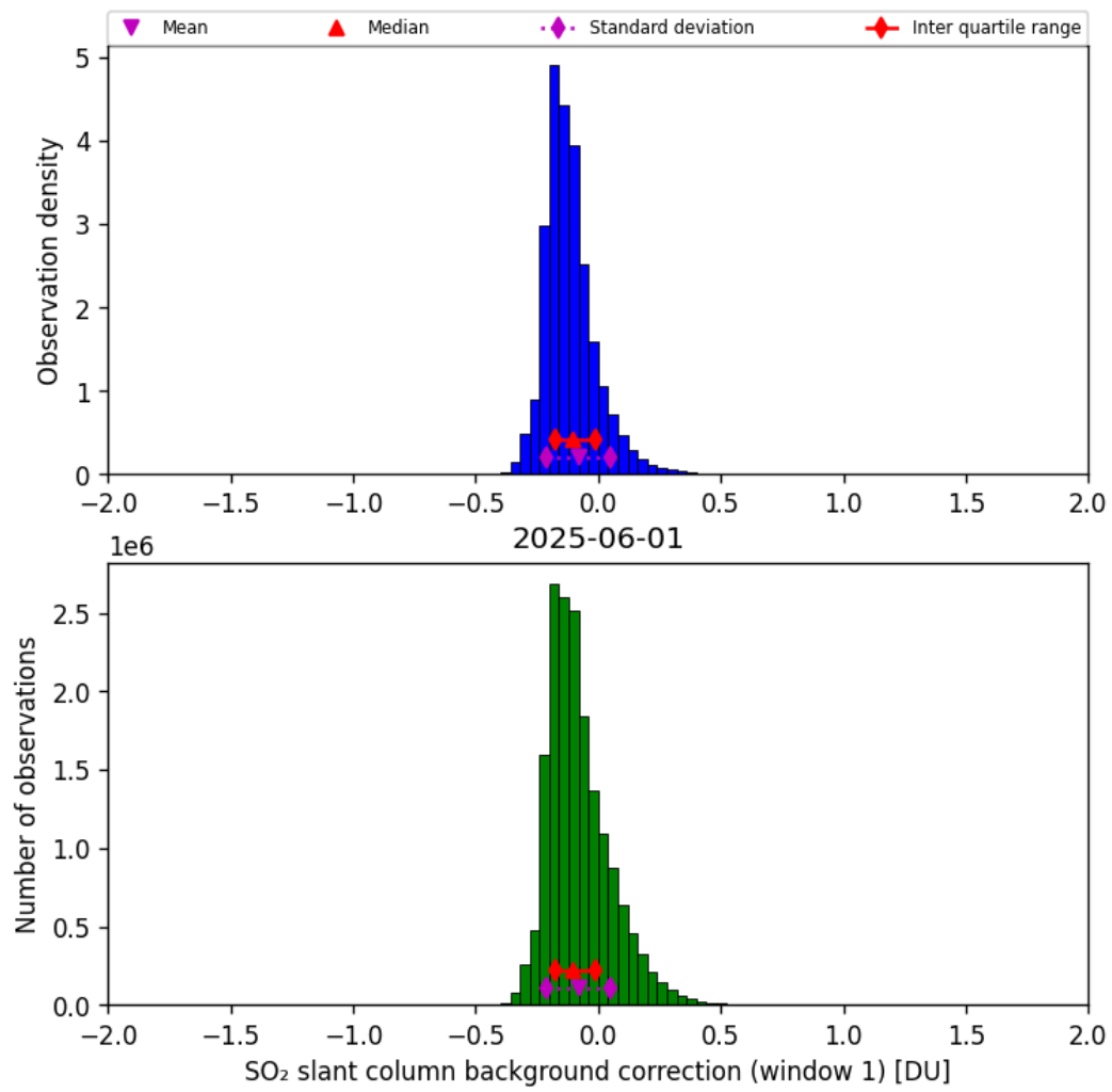
Figure 66: Histogram of “SO 2 slant column background correction (window 1)” for 2025-06-01 to 2025-06-02
