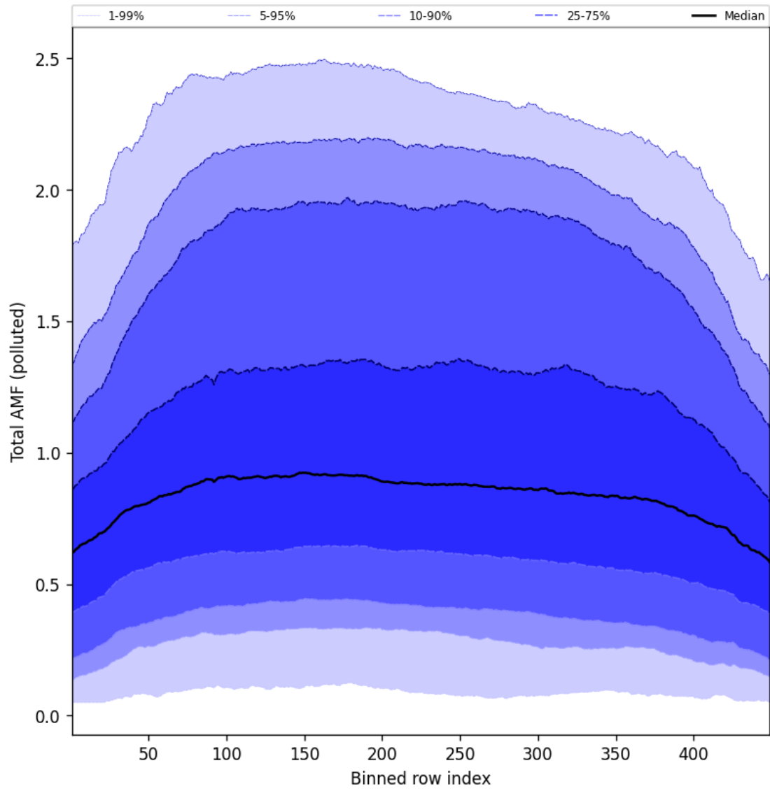
Figure 107: Along track statistics of “Total AMF (polluted)” for 2025-06-01 to 2025-06-02
