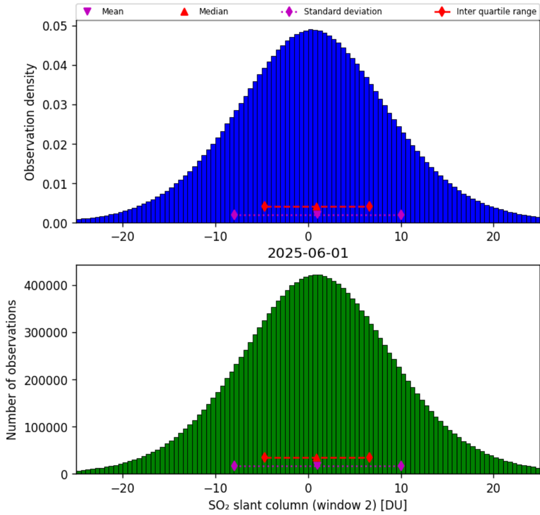
Figure 67: Histogram of “SO 2 slant column (window 2)” for 2025-06-01 to 2025-06-02
