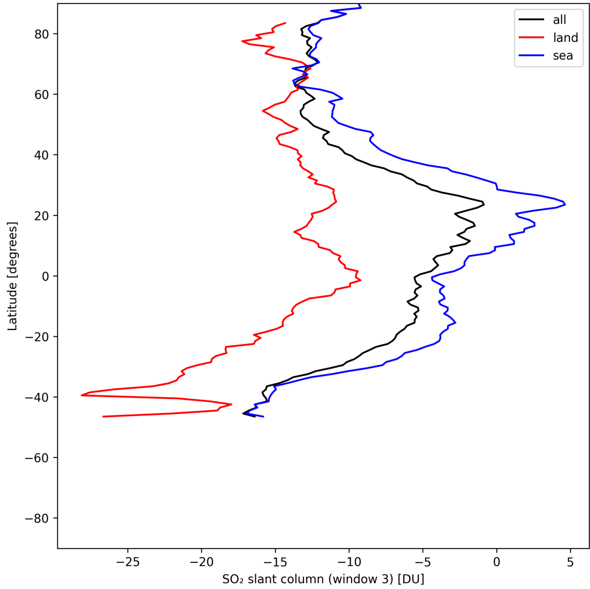
Figure 44: Zonal average of “SO 2 slant column (window 3)” for 2025-06-01 to 2025-06-02.
