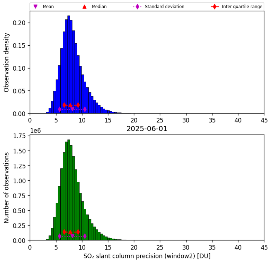
Figure 68: Histogram of “SO 2 slant column precision (window2)” for 2025-06-01 to 2025-06-02
