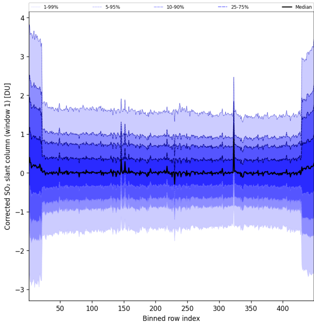
Figure 92: Along track statistics of “Corrected SO 2 slant column (window 1)” for 2025-06-01 to 2025-06-02
