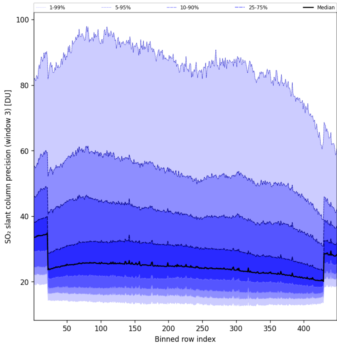
Figure 99: Along track statistics of “SO 2 slant column precision (window 3)” for 2025-06-01 to 2025-06-02
