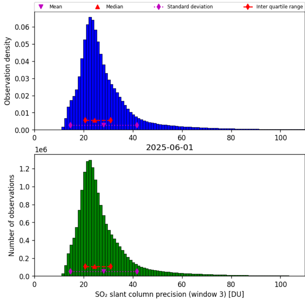
Figure 72: Histogram of “SO 2 slant column precision (window 3)” for 2025-06-01 to 2025-06-02
