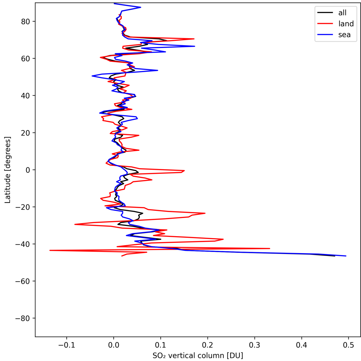
Figure 31: Zonal average of “SO 2 vertical column” for 2025-06-01 to 2025-06-02.
