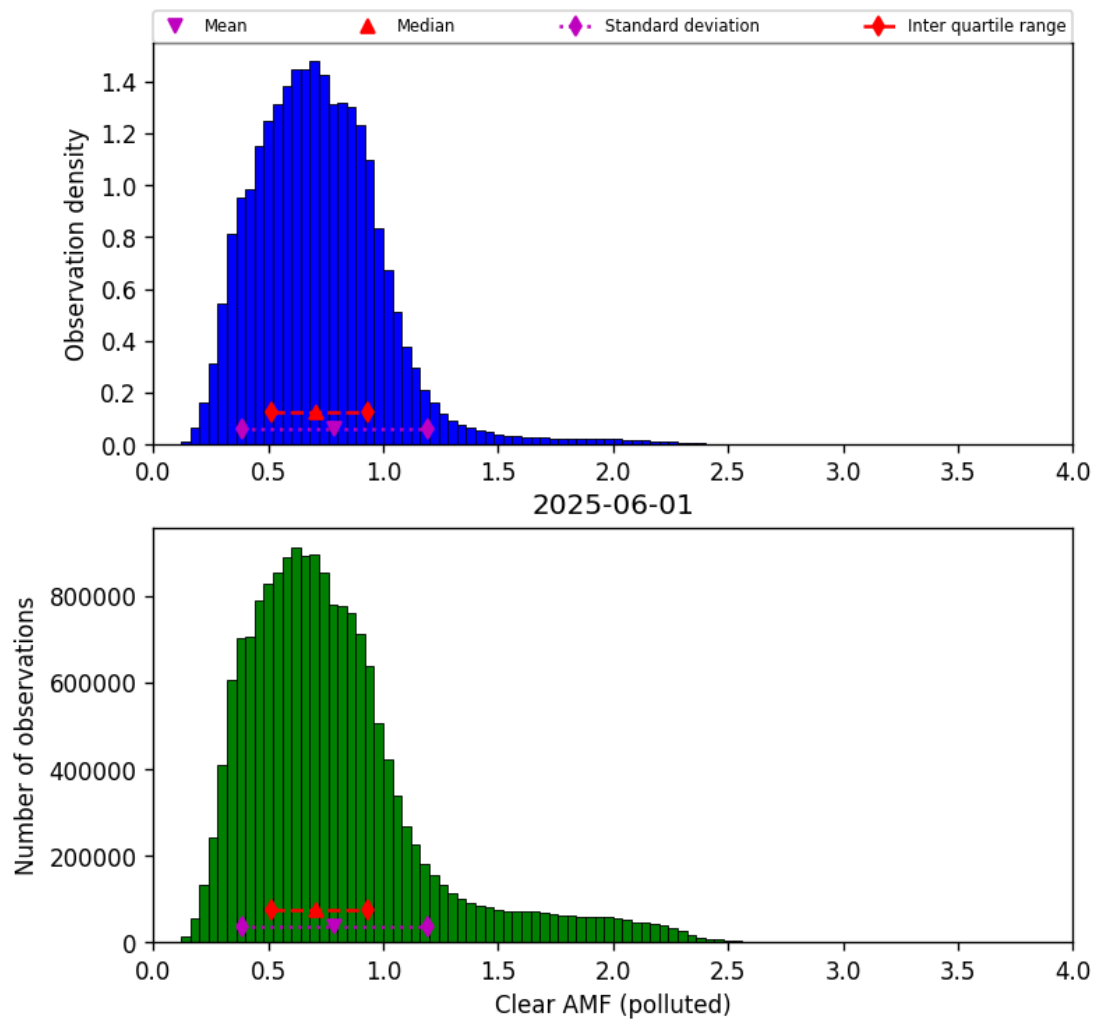
Figure 82: Histogram of “Clear AMF (polluted)” for 2025-06-01 to 2025-06-02
