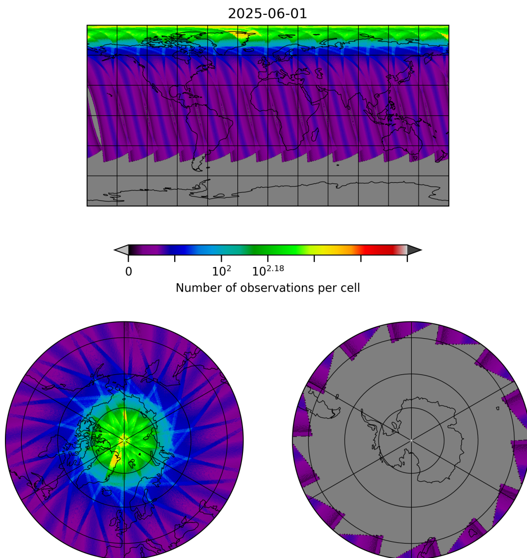
Figure 29: Map of the number of observations for 2025-06-01 to 2025-06-02
