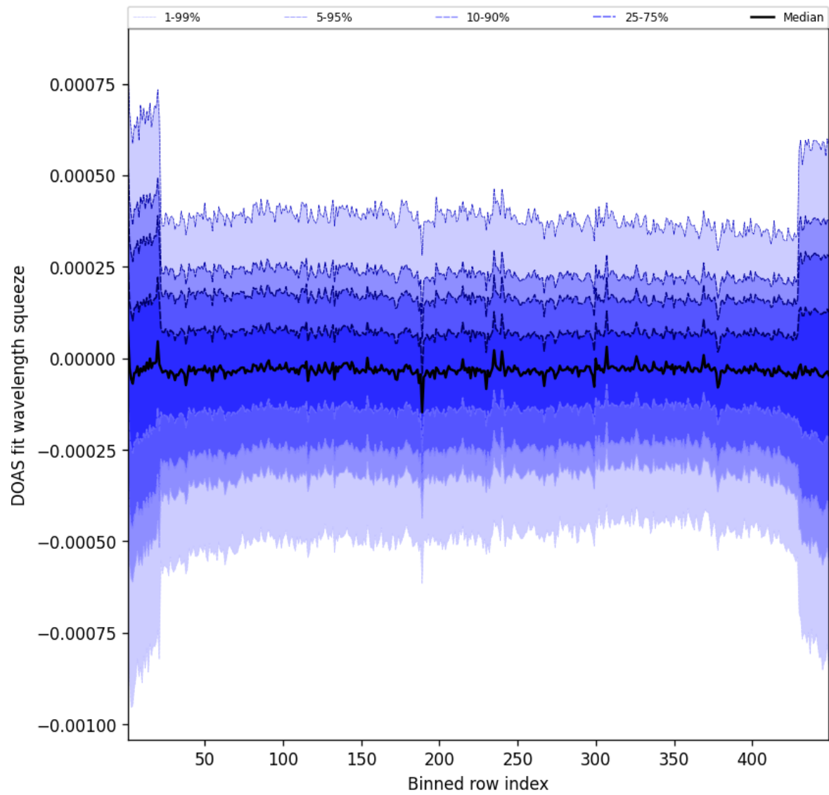
Figure 105: Along track statistics of “DOAS fit wavelength squeeze” for 2025-06-01 to 2025-06-02
