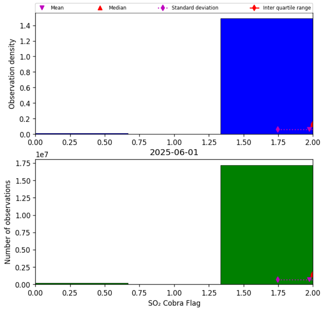
Figure 75: Histogram of “SO 2 Cobra Flag” for 2025-06-01 to 2025-06-02
