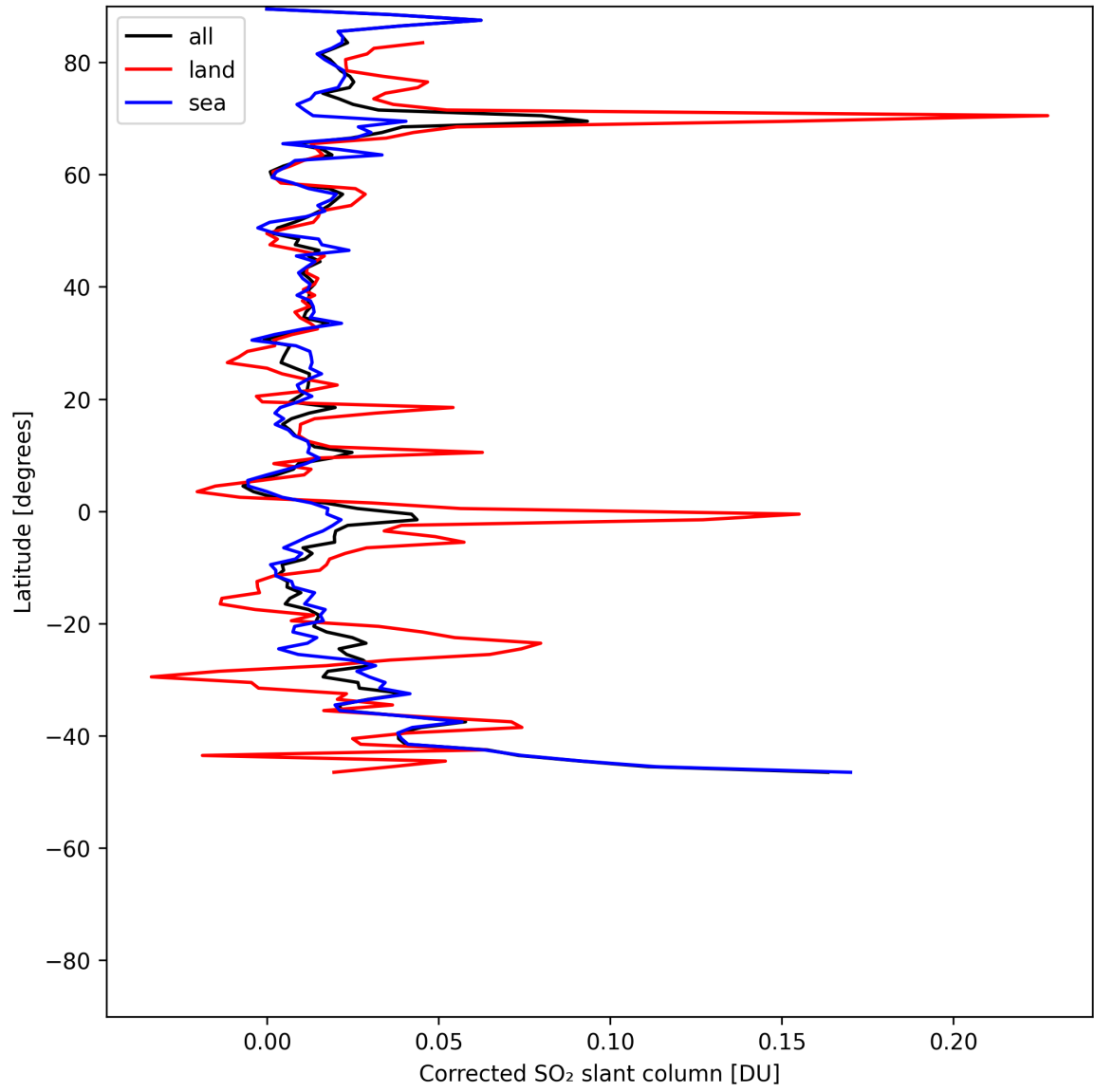
Figure 33: Zonal average of “Corrected SO 2 slant column” for 2025-06-01 to 2025-06-02.
