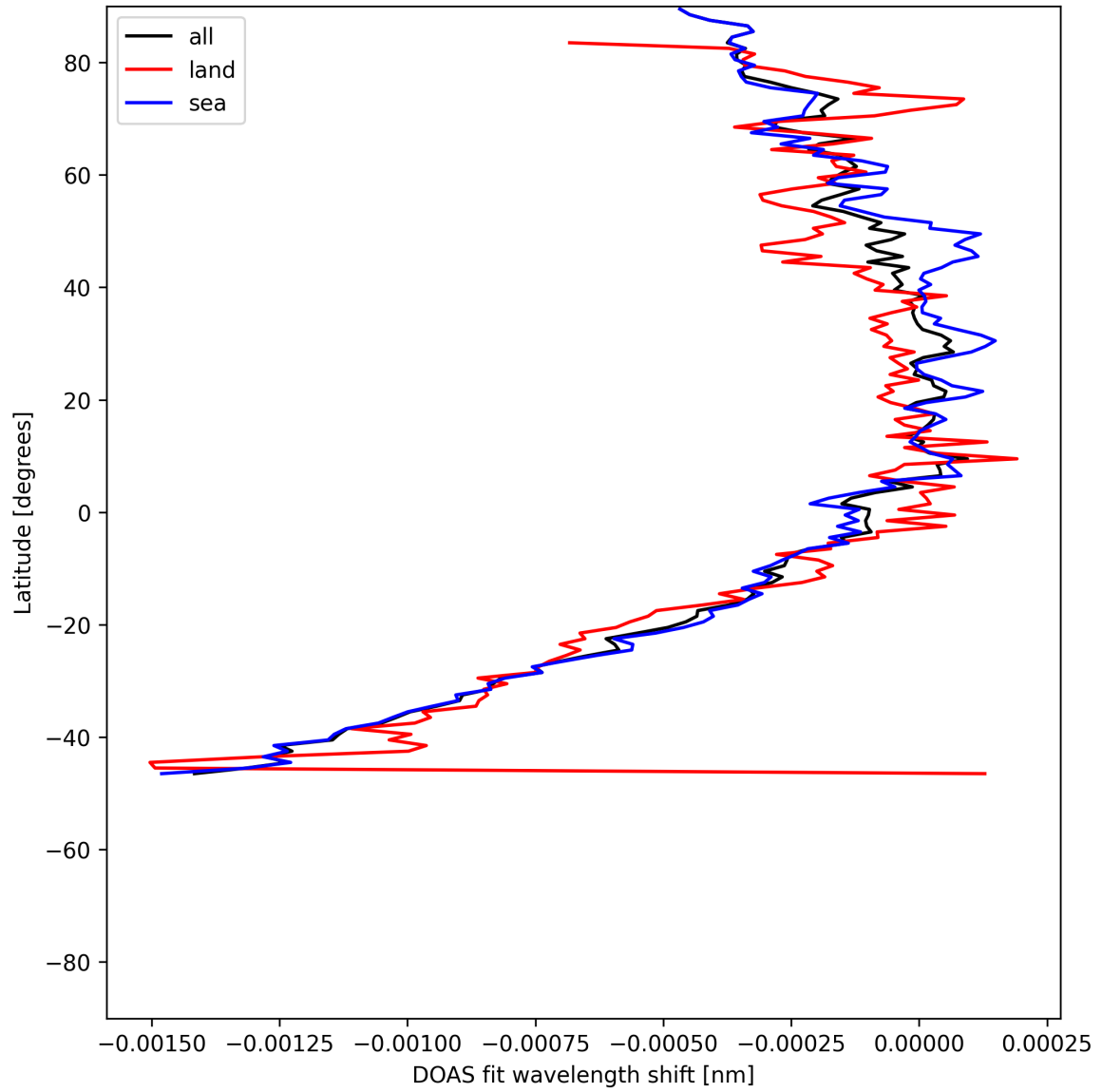
Figure 50: Zonal average of “DOAS fit wavelength shift” for 2025-06-01 to 2025-06-02.
