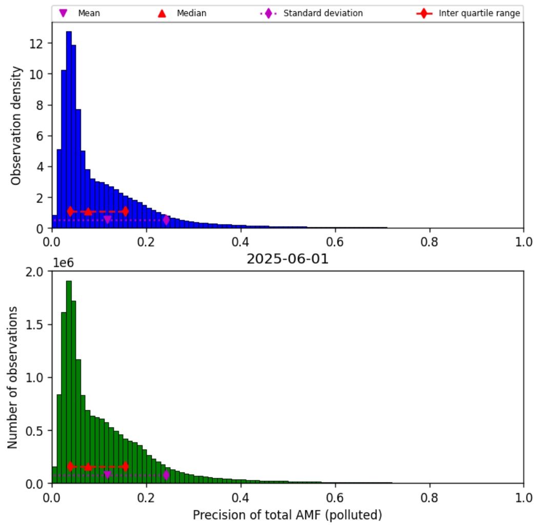
Figure 81: Histogram of “Precision of total AMF (polluted)” for 2025-06-01 to 2025-06-02
