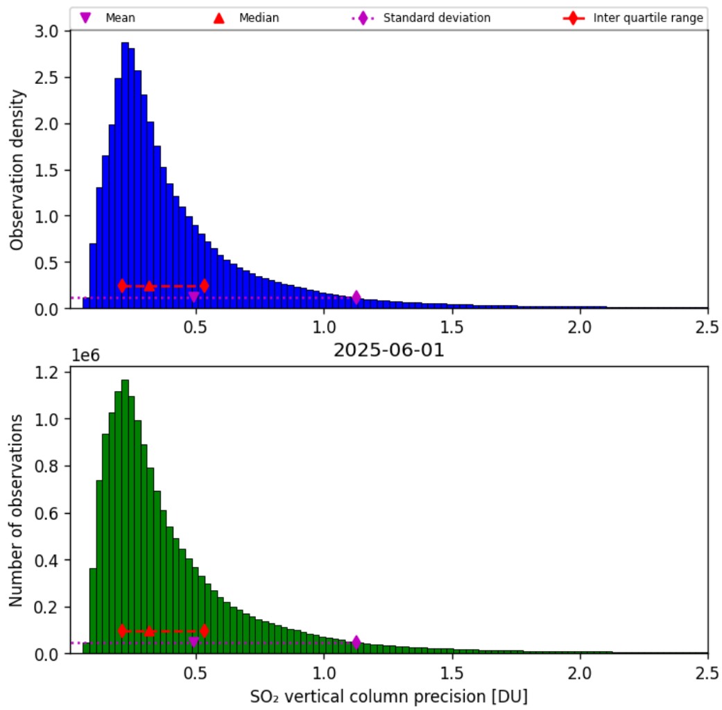
Figure 59: Histogram of “SO 2 vertical column precision” for 2025-06-01 to 2025-06-02
