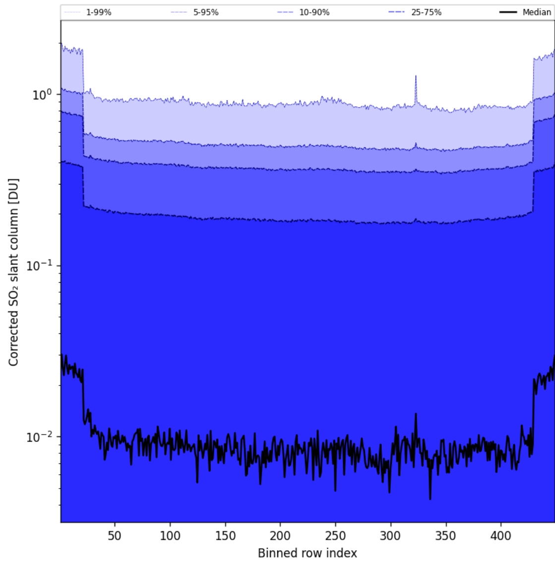
Figure 87: Along track statistics of "Corrected SO 2 slant column" for 2025-06-01 to 2025-06-02
