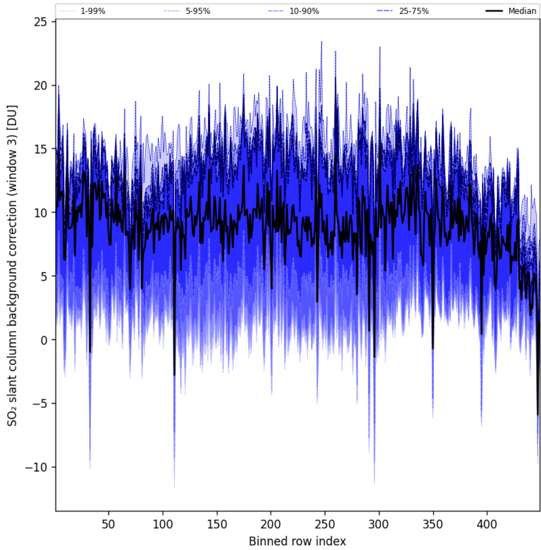
Figure 101: Along track statistics of “SO 2 slant column background correction (window 3)” for 2025-06-01 to 2025-06-02
