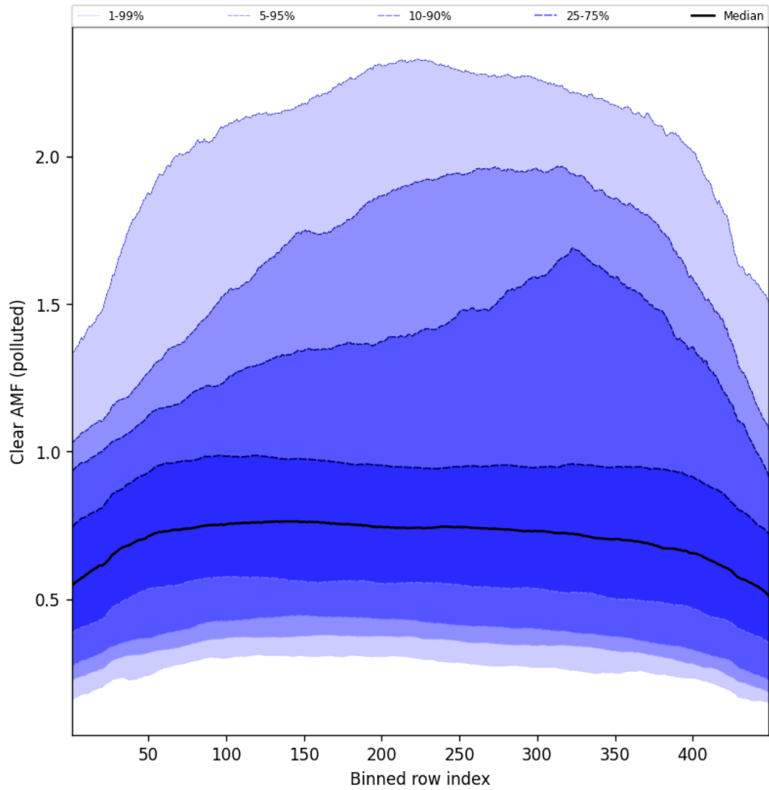
Figure 109: Along track statistics of “Clear AMF (polluted)” for 2025-06-01 to 2025-06-02
