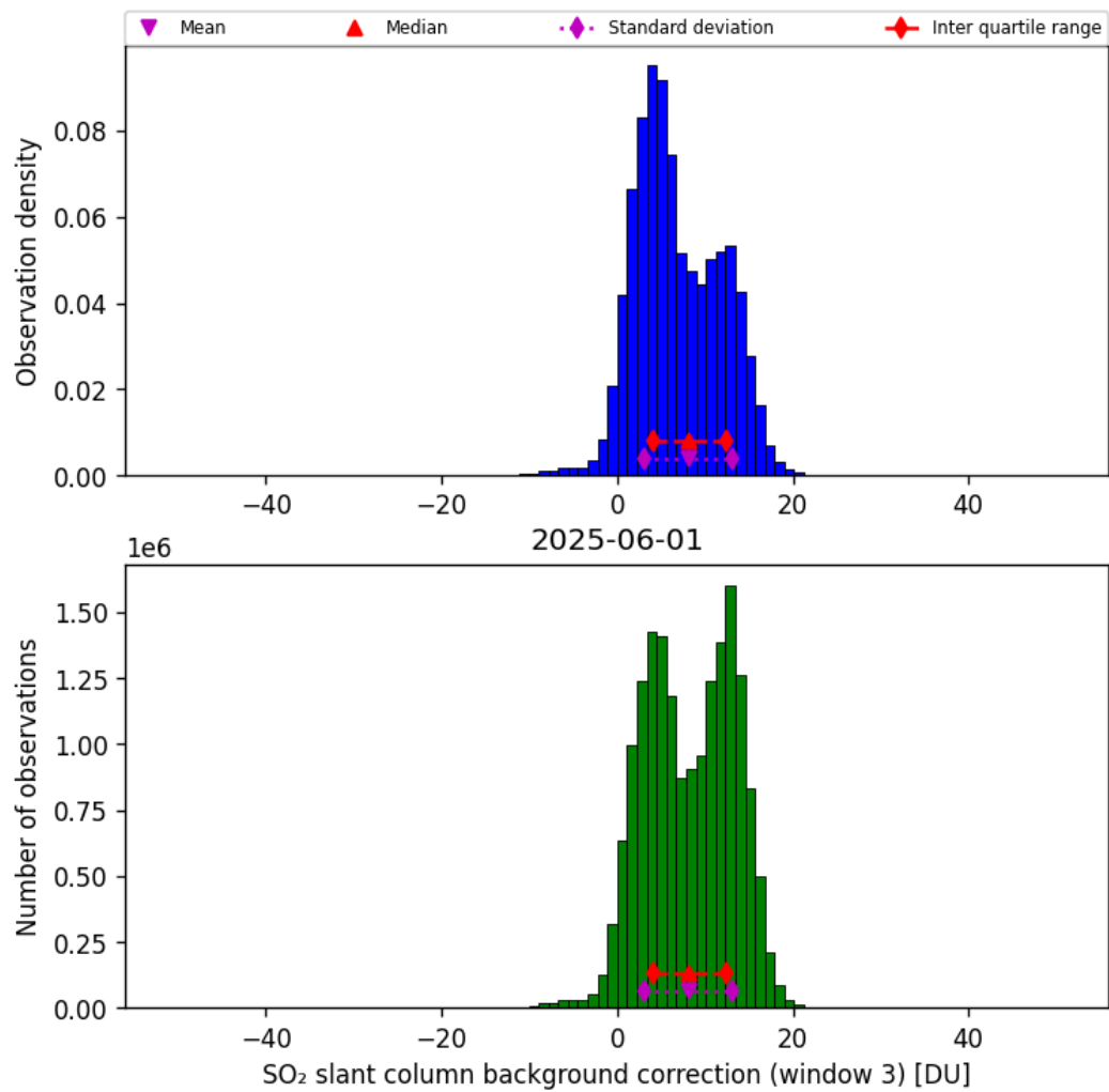
Figure 74: Histogram of “SO 2 slant column background correction (window 3)” for 2025-06-01 to 2025-06-02
