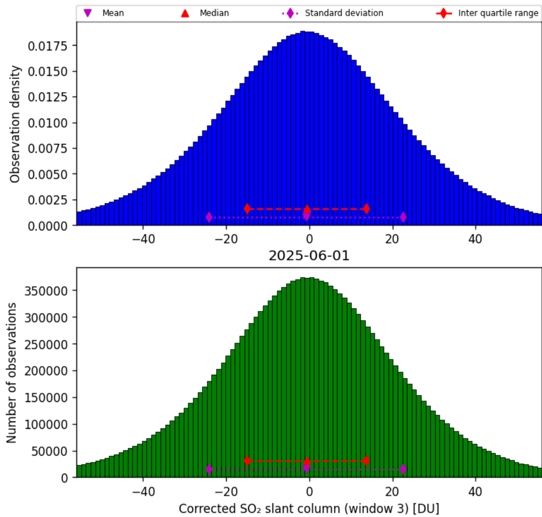
Figure 73: Histogram of “Corrected SO 2 slant column (window 3)” for 2025-06-01 to 2025-06-02
