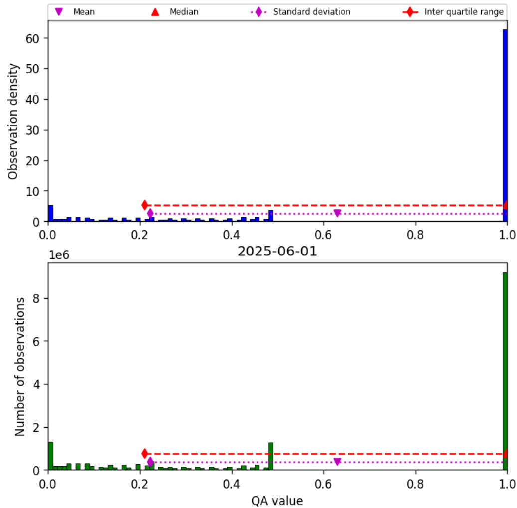
Figure 57: Histogram of “QA value” for 2025-06-01 to 2025-06-02
