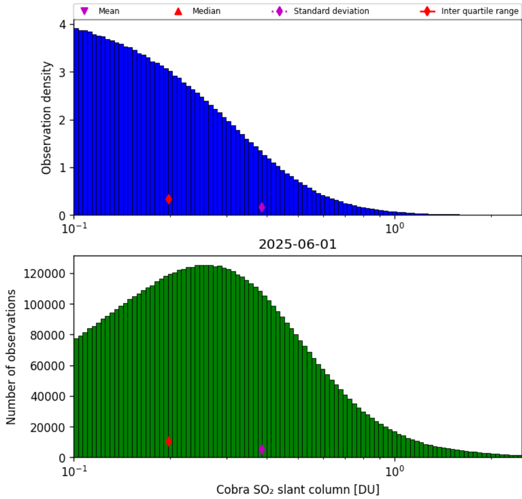
Figure 61: Histogram of “Cobra SO 2 slant column” for 2025-06-01 to 2025-06-02
