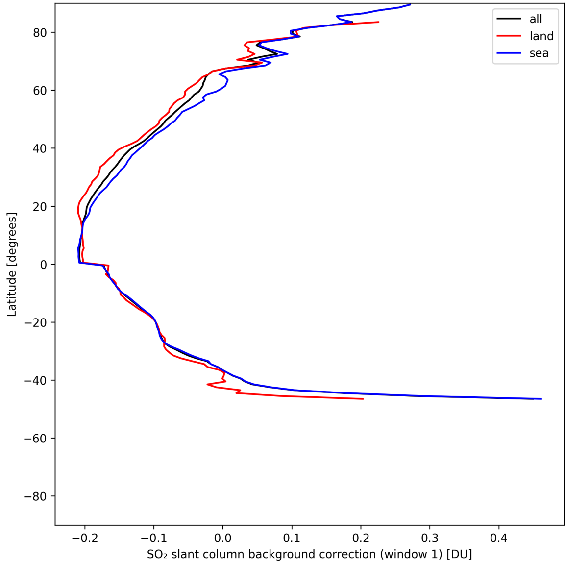
Figure 39: Zonal average of “SO 2 slant column background correction (window 1)” for 2025-06-01 to 2025-06-02.
