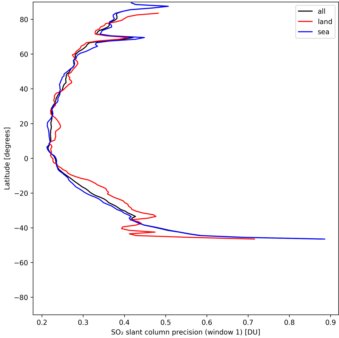
Figure 37: Zonal average of “SO 2 slant column precision (window 1)” for 2025-06-01 to 2025-06-02.
