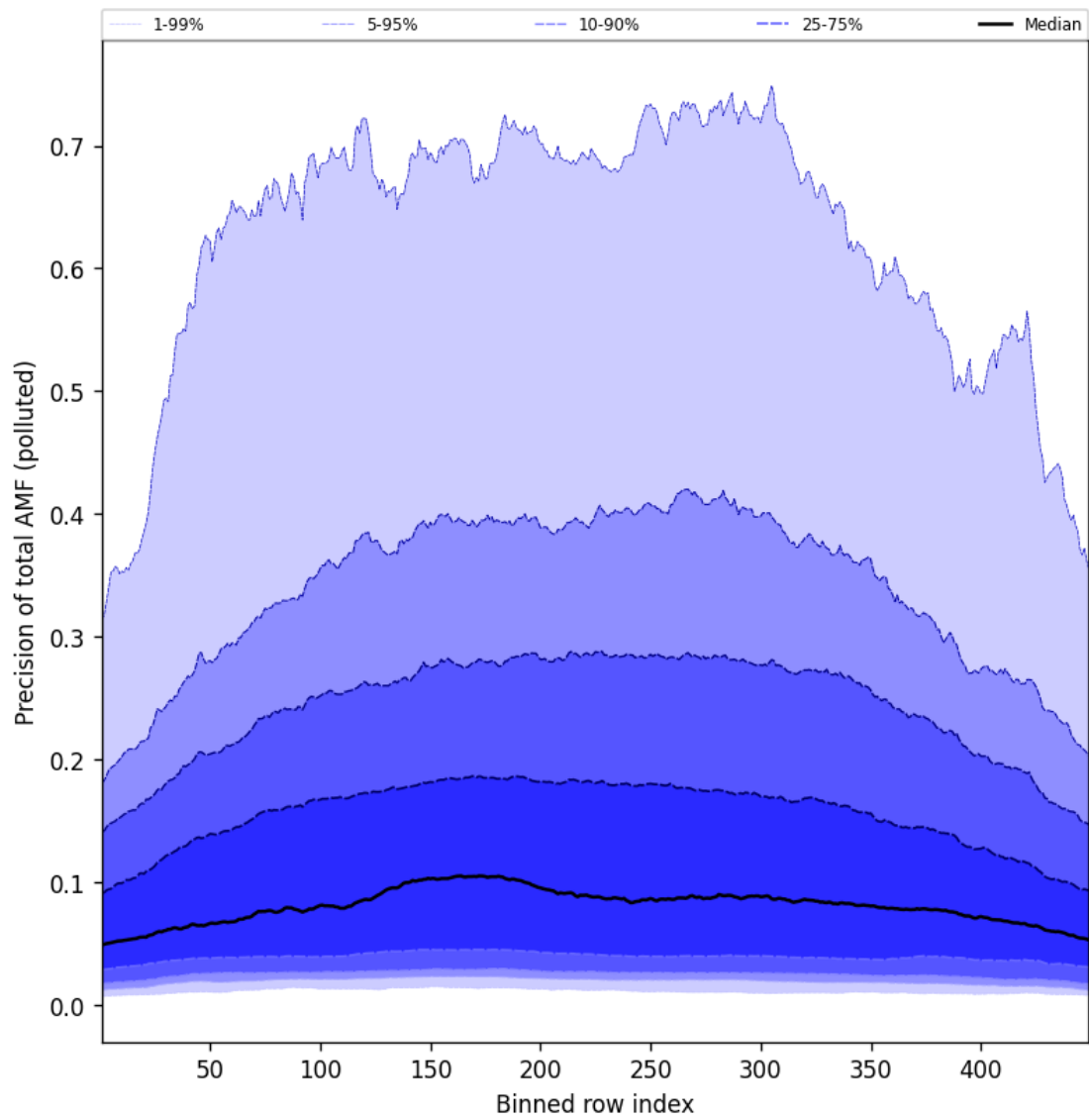
Figure 108: Along track statistics of “Precision of total AMF (polluted)” for 2025-06-01 to 2025-06-02
