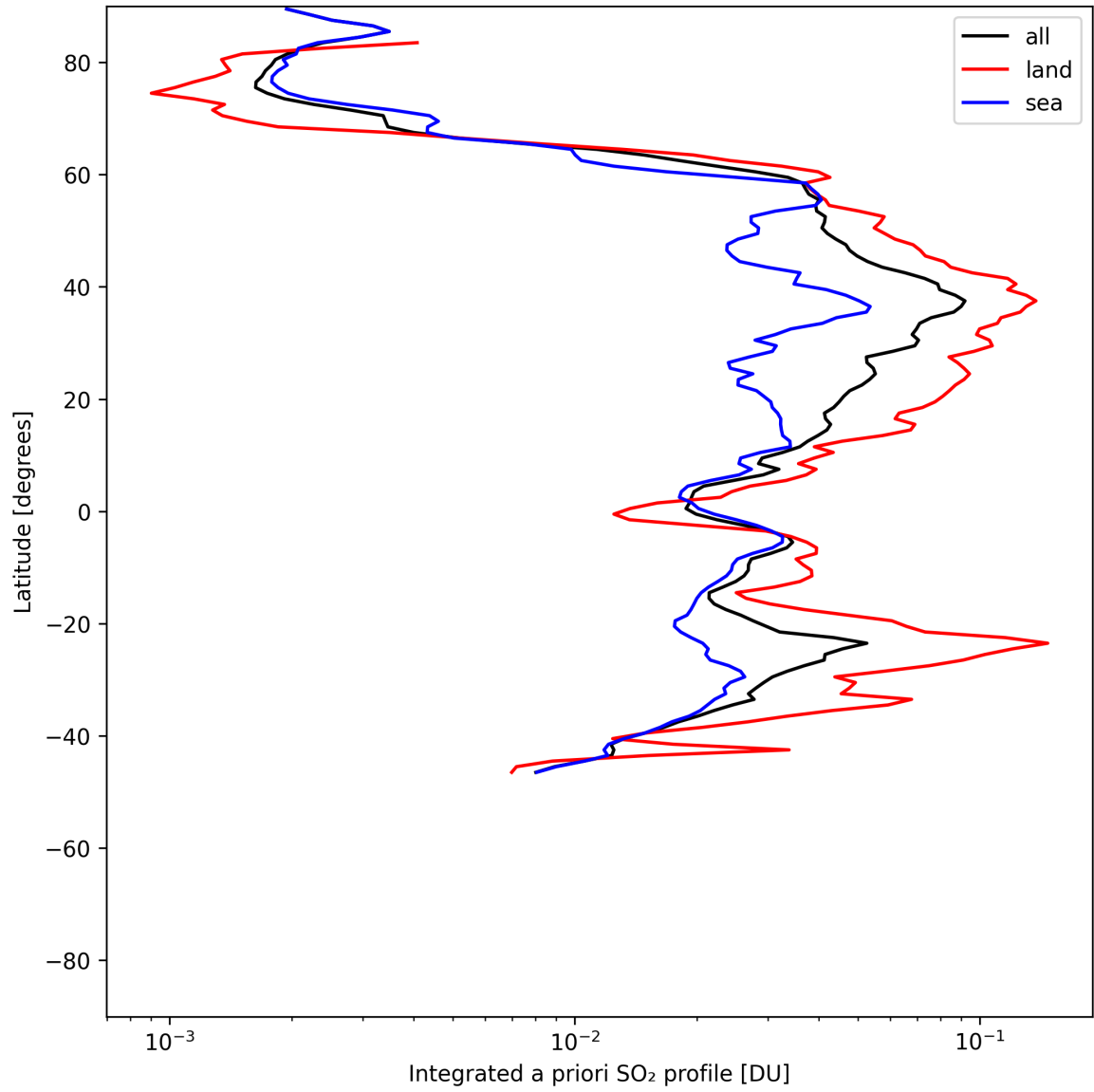
Figure 49: Zonal average of “Integrated a priori SO 2 profile” for 2025-06-01 to 2025-06-02.
