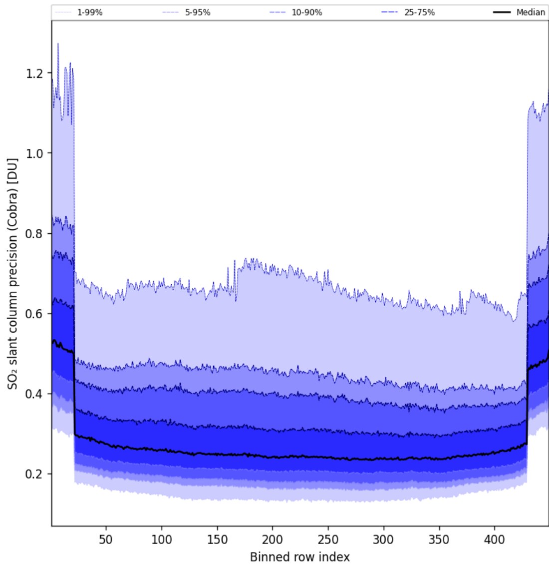
Figure 89: Along track statistics of “SO 2 slant column precision (Cobra)” for 2025-06-01 to 2025-06-02
