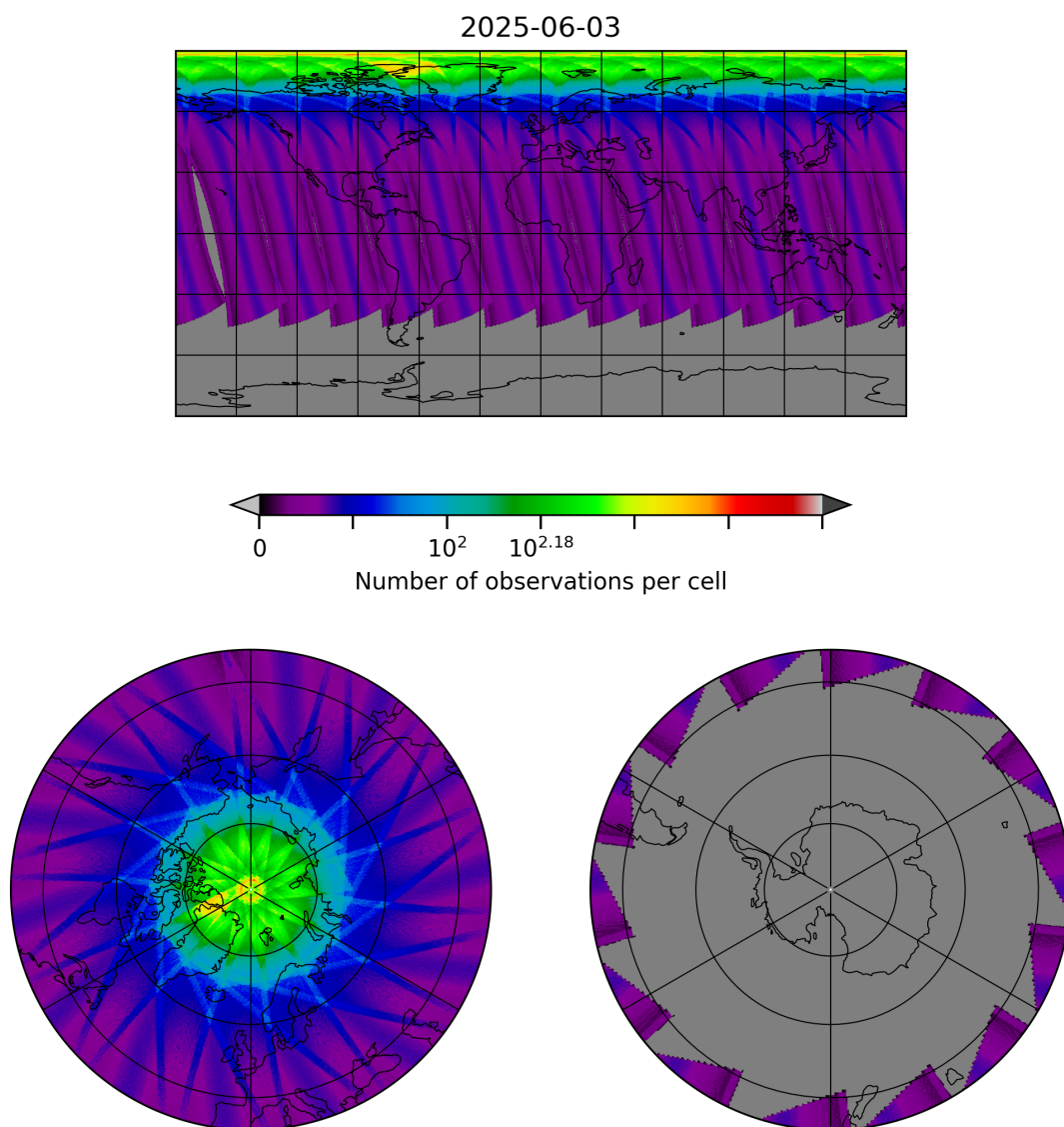
Figure 29: Map of the number of observations for 2025-06-03 to 2025-06-04
