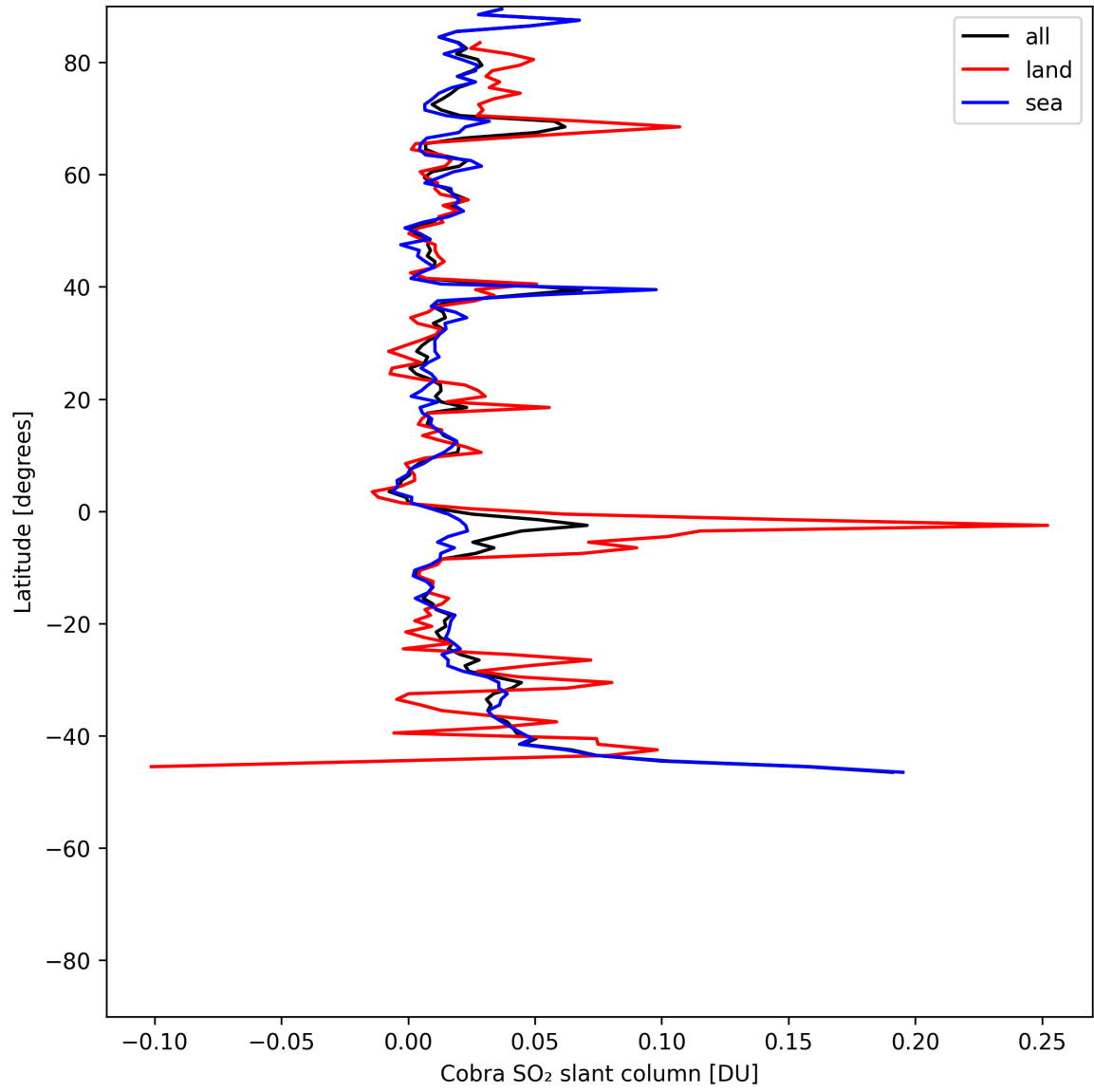
Figure 34: Zonal average of “Cobra SO 2 slant column” for 2025-06-03 to 2025-06-04.
