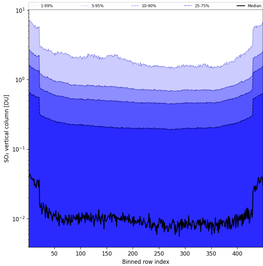
Figure 85: Along track statistics of “SO 2 vertical column” for 2025-06-03 to 2025-06-04
