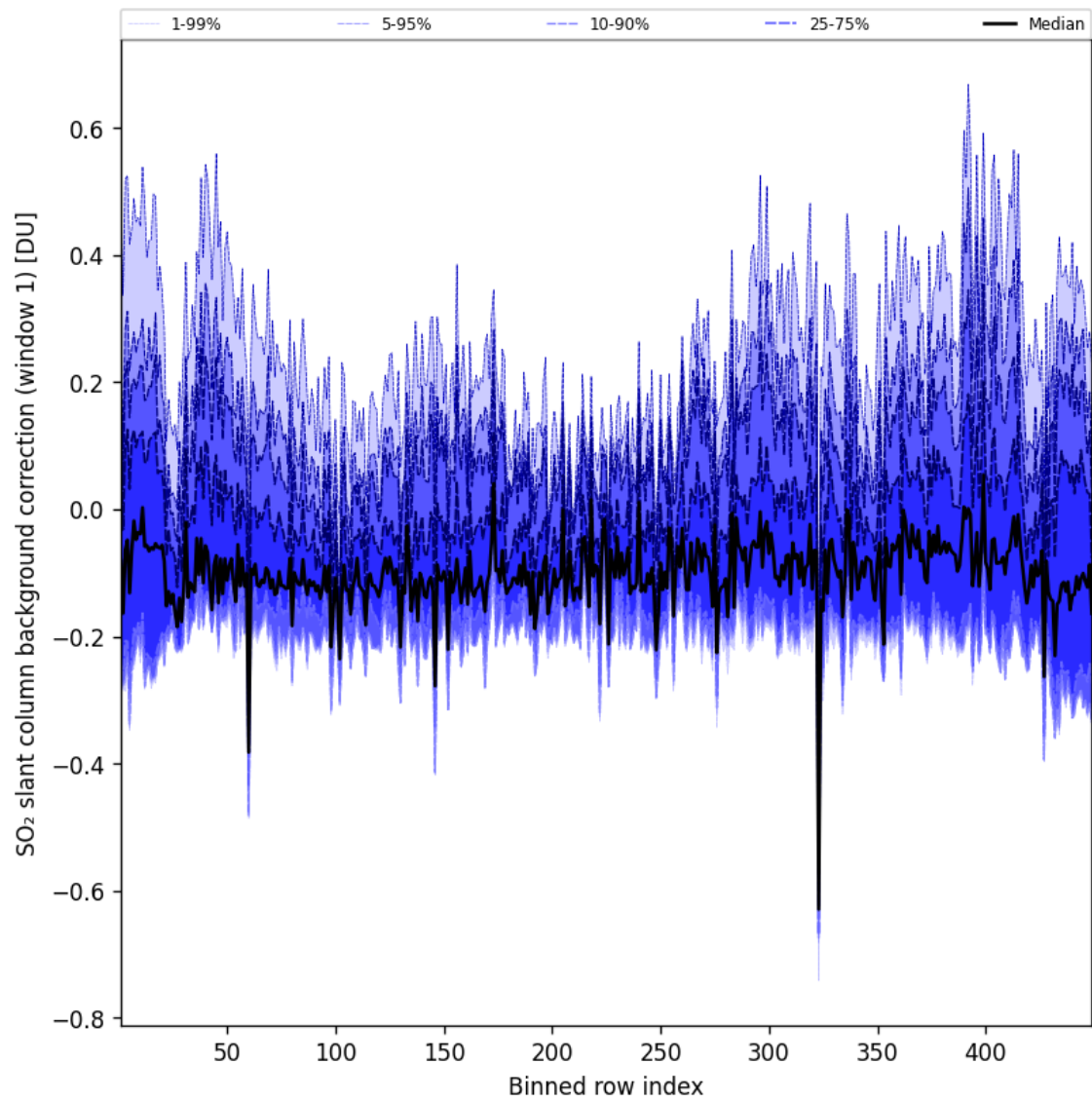
Figure 93: Along track statistics of “SO 2 slant column background correction (window 1)” for 2025-06-03 to 2025-06-04
