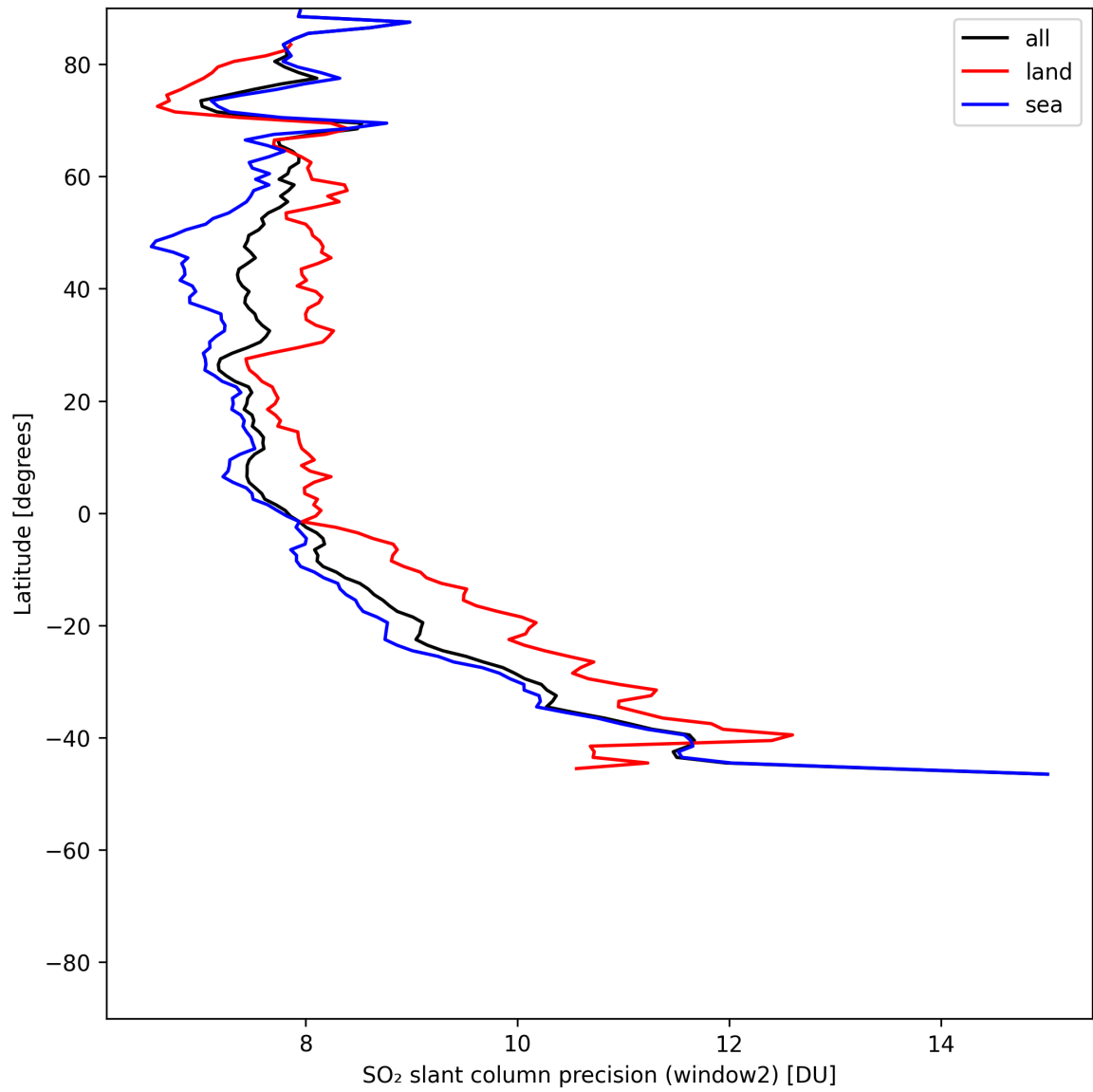
Figure 41: Zonal average of “SO 2 slant column precision (window2)” for 2025-06-03 to 2025-06-04.
