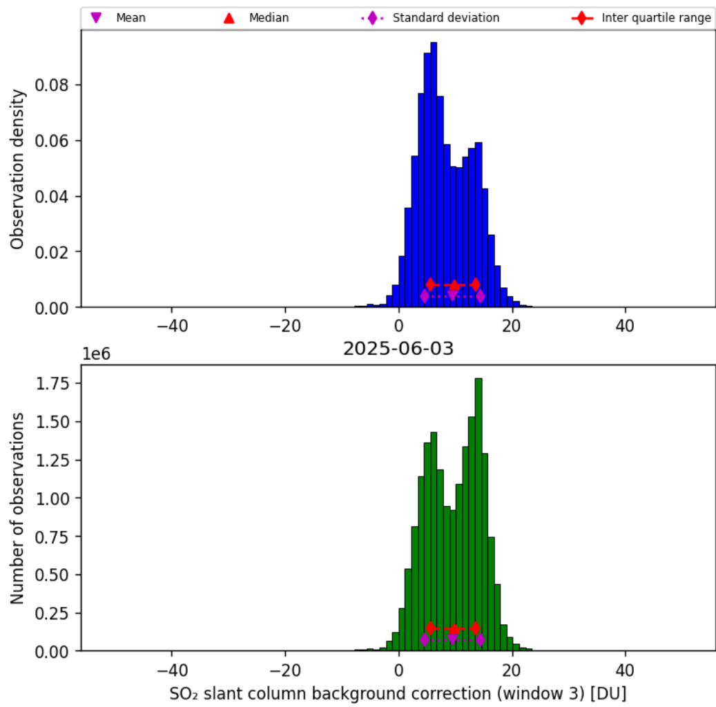
Figure 74: Histogram of “SO 2 slant column background correction (window 3)” for 2025-06-03 to 2025-06-04
