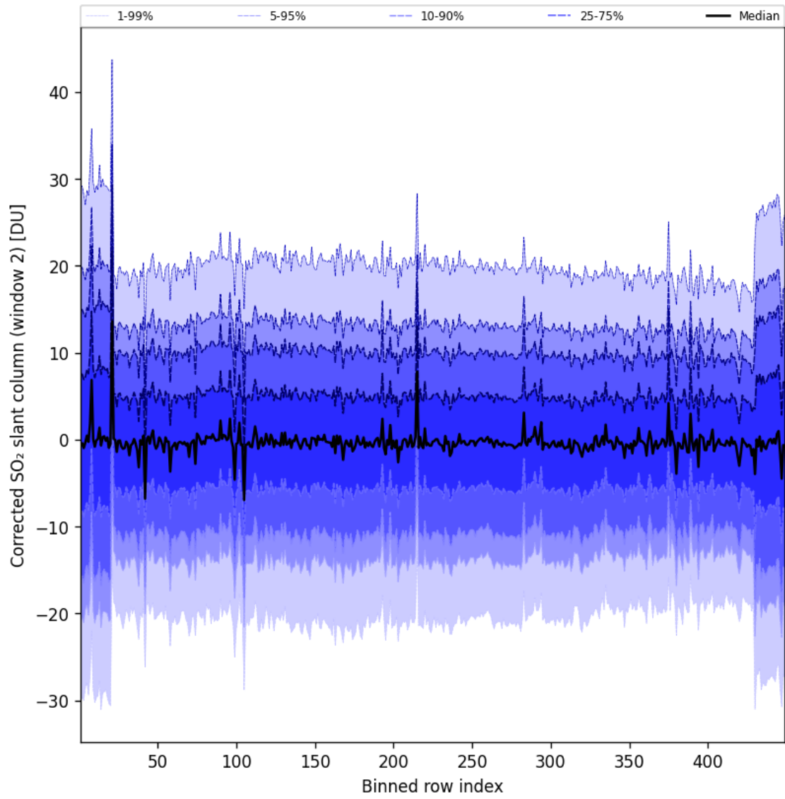
Figure 96: Along track statistics of “Corrected SO 2 slant column (window 2)” for 2025-06-03 to 2025-06-04
