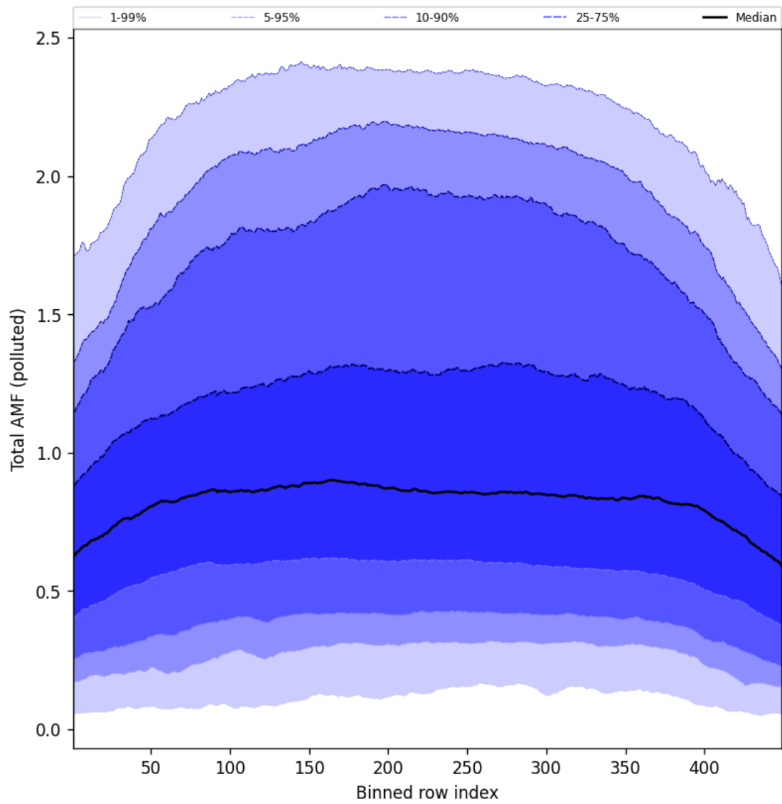
Figure 107: Along track statistics of “Total AMF (polluted)” for 2025-06-03 to 2025-06-04
