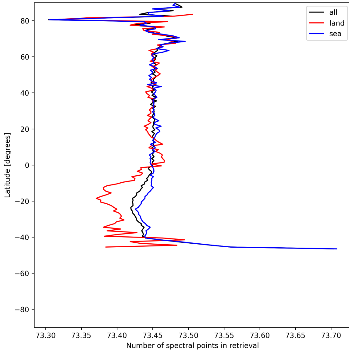
Figure 56: Zonal average of “Number of spectral points in retrieval” for 2025-06-03 to 2025-06-04.
