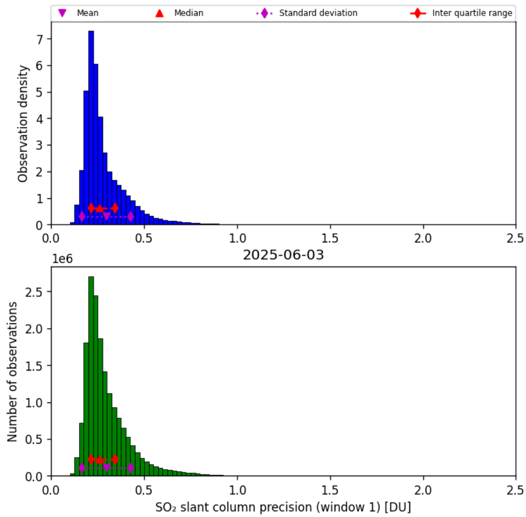
Figure 64: Histogram of “SO 2 slant column precision (window 1)” for 2025-06-03 to 2025-06-04
