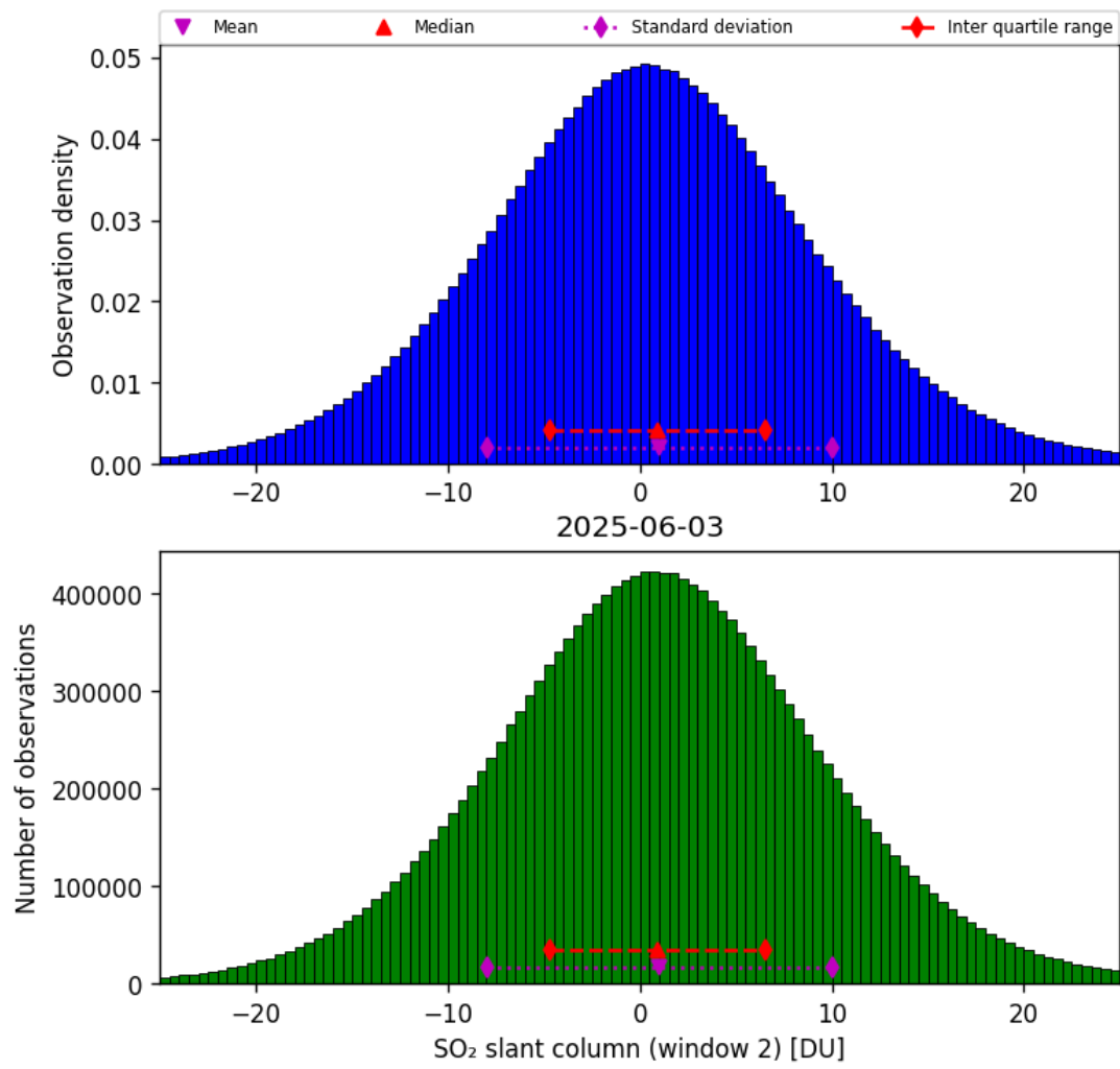
Figure 67: Histogram of “SO 2 slant column (window 2)” for 2025-06-03 to 2025-06-04
