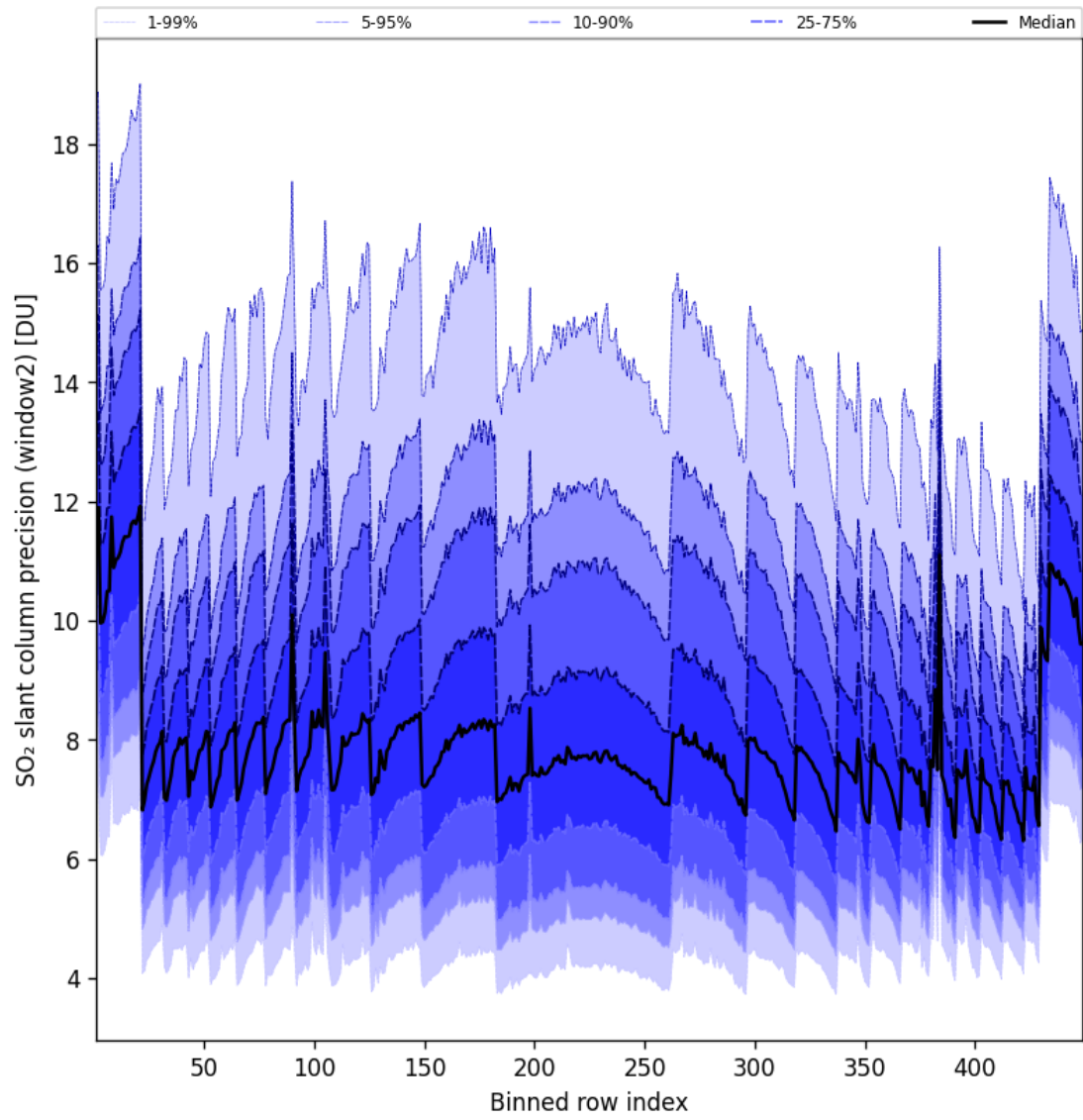
Figure 95: Along track statistics of “SO 2 slant column precision (window2)” for 2025-06-03 to 2025-06-04
