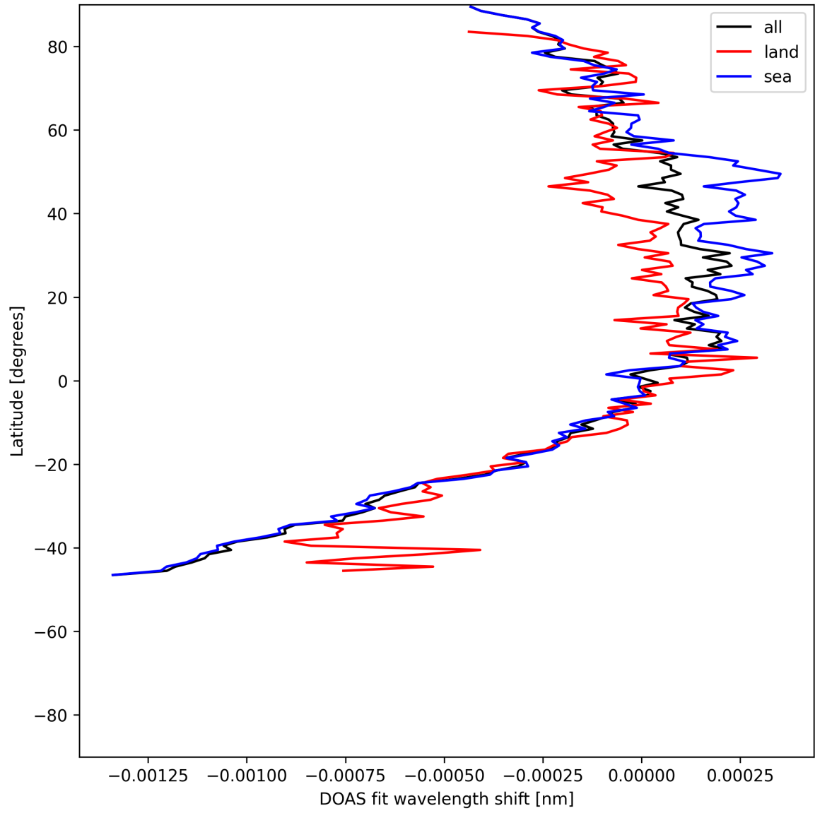
Figure 50: Zonal average of “DOAS fit wavelength shift” for 2025-06-03 to 2025-06-04.
