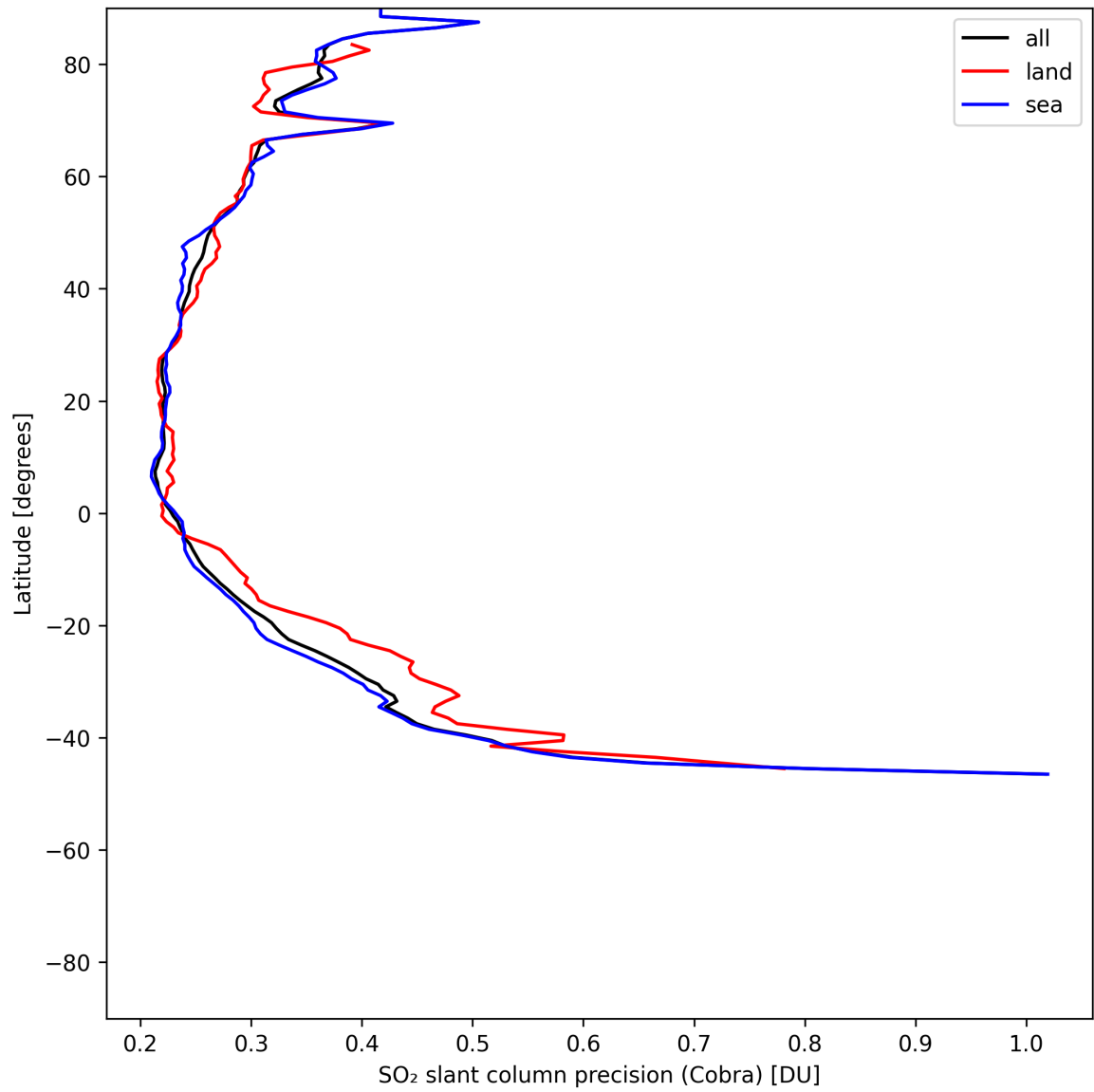
Figure 35: Zonal average of "SO 2 slant column precision (Cobra)" for 2025-06-03 to 2025-06-04.
