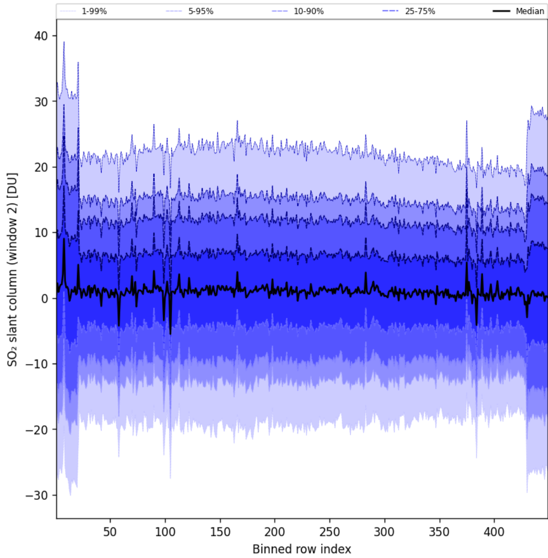
Figure 94: Along track statistics of “SO 2 slant column (window 2)” for 2025-06-03 to 2025-06-04
