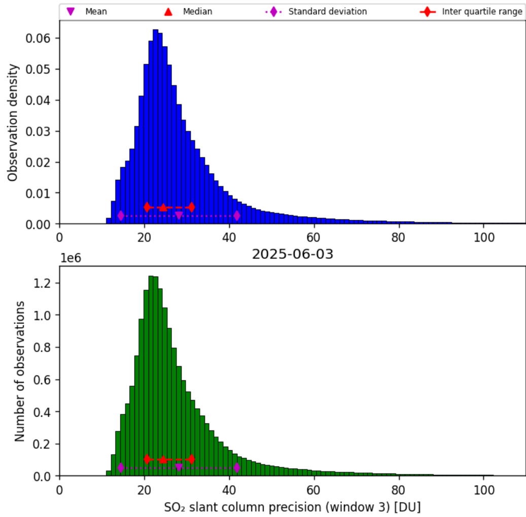
Figure 72: Histogram of “SO 2 slant column precision (window 3)” for 2025-06-03 to 2025-06-04
