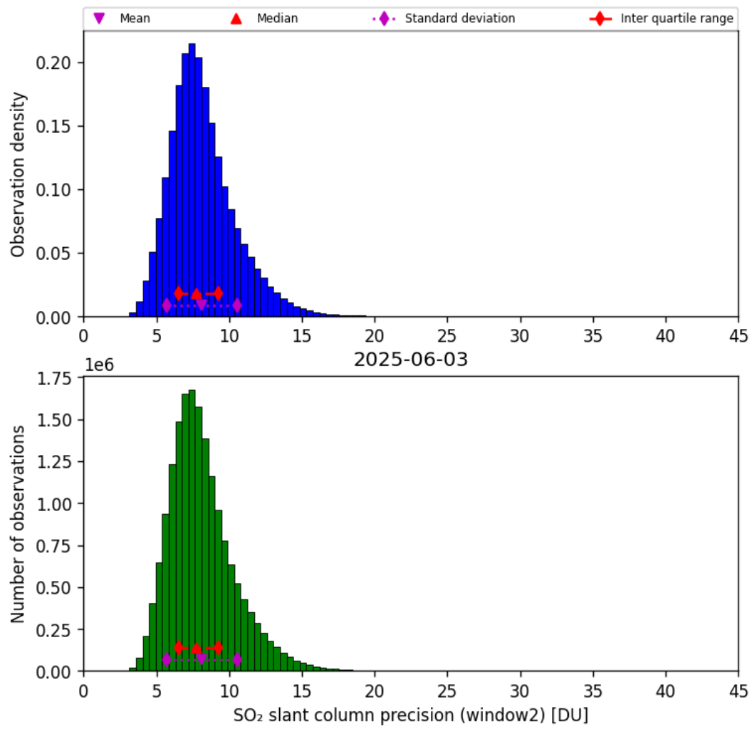
Figure 68: Histogram of “SO 2 slant column precision (window2)” for 2025-06-03 to 2025-06-04
