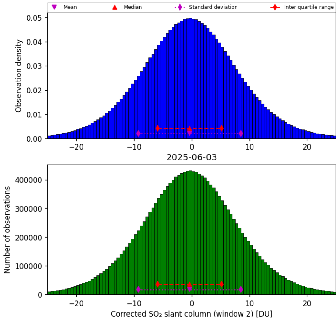
Figure 69: Histogram of “Corrected SO 2 slant column (window 2)” for 2025-06-03 to 2025-06-04
