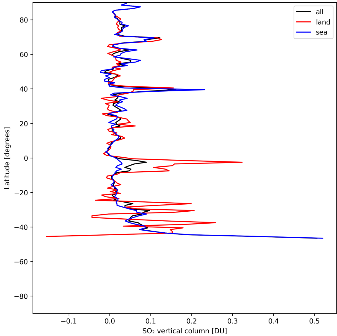
Figure 31: Zonal average of “SO 2 vertical column” for 2025-06-03 to 2025-06-04.
