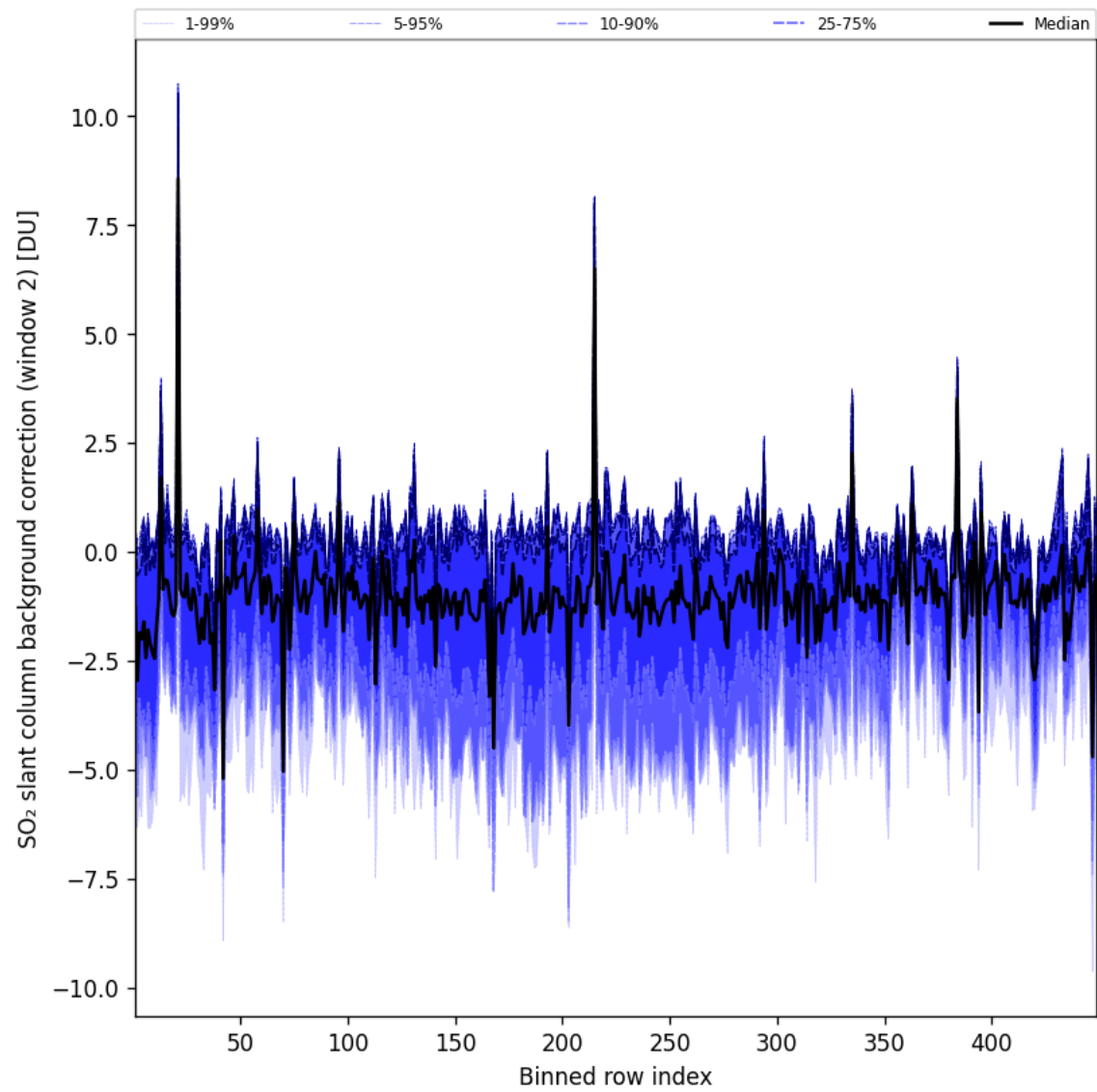
Figure 97: Along track statistics of “SO 2 slant column background correction (window 2)” for 2025-06-03 to 2025-06-04
