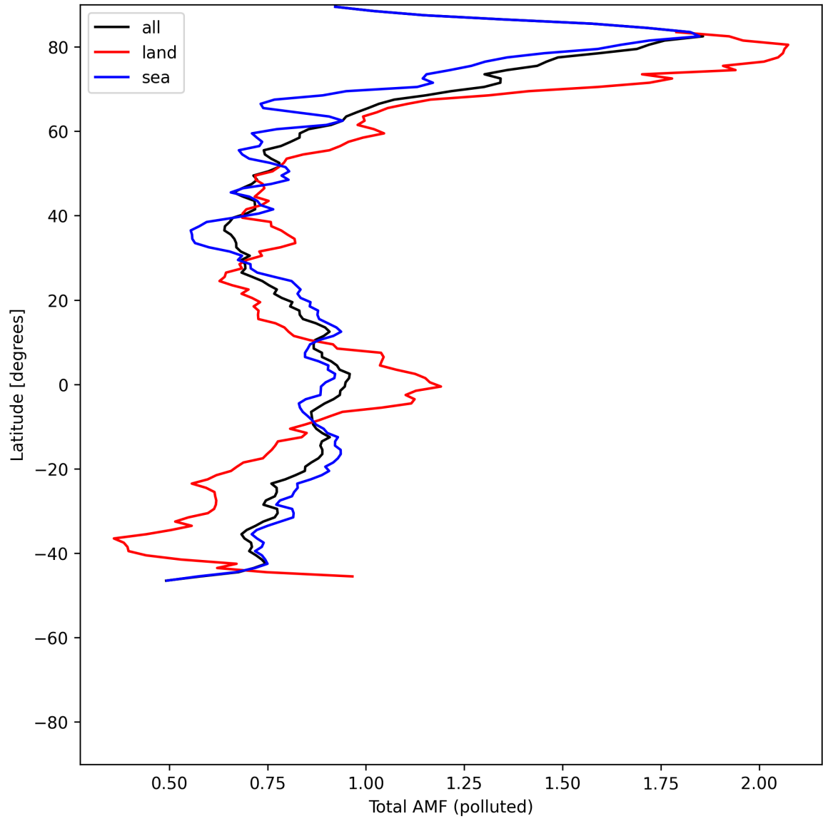
Figure 53: Zonal average of “Total AMF (polluted)” for 2025-06-03 to 2025-06-04.
