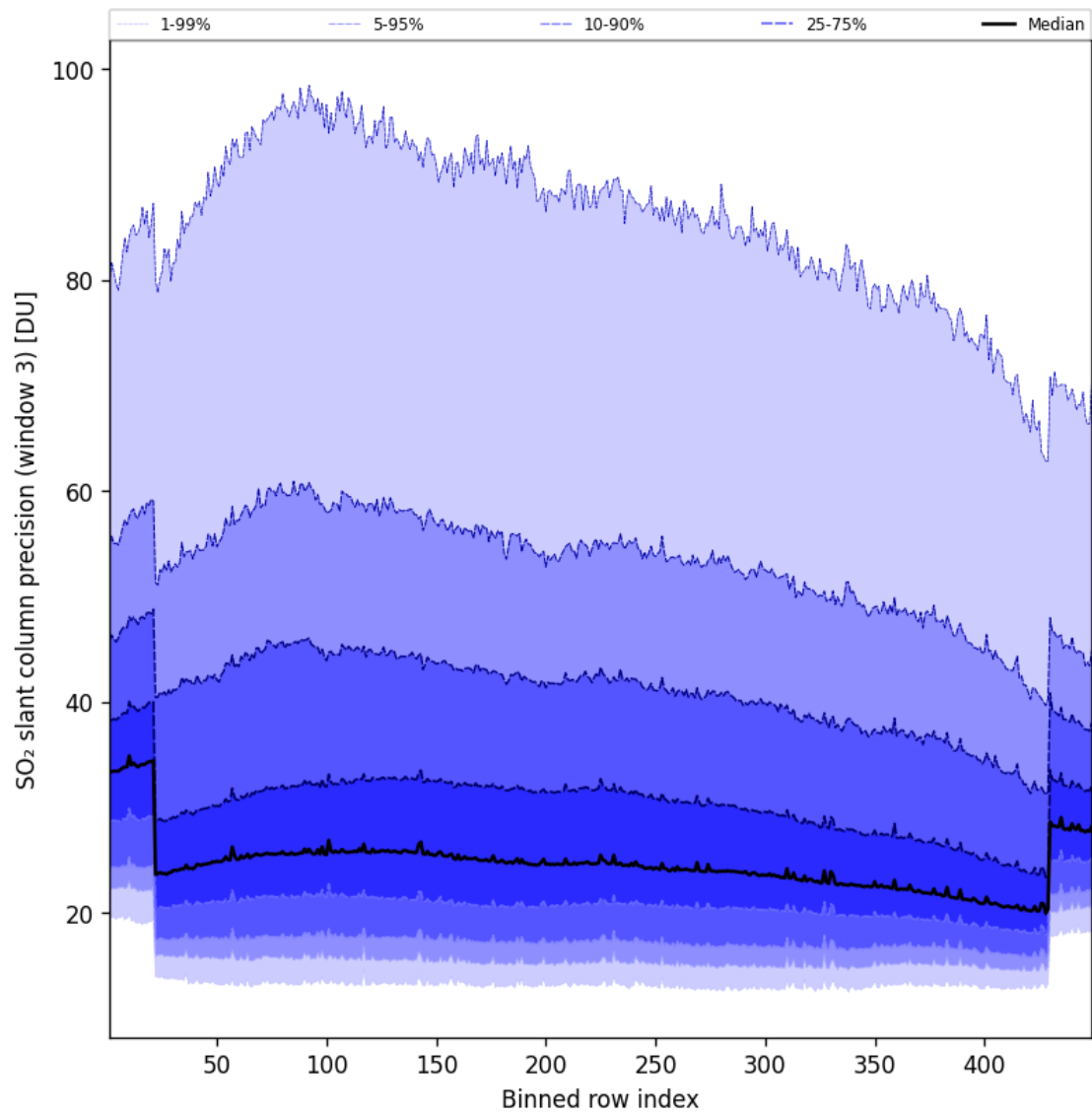
Figure 99: Along track statistics of “SO 2 slant column precision (window 3)” for 2025-06-03 to 2025-06-04
