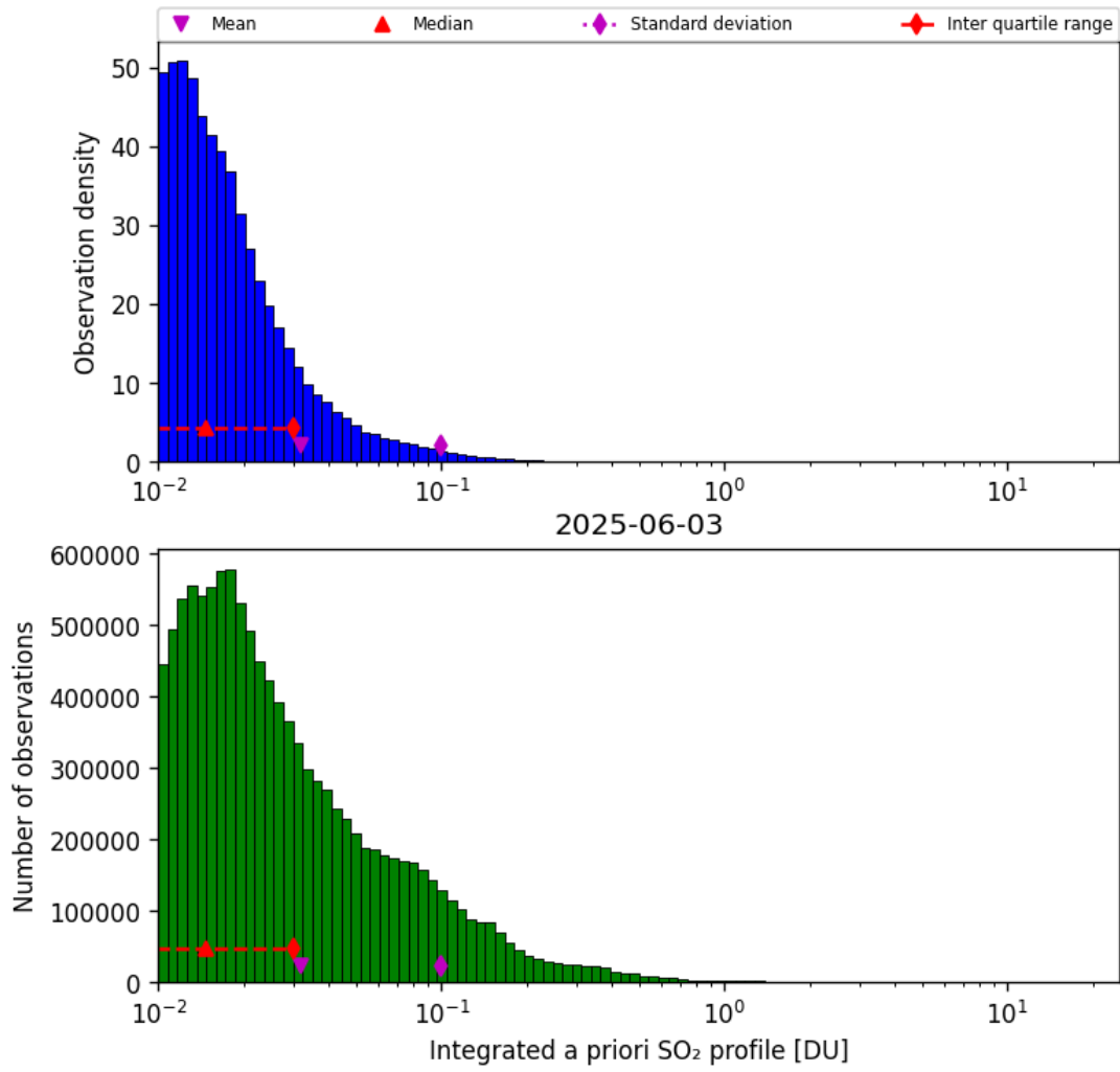
Figure 76: Histogram of “Integrated a priori SO 2 profile” for 2025-06-03 to 2025-06-04
