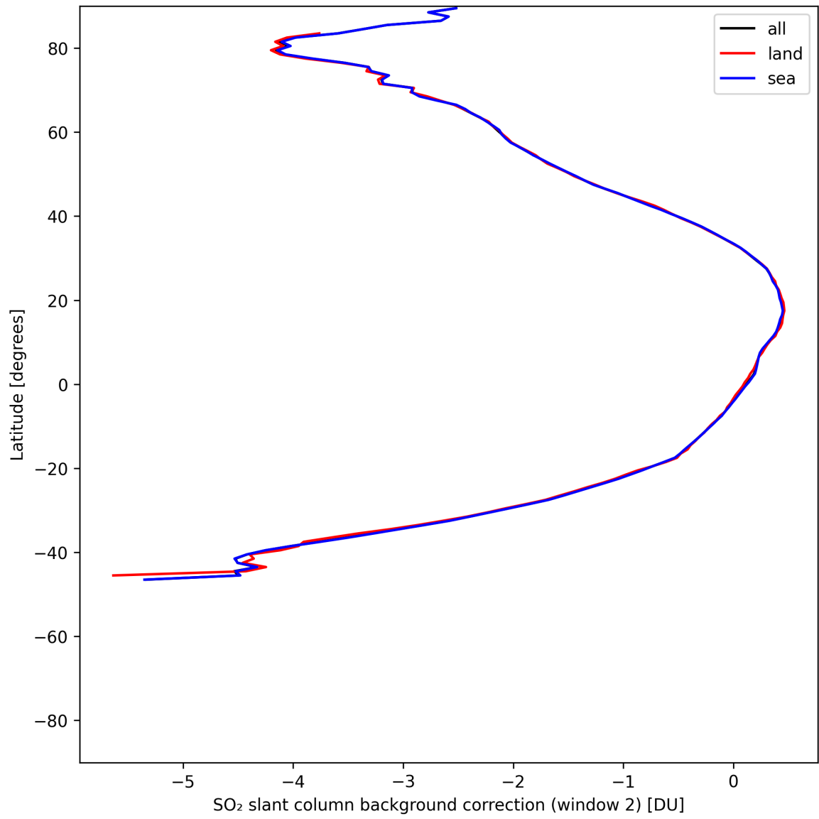
Figure 43: Zonal average of “SO 2 slant column background correction (window 2)” for 2025-06-03 to 2025-06-04.
