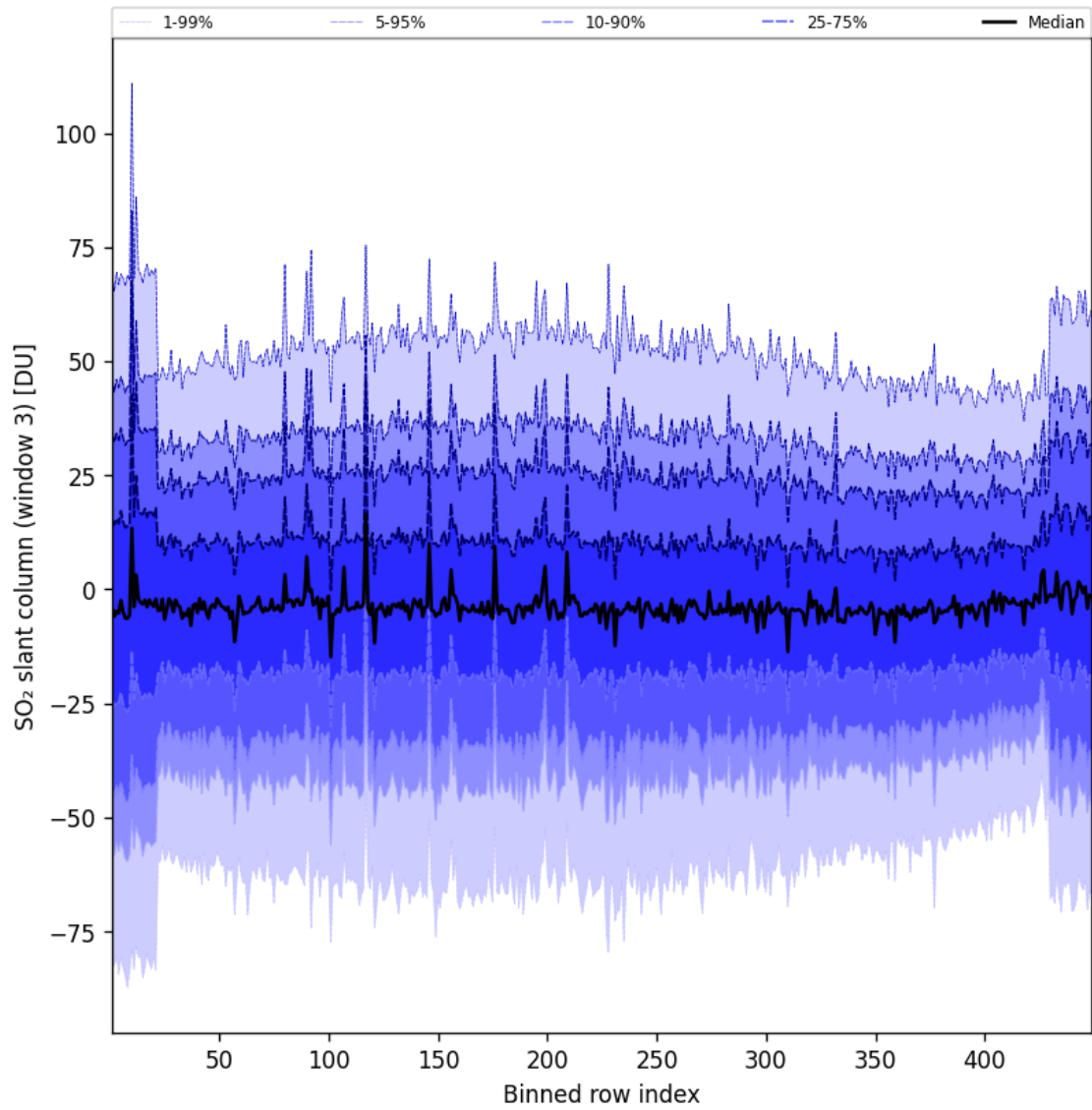
Figure 98: Along track statistics of “SO 2 slant column (window 3)” for 2025-06-03 to 2025-06-04
