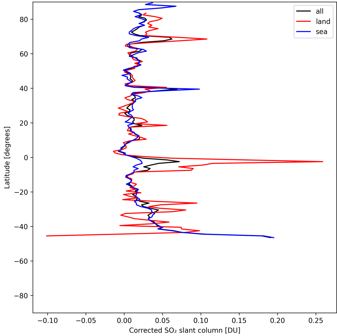
Figure 33: Zonal average of “Corrected SO 2 slant column” for 2025-06-03 to 2025-06-04.
