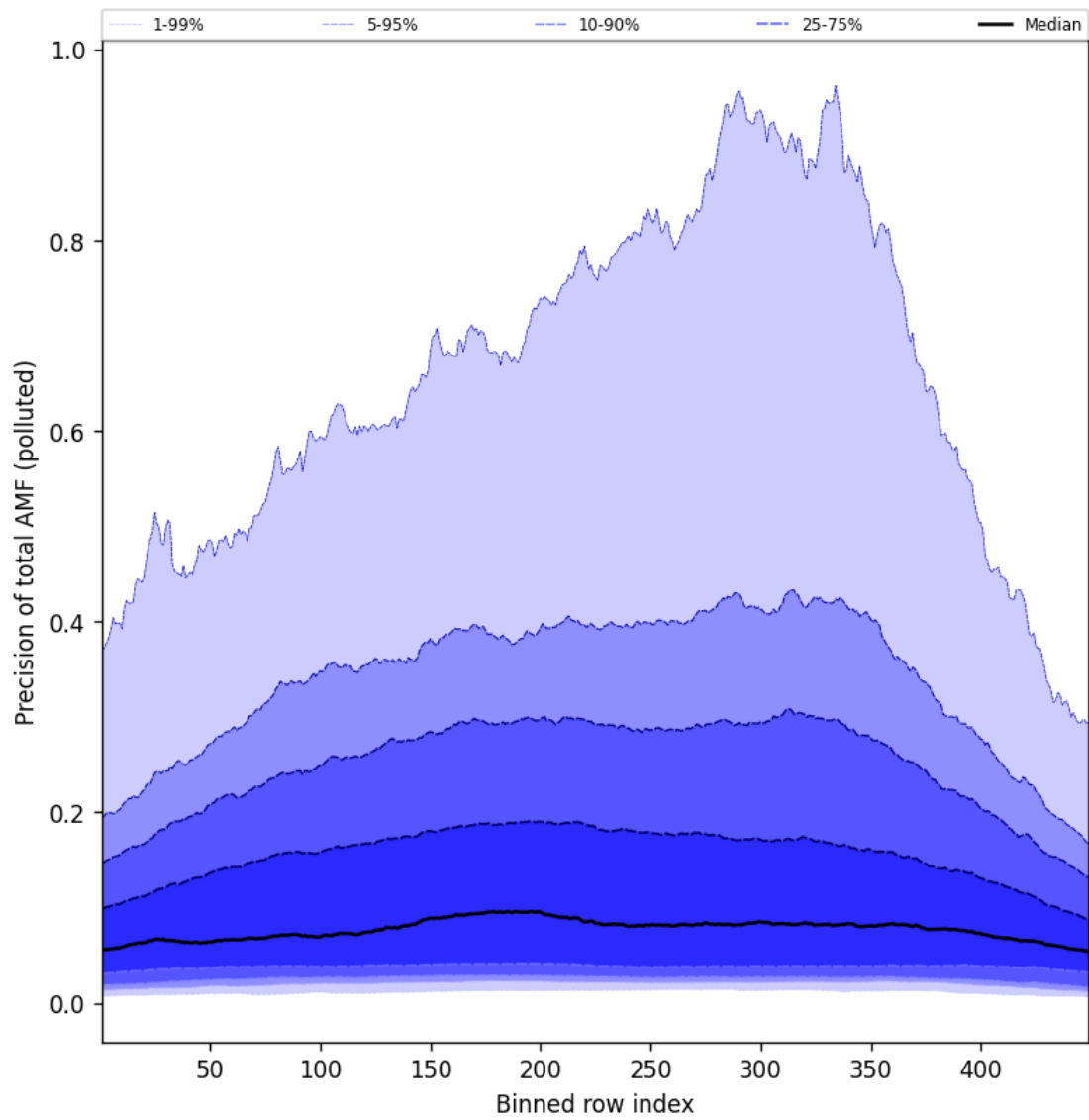
Figure 108: Along track statistics of “Precision of total AMF (polluted)” for 2025-06-03 to 2025-06-04
