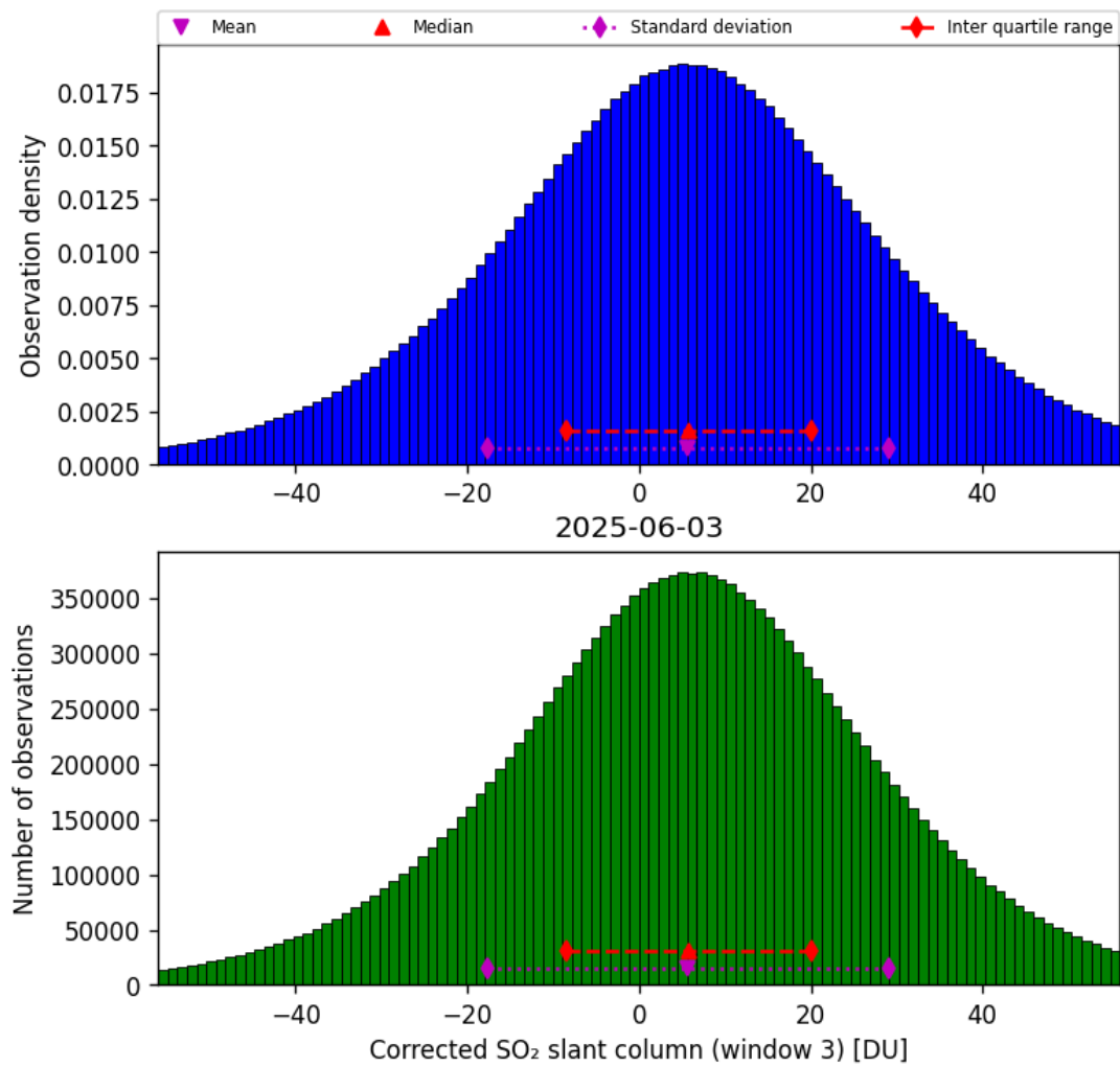
Figure 73: Histogram of “Corrected SO 2 slant column (window 3)” for 2025-06-03 to 2025-06-04
