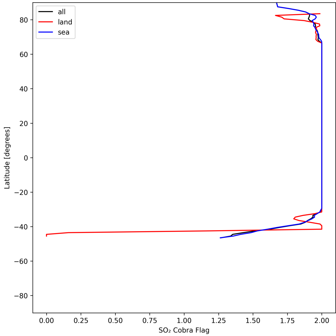
Figure 48: Zonal average of "SO 2 Cobra Flag" for 2025-06-03 to 2025-06-04.
