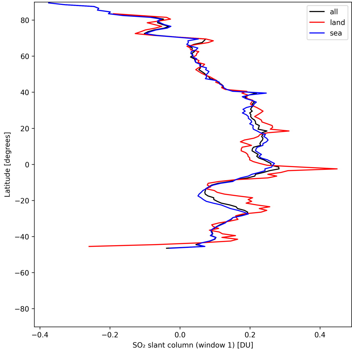
Figure 36: Zonal average of “SO 2 slant column (window 1)” for 2025-06-03 to 2025-06-04.
