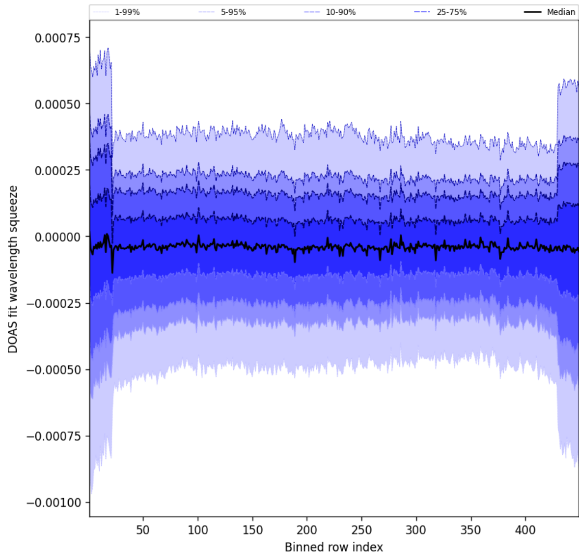
Figure 105: Along track statistics of “DOAS fit wavelength squeeze” for 2025-06-03 to 2025-06-04
