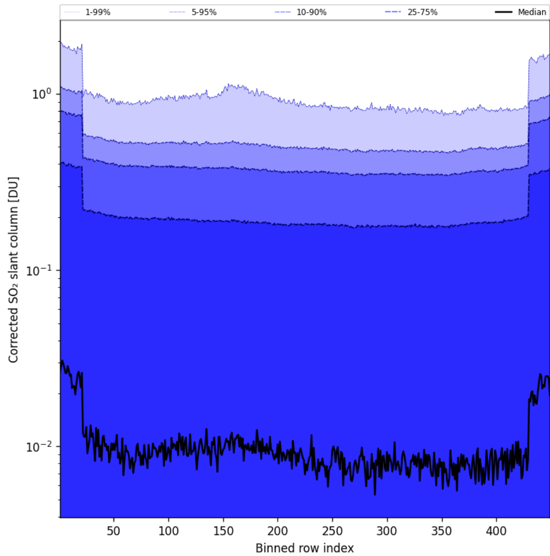
Figure 87: Along track statistics of “Corrected SO 2 slant column” for 2025-06-03 to 2025-06-04
