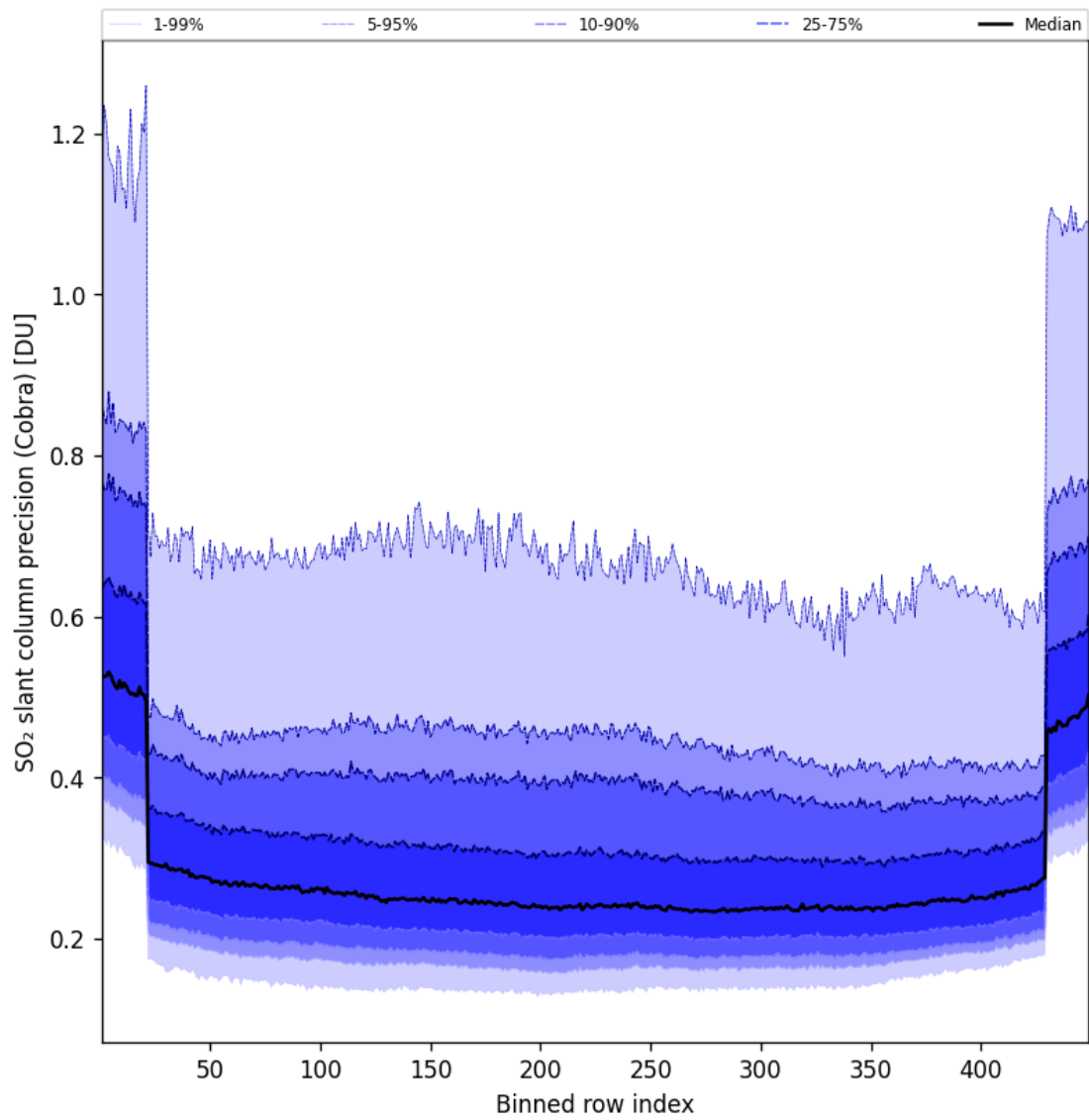
Figure 89: Along track statistics of “SO 2 slant column precision (Cobra)” for 2025-06-03 to 2025-06-04
