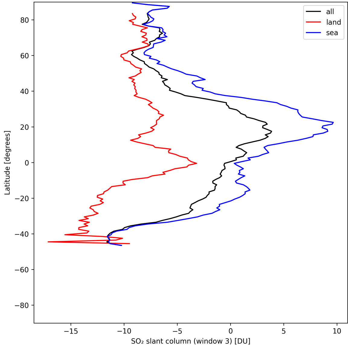
Figure 44: Zonal average of “SO 2 slant column (window 3)” for 2025-06-03 to 2025-06-04.
