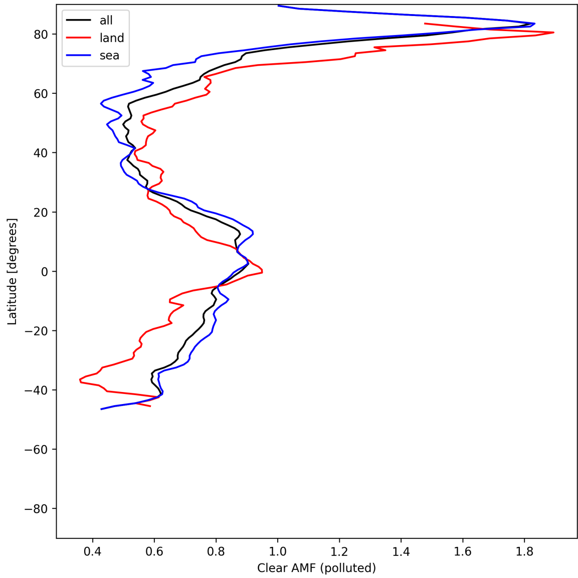
Figure 55: Zonal average of “Clear AMF (polluted)” for 2025-06-03 to 2025-06-04.
