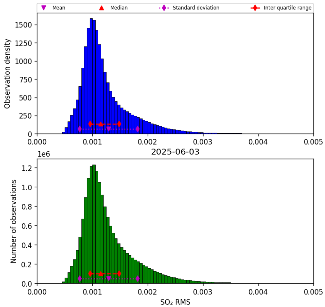
Figure 79: Histogram of “SO 2 RMS” for 2025-06-03 to 2025-06-04
