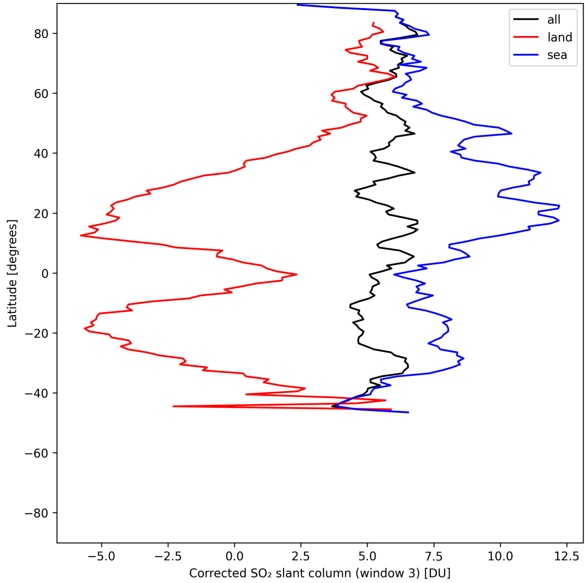
Figure 46: Zonal average of “Corrected SO 2 slant column (window 3)” for 2025-06-03 to 2025-06-04.
