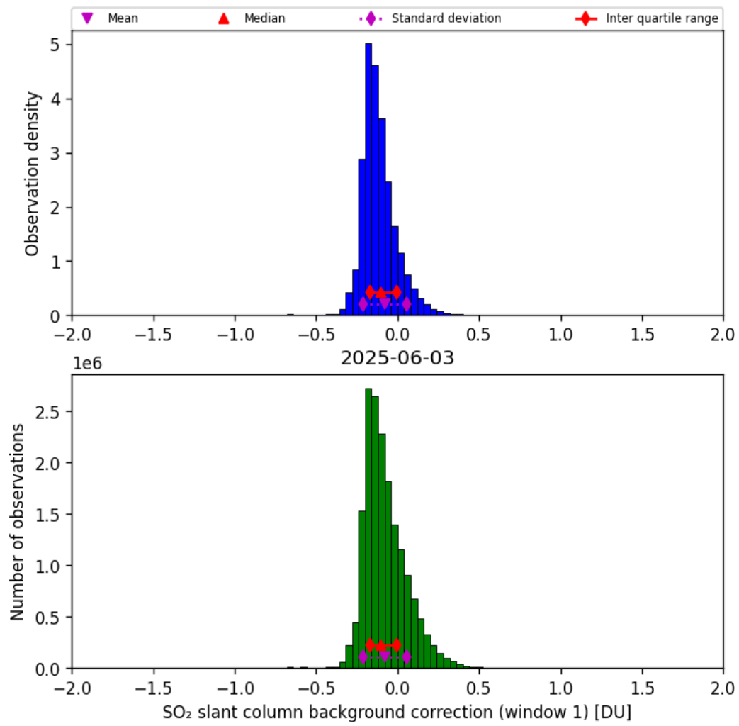
Figure 66: Histogram of “SO 2 slant column background correction (window 1)” for 2025-06-03 to 2025-06-04
