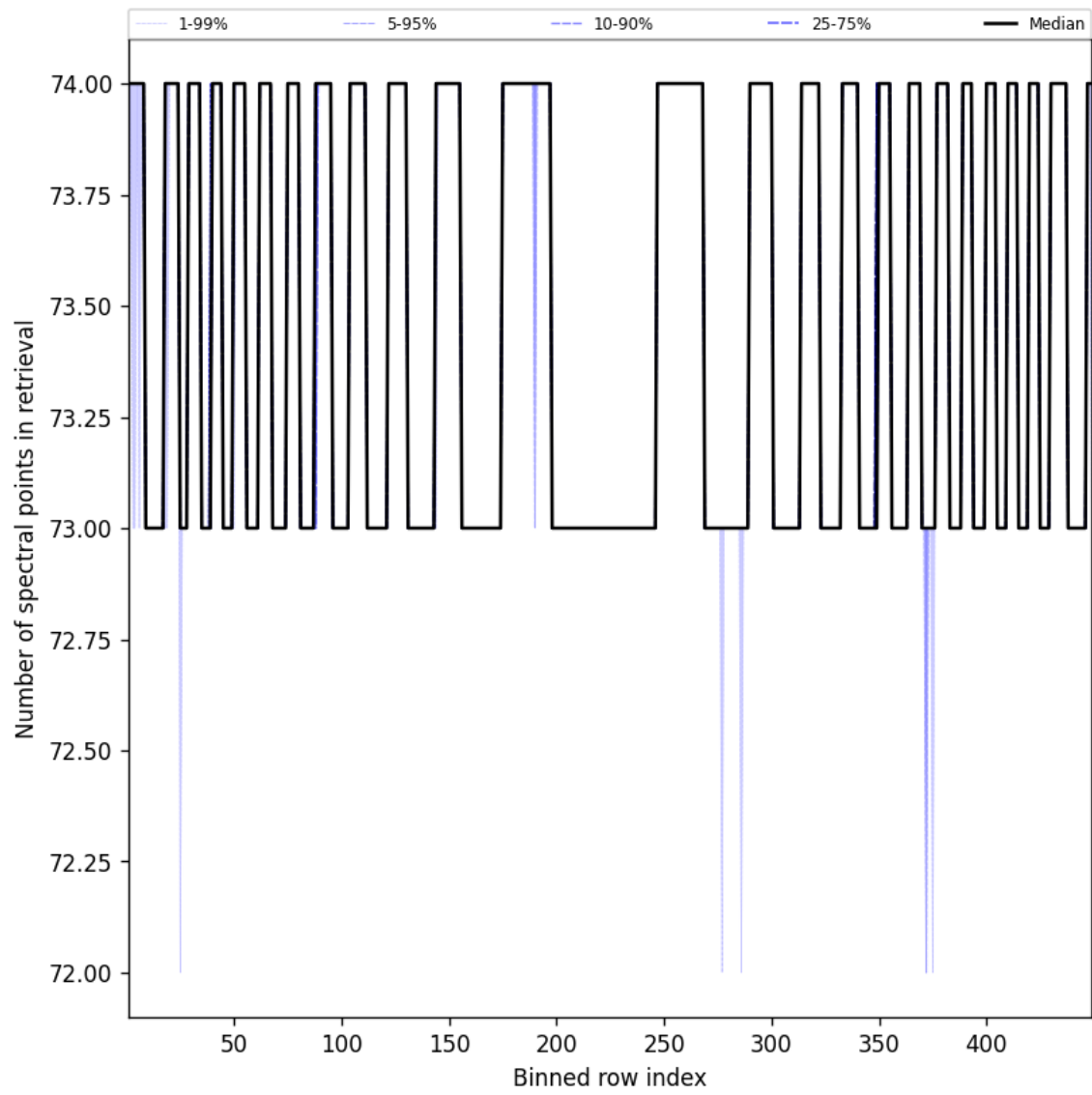
Figure 110: Along track statistics of “Number of spectral points in retrieval” for 2025-06-03 to 2025-06-04
