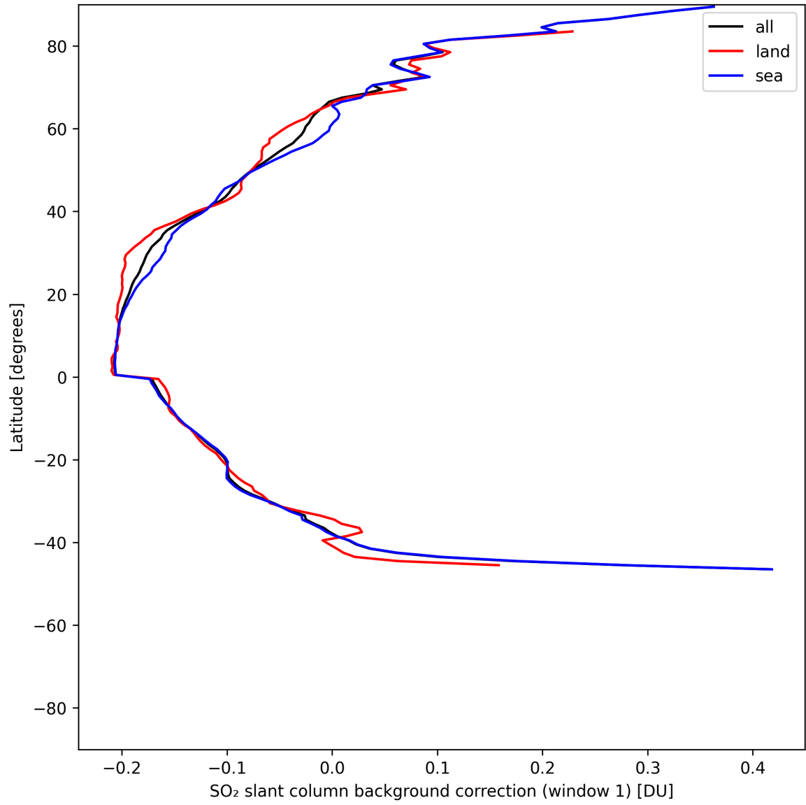
Figure 39: Zonal average of “SO 2 slant column background correction (window 1)” for 2025-06-03 to 2025-06-04.
