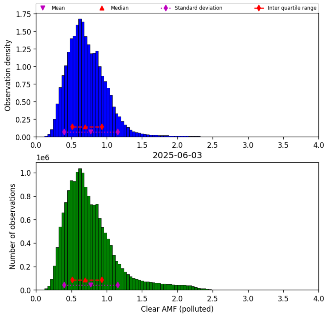
Figure 82: Histogram of “Clear AMF (polluted)” for 2025-06-03 to 2025-06-04
