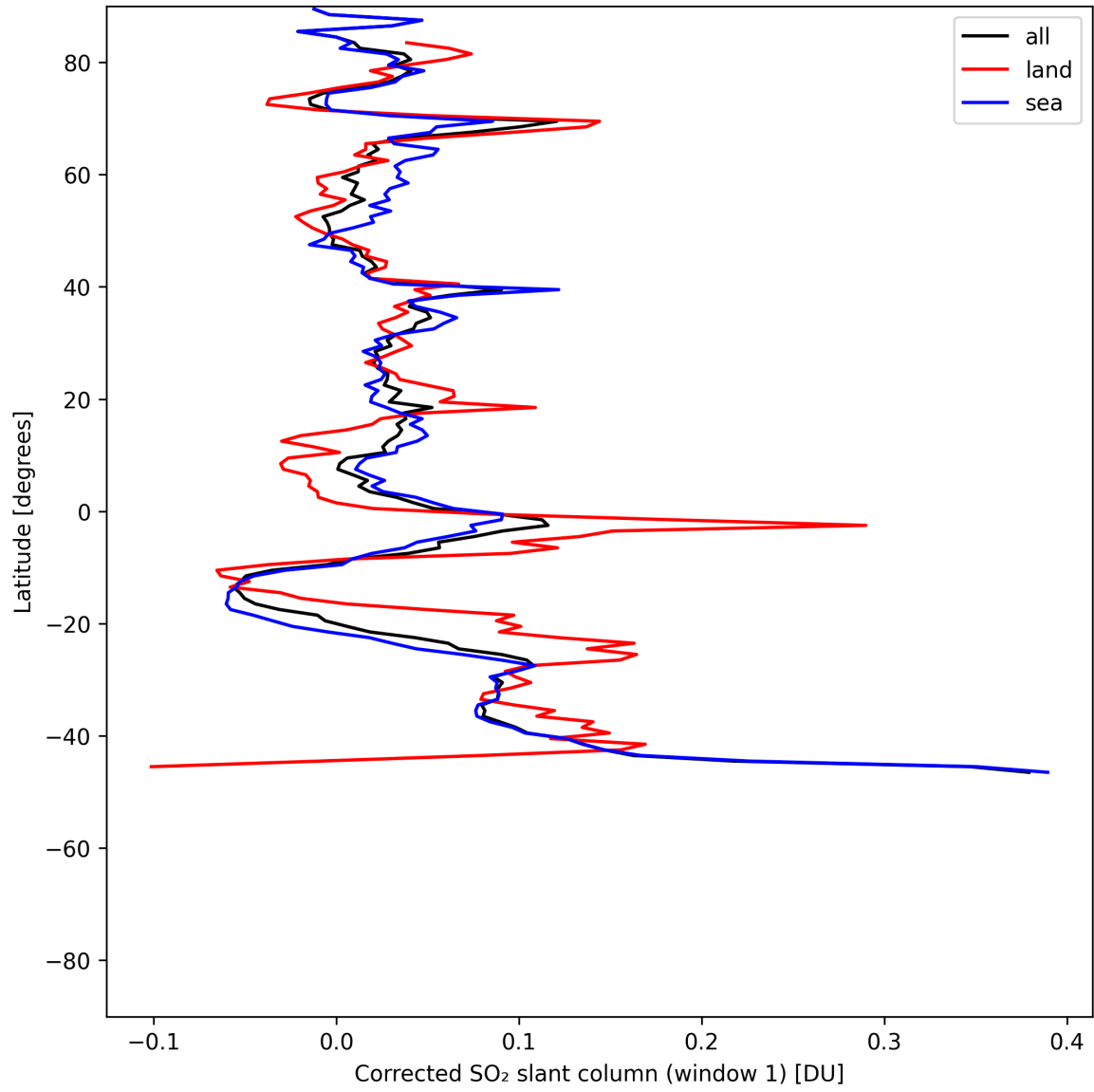
Figure 38: Zonal average of “Corrected SO 2 slant column (window 1)” for 2025-06-03 to 2025-06-04.
