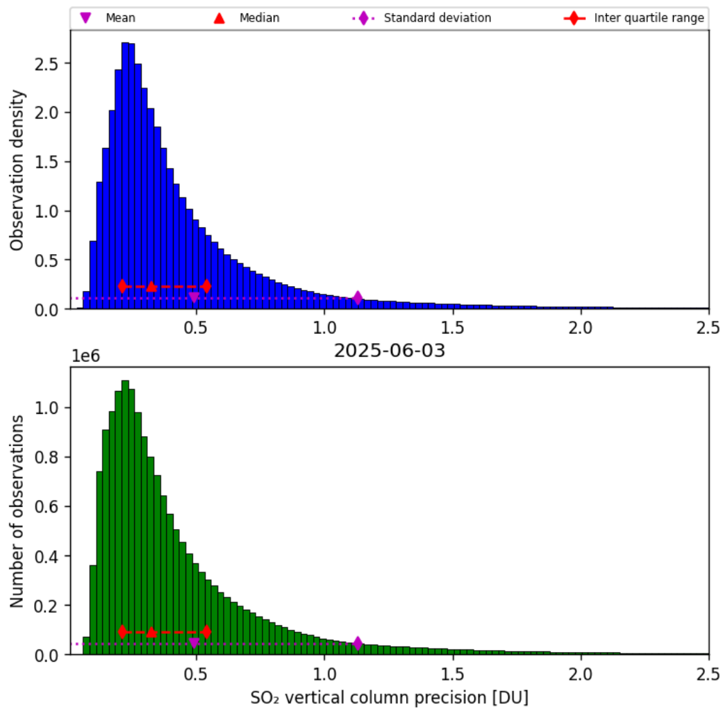
Figure 59: Histogram of “SO 2 vertical column precision” for 2025-06-03 to 2025-06-04
