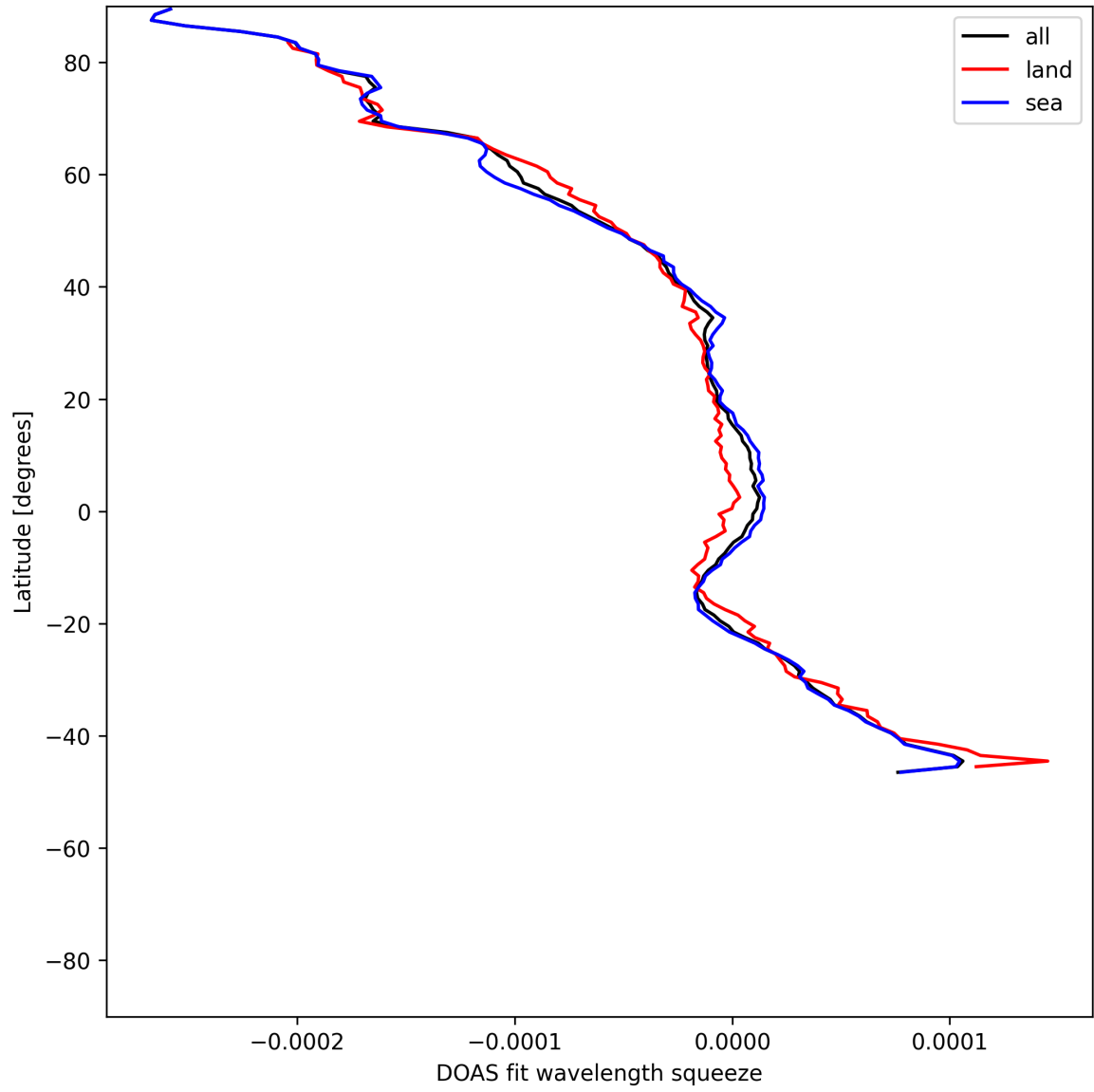
Figure 51: Zonal average of “DOAS fit wavelength squeeze” for 2025-06-03 to 2025-06-04.
