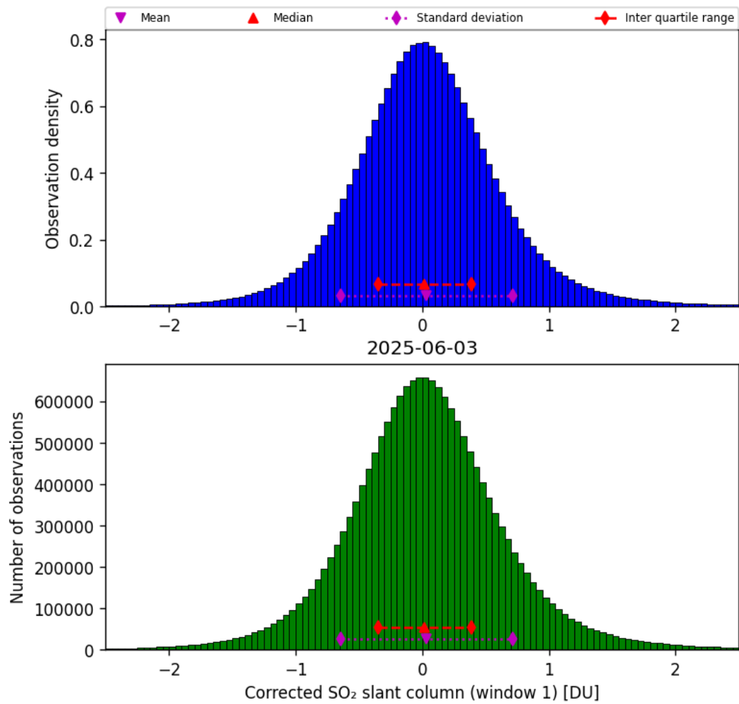
Figure 65: Histogram of “Corrected SO 2 slant column (window 1)” for 2025-06-03 to 2025-06-04
