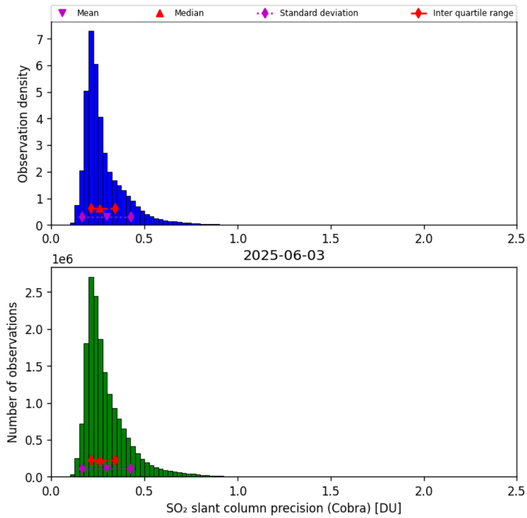
Figure 62: Histogram of “SO 2 slant column precision (Cobra)” for 2025-06-03 to 2025-06-04
