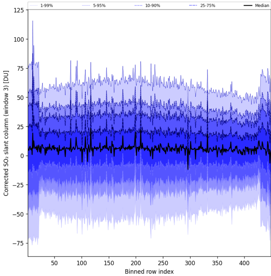
Figure 100: Along track statistics of “Corrected SO 2 slant column (window 3)” for 2025-06-03 to 2025-06-04
