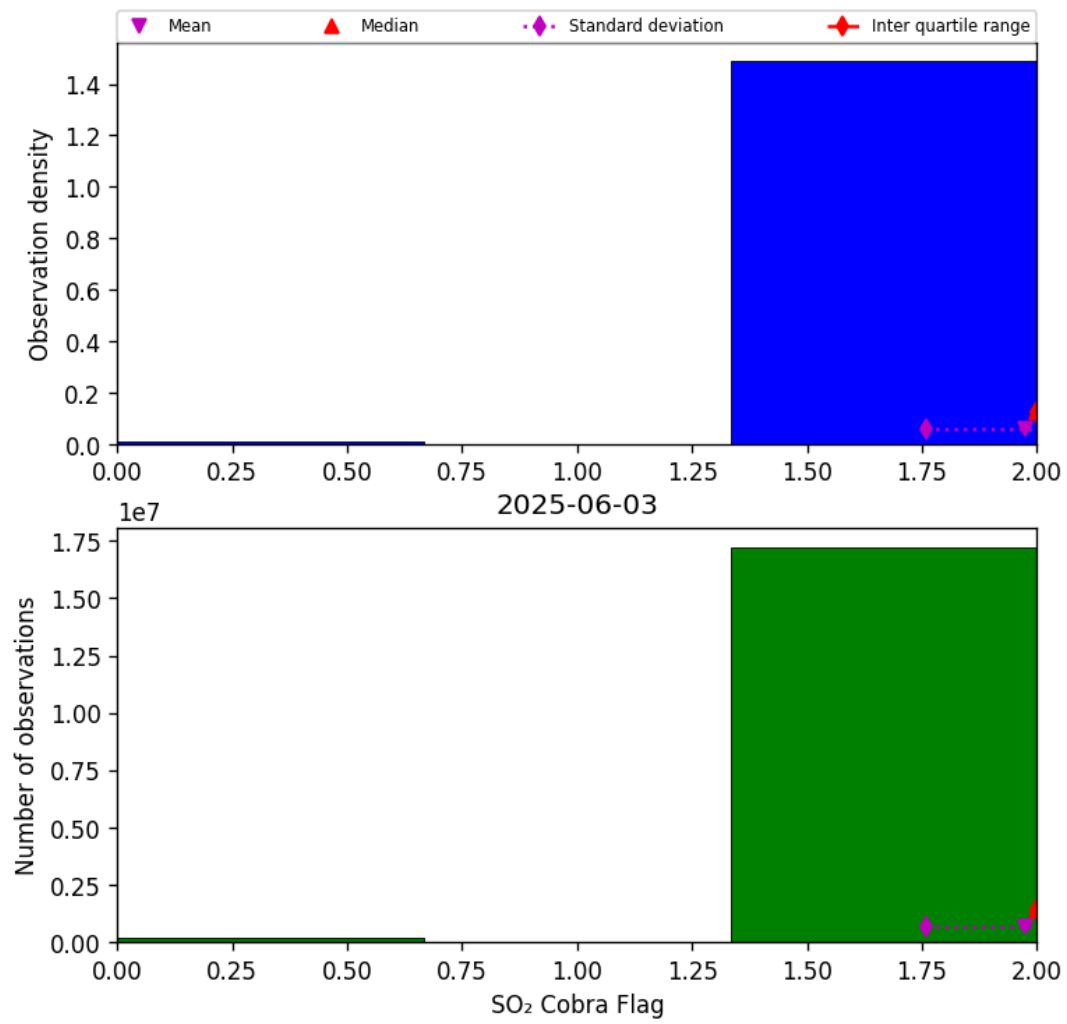
Figure 75: Histogram of “SO 2 Cobra Flag” for 2025-06-03 to 2025-06-04
