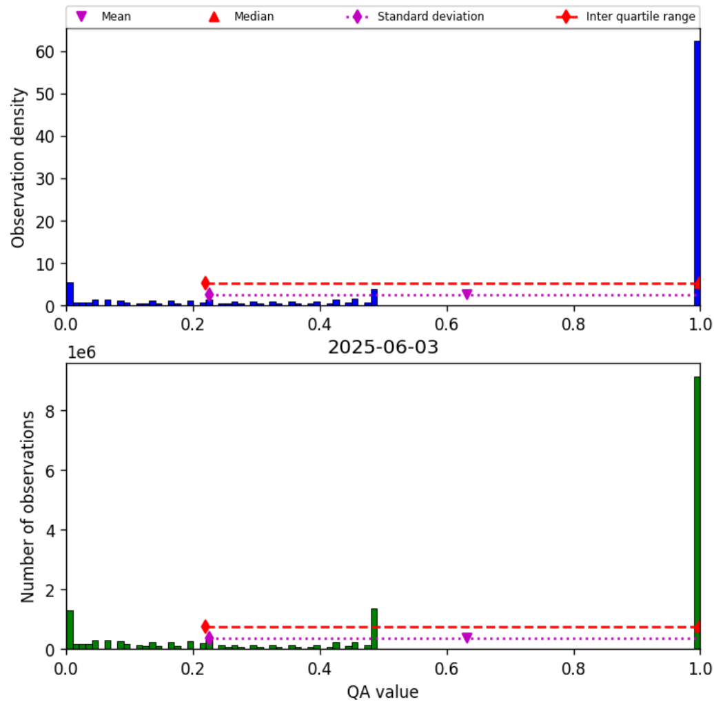
Figure 57: Histogram of “QA value” for 2025-06-03 to 2025-06-04
