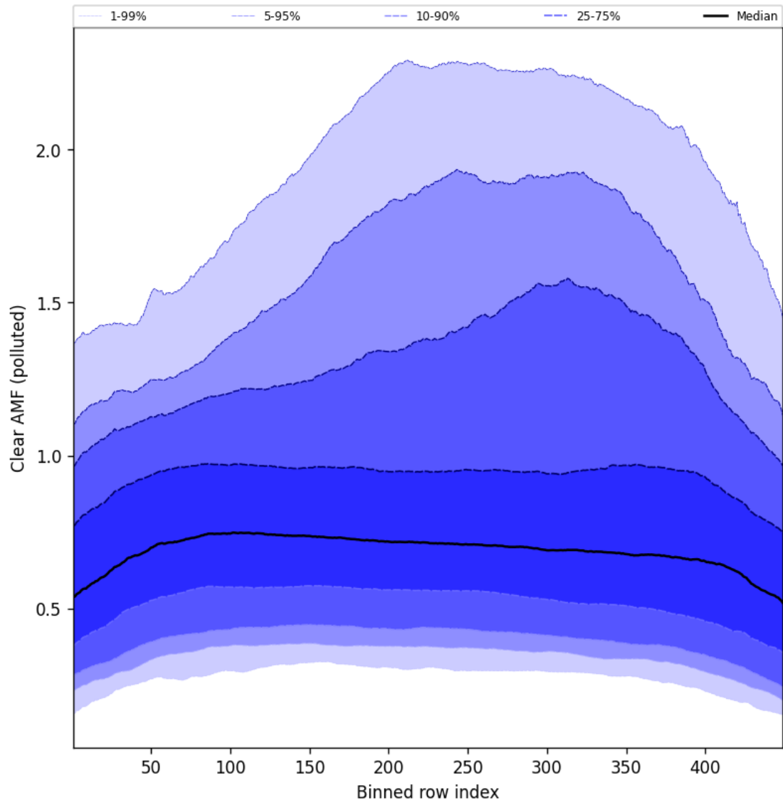
Figure 109: Along track statistics of “Clear AMF (polluted)” for 2025-06-03 to 2025-06-04
