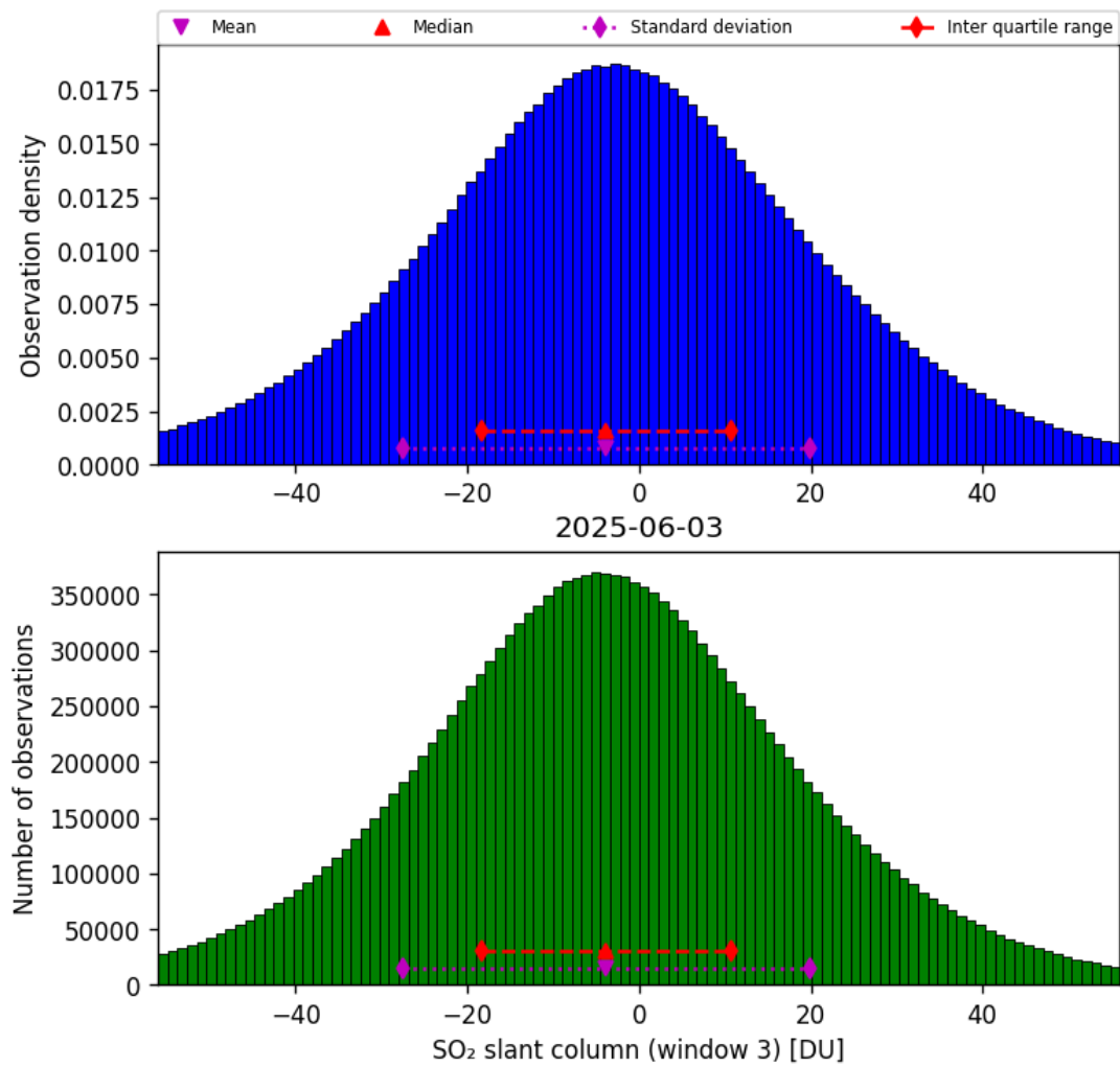
Figure 71: Histogram of “SO 2 slant column (window 3)” for 2025-06-03 to 2025-06-04
