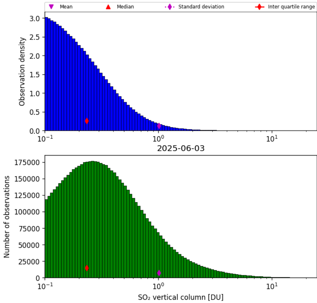
Figure 58: Histogram of “SO 2 vertical column” for 2025-06-03 to 2025-06-04
