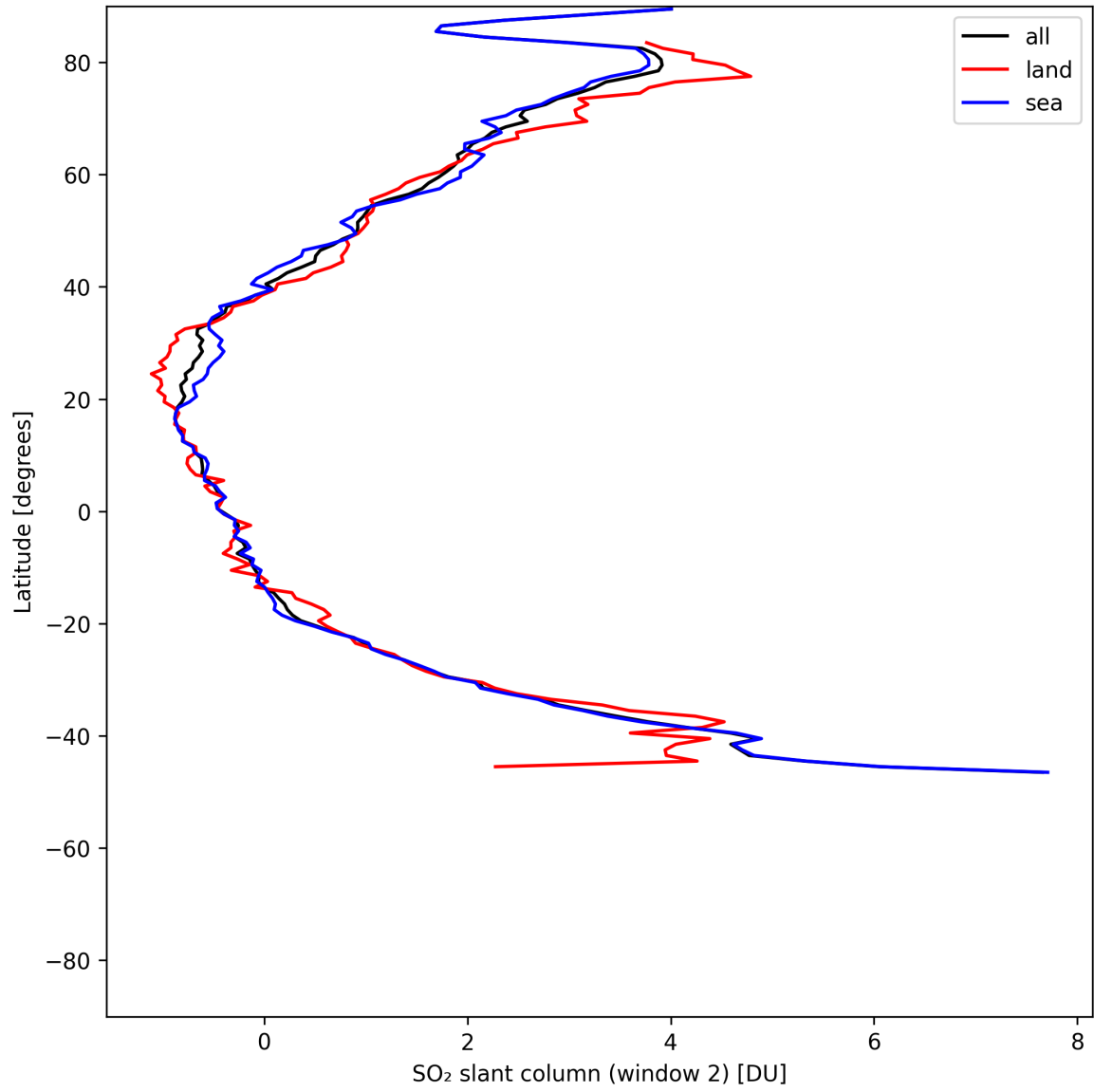
Figure 40: Zonal average of “SO 2 slant column (window 2)” for 2025-06-03 to 2025-06-04.
