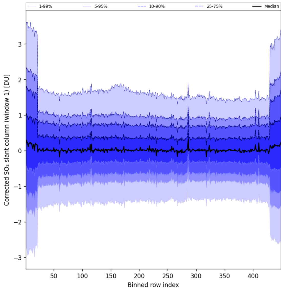
Figure 92: Along track statistics of “Corrected SO 2 slant column (window 1)” for 2025-06-03 to 2025-06-04
