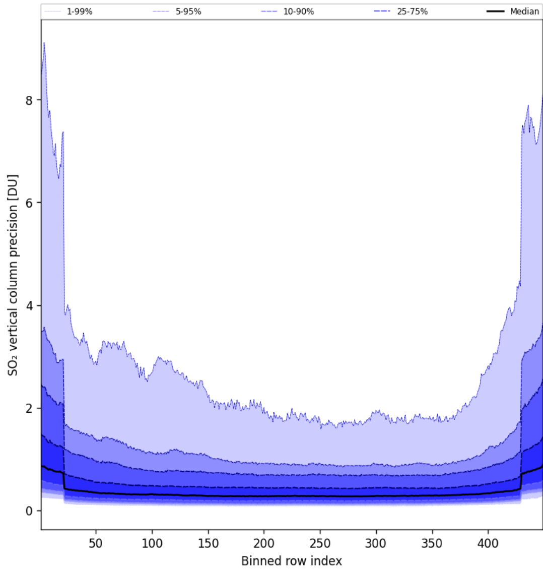
Figure 86: Along track statistics of “SO 2 vertical column precision” for 2025-06-03 to 2025-06-04
