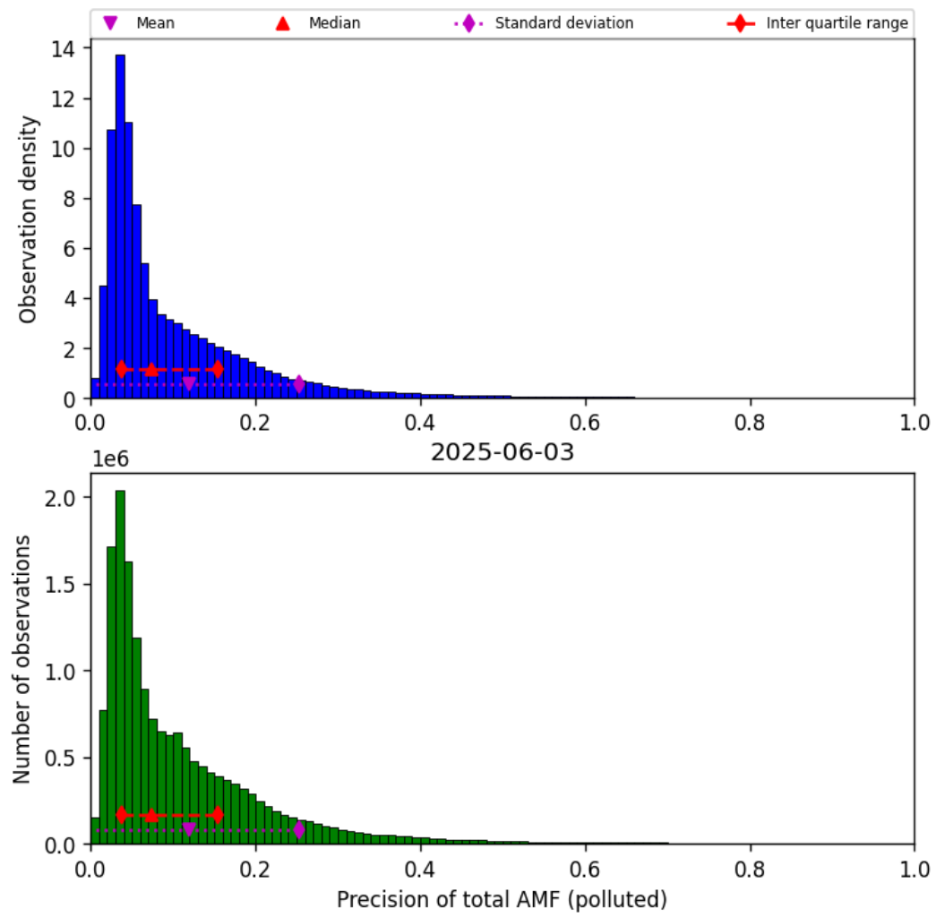
Figure 81: Histogram of “Precision of total AMF (polluted)” for 2025-06-03 to 2025-06-04
