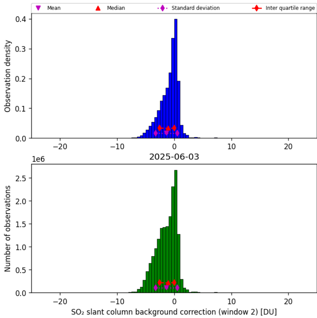
Figure 70: Histogram of “SO 2 slant column background correction (window 2)” for 2025-06-03 to 2025-06-04
