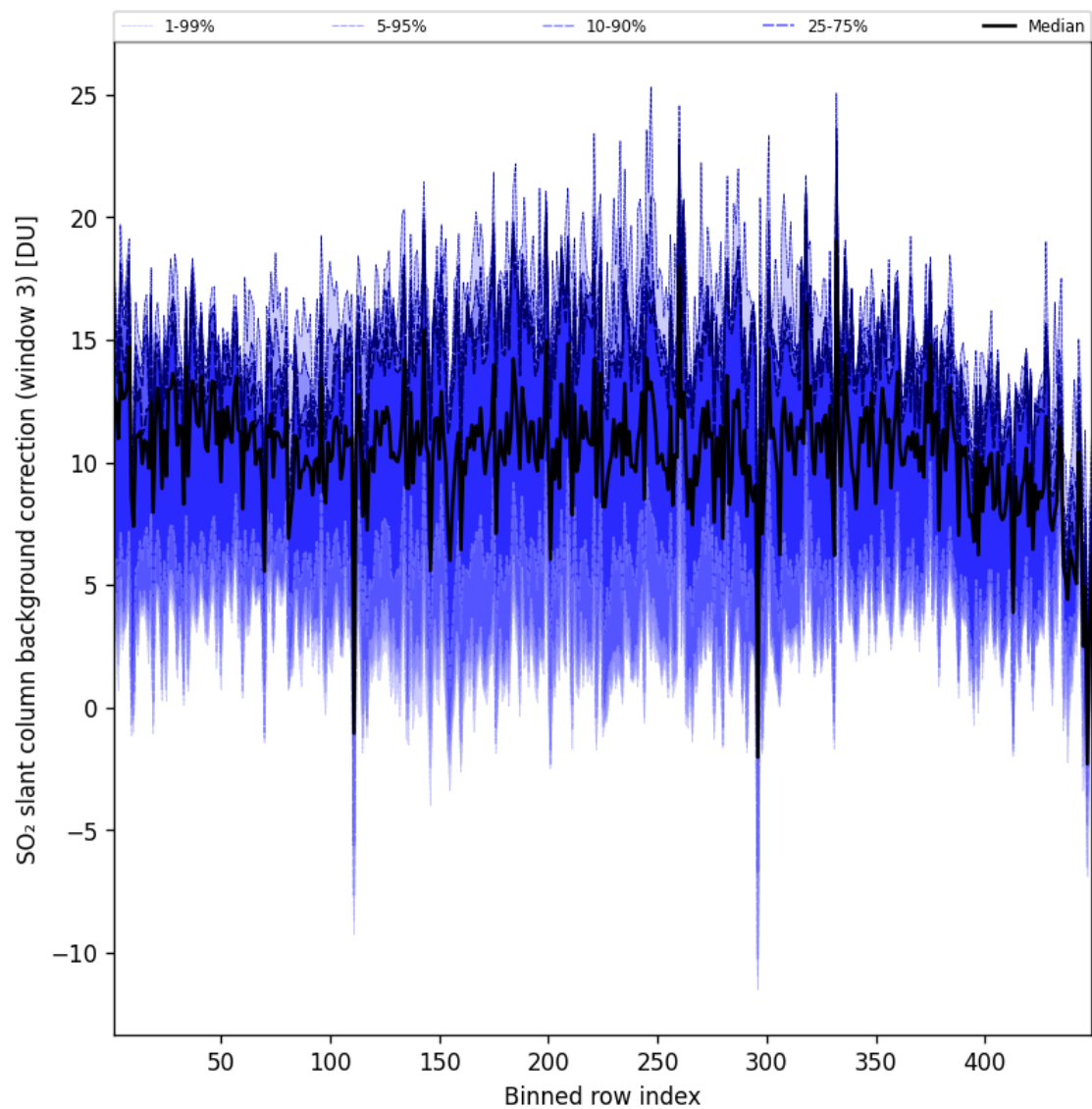
Figure 101: Along track statistics of “SO 2 slant column background correction (window 3)” for 2025-06-03 to 2025-06-04
