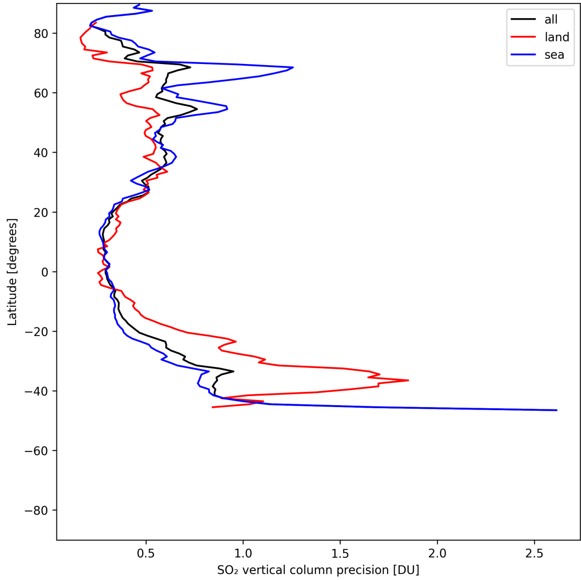
Figure 32: Zonal average of “SO 2 vertical column precision” for 2025-06-03 to 2025-06-04.
