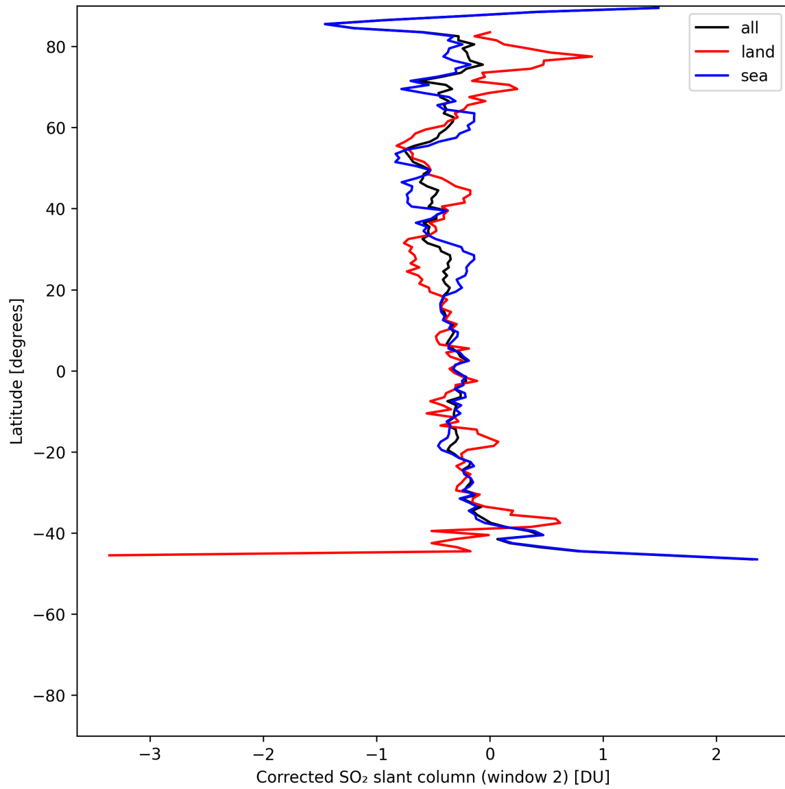
Figure 42: Zonal average of “Corrected SO 2 slant column (window 2)” for 2025-06-03 to 2025-06-04.
