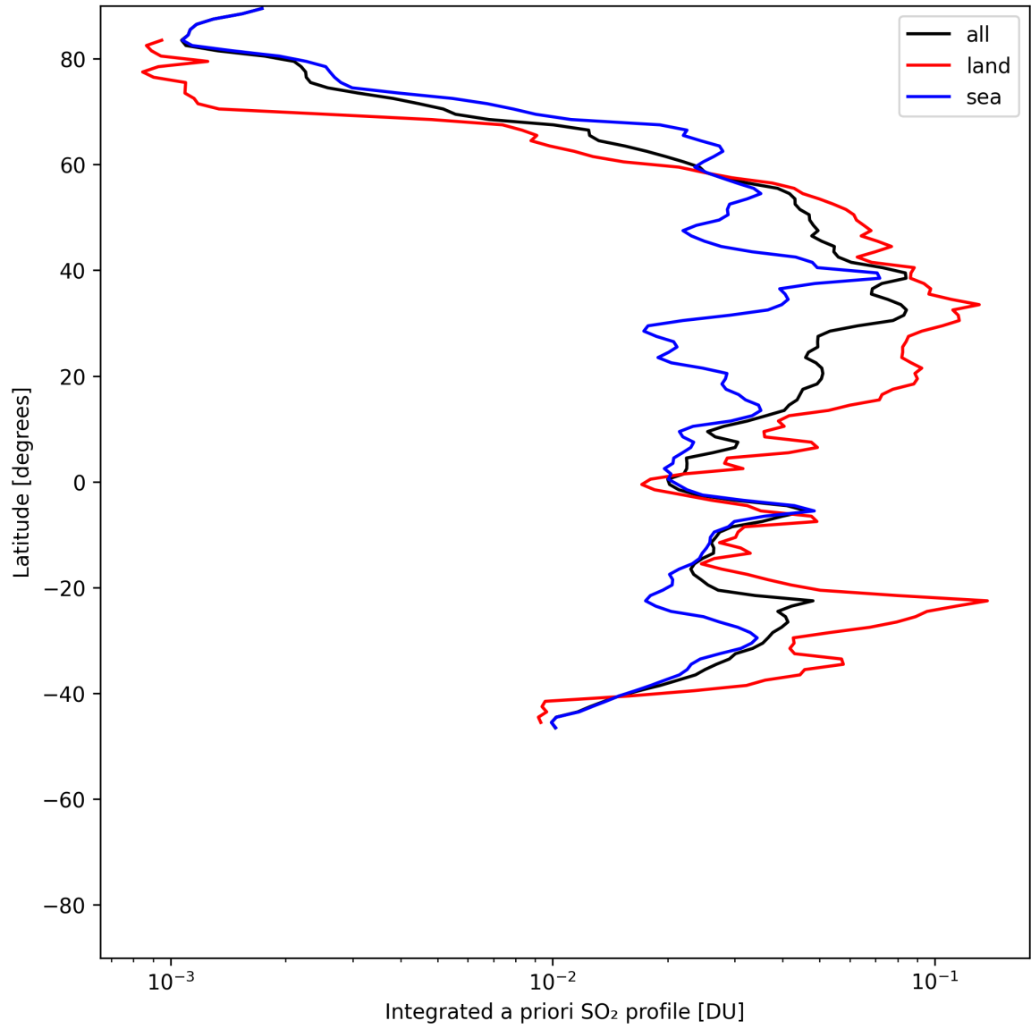
Figure 49: Zonal average of “Integrated a priori SO 2 profile” for 2025-06-03 to 2025-06-04.
