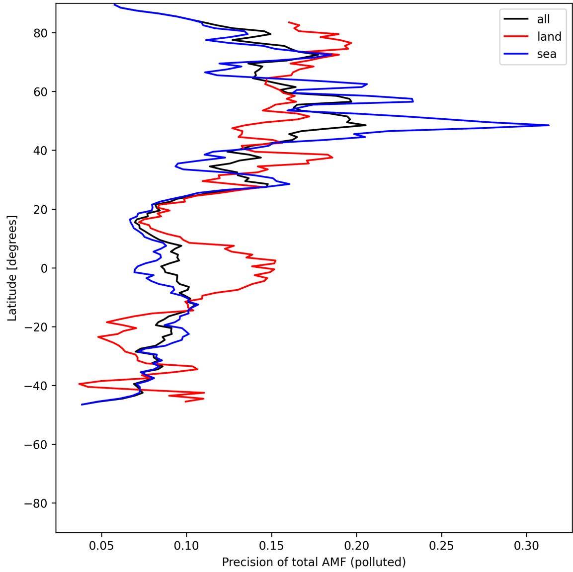
Figure 54: Zonal average of “Precision of total AMF (polluted)” for 2025-06-03 to 2025-06-04.
