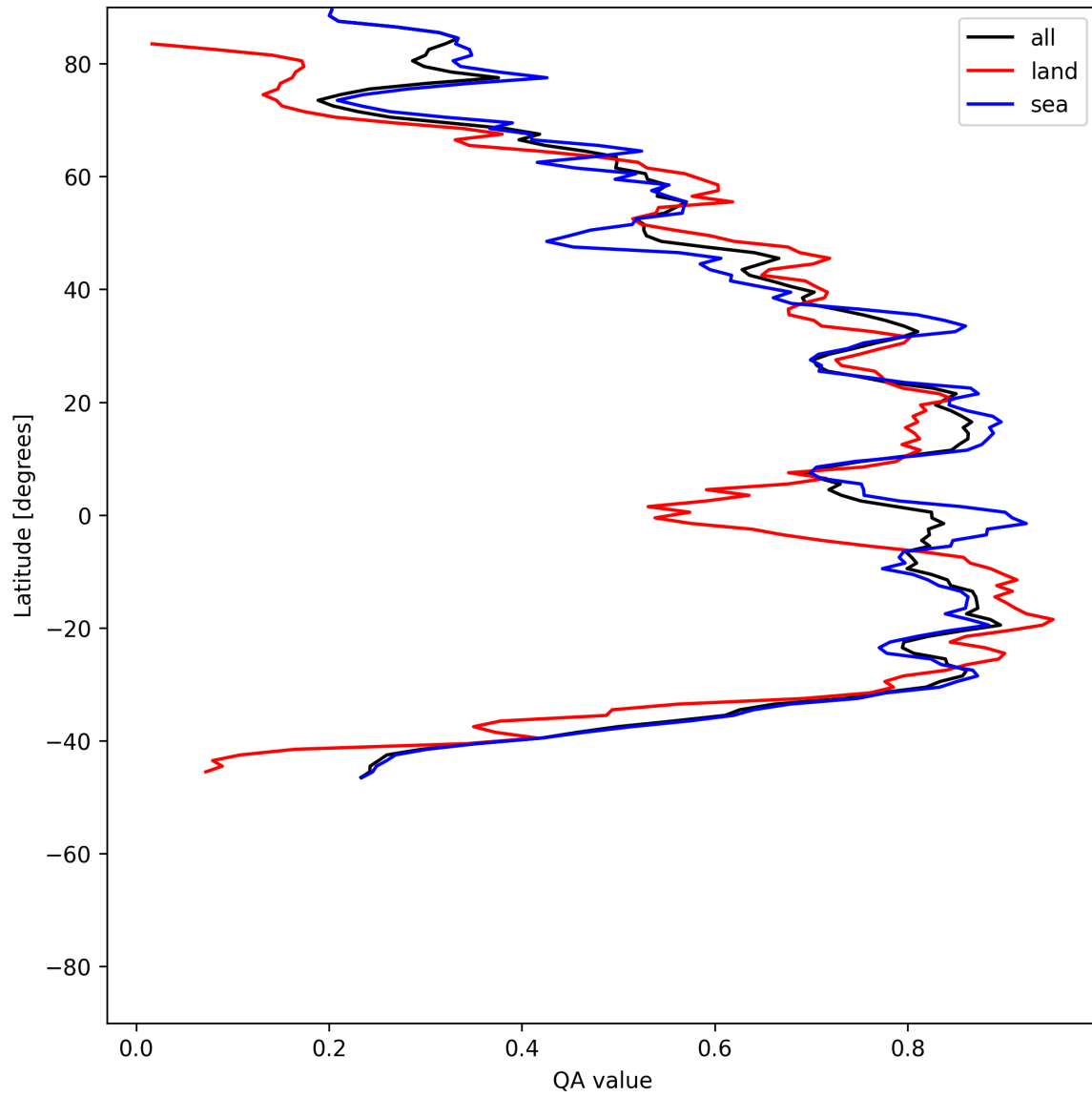
Figure 30: Zonal average of “QA value” for 2025-06-03 to 2025-06-04.
