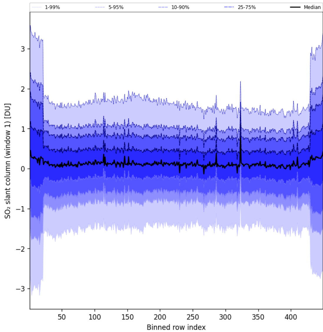
Figure 90: Along track statistics of “SO 2 slant column (window 1)” for 2025-06-03 to 2025-06-04
