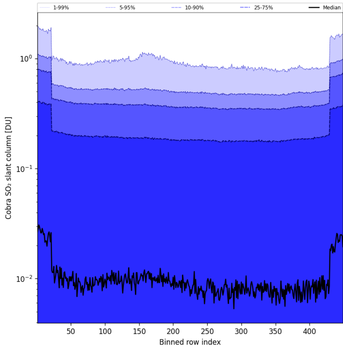
Figure 88: Along track statistics of “Cobra SO 2 slant column” for 2025-06-03 to 2025-06-04
