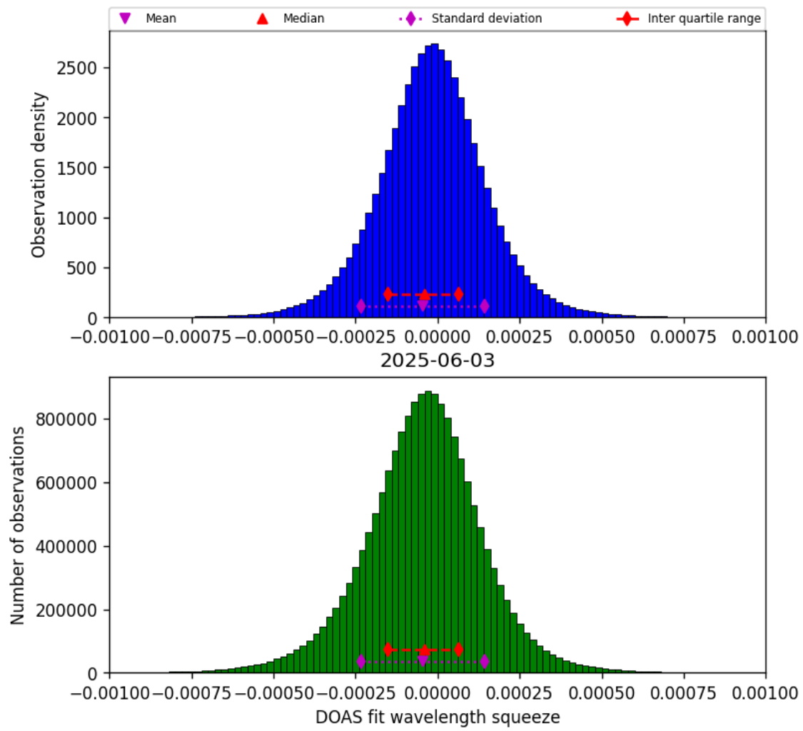
Figure 78: Histogram of “DOAS fit wavelength squeeze” for 2025-06-03 to 2025-06-04
