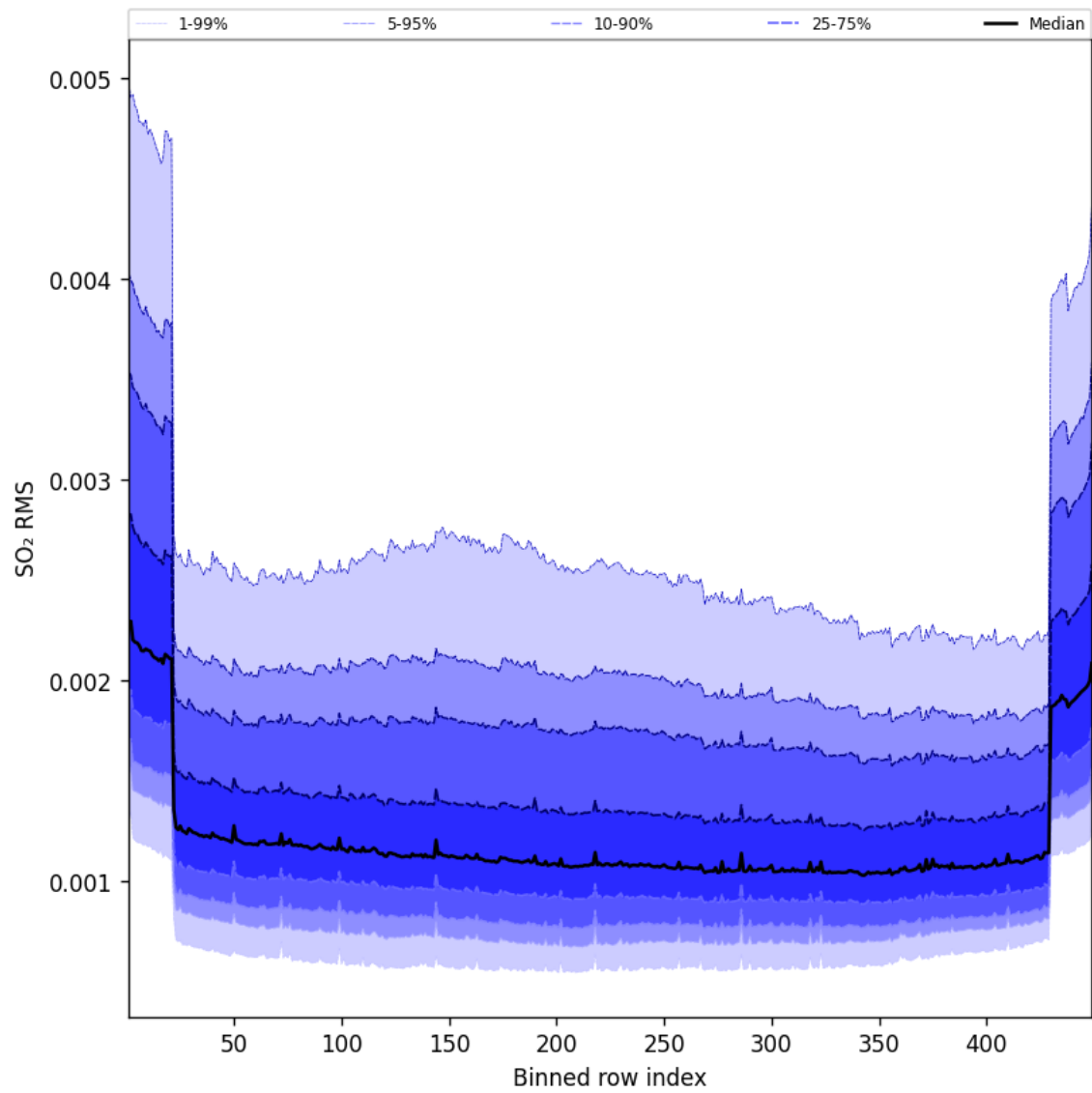
Figure 106: Along track statistics of “SO 2 RMS” for 2025-06-03 to 2025-06-04
