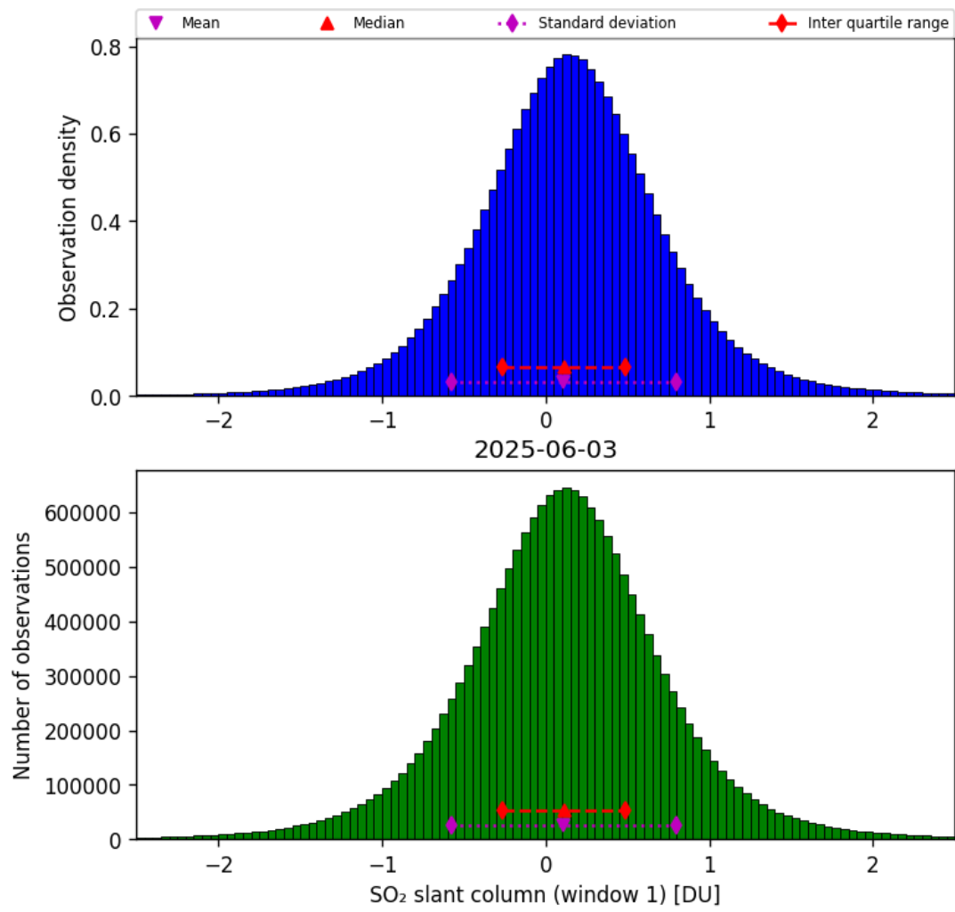
Figure 63: Histogram of “SO 2 slant column (window 1)” for 2025-06-03 to 2025-06-04
