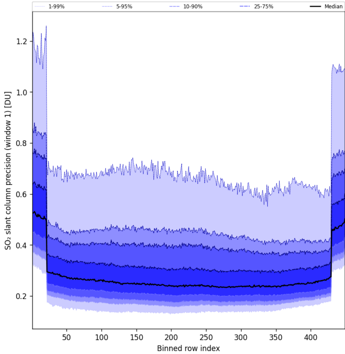
Figure 91: Along track statistics of “SO 2 slant column precision (window 1)” for 2025-06-03 to 2025-06-04
