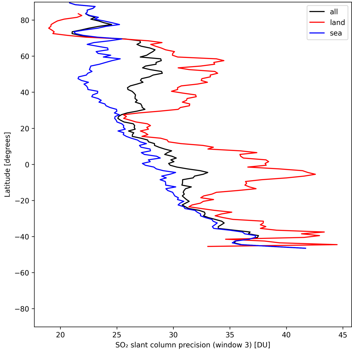
Figure 45: Zonal average of “SO 2 slant column precision (window 3)” for 2025-06-03 to 2025-06-04.
