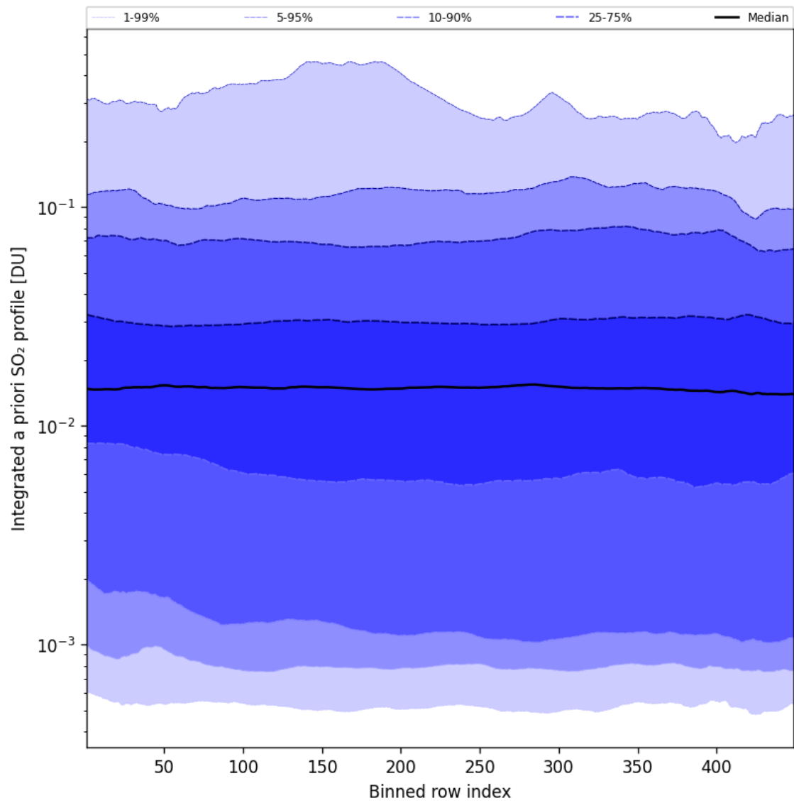
Figure 103: Along track statistics of “Integrated a priori SO 2 profile” for 2025-06-03 to 2025-06-04
