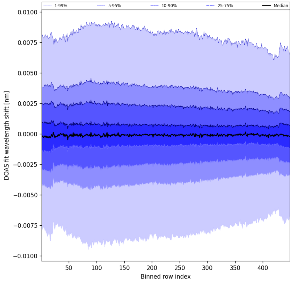
Figure 104: Along track statistics of “DOAS fit wavelength shift” for 2025-06-03 to 2025-06-04
