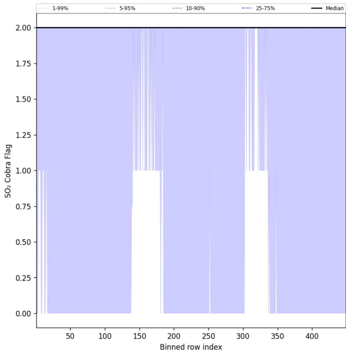
Figure 102: Along track statistics of “SO 2 Cobra Flag” for 2025-06-03 to 2025-06-04
