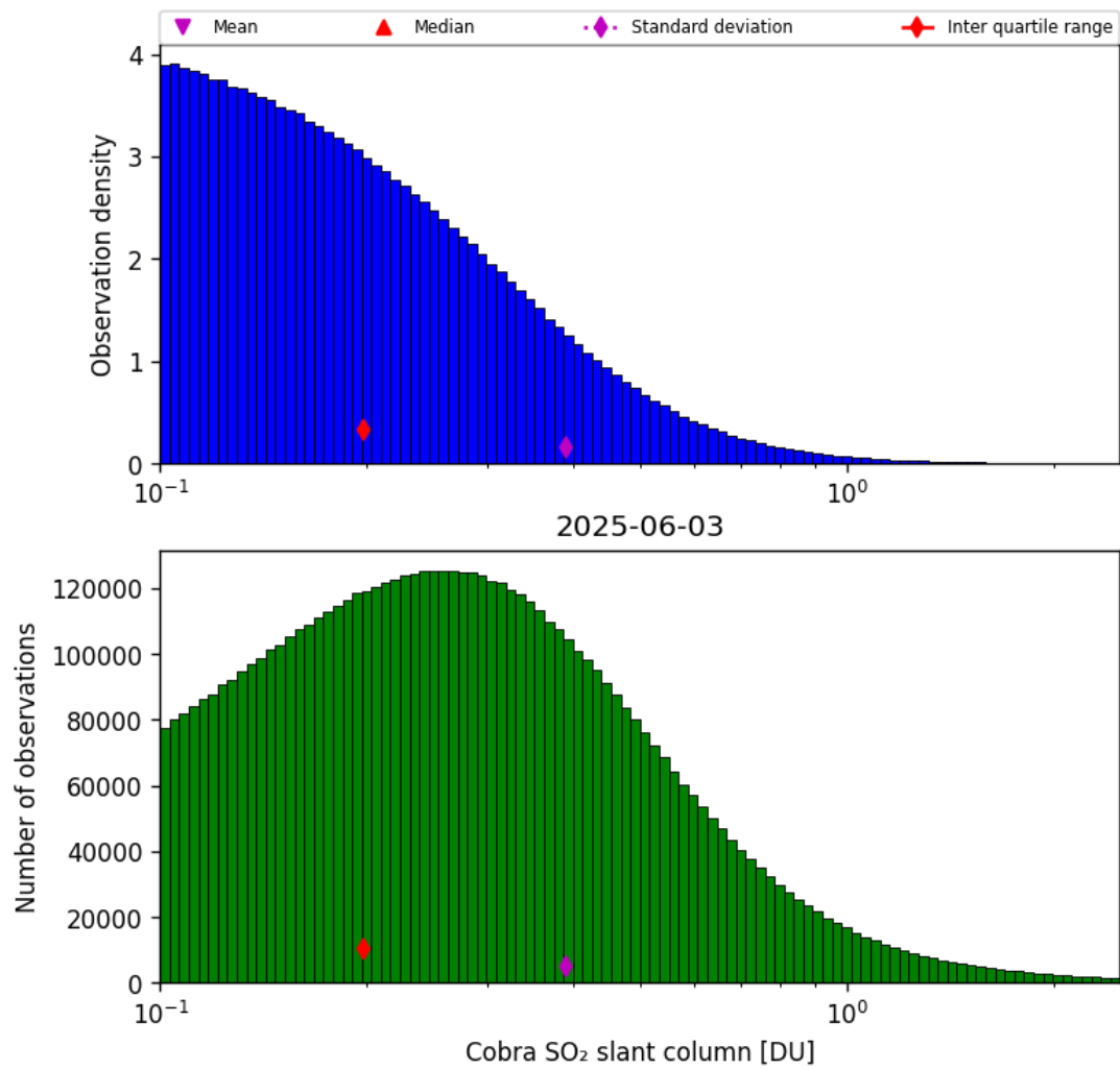
Figure 61: Histogram of “Cobra SO 2 slant column” for 2025-06-03 to 2025-06-04
