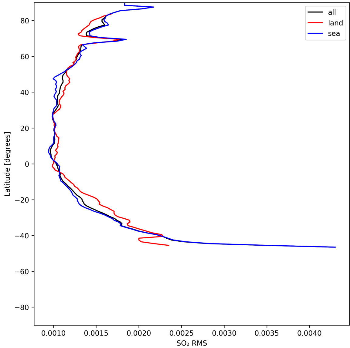
Figure 52: Zonal average of “SO 2 RMS” for 2025-06-03 to 2025-06-04.
