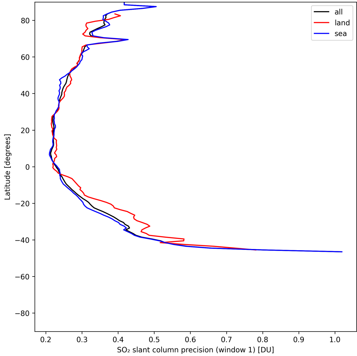
Figure 37: Zonal average of “SO 2 slant column precision (window 1)” for 2025-06-03 to 2025-06-04.
