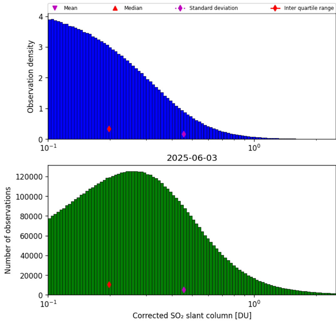
Figure 60: Histogram of “Corrected SO 2 slant column” for 2025-06-03 to 2025-06-04
