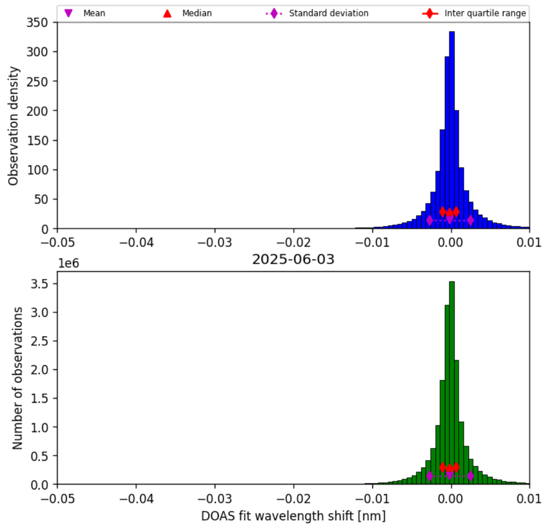
Figure 77: Histogram of “DOAS fit wavelength shift” for 2025-06-03 to 2025-06-04
