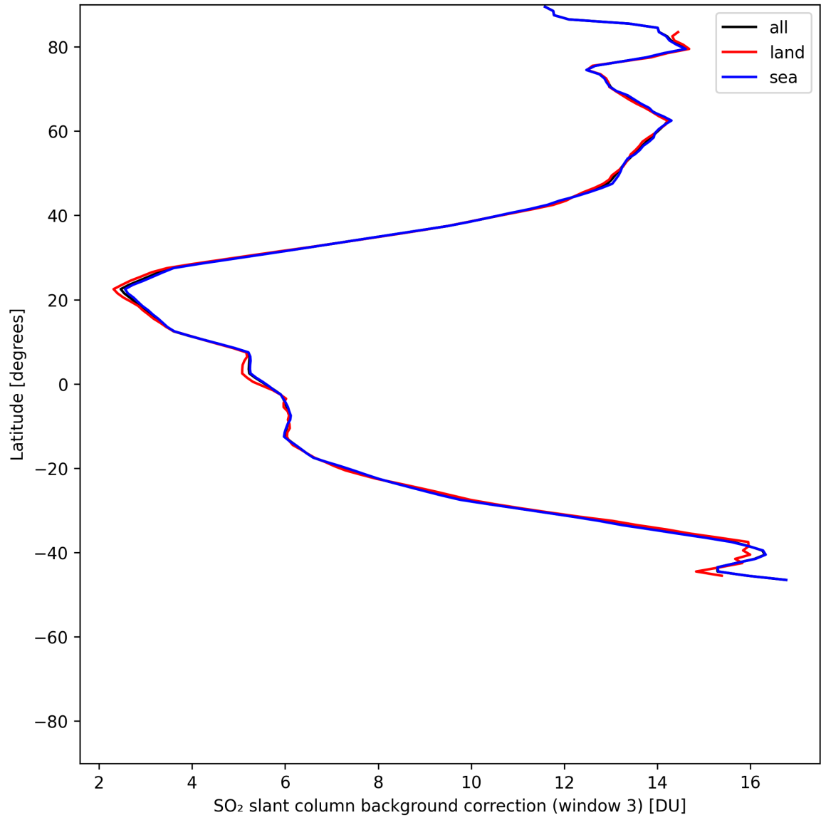
Figure 47: Zonal average of “SO 2 slant column background correction (window 3)” for 2025-06-03 to 2025-06-04.
