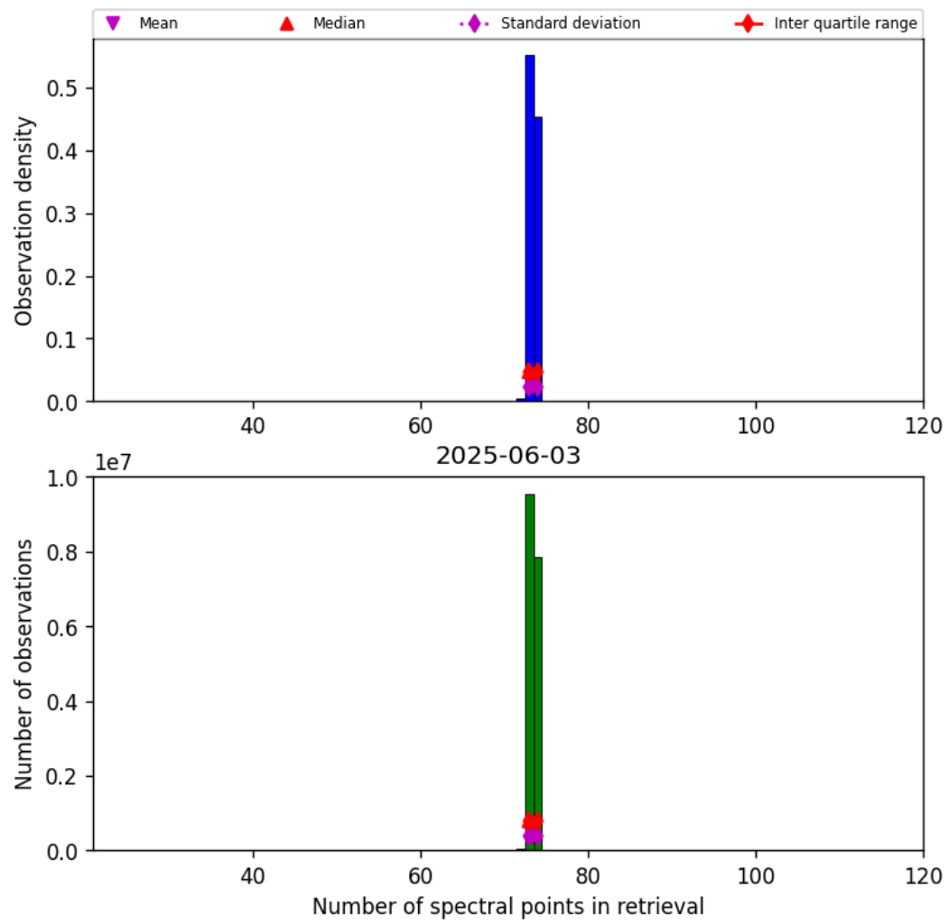
Figure 83: Histogram of “Number of spectral points in retrieval” for 2025-06-03 to 2025-06-04
