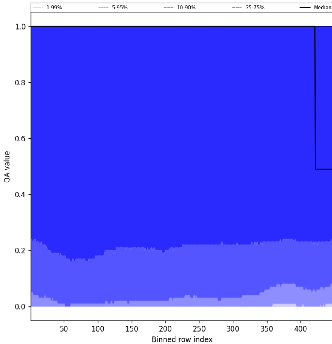
Figure 84: Along track statistics of “QA value” for 2025-06-03 to 2025-06-04
