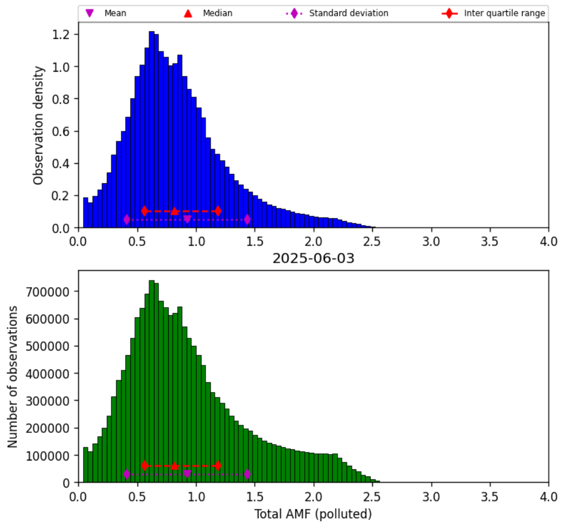
Figure 80: Histogram of “Total AMF (polluted)” for 2025-06-03 to 2025-06-04
