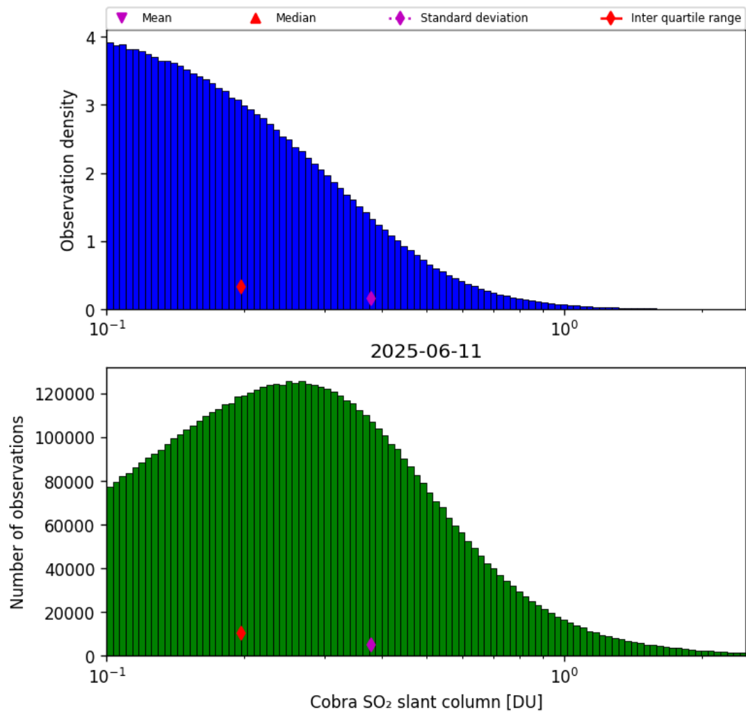
Figure 61: Histogram of “Cobra SO 2 slant column” for 2025-06-11 to 2025-06-12
