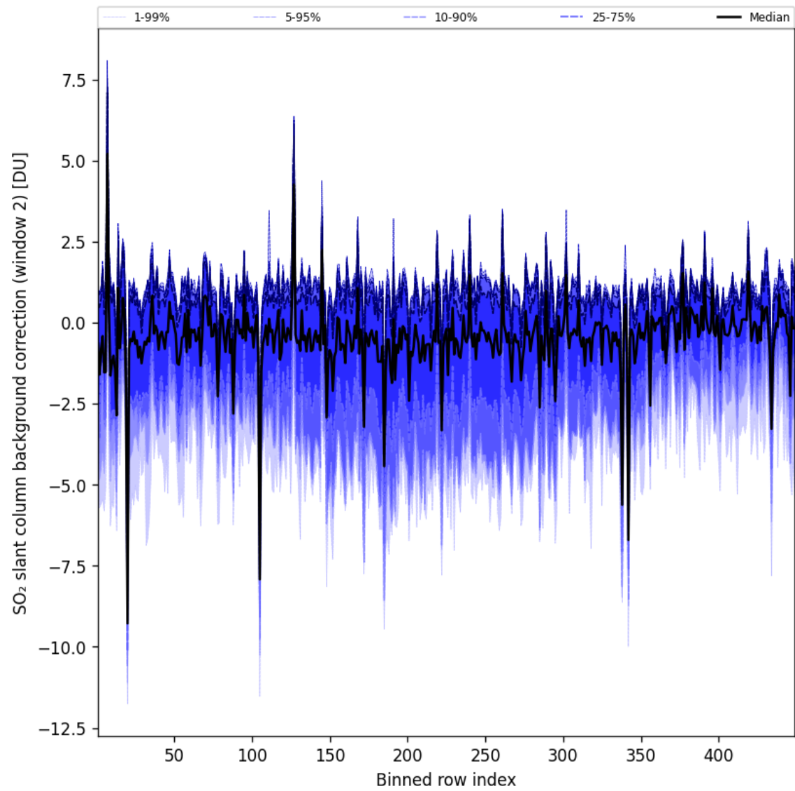
Figure 97: Along track statistics of “SO 2 slant column background correction (window 2)” for 2025-06-11 to 2025-06-12
