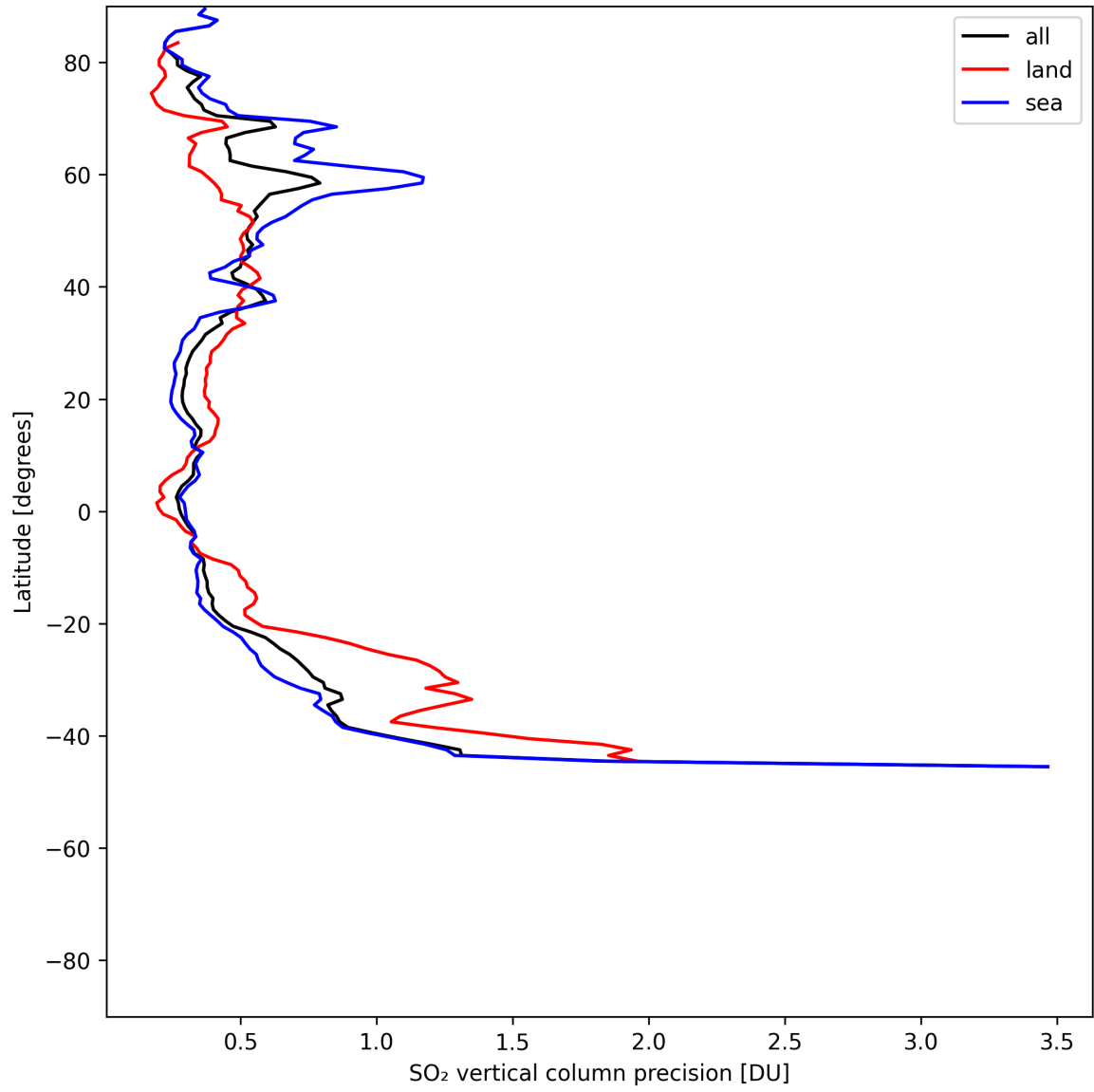
Figure 32: Zonal average of “SO 2 vertical column precision” for 2025-06-11 to 2025-06-12.
