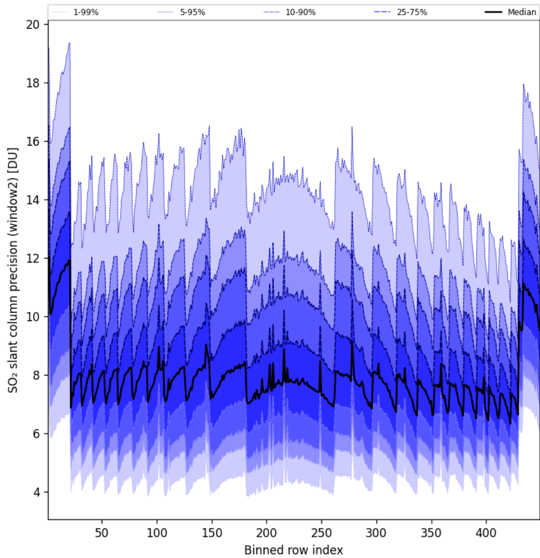
Figure 95: Along track statistics of “SO 2 slant column precision (window2)” for 2025-06-11 to 2025-06-12
