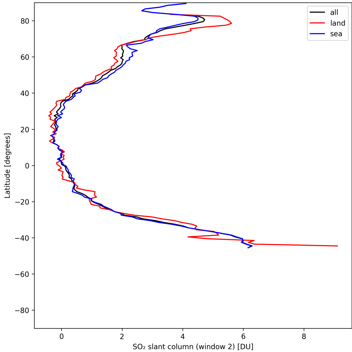
Figure 40: Zonal average of “SO 2 slant column (window 2)” for 2025-06-11 to 2025-06-12.
