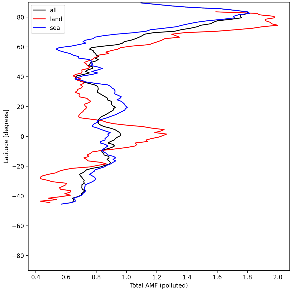
Figure 53: Zonal average of “Total AMF (polluted)” for 2025-06-11 to 2025-06-12.
