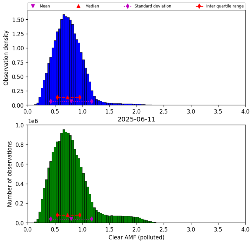
Figure 82: Histogram of “Clear AMF (polluted)” for 2025-06-11 to 2025-06-12
