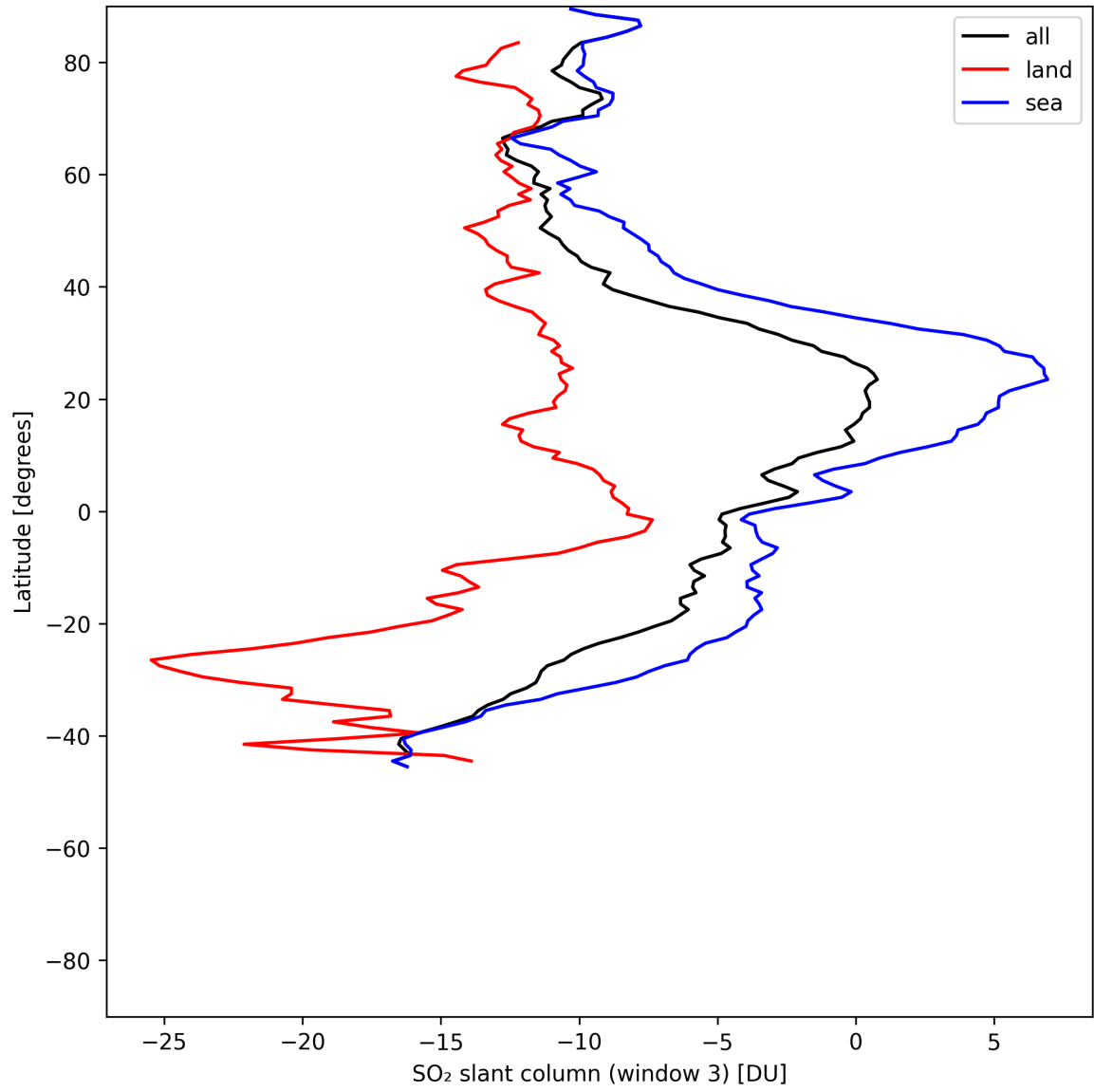
Figure 44: Zonal average of “SO 2 slant column (window 3)” for 2025-06-11 to 2025-06-12.
