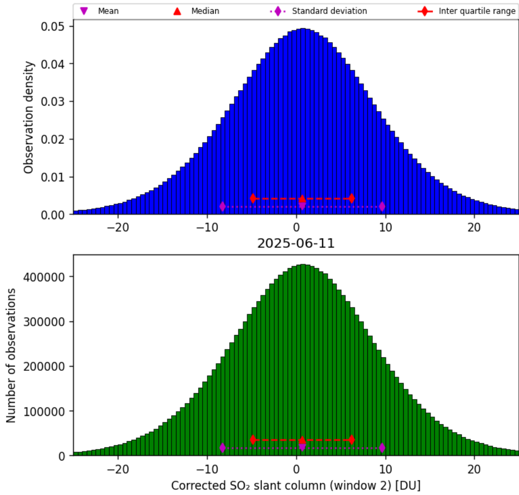
Figure 69: Histogram of “Corrected SO 2 slant column (window 2)” for 2025-06-11 to 2025-06-12
