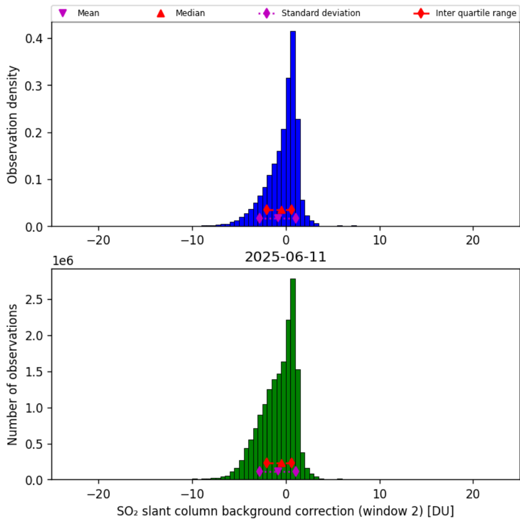
Figure 70: Histogram of “SO 2 slant column background correction (window 2)” for 2025-06-11 to 2025-06-12
