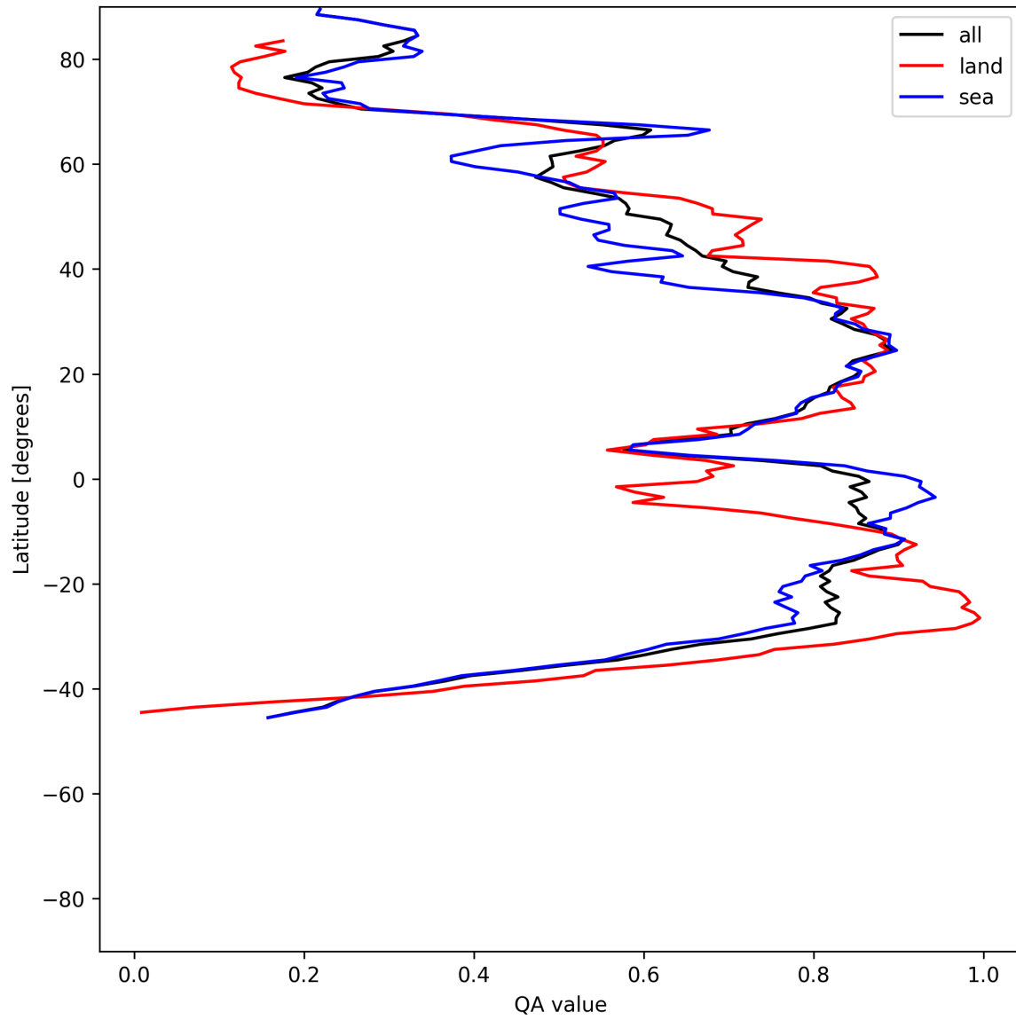
Figure 30: Zonal average of “QA value” for 2025-06-11 to 2025-06-12.
