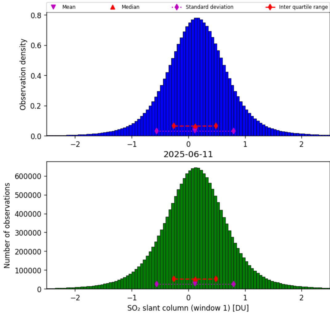
Figure 63: Histogram of “SO 2 slant column (window 1)” for 2025-06-11 to 2025-06-12
