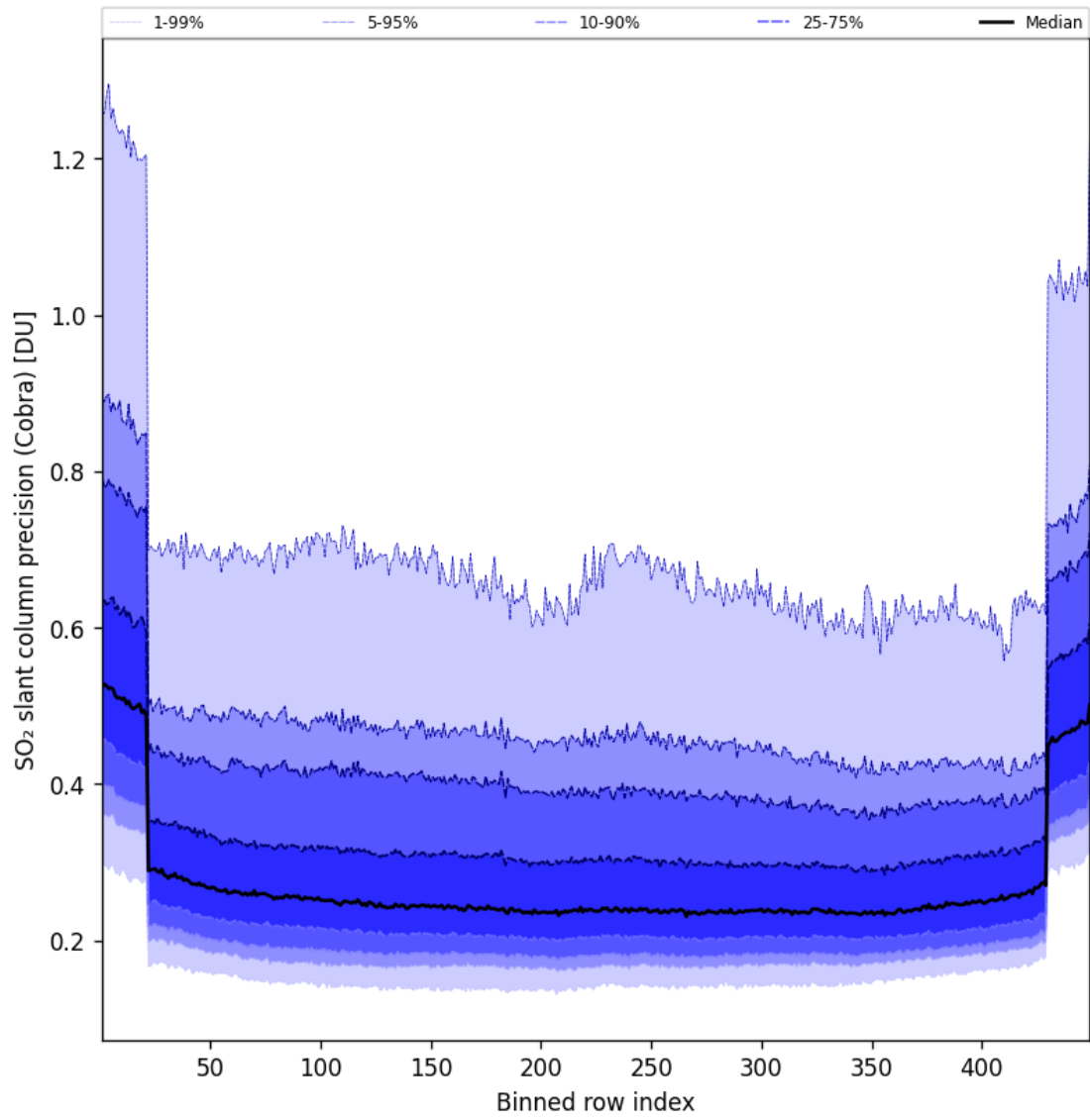
Figure 89: Along track statistics of “SO 2 slant column precision (Cobra)” for 2025-06-11 to 2025-06-12
