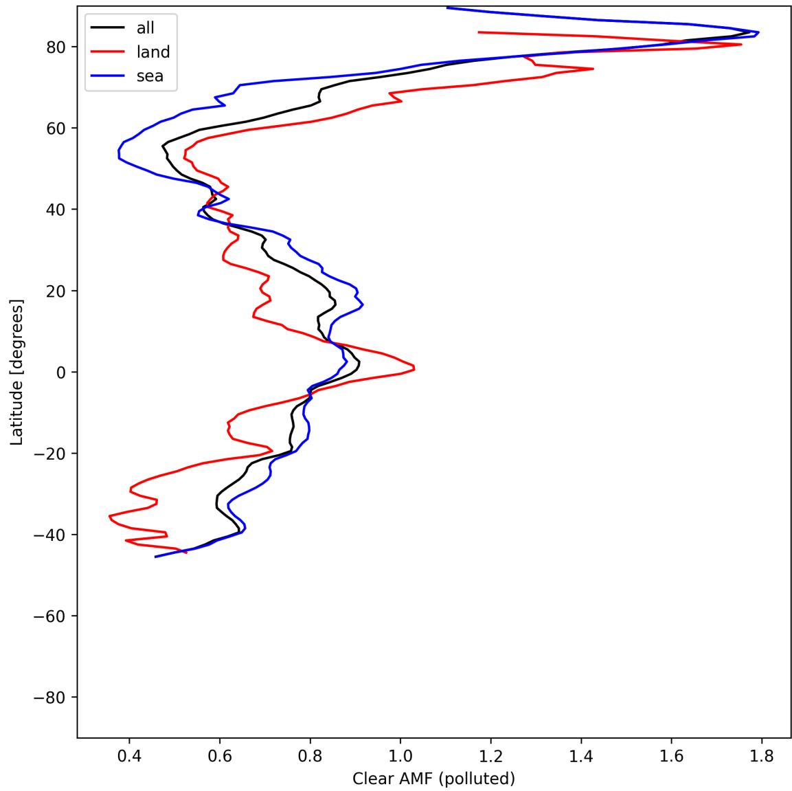
Figure 55: Zonal average of “Clear AMF (polluted)” for 2025-06-11 to 2025-06-12.
