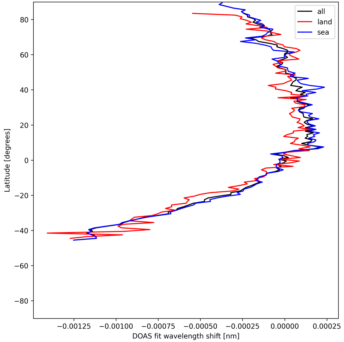
Figure 50: Zonal average of “DOAS fit wavelength shift” for 2025-06-11 to 2025-06-12.
