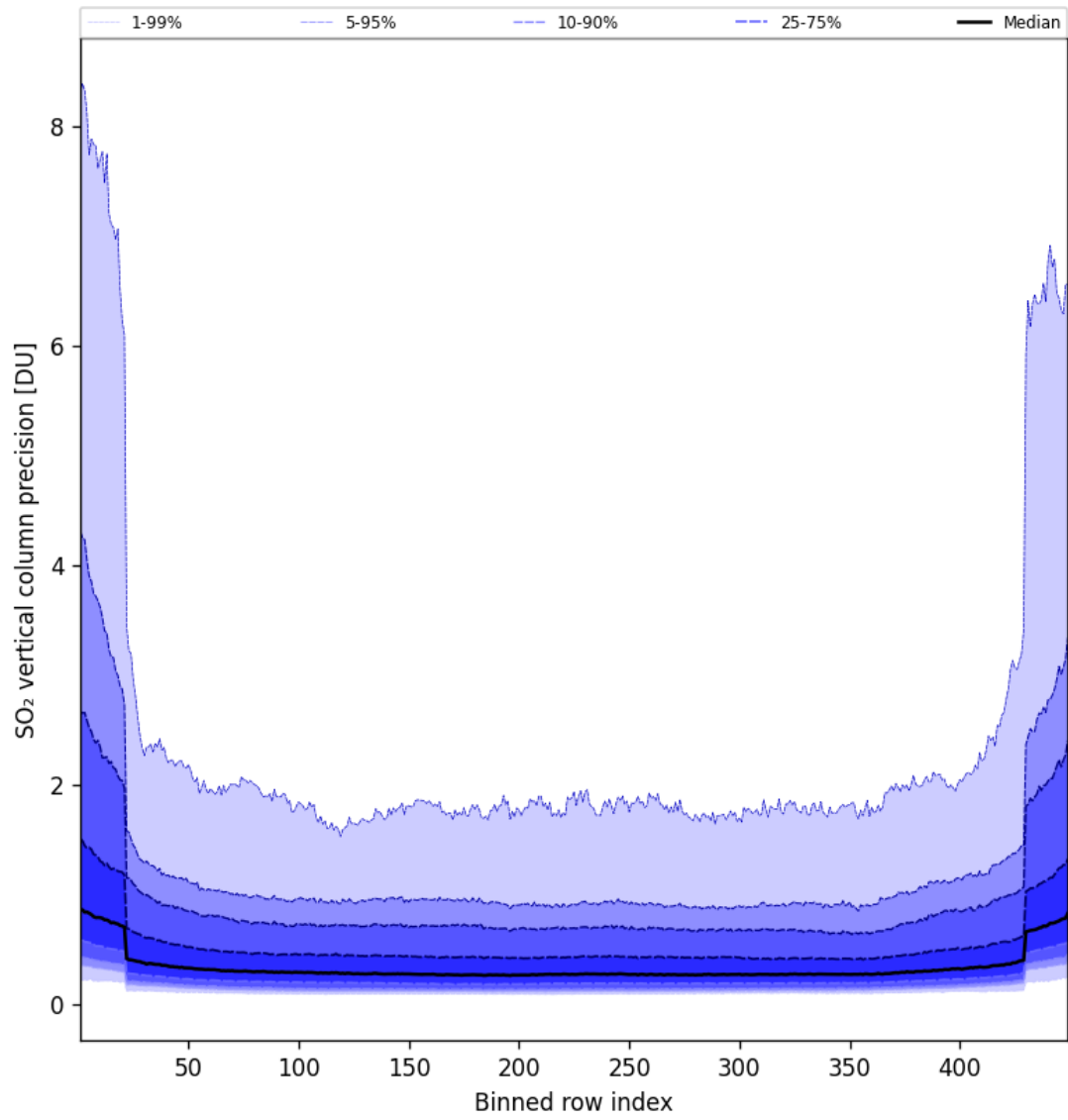
Figure 86: Along track statistics of “SO 2 vertical column precision” for 2025-06-11 to 2025-06-12
