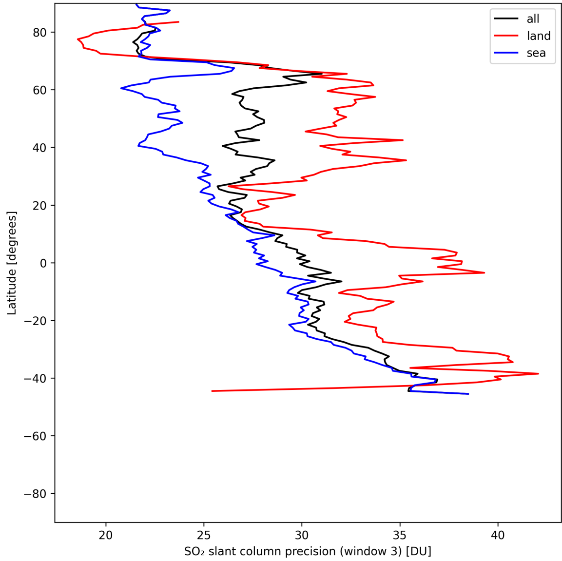
Figure 45: Zonal average of “SO 2 slant column precision (window 3)” for 2025-06-11 to 2025-06-12.
