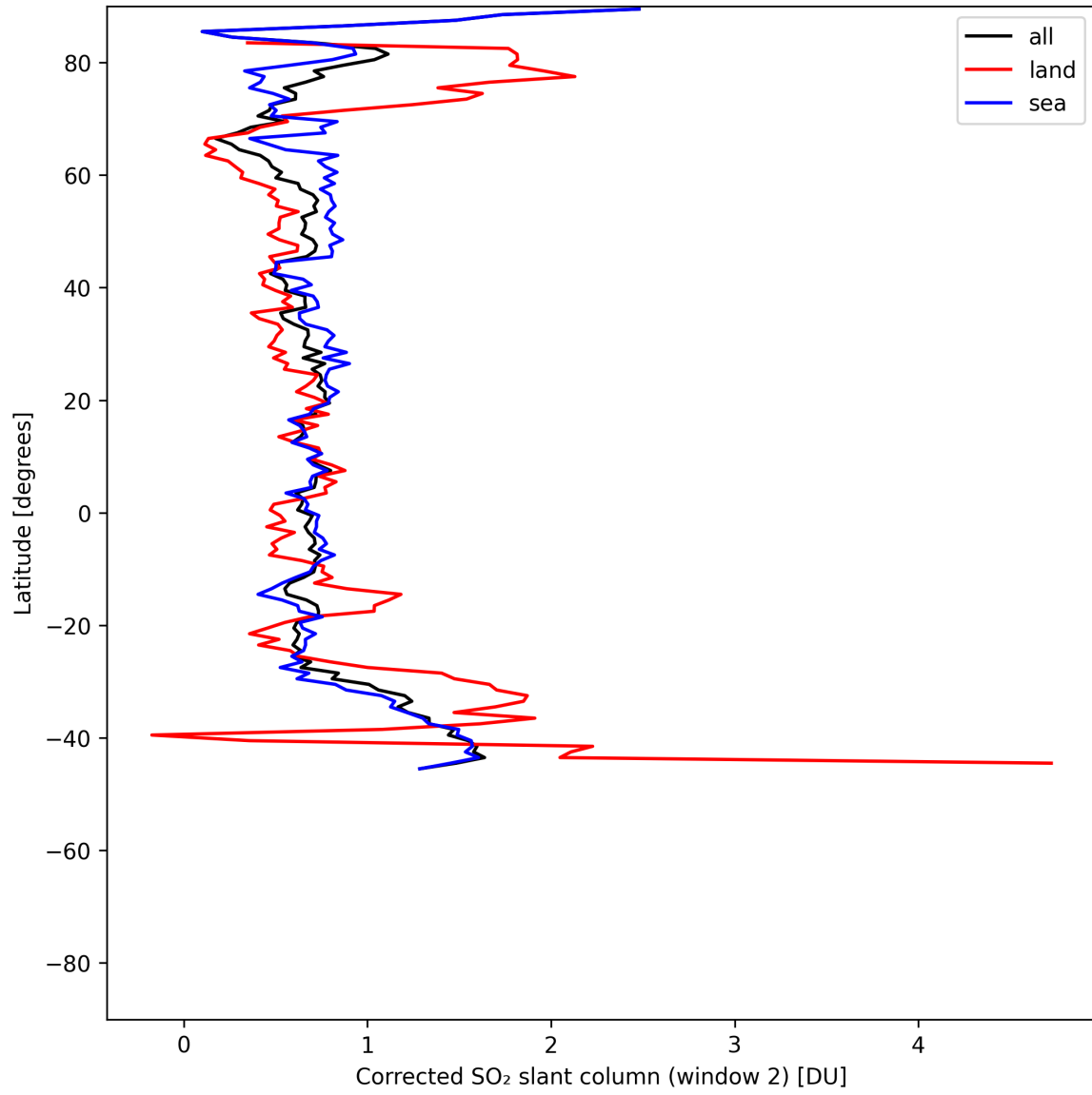
Figure 42: Zonal average of “Corrected SO 2 slant column (window 2)” for 2025-06-11 to 2025-06-12.
