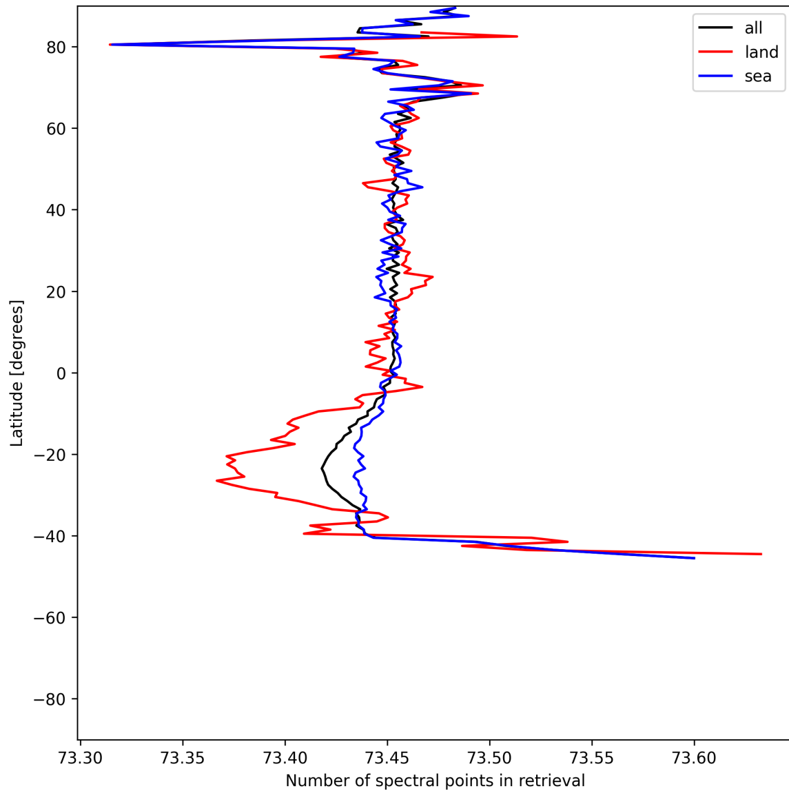
Figure 56: Zonal average of “Number of spectral points in retrieval” for 2025-06-11 to 2025-06-12.
