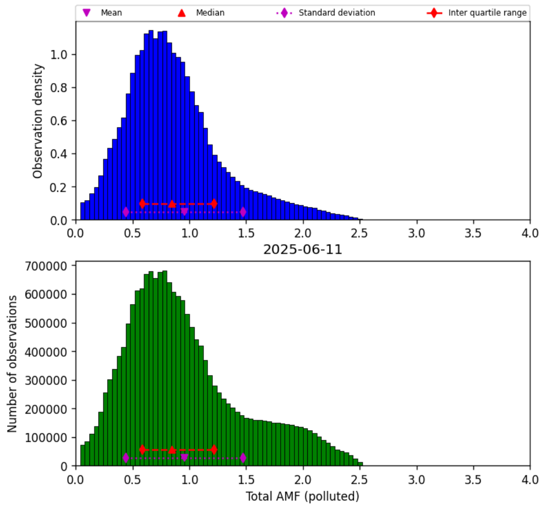
Figure 80: Histogram of “Total AMF (polluted)” for 2025-06-11 to 2025-06-12
