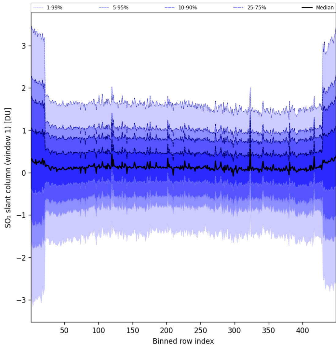
Figure 90: Along track statistics of “SO 2 slant column (window 1)” for 2025-06-11 to 2025-06-12
