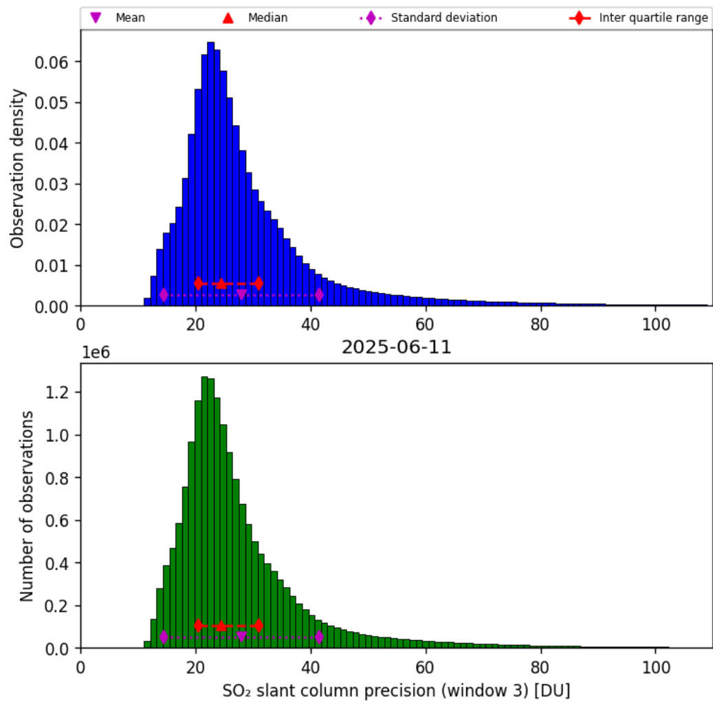
Figure 72: Histogram of “SO 2 slant column precision (window 3)” for 2025-06-11 to 2025-06-12
