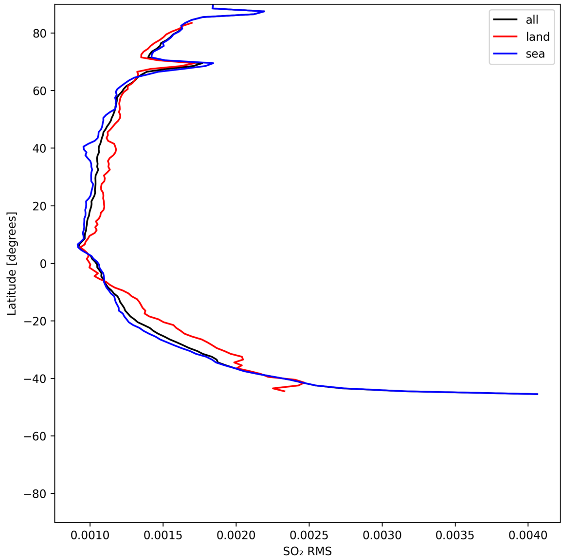
Figure 52: Zonal average of “SO 2 RMS” for 2025-06-11 to 2025-06-12.
