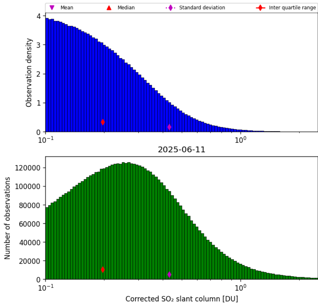
Figure 60: Histogram of “Corrected SO 2 slant column” for 2025-06-11 to 2025-06-12
