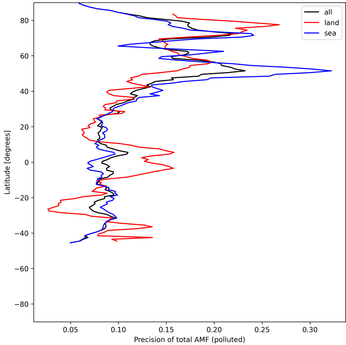
Figure 54: Zonal average of “Precision of total AMF (polluted)” for 2025-06-11 to 2025-06-12.
