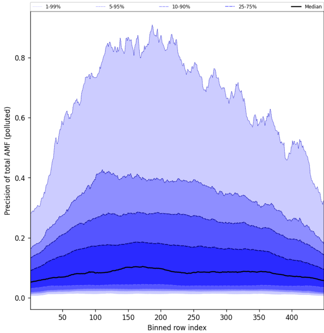
Figure 108: Along track statistics of “Precision of total AMF (polluted)” for 2025-06-11 to 2025-06-12
