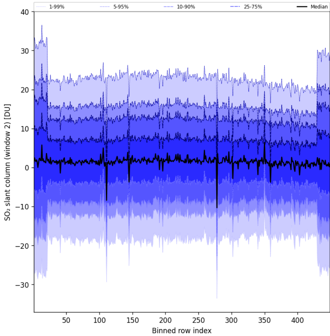
Figure 94: Along track statistics of “SO 2 slant column (window 2)” for 2025-06-11 to 2025-06-12
