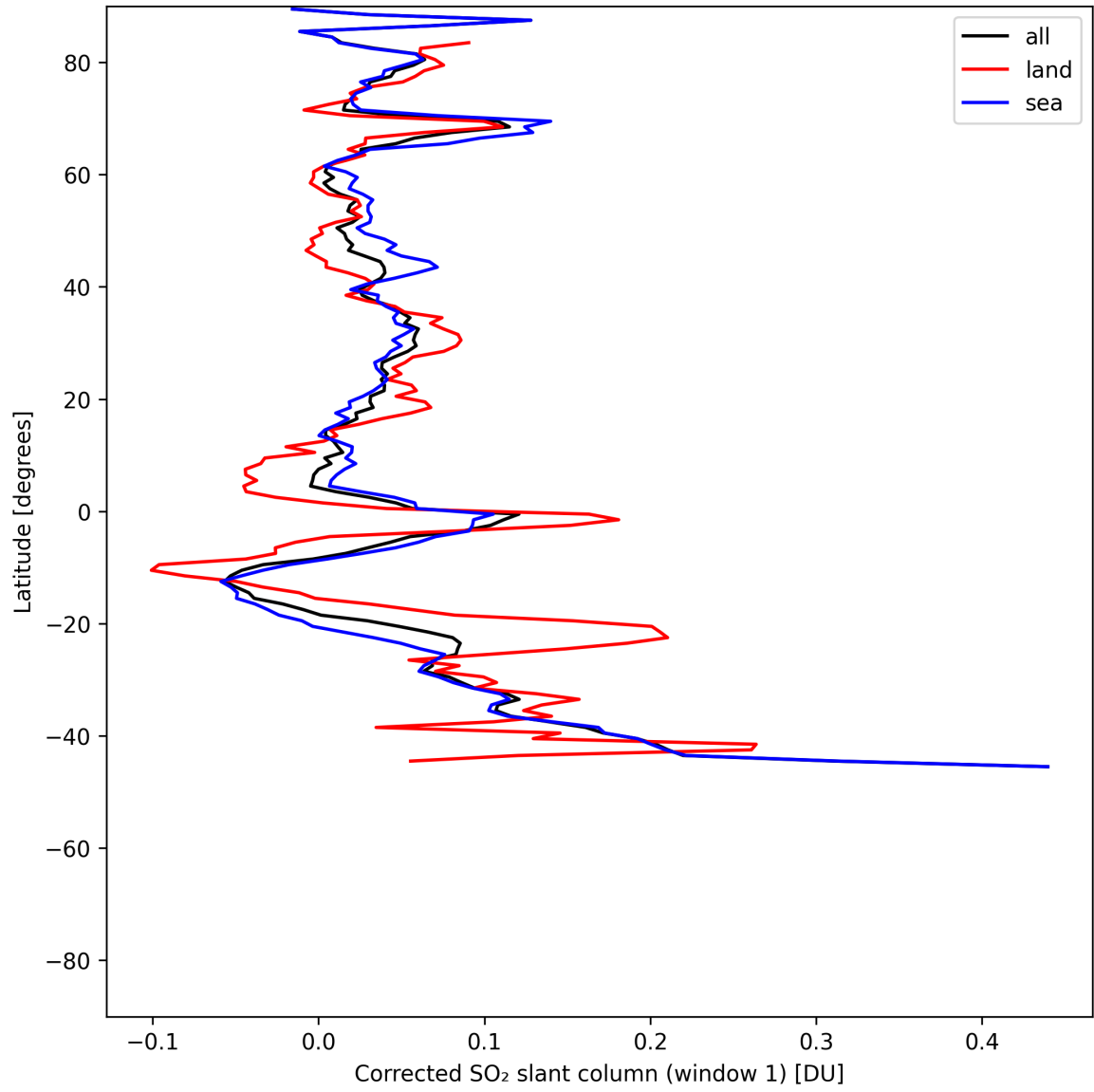
Figure 38: Zonal average of “Corrected SO 2 slant column (window 1)” for 2025-06-11 to 2025-06-12.
