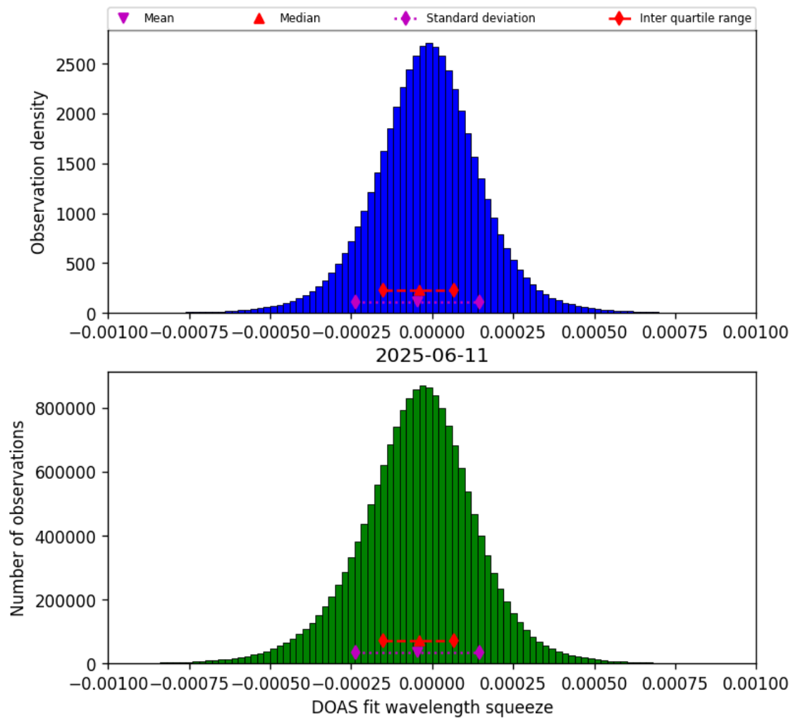
Figure 78: Histogram of “DOAS fit wavelength squeeze” for 2025-06-11 to 2025-06-12
