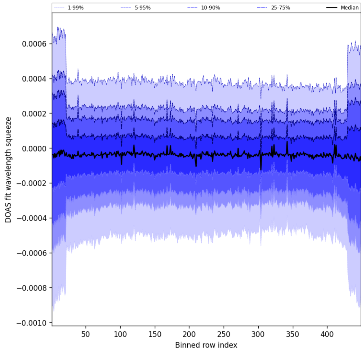
Figure 105: Along track statistics of “DOAS fit wavelength squeeze” for 2025-06-11 to 2025-06-12
