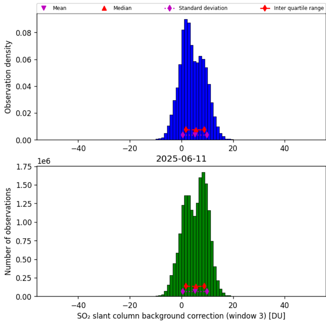
Figure 74: Histogram of “SO 2 slant column background correction (window 3)” for 2025-06-11 to 2025-06-12
