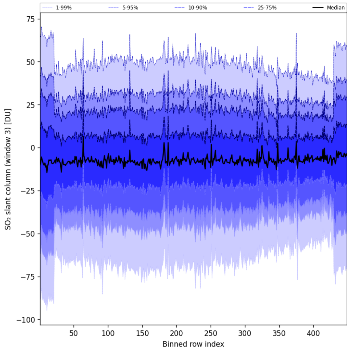
Figure 98: Along track statistics of “SO 2 slant column (window 3)” for 2025-06-11 to 2025-06-12
