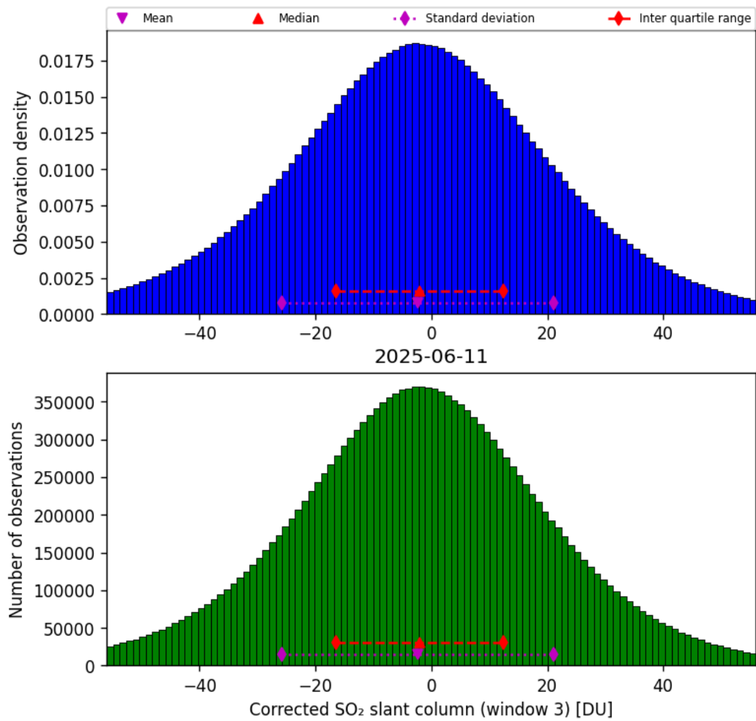
Figure 73: Histogram of “Corrected SO 2 slant column (window 3)” for 2025-06-11 to 2025-06-12
