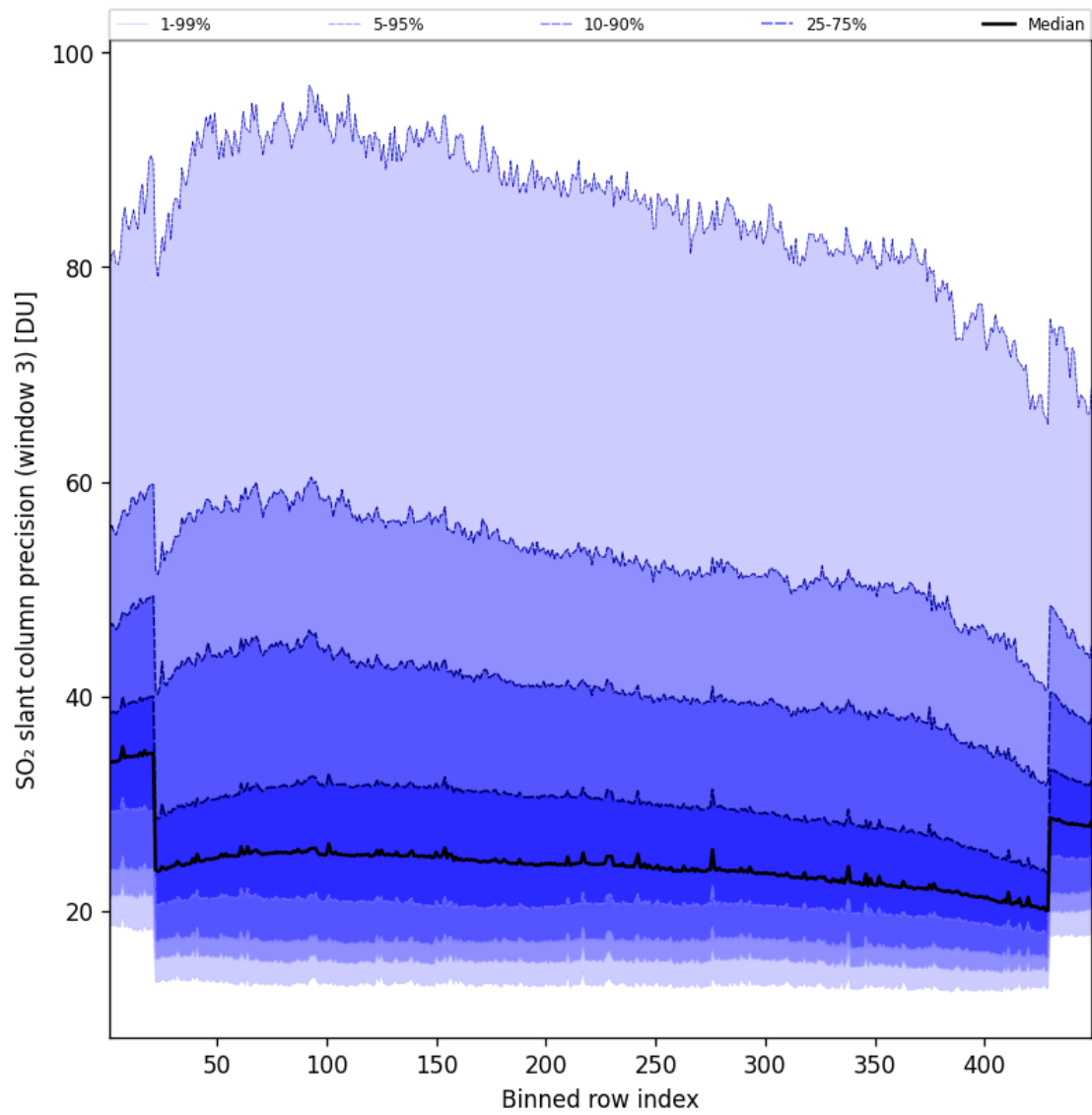
Figure 99: Along track statistics of “SO 2 slant column precision (window 3)” for 2025-06-11 to 2025-06-12
