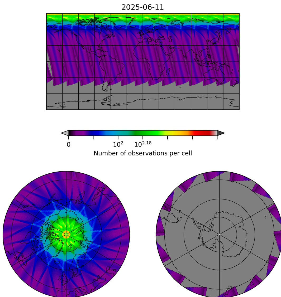
Figure 29: Map of the number of observations for 2025-06-11 to 2025-06-12
