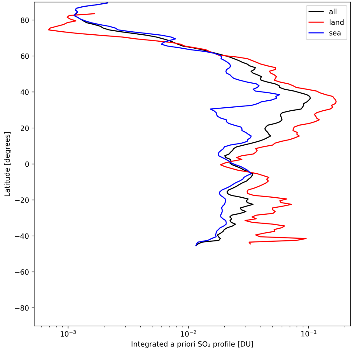
Figure 49: Zonal average of “Integrated a priori SO 2 profile” for 2025-06-11 to 2025-06-12.
