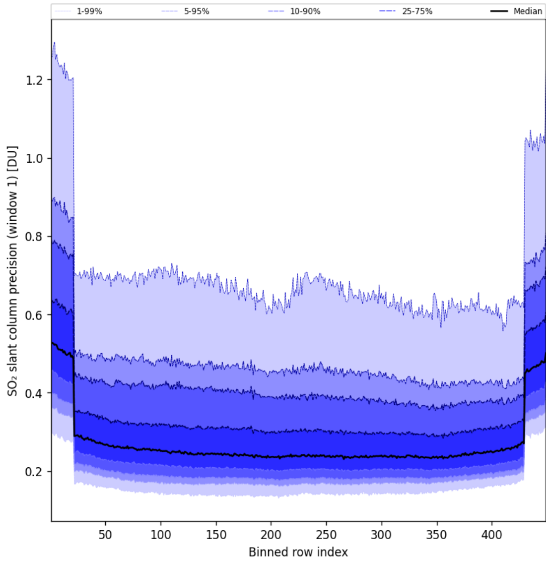
Figure 91: Along track statistics of “SO 2 slant column precision (window 1)” for 2025-06-11 to 2025-06-12
