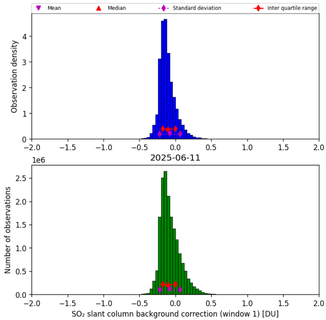
Figure 66: Histogram of “SO 2 slant column background correction (window 1)” for 2025-06-11 to 2025-06-12
