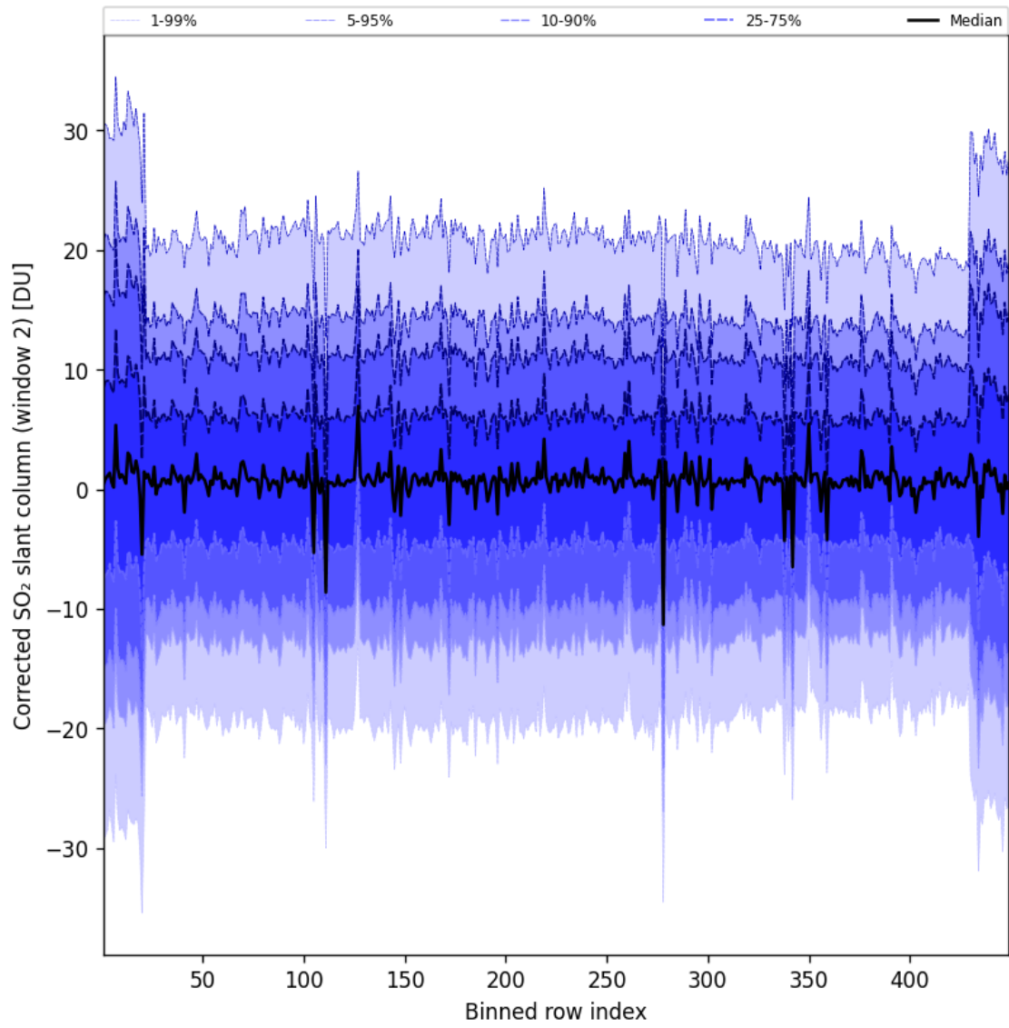
Figure 96: Along track statistics of “Corrected SO 2 slant column (window 2)” for 2025-06-11 to 2025-06-12
