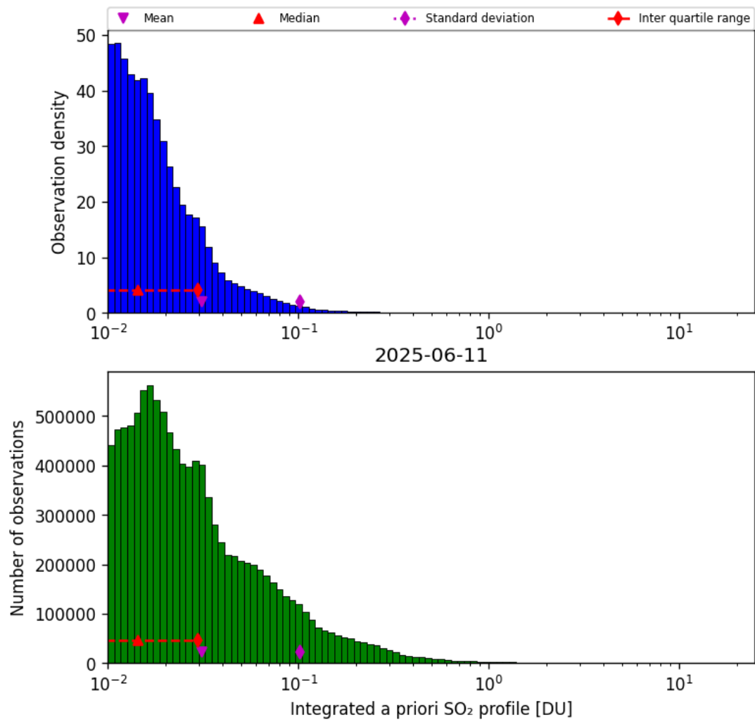
Figure 76: Histogram of “Integrated a priori SO 2 profile” for 2025-06-11 to 2025-06-12
