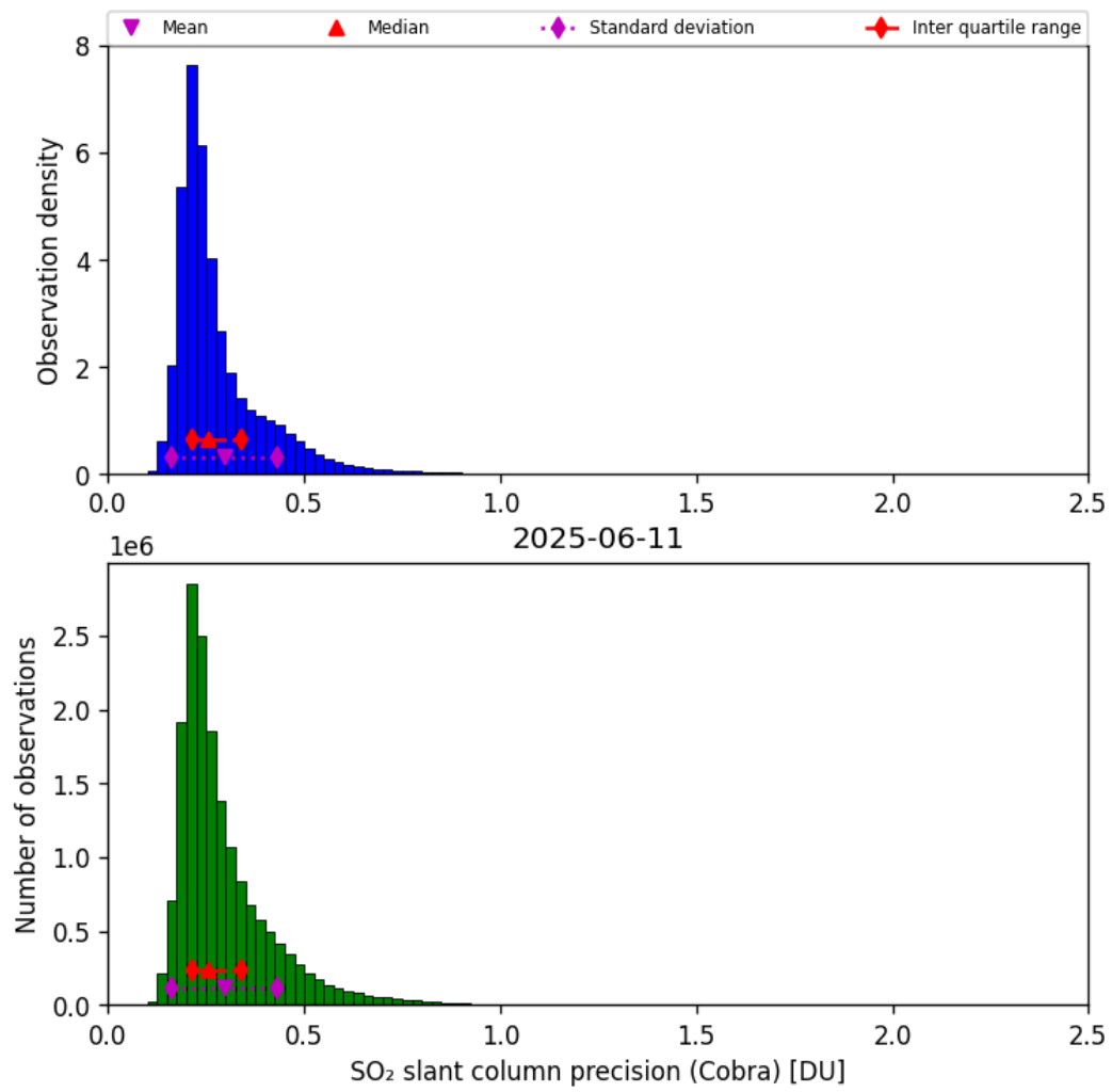
Figure 62: Histogram of “SO 2 slant column precision (Cobra)” for 2025-06-11 to 2025-06-12
