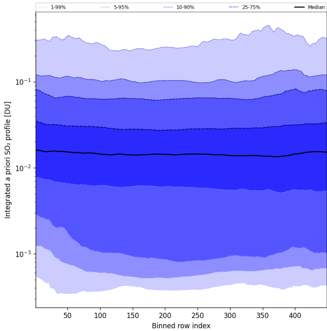
Figure 103: Along track statistics of “Integrated a priori SO 2 profile” for 2025-06-11 to 2025-06-12
