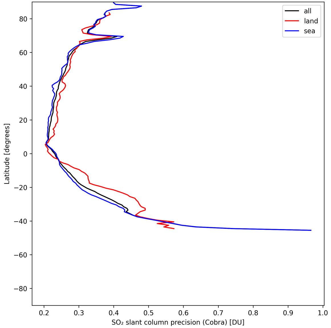
Figure 35: Zonal average of "SO 2 slant column precision (Cobra)" for 2025-06-11 to 2025-06-12.
