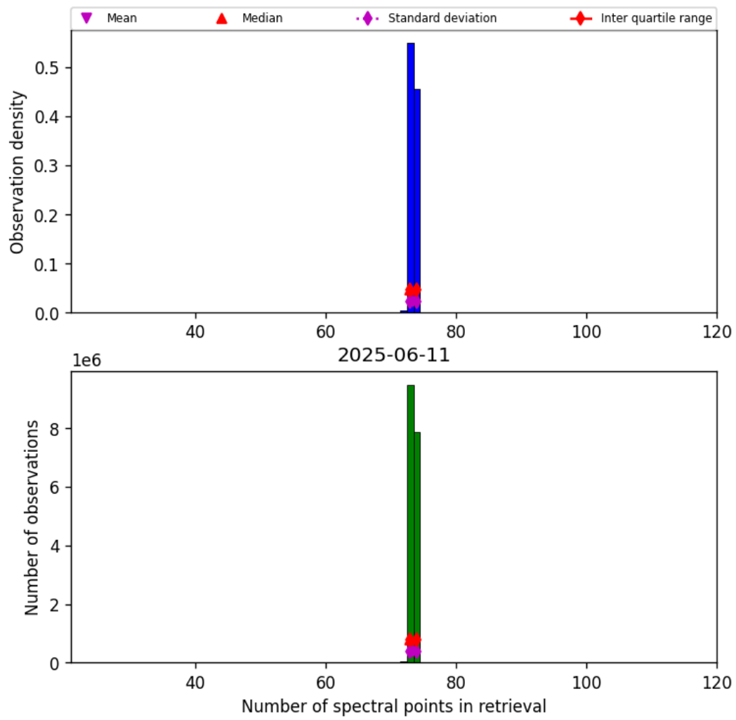
Figure 83: Histogram of “Number of spectral points in retrieval” for 2025-06-11 to 2025-06-12
