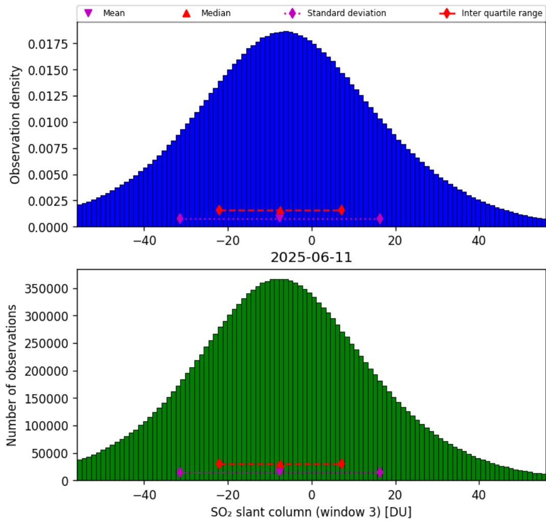
Figure 71: Histogram of “SO 2 slant column (window 3)” for 2025-06-11 to 2025-06-12
