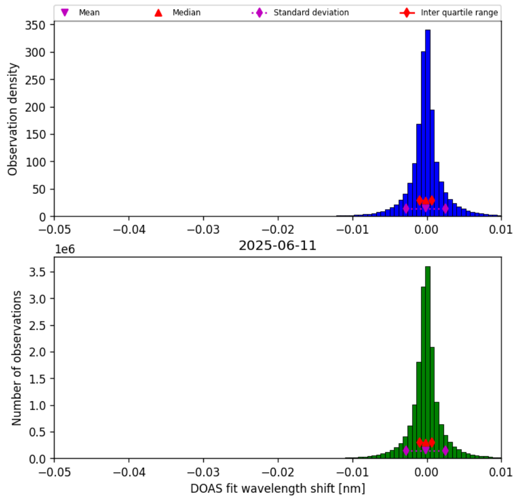
Figure 77: Histogram of “DOAS fit wavelength shift” for 2025-06-11 to 2025-06-12
