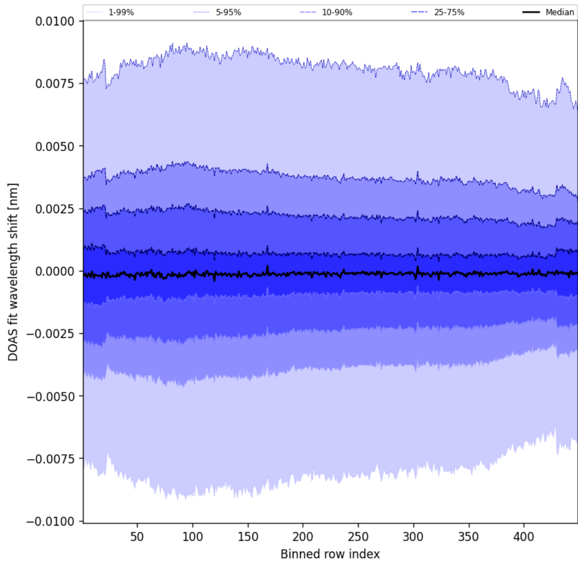
Figure 104: Along track statistics of “DOAS fit wavelength shift” for 2025-06-11 to 2025-06-12
