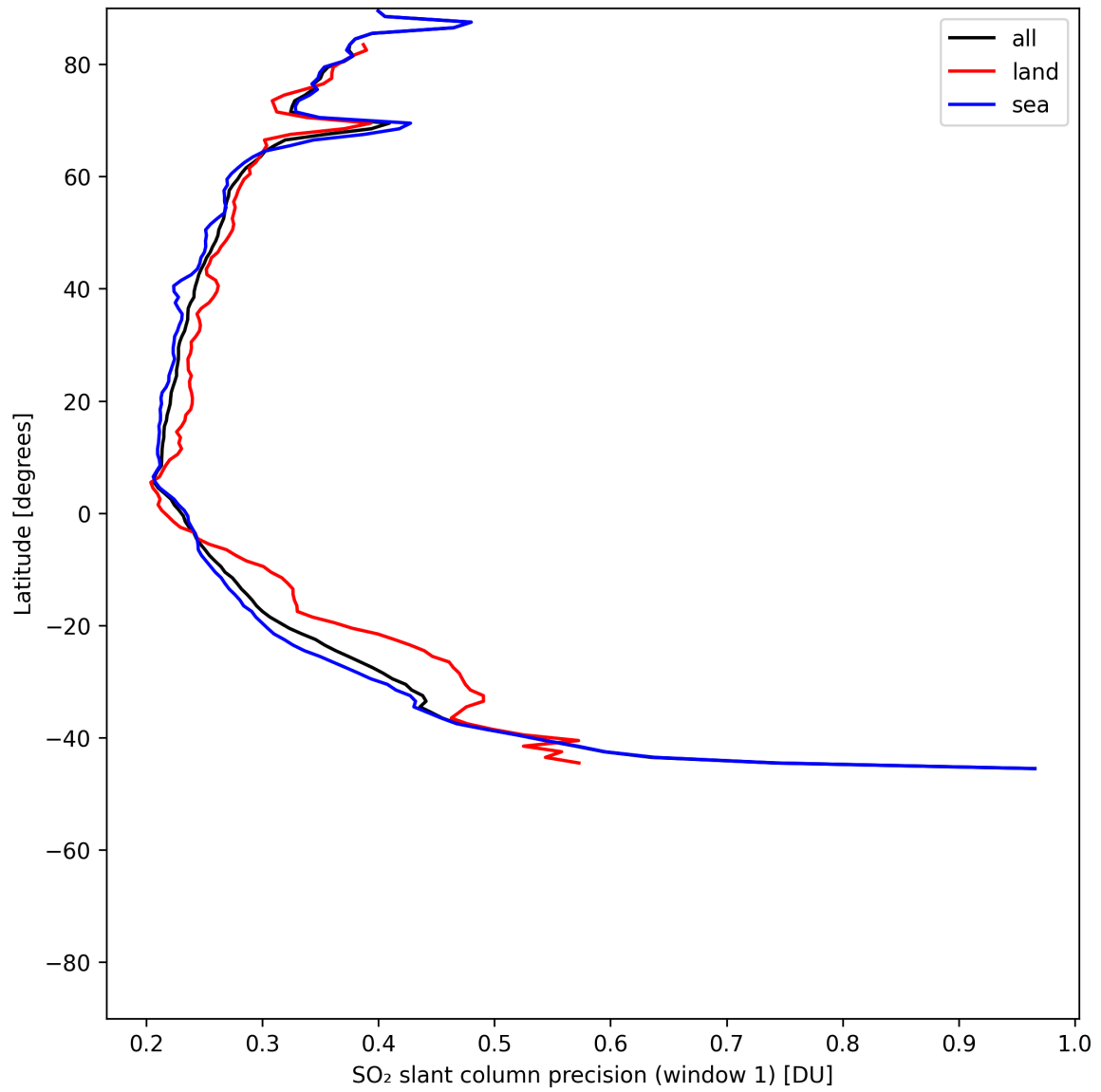
Figure 37: Zonal average of “SO 2 slant column precision (window 1)” for 2025-06-11 to 2025-06-12.
