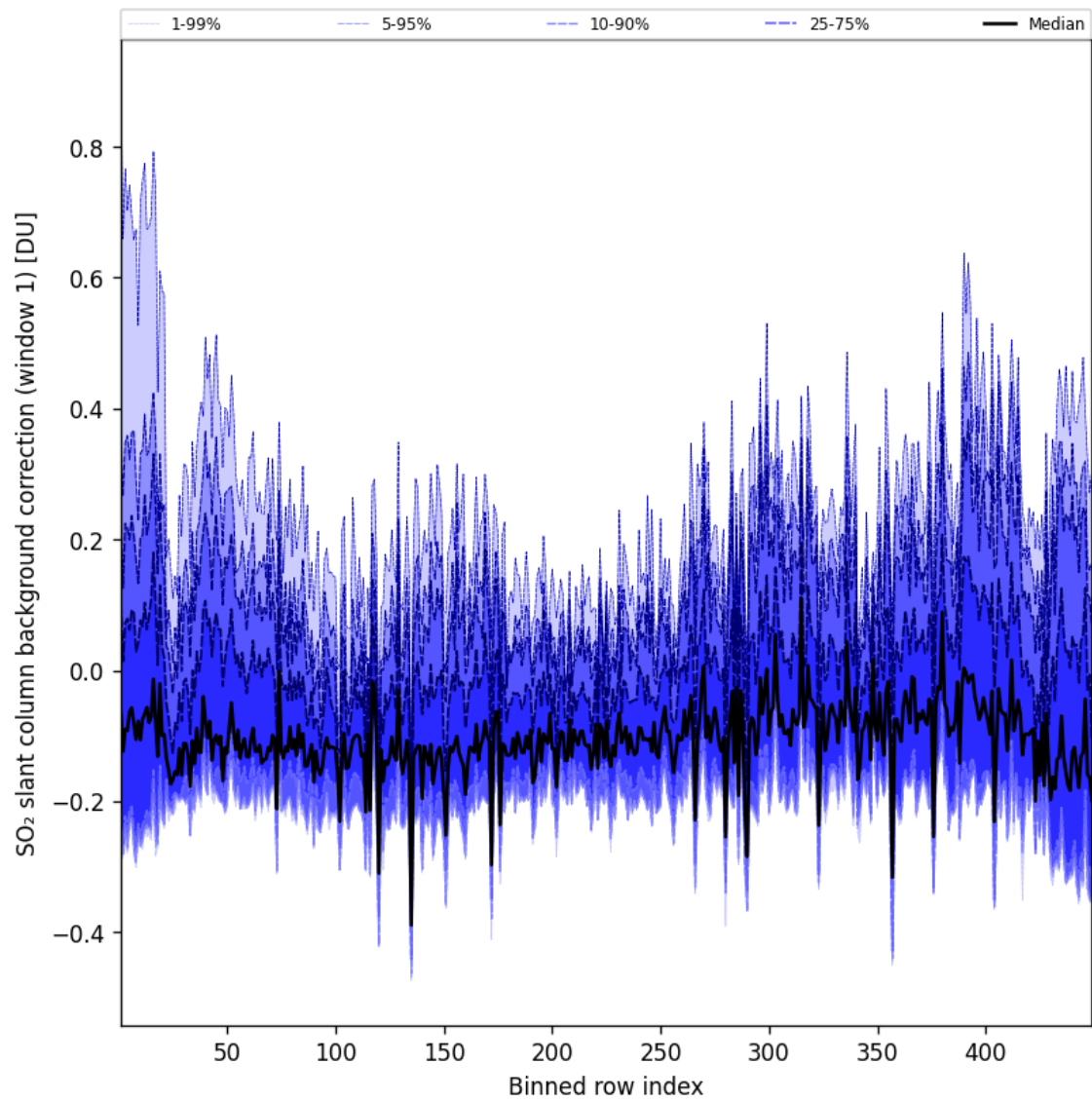
Figure 93: Along track statistics of “SO 2 slant column background correction (window 1)” for 2025-06-11 to 2025-06-12
