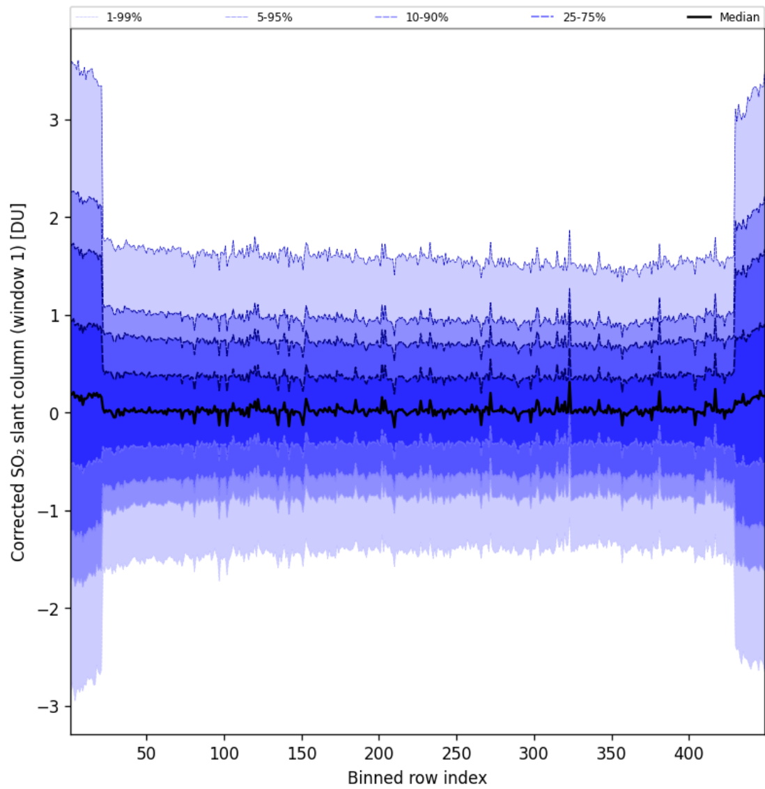
Figure 92: Along track statistics of “Corrected SO 2 slant column (window 1)” for 2025-06-11 to 2025-06-12
