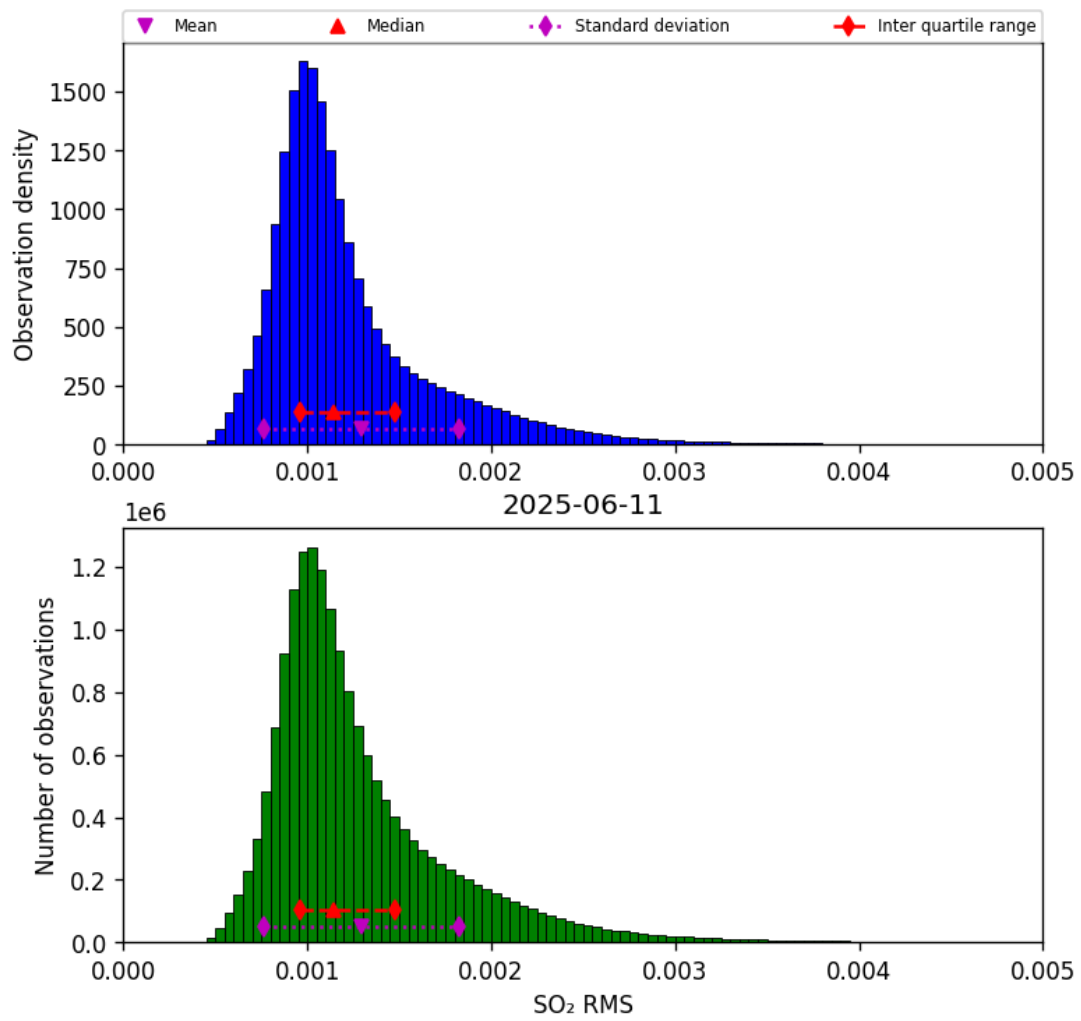
Figure 79: Histogram of “SO 2 RMS” for 2025-06-11 to 2025-06-12
