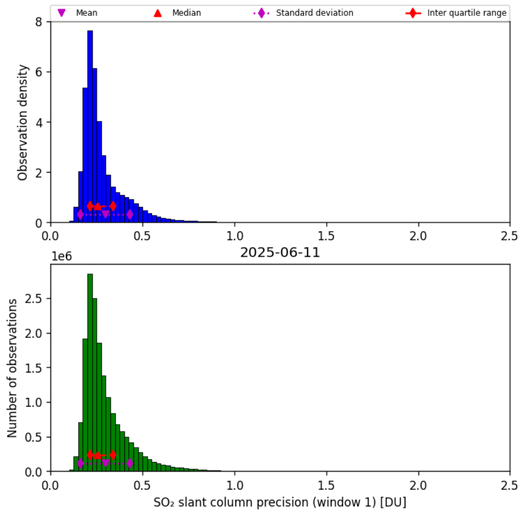
Figure 64: Histogram of “SO 2 slant column precision (window 1)” for 2025-06-11 to 2025-06-12
