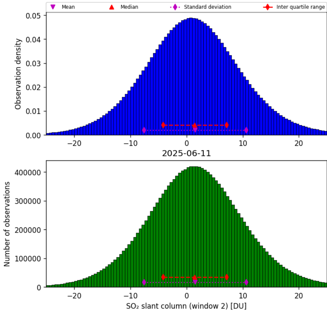
Figure 67: Histogram of “SO 2 slant column (window 2)” for 2025-06-11 to 2025-06-12
