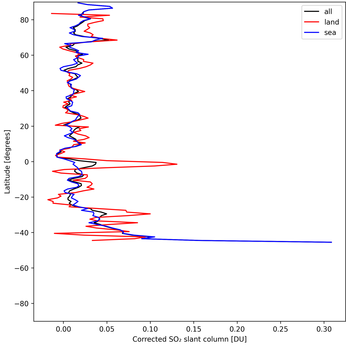
Figure 33: Zonal average of “Corrected SO 2 slant column” for 2025-06-11 to 2025-06-12.
