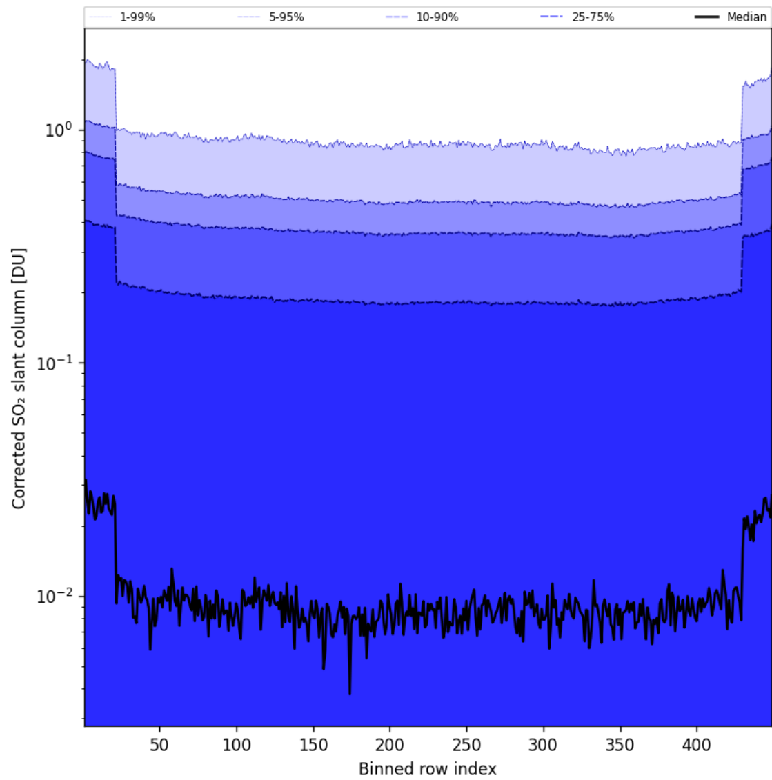
Figure 87: Along track statistics of “Corrected SO 2 slant column” for 2025-06-11 to 2025-06-12
