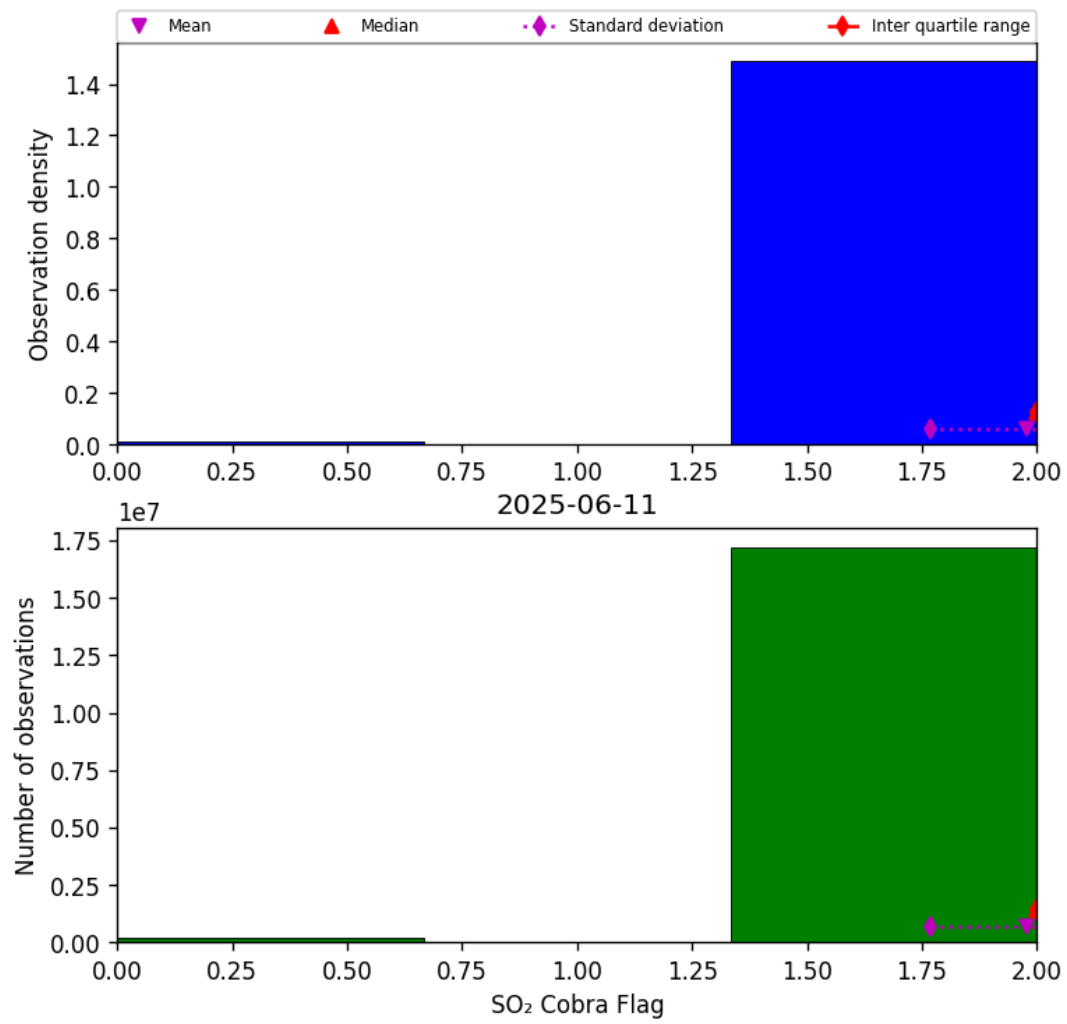
Figure 75: Histogram of “SO 2 Cobra Flag” for 2025-06-11 to 2025-06-12
