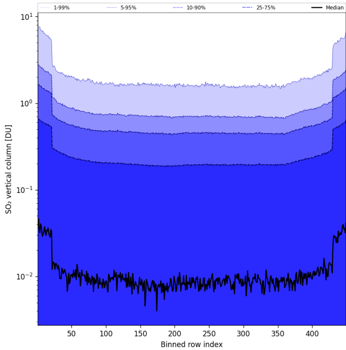
Figure 85: Along track statistics of “SO 2 vertical column” for 2025-06-11 to 2025-06-12
