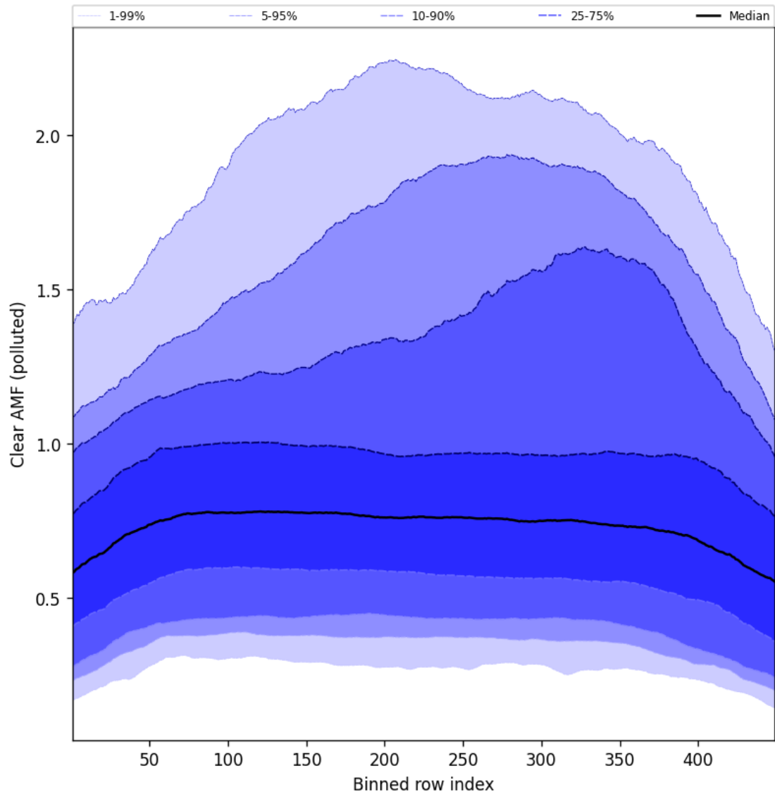
Figure 109: Along track statistics of “Clear AMF (polluted)” for 2025-06-11 to 2025-06-12
