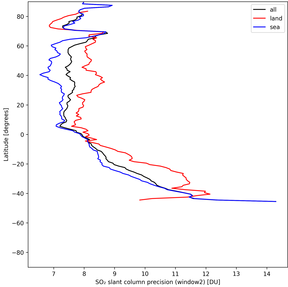
Figure 41: Zonal average of “SO 2 slant column precision (window2)” for 2025-06-11 to 2025-06-12.
