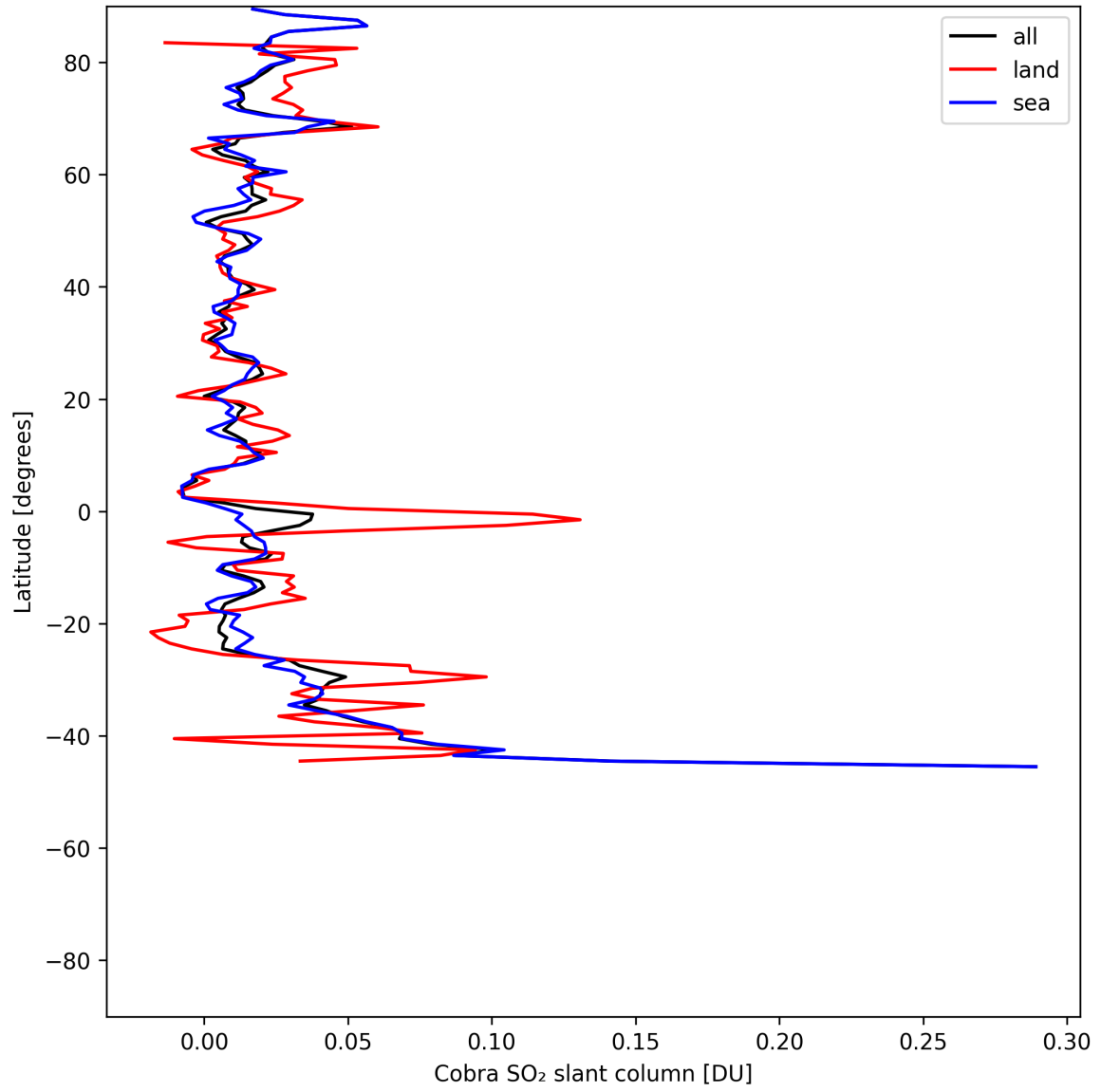
Figure 34: Zonal average of “Cobra SO 2 slant column” for 2025-06-11 to 2025-06-12.
