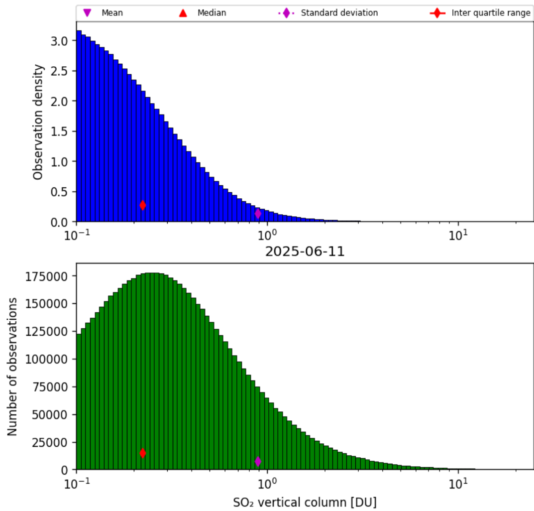
Figure 58: Histogram of “SO 2 vertical column” for 2025-06-11 to 2025-06-12
