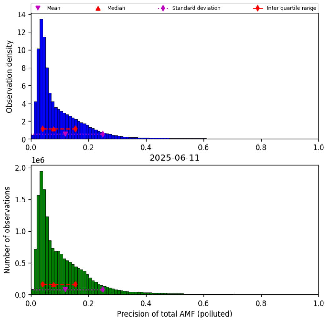
Figure 81: Histogram of “Precision of total AMF (polluted)” for 2025-06-11 to 2025-06-12
