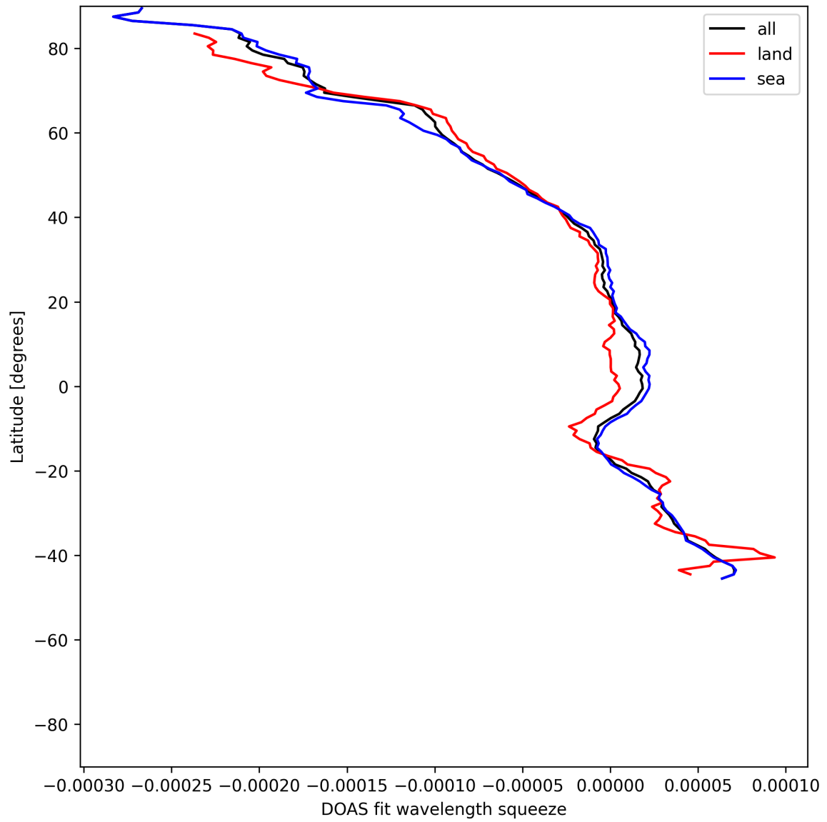
Figure 51: Zonal average of “DOAS fit wavelength squeeze” for 2025-06-11 to 2025-06-12.
