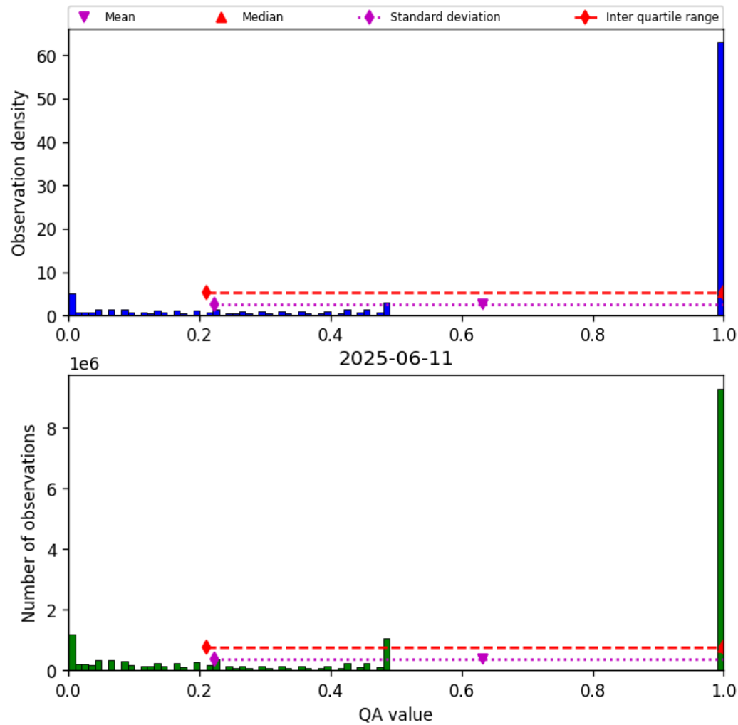
Figure 57: Histogram of “QA value” for 2025-06-11 to 2025-06-12
