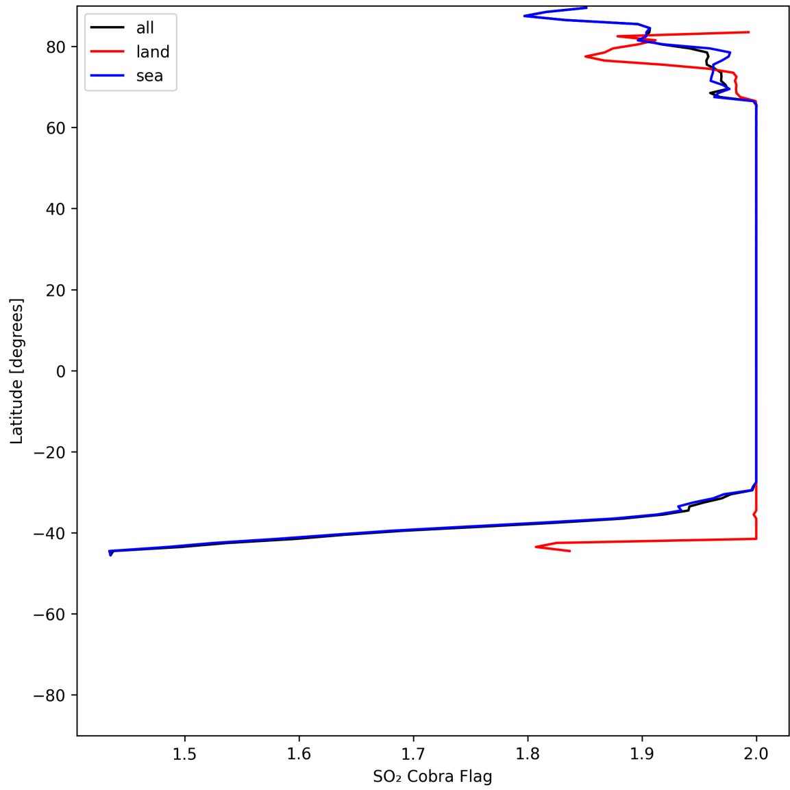
Figure 48: Zonal average of "SO 2 Cobra Flag" for 2025-06-11 to 2025-06-12.
