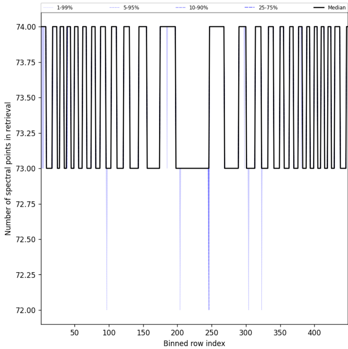
Figure 110: Along track statistics of “Number of spectral points in retrieval” for 2025-06-11 to 2025-06-12
