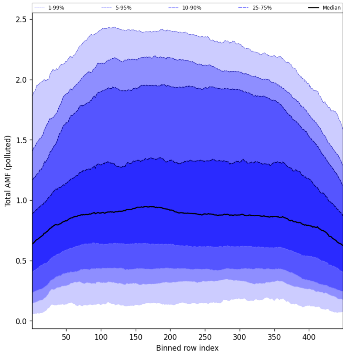
Figure 107: Along track statistics of “Total AMF (polluted)” for 2025-06-11 to 2025-06-12
