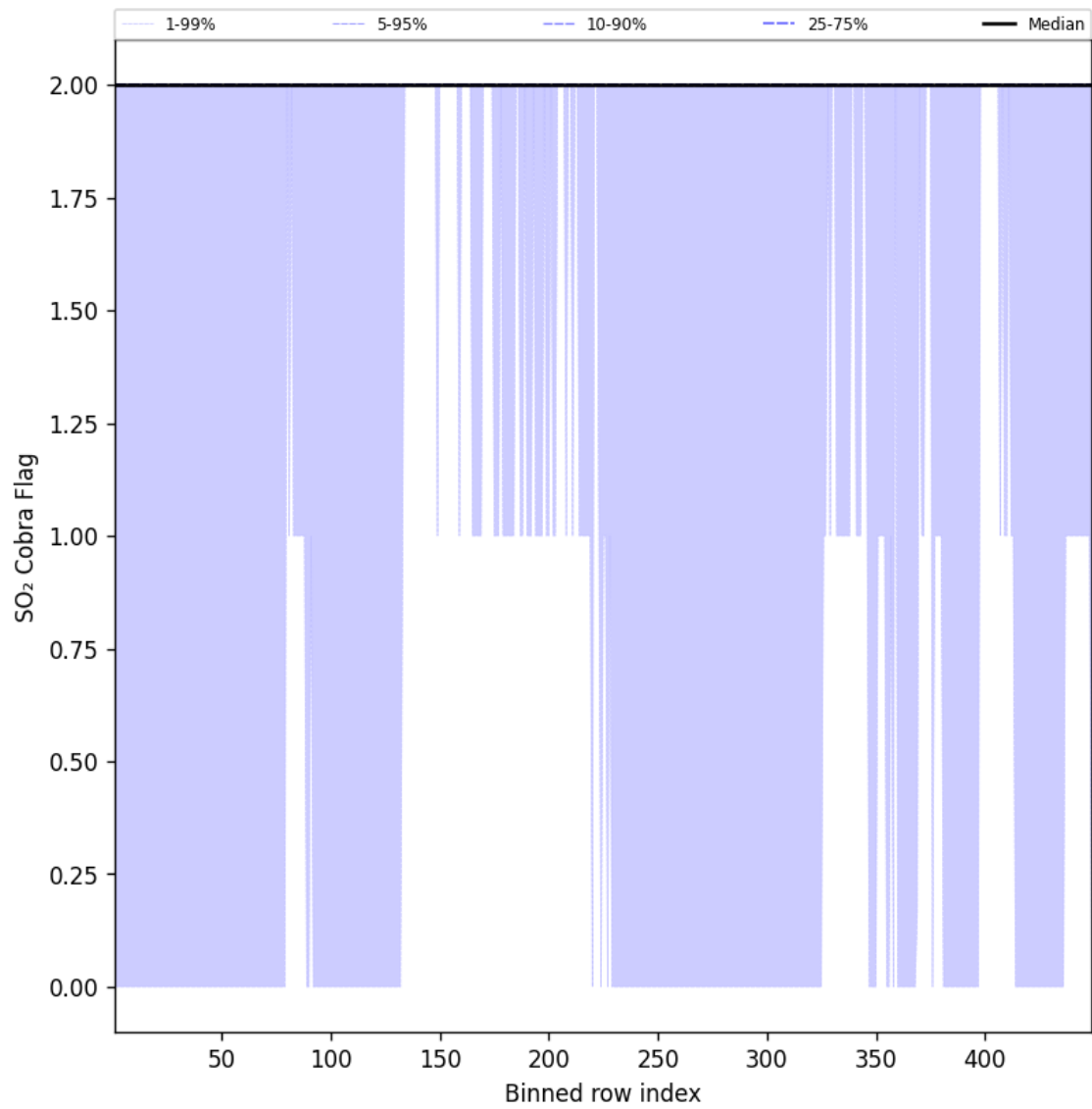
Figure 102: Along track statistics of “SO 2 Cobra Flag” for 2025-06-11 to 2025-06-12
