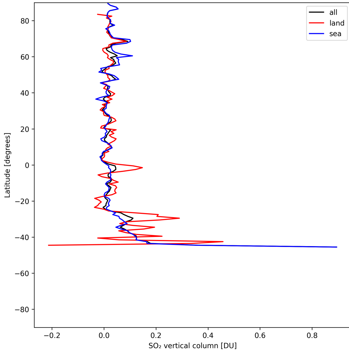
Figure 31: Zonal average of “SO 2 vertical column” for 2025-06-11 to 2025-06-12.
