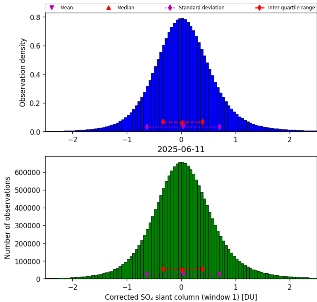
Figure 65: Histogram of “Corrected SO 2 slant column (window 1)” for 2025-06-11 to 2025-06-12
