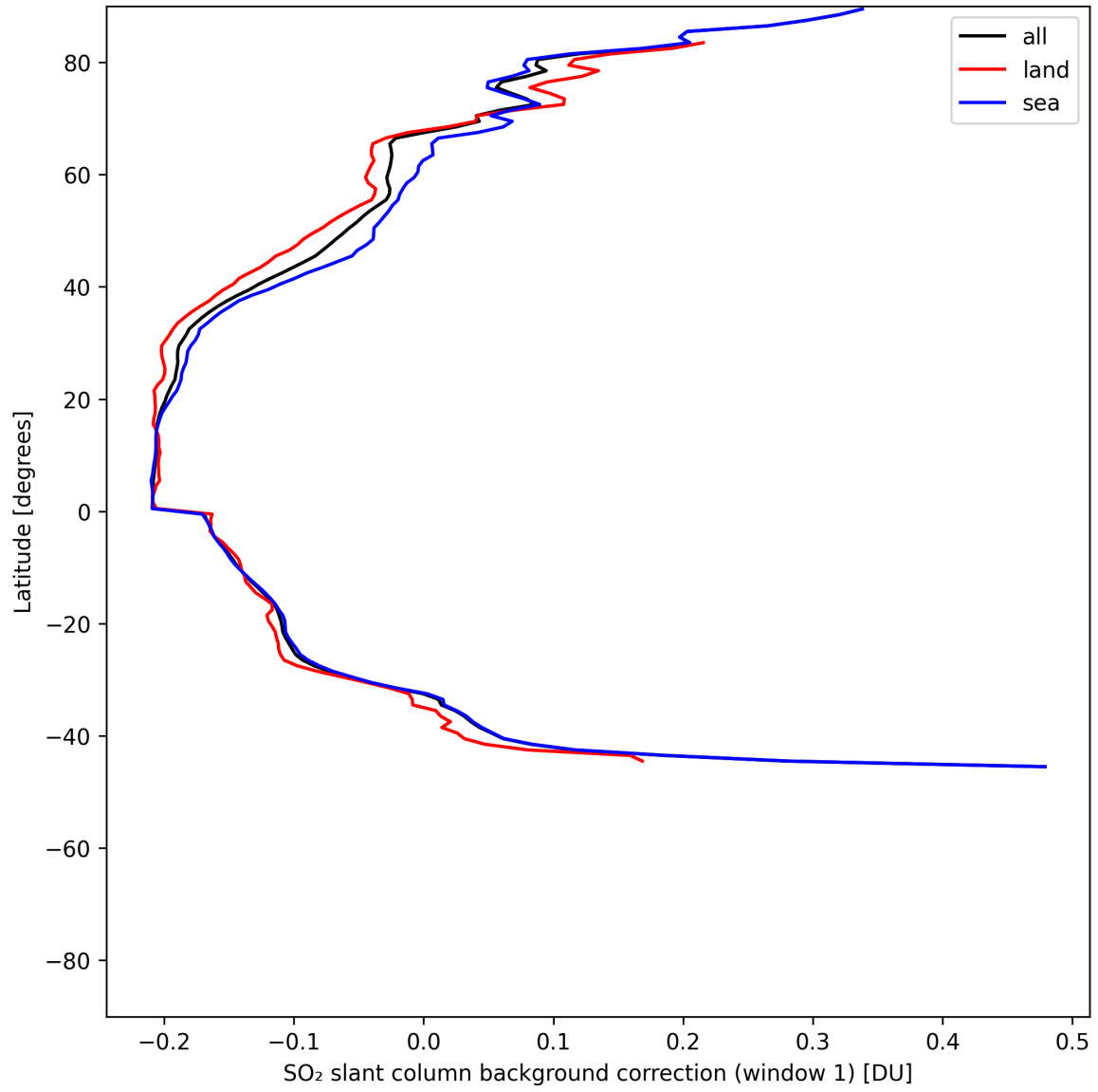
Figure 39: Zonal average of “SO 2 slant column background correction (window 1)” for 2025-06-11 to 2025-06-12.
