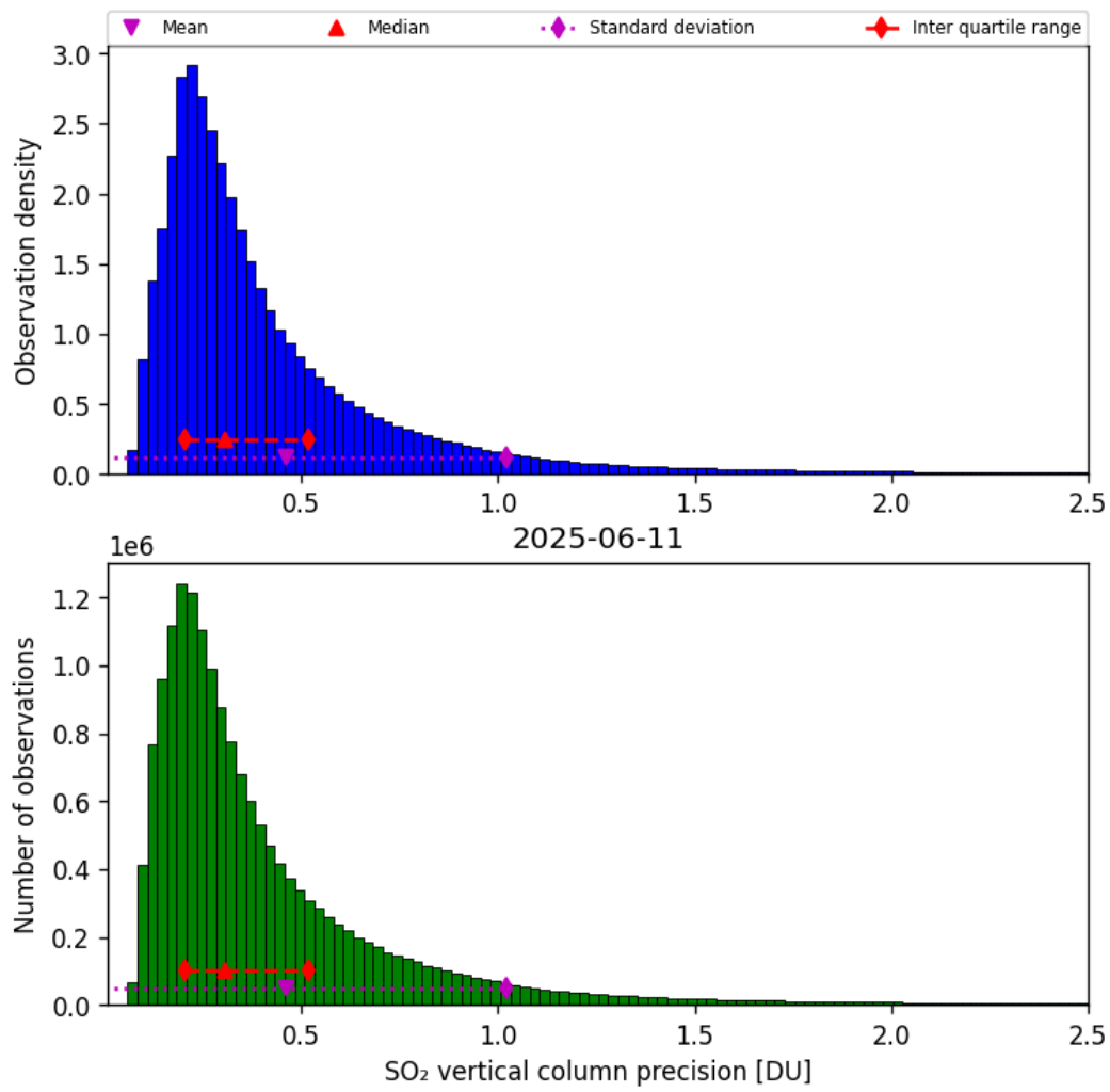
Figure 59: Histogram of “SO 2 vertical column precision” for 2025-06-11 to 2025-06-12
