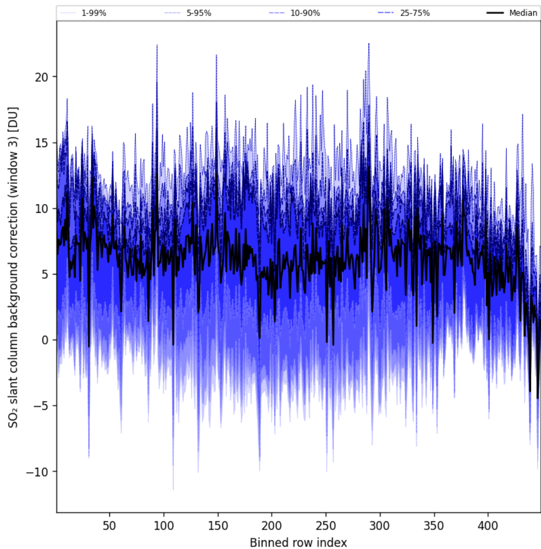
Figure 101: Along track statistics of “SO 2 slant column background correction (window 3)” for 2025-06-11 to 2025-06-12
