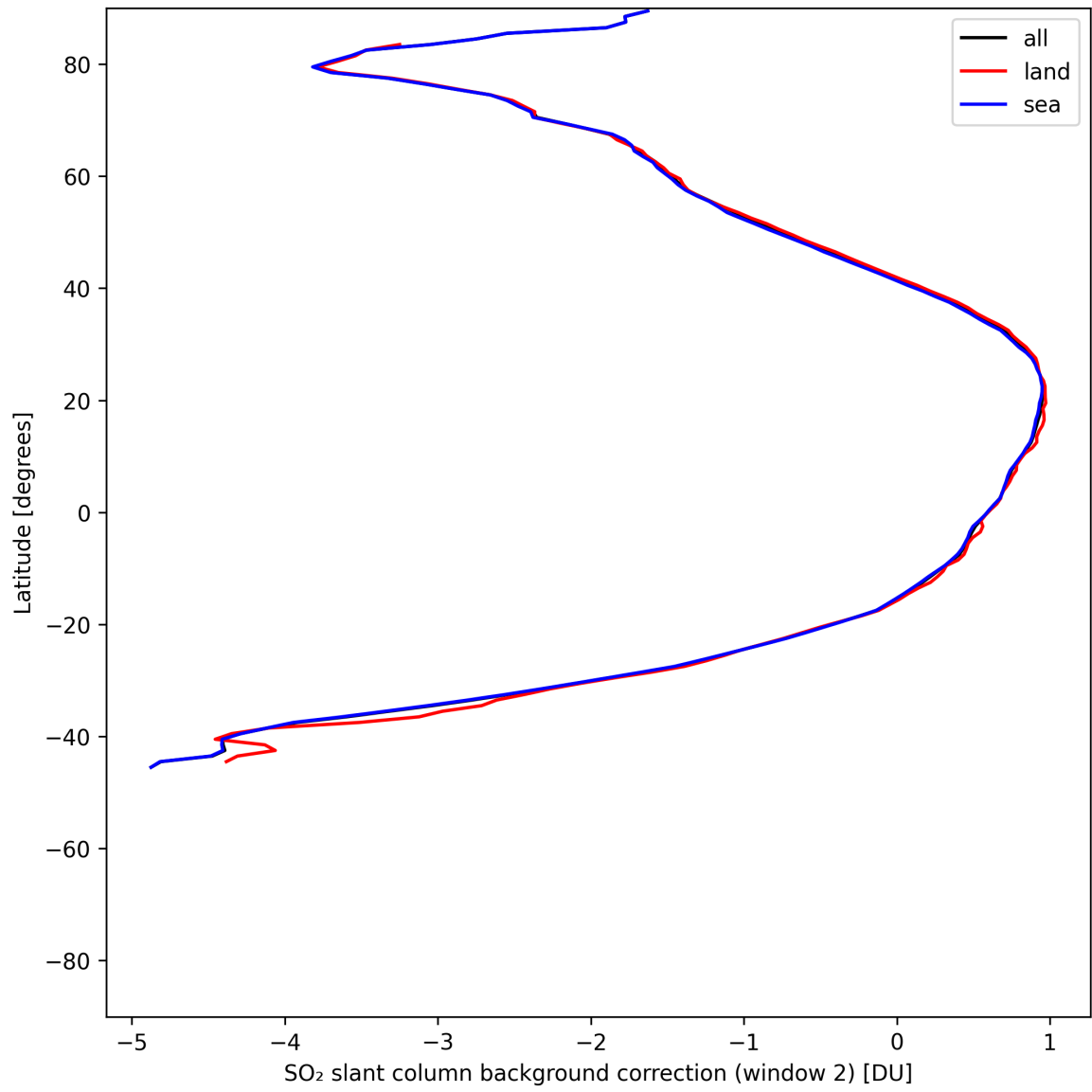
Figure 43: Zonal average of “SO 2 slant column background correction (window 2)” for 2025-06-11 to 2025-06-12.
