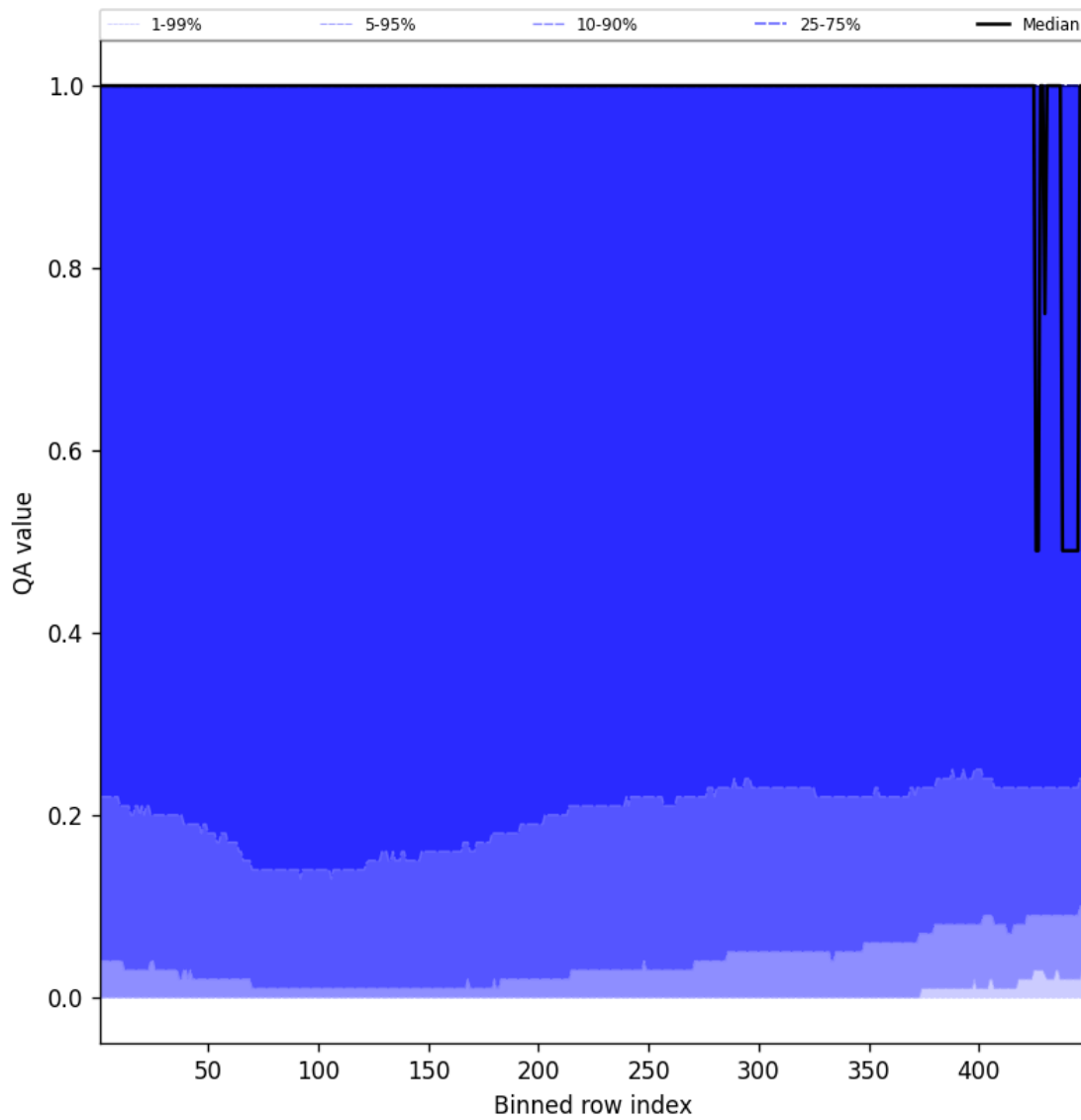
Figure 84: Along track statistics of “QA value” for 2025-06-11 to 2025-06-12
