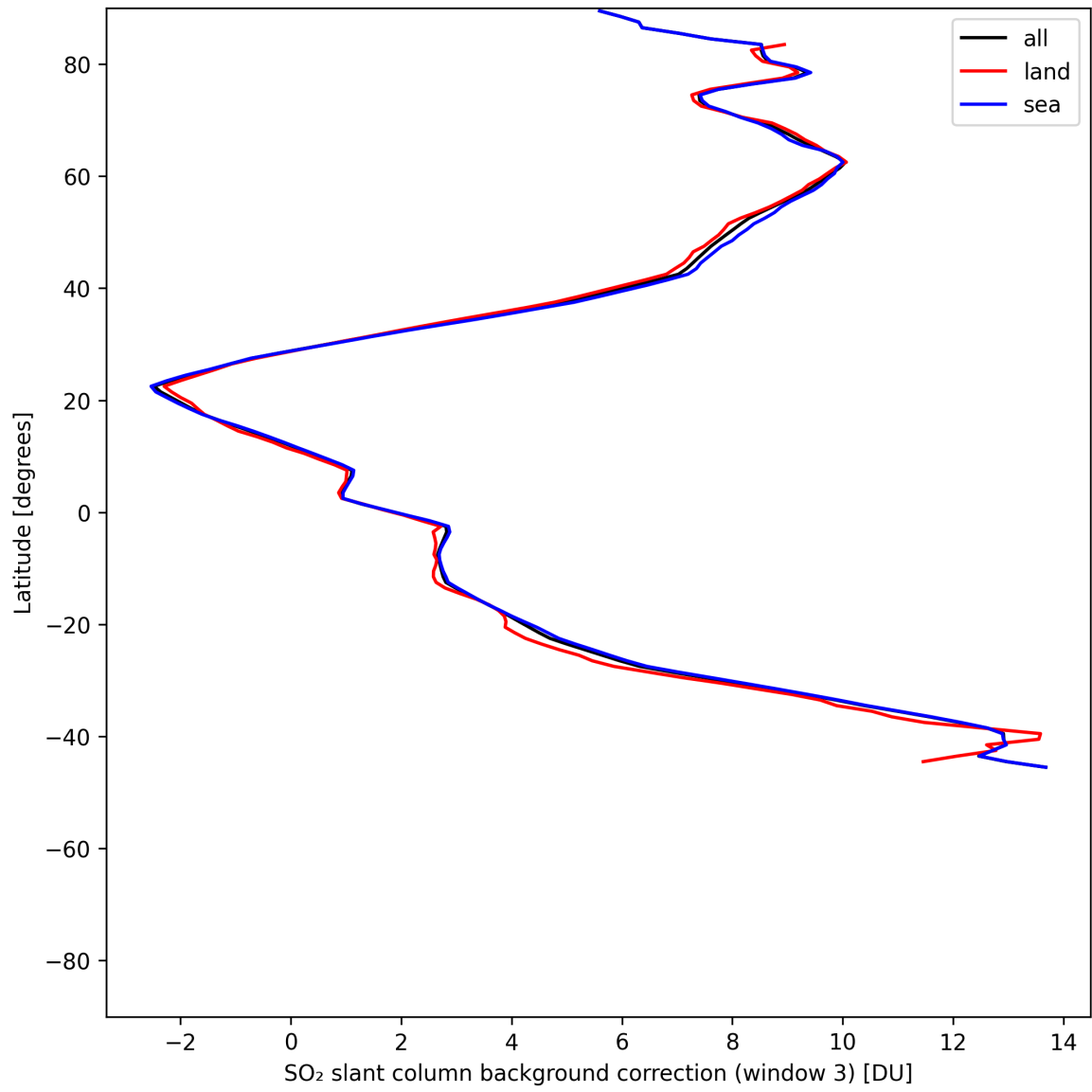
Figure 47: Zonal average of “SO 2 slant column background correction (window 3)” for 2025-06-11 to 2025-06-12.
