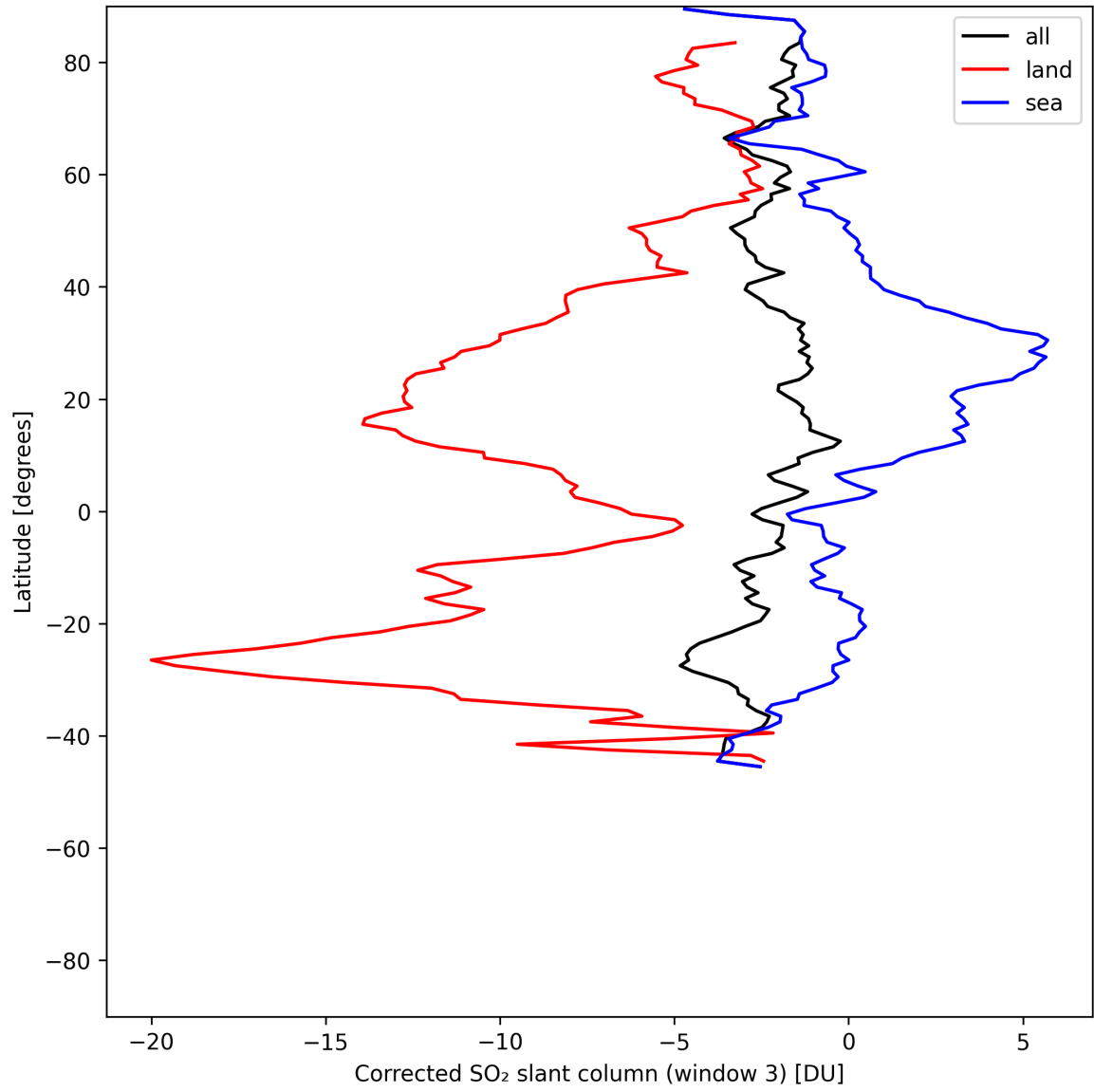
Figure 46: Zonal average of “Corrected SO 2 slant column (window 3)” for 2025-06-11 to 2025-06-12.
