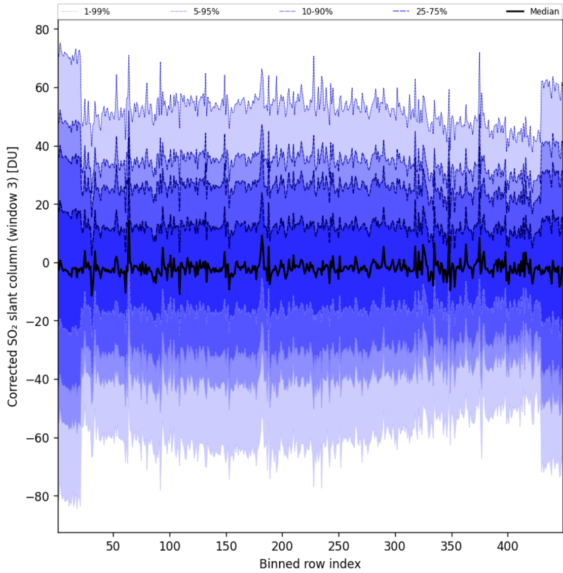
Figure 100: Along track statistics of “Corrected SO 2 slant column (window 3)” for 2025-06-11 to 2025-06-12
