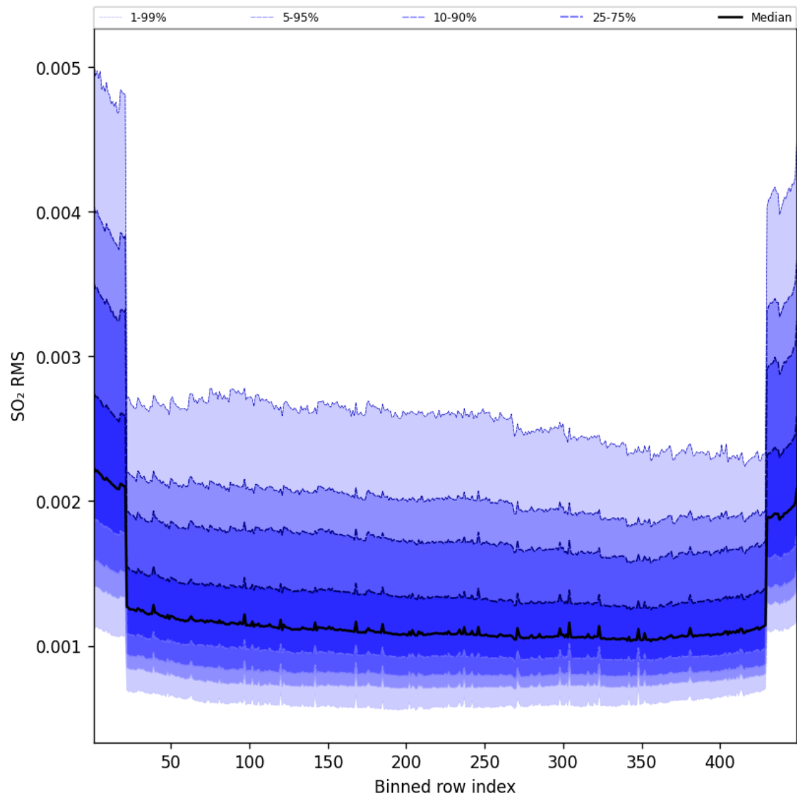
Figure 106: Along track statistics of “SO 2 RMS” for 2025-06-11 to 2025-06-12
