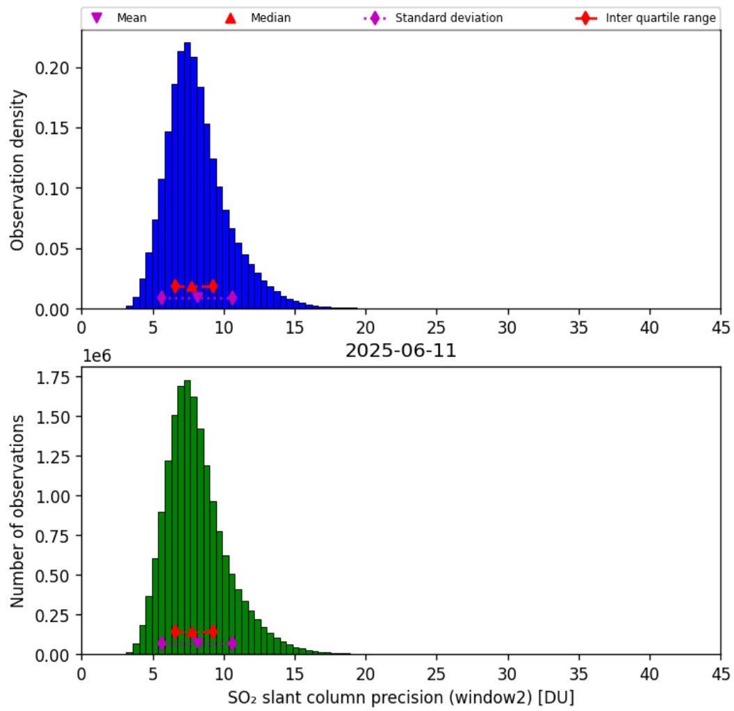
Figure 68: Histogram of “SO 2 slant column precision (window2)” for 2025-06-11 to 2025-06-12
