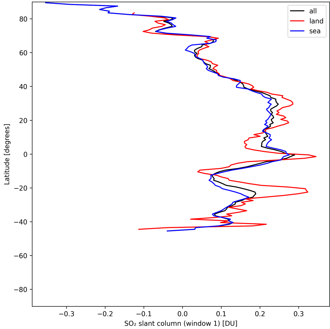
Figure 36: Zonal average of “SO 2 slant column (window 1)” for 2025-06-11 to 2025-06-12.
