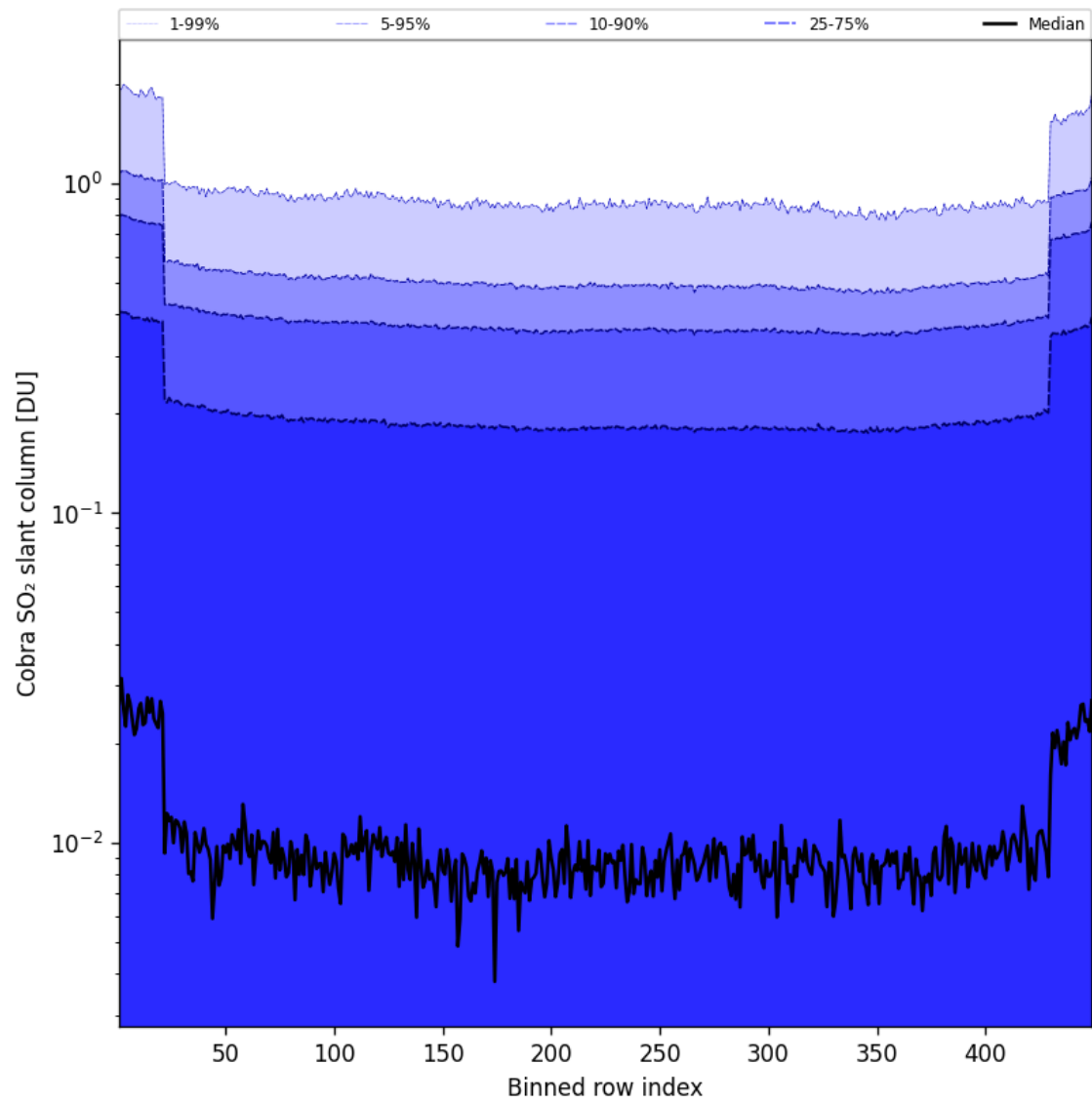
Figure 88: Along track statistics of “Cobra SO 2 slant column” for 2025-06-11 to 2025-06-12
