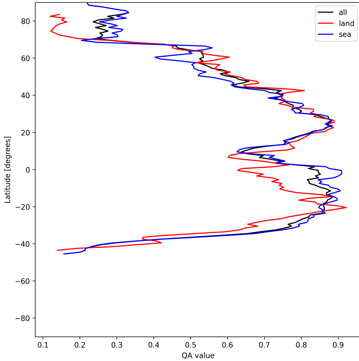
Figure 30: Zonal average of “QA value” for 2025-06-13 to 2025-06-14.
