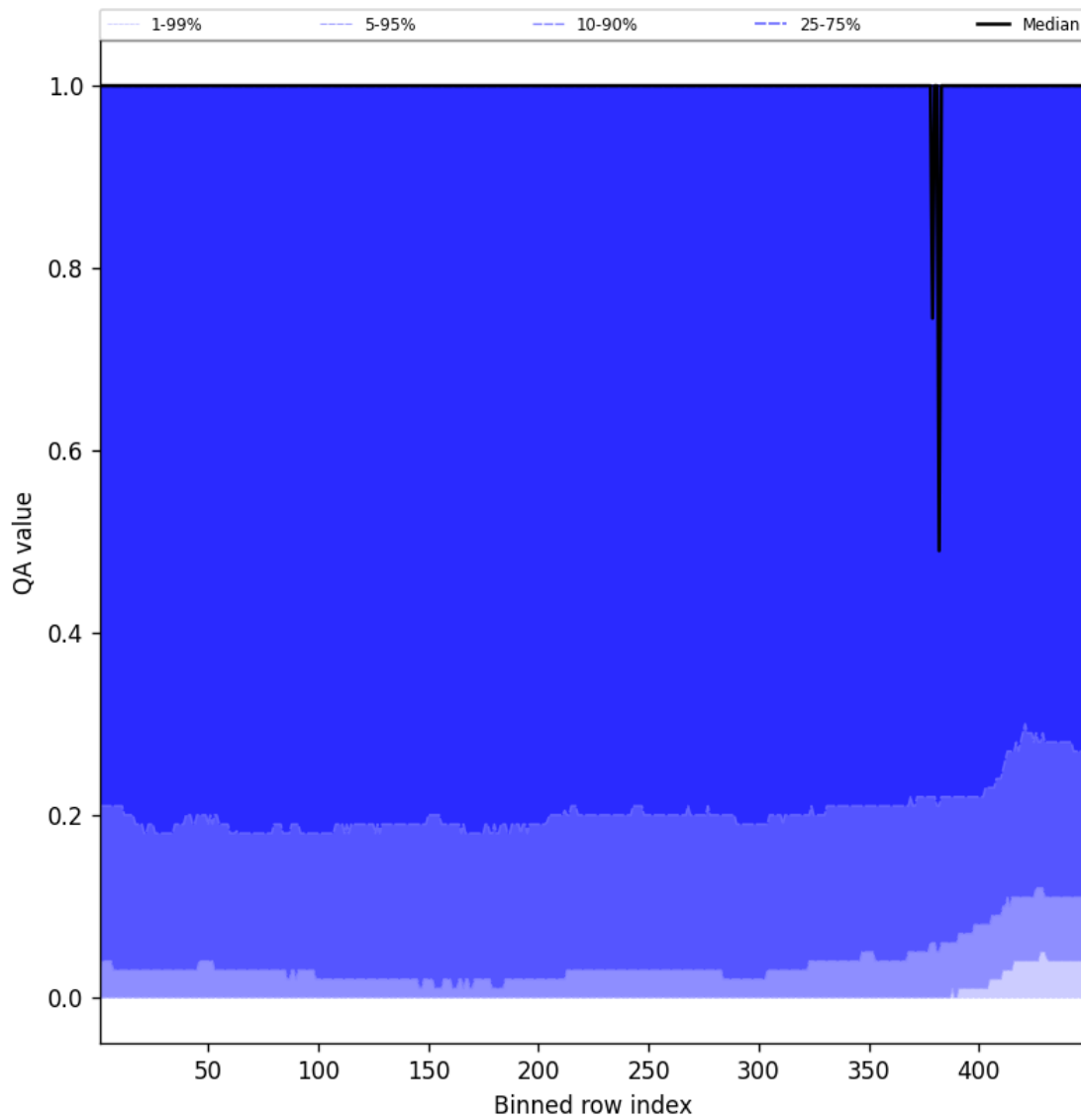
Figure 84: Along track statistics of “QA value” for 2025-06-13 to 2025-06-14
