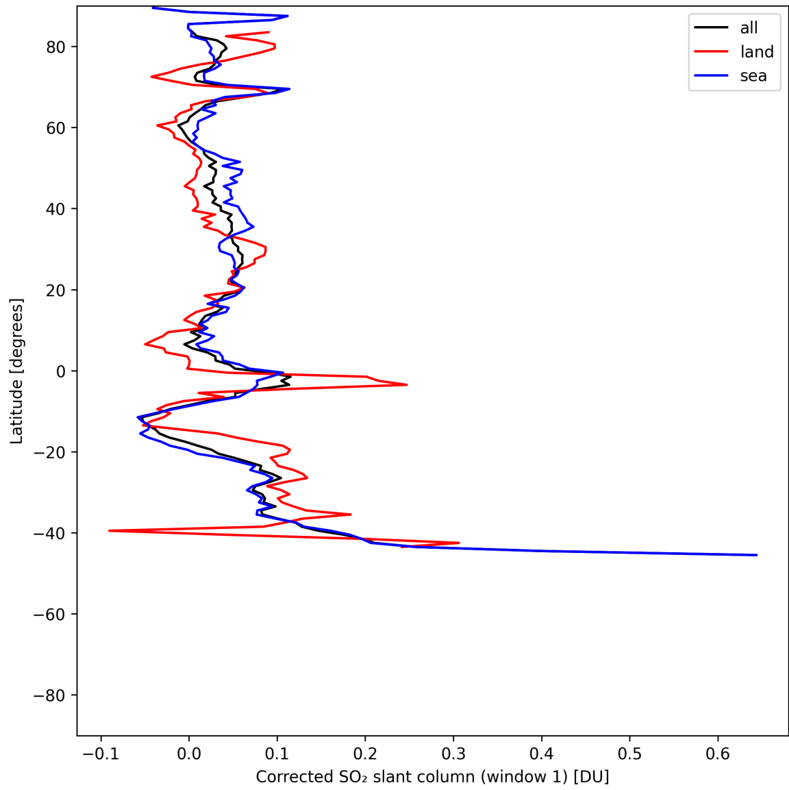
Figure 38: Zonal average of “Corrected SO 2 slant column (window 1)” for 2025-06-13 to 2025-06-14.
