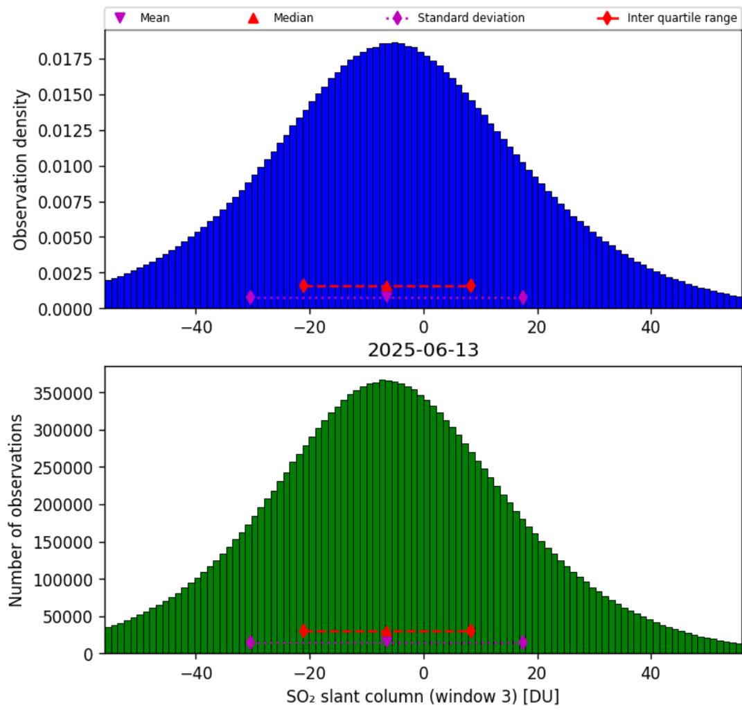
Figure 71: Histogram of “SO 2 slant column (window 3)” for 2025-06-13 to 2025-06-14
