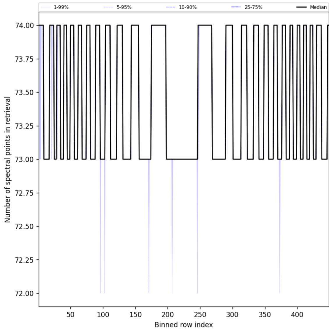
Figure 110: Along track statistics of “Number of spectral points in retrieval” for 2025-06-13 to 2025-06-14
