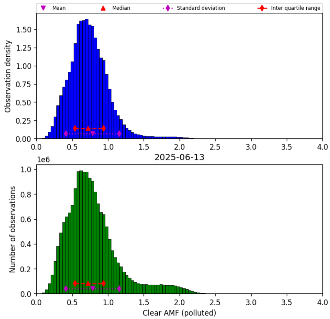
Figure 82: Histogram of “Clear AMF (polluted)” for 2025-06-13 to 2025-06-14
