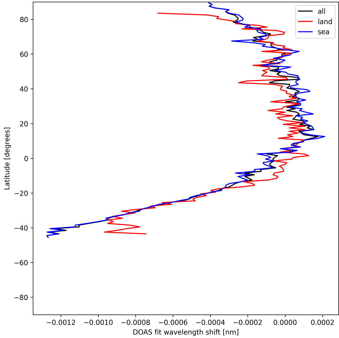
Figure 50: Zonal average of "DOAS fit wavelength shift" for 2025-06-13 to 2025-06-14.
