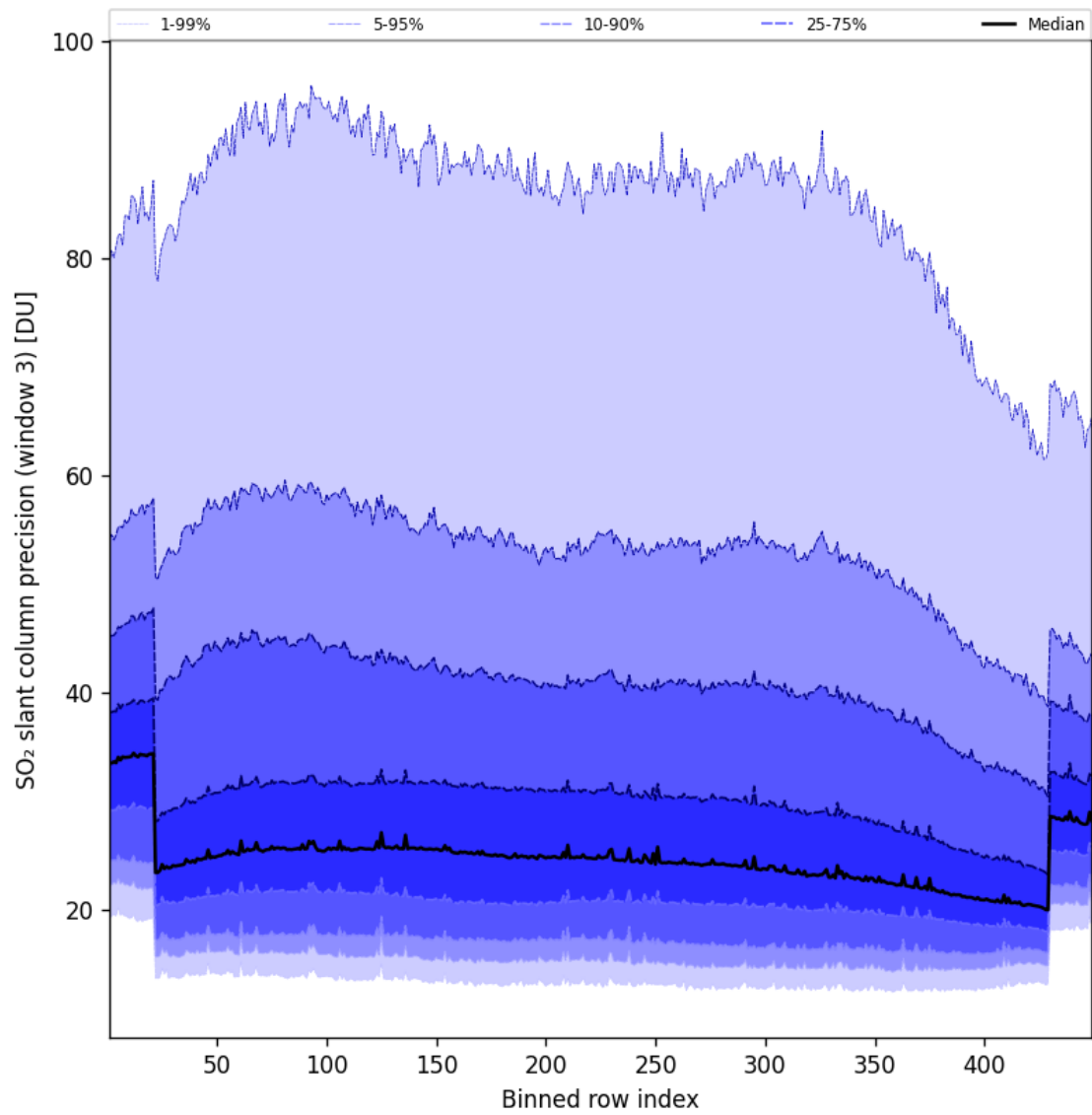
Figure 99: Along track statistics of “SO 2 slant column precision (window 3)” for 2025-06-13 to 2025-06-14
