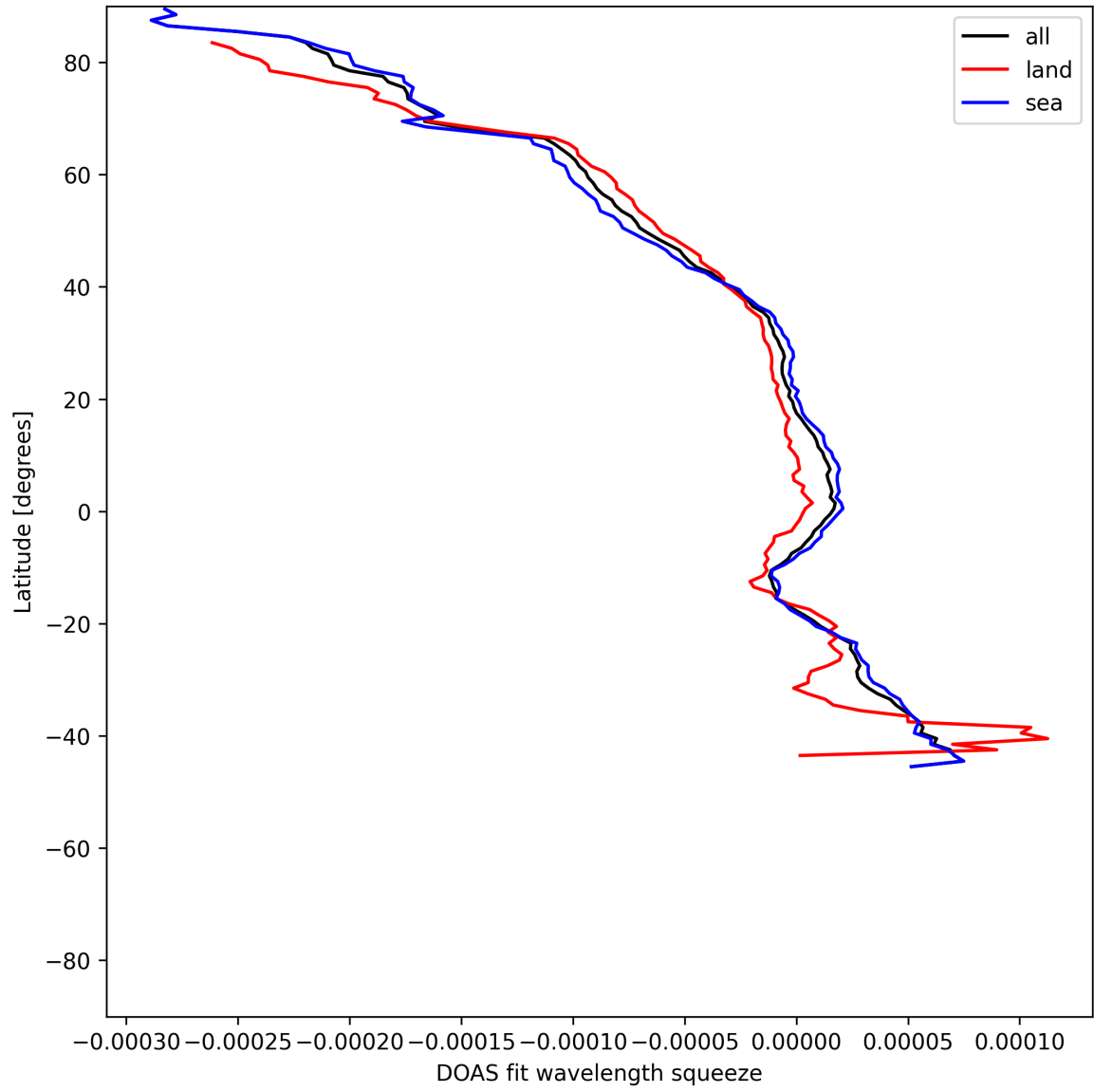
Figure 51: Zonal average of “DOAS fit wavelength squeeze” for 2025-06-13 to 2025-06-14.
