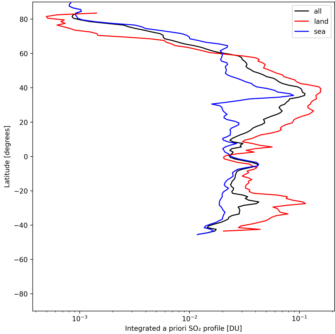
Figure 49: Zonal average of “Integrated a priori SO 2 profile” for 2025-06-13 to 2025-06-14.
