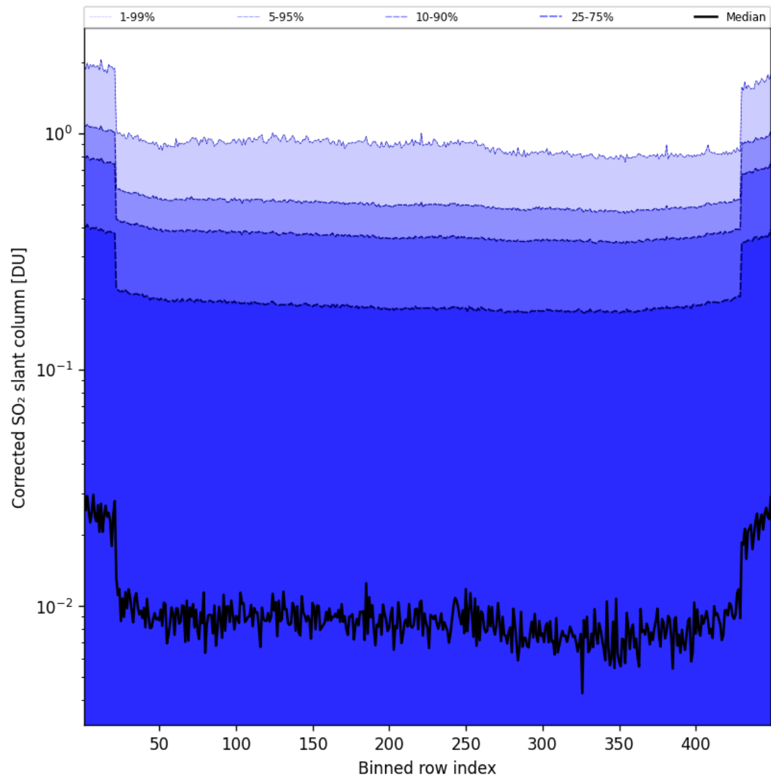
Figure 87: Along track statistics of “Corrected SO 2 slant column” for 2025-06-13 to 2025-06-14
