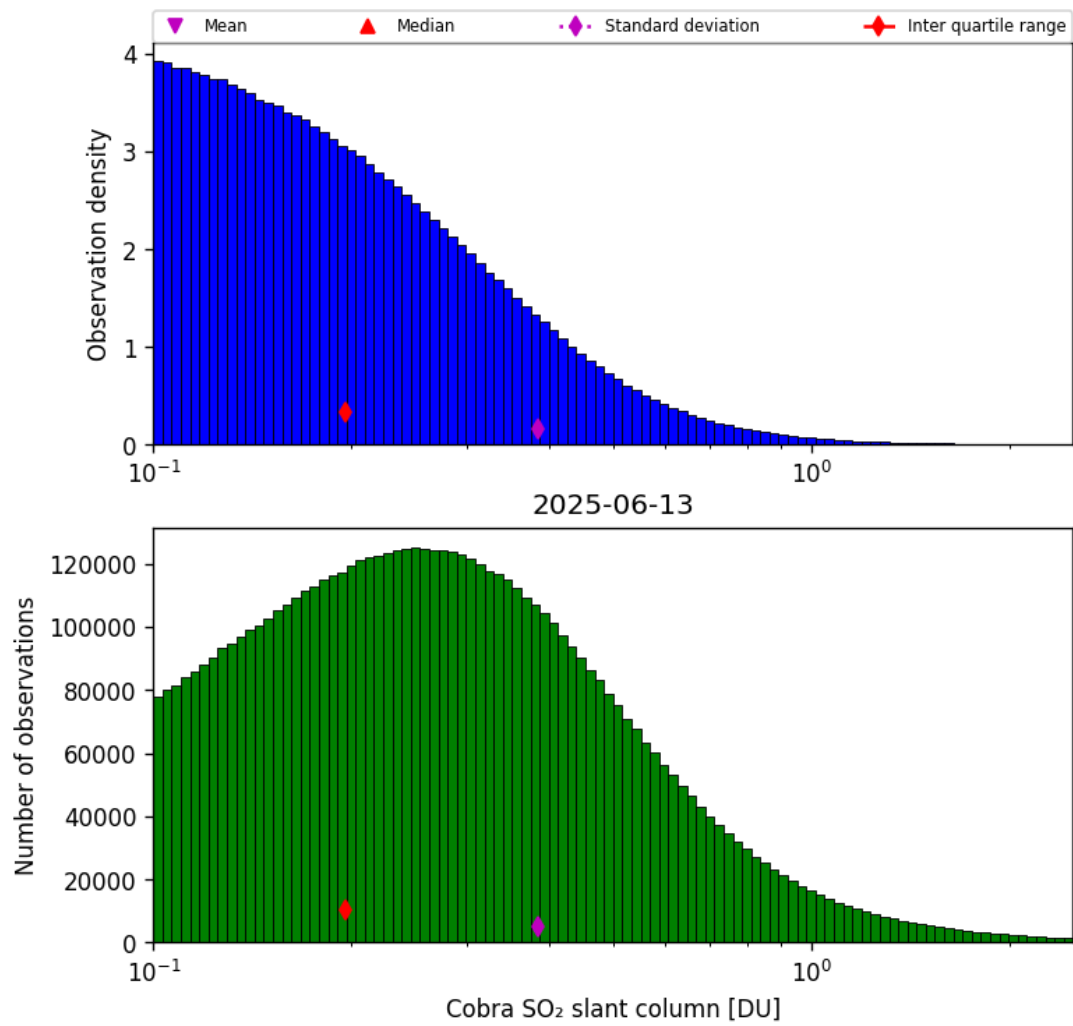
Figure 61: Histogram of “Cobra SO 2 slant column” for 2025-06-13 to 2025-06-14
