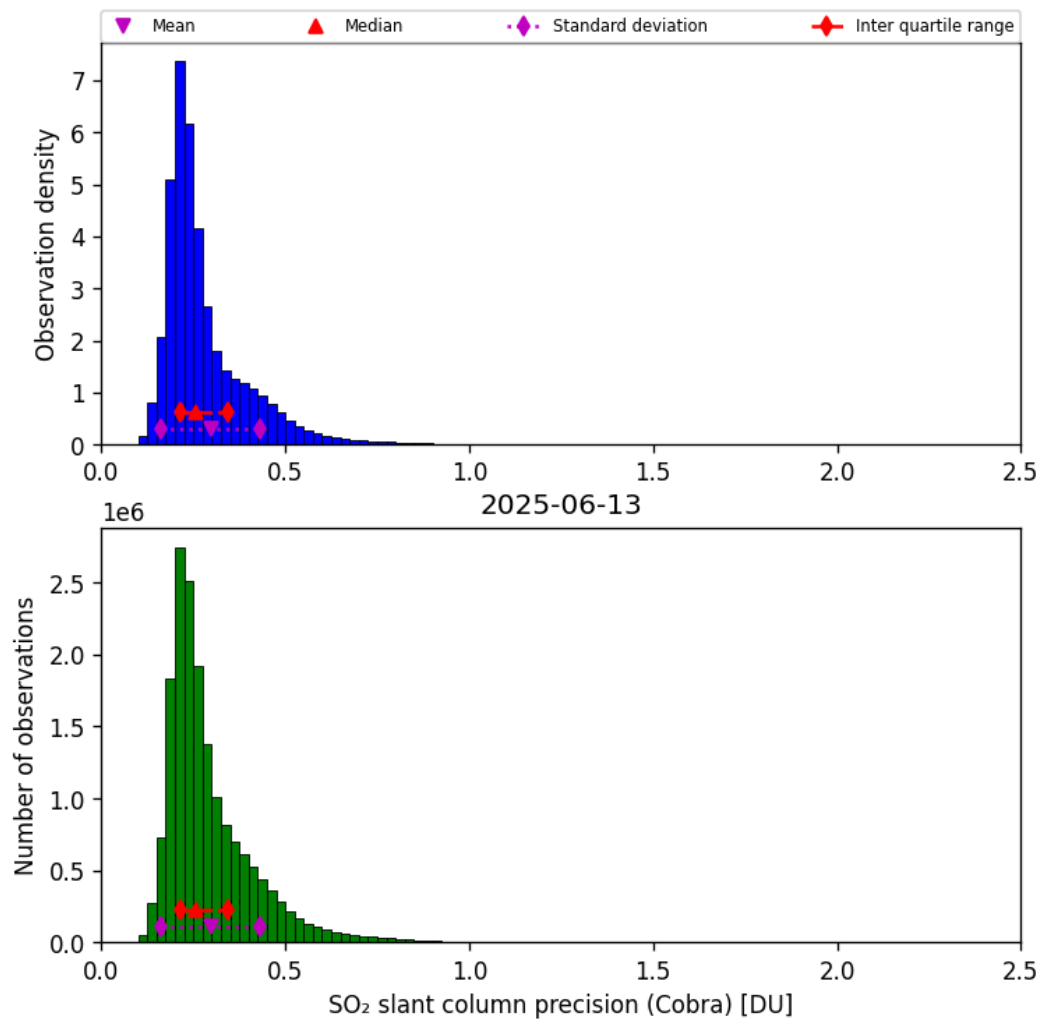
Figure 62: Histogram of “SO 2 slant column precision (Cobra)” for 2025-06-13 to 2025-06-14
