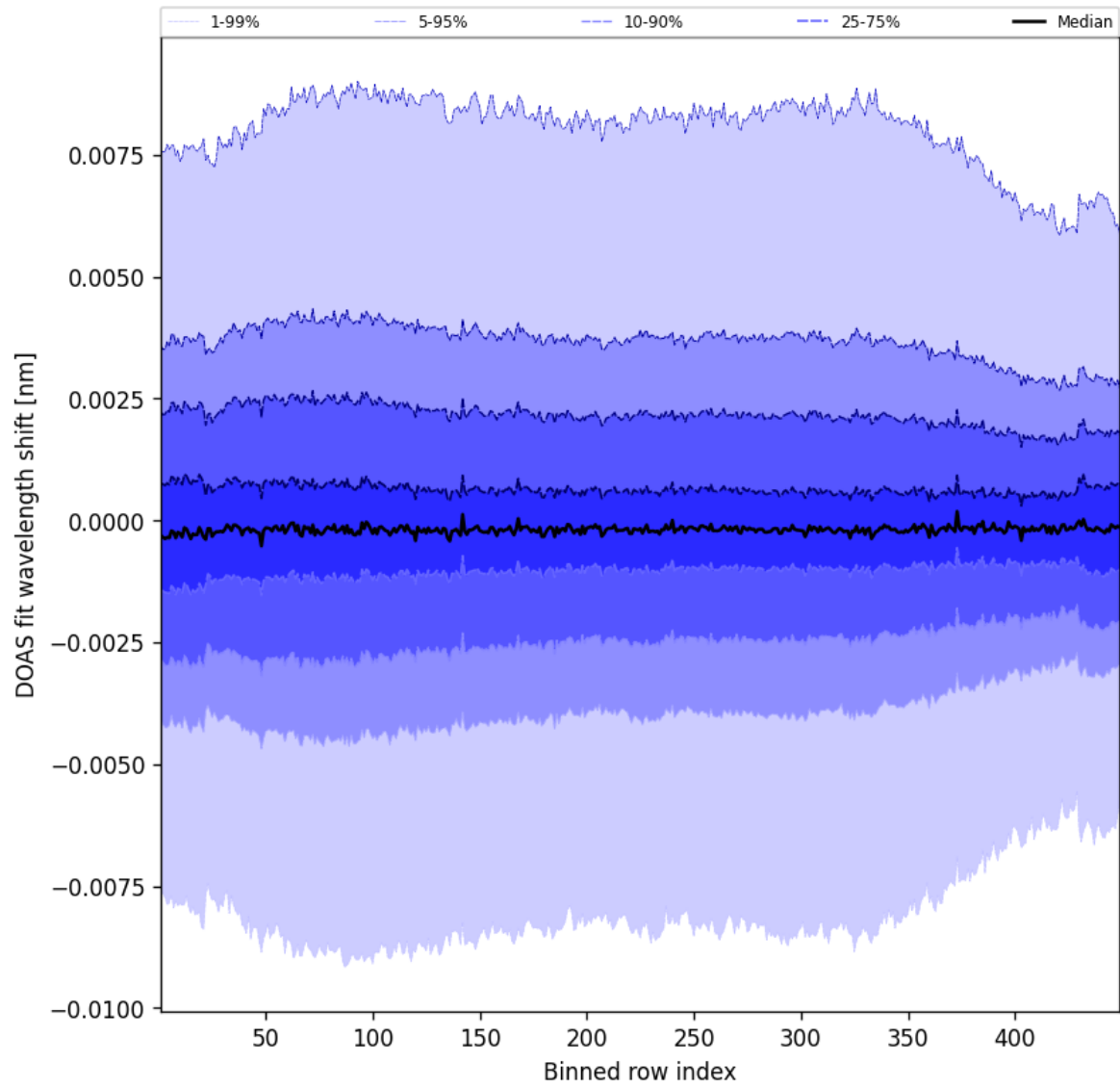
Figure 104: Along track statistics of “DOAS fit wavelength shift” for 2025-06-13 to 2025-06-14
