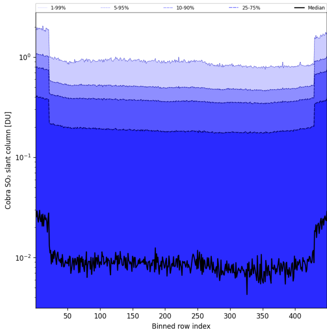
Figure 88: Along track statistics of “Cobra SO 2 slant column” for 2025-06-13 to 2025-06-14
