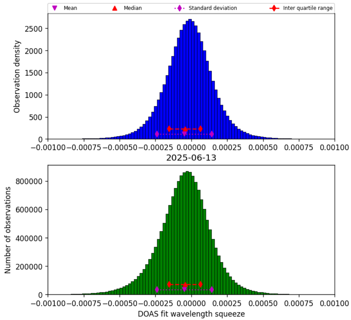
Figure 78: Histogram of “DOAS fit wavelength squeeze” for 2025-06-13 to 2025-06-14
