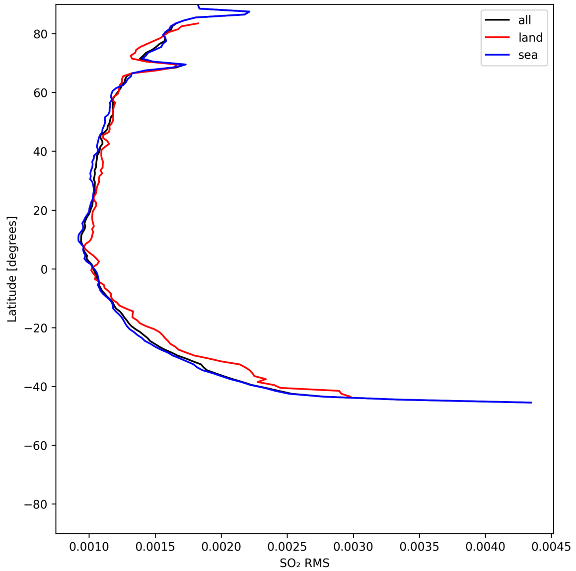
Figure 52: Zonal average of “SO 2 RMS” for 2025-06-13 to 2025-06-14.
