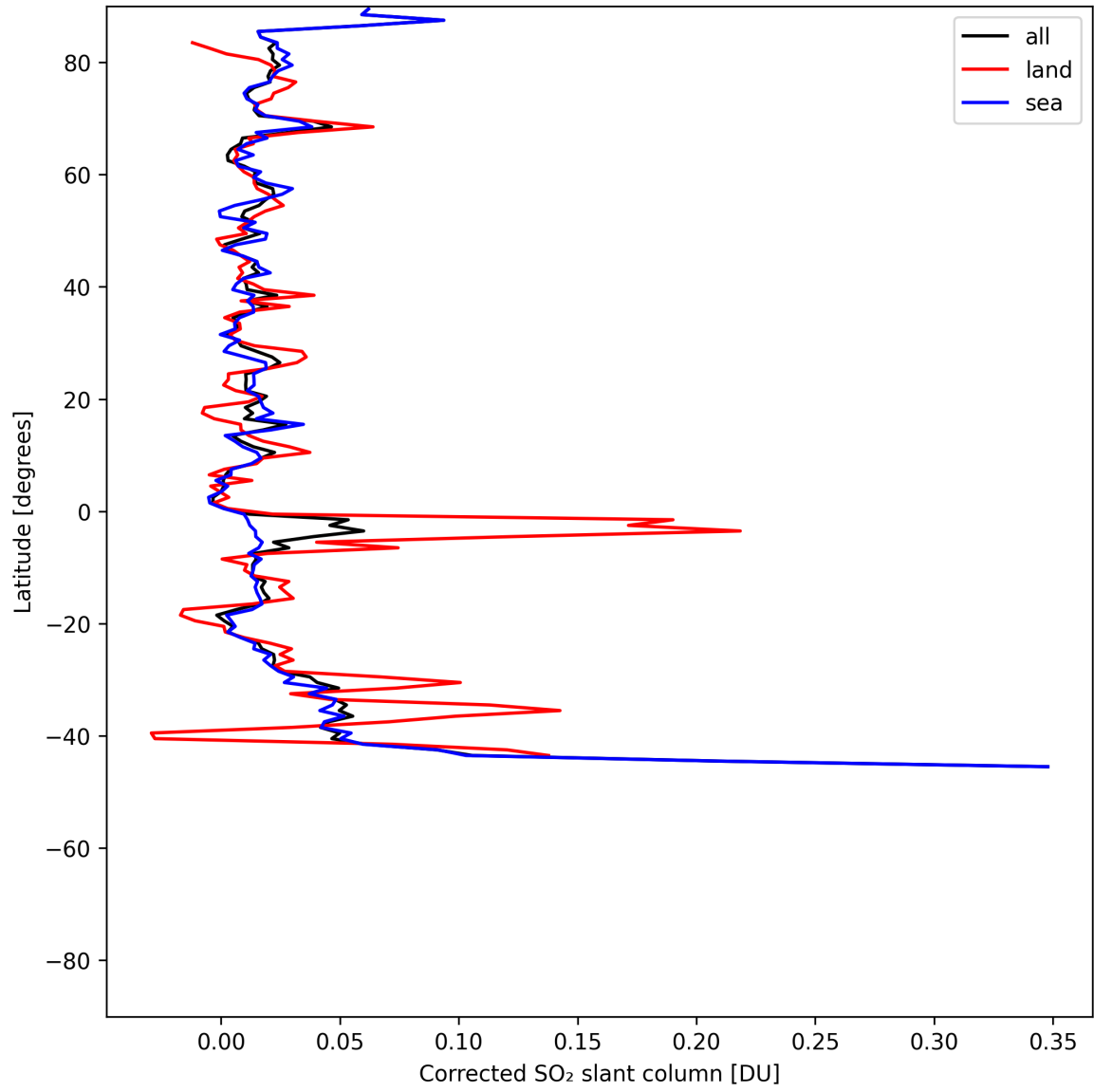
Figure 33: Zonal average of “Corrected SO 2 slant column” for 2025-06-13 to 2025-06-14.
