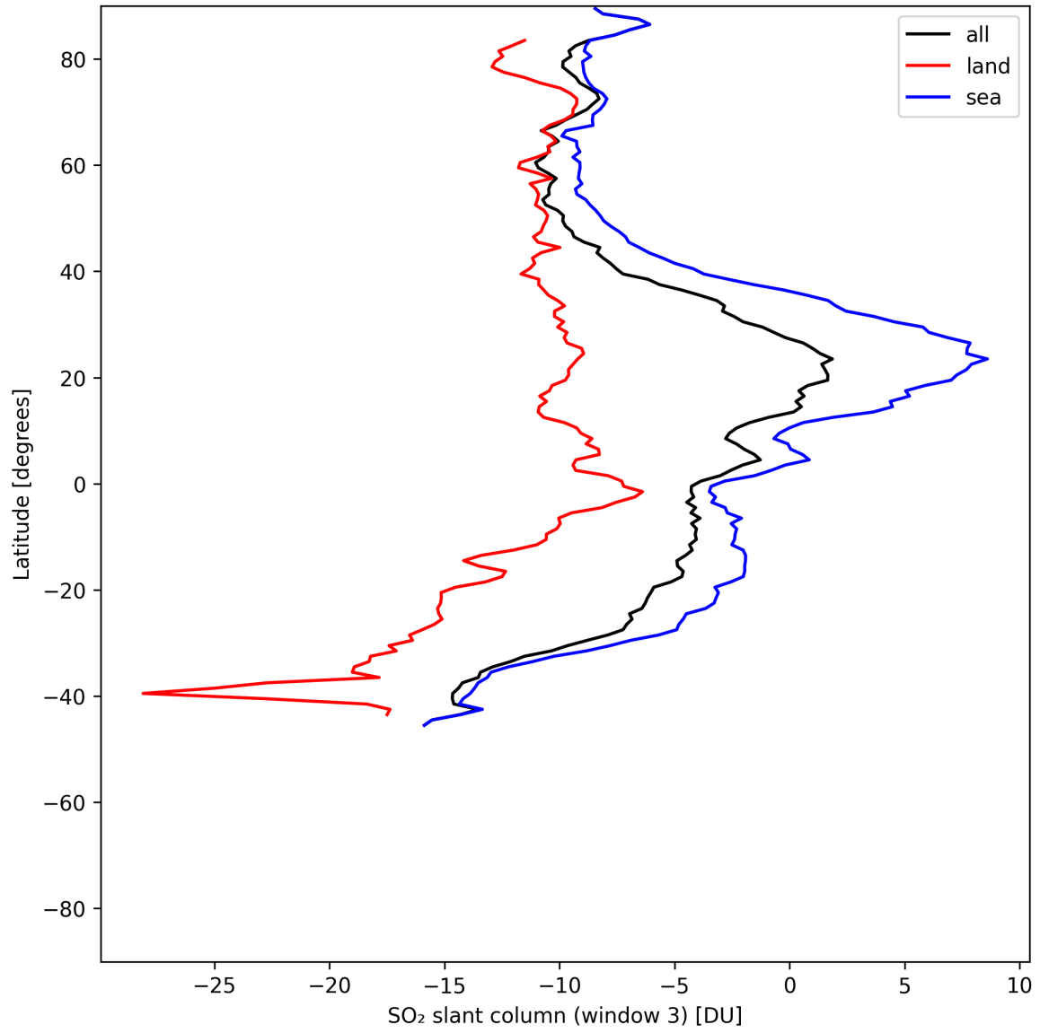
Figure 44: Zonal average of “SO 2 slant column (window 3)” for 2025-06-13 to 2025-06-14.
