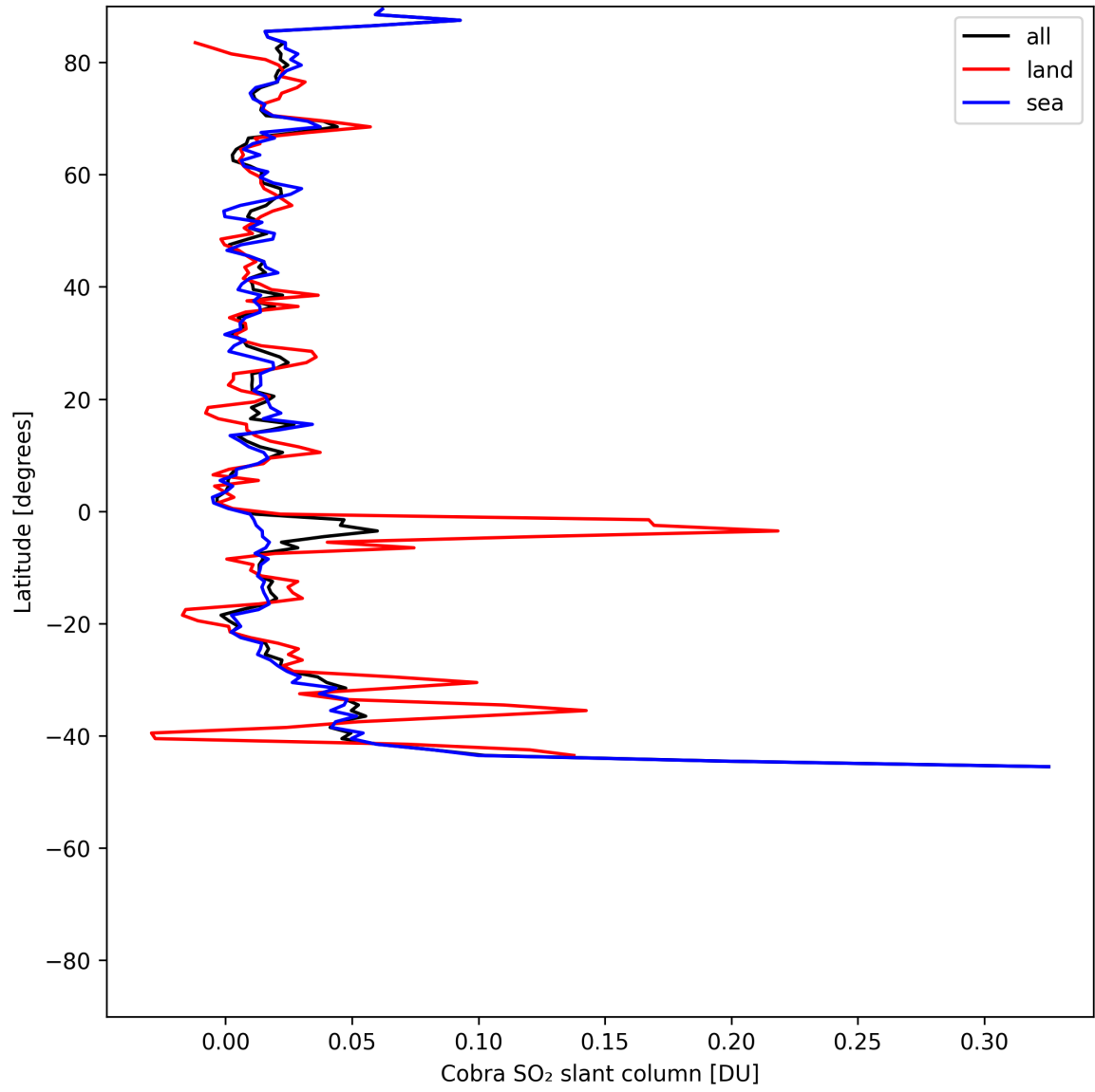
Figure 34: Zonal average of “Cobra SO 2 slant column” for 2025-06-13 to 2025-06-14.
