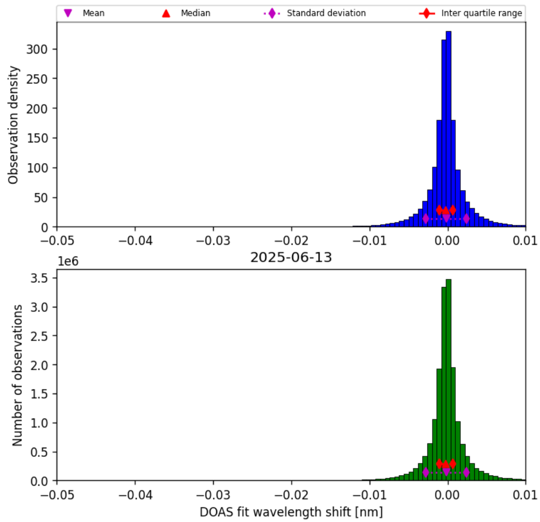
Figure 77: Histogram of “DOAS fit wavelength shift” for 2025-06-13 to 2025-06-14
