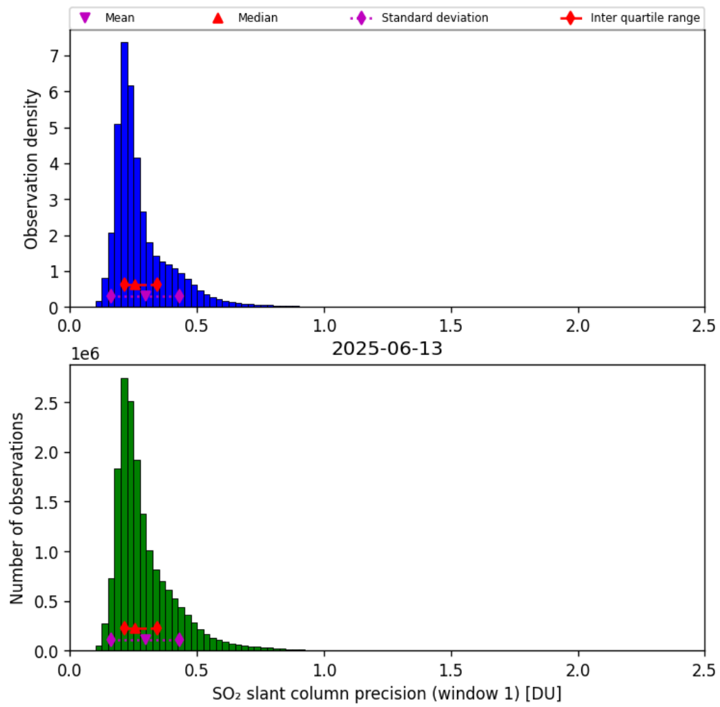
Figure 64: Histogram of “SO 2 slant column precision (window 1)” for 2025-06-13 to 2025-06-14
