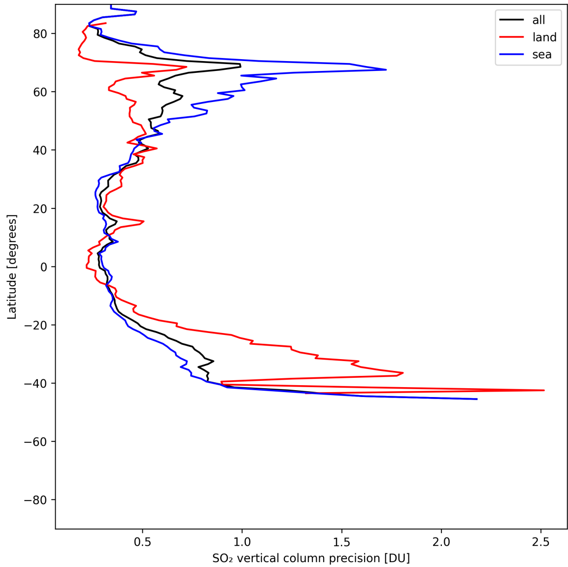
Figure 32: Zonal average of “SO 2 vertical column precision” for 2025-06-13 to 2025-06-14.
