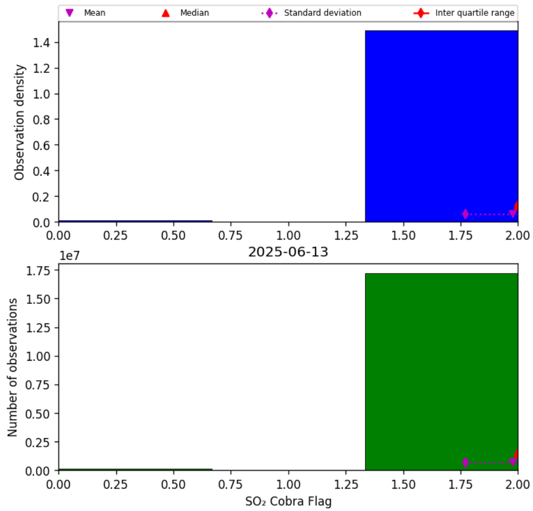
Figure 75: Histogram of “SO 2 Cobra Flag” for 2025-06-13 to 2025-06-14
