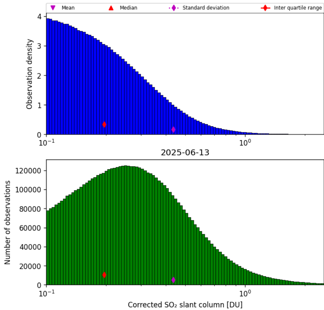
Figure 60: Histogram of “Corrected SO 2 slant column” for 2025-06-13 to 2025-06-14
