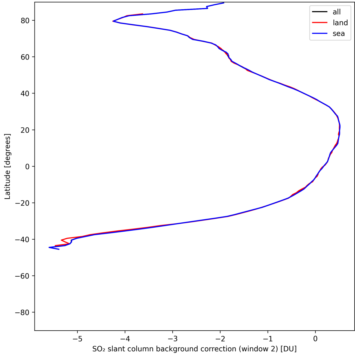
Figure 43: Zonal average of “SO 2 slant column background correction (window 2)” for 2025-06-13 to 2025-06-14.
