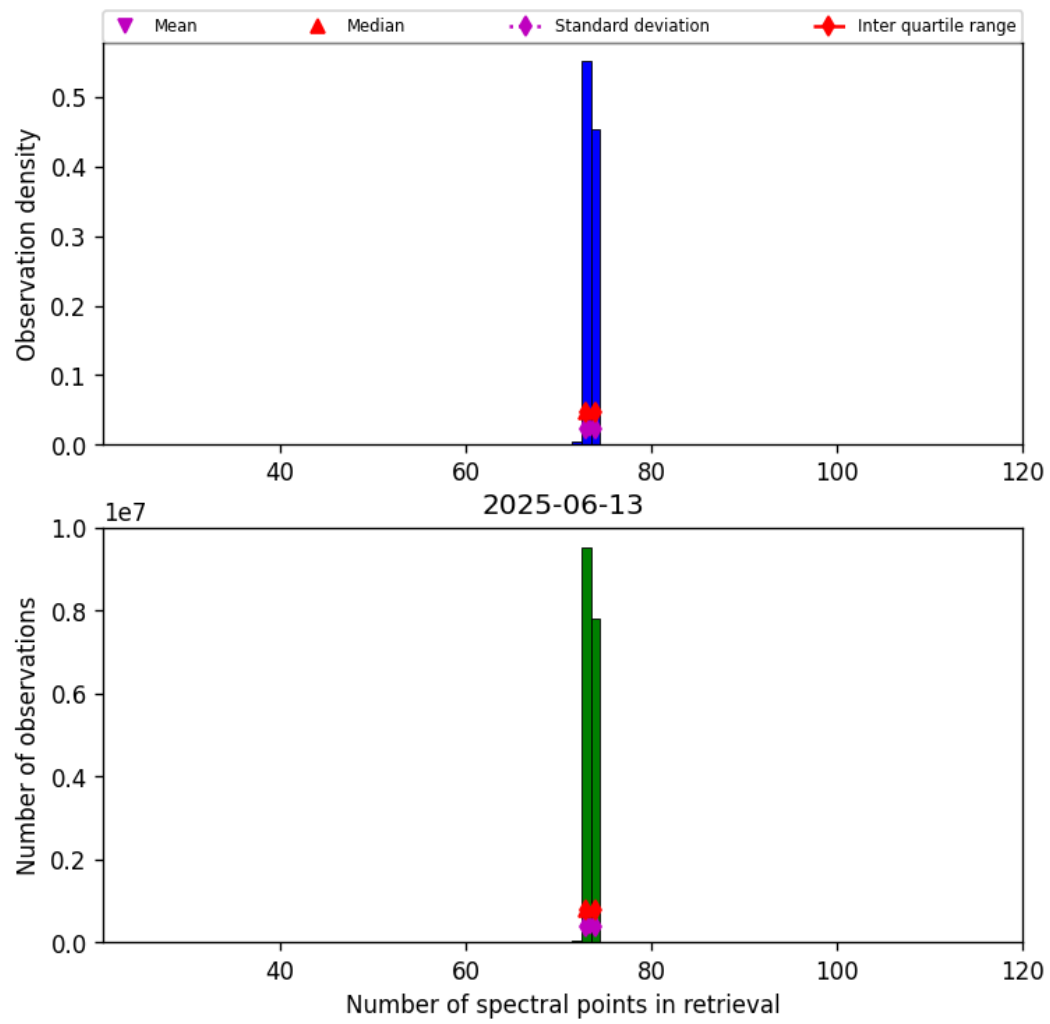
Figure 83: Histogram of “Number of spectral points in retrieval” for 2025-06-13 to 2025-06-14
