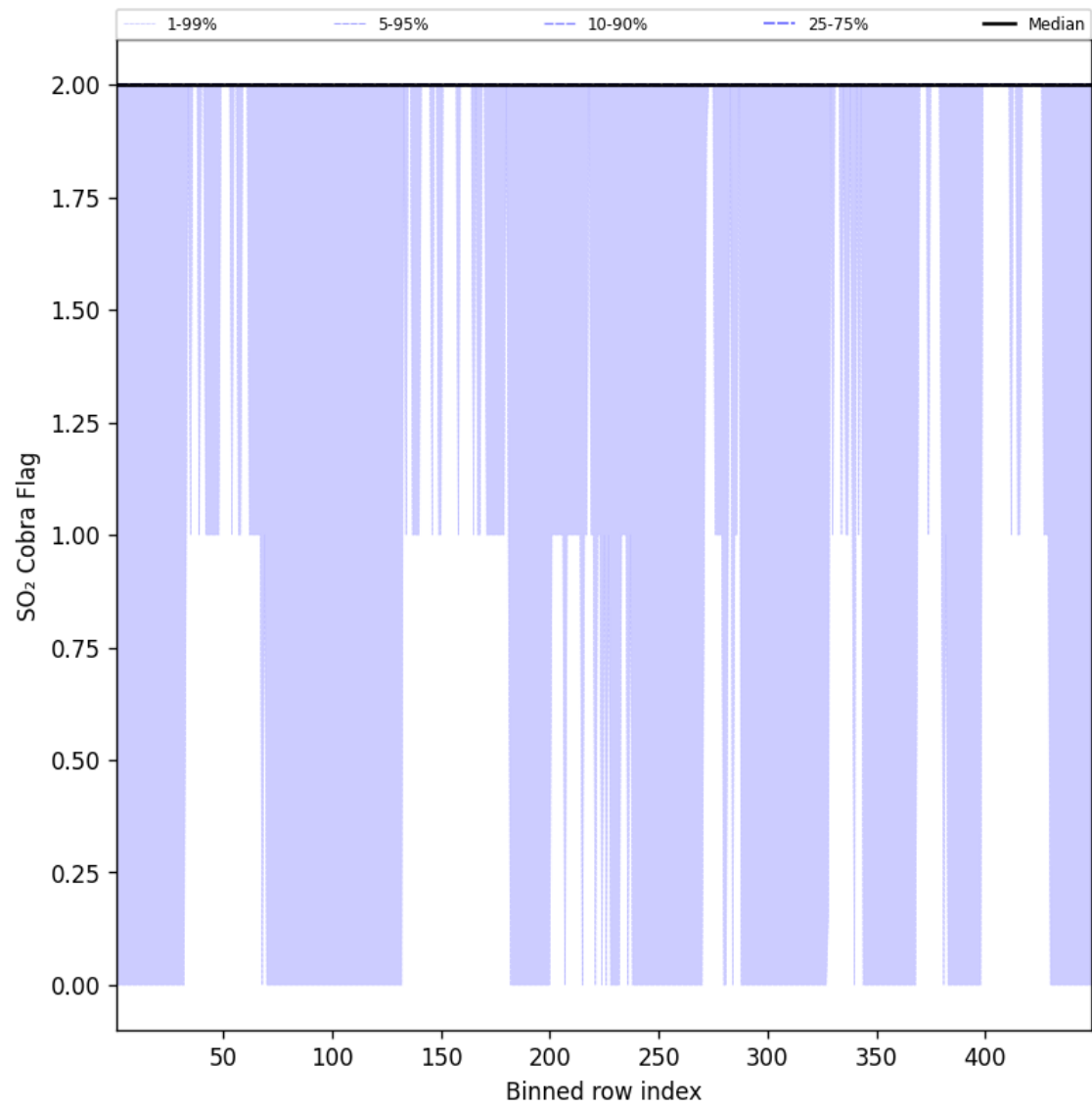
Figure 102: Along track statistics of “SO 2 Cobra Flag” for 2025-06-13 to 2025-06-14
