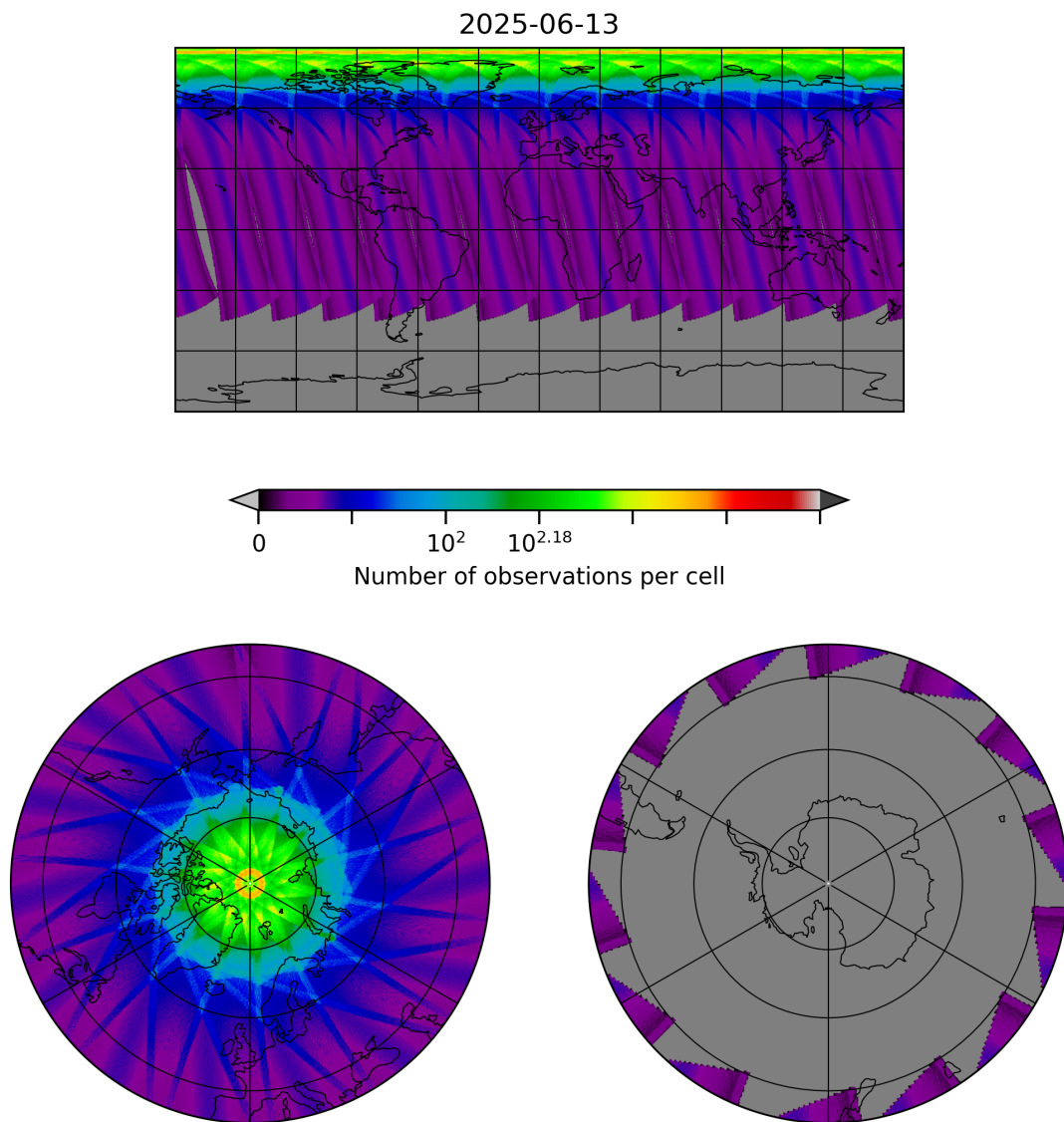
Figure 29: Map of the number of observations for 2025-06-13 to 2025-06-14
