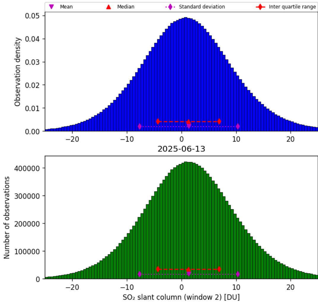
Figure 67: Histogram of “SO 2 slant column (window 2)” for 2025-06-13 to 2025-06-14
