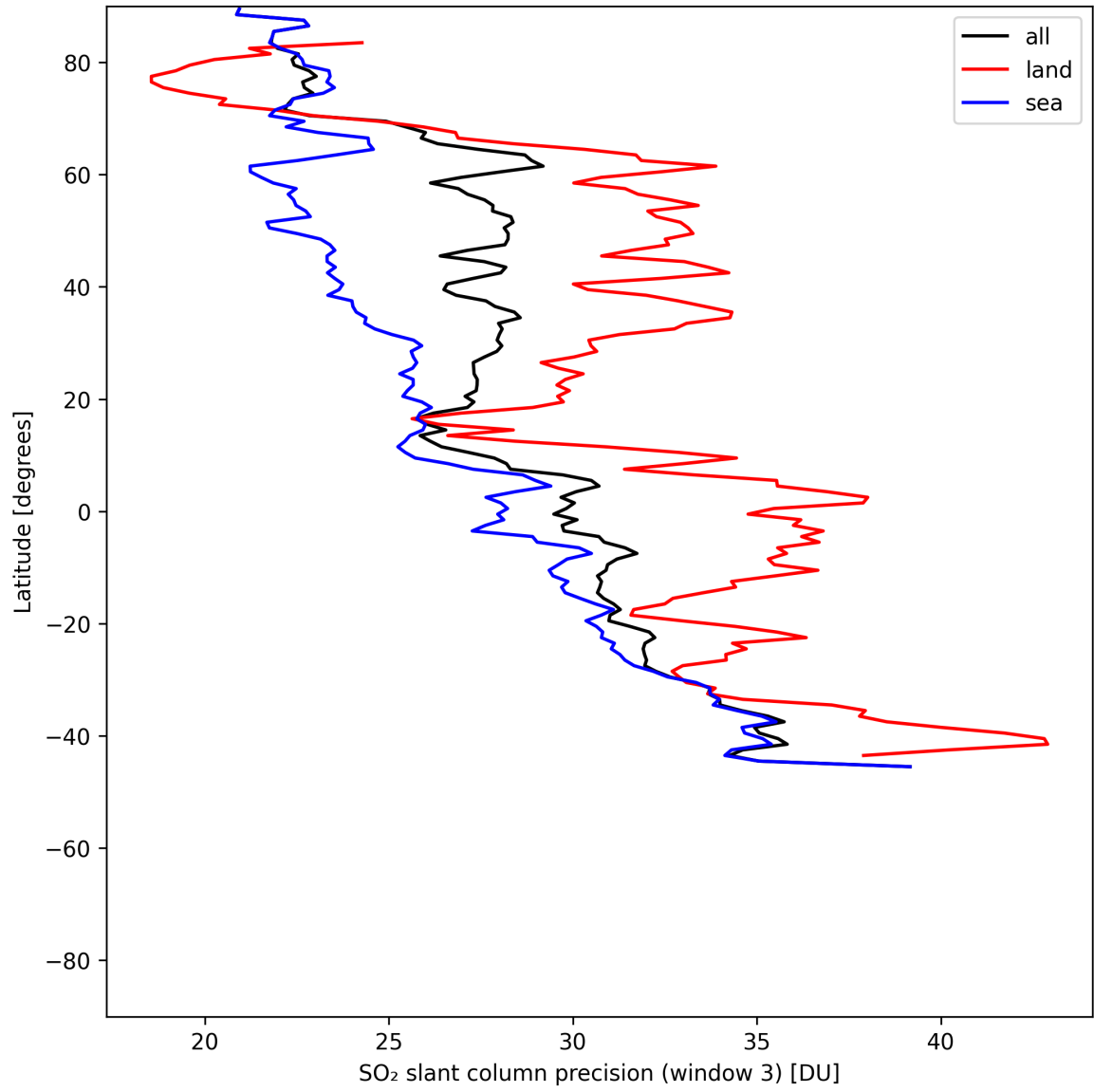
Figure 45: Zonal average of “SO 2 slant column precision (window 3)” for 2025-06-13 to 2025-06-14.
