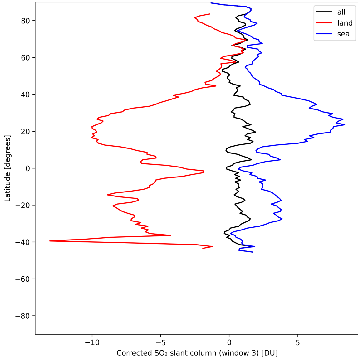
Figure 46: Zonal average of “Corrected SO 2 slant column (window 3)” for 2025-06-13 to 2025-06-14.
