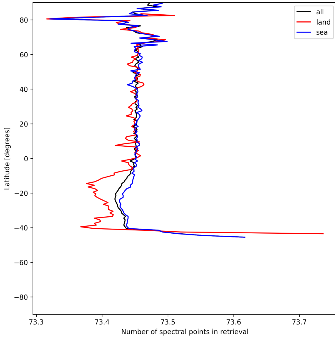
Figure 56: Zonal average of “Number of spectral points in retrieval” for 2025-06-13 to 2025-06-14.
