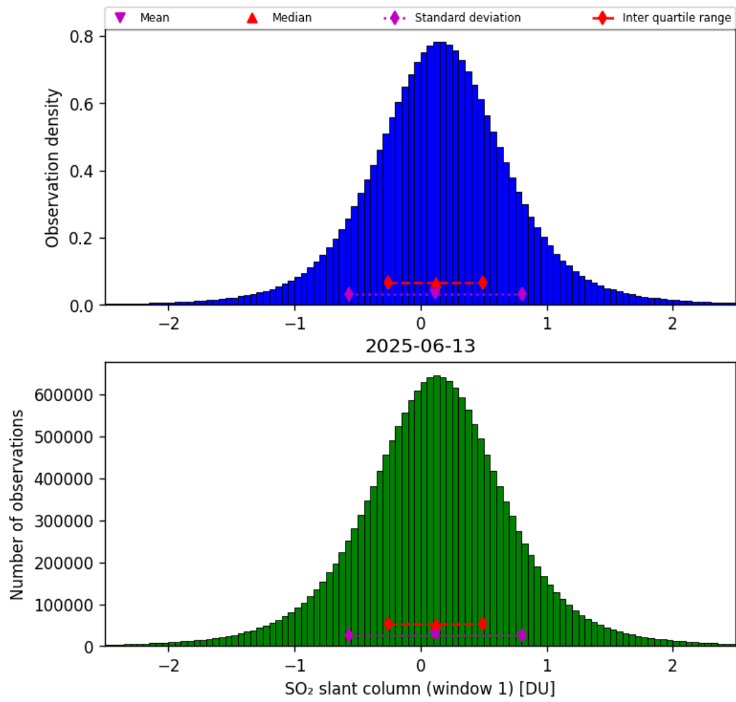
Figure 63: Histogram of “SO 2 slant column (window 1)” for 2025-06-13 to 2025-06-14
