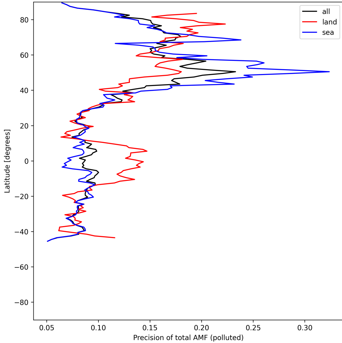
Figure 54: Zonal average of “Precision of total AMF (polluted)” for 2025-06-13 to 2025-06-14.
