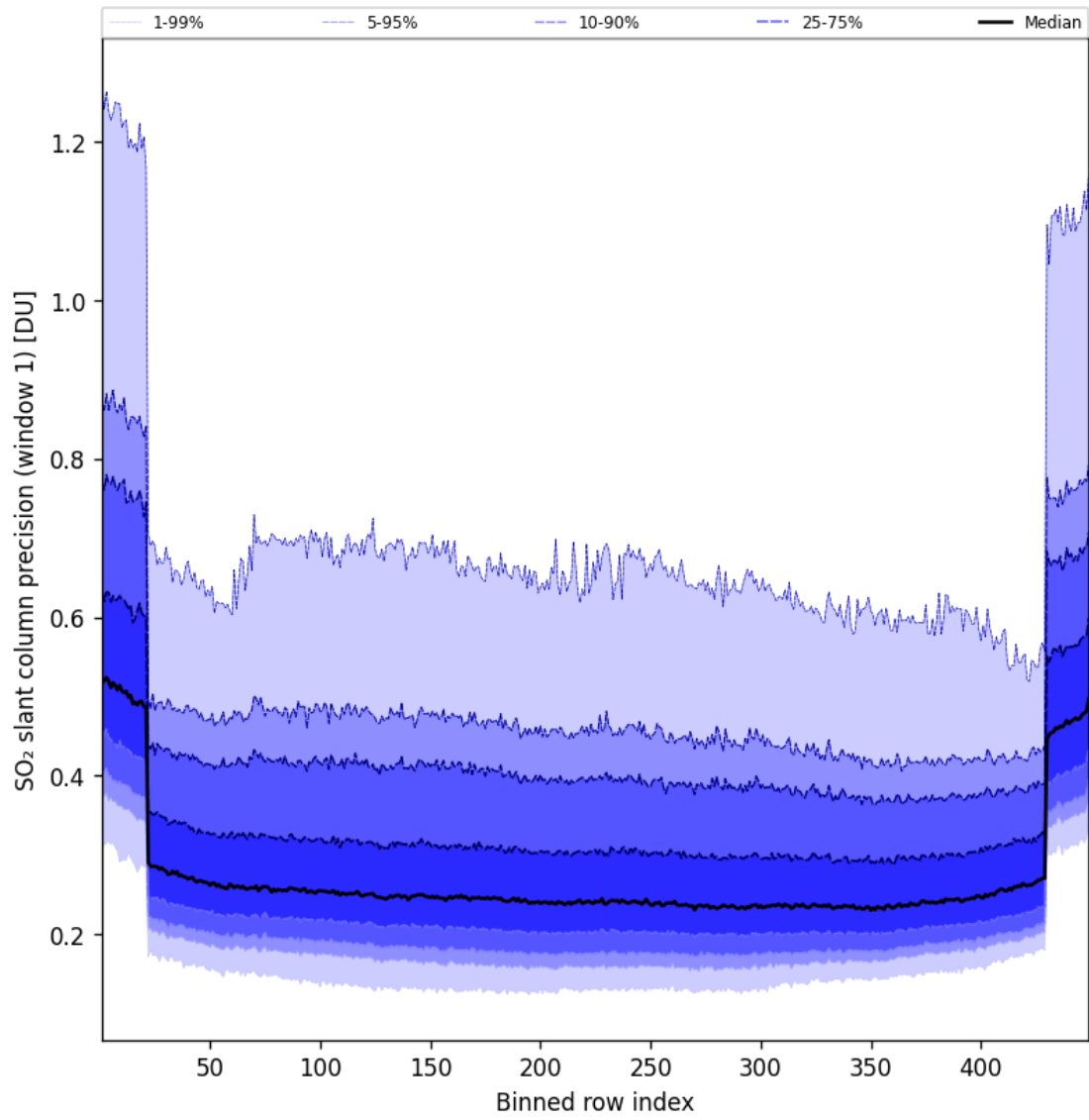
Figure 91: Along track statistics of “SO 2 slant column precision (window 1)” for 2025-06-13 to 2025-06-14
