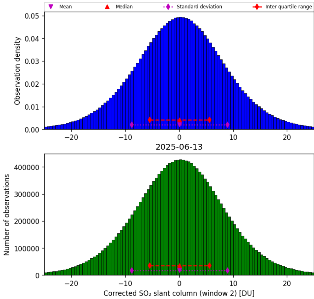
Figure 69: Histogram of “Corrected SO 2 slant column (window 2)” for 2025-06-13 to 2025-06-14
