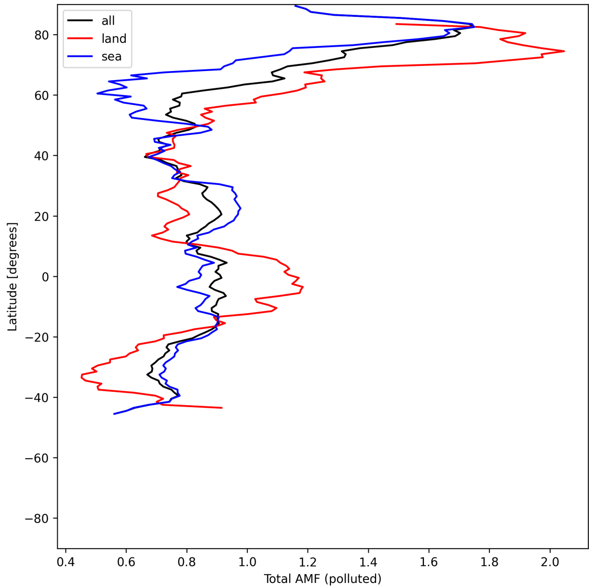
Figure 53: Zonal average of “Total AMF (polluted)” for 2025-06-13 to 2025-06-14.
