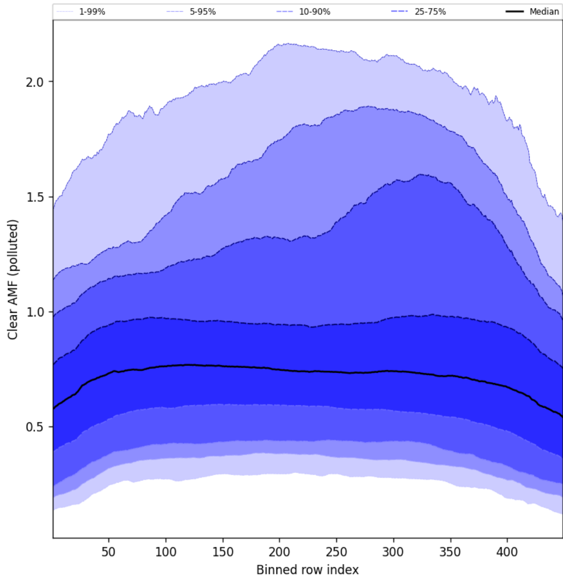
Figure 109: Along track statistics of “Clear AMF (polluted)” for 2025-06-13 to 2025-06-14
