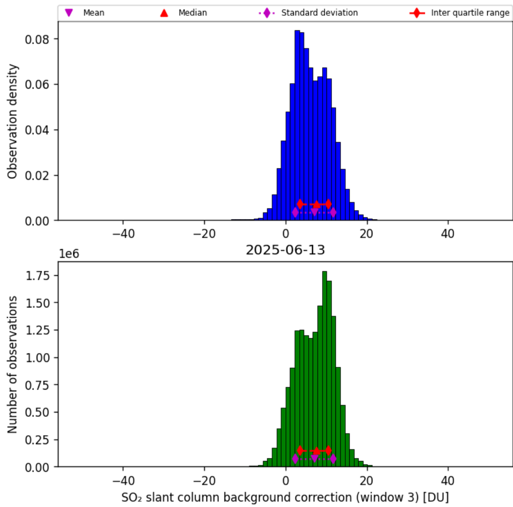
Figure 74: Histogram of “SO 2 slant column background correction (window 3)” for 2025-06-13 to 2025-06-14
