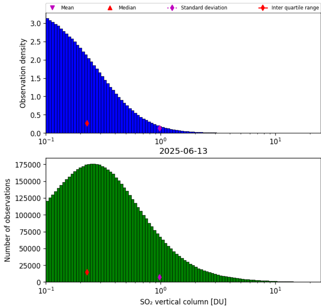
Figure 58: Histogram of “SO 2 vertical column” for 2025-06-13 to 2025-06-14
