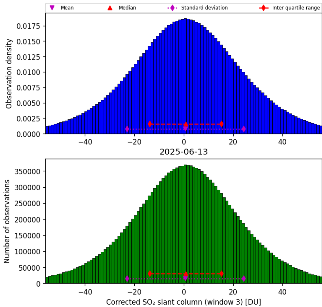
Figure 73: Histogram of “Corrected SO 2 slant column (window 3)” for 2025-06-13 to 2025-06-14
