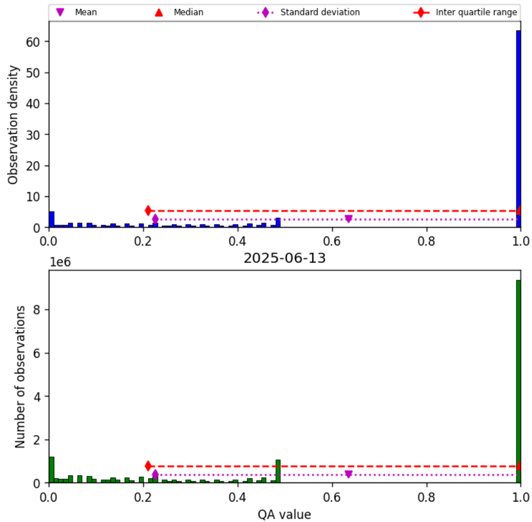
Figure 57: Histogram of “QA value” for 2025-06-13 to 2025-06-14
