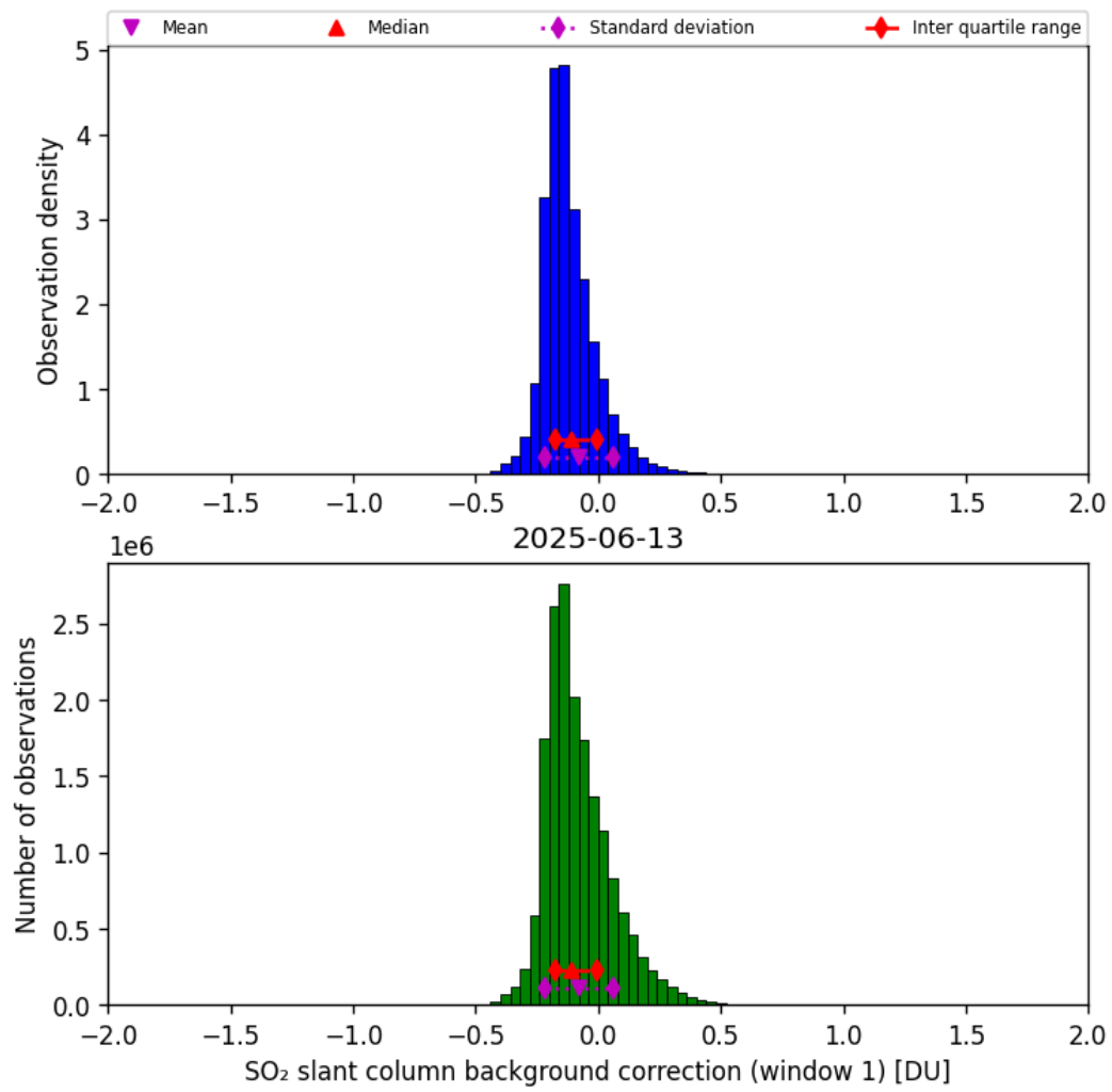
Figure 66: Histogram of “SO 2 slant column background correction (window 1)” for 2025-06-13 to 2025-06-14
