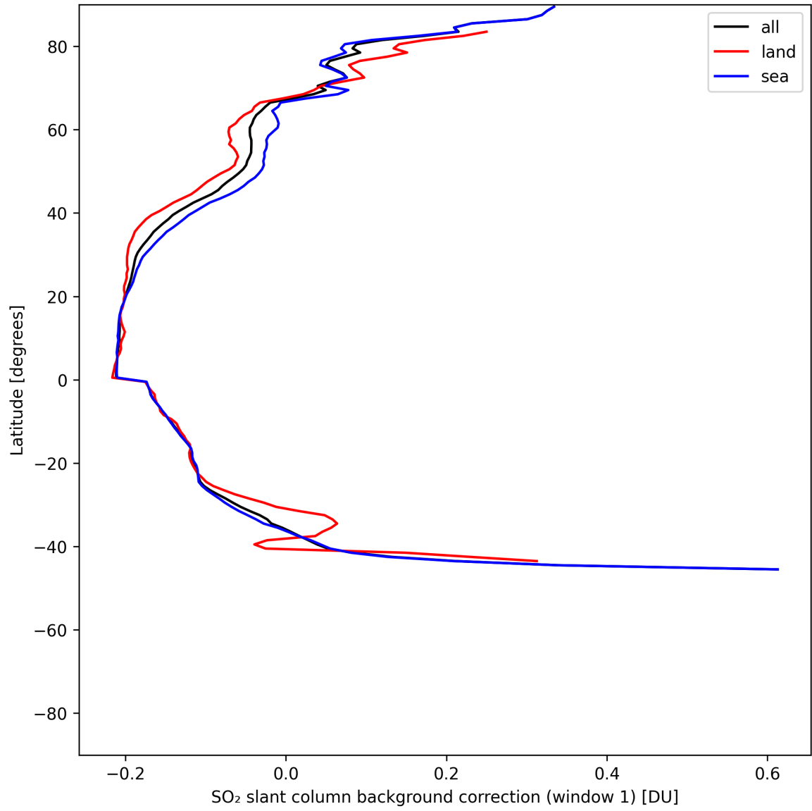
Figure 39: Zonal average of “SO 2 slant column background correction (window 1)” for 2025-06-13 to 2025-06-14.
