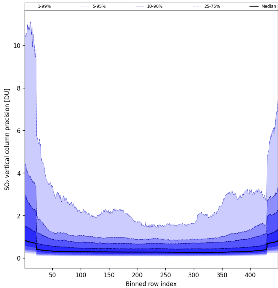
Figure 86: Along track statistics of “SO 2 vertical column precision” for 2025-06-13 to 2025-06-14
