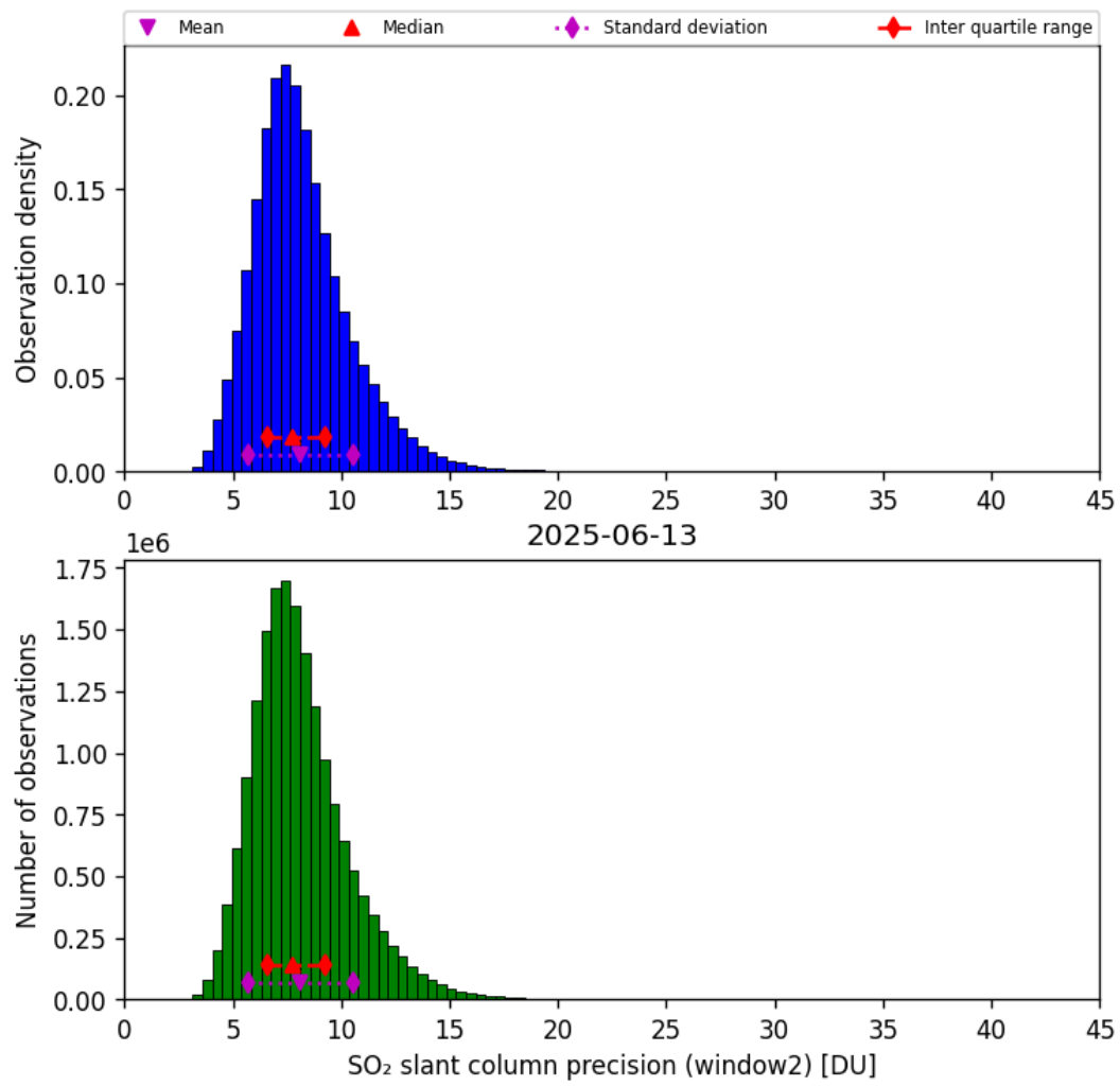
Figure 68: Histogram of “SO 2 slant column precision (window2)” for 2025-06-13 to 2025-06-14
