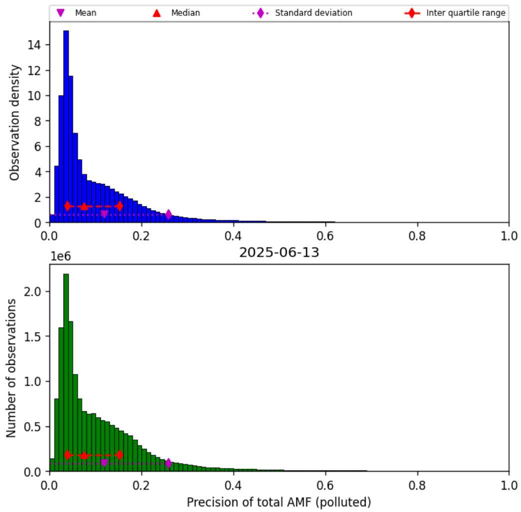
Figure 81: Histogram of “Precision of total AMF (polluted)” for 2025-06-13 to 2025-06-14
