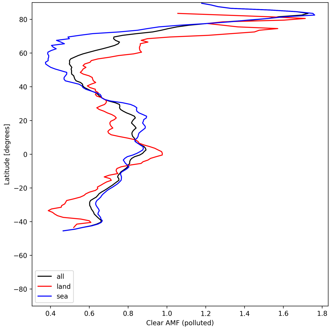
Figure 55: Zonal average of “Clear AMF (polluted)” for 2025-06-13 to 2025-06-14.
