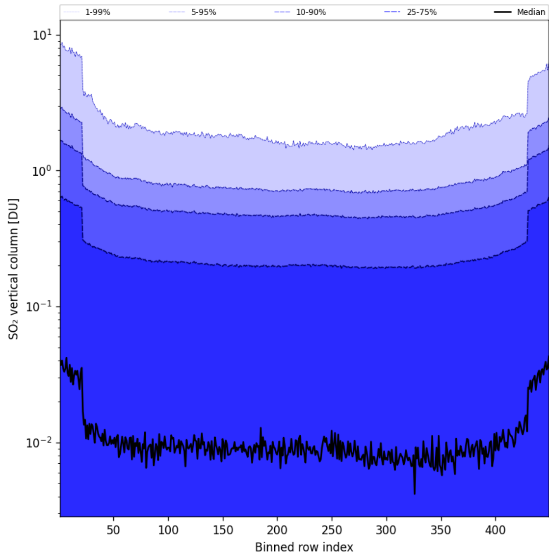
Figure 85: Along track statistics of “SO 2 vertical column” for 2025-06-13 to 2025-06-14
