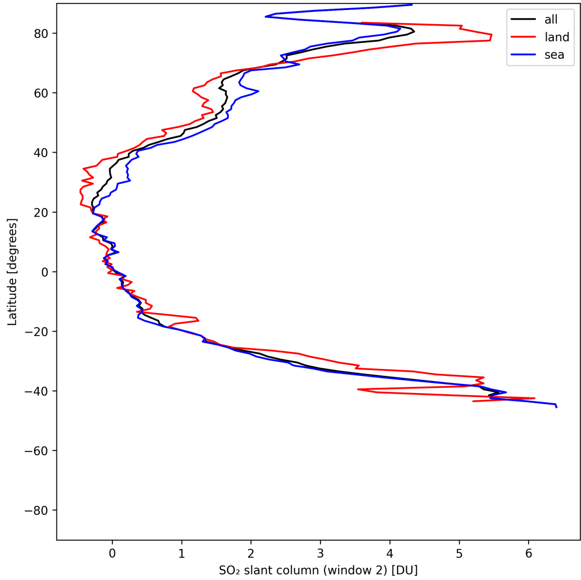
Figure 40: Zonal average of “SO 2 slant column (window 2)” for 2025-06-13 to 2025-06-14.
