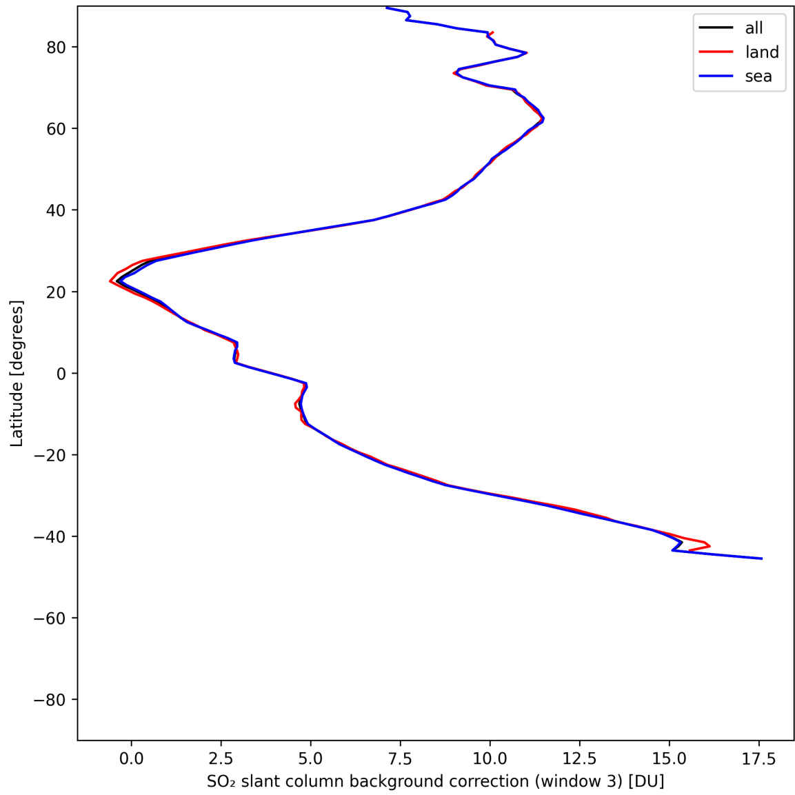
Figure 47: Zonal average of “SO 2 slant column background correction (window 3)” for 2025-06-13 to 2025-06-14.
