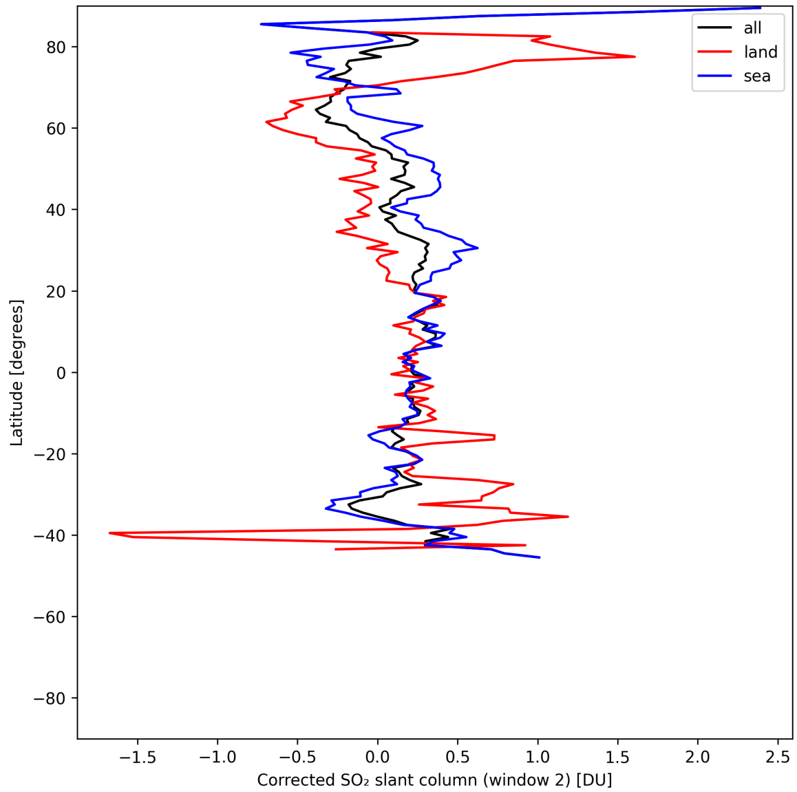
Figure 42: Zonal average of "Corrected SO 2 slant column (window 2)" for 2025-06-13 to 2025-06-14.
