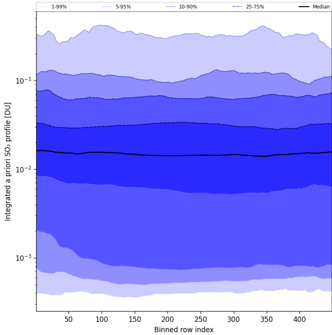
Figure 103: Along track statistics of “Integrated a priori SO 2 profile” for 2025-06-13 to 2025-06-14
