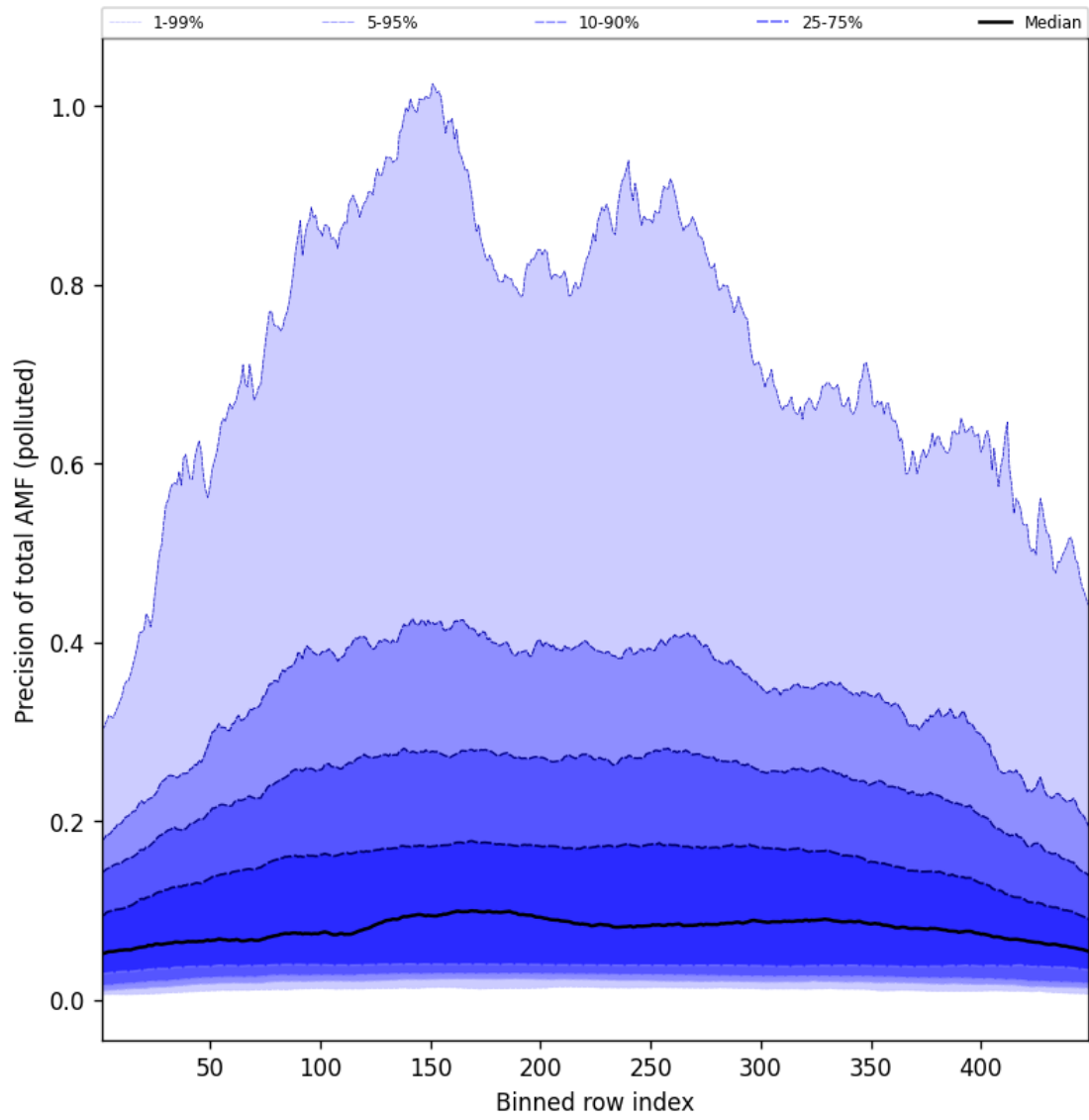
Figure 108: Along track statistics of “Precision of total AMF (polluted)” for 2025-06-13 to 2025-06-14
