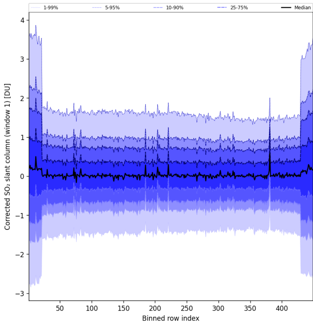
Figure 92: Along track statistics of “Corrected SO 2 slant column (window 1)” for 2025-06-13 to 2025-06-14
