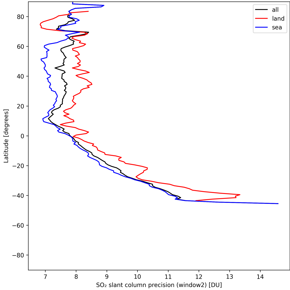
Figure 41: Zonal average of “SO 2 slant column precision (window2)” for 2025-06-13 to 2025-06-14.
