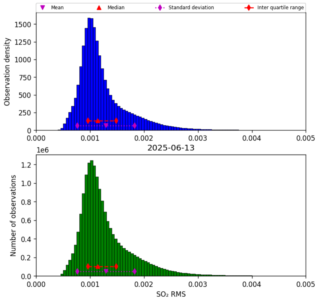
Figure 79: Histogram of “SO 2 RMS” for 2025-06-13 to 2025-06-14
