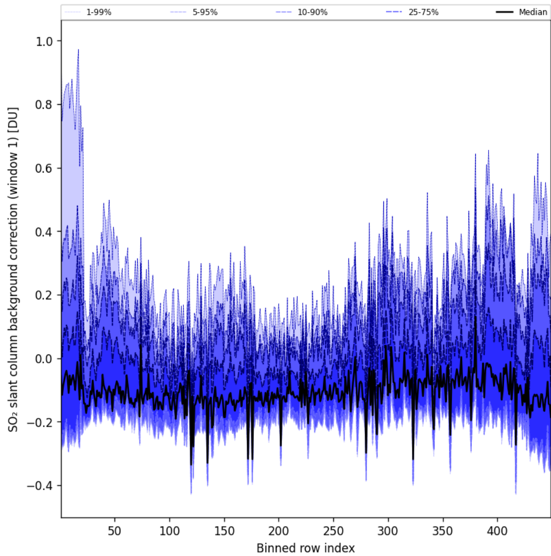
Figure 93: Along track statistics of “SO 2 slant column background correction (window 1)” for 2025-06-13 to 2025-06-14
