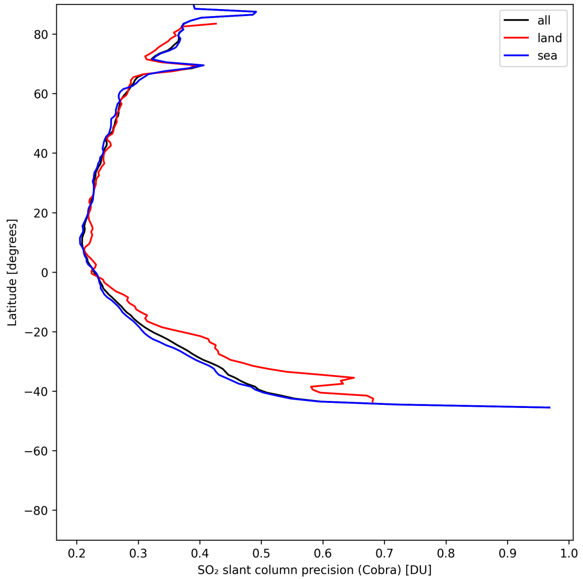
Figure 35: Zonal average of “SO 2 slant column precision (Cobra)” for 2025-06-13 to 2025-06-14.
