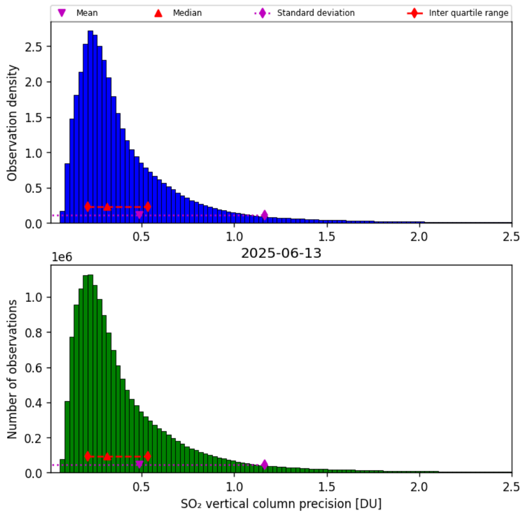
Figure 59: Histogram of “SO 2 vertical column precision” for 2025-06-13 to 2025-06-14
