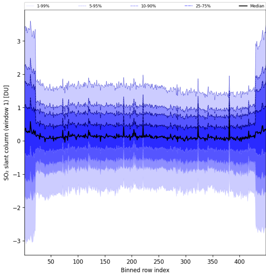
Figure 90: Along track statistics of “SO 2 slant column (window 1)” for 2025-06-13 to 2025-06-14
