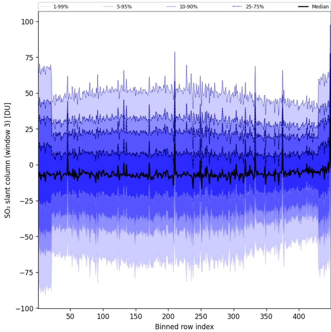
Figure 98: Along track statistics of “SO 2 slant column (window 3)” for 2025-06-13 to 2025-06-14
