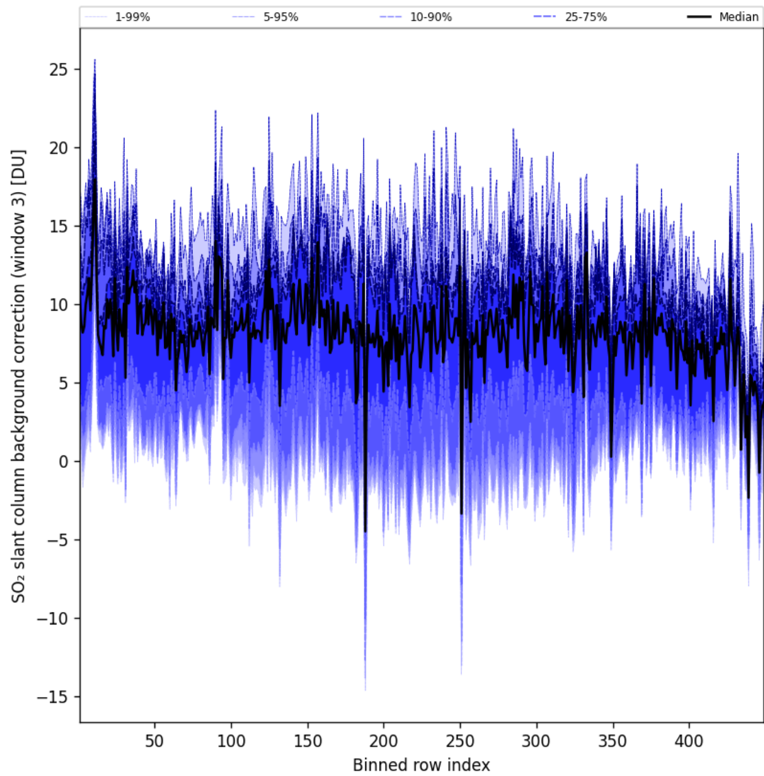
Figure 101: Along track statistics of “SO 2 slant column background correction (window 3)” for 2025-06-13 to 2025-06-14
