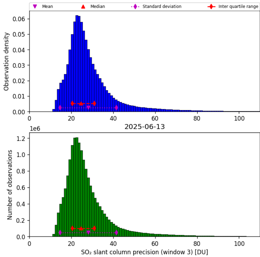
Figure 72: Histogram of “SO 2 slant column precision (window 3)” for 2025-06-13 to 2025-06-14
