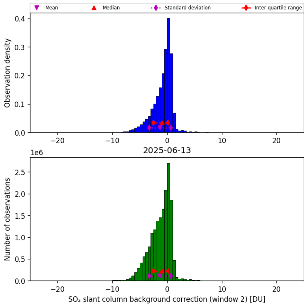
Figure 70: Histogram of “SO 2 slant column background correction (window 2)” for 2025-06-13 to 2025-06-14
