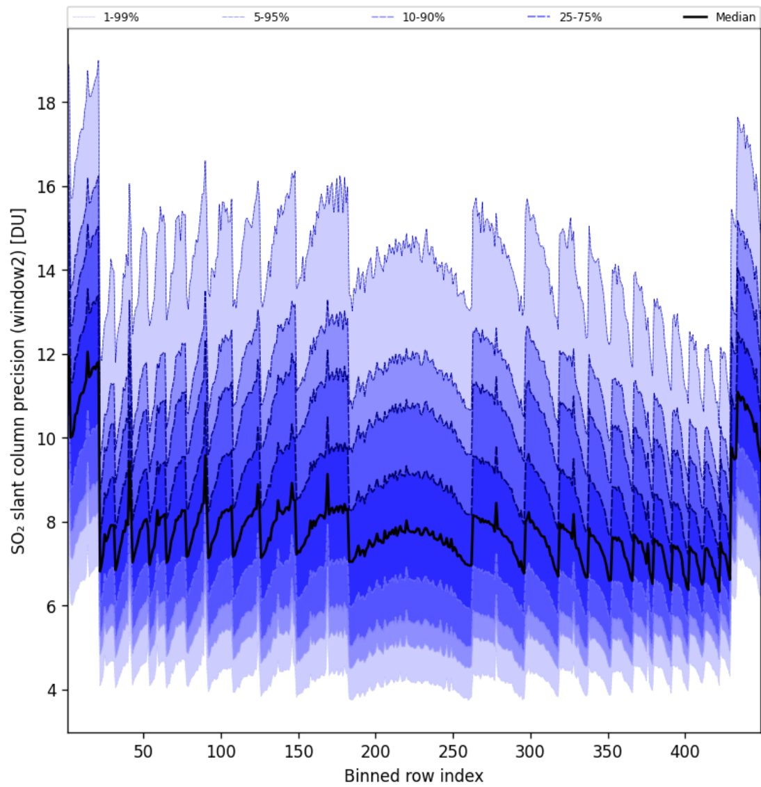
Figure 95: Along track statistics of “SO 2 slant column precision (window2)” for 2025-06-13 to 2025-06-14
