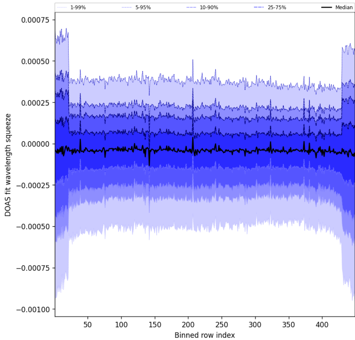
Figure 105: Along track statistics of “DOAS fit wavelength squeeze” for 2025-06-13 to 2025-06-14
