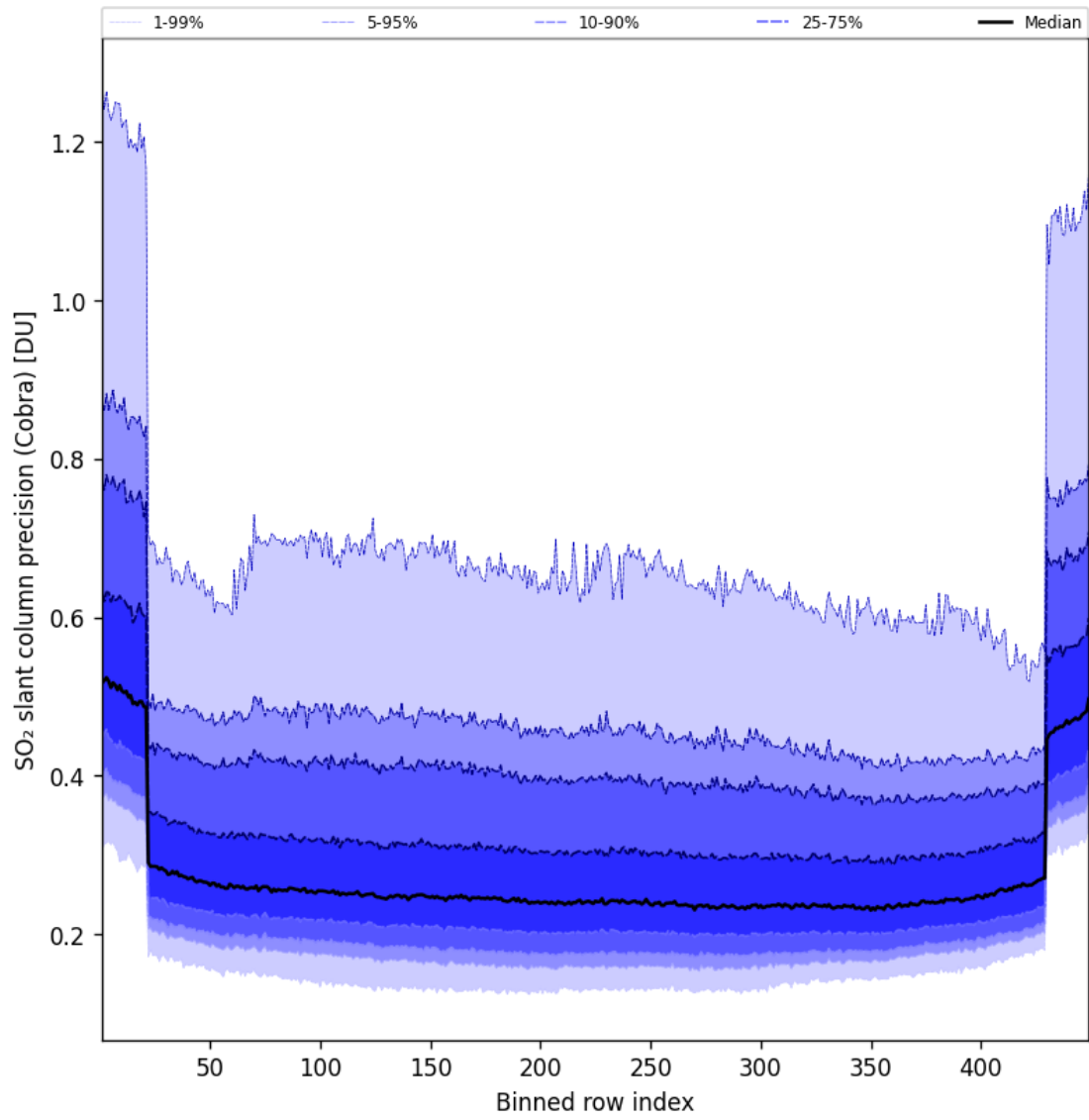
Figure 89: Along track statistics of “SO 2 slant column precision (Cobra)” for 2025-06-13 to 2025-06-14
