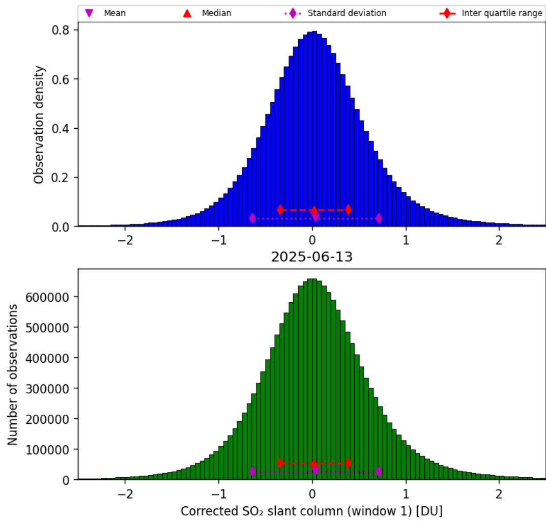
Figure 65: Histogram of “Corrected SO 2 slant column (window 1)” for 2025-06-13 to 2025-06-14
