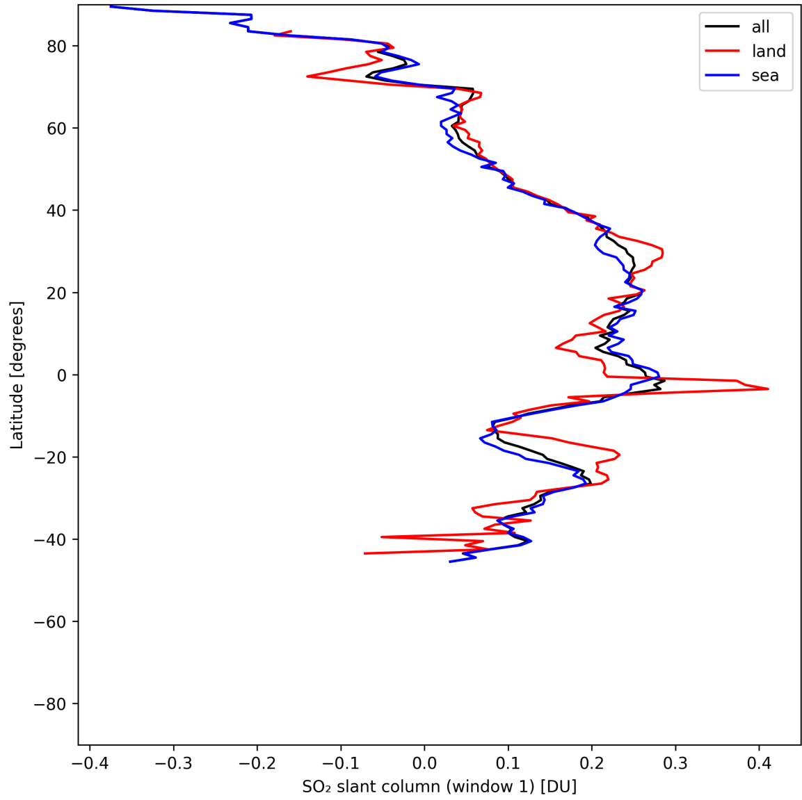
Figure 36: Zonal average of “SO 2 slant column (window 1)” for 2025-06-13 to 2025-06-14.
