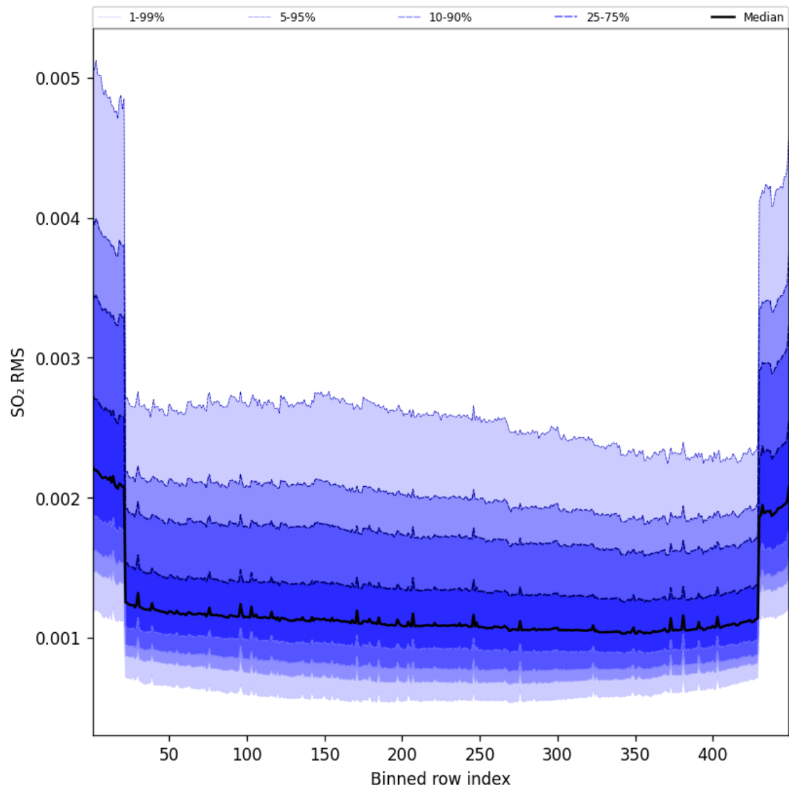
Figure 106: Along track statistics of “SO 2 RMS” for 2025-06-13 to 2025-06-14
