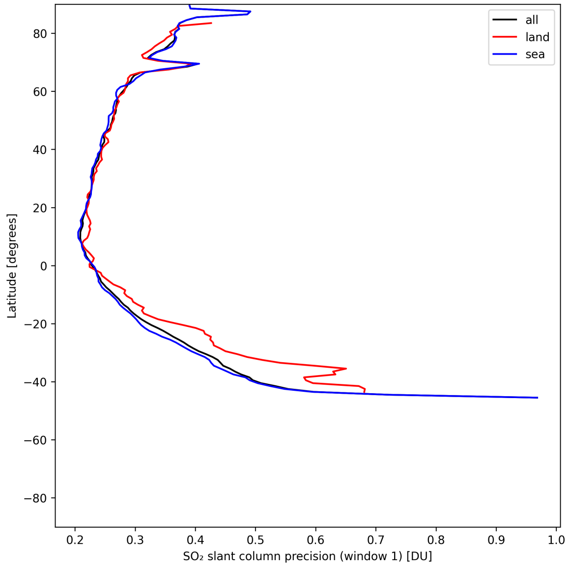
Figure 37: Zonal average of “SO 2 slant column precision (window 1)” for 2025-06-13 to 2025-06-14.
