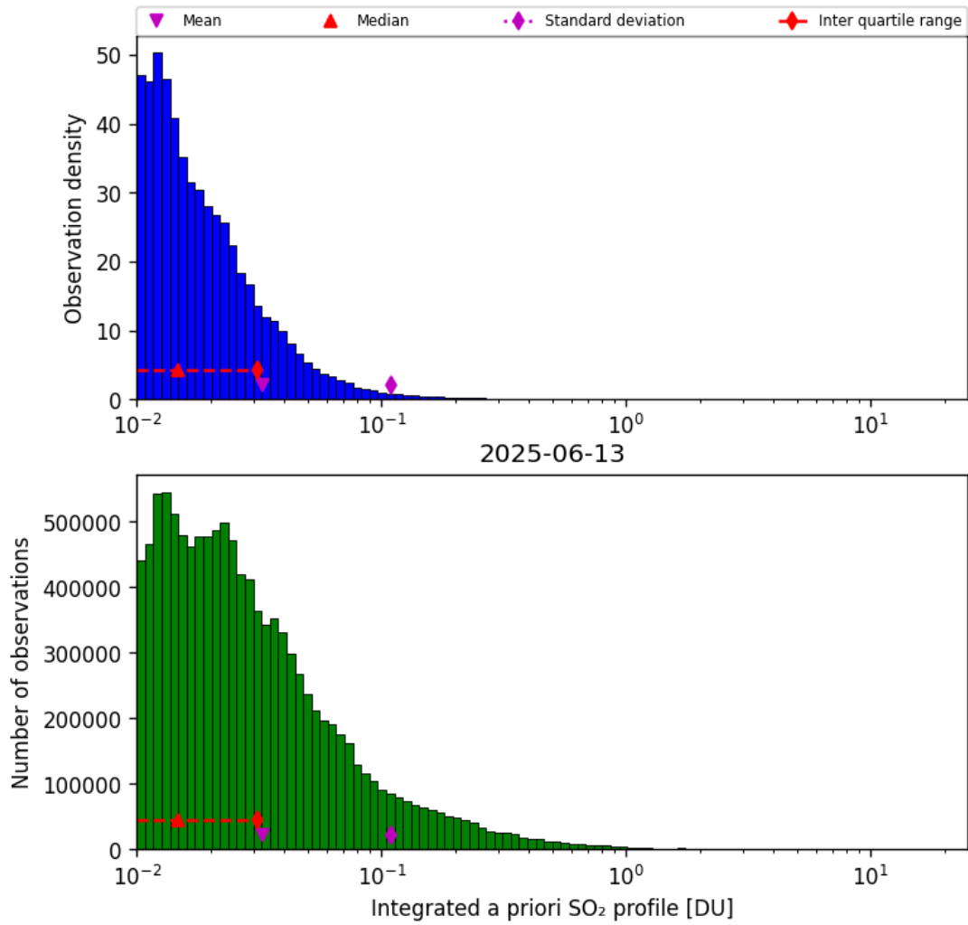
Figure 76: Histogram of “Integrated a priori SO 2 profile” for 2025-06-13 to 2025-06-14
