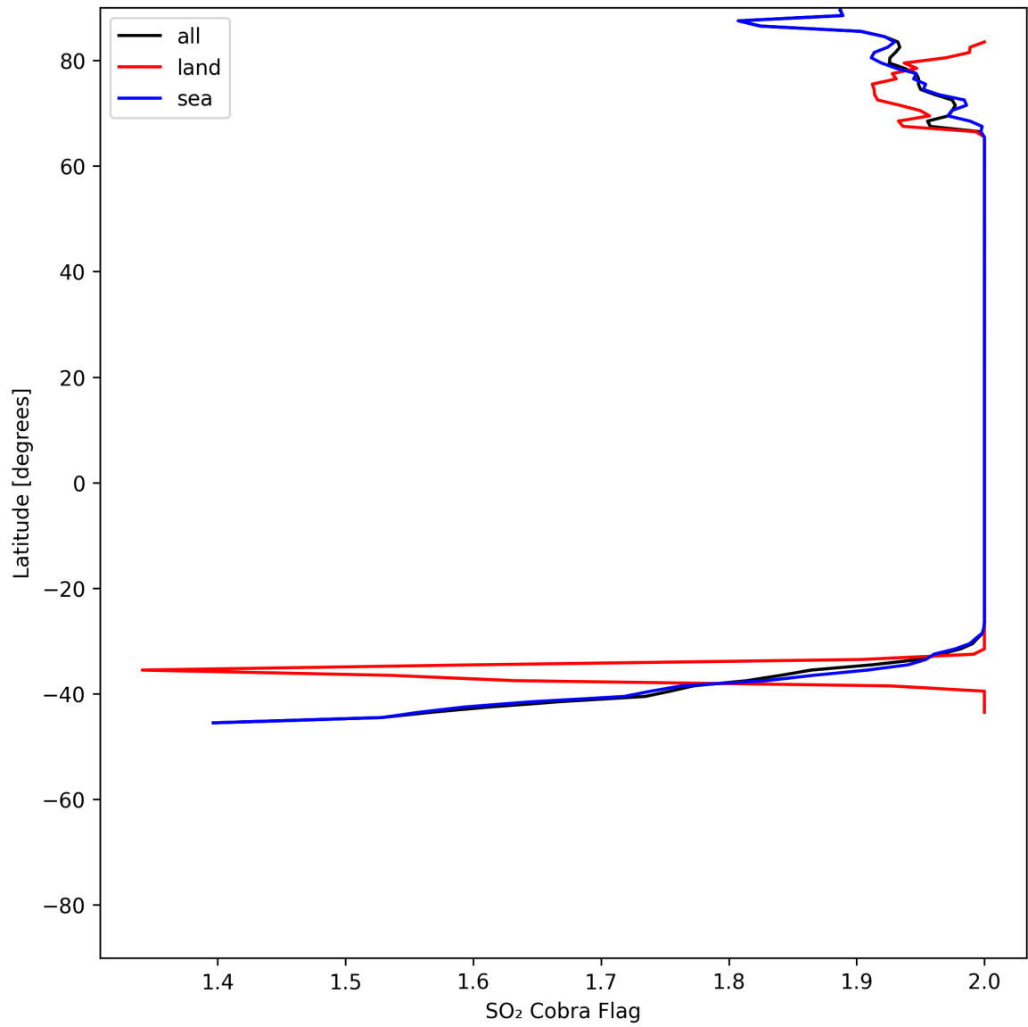
Figure 48: Zonal average of "SO 2 Cobra Flag" for 2025-06-13 to 2025-06-14.
