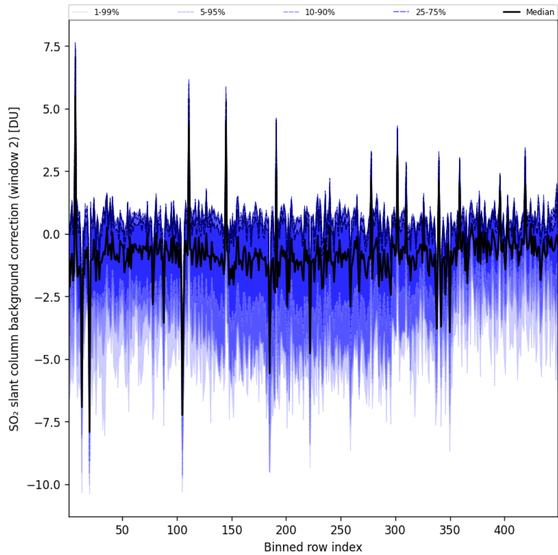
Figure 97: Along track statistics of “SO 2 slant column background correction (window 2)” for 2025-06-13 to 2025-06-14
