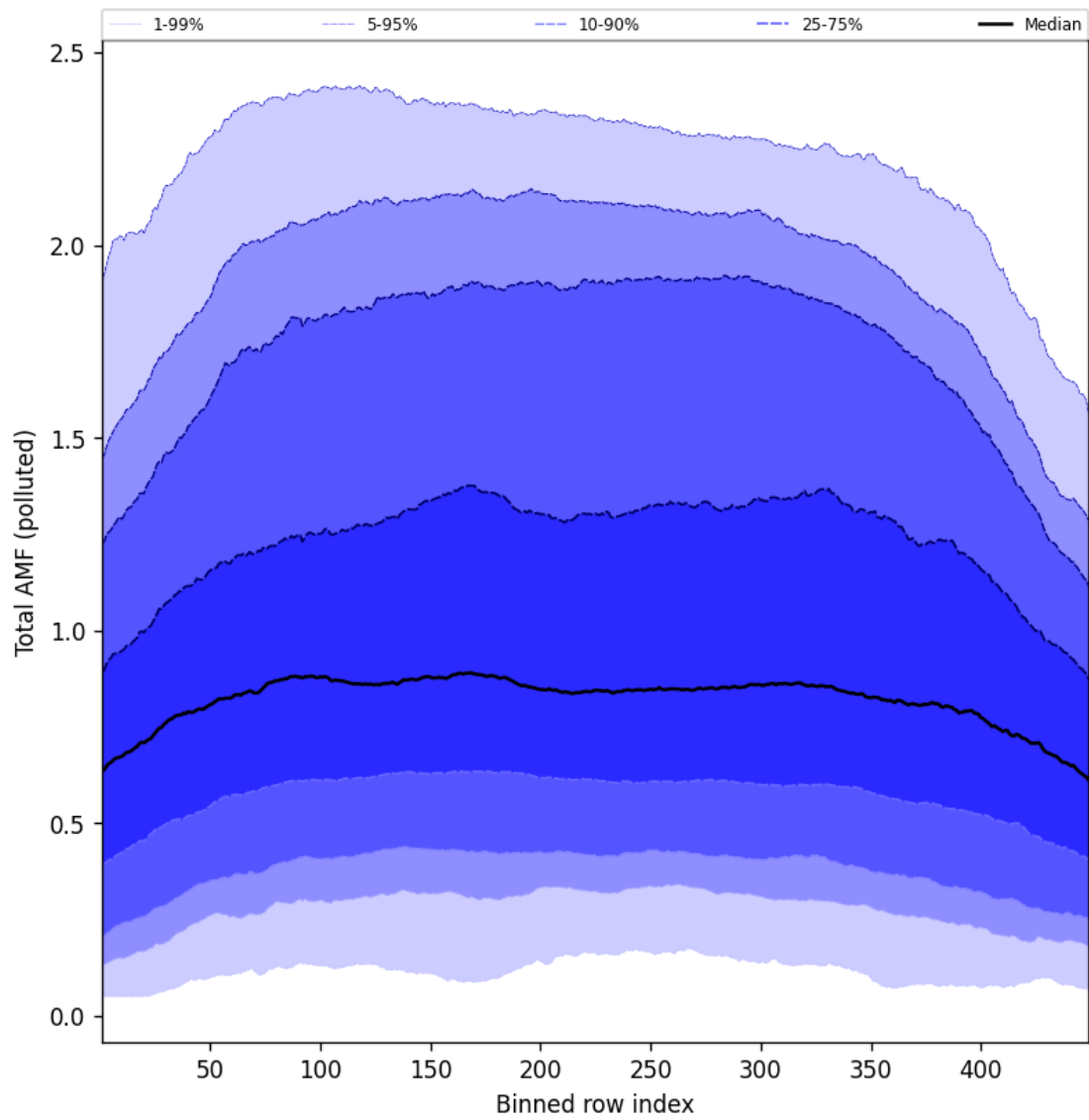
Figure 107: Along track statistics of “Total AMF (polluted)” for 2025-06-13 to 2025-06-14
