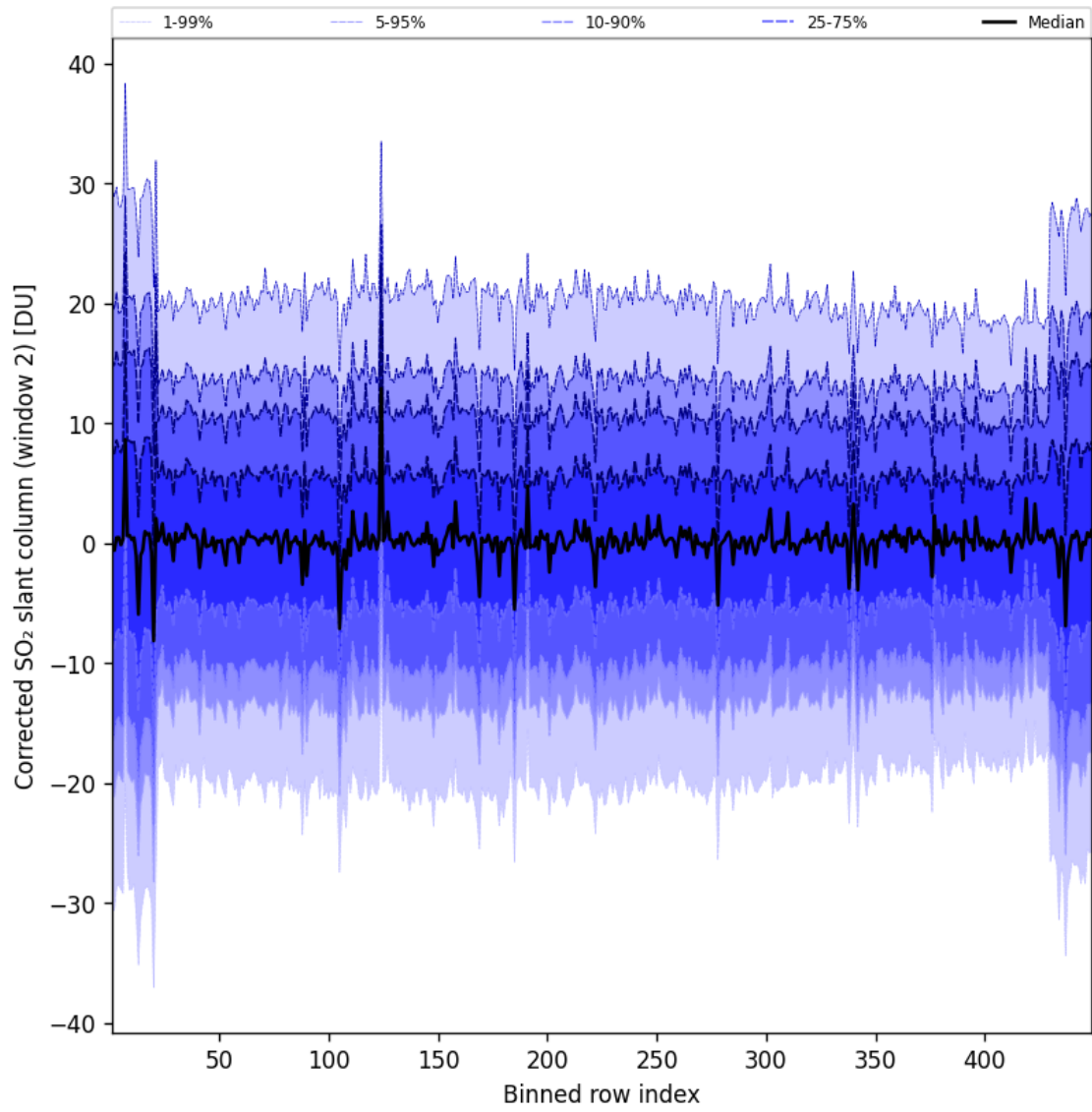
Figure 96: Along track statistics of “Corrected SO 2 slant column (window 2)” for 2025-06-13 to 2025-06-14
