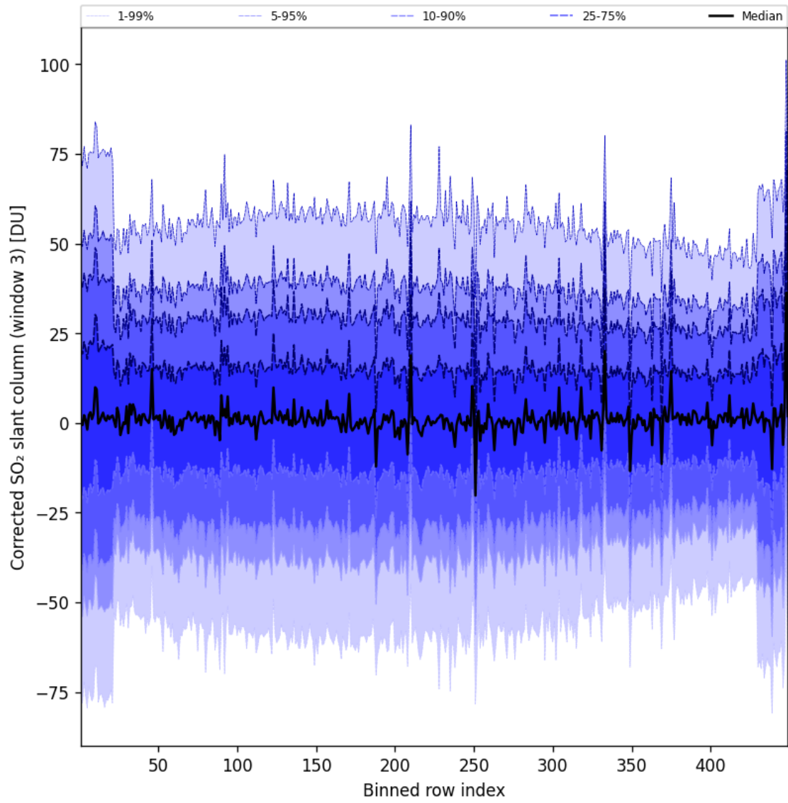
Figure 100: Along track statistics of “Corrected SO 2 slant column (window 3)” for 2025-06-13 to 2025-06-14
