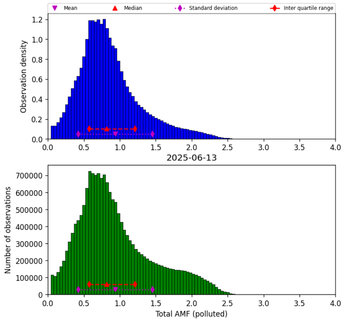
Figure 80: Histogram of “Total AMF (polluted)” for 2025-06-13 to 2025-06-14
