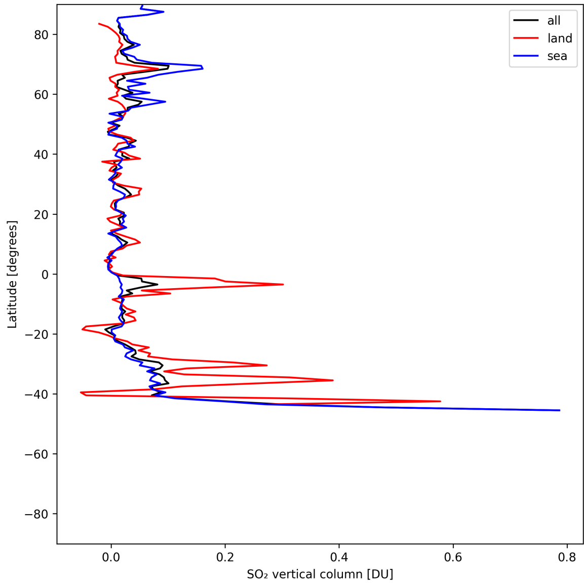
Figure 31: Zonal average of “SO 2 vertical column” for 2025-06-13 to 2025-06-14.
