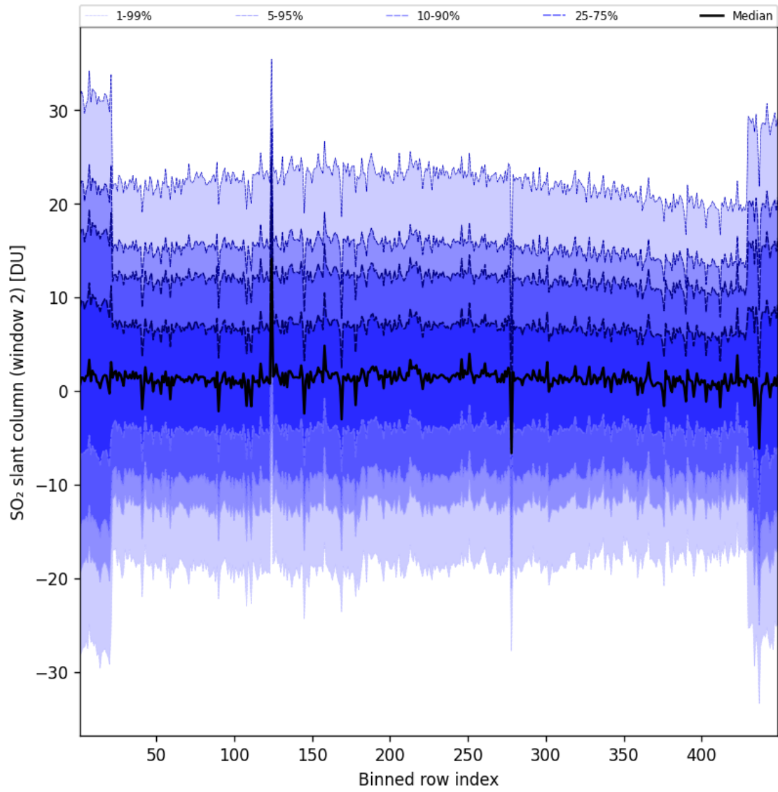
Figure 94: Along track statistics of “SO 2 slant column (window 2)” for 2025-06-13 to 2025-06-14
