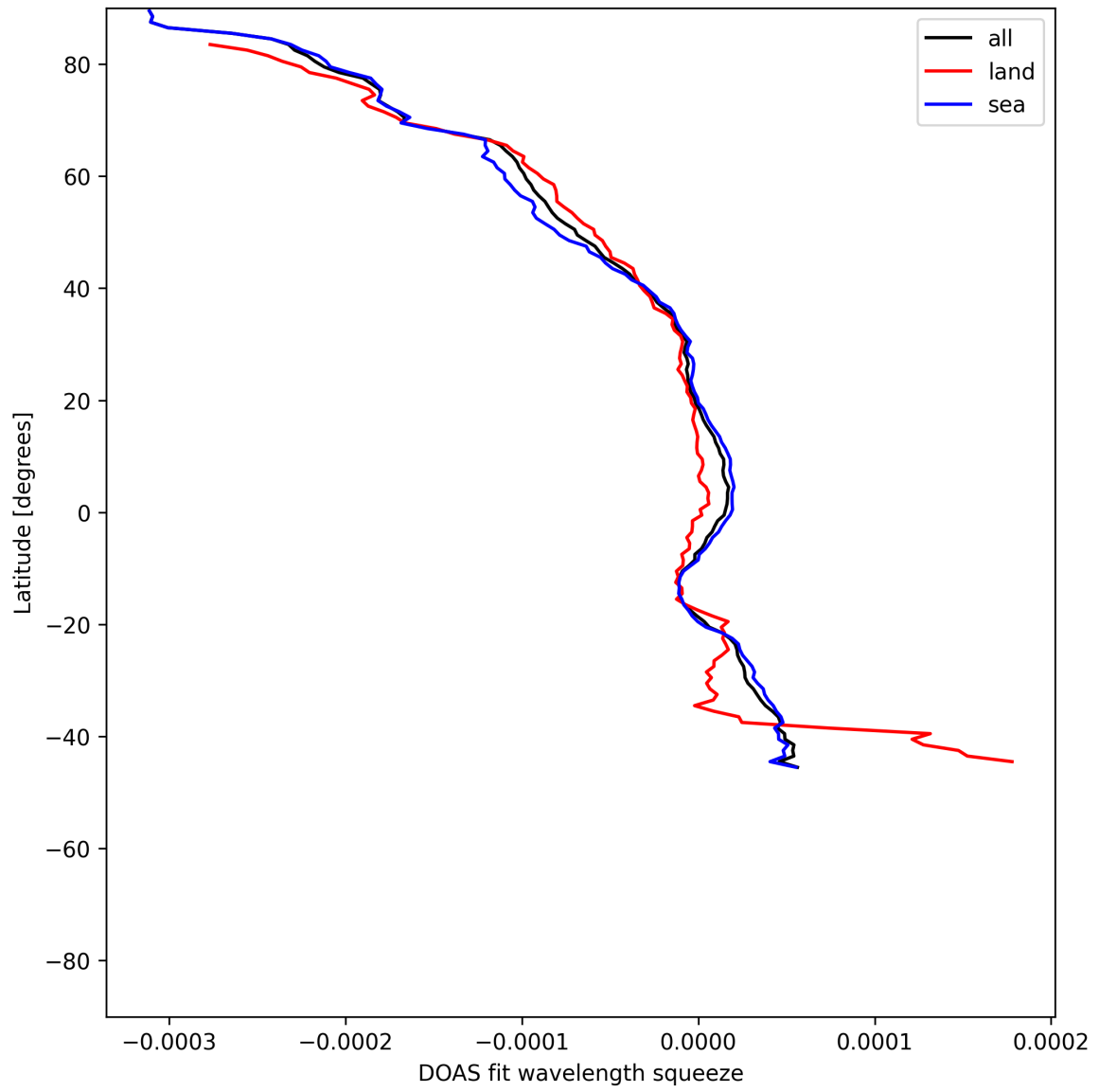
Figure 51: Zonal average of “DOAS fit wavelength squeeze” for 2025-06-14 to 2025-06-14.
