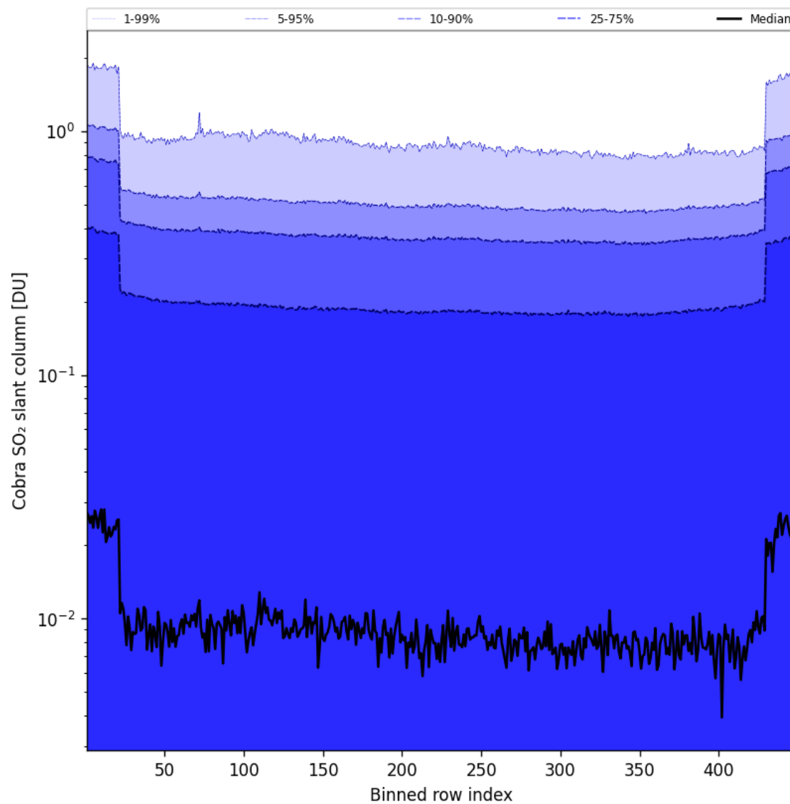
Figure 88: Along track statistics of “Cobra SO 2 slant column” for 2025-06-14 to 2025-06-14
