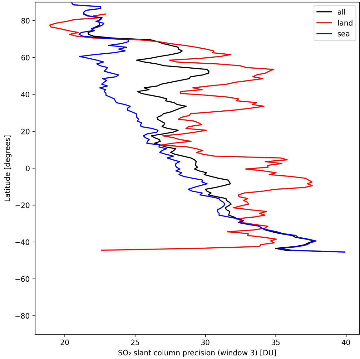
Figure 45: Zonal average of “SO 2 slant column precision (window 3)” for 2025-06-14 to 2025-06-14.
