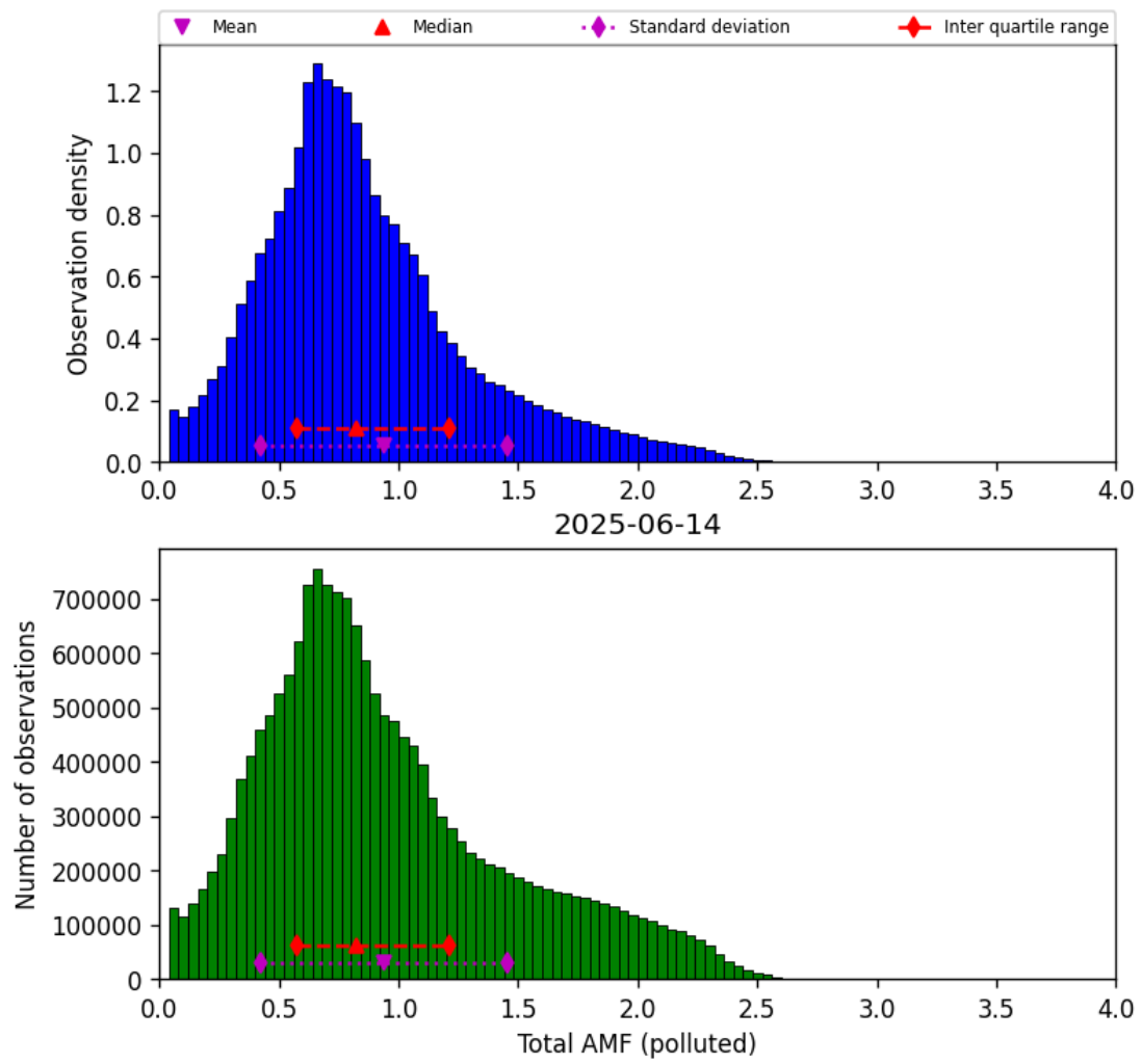
Figure 80: Histogram of “Total AMF (polluted)” for 2025-06-14 to 2025-06-14
