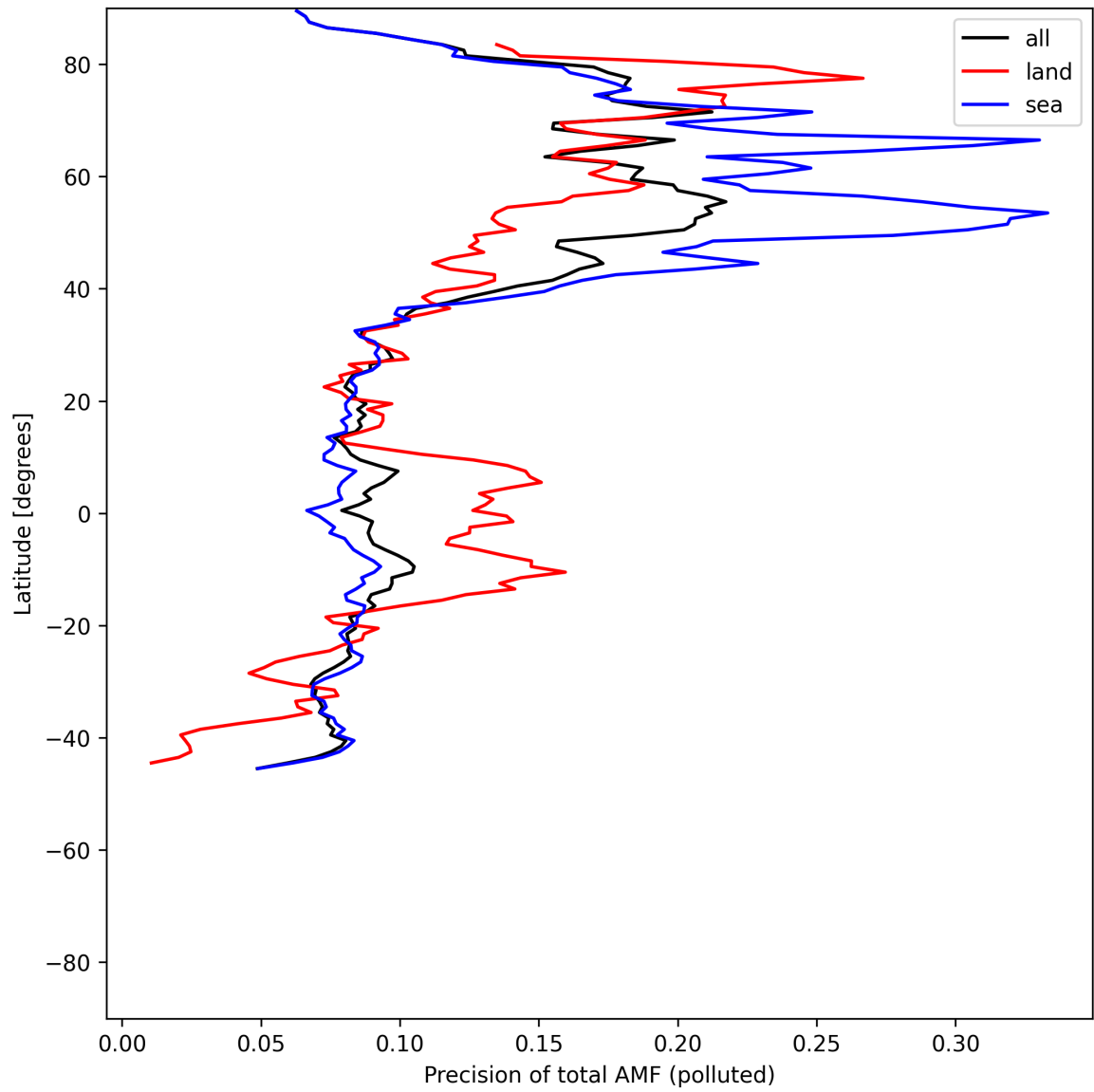
Figure 54: Zonal average of “Precision of total AMF (polluted)” for 2025-06-14 to 2025-06-14.
