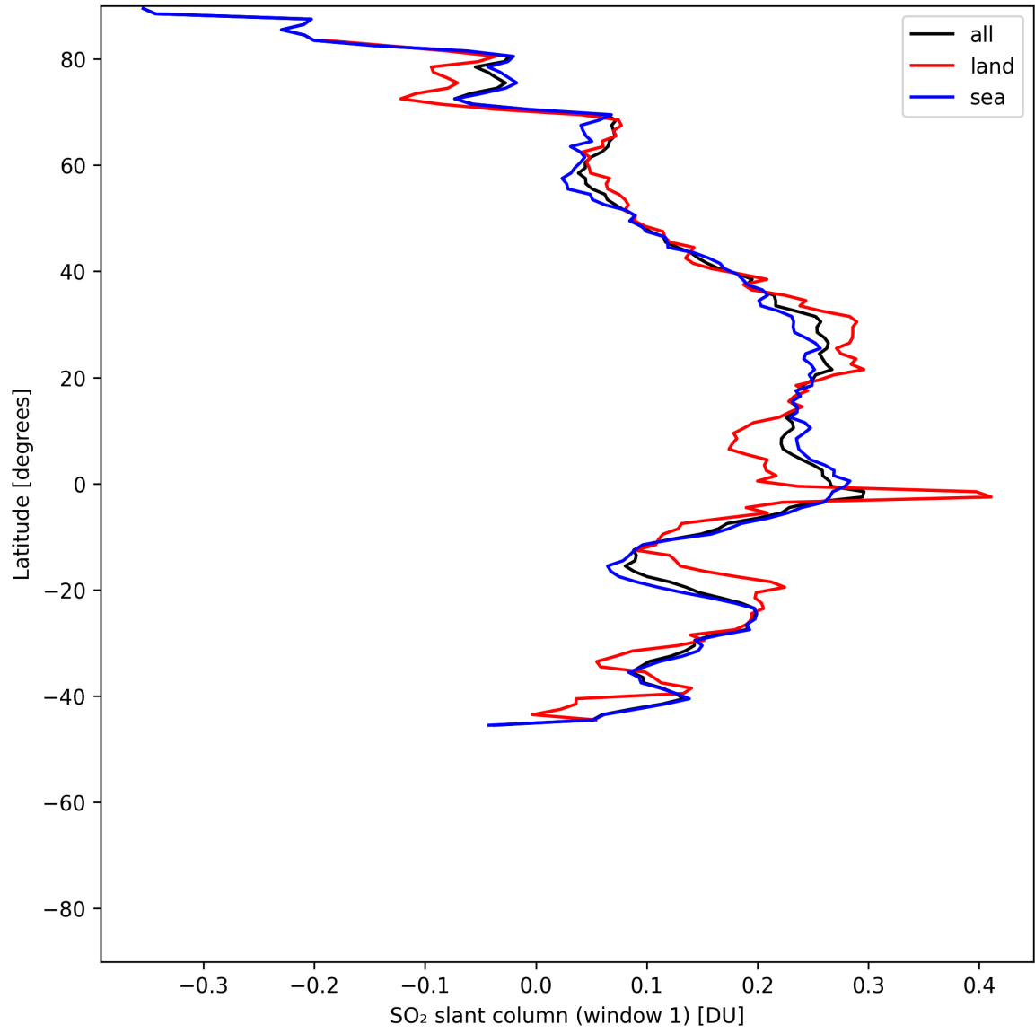
Figure 36: Zonal average of “SO 2 slant column (window 1)” for 2025-06-14 to 2025-06-14.
