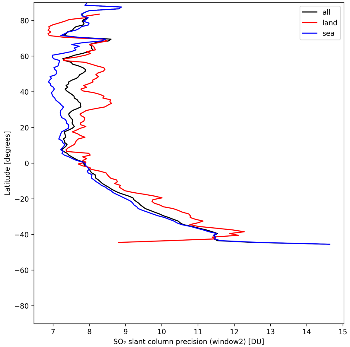
Figure 41: Zonal average of “SO 2 slant column precision (window2)” for 2025-06-14 to 2025-06-14.
