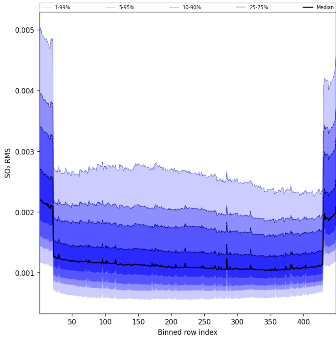
Figure 106: Along track statistics of “SO 2 RMS” for 2025-06-14 to 2025-06-14
