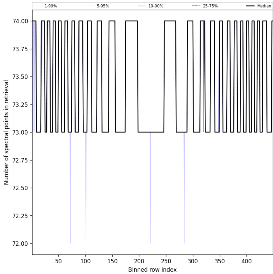
Figure 110: Along track statistics of “Number of spectral points in retrieval” for 2025-06-14 to 2025-06-14
