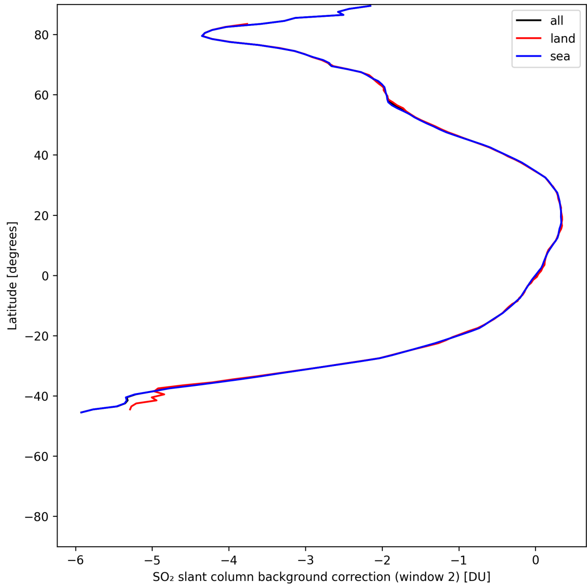
Figure 43: Zonal average of “SO 2 slant column background correction (window 2)” for 2025-06-14 to 2025-06-14.
