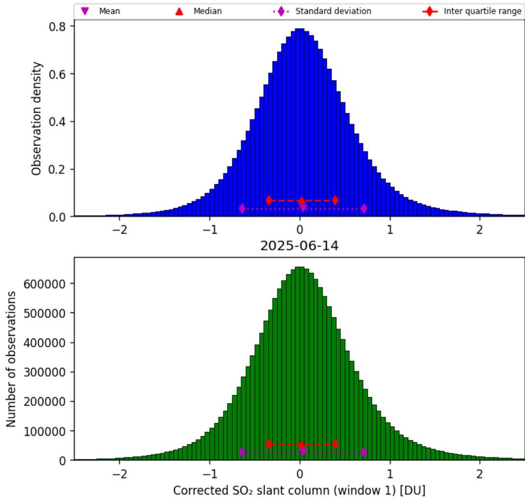
Figure 65: Histogram of “Corrected SO 2 slant column (window 1)” for 2025-06-14 to 2025-06-14
