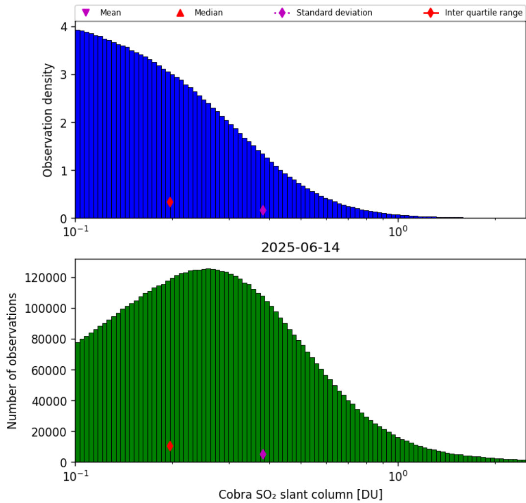
Figure 61: Histogram of “Cobra SO 2 slant column” for 2025-06-14 to 2025-06-14
