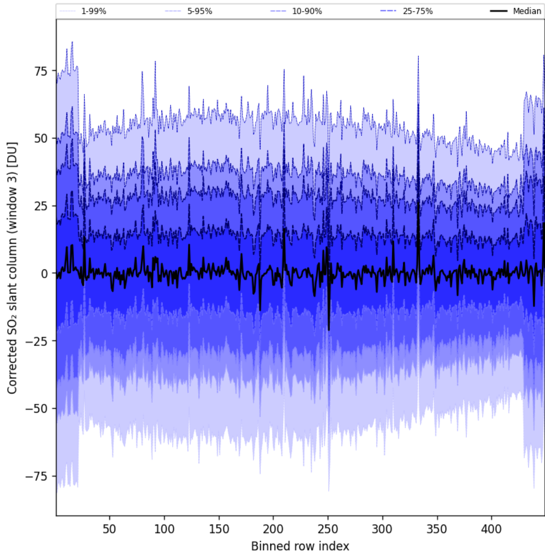
Figure 100: Along track statistics of “Corrected SO 2 slant column (window 3)” for 2025-06-14 to 2025-06-14
