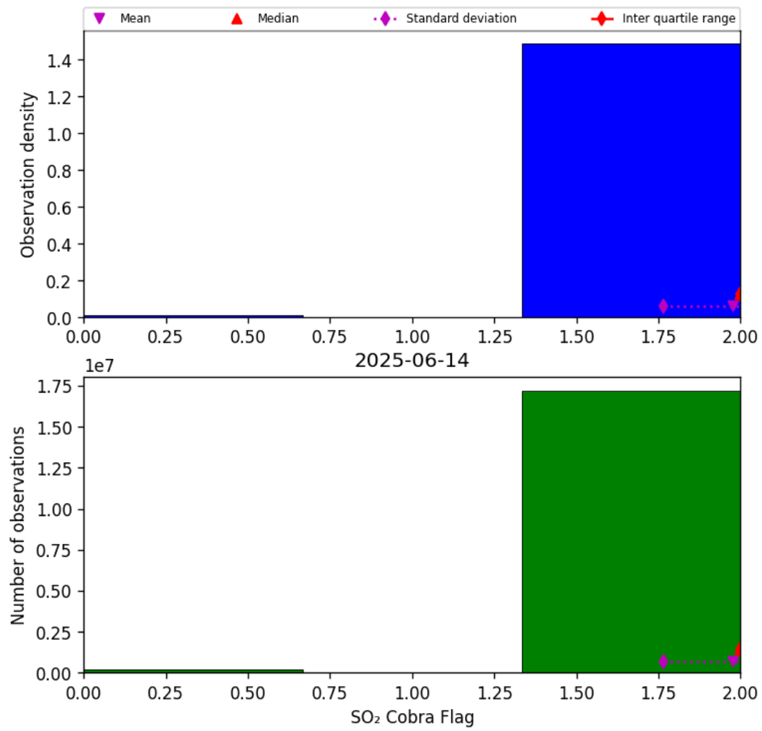
Figure 75: Histogram of “SO 2 Cobra Flag” for 2025-06-14 to 2025-06-14
