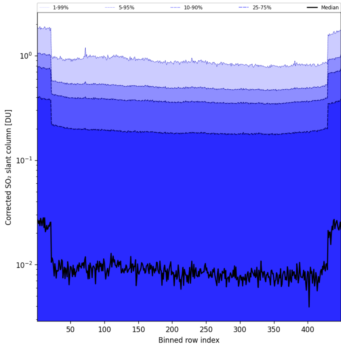
Figure 87: Along track statistics of “Corrected SO 2 slant column” for 2025-06-14 to 2025-06-14
