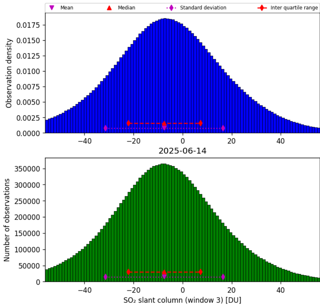
Figure 71: Histogram of “SO 2 slant column (window 3)” for 2025-06-14 to 2025-06-14
