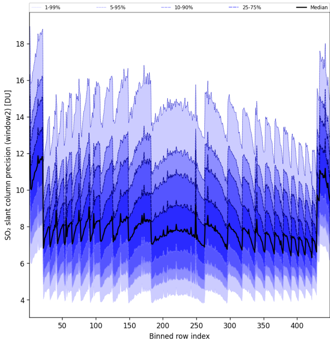
Figure 95: Along track statistics of “SO 2 slant column precision (window2)” for 2025-06-14 to 2025-06-14
