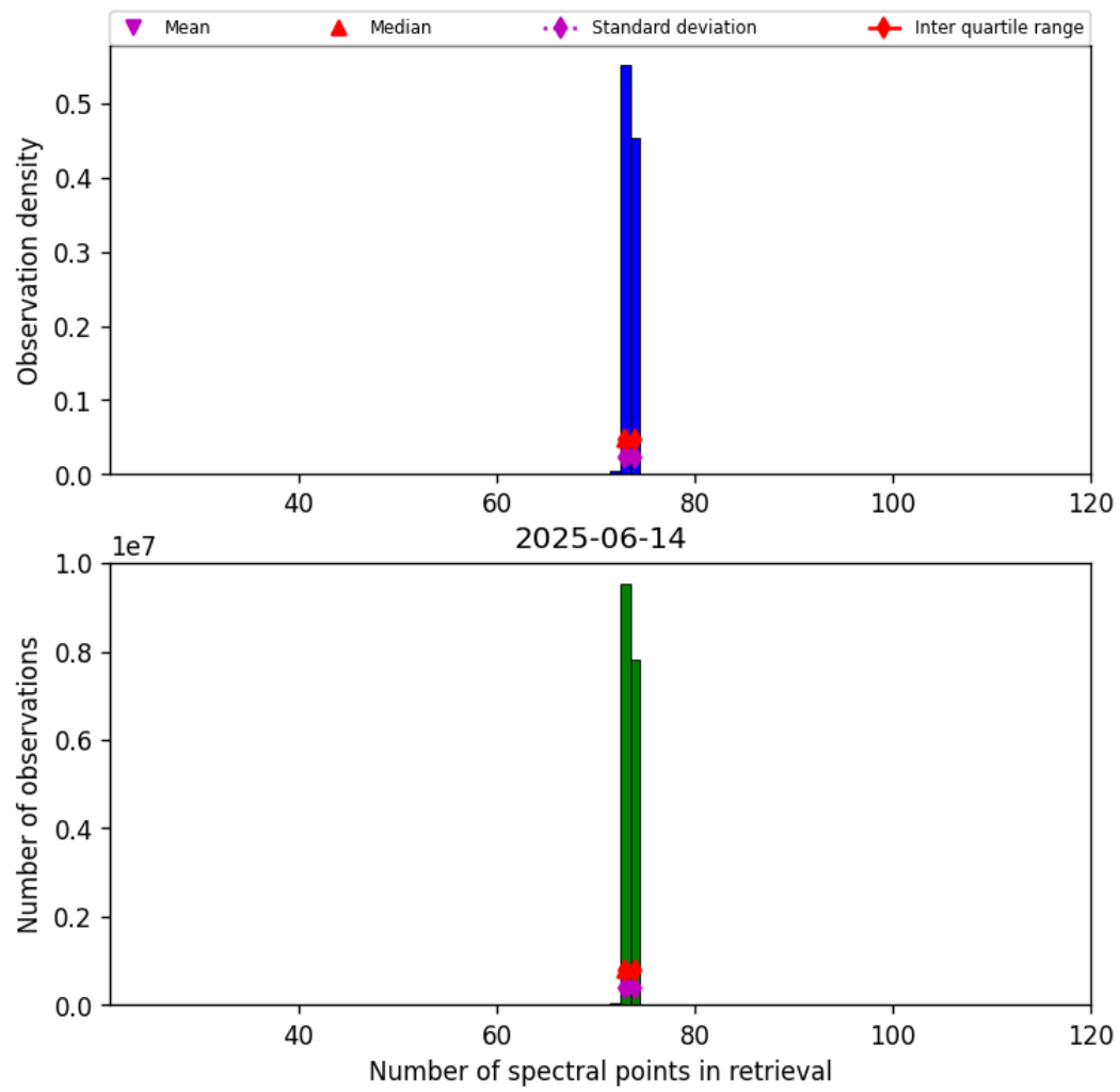
Figure 83: Histogram of “Number of spectral points in retrieval” for 2025-06-14 to 2025-06-14
