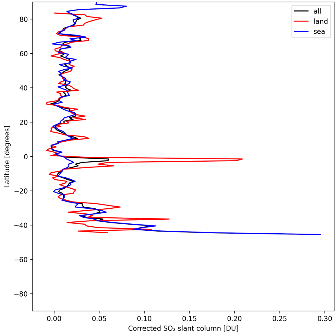
Figure 33: Zonal average of “Corrected SO 2 slant column” for 2025-06-14 to 2025-06-14.
