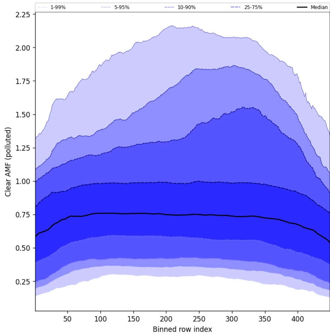
Figure 109: Along track statistics of “Clear AMF (polluted)” for 2025-06-14 to 2025-06-14
