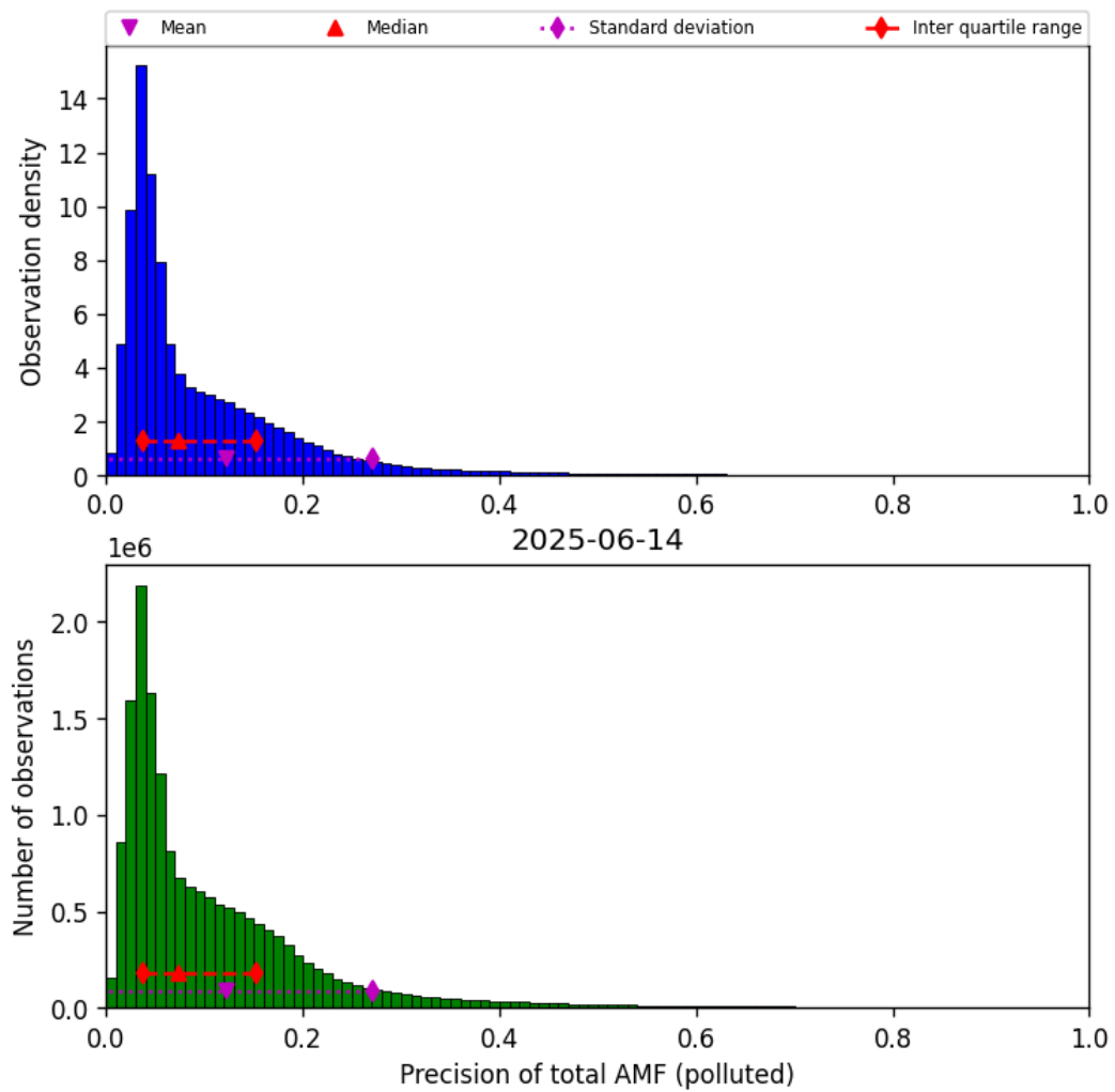
Figure 81: Histogram of “Precision of total AMF (polluted)” for 2025-06-14 to 2025-06-14
