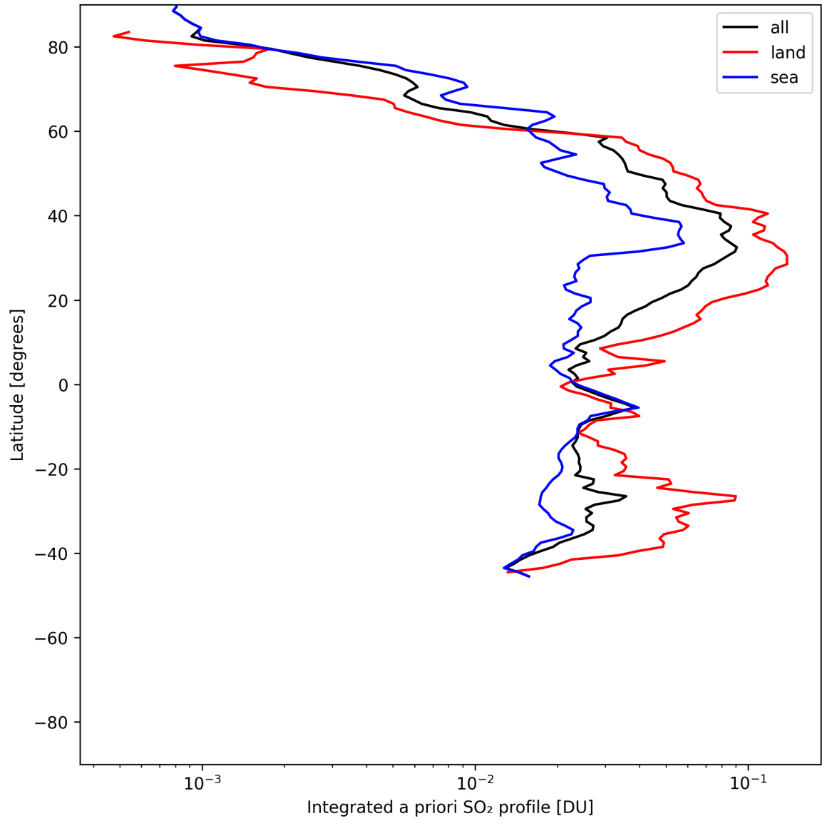
Figure 49: Zonal average of “Integrated a priori SO 2 profile” for 2025-06-14 to 2025-06-14.
