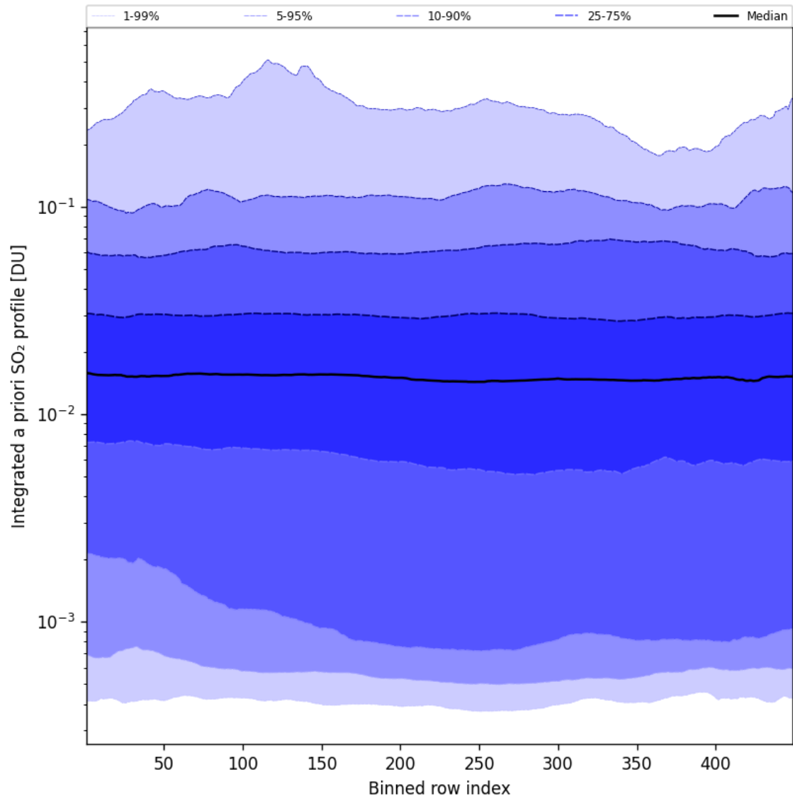
Figure 103: Along track statistics of “Integrated a priori SO 2 profile” for 2025-06-14 to 2025-06-14
