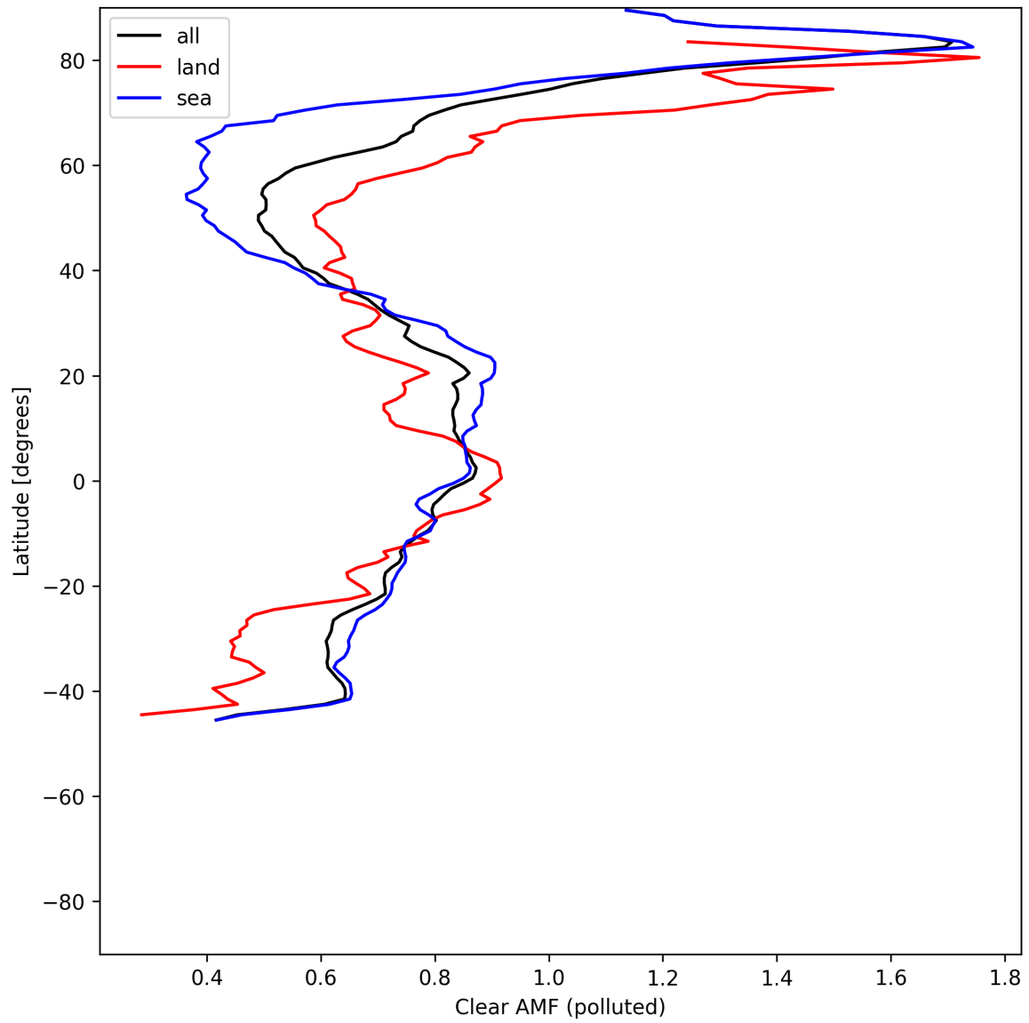
Figure 55: Zonal average of “Clear AMF (polluted)” for 2025-06-14 to 2025-06-14.
