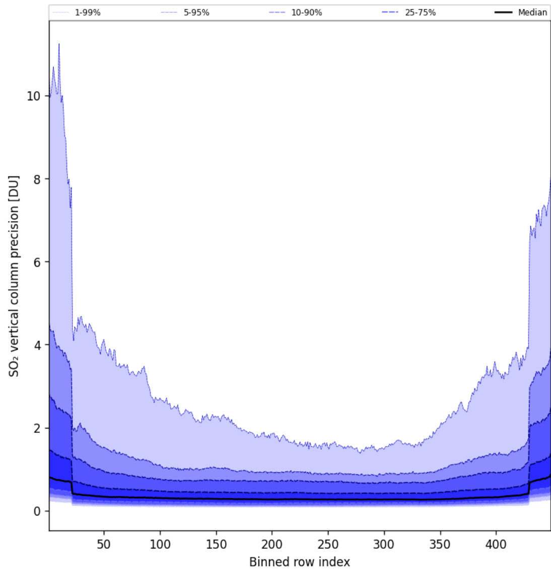
Figure 86: Along track statistics of “SO 2 vertical column precision” for 2025-06-14 to 2025-06-14
