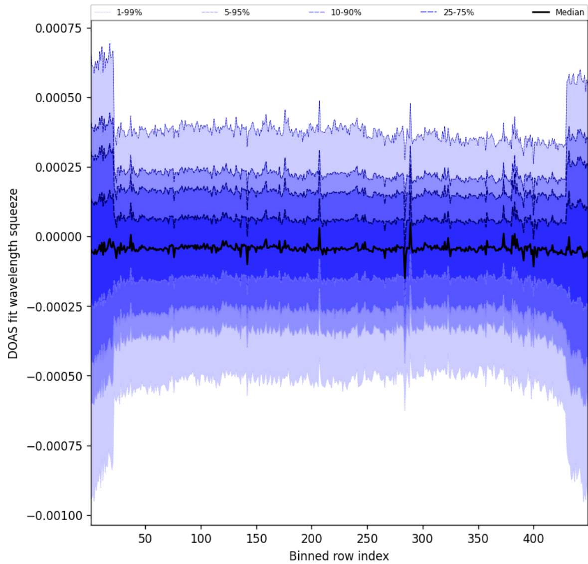
Figure 105: Along track statistics of “DOAS fit wavelength squeeze” for 2025-06-14 to 2025-06-14
