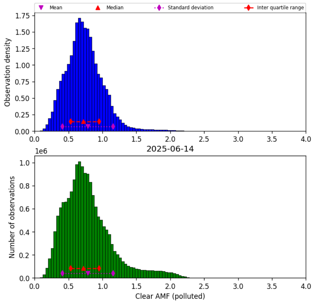
Figure 82: Histogram of “Clear AMF (polluted)” for 2025-06-14 to 2025-06-14
