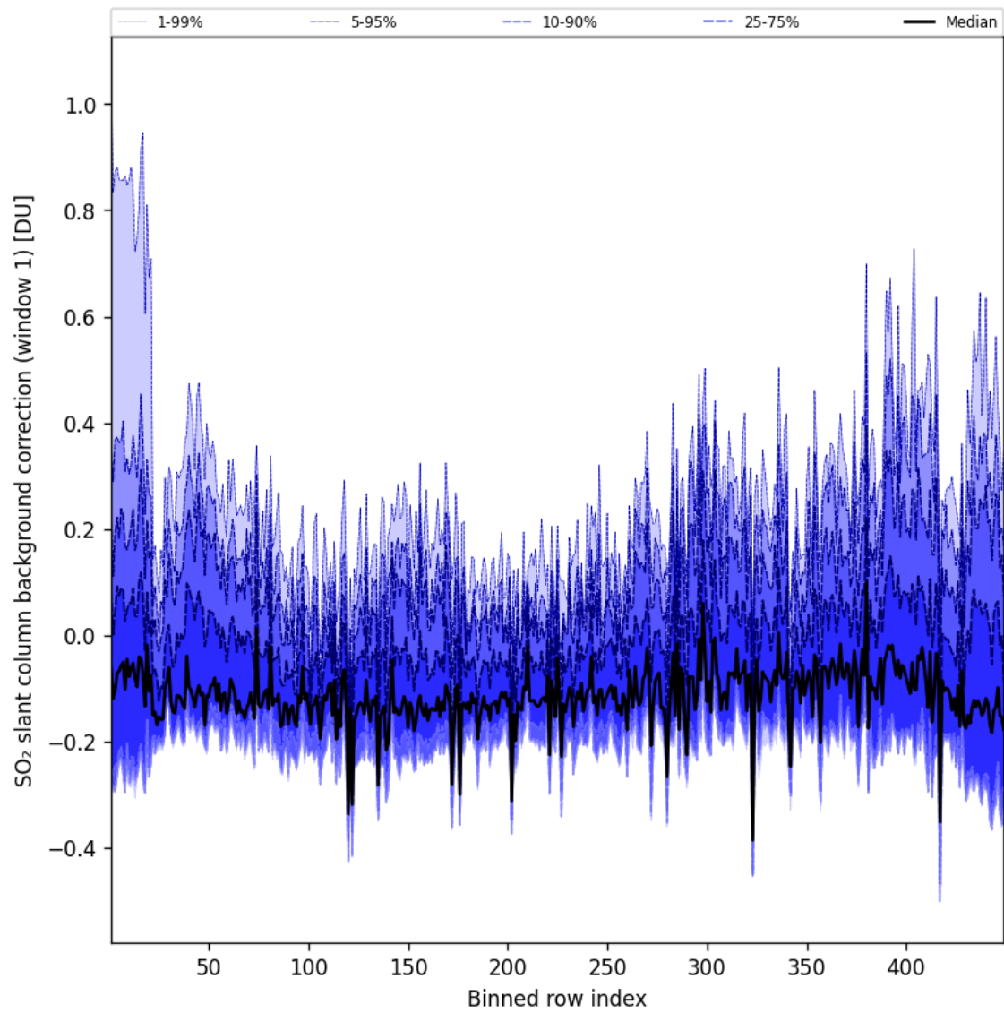
Figure 93: Along track statistics of “SO 2 slant column background correction (window 1)” for 2025-06-14 to 2025-06-14
