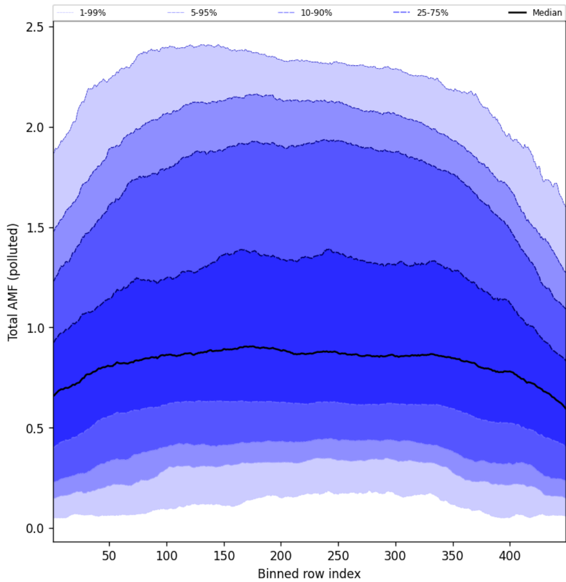
Figure 107: Along track statistics of “Total AMF (polluted)” for 2025-06-14 to 2025-06-14
