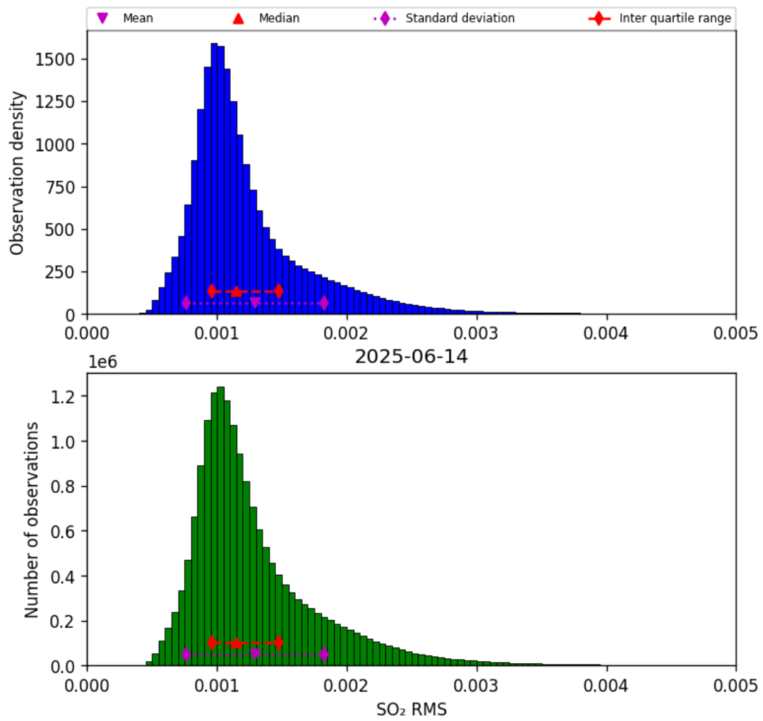
Figure 79: Histogram of “SO 2 RMS” for 2025-06-14 to 2025-06-14
