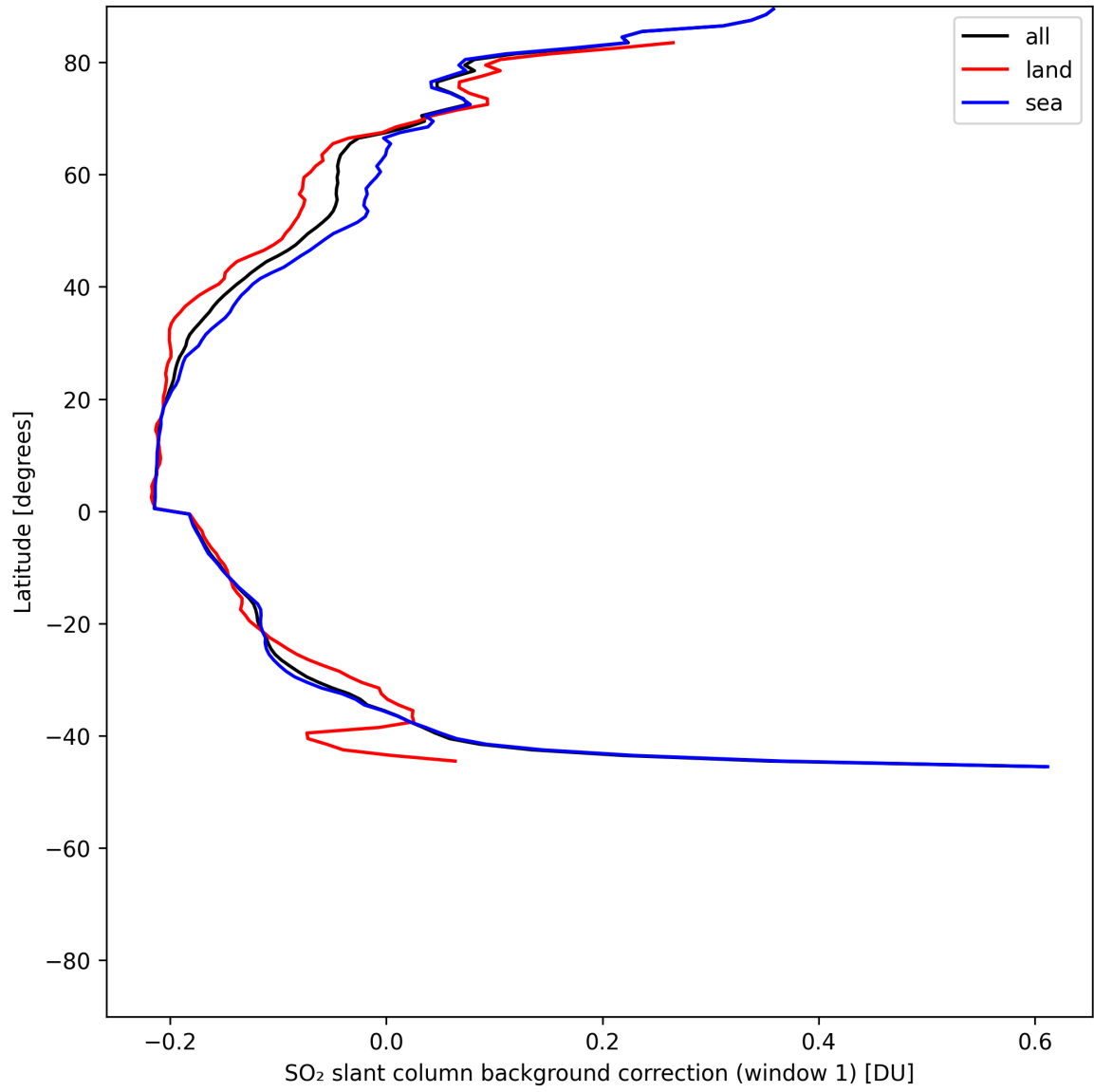
Figure 39: Zonal average of "SO 2 slant column background correction (window 1)" for 2025-06-14 to 2025-06-14.
