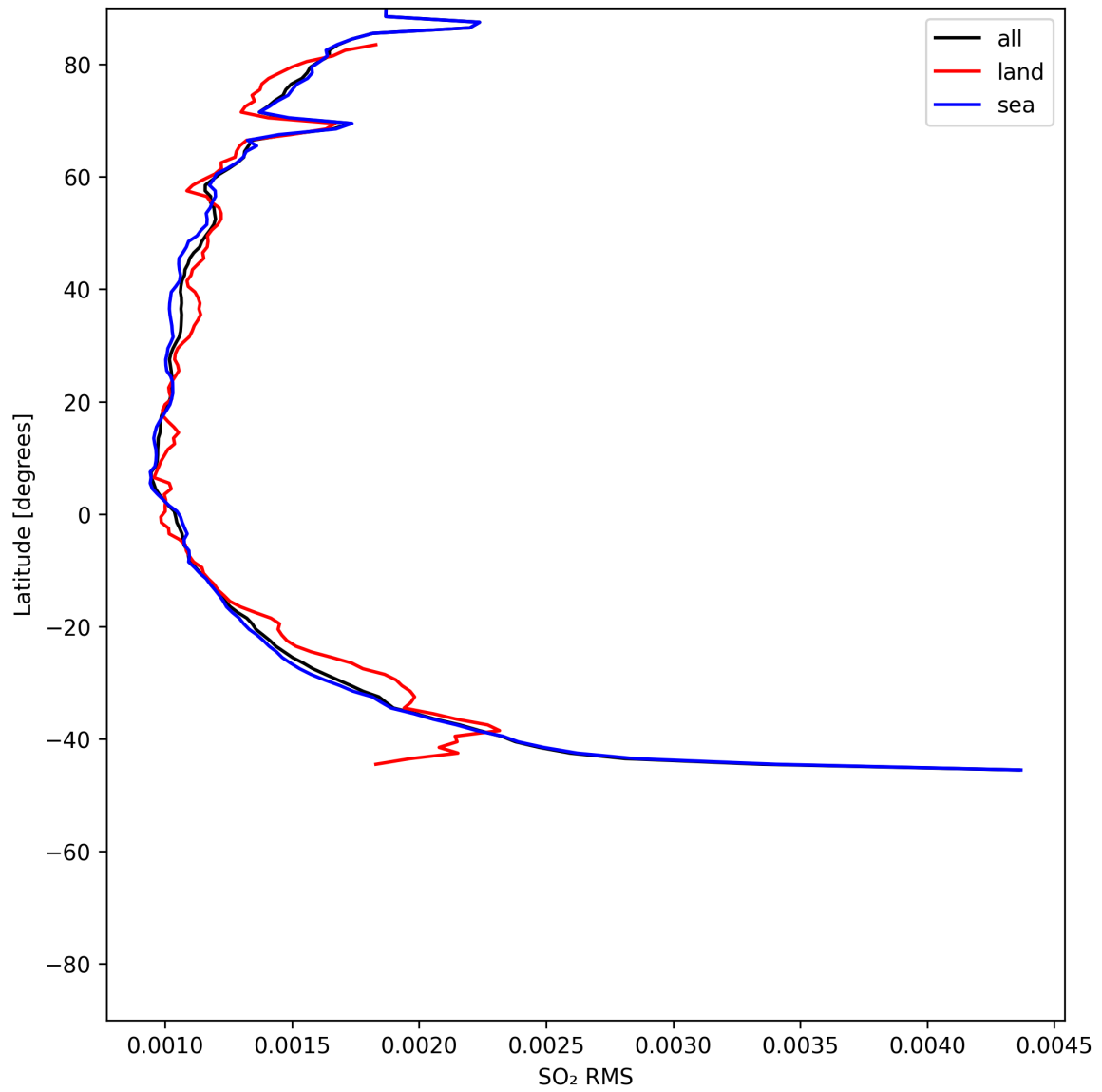
Figure 52: Zonal average of “SO 2 RMS” for 2025-06-14 to 2025-06-14.
