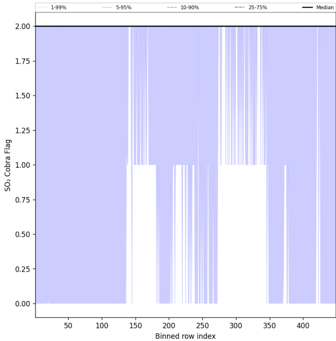
Figure 102: Along track statistics of “SO 2 Cobra Flag” for 2025-06-14 to 2025-06-14
