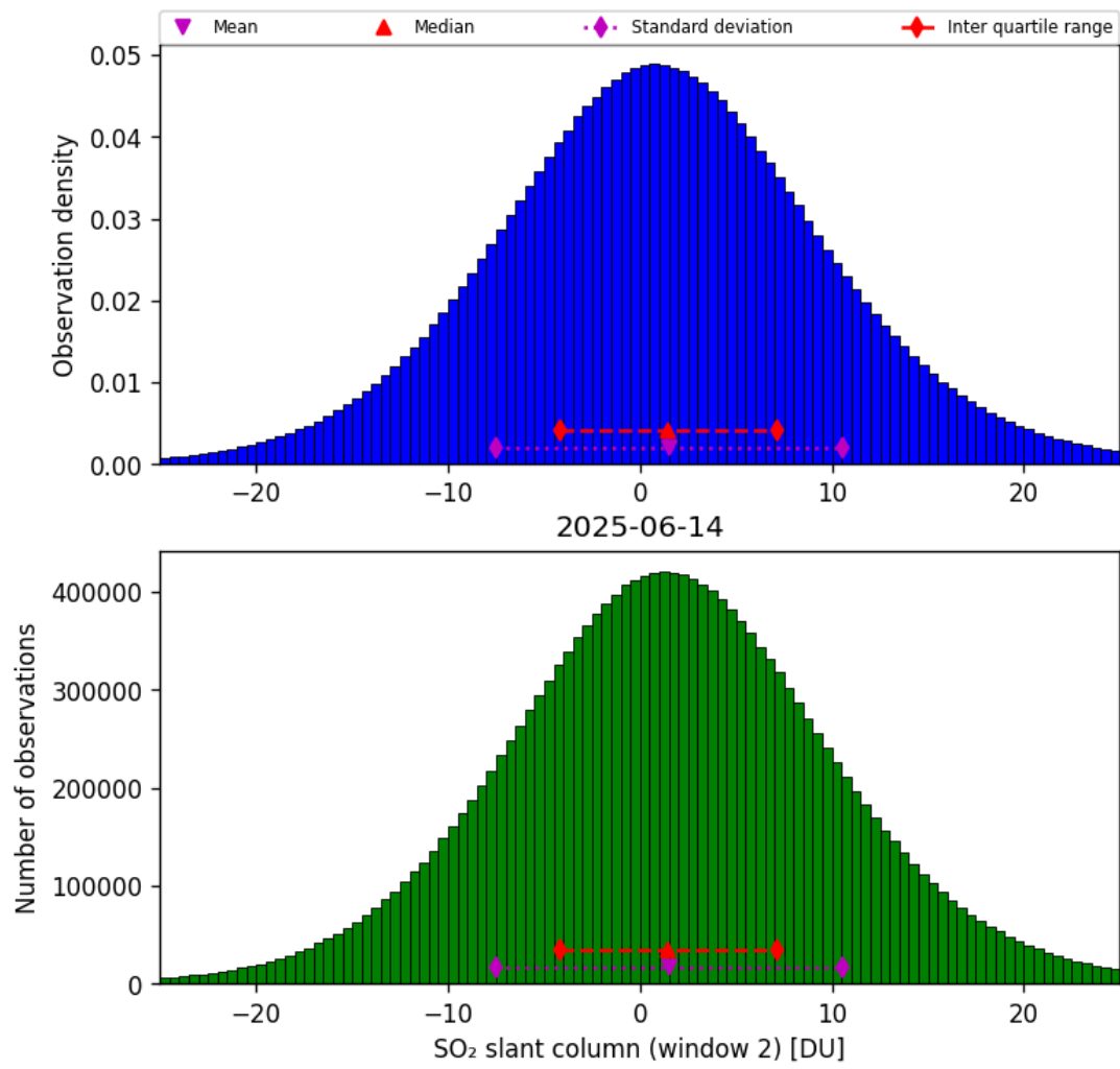
Figure 67: Histogram of “SO 2 slant column (window 2)” for 2025-06-14 to 2025-06-14
