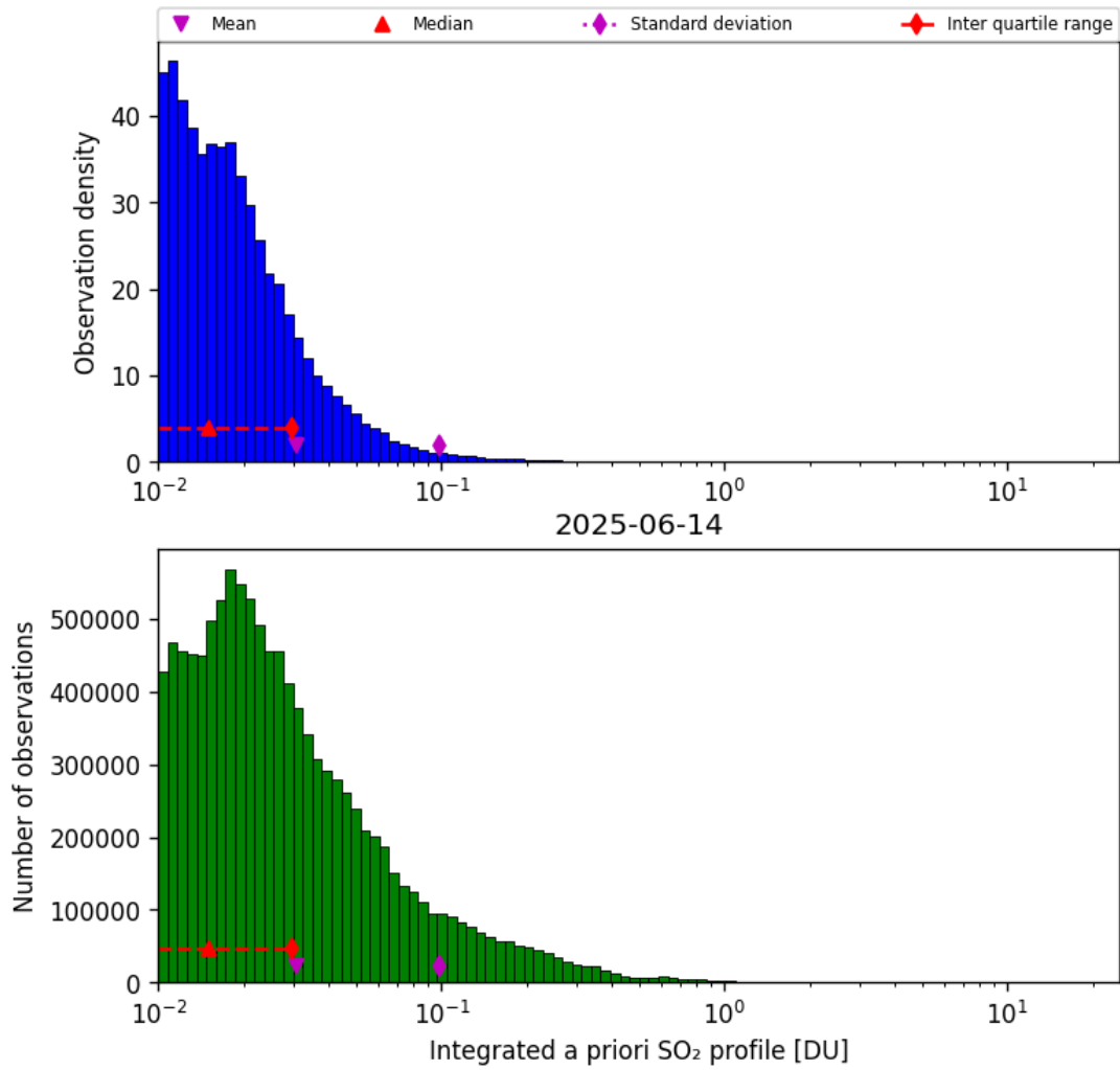
Figure 76: Histogram of “Integrated a priori SO 2 profile” for 2025-06-14 to 2025-06-14
