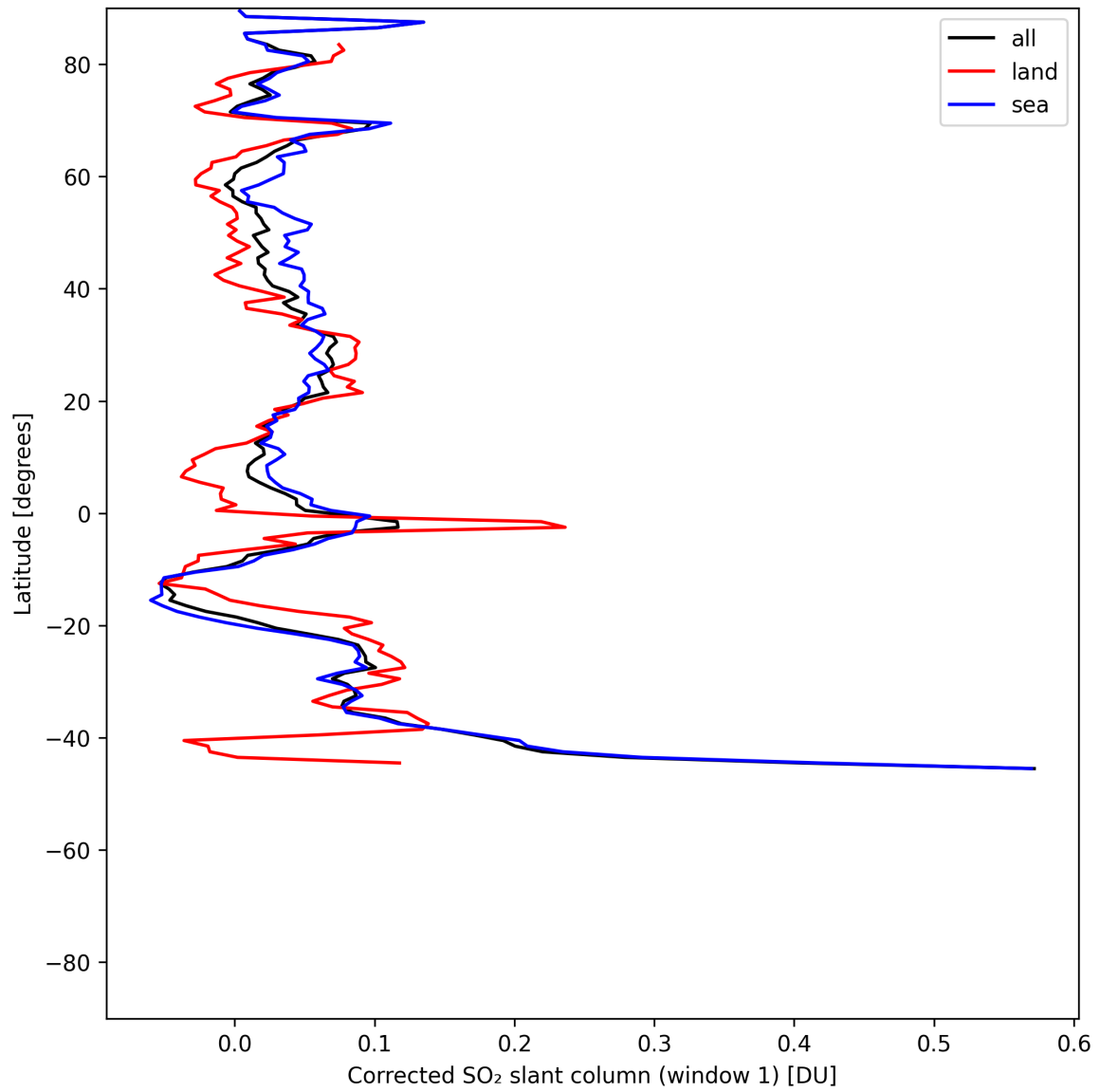
Figure 38: Zonal average of “Corrected SO 2 slant column (window 1)” for 2025-06-14 to 2025-06-14.
