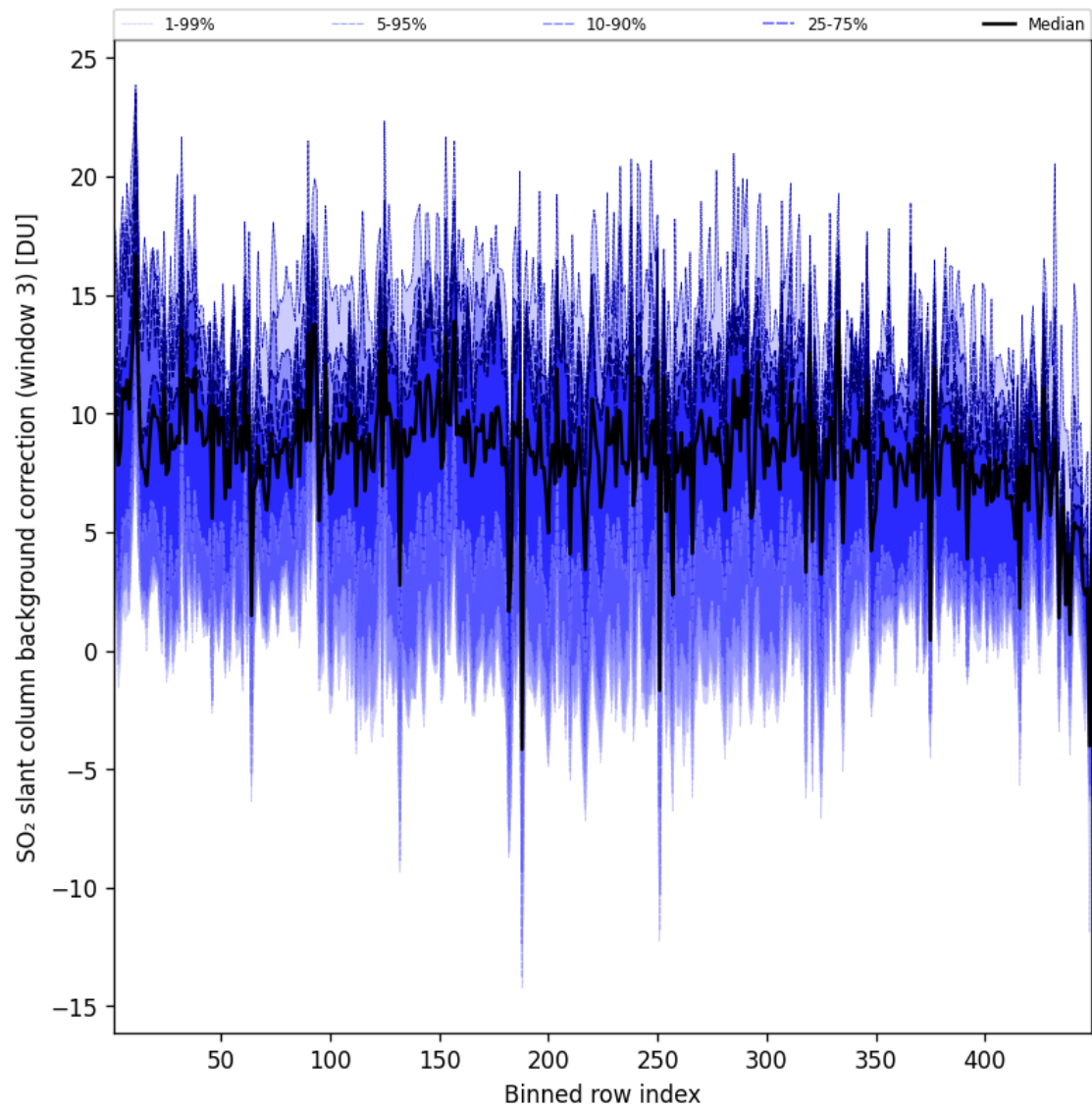
Figure 101: Along track statistics of “SO 2 slant column background correction (window 3)” for 2025-06-14 to 2025-06-14
