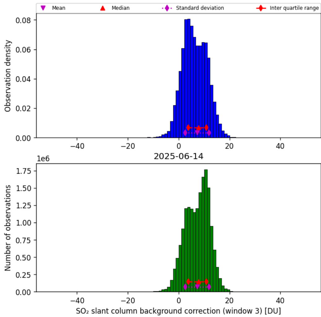
Figure 74: Histogram of “SO 2 slant column background correction (window 3)” for 2025-06-14 to 2025-06-14
