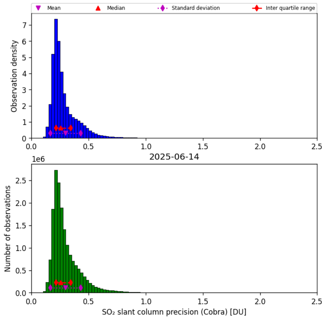
Figure 62: Histogram of “SO 2 slant column precision (Cobra)” for 2025-06-14 to 2025-06-14
