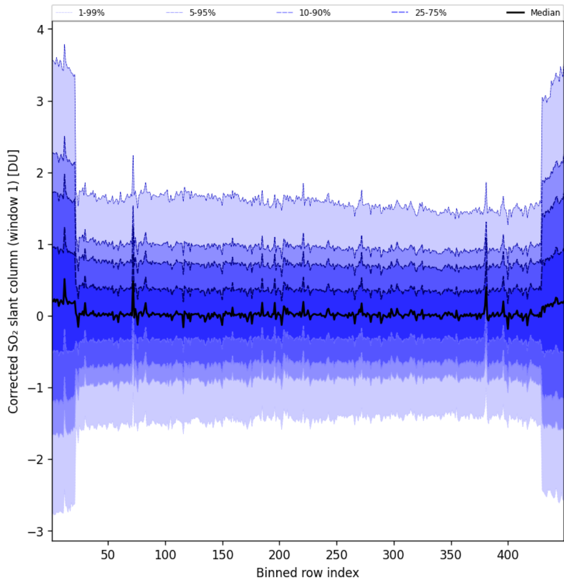
Figure 92: Along track statistics of “Corrected SO 2 slant column (window 1)” for 2025-06-14 to 2025-06-14
