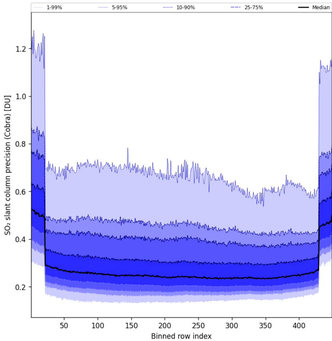
Figure 89: Along track statistics of “SO 2 slant column precision (Cobra)” for 2025-06-14 to 2025-06-14
