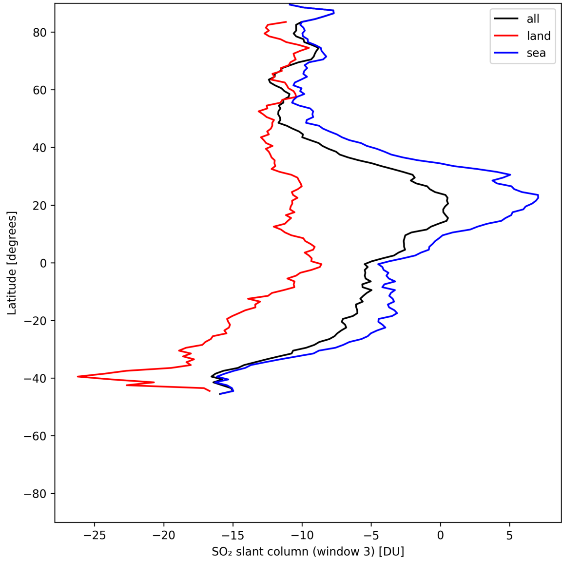
Figure 44: Zonal average of “SO 2 slant column (window 3)” for 2025-06-14 to 2025-06-14.
