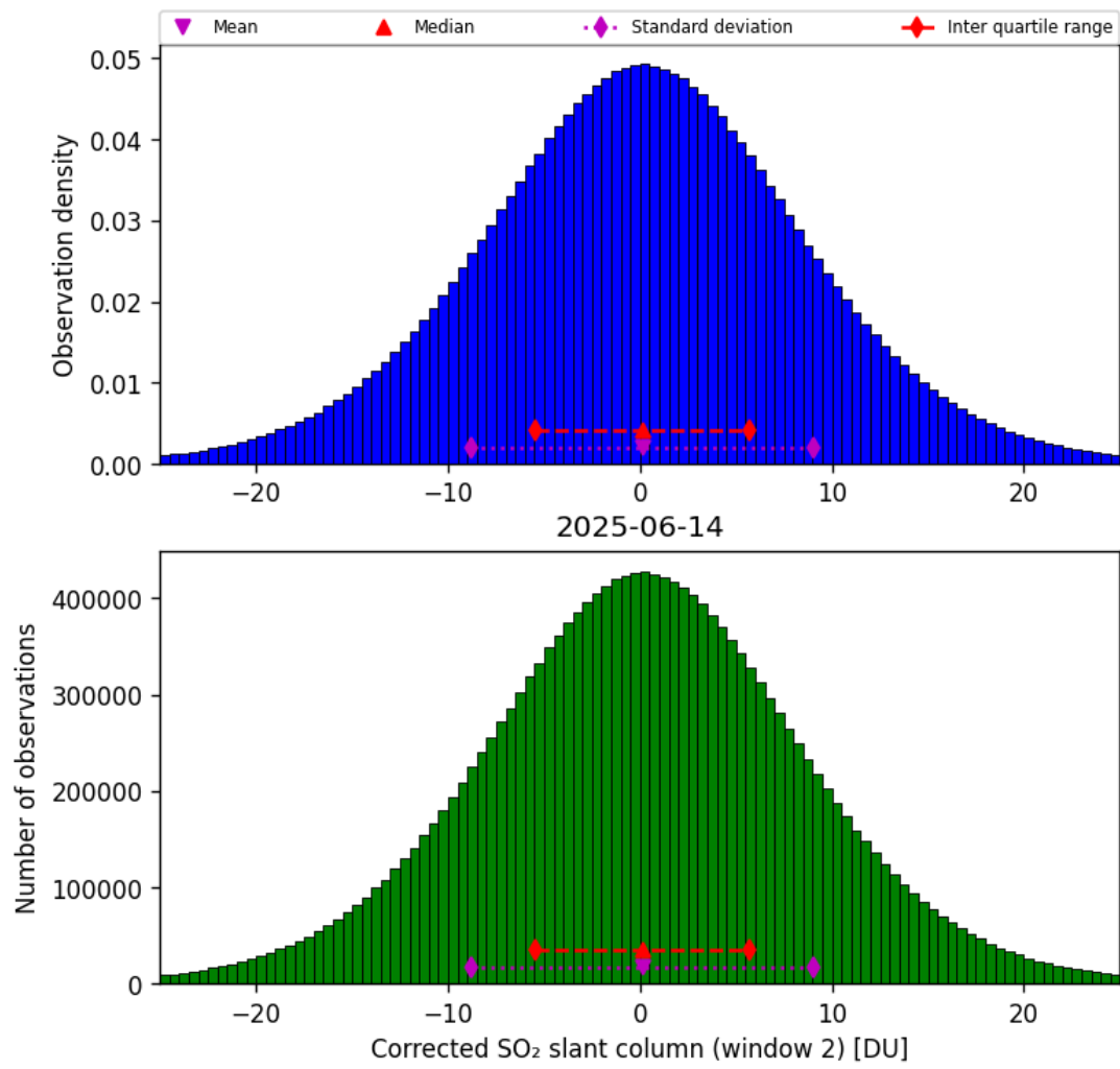
Figure 69: Histogram of “Corrected SO 2 slant column (window 2)” for 2025-06-14 to 2025-06-14
