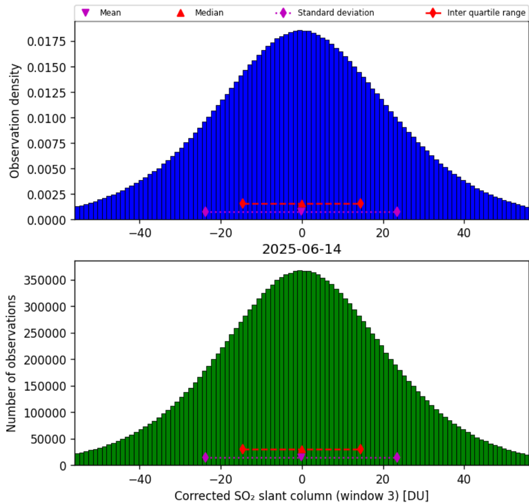
Figure 73: Histogram of “Corrected SO 2 slant column (window 3)” for 2025-06-14 to 2025-06-14
