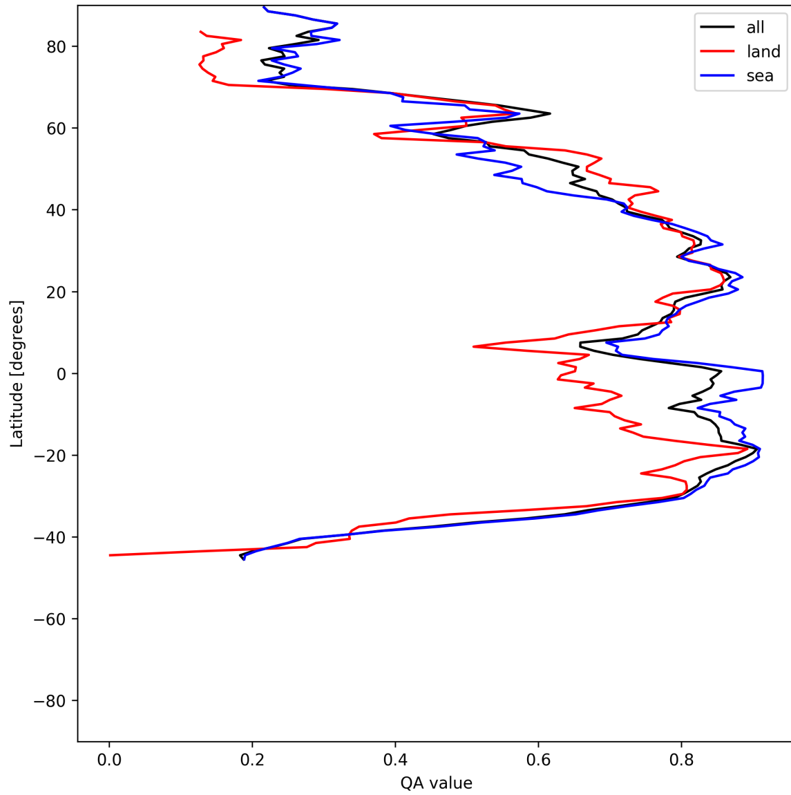
Figure 30: Zonal average of “QA value” for 2025-06-14 to 2025-06-14.
