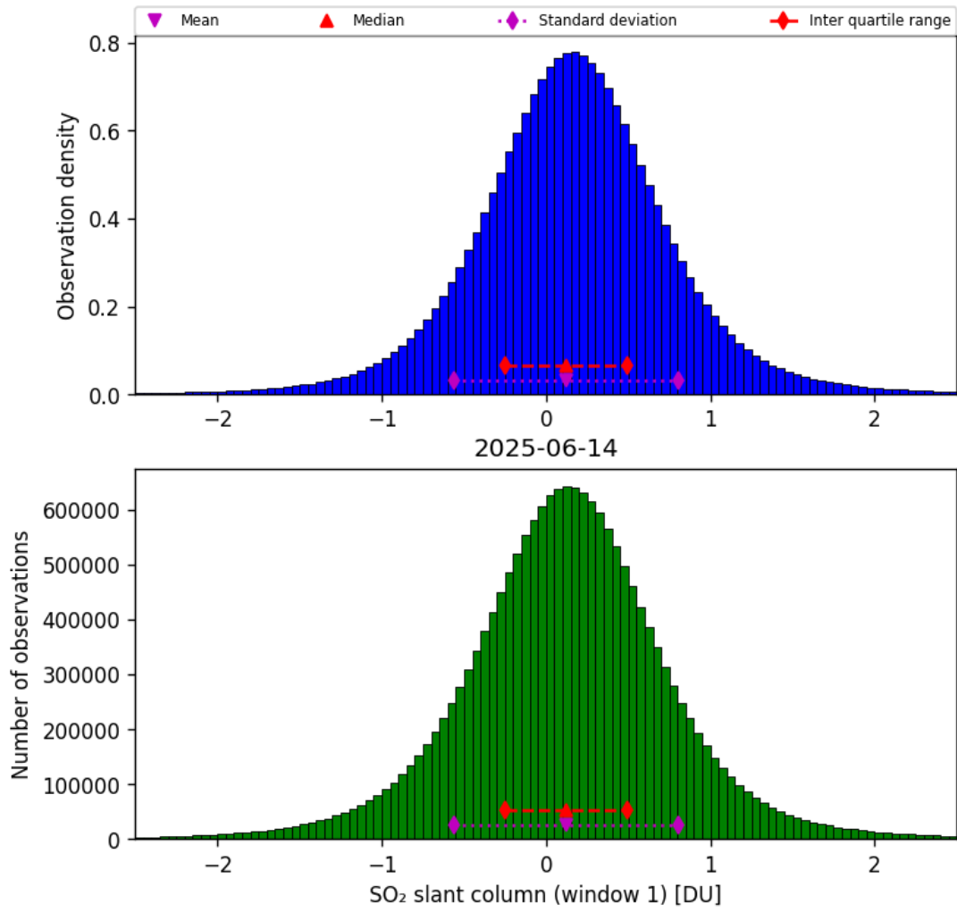
Figure 63: Histogram of “SO 2 slant column (window 1)” for 2025-06-14 to 2025-06-14
