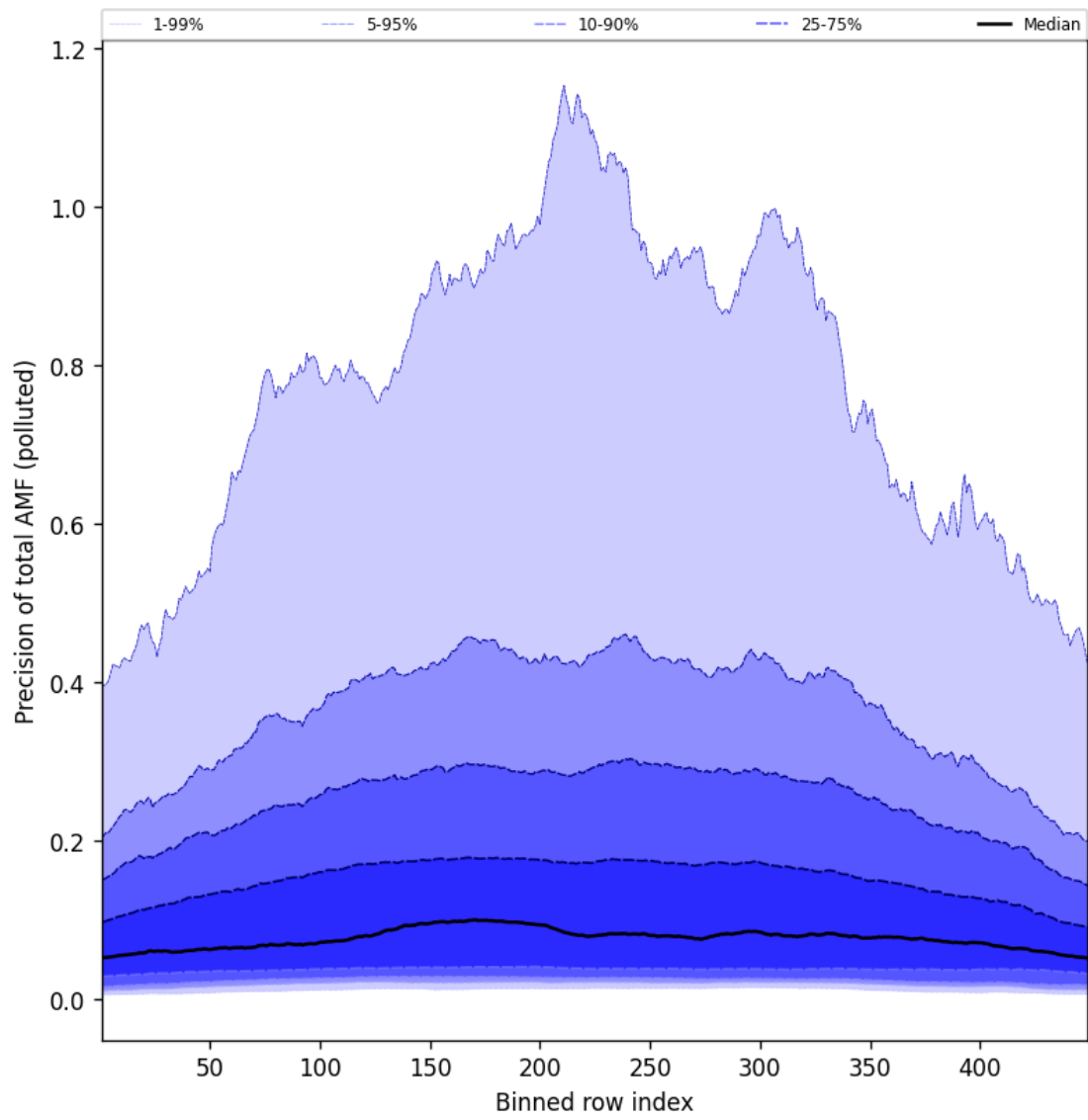
Figure 108: Along track statistics of “Precision of total AMF (polluted)” for 2025-06-14 to 2025-06-14
