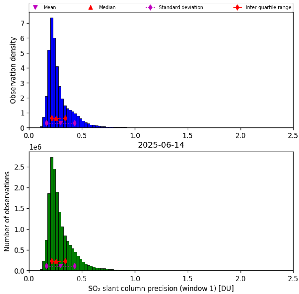
Figure 64: Histogram of “SO 2 slant column precision (window 1)” for 2025-06-14 to 2025-06-14
