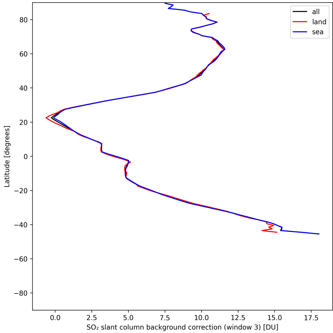
Figure 47: Zonal average of “SO 2 slant column background correction (window 3)” for 2025-06-14 to 2025-06-14.
