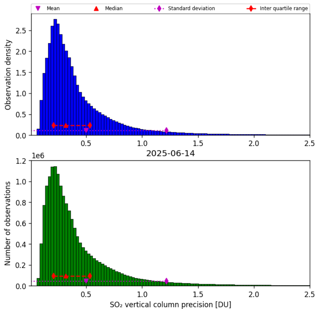
Figure 59: Histogram of “SO 2 vertical column precision” for 2025-06-14 to 2025-06-14
