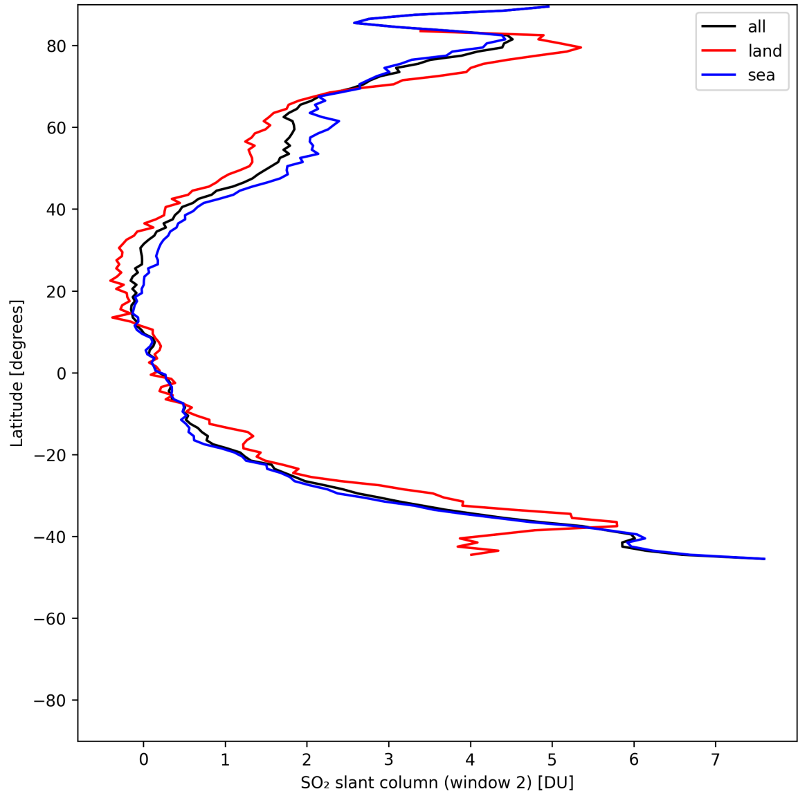
Figure 40: Zonal average of “SO 2 slant column (window 2)” for 2025-06-14 to 2025-06-14.
