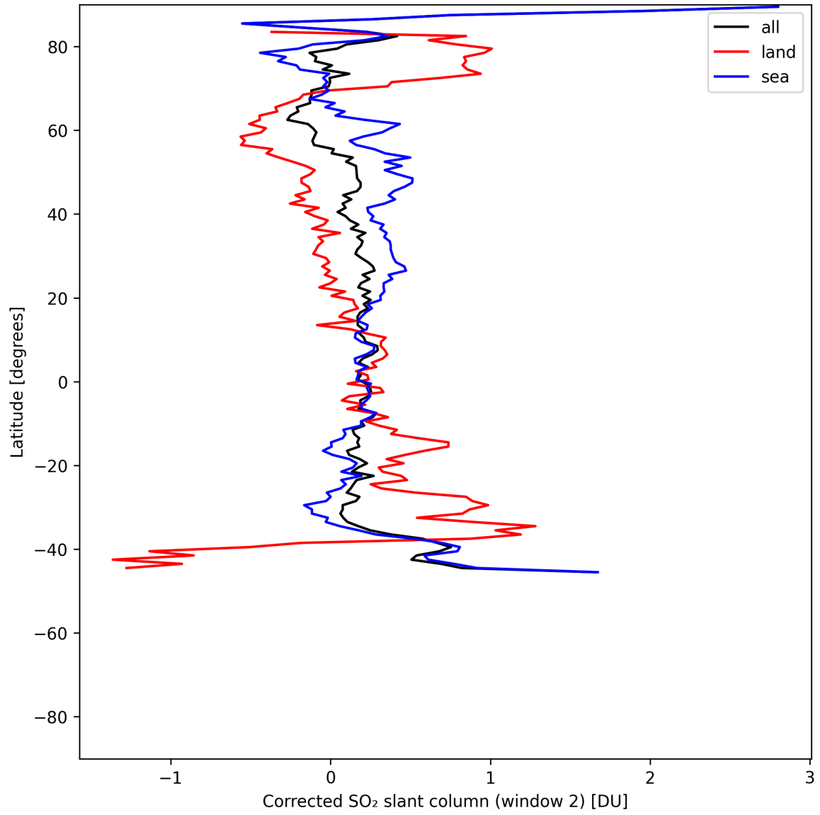
Figure 42: Zonal average of “Corrected SO 2 slant column (window 2)” for 2025-06-14 to 2025-06-14.
