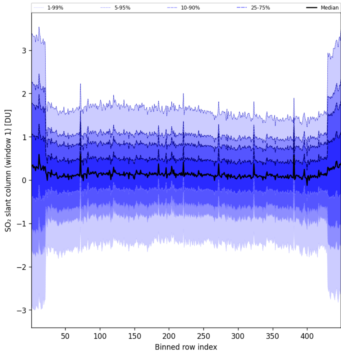
Figure 90: Along track statistics of “SO 2 slant column (window 1)” for 2025-06-14 to 2025-06-14
