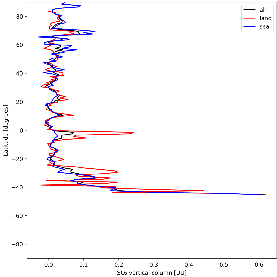
Figure 31: Zonal average of “SO 2 vertical column” for 2025-06-14 to 2025-06-14.
