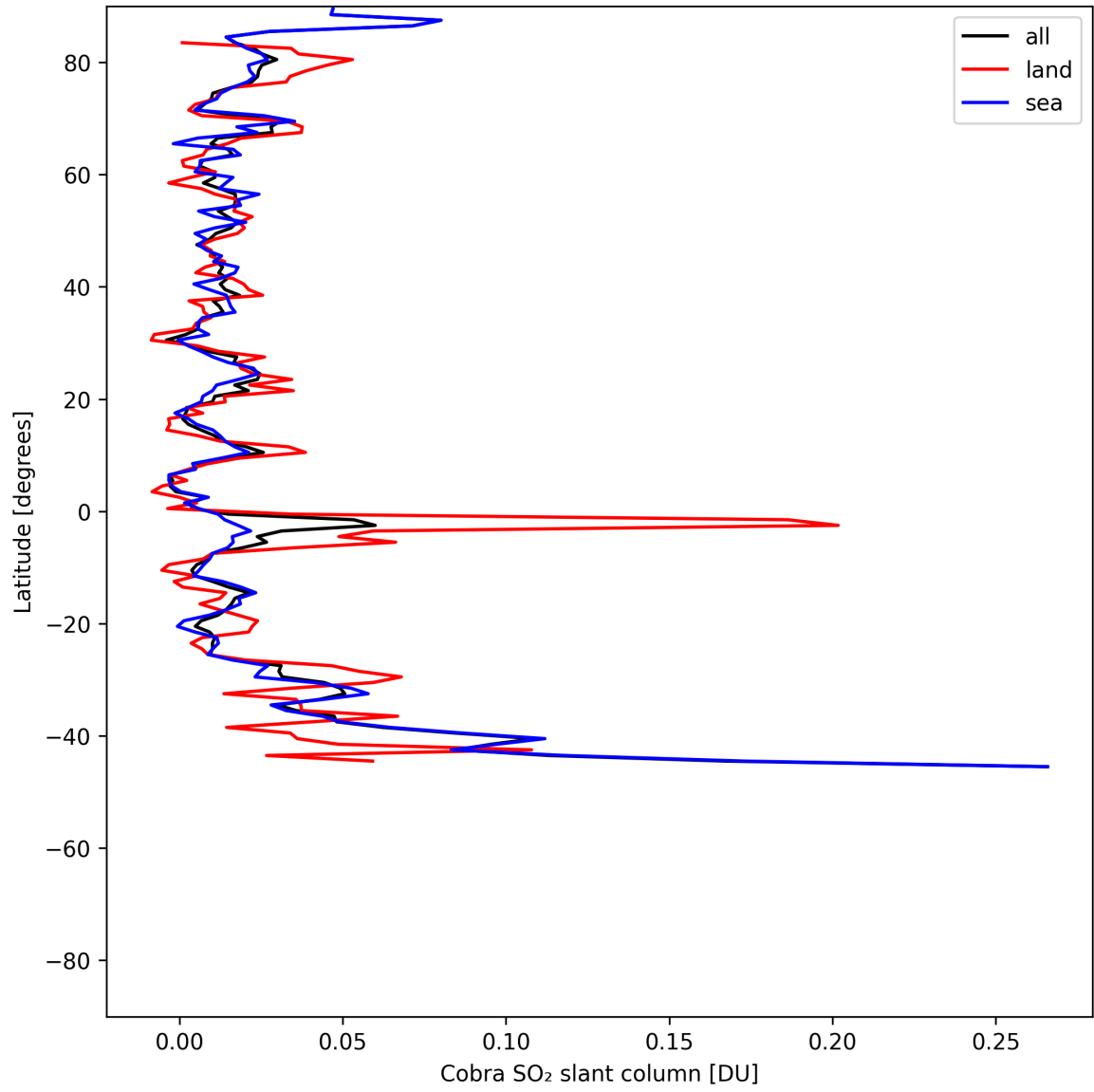
Figure 34: Zonal average of “Cobra SO 2 slant column” for 2025-06-14 to 2025-06-14.
