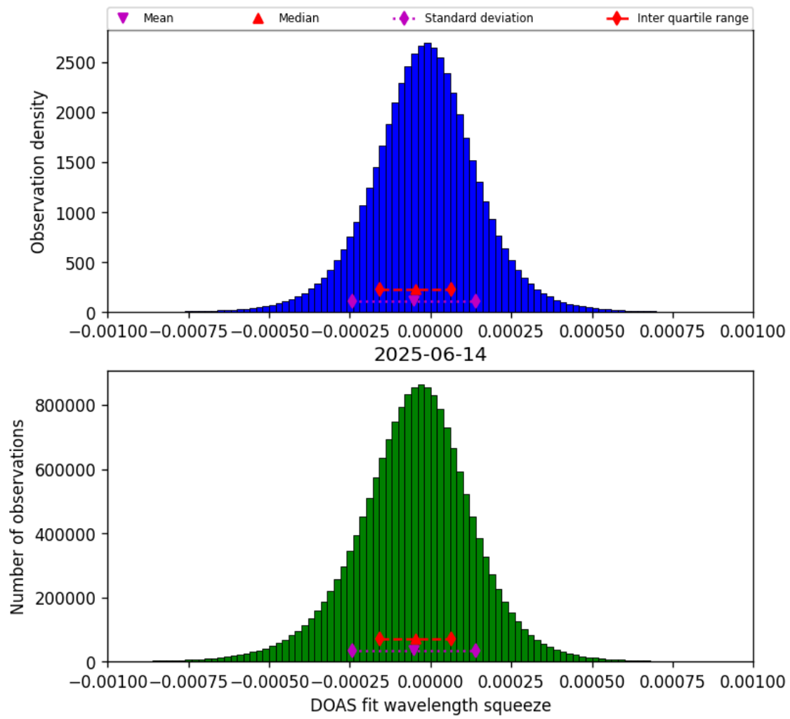
Figure 78: Histogram of “DOAS fit wavelength squeeze” for 2025-06-14 to 2025-06-14
