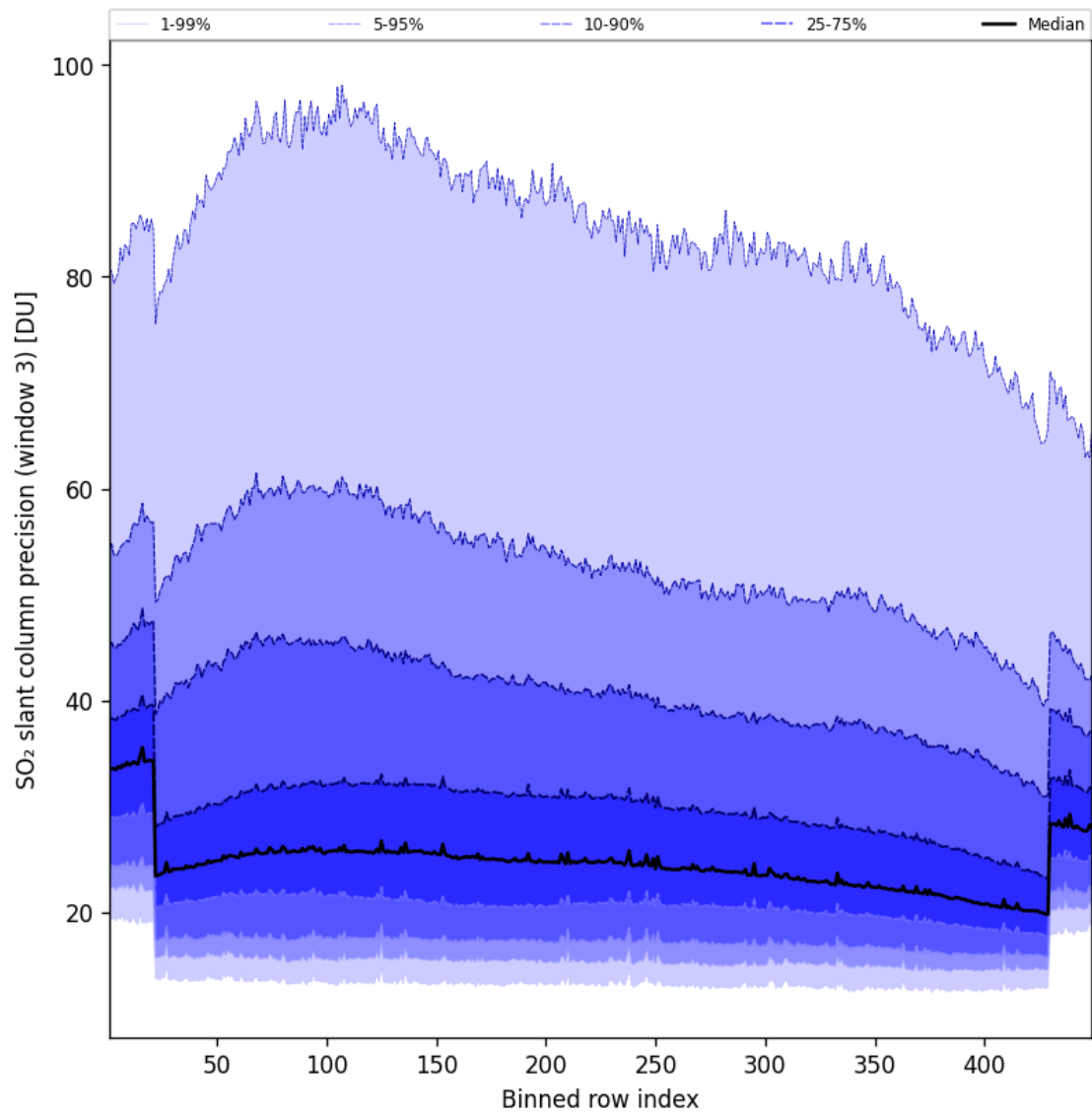
Figure 99: Along track statistics of “SO 2 slant column precision (window 3)” for 2025-06-14 to 2025-06-14
