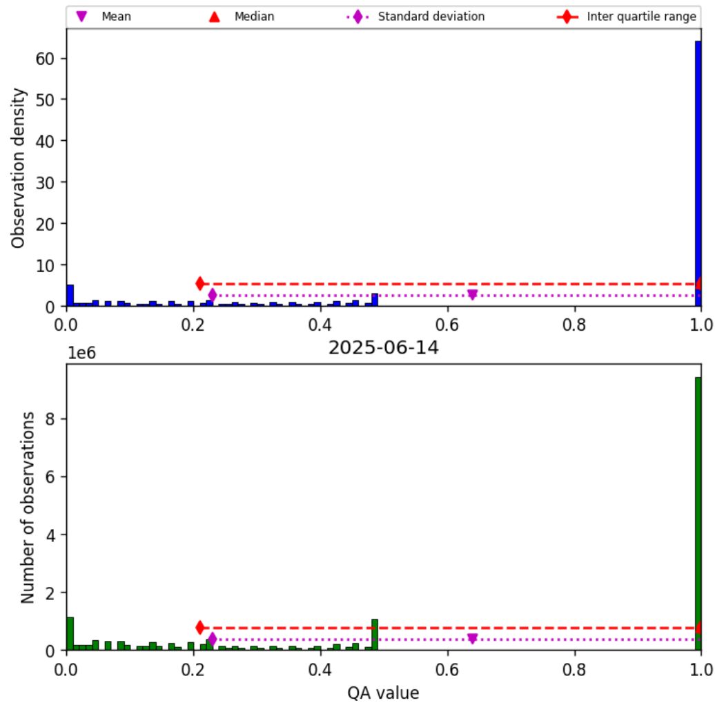
Figure 57: Histogram of “QA value” for 2025-06-14 to 2025-06-14
