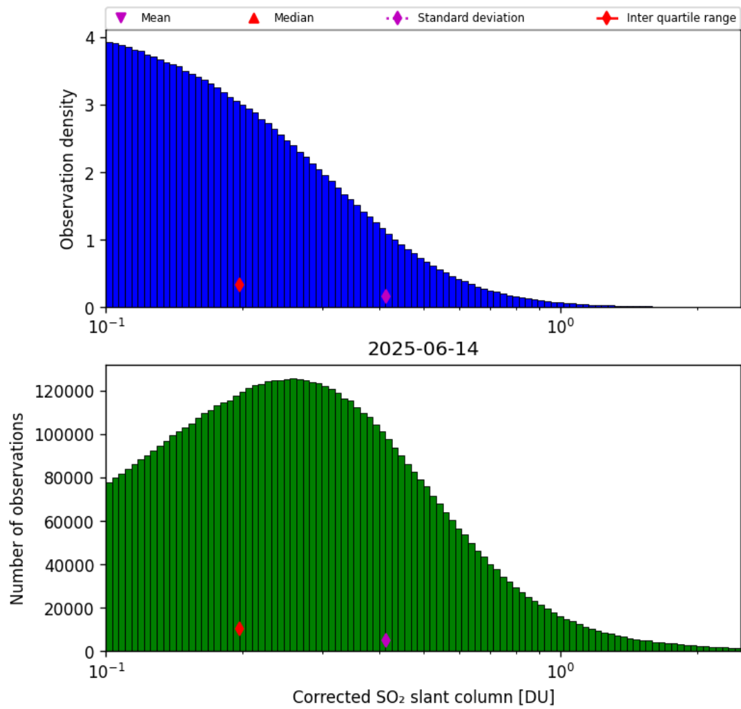
Figure 60: Histogram of “Corrected SO 2 slant column” for 2025-06-14 to 2025-06-14
