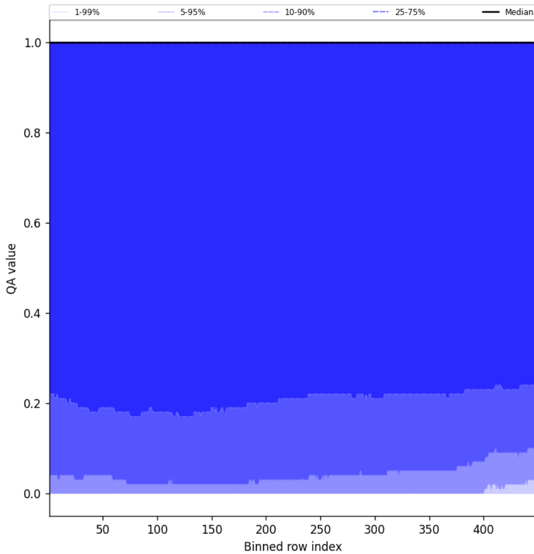
Figure 84: Along track statistics of “QA value” for 2025-06-14 to 2025-06-14
