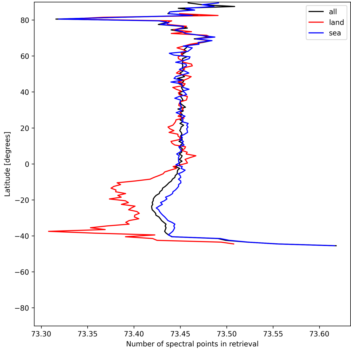
Figure 56: Zonal average of “Number of spectral points in retrieval” for 2025-06-14 to 2025-06-14.
