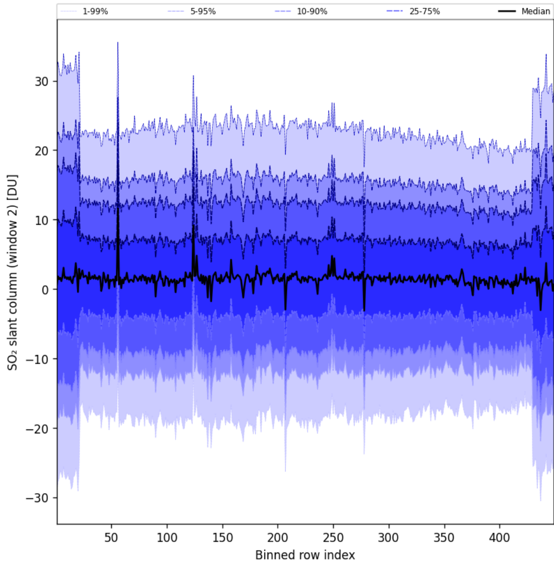
Figure 94: Along track statistics of “SO 2 slant column (window 2)” for 2025-06-14 to 2025-06-14
