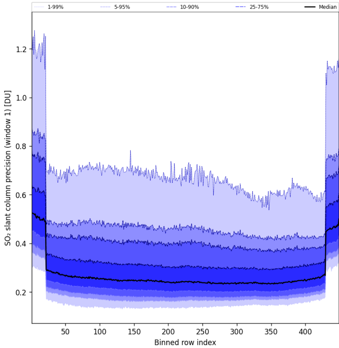
Figure 91: Along track statistics of “SO 2 slant column precision (window 1)” for 2025-06-14 to 2025-06-14
