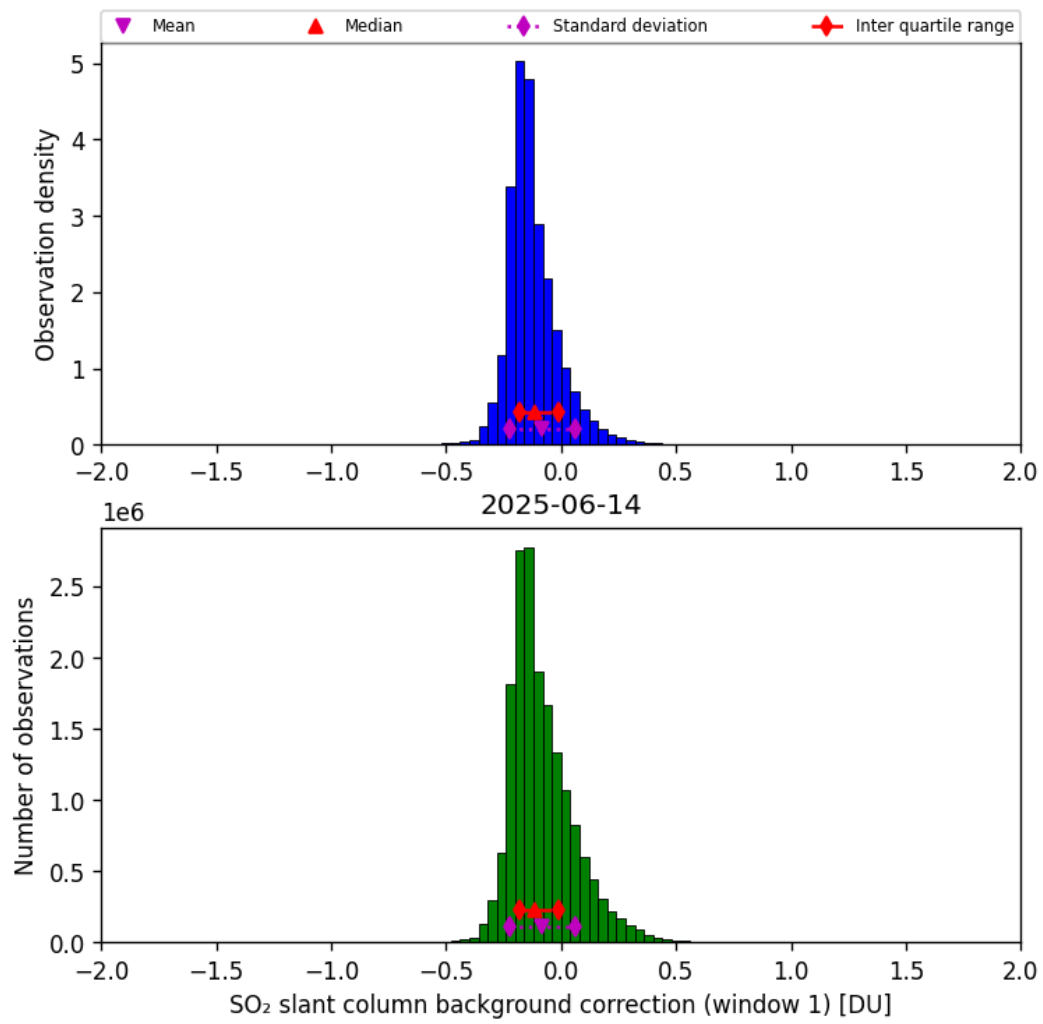
Figure 66: Histogram of “SO 2 slant column background correction (window 1)” for 2025-06-14 to 2025-06-14
