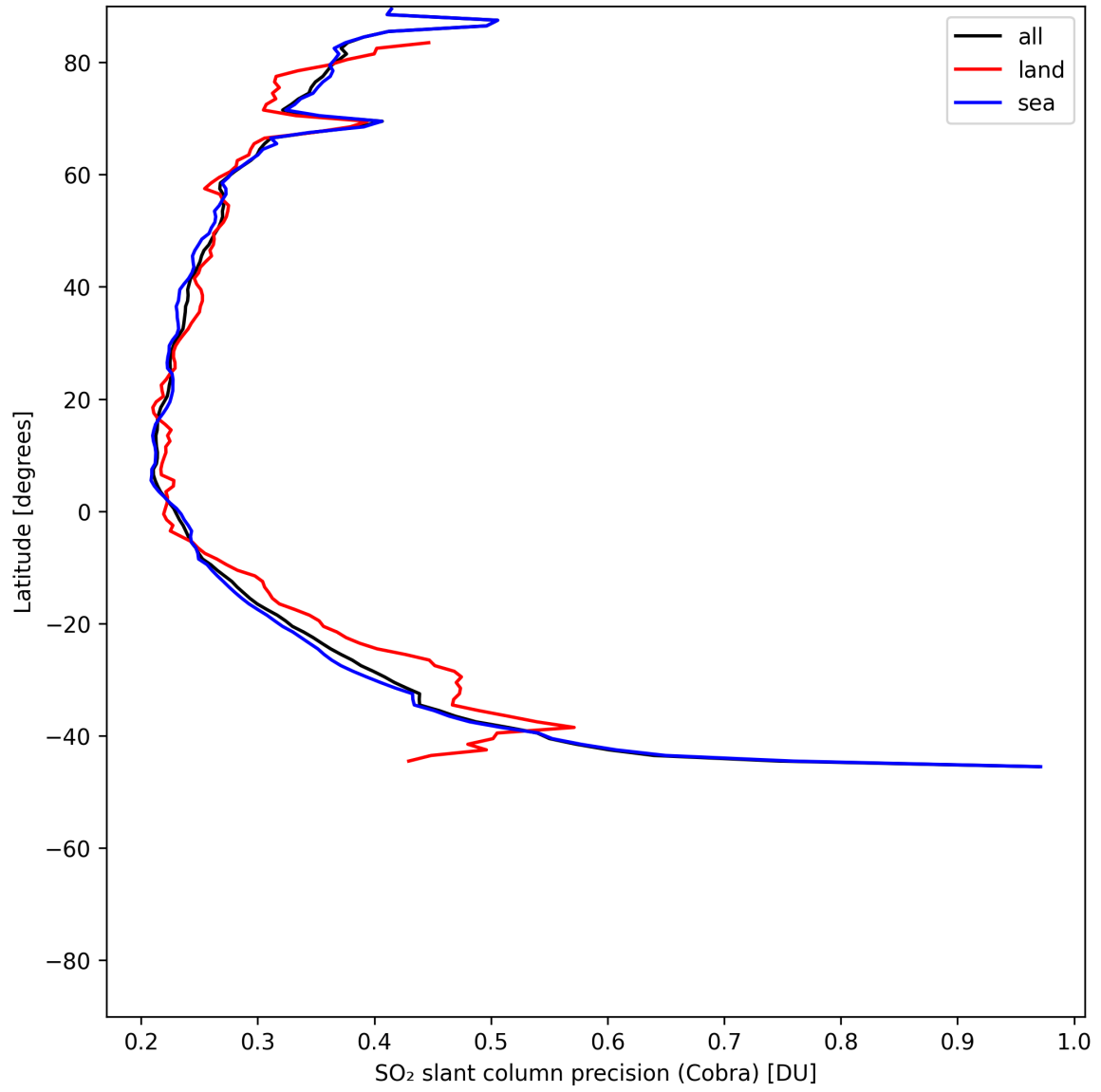
Figure 35: Zonal average of “SO 2 slant column precision (Cobra)” for 2025-06-14 to 2025-06-14.
