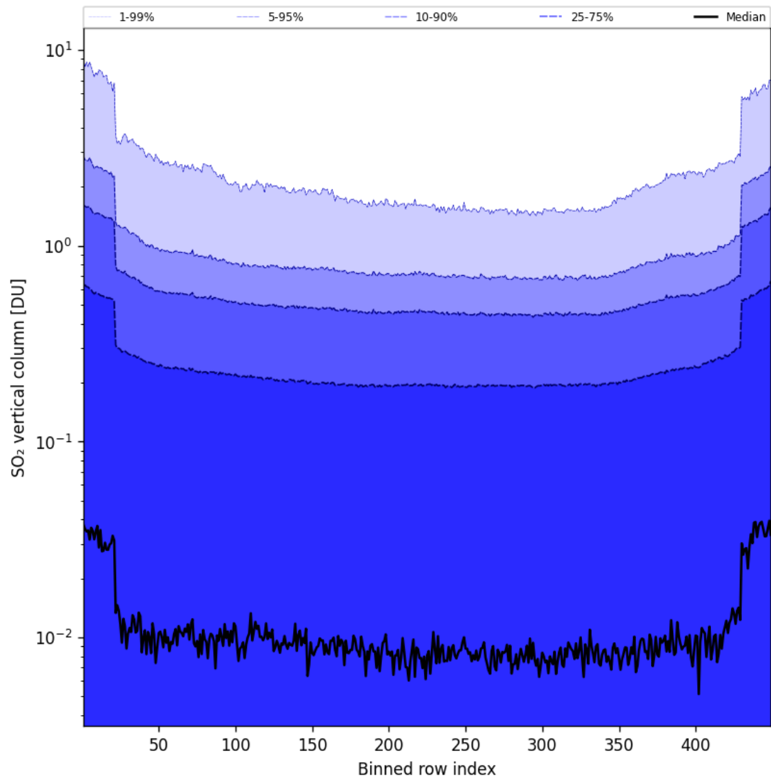
Figure 85: Along track statistics of “SO 2 vertical column” for 2025-06-14 to 2025-06-14
