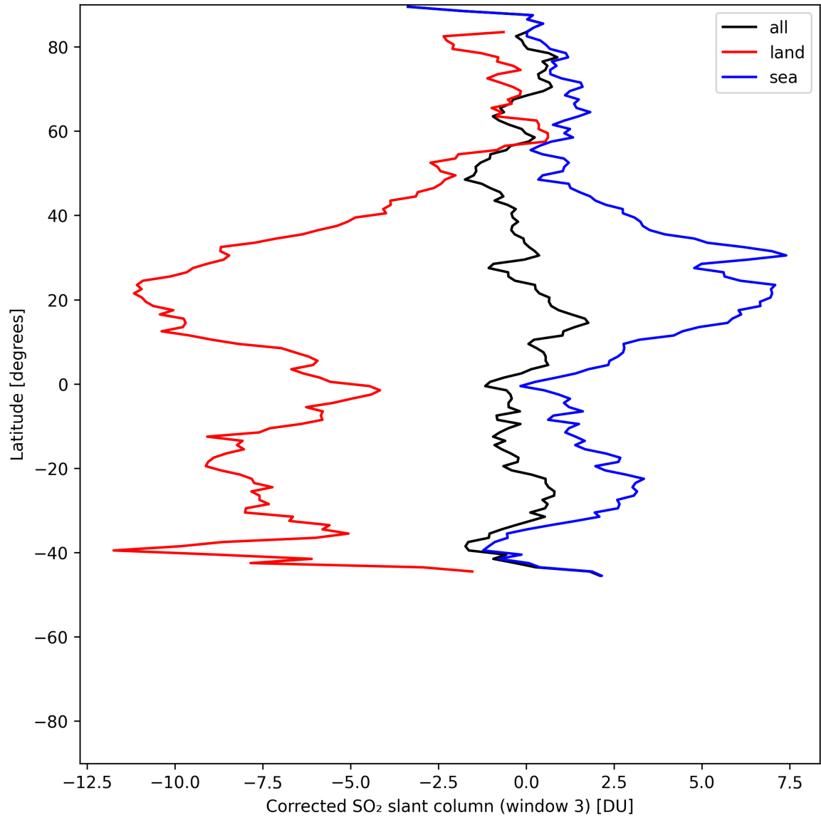
Figure 46: Zonal average of “Corrected SO 2 slant column (window 3)” for 2025-06-14 to 2025-06-14.
