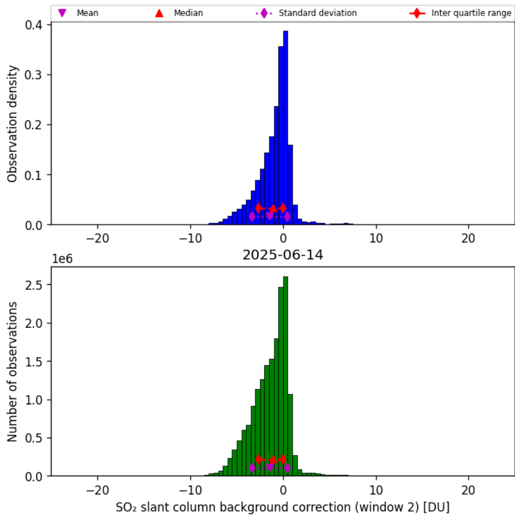
Figure 70: Histogram of “SO 2 slant column background correction (window 2)” for 2025-06-14 to 2025-06-14
