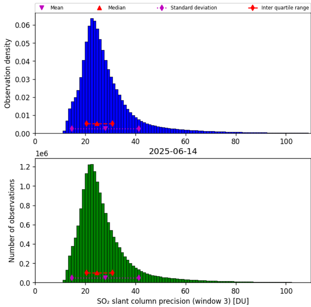
Figure 72: Histogram of “SO 2 slant column precision (window 3)” for 2025-06-14 to 2025-06-14
