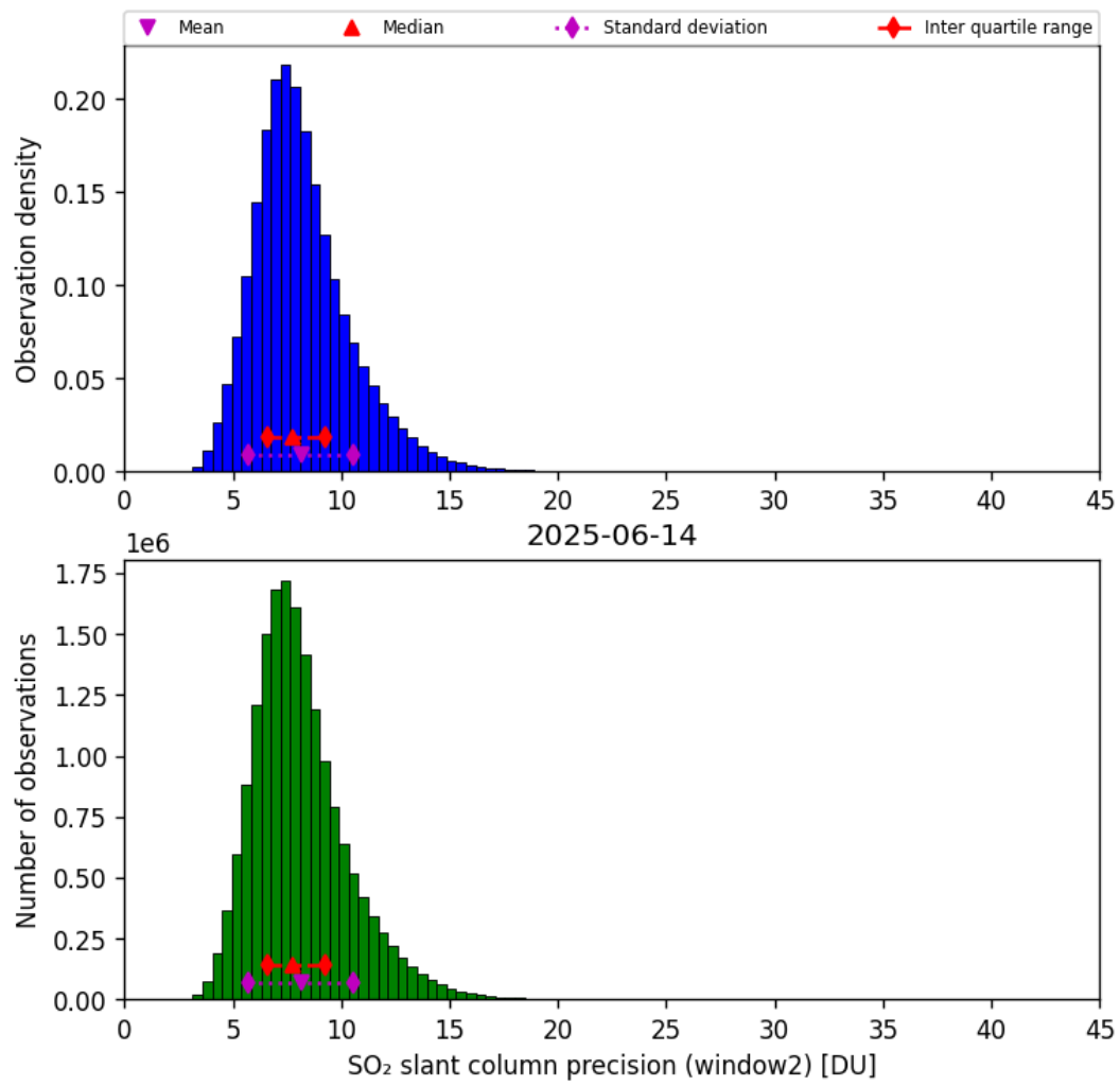
Figure 68: Histogram of “SO 2 slant column precision (window2)” for 2025-06-14 to 2025-06-14
