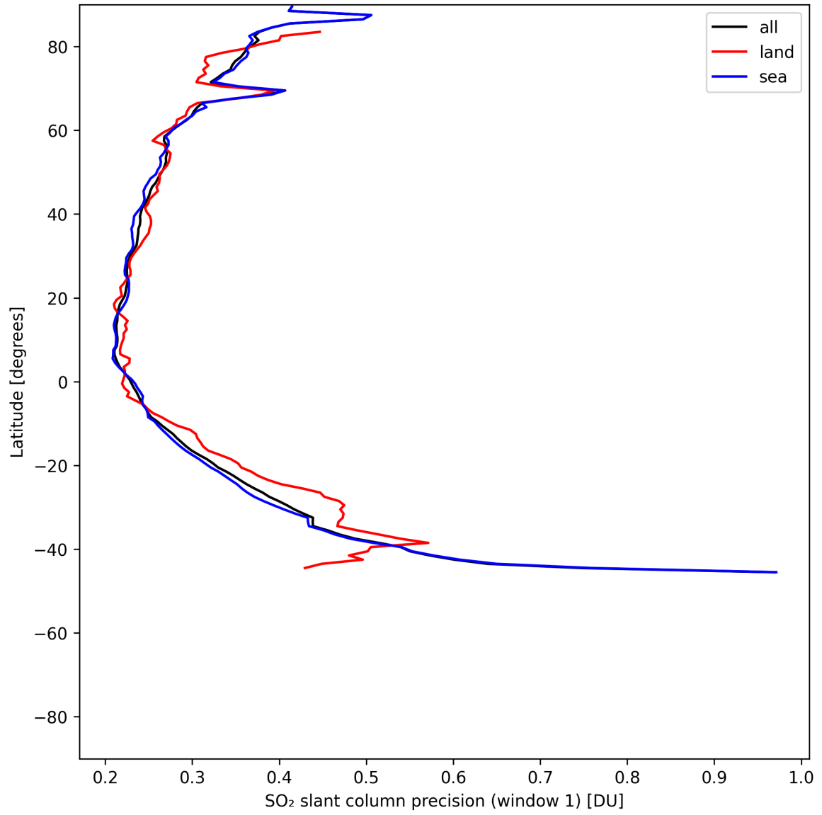
Figure 37: Zonal average of “SO 2 slant column precision (window 1)” for 2025-06-14 to 2025-06-14.
