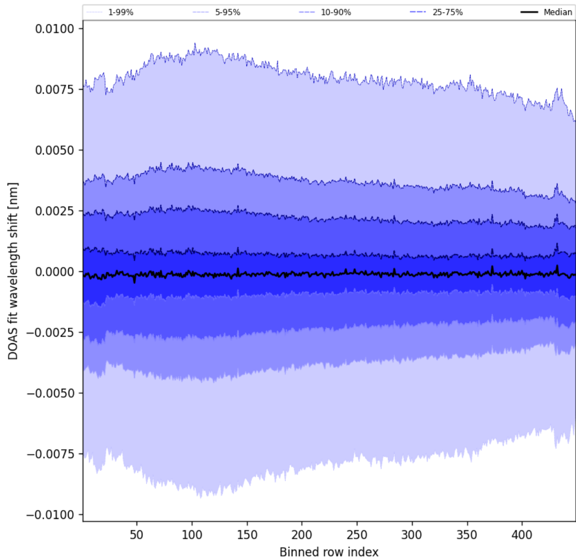
Figure 104: Along track statistics of “DOAS fit wavelength shift” for 2025-06-14 to 2025-06-14
