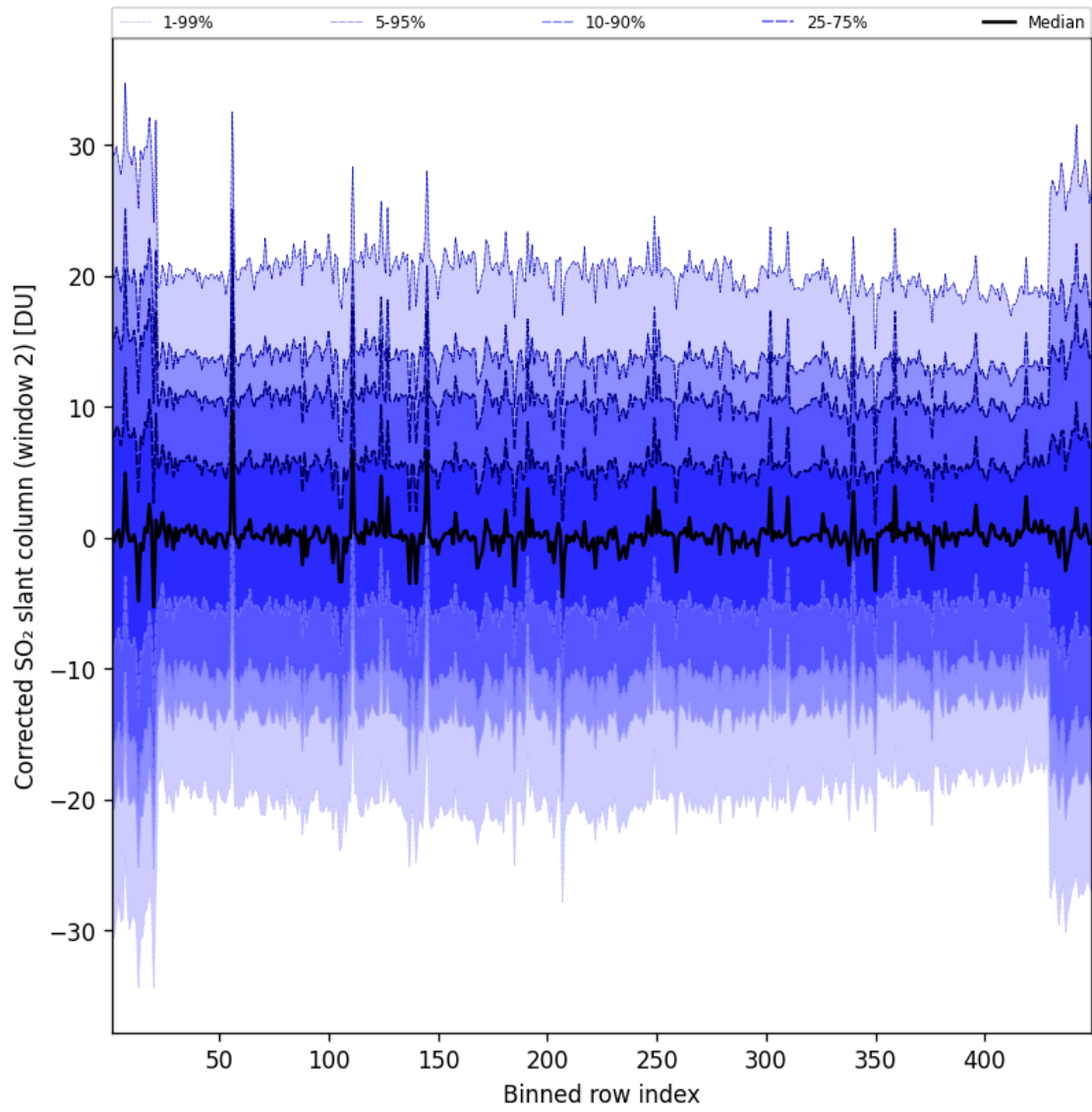
Figure 96: Along track statistics of “Corrected SO 2 slant column (window 2)” for 2025-06-14 to 2025-06-14
