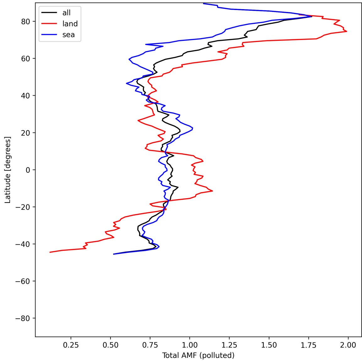
Figure 53: Zonal average of “Total AMF (polluted)” for 2025-06-14 to 2025-06-14.
