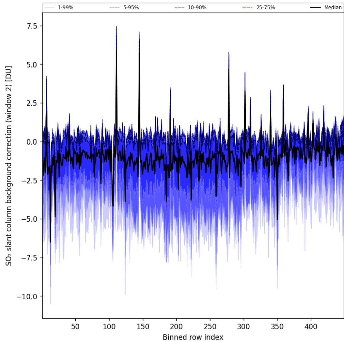
Figure 97: Along track statistics of “SO 2 slant column background correction (window 2)” for 2025-06-14 to 2025-06-14
