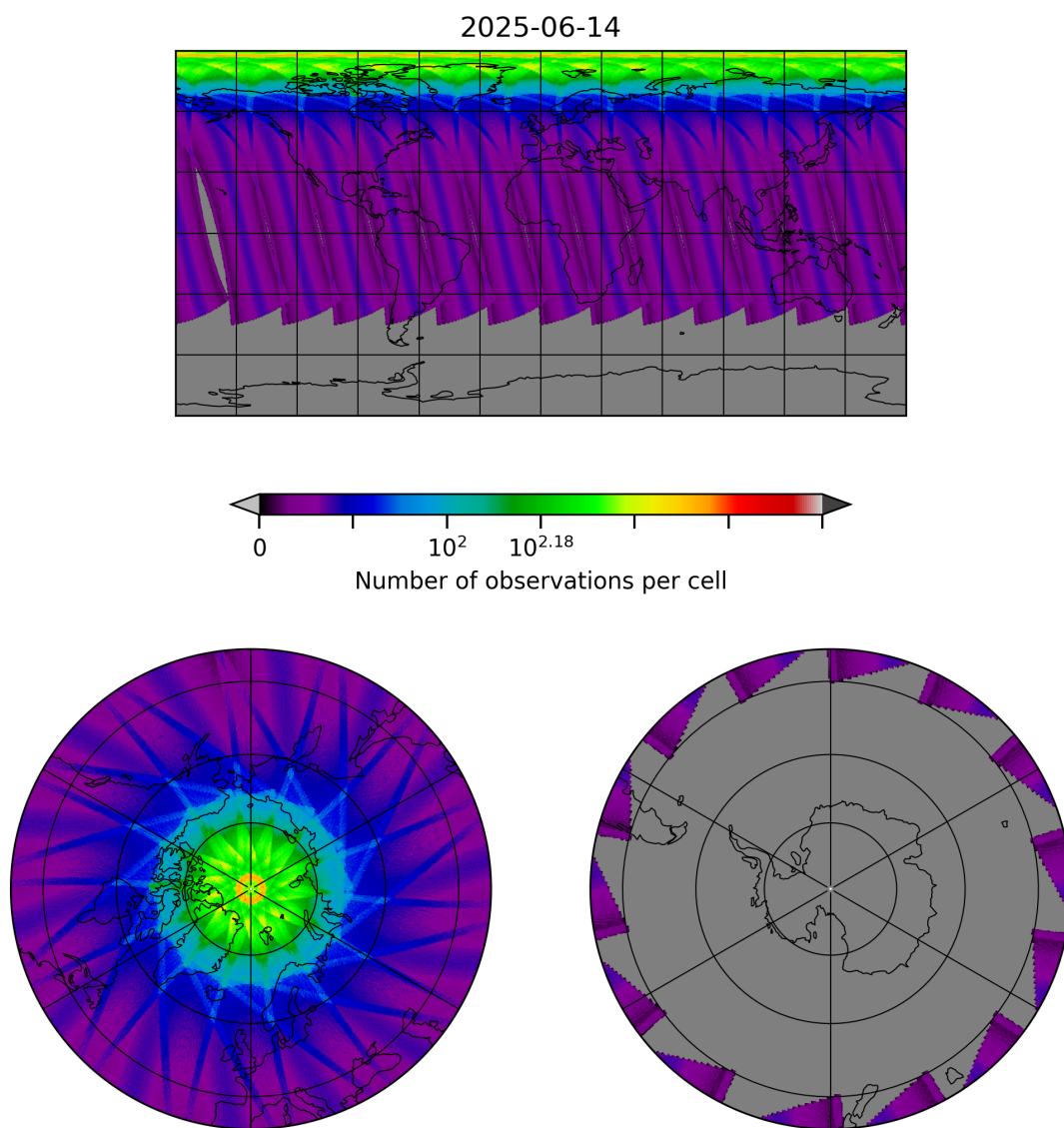
Figure 29: Map of the number of observations for 2025-06-14 to 2025-06-14
