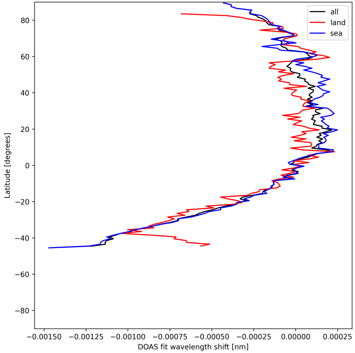
Figure 50: Zonal average of “DOAS fit wavelength shift” for 2025-06-14 to 2025-06-14.
