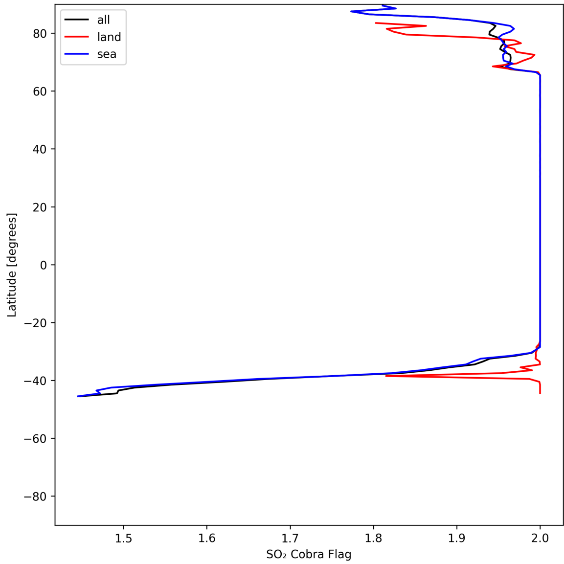
Figure 48: Zonal average of "SO 2 Cobra Flag" for 2025-06-14 to 2025-06-14.
