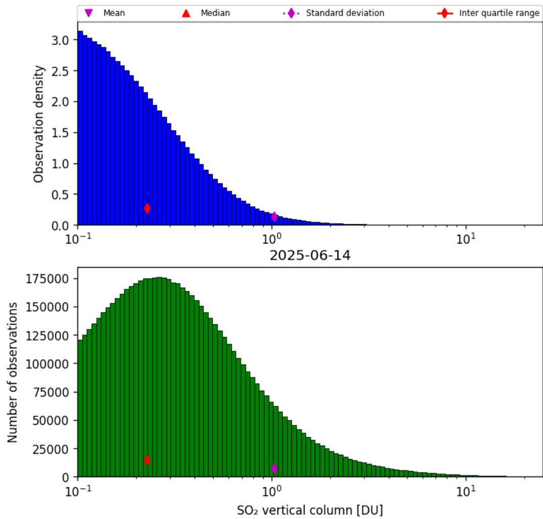
Figure 58: Histogram of “SO 2 vertical column” for 2025-06-14 to 2025-06-14
