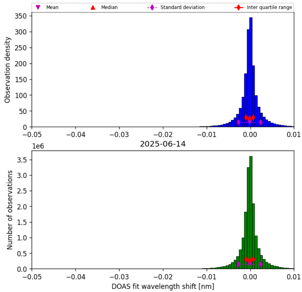
Figure 77: Histogram of “DOAS fit wavelength shift” for 2025-06-14 to 2025-06-14
