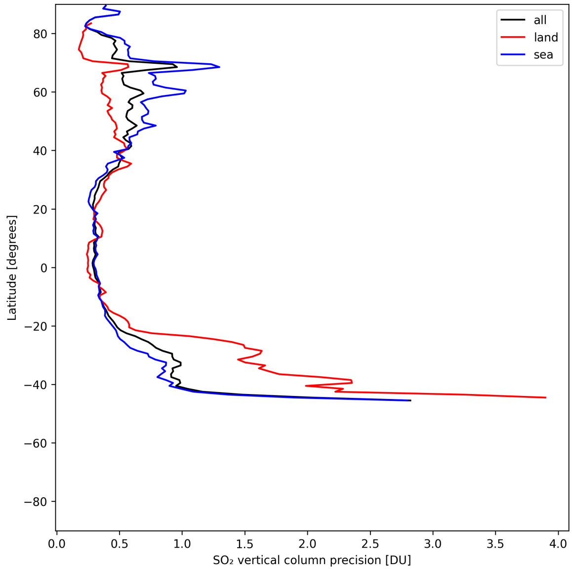
Figure 32: Zonal average of “SO 2 vertical column precision” for 2025-06-14 to 2025-06-14.
