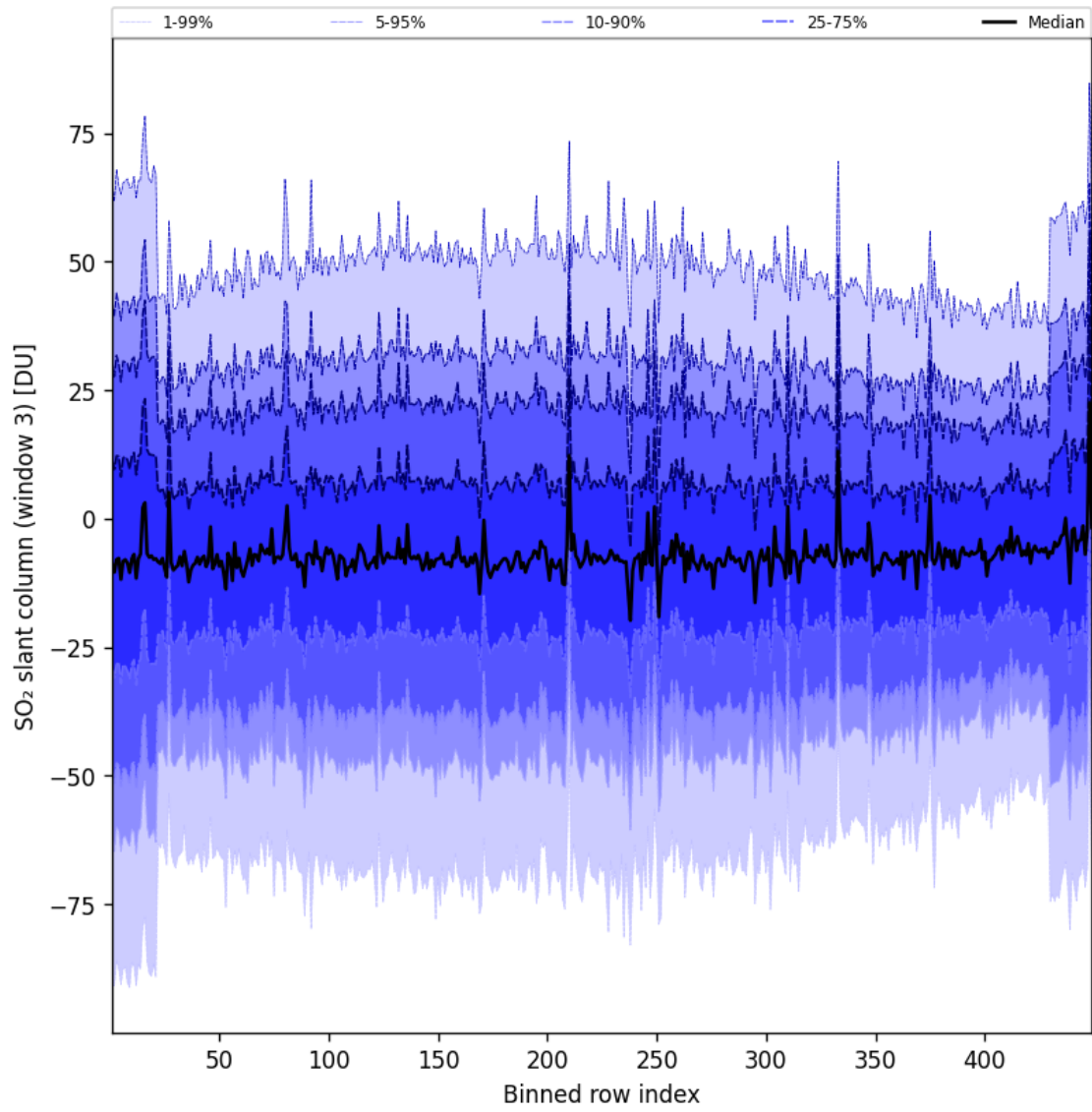
Figure 98: Along track statistics of “SO 2 slant column (window 3)” for 2025-06-14 to 2025-06-14
