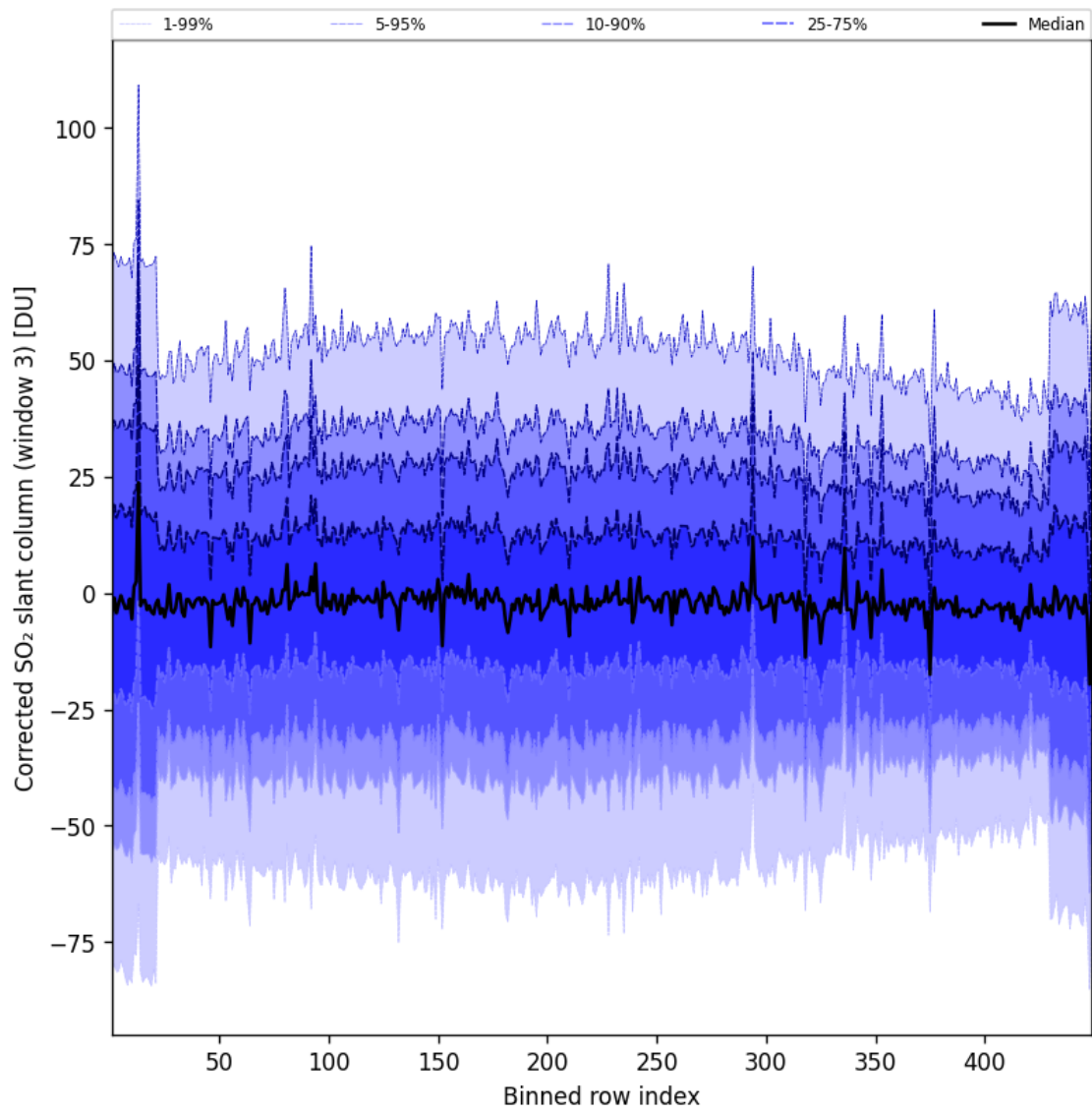
Figure 100: Along track statistics of “Corrected SO 2 slant column (window 3)” for 2025-06-16 to 2025-06-17
