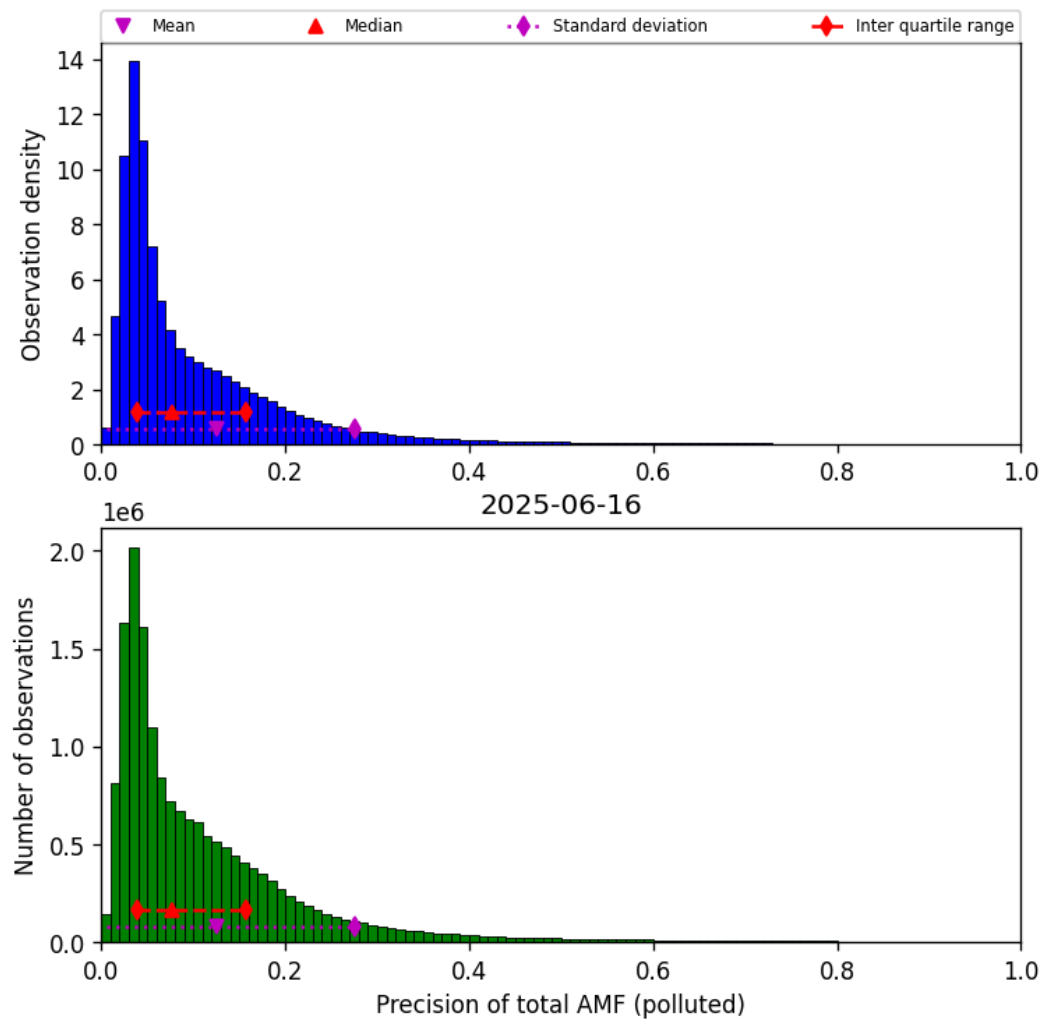
Figure 81: Histogram of “Precision of total AMF (polluted)” for 2025-06-16 to 2025-06-17
