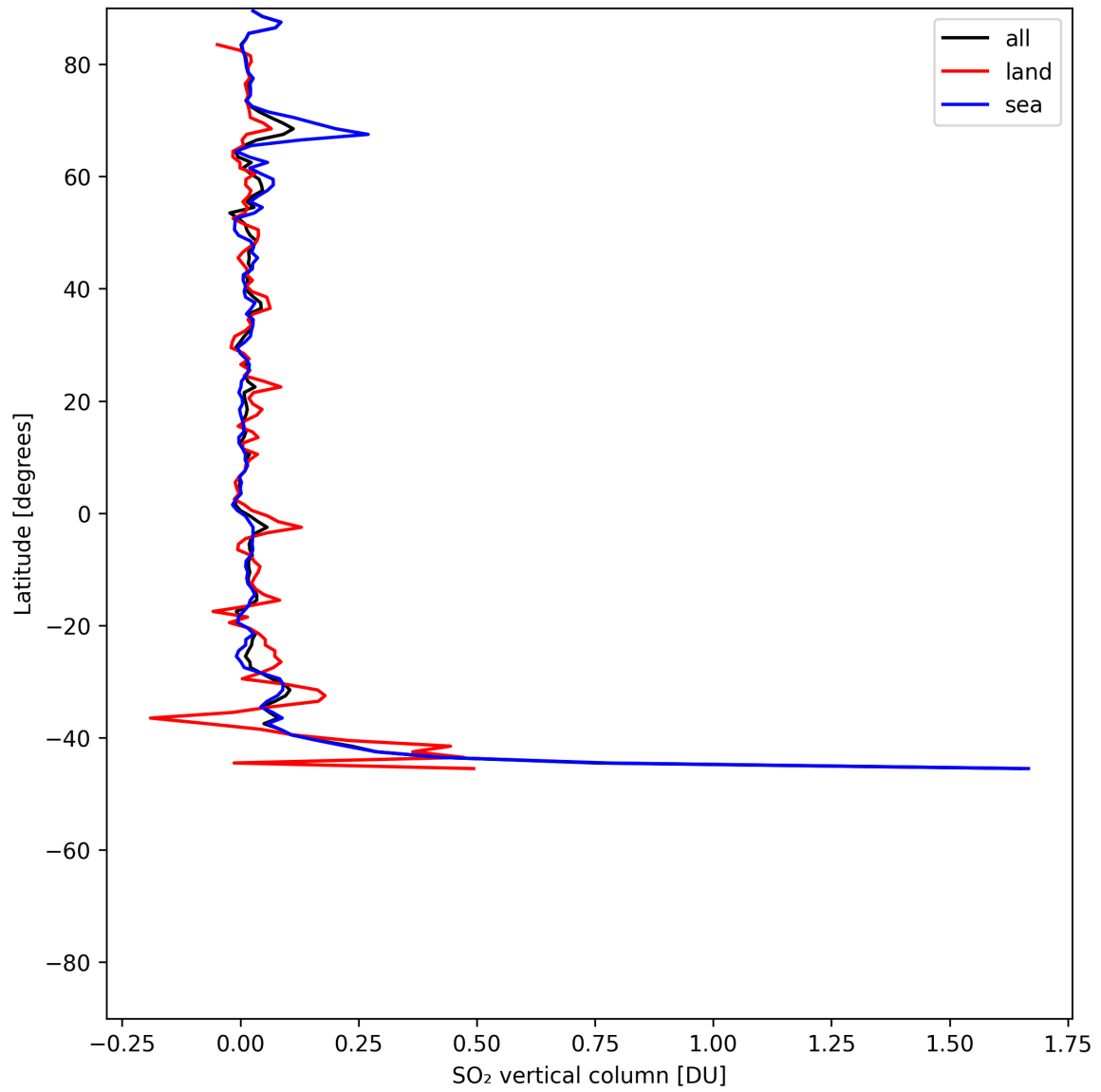
Figure 31: Zonal average of “SO 2 vertical column” for 2025-06-16 to 2025-06-17.
