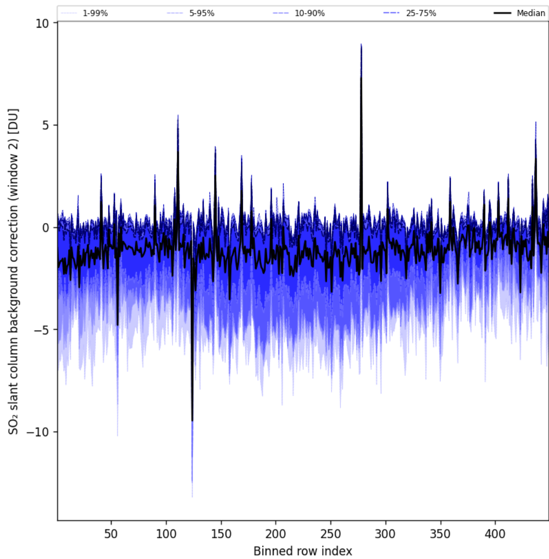
Figure 97: Along track statistics of “SO 2 slant column background correction (window 2)” for 2025-06-16 to 2025-06-17
