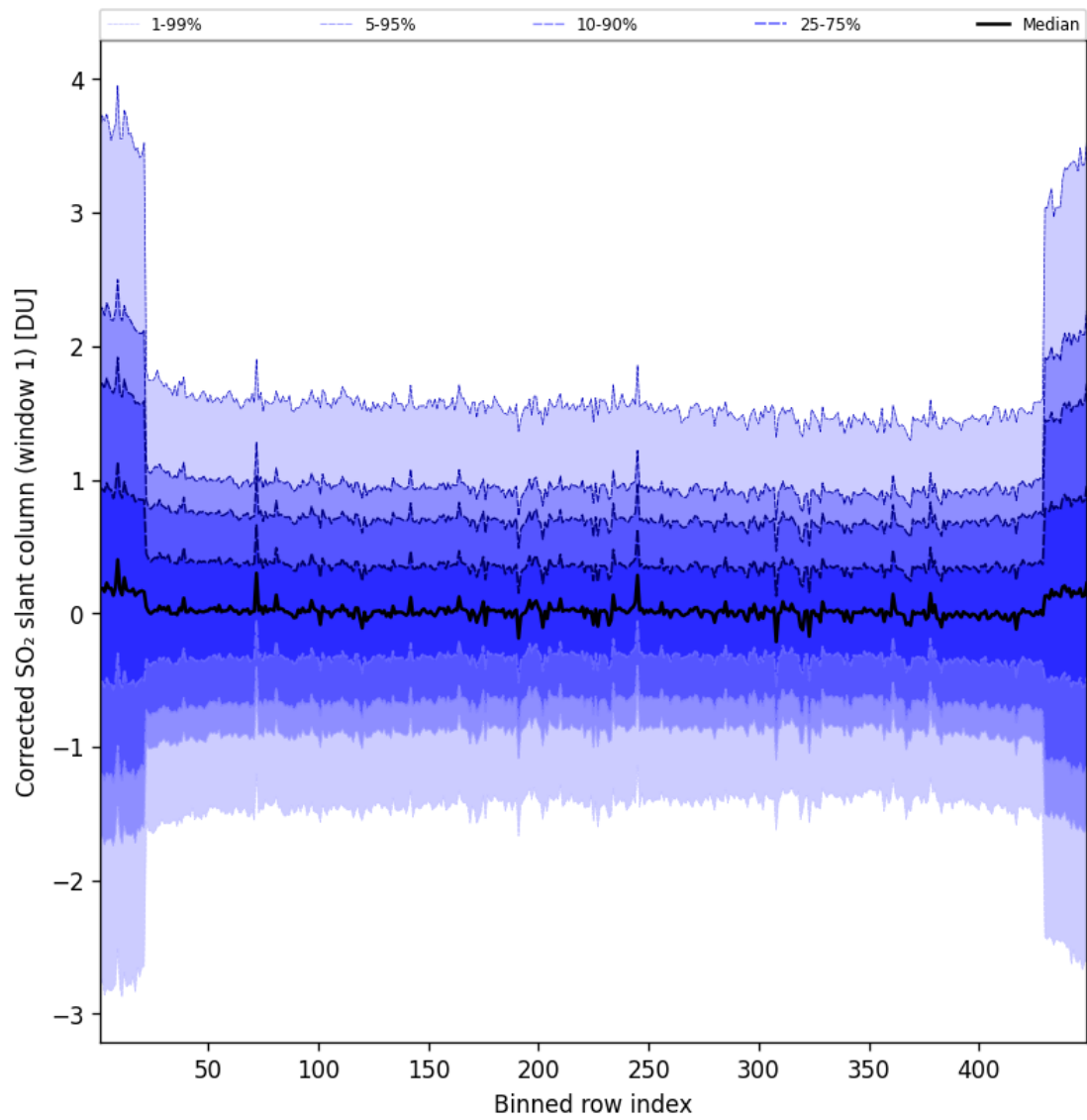
Figure 92: Along track statistics of “Corrected SO 2 slant column (window 1)” for 2025-06-16 to 2025-06-17
