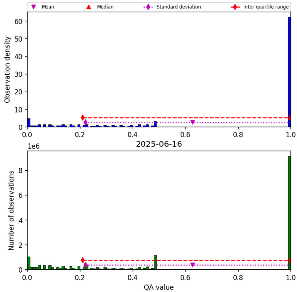
Figure 57: Histogram of “QA value” for 2025-06-16 to 2025-06-17
