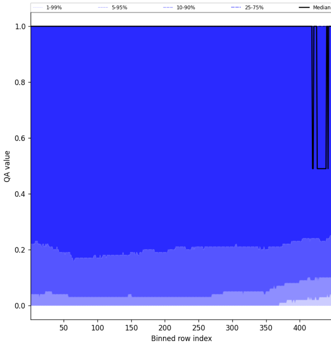
Figure 84: Along track statistics of “QA value” for 2025-06-16 to 2025-06-17
