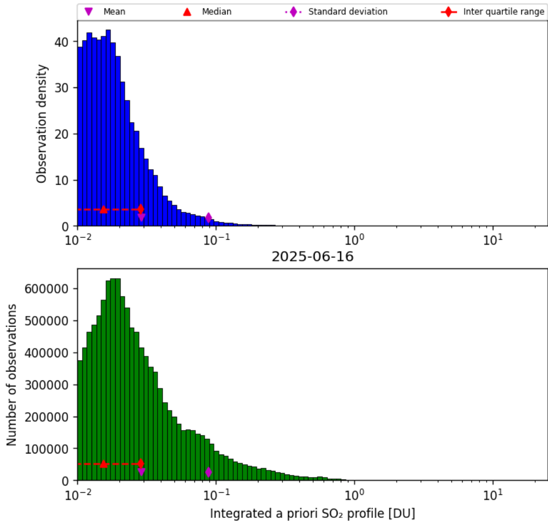
Figure 76: Histogram of “Integrated a priori SO 2 profile” for 2025-06-16 to 2025-06-17
