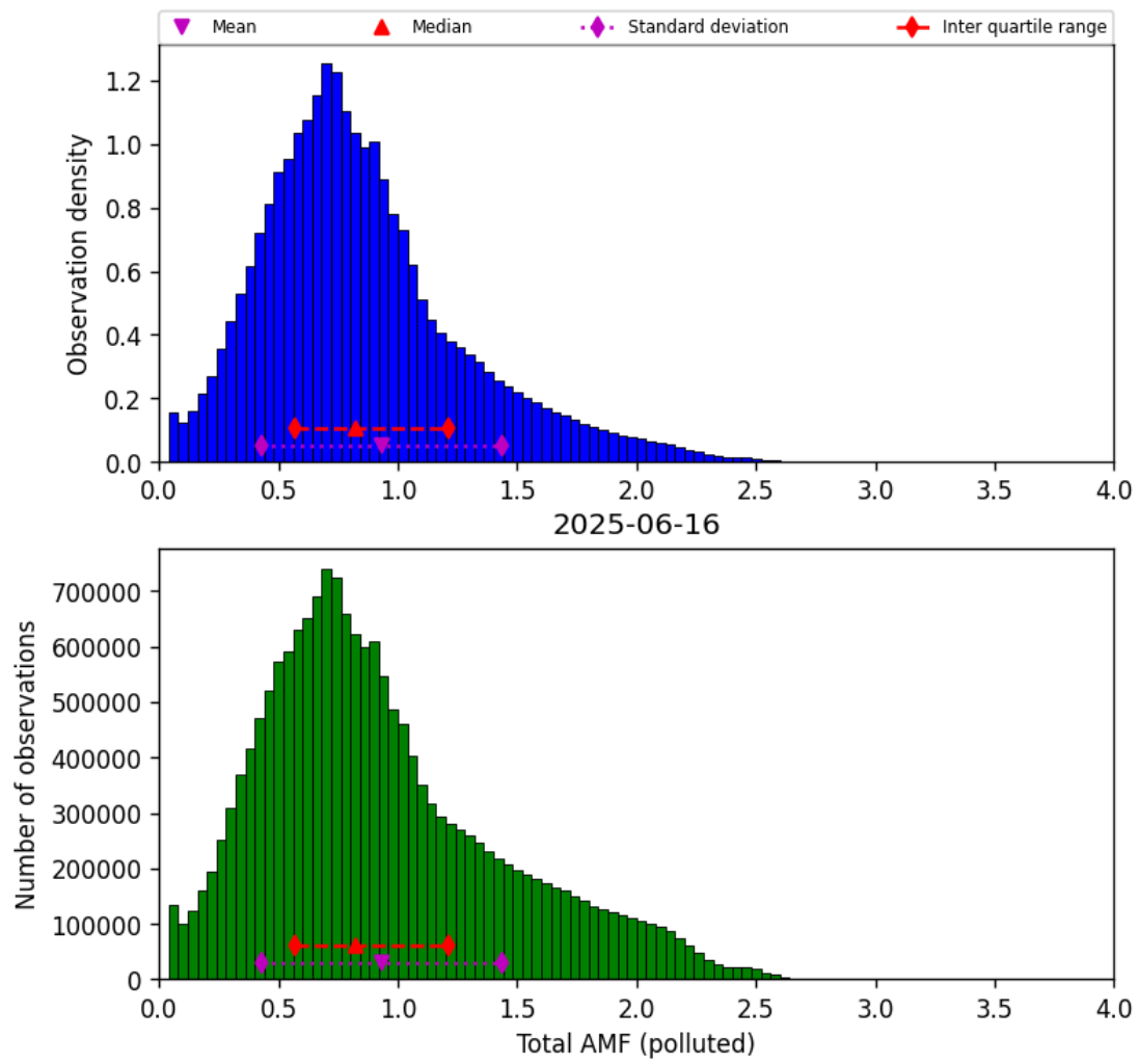
Figure 80: Histogram of “Total AMF (polluted)” for 2025-06-16 to 2025-06-17
