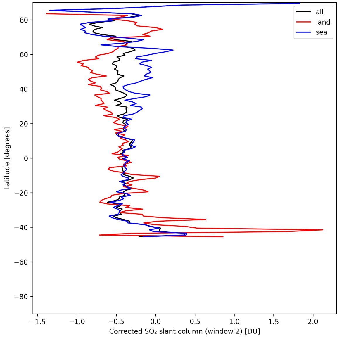
Figure 42: Zonal average of “Corrected SO 2 slant column (window 2)” for 2025-06-16 to 2025-06-17.
