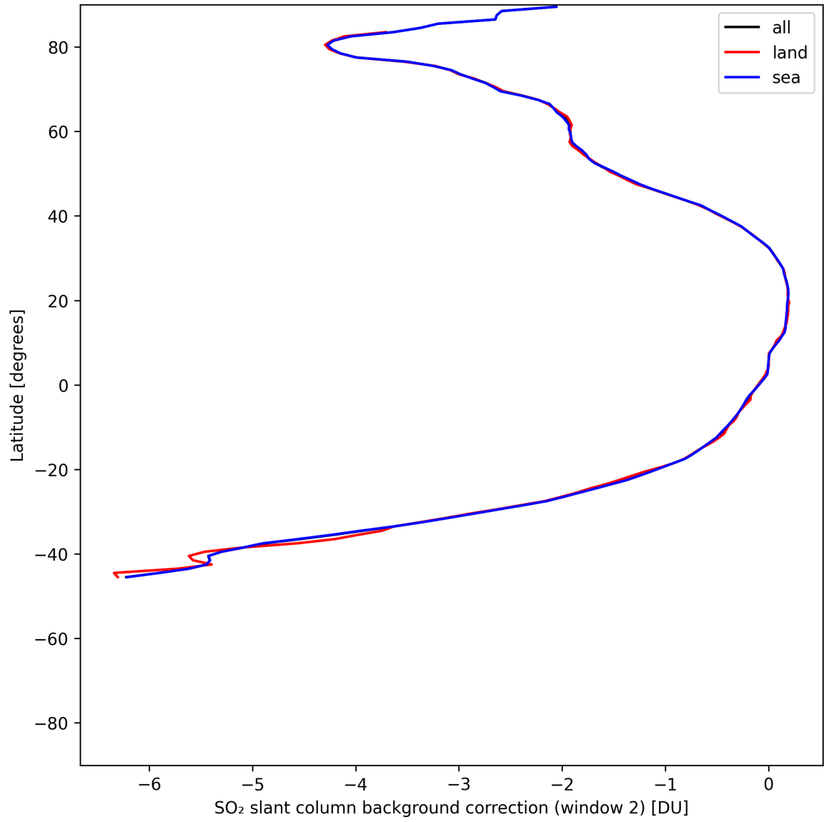
Figure 43: Zonal average of “SO 2 slant column background correction (window 2)” for 2025-06-16 to 2025-06-17.
