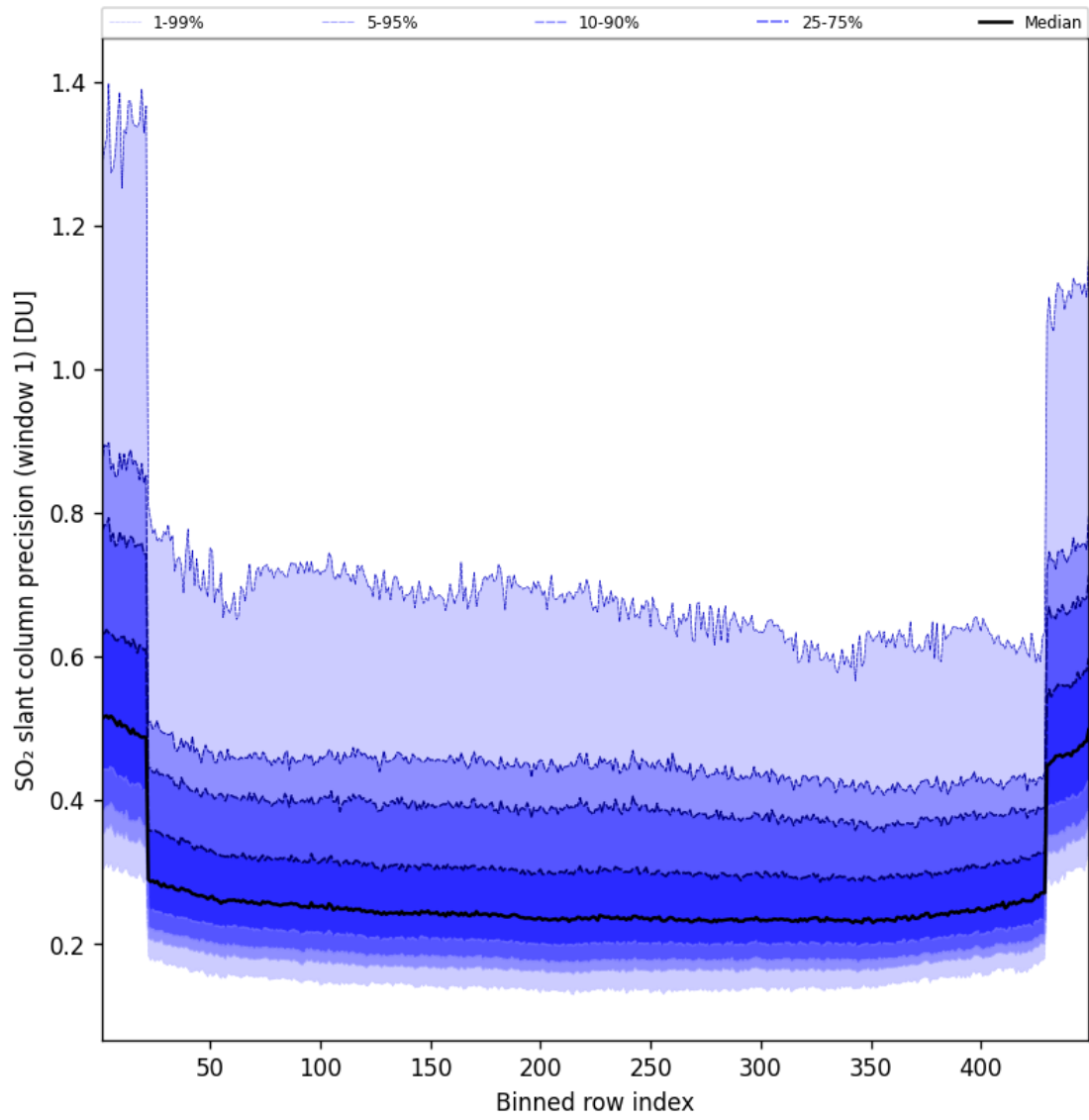
Figure 91: Along track statistics of “SO 2 slant column precision (window 1)” for 2025-06-16 to 2025-06-17
