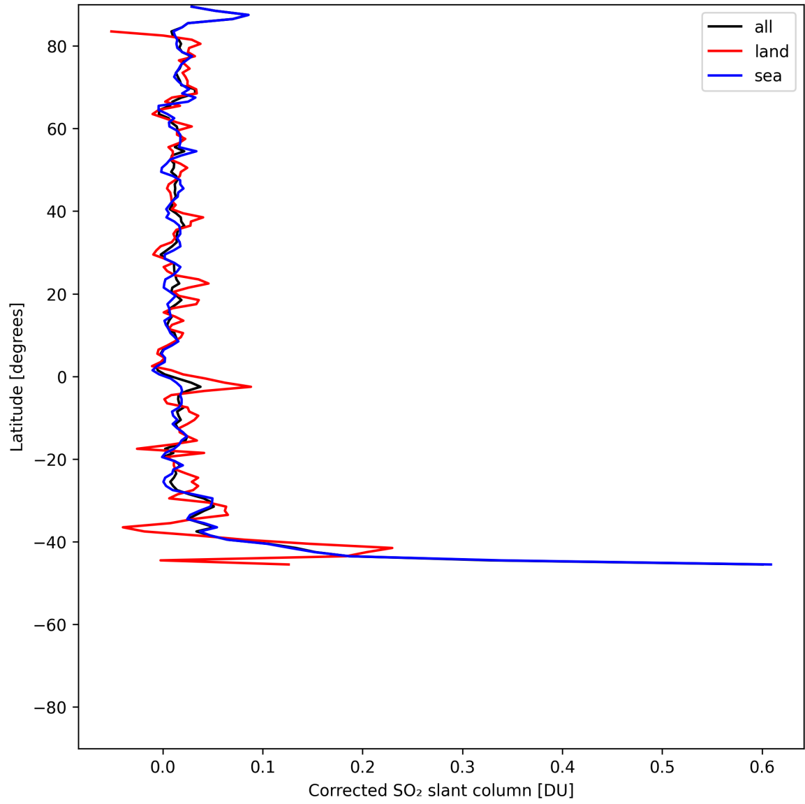
Figure 33: Zonal average of “Corrected SO 2 slant column” for 2025-06-16 to 2025-06-17.
