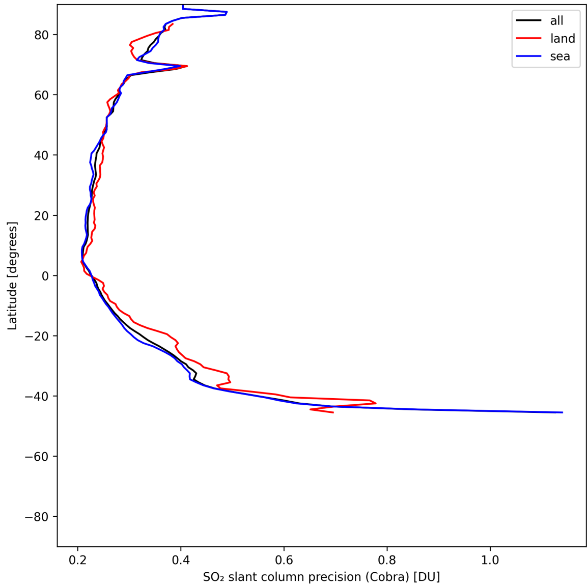
Figure 35: Zonal average of “SO 2 slant column precision (Cobra)” for 2025-06-16 to 2025-06-17.
