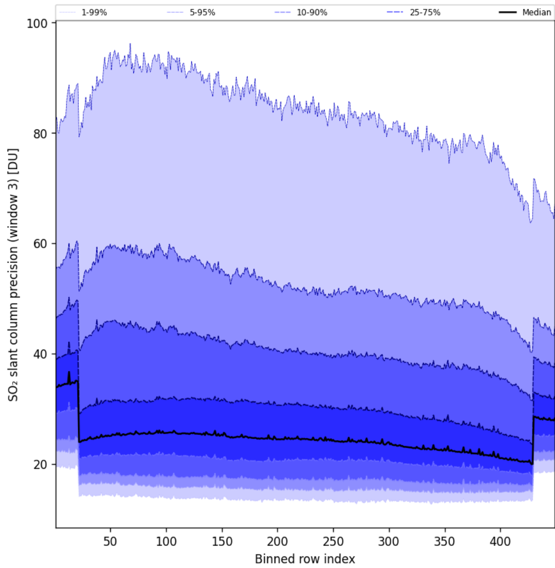
Figure 99: Along track statistics of “SO 2 slant column precision (window 3)” for 2025-06-16 to 2025-06-17
