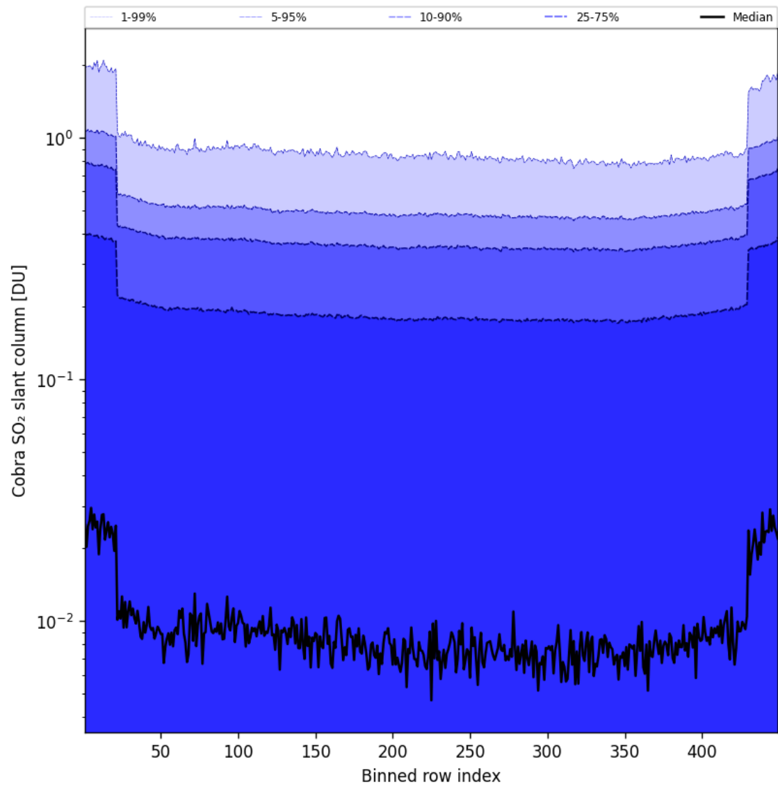
Figure 88: Along track statistics of “Cobra SO 2 slant column” for 2025-06-16 to 2025-06-17
