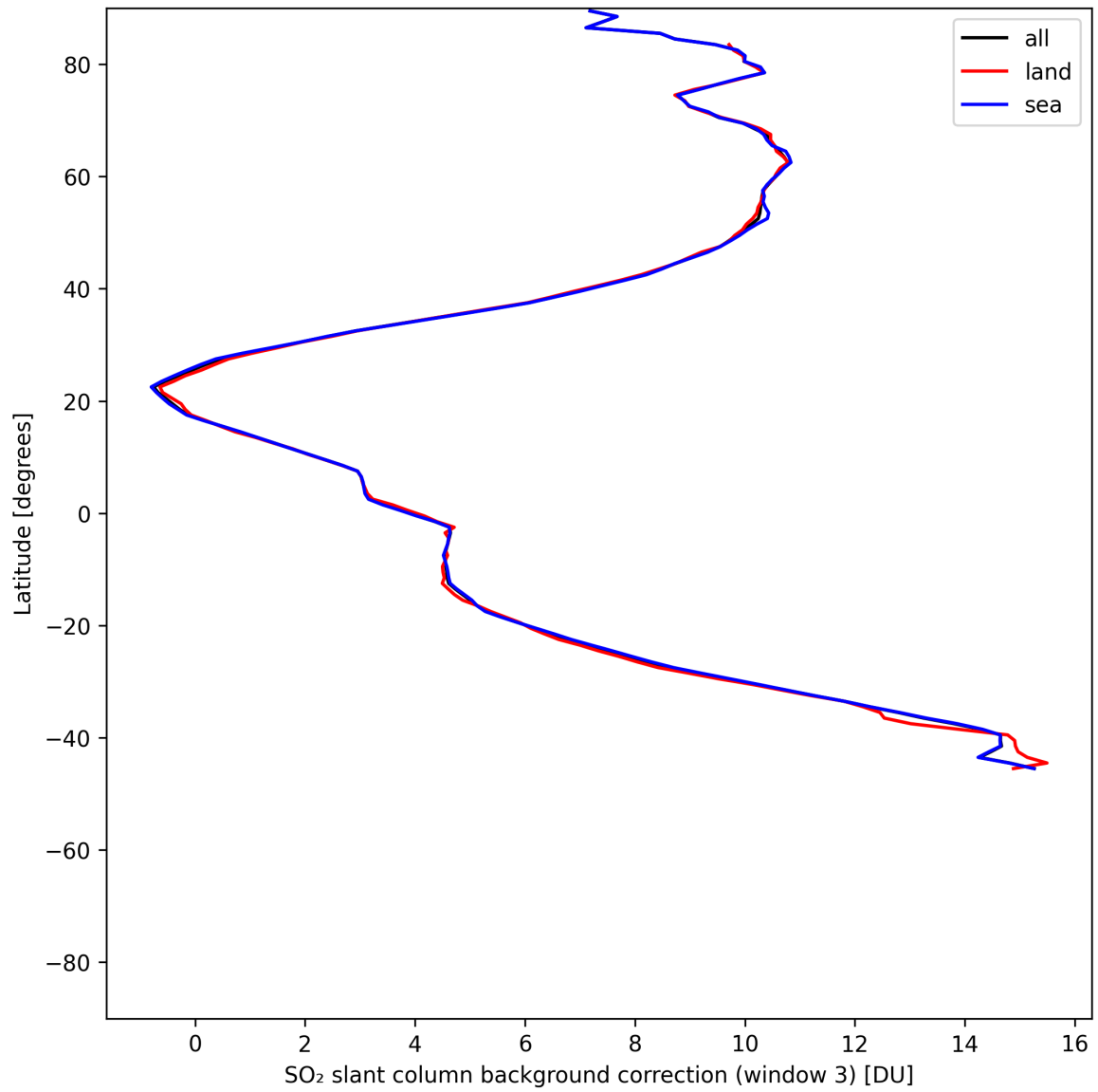
Figure 47: Zonal average of “SO 2 slant column background correction (window 3)” for 2025-06-16 to 2025-06-17.
