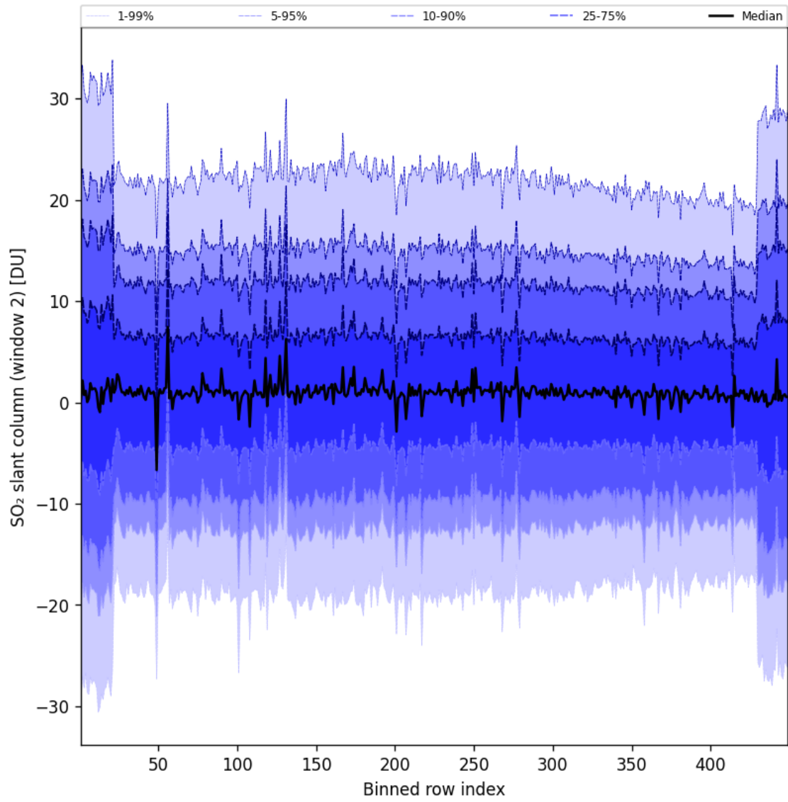
Figure 94: Along track statistics of “SO 2 slant column (window 2)” for 2025-06-16 to 2025-06-17
