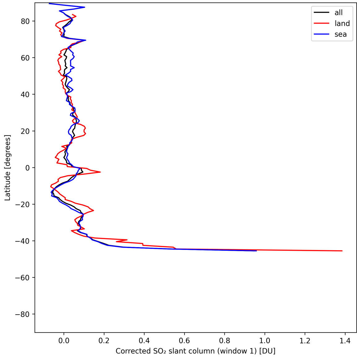
Figure 38: Zonal average of “Corrected SO 2 slant column (window 1)” for 2025-06-16 to 2025-06-17.
