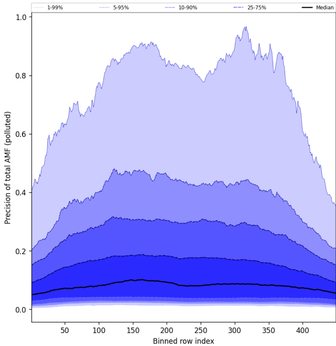
Figure 108: Along track statistics of “Precision of total AMF (polluted)” for 2025-06-16 to 2025-06-17
