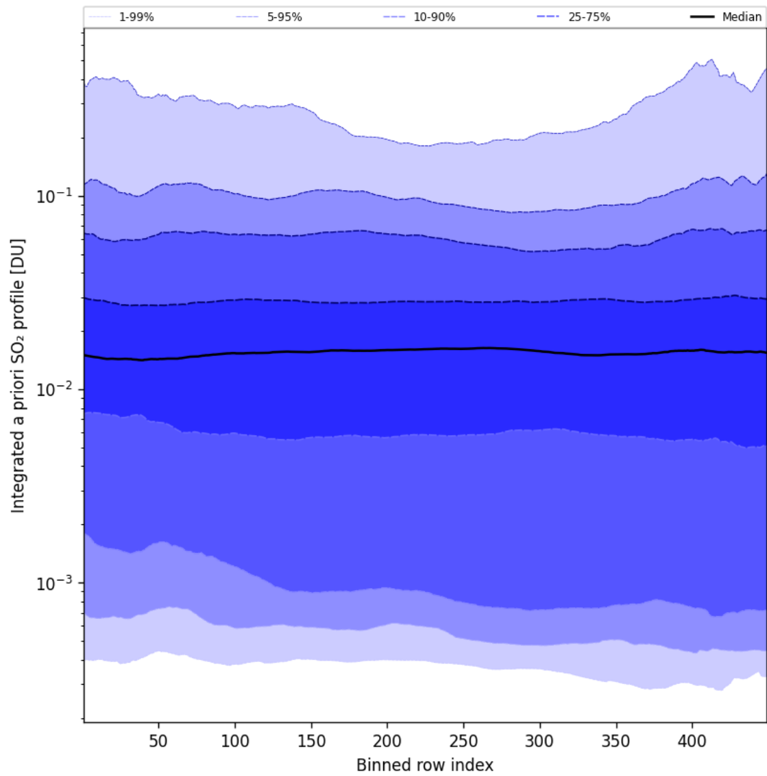
Figure 103: Along track statistics of “Integrated a priori SO 2 profile” for 2025-06-16 to 2025-06-17
