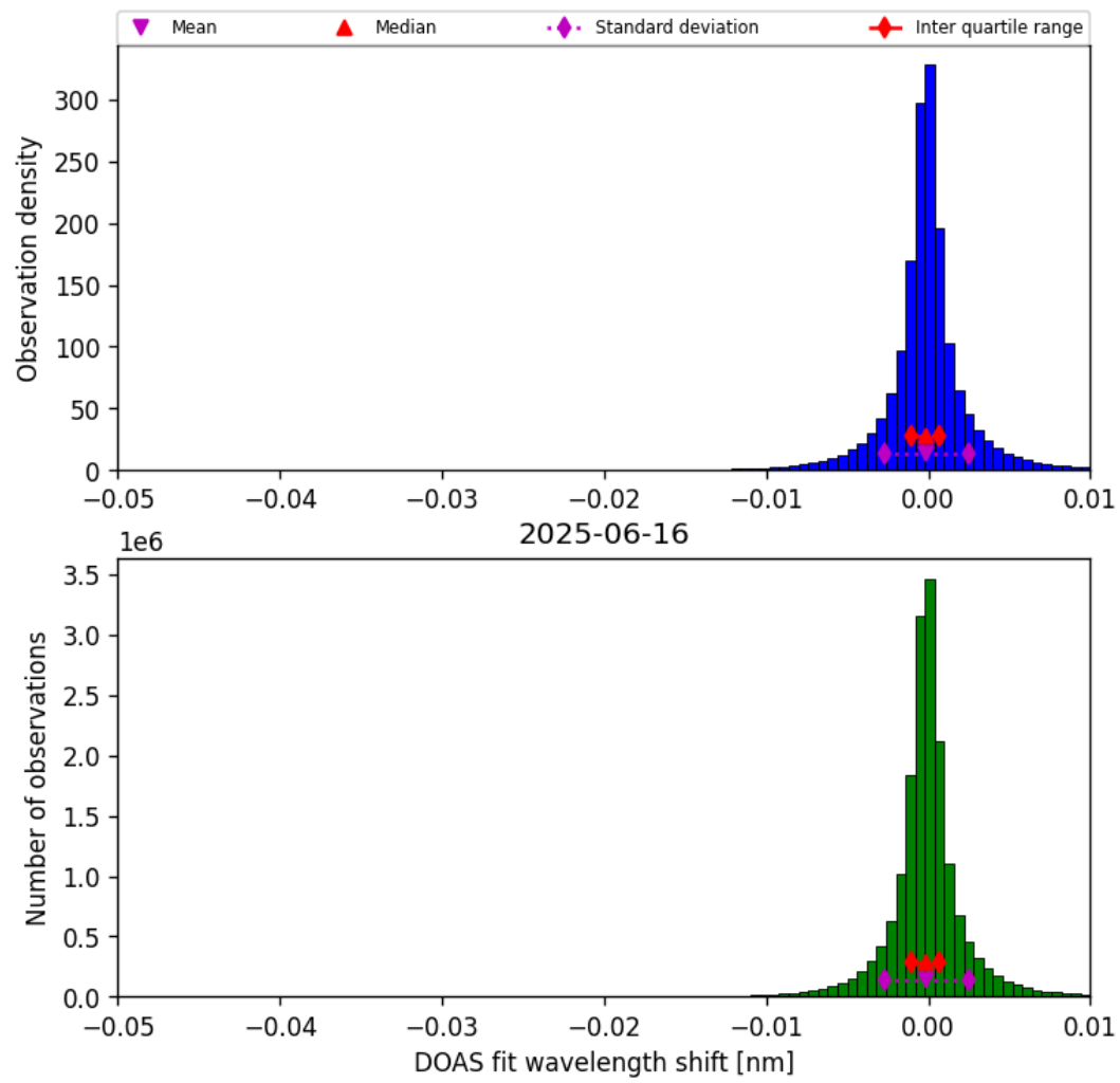
Figure 77: Histogram of “DOAS fit wavelength shift” for 2025-06-16 to 2025-06-17
