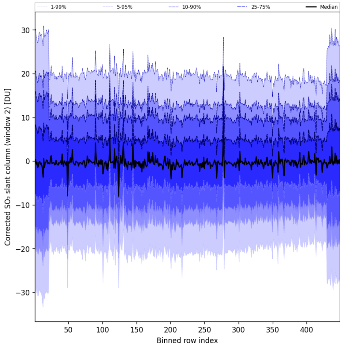
Figure 96: Along track statistics of “Corrected SO 2 slant column (window 2)” for 2025-06-16 to 2025-06-17
