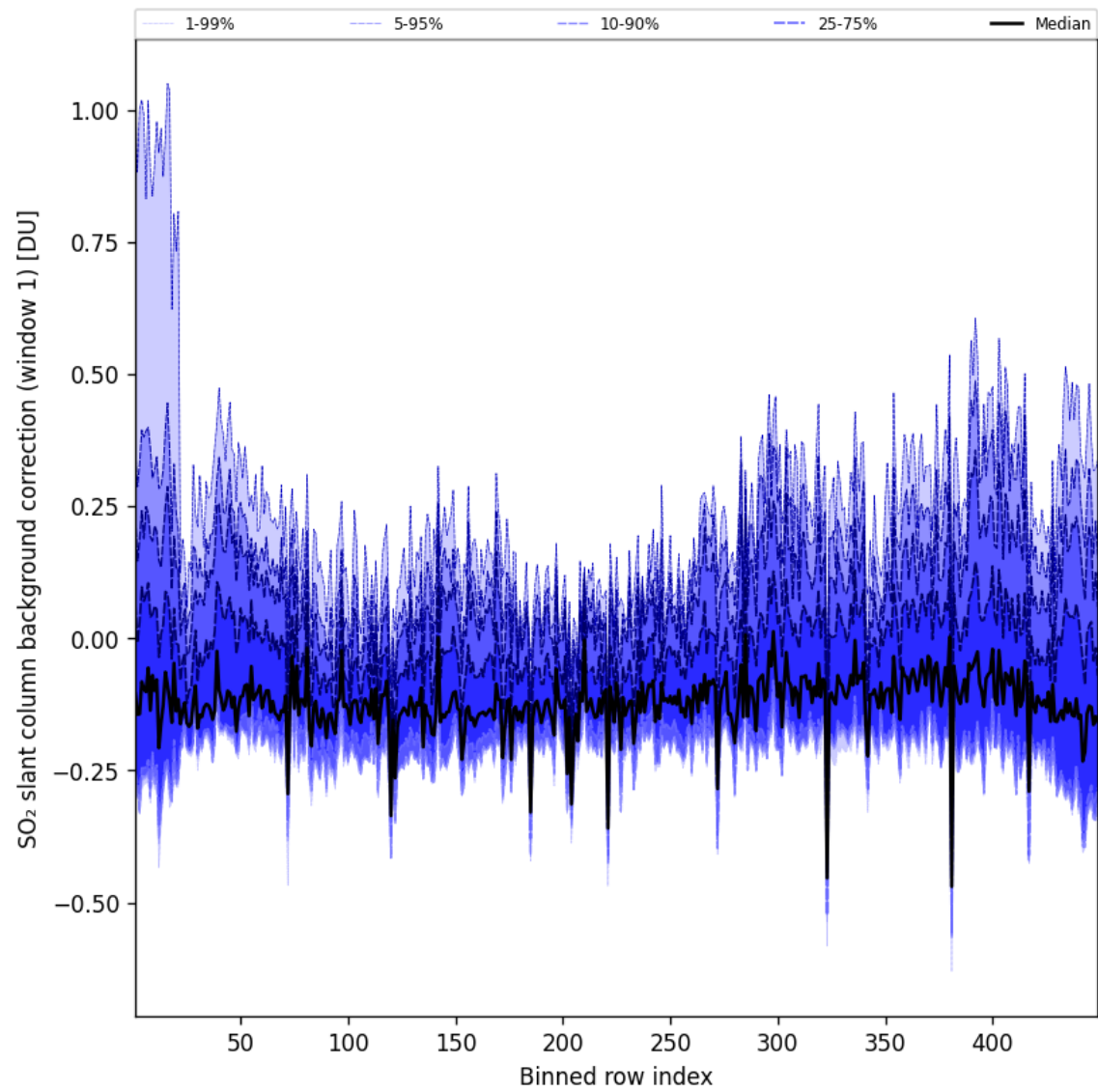
Figure 93: Along track statistics of “SO 2 slant column background correction (window 1)” for 2025-06-16 to 2025-06-17
