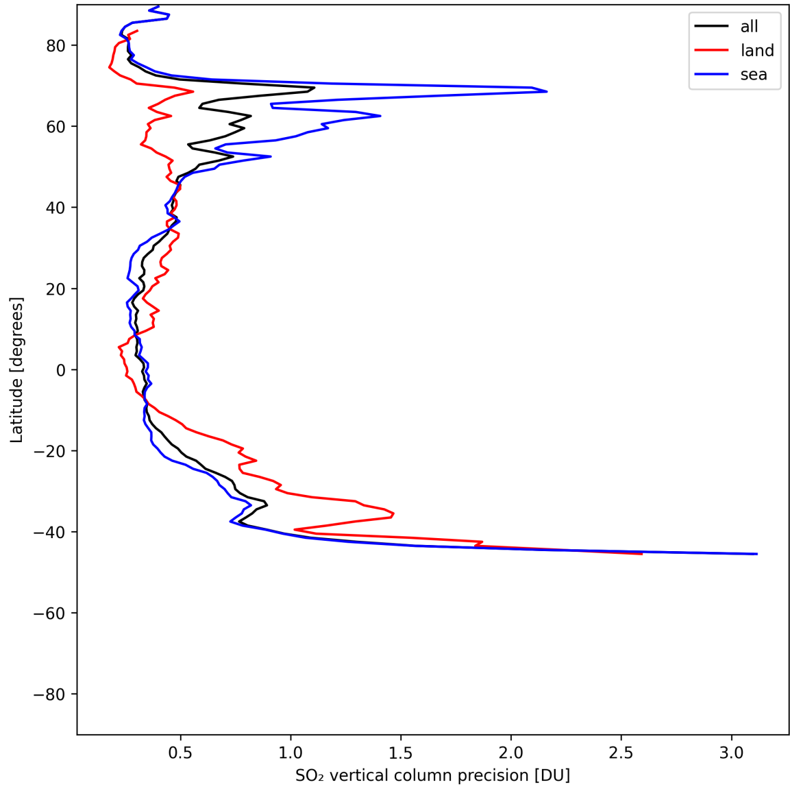
Figure 32: Zonal average of “SO 2 vertical column precision” for 2025-06-16 to 2025-06-17.
