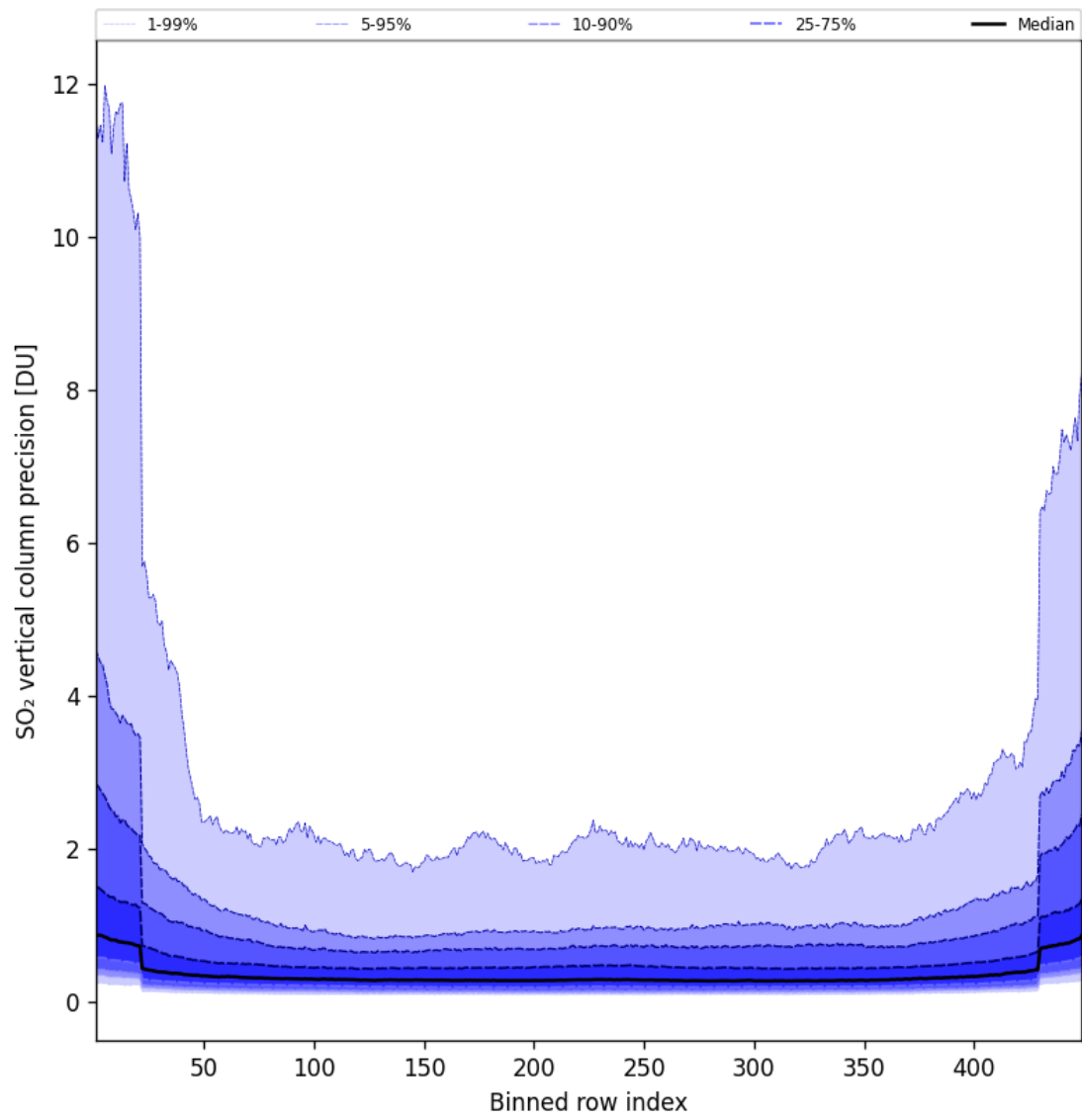
Figure 86: Along track statistics of “SO 2 vertical column precision” for 2025-06-16 to 2025-06-17
