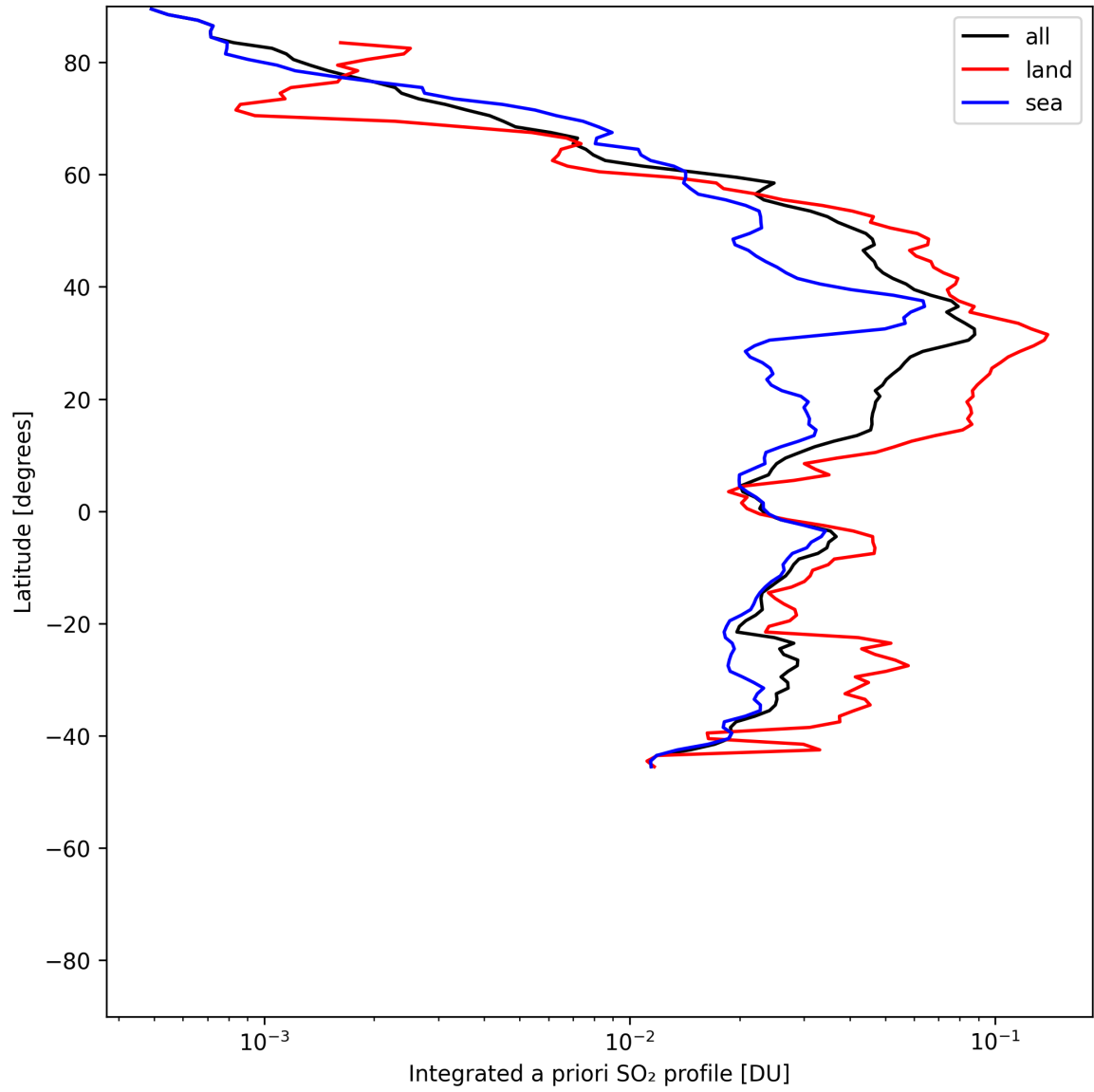
Figure 49: Zonal average of “Integrated a priori SO 2 profile” for 2025-06-16 to 2025-06-17.
