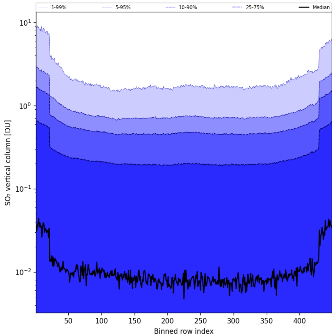
Figure 85: Along track statistics of “SO 2 vertical column” for 2025-06-16 to 2025-06-17
