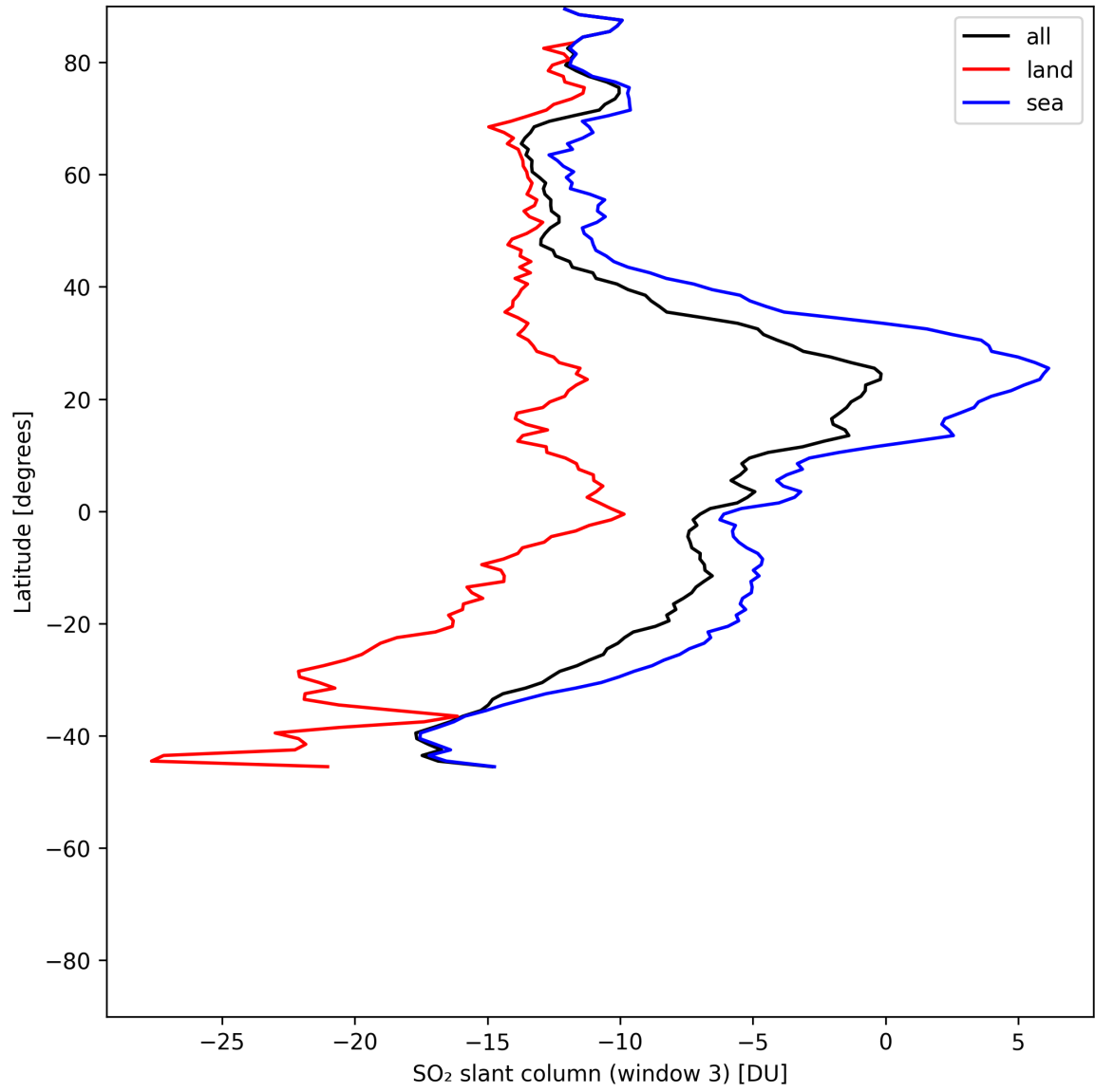
Figure 44: Zonal average of “SO 2 slant column (window 3)” for 2025-06-16 to 2025-06-17.
