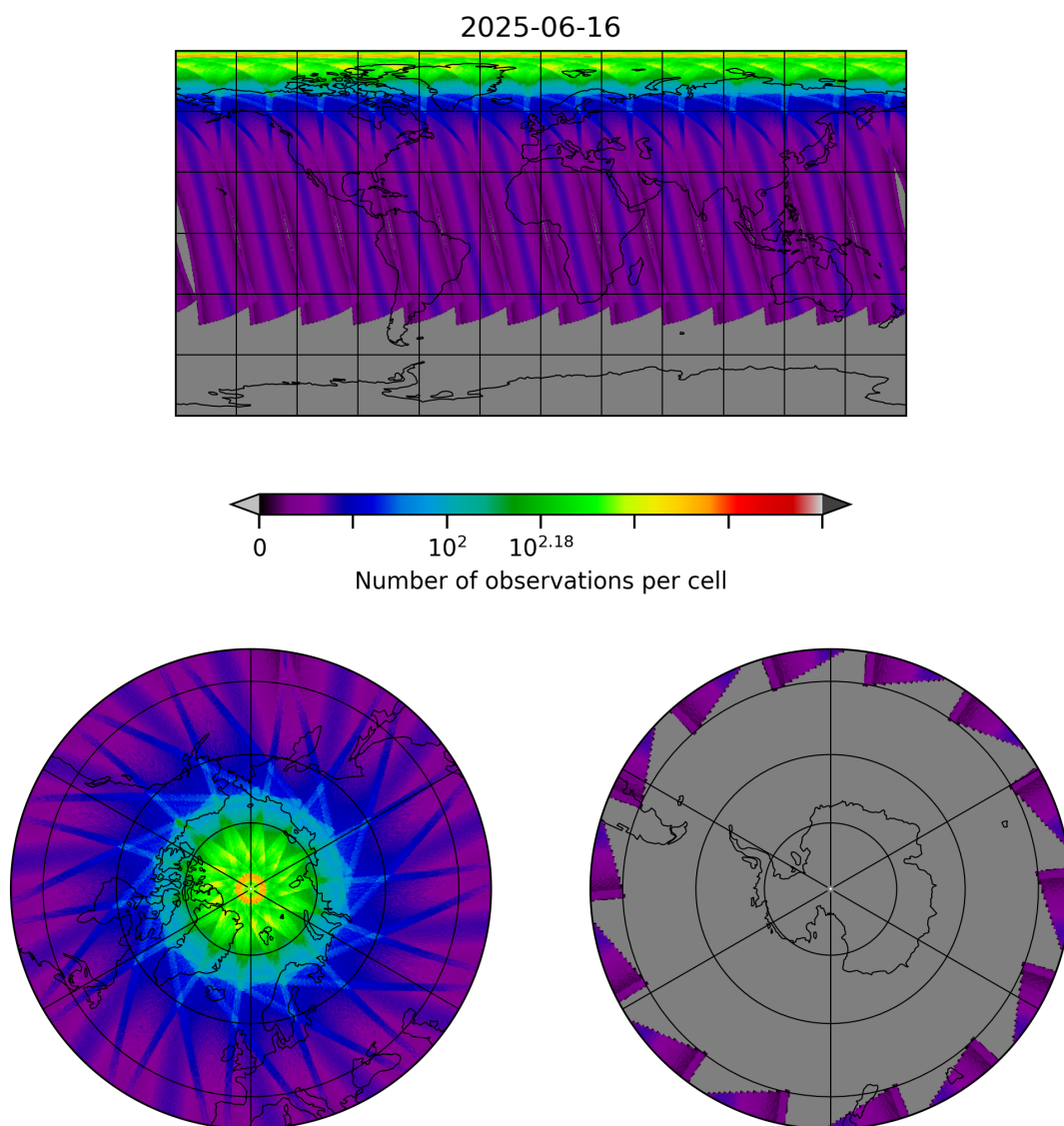
Figure 29: Map of the number of observations for 2025-06-16 to 2025-06-17
