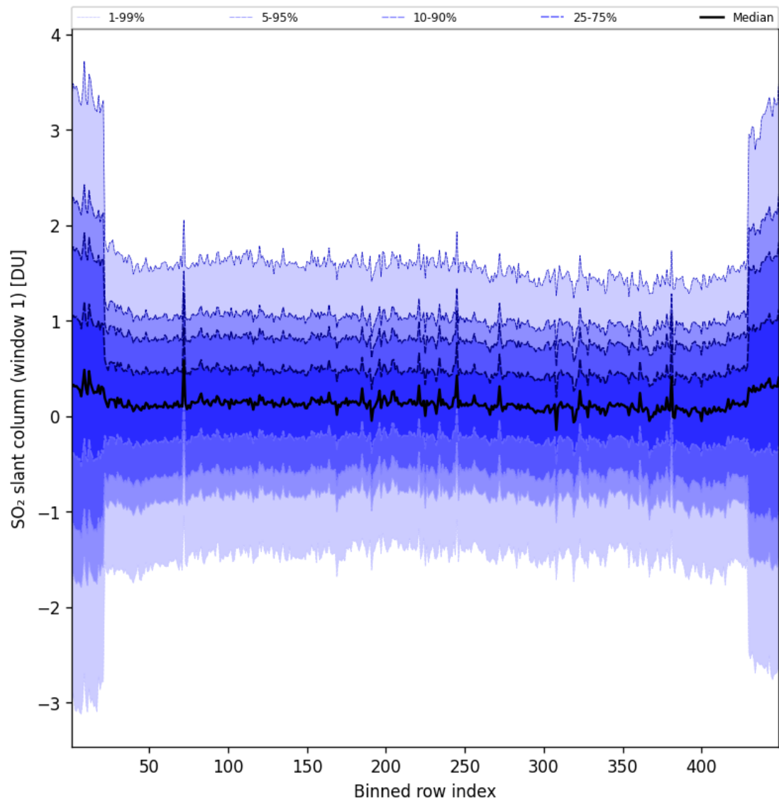
Figure 90: Along track statistics of "SO 2 slant column (window 1)" for 2025-06-16 to 2025-06-17
