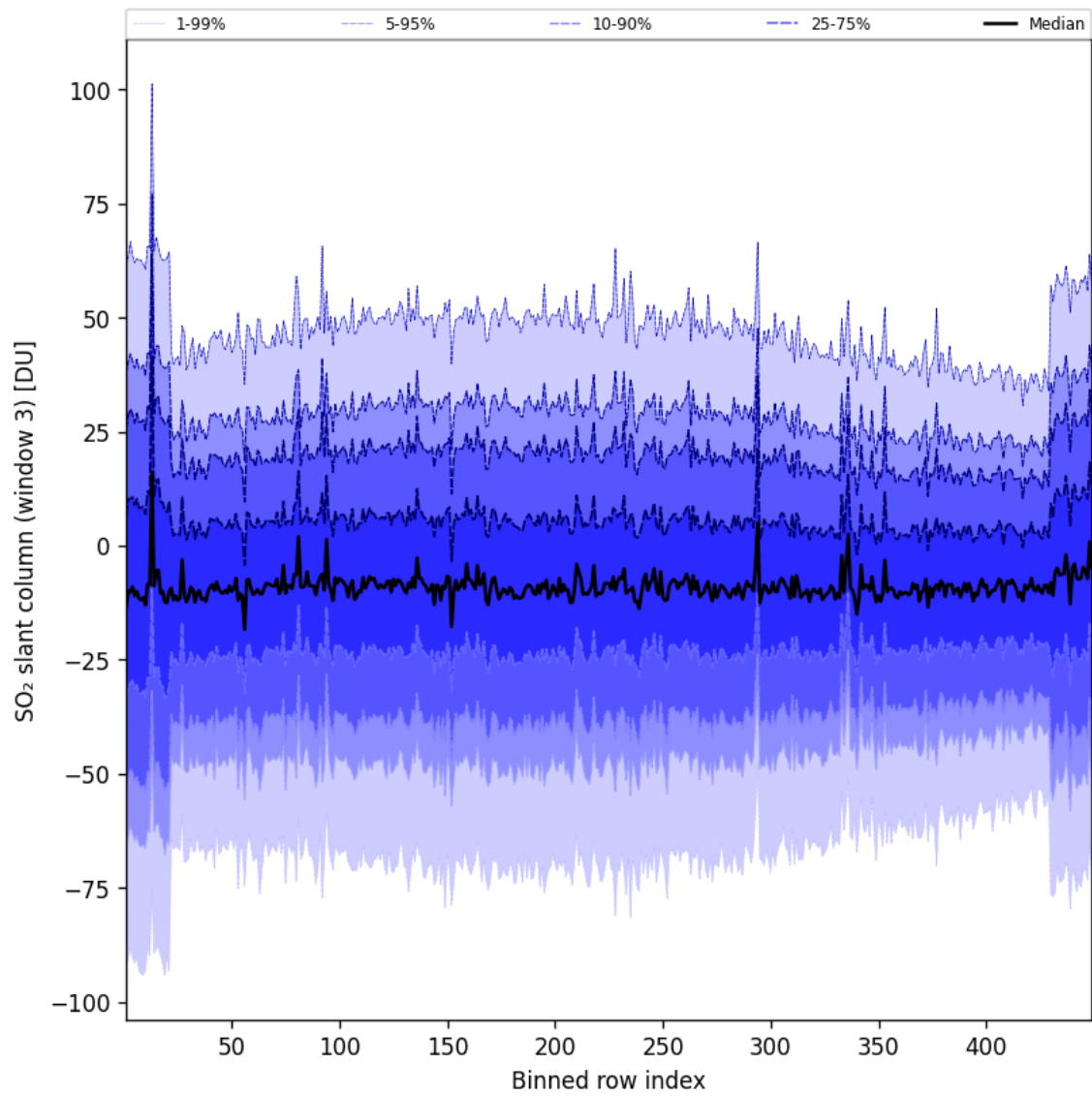
Figure 98: Along track statistics of “SO 2 slant column (window 3)” for 2025-06-16 to 2025-06-17
