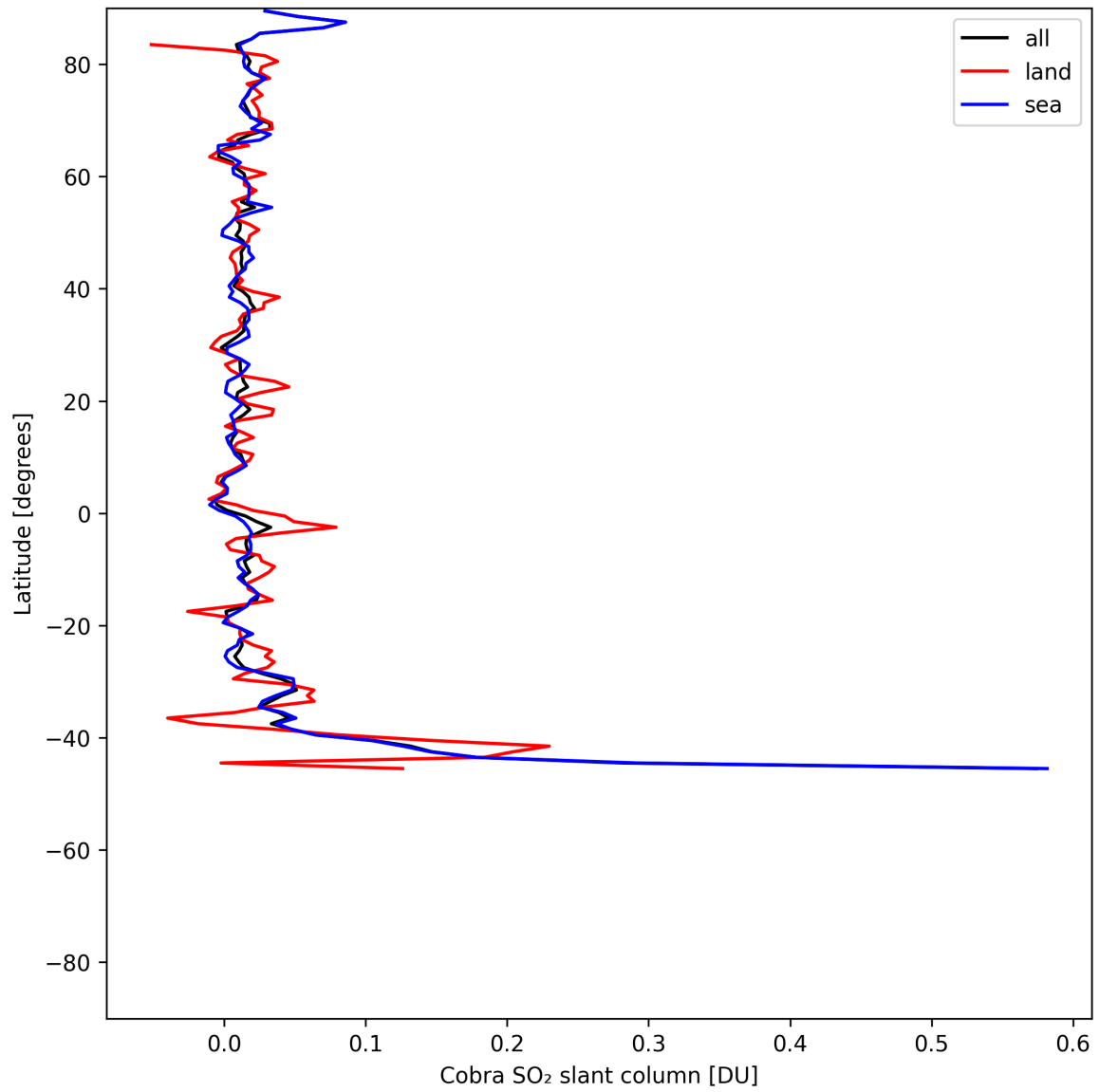
Figure 34: Zonal average of “Cobra SO 2 slant column” for 2025-06-16 to 2025-06-17.
