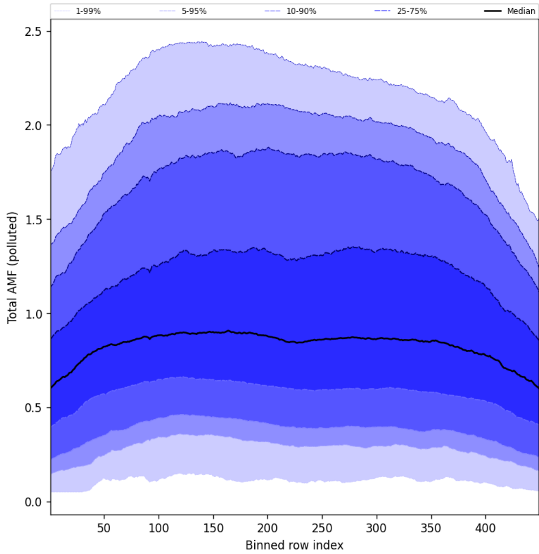
Figure 107: Along track statistics of “Total AMF (polluted)” for 2025-06-16 to 2025-06-17
