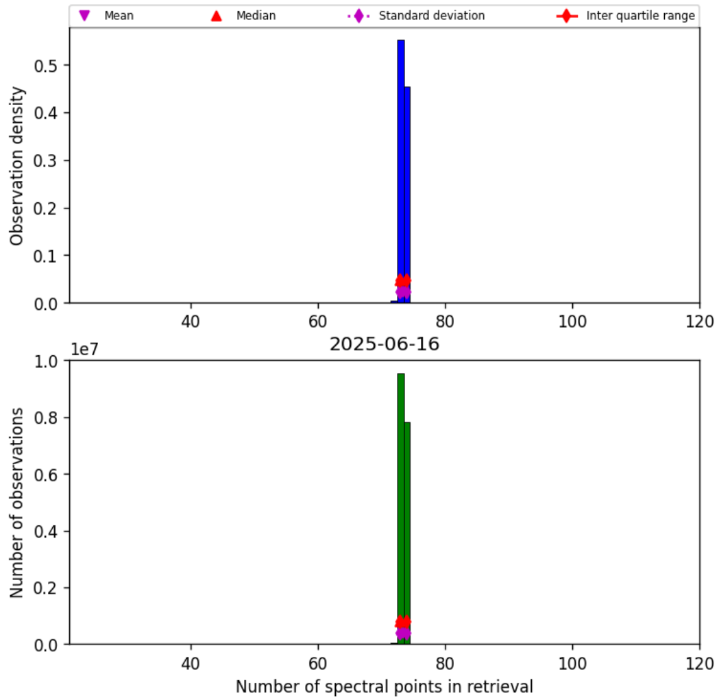
Figure 83: Histogram of “Number of spectral points in retrieval” for 2025-06-16 to 2025-06-17
