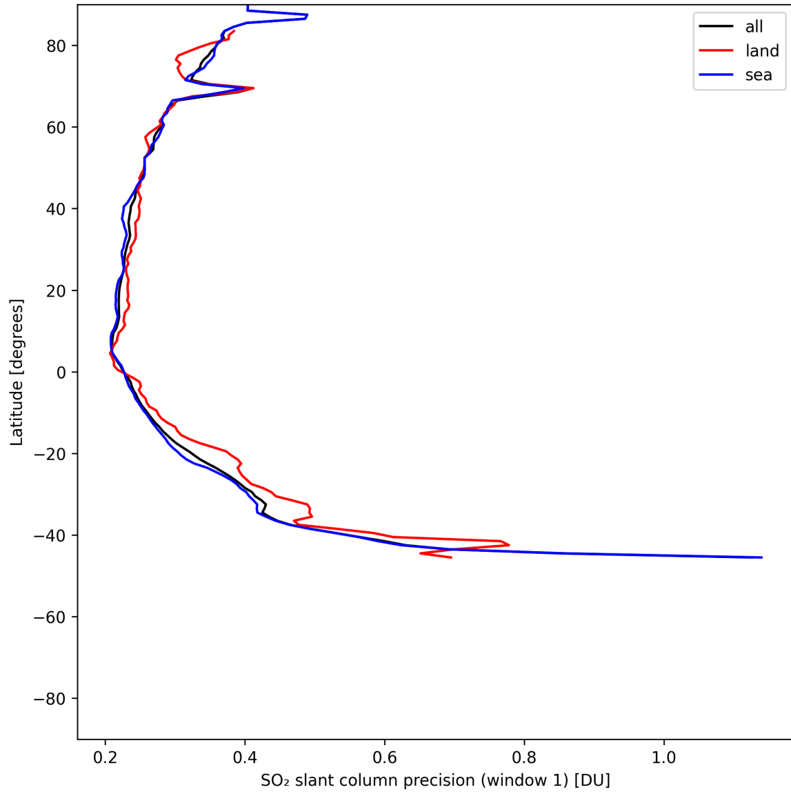
Figure 37: Zonal average of “SO 2 slant column precision (window 1)” for 2025-06-16 to 2025-06-17.
