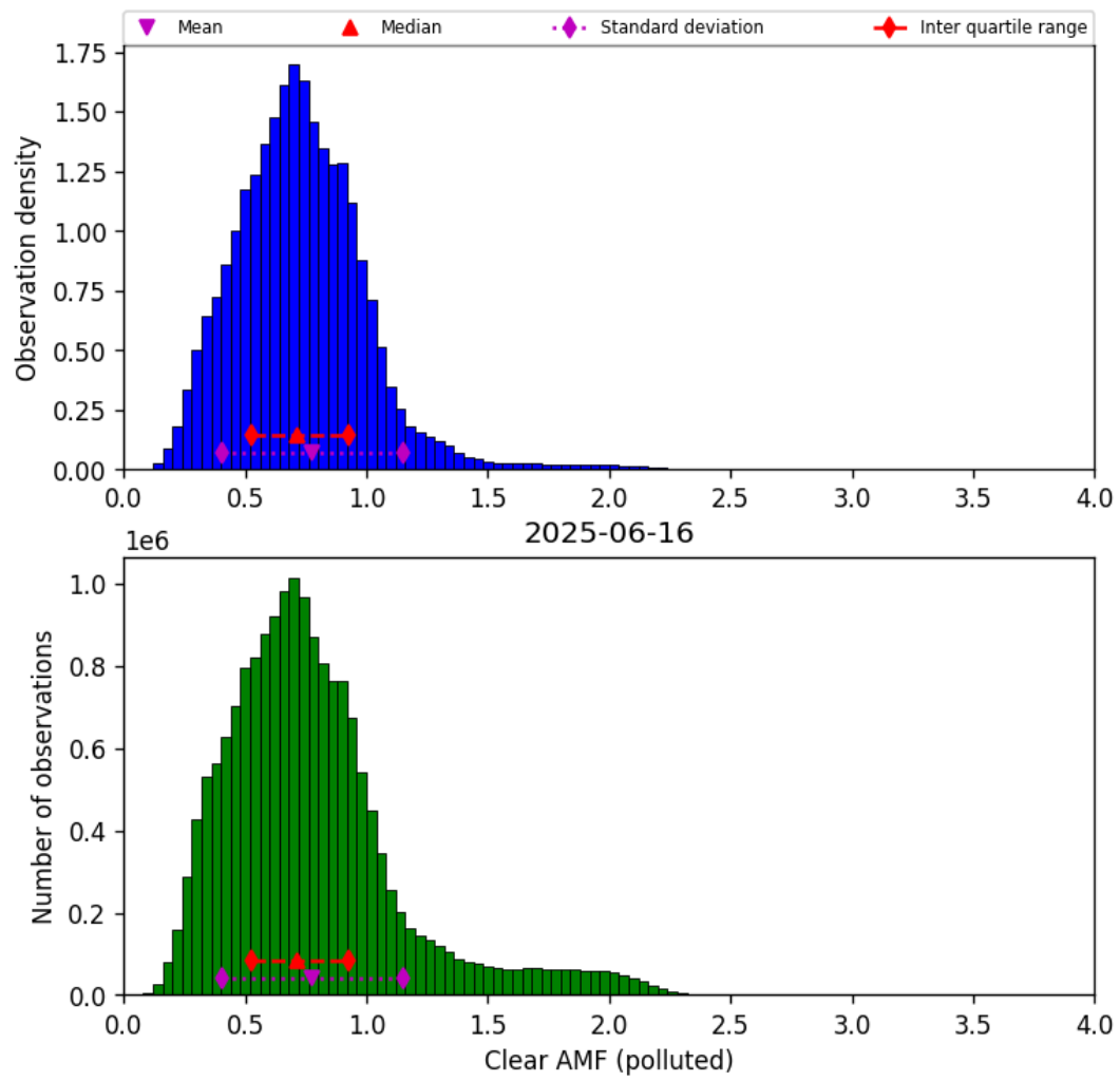
Figure 82: Histogram of “Clear AMF (polluted)” for 2025-06-16 to 2025-06-17
