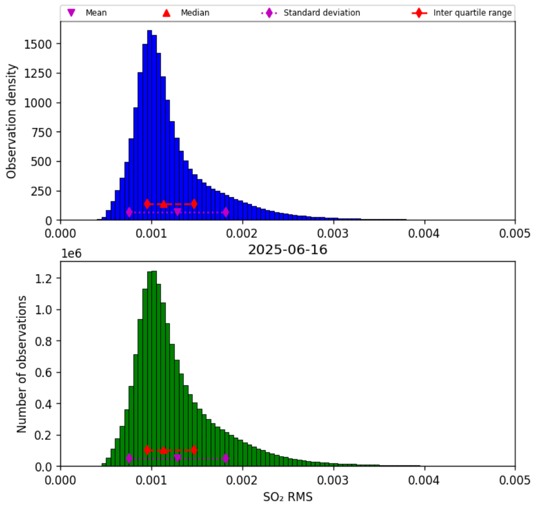
Figure 79: Histogram of “SO 2 RMS” for 2025-06-16 to 2025-06-17
