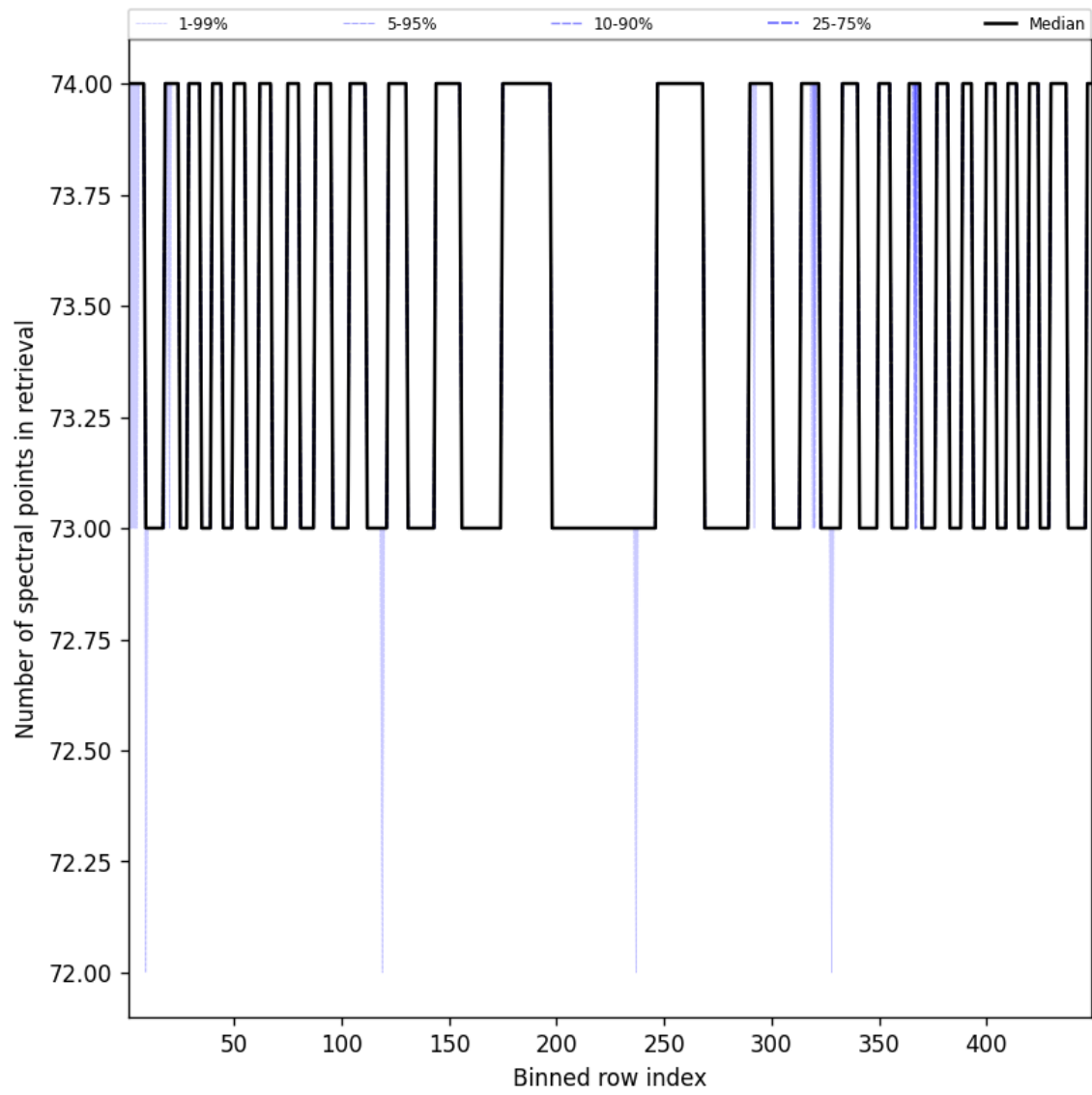
Figure 110: Along track statistics of “Number of spectral points in retrieval” for 2025-06-16 to 2025-06-17
