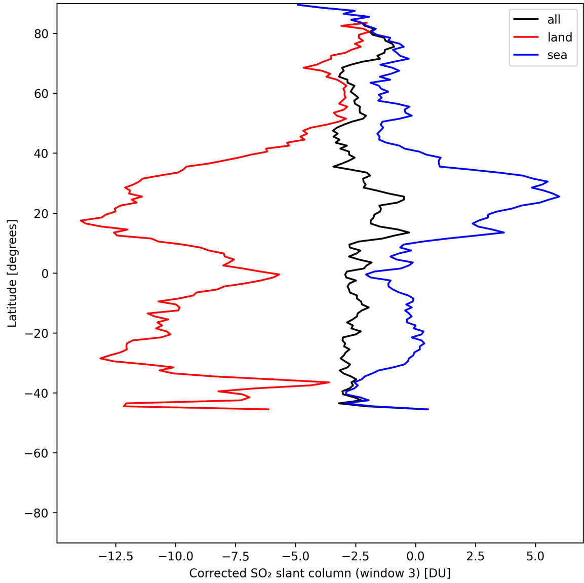
Figure 46: Zonal average of “Corrected SO 2 slant column (window 3)” for 2025-06-16 to 2025-06-17.
