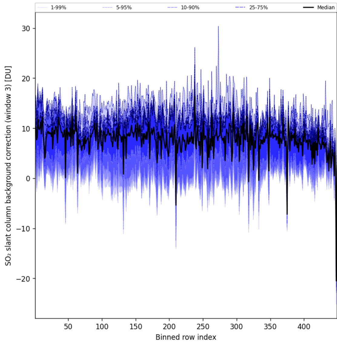
Figure 101: Along track statistics of “SO 2 slant column background correction (window 3)” for 2025-06-16 to 2025-06-17
