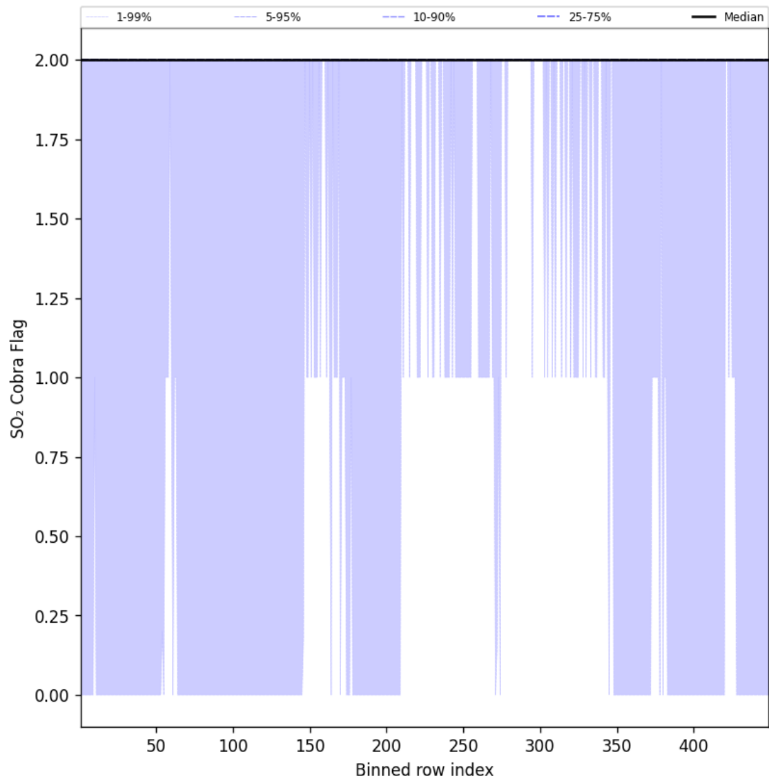
Figure 102: Along track statistics of “SO 2 Cobra Flag” for 2025-06-16 to 2025-06-17
