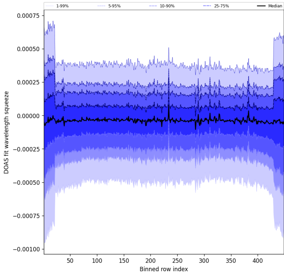
Figure 105: Along track statistics of “DOAS fit wavelength squeeze” for 2025-06-16 to 2025-06-17
