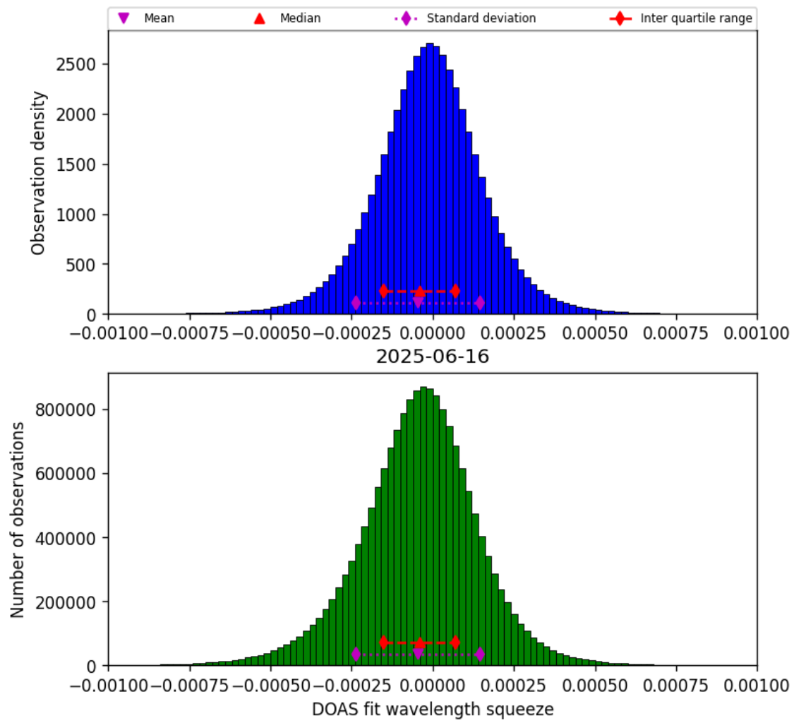
Figure 78: Histogram of “DOAS fit wavelength squeeze” for 2025-06-16 to 2025-06-17
