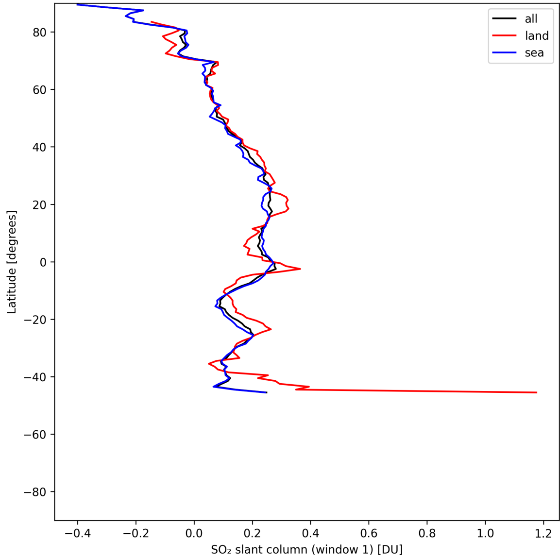
Figure 36: Zonal average of “SO 2 slant column (window 1)” for 2025-06-16 to 2025-06-17.
