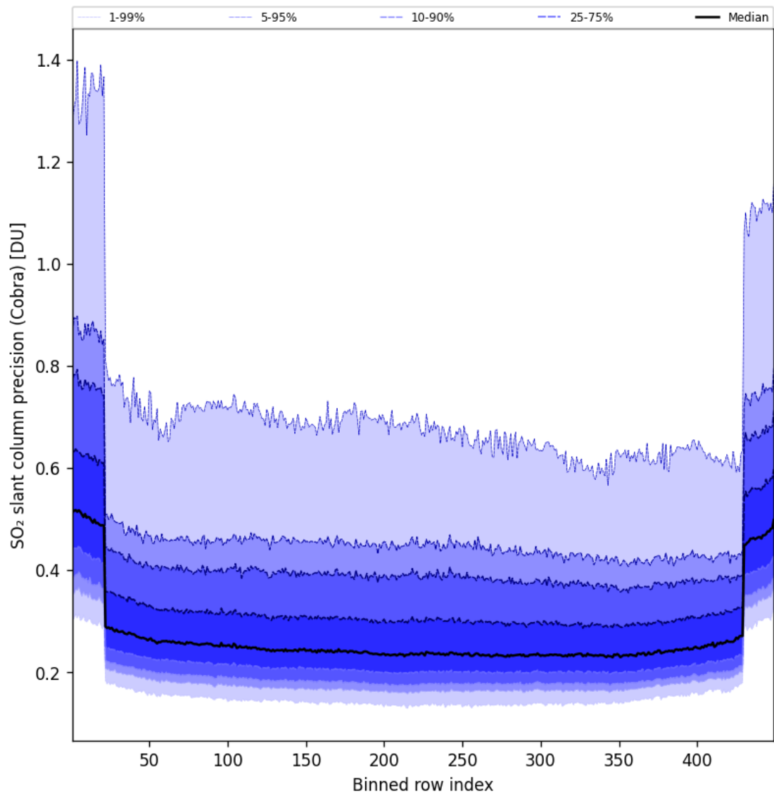
Figure 89: Along track statistics of “SO 2 slant column precision (Cobra)” for 2025-06-16 to 2025-06-17
