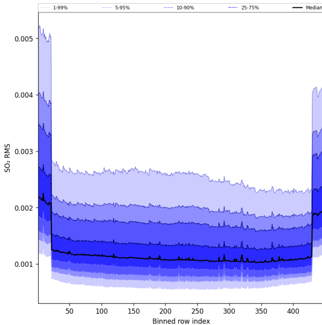
Figure 106: Along track statistics of “SO 2 RMS” for 2025-06-16 to 2025-06-17
