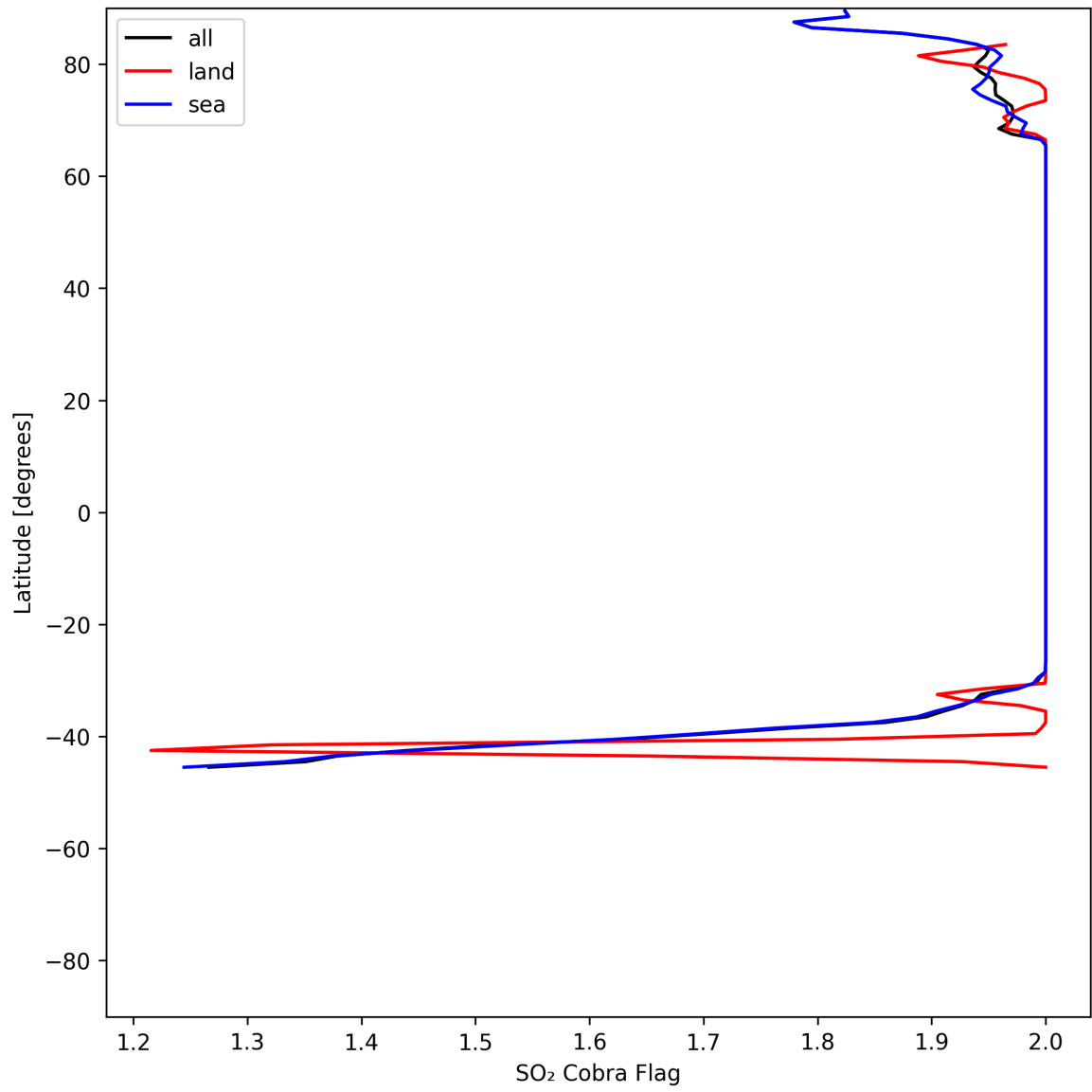
Figure 48: Zonal average of "SO 2 Cobra Flag" for 2025-06-16 to 2025-06-17.
