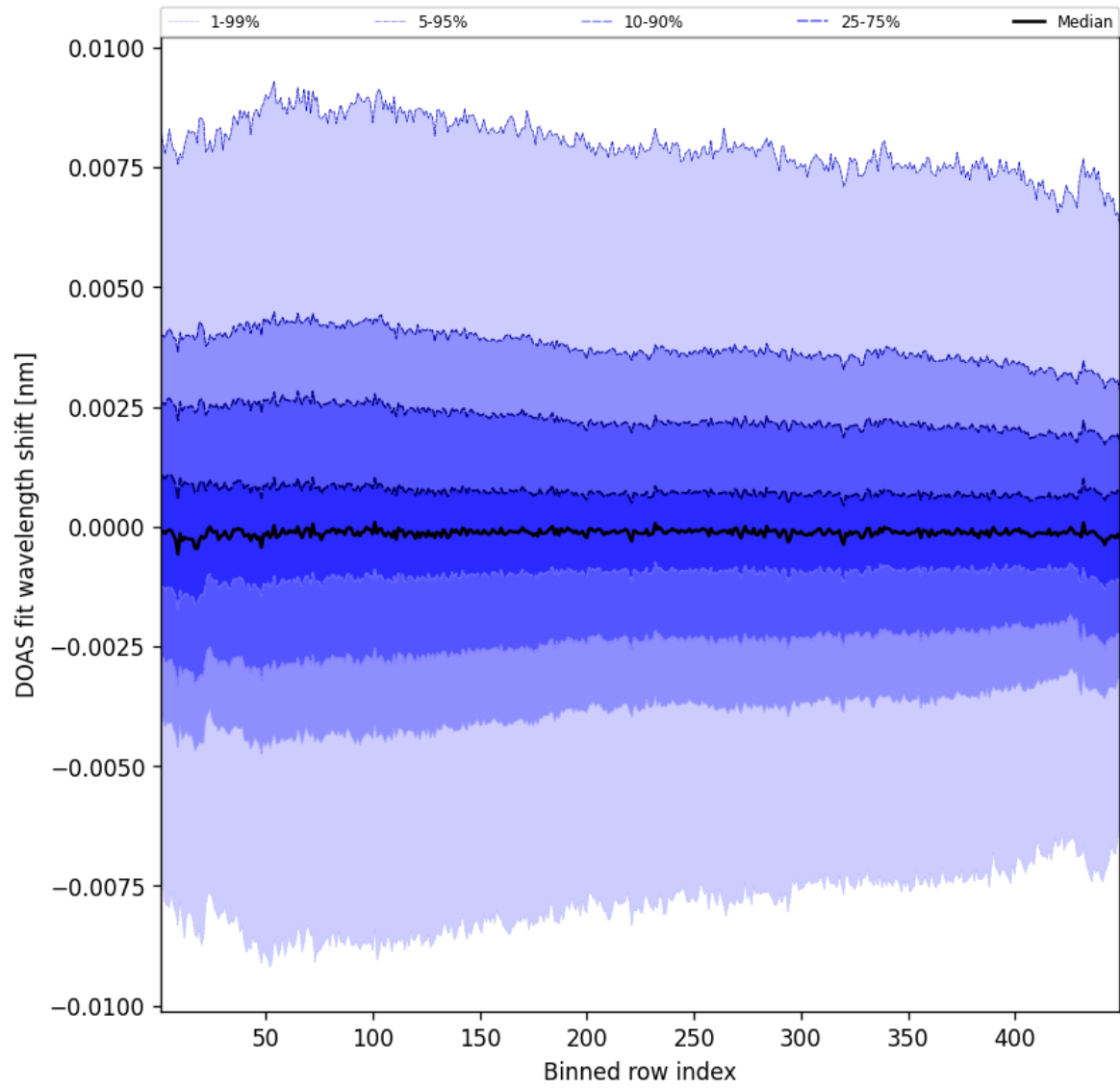
Figure 104: Along track statistics of “DOAS fit wavelength shift” for 2025-06-16 to 2025-06-17
