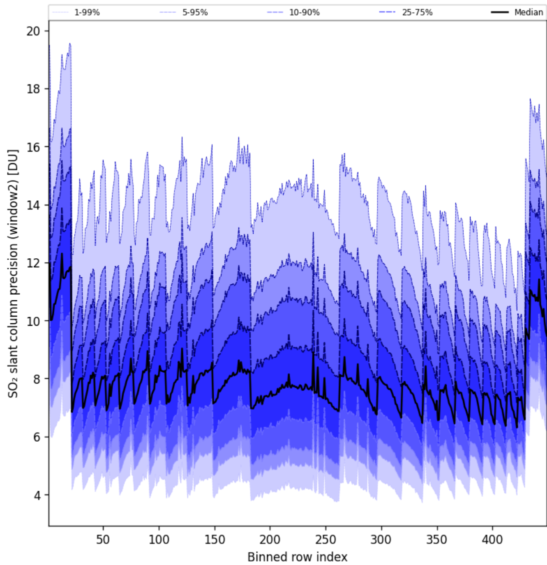
Figure 95: Along track statistics of “SO 2 slant column precision (window2)” for 2025-06-16 to 2025-06-17
