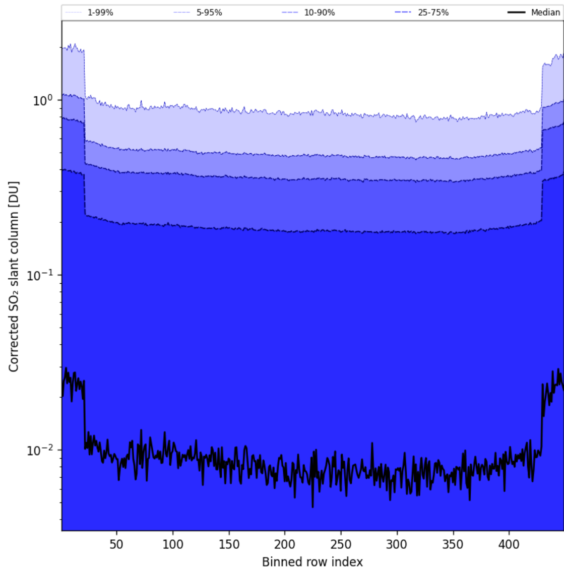
Figure 87: Along track statistics of “Corrected SO 2 slant column” for 2025-06-16 to 2025-06-17
