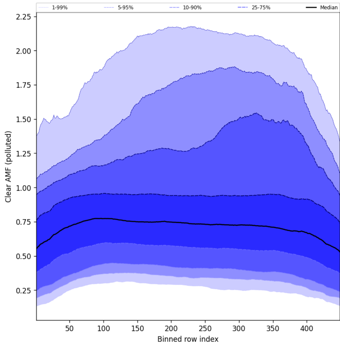
Figure 109: Along track statistics of “Clear AMF (polluted)” for 2025-06-16 to 2025-06-17
