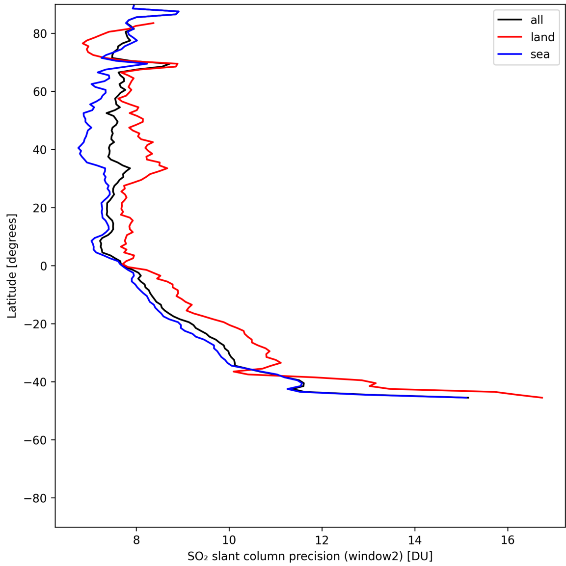
Figure 41: Zonal average of “SO 2 slant column precision (window2)” for 2025-06-16 to 2025-06-17.
