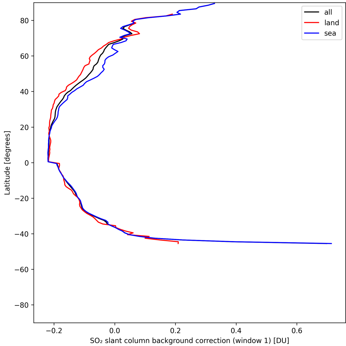
Figure 39: Zonal average of "SO 2 slant column background correction (window 1)" for 2025-06-16 to 2025-06-17.
