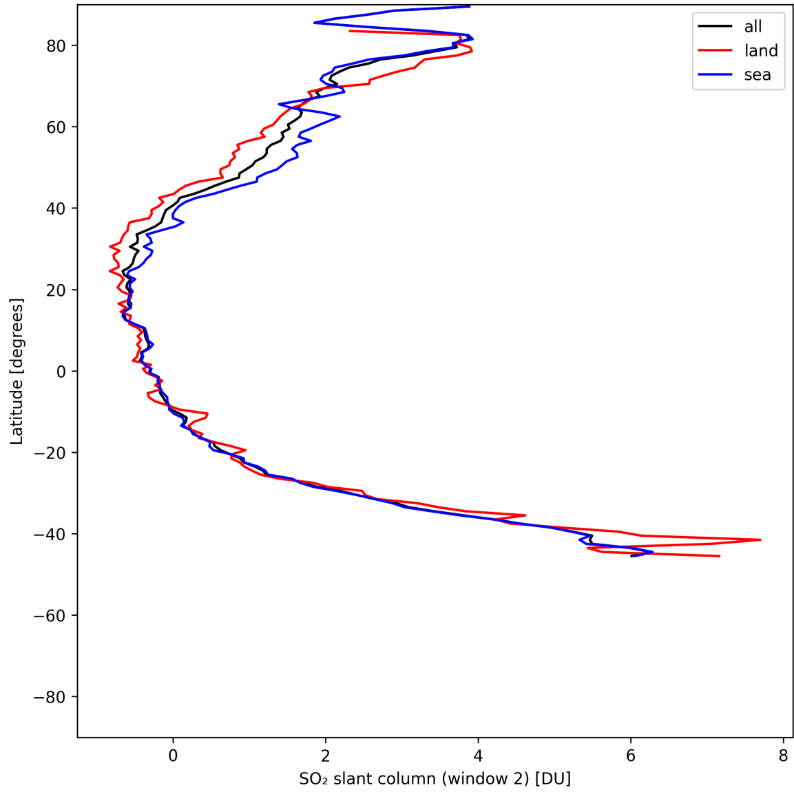
Figure 40: Zonal average of “SO 2 slant column (window 2)” for 2025-06-16 to 2025-06-17.
