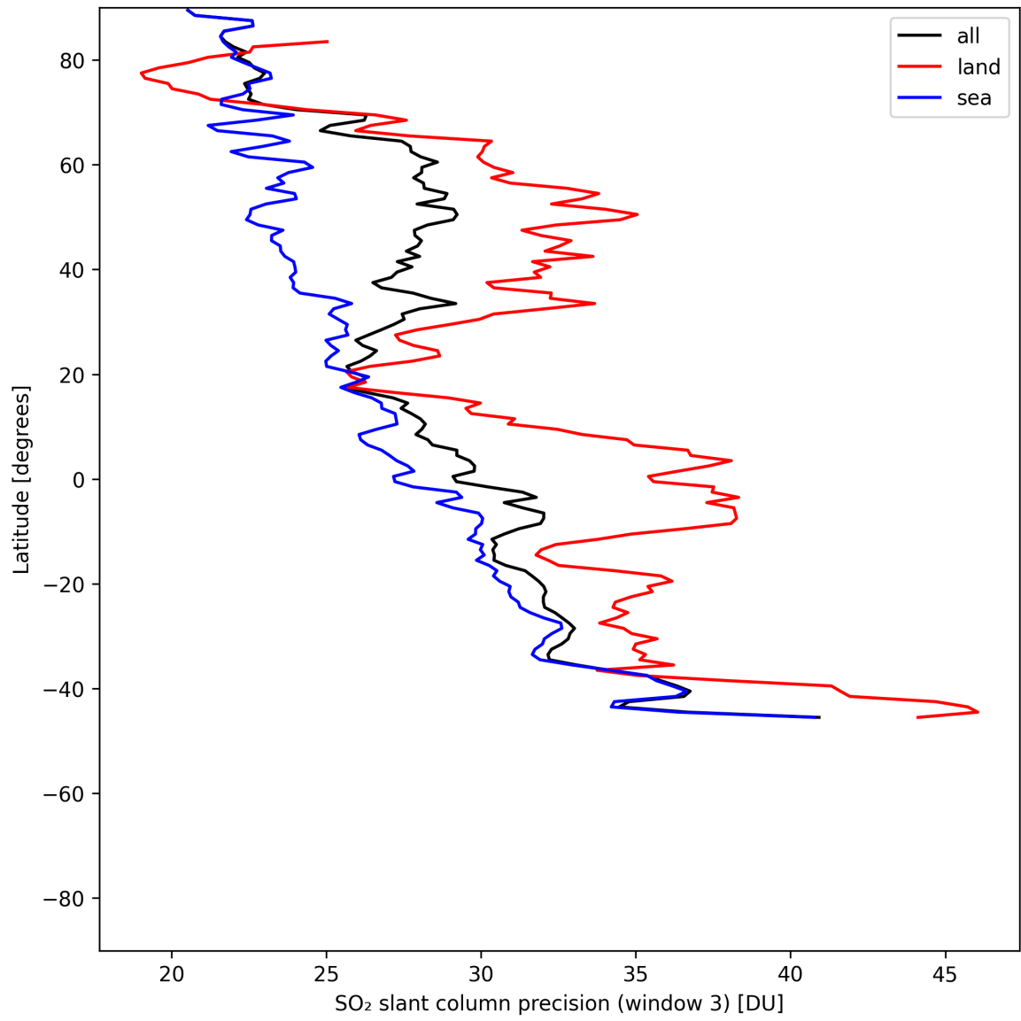
Figure 45: Zonal average of “SO 2 slant column precision (window 3)” for 2025-06-16 to 2025-06-17.
