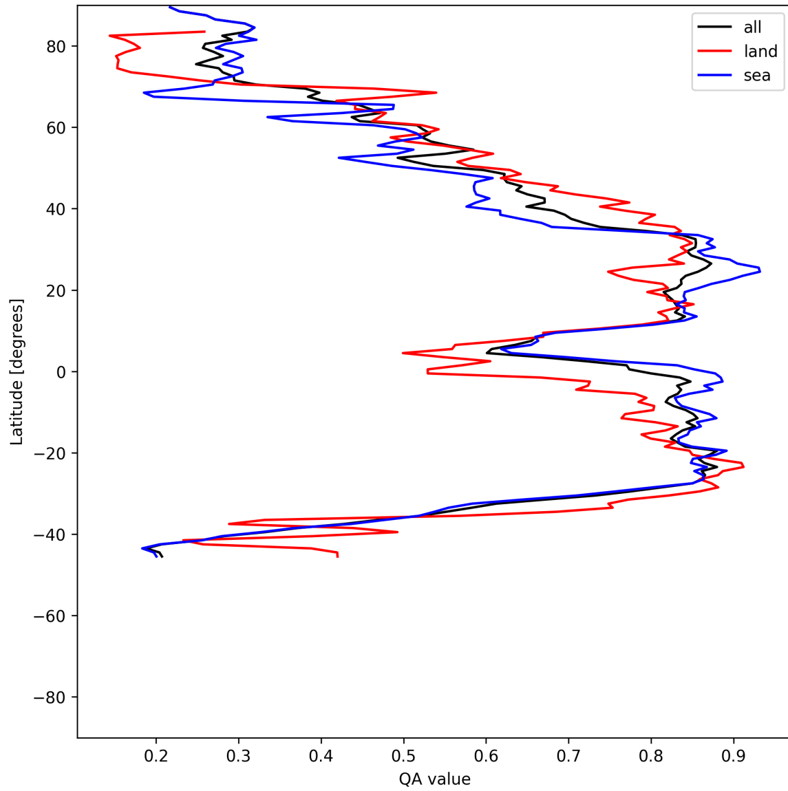
Figure 30: Zonal average of “QA value” for 2025-06-16 to 2025-06-17.
