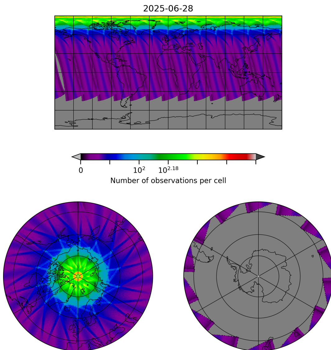
Figure 29: Map of the number of observations for 2025-06-28 to 2025-06-29
