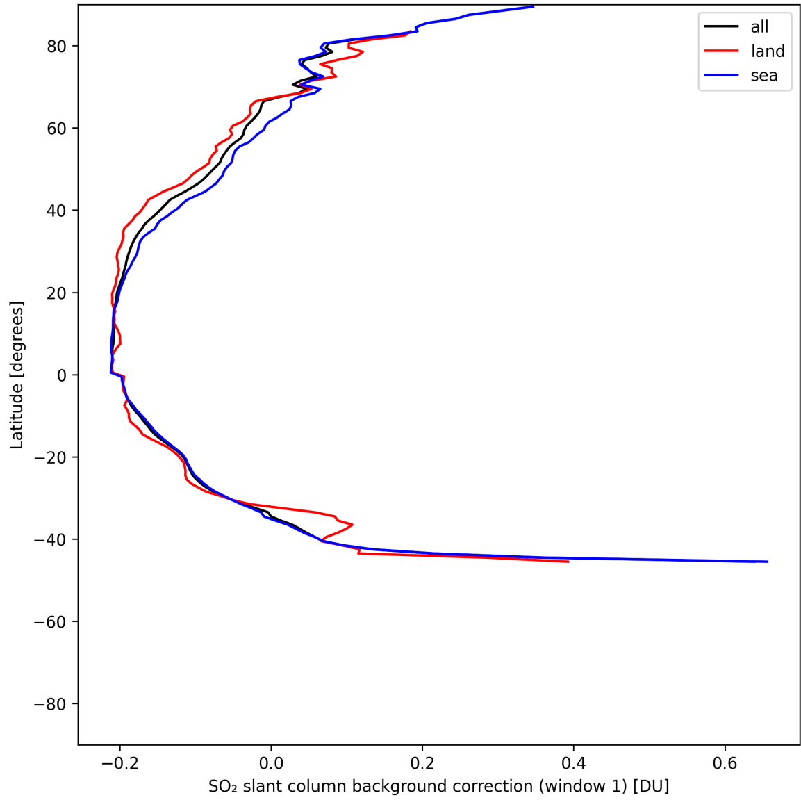
Figure 39: Zonal average of “SO 2 slant column background correction (window 1)” for 2025-06-28 to 2025-06-29.
