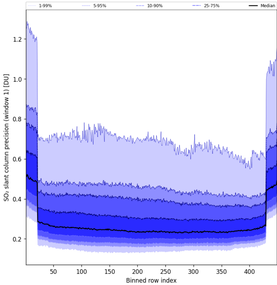
Figure 91: Along track statistics of “SO 2 slant column precision (window 1)” for 2025-06-28 to 2025-06-29
