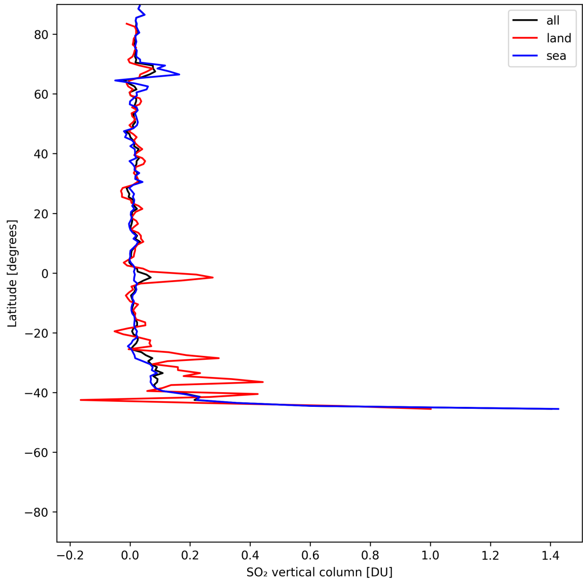
Figure 31: Zonal average of “SO 2 vertical column” for 2025-06-28 to 2025-06-29.
