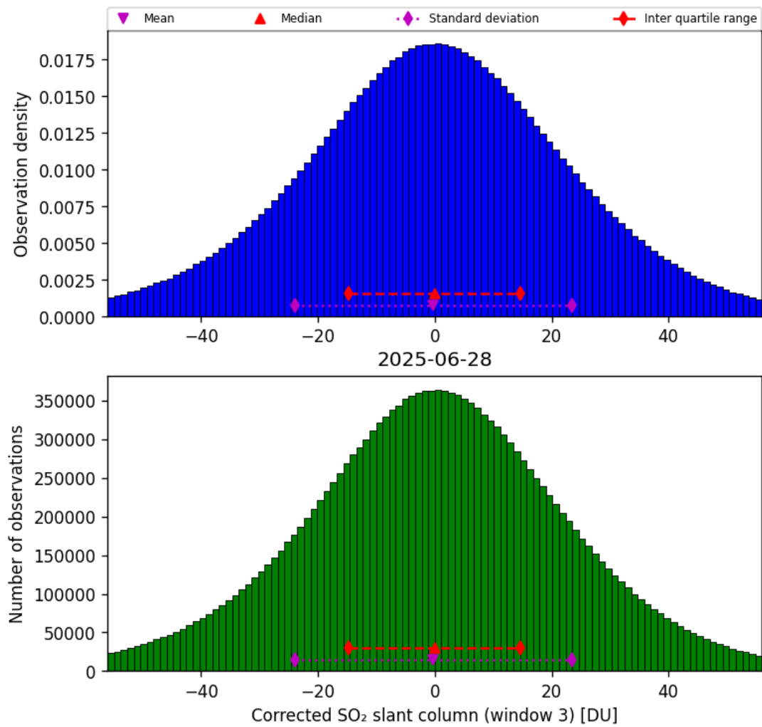
Figure 73: Histogram of “Corrected SO 2 slant column (window 3)” for 2025-06-28 to 2025-06-29
