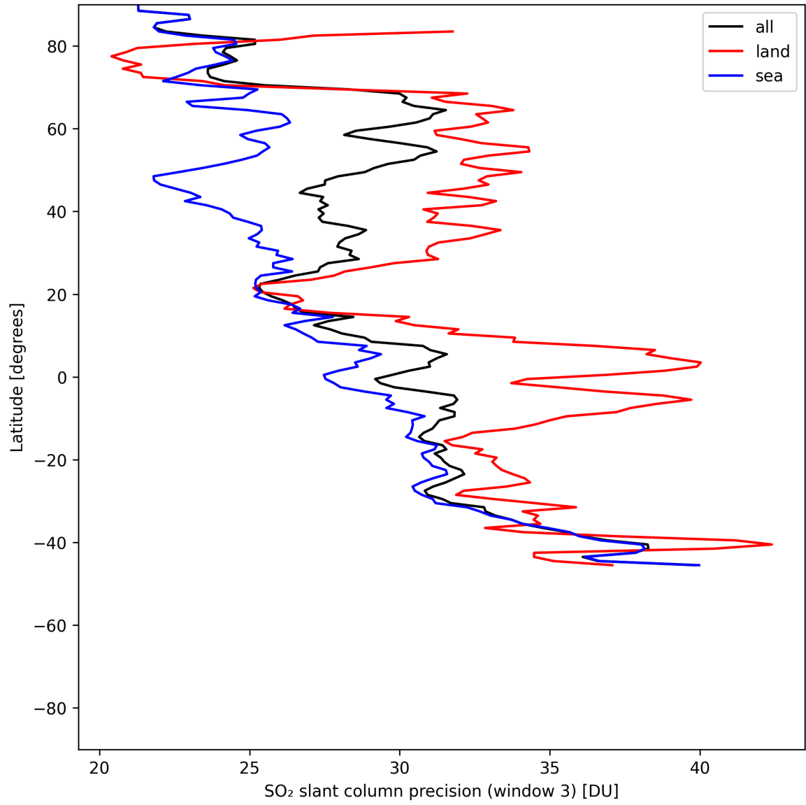
Figure 45: Zonal average of “SO 2 slant column precision (window 3)” for 2025-06-28 to 2025-06-29.
