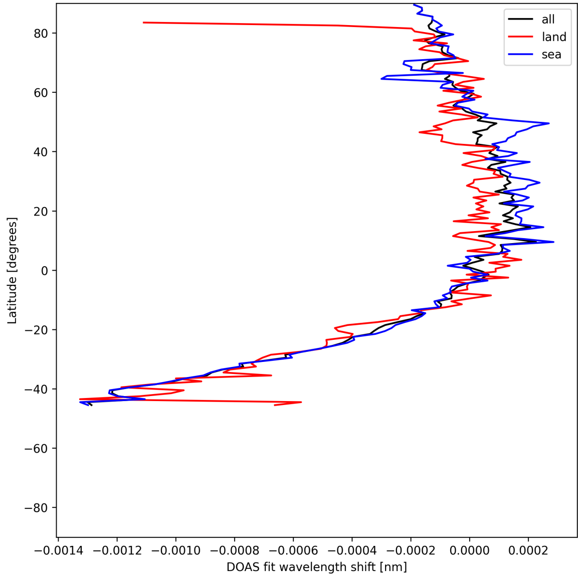
Figure 50: Zonal average of “DOAS fit wavelength shift” for 2025-06-28 to 2025-06-29.
