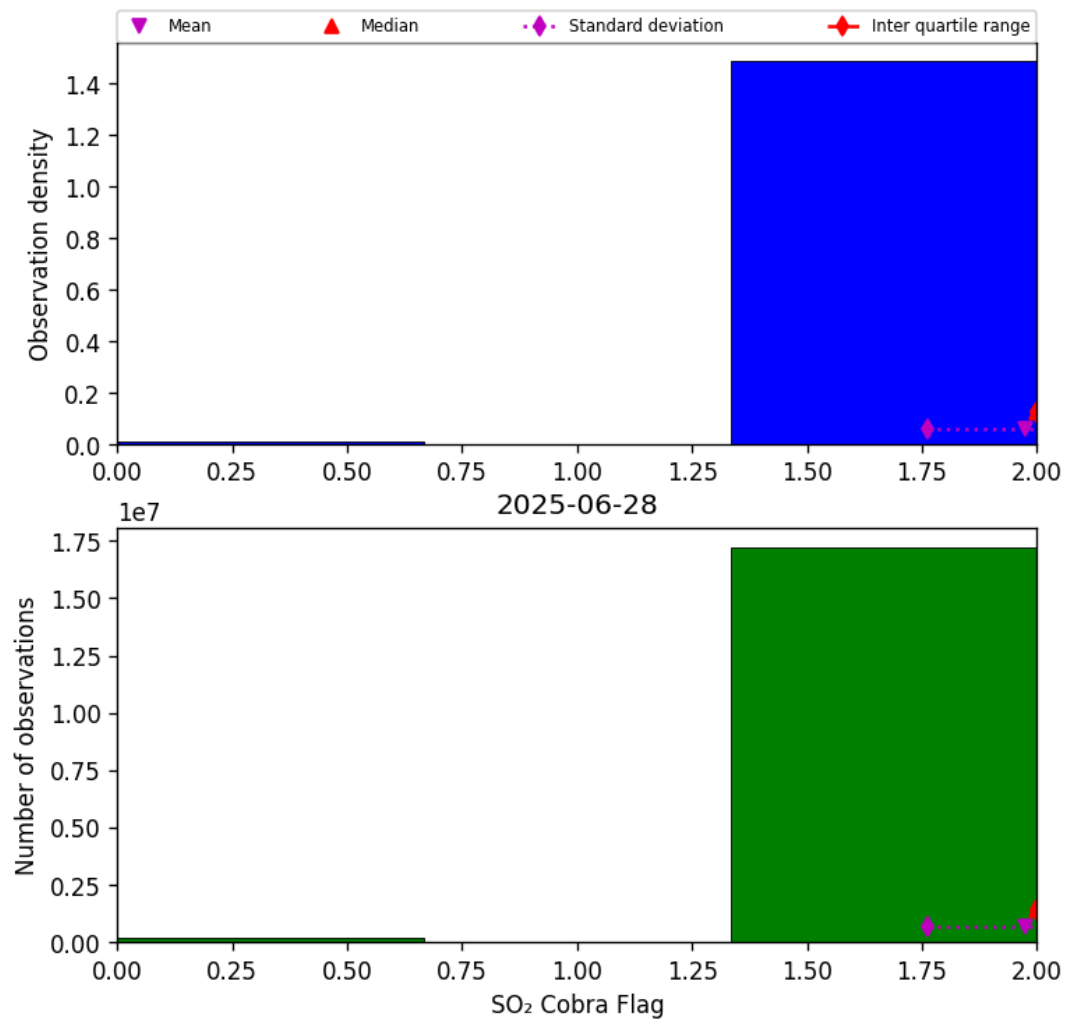
Figure 75: Histogram of “SO 2 Cobra Flag” for 2025-06-28 to 2025-06-29
