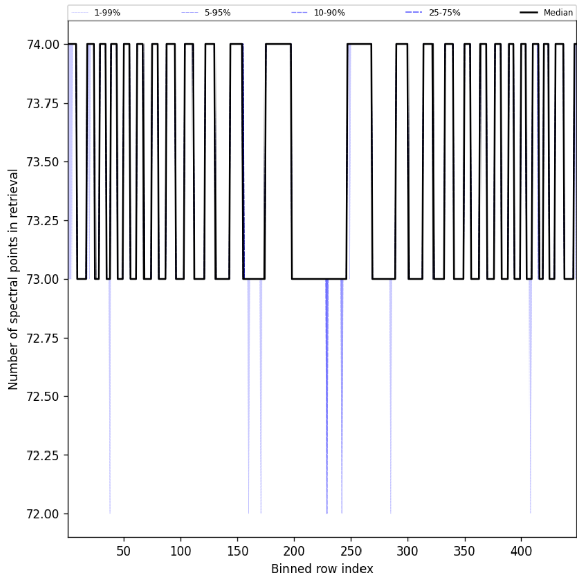
Figure 110: Along track statistics of “Number of spectral points in retrieval” for 2025-06-28 to 2025-06-29
