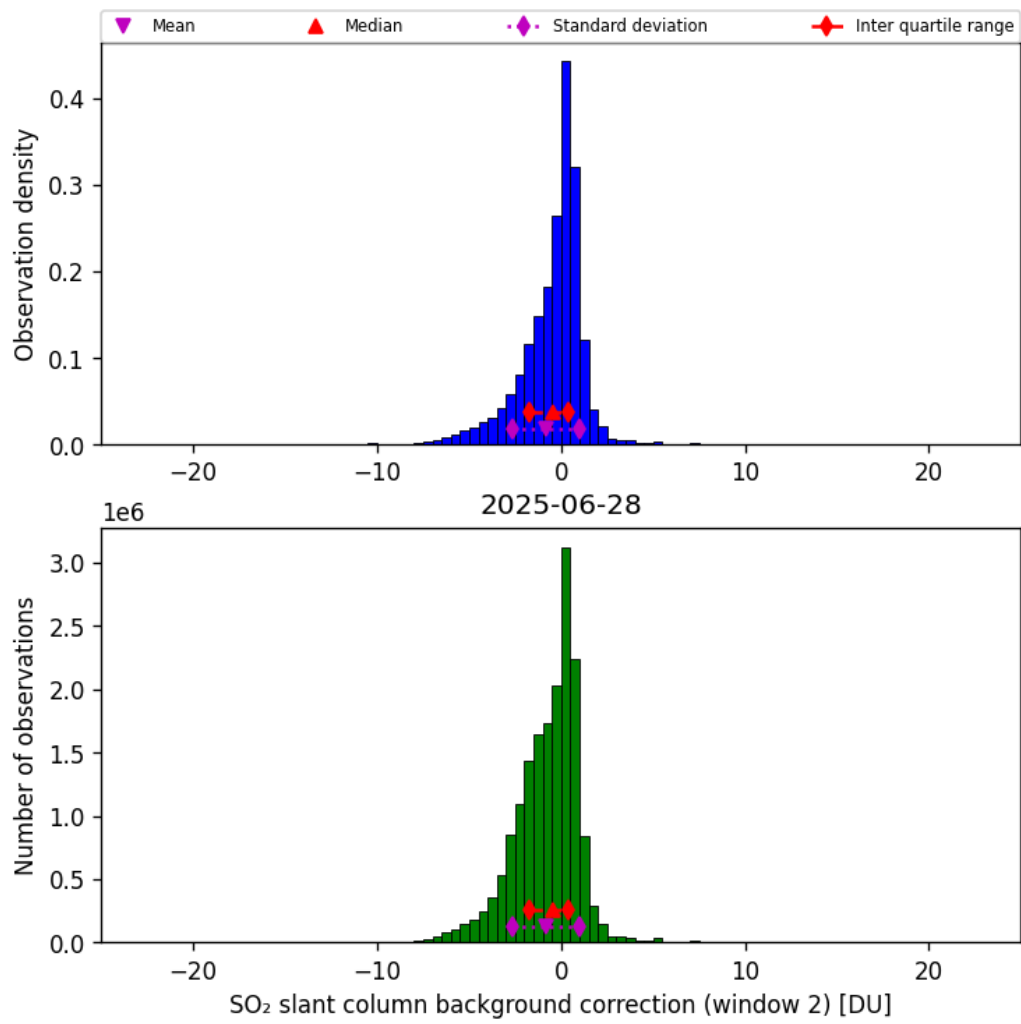
Figure 70: Histogram of “SO 2 slant column background correction (window 2)” for 2025-06-28 to 2025-06-29
