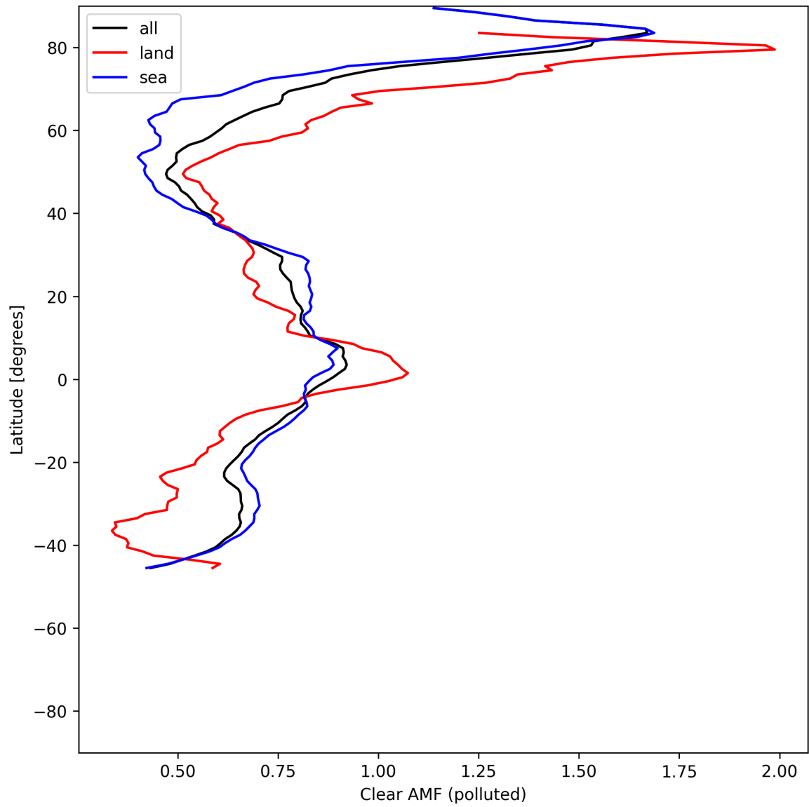
Figure 55: Zonal average of “Clear AMF (polluted)” for 2025-06-28 to 2025-06-29.
