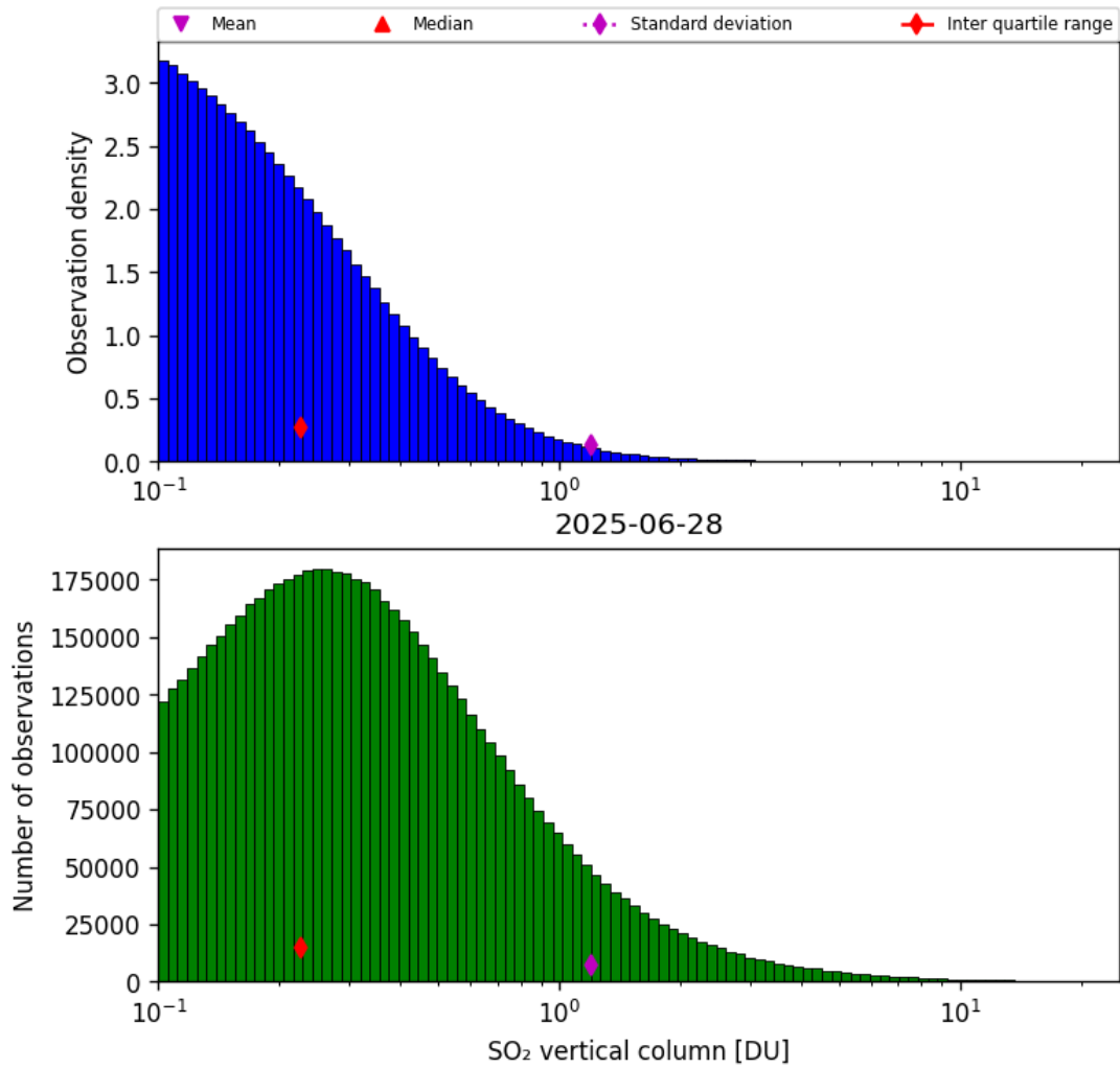
Figure 58: Histogram of “SO 2 vertical column” for 2025-06-28 to 2025-06-29
