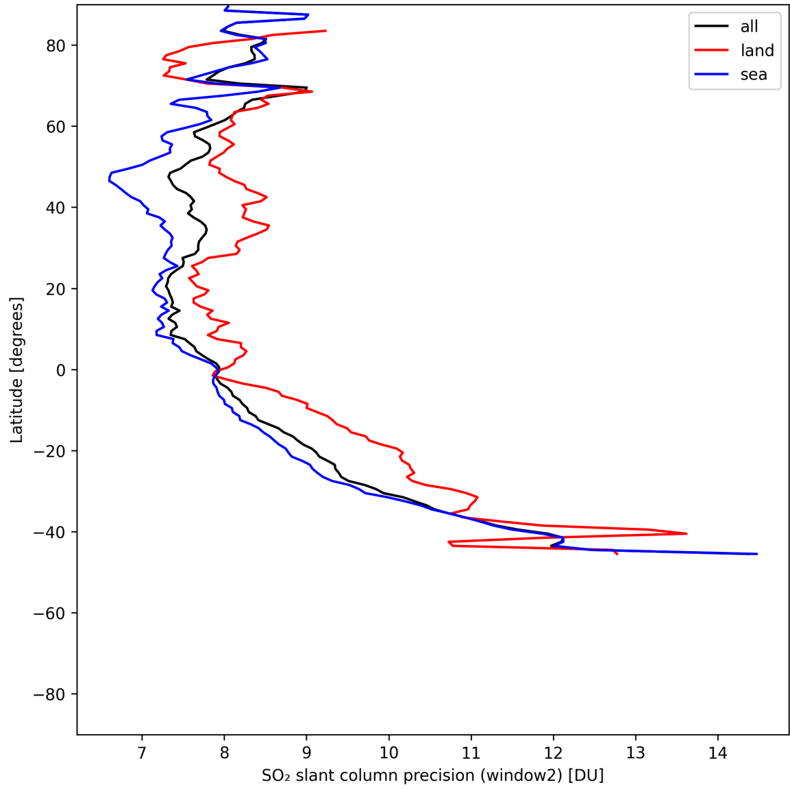
Figure 41: Zonal average of “SO 2 slant column precision (window2)” for 2025-06-28 to 2025-06-29.
