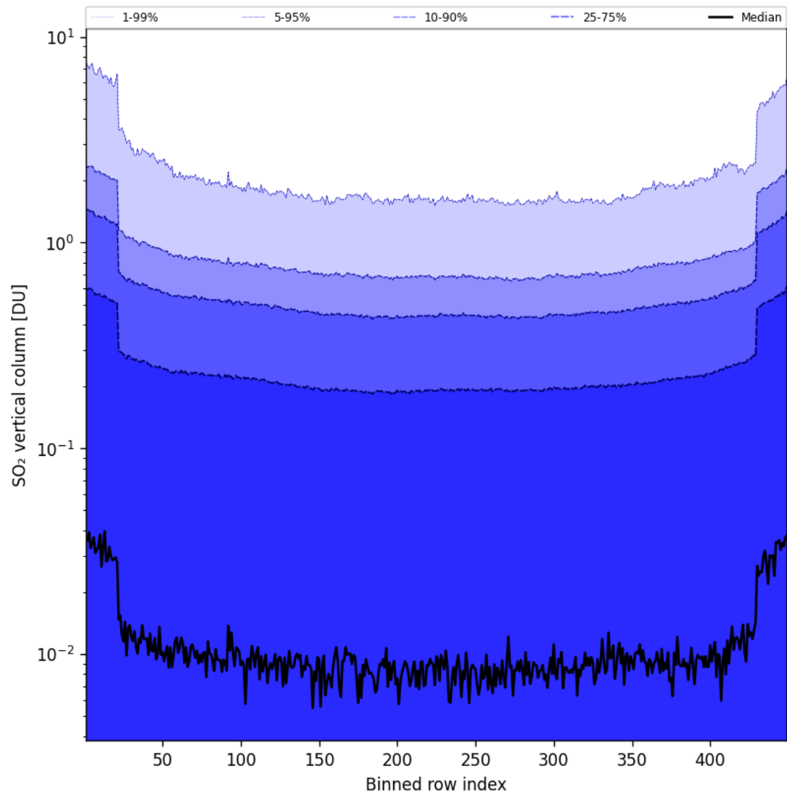
Figure 85: Along track statistics of “SO 2 vertical column” for 2025-06-28 to 2025-06-29
