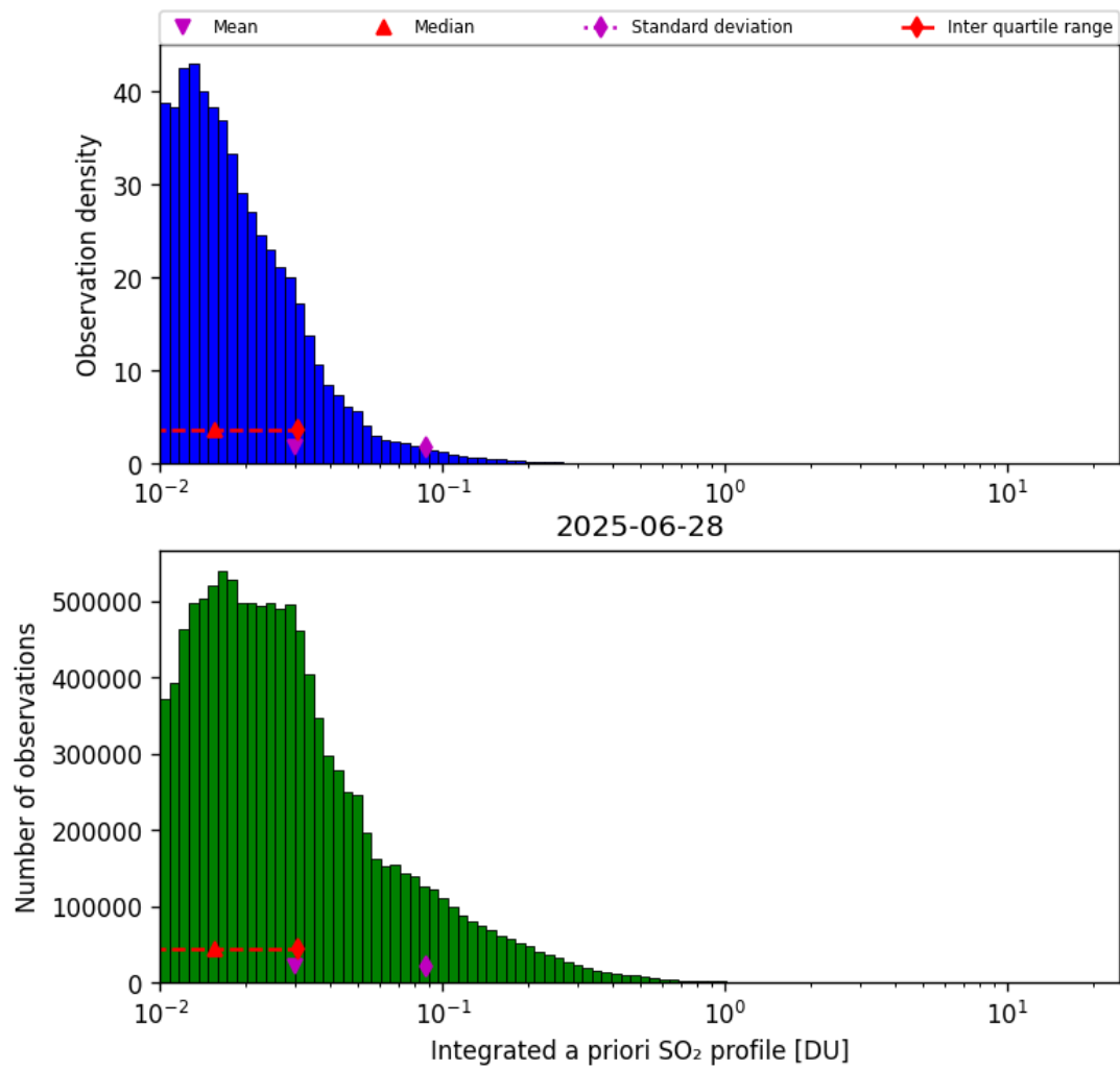
Figure 76: Histogram of “Integrated a priori SO 2 profile” for 2025-06-28 to 2025-06-29
