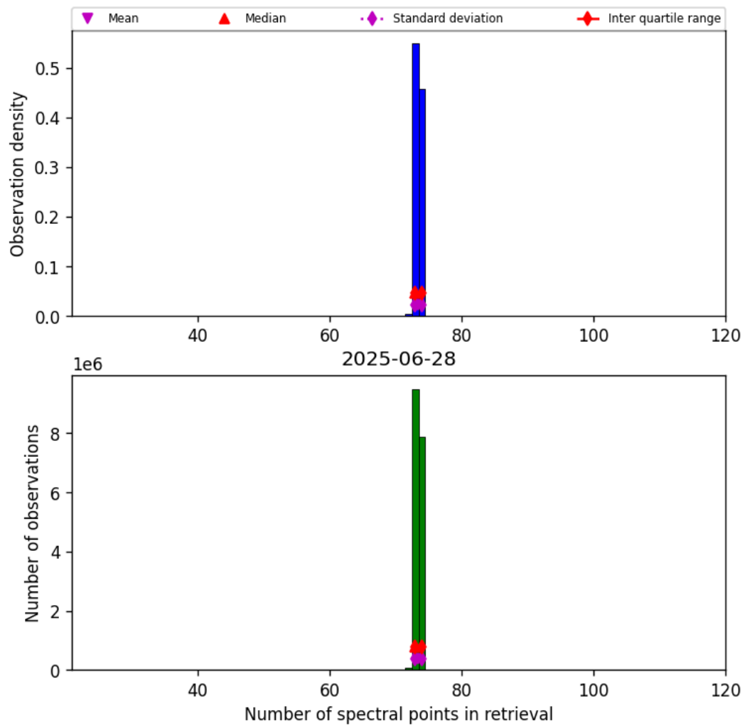
Figure 83: Histogram of “Number of spectral points in retrieval” for 2025-06-28 to 2025-06-29
