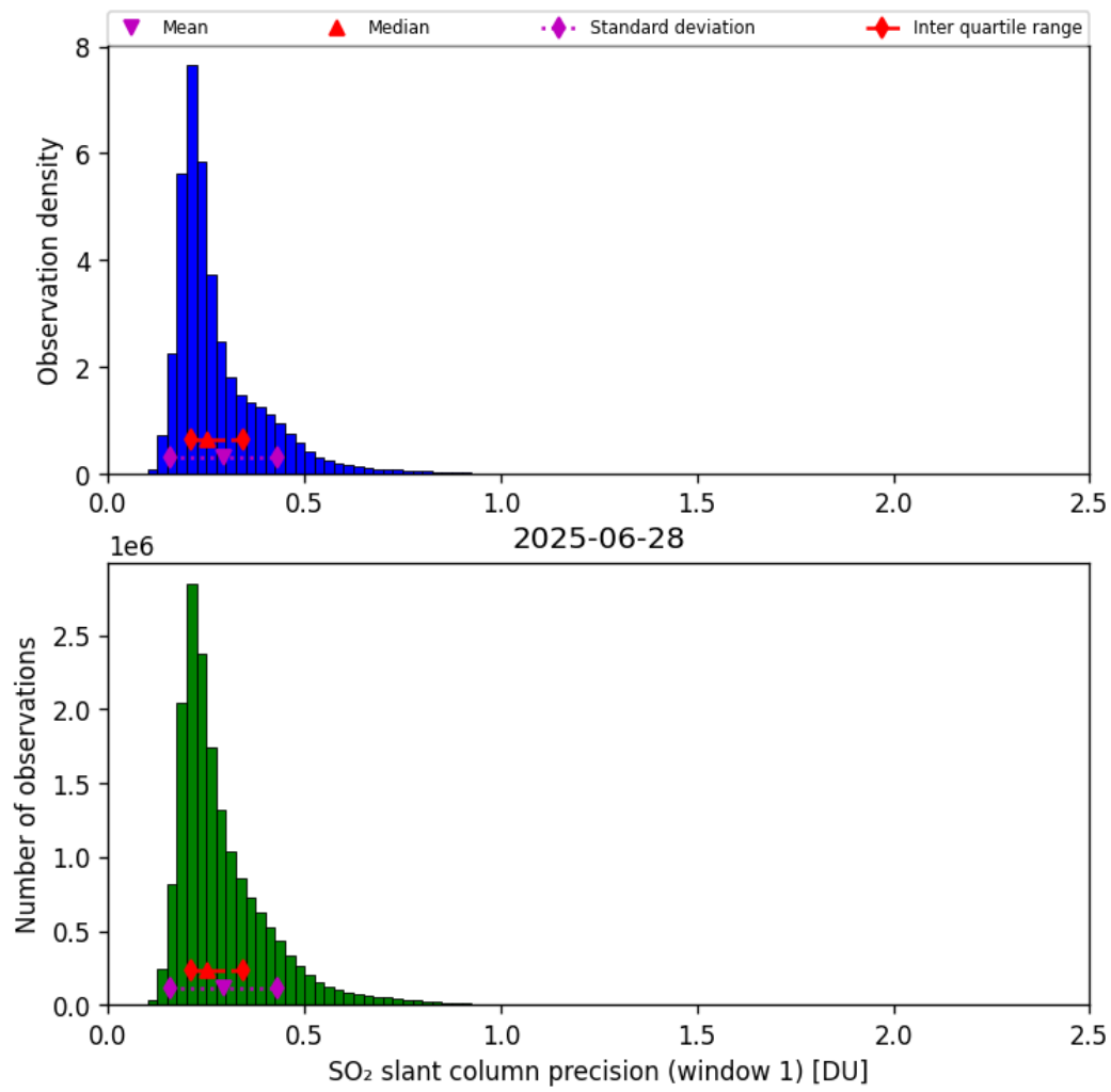
Figure 64: Histogram of “SO 2 slant column precision (window 1)” for 2025-06-28 to 2025-06-29
