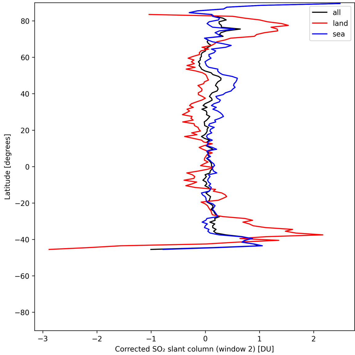
Figure 42: Zonal average of “Corrected SO 2 slant column (window 2)” for 2025-06-28 to 2025-06-29.
