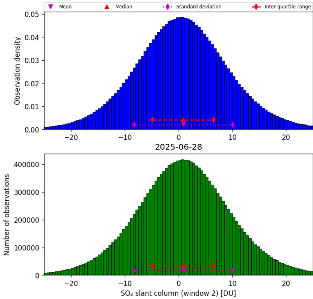
Figure 67: Histogram of “SO 2 slant column (window 2)” for 2025-06-28 to 2025-06-29
