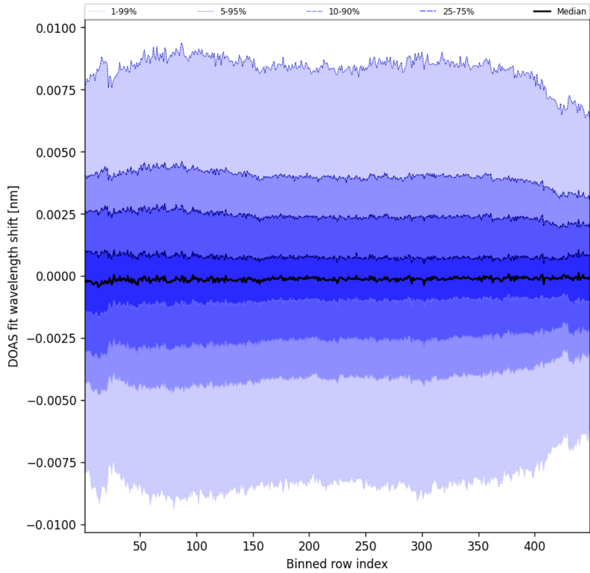
Figure 104: Along track statistics of “DOAS fit wavelength shift” for 2025-06-28 to 2025-06-29
