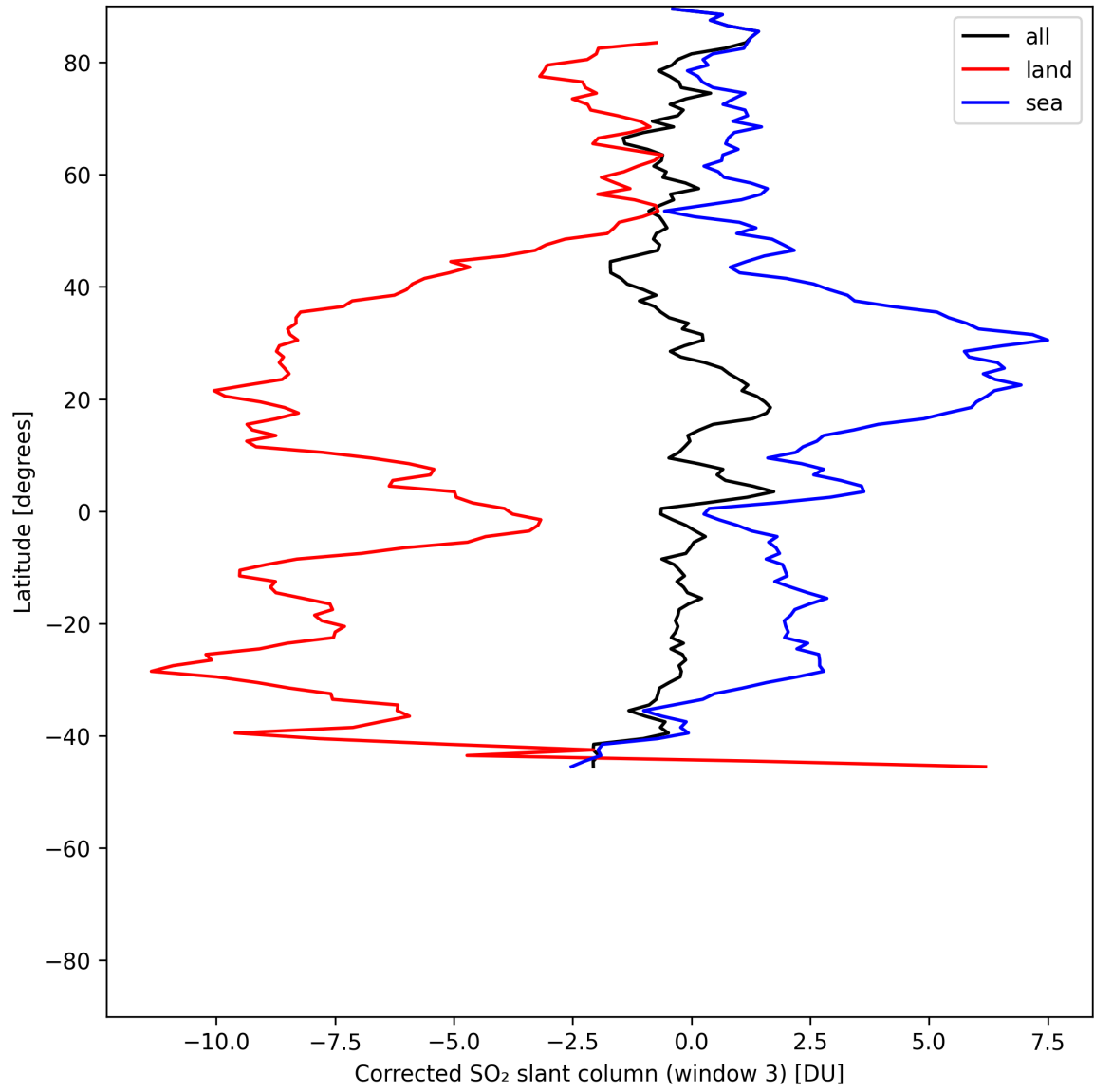
Figure 46: Zonal average of “Corrected SO 2 slant column (window 3)” for 2025-06-28 to 2025-06-29.
