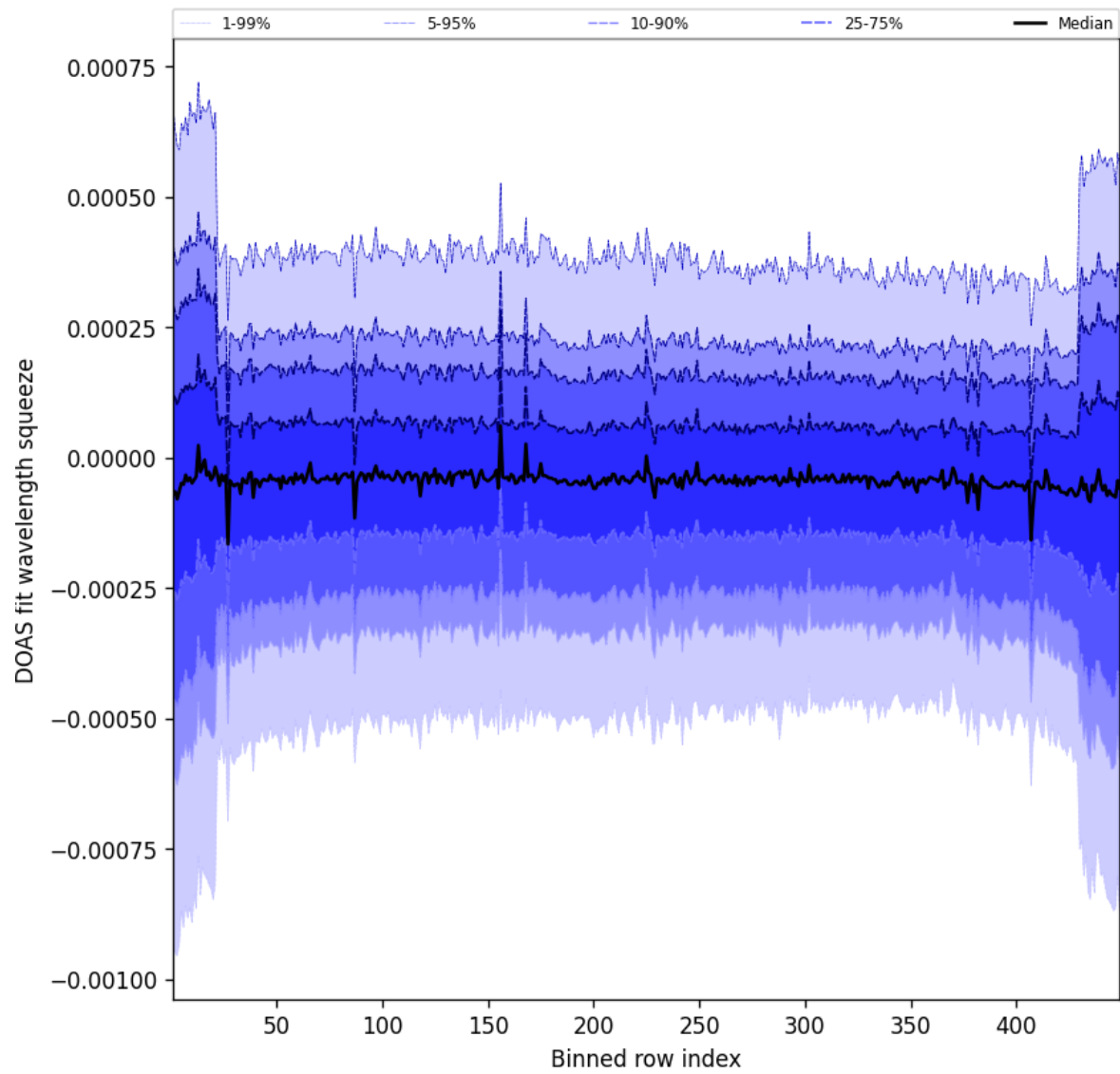
Figure 105: Along track statistics of “DOAS fit wavelength squeeze” for 2025-06-28 to 2025-06-29
