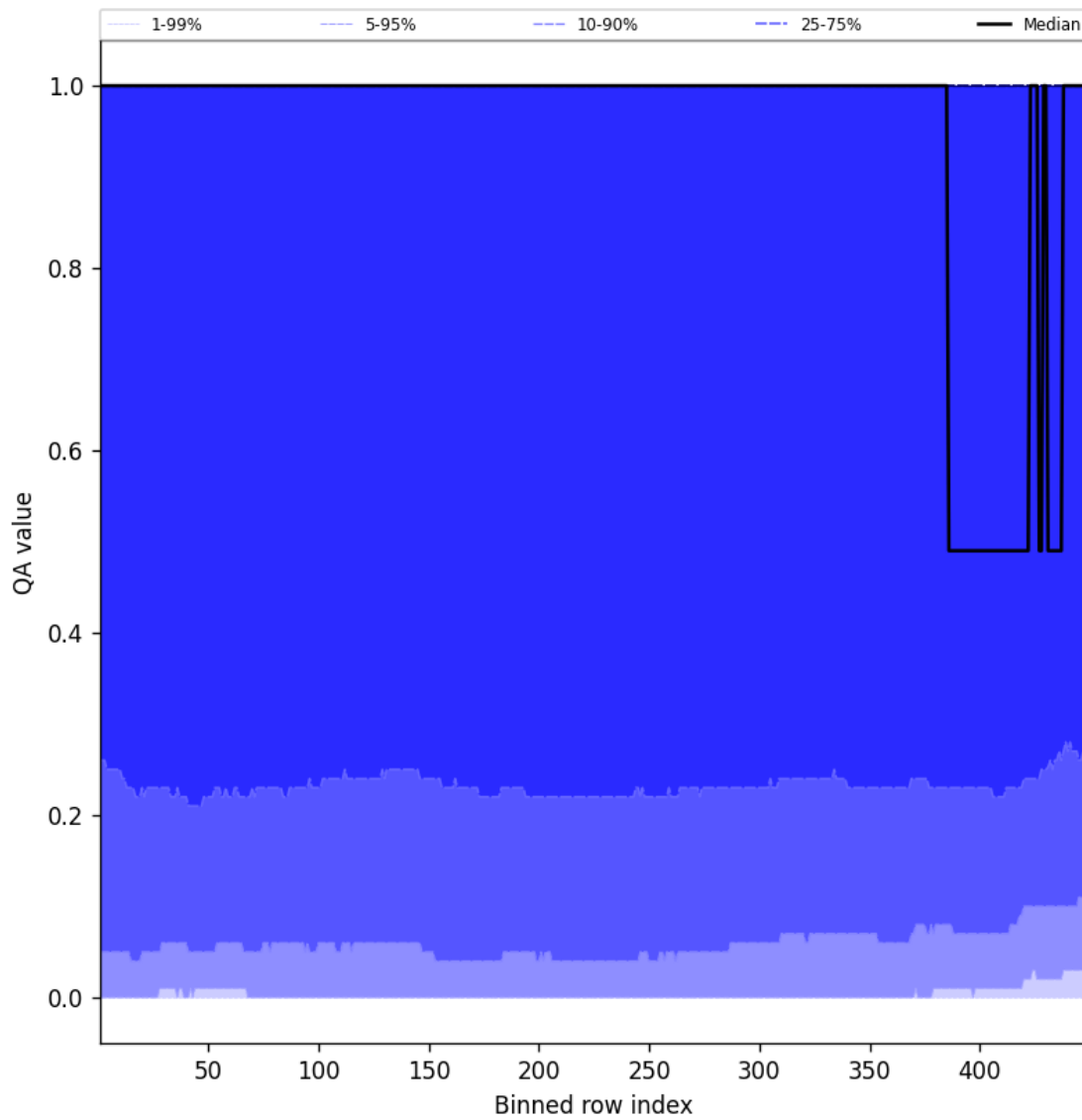
Figure 84: Along track statistics of “QA value” for 2025-06-28 to 2025-06-29
