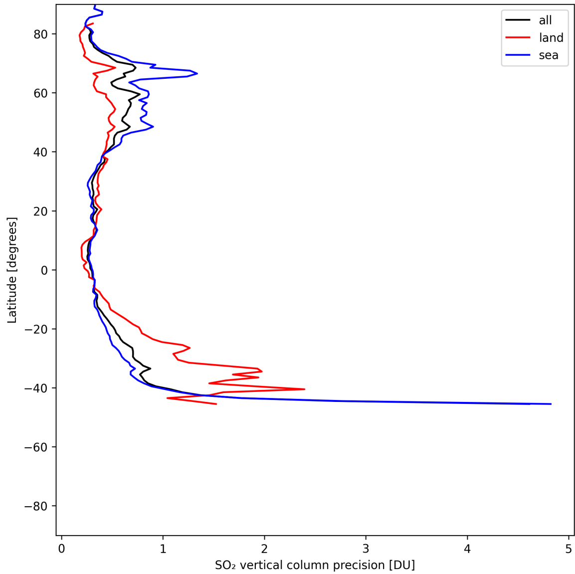
Figure 32: Zonal average of “SO 2 vertical column precision” for 2025-06-28 to 2025-06-29.
