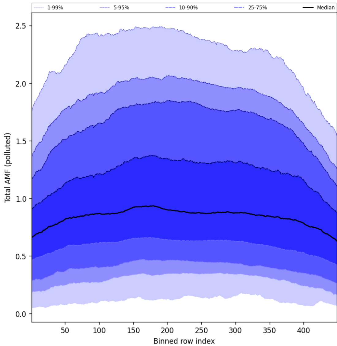
Figure 107: Along track statistics of “Total AMF (polluted)” for 2025-06-28 to 2025-06-29
