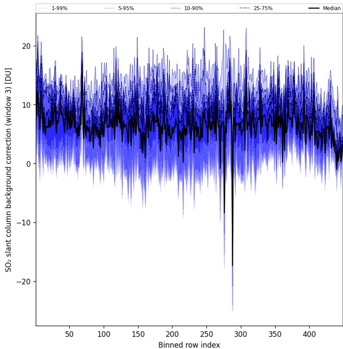
Figure 101: Along track statistics of “SO 2 slant column background correction (window 3)” for 2025-06-28 to 2025-06-29
