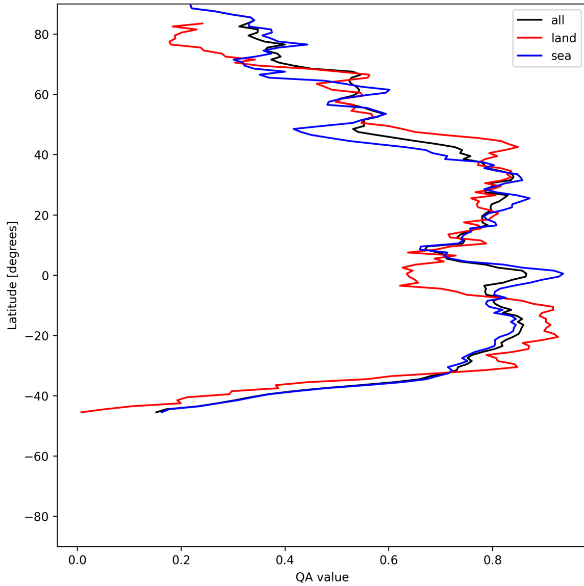
Figure 30: Zonal average of “QA value” for 2025-06-28 to 2025-06-29.
