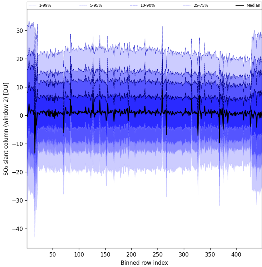
Figure 94: Along track statistics of “SO 2 slant column (window 2)” for 2025-06-28 to 2025-06-29
