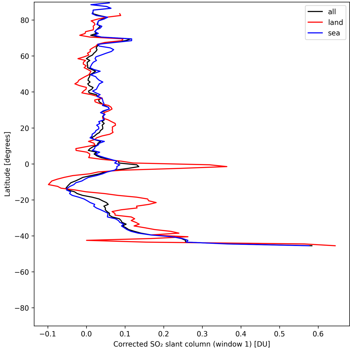
Figure 38: Zonal average of “Corrected SO 2 slant column (window 1)” for 2025-06-28 to 2025-06-29.
