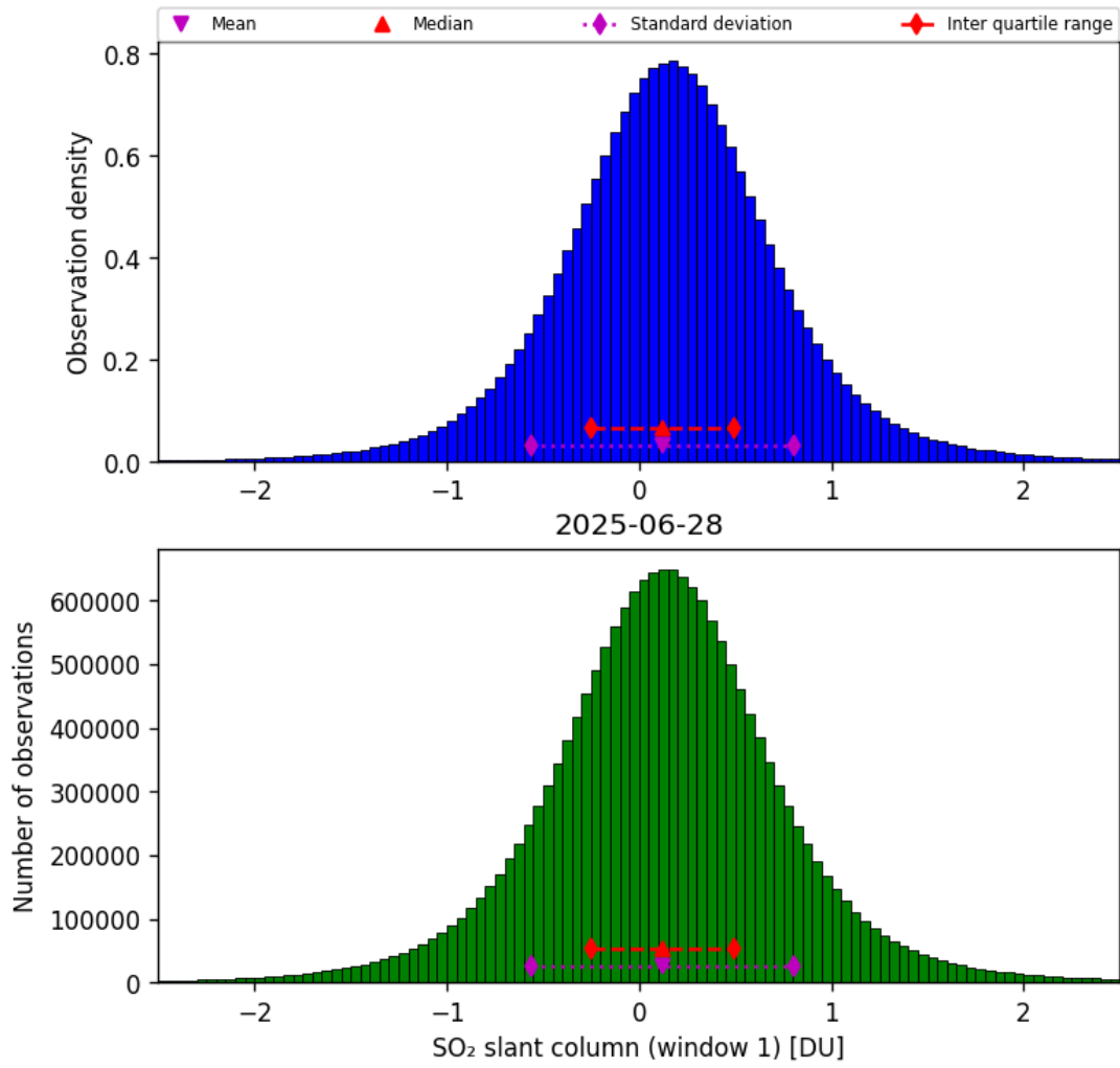
Figure 63: Histogram of “SO 2 slant column (window 1)” for 2025-06-28 to 2025-06-29
