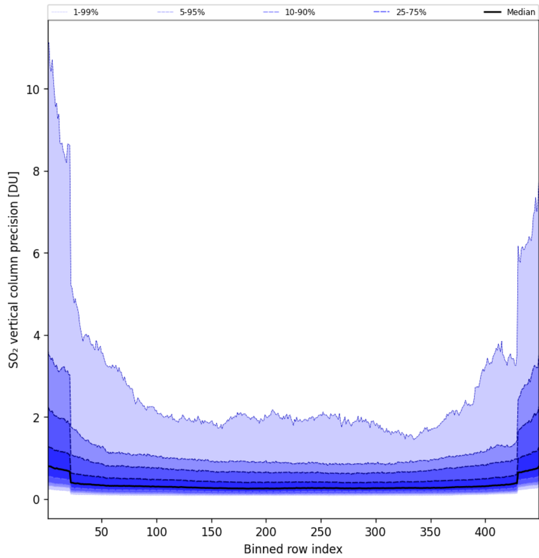
Figure 86: Along track statistics of “SO 2 vertical column precision” for 2025-06-28 to 2025-06-29
