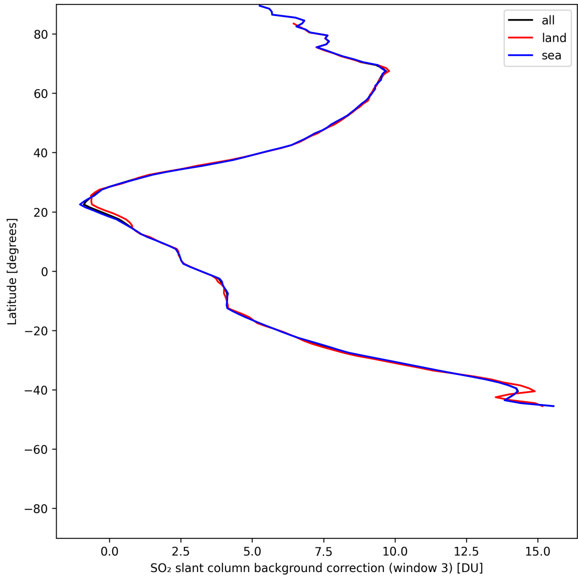
Figure 47: Zonal average of “SO 2 slant column background correction (window 3)” for 2025-06-28 to 2025-06-29.
