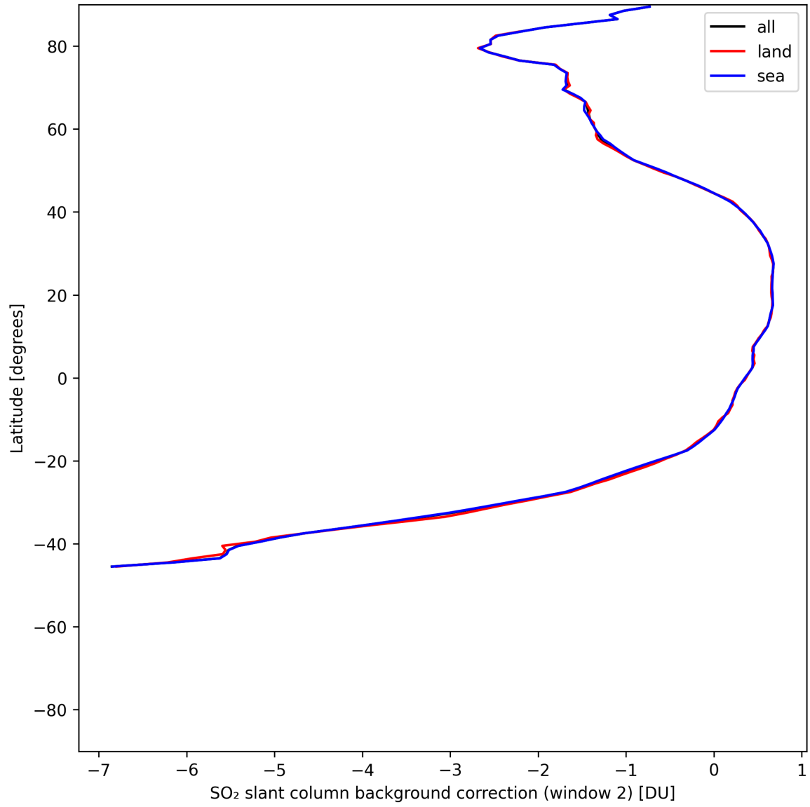
Figure 43: Zonal average of “SO 2 slant column background correction (window 2)” for 2025-06-28 to 2025-06-29.
