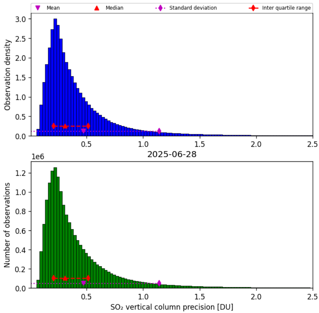
Figure 59: Histogram of “SO 2 vertical column precision” for 2025-06-28 to 2025-06-29
