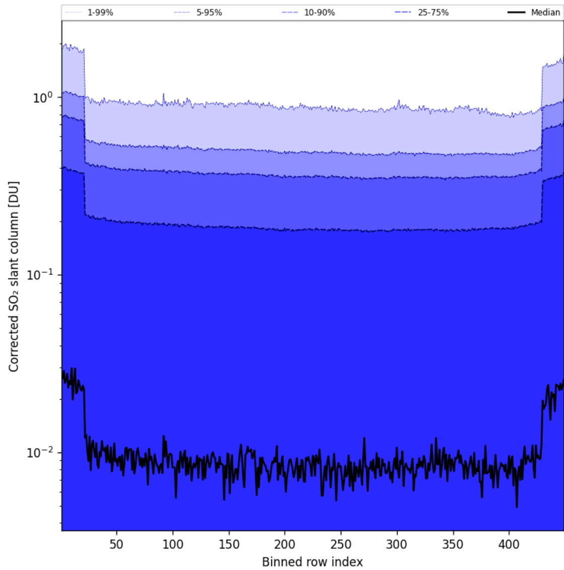
Figure 87: Along track statistics of "Corrected SO 2 slant column" for 2025-06-28 to 2025-06-29
