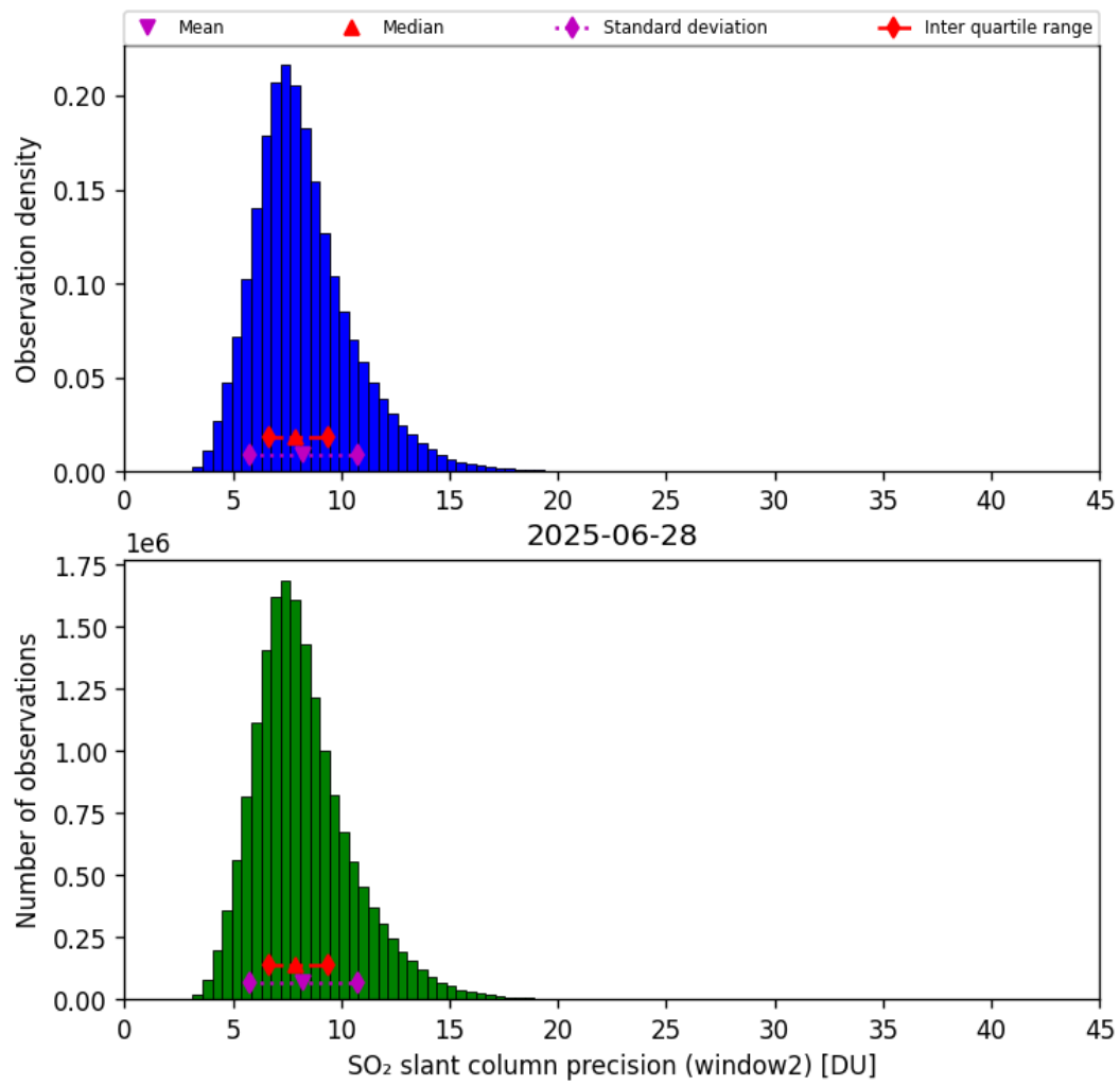
Figure 68: Histogram of “SO 2 slant column precision (window2)” for 2025-06-28 to 2025-06-29
