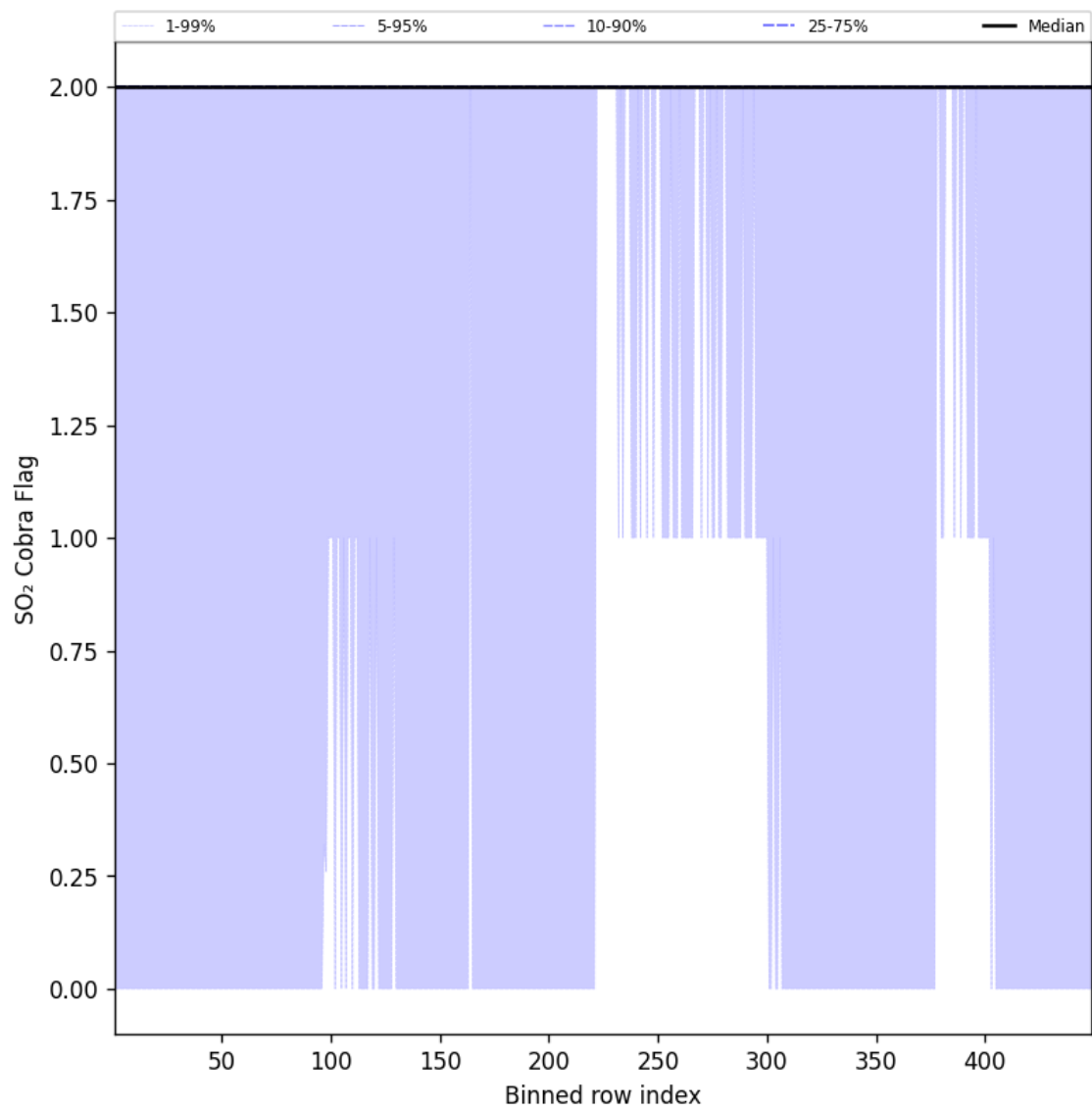
Figure 102: Along track statistics of "SO 2 Cobra Flag" for 2025-06-28 to 2025-06-29
