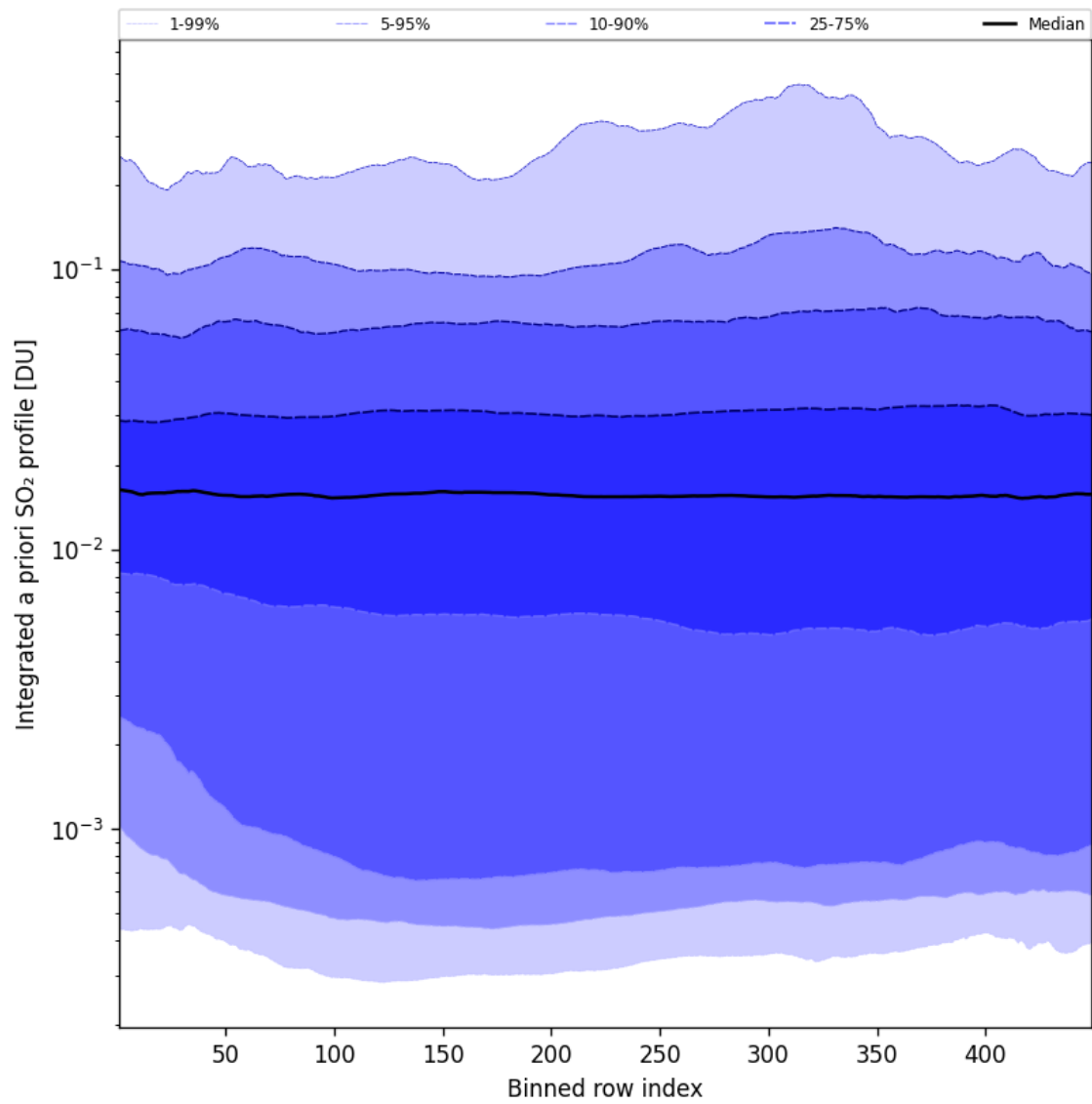
Figure 103: Along track statistics of “Integrated a priori SO 2 profile” for 2025-06-28 to 2025-06-29
