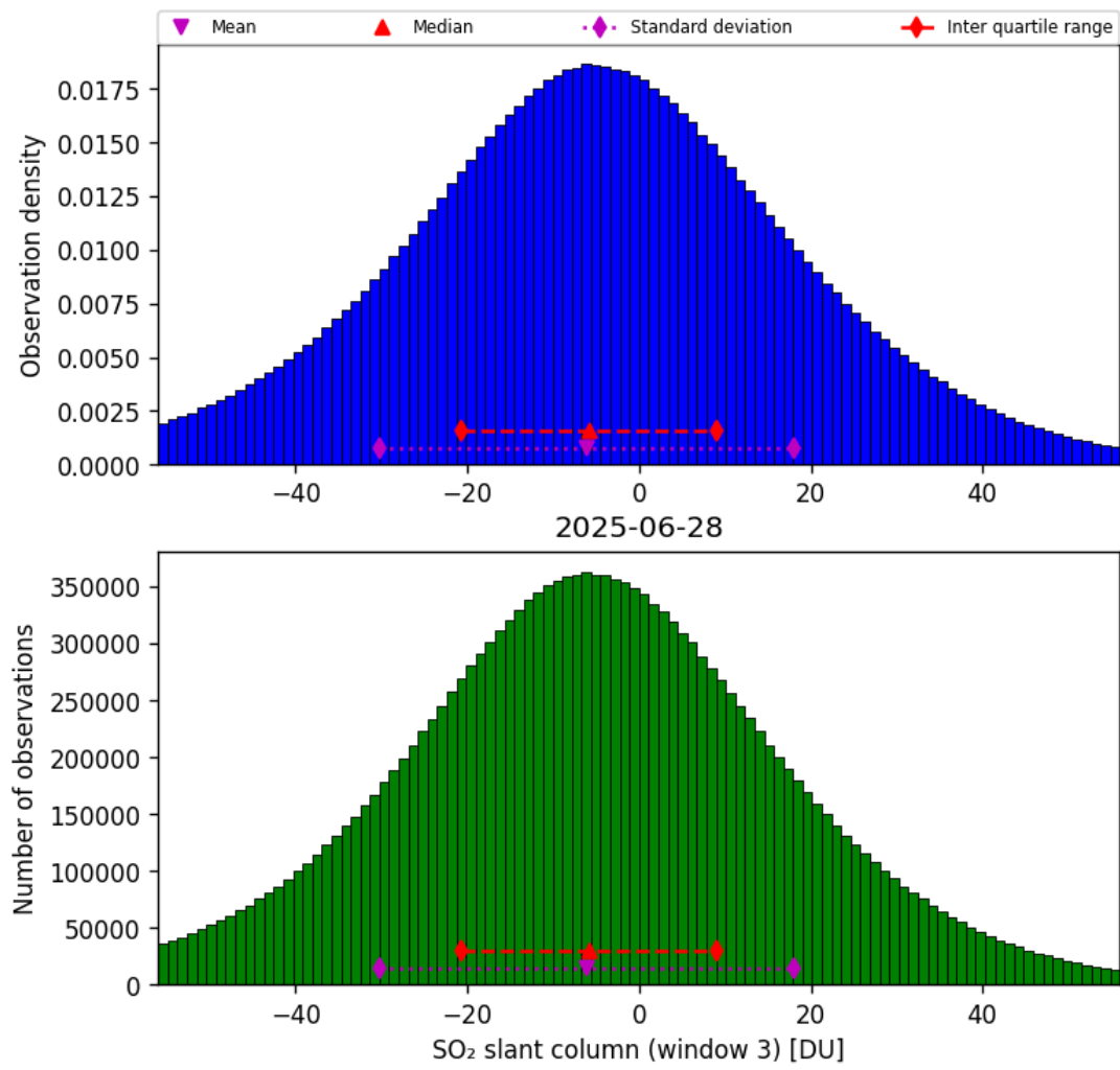
Figure 71: Histogram of “SO 2 slant column (window 3)” for 2025-06-28 to 2025-06-29
