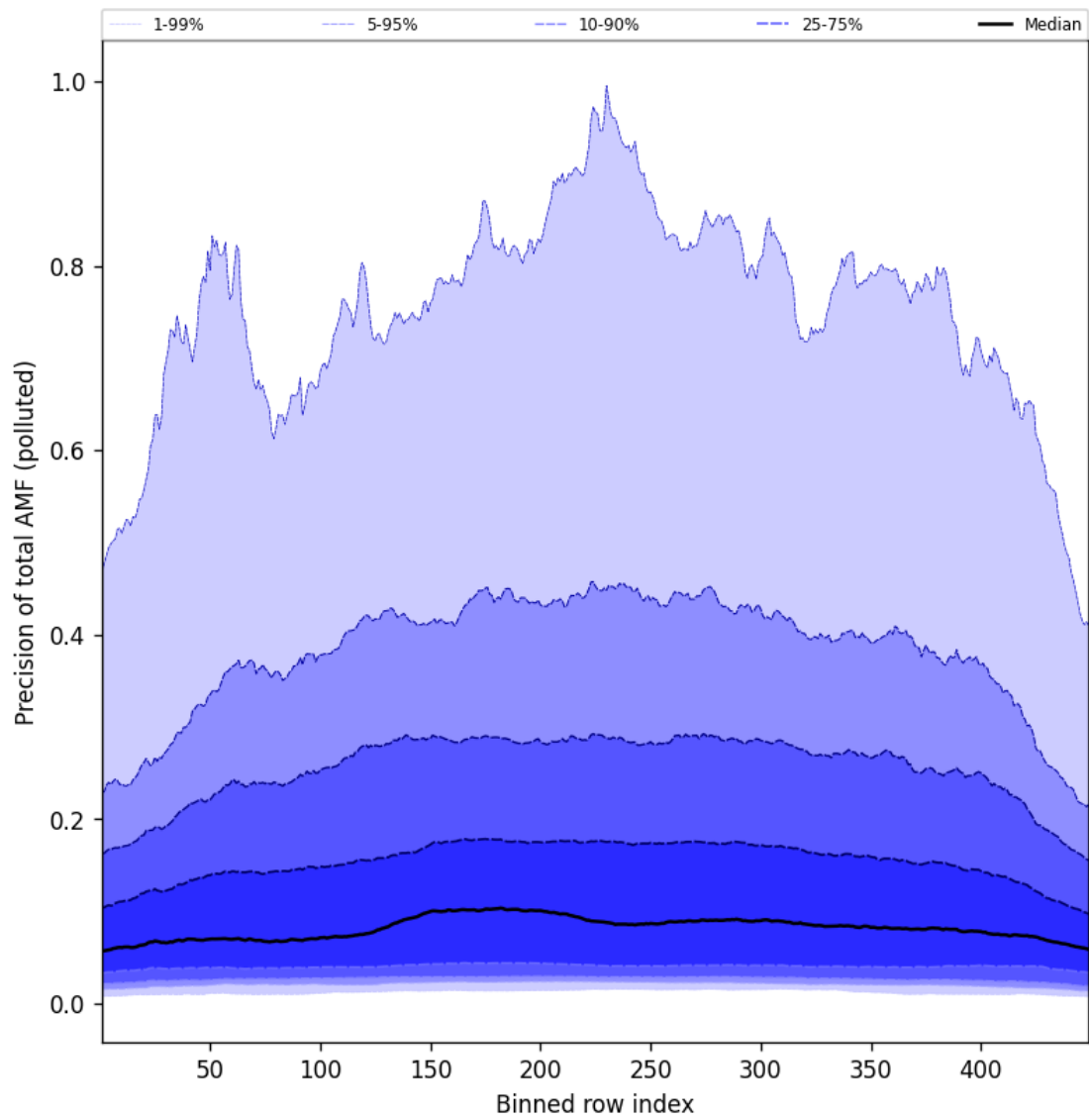
Figure 108: Along track statistics of “Precision of total AMF (polluted)” for 2025-06-28 to 2025-06-29
