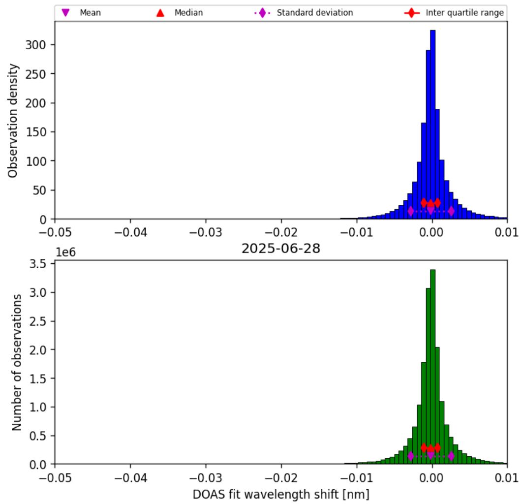
Figure 77: Histogram of “DOAS fit wavelength shift” for 2025-06-28 to 2025-06-29
