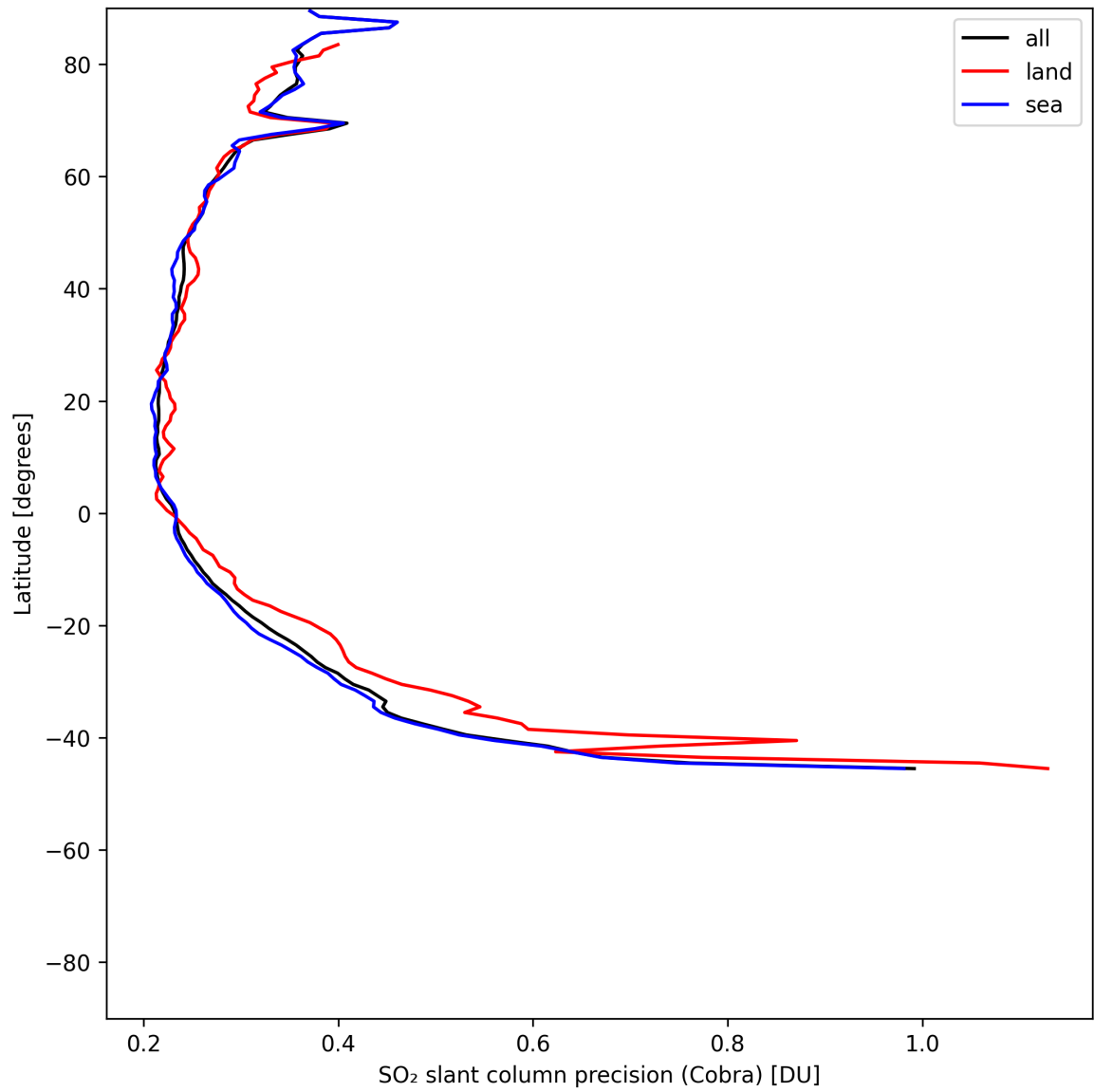
Figure 35: Zonal average of “SO 2 slant column precision (Cobra)” for 2025-06-28 to 2025-06-29.
