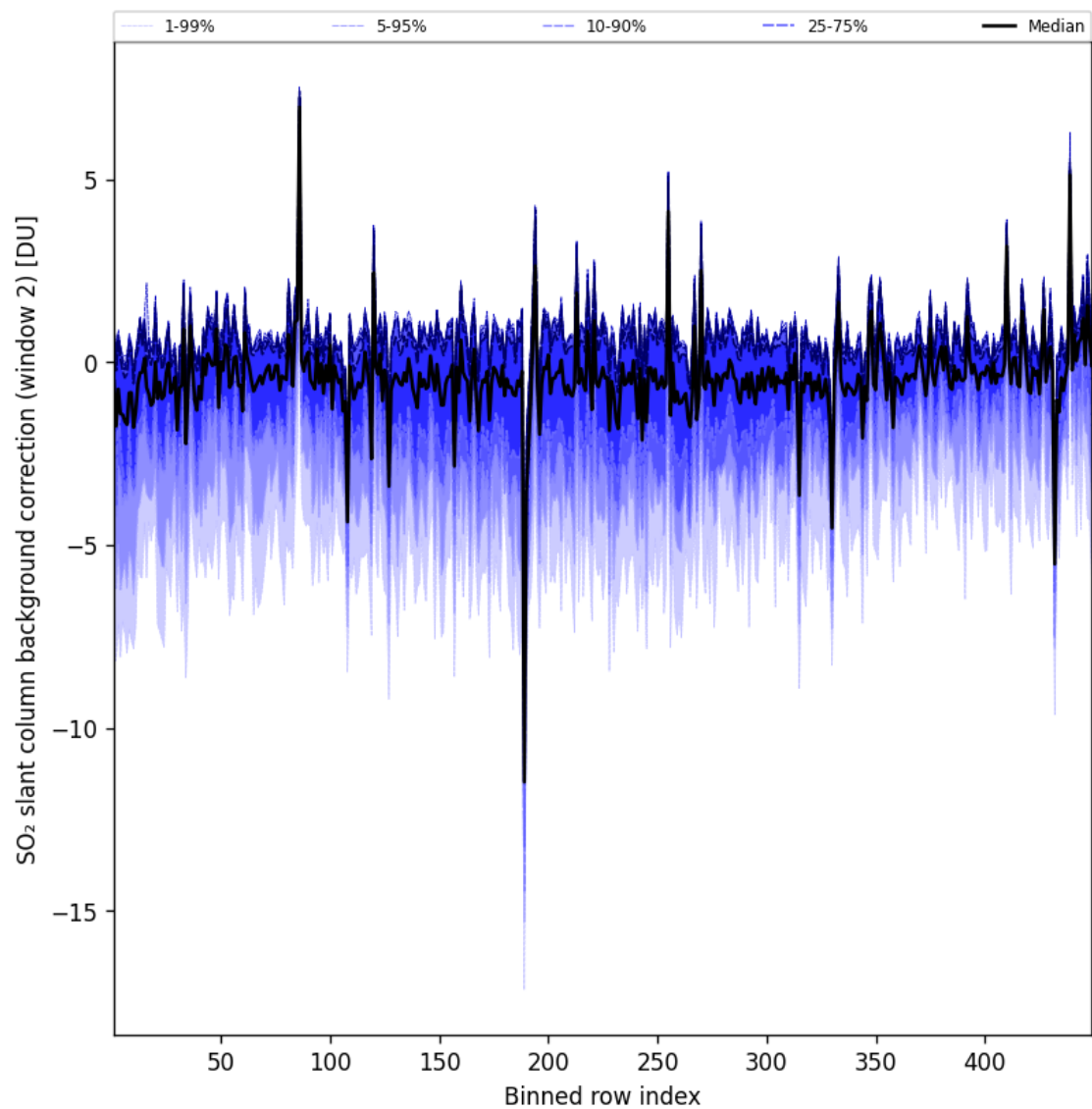
Figure 97: Along track statistics of “SO 2 slant column background correction (window 2)” for 2025-06-28 to 2025-06-29
