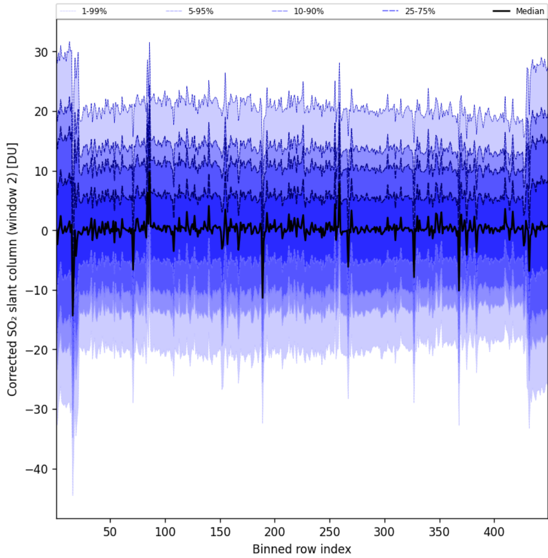
Figure 96: Along track statistics of “Corrected SO 2 slant column (window 2)” for 2025-06-28 to 2025-06-29
