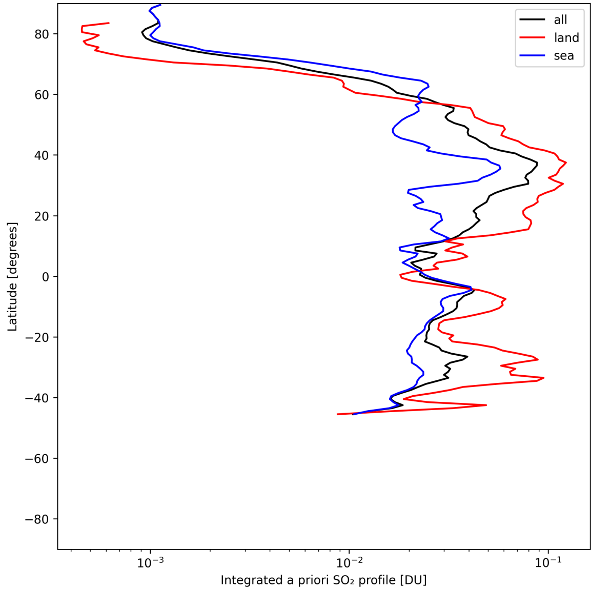
Figure 49: Zonal average of “Integrated a priori SO 2 profile” for 2025-06-28 to 2025-06-29.
