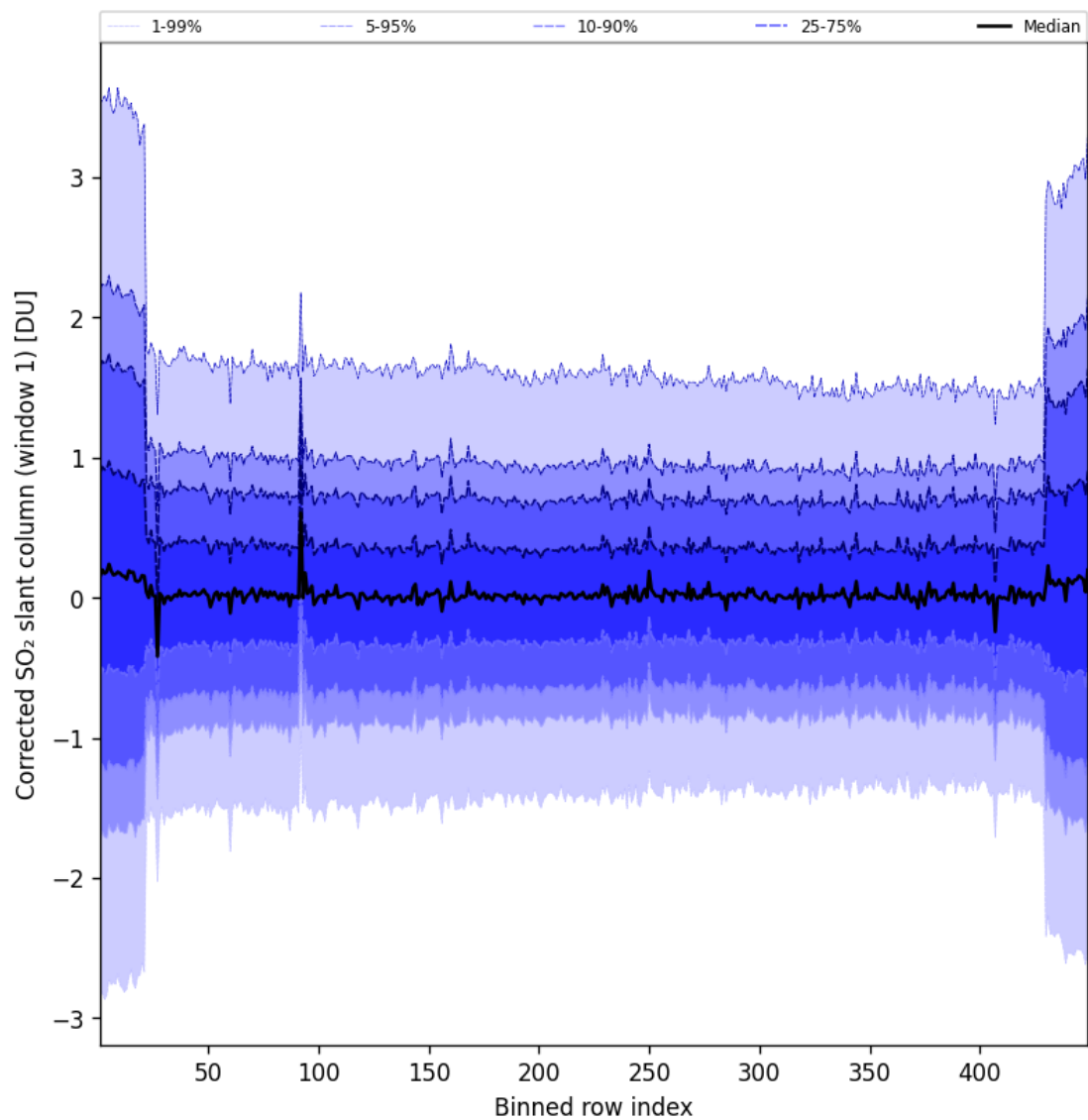
Figure 92: Along track statistics of “Corrected SO 2 slant column (window 1)” for 2025-06-28 to 2025-06-29
