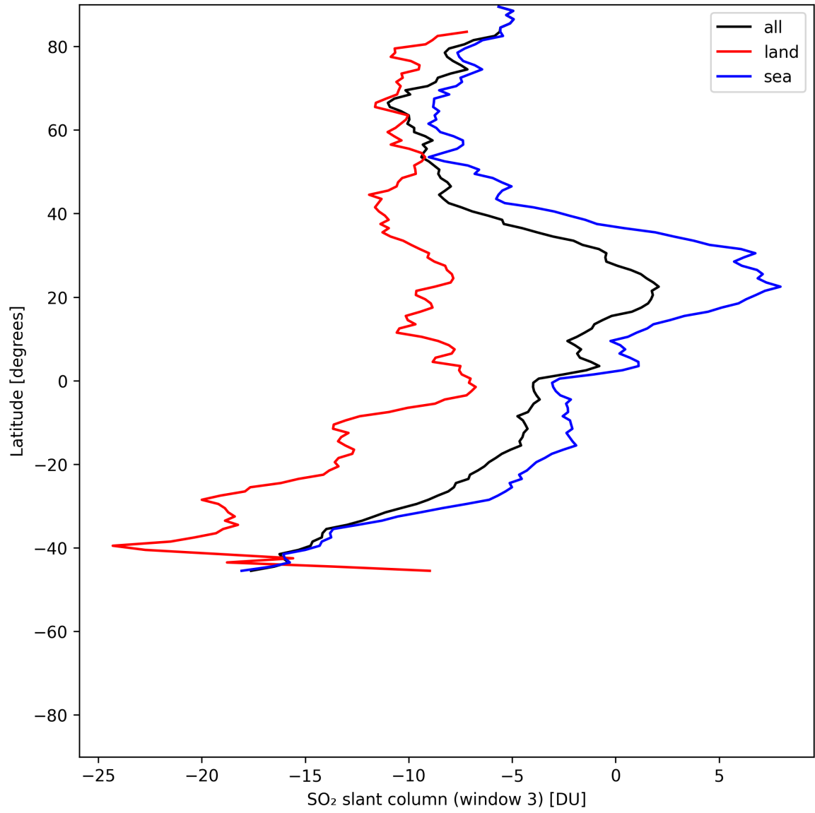
Figure 44: Zonal average of “SO 2 slant column (window 3)” for 2025-06-28 to 2025-06-29.
