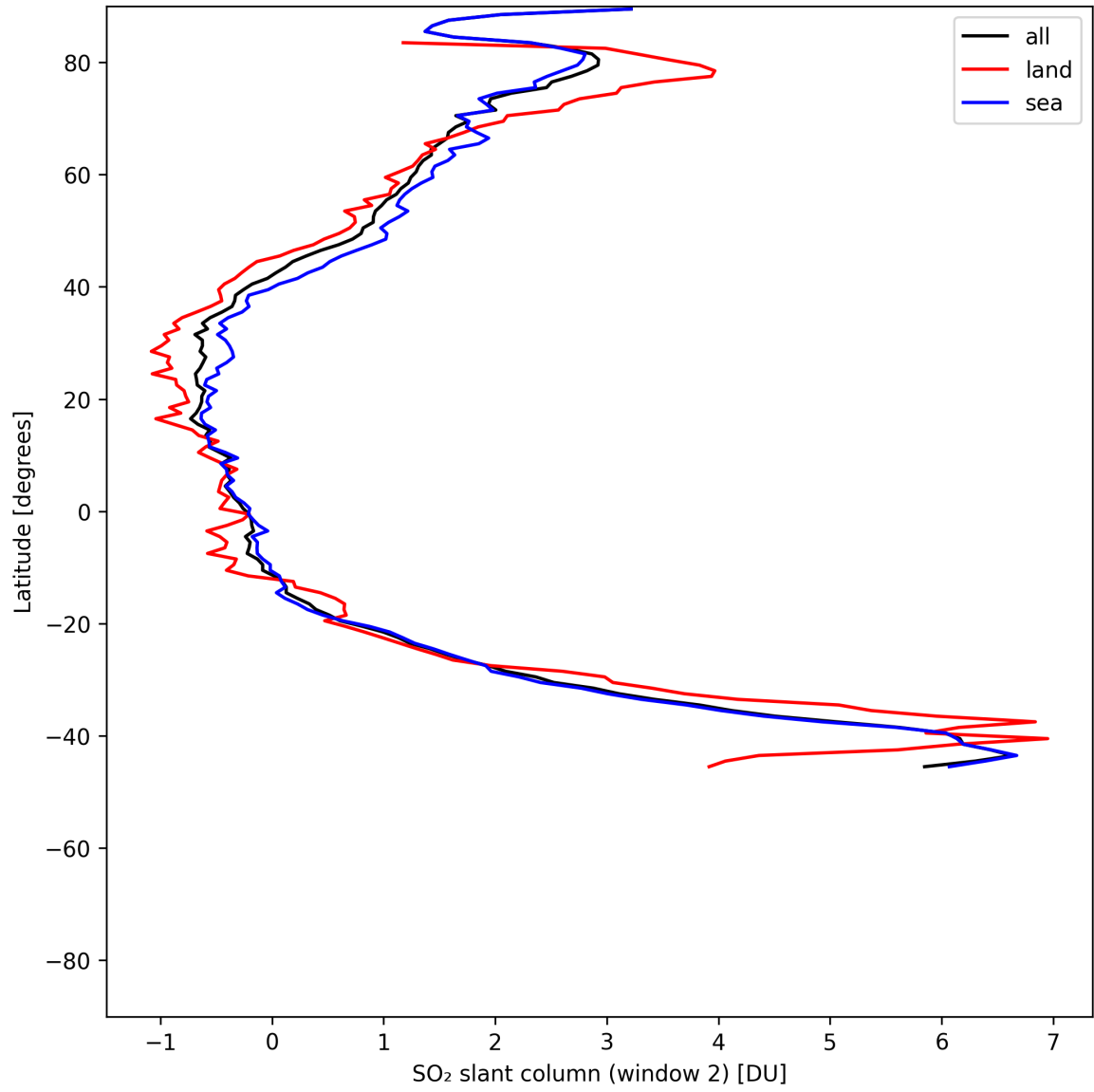
Figure 40: Zonal average of “SO 2 slant column (window 2)” for 2025-06-28 to 2025-06-29.
