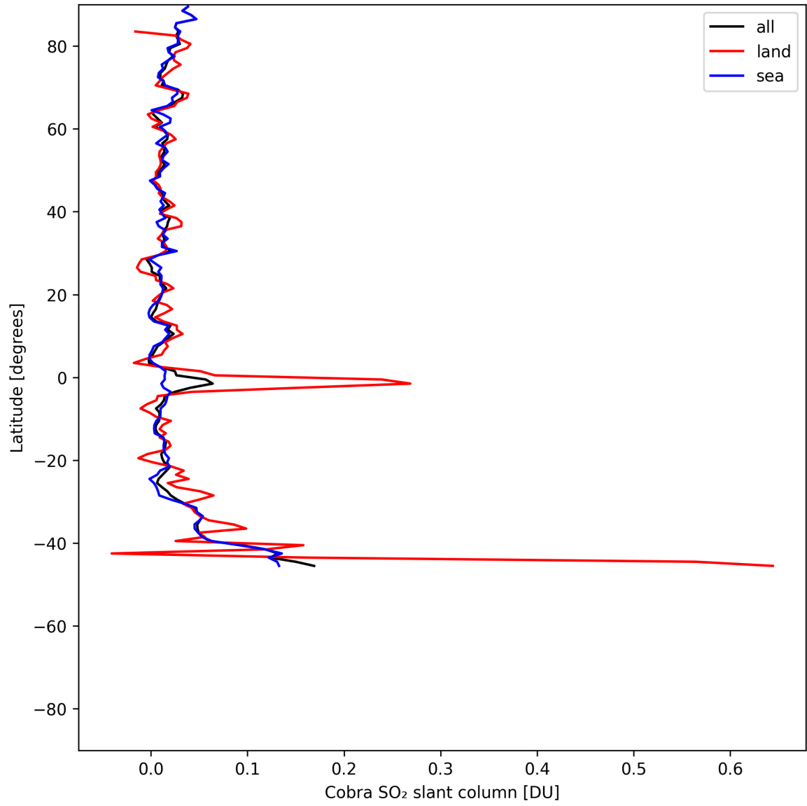
Figure 34: Zonal average of “Cobra SO 2 slant column” for 2025-06-28 to 2025-06-29.
