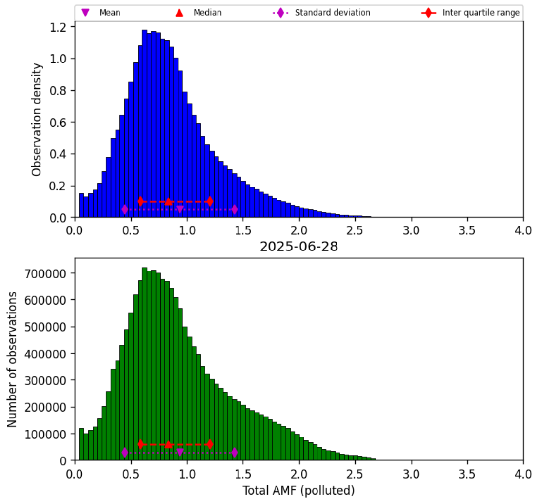
Figure 80: Histogram of “Total AMF (polluted)” for 2025-06-28 to 2025-06-29
