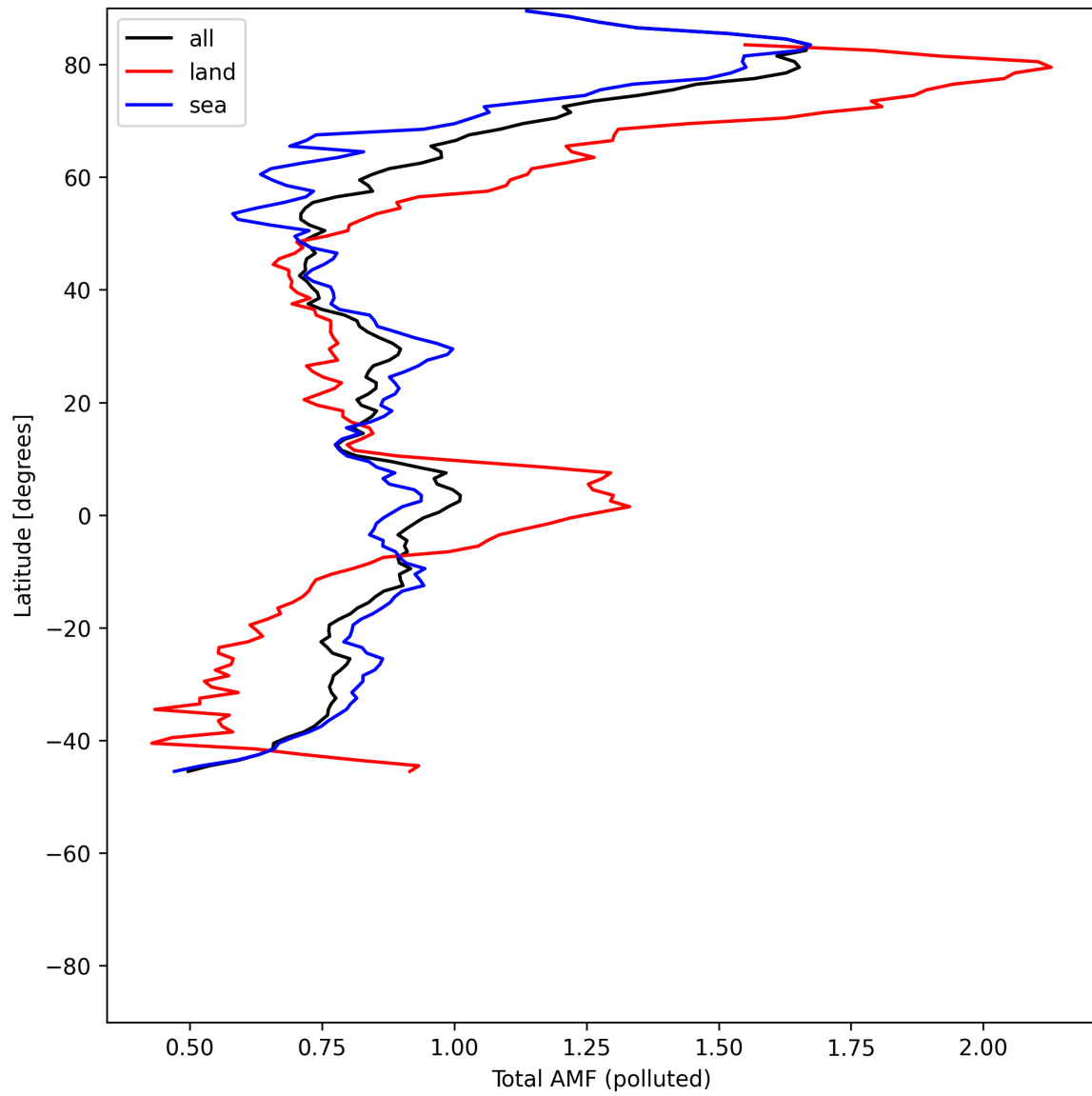
Figure 53: Zonal average of “Total AMF (polluted)” for 2025-06-28 to 2025-06-29.
