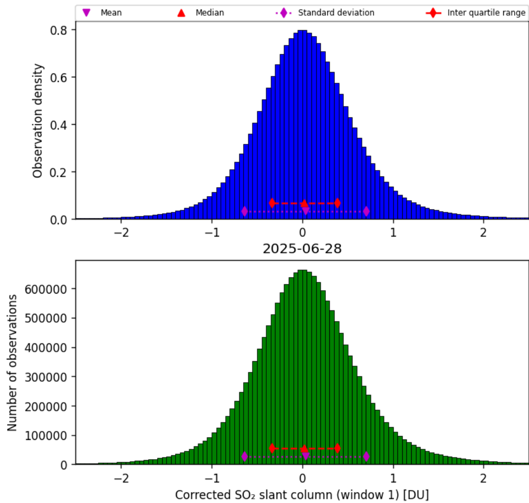
Figure 65: Histogram of “Corrected SO 2 slant column (window 1)” for 2025-06-28 to 2025-06-29
