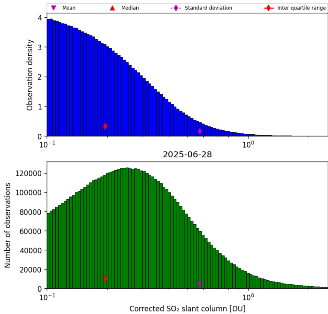
Figure 60: Histogram of “Corrected SO 2 slant column” for 2025-06-28 to 2025-06-29
