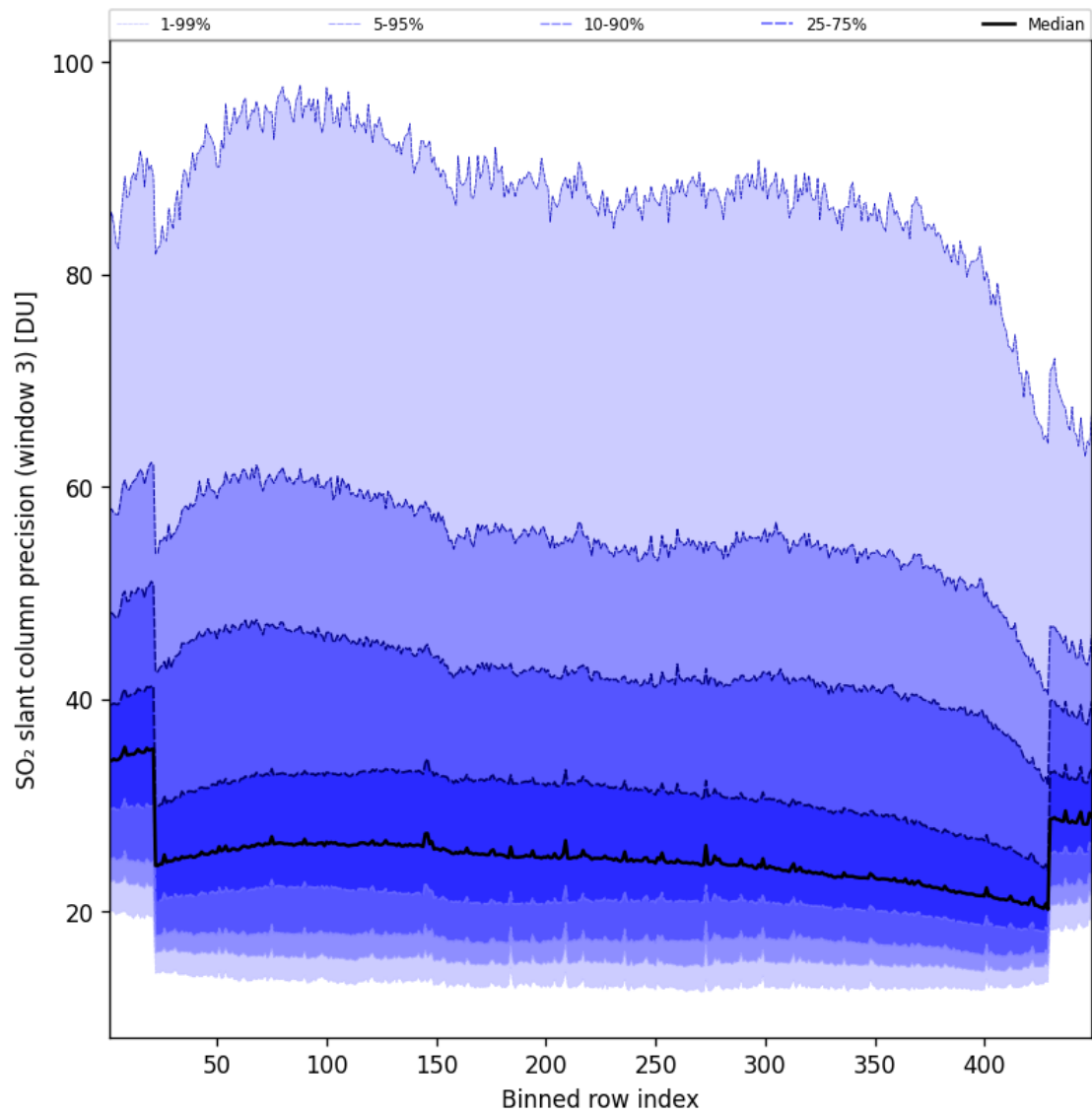
Figure 99: Along track statistics of “SO 2 slant column precision (window 3)” for 2025-06-28 to 2025-06-29
