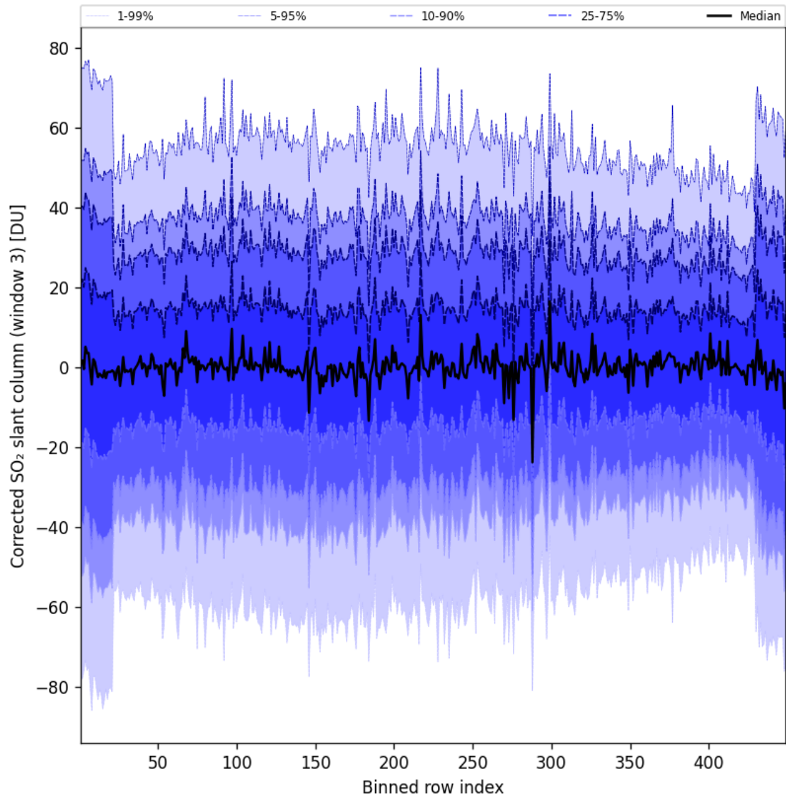
Figure 100: Along track statistics of “Corrected SO 2 slant column (window 3)” for 2025-06-28 to 2025-06-29
