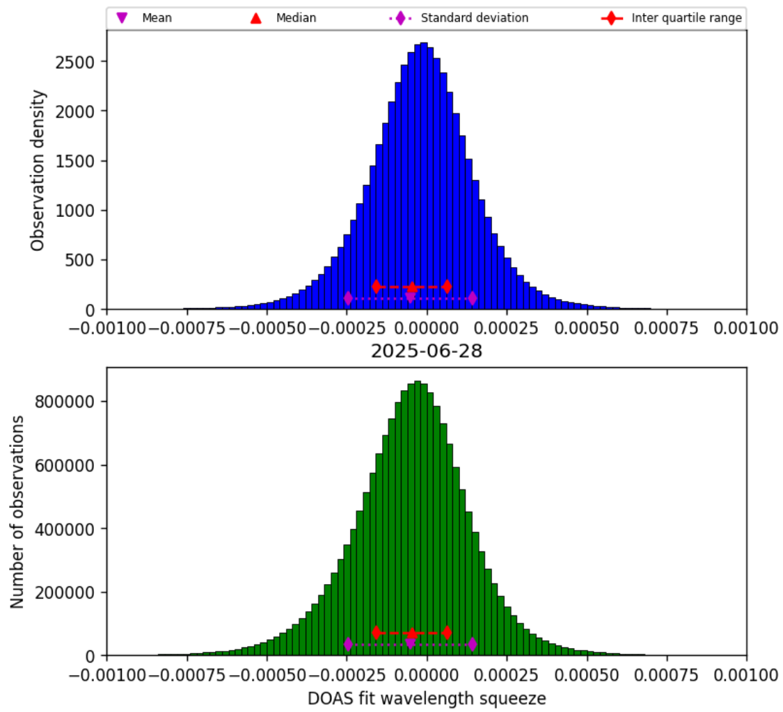
Figure 78: Histogram of “DOAS fit wavelength squeeze” for 2025-06-28 to 2025-06-29
