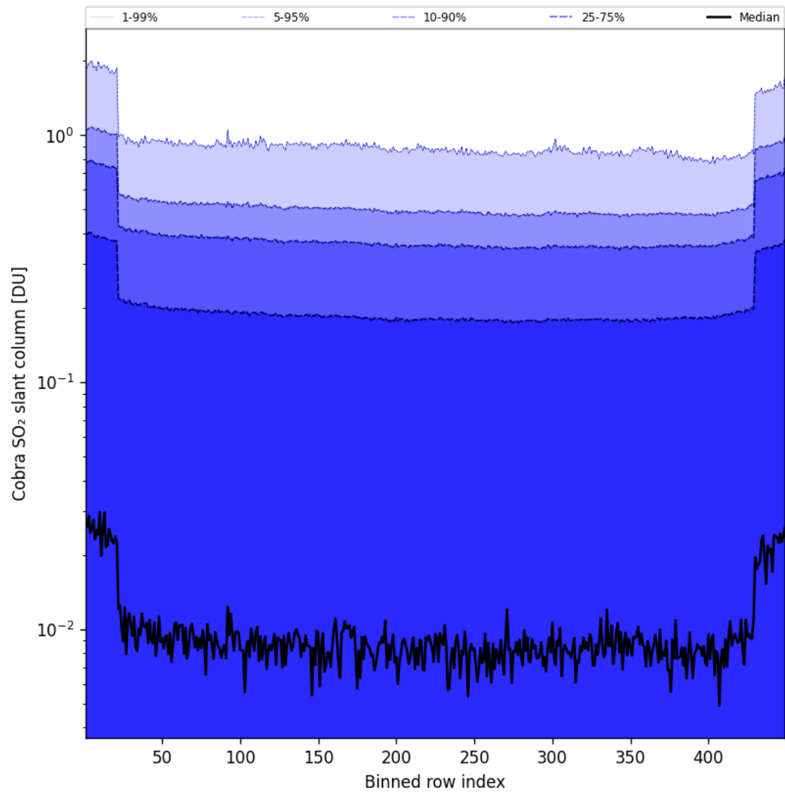
Figure 88: Along track statistics of “Cobra SO 2 slant column” for 2025-06-28 to 2025-06-29
