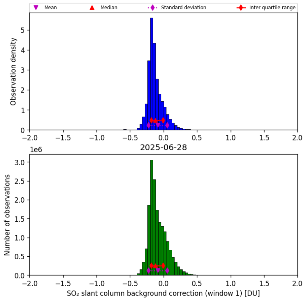
Figure 66: Histogram of “SO 2 slant column background correction (window 1)” for 2025-06-28 to 2025-06-29
