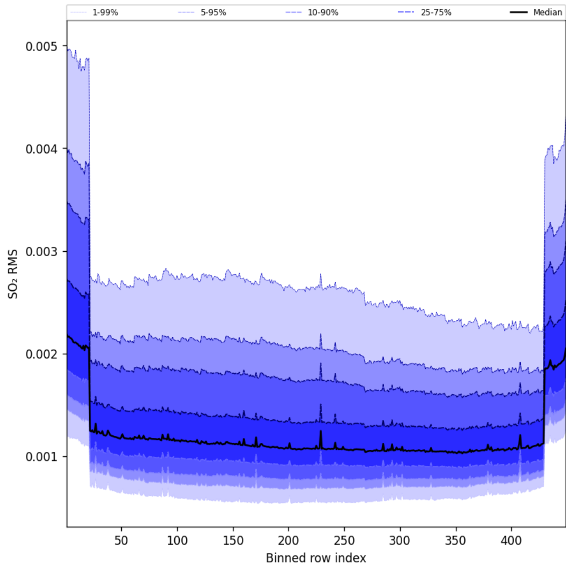
Figure 106: Along track statistics of “SO 2 RMS” for 2025-06-28 to 2025-06-29
