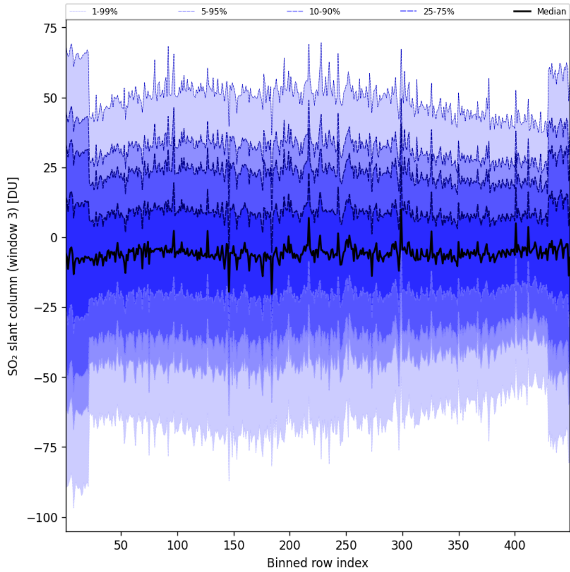
Figure 98: Along track statistics of “SO 2 slant column (window 3)” for 2025-06-28 to 2025-06-29
