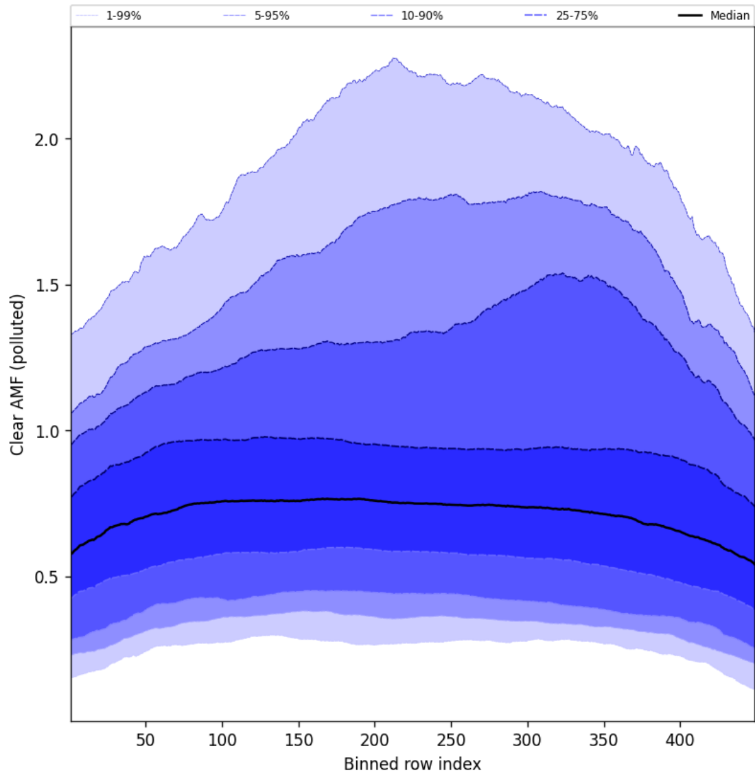
Figure 109: Along track statistics of “Clear AMF (polluted)” for 2025-06-28 to 2025-06-29
