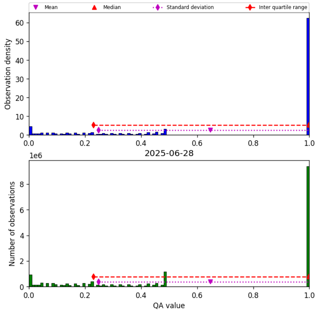
Figure 57: Histogram of “QA value” for 2025-06-28 to 2025-06-29
