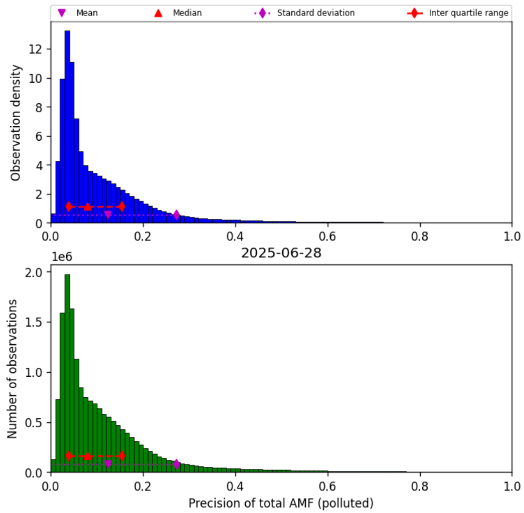
Figure 81: Histogram of “Precision of total AMF (polluted)” for 2025-06-28 to 2025-06-29
