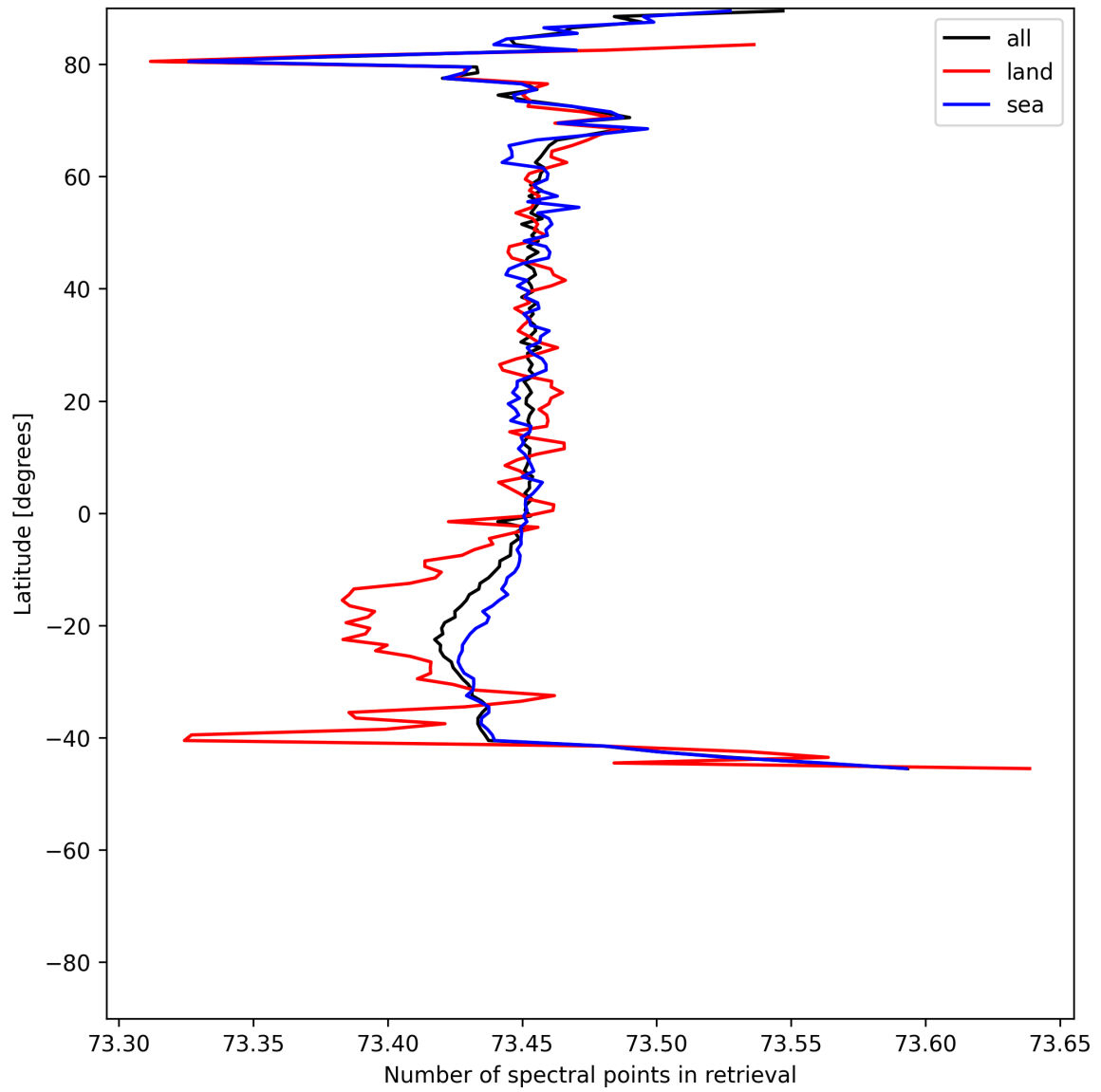
Figure 56: Zonal average of “Number of spectral points in retrieval” for 2025-06-28 to 2025-06-29.
