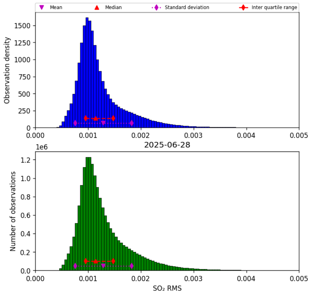
Figure 79: Histogram of “SO 2 RMS” for 2025-06-28 to 2025-06-29
