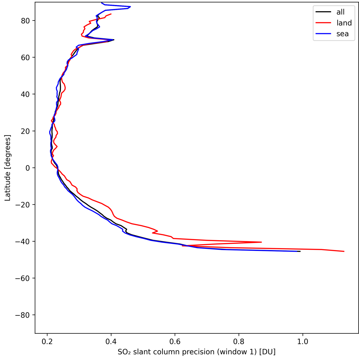
Figure 37: Zonal average of “SO 2 slant column precision (window 1)” for 2025-06-28 to 2025-06-29.
