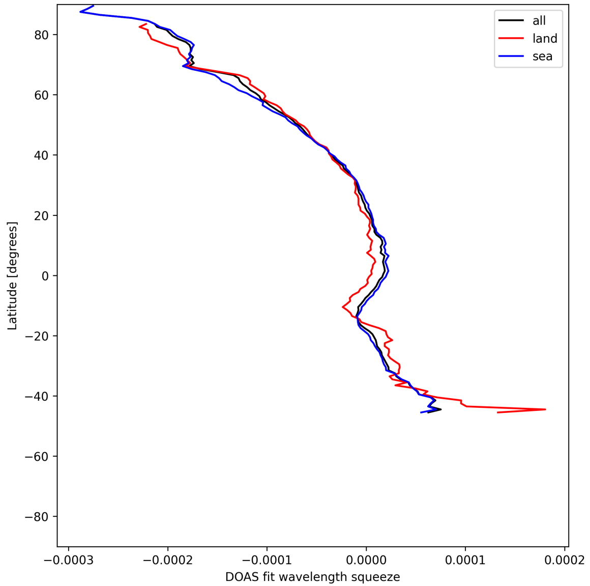
Figure 51: Zonal average of “DOAS fit wavelength squeeze” for 2025-06-28 to 2025-06-29.
