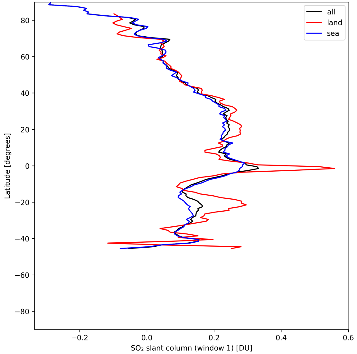
Figure 36: Zonal average of “SO 2 slant column (window 1)” for 2025-06-28 to 2025-06-29.
