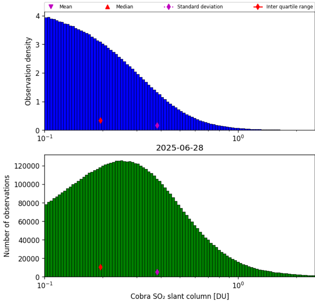
Figure 61: Histogram of “Cobra SO 2 slant column” for 2025-06-28 to 2025-06-29
