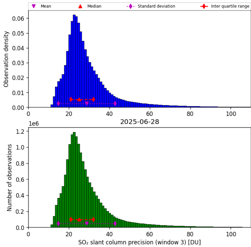
Figure 72: Histogram of “SO 2 slant column precision (window 3)” for 2025-06-28 to 2025-06-29
