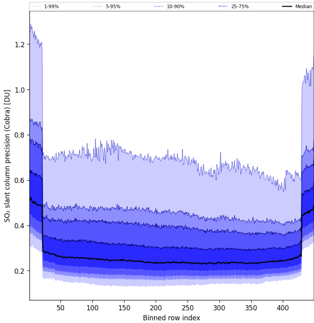
Figure 89: Along track statistics of “SO 2 slant column precision (Cobra)” for 2025-06-28 to 2025-06-29
