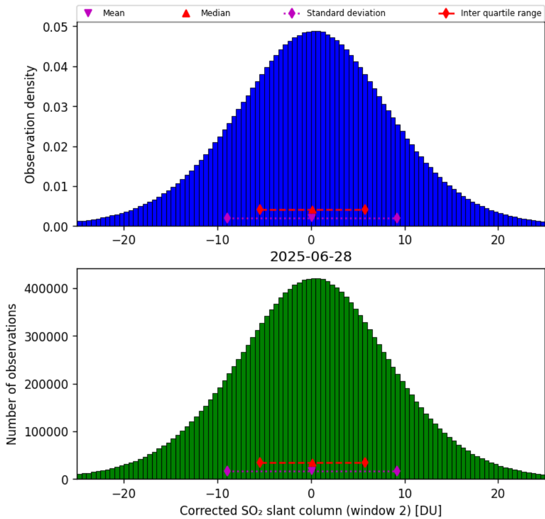
Figure 69: Histogram of “Corrected SO 2 slant column (window 2)” for 2025-06-28 to 2025-06-29
