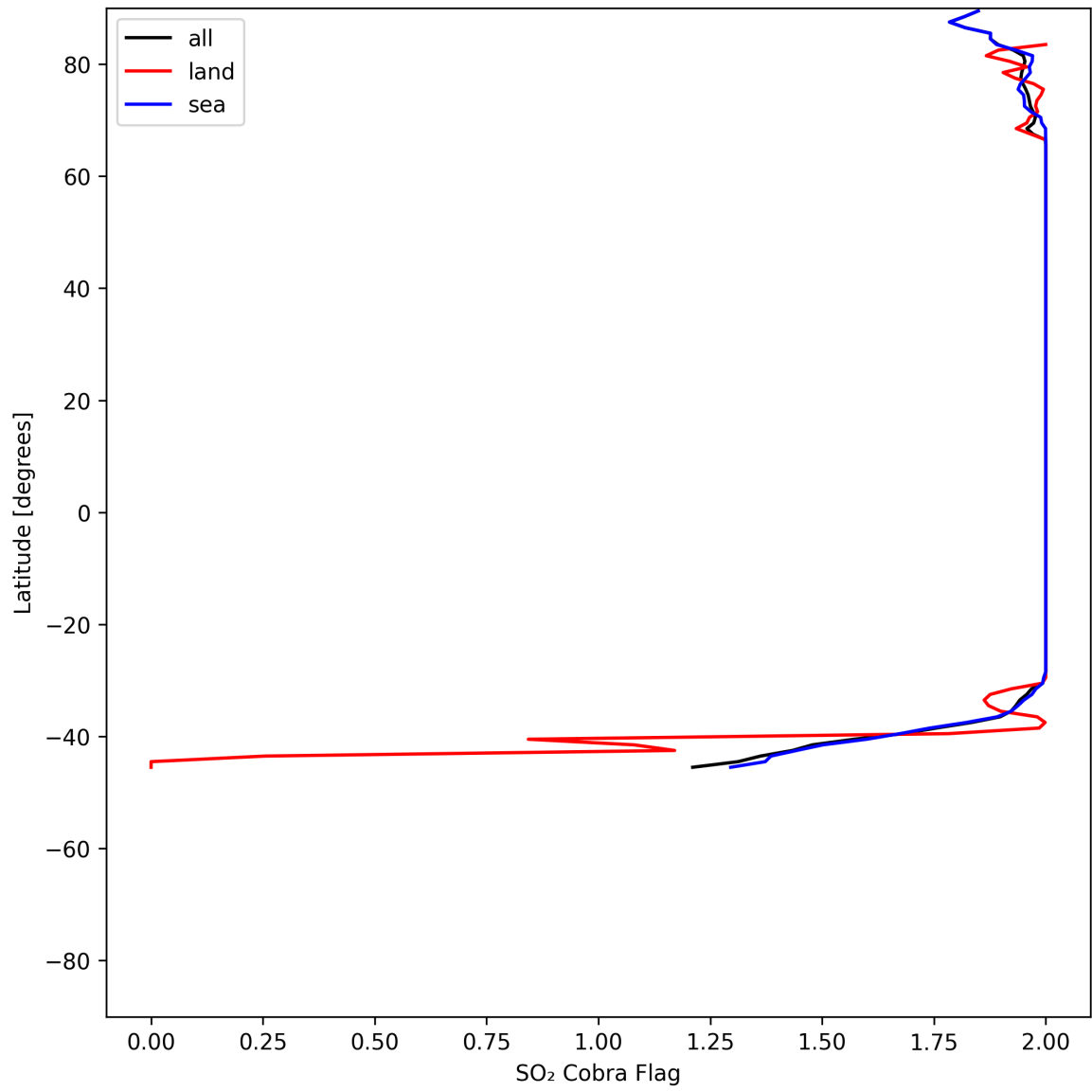
Figure 48: Zonal average of “SO 2 Cobra Flag” for 2025-06-28 to 2025-06-29.
