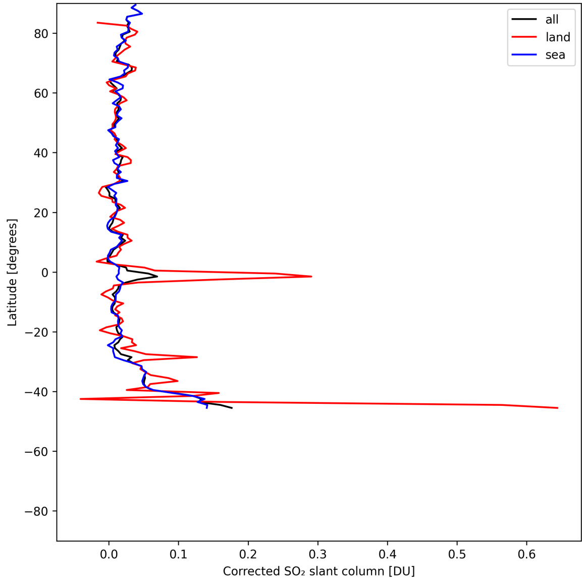
Figure 33: Zonal average of “Corrected SO 2 slant column” for 2025-06-28 to 2025-06-29.
