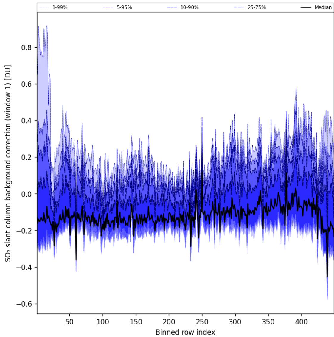
Figure 93: Along track statistics of “SO 2 slant column background correction (window 1)” for 2025-06-28 to 2025-06-29
