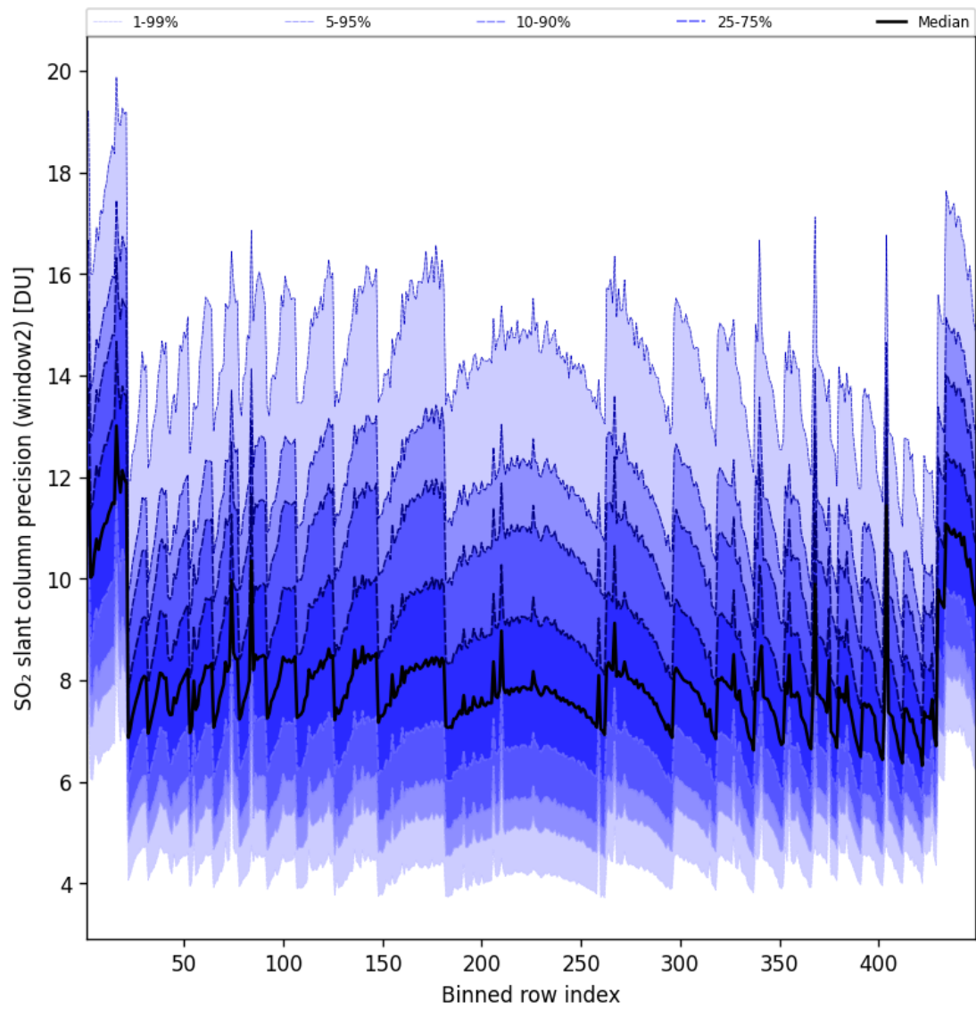
Figure 95: Along track statistics of “SO 2 slant column precision (window2)” for 2025-06-28 to 2025-06-29
