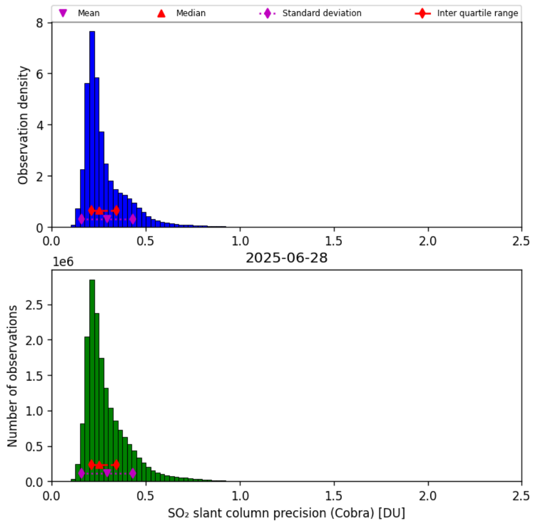
Figure 62: Histogram of “SO 2 slant column precision (Cobra)” for 2025-06-28 to 2025-06-29
