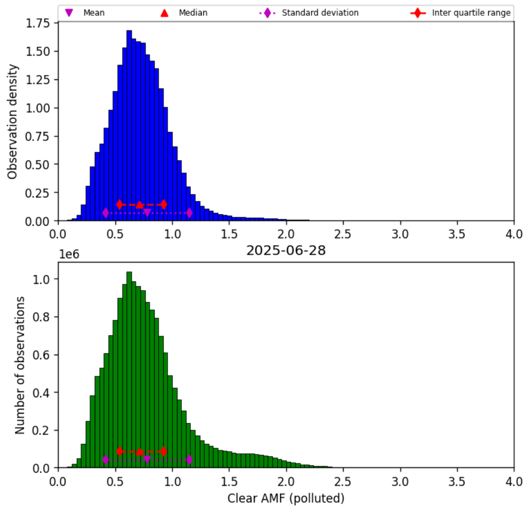
Figure 82: Histogram of “Clear AMF (polluted)” for 2025-06-28 to 2025-06-29
