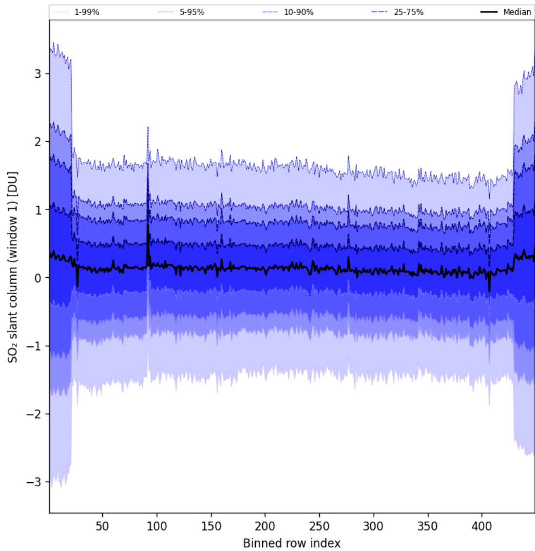
Figure 90: Along track statistics of “SO 2 slant column (window 1)” for 2025-06-28 to 2025-06-29
