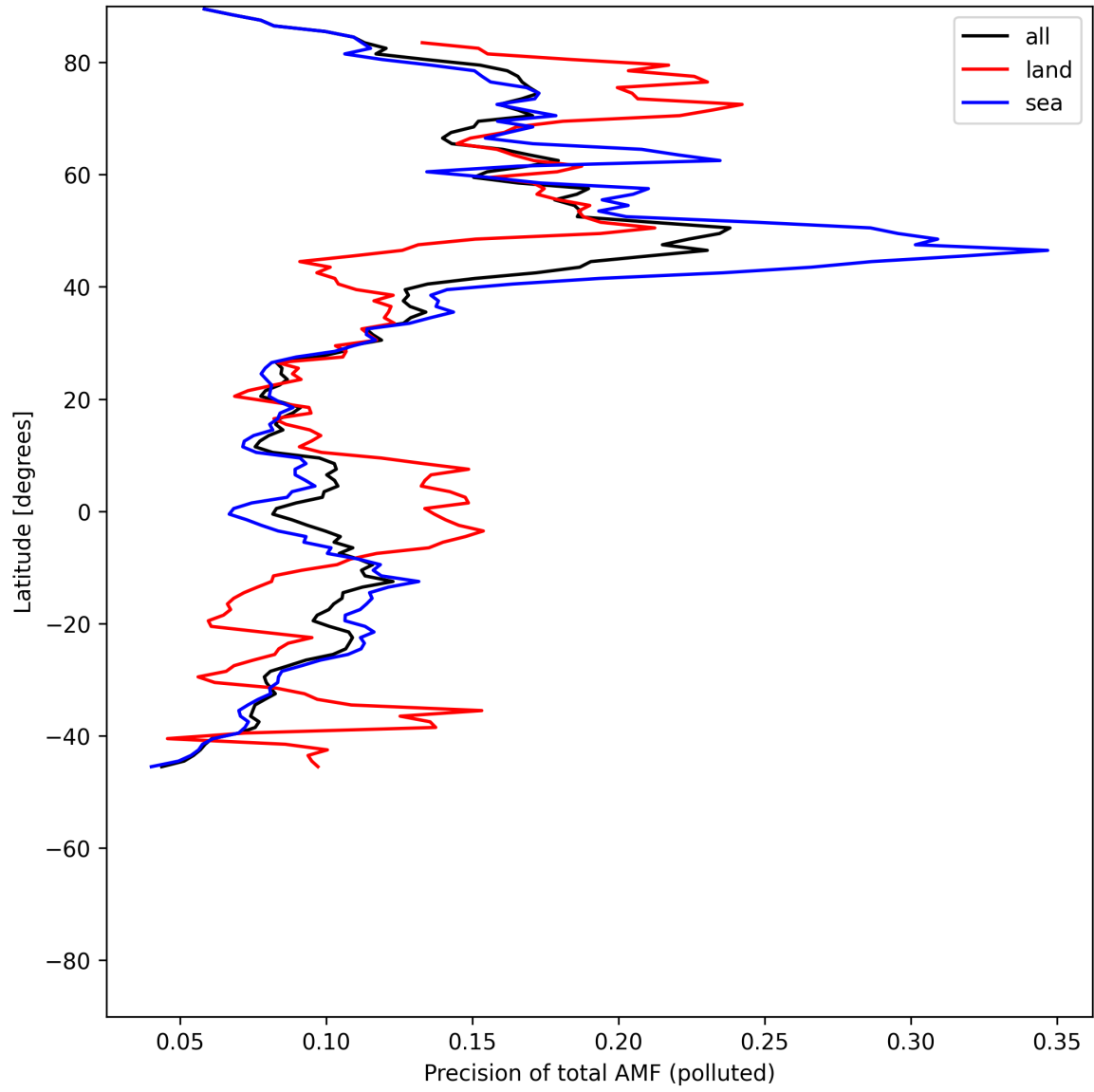
Figure 54: Zonal average of “Precision of total AMF (polluted)” for 2025-06-28 to 2025-06-29.
