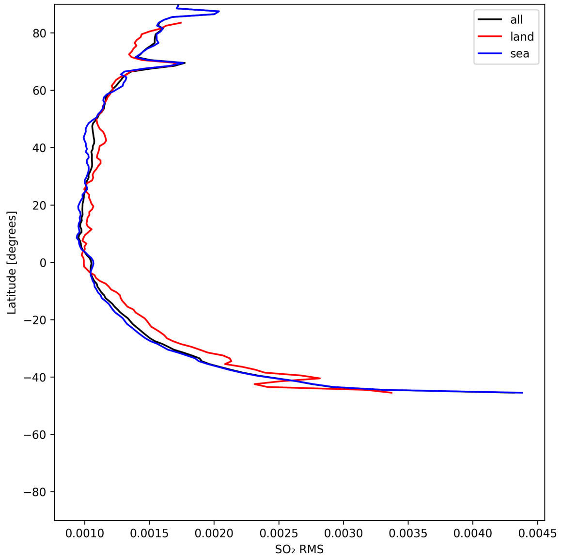
Figure 52: Zonal average of “SO 2 RMS” for 2025-06-28 to 2025-06-29.
