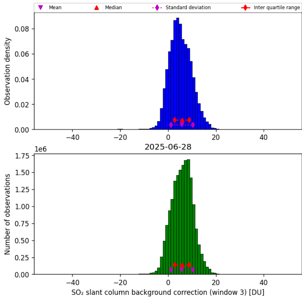
Figure 74: Histogram of “SO 2 slant column background correction (window 3)” for 2025-06-28 to 2025-06-29
