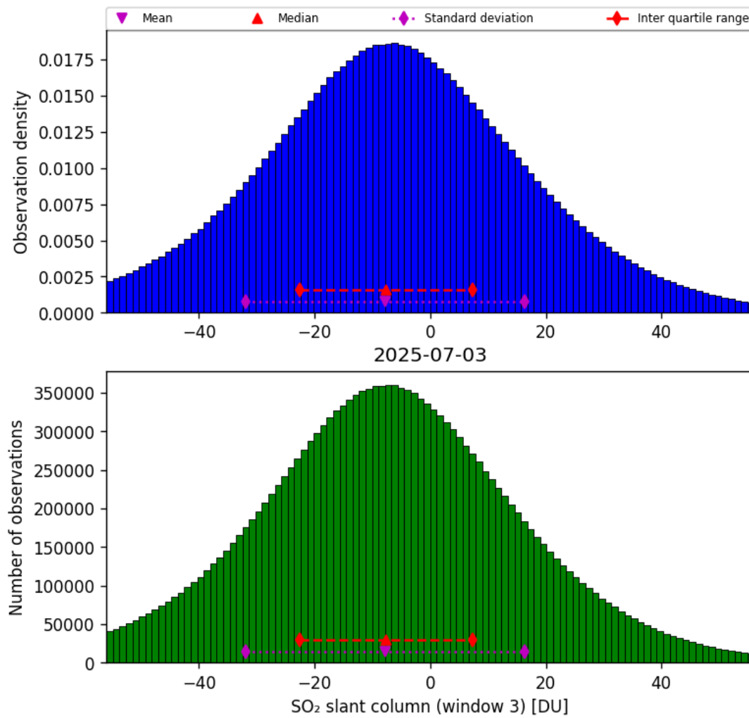
Figure 71: Histogram of “SO 2 slant column (window 3)” for 2025-07-03 to 2025-07-04
