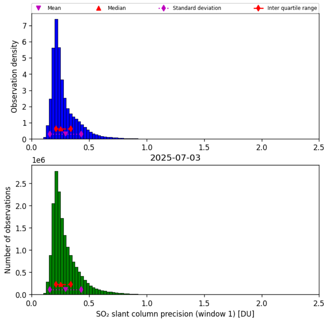
Figure 64: Histogram of “SO 2 slant column precision (window 1)” for 2025-07-03 to 2025-07-04
