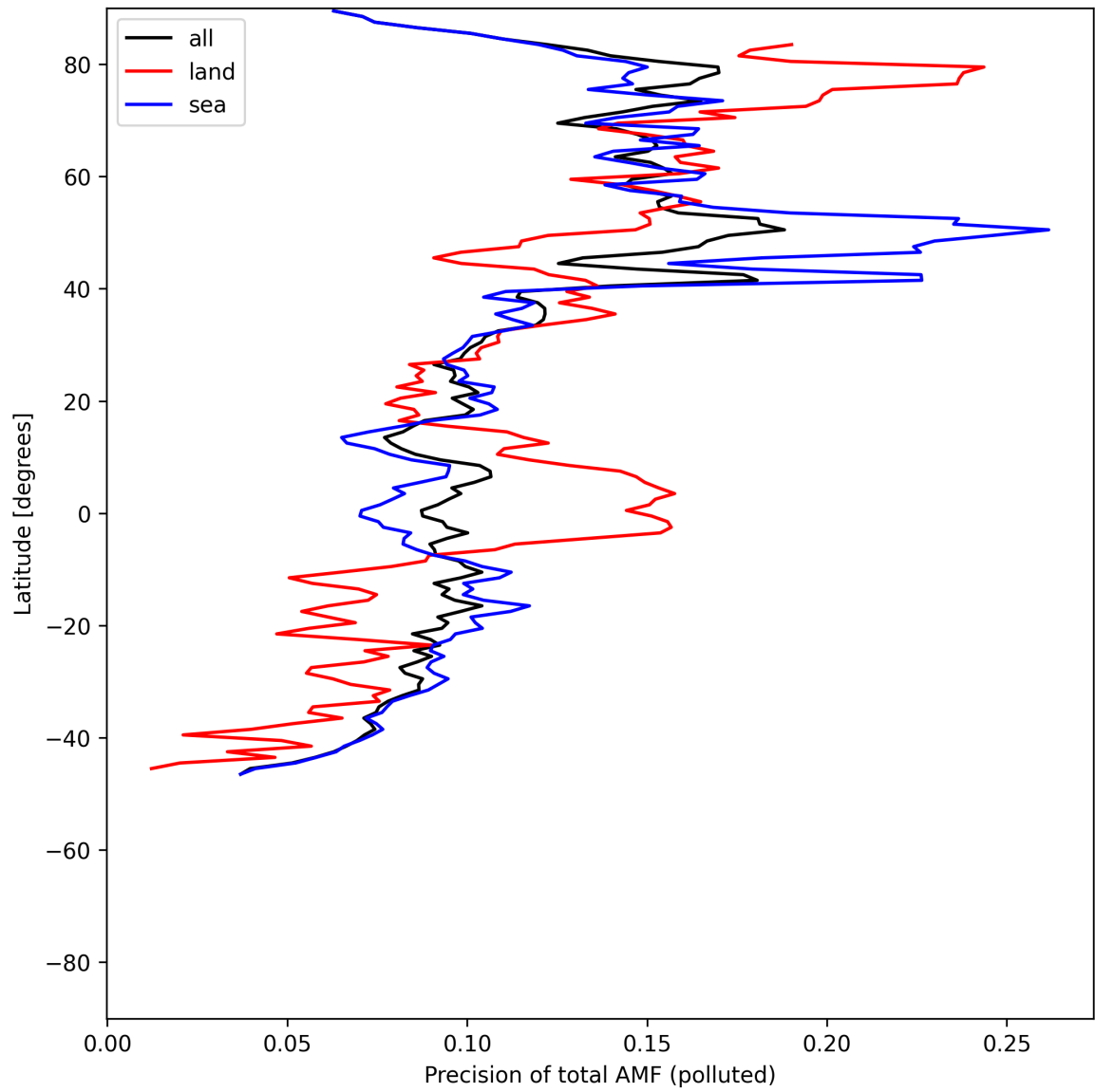
Figure 54: Zonal average of “Precision of total AMF (polluted)” for 2025-07-03 to 2025-07-04.
