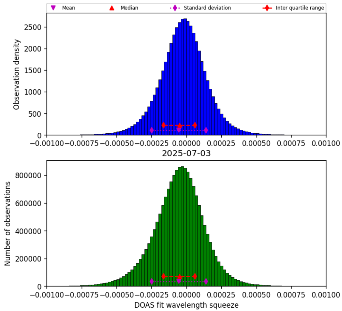
Figure 78: Histogram of “DOAS fit wavelength squeeze” for 2025-07-03 to 2025-07-04
