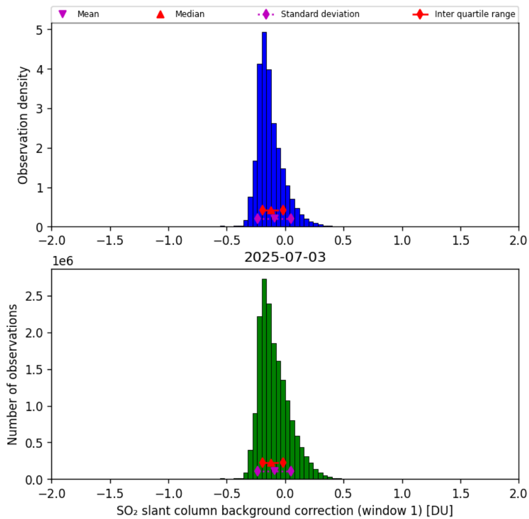
Figure 66: Histogram of “SO 2 slant column background correction (window 1)” for 2025-07-03 to 2025-07-04
