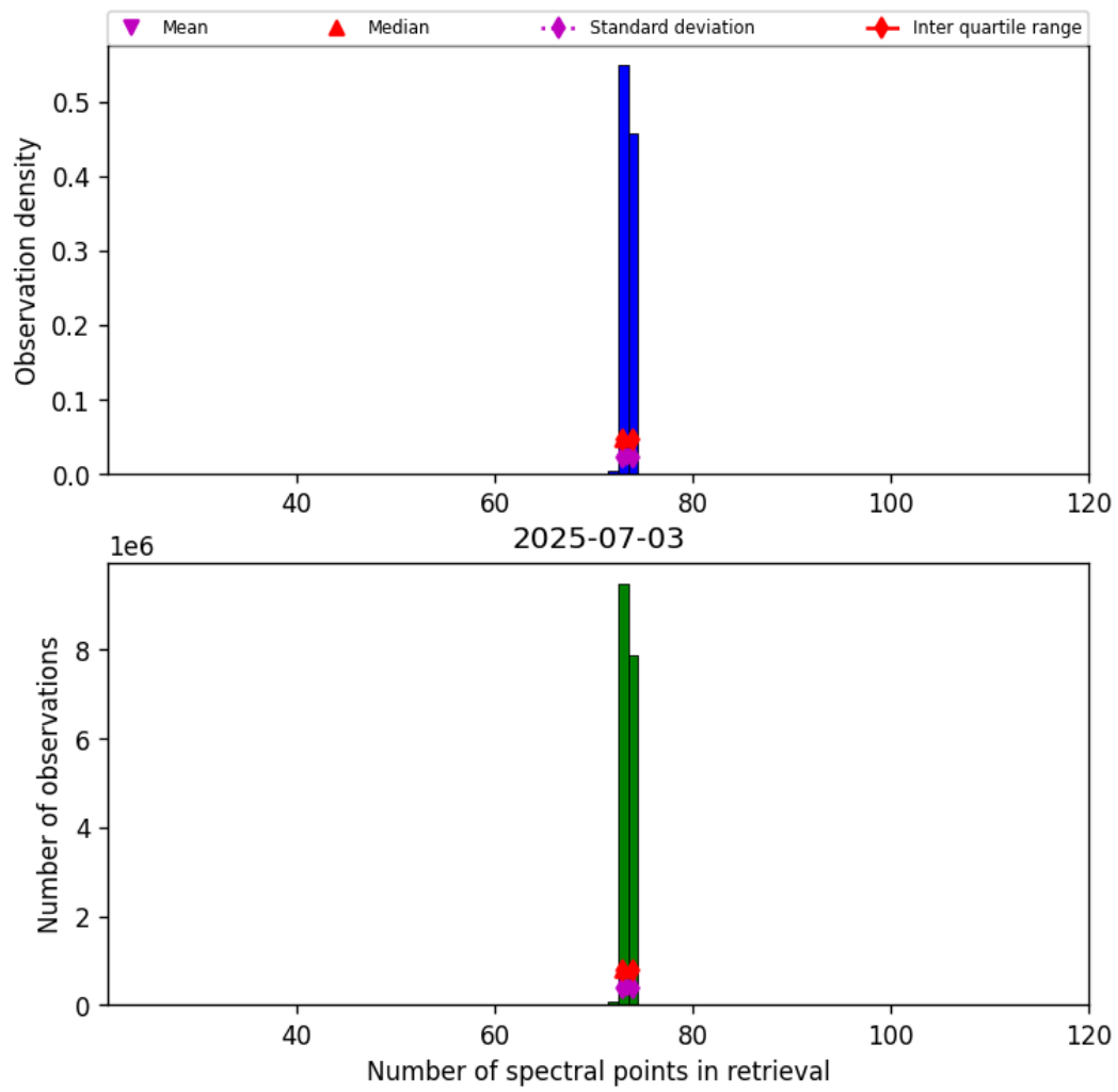
Figure 83: Histogram of “Number of spectral points in retrieval” for 2025-07-03 to 2025-07-04
