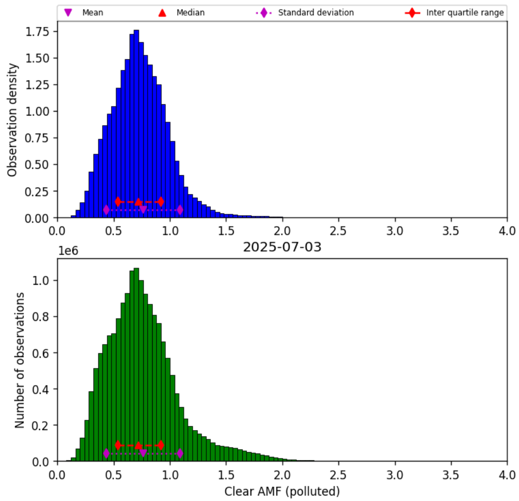
Figure 82: Histogram of “Clear AMF (polluted)” for 2025-07-03 to 2025-07-04
