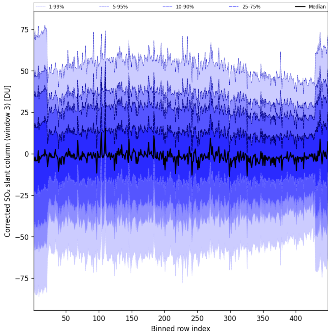
Figure 100: Along track statistics of “Corrected SO 2 slant column (window 3)” for 2025-07-03 to 2025-07-04
