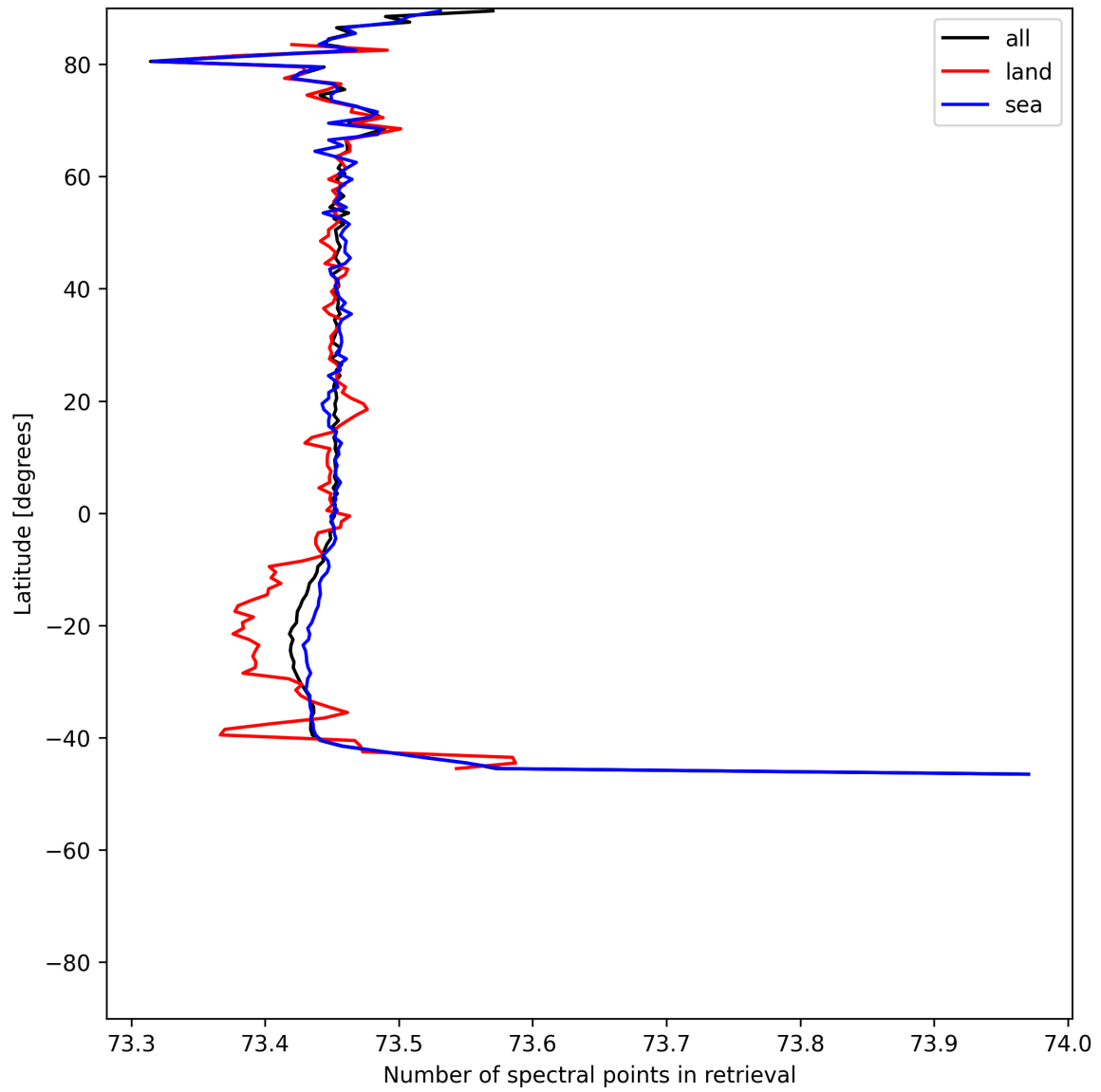
Figure 56: Zonal average of “Number of spectral points in retrieval” for 2025-07-03 to 2025-07-04.
