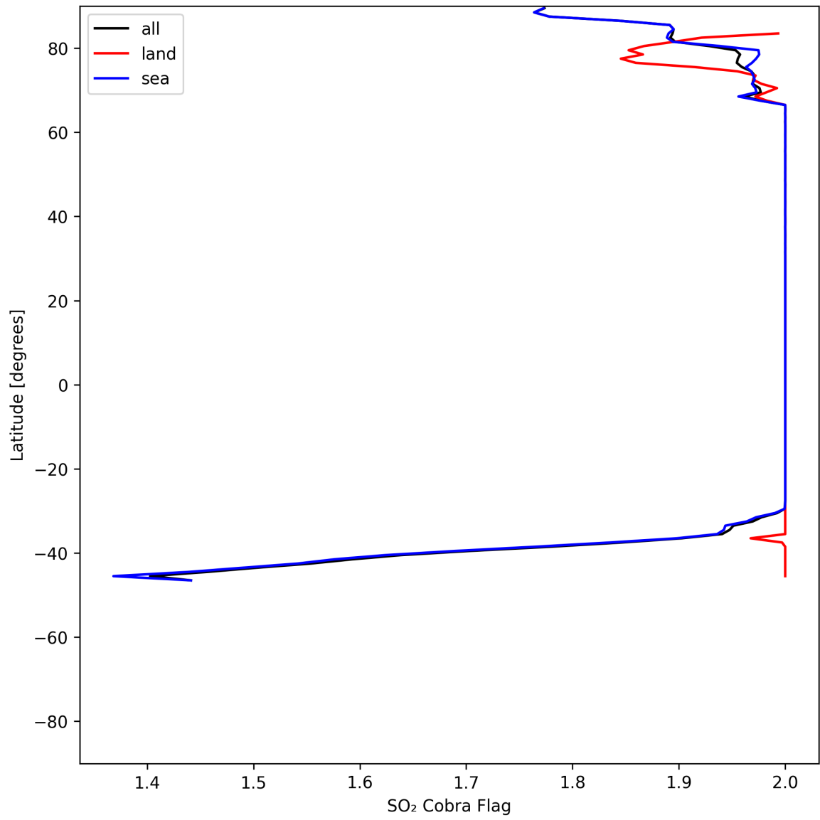
Figure 48: Zonal average of “SO 2 Cobra Flag” for 2025-07-03 to 2025-07-04.
