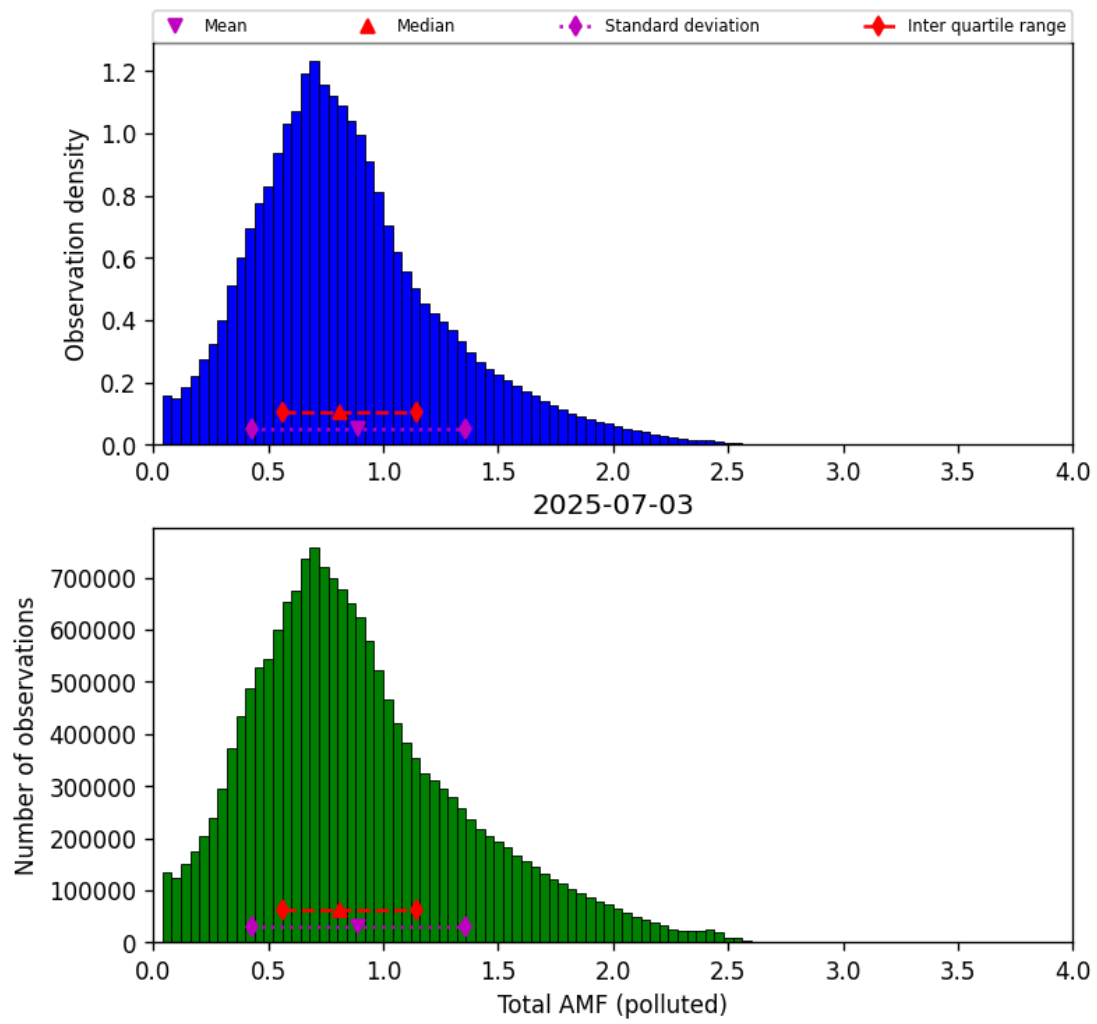
Figure 80: Histogram of “Total AMF (polluted)” for 2025-07-03 to 2025-07-04
