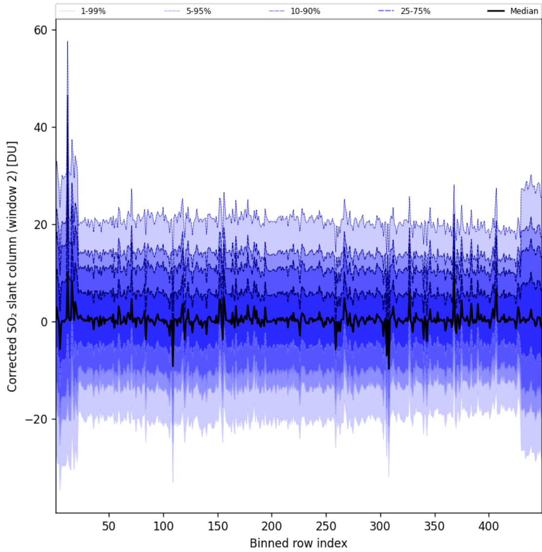
Figure 96: Along track statistics of "Corrected SO 2 slant column (window 2)" for 2025-07-03 to 2025-07-04
