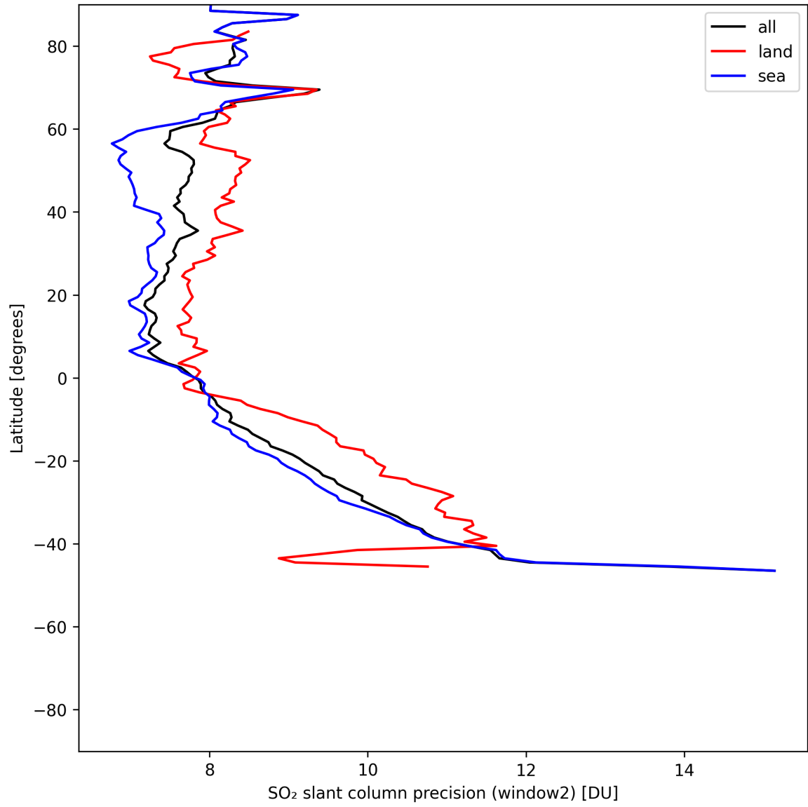
Figure 41: Zonal average of “SO 2 slant column precision (window2)” for 2025-07-03 to 2025-07-04.
