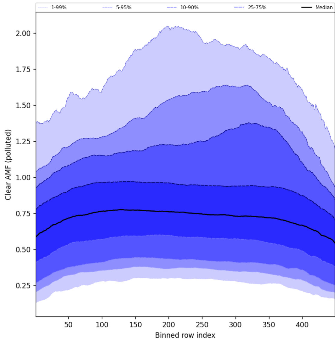
Figure 109: Along track statistics of “Clear AMF (polluted)” for 2025-07-03 to 2025-07-04
