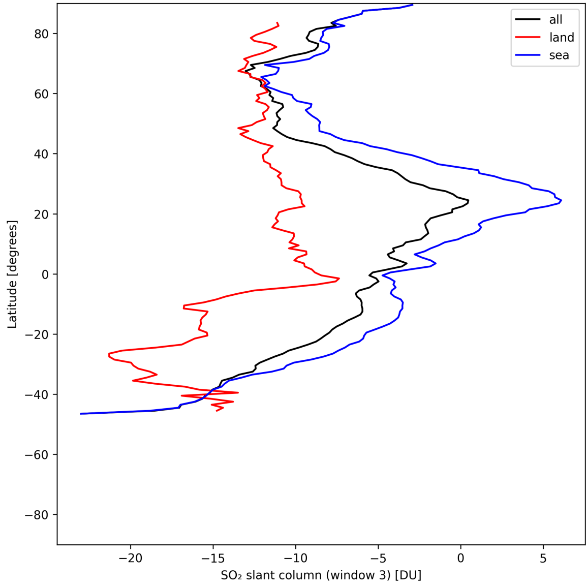
Figure 44: Zonal average of “SO 2 slant column (window 3)” for 2025-07-03 to 2025-07-04.
