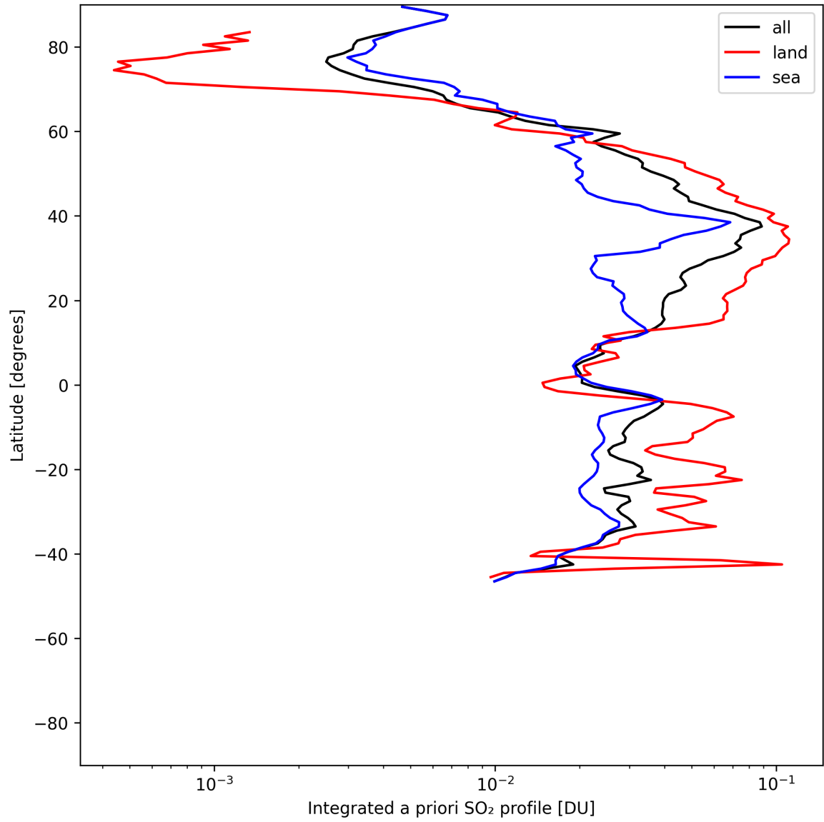
Figure 49: Zonal average of “Integrated a priori SO 2 profile” for 2025-07-03 to 2025-07-04.
