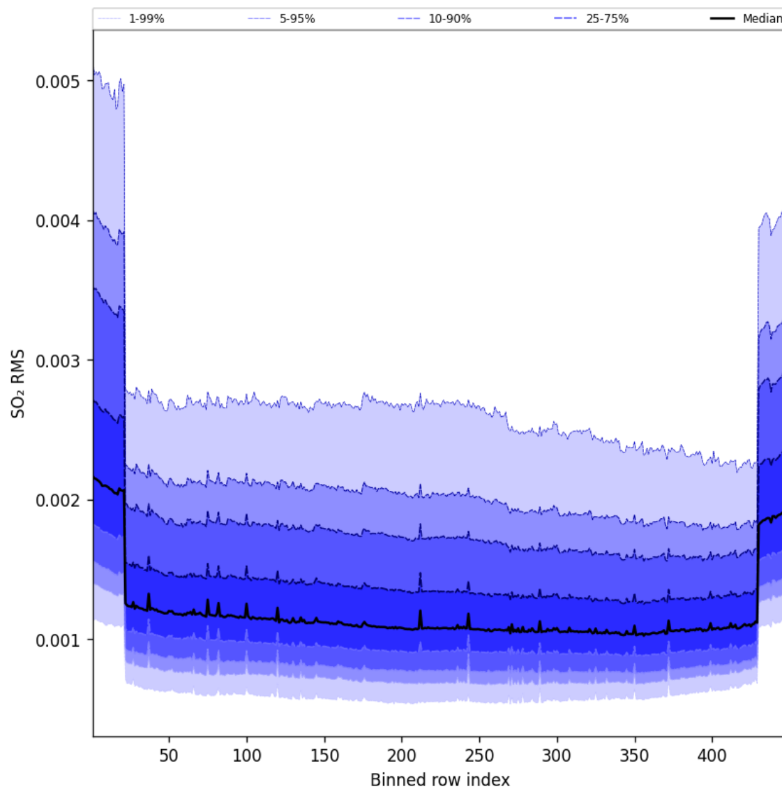
Figure 106: Along track statistics of “SO 2 RMS” for 2025-07-03 to 2025-07-04
