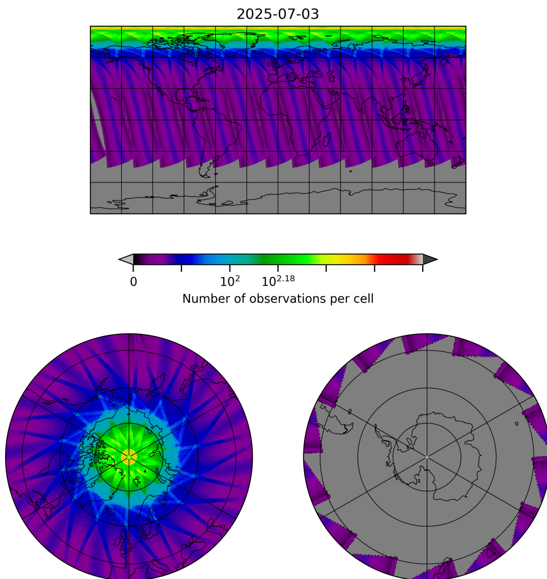
Figure 29: Map of the number of observations for 2025-07-03 to 2025-07-04
