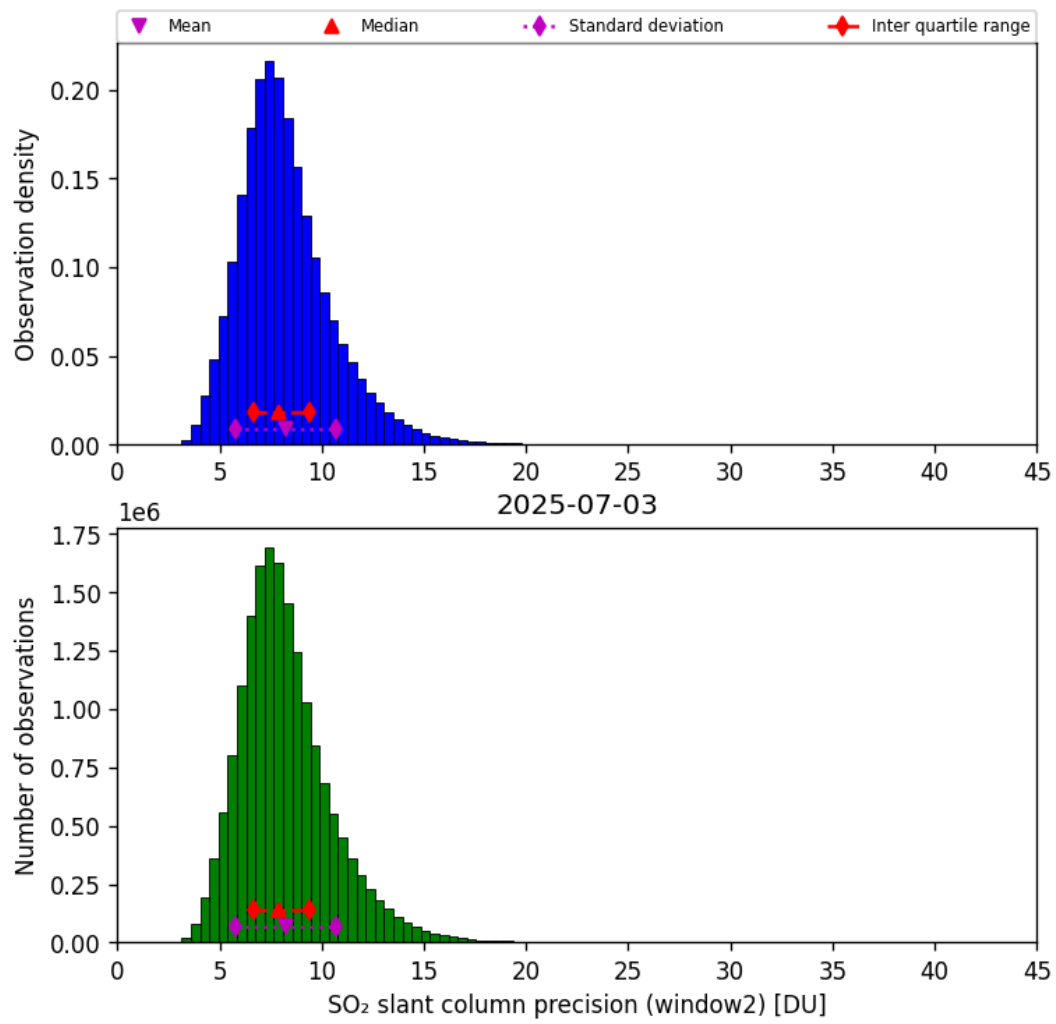
Figure 68: Histogram of “SO 2 slant column precision (window2)” for 2025-07-03 to 2025-07-04
