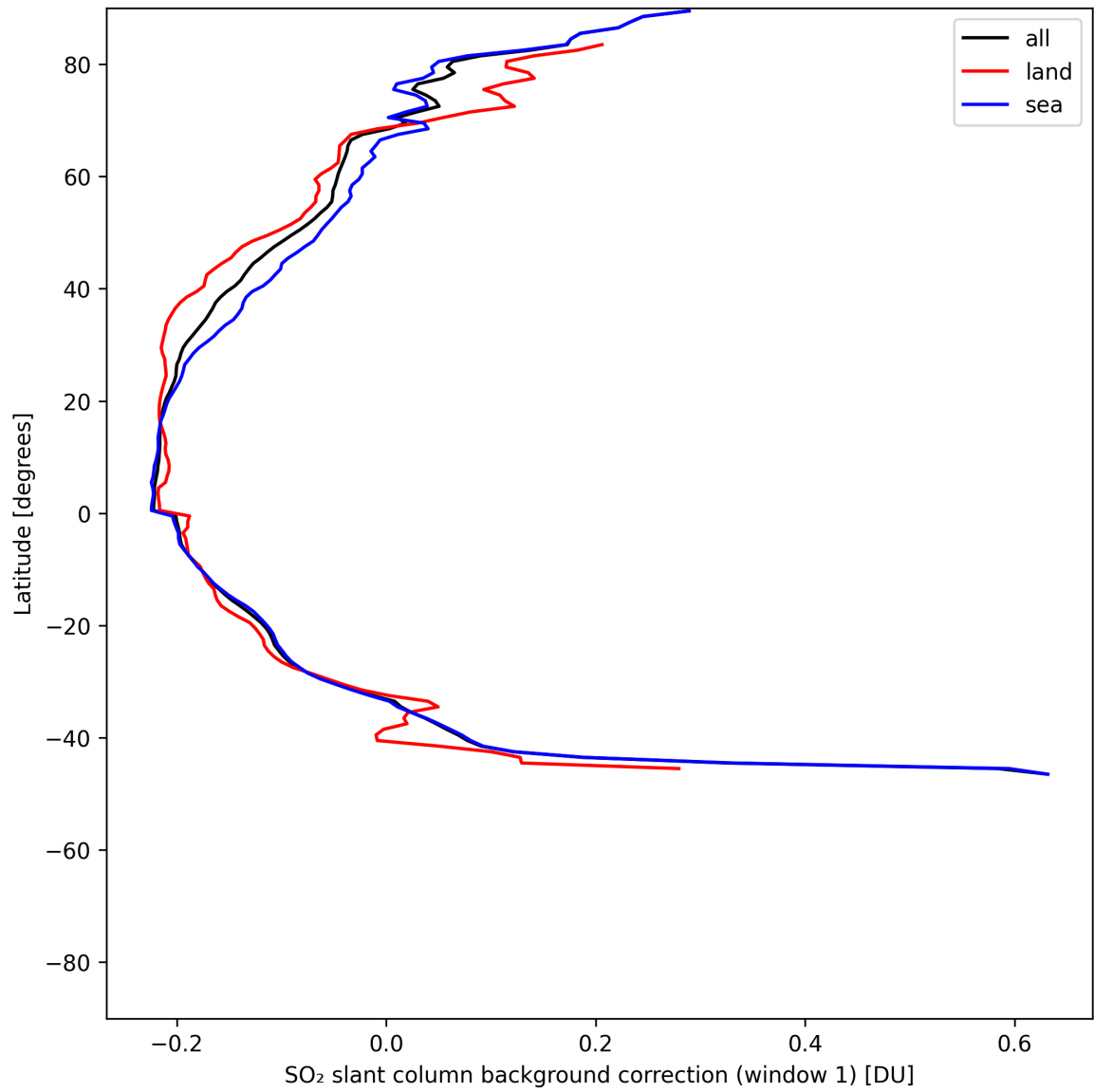
Figure 39: Zonal average of “SO 2 slant column background correction (window 1)” for 2025-07-03 to 2025-07-04.
