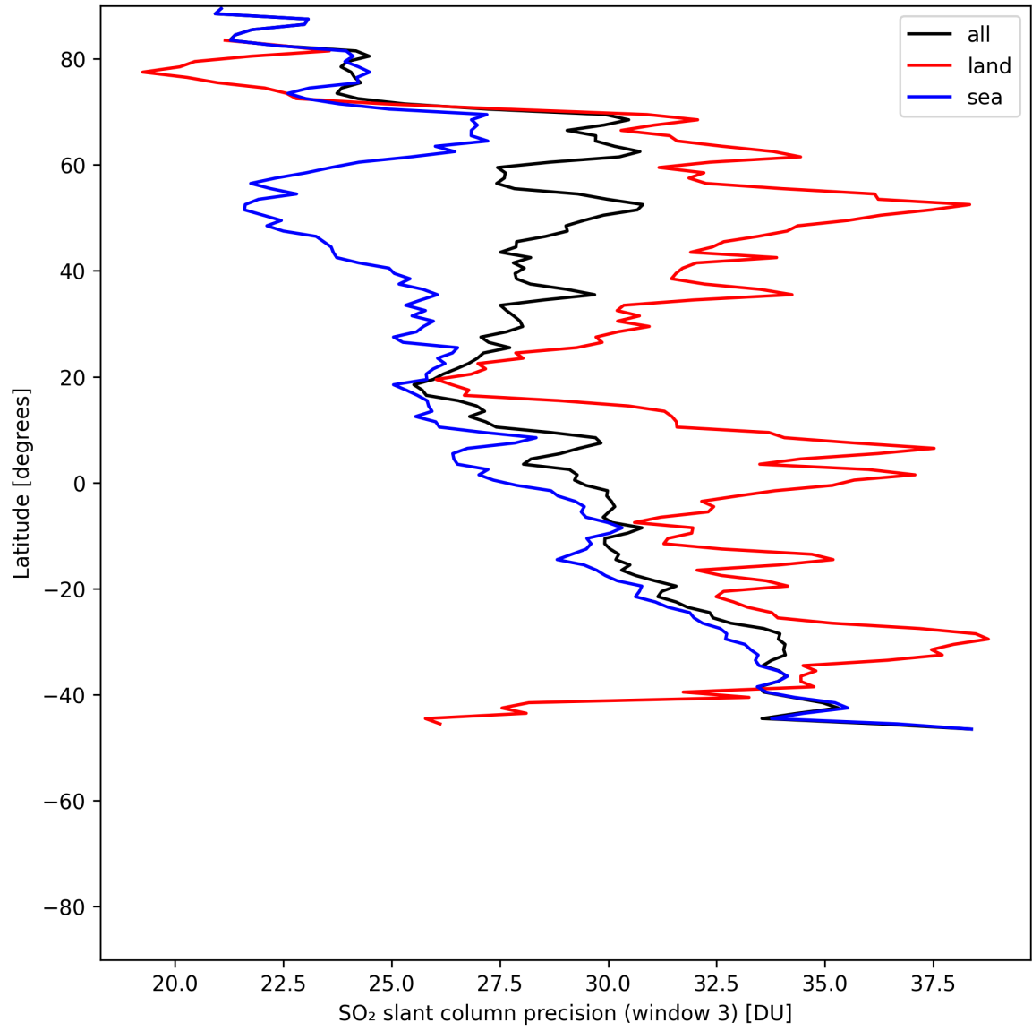
Figure 45: Zonal average of “SO 2 slant column precision (window 3)” for 2025-07-03 to 2025-07-04.
