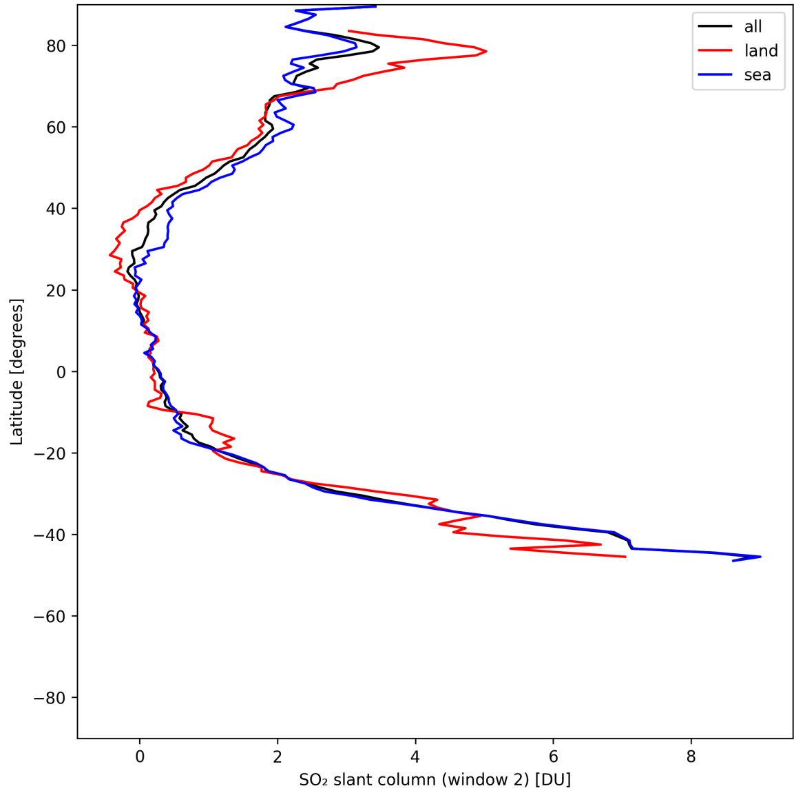
Figure 40: Zonal average of “SO 2 slant column (window 2)” for 2025-07-03 to 2025-07-04.
