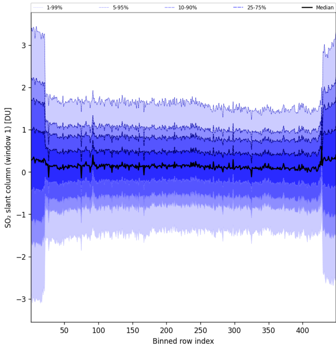
Figure 90: Along track statistics of “SO 2 slant column (window 1)” for 2025-07-03 to 2025-07-04
