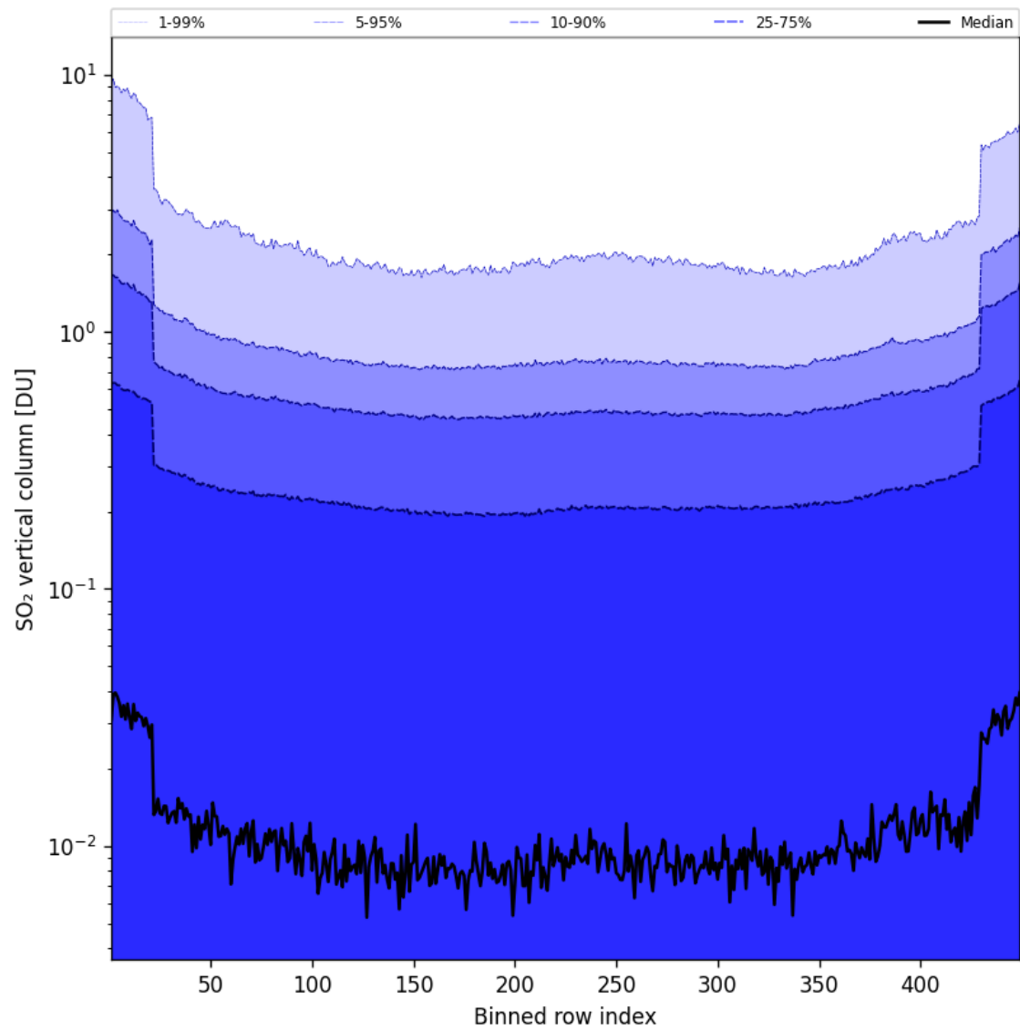
Figure 85: Along track statistics of “SO 2 vertical column” for 2025-07-03 to 2025-07-04
