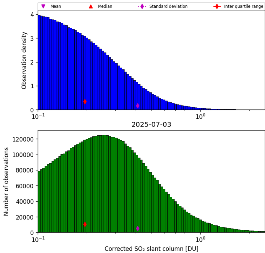
Figure 60: Histogram of “Corrected SO 2 slant column” for 2025-07-03 to 2025-07-04
