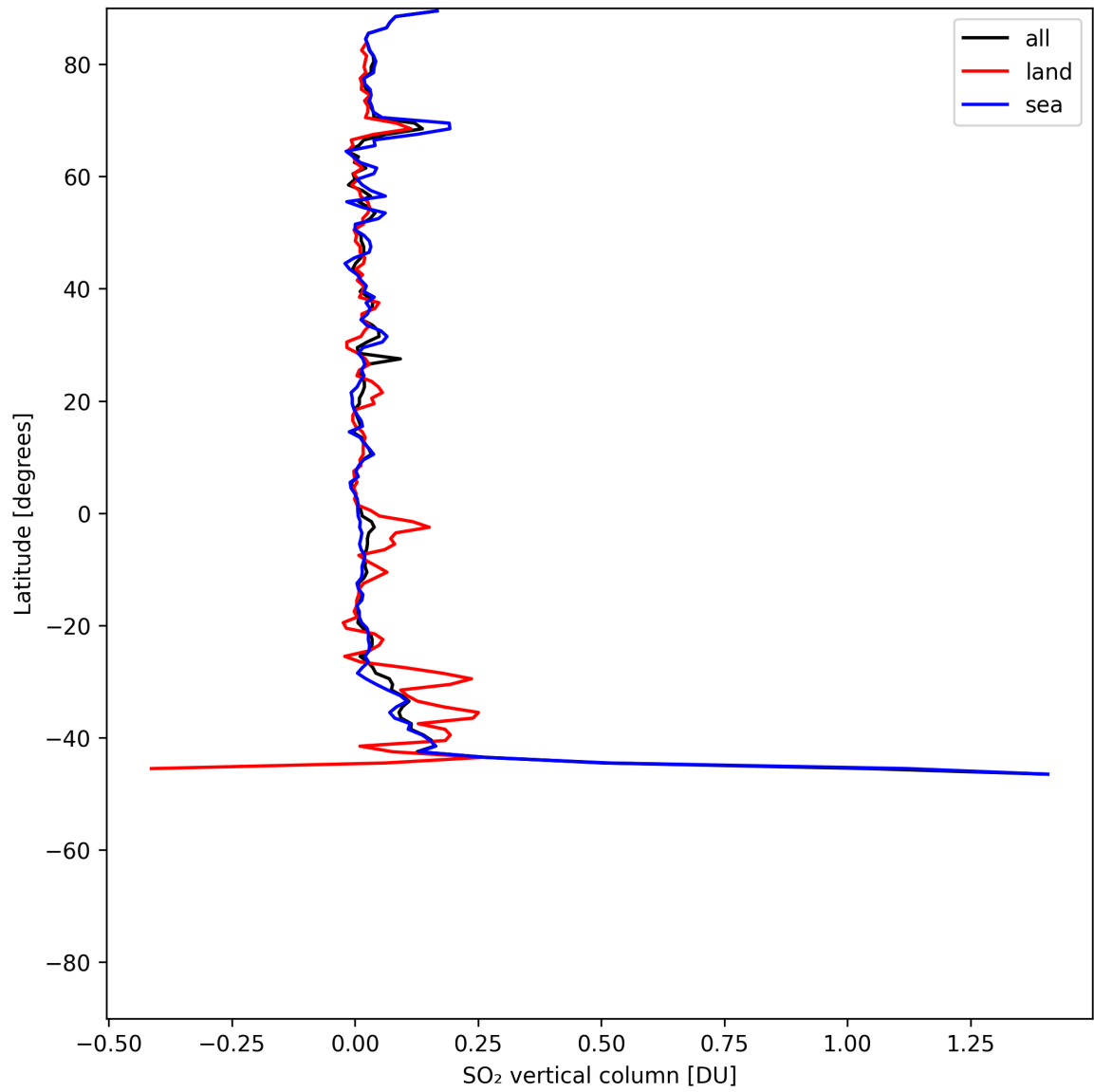
Figure 31: Zonal average of “SO 2 vertical column” for 2025-07-03 to 2025-07-04.
