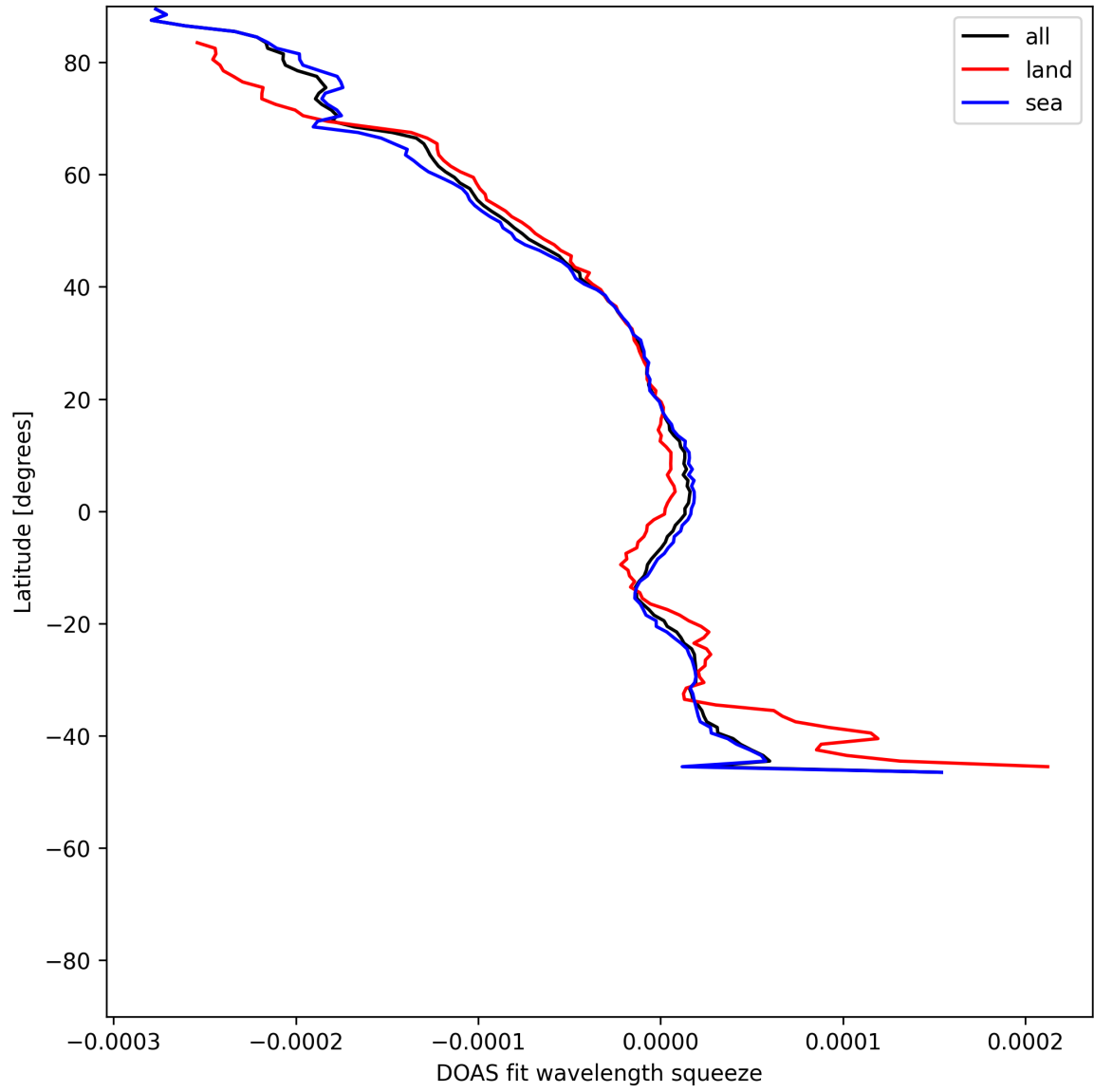
Figure 51: Zonal average of “DOAS fit wavelength squeeze” for 2025-07-03 to 2025-07-04.
