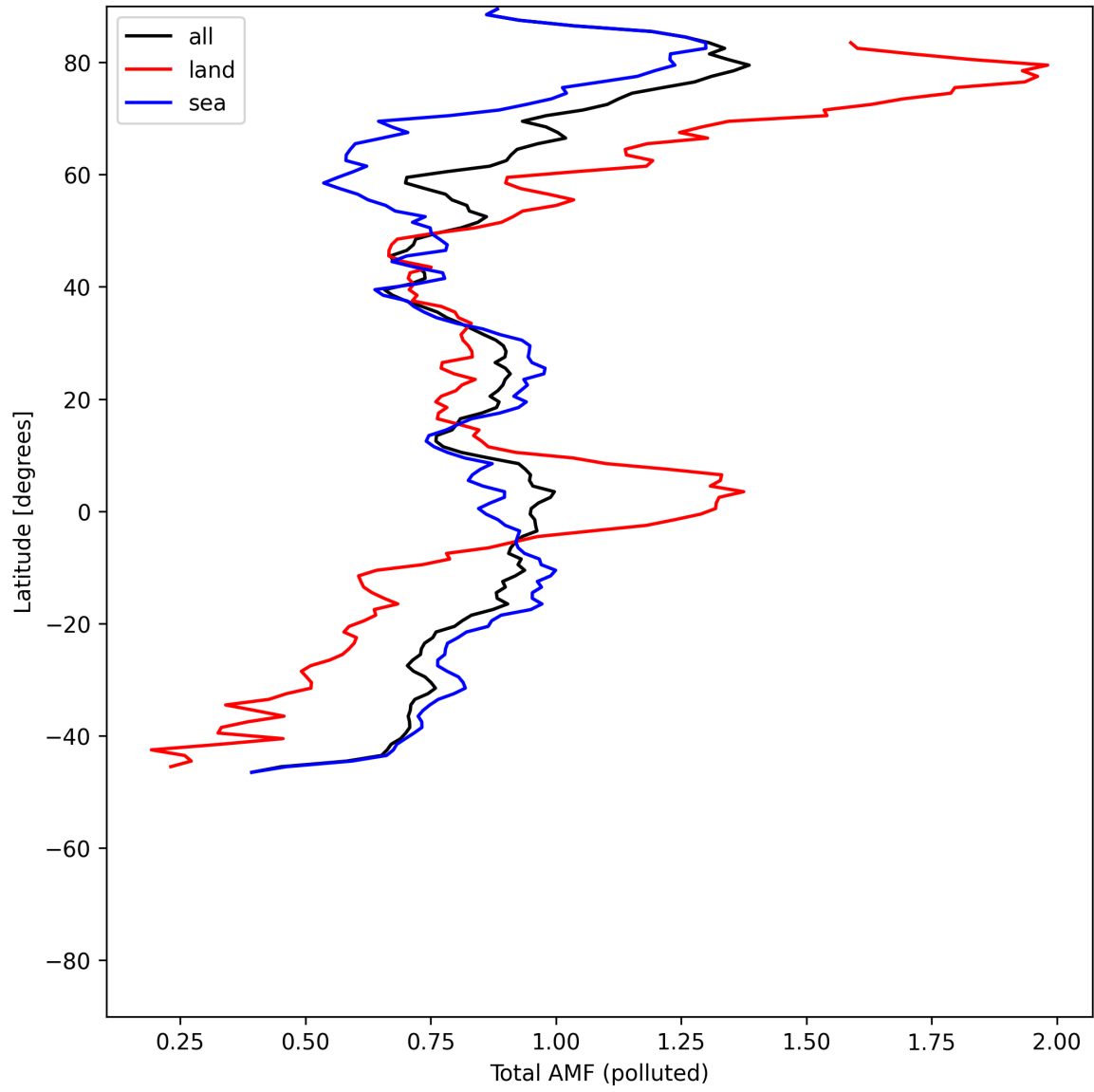
Figure 53: Zonal average of “Total AMF (polluted)” for 2025-07-03 to 2025-07-04.
