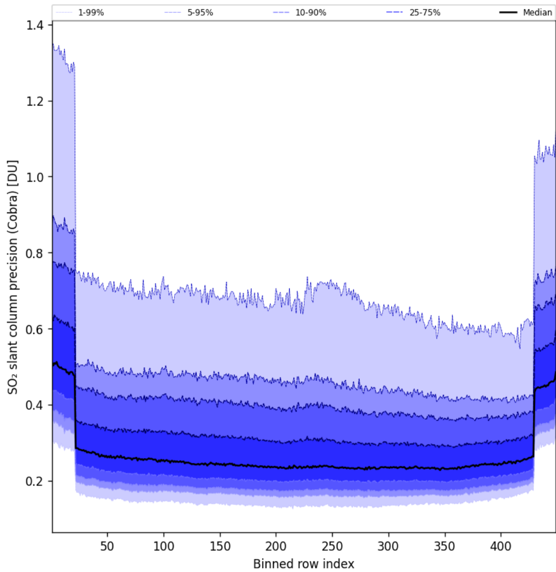
Figure 89: Along track statistics of “SO 2 slant column precision (Cobra)” for 2025-07-03 to 2025-07-04
