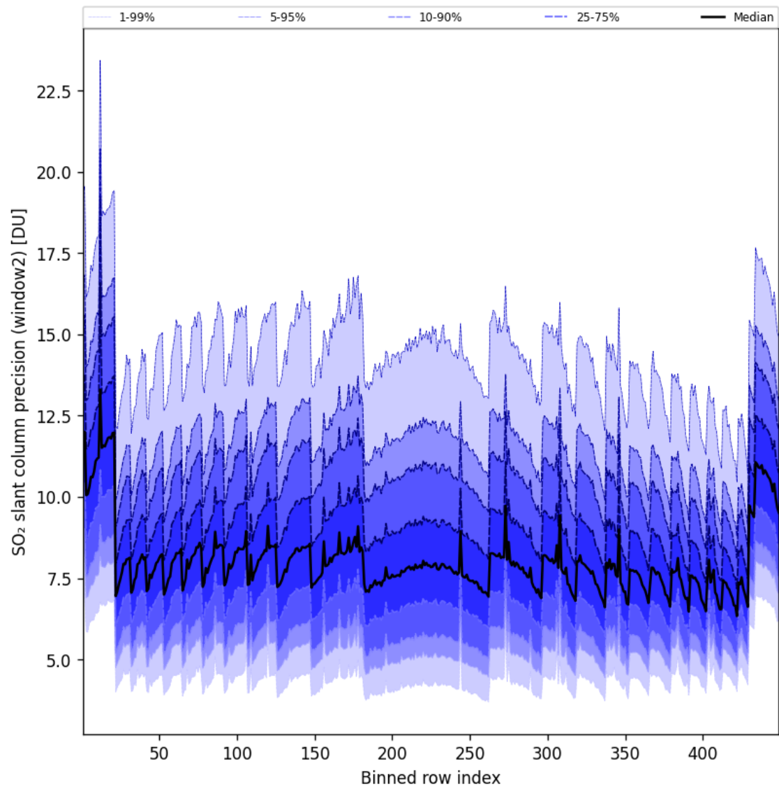
Figure 95: Along track statistics of “SO 2 slant column precision (window2)” for 2025-07-03 to 2025-07-04
