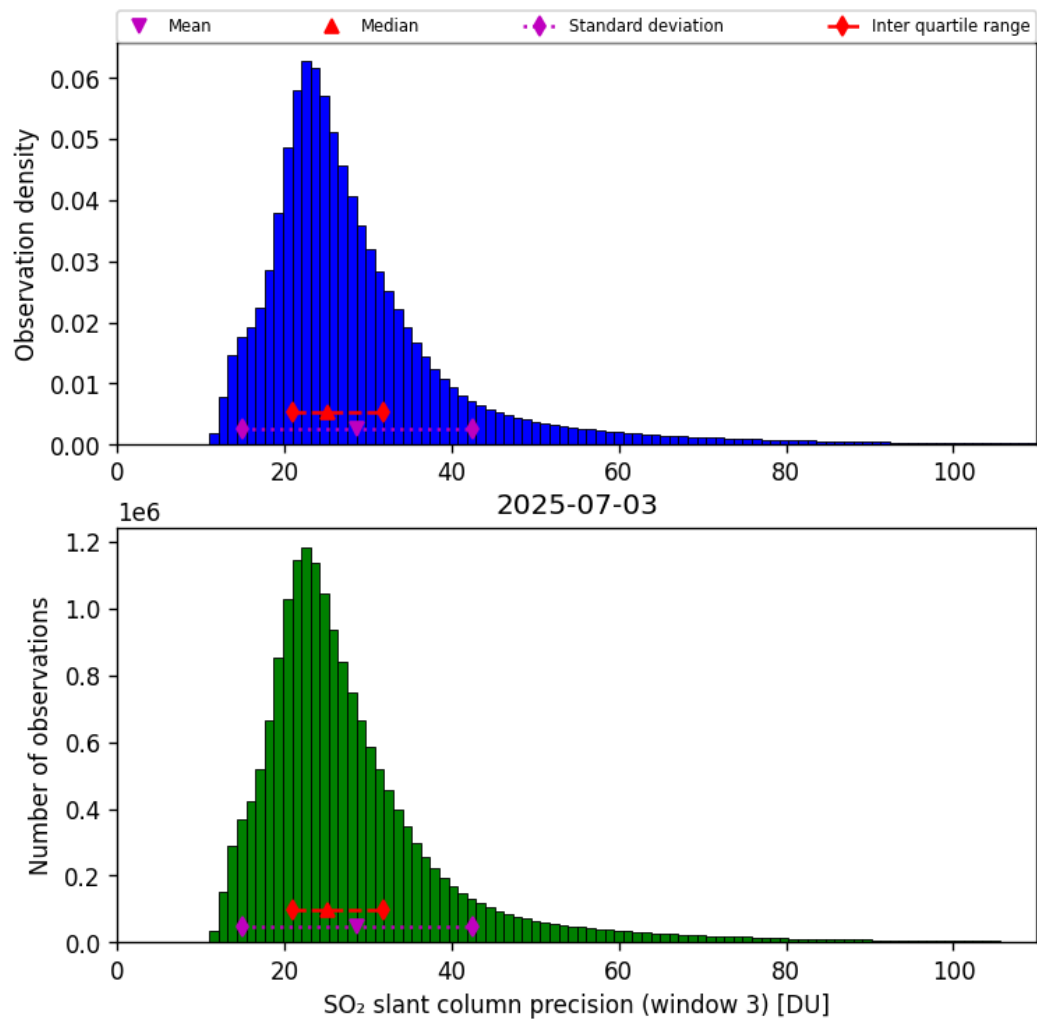
Figure 72: Histogram of “SO 2 slant column precision (window 3)” for 2025-07-03 to 2025-07-04
