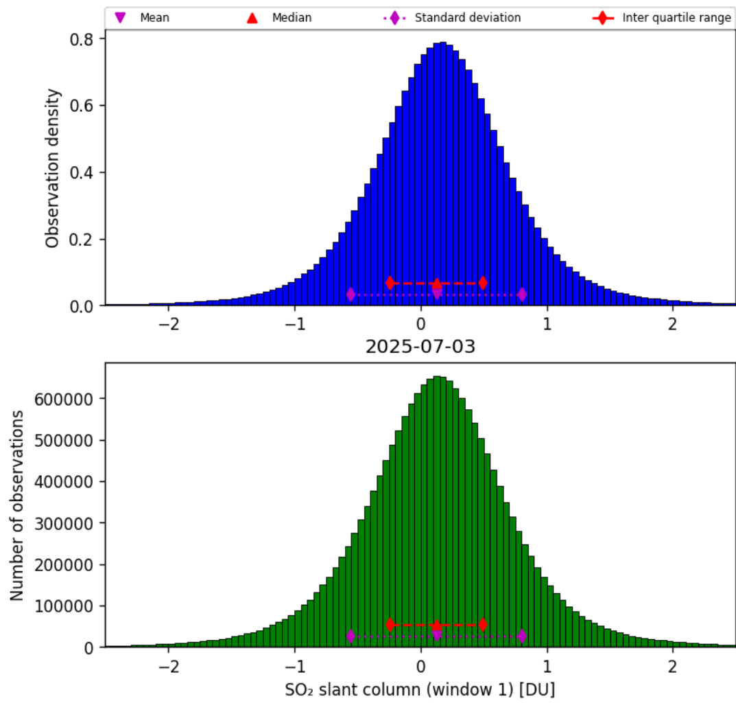
Figure 63: Histogram of “SO 2 slant column (window 1)” for 2025-07-03 to 2025-07-04
