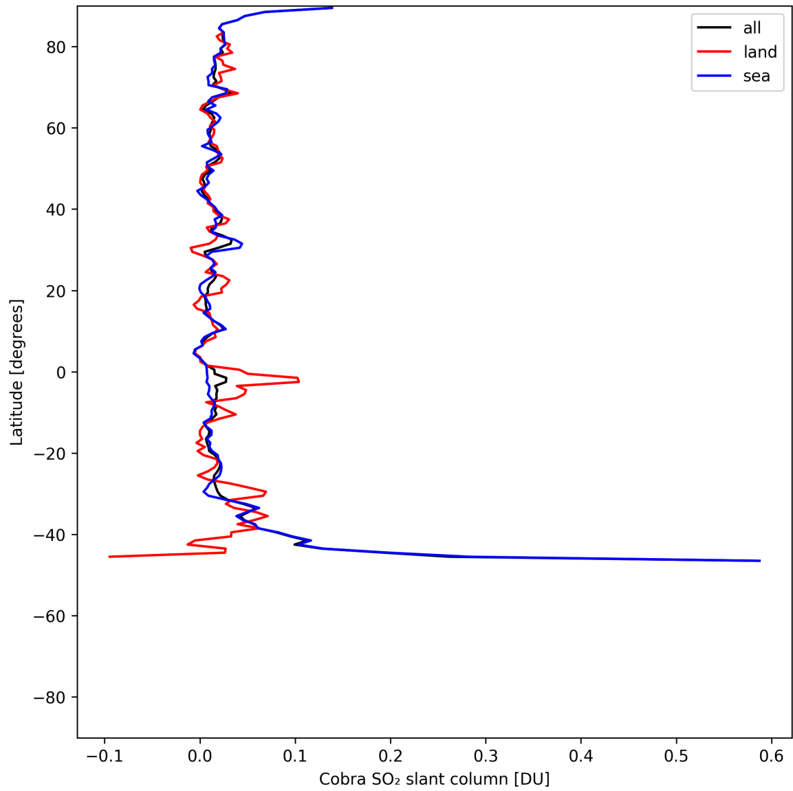
Figure 34: Zonal average of “Cobra SO 2 slant column” for 2025-07-03 to 2025-07-04.
