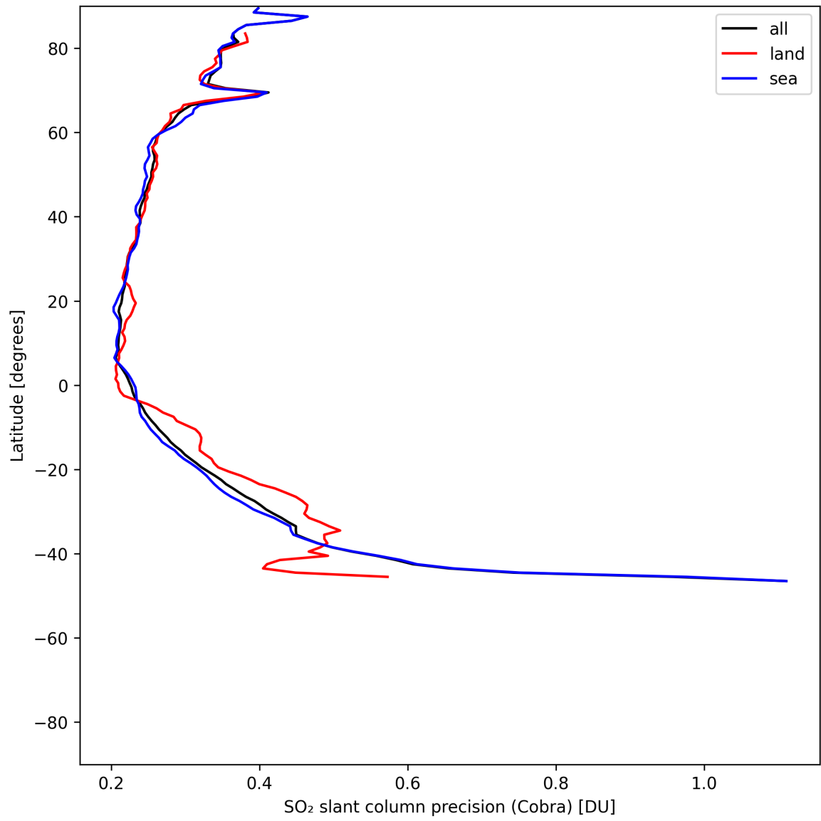
Figure 35: Zonal average of “SO 2 slant column precision (Cobra)” for 2025-07-03 to 2025-07-04.
