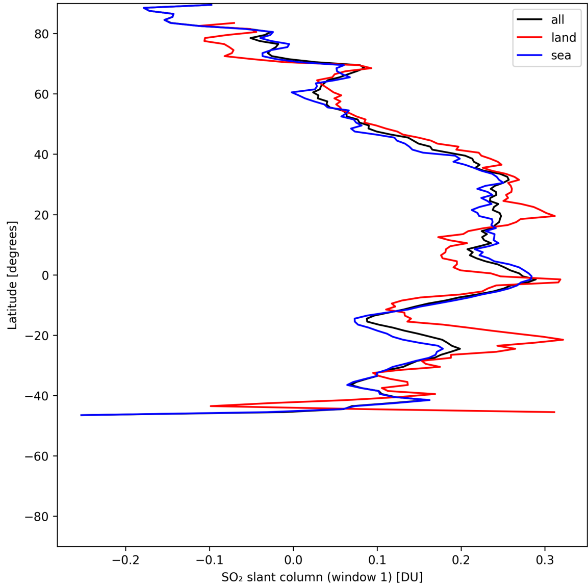
Figure 36: Zonal average of “SO 2 slant column (window 1)” for 2025-07-03 to 2025-07-04.
