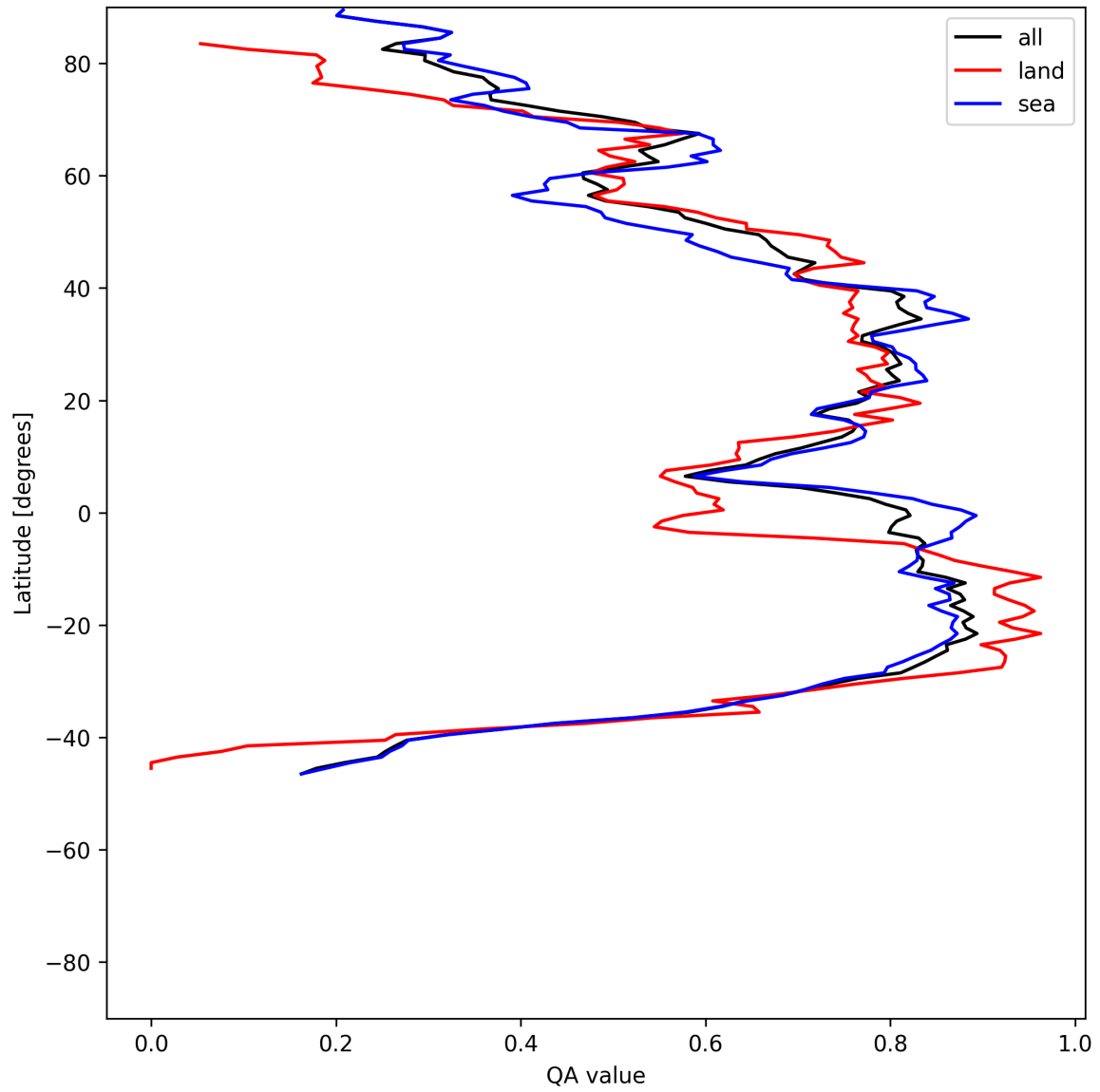
Figure 30: Zonal average of “QA value” for 2025-07-03 to 2025-07-04.
