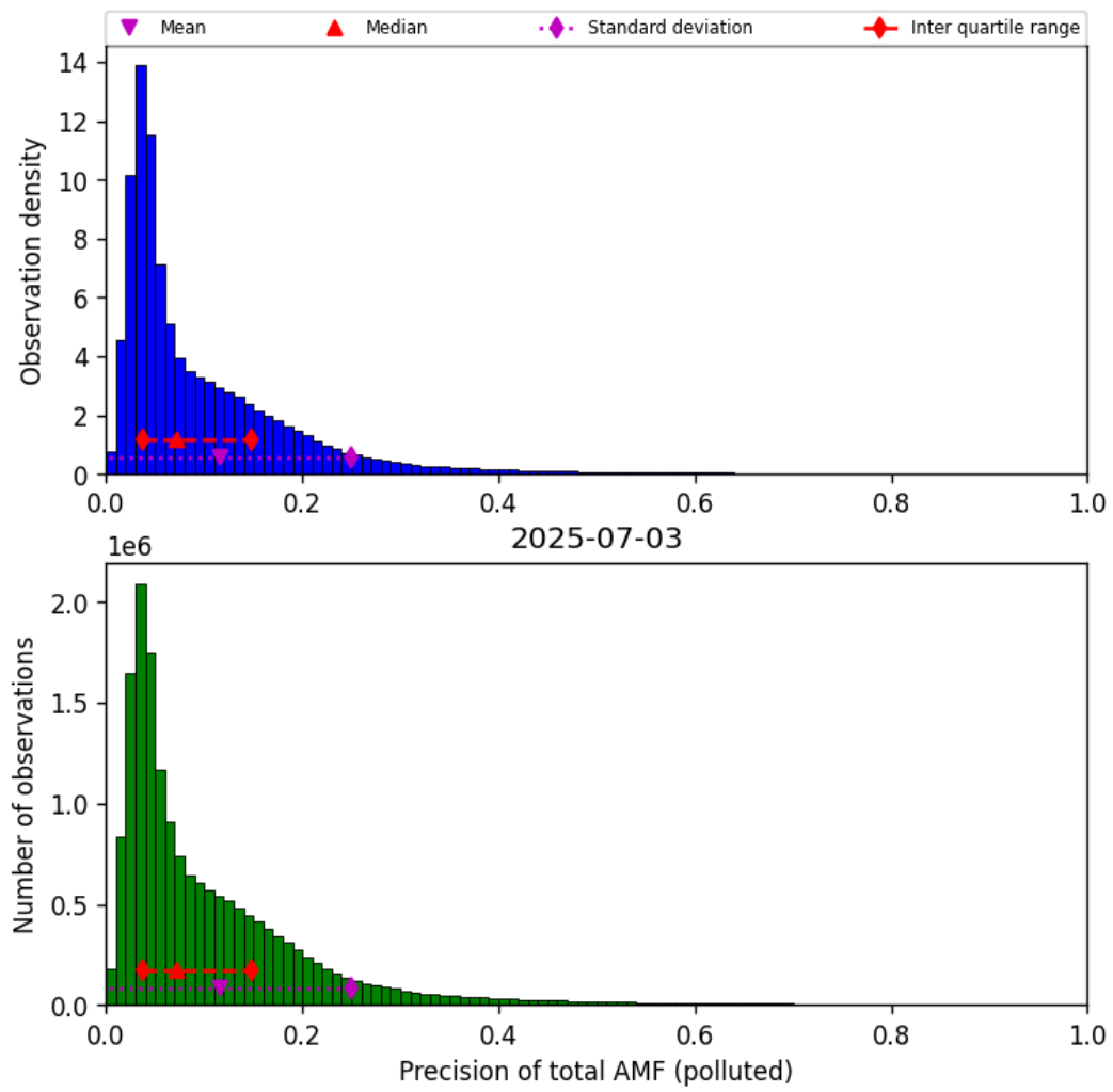
Figure 81: Histogram of “Precision of total AMF (polluted)” for 2025-07-03 to 2025-07-04
