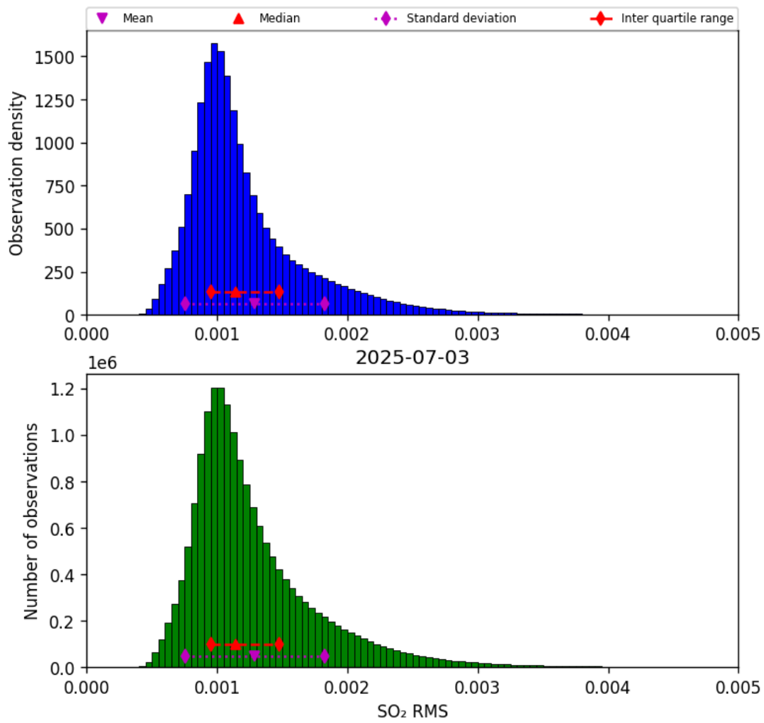
Figure 79: Histogram of “SO 2 RMS” for 2025-07-03 to 2025-07-04
