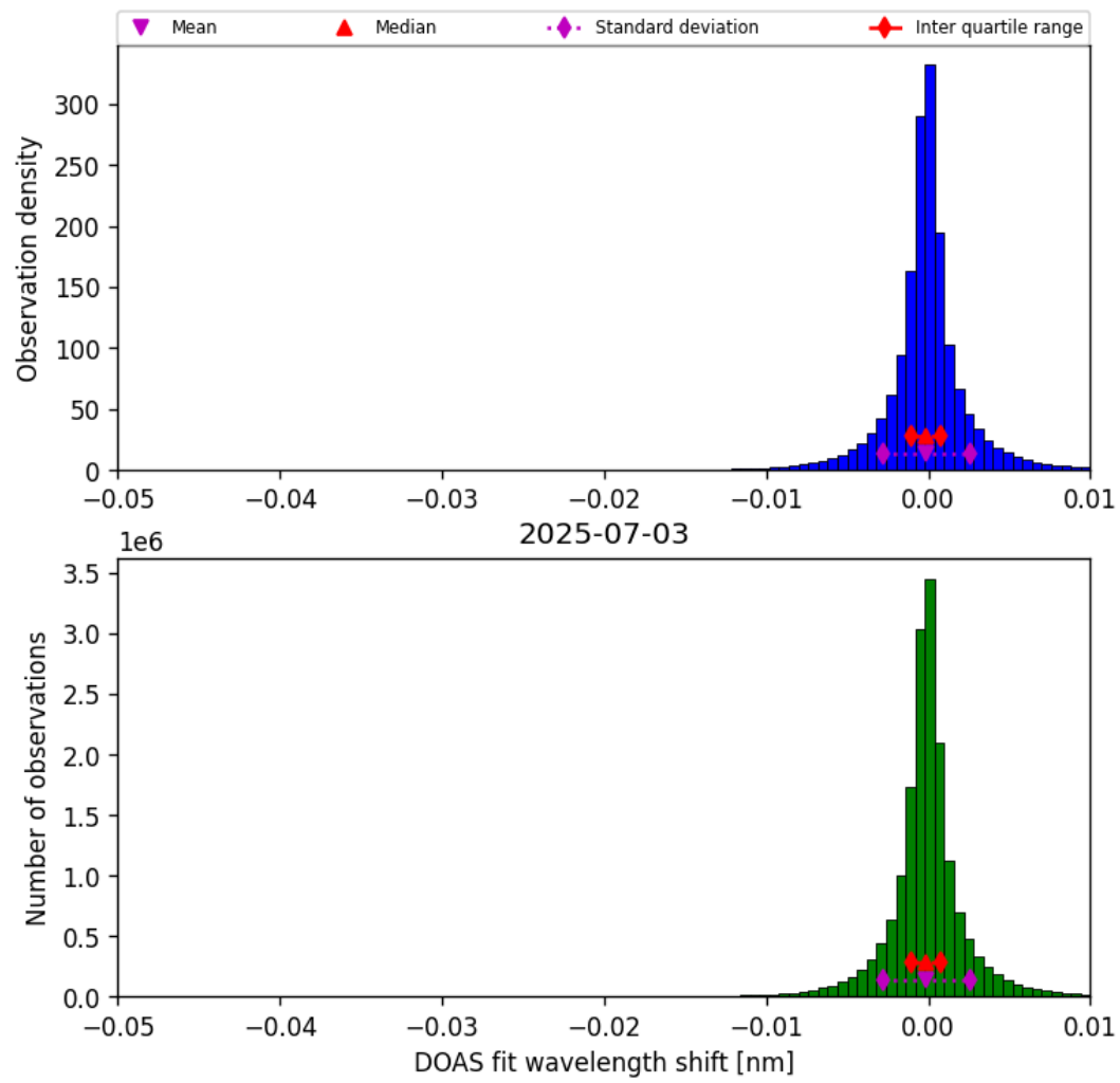
Figure 77: Histogram of “DOAS fit wavelength shift” for 2025-07-03 to 2025-07-04
