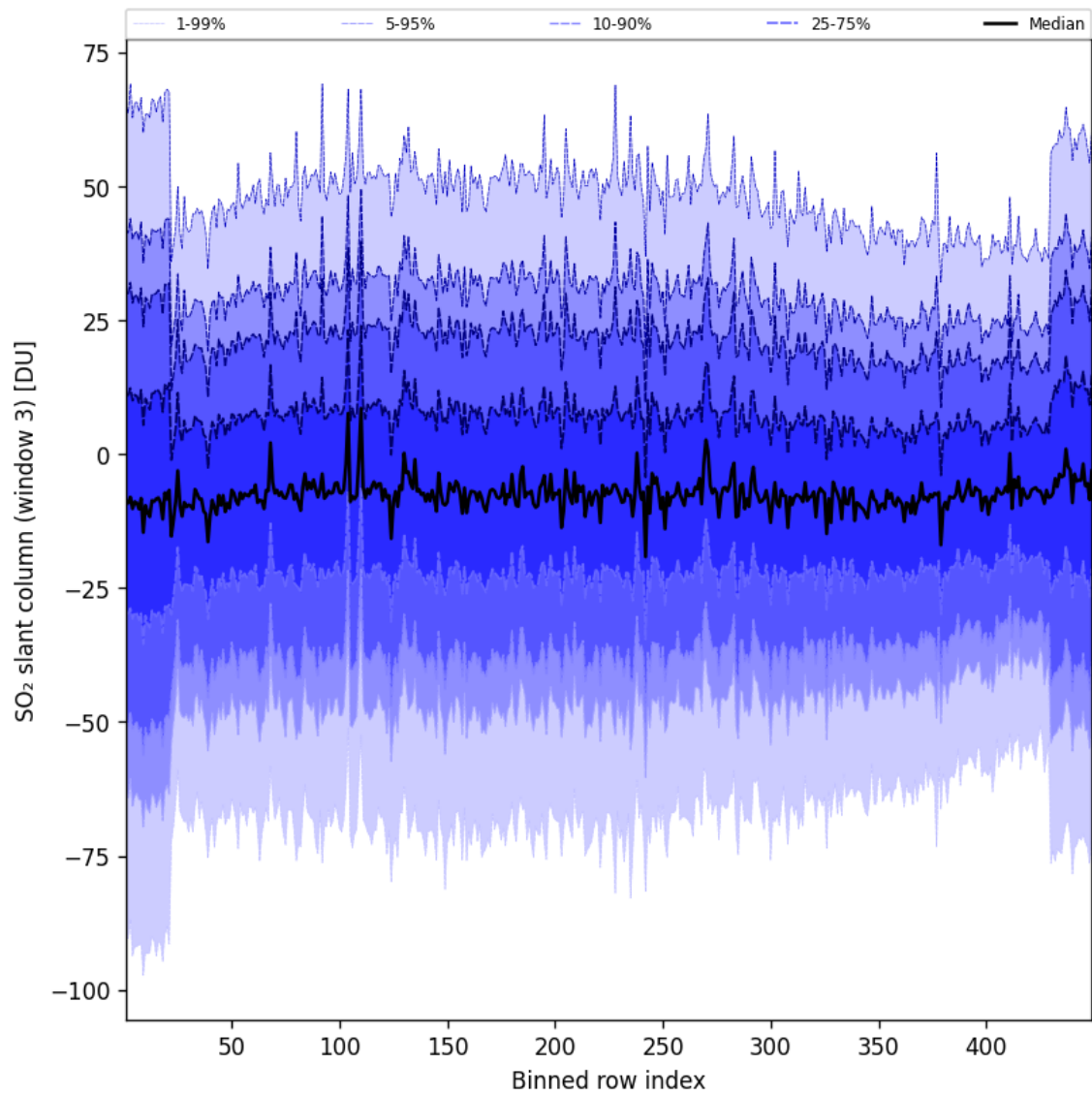
Figure 98: Along track statistics of “SO 2 slant column (window 3)” for 2025-07-03 to 2025-07-04
