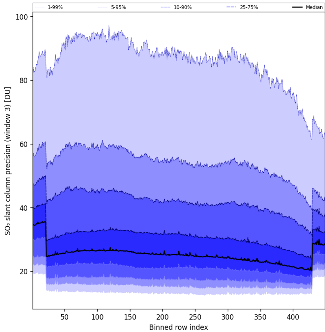
Figure 99: Along track statistics of “SO 2 slant column precision (window 3)” for 2025-07-03 to 2025-07-04
