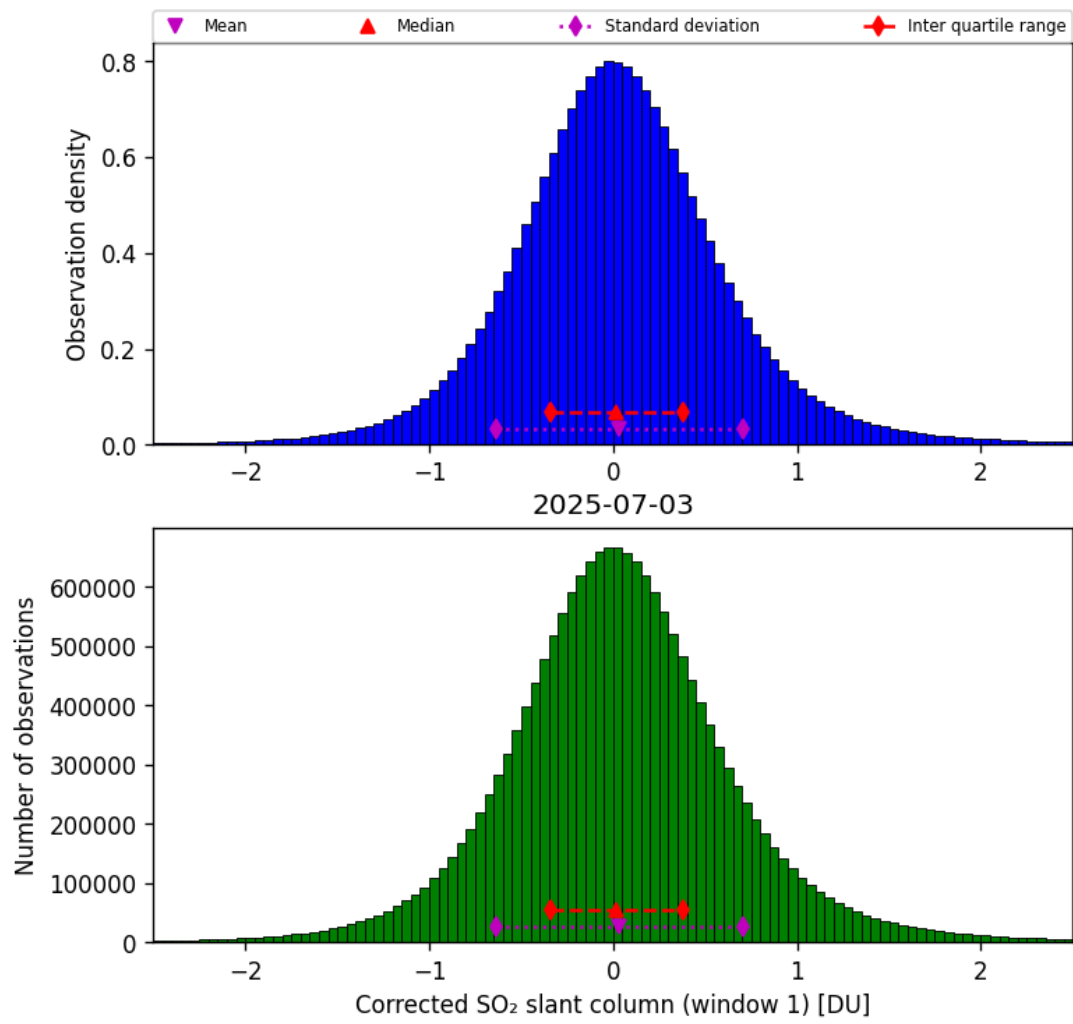
Figure 65: Histogram of “Corrected SO 2 slant column (window 1)” for 2025-07-03 to 2025-07-04
