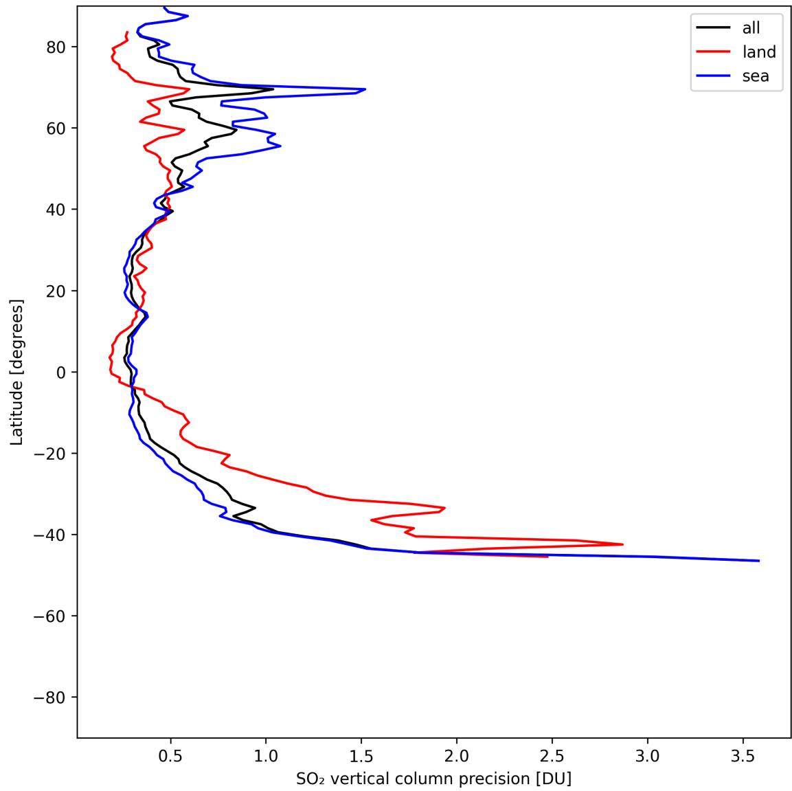
Figure 32: Zonal average of “SO 2 vertical column precision” for 2025-07-03 to 2025-07-04.
