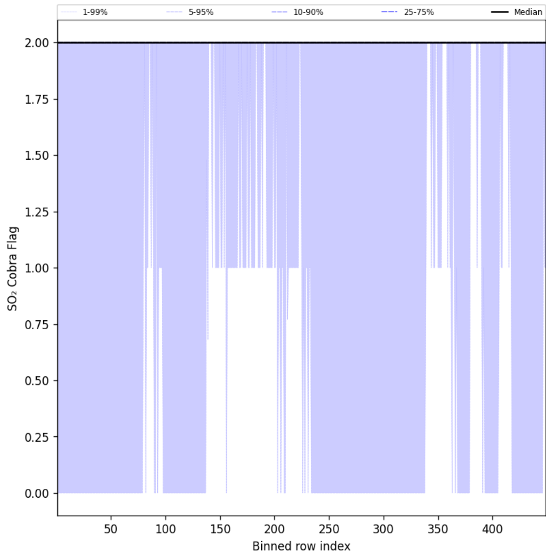
Figure 102: Along track statistics of “SO 2 Cobra Flag” for 2025-07-03 to 2025-07-04
