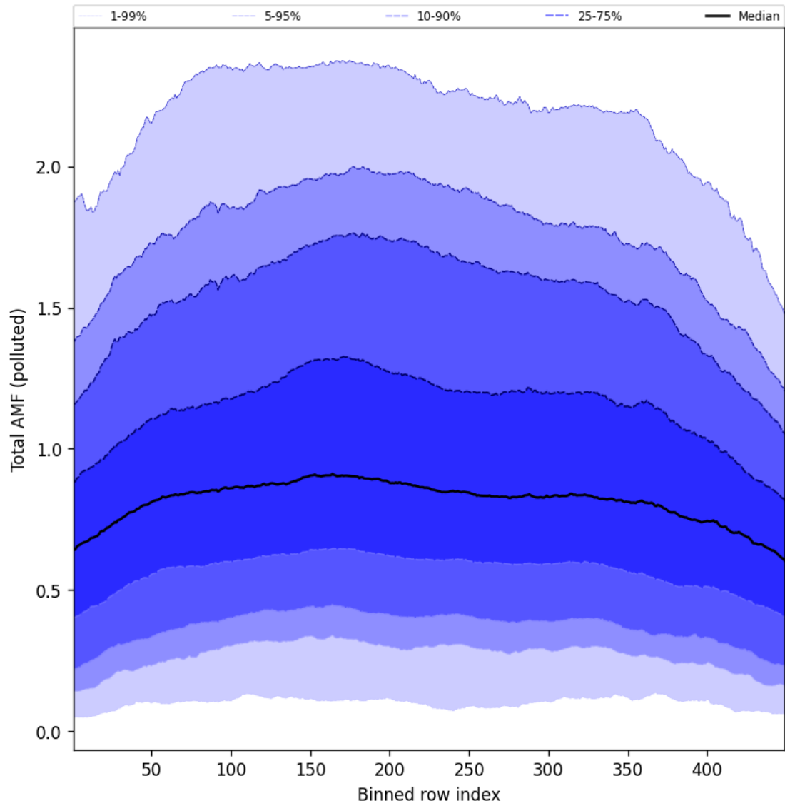
Figure 107: Along track statistics of “Total AMF (polluted)” for 2025-07-03 to 2025-07-04
