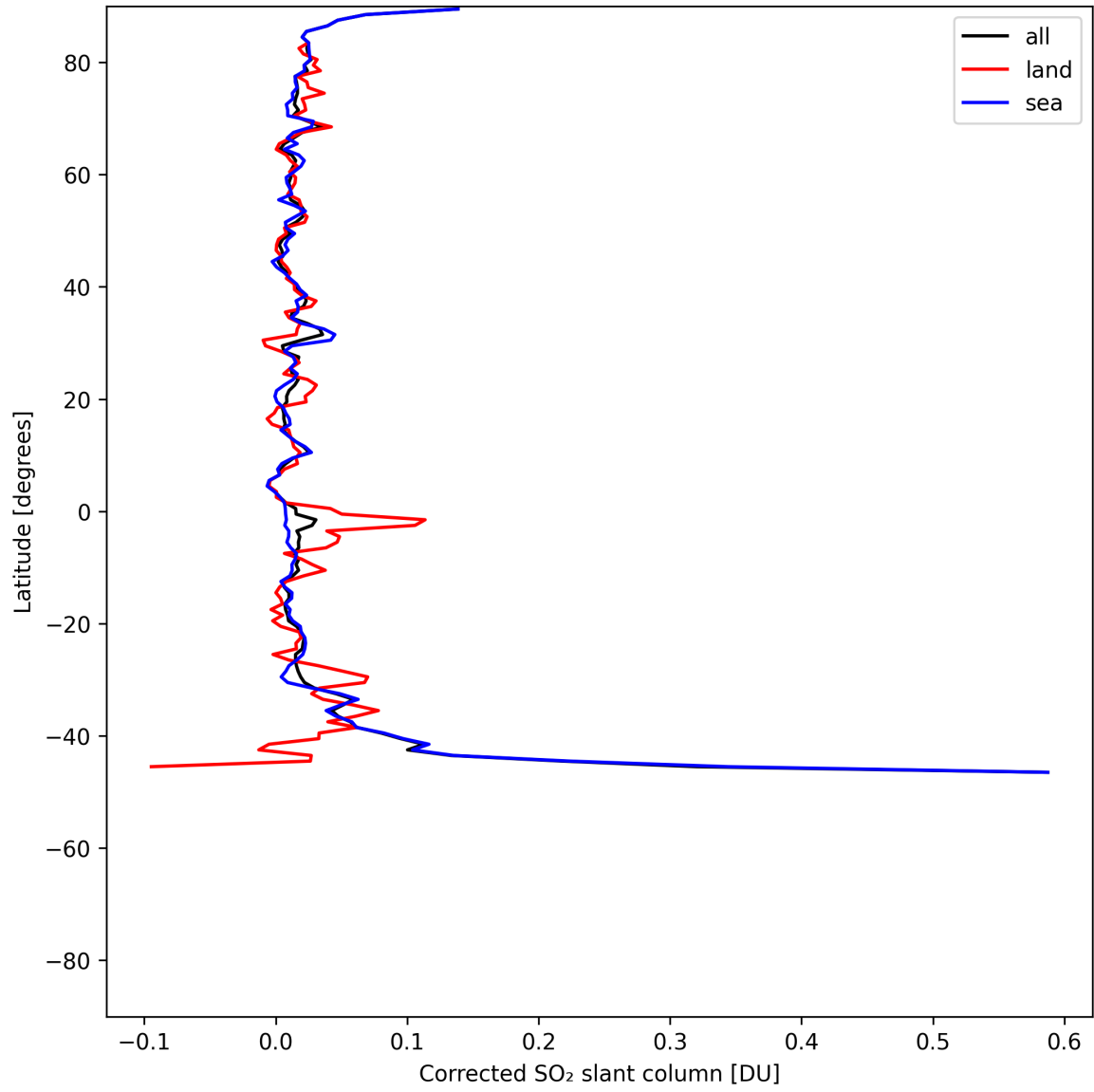
Figure 33: Zonal average of “Corrected SO 2 slant column” for 2025-07-03 to 2025-07-04.
