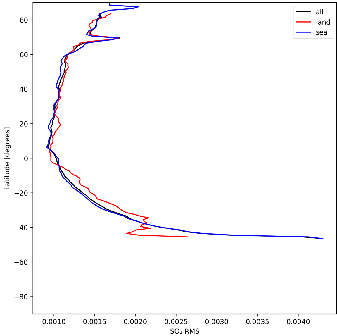
Figure 52: Zonal average of “SO 2 RMS” for 2025-07-03 to 2025-07-04.
