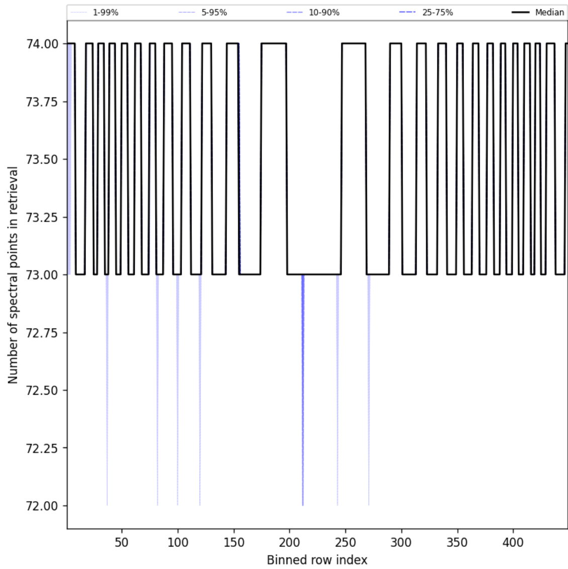
Figure 110: Along track statistics of “Number of spectral points in retrieval” for 2025-07-03 to 2025-07-04
