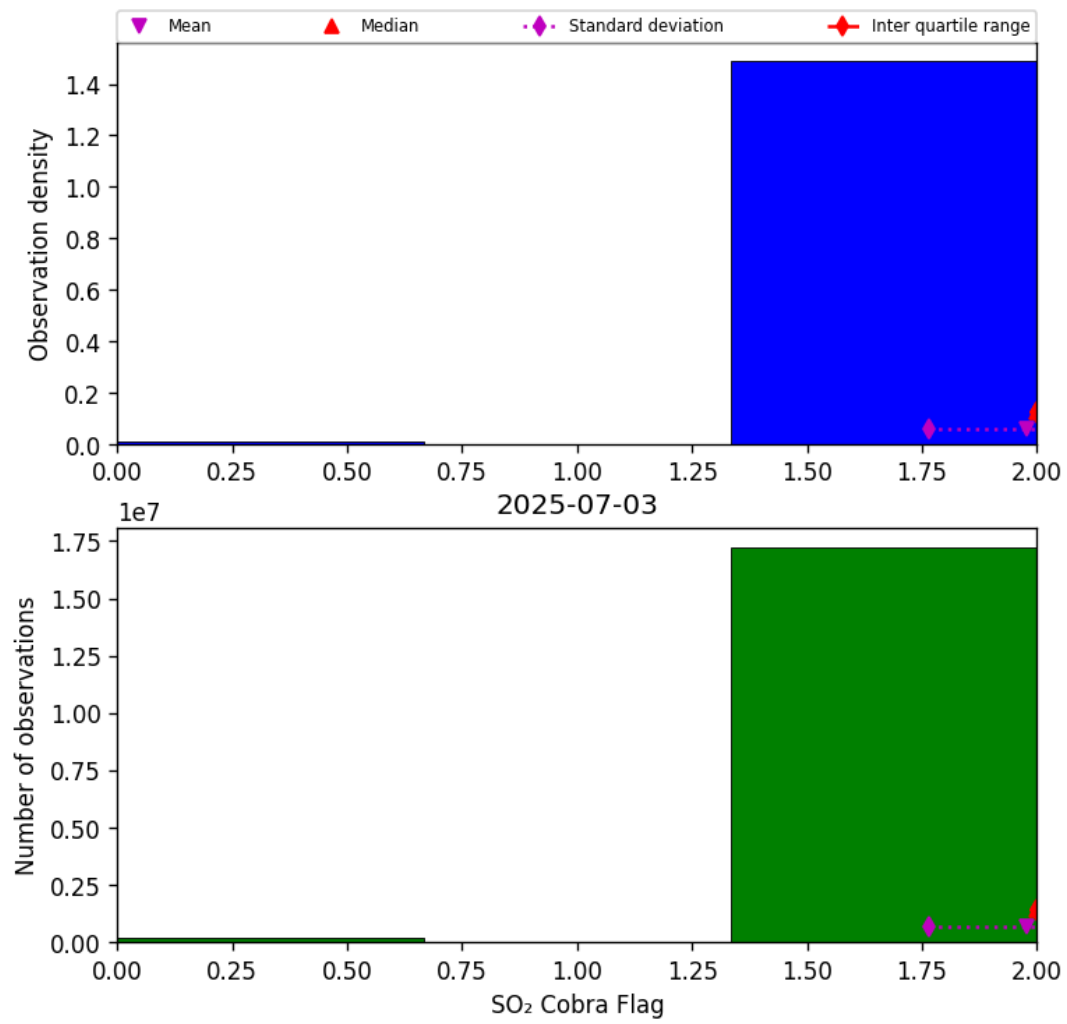
Figure 75: Histogram of “SO 2 Cobra Flag” for 2025-07-03 to 2025-07-04
