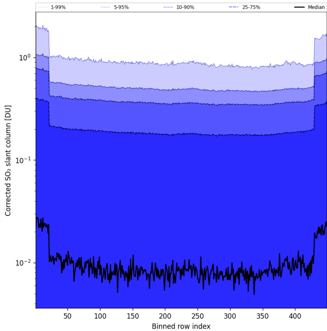
Figure 87: Along track statistics of "Corrected SO 2 slant column" for 2025-07-03 to 2025-07-04
