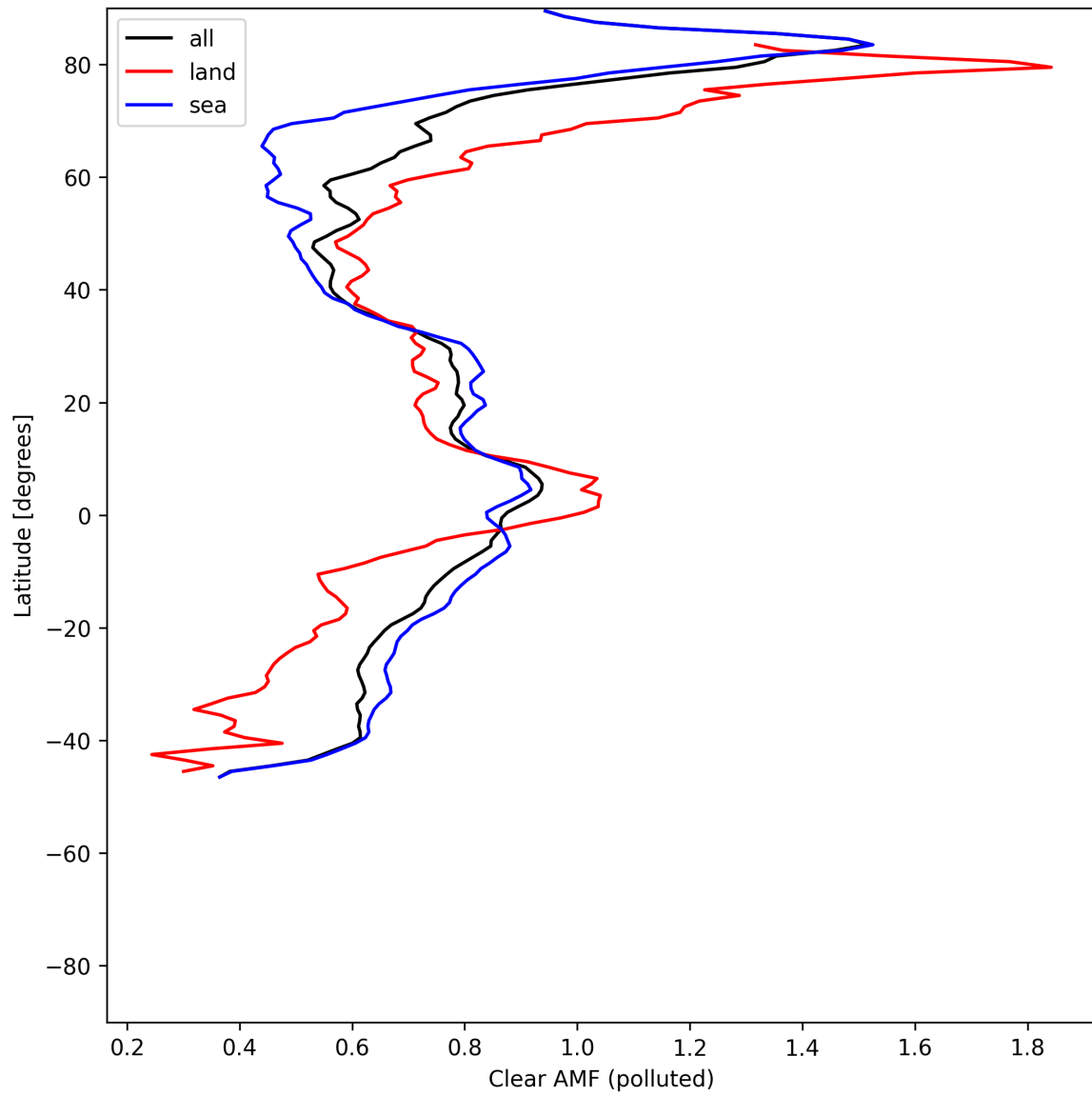
Figure 55: Zonal average of “Clear AMF (polluted)” for 2025-07-03 to 2025-07-04.
