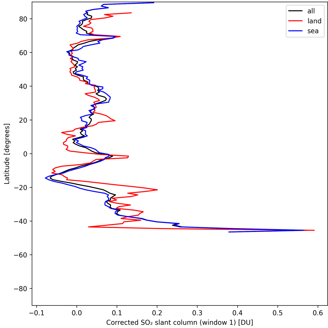
Figure 38: Zonal average of “Corrected SO 2 slant column (window 1)” for 2025-07-03 to 2025-07-04.
