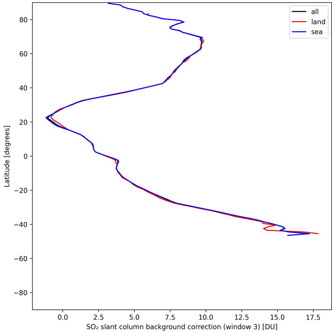
Figure 47: Zonal average of “SO 2 slant column background correction (window 3)” for 2025-07-03 to 2025-07-04.
