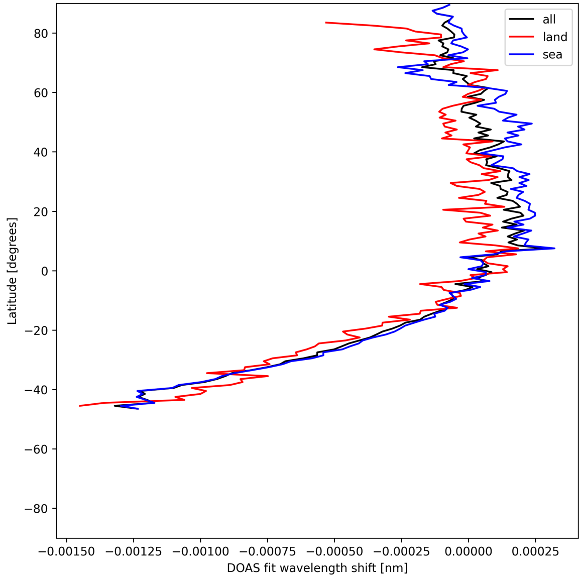
Figure 50: Zonal average of “DOAS fit wavelength shift” for 2025-07-03 to 2025-07-04.
