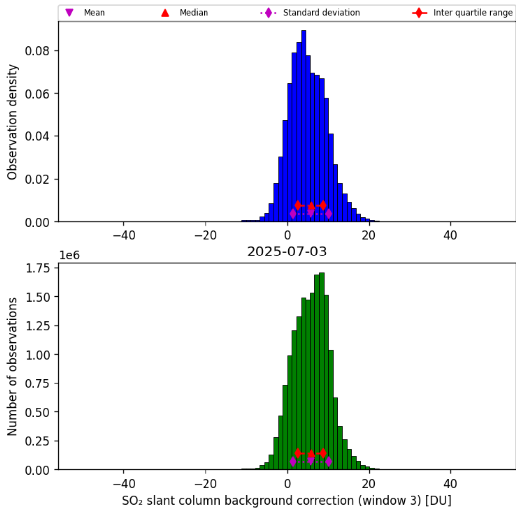
Figure 74: Histogram of “SO 2 slant column background correction (window 3)” for 2025-07-03 to 2025-07-04
