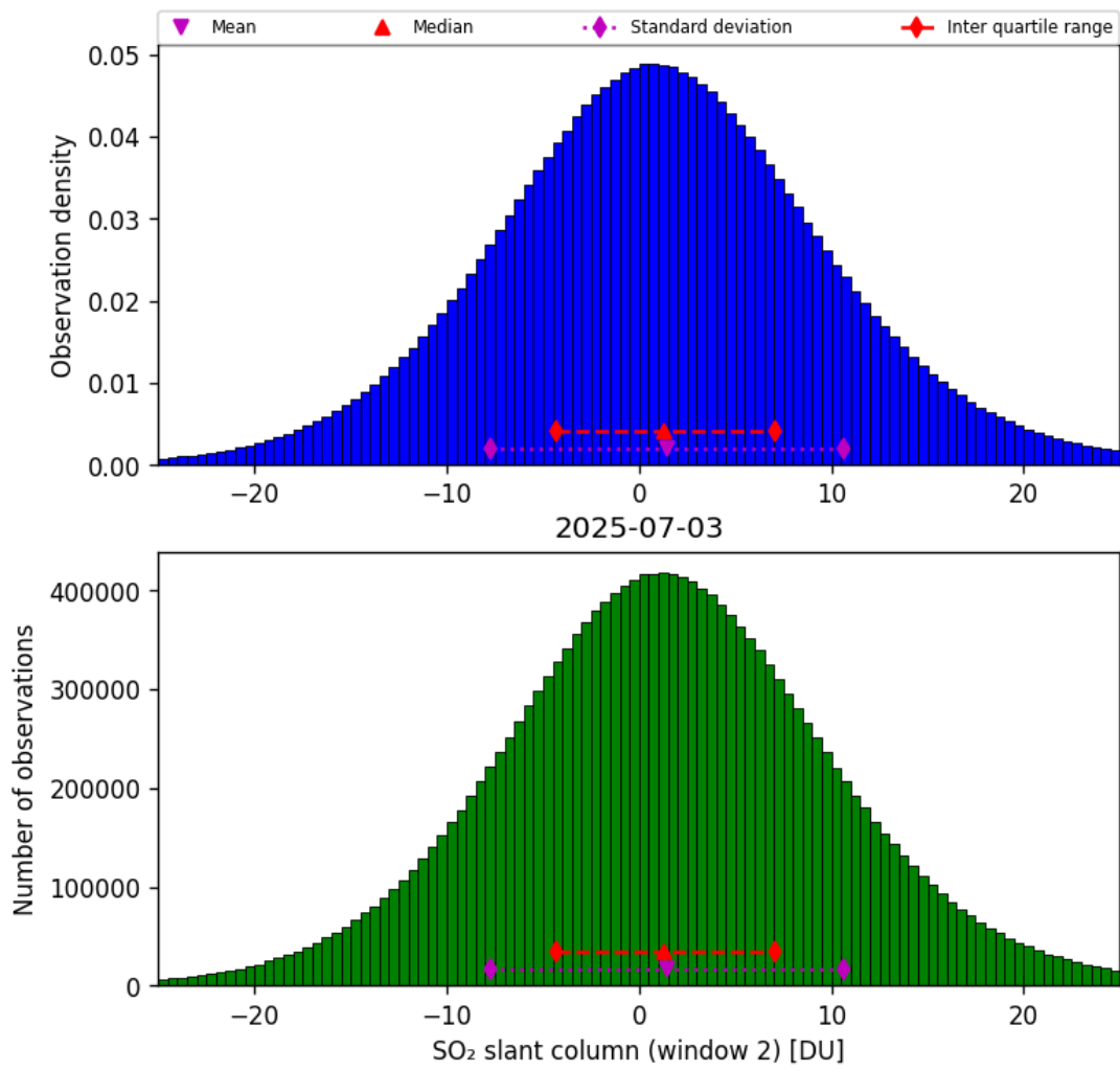
Figure 67: Histogram of “SO 2 slant column (window 2)” for 2025-07-03 to 2025-07-04
