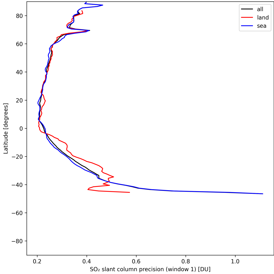
Figure 37: Zonal average of “SO 2 slant column precision (window 1)” for 2025-07-03 to 2025-07-04.
