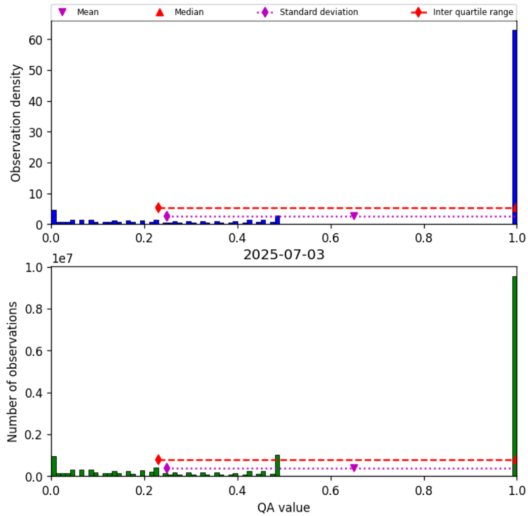
Figure 57: Histogram of “QA value” for 2025-07-03 to 2025-07-04
