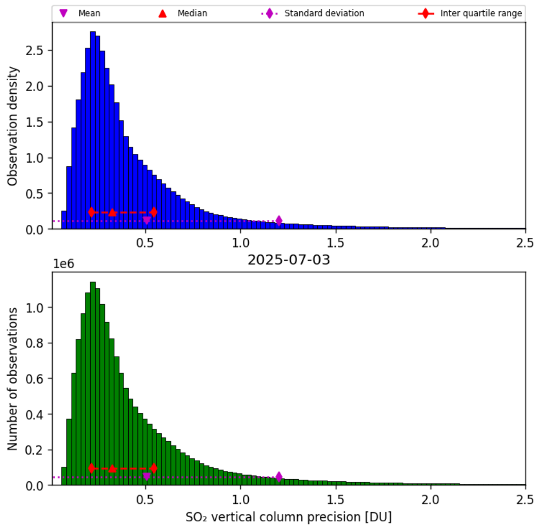
Figure 59: Histogram of “SO 2 vertical column precision” for 2025-07-03 to 2025-07-04
