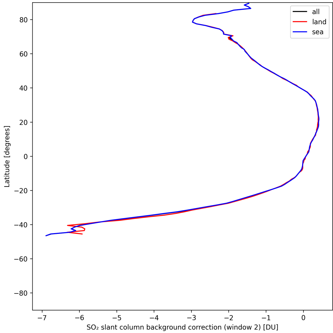
Figure 43: Zonal average of “SO 2 slant column background correction (window 2)” for 2025-07-03 to 2025-07-04.
