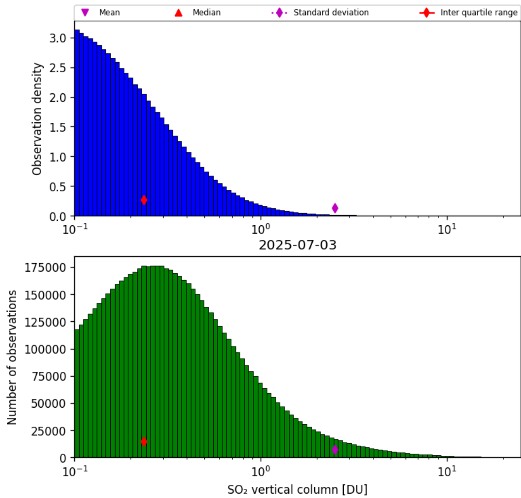
Figure 58: Histogram of “SO 2 vertical column” for 2025-07-03 to 2025-07-04
