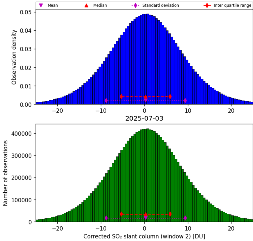
Figure 69: Histogram of “Corrected SO 2 slant column (window 2)” for 2025-07-03 to 2025-07-04
