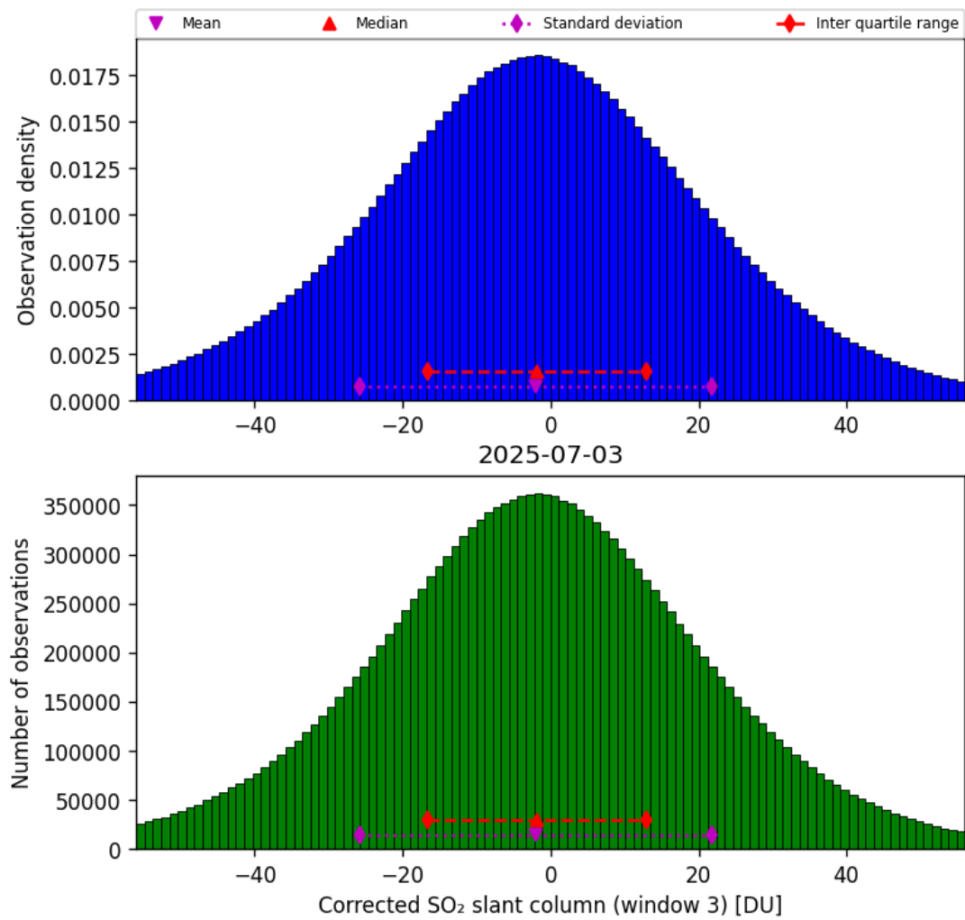
Figure 73: Histogram of “Corrected SO 2 slant column (window 3)” for 2025-07-03 to 2025-07-04
