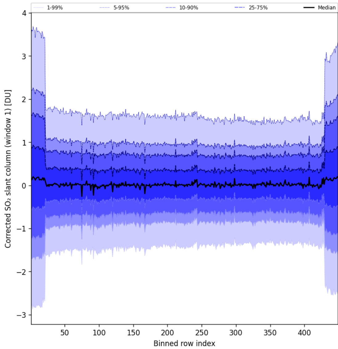
Figure 92: Along track statistics of “Corrected SO 2 slant column (window 1)” for 2025-07-03 to 2025-07-04
