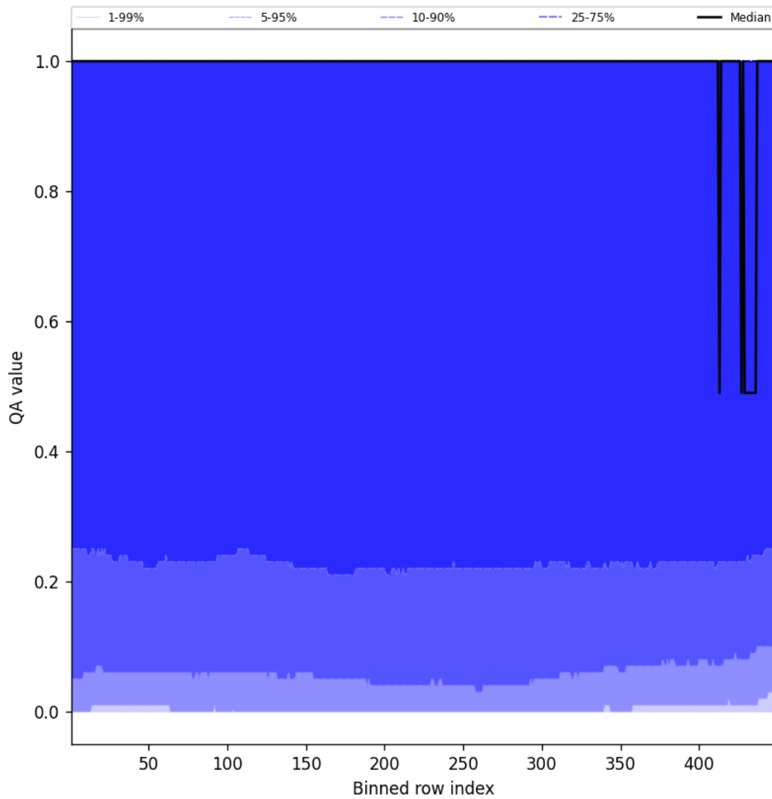
Figure 84: Along track statistics of "QA value" for 2025-07-03 to 2025-07-04
