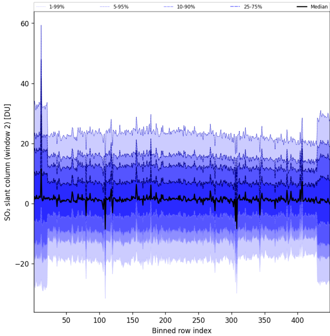
Figure 94: Along track statistics of “SO 2 slant column (window 2)” for 2025-07-03 to 2025-07-04
