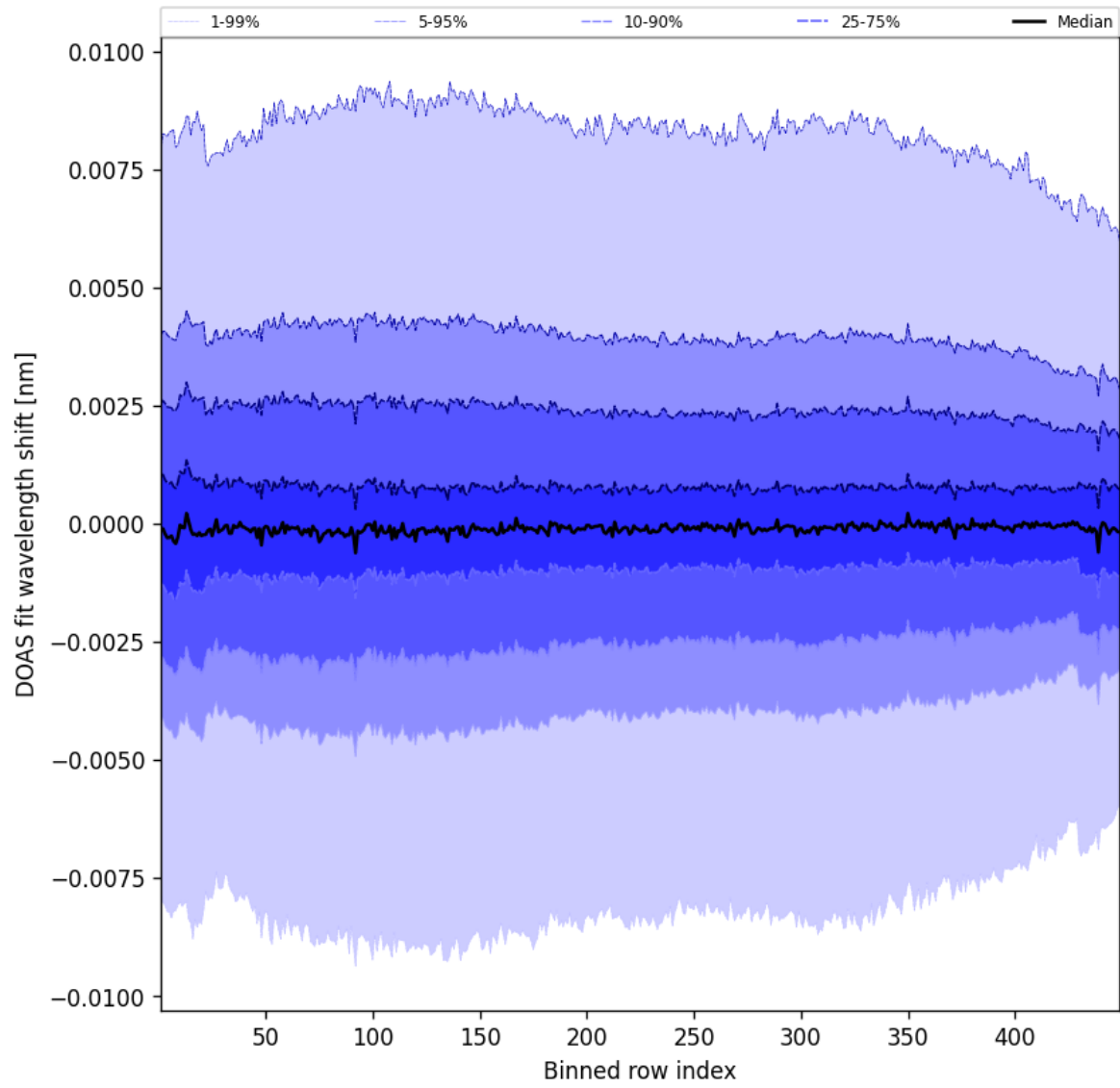
Figure 104: Along track statistics of “DOAS fit wavelength shift” for 2025-07-03 to 2025-07-04
