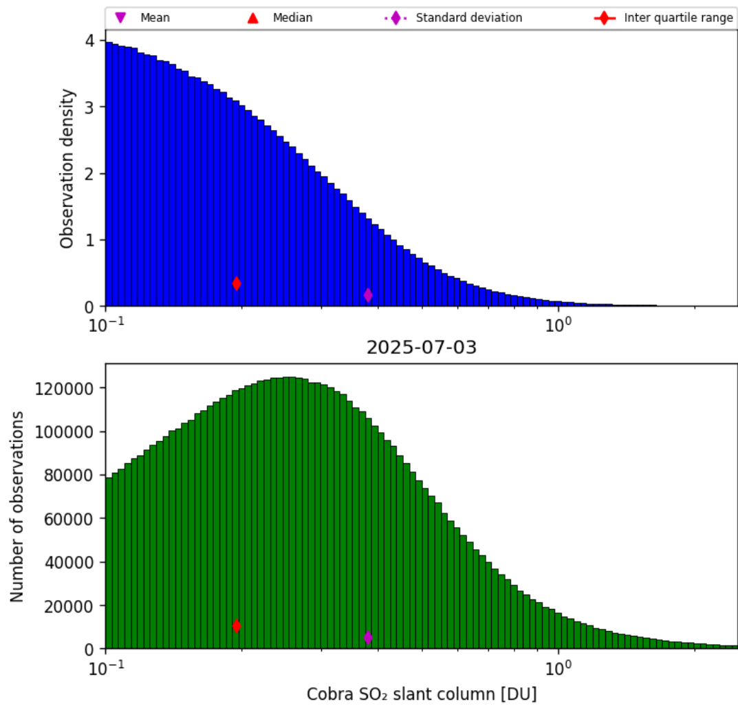
Figure 61: Histogram of “Cobra SO 2 slant column” for 2025-07-03 to 2025-07-04
