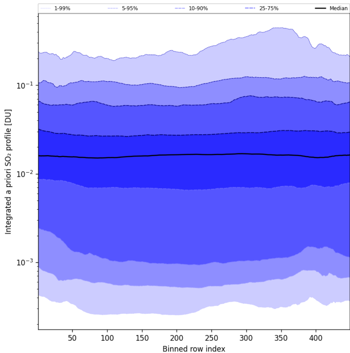
Figure 103: Along track statistics of “Integrated a priori SO 2 profile” for 2025-07-03 to 2025-07-04
