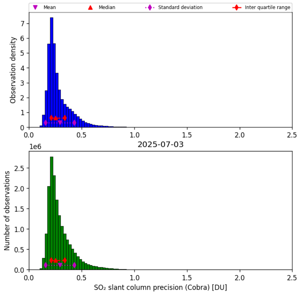
Figure 62: Histogram of “SO 2 slant column precision (Cobra)” for 2025-07-03 to 2025-07-04
