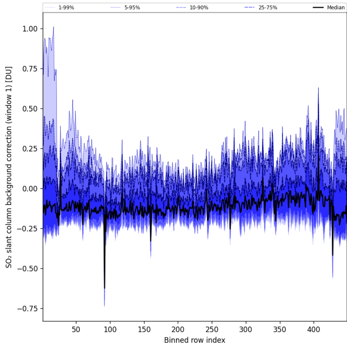
Figure 93: Along track statistics of “SO 2 slant column background correction (window 1)” for 2025-07-03 to 2025-07-04
