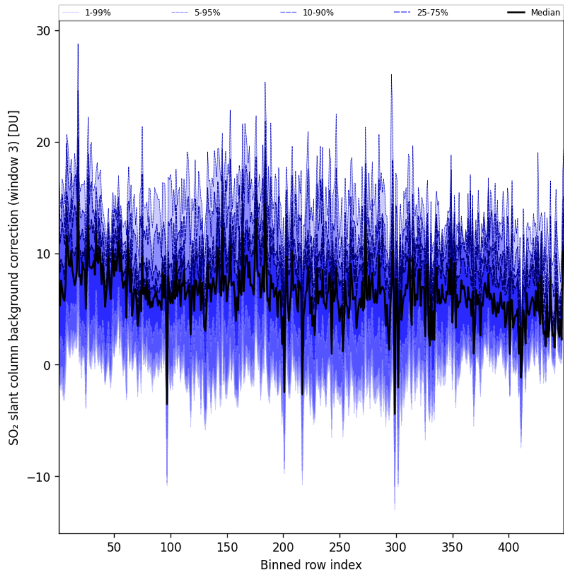
Figure 101: Along track statistics of “SO 2 slant column background correction (window 3)” for 2025-07-03 to 2025-07-04
