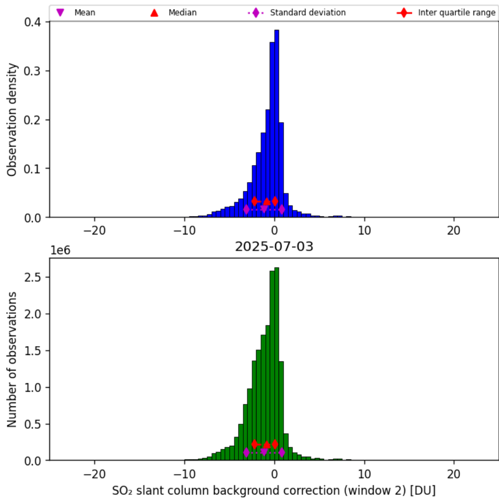
Figure 70: Histogram of “SO 2 slant column background correction (window 2)” for 2025-07-03 to 2025-07-04
