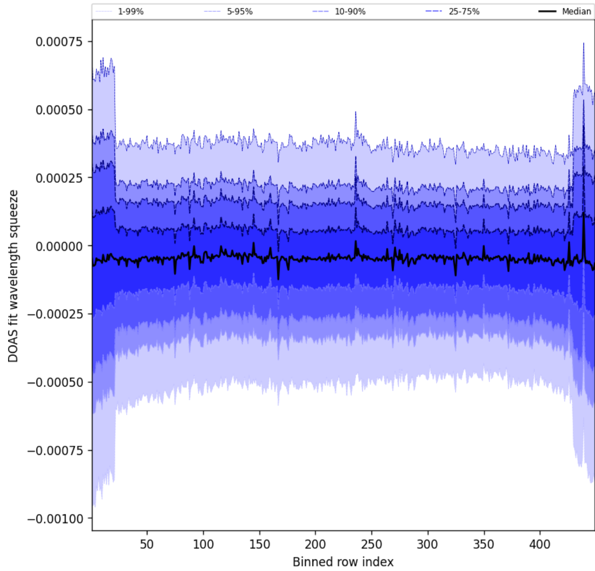
Figure 105: Along track statistics of “DOAS fit wavelength squeeze” for 2025-07-03 to 2025-07-04
