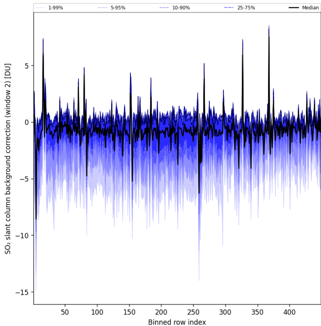
Figure 97: Along track statistics of “SO 2 slant column background correction (window 2)” for 2025-07-03 to 2025-07-04
