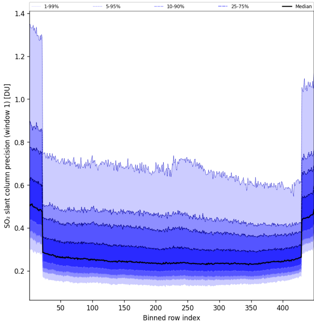
Figure 91: Along track statistics of “SO 2 slant column precision (window 1)” for 2025-07-03 to 2025-07-04
