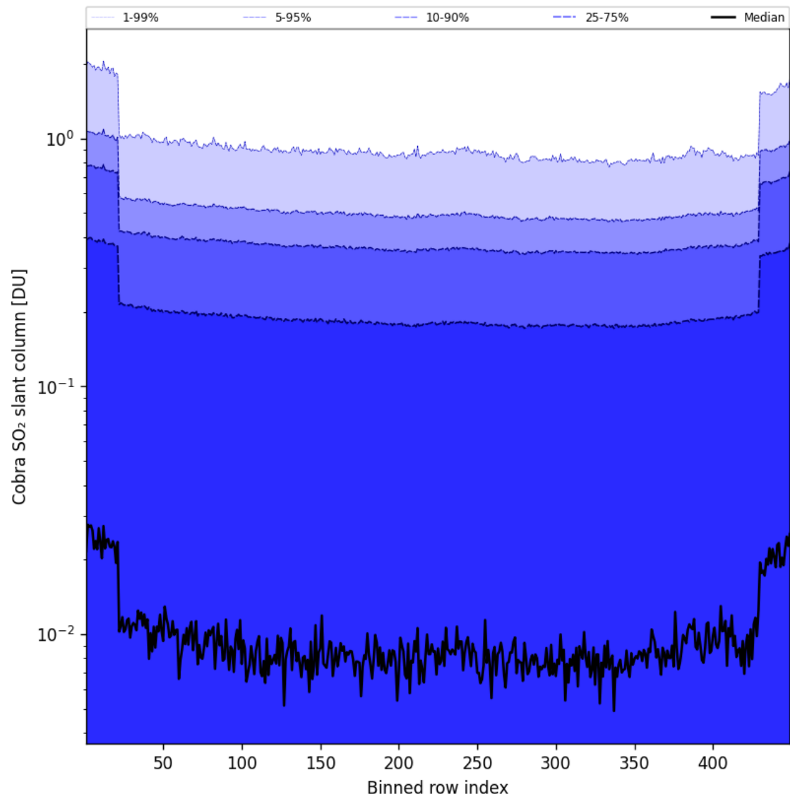
Figure 88: Along track statistics of “Cobra SO 2 slant column” for 2025-07-03 to 2025-07-04
