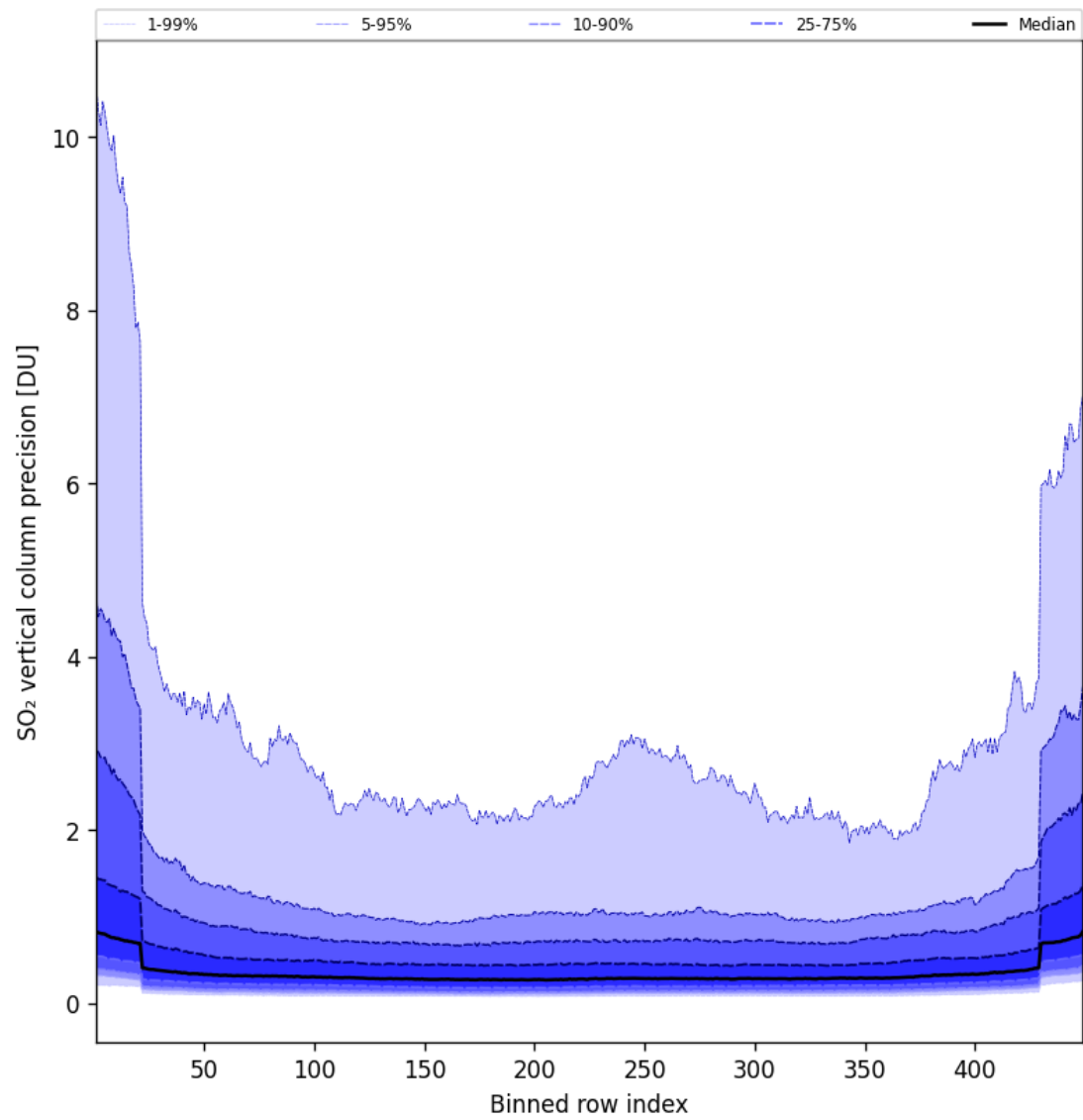
Figure 86: Along track statistics of “SO 2 vertical column precision” for 2025-07-03 to 2025-07-04
