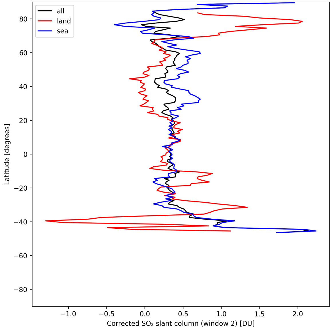
Figure 42: Zonal average of “Corrected SO 2 slant column (window 2)” for 2025-07-03 to 2025-07-04.
