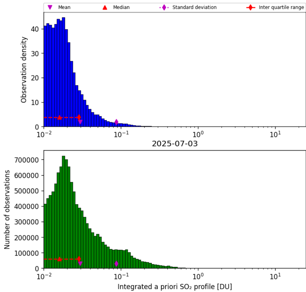
Figure 76: Histogram of “Integrated a priori SO 2 profile” for 2025-07-03 to 2025-07-04
