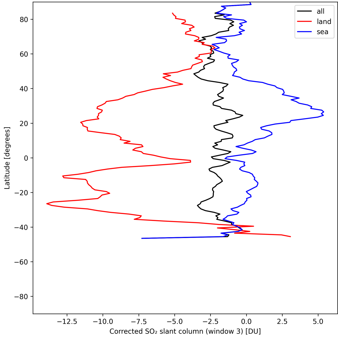
Figure 46: Zonal average of “Corrected SO 2 slant column (window 3)” for 2025-07-03 to 2025-07-04.
