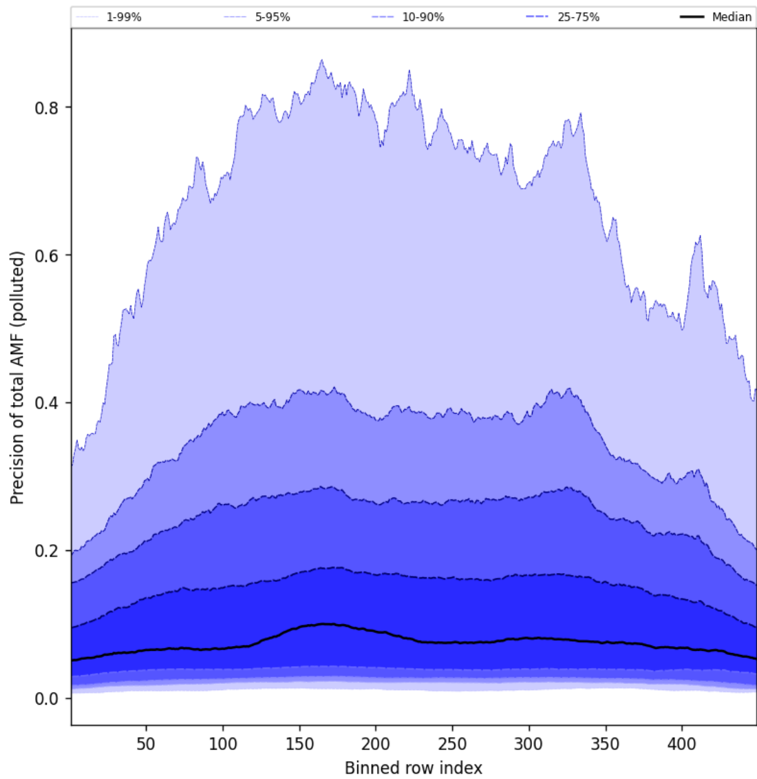
Figure 108: Along track statistics of “Precision of total AMF (polluted)” for 2025-07-03 to 2025-07-04
