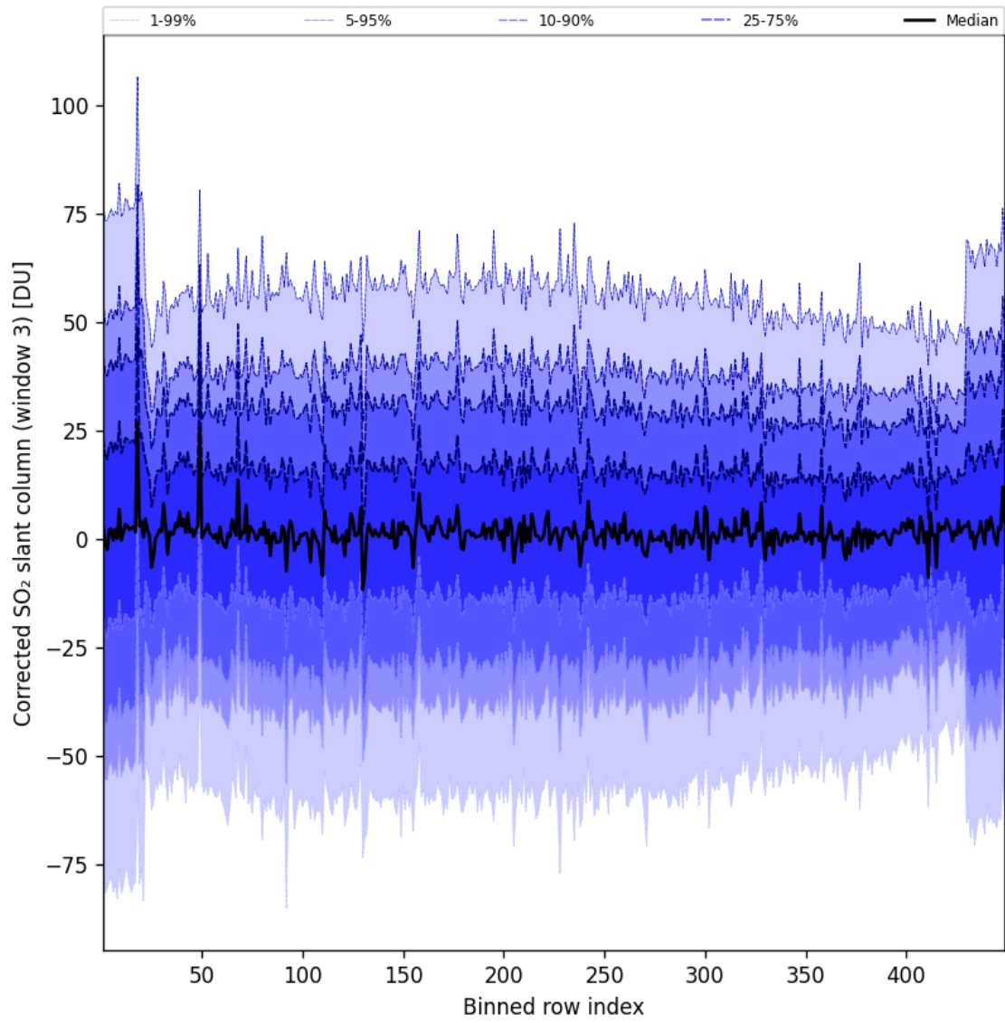
Figure 100: Along track statistics of “Corrected SO 2 slant column (window 3)” for 2025-07-06 to 2025-07-06
