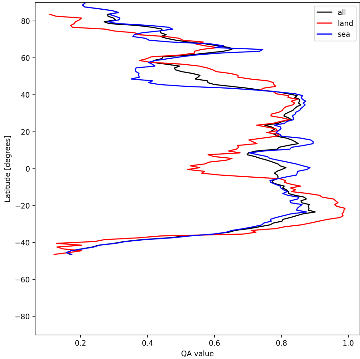
Figure 30: Zonal average of “QA value” for 2025-07-06 to 2025-07-06.
