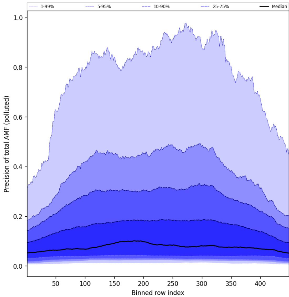
Figure 108: Along track statistics of “Precision of total AMF (polluted)” for 2025-07-06 to 2025-07-06
