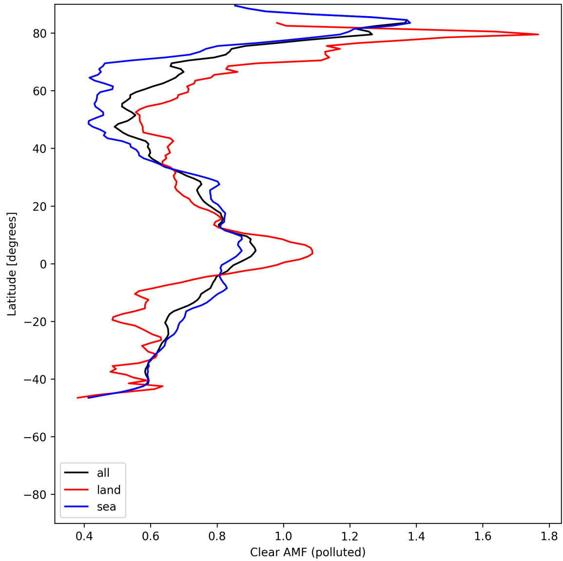
Figure 55: Zonal average of “Clear AMF (polluted)” for 2025-07-06 to 2025-07-06.
