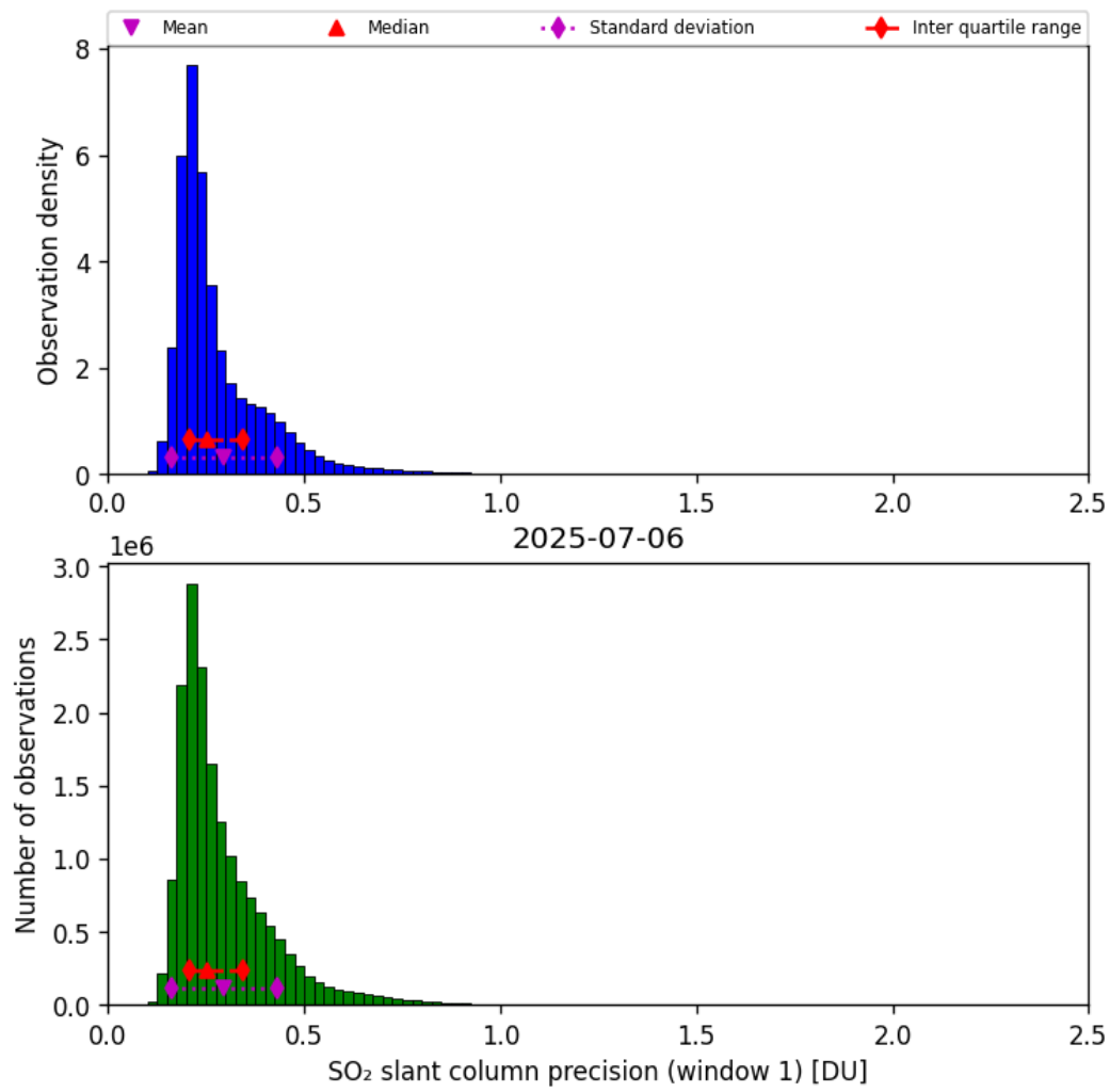
Figure 64: Histogram of “SO 2 slant column precision (window 1)” for 2025-07-06 to 2025-07-06
