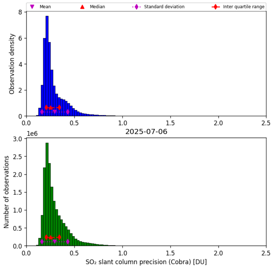
Figure 62: Histogram of “SO 2 slant column precision (Cobra)” for 2025-07-06 to 2025-07-06
