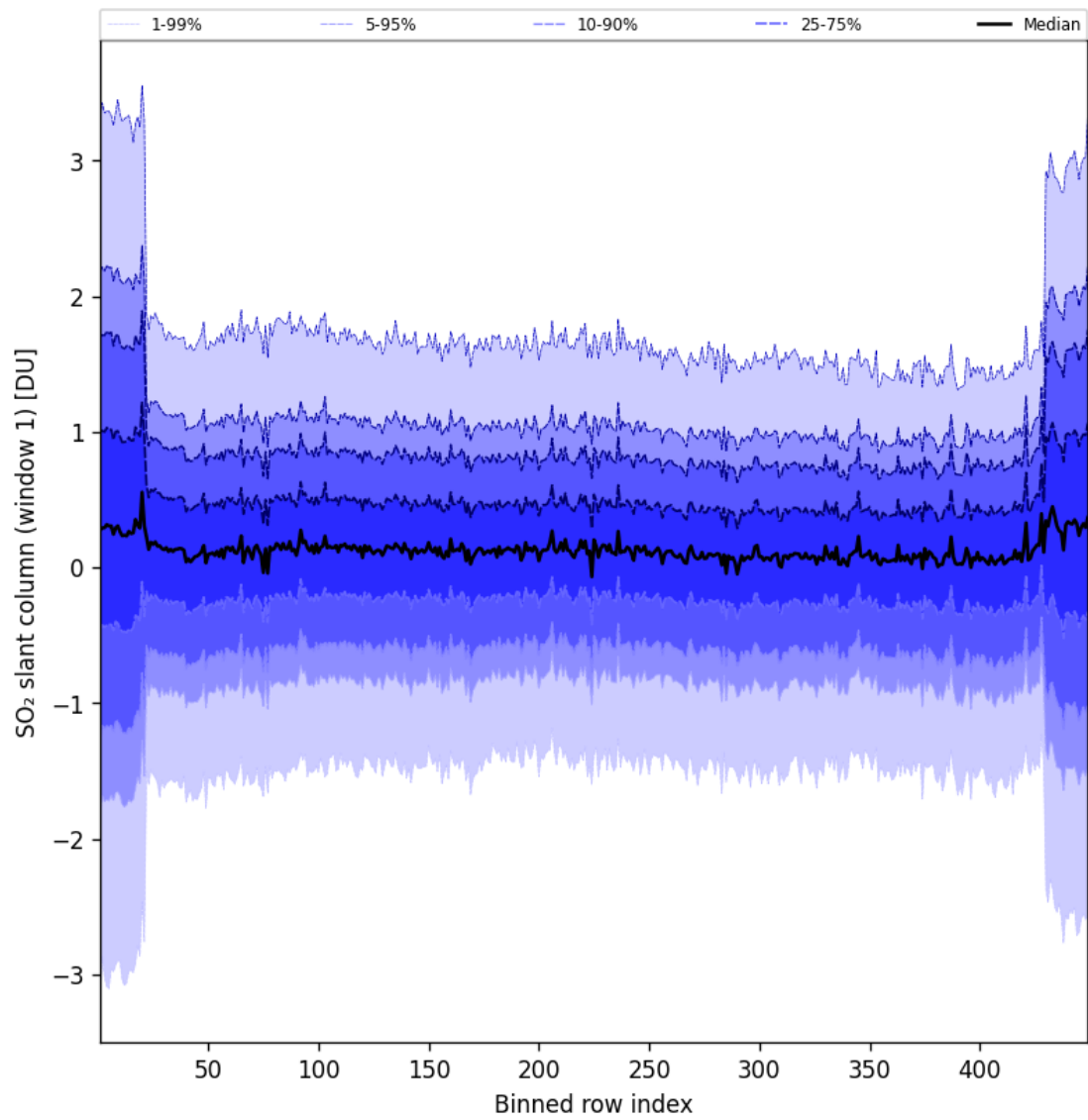
Figure 90: Along track statistics of “SO 2 slant column (window 1)” for 2025-07-06 to 2025-07-06
