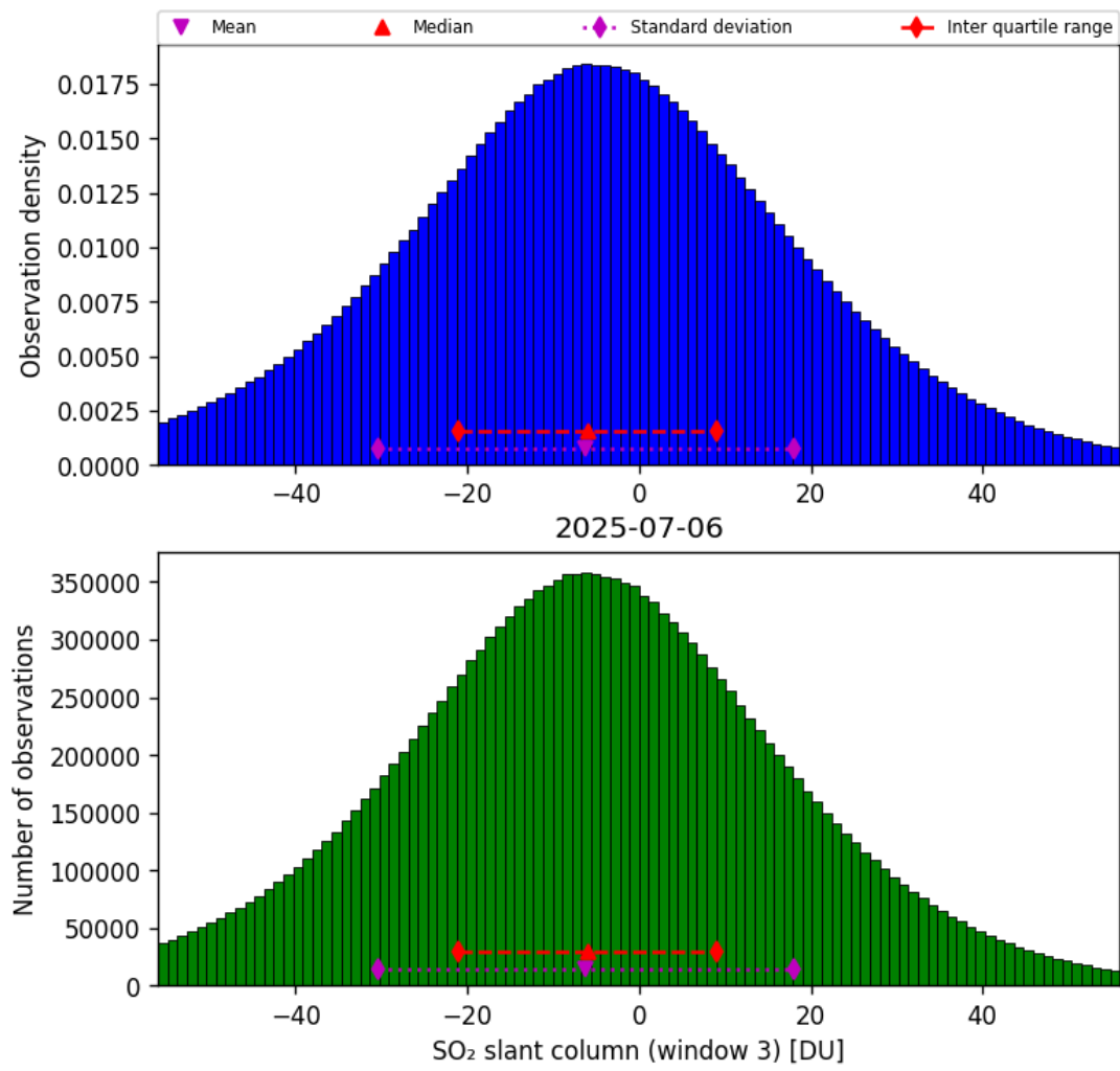
Figure 71: Histogram of “SO 2 slant column (window 3)” for 2025-07-06 to 2025-07-06
