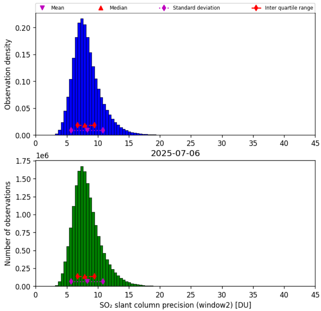
Figure 68: Histogram of “SO 2 slant column precision (window2)” for 2025-07-06 to 2025-07-06
