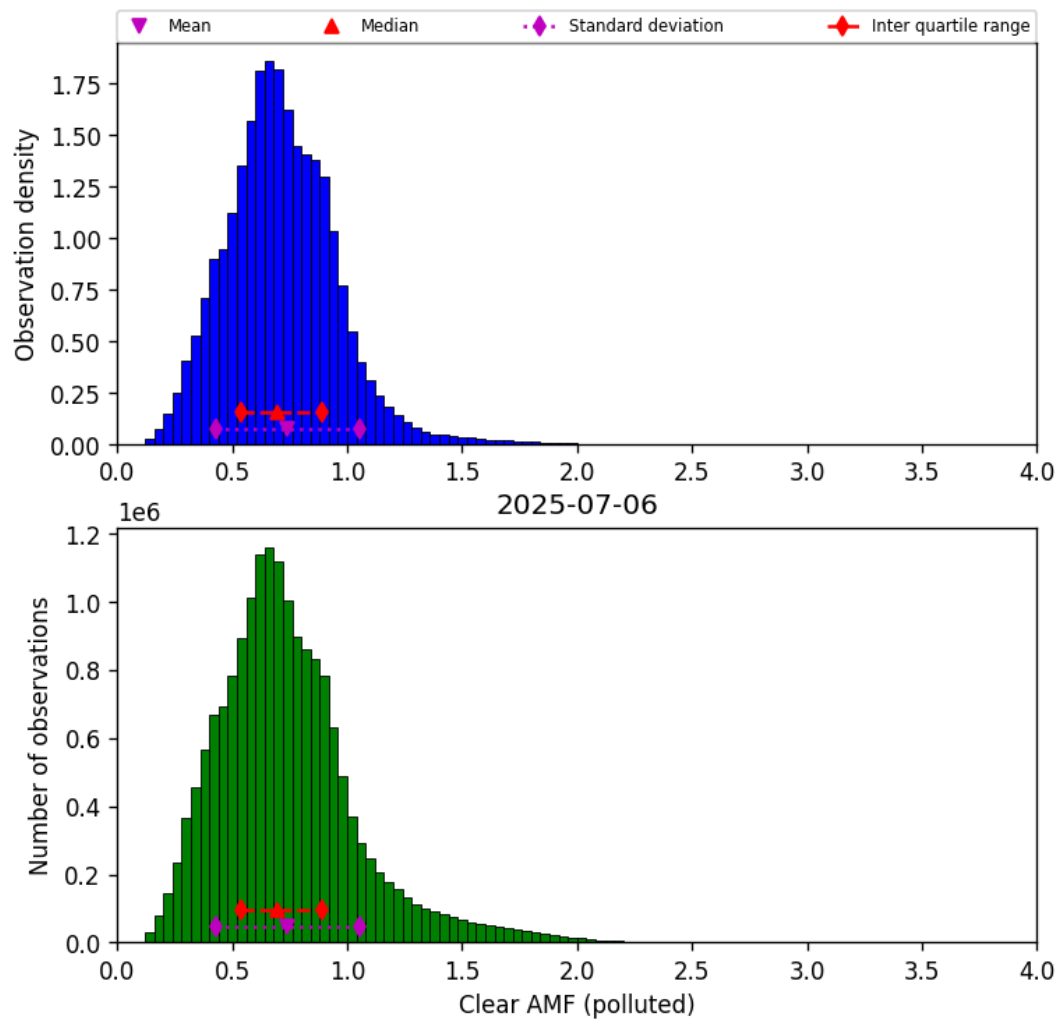
Figure 82: Histogram of “Clear AMF (polluted)” for 2025-07-06 to 2025-07-06
