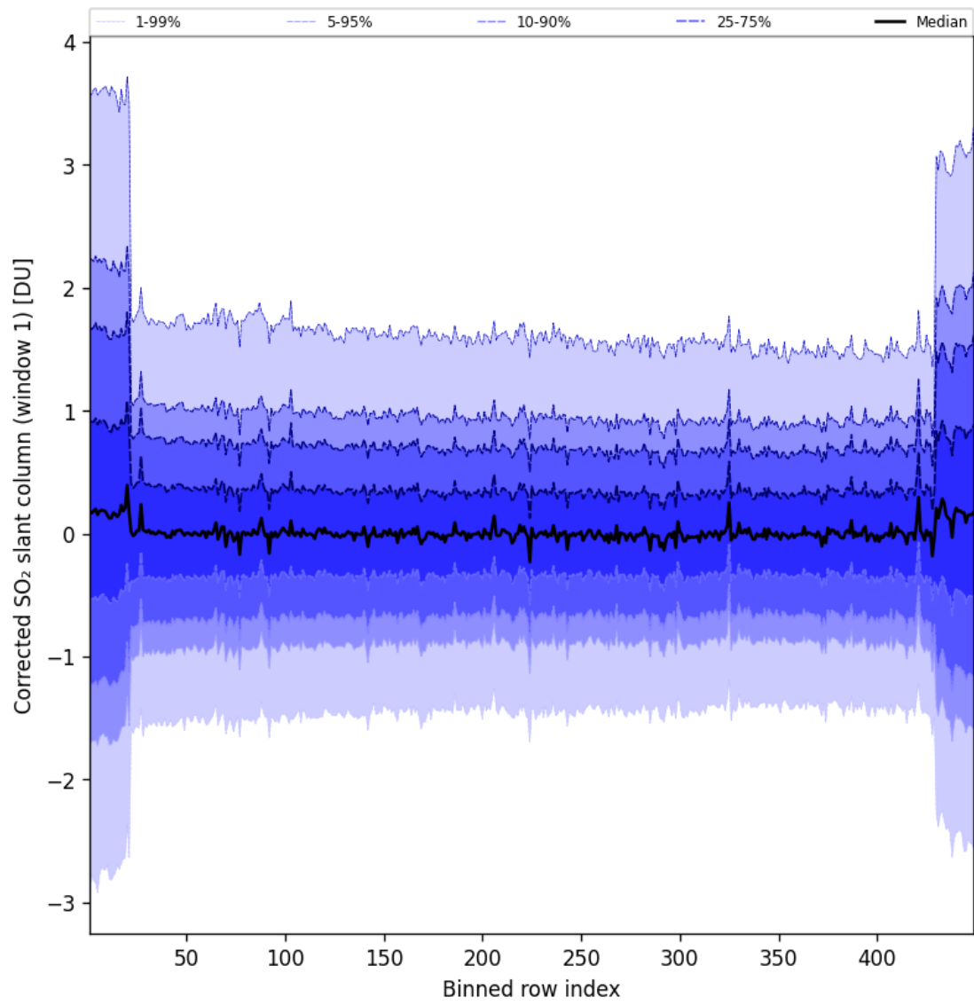
Figure 92: Along track statistics of “Corrected SO 2 slant column (window 1)” for 2025-07-06 to 2025-07-06
