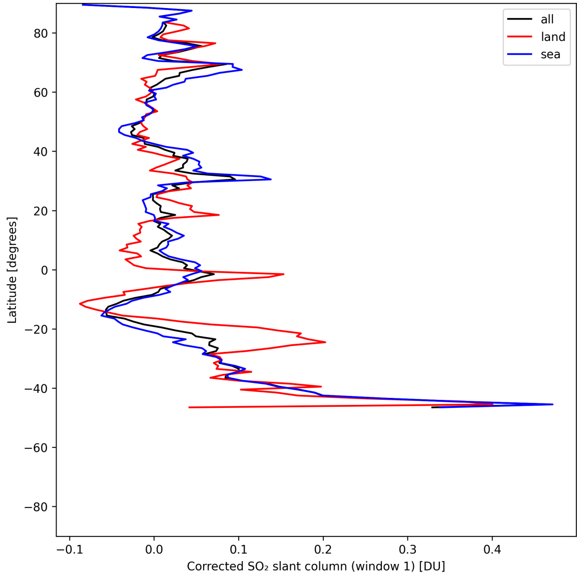
Figure 38: Zonal average of “Corrected SO 2 slant column (window 1)” for 2025-07-06 to 2025-07-06.
