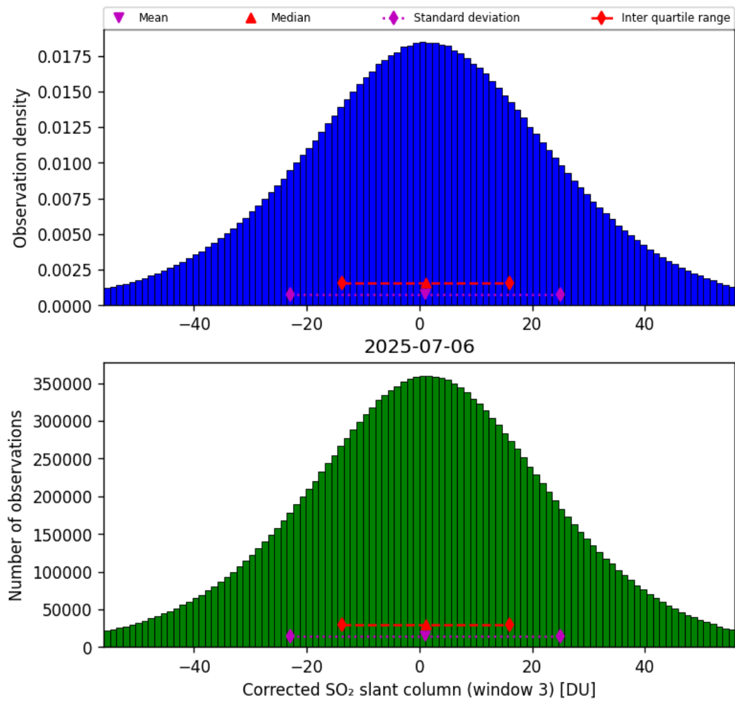
Figure 73: Histogram of “Corrected SO 2 slant column (window 3)” for 2025-07-06 to 2025-07-06
