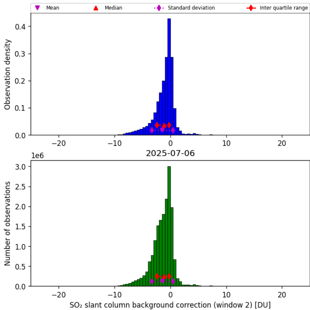
Figure 70: Histogram of “SO 2 slant column background correction (window 2)” for 2025-07-06 to 2025-07-06
