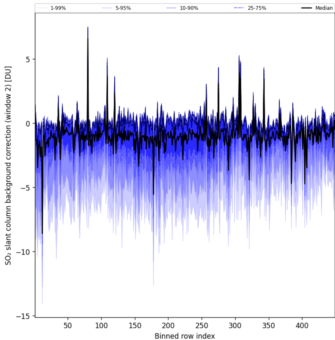
Figure 97: Along track statistics of “SO 2 slant column background correction (window 2)” for 2025-07-06 to 2025-07-06
