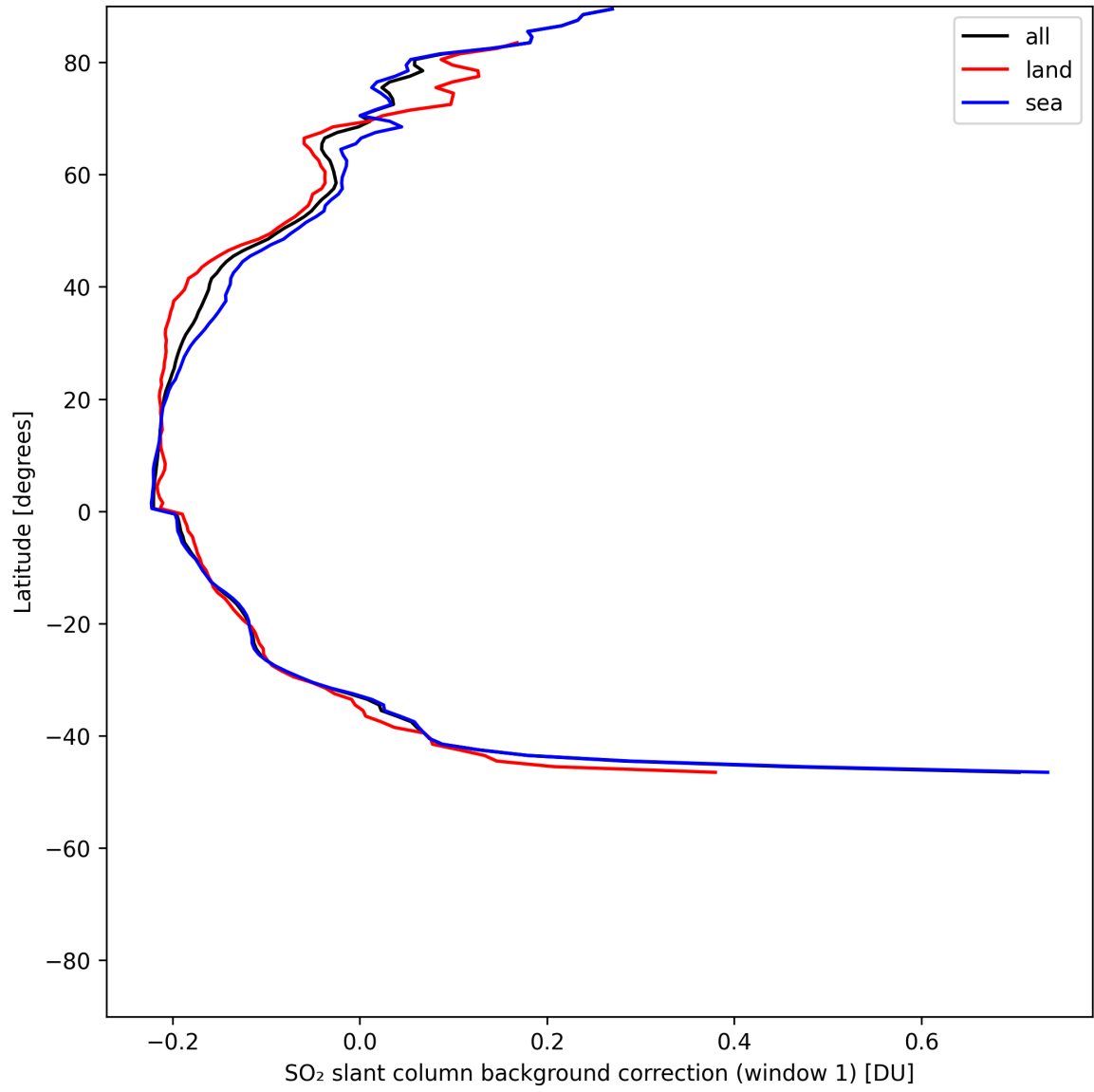
Figure 39: Zonal average of “SO 2 slant column background correction (window 1)” for 2025-07-06 to 2025-07-06.
