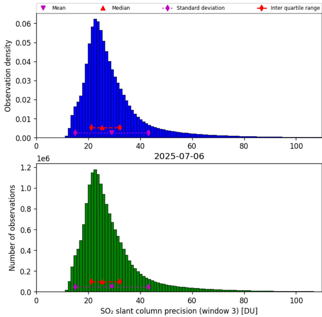
Figure 72: Histogram of “SO 2 slant column precision (window 3)” for 2025-07-06 to 2025-07-06
