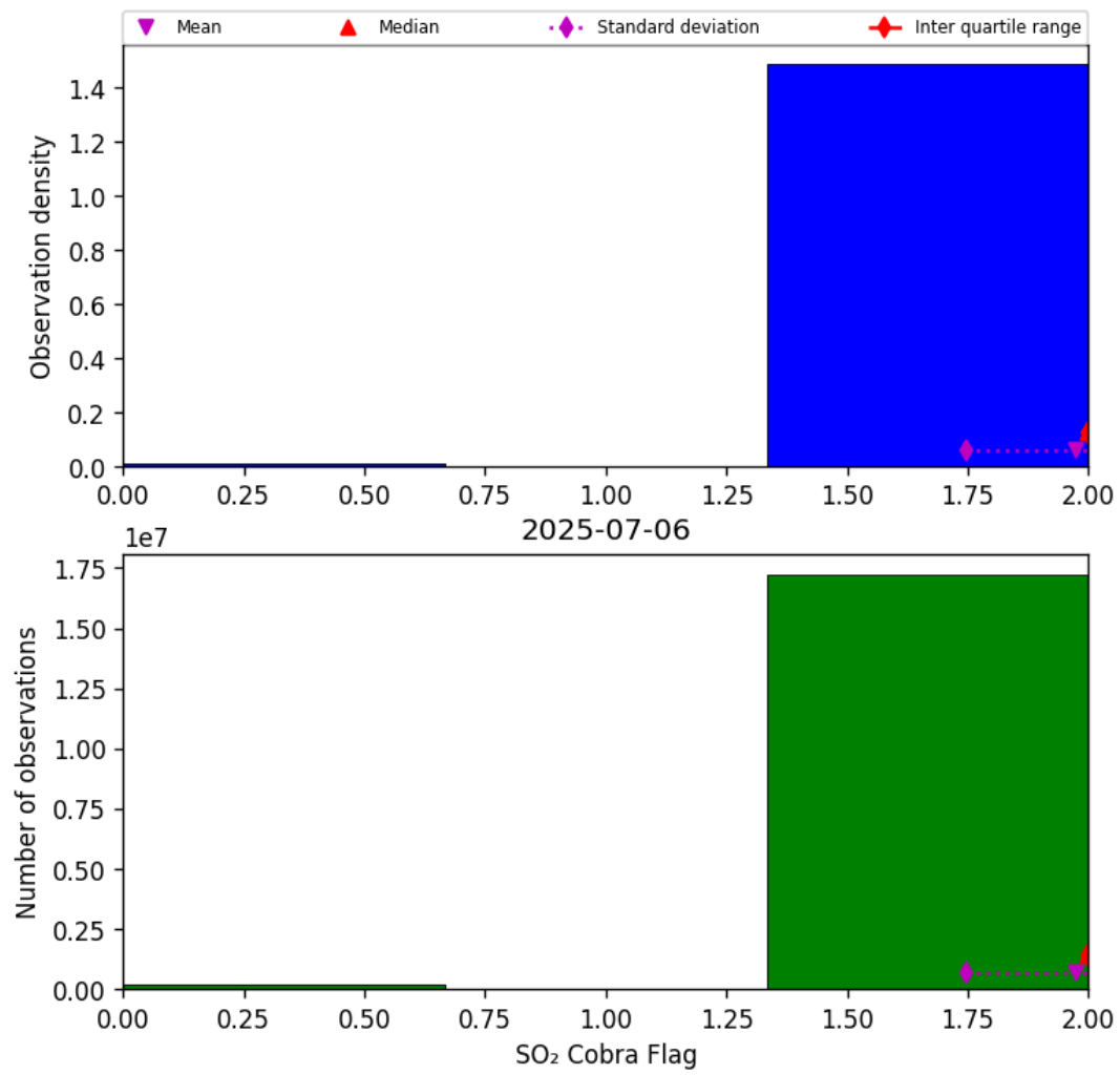
Figure 75: Histogram of “SO 2 Cobra Flag” for 2025-07-06 to 2025-07-06
