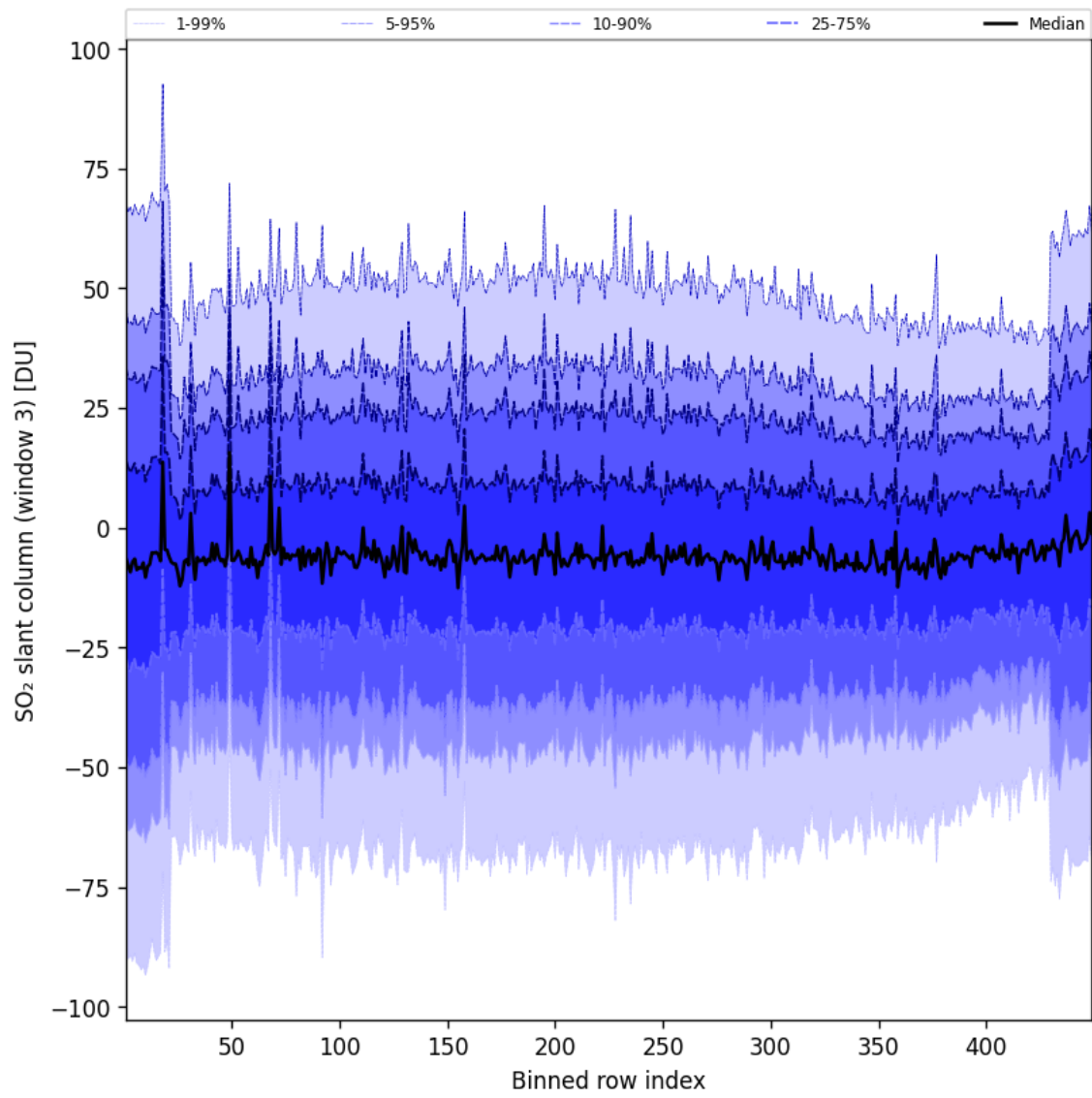
Figure 98: Along track statistics of “SO 2 slant column (window 3)” for 2025-07-06 to 2025-07-06
