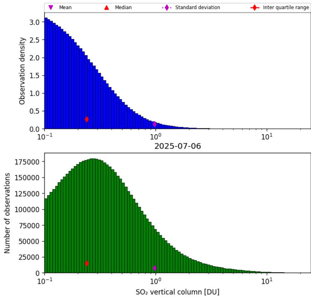
Figure 58: Histogram of “SO 2 vertical column” for 2025-07-06 to 2025-07-06
