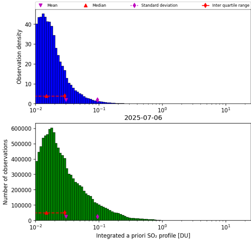
Figure 76: Histogram of “Integrated a priori SO 2 profile” for 2025-07-06 to 2025-07-06
