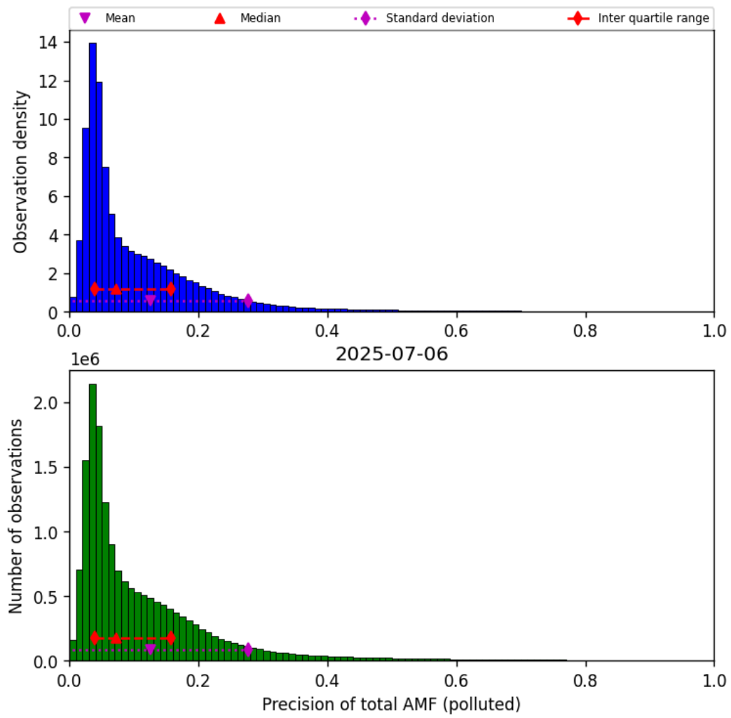
Figure 81: Histogram of “Precision of total AMF (polluted)” for 2025-07-06 to 2025-07-06
