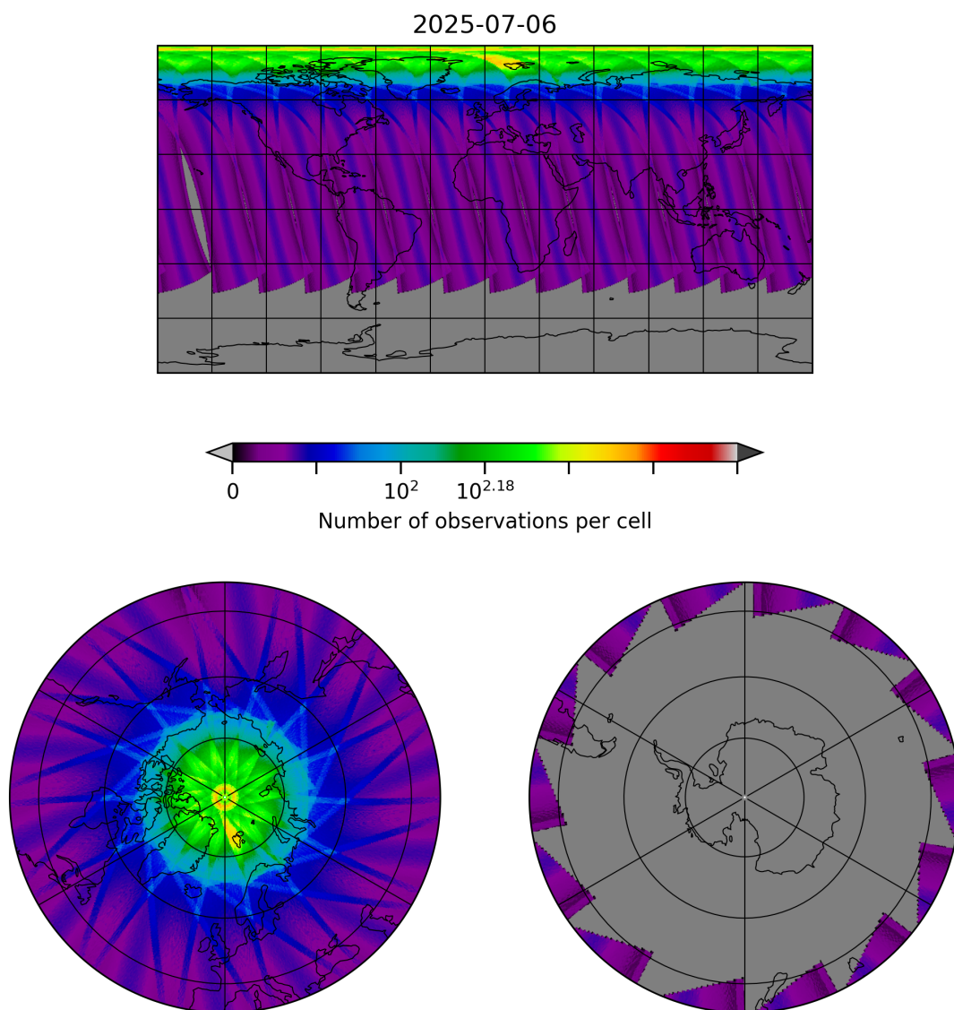
Figure 29: Map of the number of observations for 2025-07-06 to 2025-07-06
