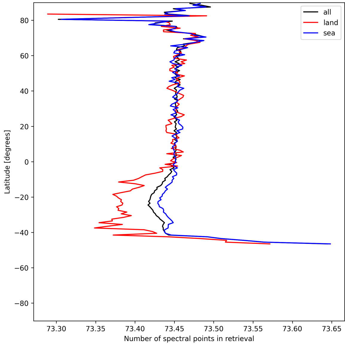
Figure 56: Zonal average of “Number of spectral points in retrieval” for 2025-07-06 to 2025-07-06.
