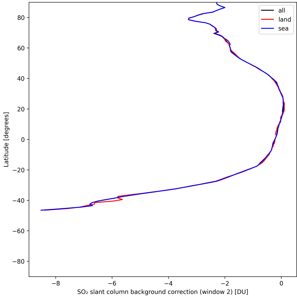
Figure 43: Zonal average of “SO 2 slant column background correction (window 2)” for 2025-07-06 to 2025-07-06.
