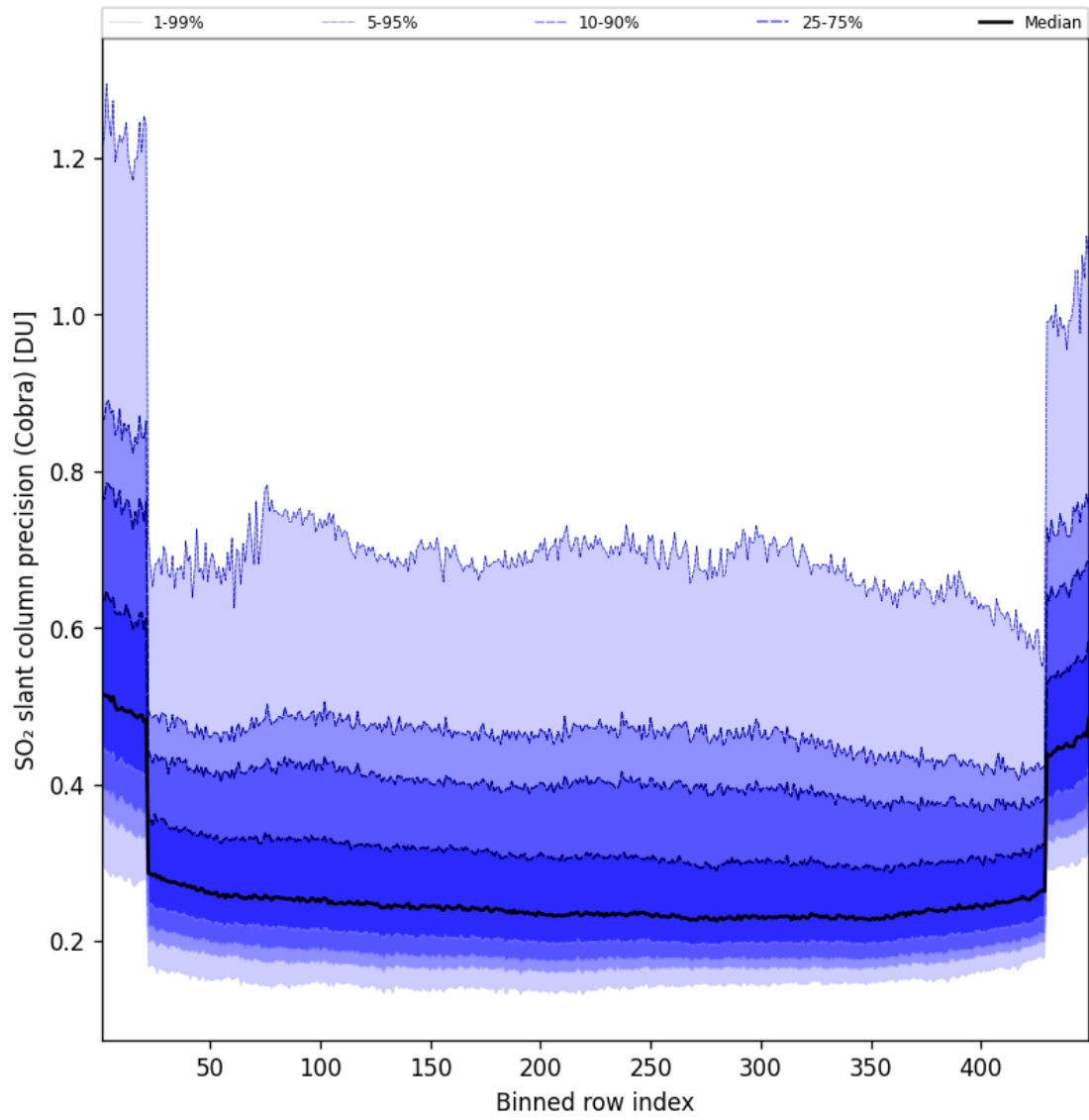
Figure 89: Along track statistics of “SO 2 slant column precision (Cobra)” for 2025-07-06 to 2025-07-06
