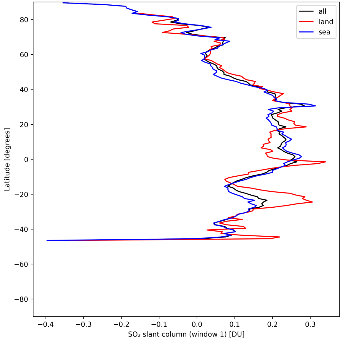
Figure 36: Zonal average of “SO 2 slant column (window 1)” for 2025-07-06 to 2025-07-06.
