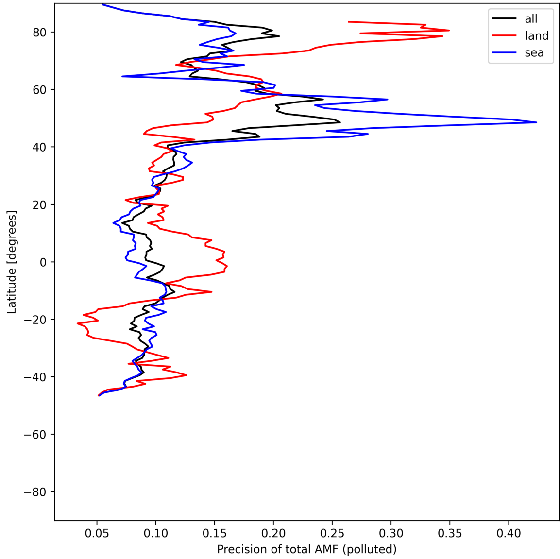
Figure 54: Zonal average of “Precision of total AMF (polluted)” for 2025-07-06 to 2025-07-06.
