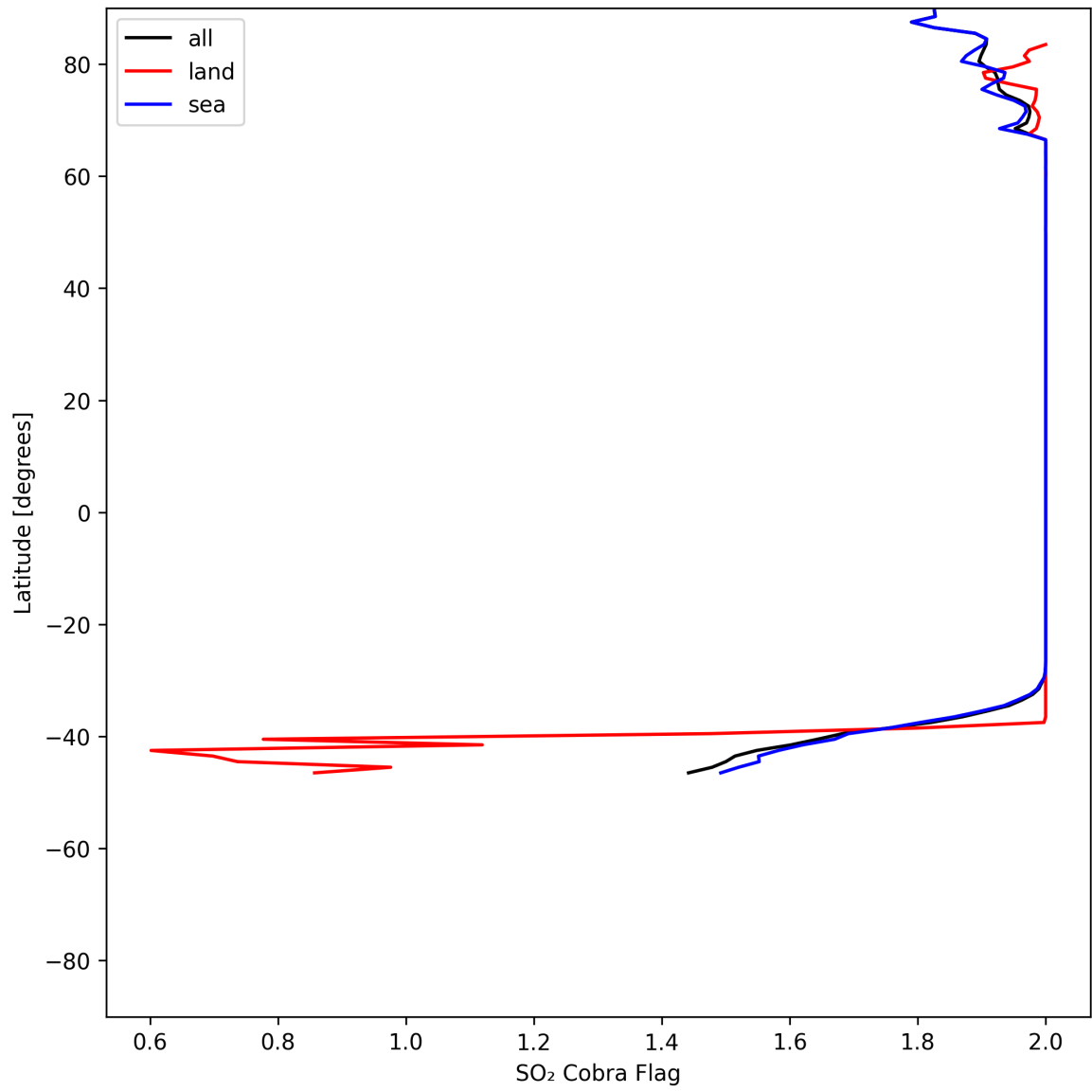
Figure 48: Zonal average of “SO 2 Cobra Flag” for 2025-07-06 to 2025-07-06.
