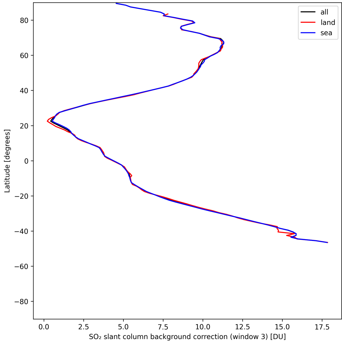
Figure 47: Zonal average of “SO 2 slant column background correction (window 3)” for 2025-07-06 to 2025-07-06.
