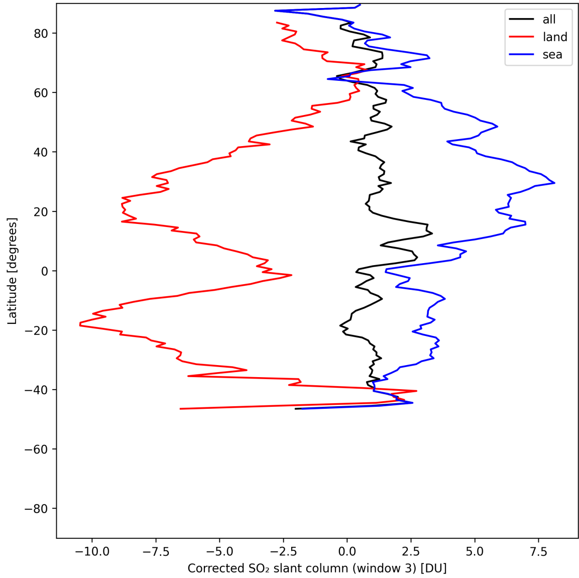
Figure 46: Zonal average of “Corrected SO 2 slant column (window 3)” for 2025-07-06 to 2025-07-06.
