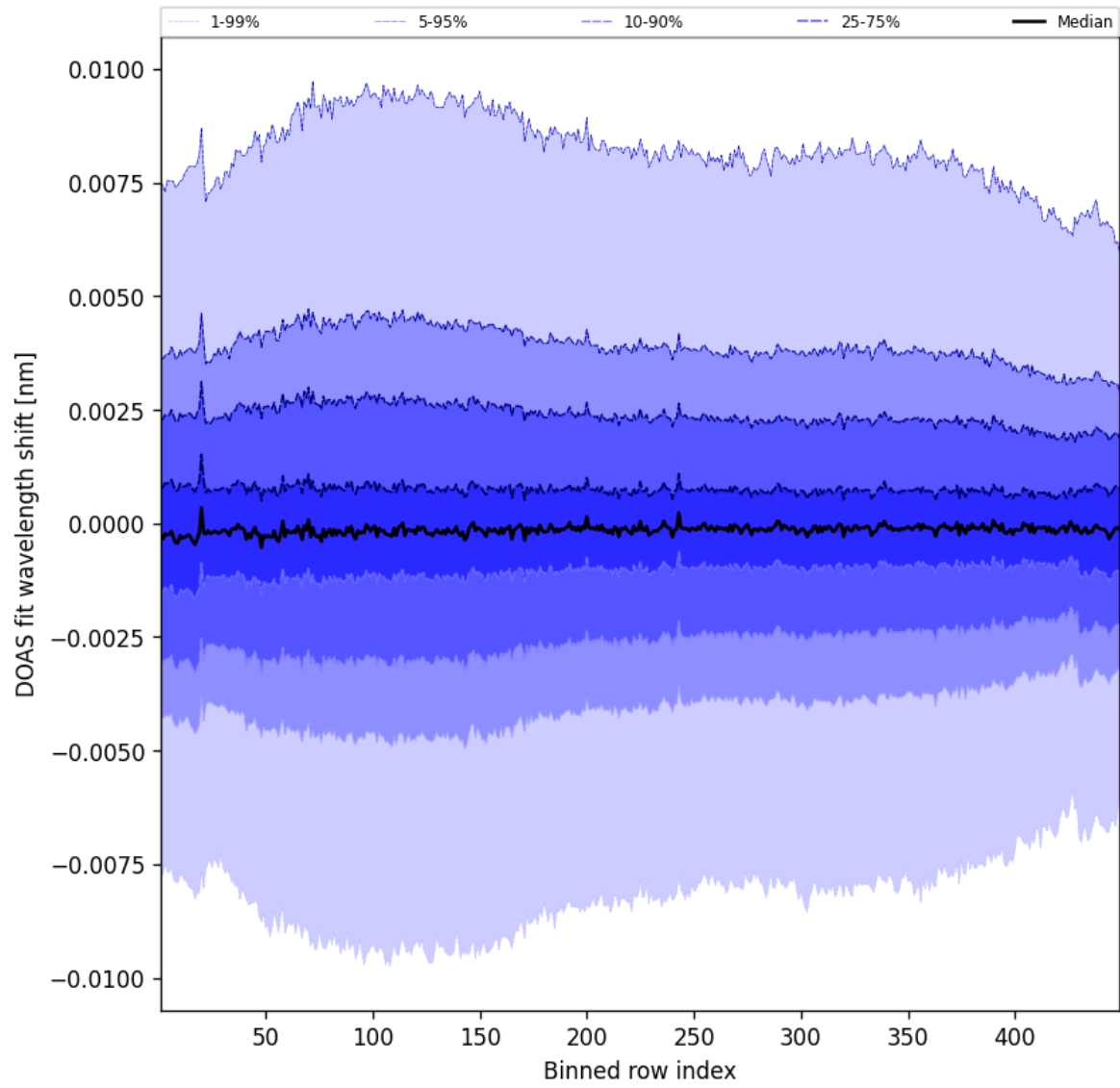
Figure 104: Along track statistics of “DOAS fit wavelength shift” for 2025-07-06 to 2025-07-06
