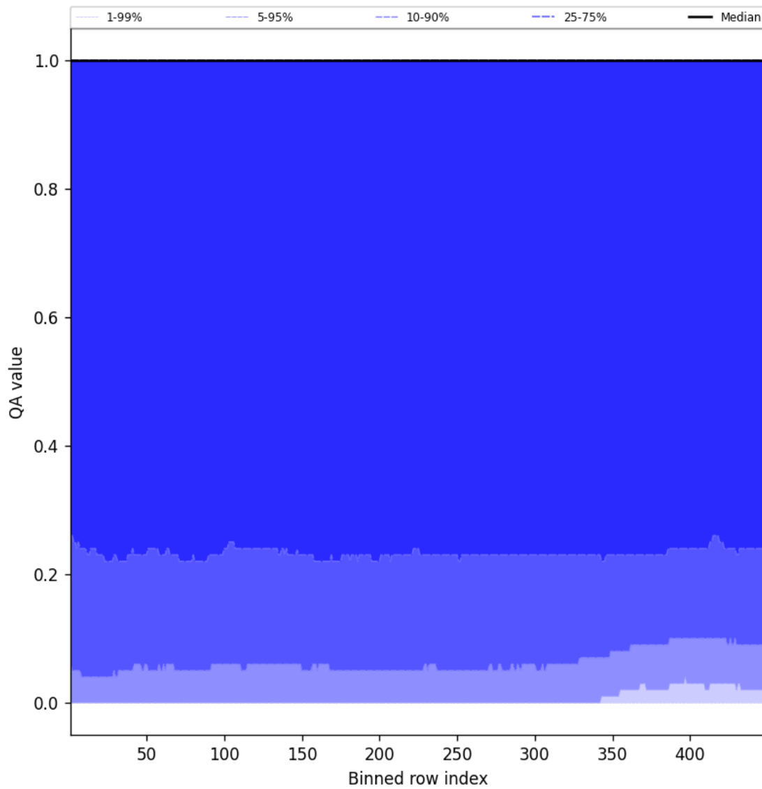
Figure 84: Along track statistics of “QA value” for 2025-07-06 to 2025-07-06
