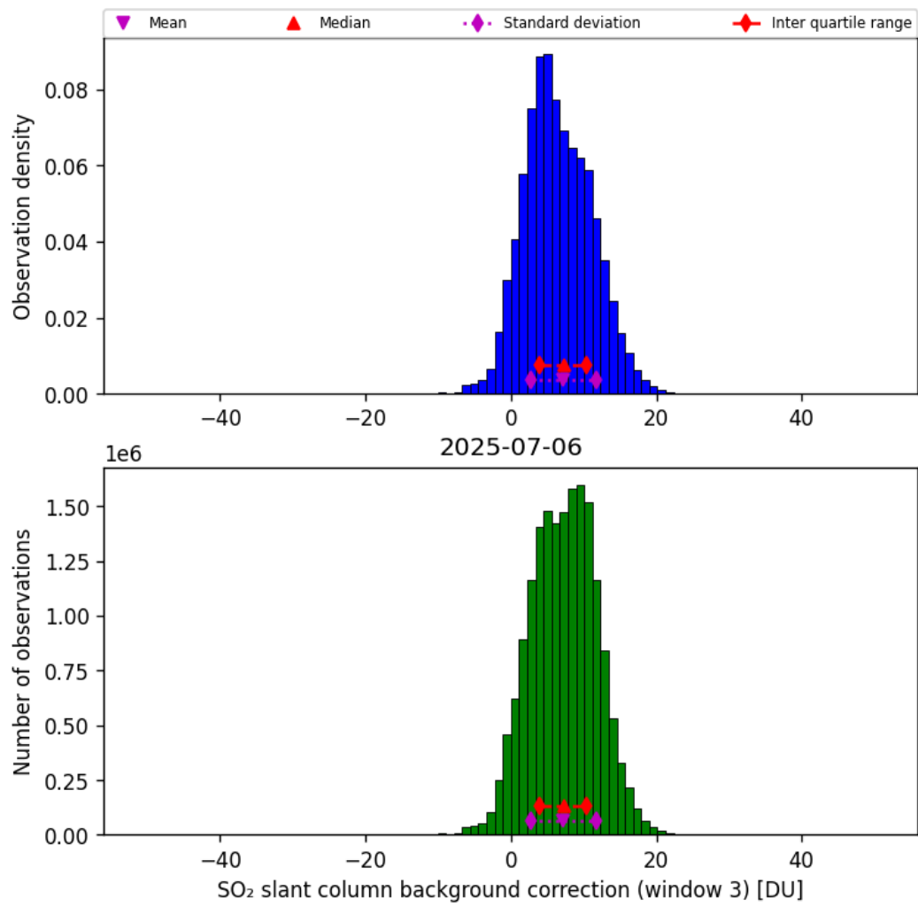
Figure 74: Histogram of “SO 2 slant column background correction (window 3)” for 2025-07-06 to 2025-07-06
