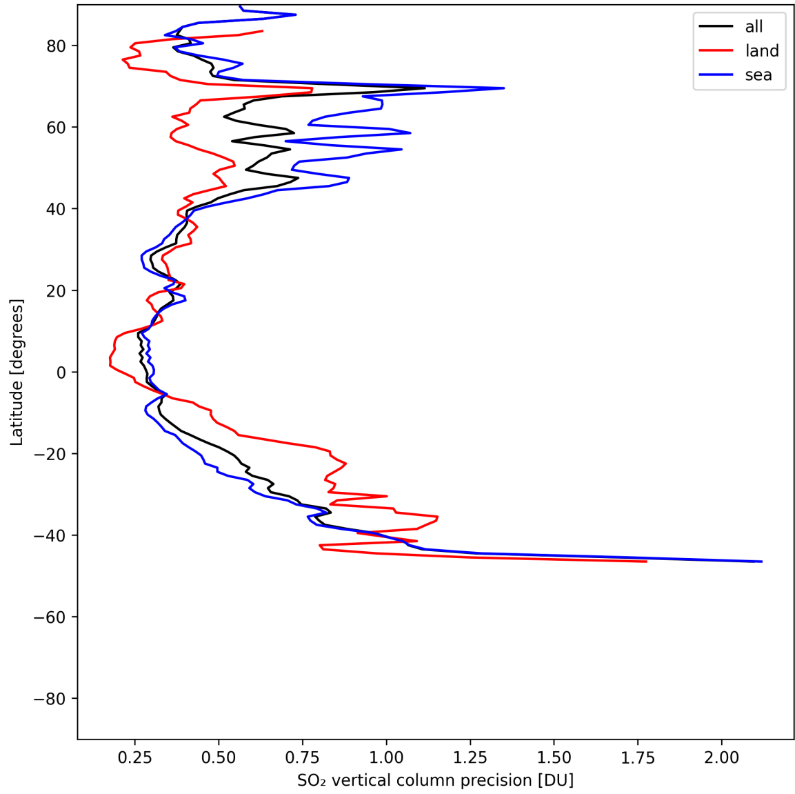
Figure 32: Zonal average of “SO 2 vertical column precision” for 2025-07-06 to 2025-07-06.
