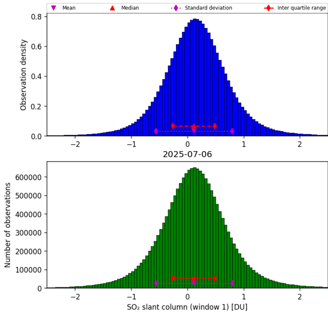
Figure 63: Histogram of “SO 2 slant column (window 1)” for 2025-07-06 to 2025-07-06
