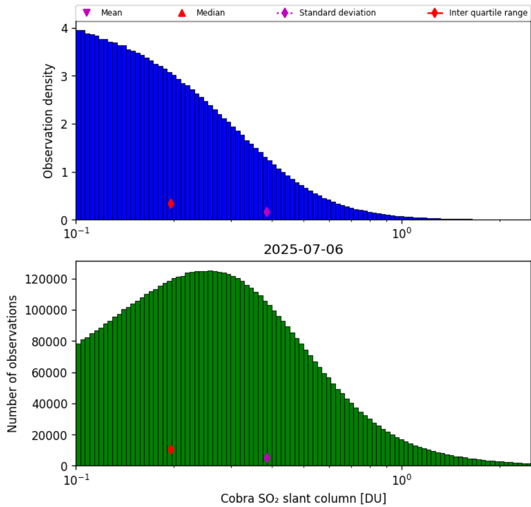
Figure 61: Histogram of “Cobra SO 2 slant column” for 2025-07-06 to 2025-07-06
