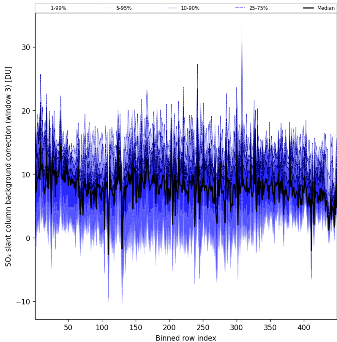
Figure 101: Along track statistics of “SO 2 slant column background correction (window 3)” for 2025-07-06 to 2025-07-06
