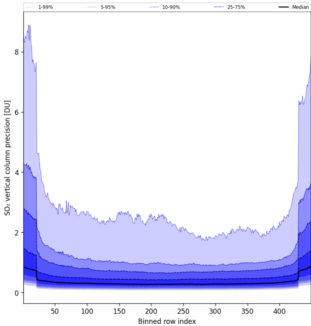
Figure 86: Along track statistics of “SO 2 vertical column precision” for 2025-07-06 to 2025-07-06
