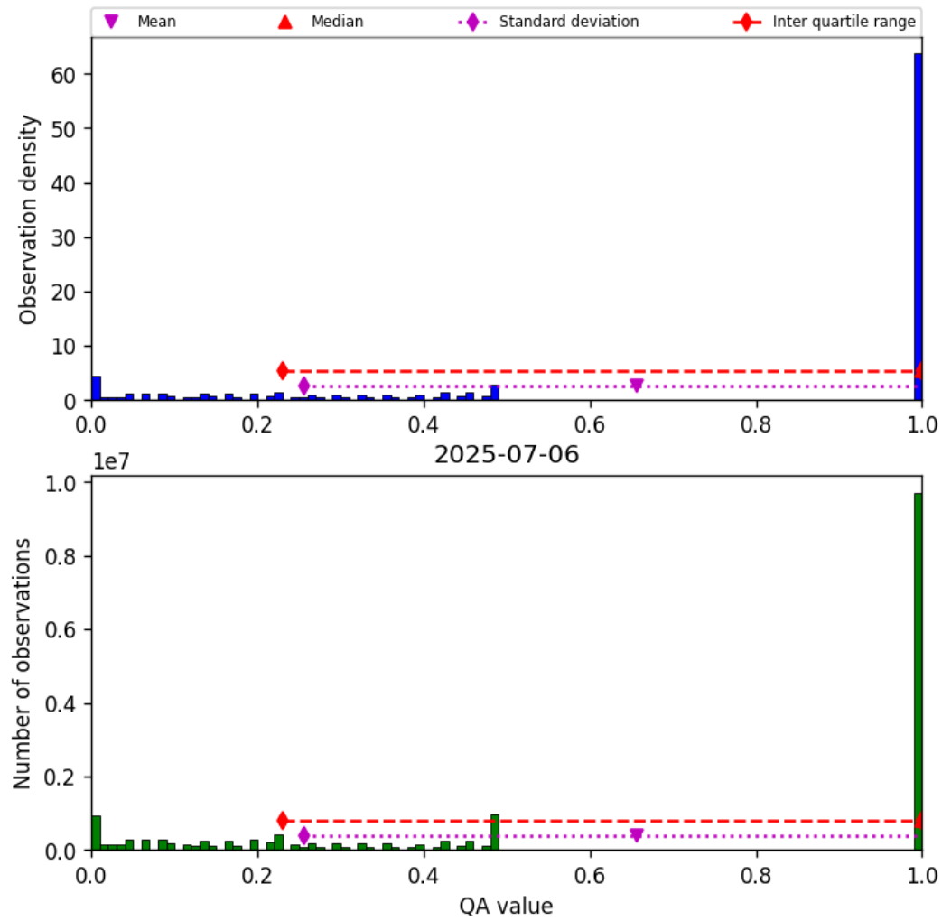
Figure 57: Histogram of “QA value” for 2025-07-06 to 2025-07-06
