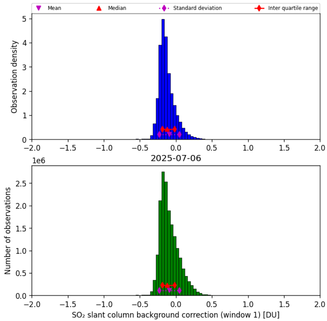
Figure 66: Histogram of “SO 2 slant column background correction (window 1)” for 2025-07-06 to 2025-07-06
