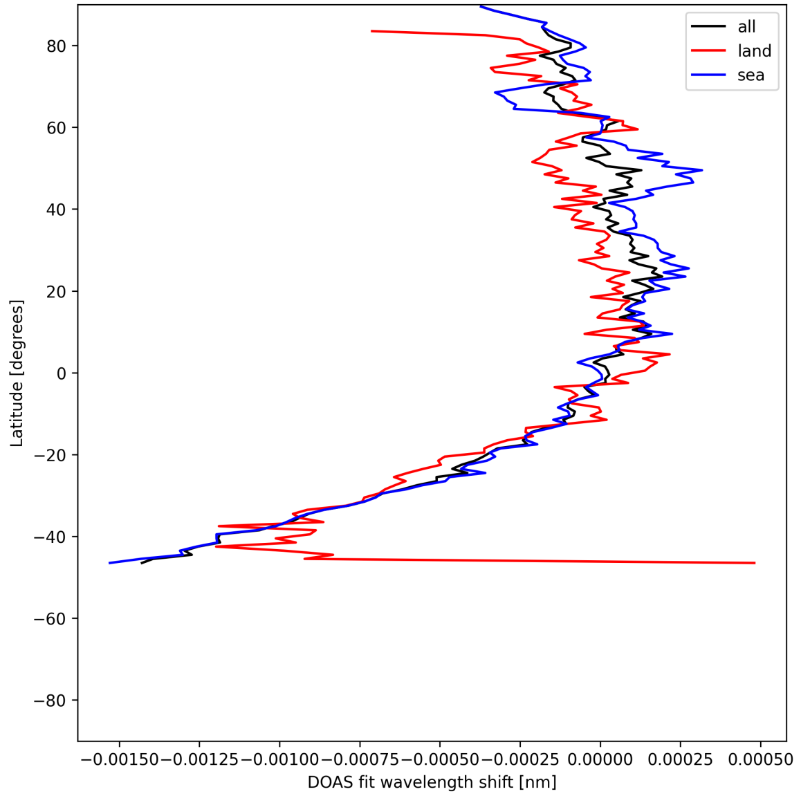
Figure 50: Zonal average of “DOAS fit wavelength shift” for 2025-07-06 to 2025-07-06.
