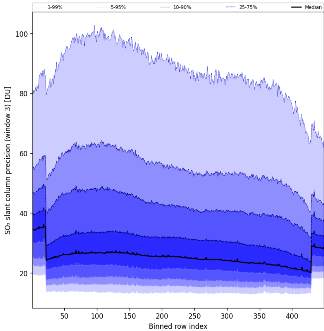
Figure 99: Along track statistics of “SO 2 slant column precision (window 3)” for 2025-07-06 to 2025-07-06
