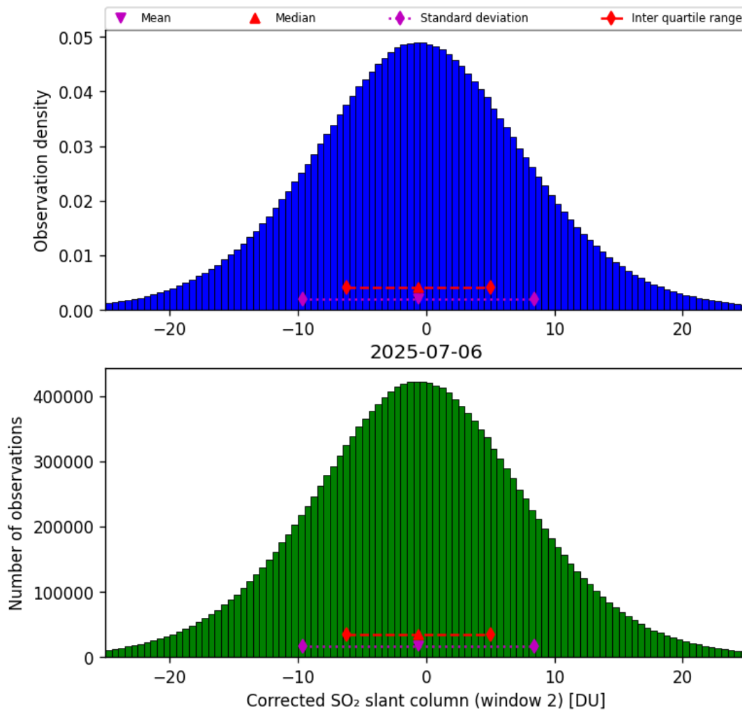
Figure 69: Histogram of “Corrected SO 2 slant column (window 2)” for 2025-07-06 to 2025-07-06
