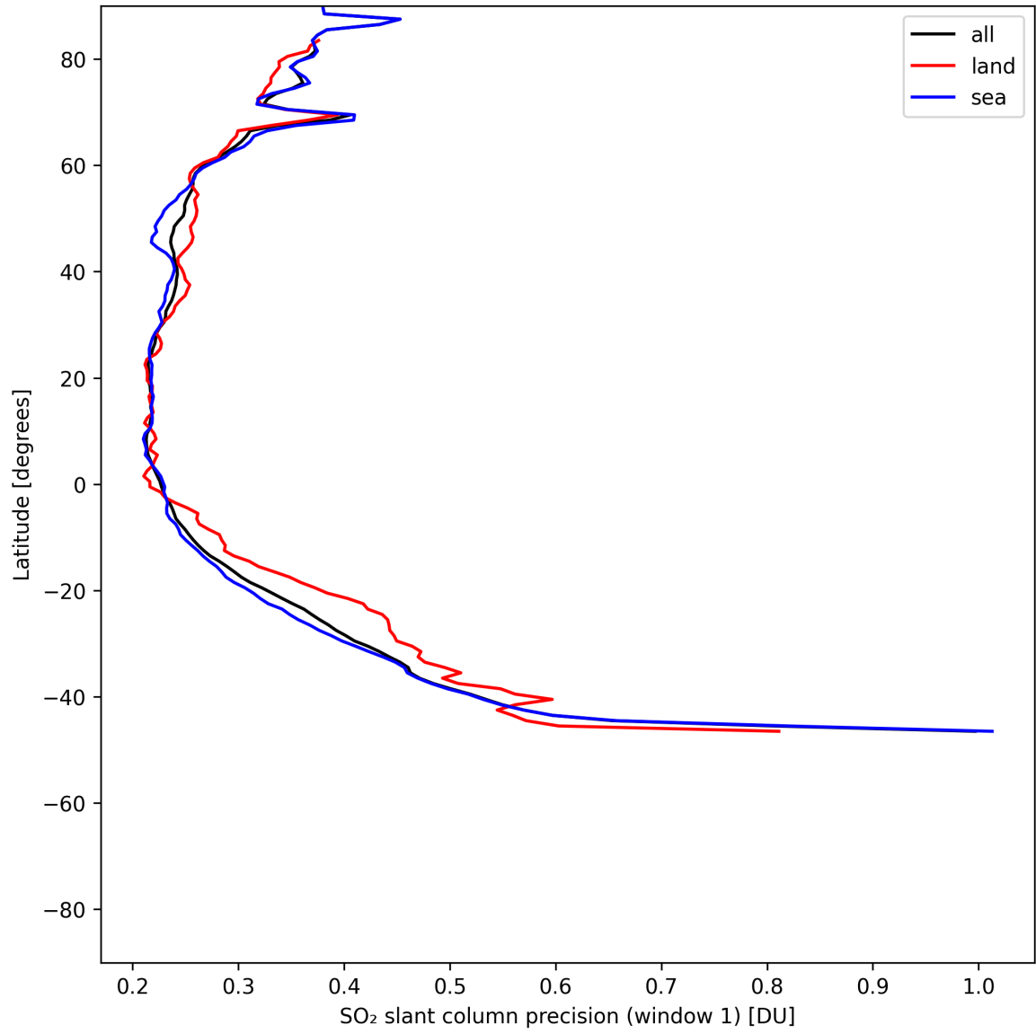
Figure 37: Zonal average of “SO 2 slant column precision (window 1)” for 2025-07-06 to 2025-07-06.
