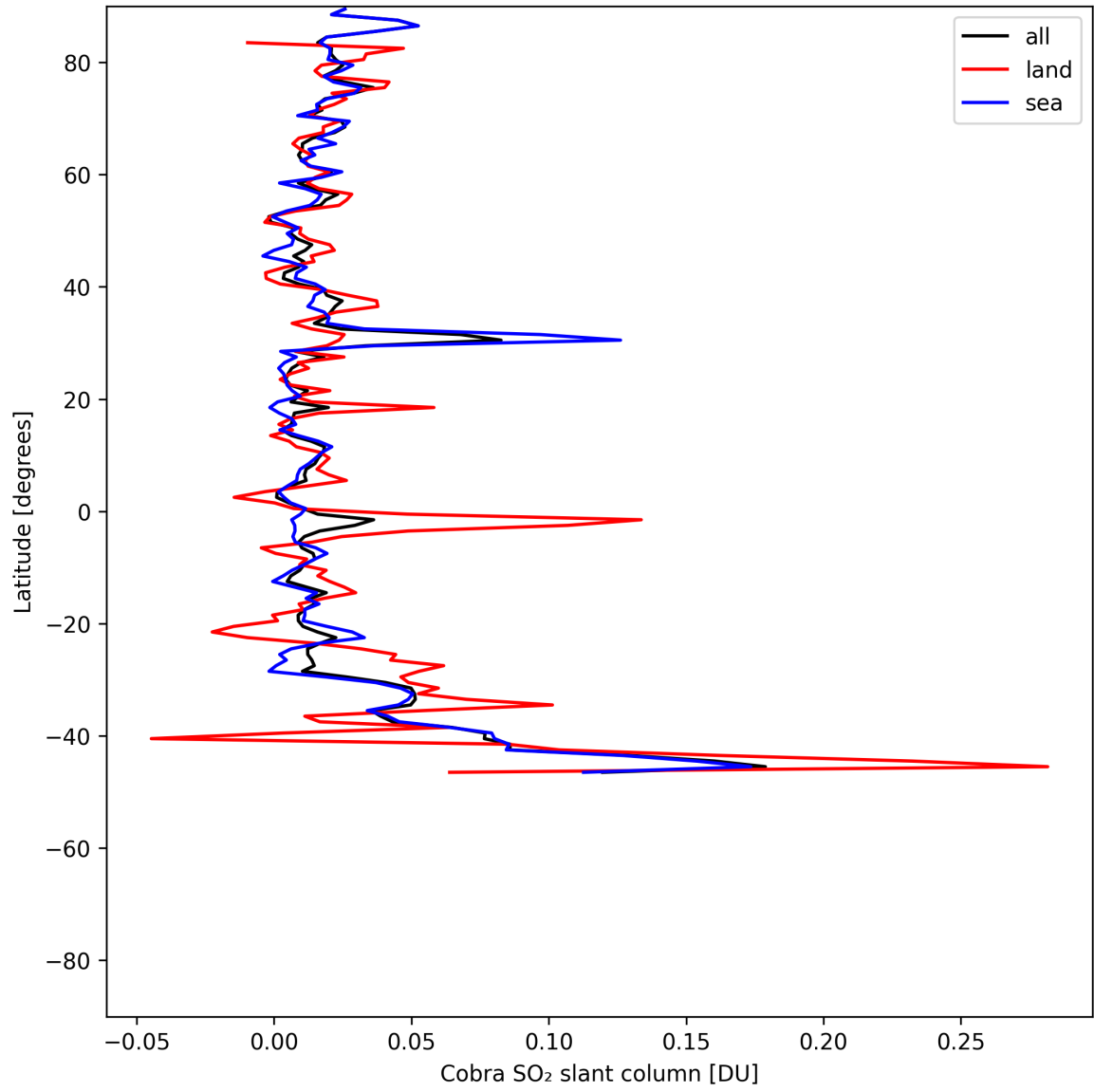
Figure 34: Zonal average of “Cobra SO 2 slant column” for 2025-07-06 to 2025-07-06.
