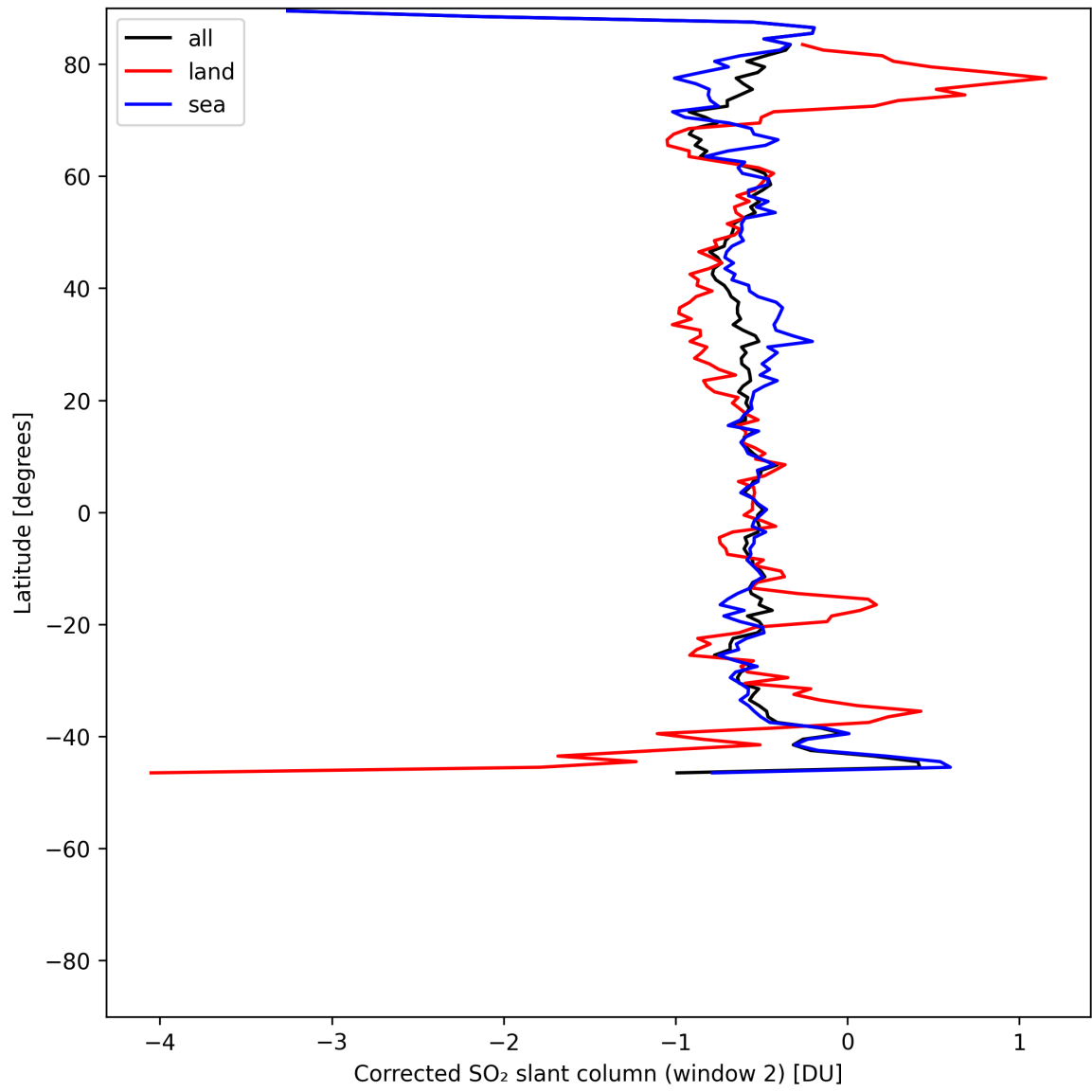
Figure 42: Zonal average of “Corrected SO 2 slant column (window 2)” for 2025-07-06 to 2025-07-06.
