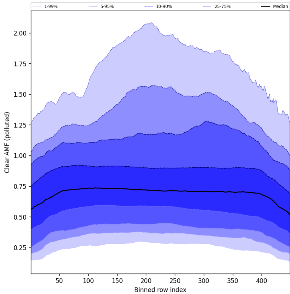
Figure 109: Along track statistics of “Clear AMF (polluted)” for 2025-07-06 to 2025-07-06
