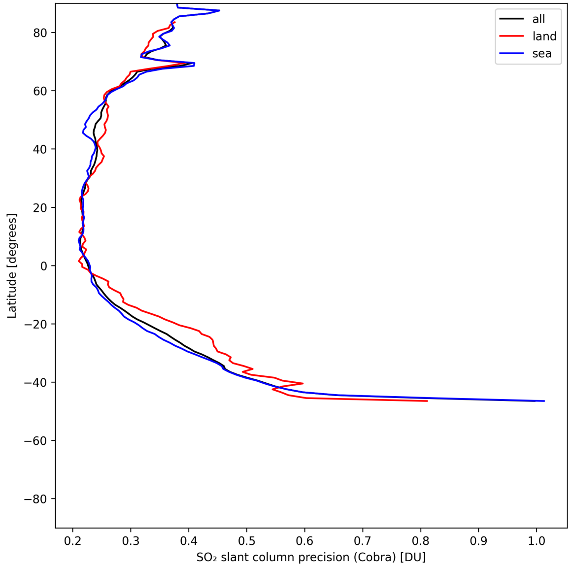
Figure 35: Zonal average of “SO 2 slant column precision (Cobra)” for 2025-07-06 to 2025-07-06.
