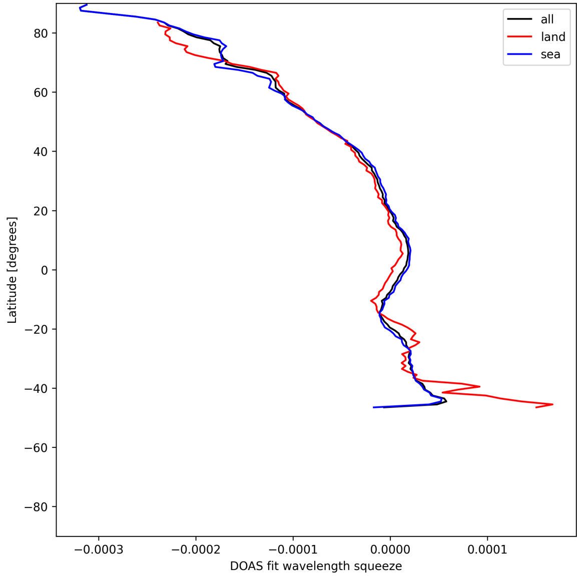
Figure 51: Zonal average of “DOAS fit wavelength squeeze” for 2025-07-06 to 2025-07-06.
