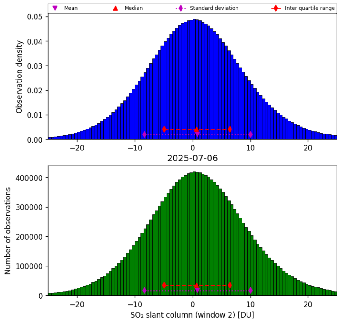
Figure 67: Histogram of “SO 2 slant column (window 2)” for 2025-07-06 to 2025-07-06
