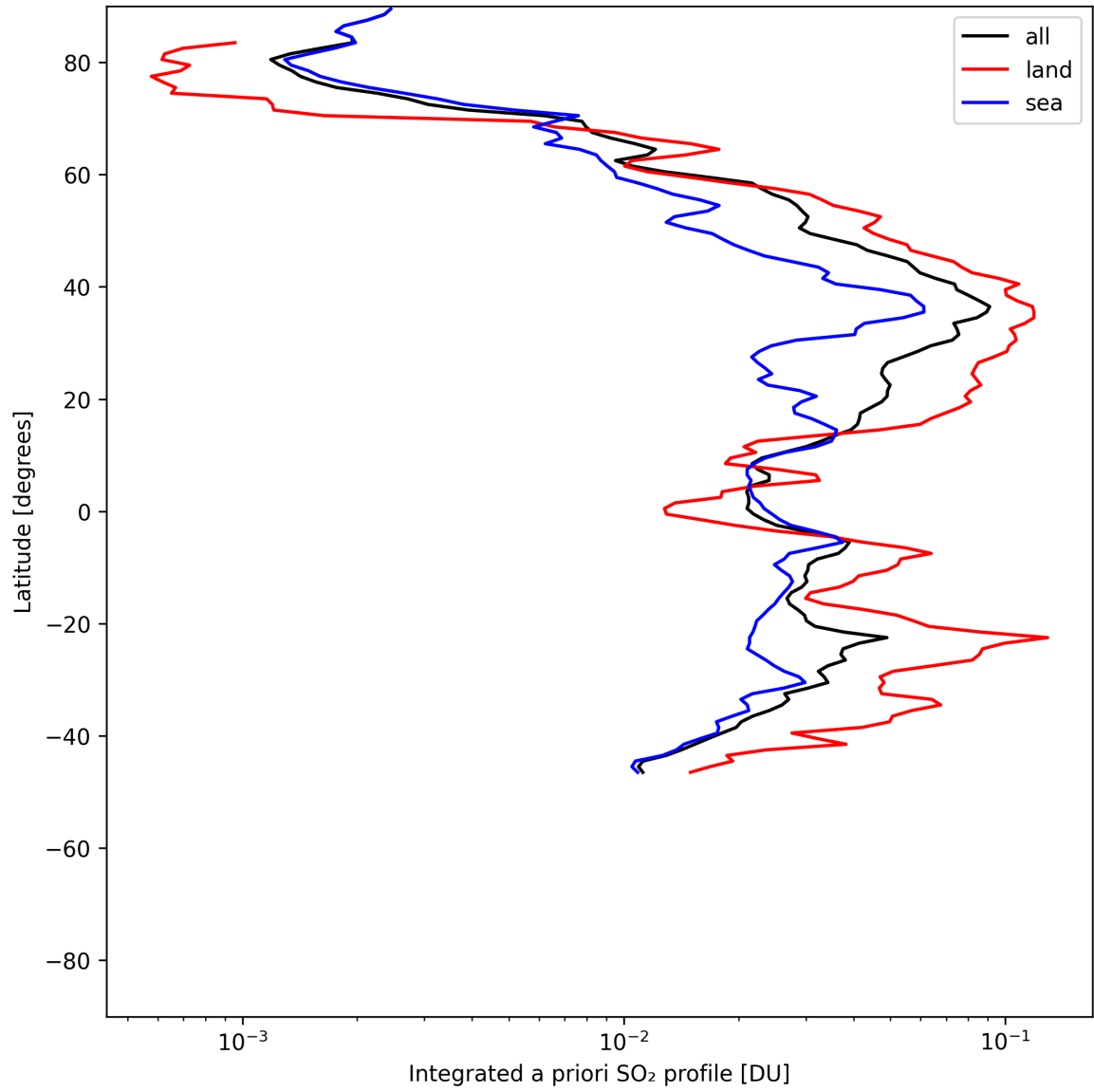
Figure 49: Zonal average of “Integrated a priori SO 2 profile” for 2025-07-06 to 2025-07-06.
