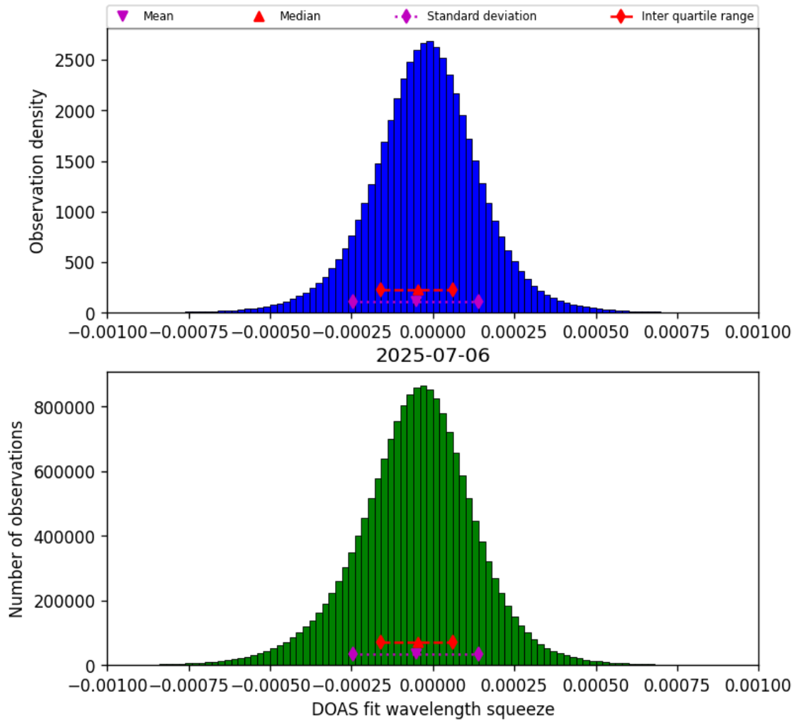
Figure 78: Histogram of “DOAS fit wavelength squeeze” for 2025-07-06 to 2025-07-06
