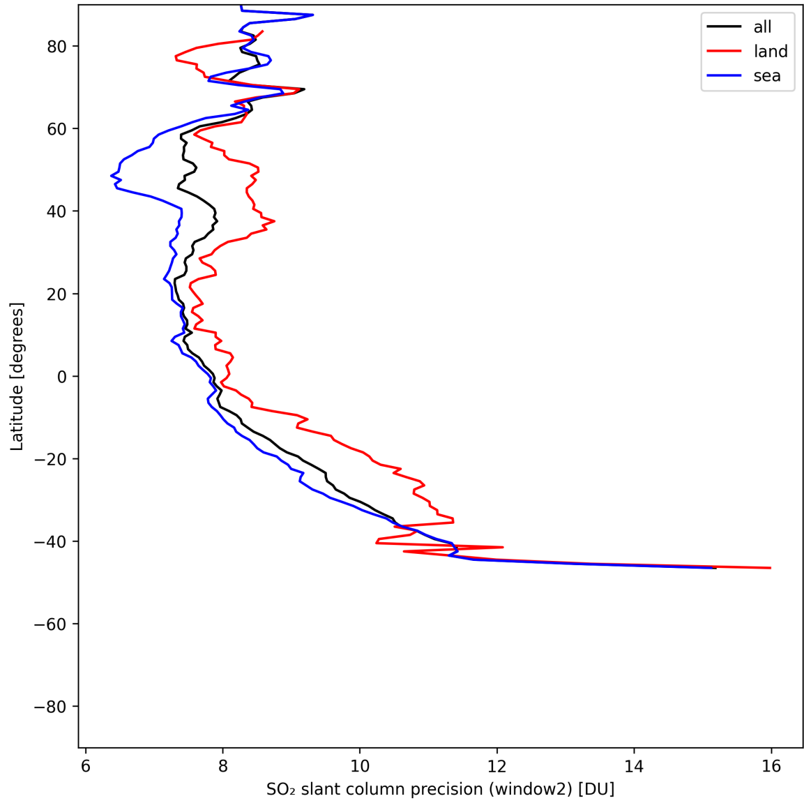
Figure 41: Zonal average of “SO 2 slant column precision (window2)” for 2025-07-06 to 2025-07-06.
