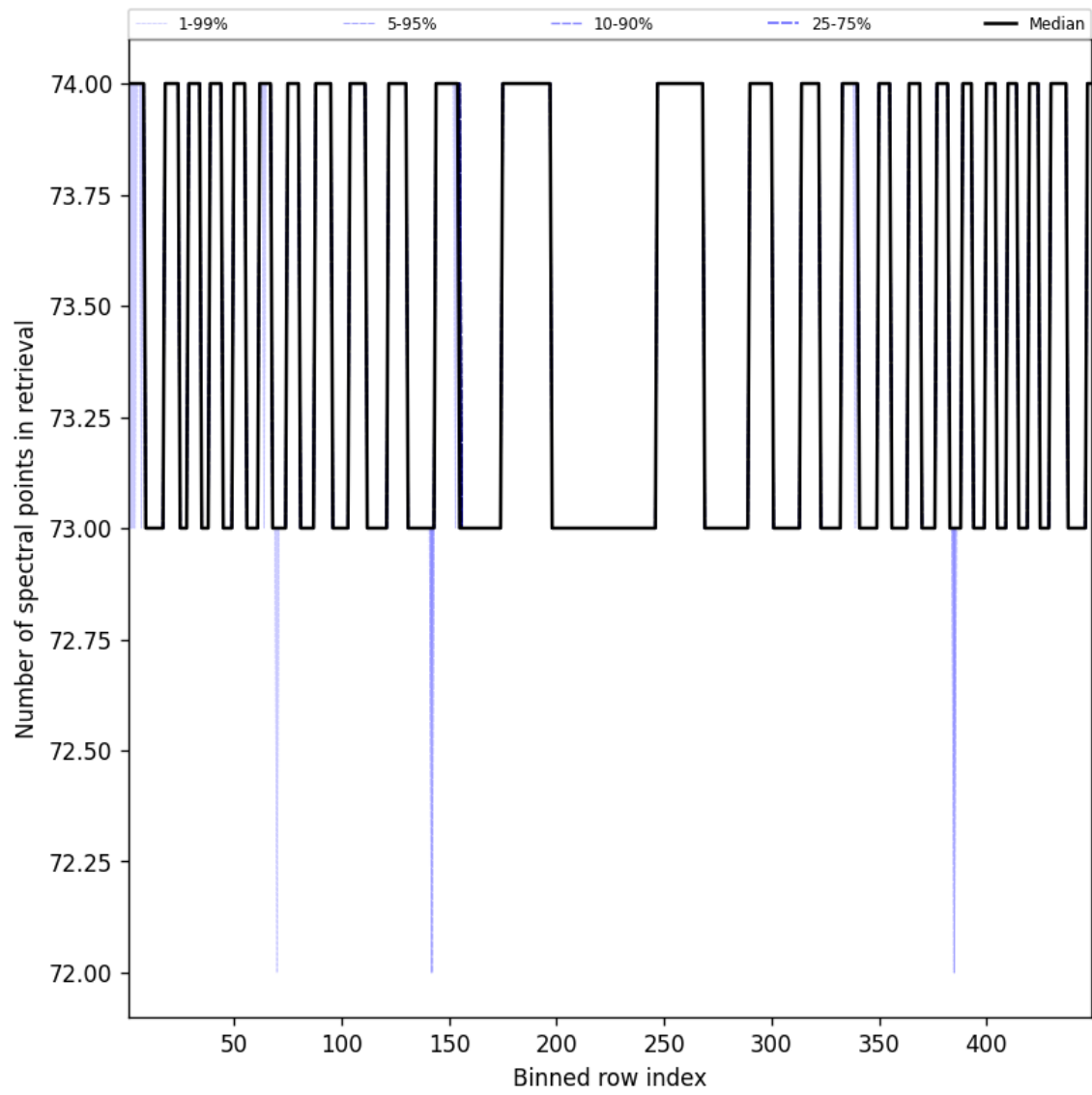
Figure 110: Along track statistics of “Number of spectral points in retrieval” for 2025-07-06 to 2025-07-06
