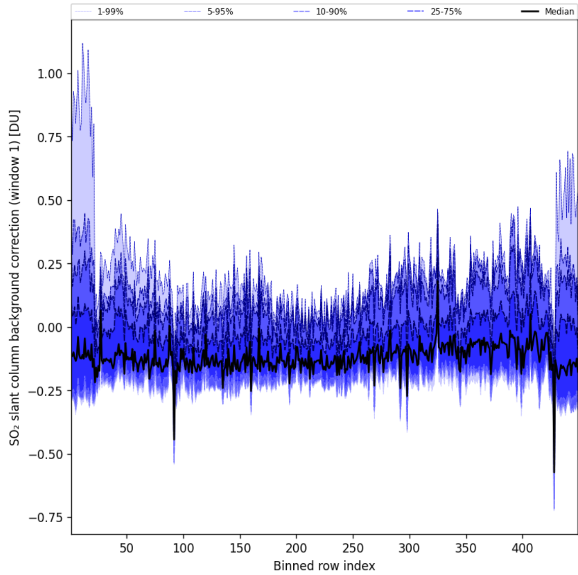
Figure 93: Along track statistics of “SO 2 slant column background correction (window 1)” for 2025-07-06 to 2025-07-06
