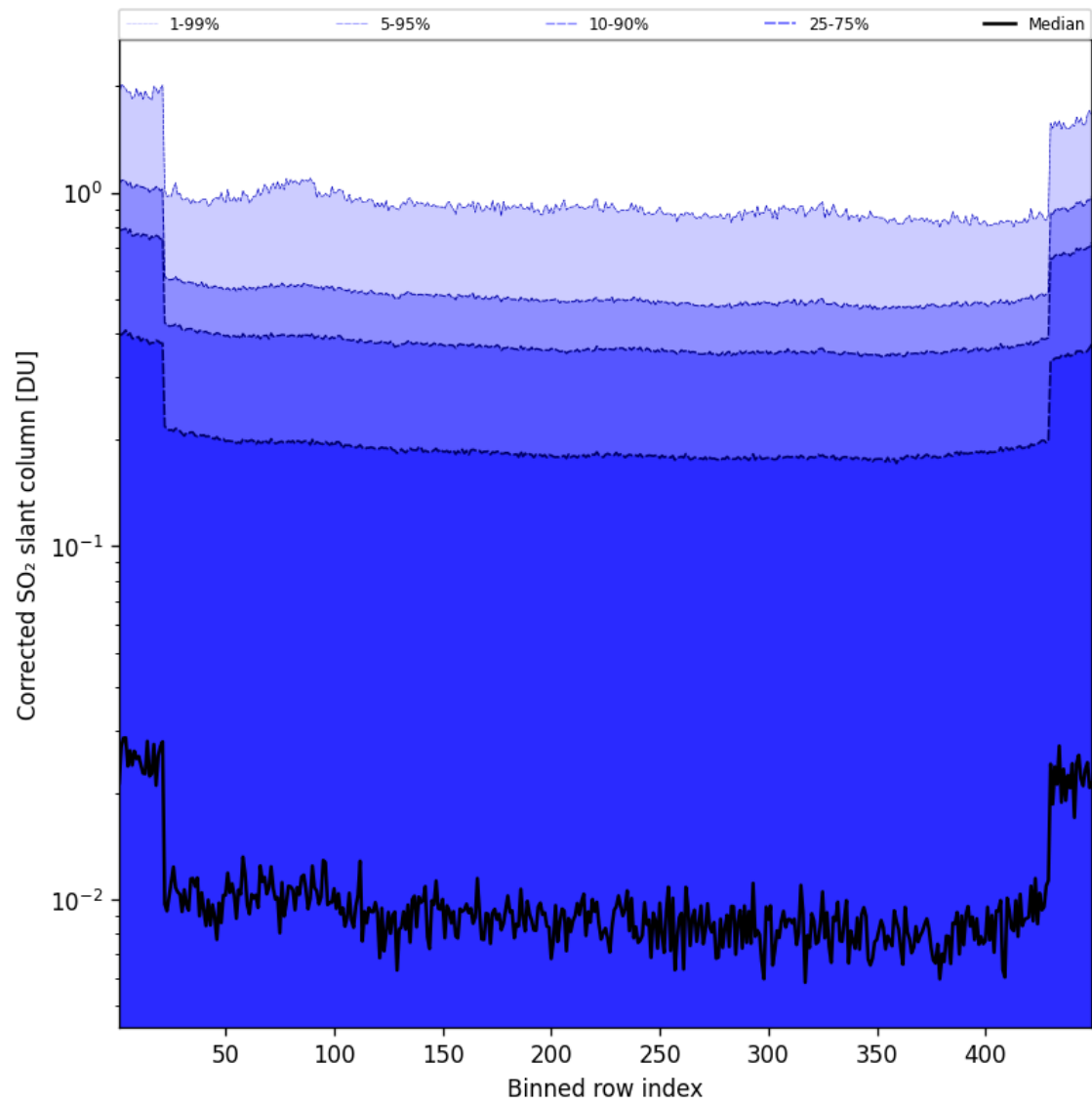
Figure 87: Along track statistics of "Corrected SO 2 slant column" for 2025-07-06 to 2025-07-06
