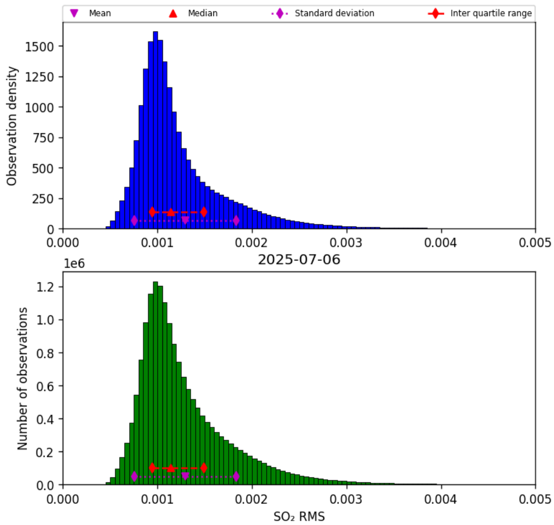
Figure 79: Histogram of “SO 2 RMS” for 2025-07-06 to 2025-07-06
