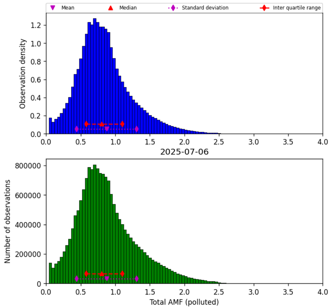
Figure 80: Histogram of “Total AMF (polluted)” for 2025-07-06 to 2025-07-06
