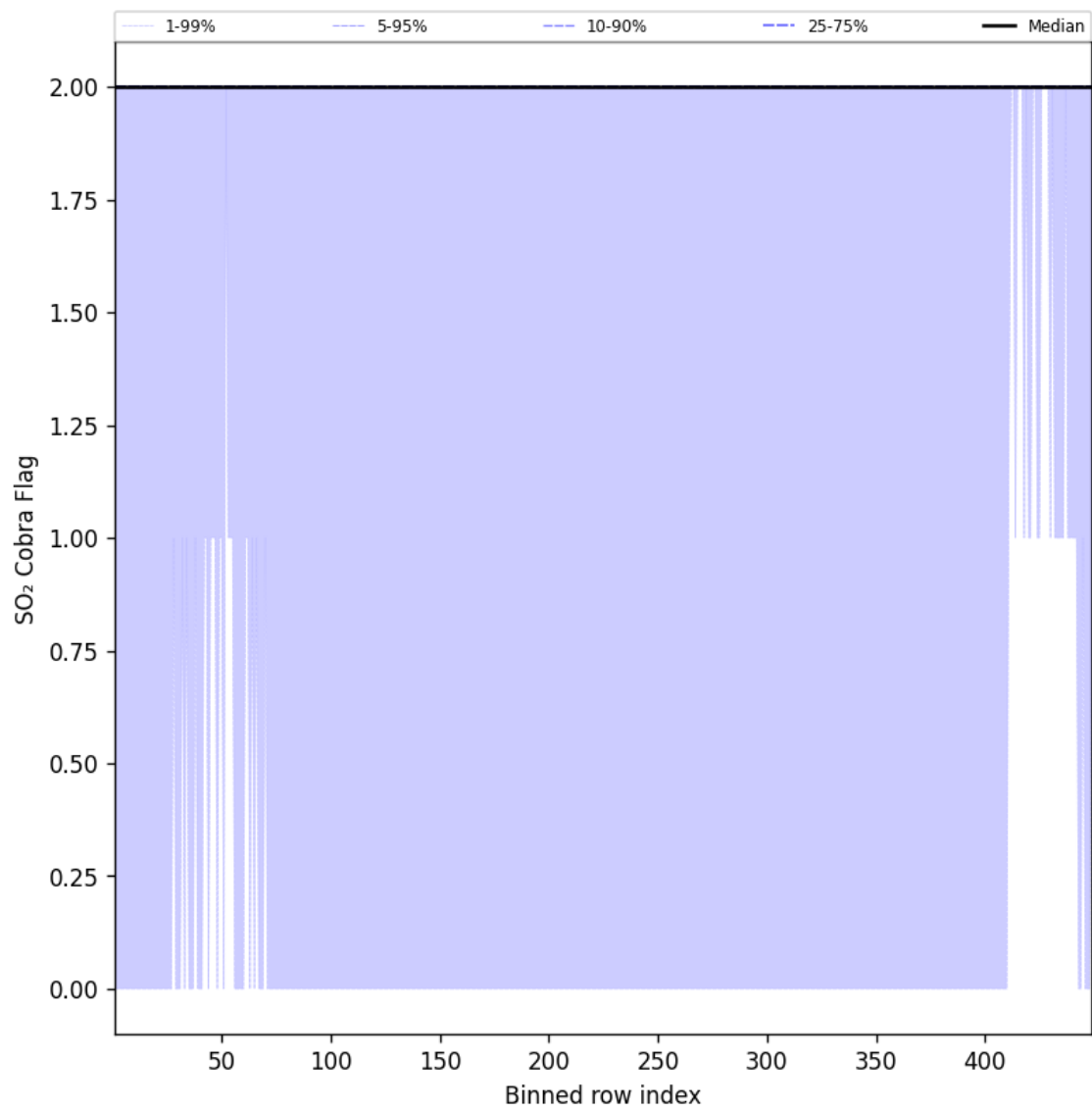
Figure 102: Along track statistics of “SO 2 Cobra Flag” for 2025-07-06 to 2025-07-06
