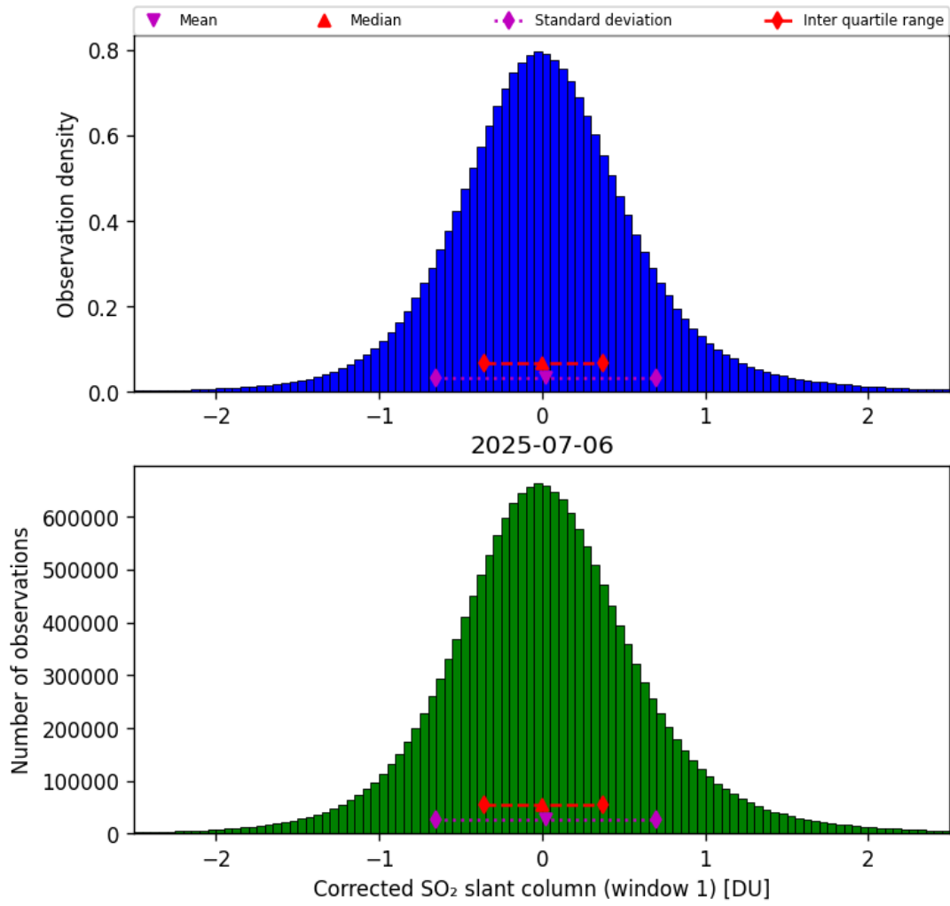
Figure 65: Histogram of “Corrected SO 2 slant column (window 1)” for 2025-07-06 to 2025-07-06
