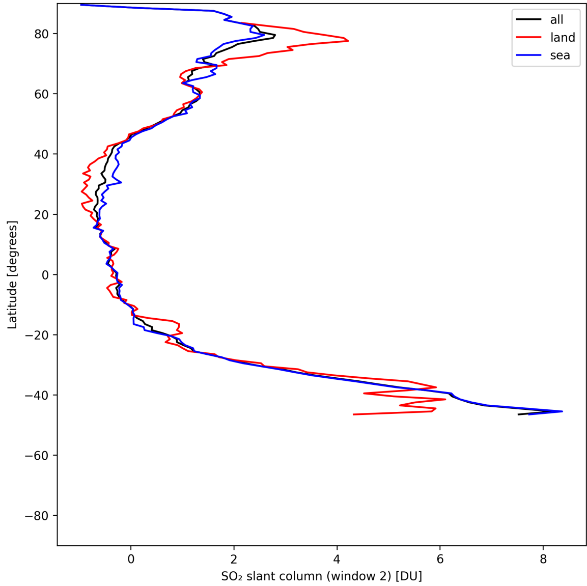
Figure 40: Zonal average of “SO 2 slant column (window 2)” for 2025-07-06 to 2025-07-06.
