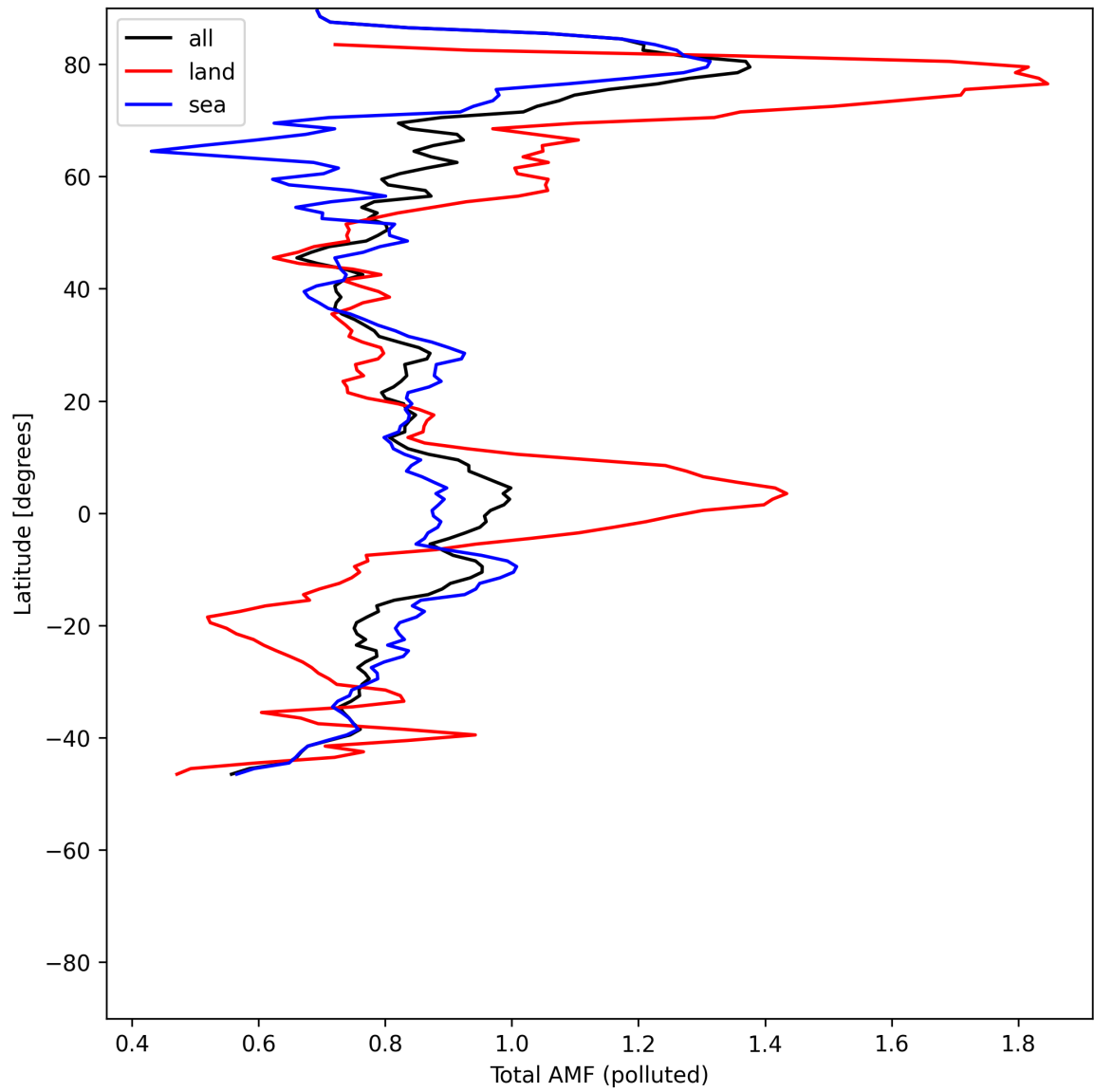
Figure 53: Zonal average of “Total AMF (polluted)” for 2025-07-06 to 2025-07-06.
