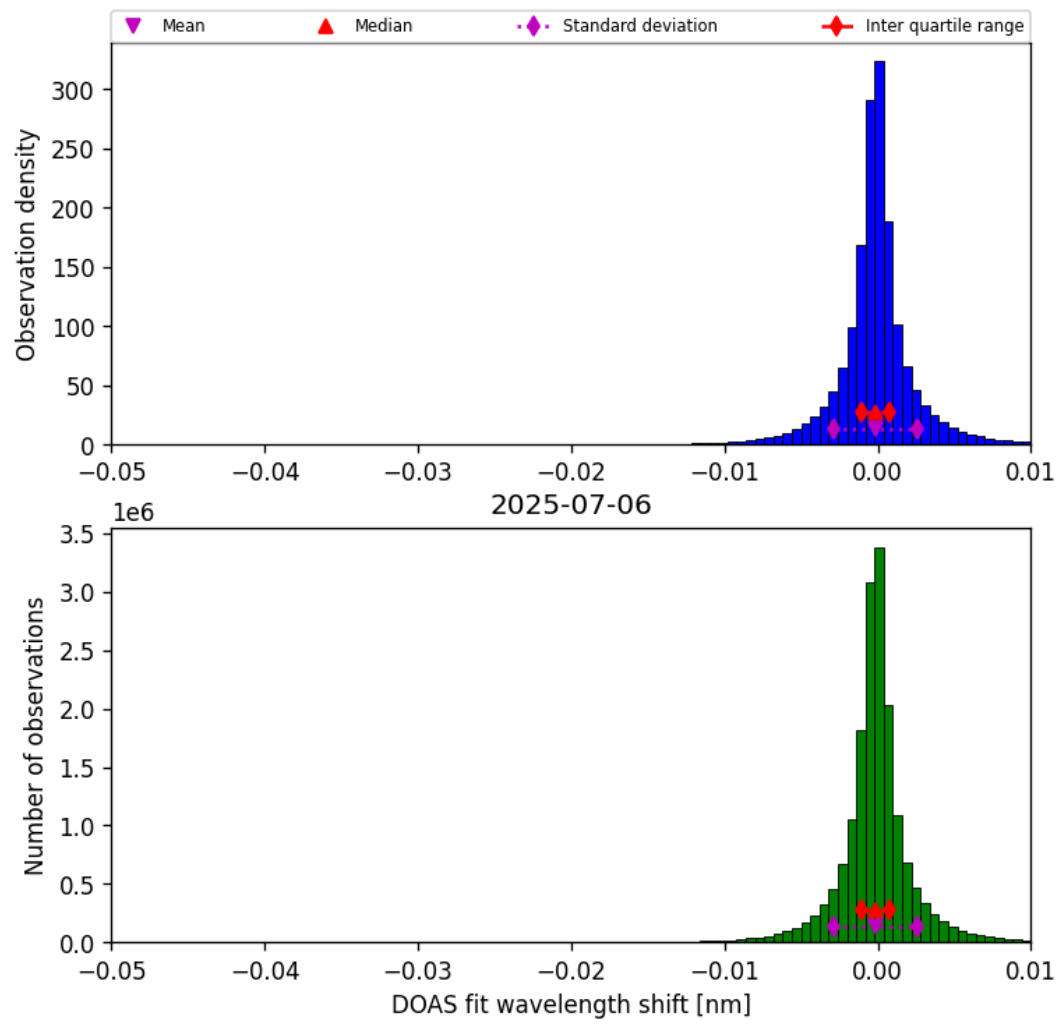
Figure 77: Histogram of “DOAS fit wavelength shift” for 2025-07-06 to 2025-07-06
