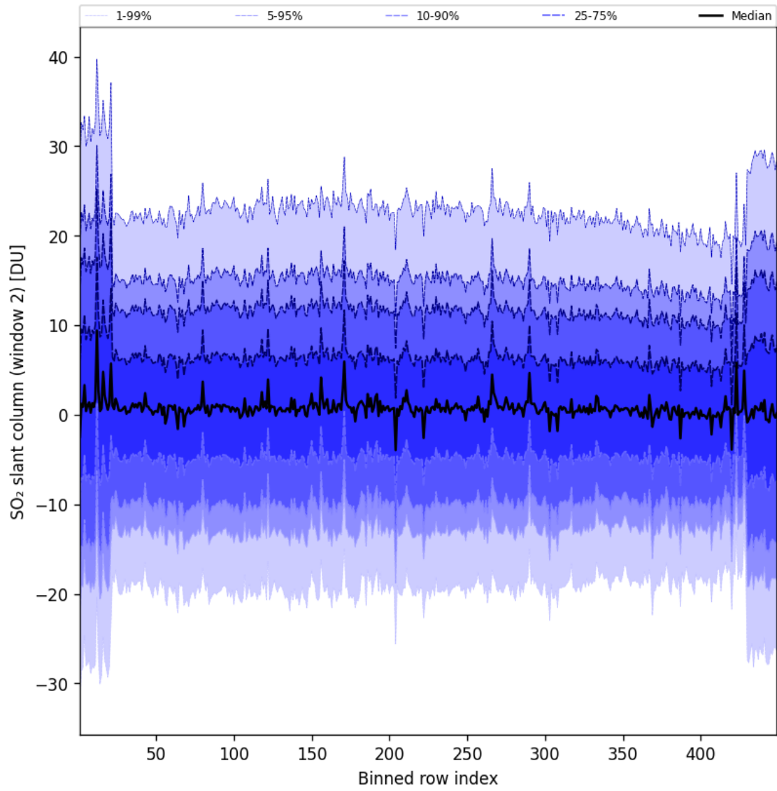
Figure 94: Along track statistics of “SO 2 slant column (window 2)” for 2025-07-06 to 2025-07-06
