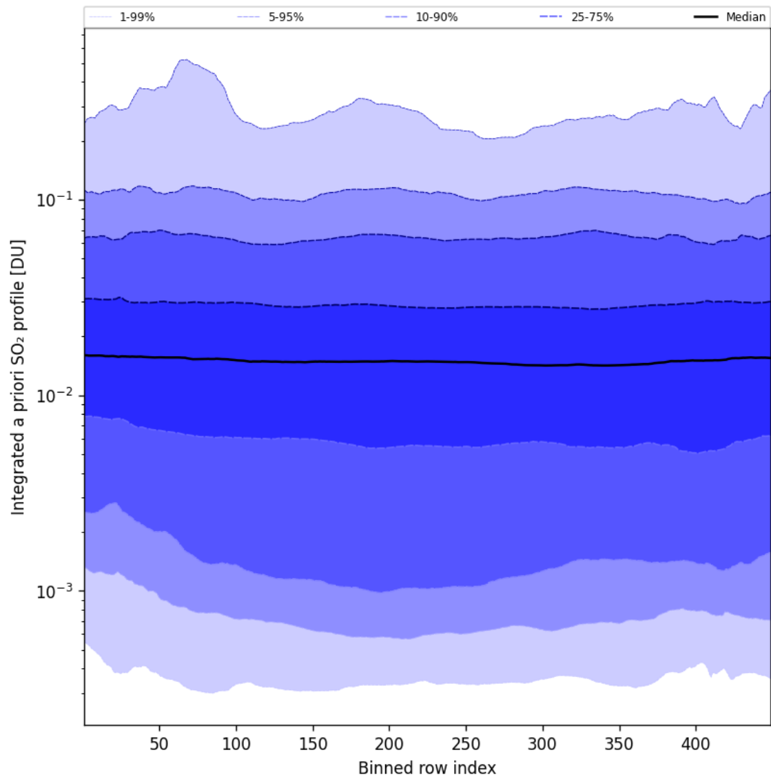
Figure 103: Along track statistics of “Integrated a priori SO 2 profile” for 2025-07-06 to 2025-07-06
