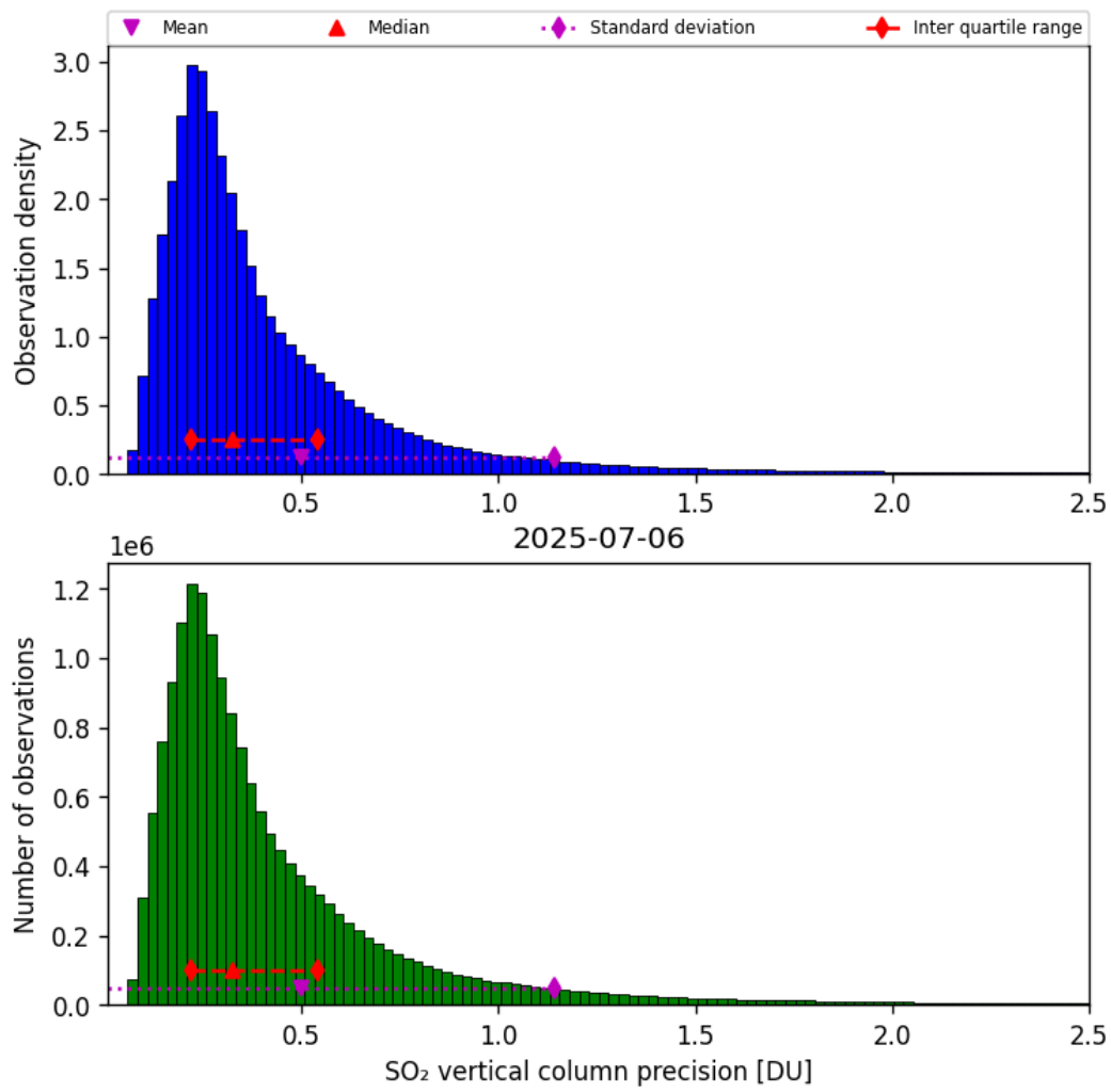
Figure 59: Histogram of “SO 2 vertical column precision” for 2025-07-06 to 2025-07-06
