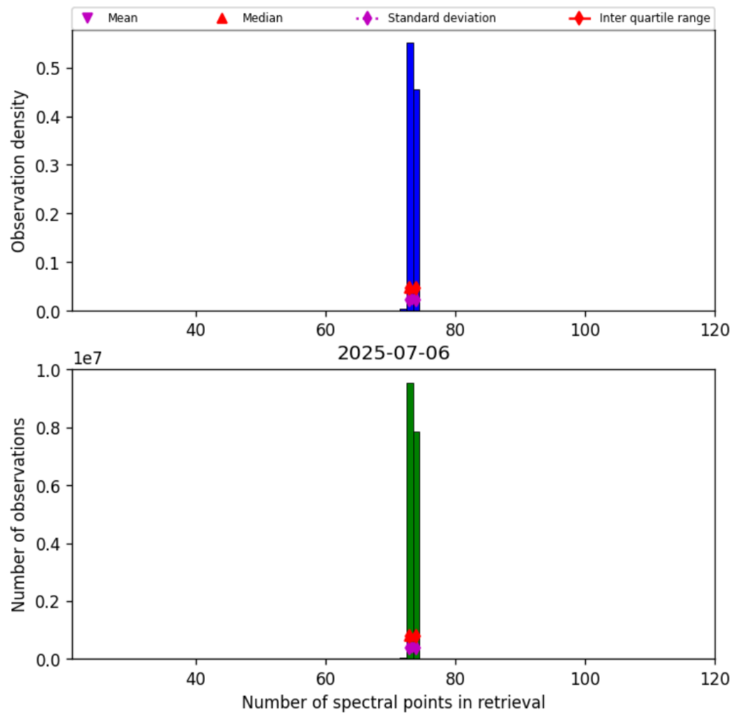
Figure 83: Histogram of “Number of spectral points in retrieval” for 2025-07-06 to 2025-07-06
