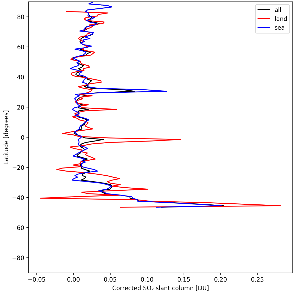
Figure 33: Zonal average of “Corrected SO 2 slant column” for 2025-07-06 to 2025-07-06.
