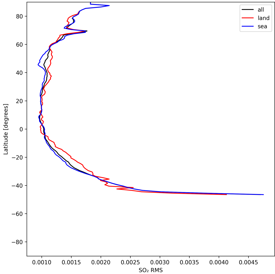
Figure 52: Zonal average of “SO 2 RMS” for 2025-07-06 to 2025-07-06.
