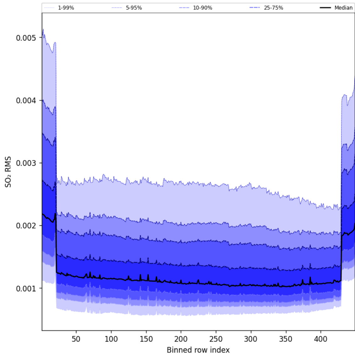
Figure 106: Along track statistics of “SO 2 RMS” for 2025-07-06 to 2025-07-06
