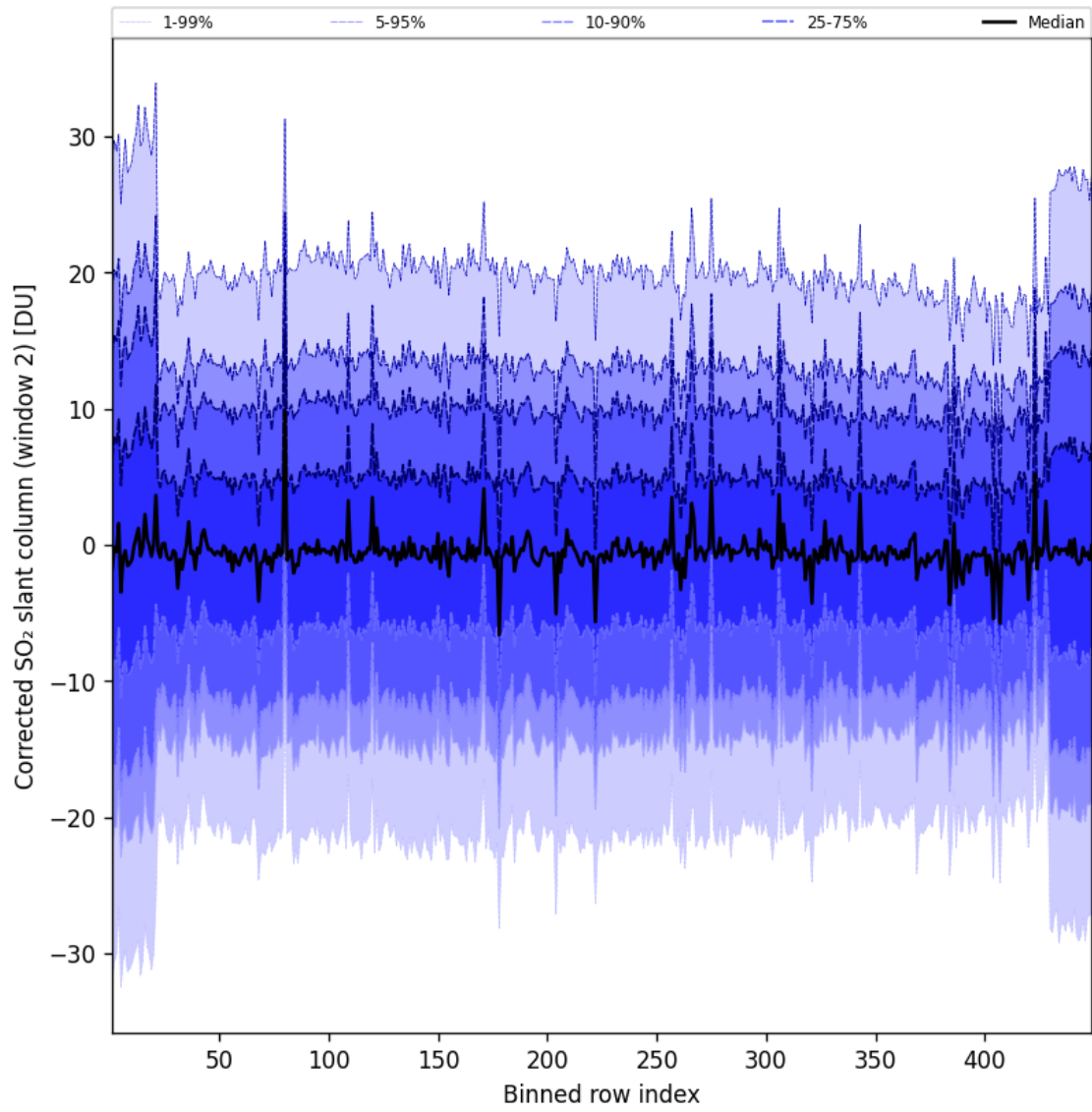
Figure 96: Along track statistics of “Corrected SO 2 slant column (window 2)” for 2025-07-06 to 2025-07-06
