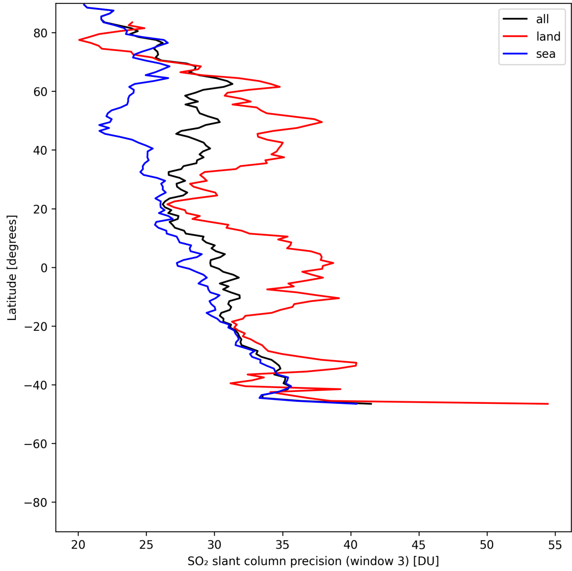
Figure 45: Zonal average of “SO 2 slant column precision (window 3)” for 2025-07-06 to 2025-07-06.
