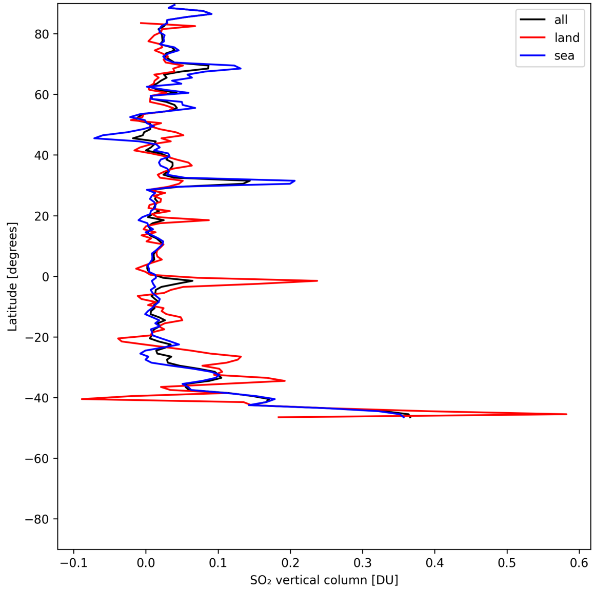
Figure 31: Zonal average of “SO 2 vertical column” for 2025-07-06 to 2025-07-06.
