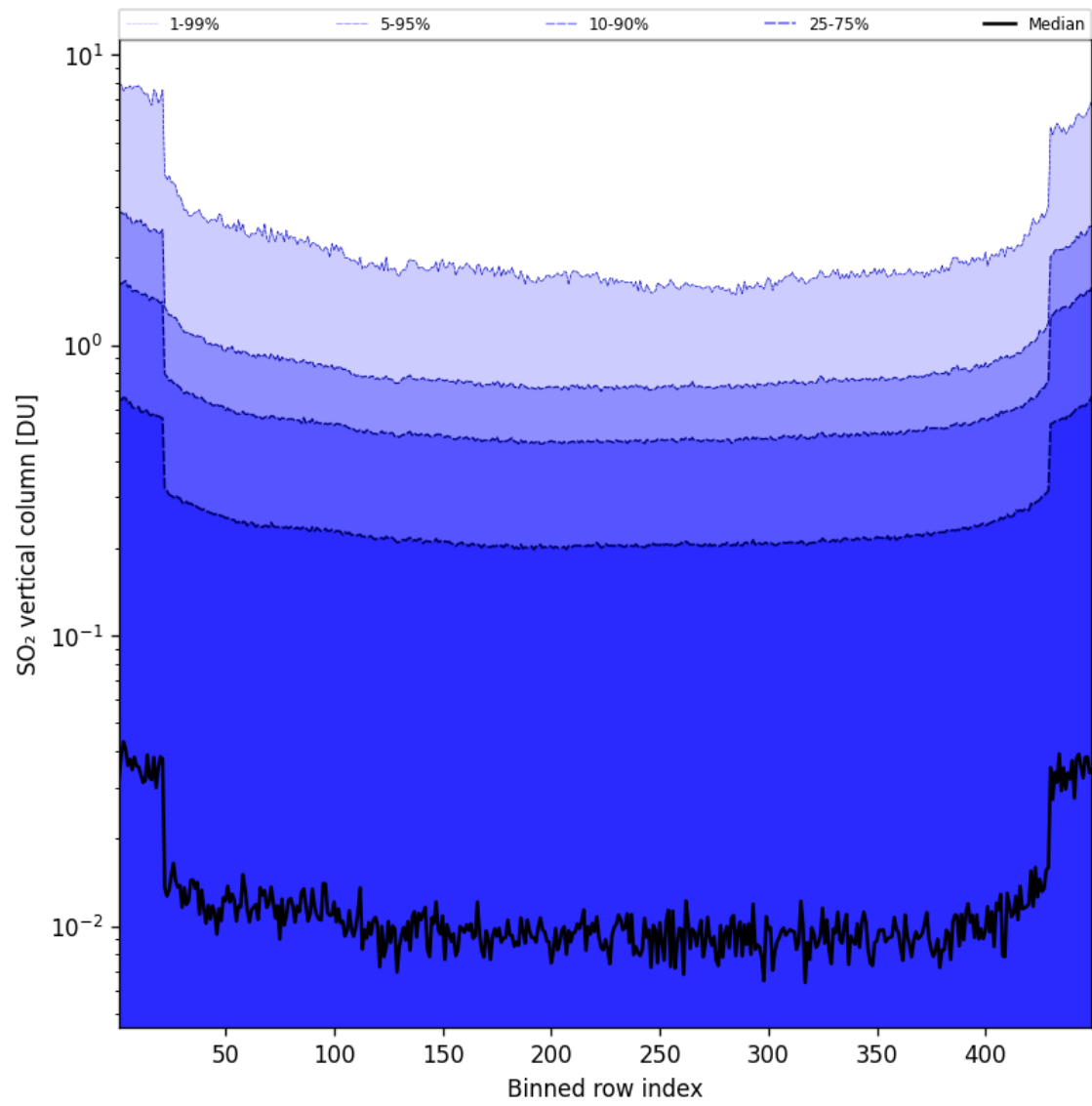
Figure 85: Along track statistics of “SO 2 vertical column” for 2025-07-06 to 2025-07-06
