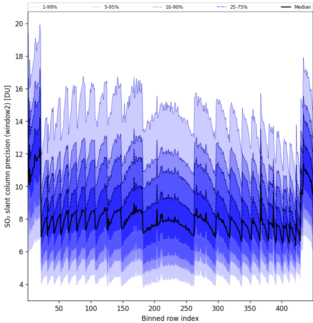
Figure 95: Along track statistics of “SO 2 slant column precision (window2)” for 2025-07-06 to 2025-07-06
