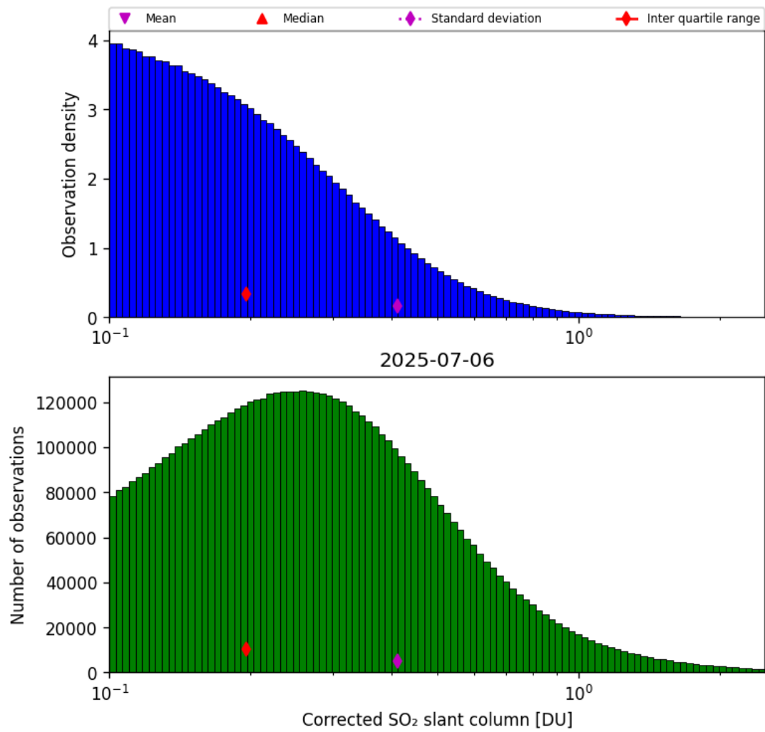
Figure 60: Histogram of “Corrected SO 2 slant column” for 2025-07-06 to 2025-07-06
