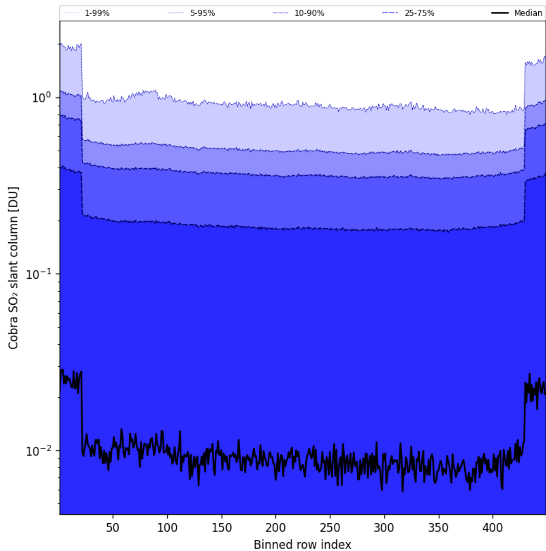
Figure 88: Along track statistics of “Cobra SO 2 slant column” for 2025-07-06 to 2025-07-06
