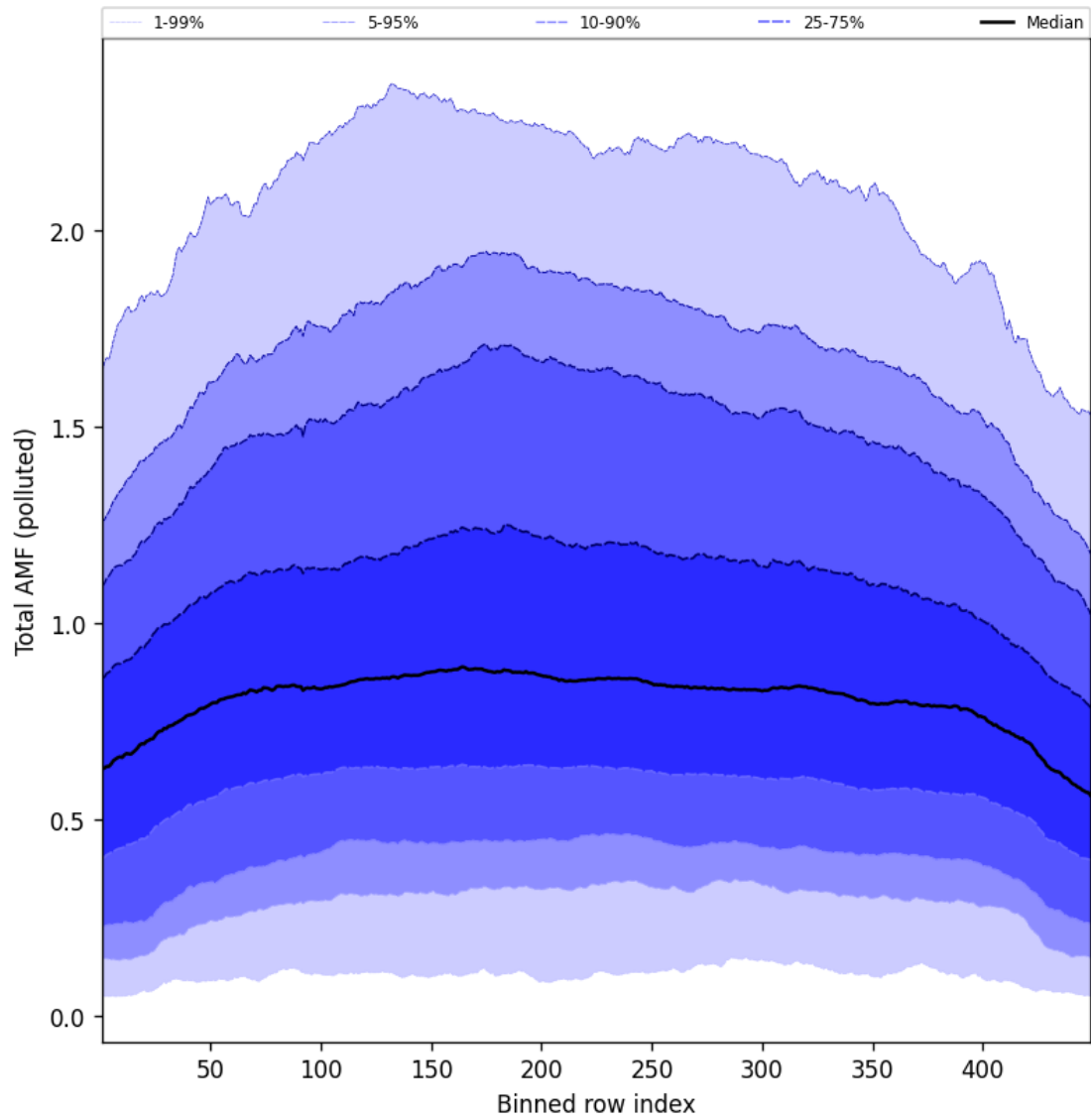
Figure 107: Along track statistics of “Total AMF (polluted)” for 2025-07-06 to 2025-07-06
