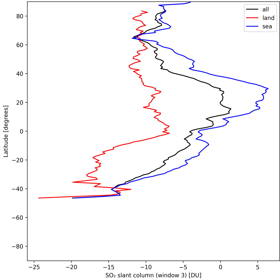
Figure 44: Zonal average of “SO 2 slant column (window 3)” for 2025-07-06 to 2025-07-06.
