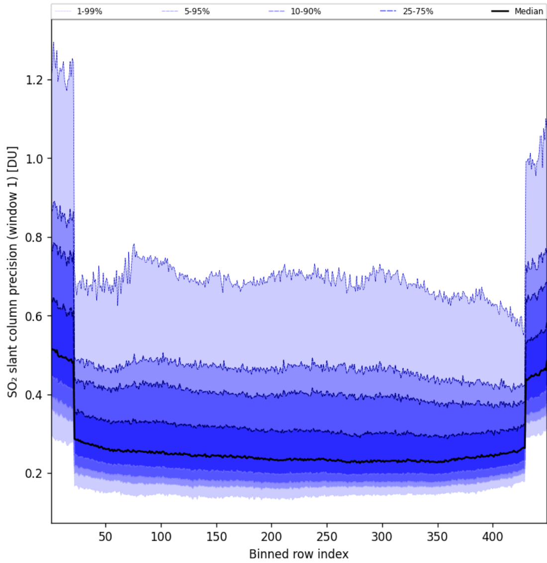
Figure 91: Along track statistics of “SO 2 slant column precision (window 1)” for 2025-07-06 to 2025-07-06
