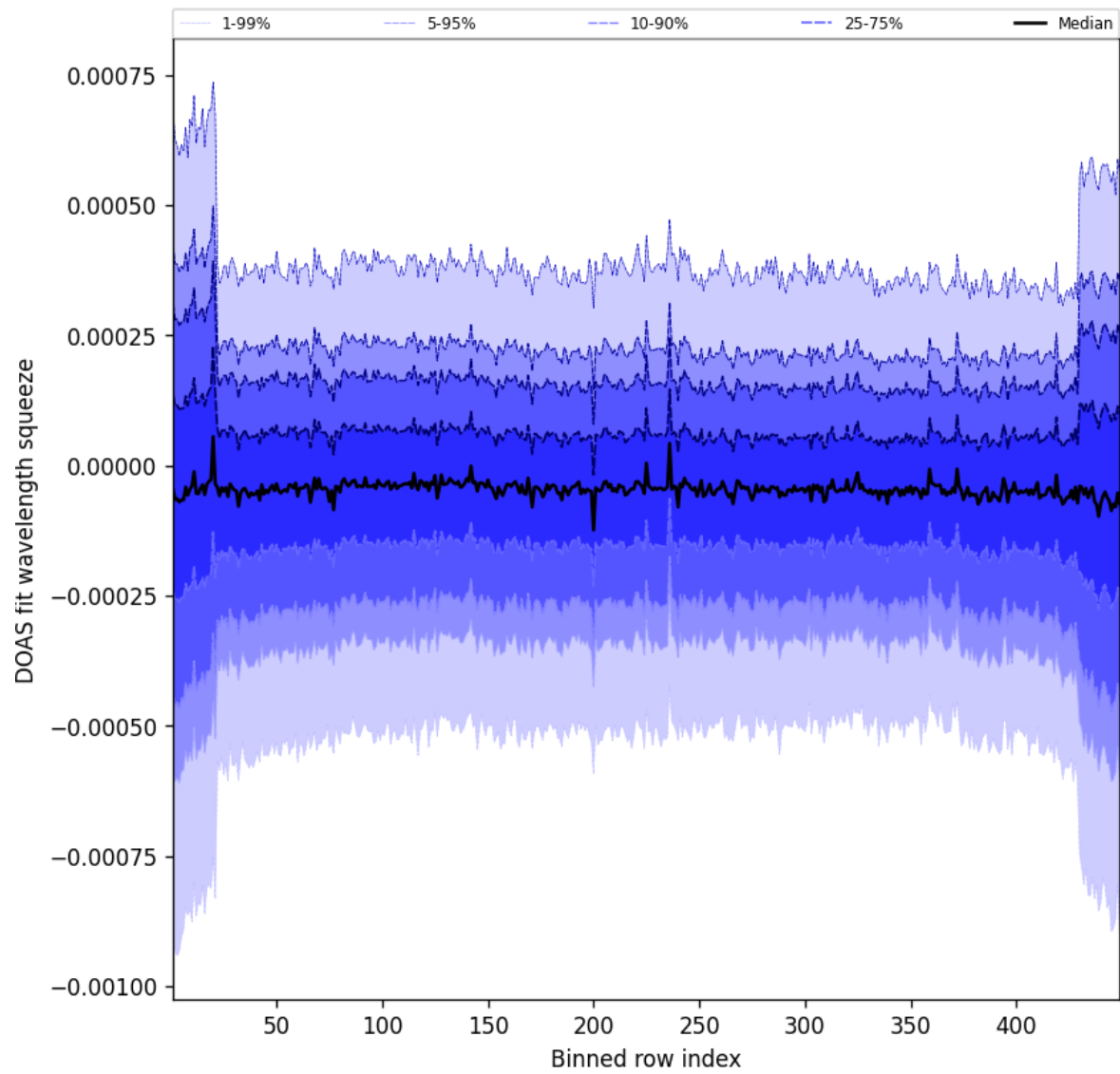
Figure 105: Along track statistics of “DOAS fit wavelength squeeze” for 2025-07-06 to 2025-07-06
