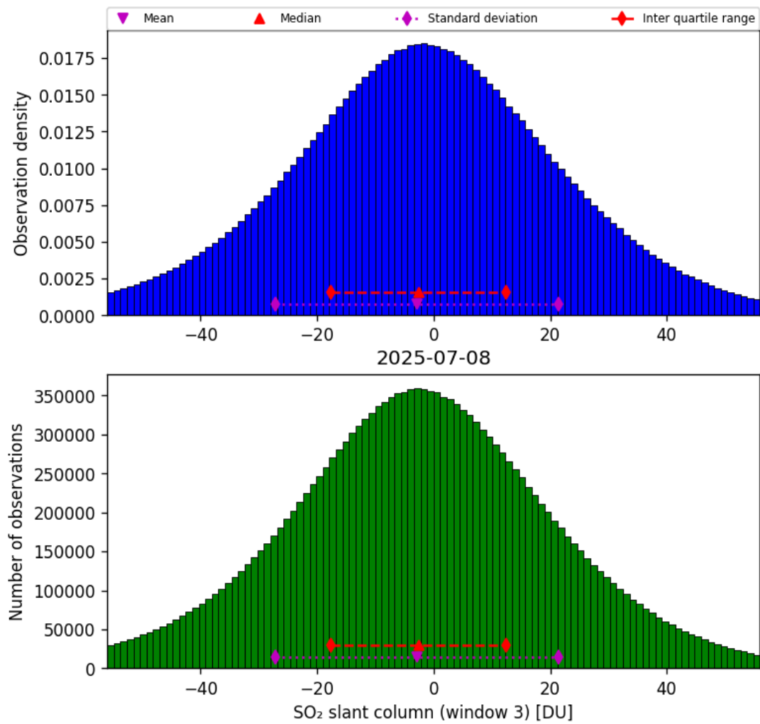
Figure 71: Histogram of “SO 2 slant column (window 3)” for 2025-07-08 to 2025-07-09
