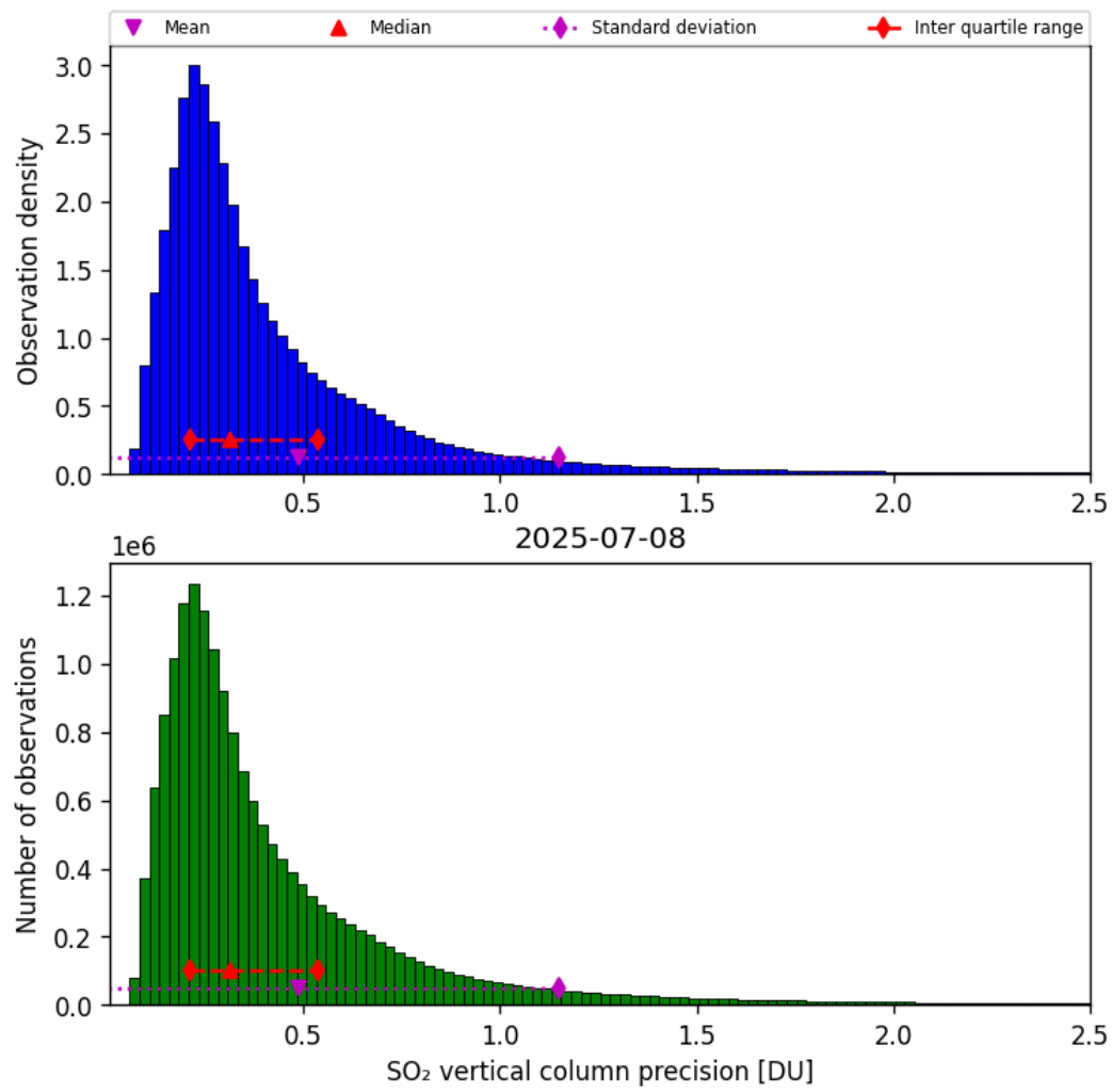
Figure 59: Histogram of “SO 2 vertical column precision” for 2025-07-08 to 2025-07-09
