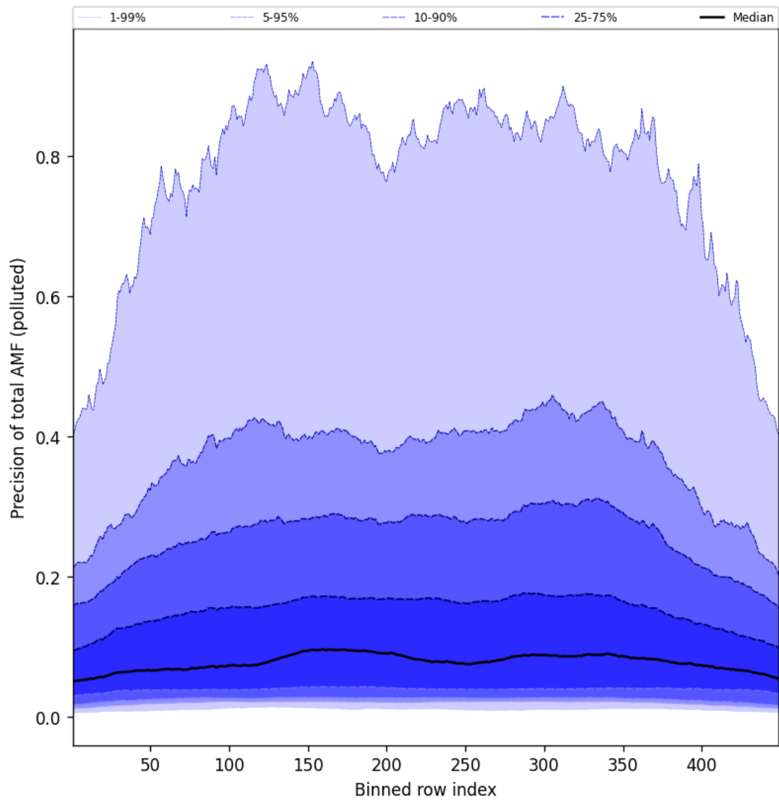
Figure 108: Along track statistics of “Precision of total AMF (polluted)” for 2025-07-08 to 2025-07-09
