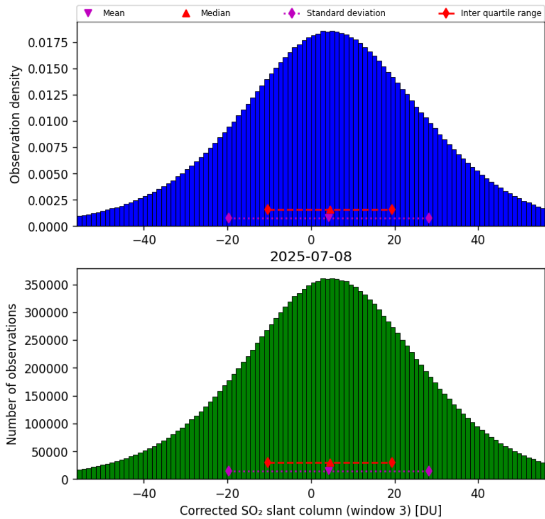
Figure 73: Histogram of “Corrected SO 2 slant column (window 3)” for 2025-07-08 to 2025-07-09
