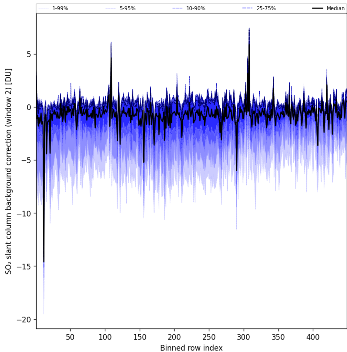
Figure 97: Along track statistics of “SO 2 slant column background correction (window 2)” for 2025-07-08 to 2025-07-09
