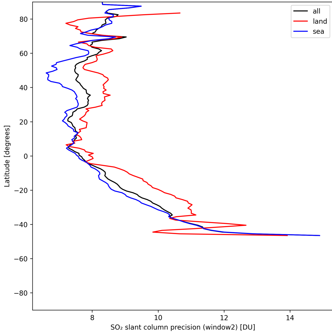
Figure 41: Zonal average of “SO 2 slant column precision (window2)” for 2025-07-08 to 2025-07-09.
