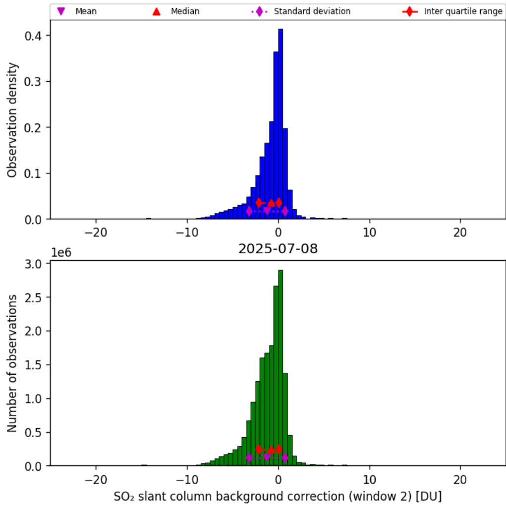
Figure 70: Histogram of “SO 2 slant column background correction (window 2)” for 2025-07-08 to 2025-07-09
