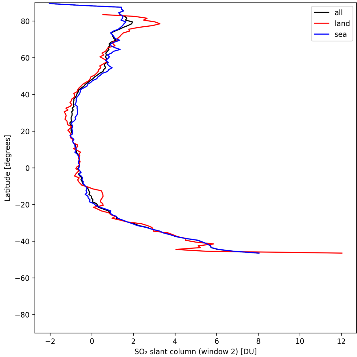
Figure 40: Zonal average of “SO 2 slant column (window 2)” for 2025-07-08 to 2025-07-09.
