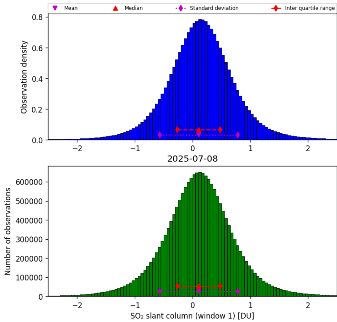
Figure 63: Histogram of “SO 2 slant column (window 1)” for 2025-07-08 to 2025-07-09
