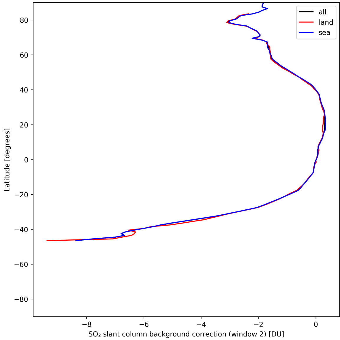
Figure 43: Zonal average of “SO 2 slant column background correction (window 2)” for 2025-07-08 to 2025-07-09.
