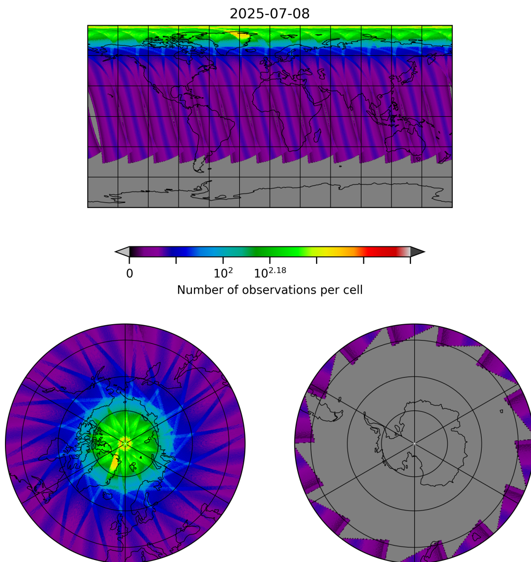
Figure 29: Map of the number of observations for 2025-07-08 to 2025-07-09
