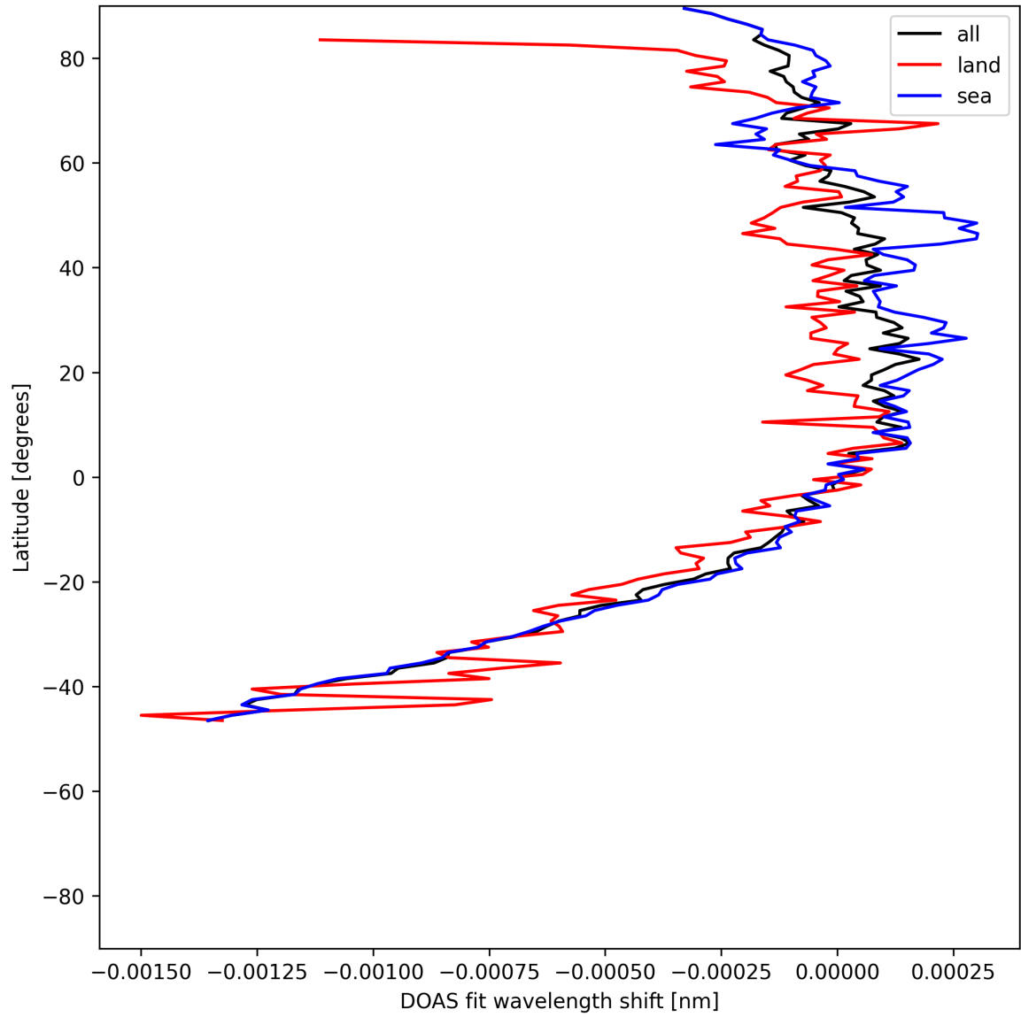
Figure 50: Zonal average of "DOAS fit wavelength shift" for 2025-07-08 to 2025-07-09.
