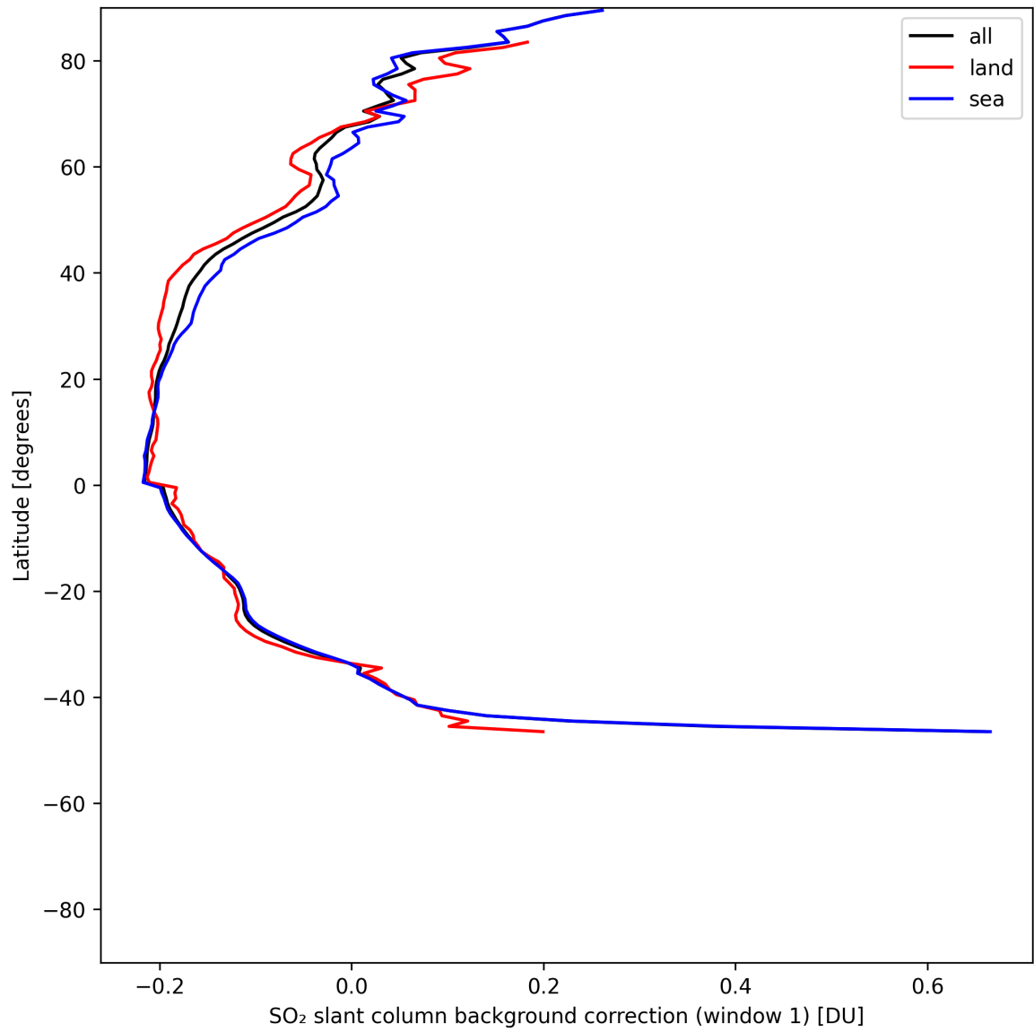
Figure 39: Zonal average of “SO 2 slant column background correction (window 1)” for 2025-07-08 to 2025-07-09.
