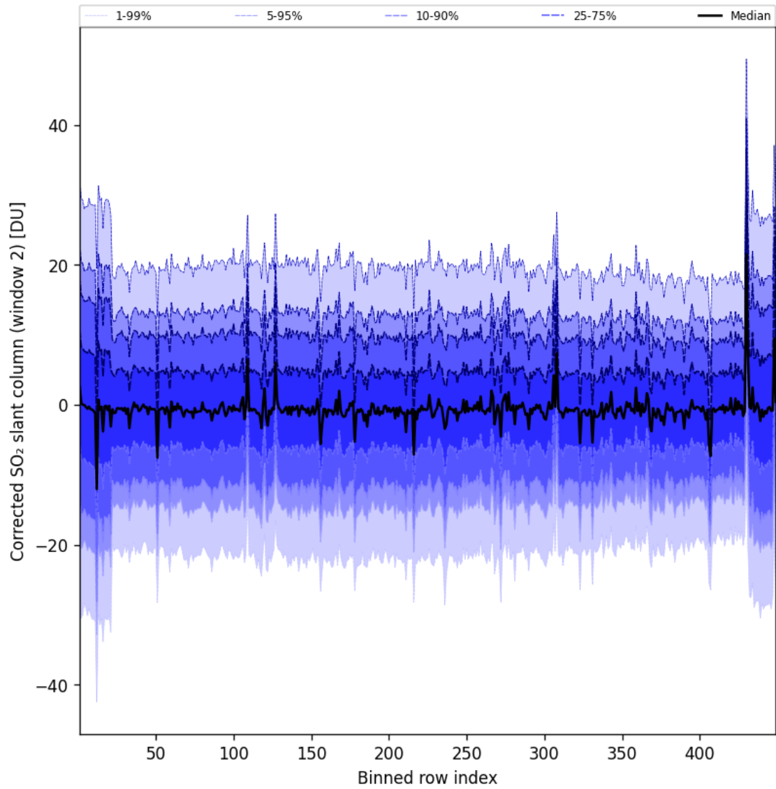
Figure 96: Along track statistics of “Corrected SO 2 slant column (window 2)” for 2025-07-08 to 2025-07-09
