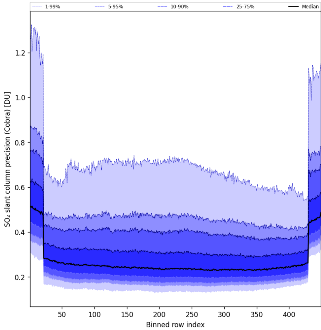
Figure 89: Along track statistics of “SO 2 slant column precision (Cobra)” for 2025-07-08 to 2025-07-09
