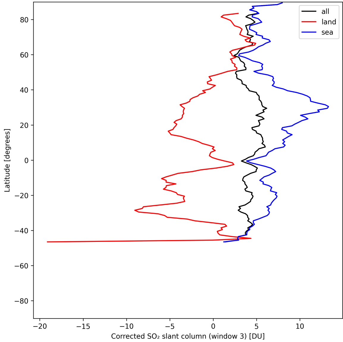
Figure 46: Zonal average of “Corrected SO 2 slant column (window 3)” for 2025-07-08 to 2025-07-09.
