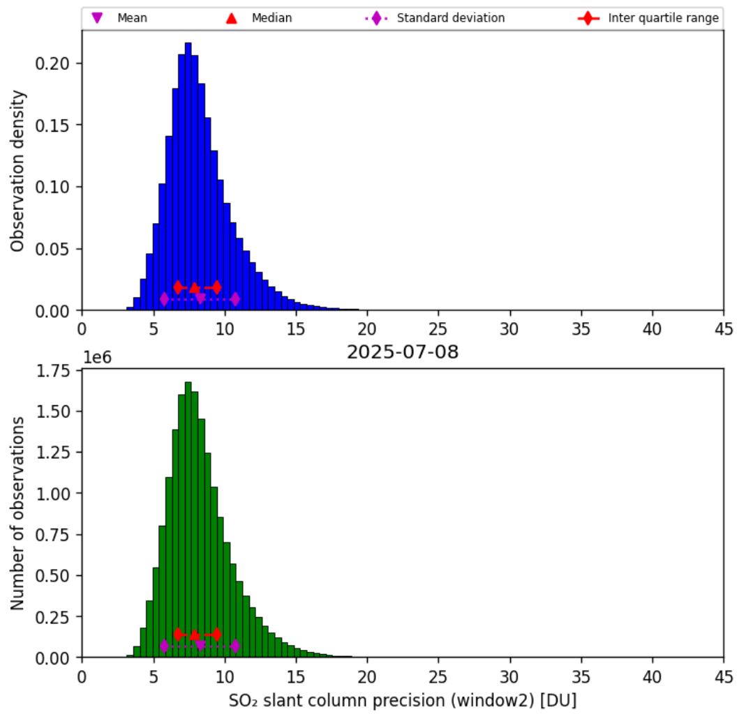
Figure 68: Histogram of “SO 2 slant column precision (window2)” for 2025-07-08 to 2025-07-09
