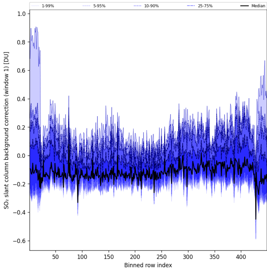
Figure 93: Along track statistics of “SO 2 slant column background correction (window 1)” for 2025-07-08 to 2025-07-09
