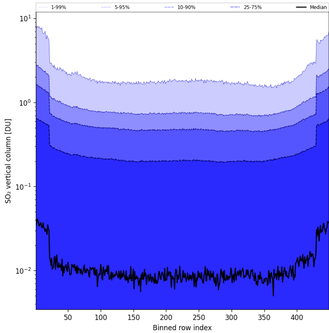
Figure 85: Along track statistics of “SO 2 vertical column” for 2025-07-08 to 2025-07-09
