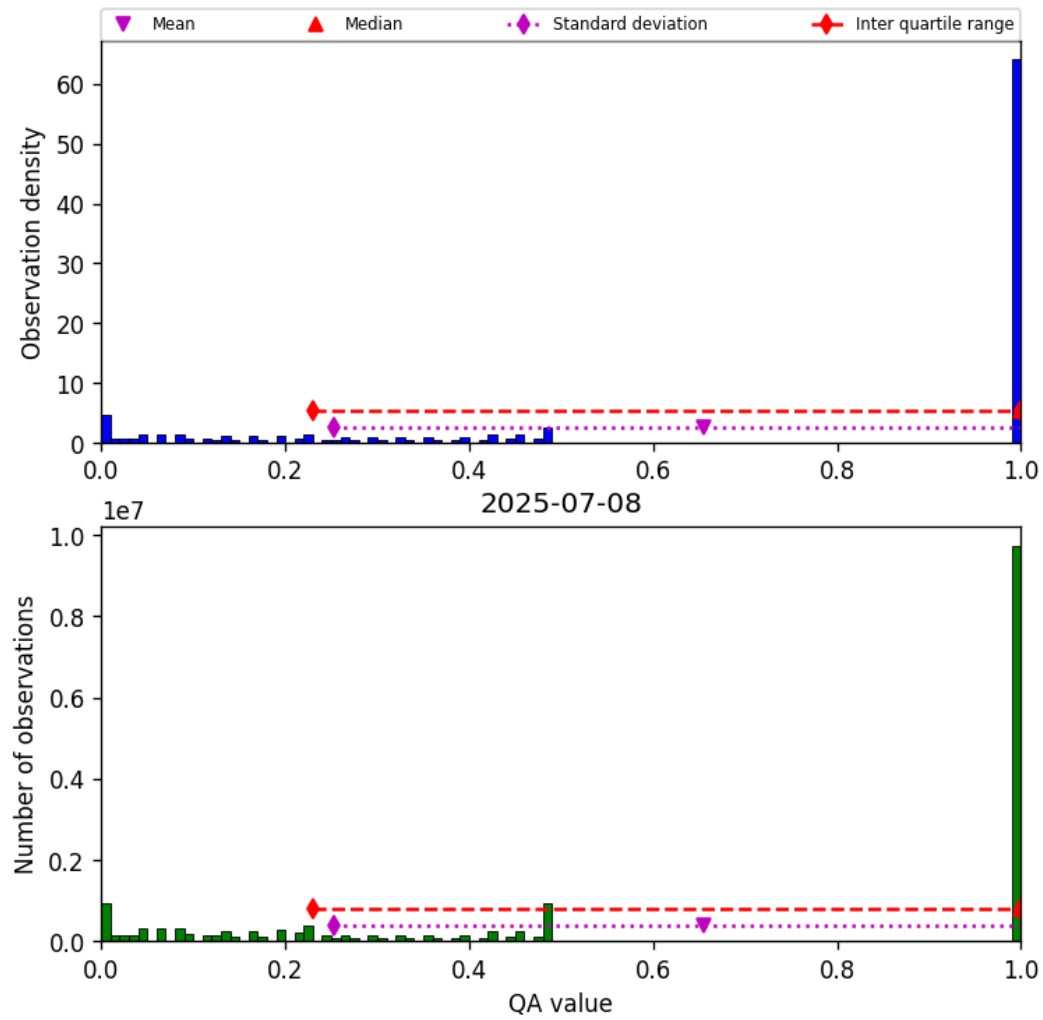
Figure 57: Histogram of “QA value” for 2025-07-08 to 2025-07-09
