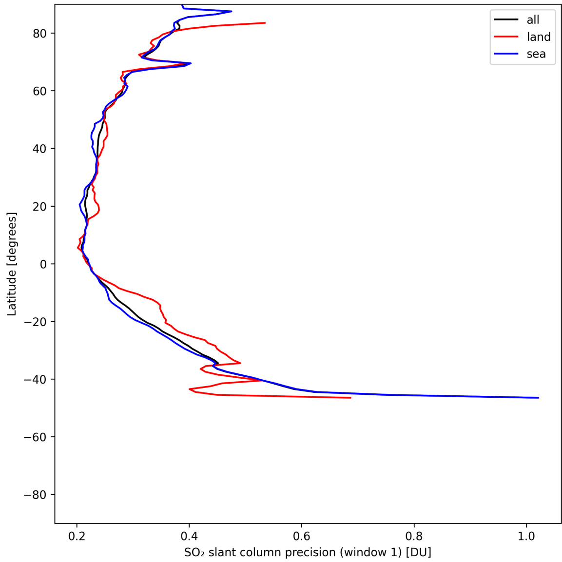
Figure 37: Zonal average of “SO 2 slant column precision (window 1)” for 2025-07-08 to 2025-07-09.
