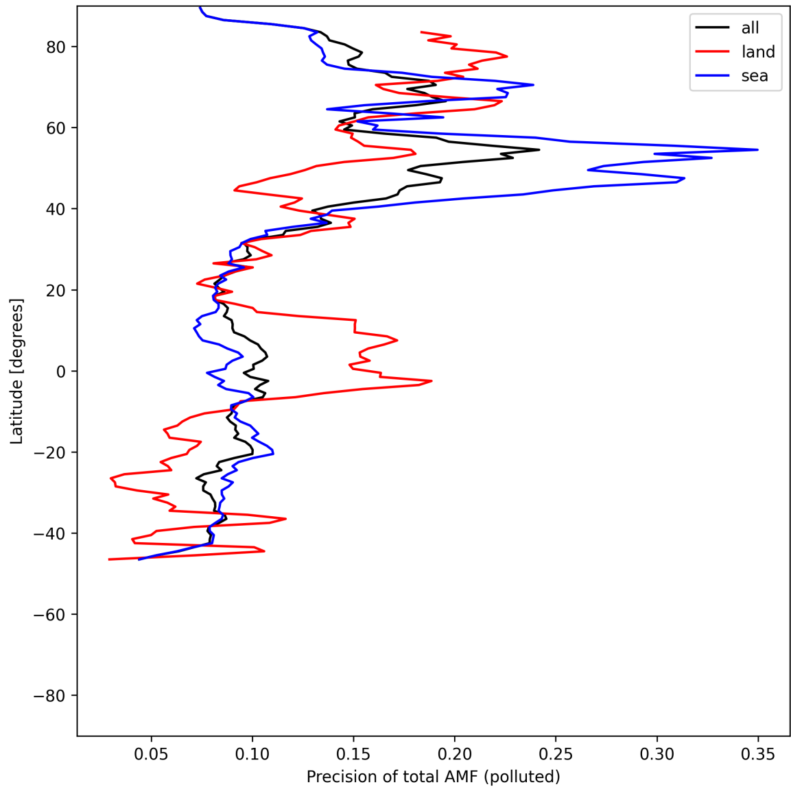
Figure 54: Zonal average of “Precision of total AMF (polluted)” for 2025-07-08 to 2025-07-09.
