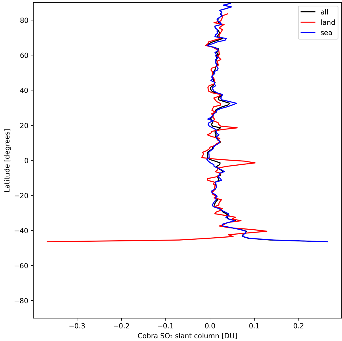
Figure 34: Zonal average of “Cobra SO 2 slant column” for 2025-07-08 to 2025-07-09.
