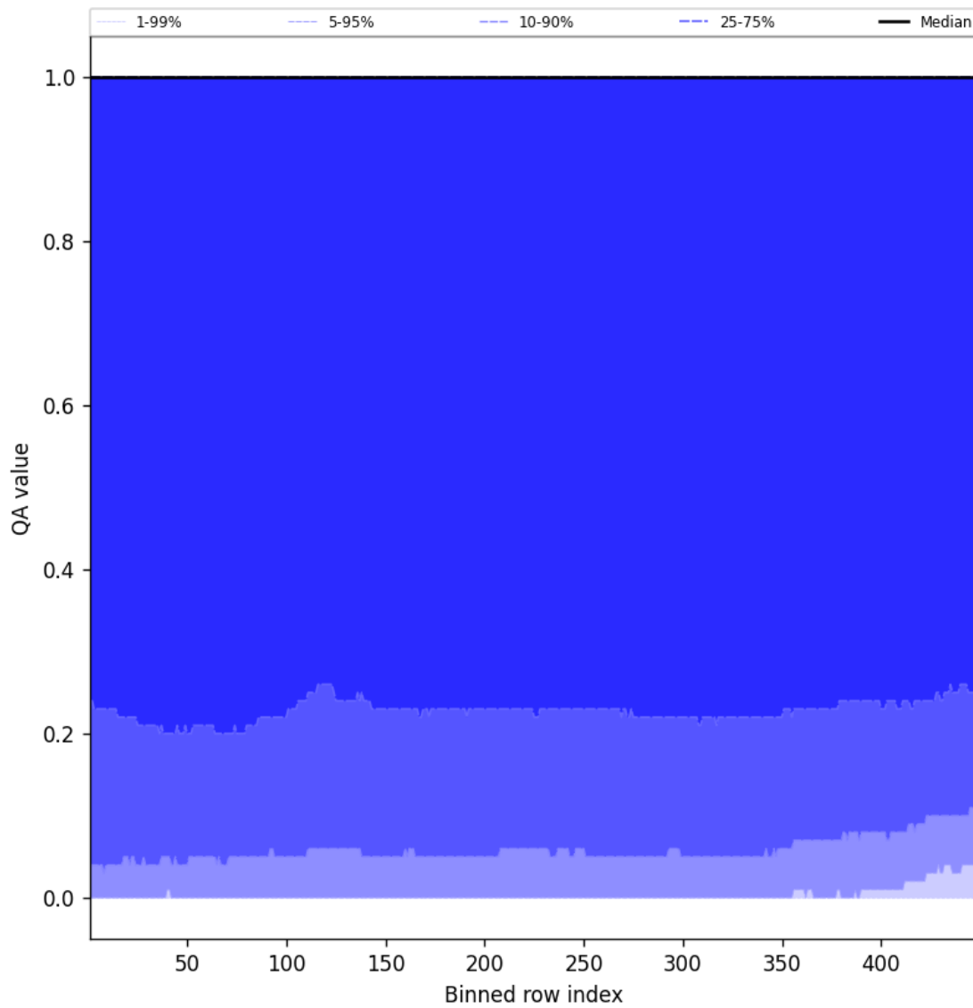
Figure 84: Along track statistics of “QA value” for 2025-07-08 to 2025-07-09
