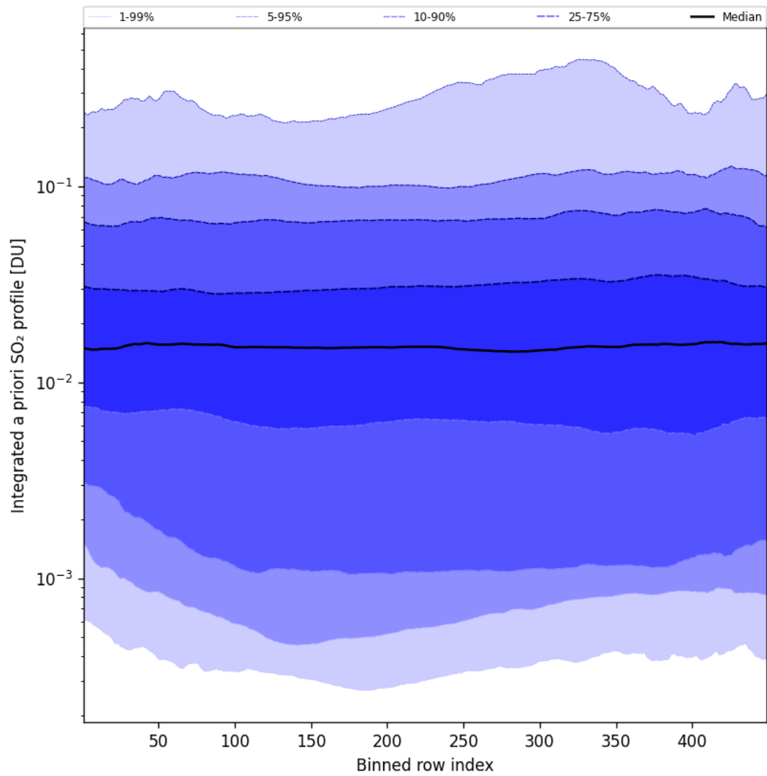
Figure 103: Along track statistics of “Integrated a priori SO 2 profile” for 2025-07-08 to 2025-07-09
