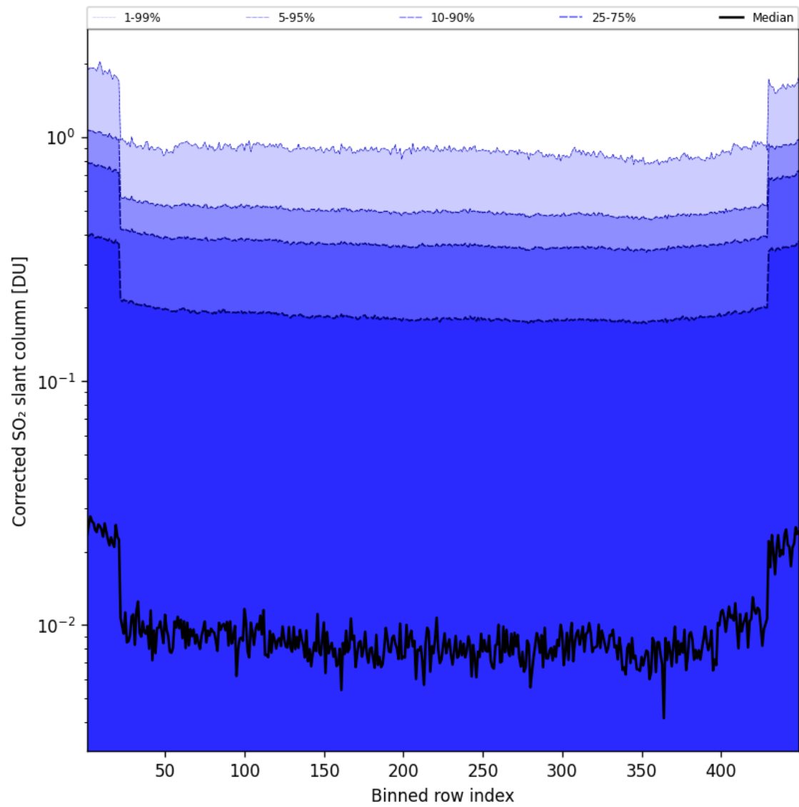
Figure 87: Along track statistics of “Corrected SO 2 slant column” for 2025-07-08 to 2025-07-09
