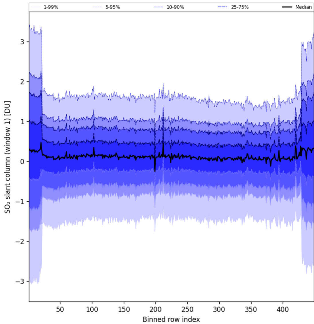
Figure 90: Along track statistics of “SO 2 slant column (window 1)” for 2025-07-08 to 2025-07-09
