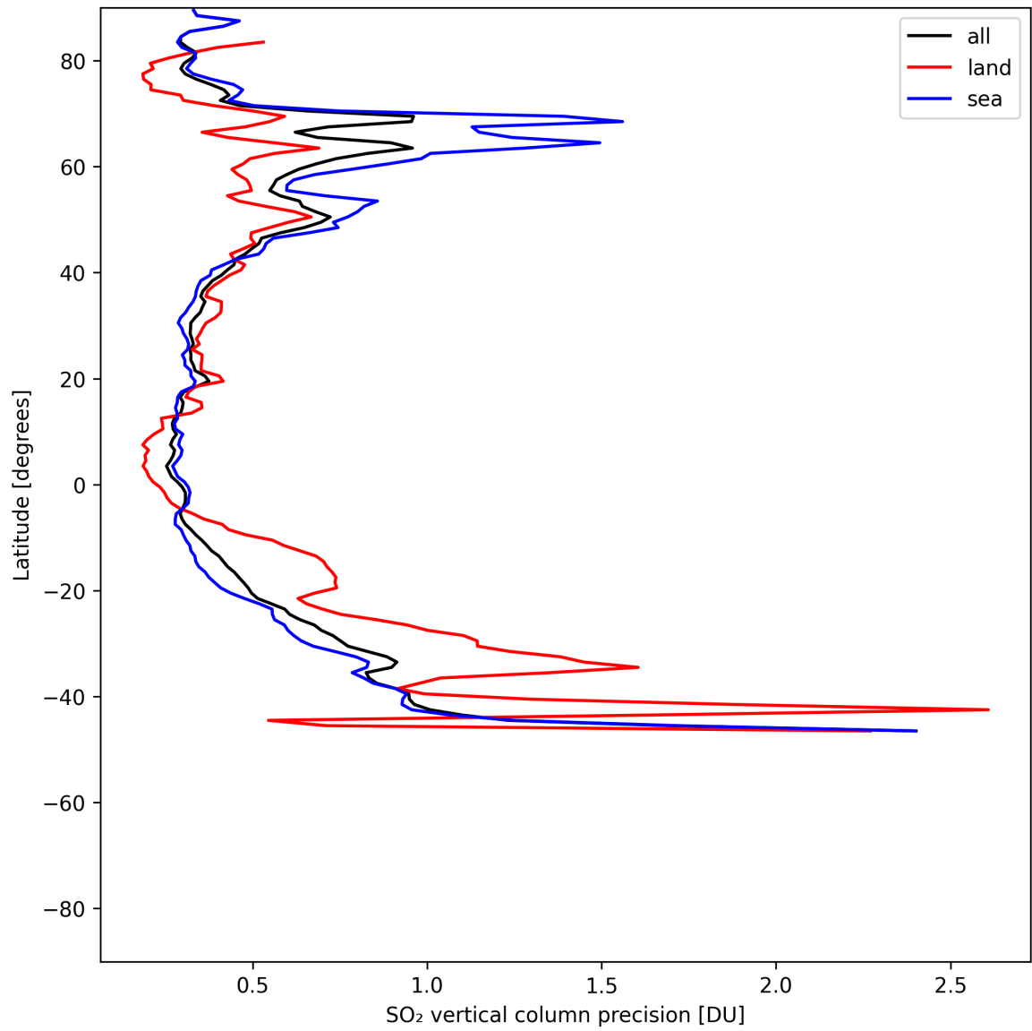
Figure 32: Zonal average of “SO 2 vertical column precision” for 2025-07-08 to 2025-07-09.
