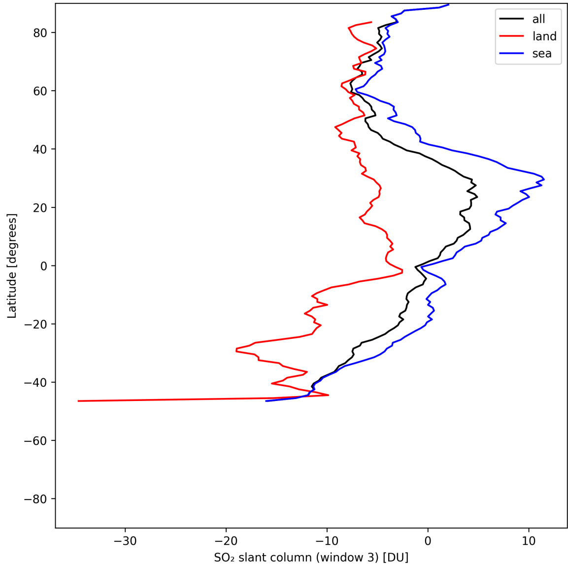
Figure 44: Zonal average of “SO 2 slant column (window 3)” for 2025-07-08 to 2025-07-09.
