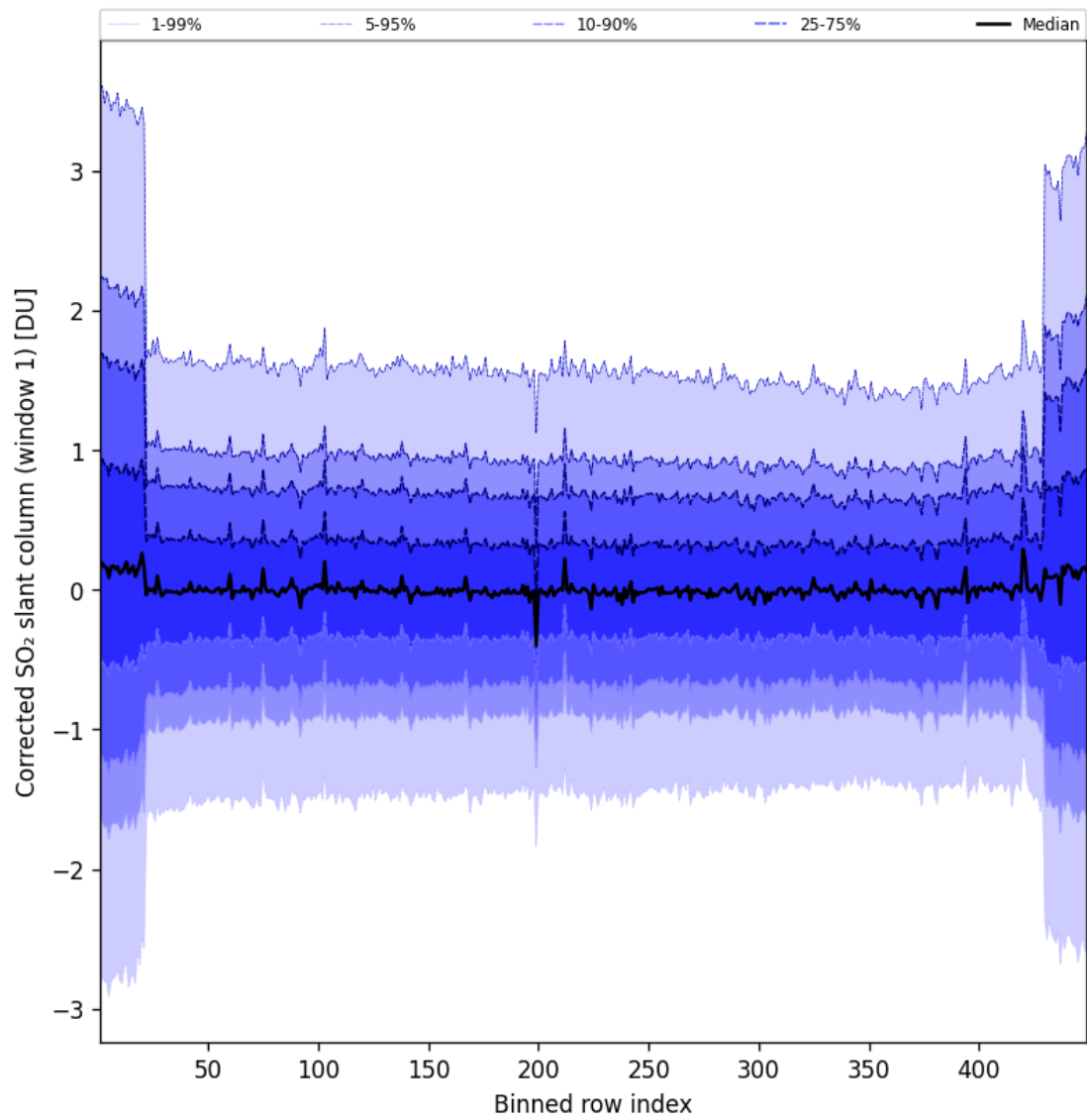
Figure 92: Along track statistics of “Corrected SO 2 slant column (window 1)” for 2025-07-08 to 2025-07-09
