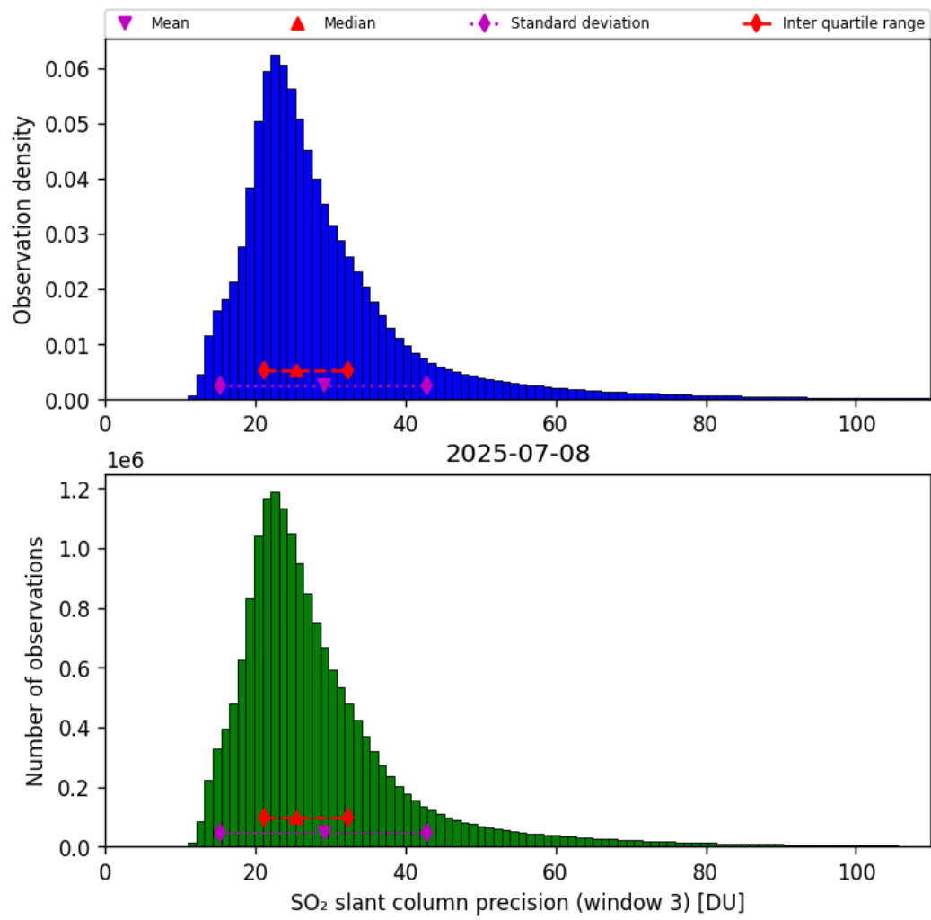
Figure 72: Histogram of “SO 2 slant column precision (window 3)” for 2025-07-08 to 2025-07-09
