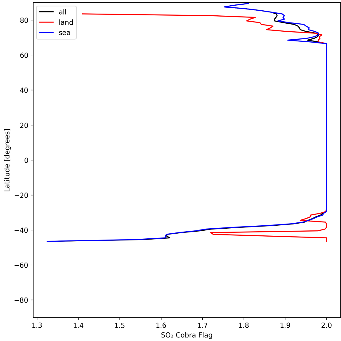
Figure 48: Zonal average of "SO 2 Cobra Flag" for 2025-07-08 to 2025-07-09.
