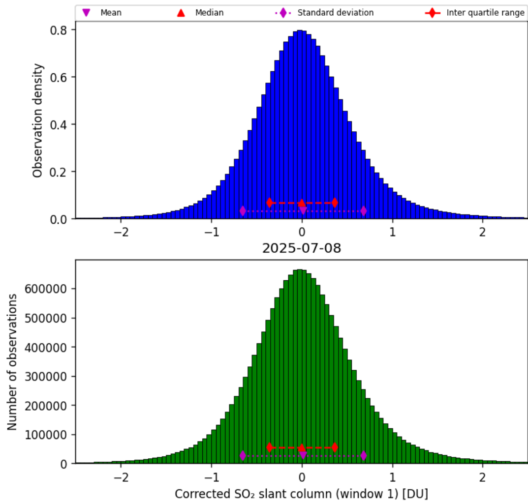
Figure 65: Histogram of “Corrected SO 2 slant column (window 1)” for 2025-07-08 to 2025-07-09
