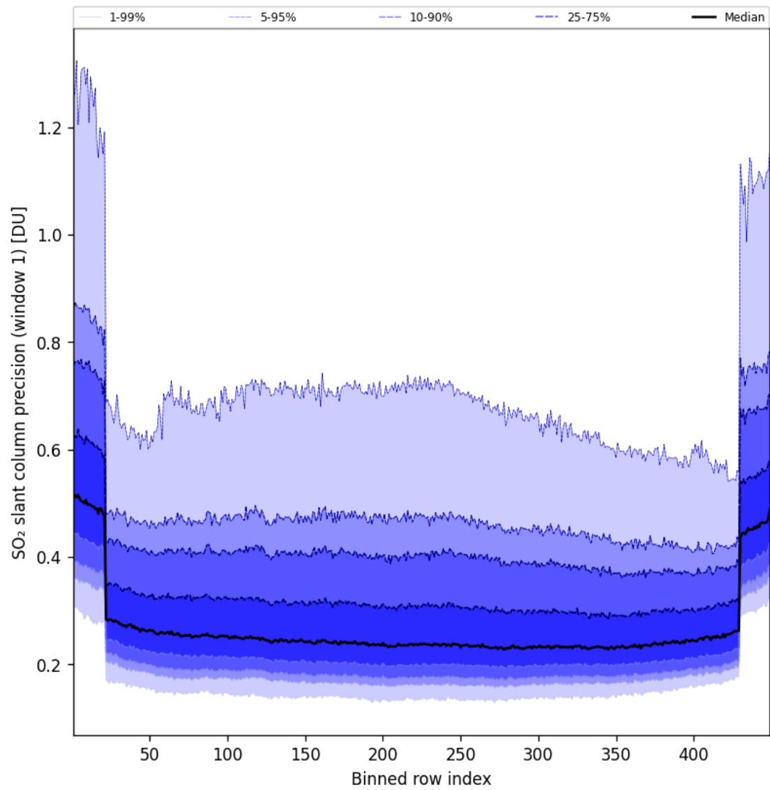
Figure 91: Along track statistics of “SO 2 slant column precision (window 1)” for 2025-07-08 to 2025-07-09
