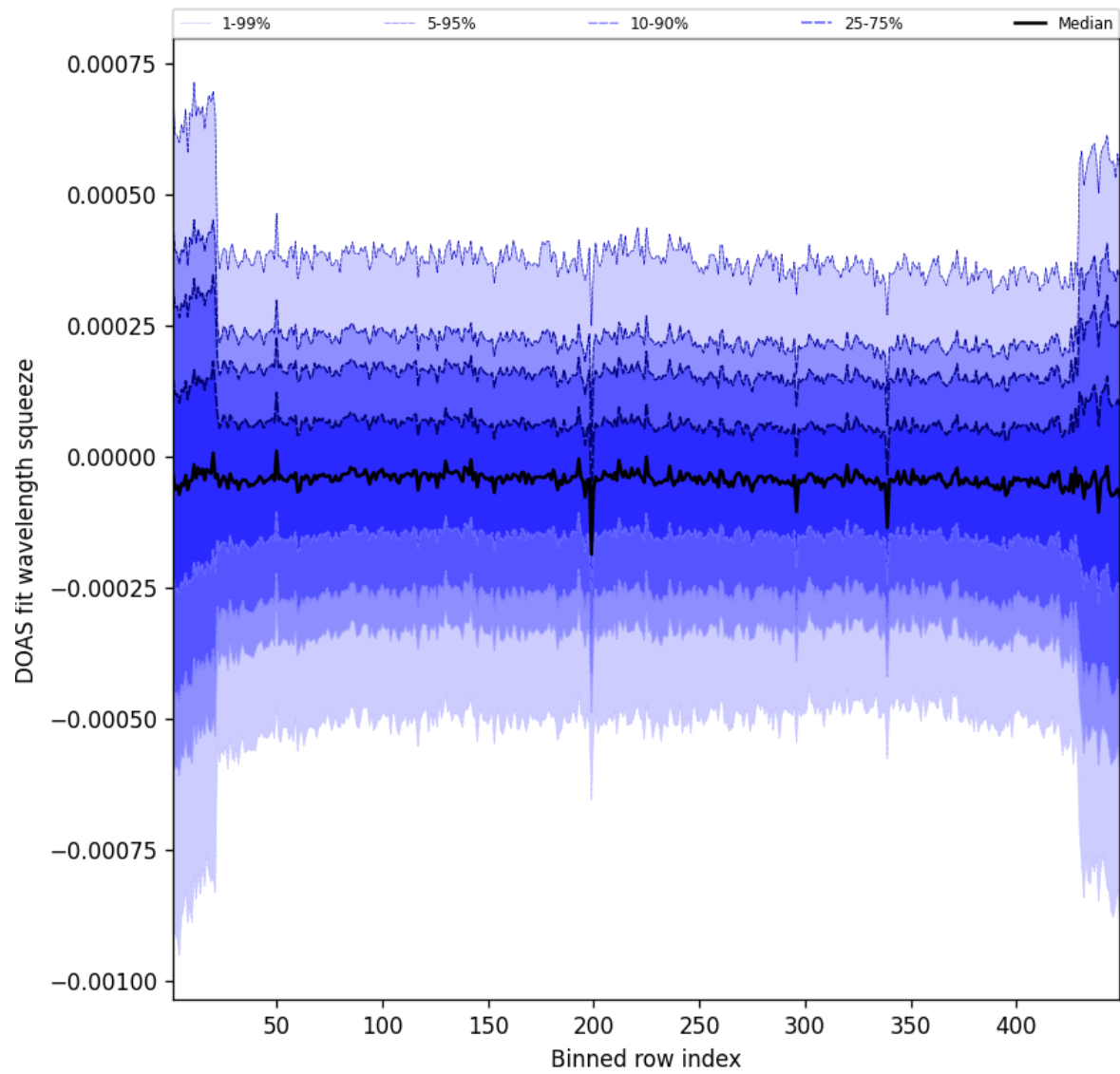
Figure 105: Along track statistics of “DOAS fit wavelength squeeze” for 2025-07-08 to 2025-07-09
