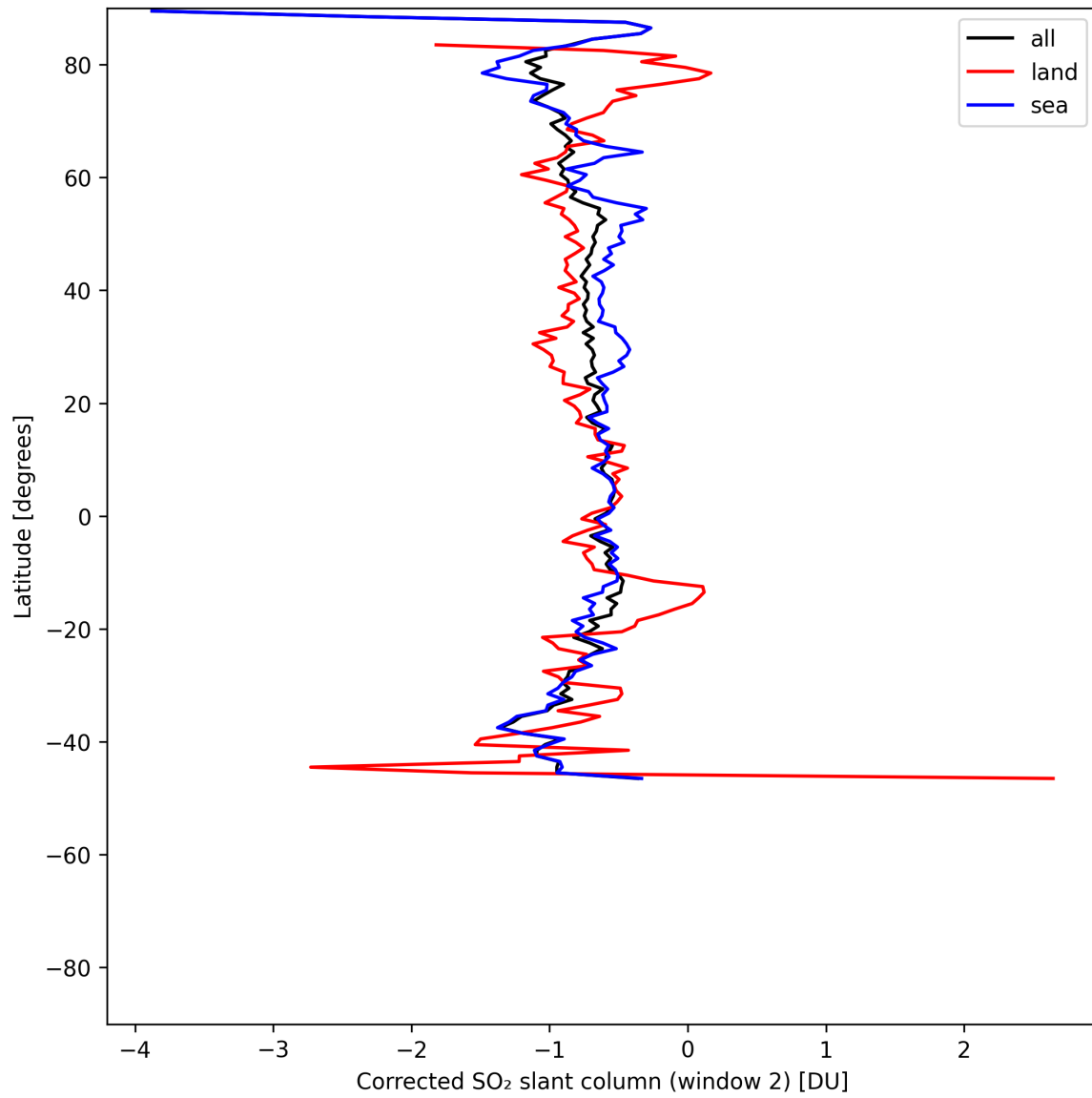
Figure 42: Zonal average of “Corrected SO 2 slant column (window 2)” for 2025-07-08 to 2025-07-09.
