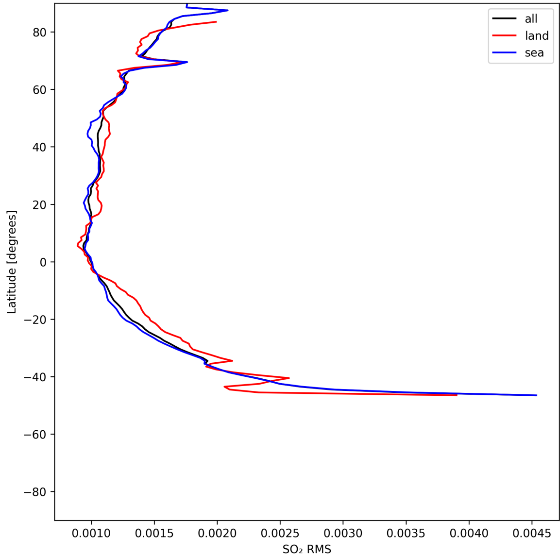
Figure 52: Zonal average of “SO 2 RMS” for 2025-07-08 to 2025-07-09.
