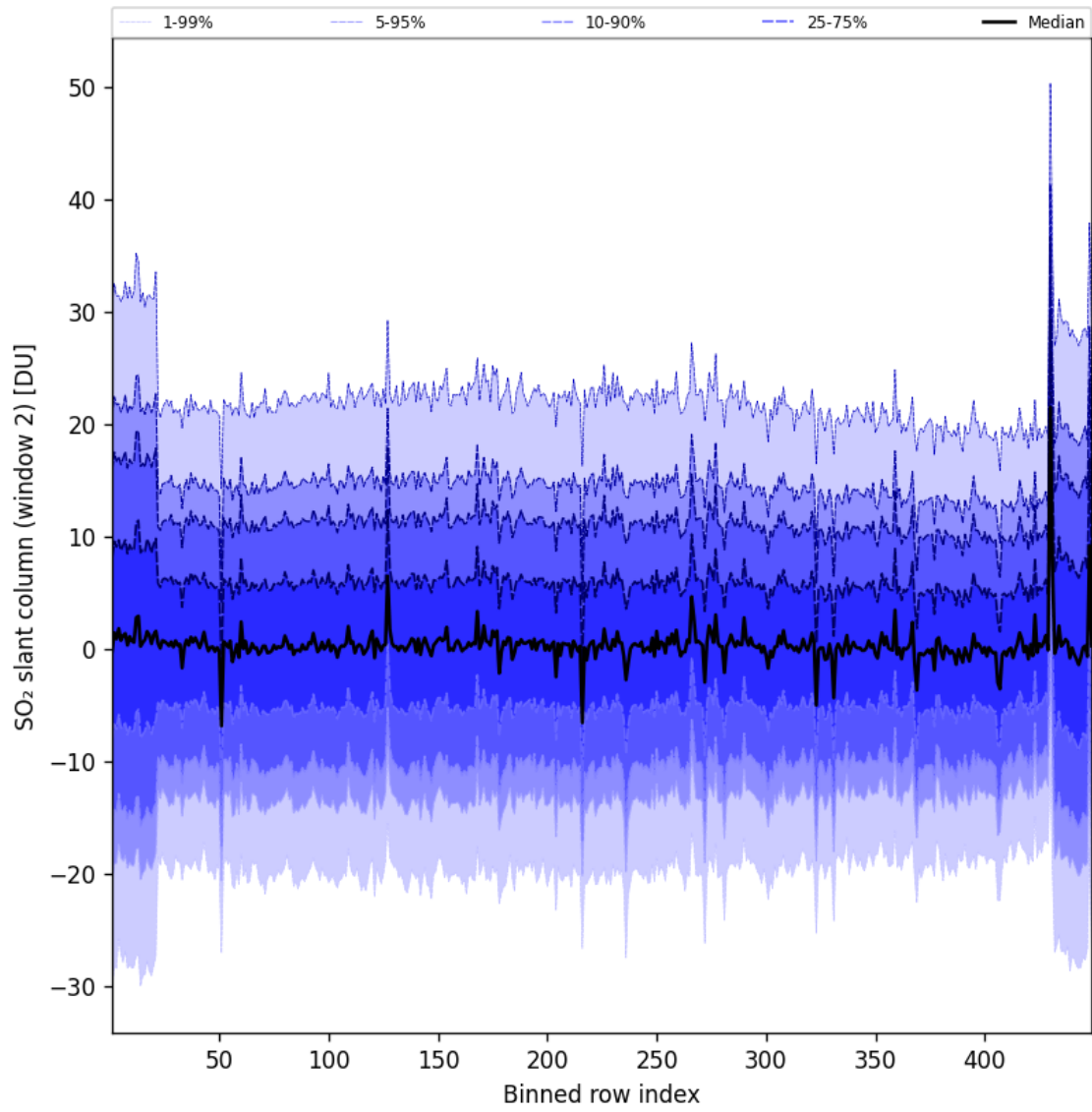
Figure 94: Along track statistics of “SO 2 slant column (window 2)” for 2025-07-08 to 2025-07-09
