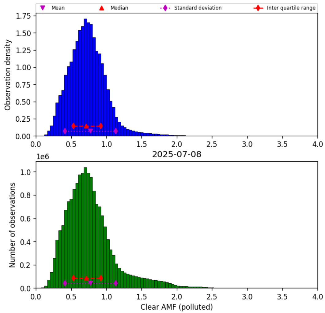
Figure 82: Histogram of “Clear AMF (polluted)” for 2025-07-08 to 2025-07-09
