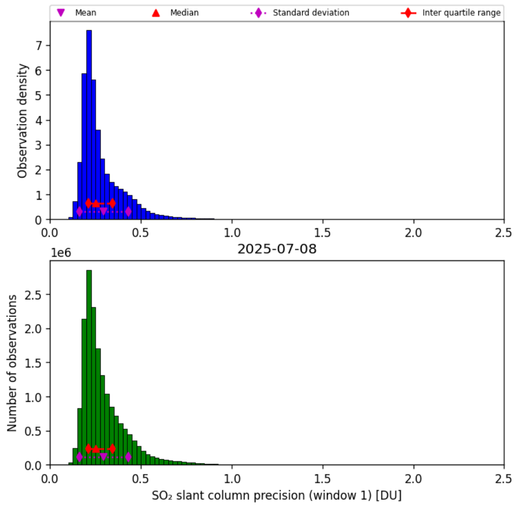
Figure 64: Histogram of “SO 2 slant column precision (window 1)” for 2025-07-08 to 2025-07-09
