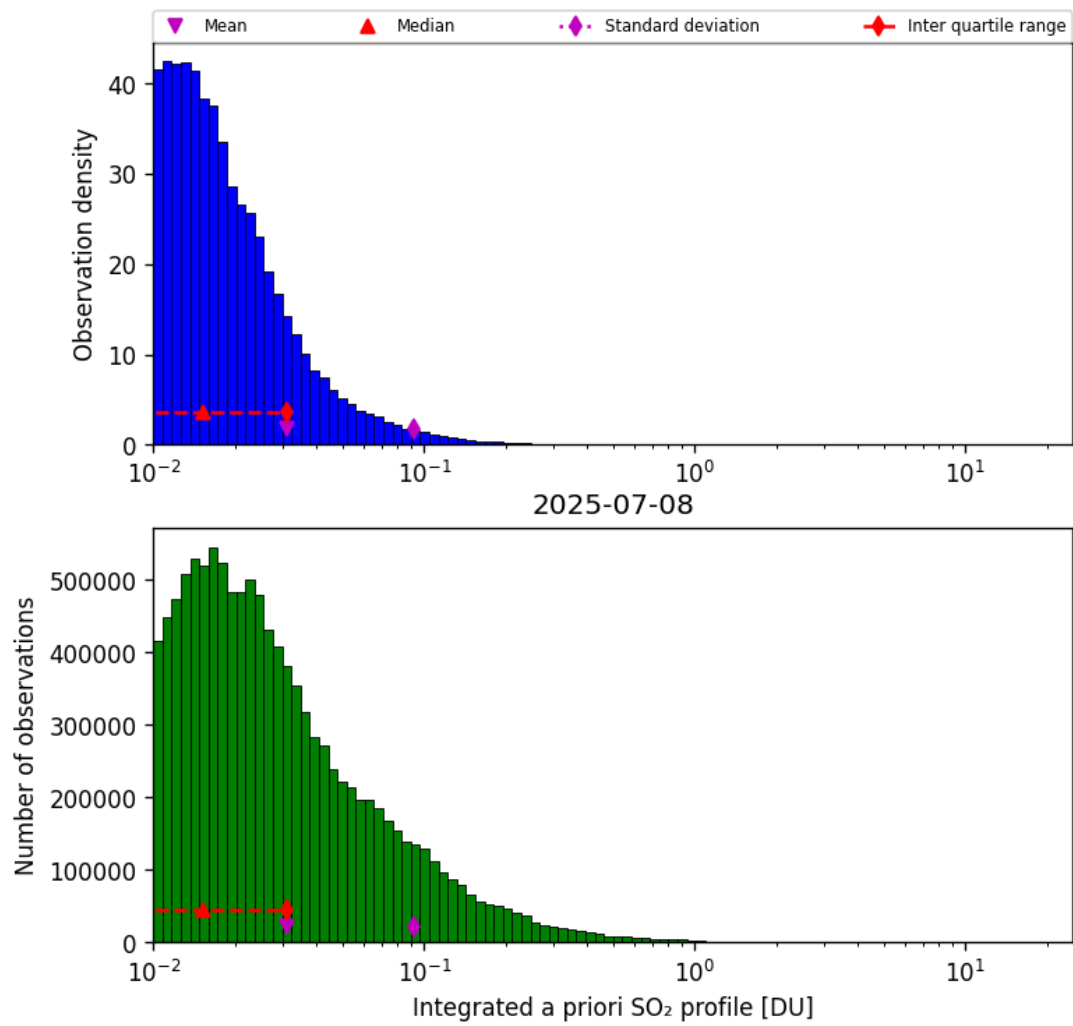
Figure 76: Histogram of “Integrated a priori SO 2 profile” for 2025-07-08 to 2025-07-09
