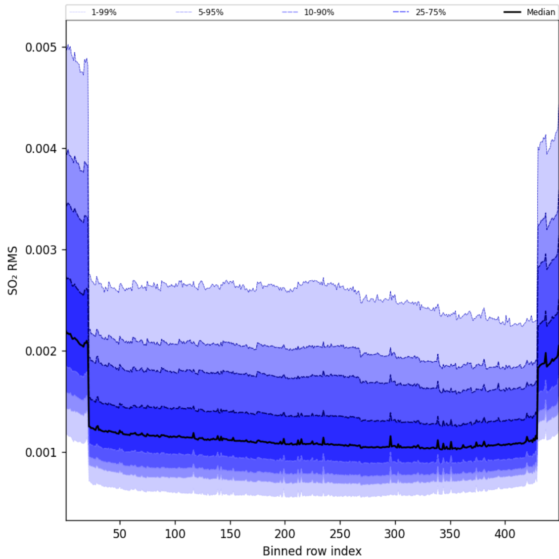
Figure 106: Along track statistics of “SO 2 RMS” for 2025-07-08 to 2025-07-09
