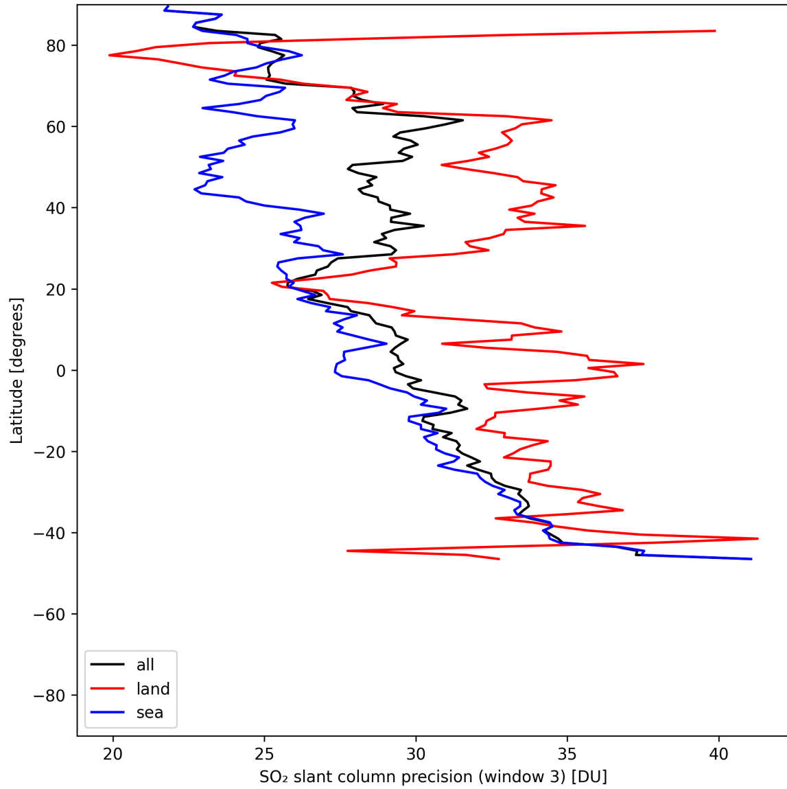
Figure 45: Zonal average of “SO 2 slant column precision (window 3)” for 2025-07-08 to 2025-07-09.
