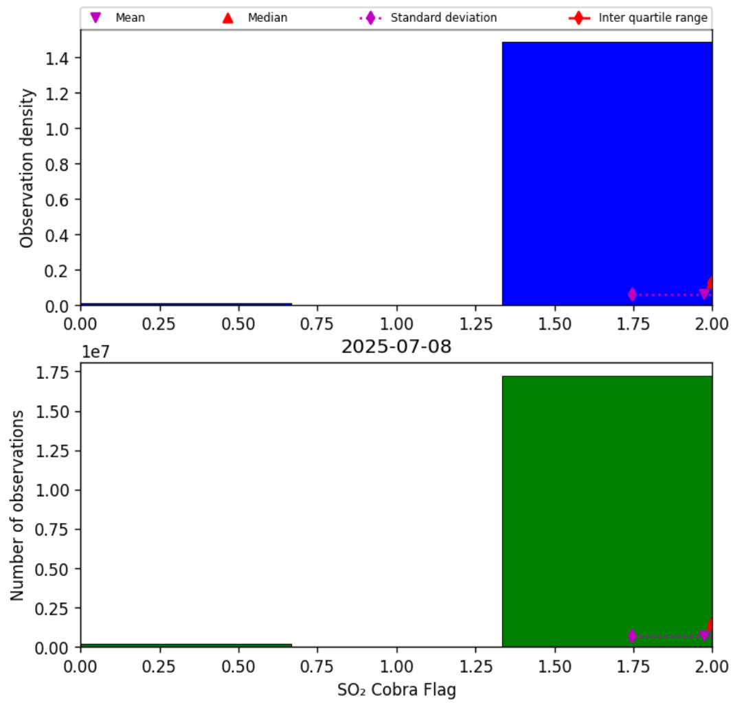
Figure 75: Histogram of “SO 2 Cobra Flag” for 2025-07-08 to 2025-07-09
