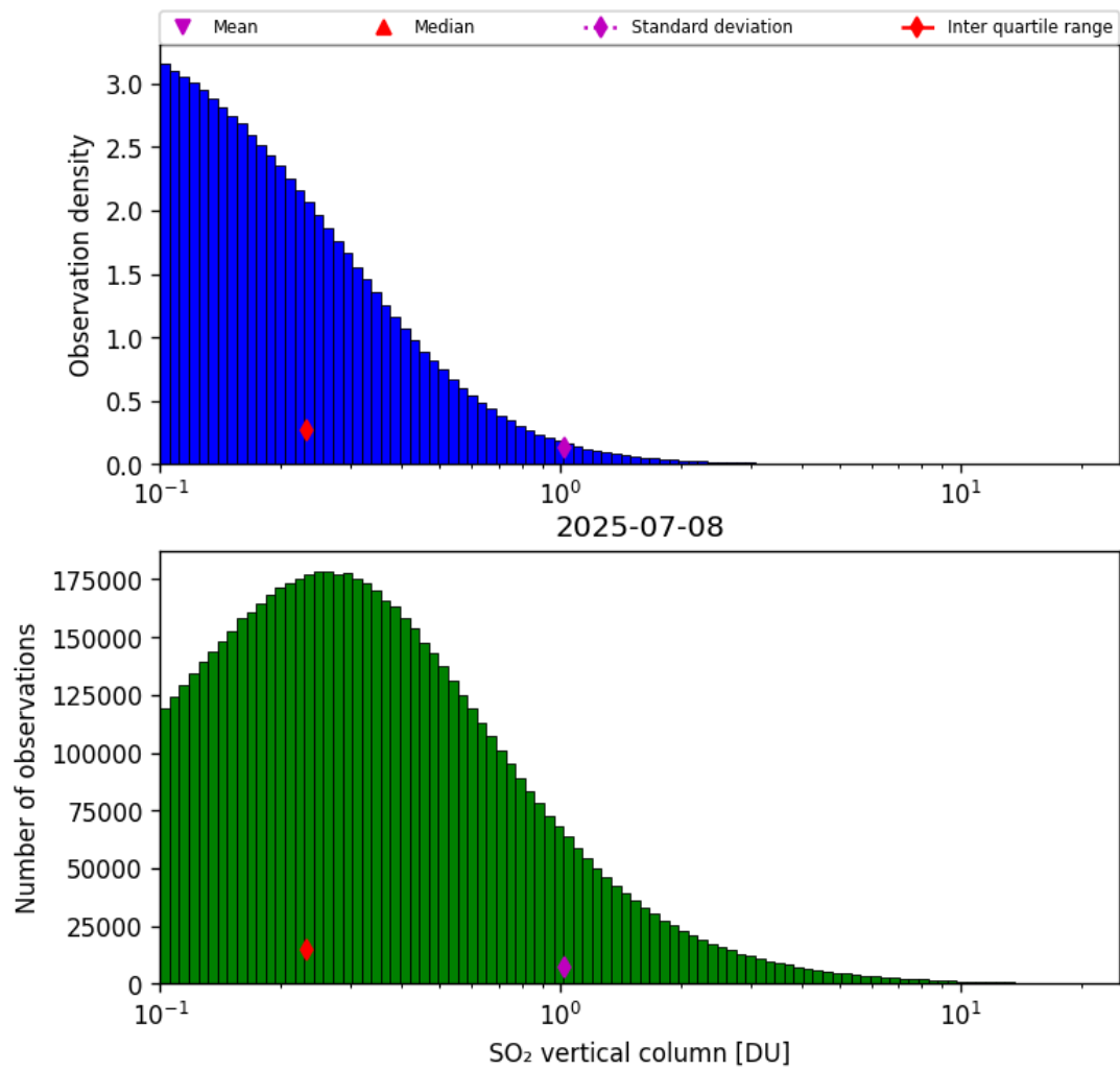
Figure 58: Histogram of “SO 2 vertical column” for 2025-07-08 to 2025-07-09
