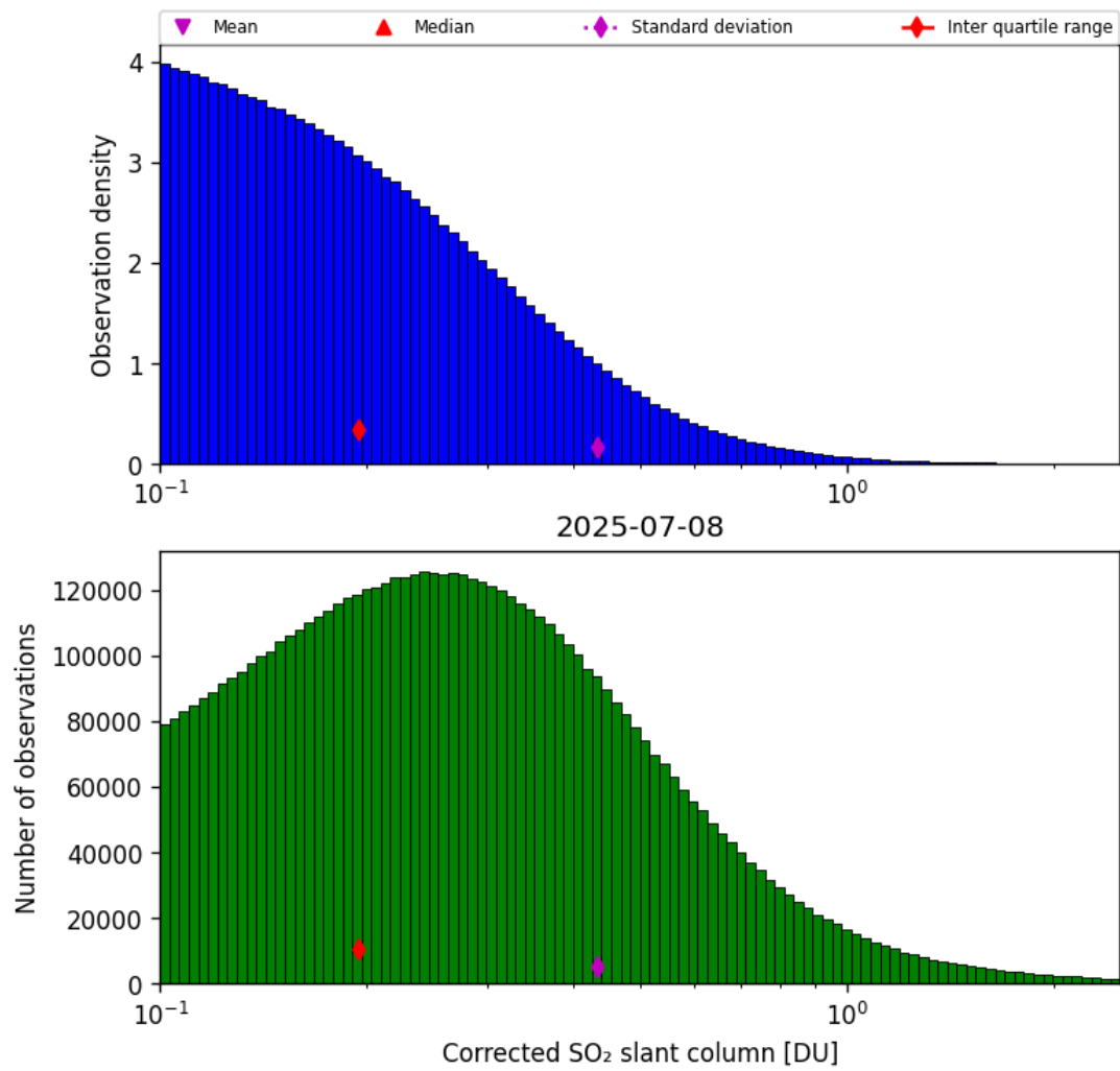
Figure 60: Histogram of “Corrected SO 2 slant column” for 2025-07-08 to 2025-07-09
