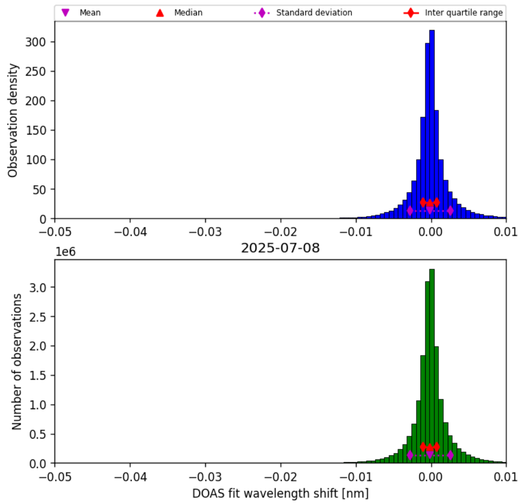
Figure 77: Histogram of “DOAS fit wavelength shift” for 2025-07-08 to 2025-07-09
