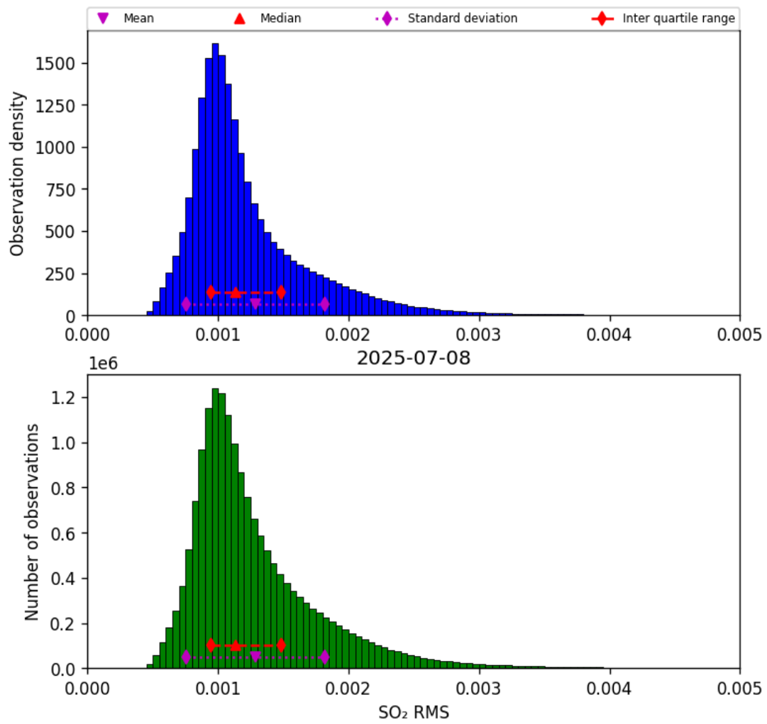
Figure 79: Histogram of “SO 2 RMS” for 2025-07-08 to 2025-07-09
