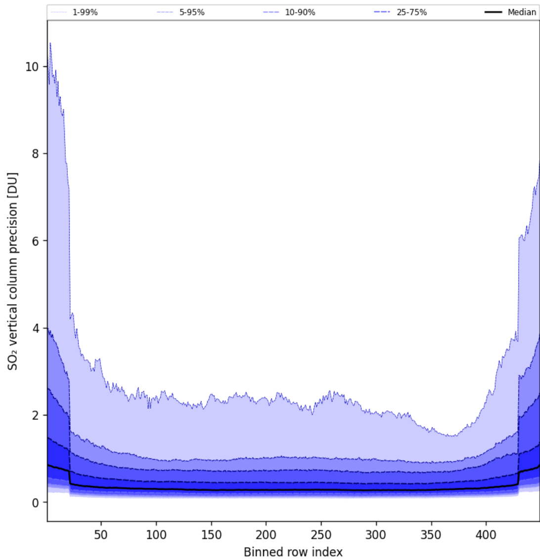
Figure 86: Along track statistics of “SO 2 vertical column precision” for 2025-07-08 to 2025-07-09
