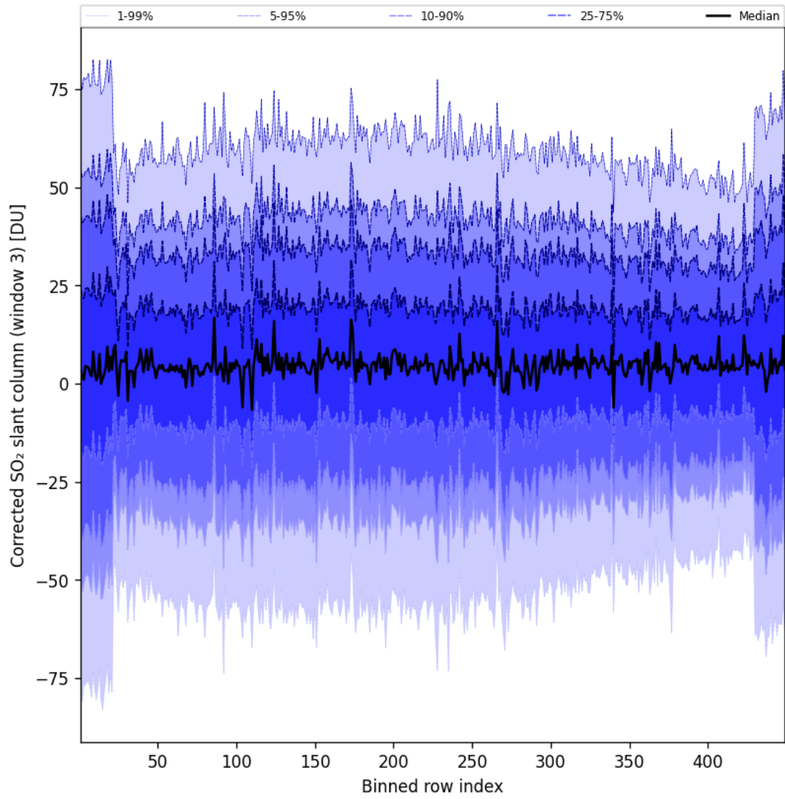
Figure 100: Along track statistics of “Corrected SO 2 slant column (window 3)” for 2025-07-08 to 2025-07-09
