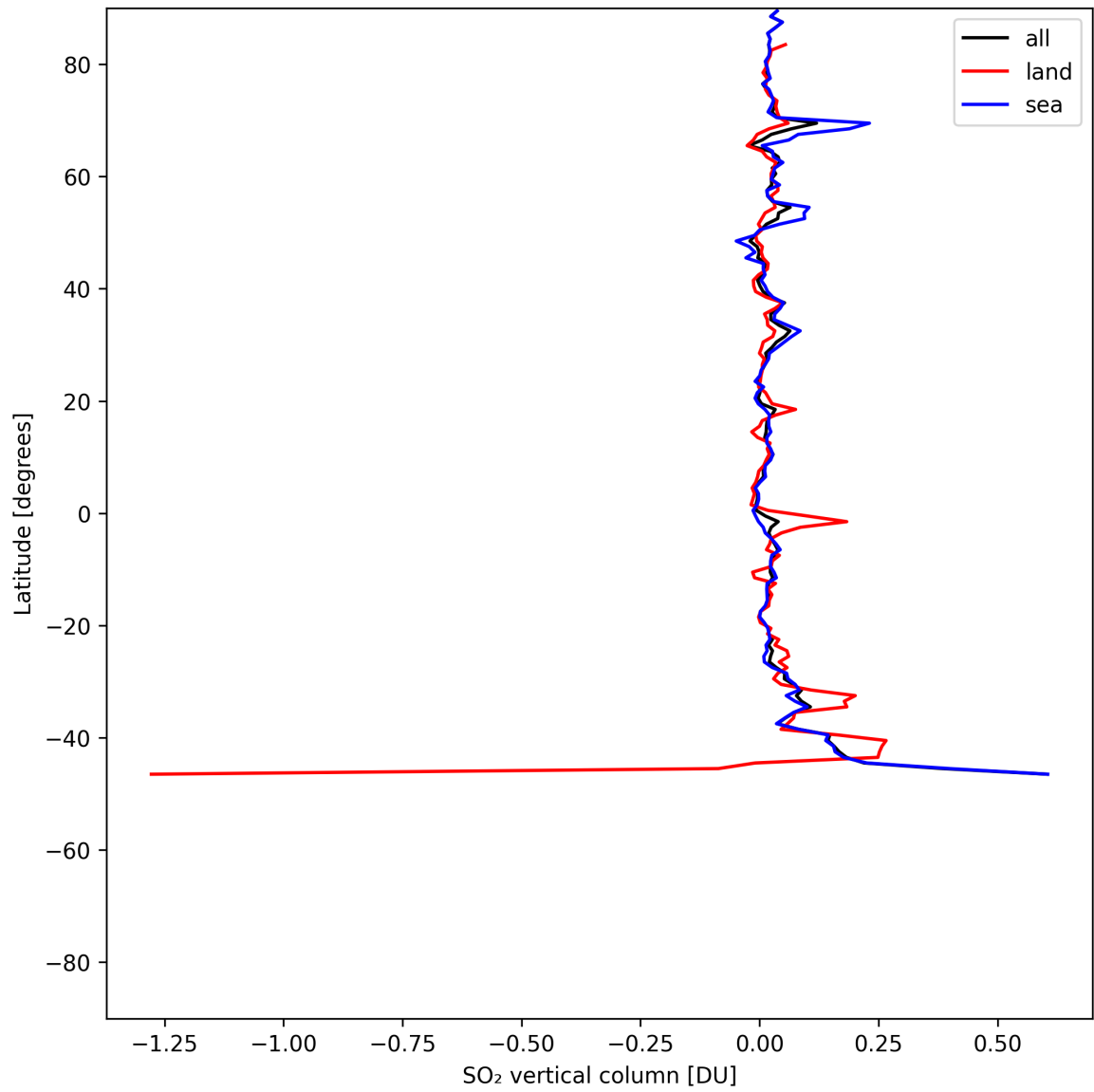
Figure 31: Zonal average of “SO 2 vertical column” for 2025-07-08 to 2025-07-09.
