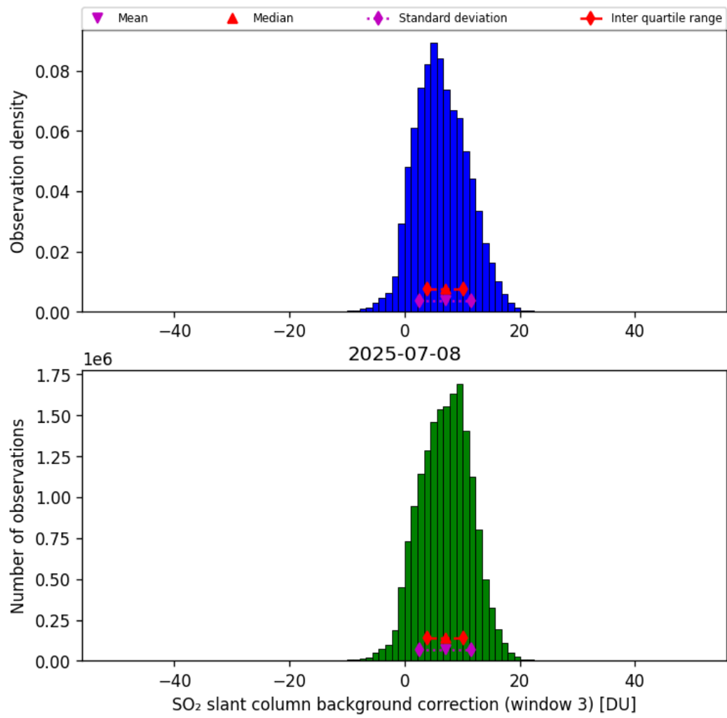
Figure 74: Histogram of “SO 2 slant column background correction (window 3)” for 2025-07-08 to 2025-07-09
