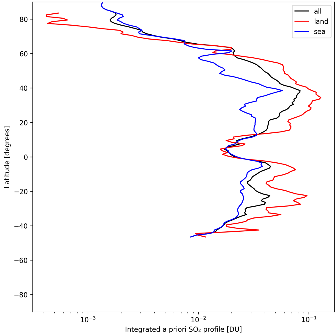
Figure 49: Zonal average of “Integrated a priori SO 2 profile” for 2025-07-08 to 2025-07-09.
