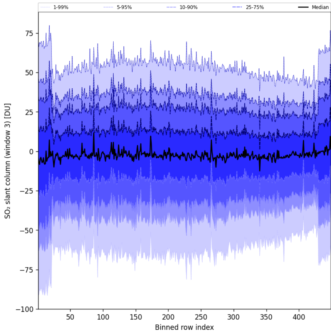
Figure 98: Along track statistics of “SO 2 slant column (window 3)” for 2025-07-08 to 2025-07-09
