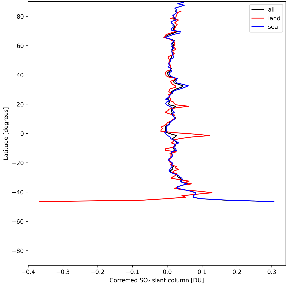
Figure 33: Zonal average of “Corrected SO 2 slant column” for 2025-07-08 to 2025-07-09.
