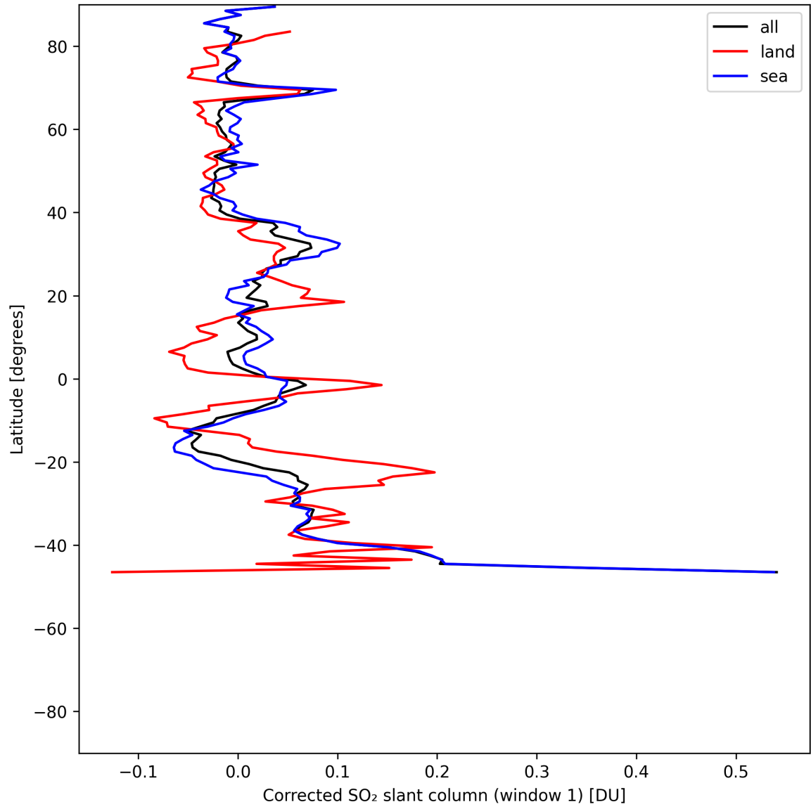
Figure 38: Zonal average of “Corrected SO 2 slant column (window 1)” for 2025-07-08 to 2025-07-09.
