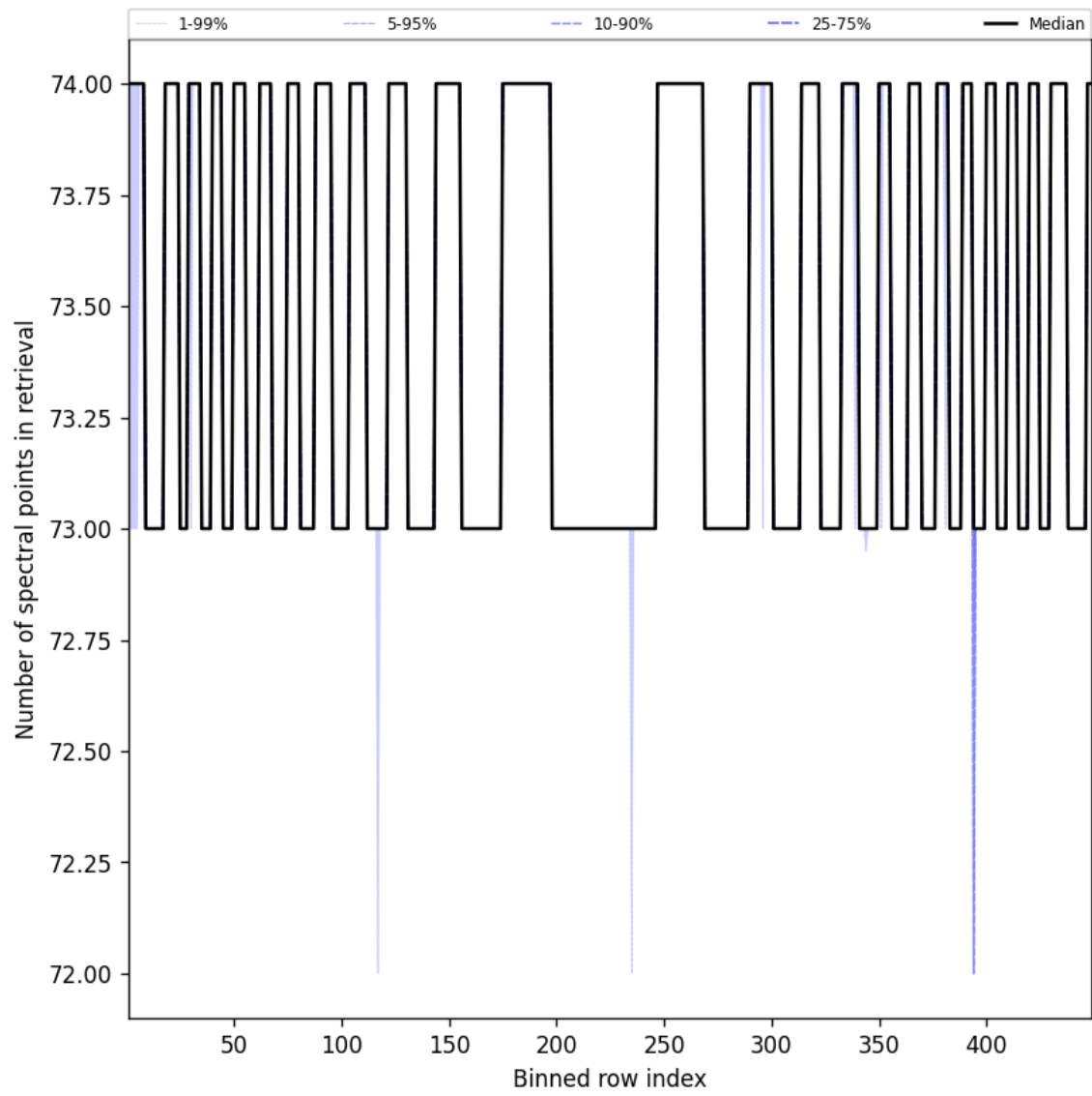
Figure 110: Along track statistics of “Number of spectral points in retrieval” for 2025-07-08 to 2025-07-09
