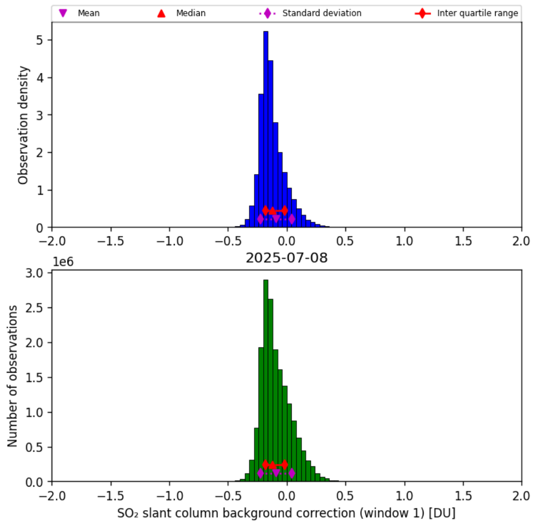
Figure 66: Histogram of “SO 2 slant column background correction (window 1)” for 2025-07-08 to 2025-07-09
