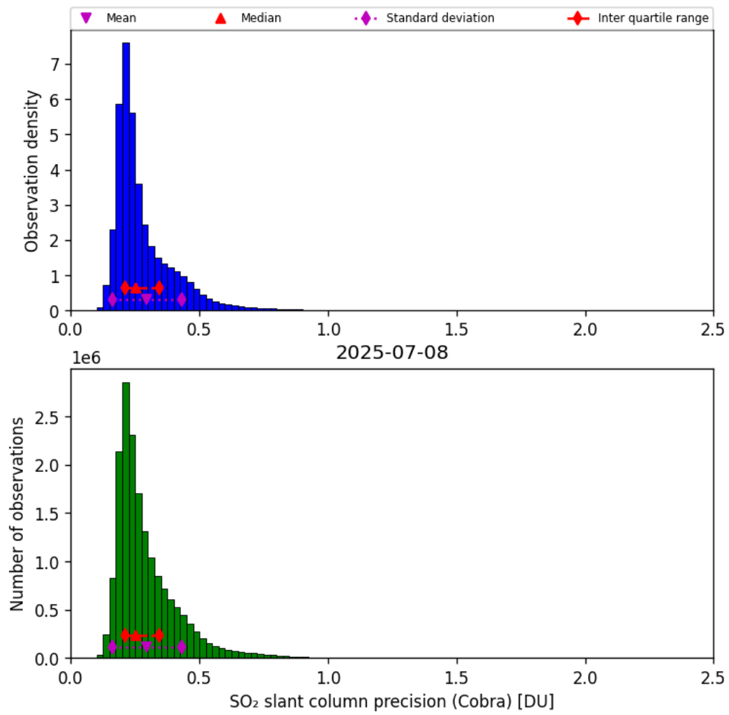
Figure 62: Histogram of “SO 2 slant column precision (Cobra)” for 2025-07-08 to 2025-07-09
