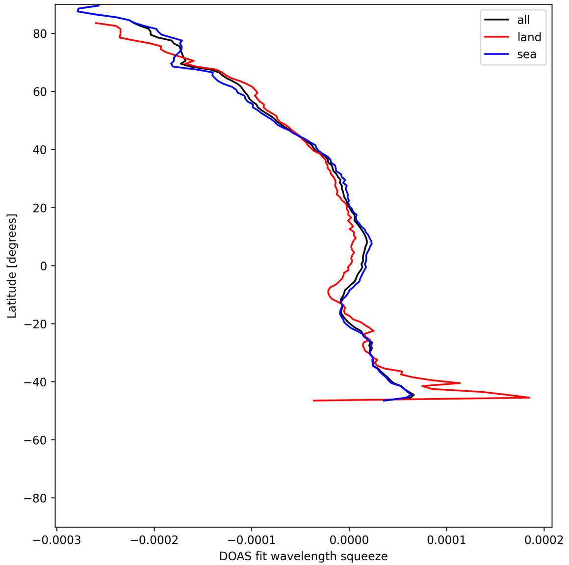
Figure 51: Zonal average of “DOAS fit wavelength squeeze” for 2025-07-08 to 2025-07-09.
