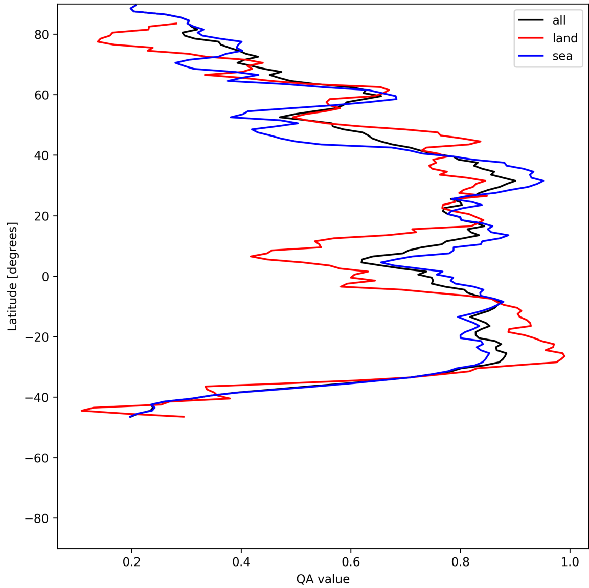
Figure 30: Zonal average of “QA value” for 2025-07-08 to 2025-07-09.
