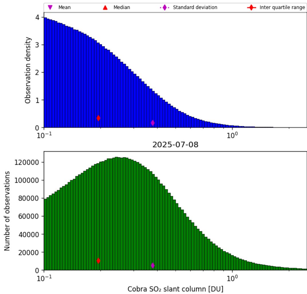
Figure 61: Histogram of “Cobra SO 2 slant column” for 2025-07-08 to 2025-07-09
