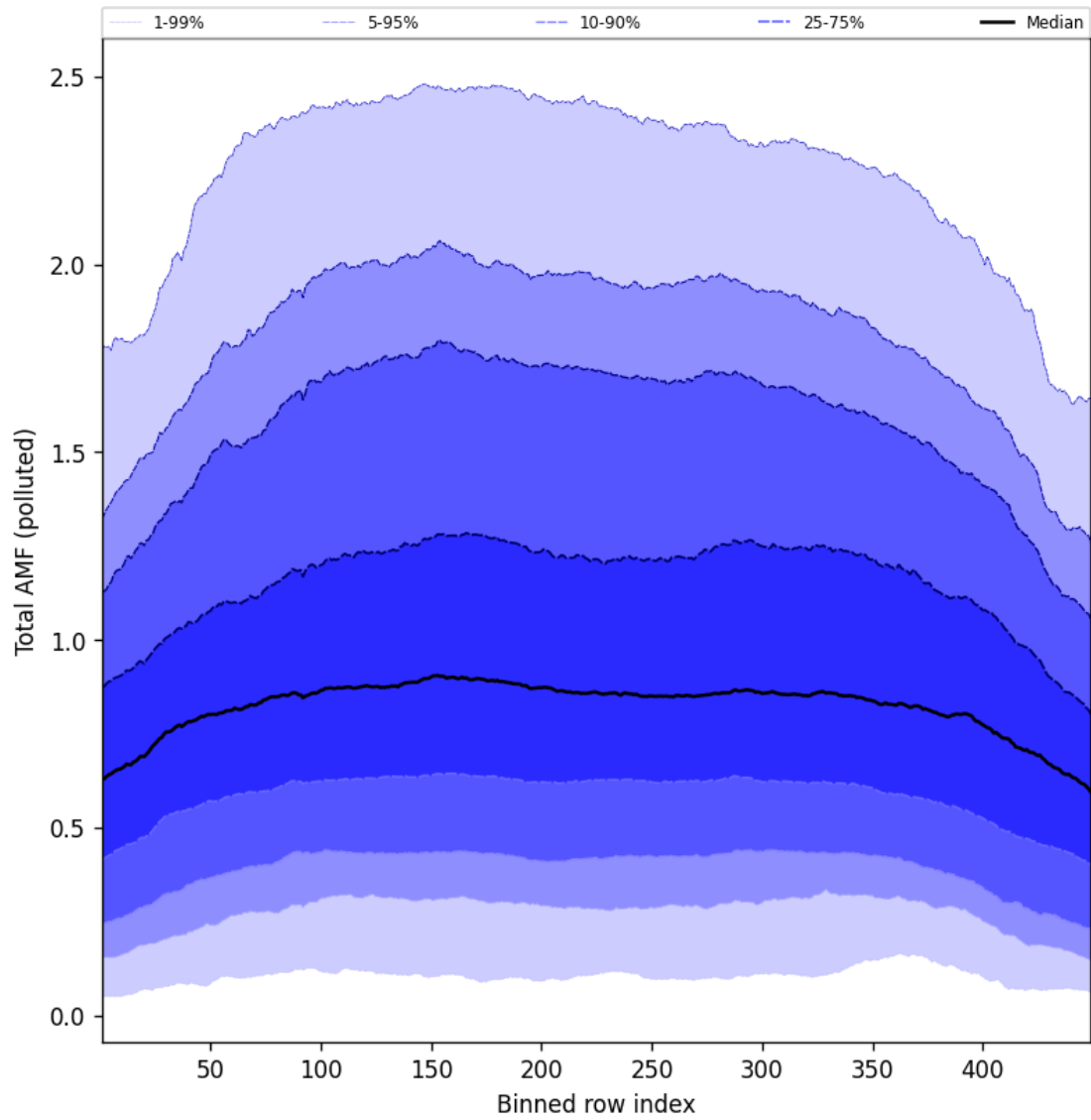
Figure 107: Along track statistics of “Total AMF (polluted)” for 2025-07-08 to 2025-07-09
