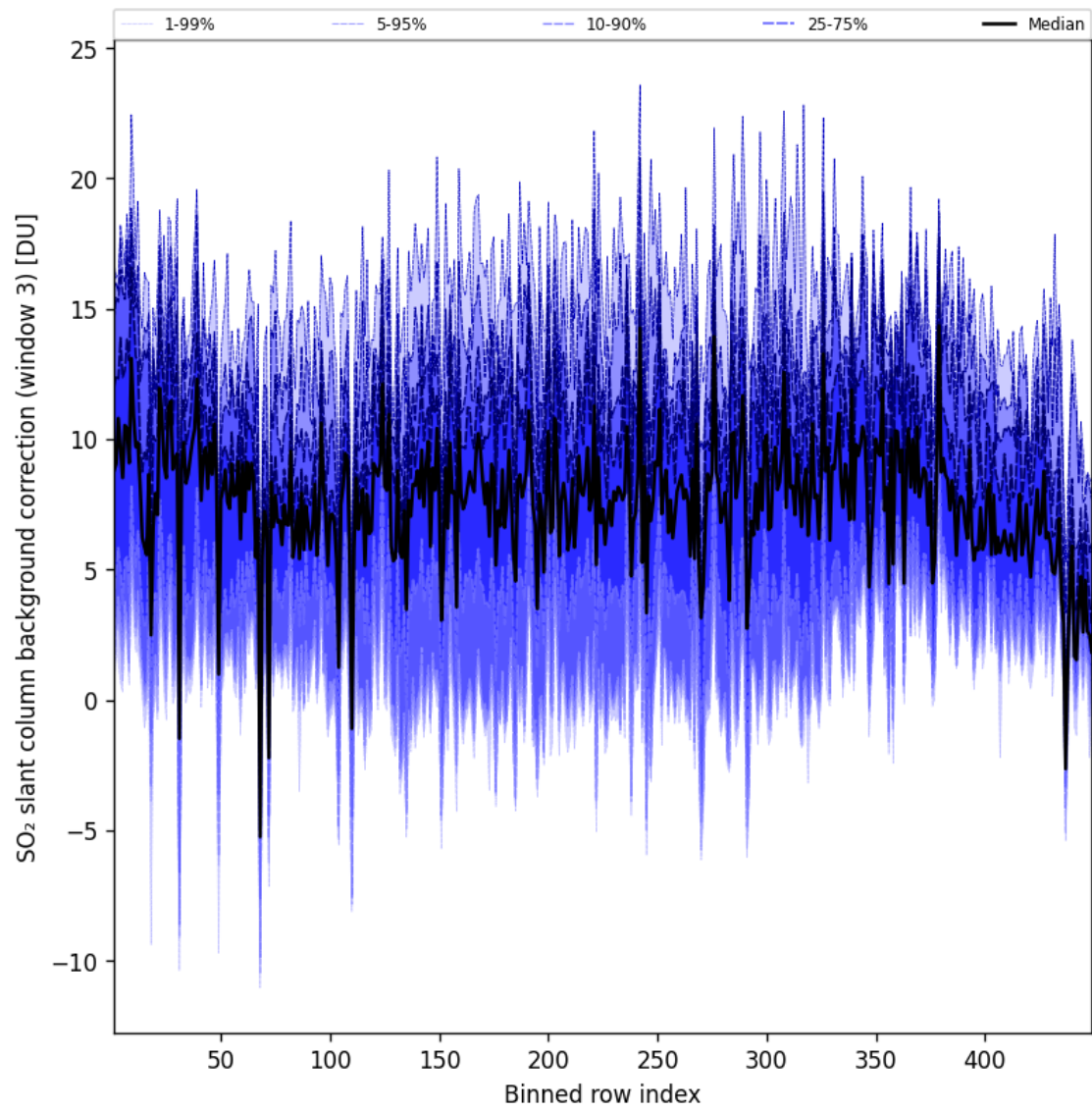
Figure 101: Along track statistics of “SO 2 slant column background correction (window 3)” for 2025-07-08 to 2025-07-09
