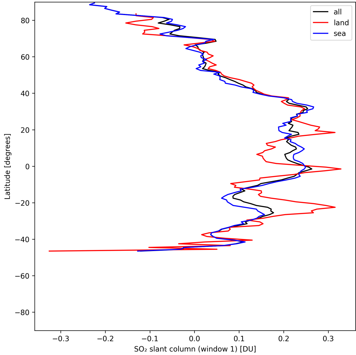
Figure 36: Zonal average of “SO 2 slant column (window 1)” for 2025-07-08 to 2025-07-09.
