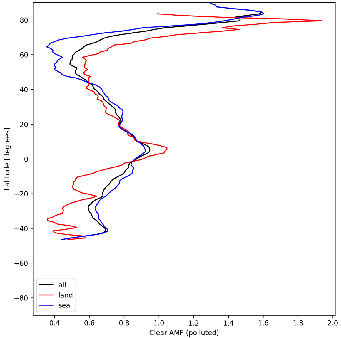
Figure 55: Zonal average of “Clear AMF (polluted)” for 2025-07-08 to 2025-07-09.
