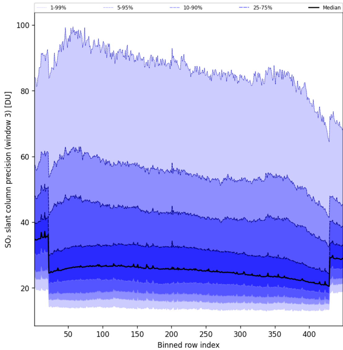
Figure 99: Along track statistics of “SO 2 slant column precision (window 3)” for 2025-07-08 to 2025-07-09
