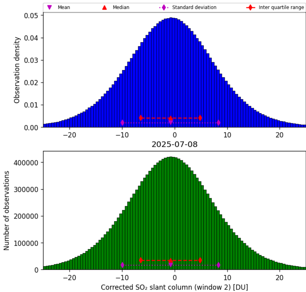
Figure 69: Histogram of “Corrected SO 2 slant column (window 2)” for 2025-07-08 to 2025-07-09
