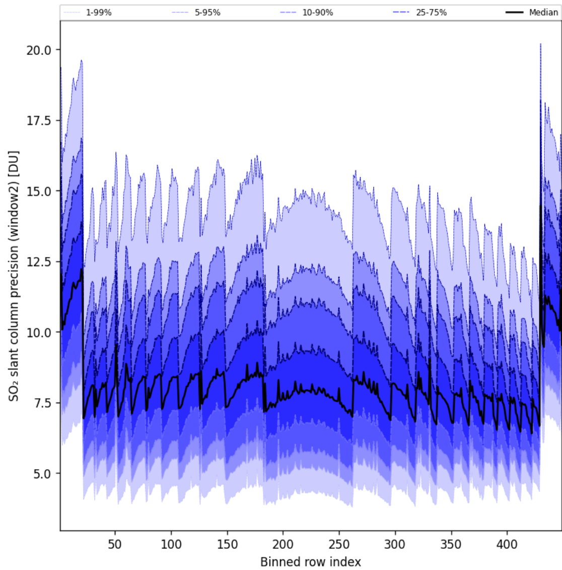
Figure 95: Along track statistics of “SO 2 slant column precision (window2)” for 2025-07-08 to 2025-07-09
