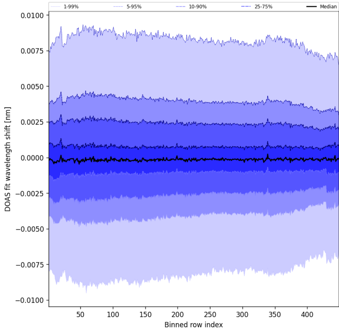
Figure 104: Along track statistics of “DOAS fit wavelength shift” for 2025-07-08 to 2025-07-09
