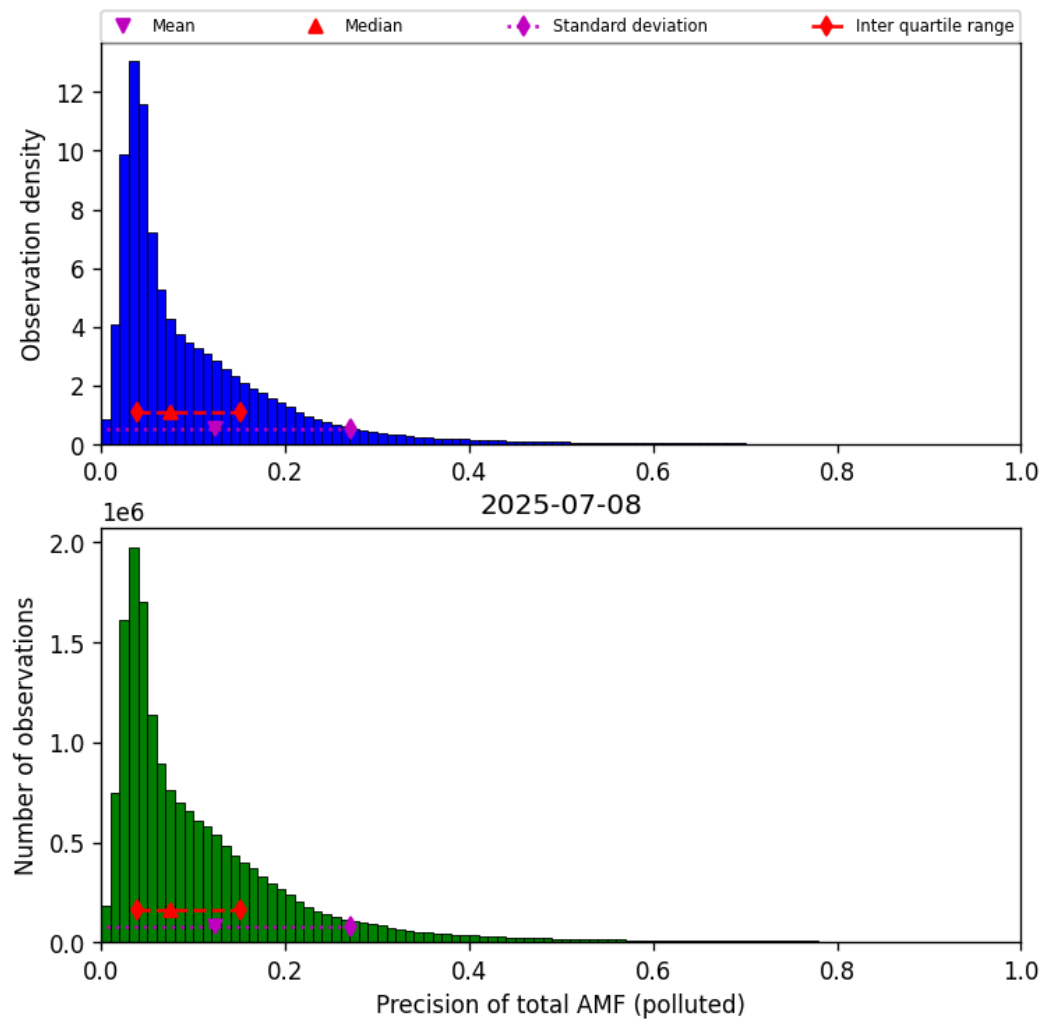
Figure 81: Histogram of “Precision of total AMF (polluted)” for 2025-07-08 to 2025-07-09
