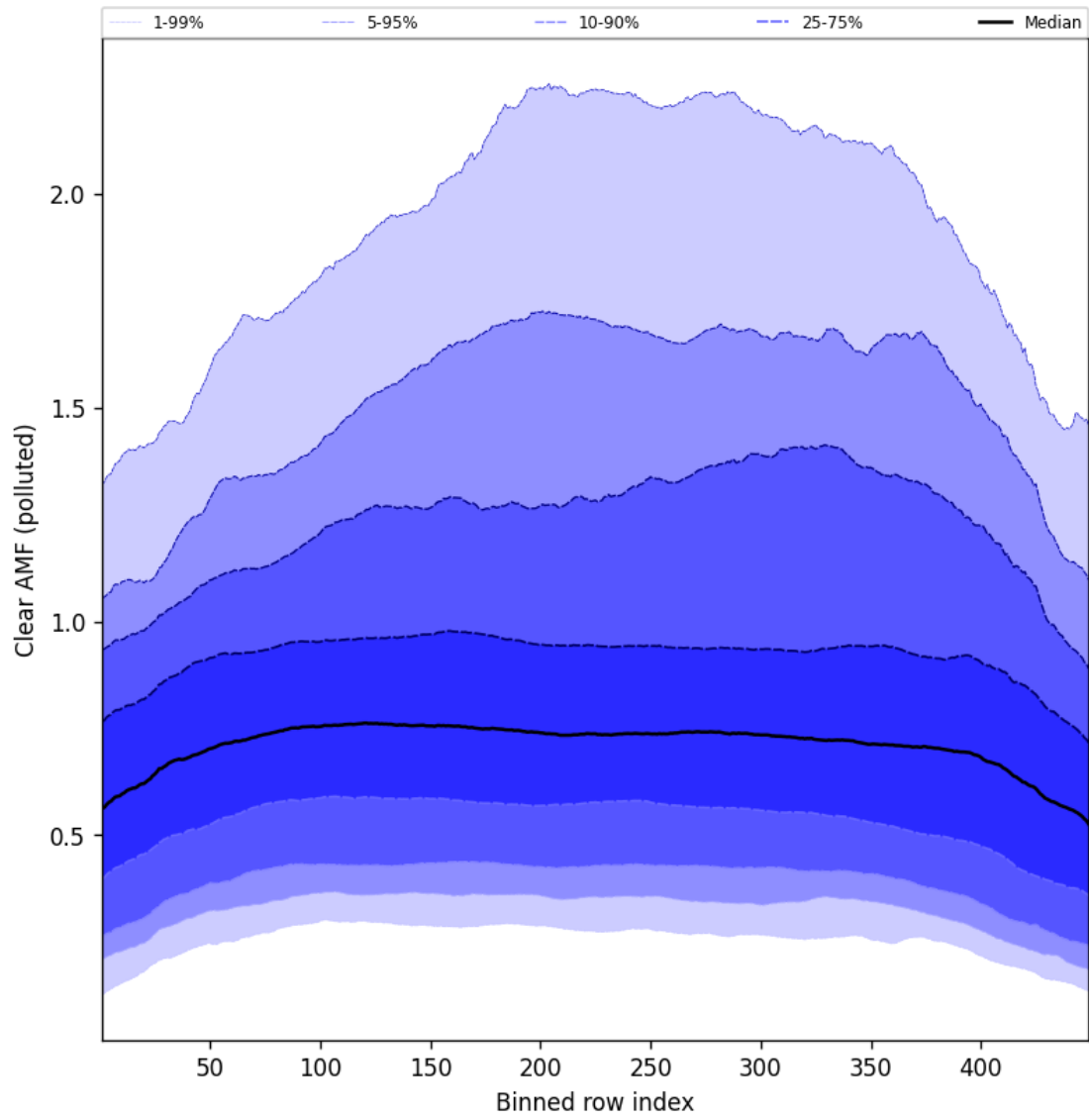
Figure 109: Along track statistics of “Clear AMF (polluted)” for 2025-07-08 to 2025-07-09
