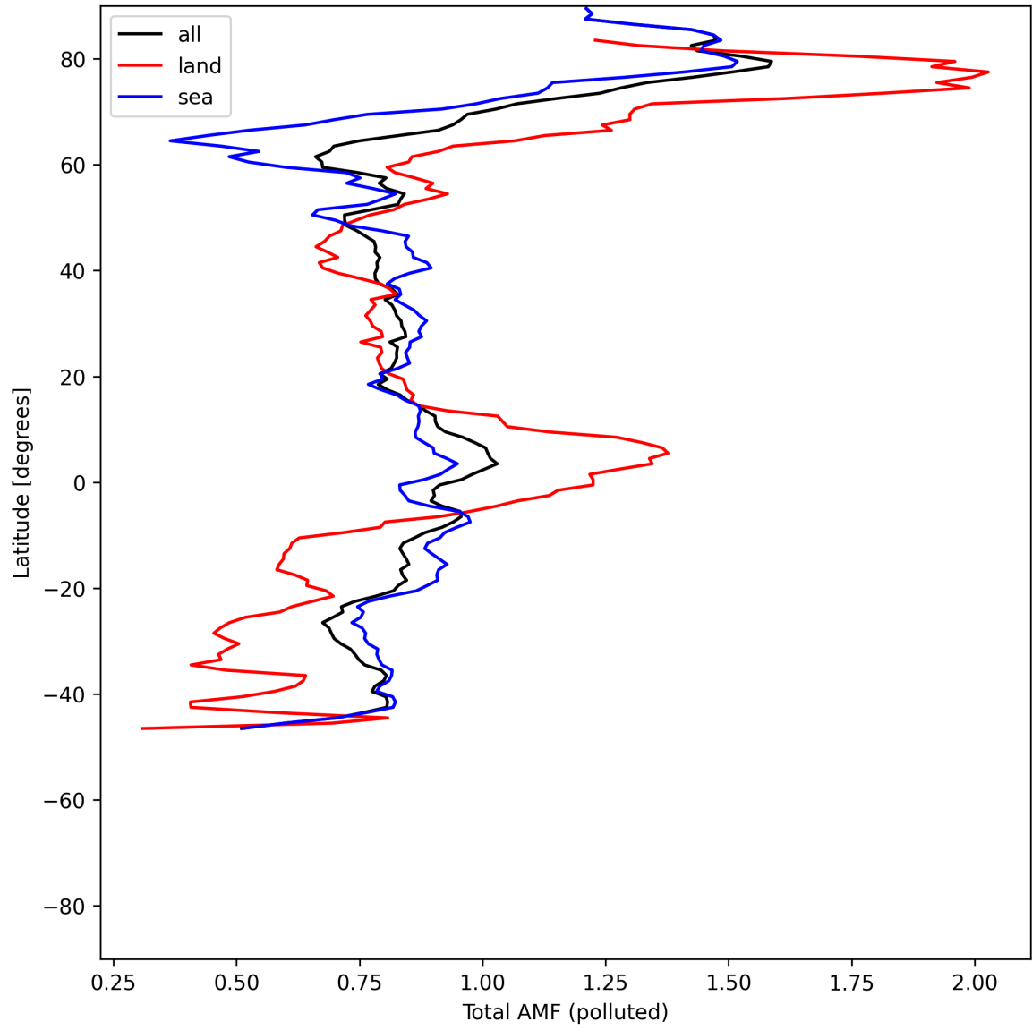
Figure 53: Zonal average of “Total AMF (polluted)” for 2025-07-08 to 2025-07-09.
