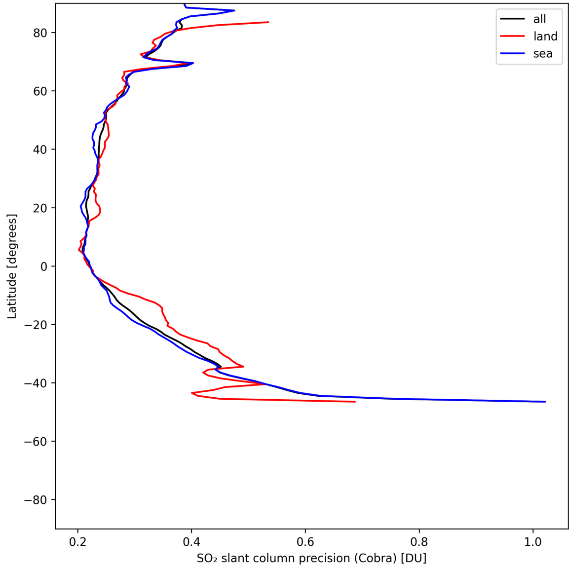
Figure 35: Zonal average of “SO 2 slant column precision (Cobra)” for 2025-07-08 to 2025-07-09.
