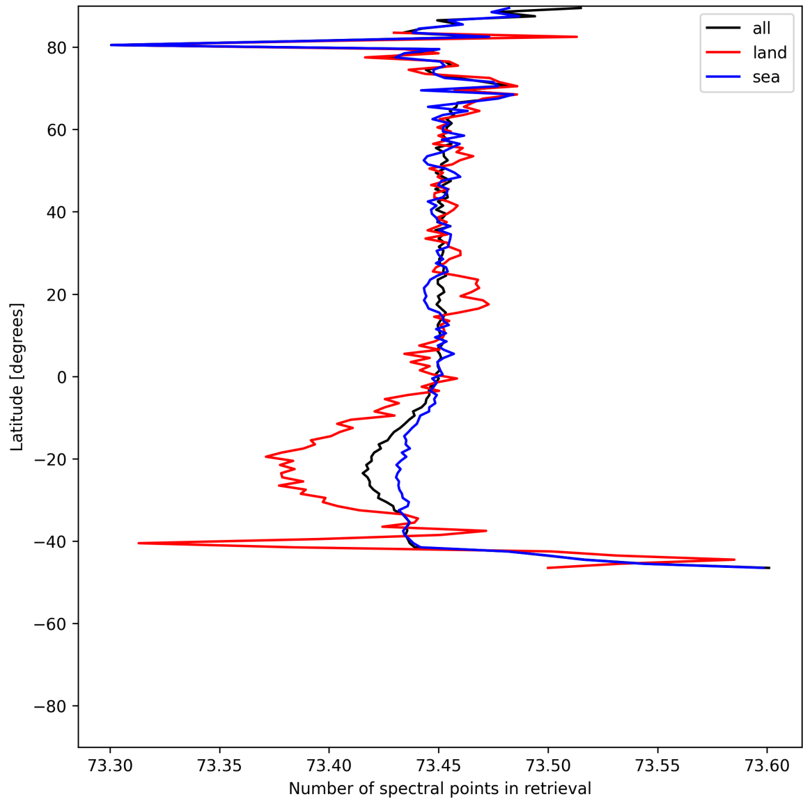
Figure 56: Zonal average of “Number of spectral points in retrieval” for 2025-07-08 to 2025-07-09.
