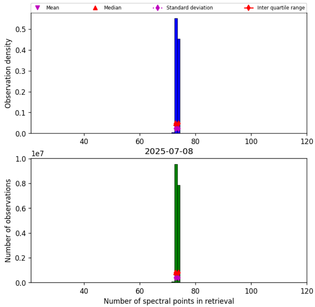
Figure 83: Histogram of “Number of spectral points in retrieval” for 2025-07-08 to 2025-07-09
