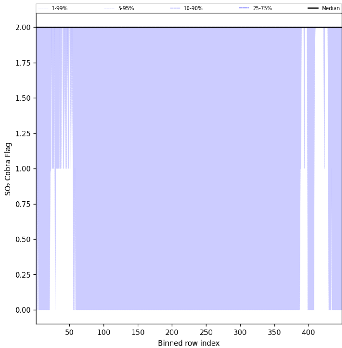
Figure 102: Along track statistics of “SO 2 Cobra Flag” for 2025-07-08 to 2025-07-09
