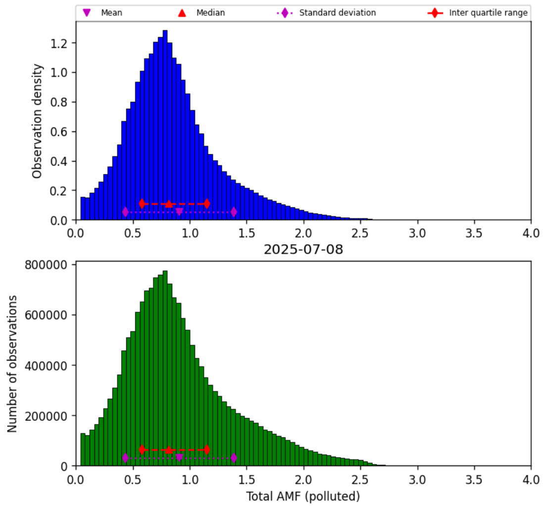
Figure 80: Histogram of “Total AMF (polluted)” for 2025-07-08 to 2025-07-09
