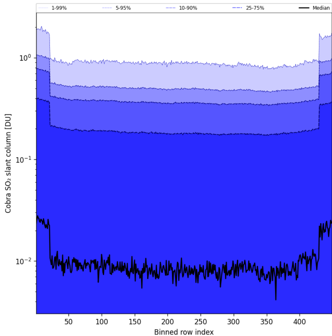
Figure 88: Along track statistics of “Cobra SO 2 slant column” for 2025-07-08 to 2025-07-09
