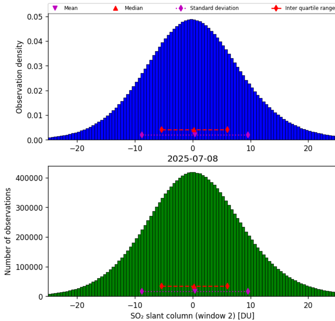
Figure 67: Histogram of “SO 2 slant column (window 2)” for 2025-07-08 to 2025-07-09
