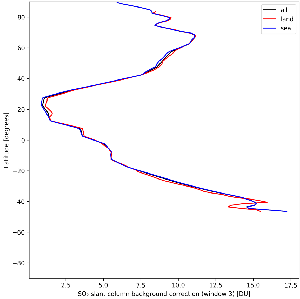
Figure 47: Zonal average of “SO 2 slant column background correction (window 3)” for 2025-07-08 to 2025-07-09.
