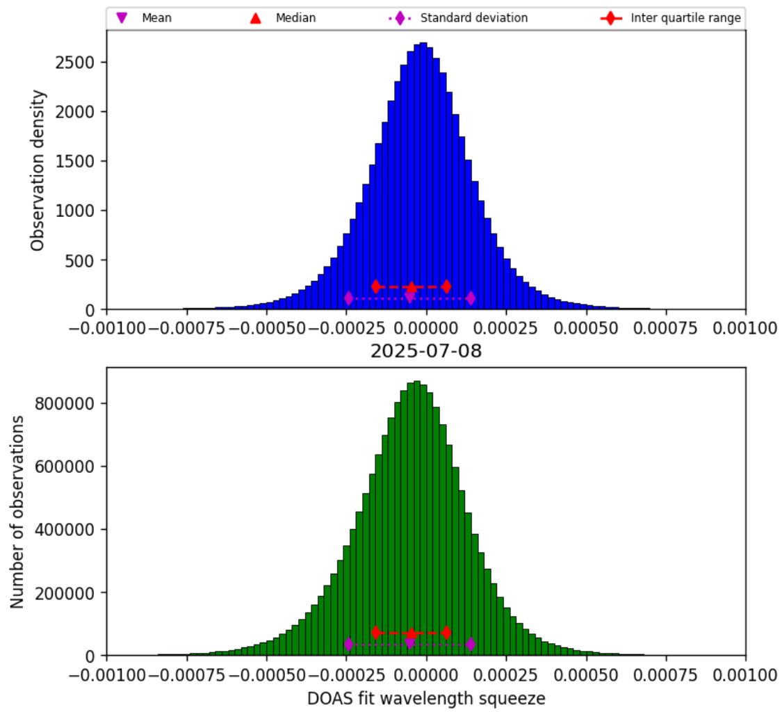
Figure 78: Histogram of “DOAS fit wavelength squeeze” for 2025-07-08 to 2025-07-09
