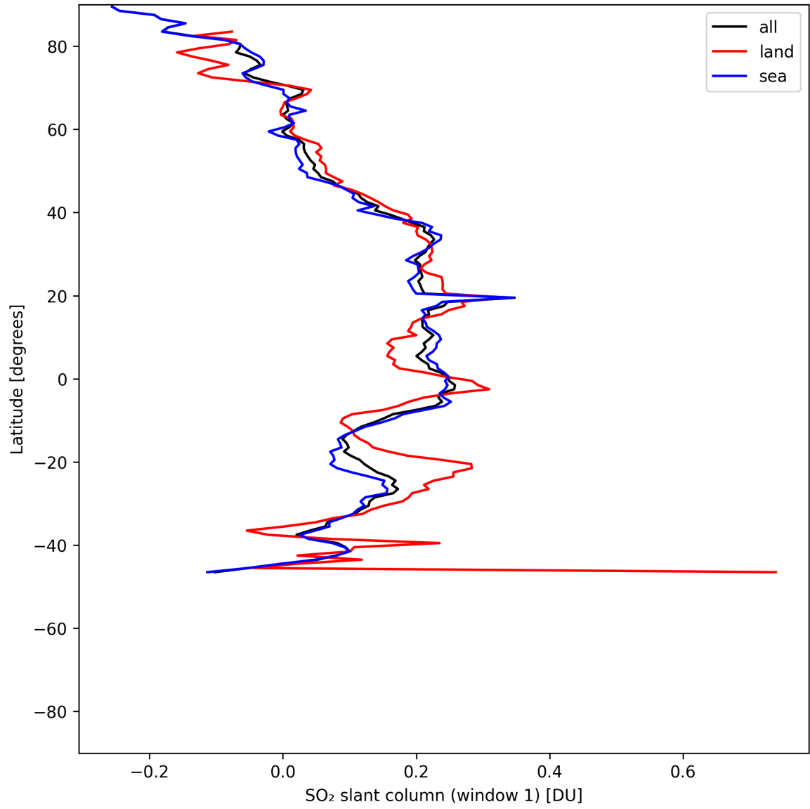
Figure 36: Zonal average of “SO 2 slant column (window 1)” for 2025-07-09 to 2025-07-10.
