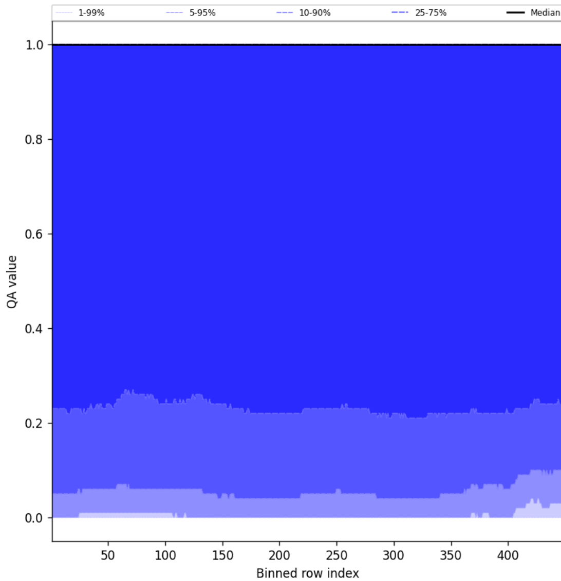
Figure 84: Along track statistics of “QA value” for 2025-07-09 to 2025-07-10
