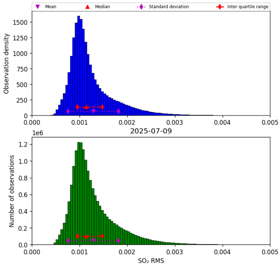
Figure 79: Histogram of “SO 2 RMS” for 2025-07-09 to 2025-07-10
