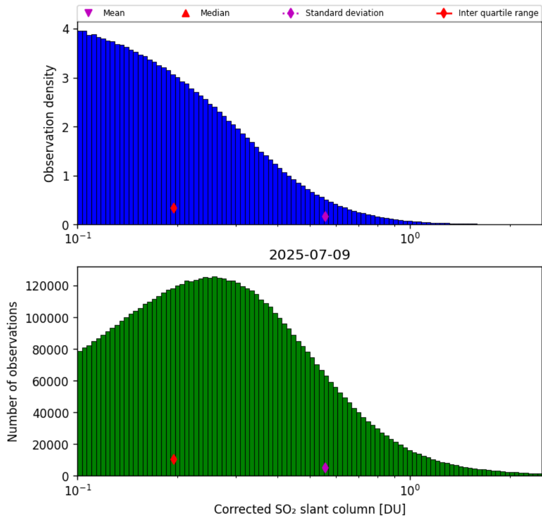
Figure 60: Histogram of “Corrected SO 2 slant column” for 2025-07-09 to 2025-07-10
