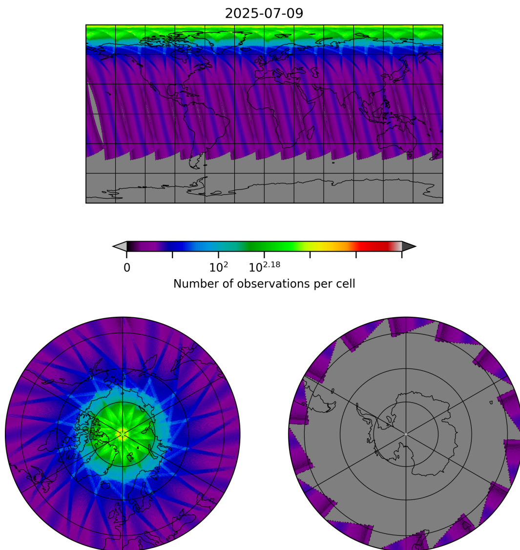
Figure 29: Map of the number of observations for 2025-07-09 to 2025-07-10
