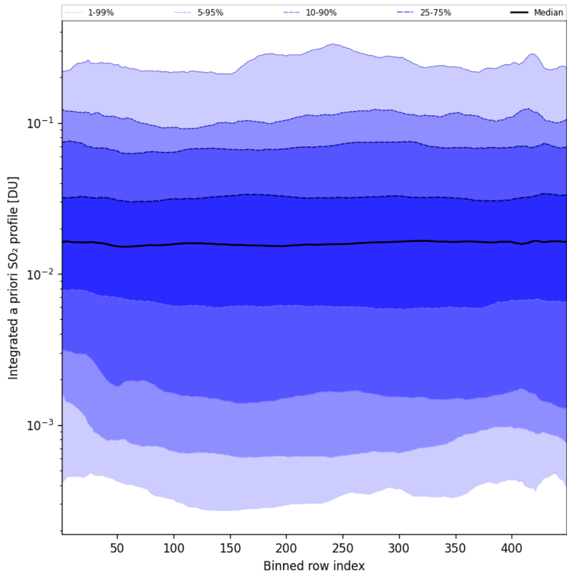
Figure 103: Along track statistics of “Integrated a priori SO 2 profile” for 2025-07-09 to 2025-07-10
