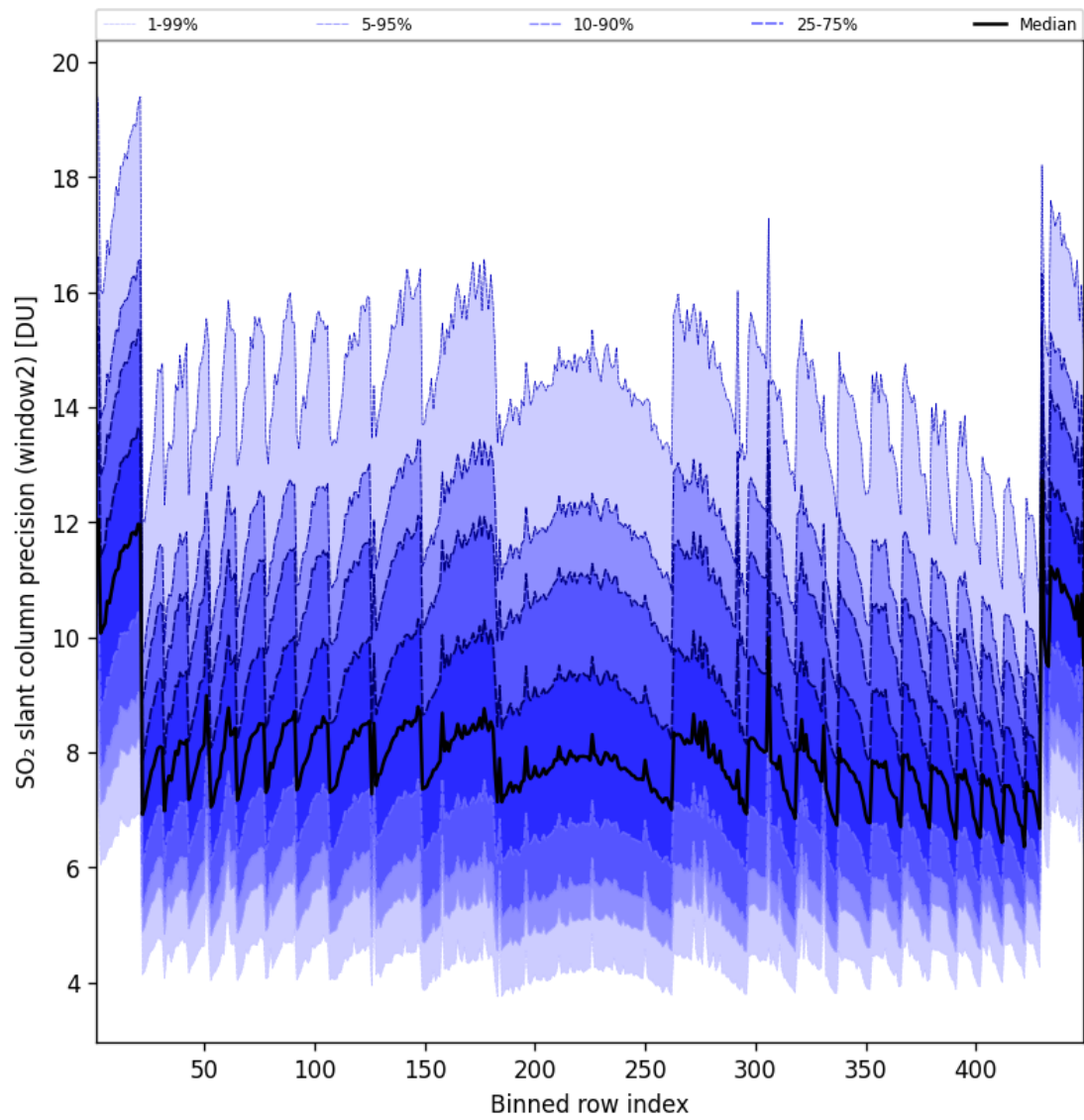
Figure 95: Along track statistics of “SO 2 slant column precision (window2)” for 2025-07-09 to 2025-07-10
