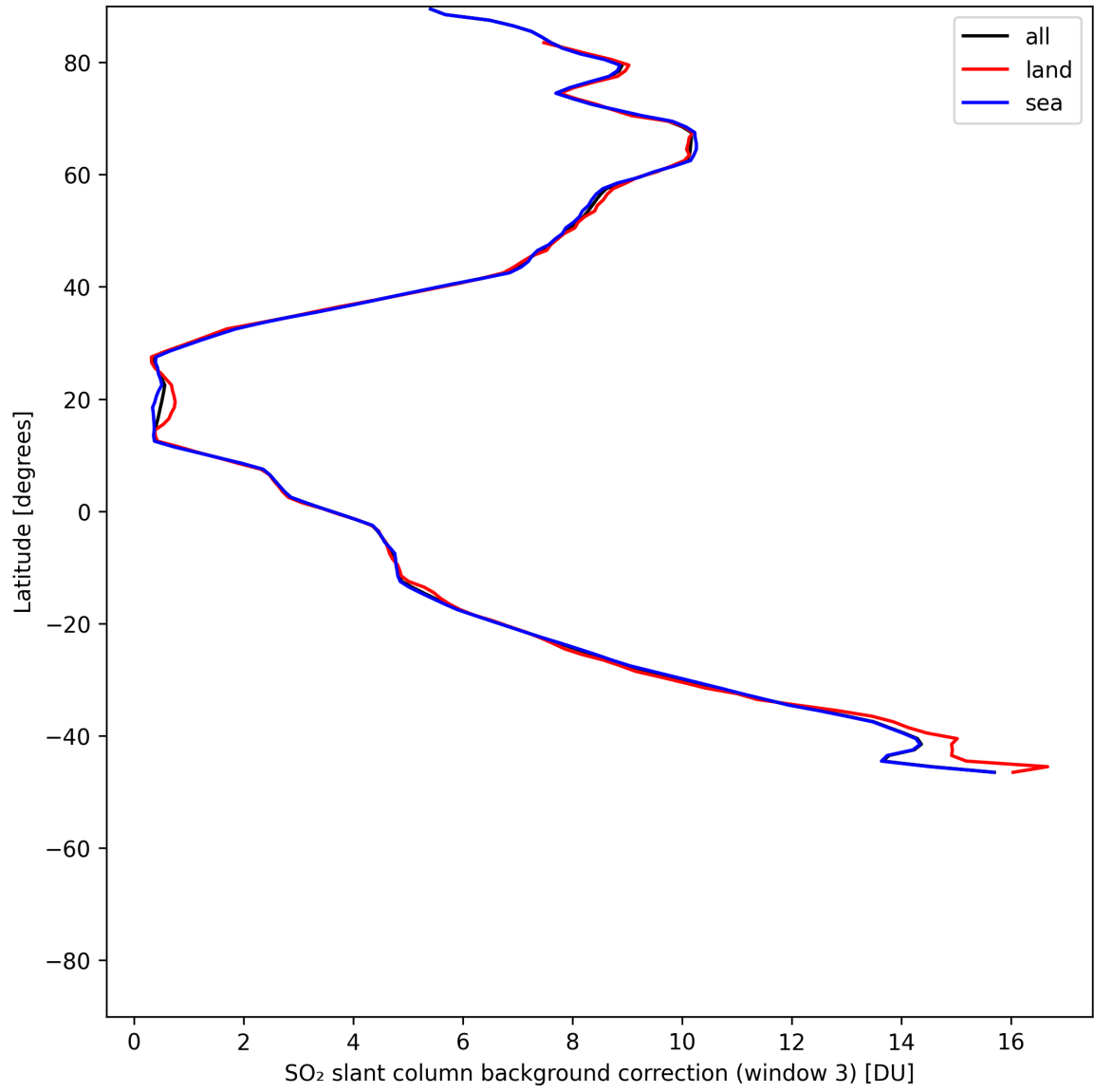
Figure 47: Zonal average of “SO 2 slant column background correction (window 3)” for 2025-07-09 to 2025-07-10.
