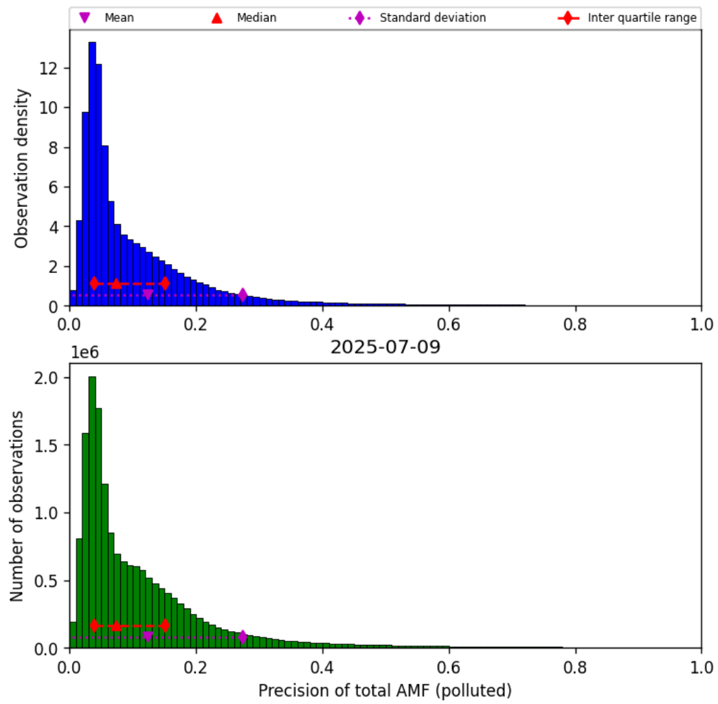
Figure 81: Histogram of “Precision of total AMF (polluted)” for 2025-07-09 to 2025-07-10
