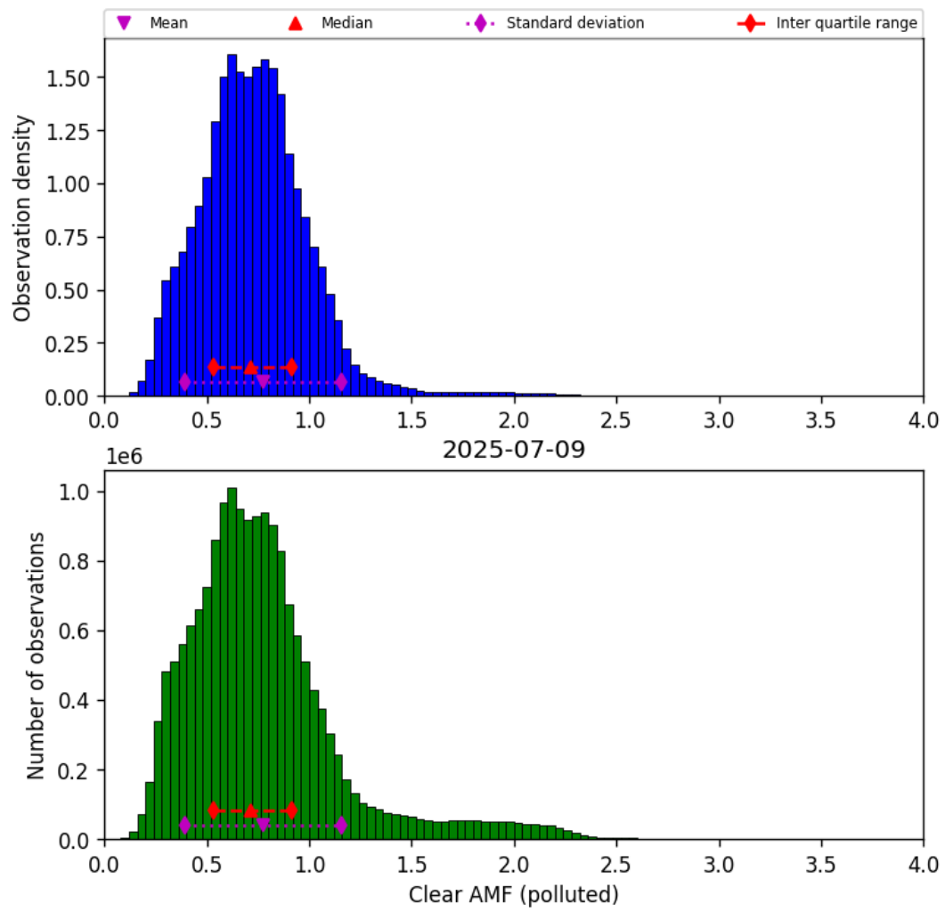
Figure 82: Histogram of “Clear AMF (polluted)” for 2025-07-09 to 2025-07-10
