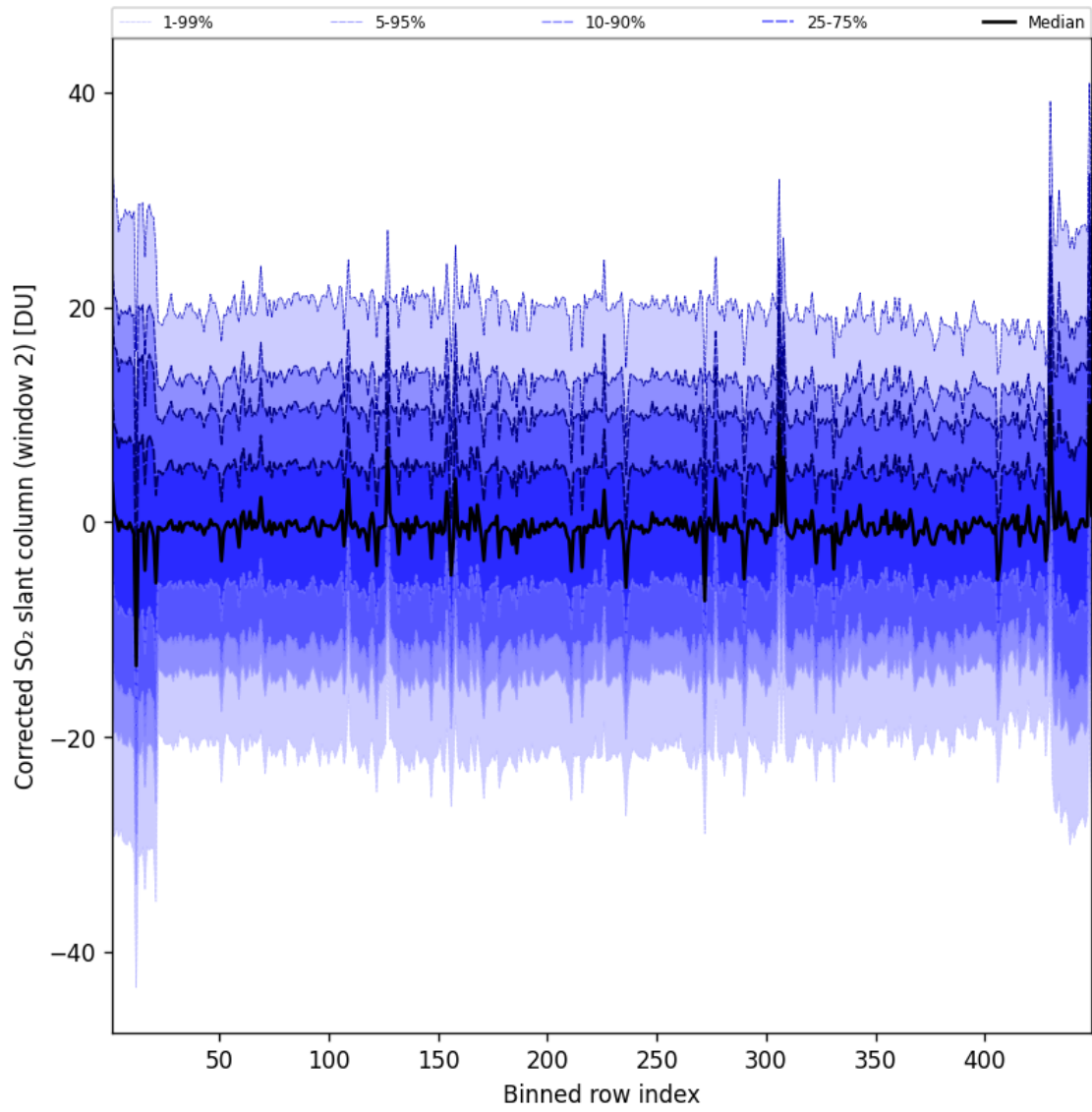
Figure 96: Along track statistics of “Corrected SO 2 slant column (window 2)” for 2025-07-09 to 2025-07-10
