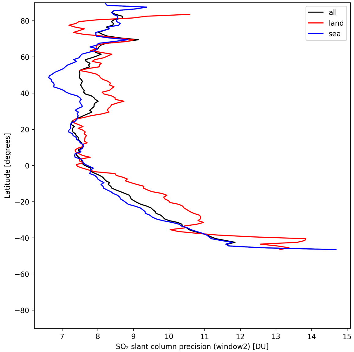
Figure 41: Zonal average of “SO 2 slant column precision (window2)” for 2025-07-09 to 2025-07-10.
