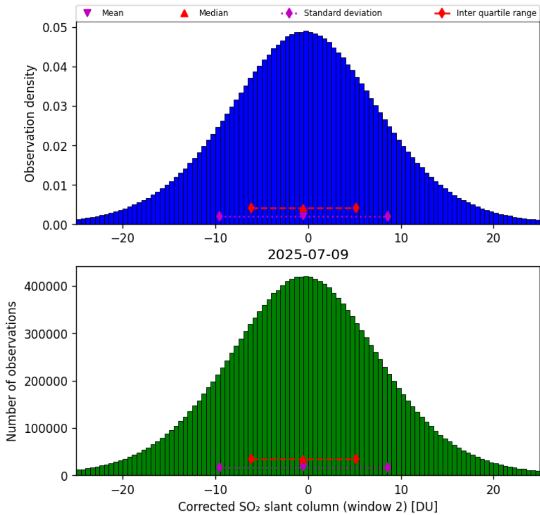
Figure 69: Histogram of “Corrected SO 2 slant column (window 2)” for 2025-07-09 to 2025-07-10
