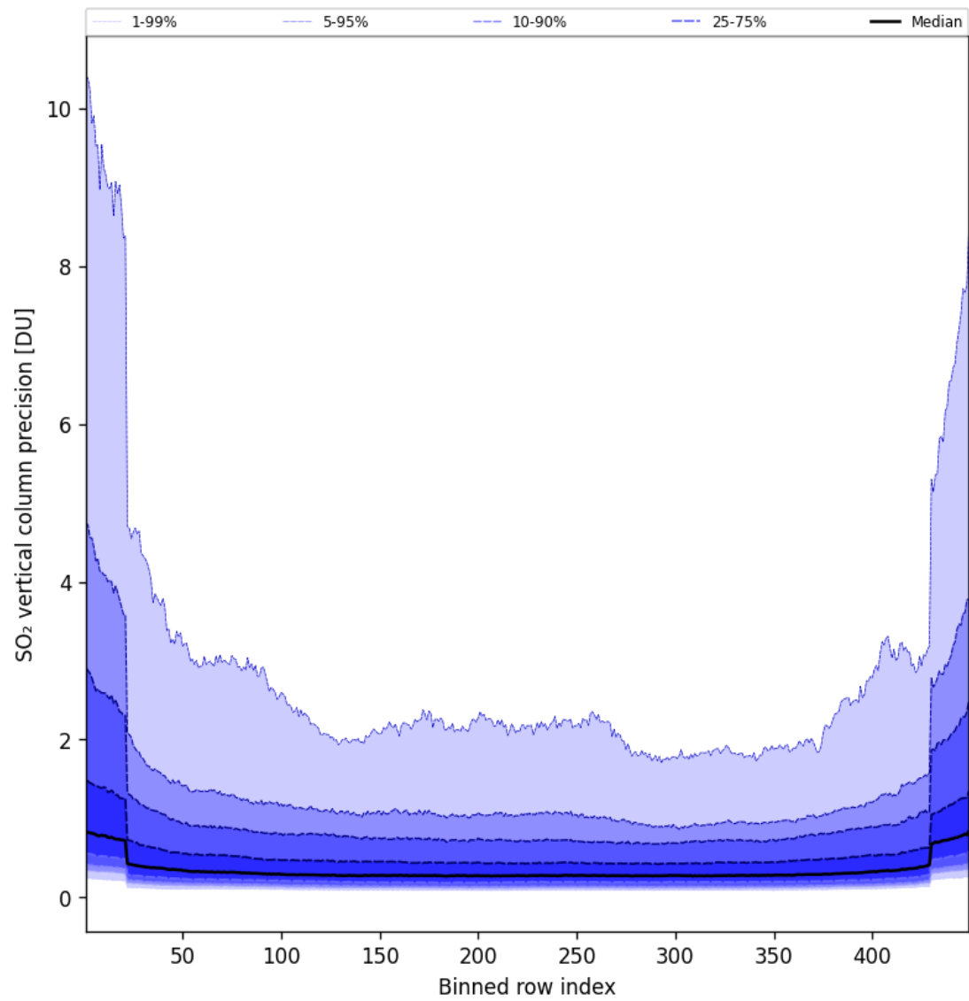
Figure 86: Along track statistics of “SO 2 vertical column precision” for 2025-07-09 to 2025-07-10
