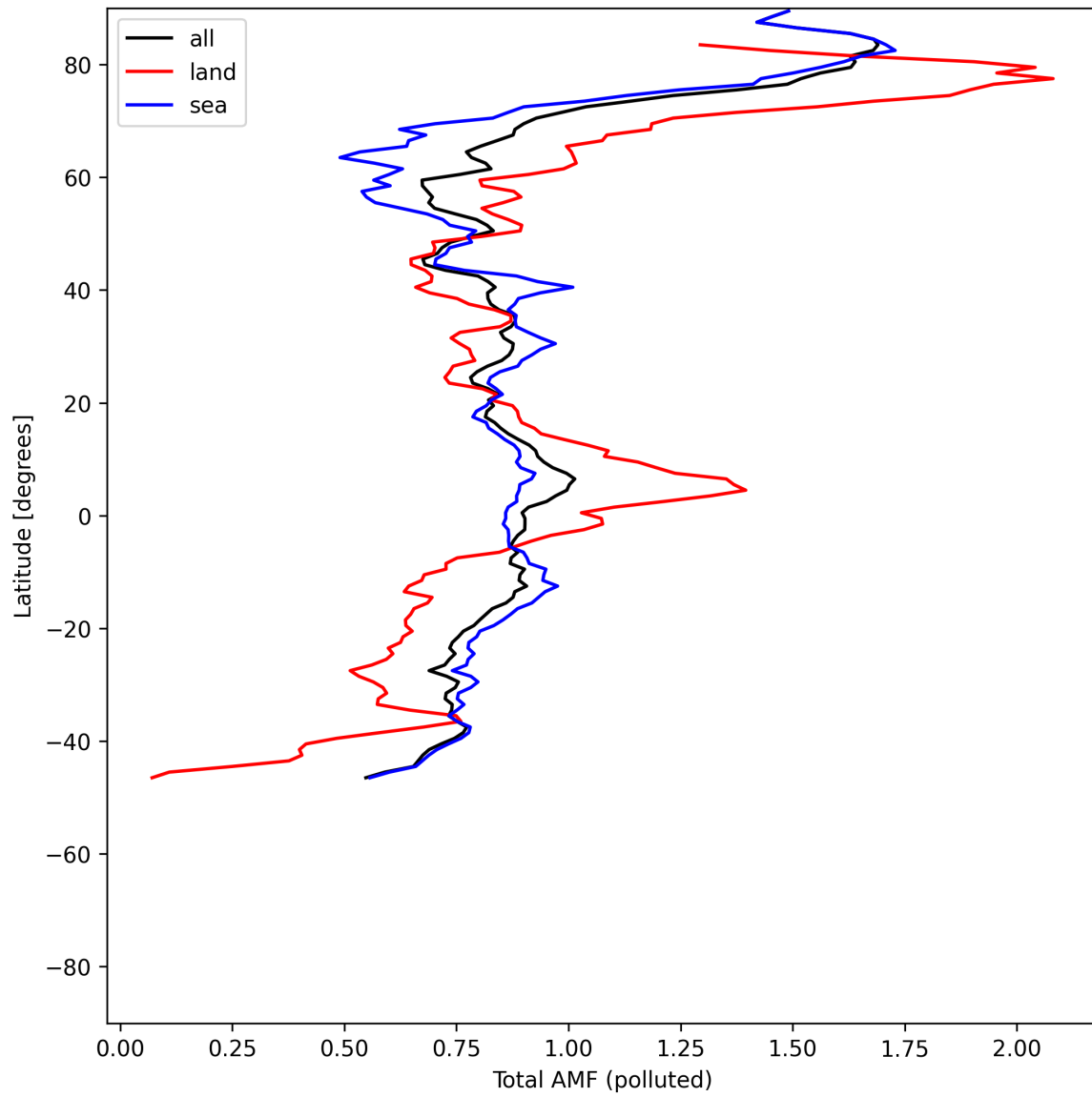
Figure 53: Zonal average of “Total AMF (polluted)” for 2025-07-09 to 2025-07-10.
