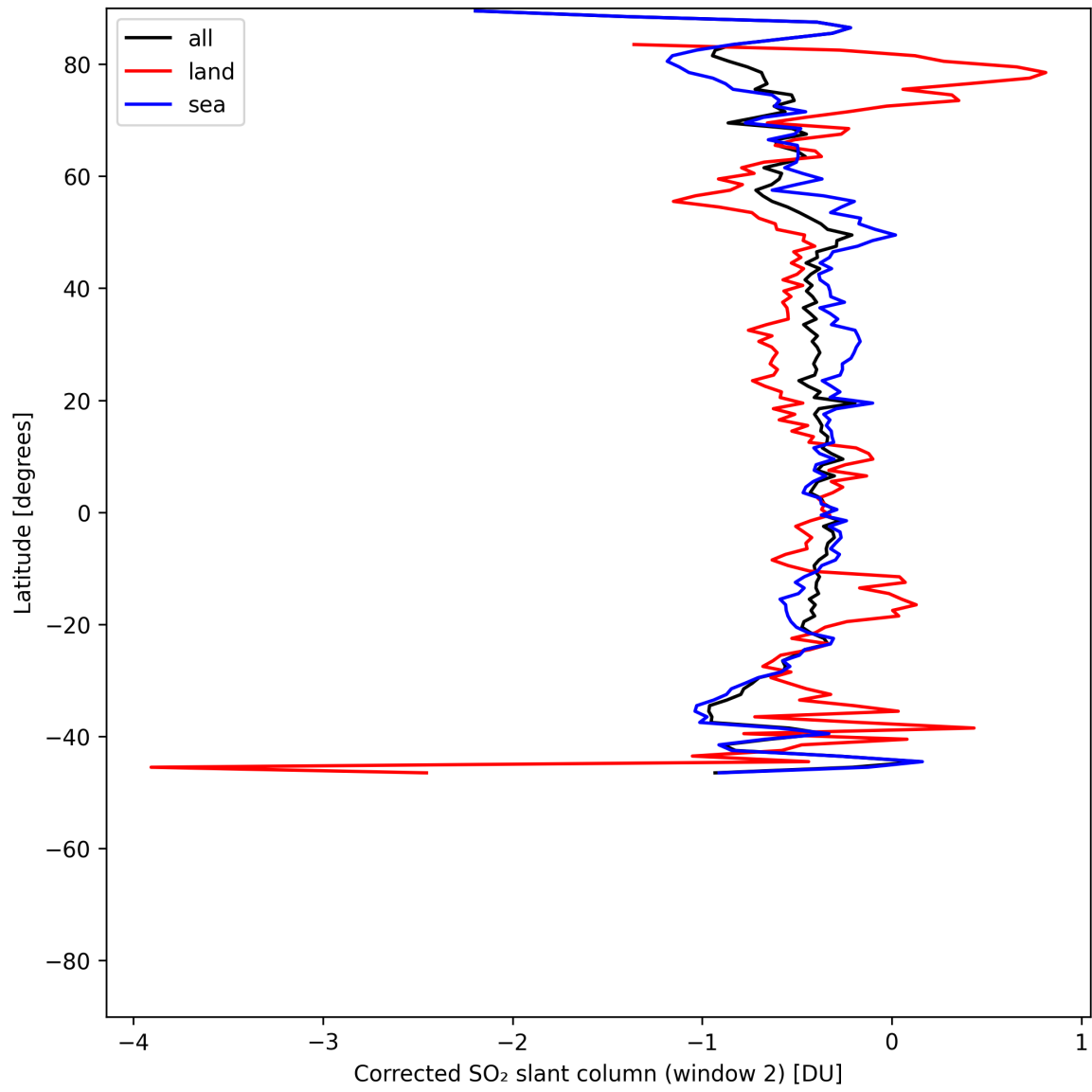
Figure 42: Zonal average of “Corrected SO 2 slant column (window 2)” for 2025-07-09 to 2025-07-10.
