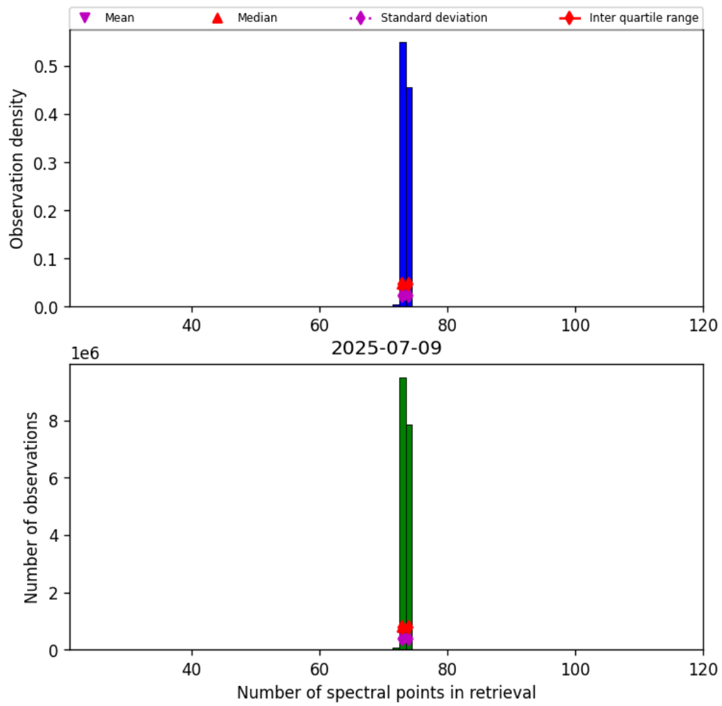
Figure 83: Histogram of “Number of spectral points in retrieval” for 2025-07-09 to 2025-07-10
