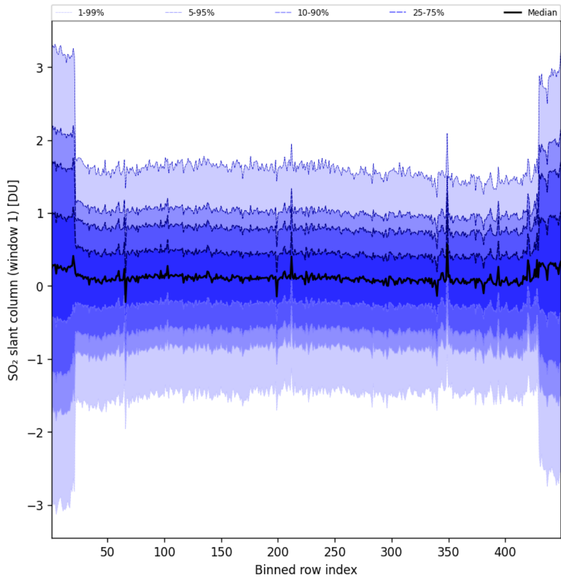
Figure 90: Along track statistics of “SO 2 slant column (window 1)” for 2025-07-09 to 2025-07-10
