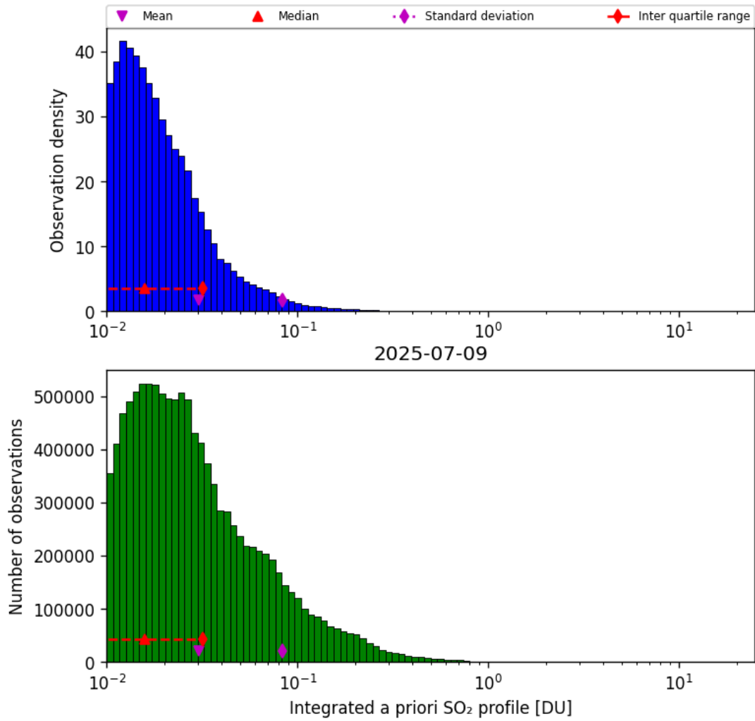
Figure 76: Histogram of “Integrated a priori SO 2 profile” for 2025-07-09 to 2025-07-10
