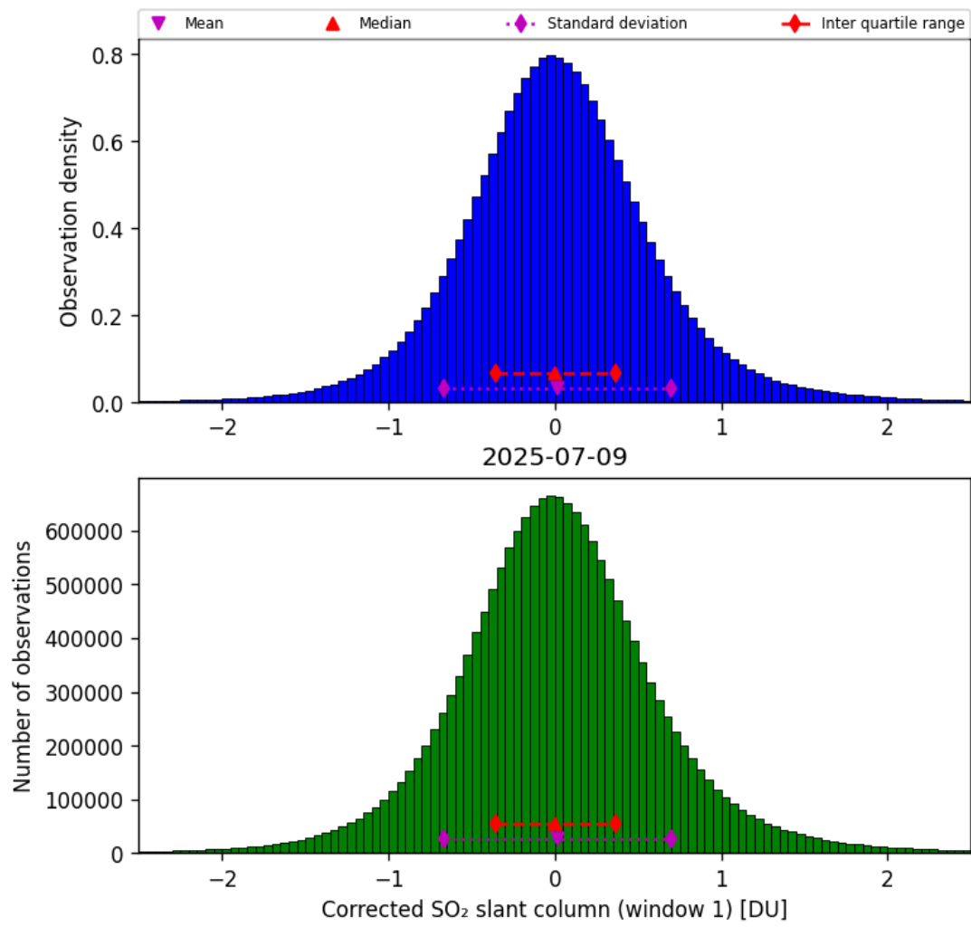
Figure 65: Histogram of “Corrected SO 2 slant column (window 1)” for 2025-07-09 to 2025-07-10
