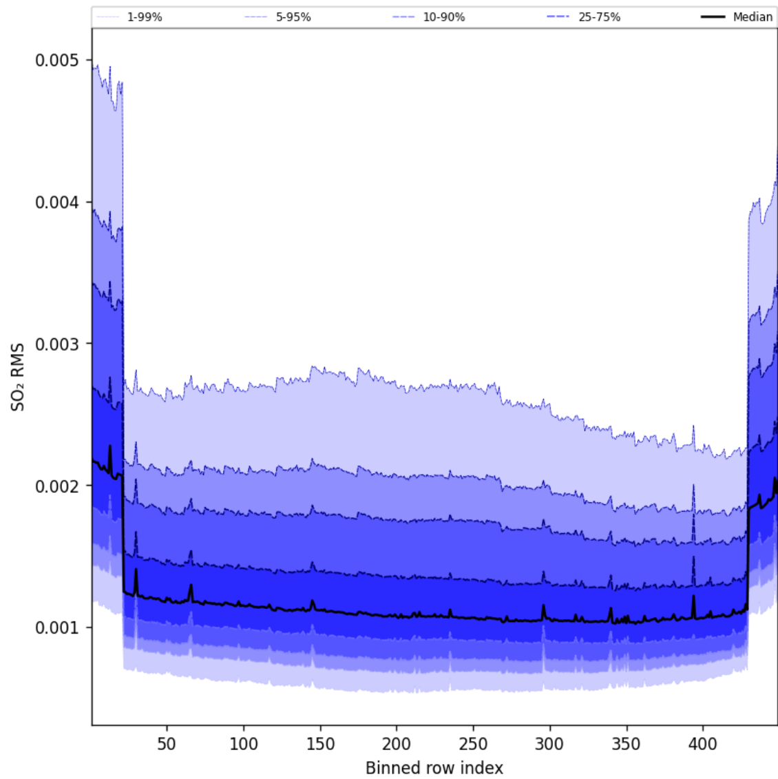
Figure 106: Along track statistics of “SO 2 RMS” for 2025-07-09 to 2025-07-10
