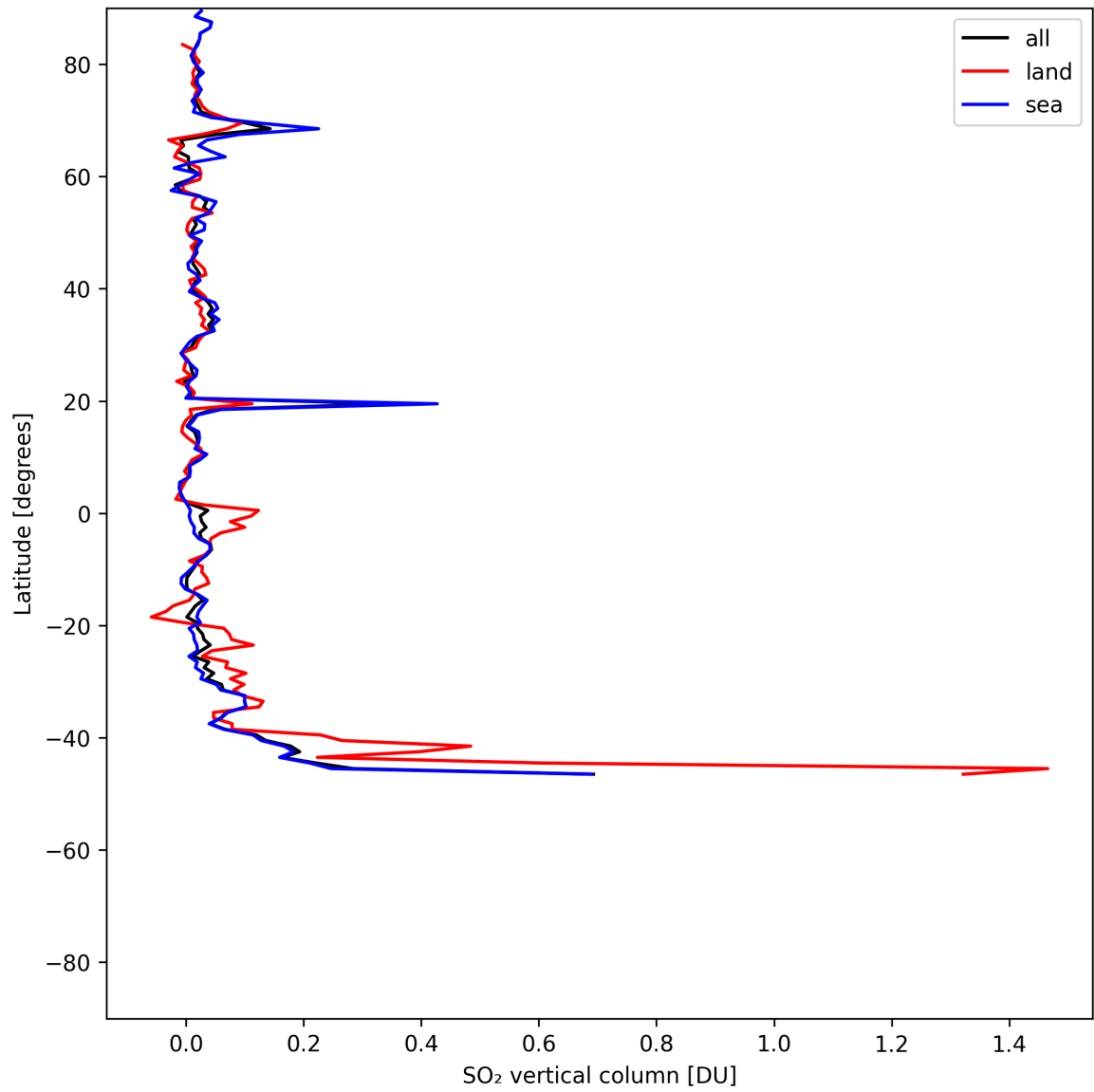
Figure 31: Zonal average of “SO 2 vertical column” for 2025-07-09 to 2025-07-10.
