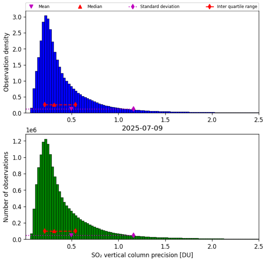
Figure 59: Histogram of “SO 2 vertical column precision” for 2025-07-09 to 2025-07-10
