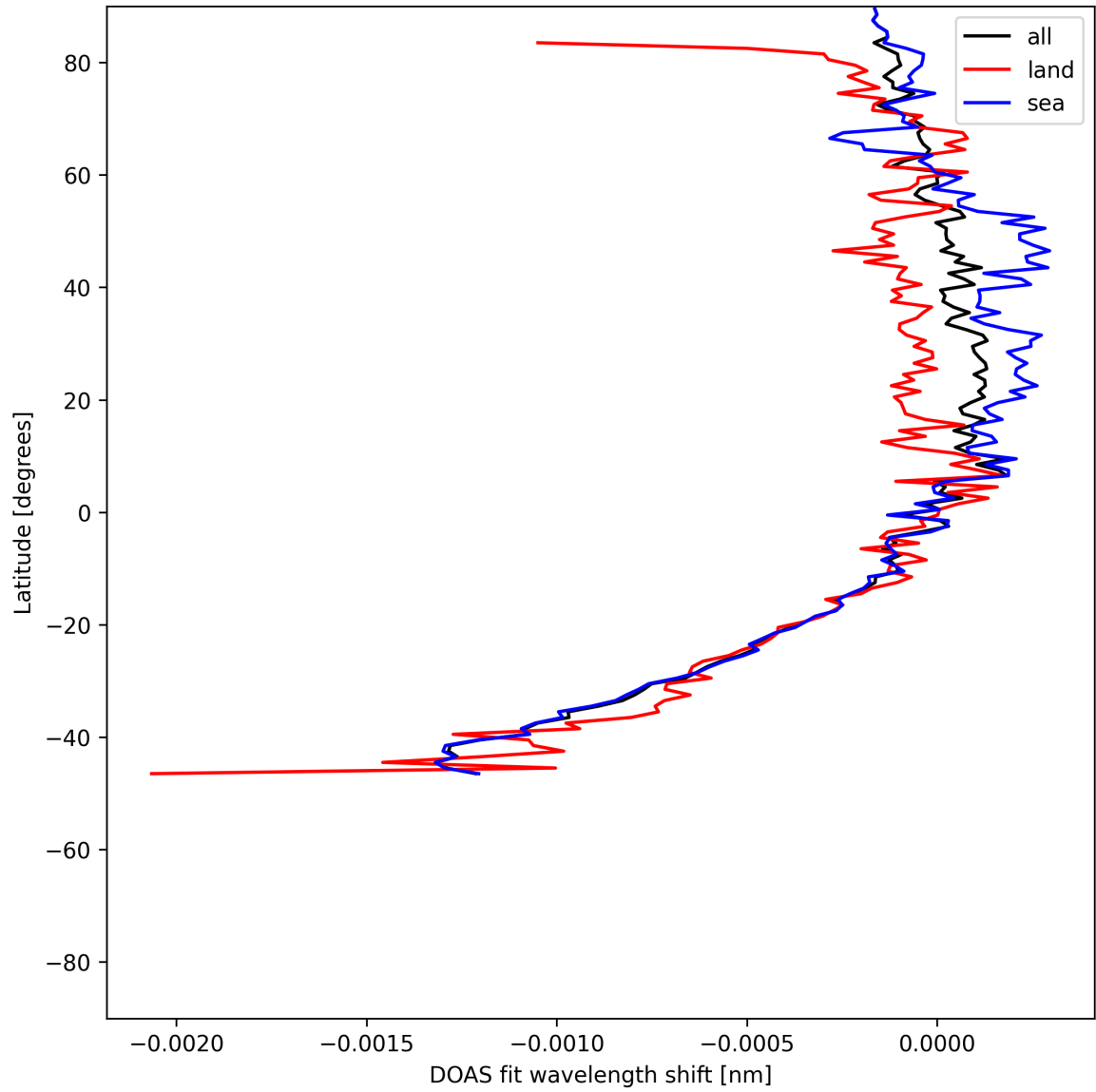
Figure 50: Zonal average of “DOAS fit wavelength shift” for 2025-07-09 to 2025-07-10.
