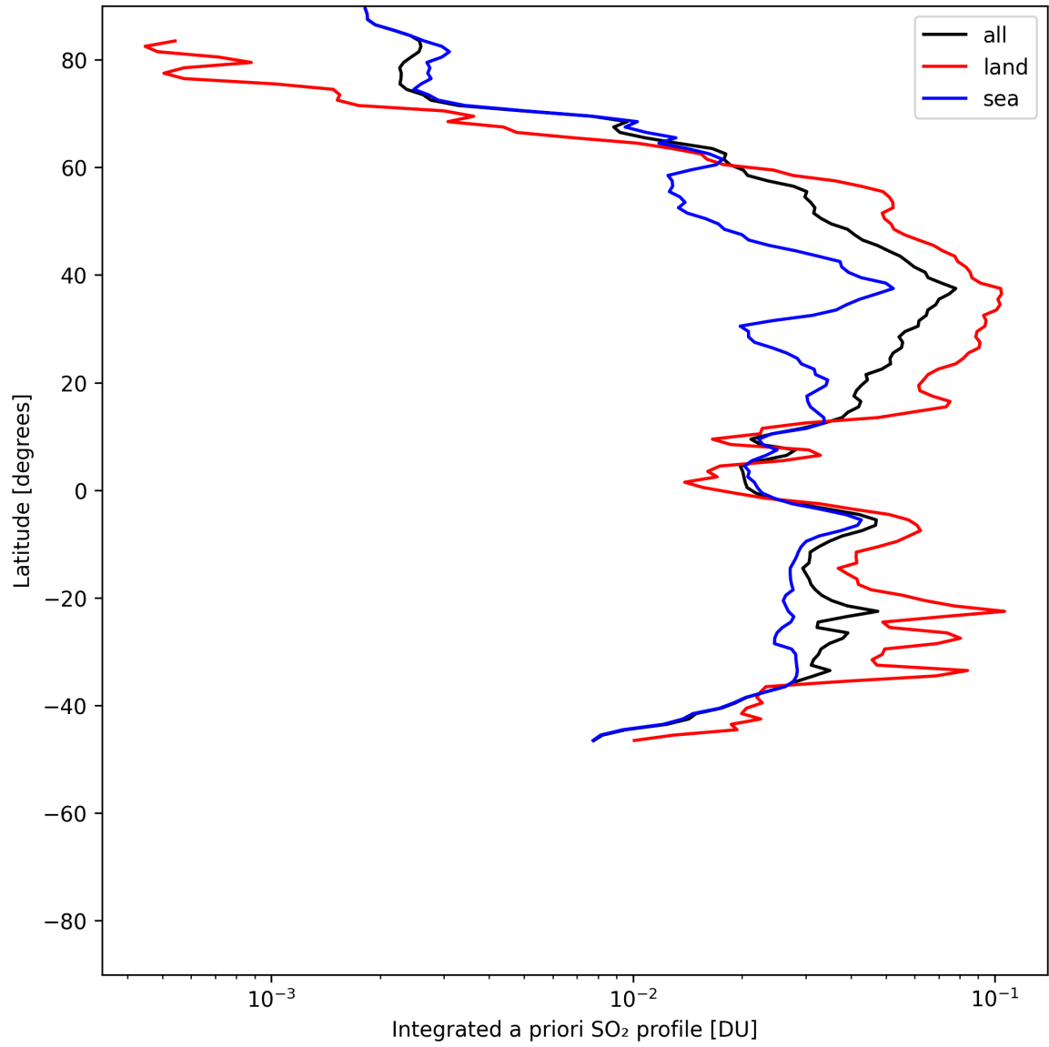
Figure 49: Zonal average of “Integrated a priori SO 2 profile” for 2025-07-09 to 2025-07-10.
