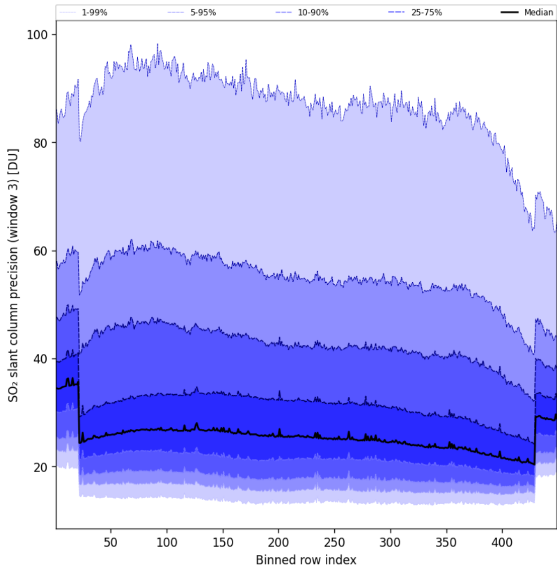
Figure 99: Along track statistics of “SO 2 slant column precision (window 3)” for 2025-07-09 to 2025-07-10
