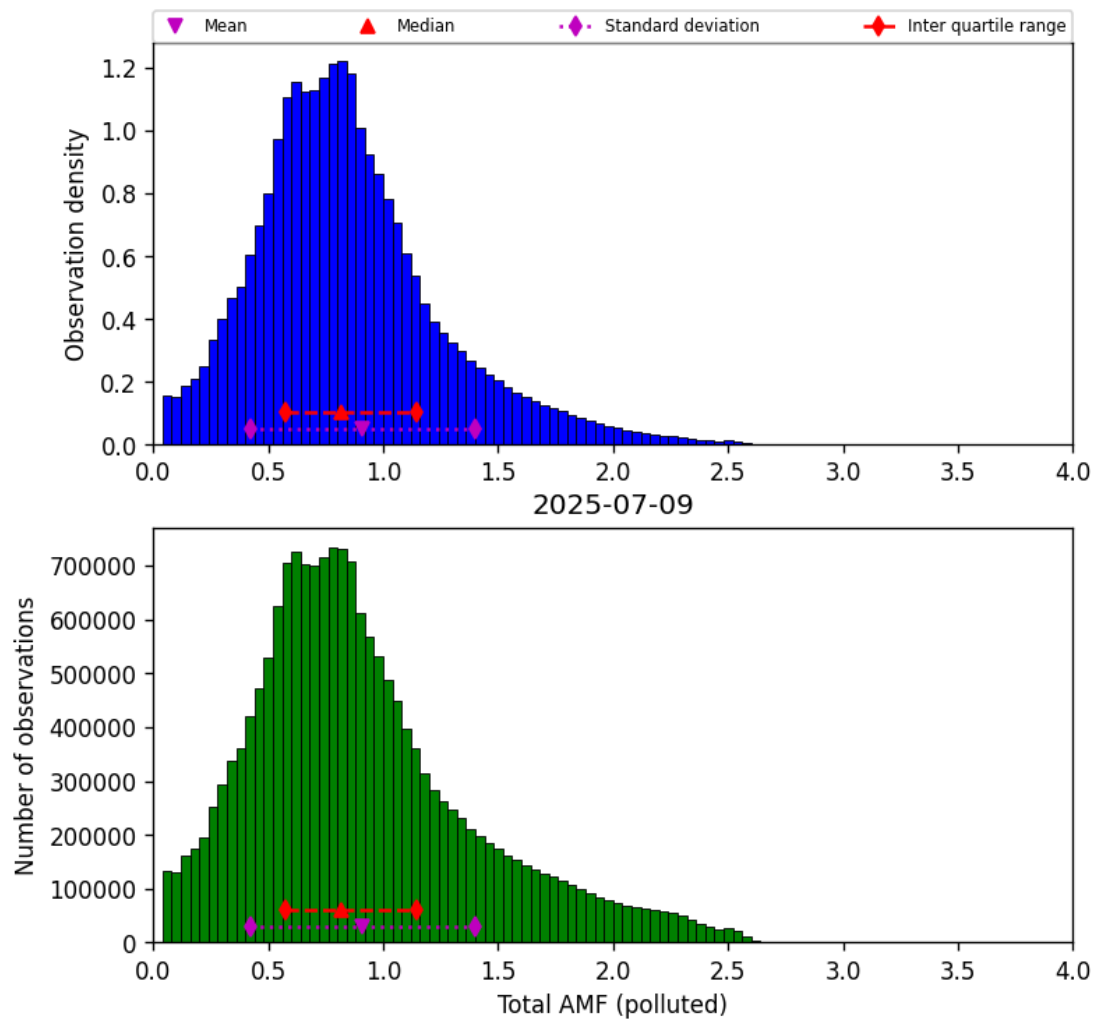
Figure 80: Histogram of “Total AMF (polluted)” for 2025-07-09 to 2025-07-10
