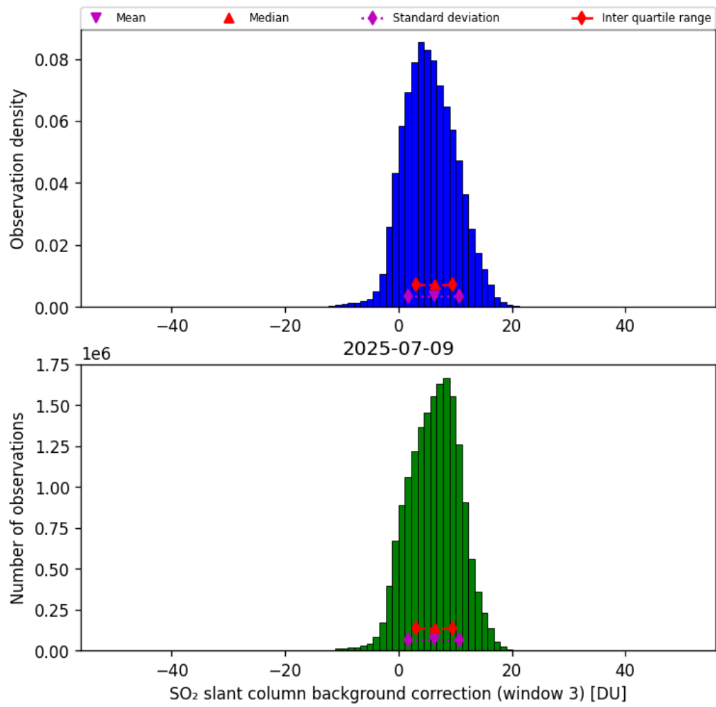
Figure 74: Histogram of “SO 2 slant column background correction (window 3)” for 2025-07-09 to 2025-07-10
