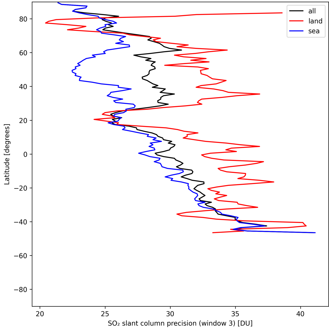
Figure 45: Zonal average of “SO 2 slant column precision (window 3)” for 2025-07-09 to 2025-07-10.
