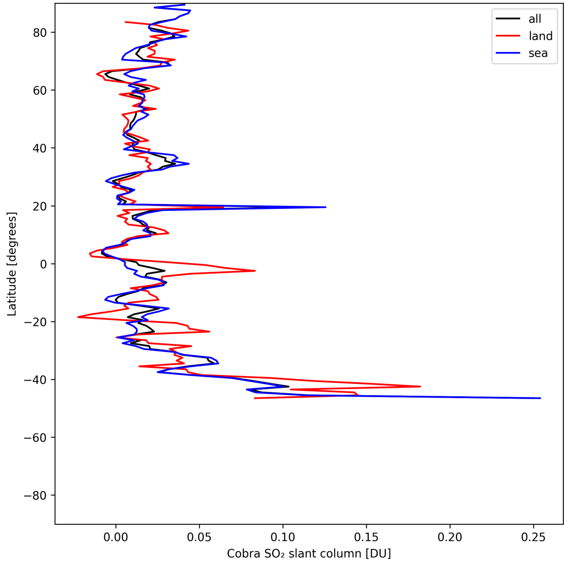
Figure 34: Zonal average of “Cobra SO 2 slant column” for 2025-07-09 to 2025-07-10.
