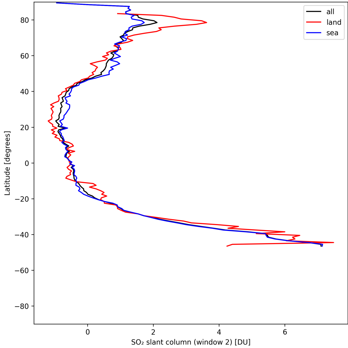
Figure 40: Zonal average of “SO 2 slant column (window 2)” for 2025-07-09 to 2025-07-10.
