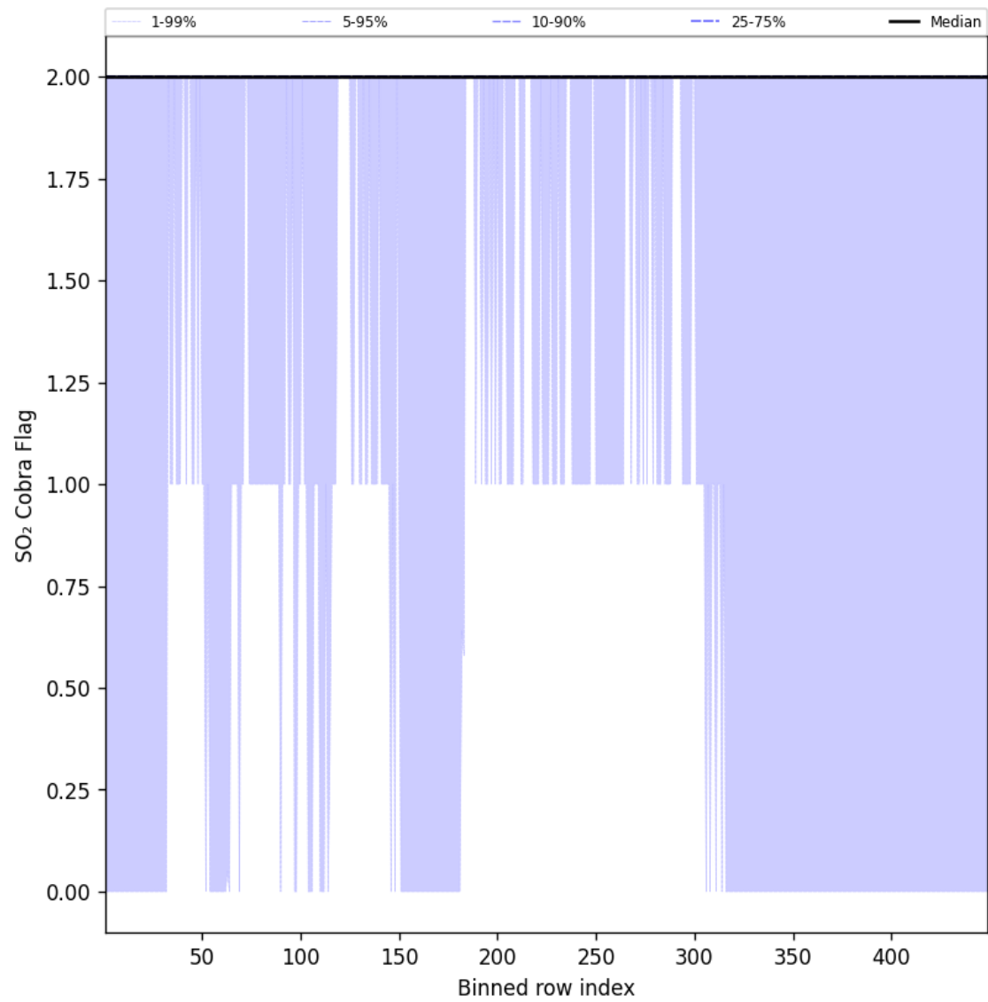
Figure 102: Along track statistics of “SO 2 Cobra Flag” for 2025-07-09 to 2025-07-10
