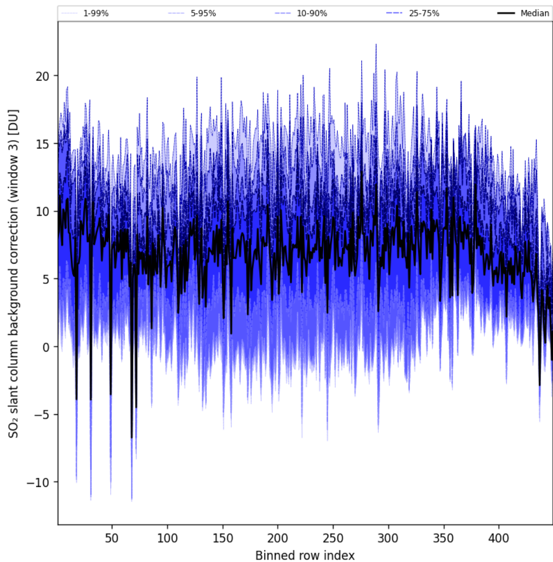
Figure 101: Along track statistics of “SO 2 slant column background correction (window 3)” for 2025-07-09 to 2025-07-10
