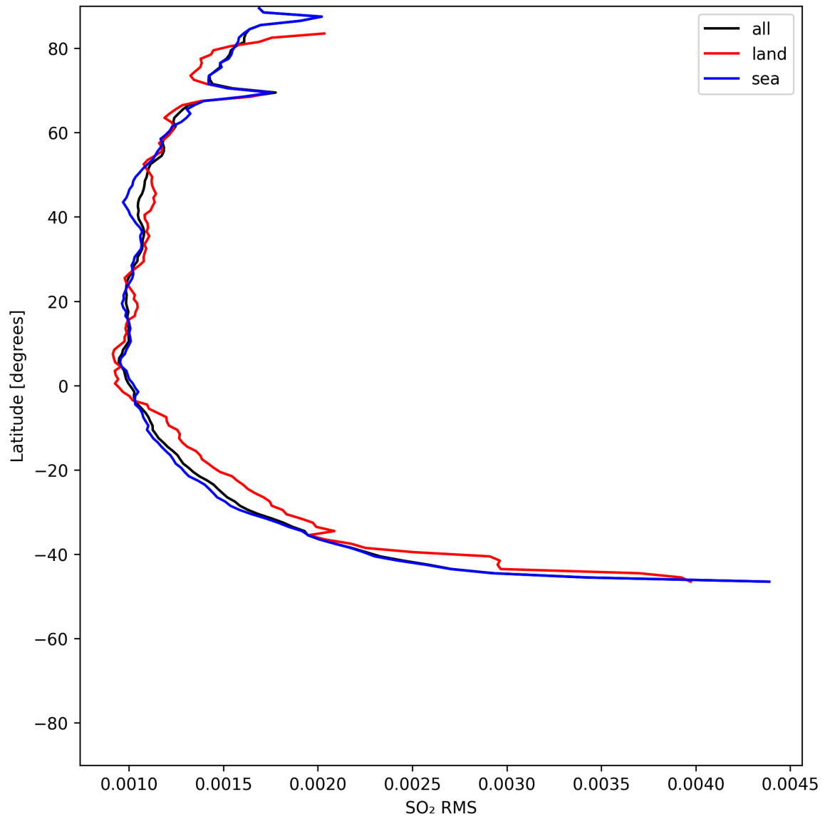
Figure 52: Zonal average of “SO 2 RMS” for 2025-07-09 to 2025-07-10.
