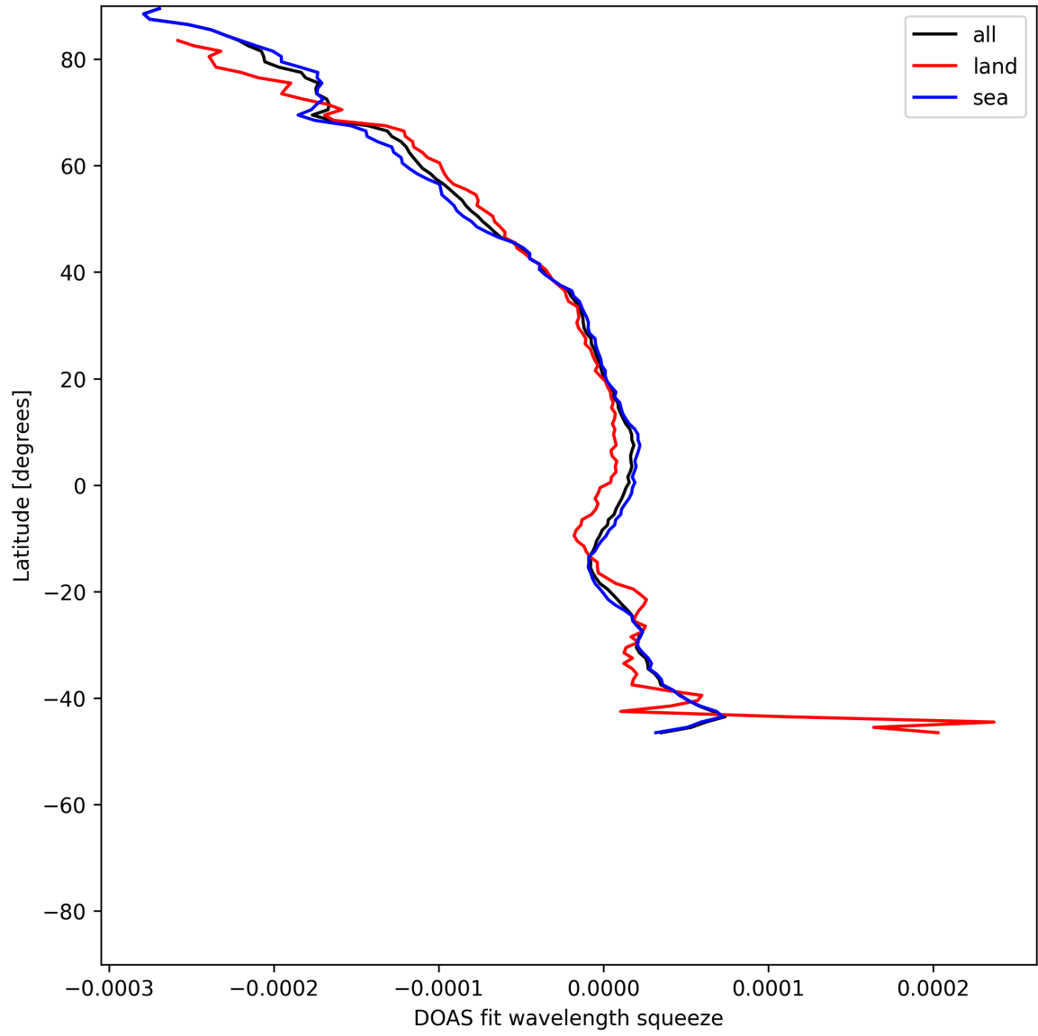
Figure 51: Zonal average of “DOAS fit wavelength squeeze” for 2025-07-09 to 2025-07-10.
