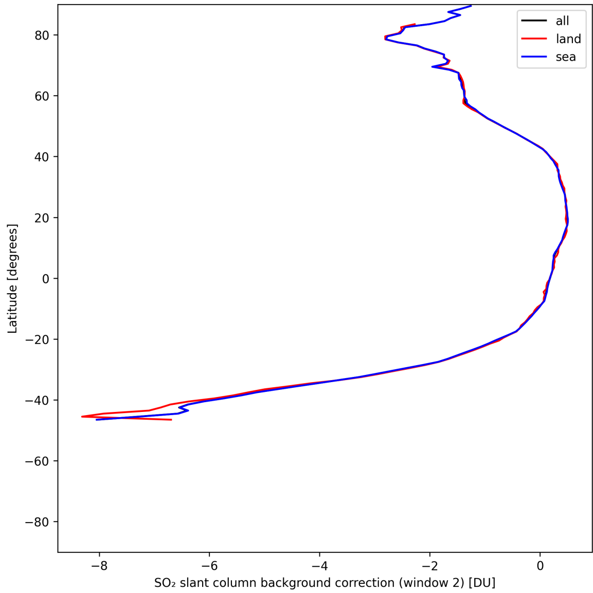
Figure 43: Zonal average of “SO 2 slant column background correction (window 2)” for 2025-07-09 to 2025-07-10.
