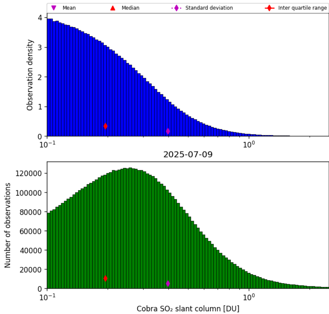
Figure 61: Histogram of “Cobra SO 2 slant column” for 2025-07-09 to 2025-07-10
