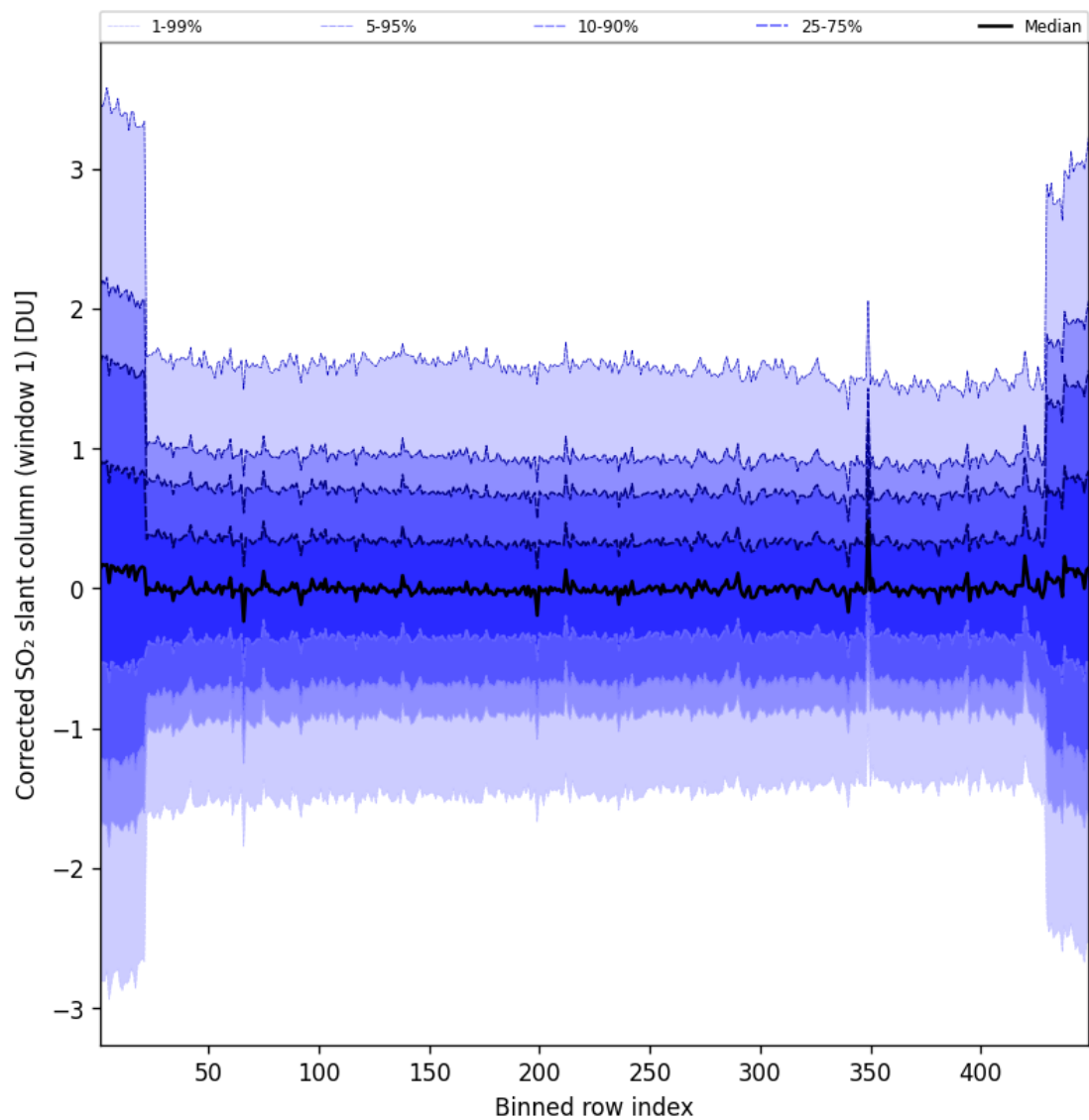
Figure 92: Along track statistics of “Corrected SO 2 slant column (window 1)” for 2025-07-09 to 2025-07-10
