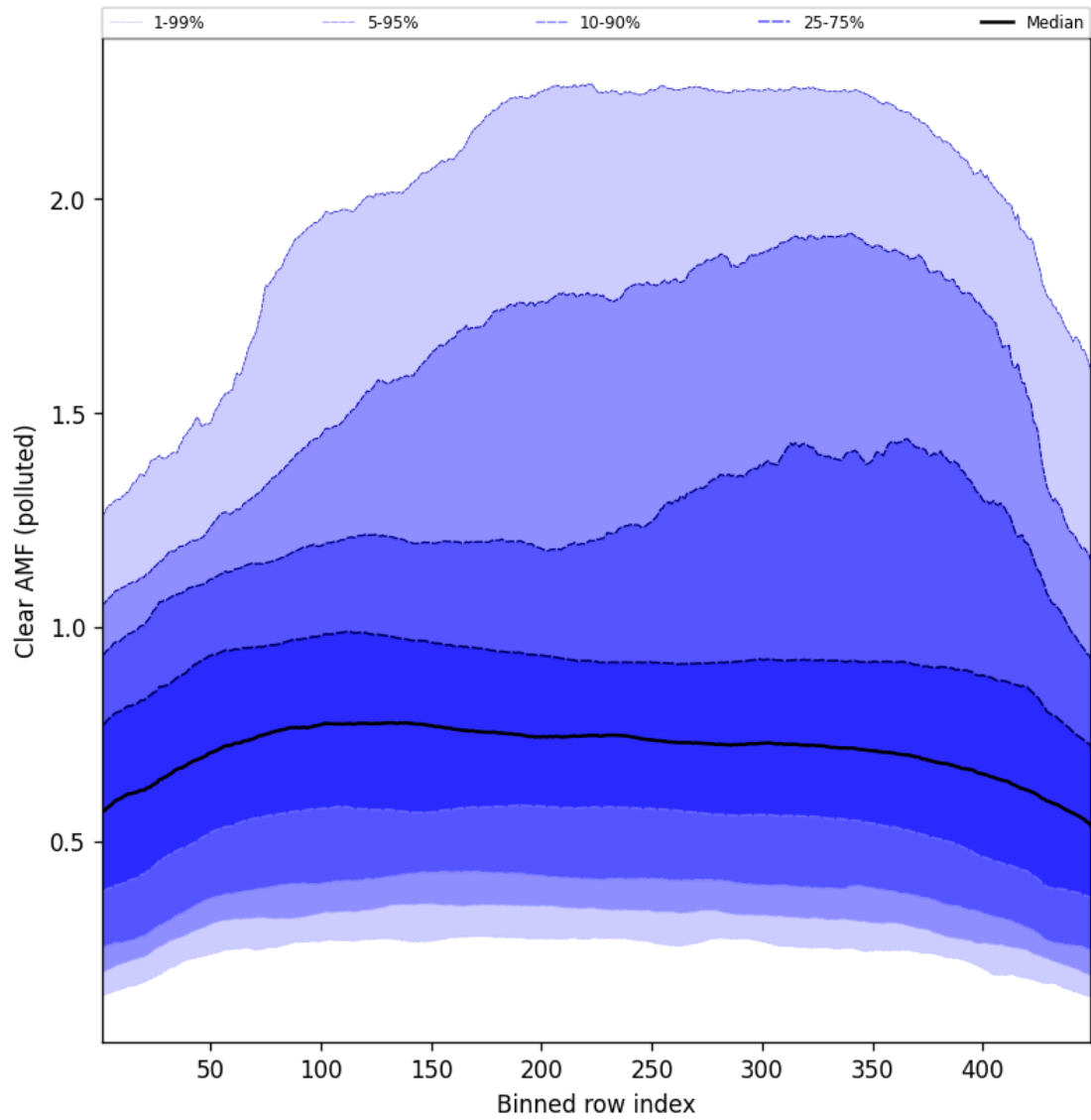
Figure 109: Along track statistics of “Clear AMF (polluted)” for 2025-07-09 to 2025-07-10
