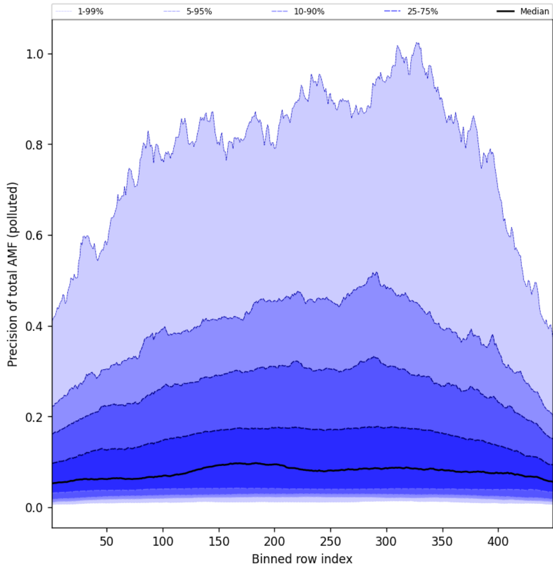
Figure 108: Along track statistics of “Precision of total AMF (polluted)” for 2025-07-09 to 2025-07-10
