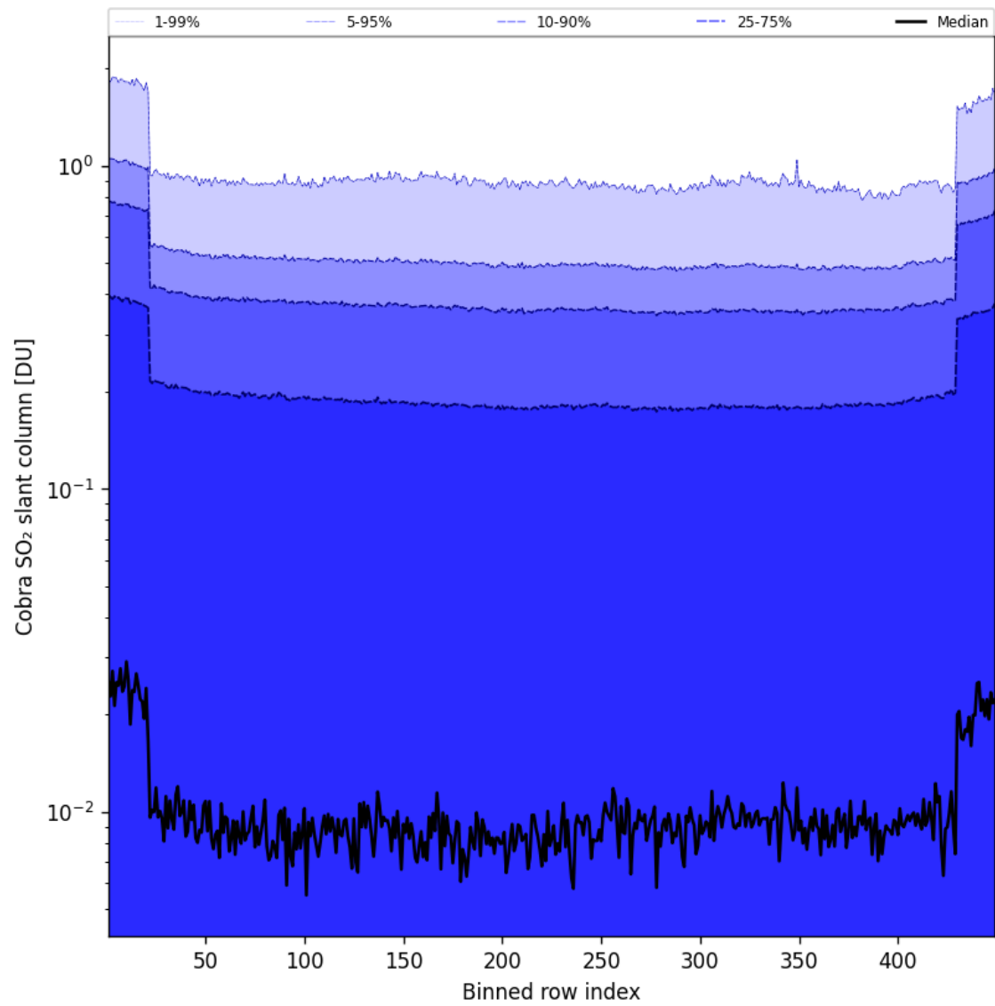
Figure 88: Along track statistics of “Cobra SO 2 slant column” for 2025-07-09 to 2025-07-10
