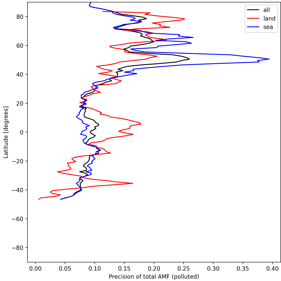
Figure 54: Zonal average of “Precision of total AMF (polluted)” for 2025-07-09 to 2025-07-10.
