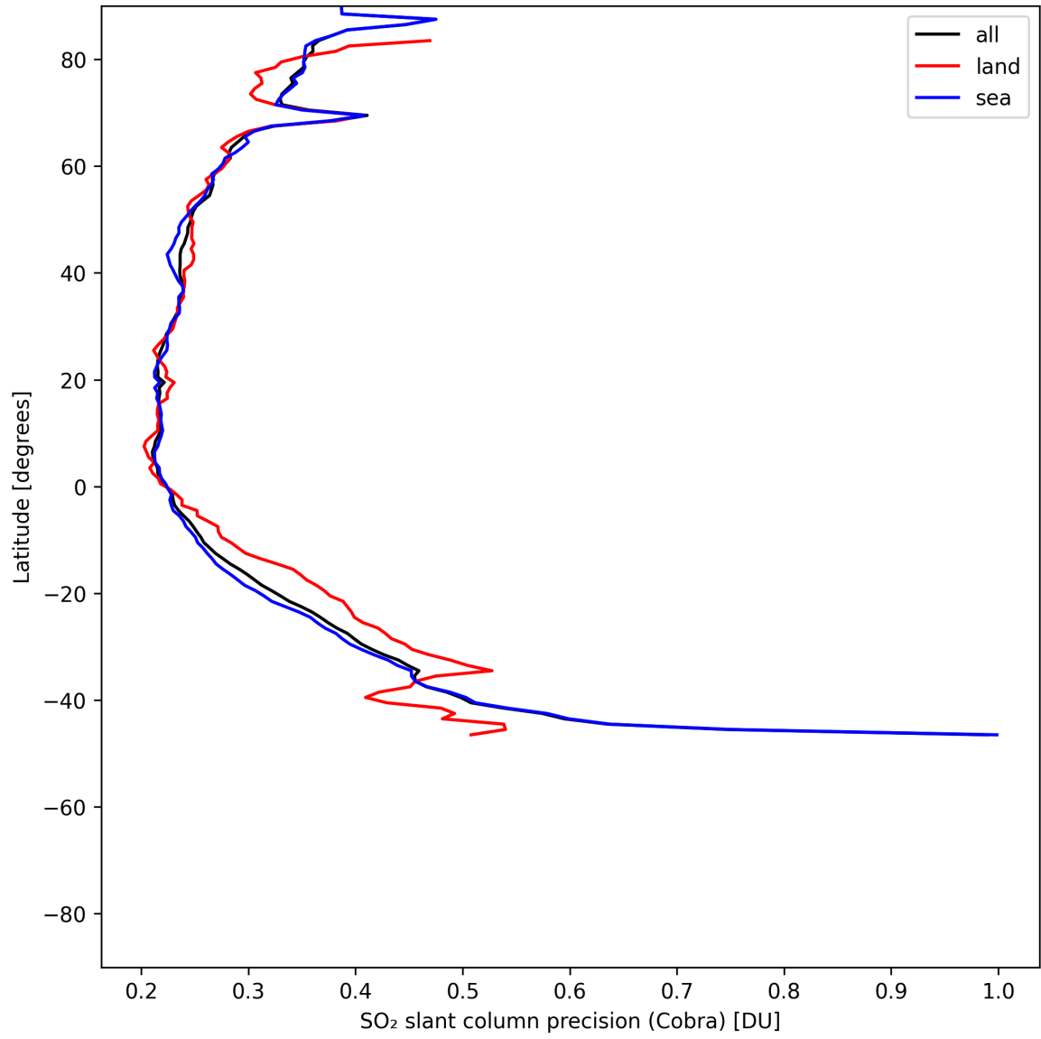
Figure 35: Zonal average of “SO 2 slant column precision (Cobra)” for 2025-07-09 to 2025-07-10.
