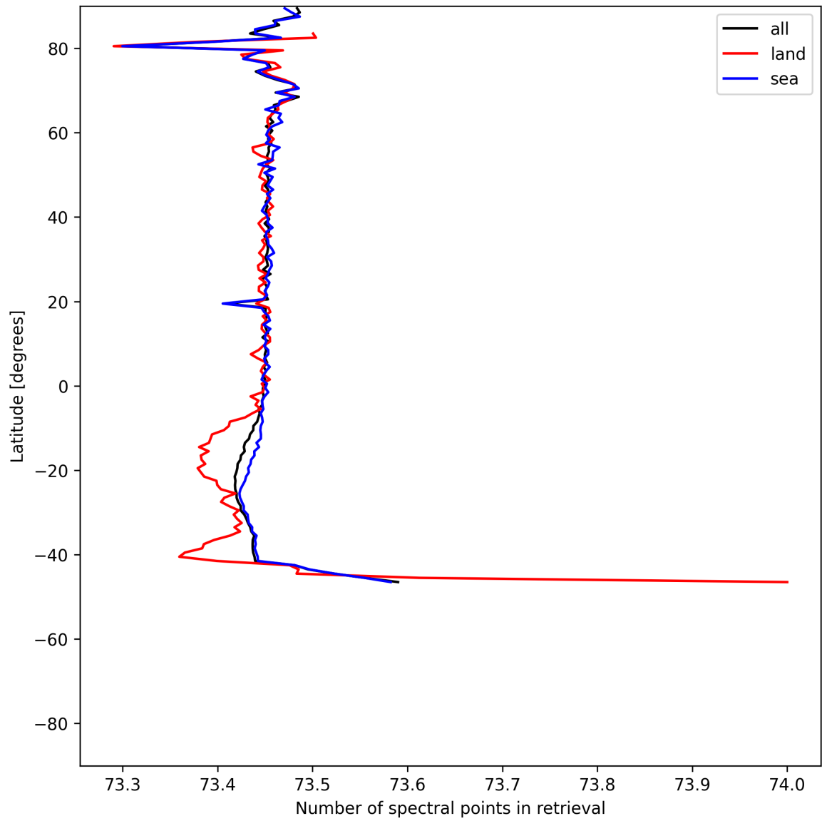
Figure 56: Zonal average of “Number of spectral points in retrieval” for 2025-07-09 to 2025-07-10.
