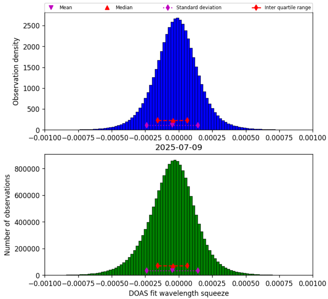
Figure 78: Histogram of “DOAS fit wavelength squeeze” for 2025-07-09 to 2025-07-10
