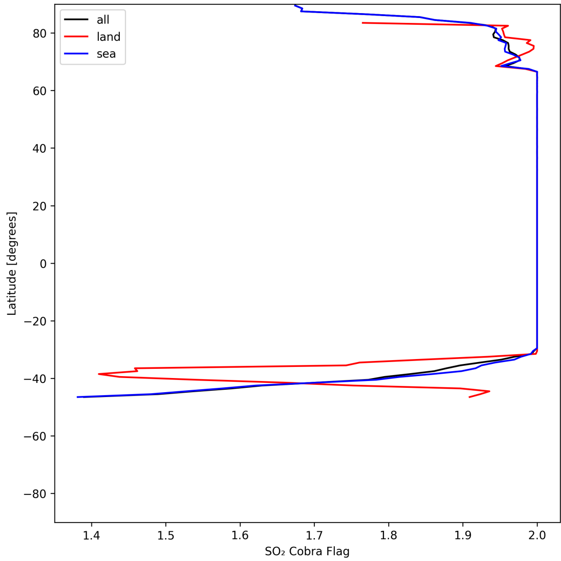
Figure 48: Zonal average of “SO 2 Cobra Flag” for 2025-07-09 to 2025-07-10.
