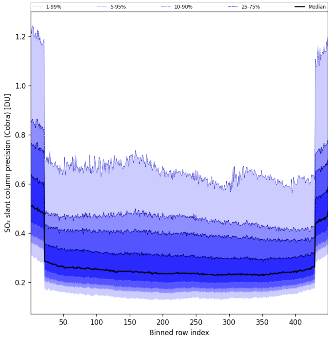
Figure 89: Along track statistics of “SO 2 slant column precision (Cobra)” for 2025-07-09 to 2025-07-10
