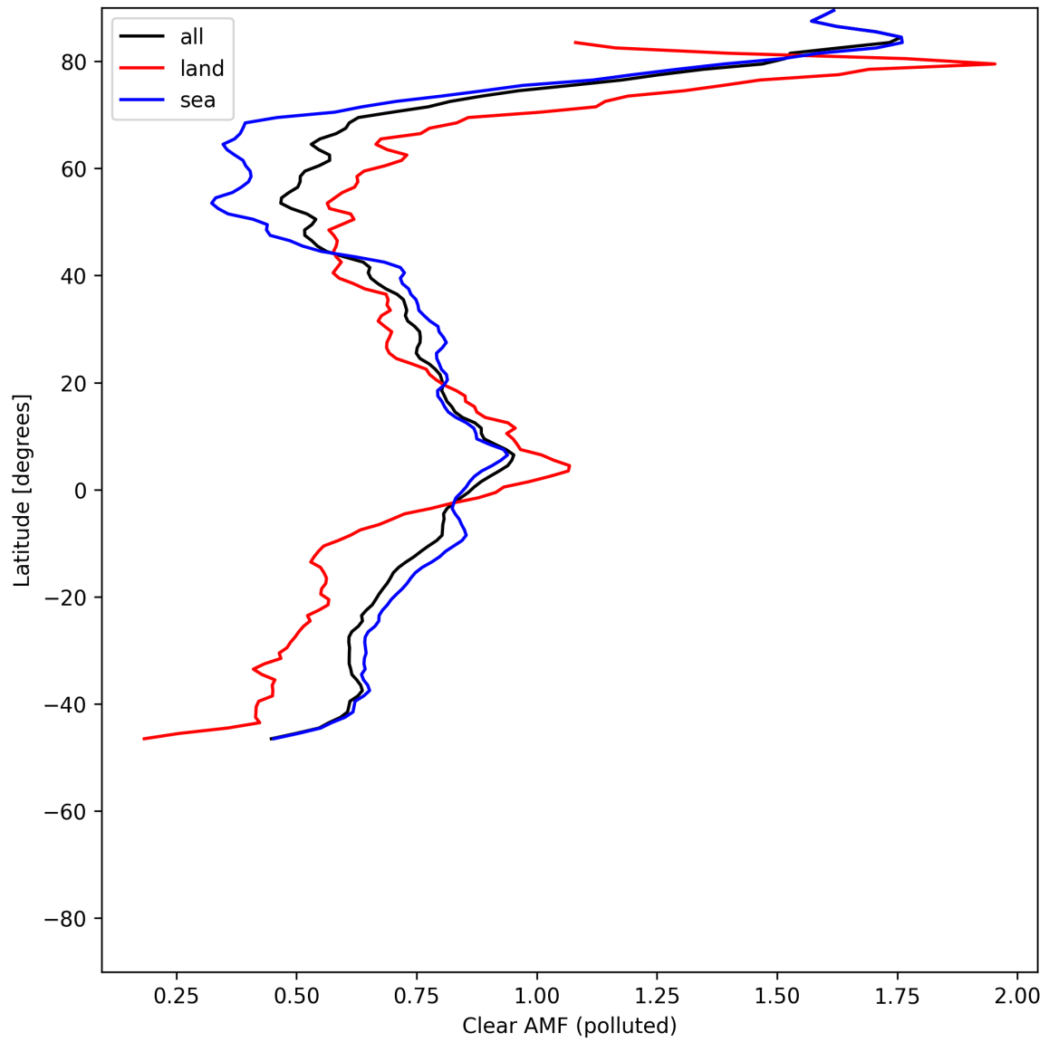
Figure 55: Zonal average of “Clear AMF (polluted)” for 2025-07-09 to 2025-07-10.
