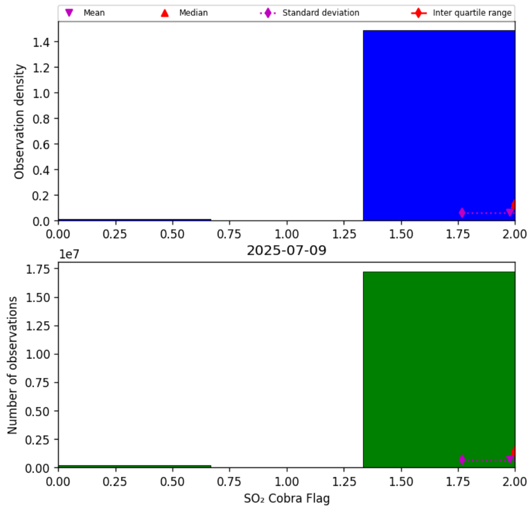
Figure 75: Histogram of “SO 2 Cobra Flag” for 2025-07-09 to 2025-07-10
