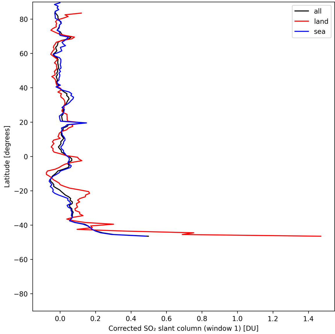
Figure 38: Zonal average of “Corrected SO 2 slant column (window 1)” for 2025-07-09 to 2025-07-10.
