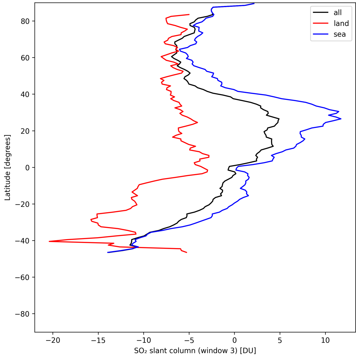
Figure 44: Zonal average of “SO 2 slant column (window 3)” for 2025-07-09 to 2025-07-10.
