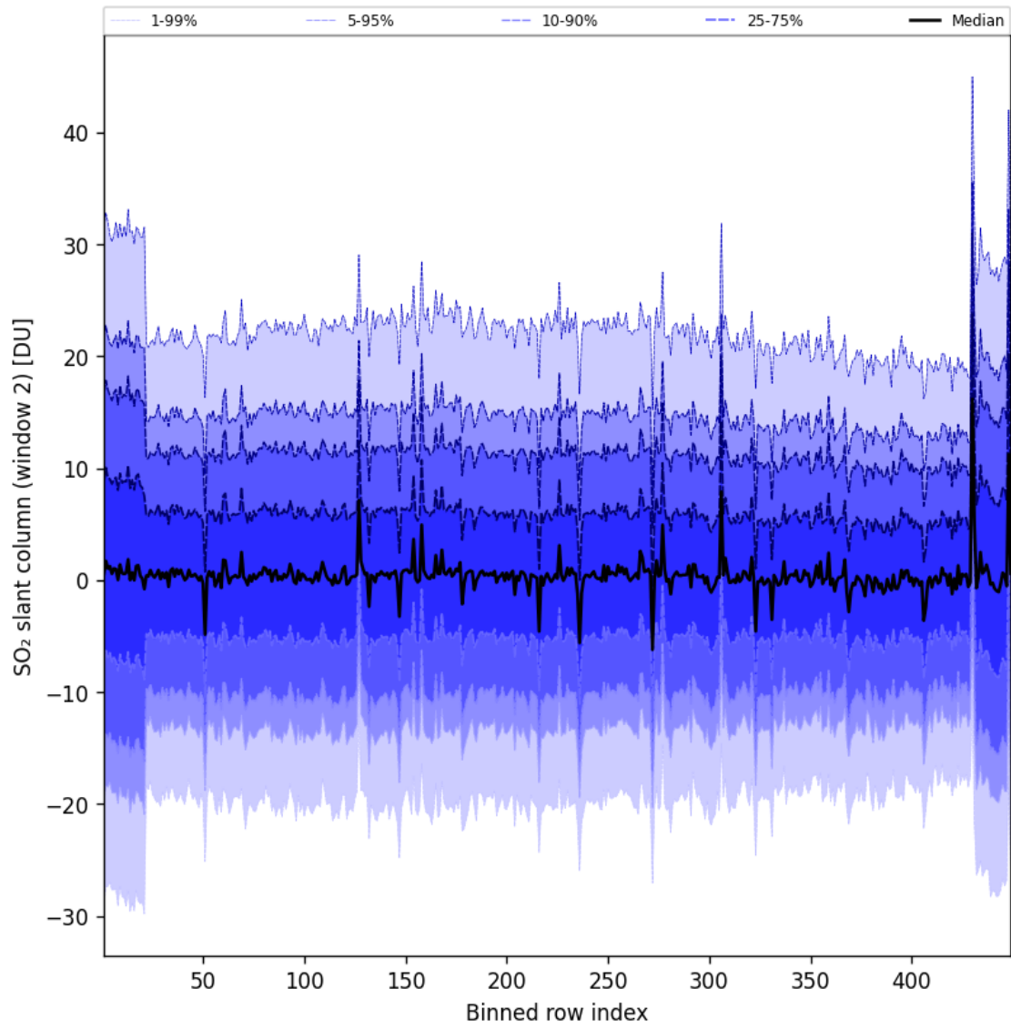
Figure 94: Along track statistics of “SO 2 slant column (window 2)” for 2025-07-09 to 2025-07-10
