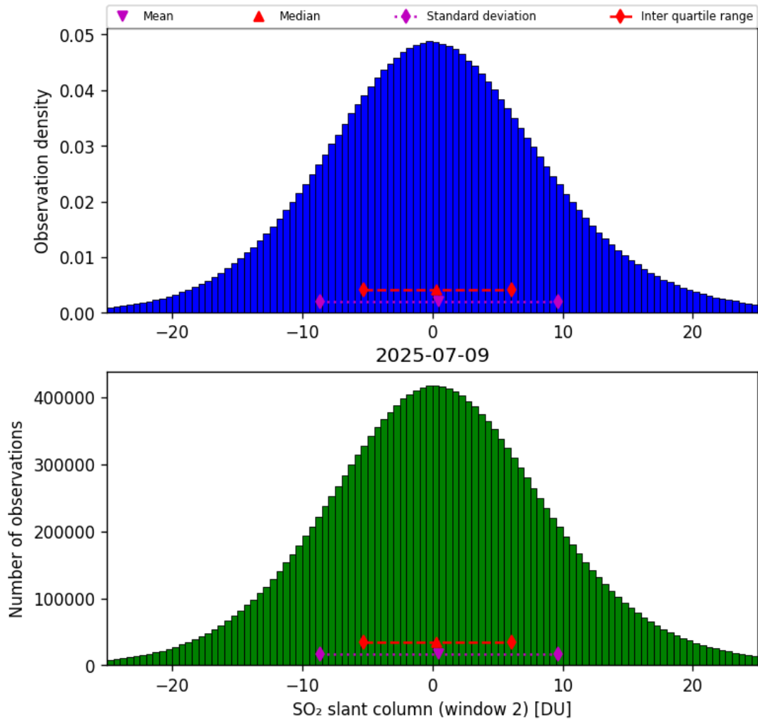
Figure 67: Histogram of “SO 2 slant column (window 2)” for 2025-07-09 to 2025-07-10
