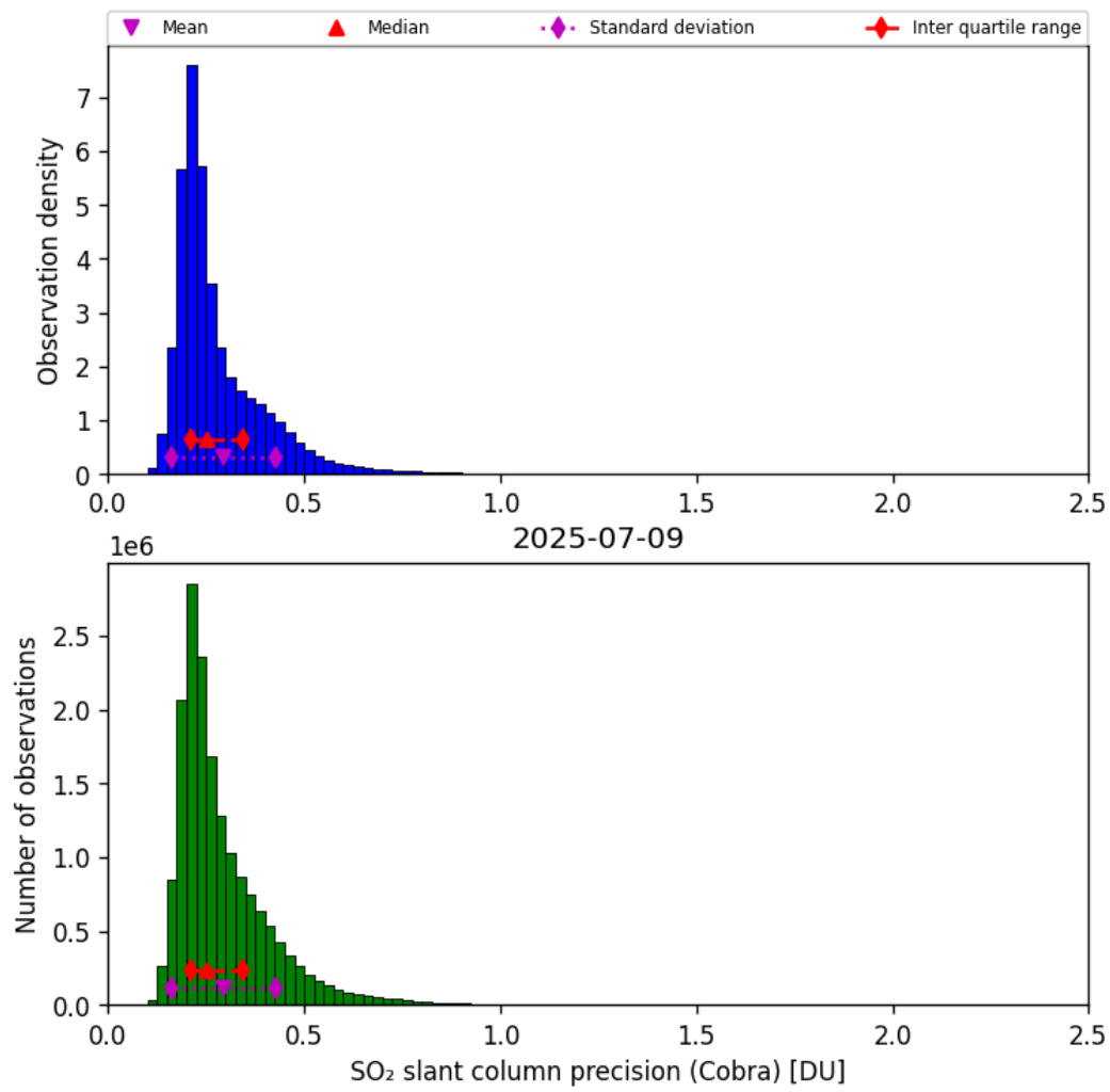
Figure 62: Histogram of “SO 2 slant column precision (Cobra)” for 2025-07-09 to 2025-07-10
