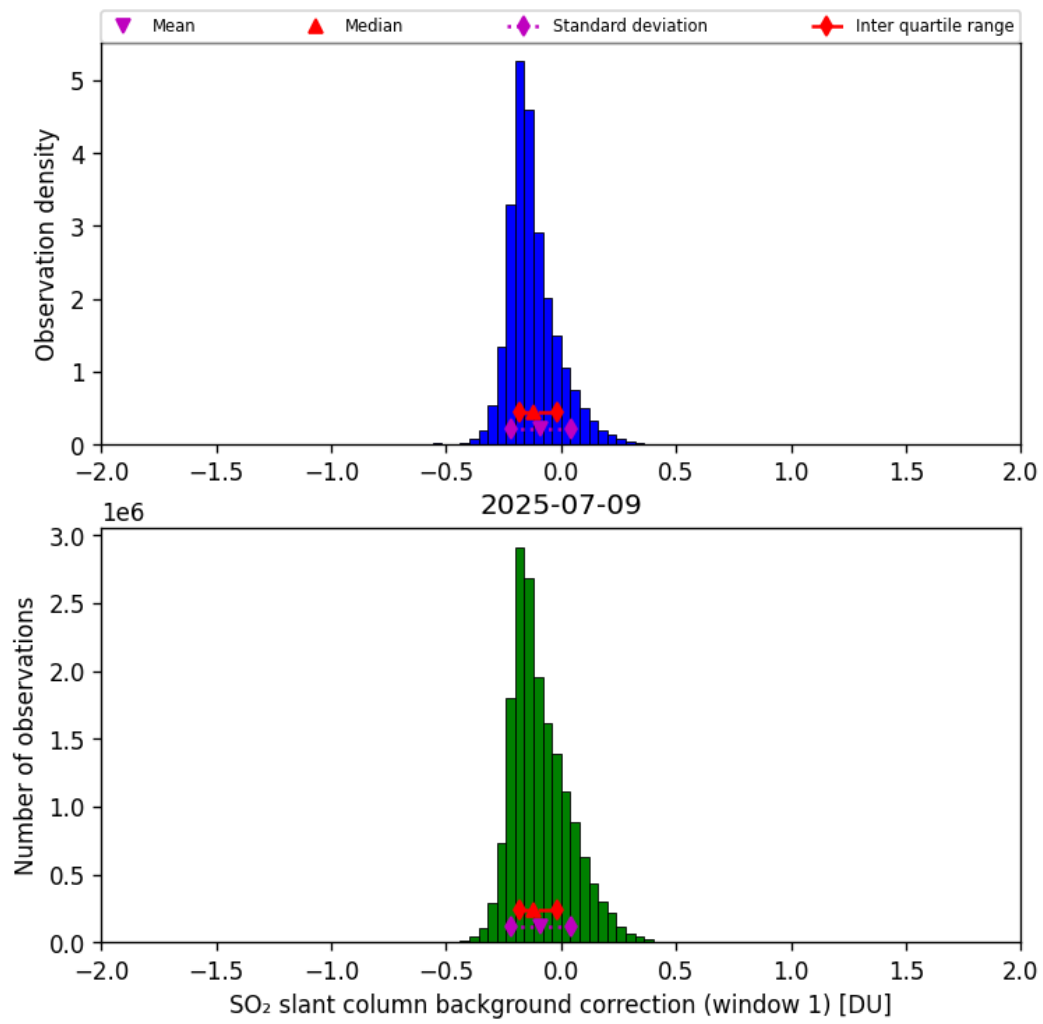
Figure 66: Histogram of “SO 2 slant column background correction (window 1)” for 2025-07-09 to 2025-07-10
