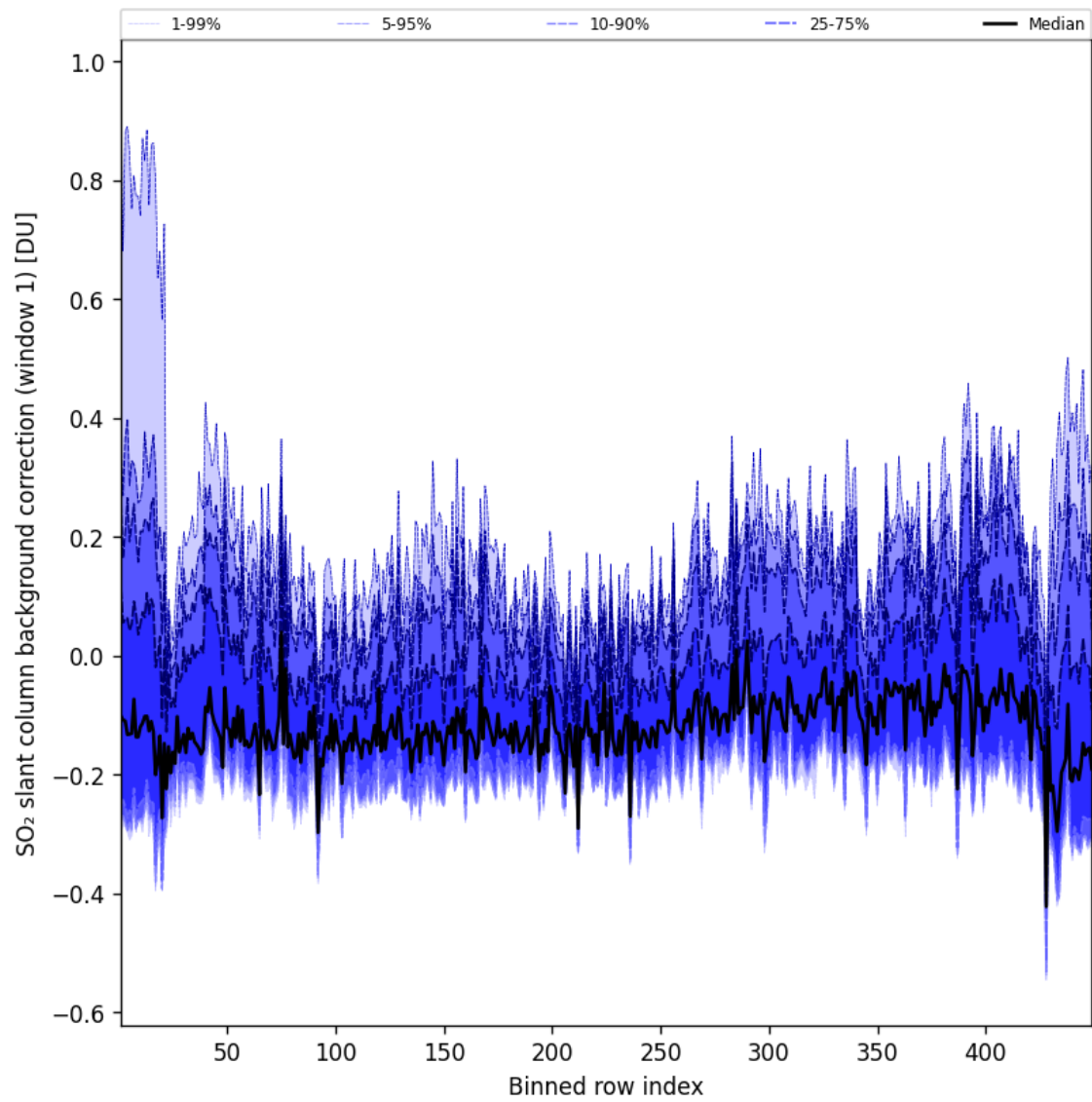
Figure 93: Along track statistics of “SO 2 slant column background correction (window 1)” for 2025-07-09 to 2025-07-10
