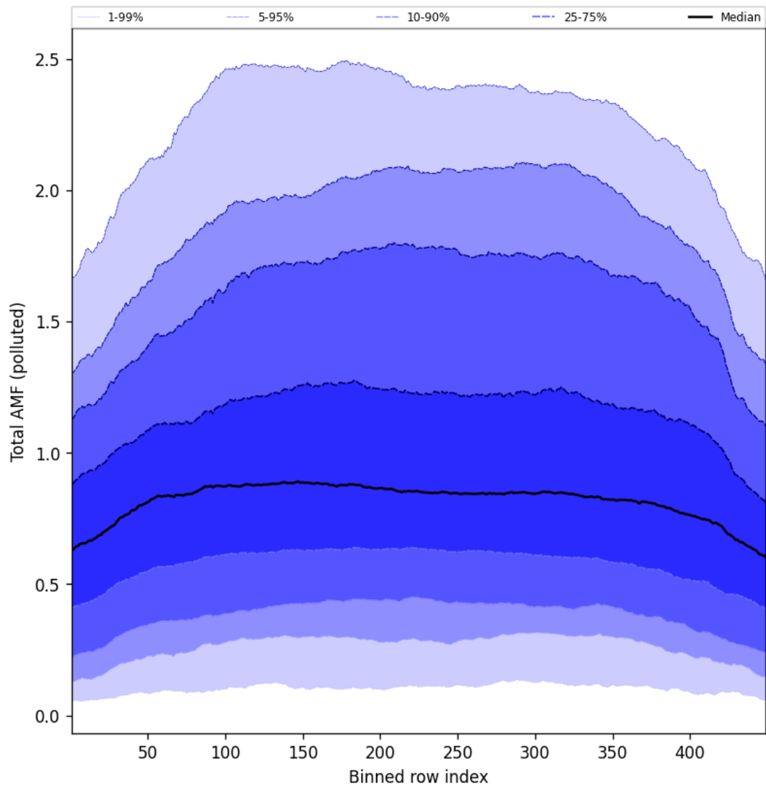
Figure 107: Along track statistics of “Total AMF (polluted)” for 2025-07-09 to 2025-07-10
