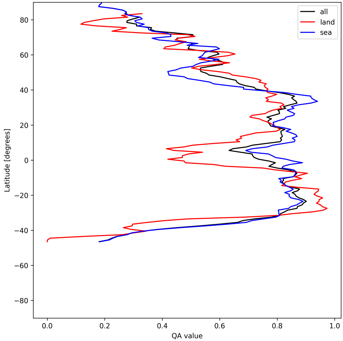
Figure 30: Zonal average of “QA value” for 2025-07-09 to 2025-07-10.
