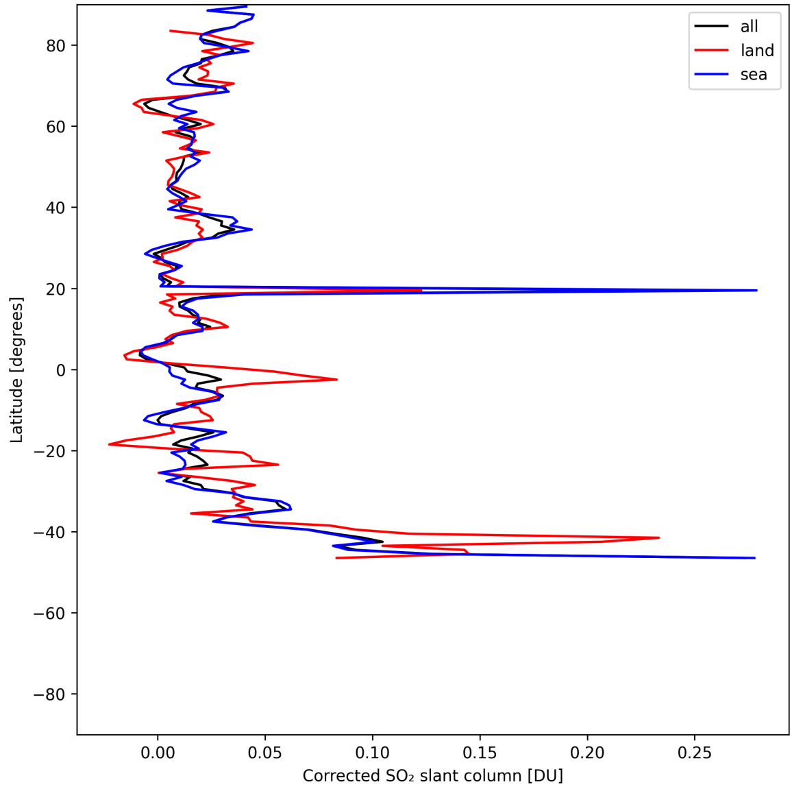
Figure 33: Zonal average of “Corrected SO 2 slant column” for 2025-07-09 to 2025-07-10.
