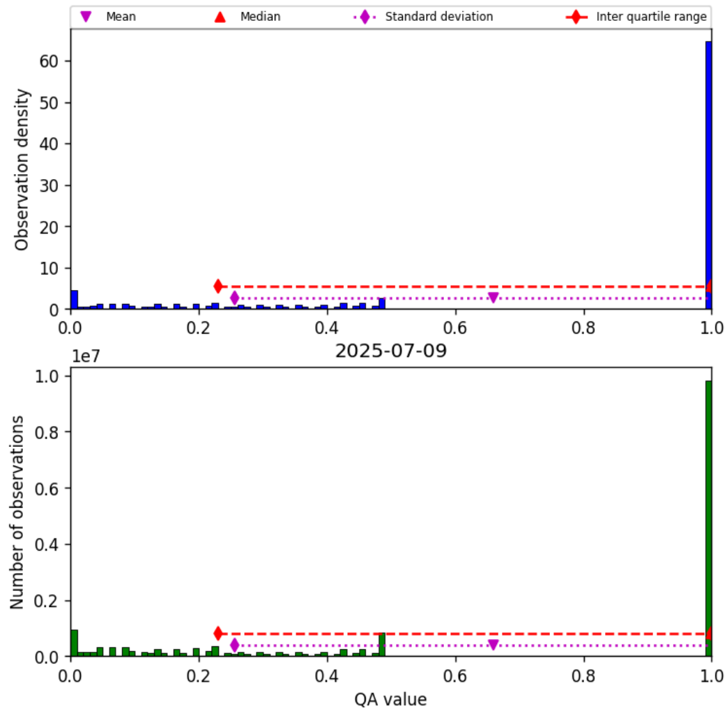
Figure 57: Histogram of “QA value” for 2025-07-09 to 2025-07-10
