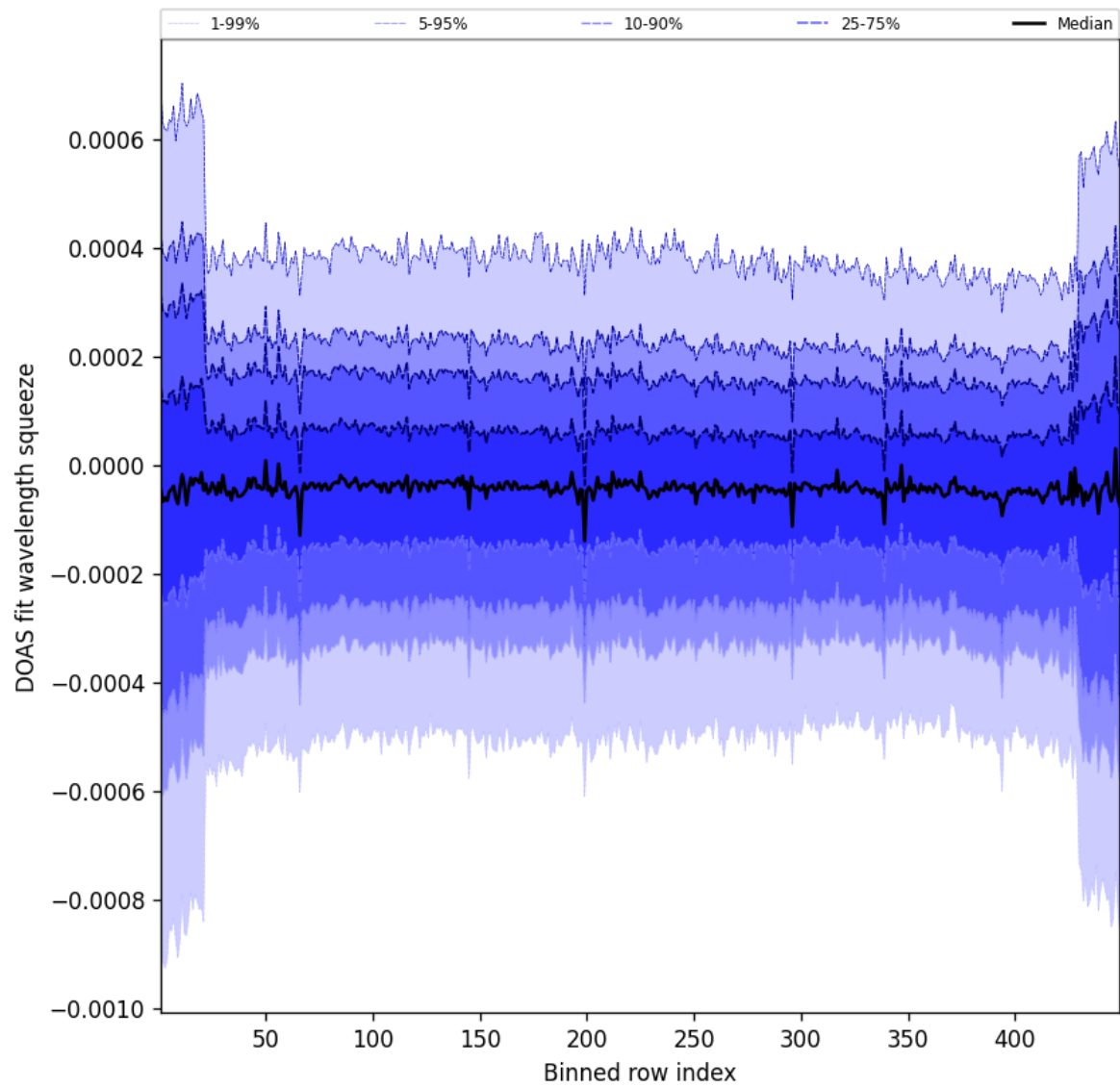
Figure 105: Along track statistics of “DOAS fit wavelength squeeze” for 2025-07-09 to 2025-07-10
