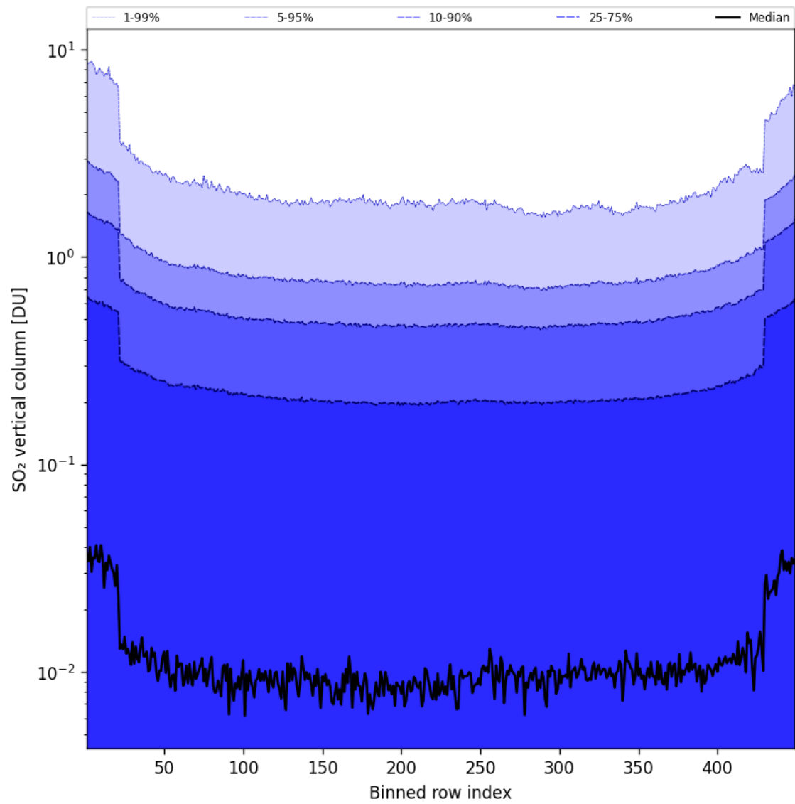
Figure 85: Along track statistics of “SO 2 vertical column” for 2025-07-09 to 2025-07-10
