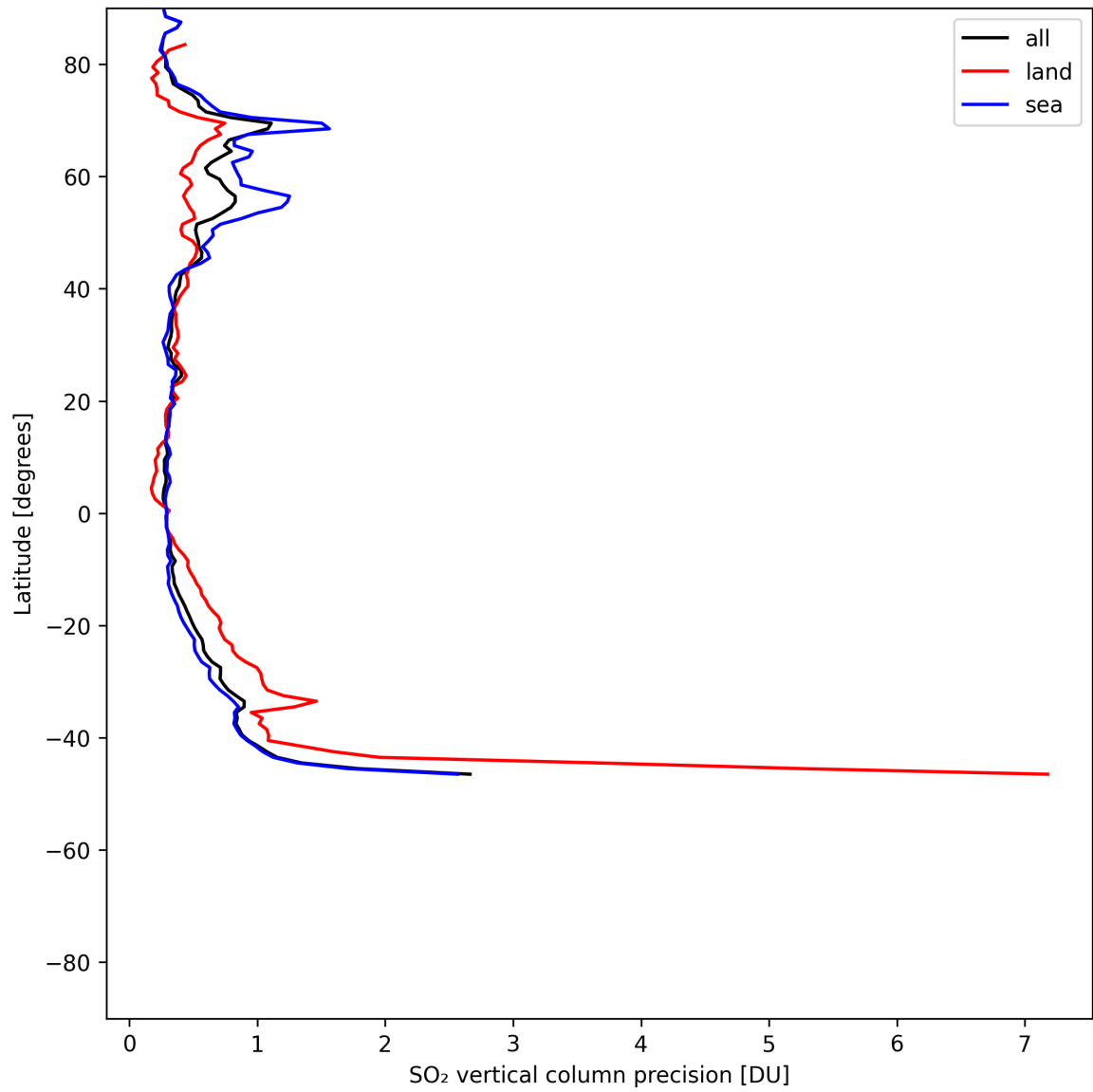
Figure 32: Zonal average of “SO 2 vertical column precision” for 2025-07-09 to 2025-07-10.
