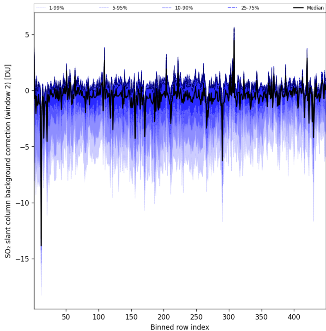
Figure 97: Along track statistics of “SO 2 slant column background correction (window 2)” for 2025-07-09 to 2025-07-10
