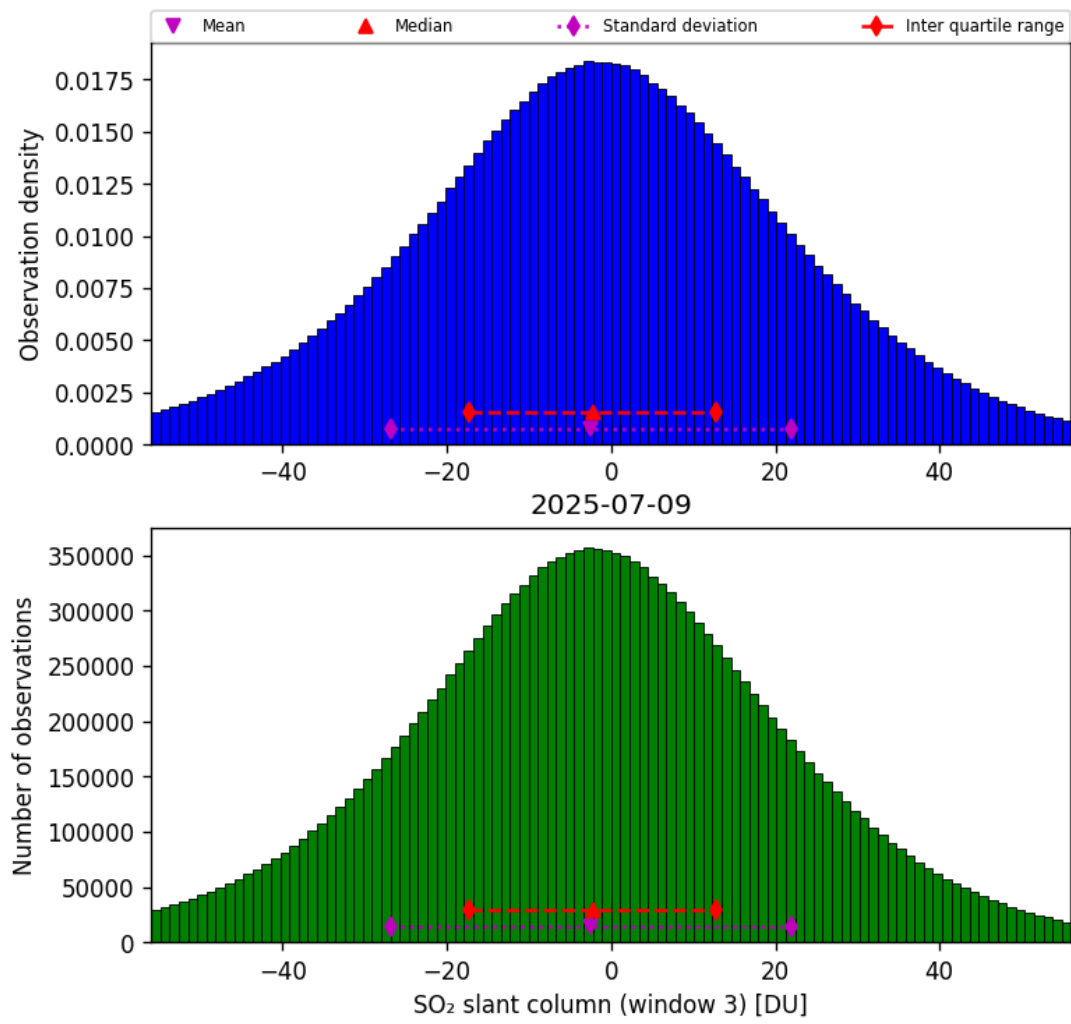
Figure 71: Histogram of “SO 2 slant column (window 3)” for 2025-07-09 to 2025-07-10
