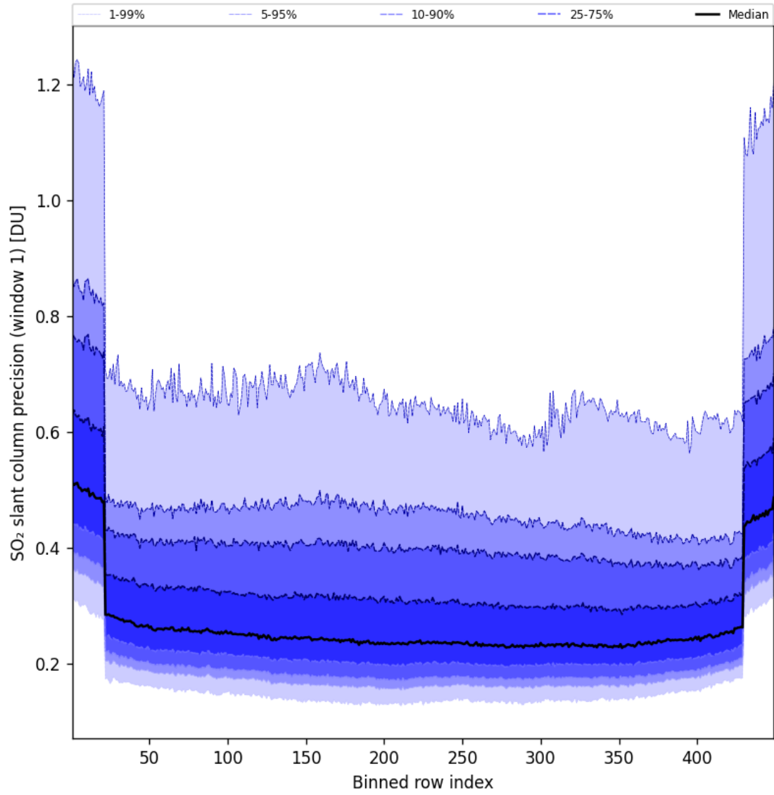
Figure 91: Along track statistics of “SO 2 slant column precision (window 1)” for 2025-07-09 to 2025-07-10
