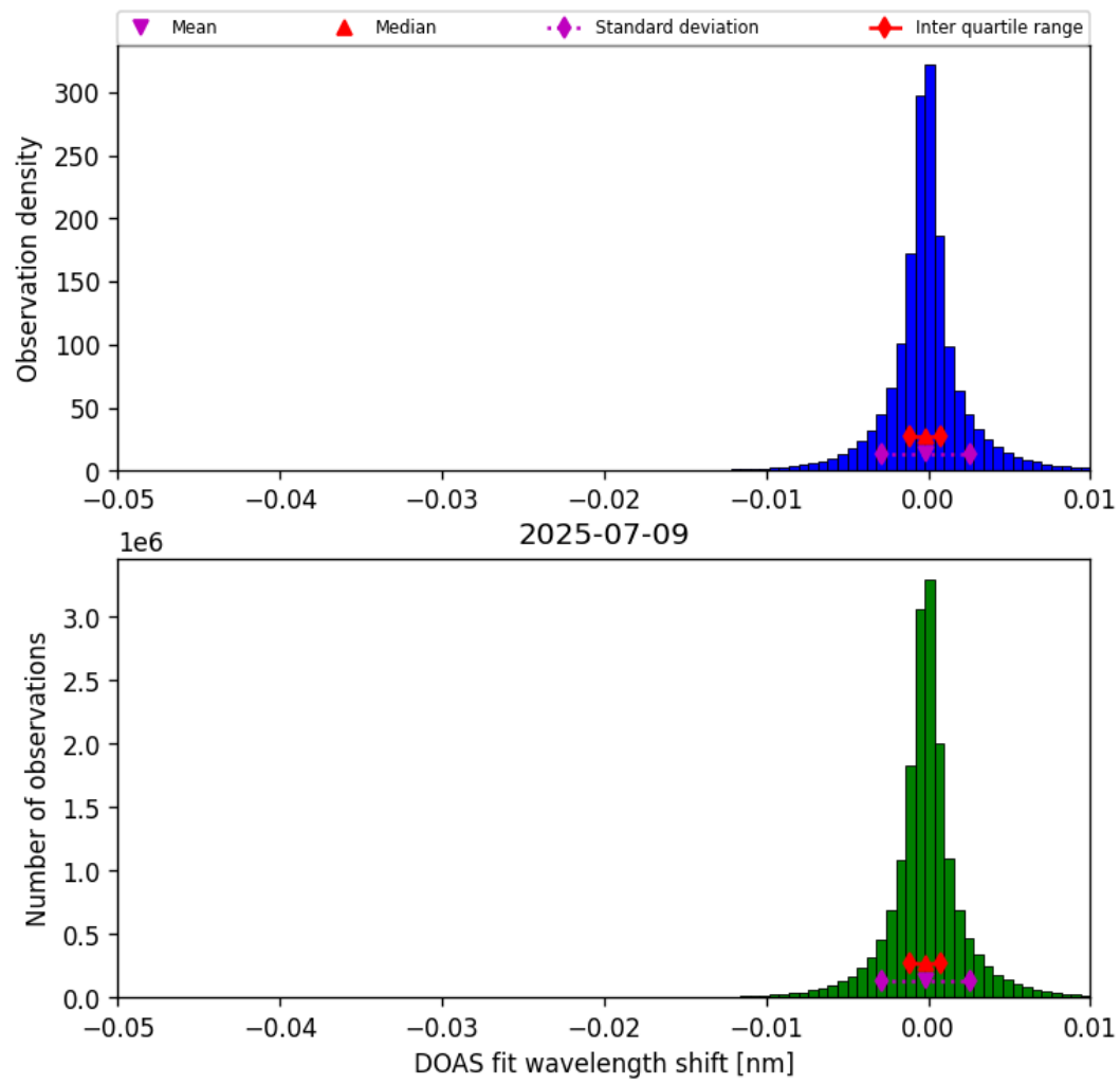
Figure 77: Histogram of “DOAS fit wavelength shift” for 2025-07-09 to 2025-07-10
