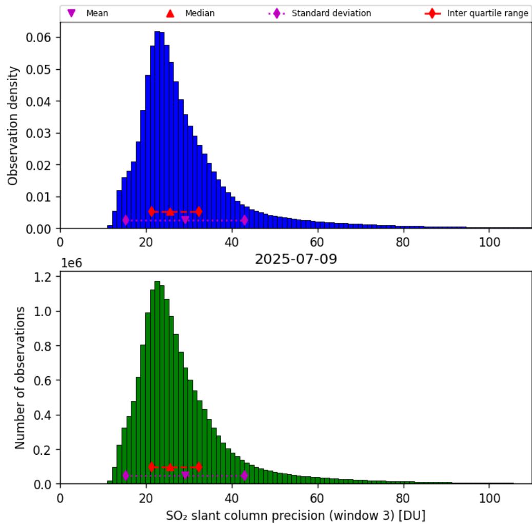
Figure 72: Histogram of “SO 2 slant column precision (window 3)” for 2025-07-09 to 2025-07-10
