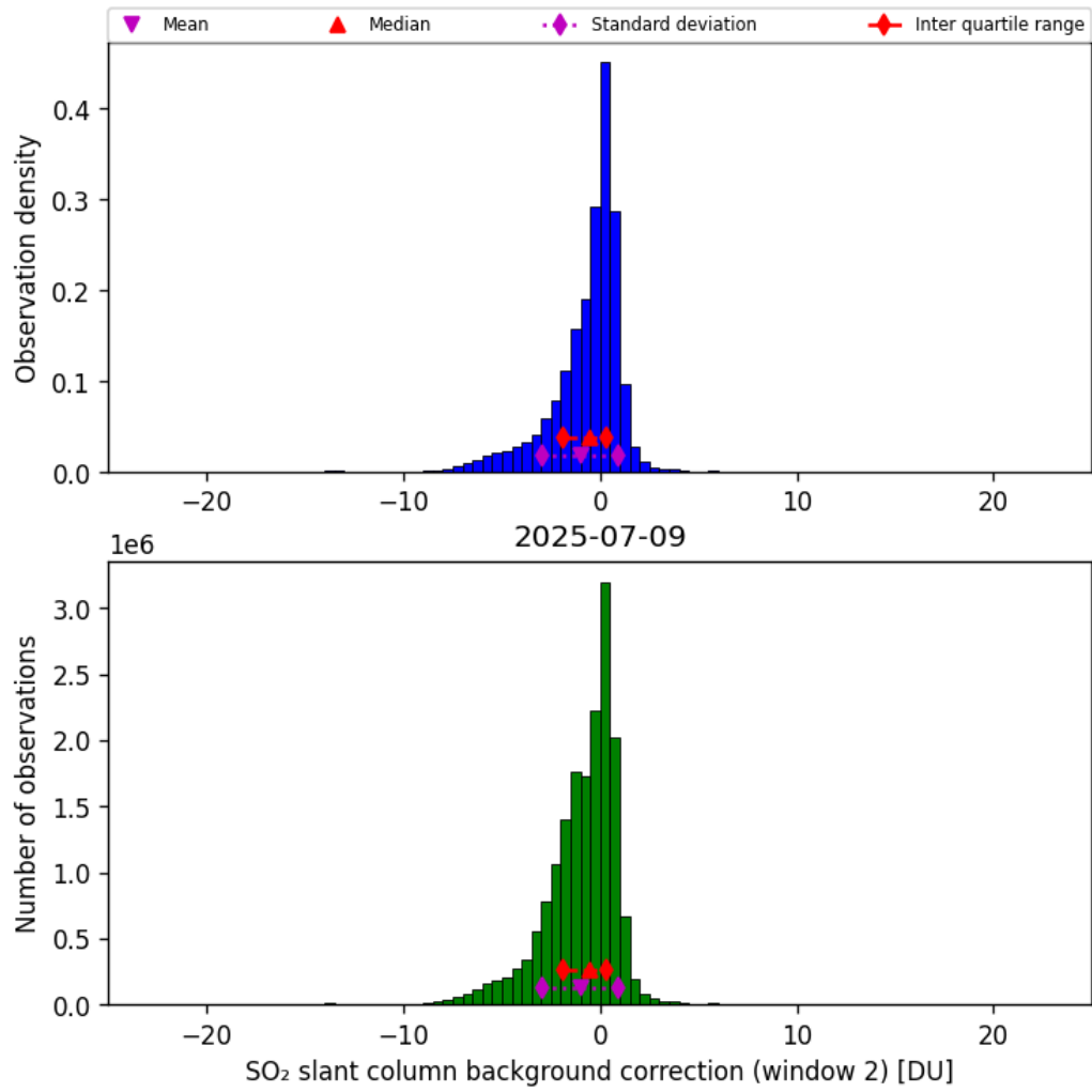
Figure 70: Histogram of “SO 2 slant column background correction (window 2)” for 2025-07-09 to 2025-07-10
