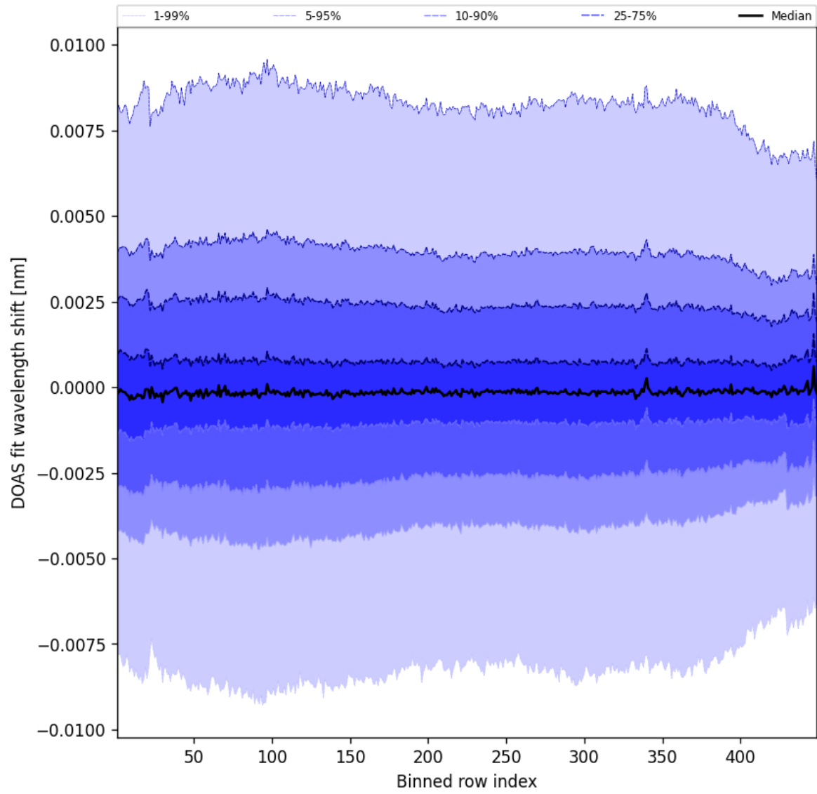
Figure 104: Along track statistics of “DOAS fit wavelength shift” for 2025-07-09 to 2025-07-10
