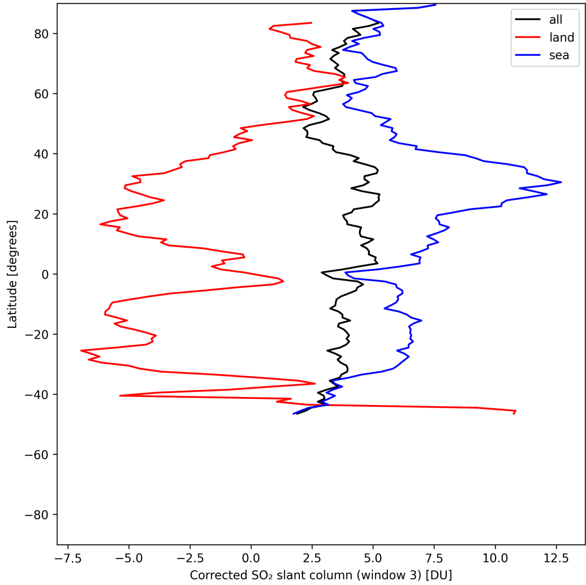
Figure 46: Zonal average of “Corrected SO 2 slant column (window 3)” for 2025-07-09 to 2025-07-10.
