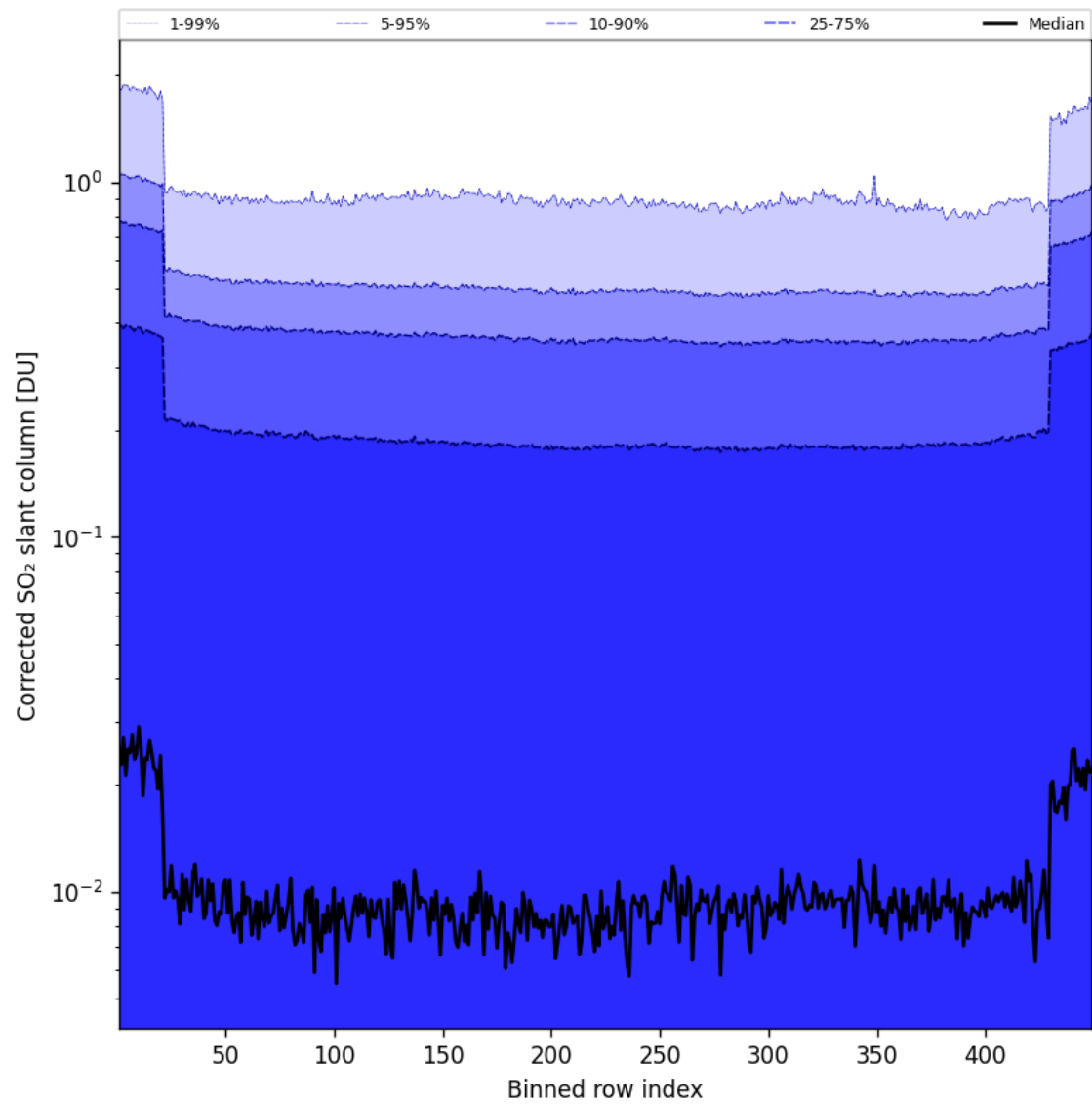
Figure 87: Along track statistics of “Corrected SO 2 slant column” for 2025-07-09 to 2025-07-10
