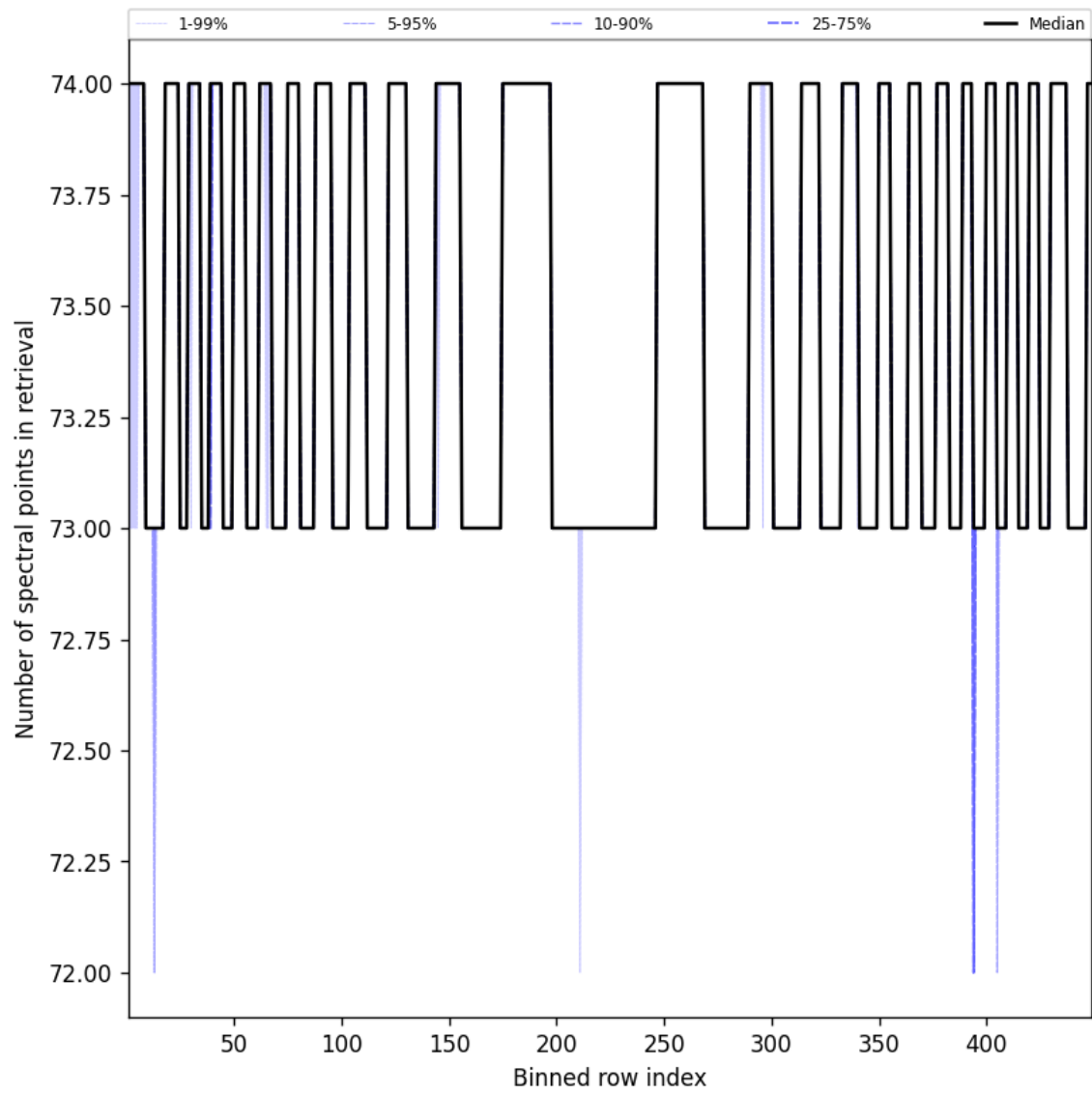
Figure 110: Along track statistics of “Number of spectral points in retrieval” for 2025-07-09 to 2025-07-10
