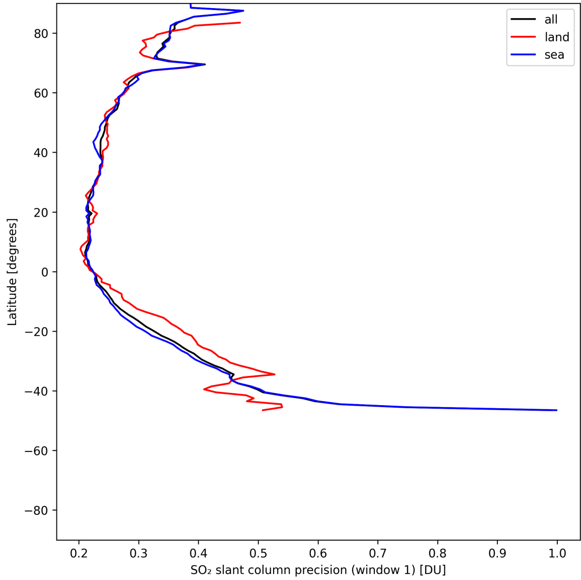
Figure 37: Zonal average of “SO 2 slant column precision (window 1)” for 2025-07-09 to 2025-07-10.
