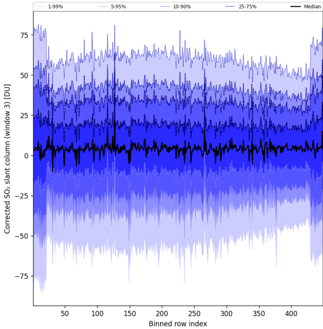
Figure 100: Along track statistics of “Corrected SO 2 slant column (window 3)” for 2025-07-09 to 2025-07-10
