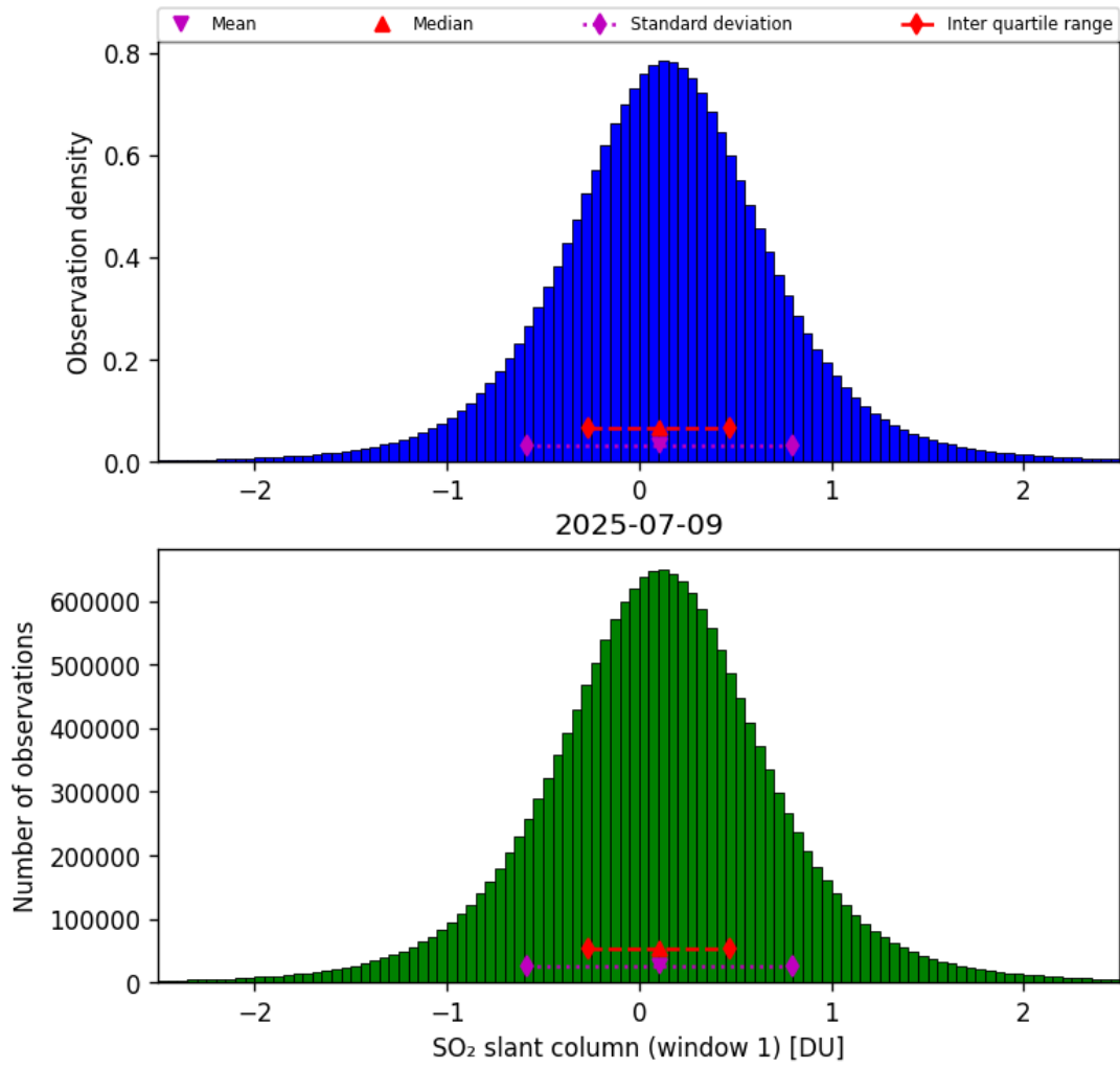
Figure 63: Histogram of “SO 2 slant column (window 1)” for 2025-07-09 to 2025-07-10
