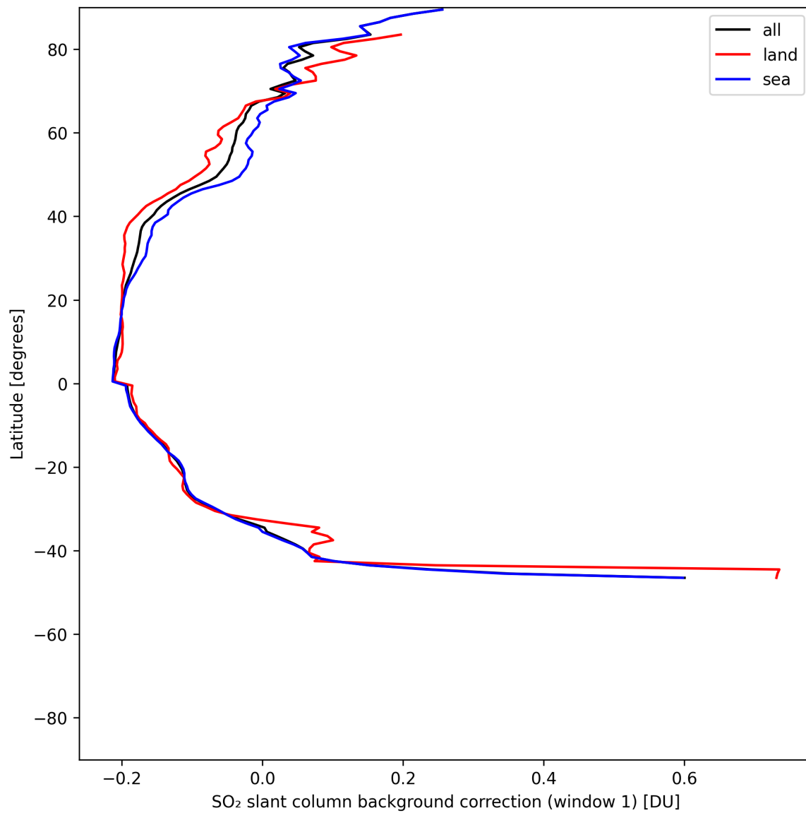
Figure 39: Zonal average of "SO 2 slant column background correction (window 1)" for 2025-07-09 to 2025-07-10.
