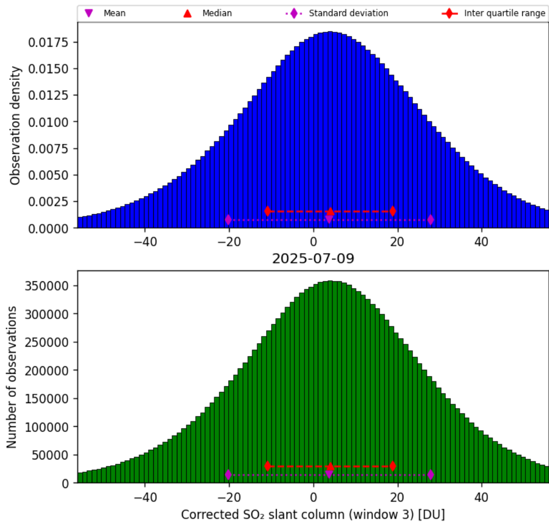
Figure 73: Histogram of “Corrected SO 2 slant column (window 3)” for 2025-07-09 to 2025-07-10
