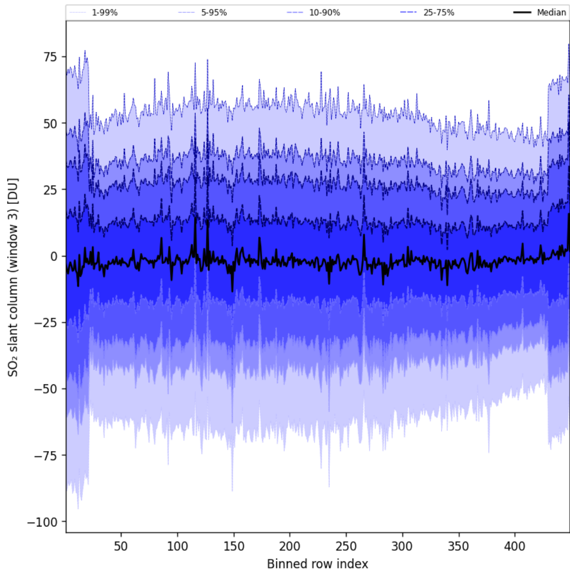
Figure 98: Along track statistics of “SO 2 slant column (window 3)” for 2025-07-09 to 2025-07-10
