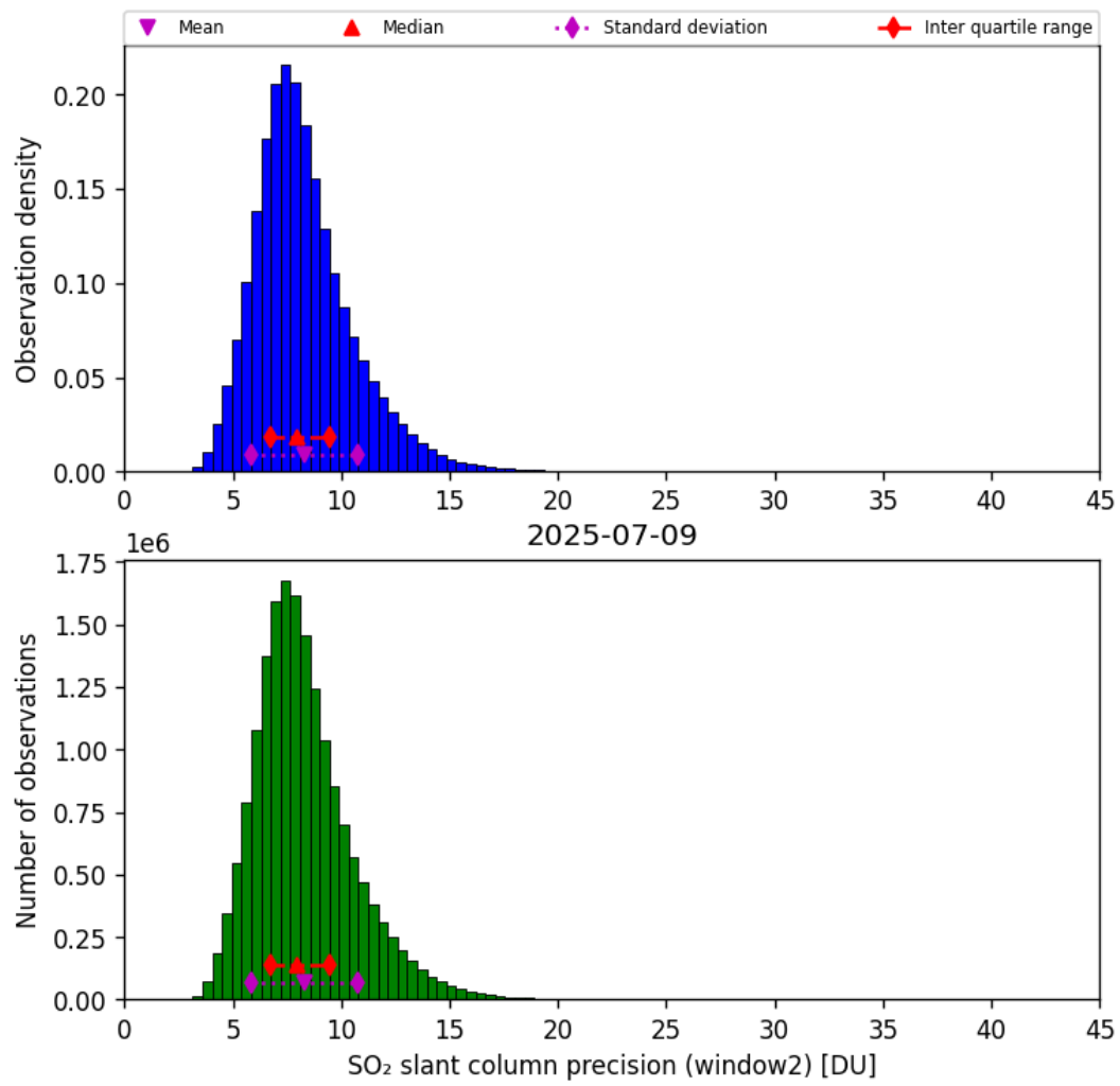
Figure 68: Histogram of “SO 2 slant column precision (window2)” for 2025-07-09 to 2025-07-10
