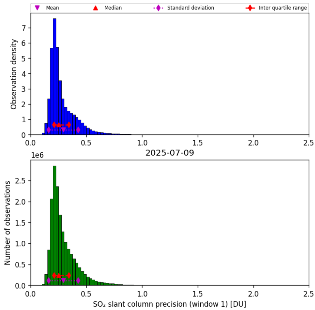
Figure 64: Histogram of “SO 2 slant column precision (window 1)” for 2025-07-09 to 2025-07-10
