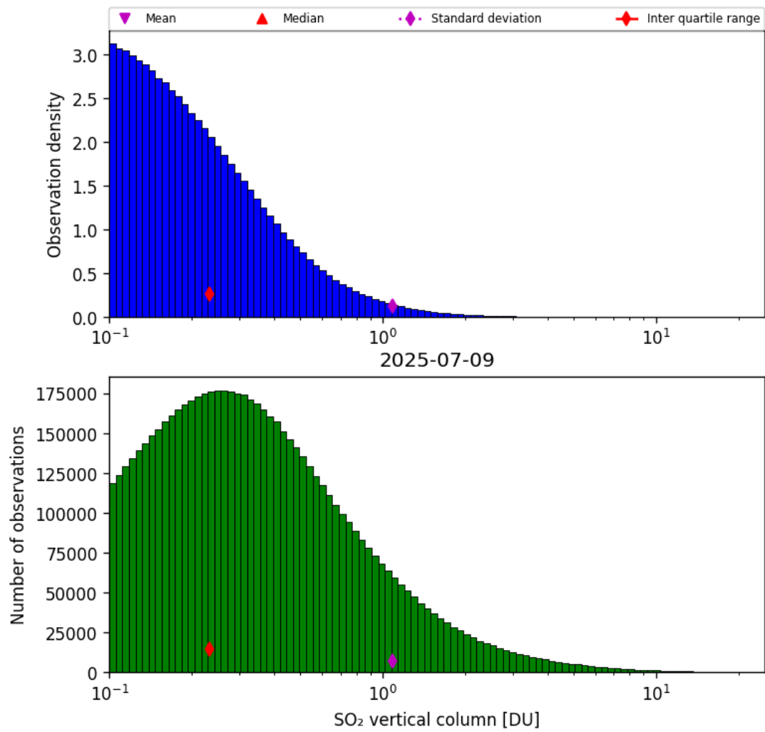
Figure 58: Histogram of “SO 2 vertical column” for 2025-07-09 to 2025-07-10
