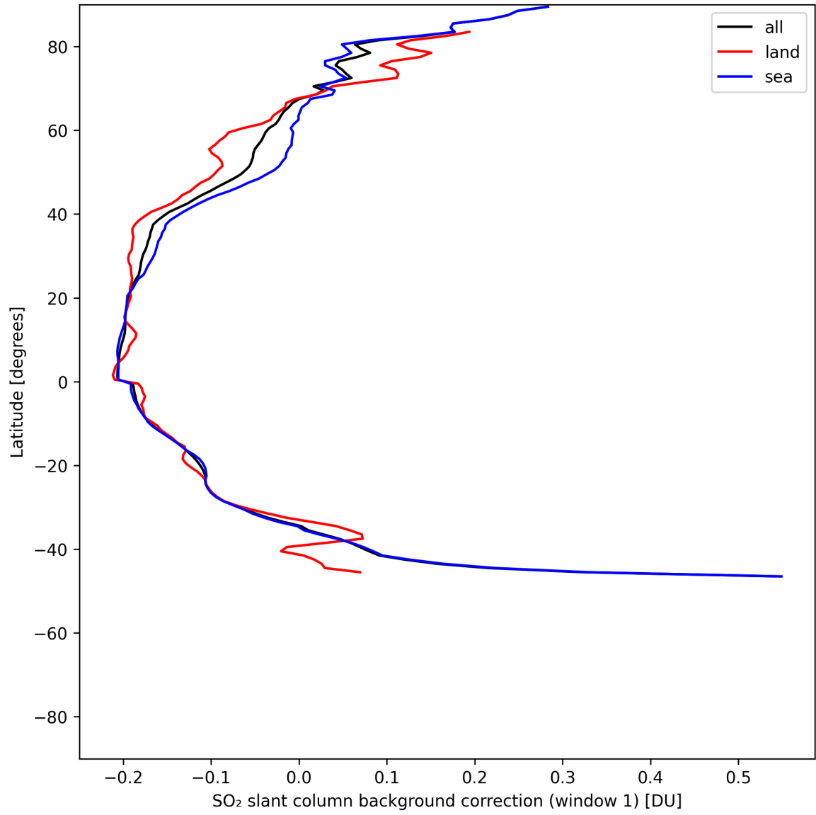
Figure 39: Zonal average of “SO 2 slant column background correction (window 1)” for 2025-07-10 to 2025-07-11.
