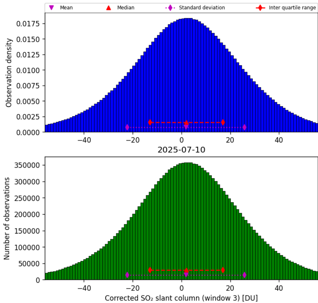
Figure 73: Histogram of “Corrected SO 2 slant column (window 3)” for 2025-07-10 to 2025-07-11
