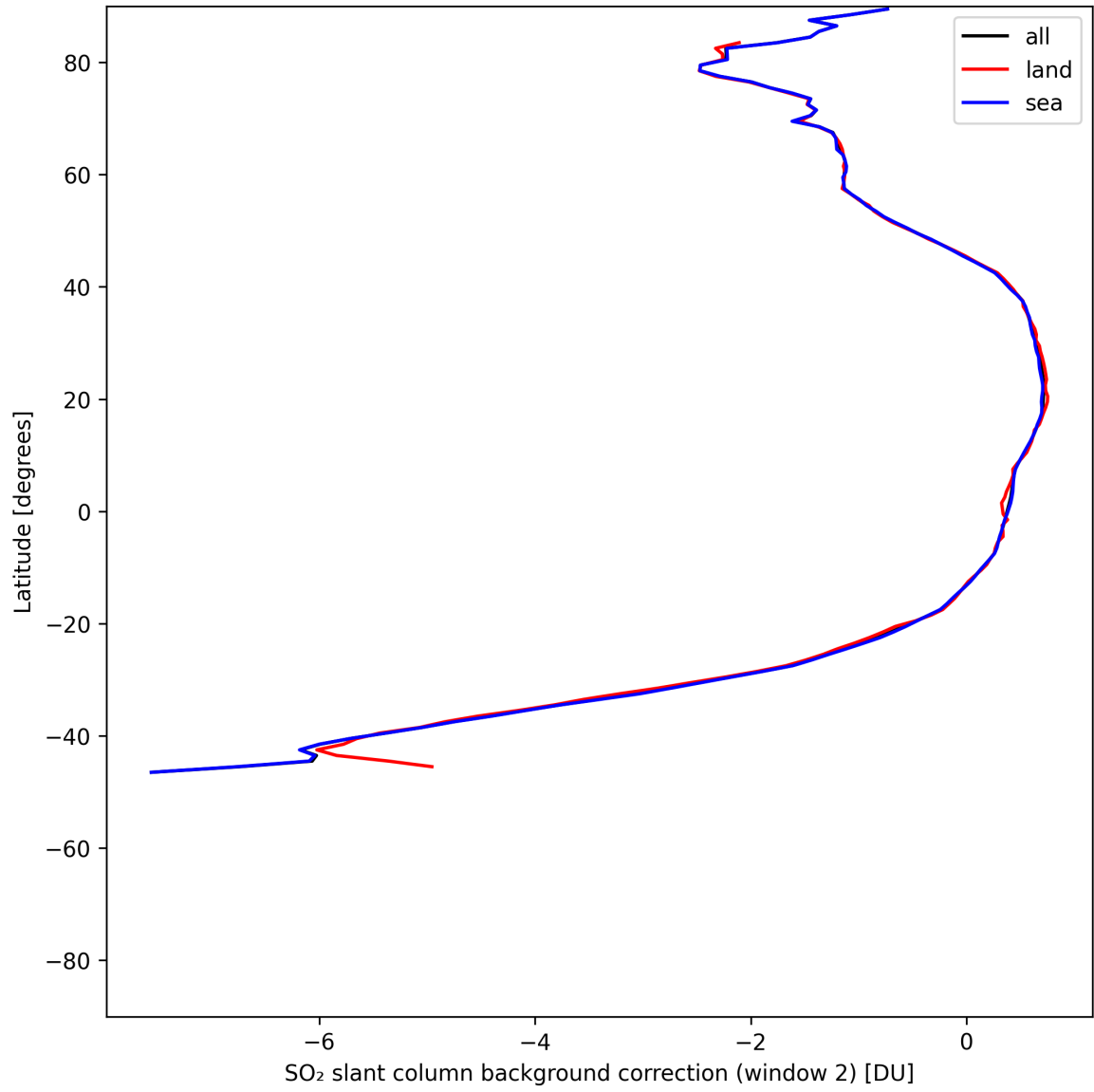
Figure 43: Zonal average of “SO 2 slant column background correction (window 2)” for 2025-07-10 to 2025-07-11.
