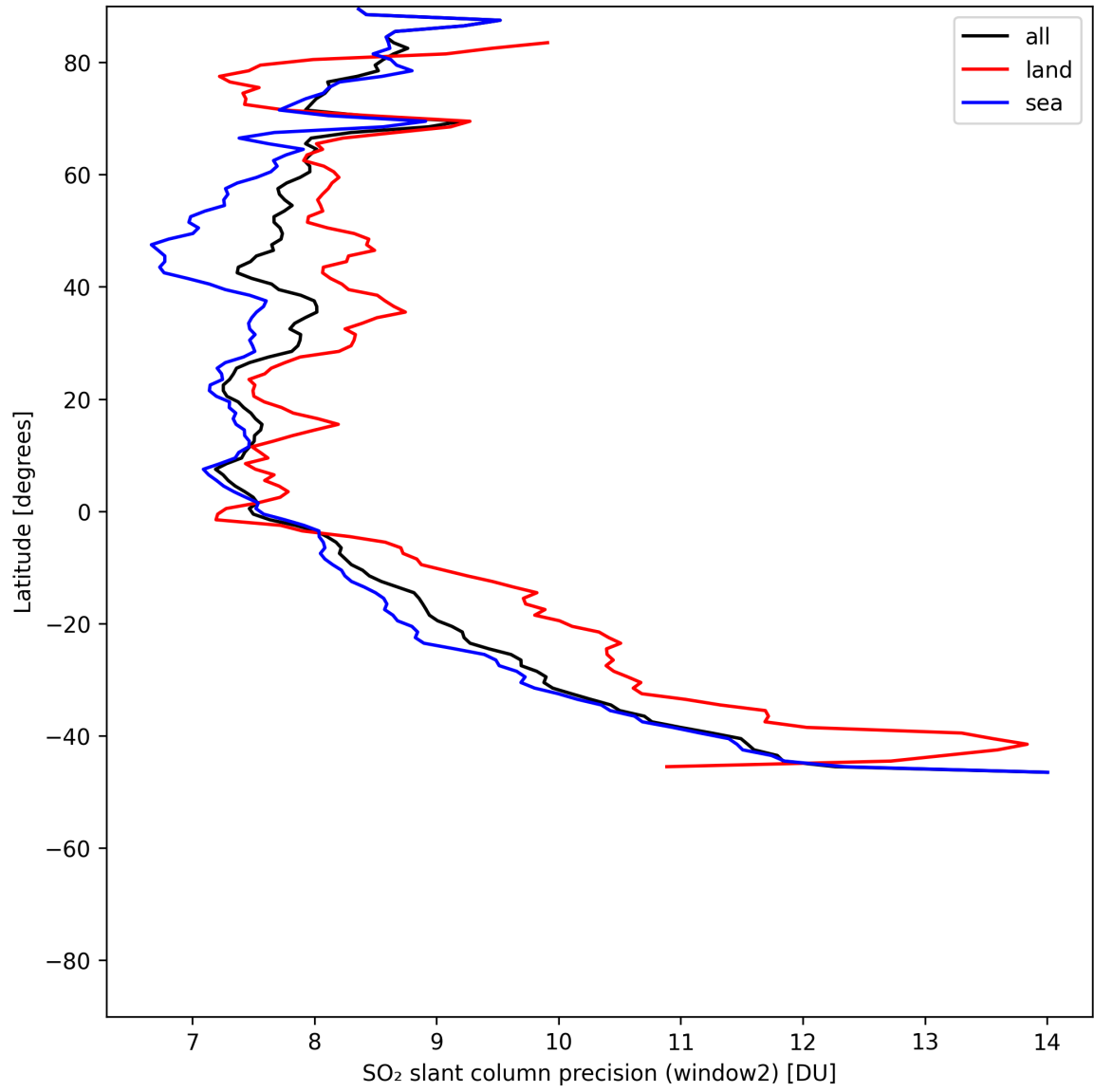
Figure 41: Zonal average of “SO 2 slant column precision (window2)” for 2025-07-10 to 2025-07-11.
