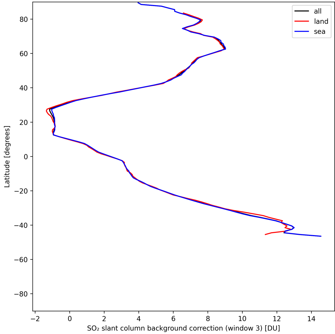
Figure 47: Zonal average of “SO 2 slant column background correction (window 3)” for 2025-07-10 to 2025-07-11.
