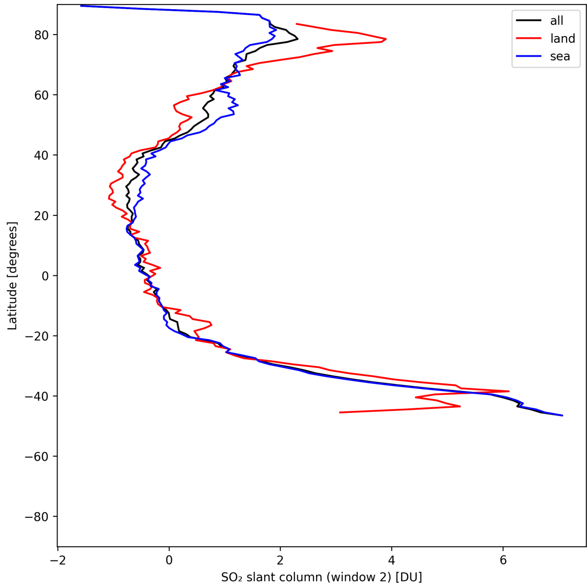
Figure 40: Zonal average of “SO 2 slant column (window 2)” for 2025-07-10 to 2025-07-11.
