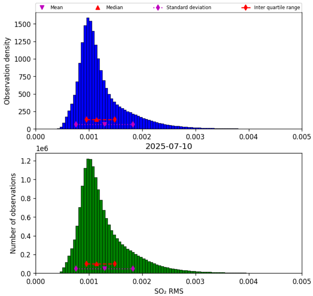
Figure 79: Histogram of “SO 2 RMS” for 2025-07-10 to 2025-07-11
