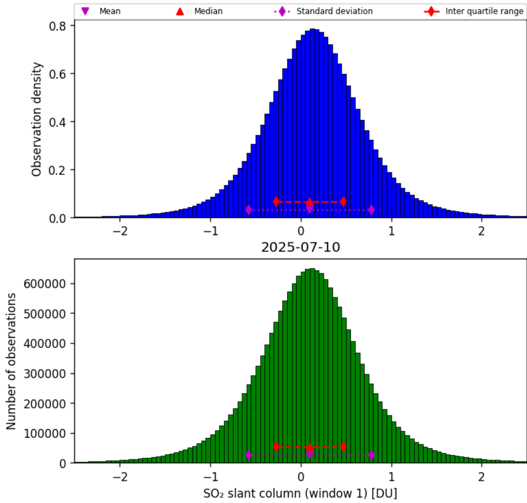
Figure 63: Histogram of “SO 2 slant column (window 1)” for 2025-07-10 to 2025-07-11
