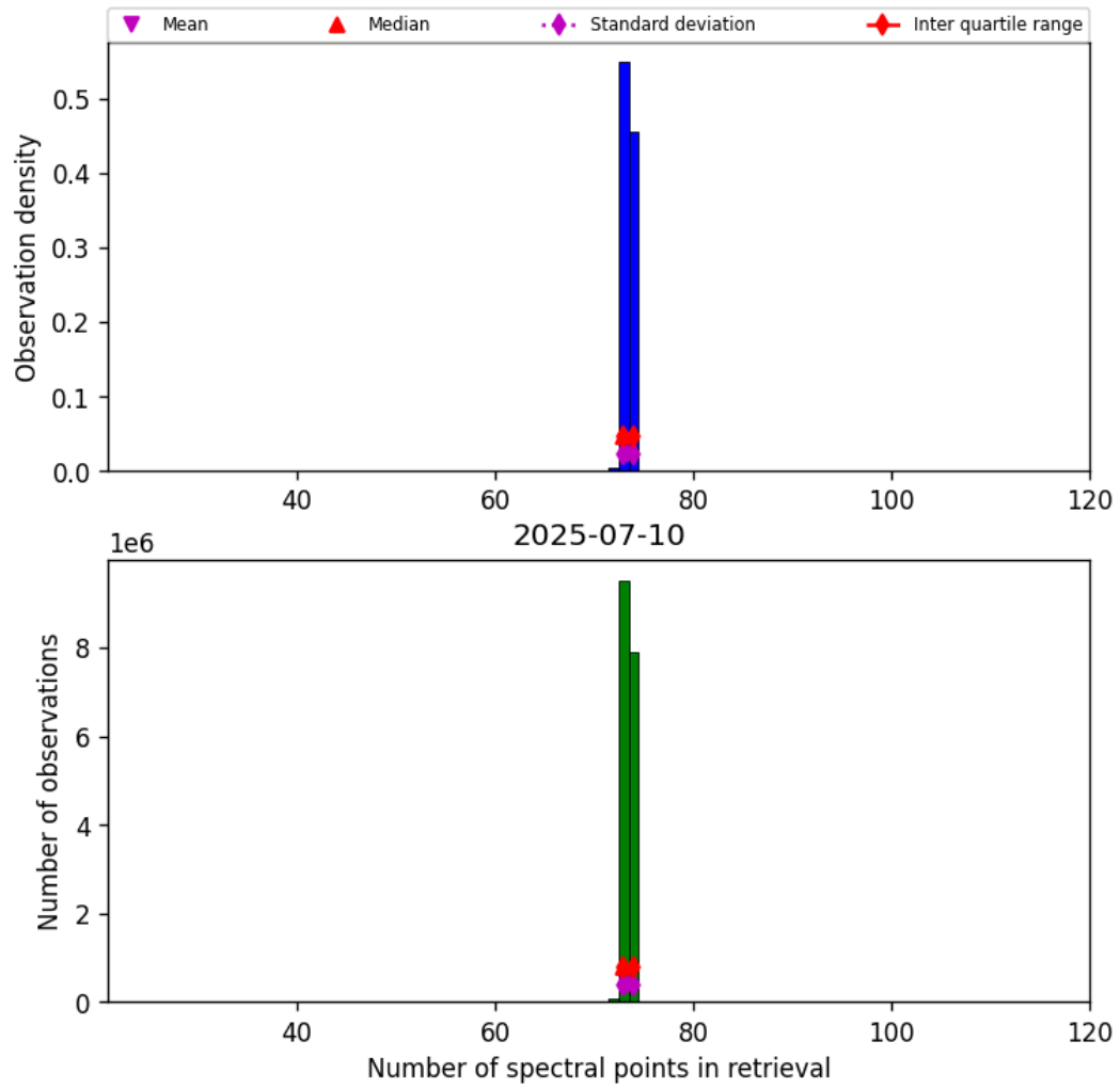
Figure 83: Histogram of “Number of spectral points in retrieval” for 2025-07-10 to 2025-07-11
