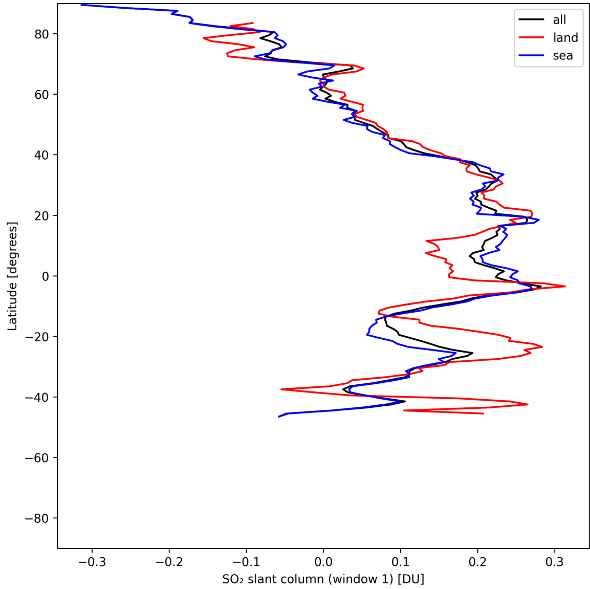
Figure 36: Zonal average of “SO 2 slant column (window 1)” for 2025-07-10 to 2025-07-11.
