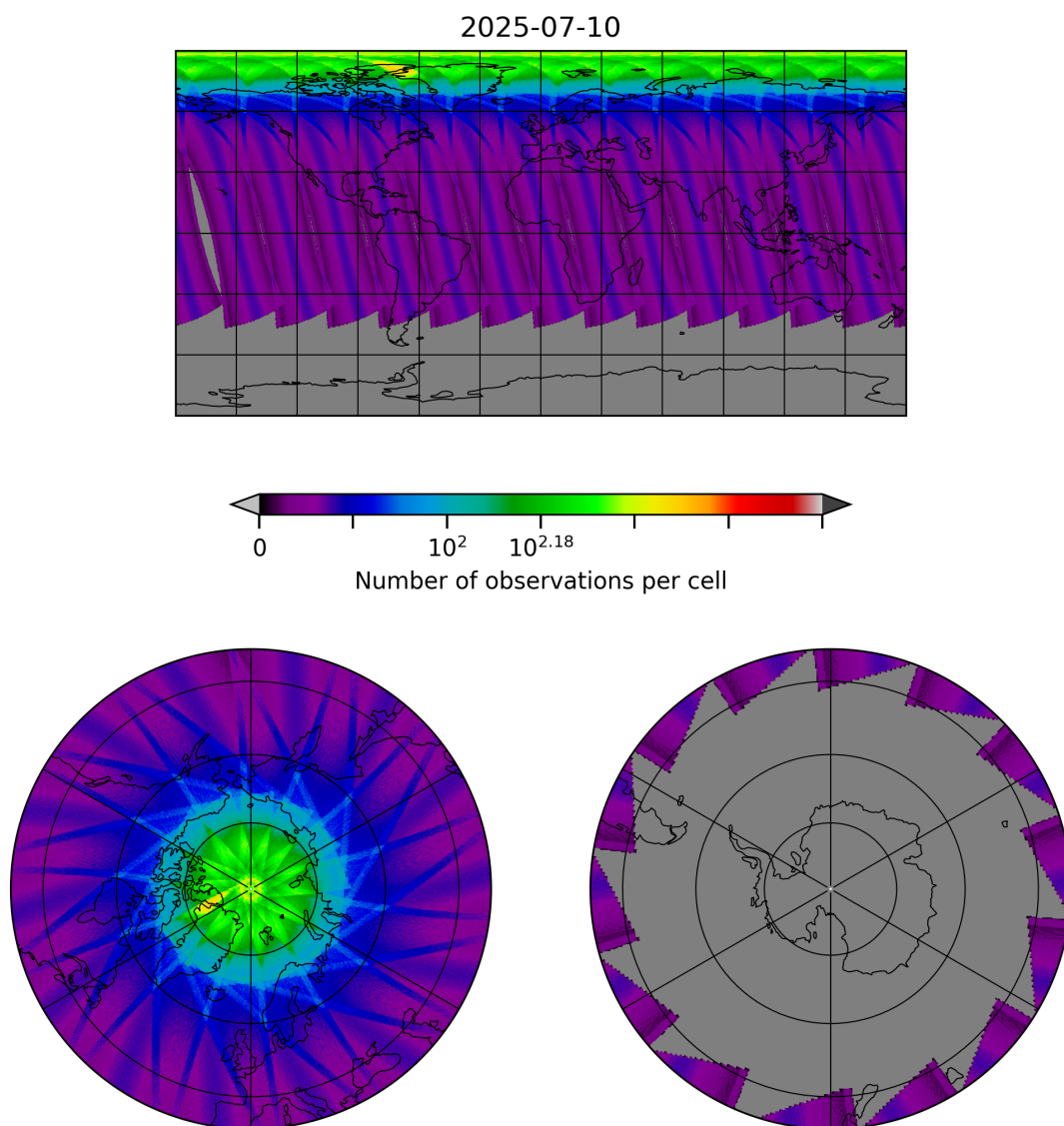
Figure 29: Map of the number of observations for 2025-07-10 to 2025-07-11
