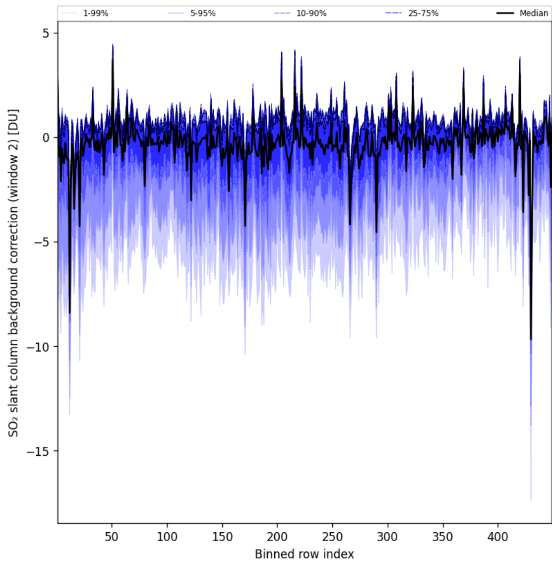
Figure 97: Along track statistics of “SO 2 slant column background correction (window 2)” for 2025-07-10 to 2025-07-11
