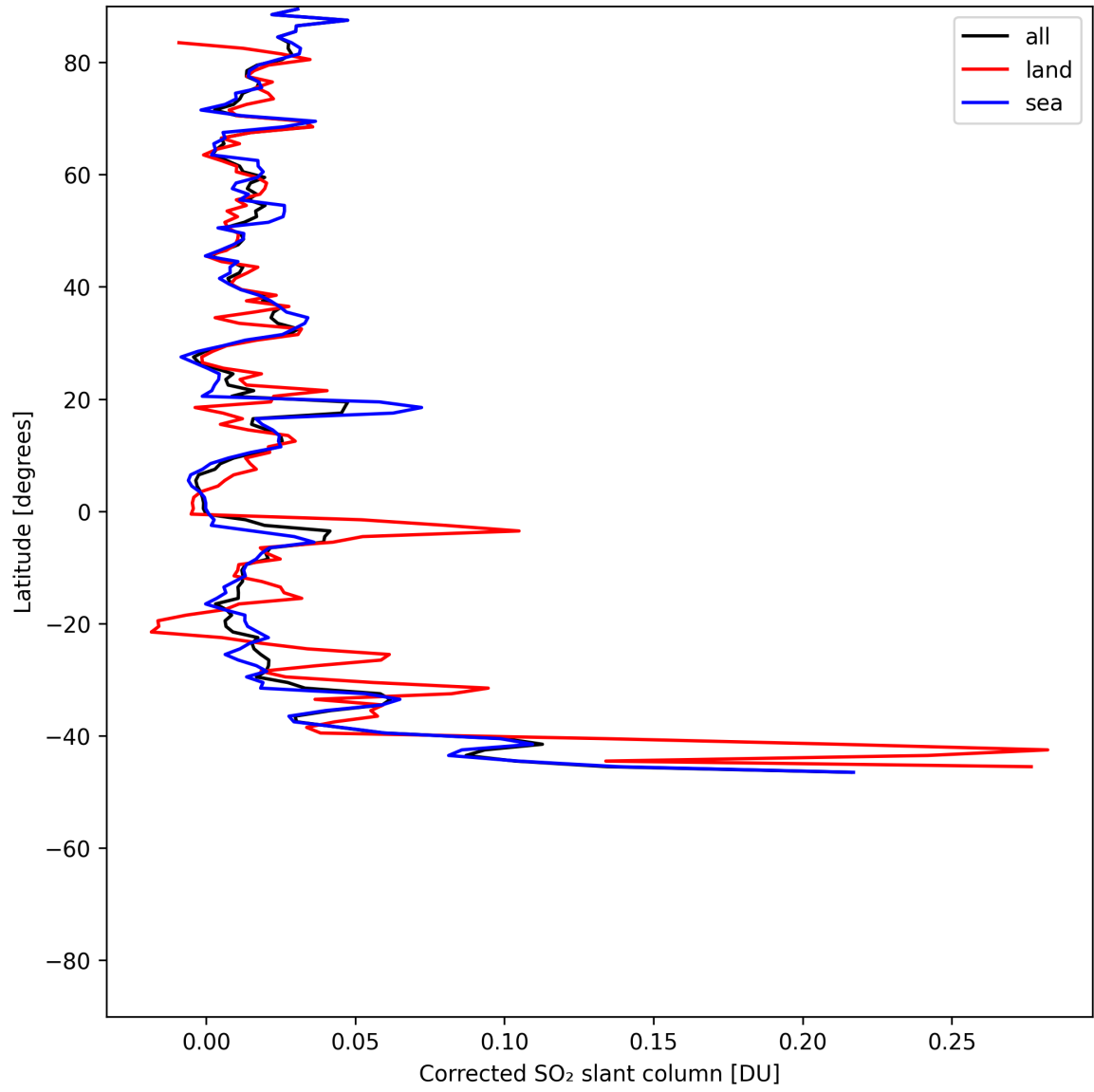
Figure 33: Zonal average of “Corrected SO 2 slant column” for 2025-07-10 to 2025-07-11.
