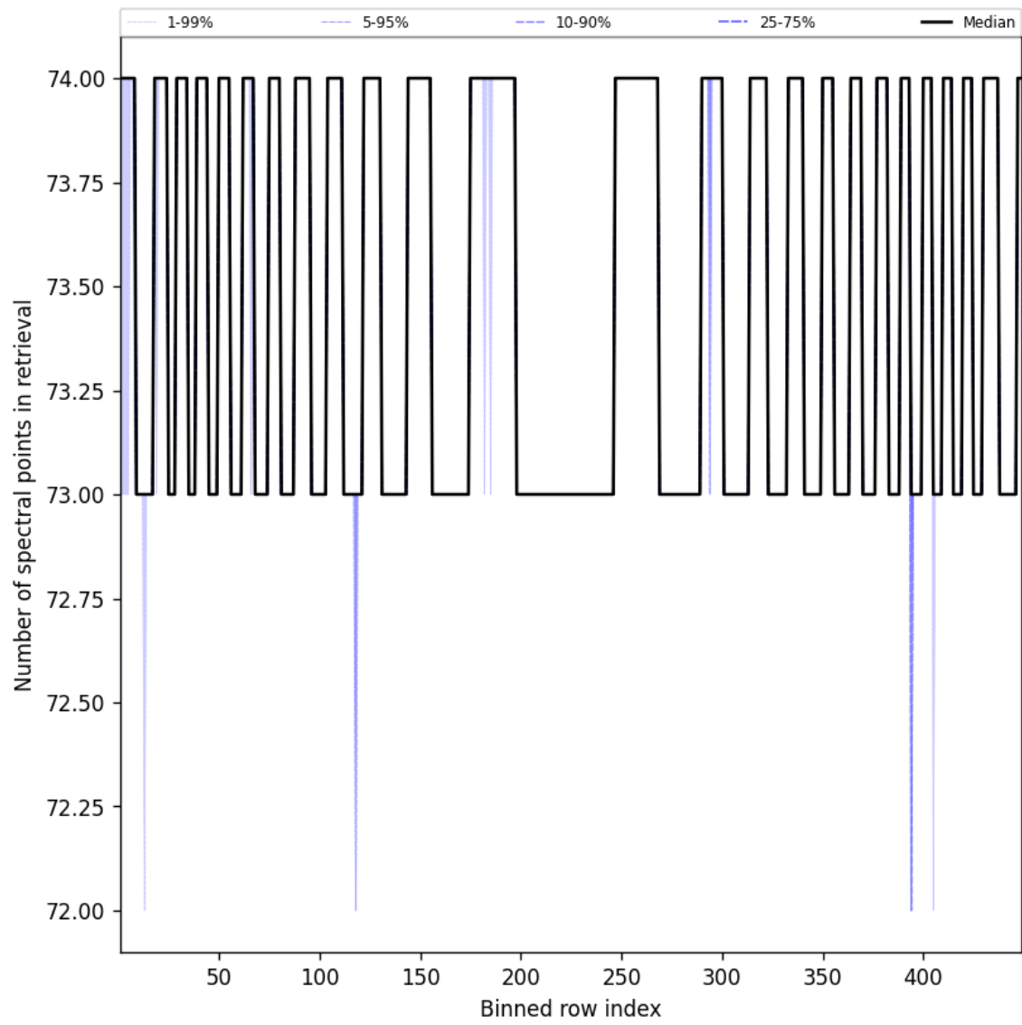
Figure 110: Along track statistics of “Number of spectral points in retrieval” for 2025-07-10 to 2025-07-11
