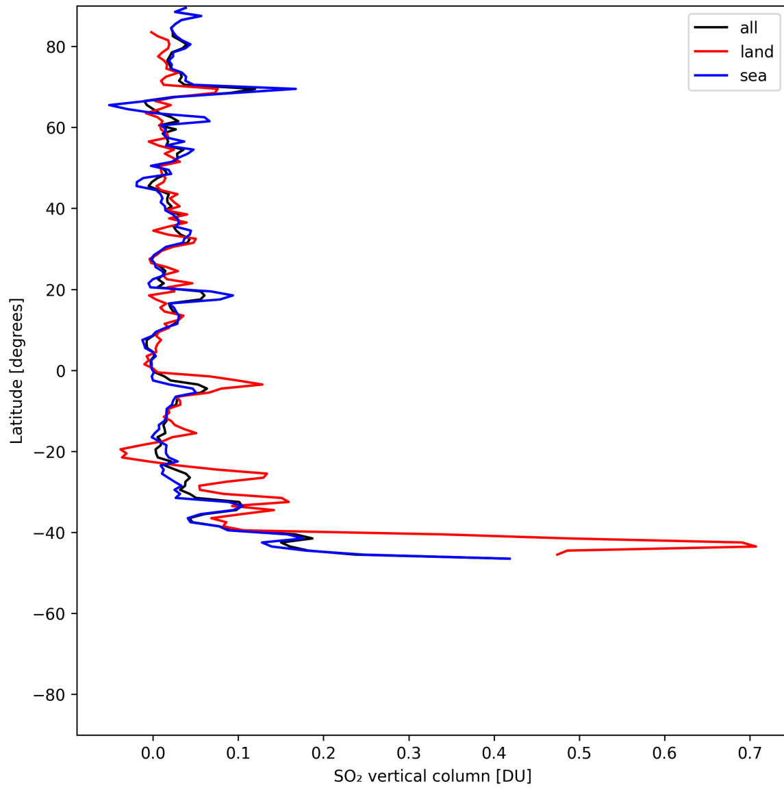
Figure 31: Zonal average of “SO 2 vertical column” for 2025-07-10 to 2025-07-11.
