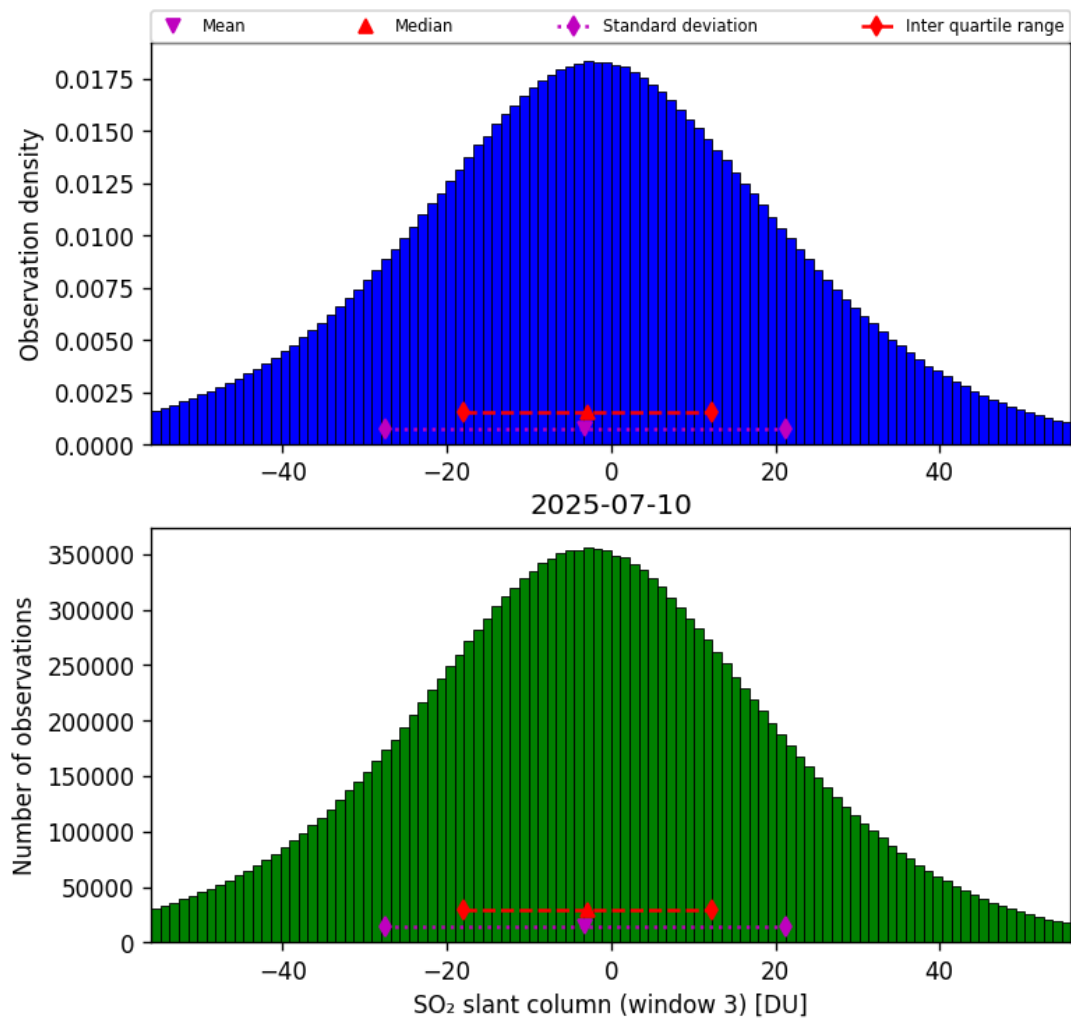
Figure 71: Histogram of “SO 2 slant column (window 3)” for 2025-07-10 to 2025-07-11
