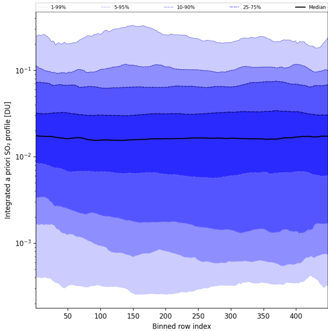
Figure 103: Along track statistics of “Integrated a priori SO 2 profile” for 2025-07-10 to 2025-07-11
