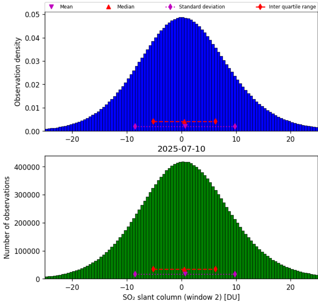
Figure 67: Histogram of “SO 2 slant column (window 2)” for 2025-07-10 to 2025-07-11
