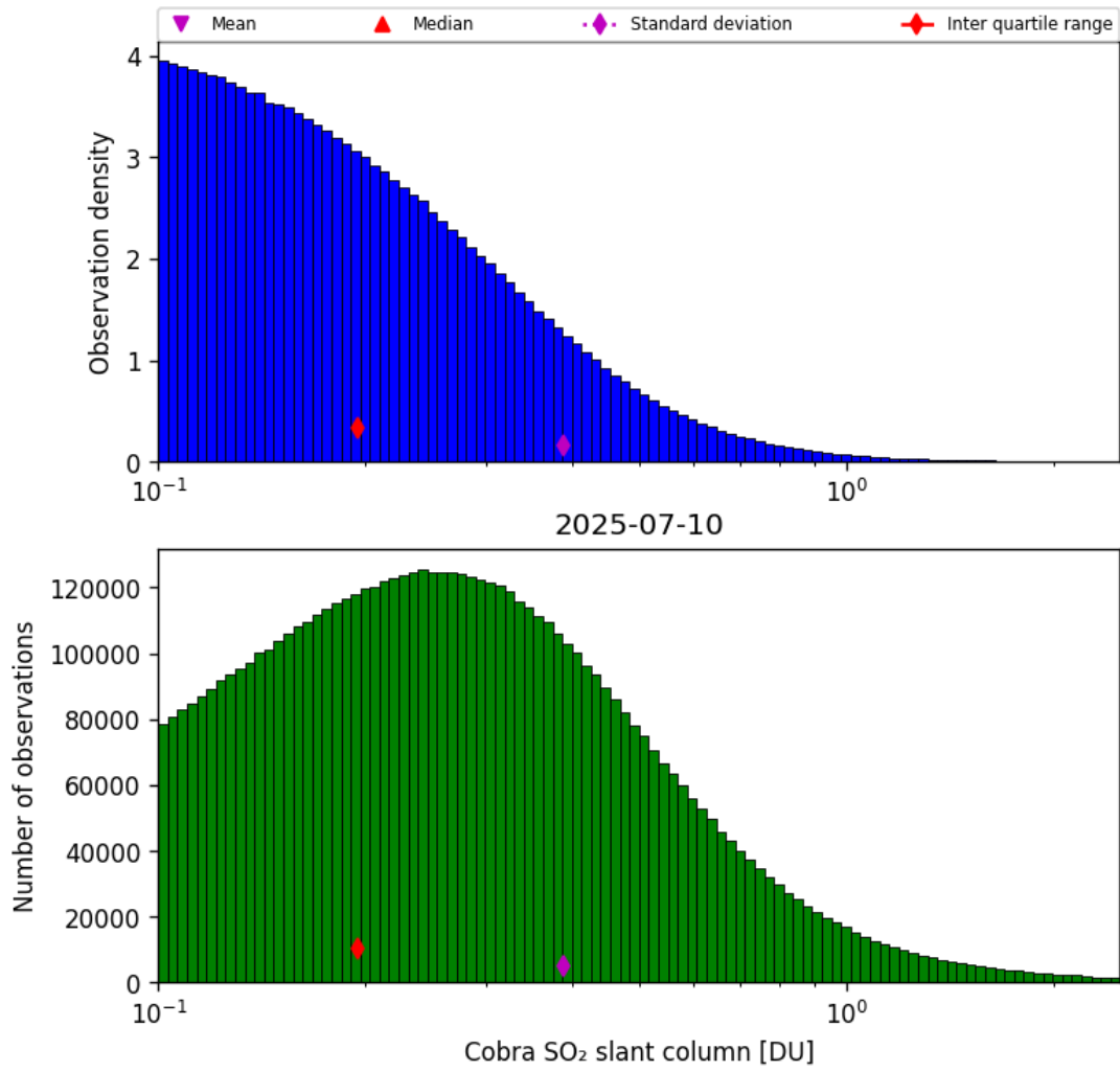
Figure 61: Histogram of “Cobra SO 2 slant column” for 2025-07-10 to 2025-07-11
