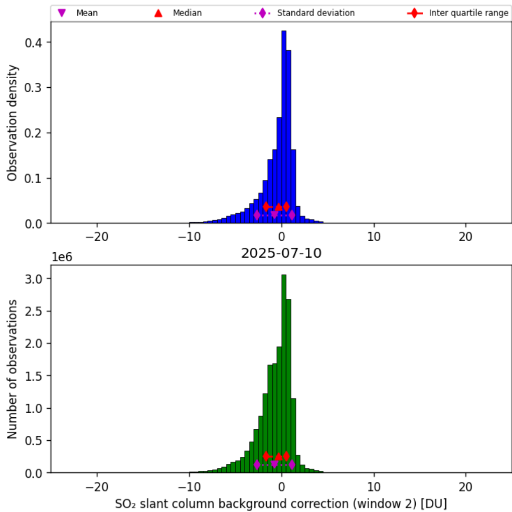
Figure 70: Histogram of “SO 2 slant column background correction (window 2)” for 2025-07-10 to 2025-07-11
