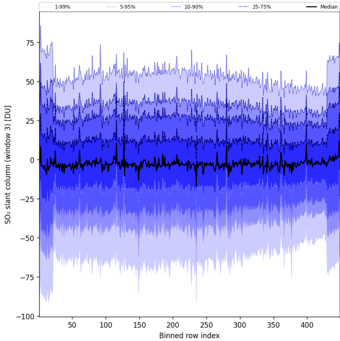
Figure 98: Along track statistics of “SO 2 slant column (window 3)” for 2025-07-10 to 2025-07-11
