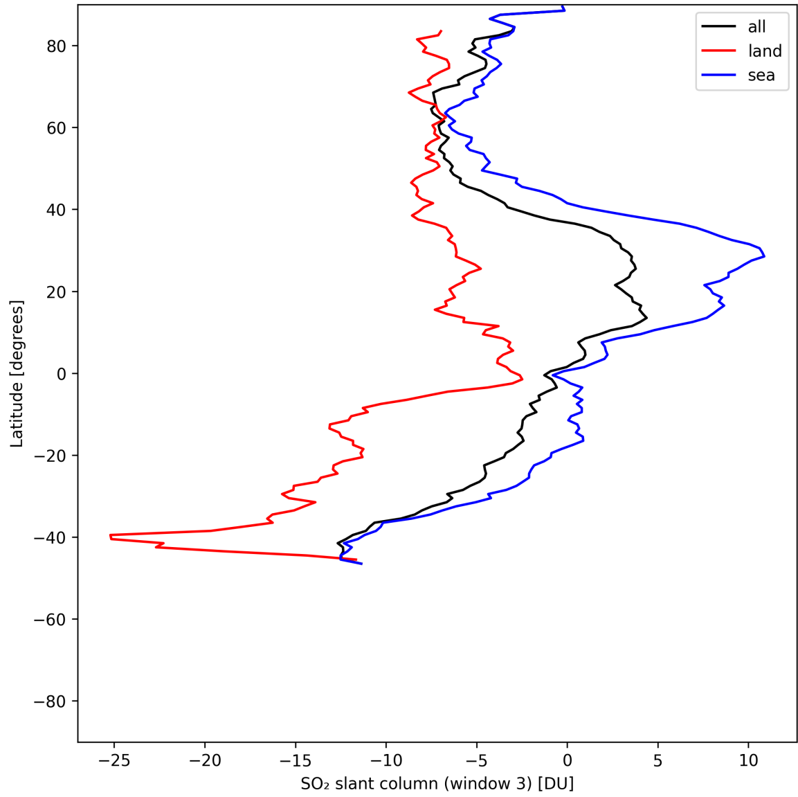
Figure 44: Zonal average of “SO 2 slant column (window 3)” for 2025-07-10 to 2025-07-11.
