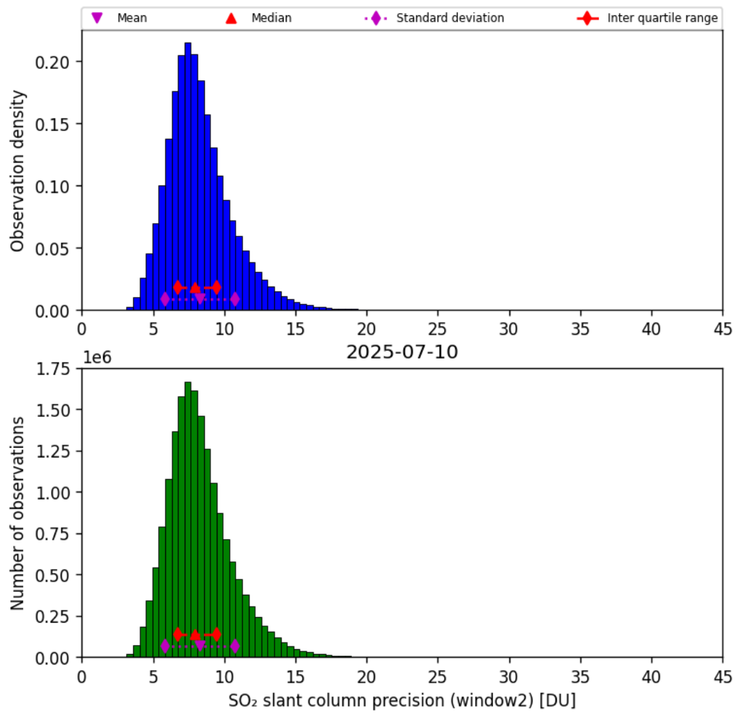
Figure 68: Histogram of “SO 2 slant column precision (window2)” for 2025-07-10 to 2025-07-11
