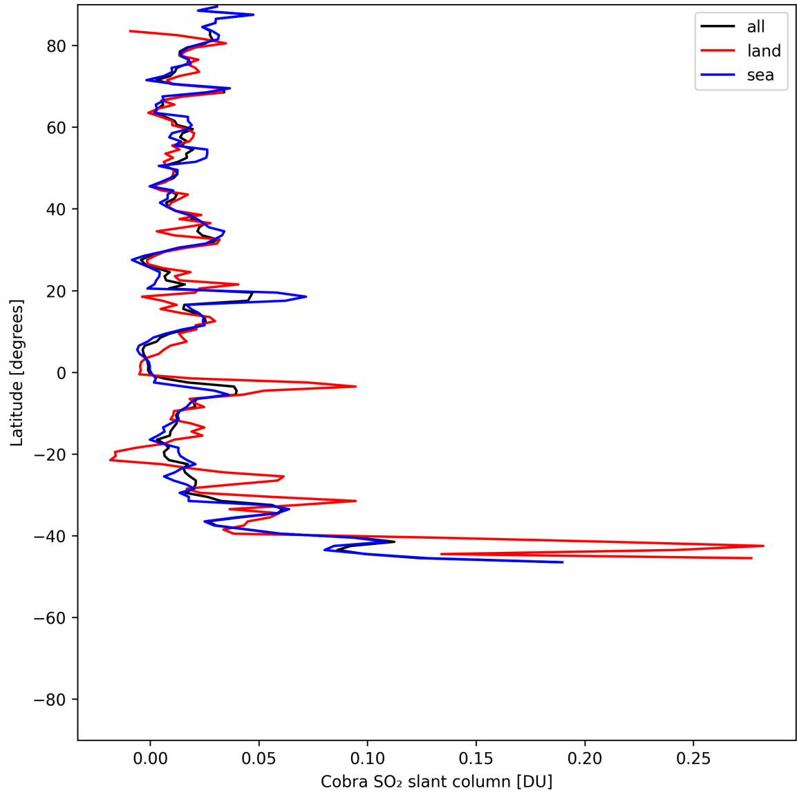
Figure 34: Zonal average of “Cobra SO 2 slant column” for 2025-07-10 to 2025-07-11.
