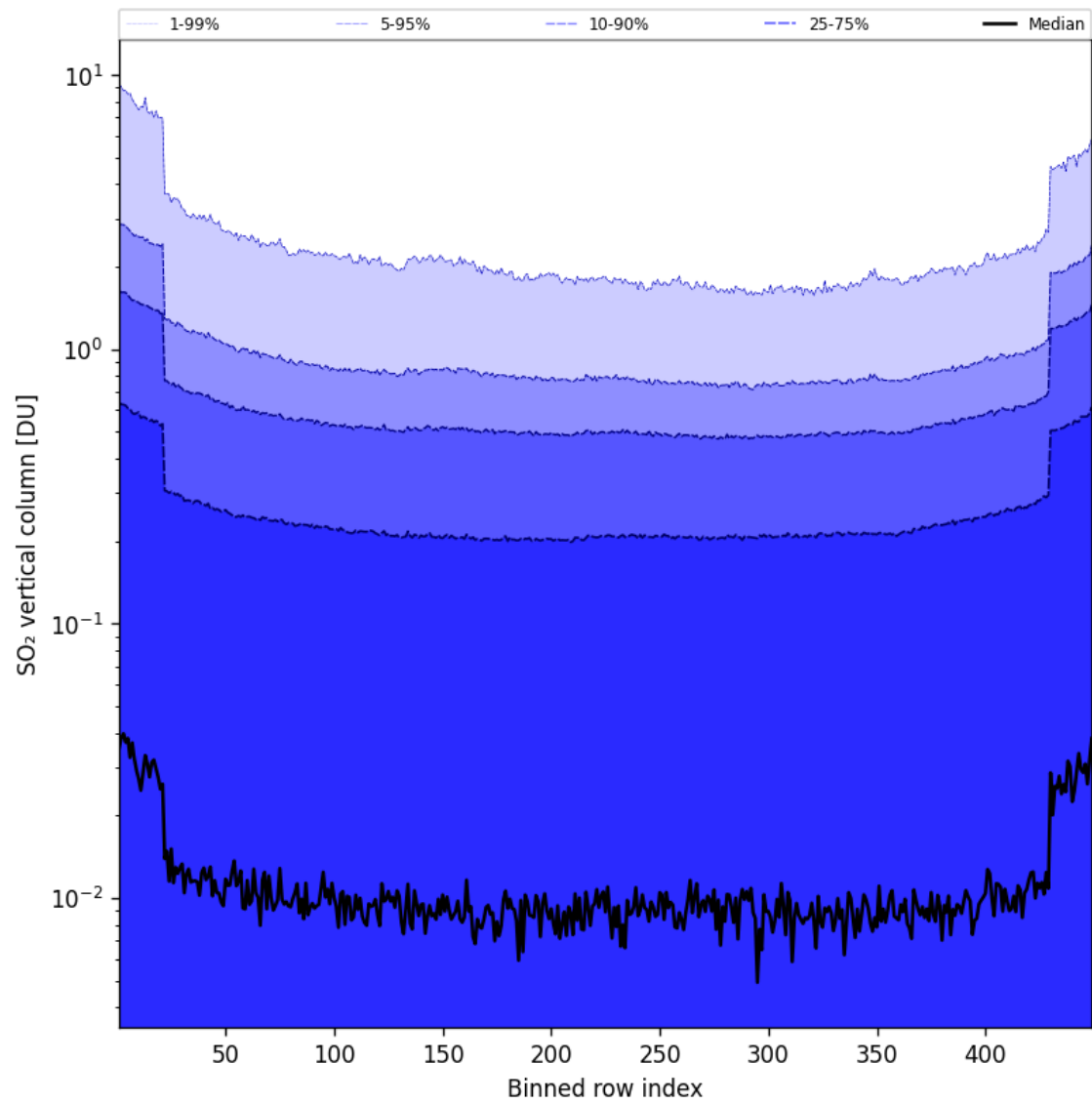
Figure 85: Along track statistics of “SO 2 vertical column” for 2025-07-10 to 2025-07-11
