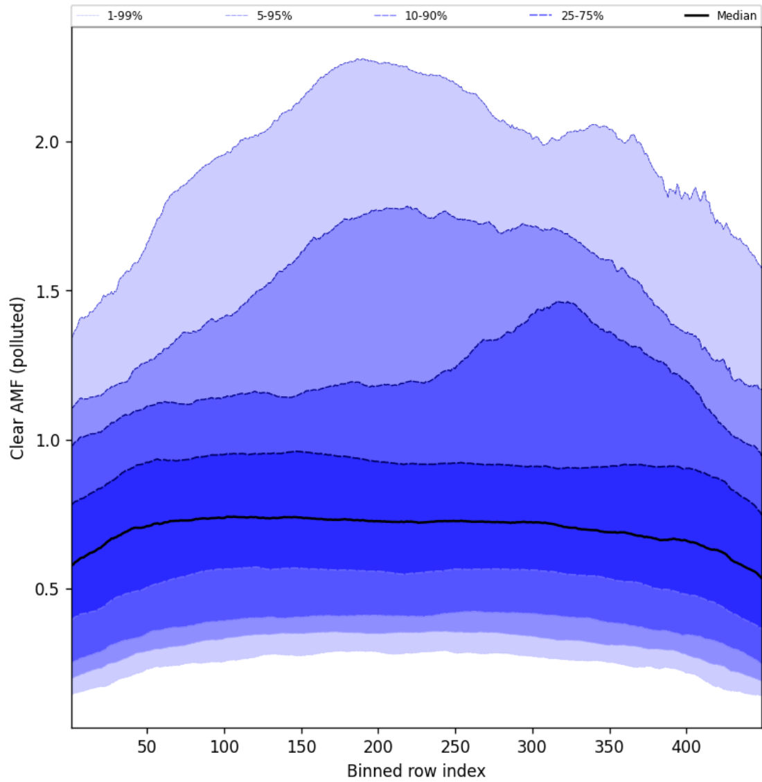
Figure 109: Along track statistics of “Clear AMF (polluted)” for 2025-07-10 to 2025-07-11
