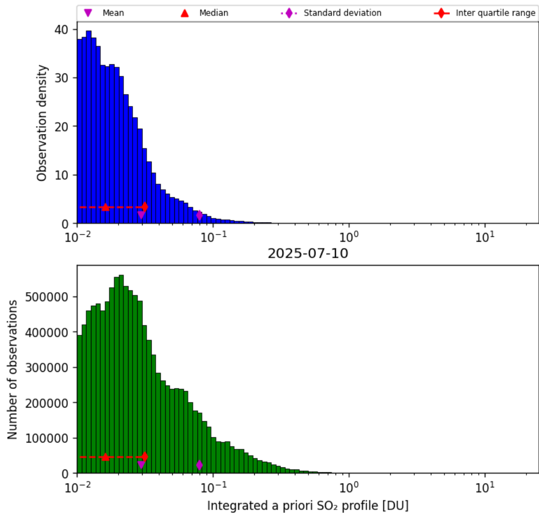
Figure 76: Histogram of “Integrated a priori SO 2 profile” for 2025-07-10 to 2025-07-11
