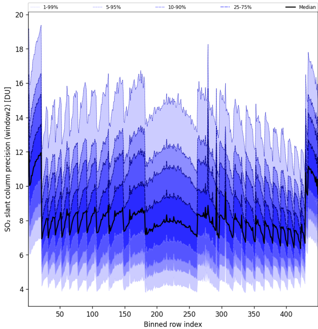
Figure 95: Along track statistics of “SO 2 slant column precision (window2)” for 2025-07-10 to 2025-07-11
