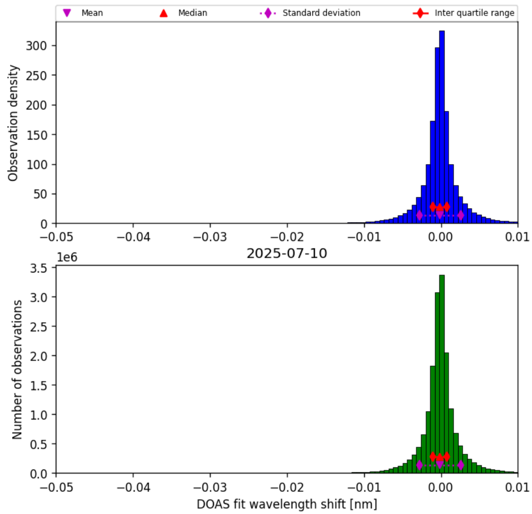
Figure 77: Histogram of “DOAS fit wavelength shift” for 2025-07-10 to 2025-07-11
