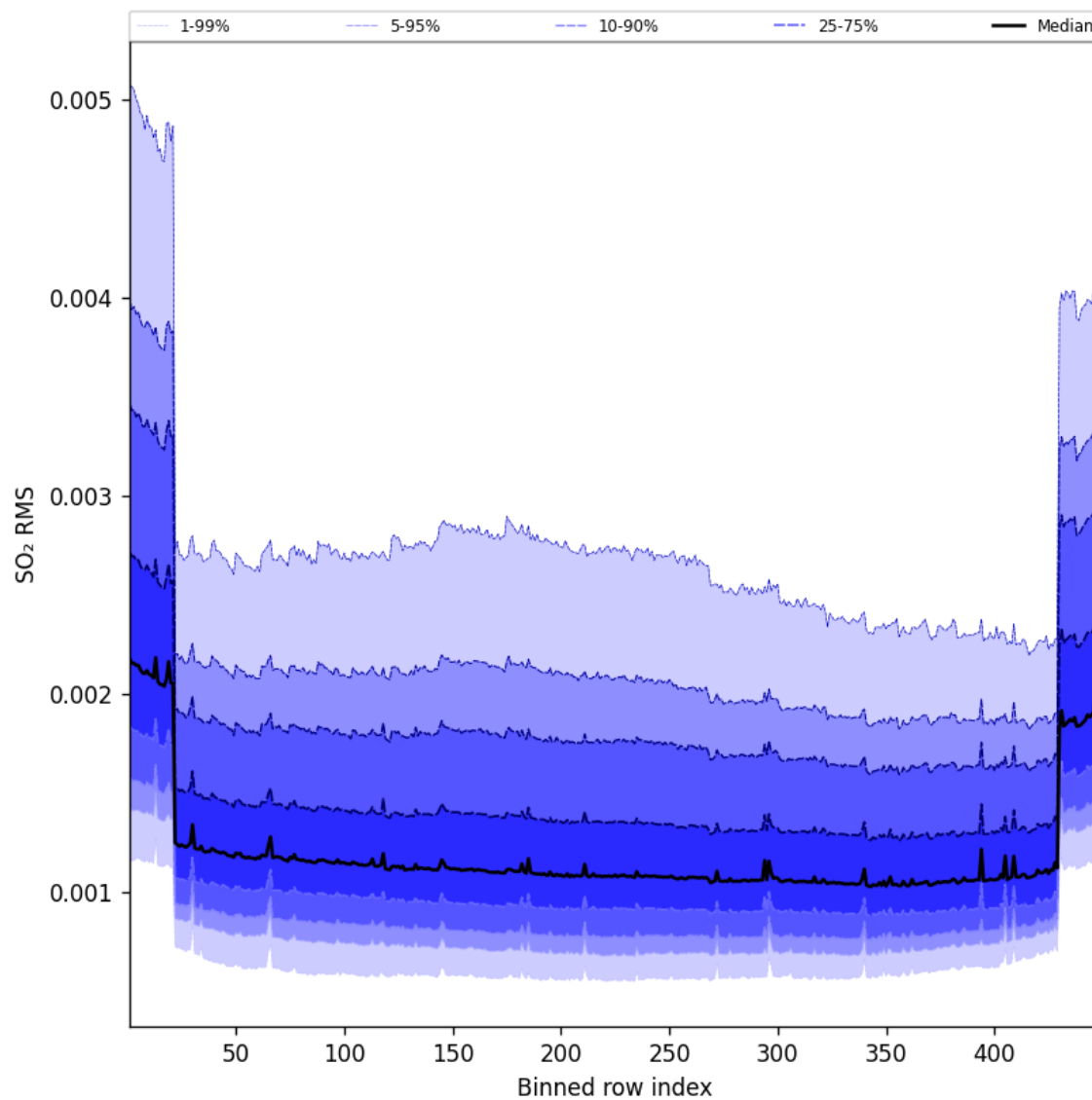
Figure 106: Along track statistics of “SO 2 RMS” for 2025-07-10 to 2025-07-11
