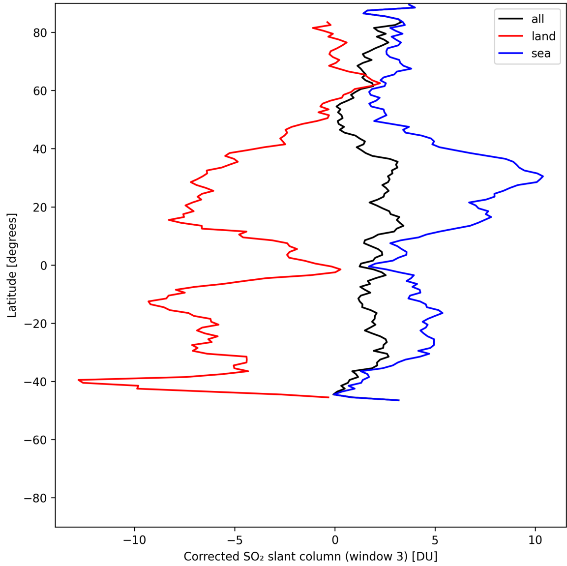
Figure 46: Zonal average of “Corrected SO 2 slant column (window 3)” for 2025-07-10 to 2025-07-11.
