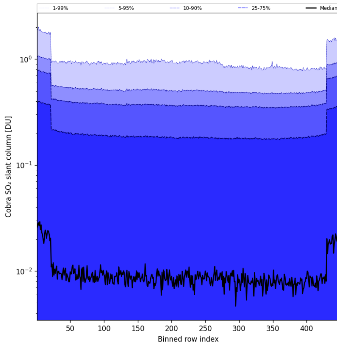
Figure 88: Along track statistics of “Cobra SO 2 slant column” for 2025-07-10 to 2025-07-11
