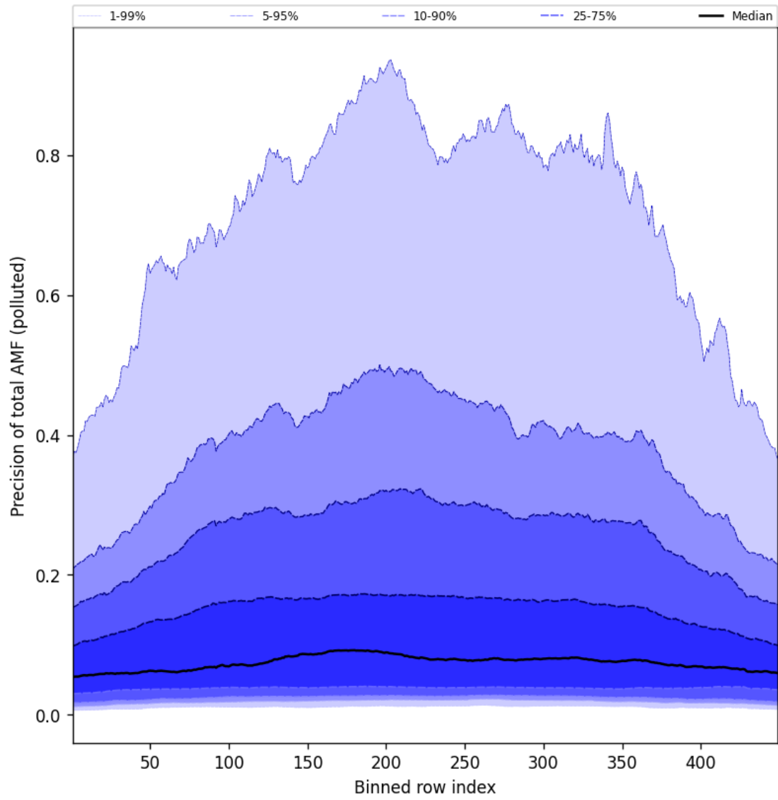
Figure 108: Along track statistics of “Precision of total AMF (polluted)” for 2025-07-10 to 2025-07-11
