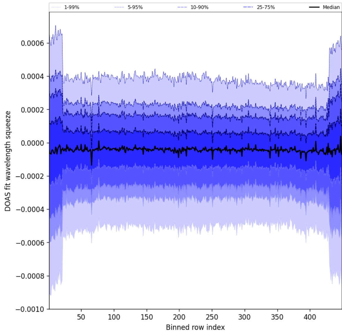
Figure 105: Along track statistics of “DOAS fit wavelength squeeze” for 2025-07-10 to 2025-07-11
