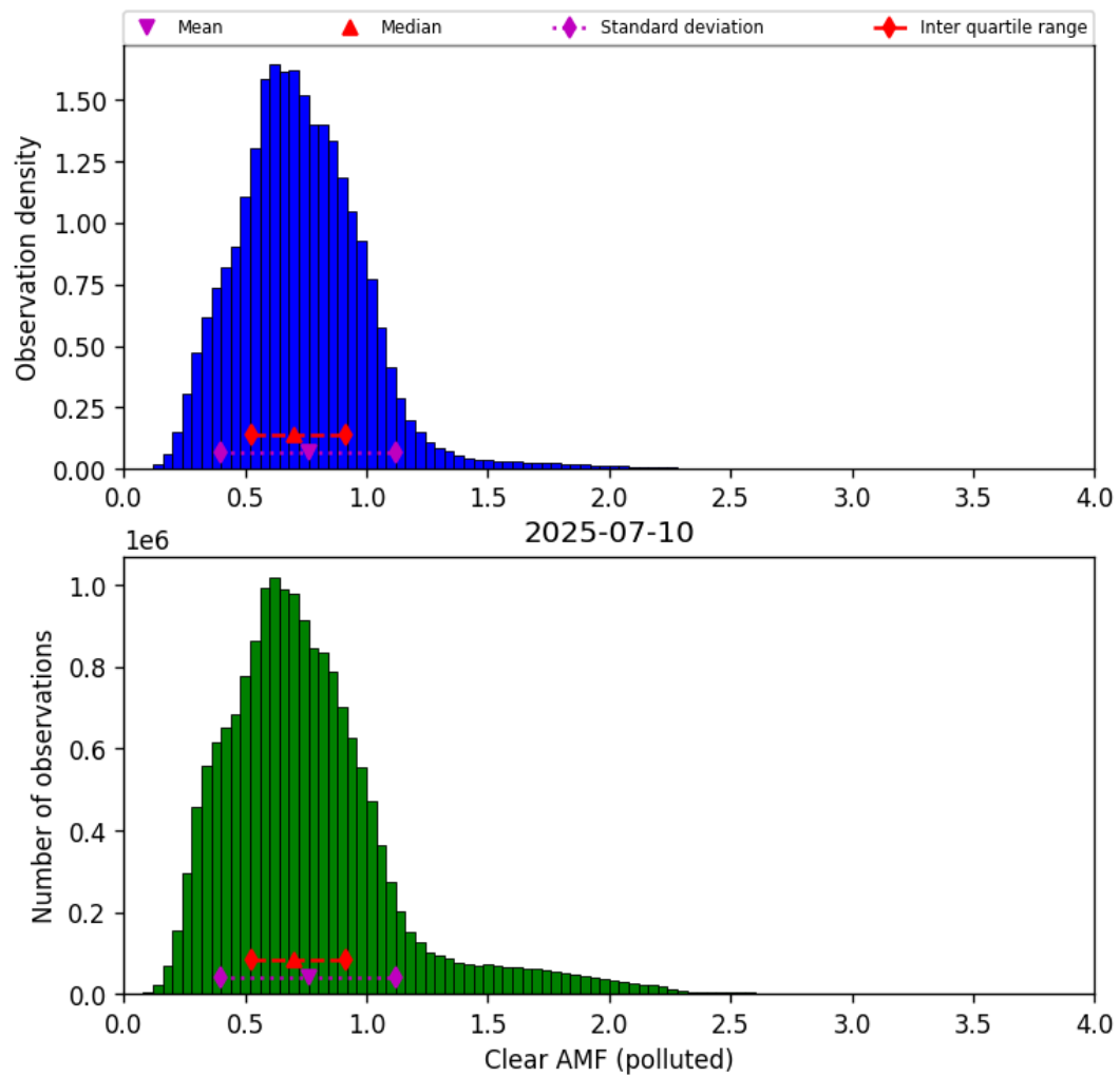
Figure 82: Histogram of “Clear AMF (polluted)” for 2025-07-10 to 2025-07-11
