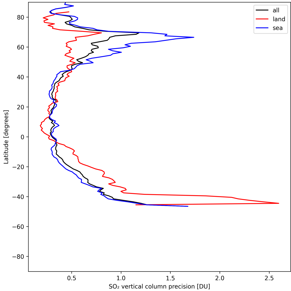
Figure 32: Zonal average of “SO 2 vertical column precision” for 2025-07-10 to 2025-07-11.
