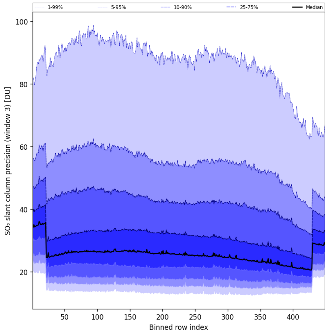
Figure 99: Along track statistics of “SO 2 slant column precision (window 3)” for 2025-07-10 to 2025-07-11
