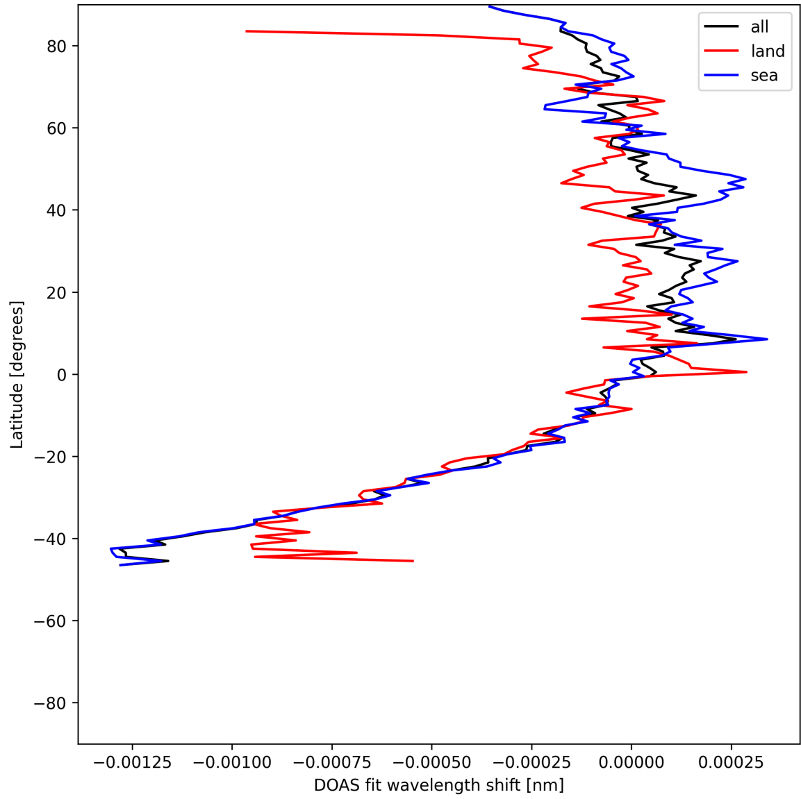
Figure 50: Zonal average of “DOAS fit wavelength shift” for 2025-07-10 to 2025-07-11.
