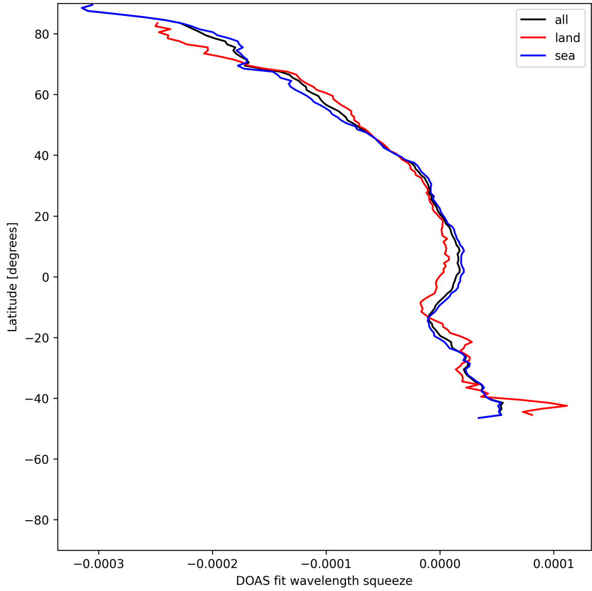
Figure 51: Zonal average of “DOAS fit wavelength squeeze” for 2025-07-10 to 2025-07-11.
