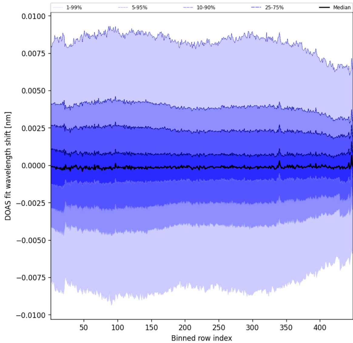
Figure 104: Along track statistics of “DOAS fit wavelength shift” for 2025-07-10 to 2025-07-11
