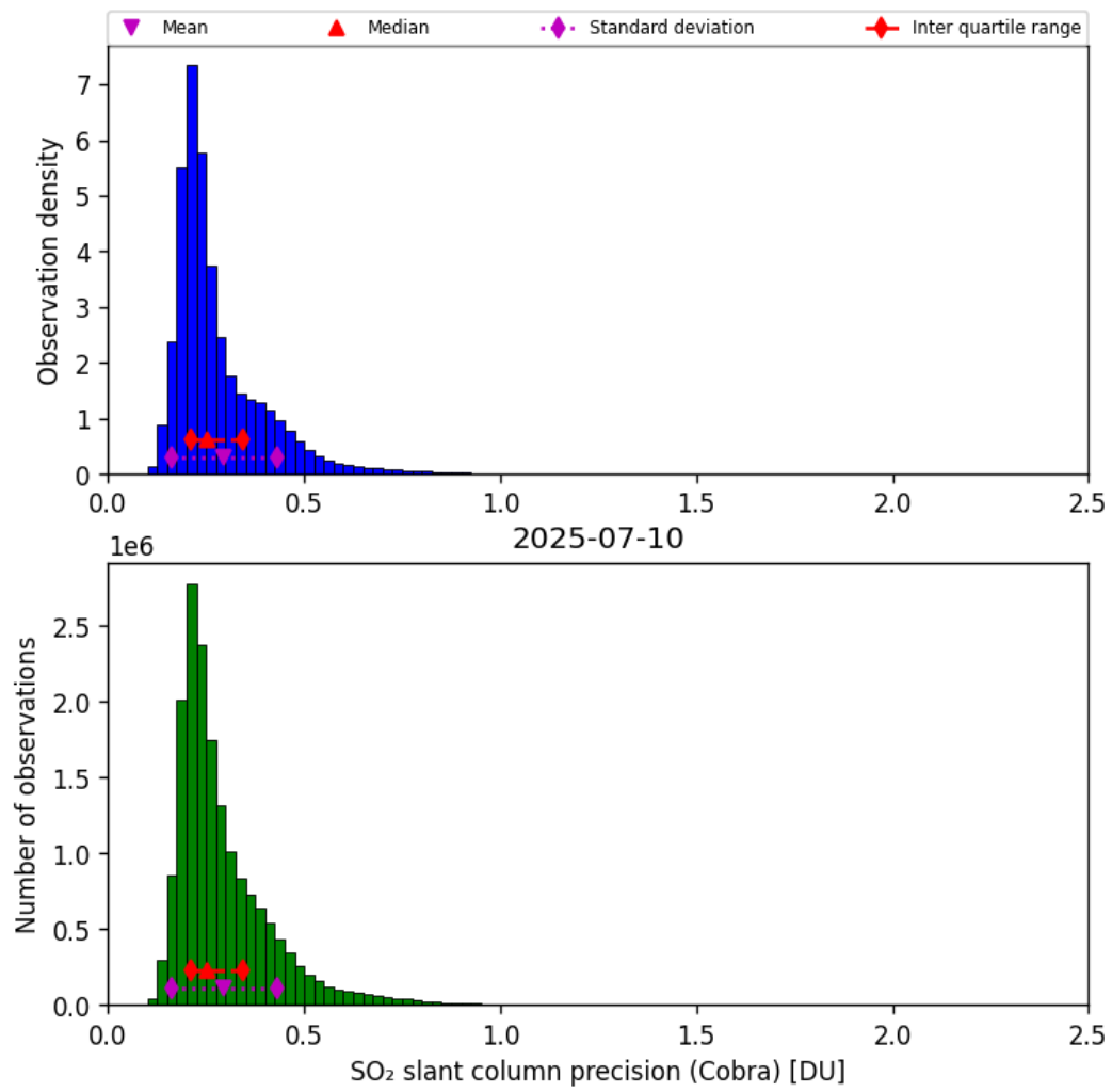
Figure 62: Histogram of “SO 2 slant column precision (Cobra)” for 2025-07-10 to 2025-07-11
