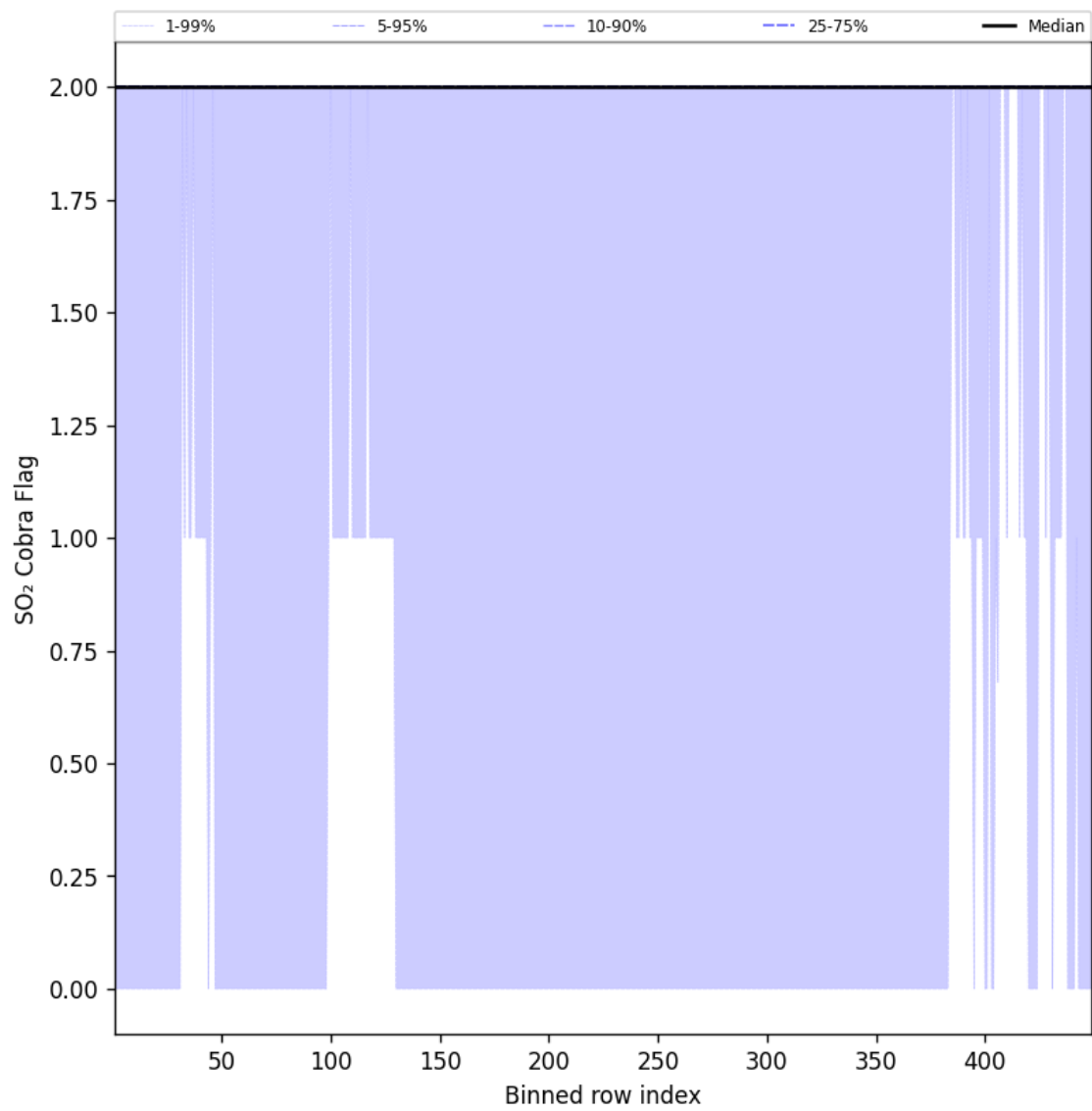
Figure 102: Along track statistics of “SO 2 Cobra Flag” for 2025-07-10 to 2025-07-11
