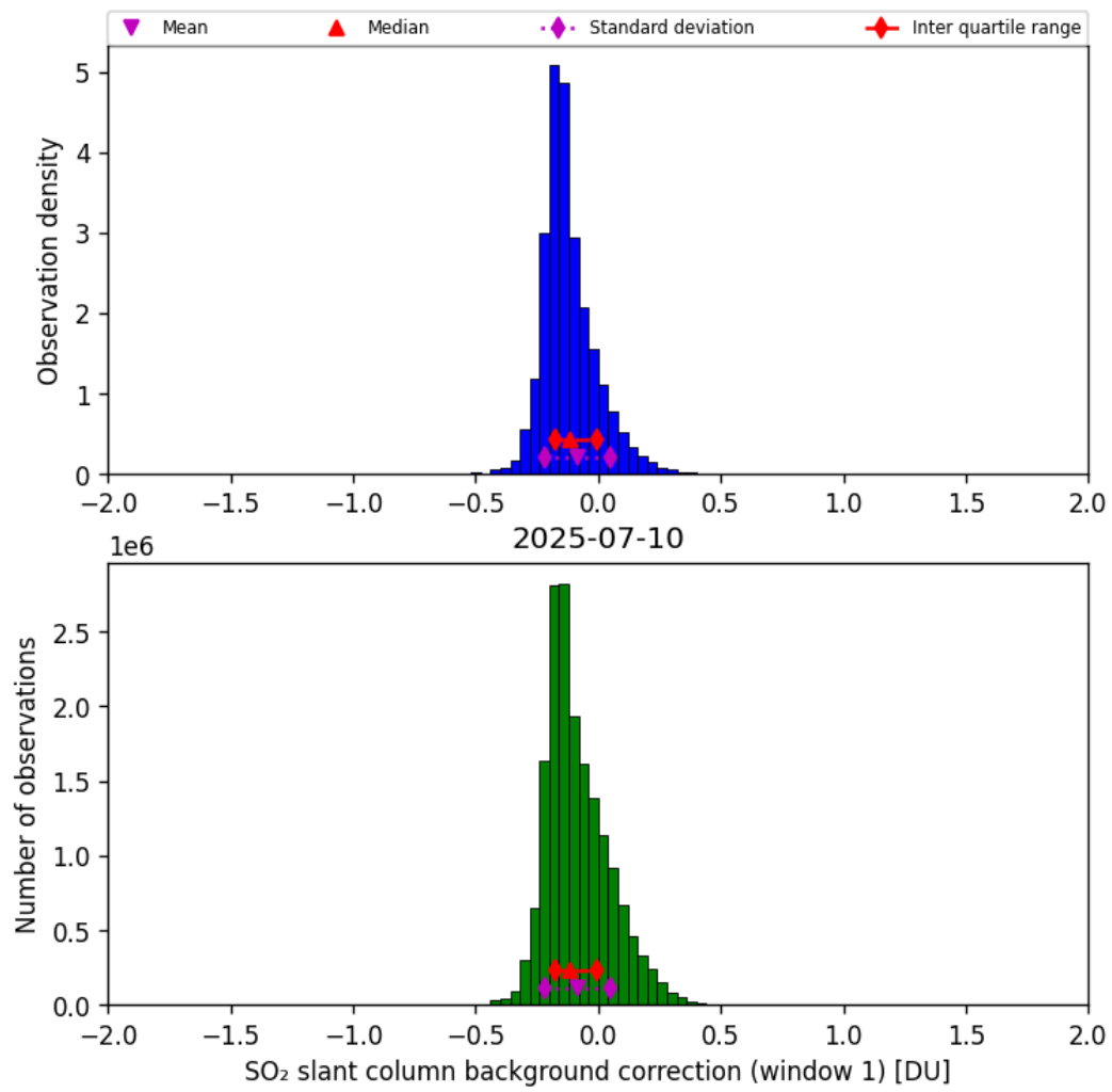
Figure 66: Histogram of “SO 2 slant column background correction (window 1)” for 2025-07-10 to 2025-07-11
