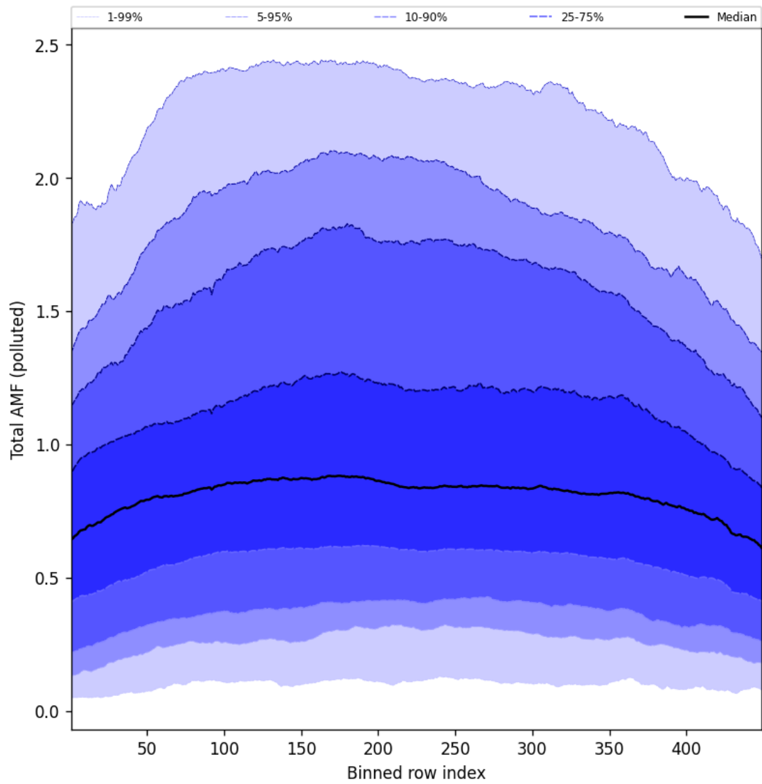
Figure 107: Along track statistics of “Total AMF (polluted)” for 2025-07-10 to 2025-07-11
