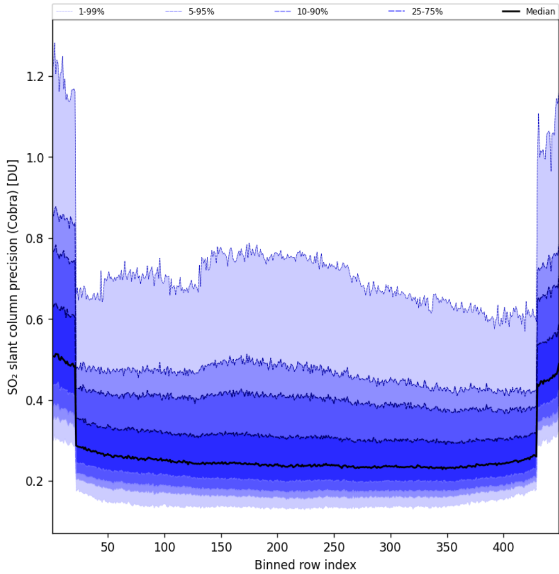
Figure 89: Along track statistics of “SO 2 slant column precision (Cobra)” for 2025-07-10 to 2025-07-11
