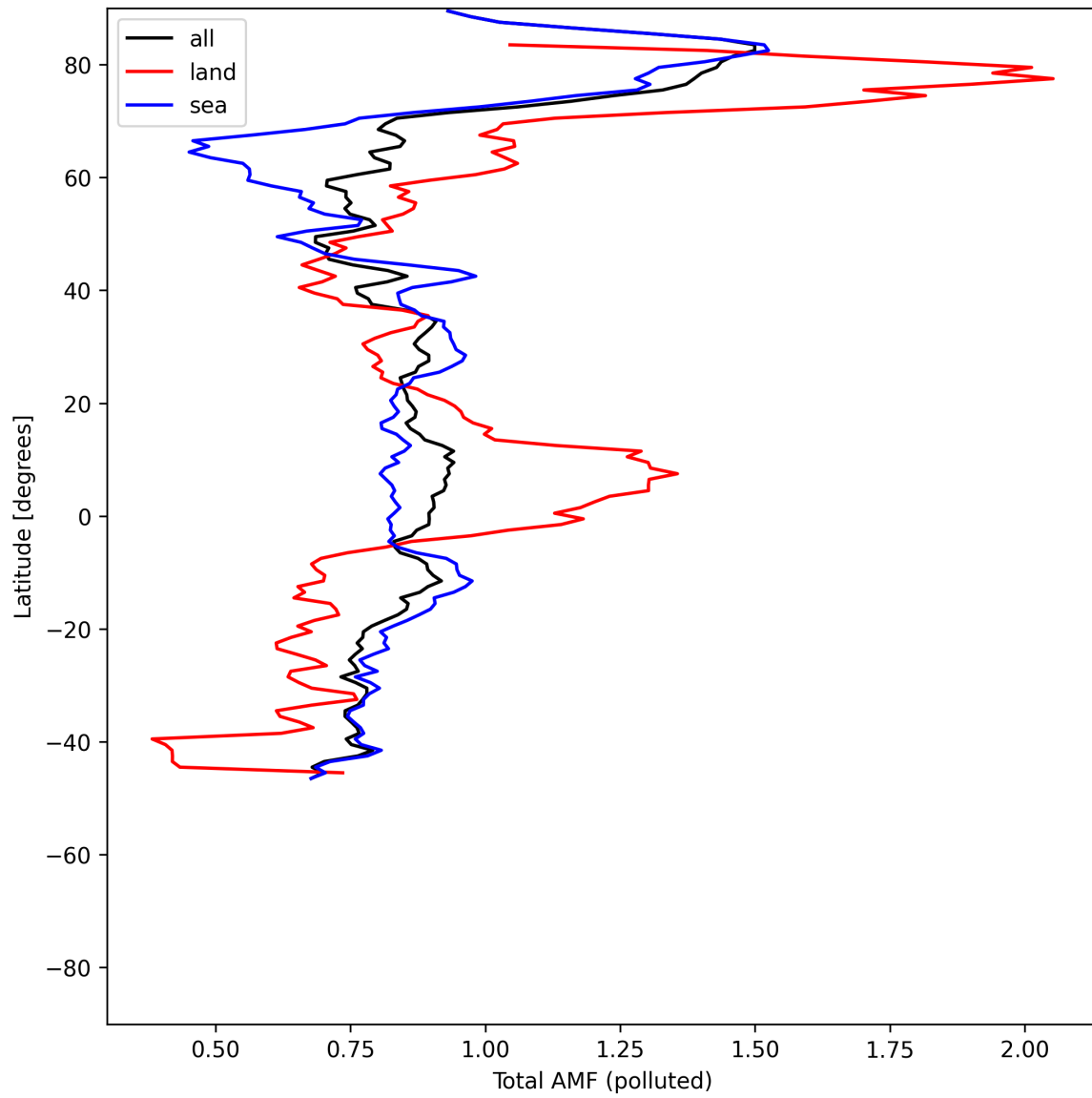
Figure 53: Zonal average of “Total AMF (polluted)” for 2025-07-10 to 2025-07-11.
