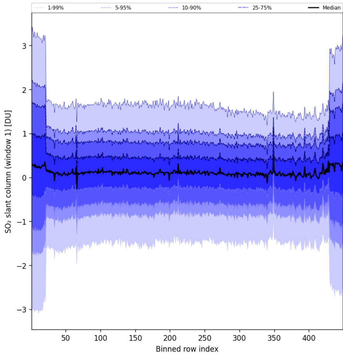
Figure 90: Along track statistics of "SO 2 slant column (window 1)" for 2025-07-10 to 2025-07-11
