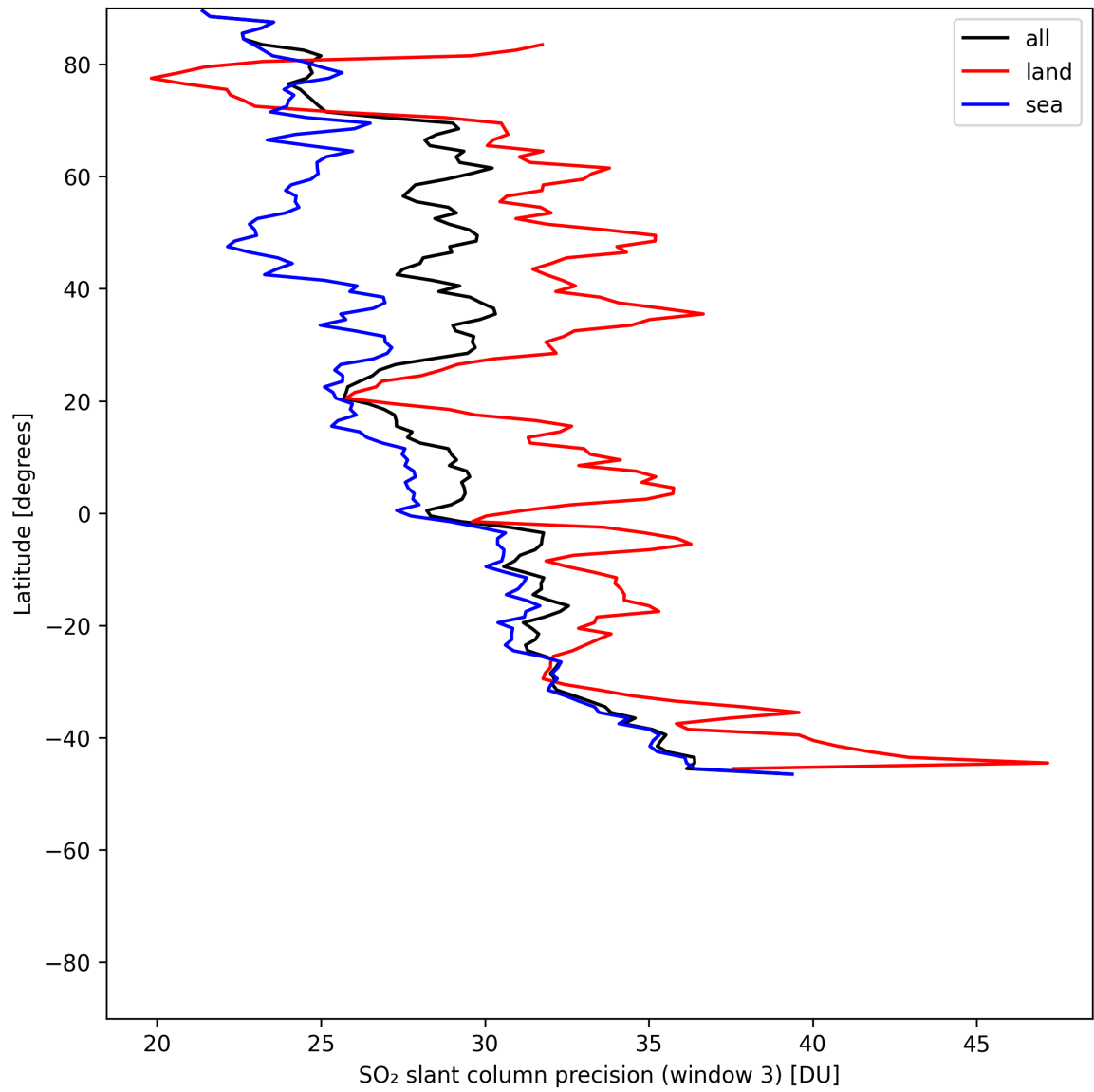
Figure 45: Zonal average of “SO 2 slant column precision (window 3)” for 2025-07-10 to 2025-07-11.
