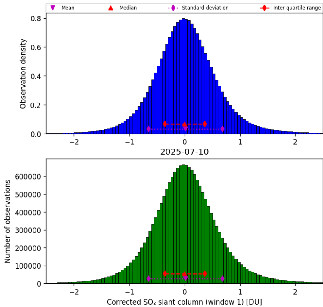
Figure 65: Histogram of “Corrected SO 2 slant column (window 1)” for 2025-07-10 to 2025-07-11
