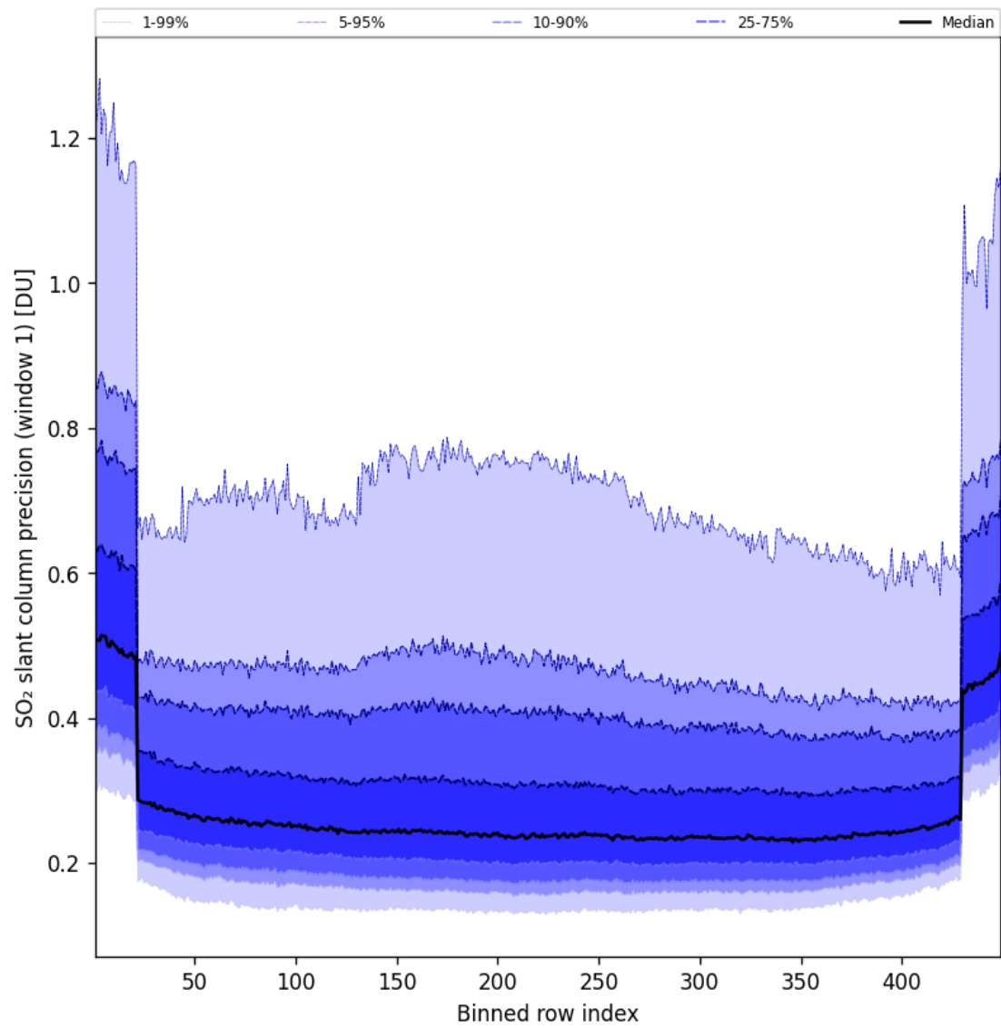
Figure 91: Along track statistics of “SO 2 slant column precision (window 1)” for 2025-07-10 to 2025-07-11
