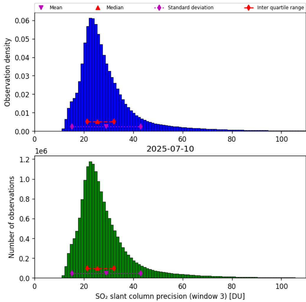
Figure 72: Histogram of “SO 2 slant column precision (window 3)” for 2025-07-10 to 2025-07-11
