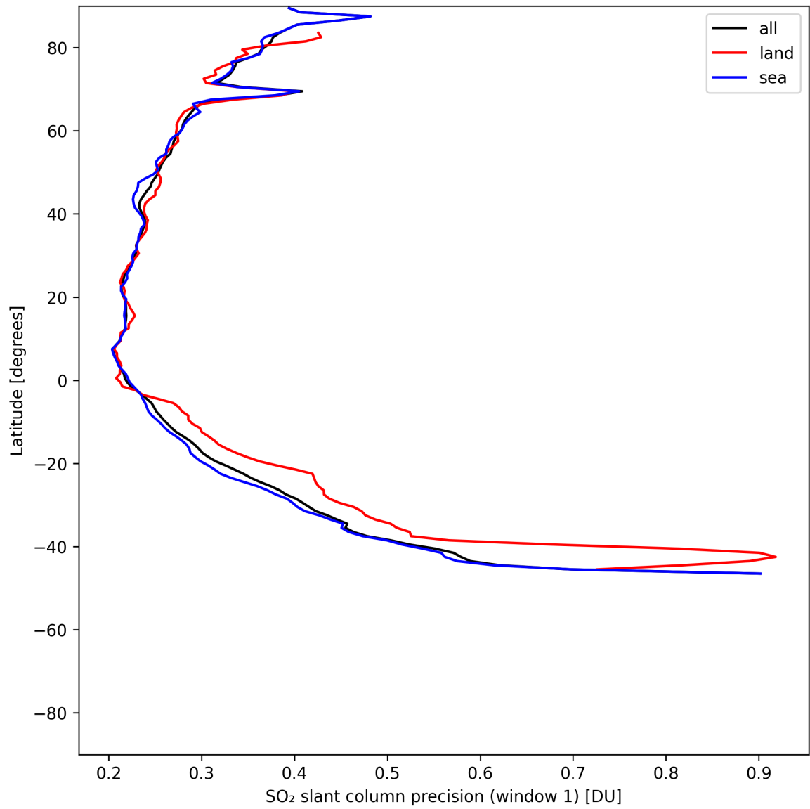
Figure 37: Zonal average of “SO 2 slant column precision (window 1)” for 2025-07-10 to 2025-07-11.
