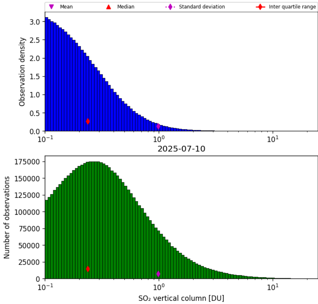
Figure 58: Histogram of “SO 2 vertical column” for 2025-07-10 to 2025-07-11
