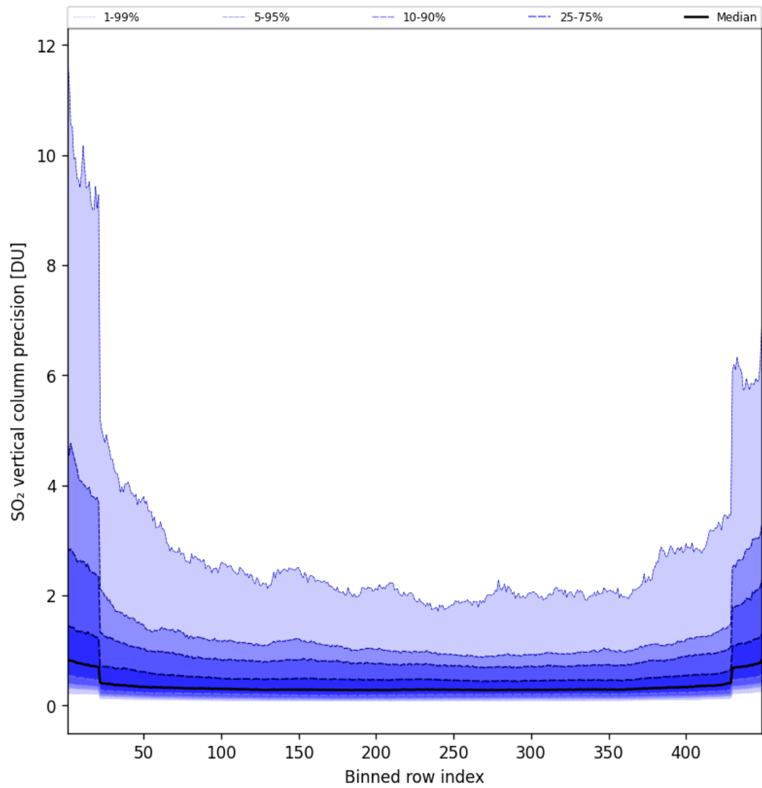
Figure 86: Along track statistics of “SO 2 vertical column precision” for 2025-07-10 to 2025-07-11
