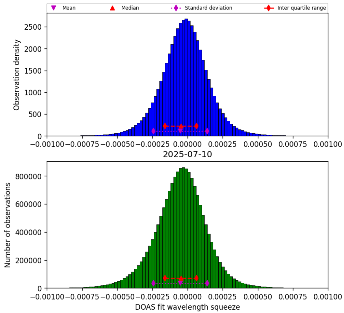
Figure 78: Histogram of “DOAS fit wavelength squeeze” for 2025-07-10 to 2025-07-11
