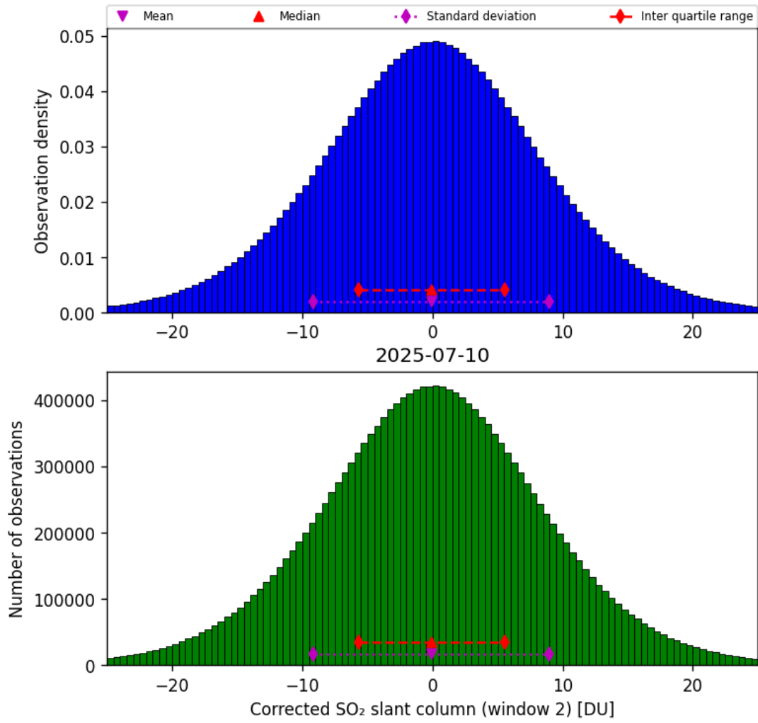
Figure 69: Histogram of “Corrected SO 2 slant column (window 2)” for 2025-07-10 to 2025-07-11
