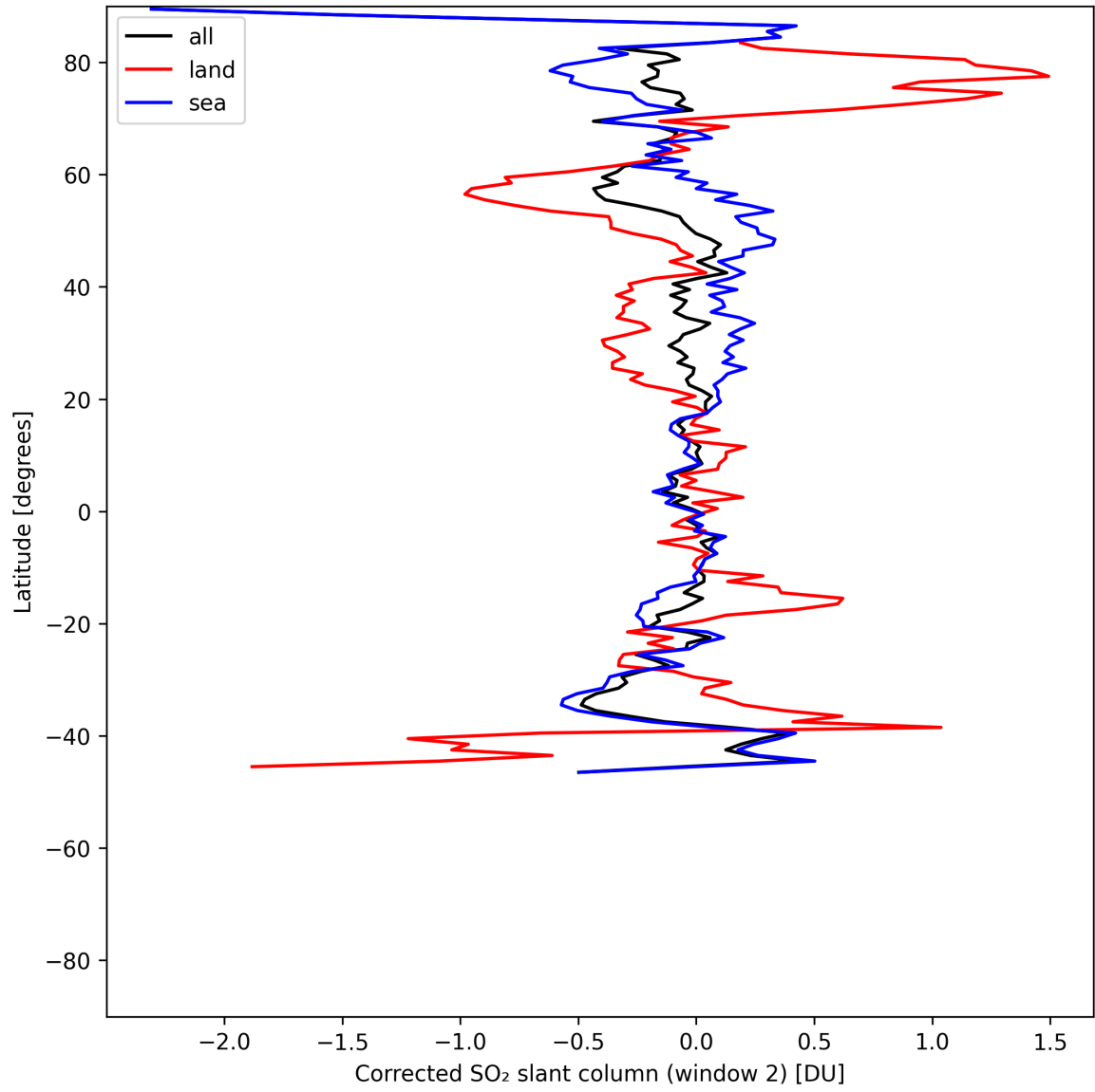
Figure 42: Zonal average of “Corrected SO 2 slant column (window 2)” for 2025-07-10 to 2025-07-11.
