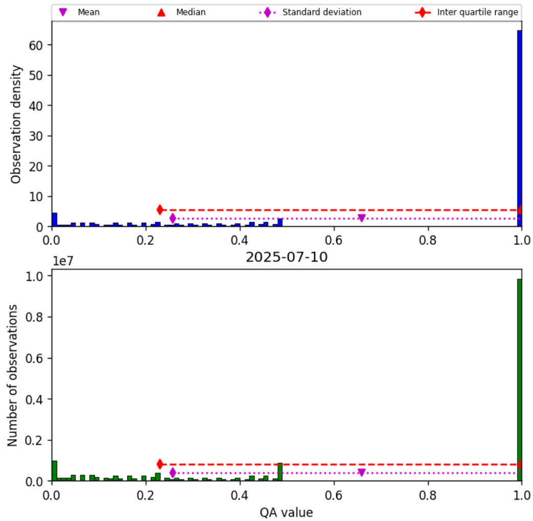
Figure 57: Histogram of “QA value” for 2025-07-10 to 2025-07-11
