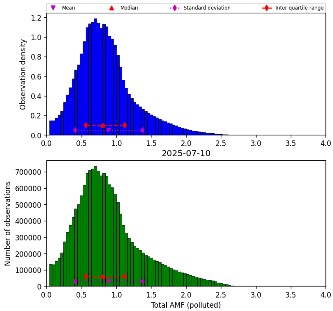
Figure 80: Histogram of “Total AMF (polluted)” for 2025-07-10 to 2025-07-11
