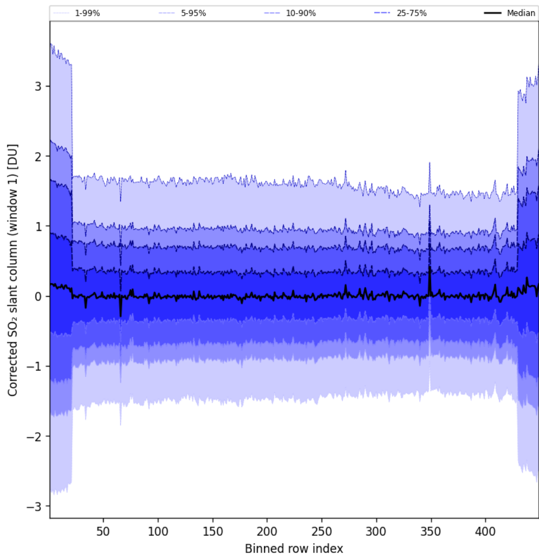
Figure 92: Along track statistics of “Corrected SO 2 slant column (window 1)” for 2025-07-10 to 2025-07-11
