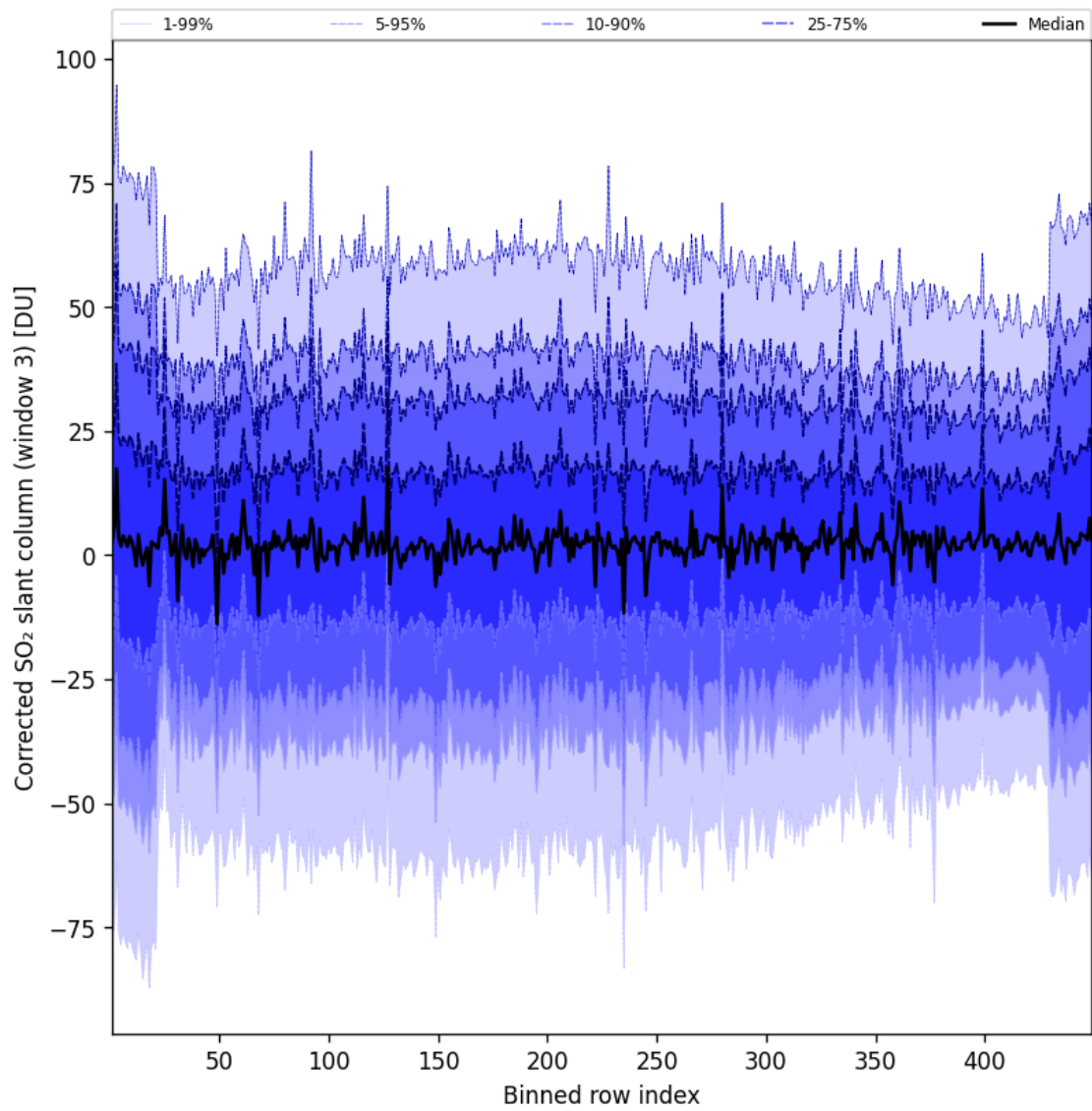
Figure 100: Along track statistics of “Corrected SO 2 slant column (window 3)” for 2025-07-10 to 2025-07-11
