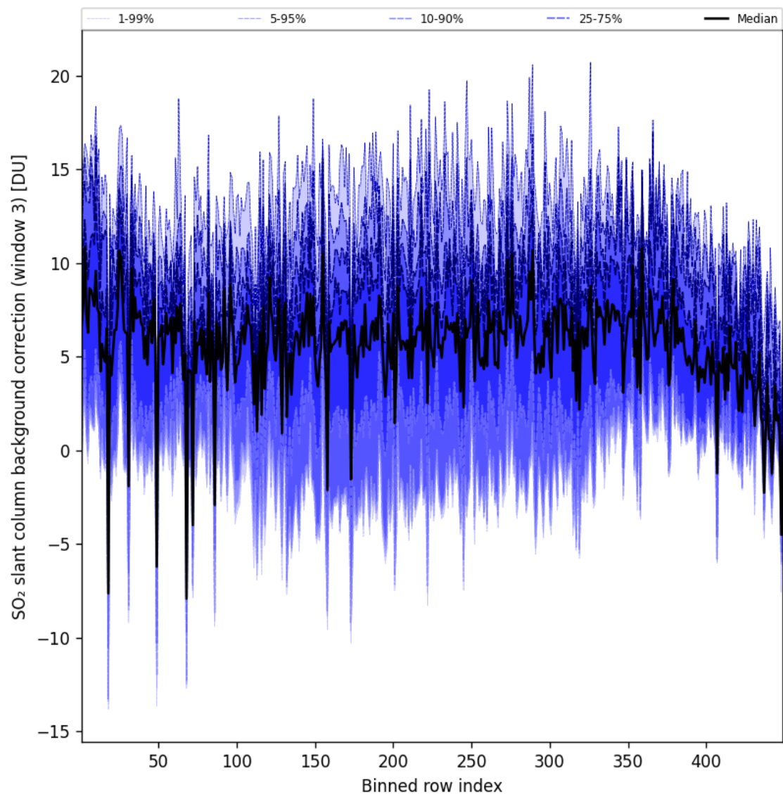
Figure 101: Along track statistics of “SO 2 slant column background correction (window 3)” for 2025-07-10 to 2025-07-11
