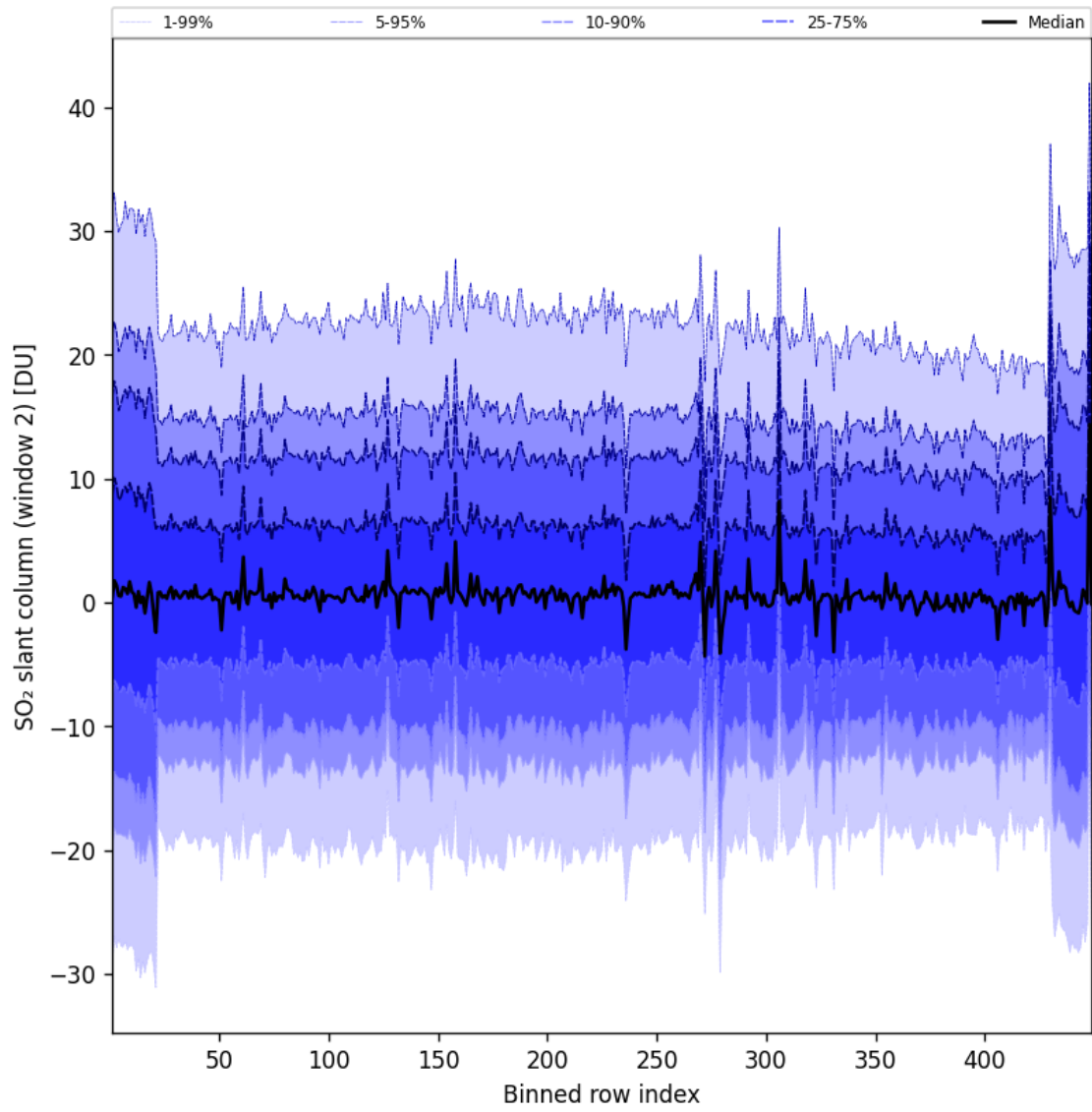
Figure 94: Along track statistics of “SO 2 slant column (window 2)” for 2025-07-10 to 2025-07-11
