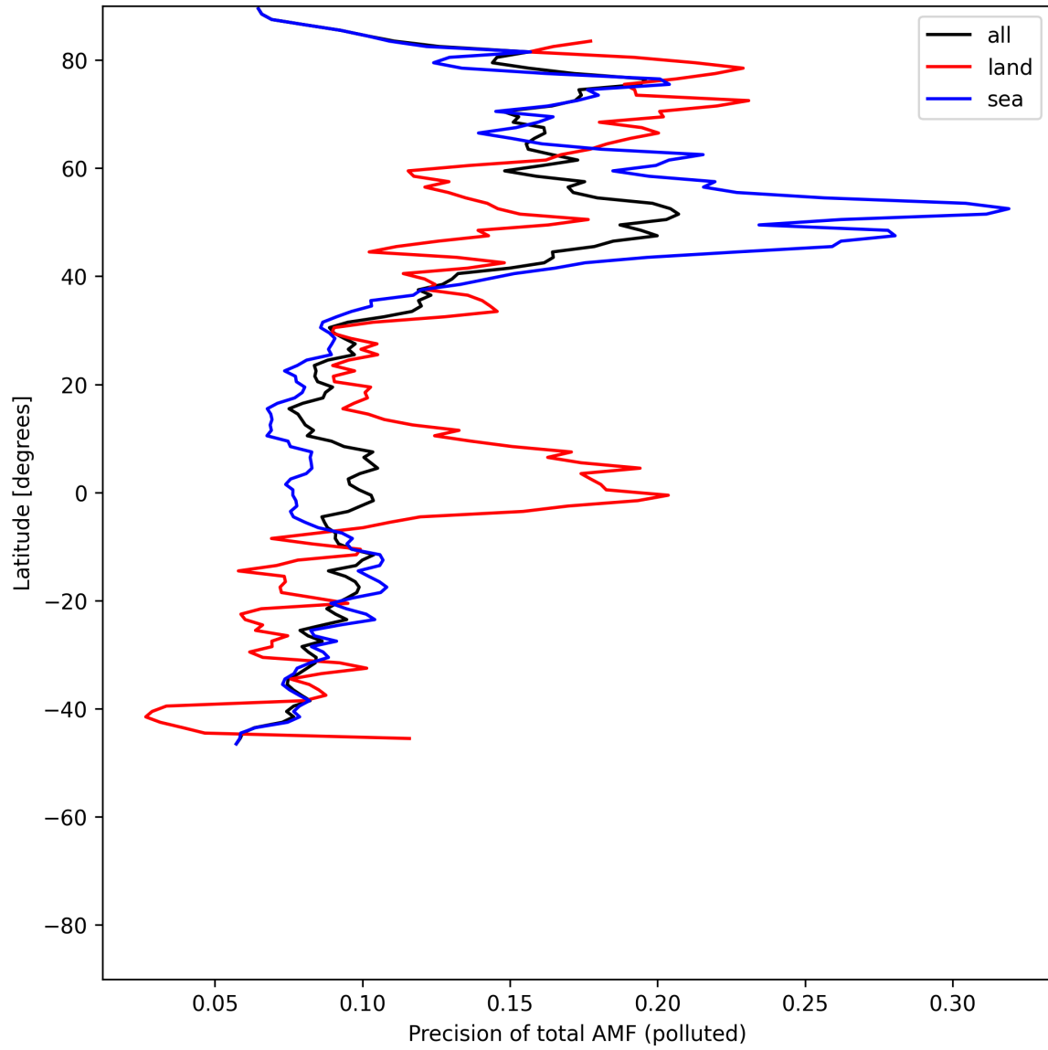
Figure 54: Zonal average of “Precision of total AMF (polluted)” for 2025-07-10 to 2025-07-11.
