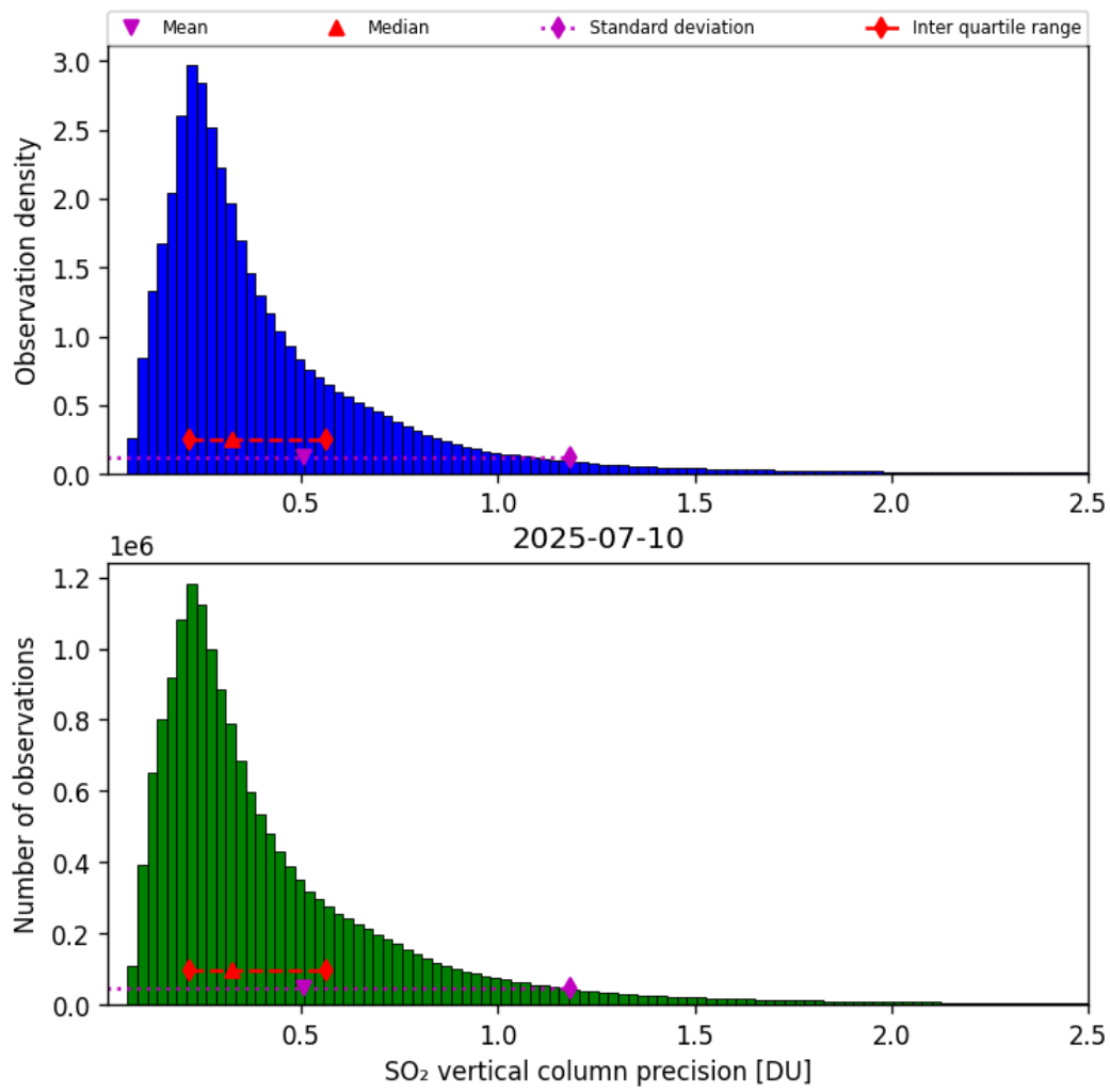
Figure 59: Histogram of “SO 2 vertical column precision” for 2025-07-10 to 2025-07-11
