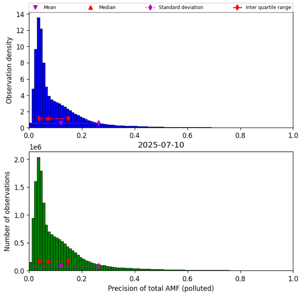
Figure 81: Histogram of “Precision of total AMF (polluted)” for 2025-07-10 to 2025-07-11
