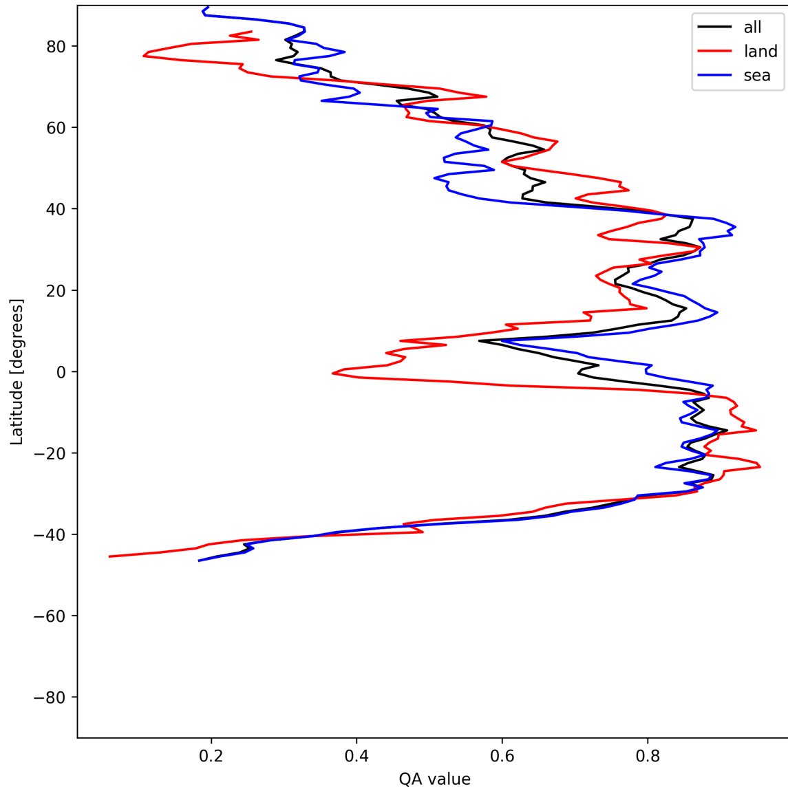
Figure 30: Zonal average of “QA value” for 2025-07-10 to 2025-07-11.
