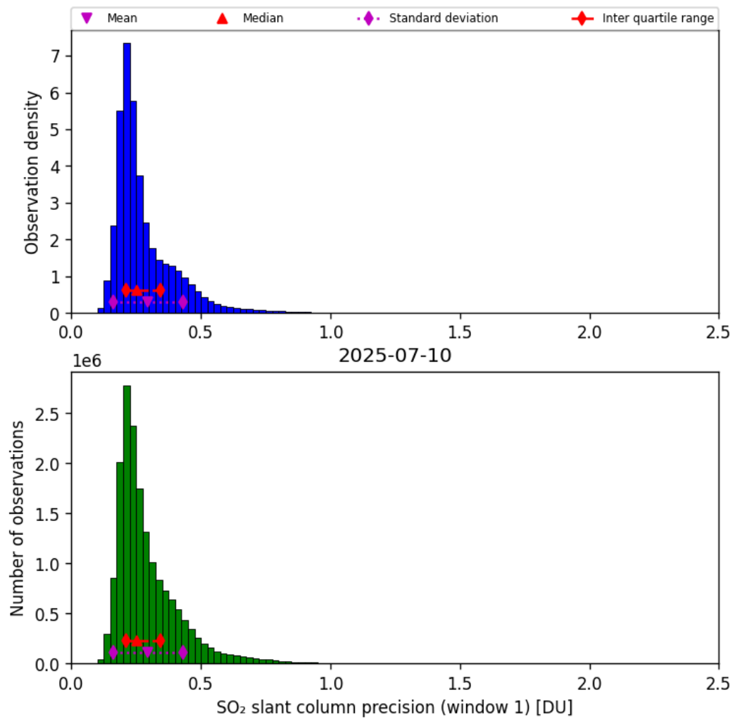
Figure 64: Histogram of “SO 2 slant column precision (window 1)” for 2025-07-10 to 2025-07-11
