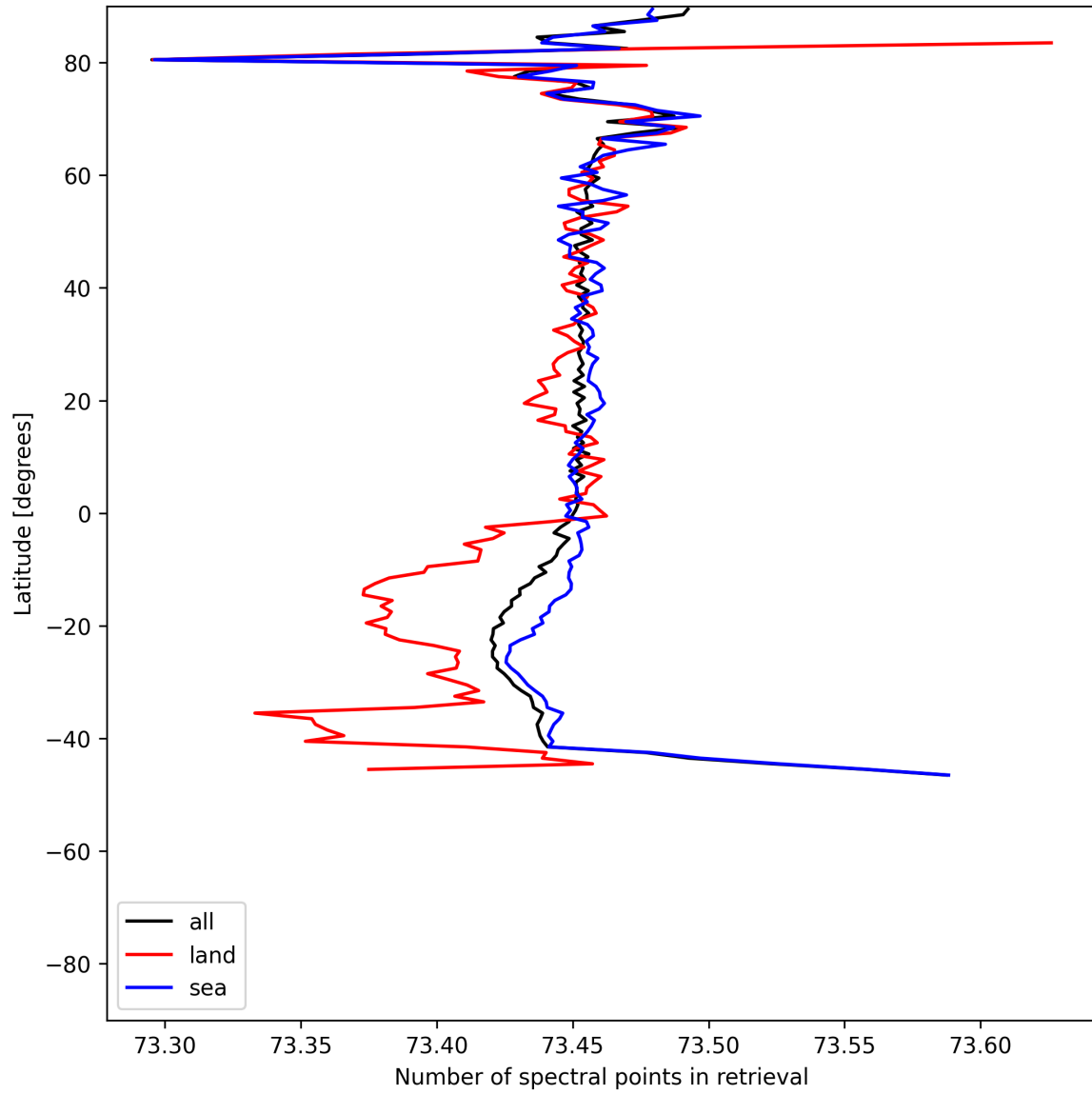
Figure 56: Zonal average of “Number of spectral points in retrieval” for 2025-07-10 to 2025-07-11.
