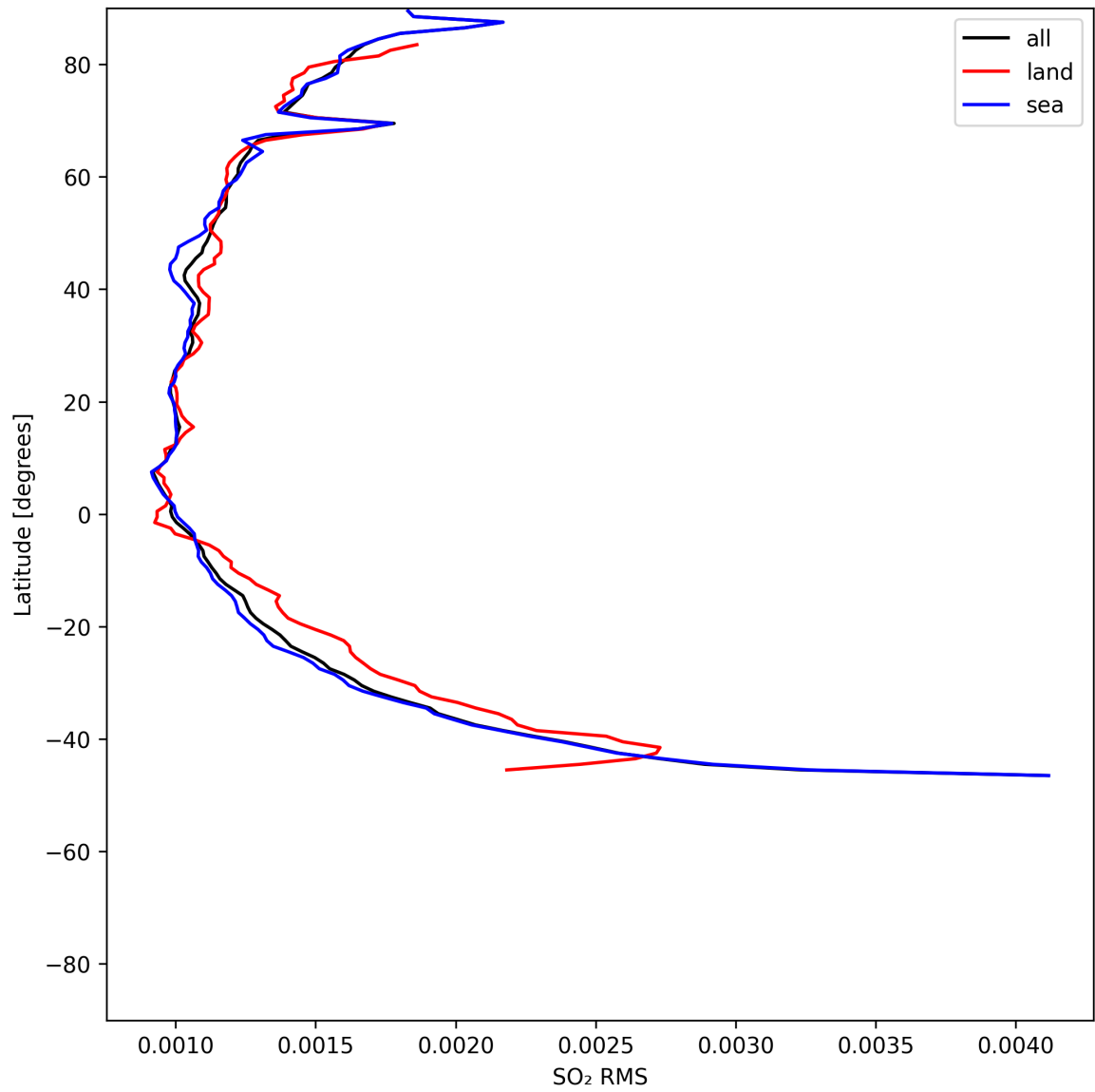
Figure 52: Zonal average of “SO 2 RMS” for 2025-07-10 to 2025-07-11.
