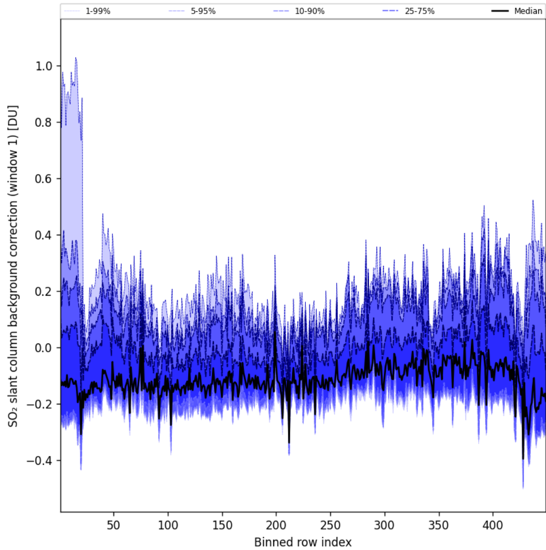
Figure 93: Along track statistics of “SO 2 slant column background correction (window 1)” for 2025-07-10 to 2025-07-11
