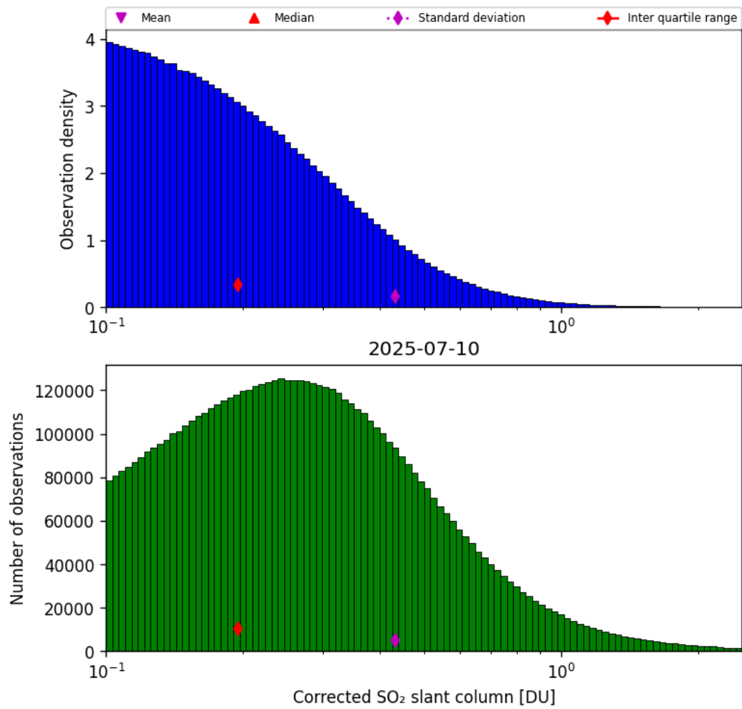
Figure 60: Histogram of “Corrected SO 2 slant column” for 2025-07-10 to 2025-07-11
