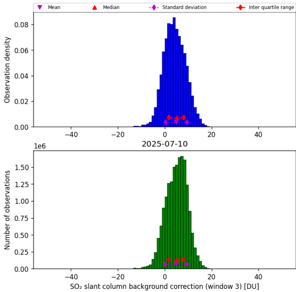
Figure 74: Histogram of “SO 2 slant column background correction (window 3)” for 2025-07-10 to 2025-07-11
