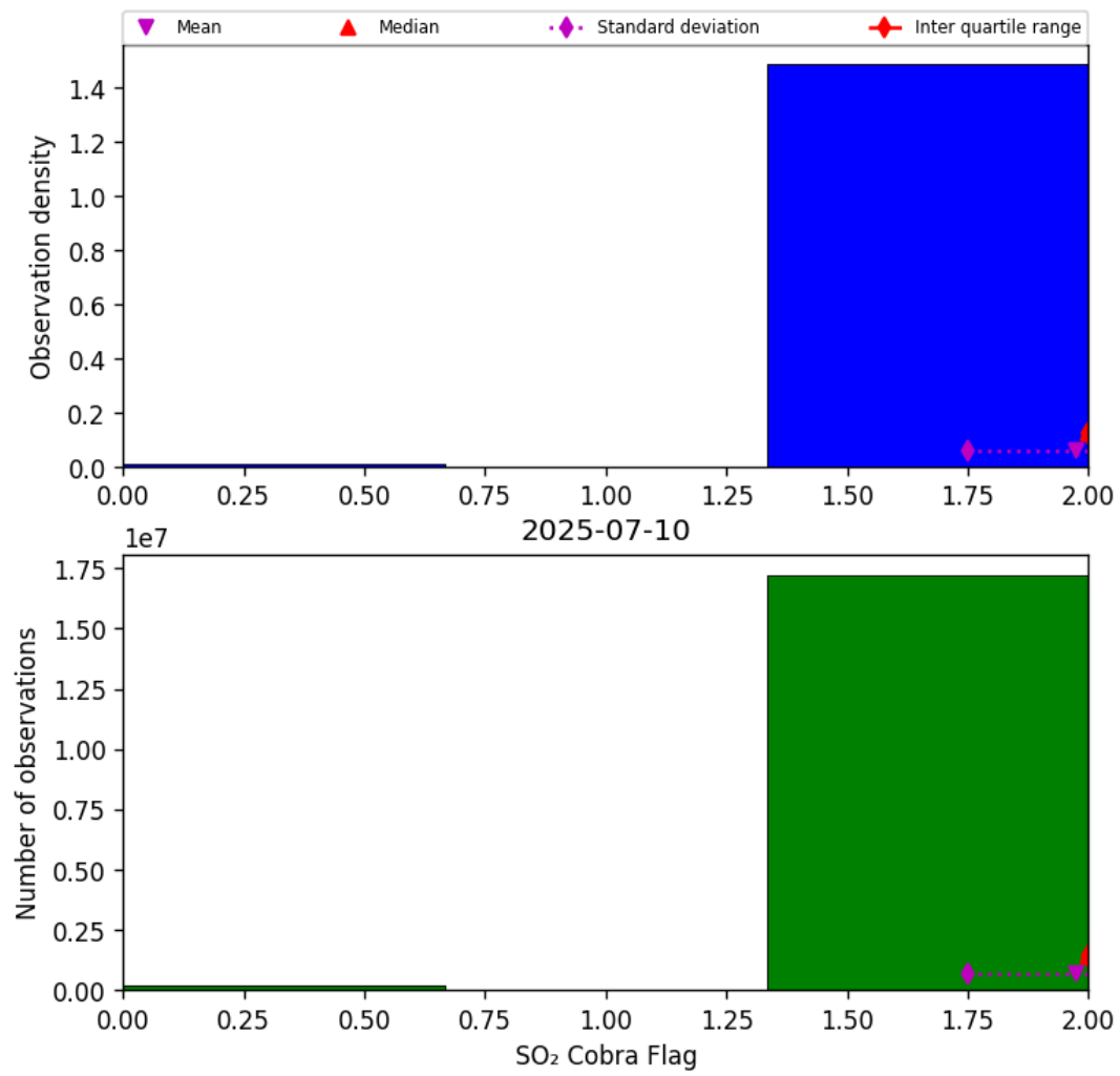
Figure 75: Histogram of “SO 2 Cobra Flag” for 2025-07-10 to 2025-07-11
