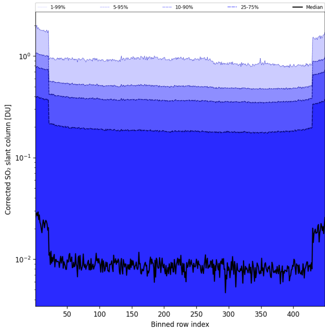
Figure 87: Along track statistics of “Corrected SO 2 slant column” for 2025-07-10 to 2025-07-11
