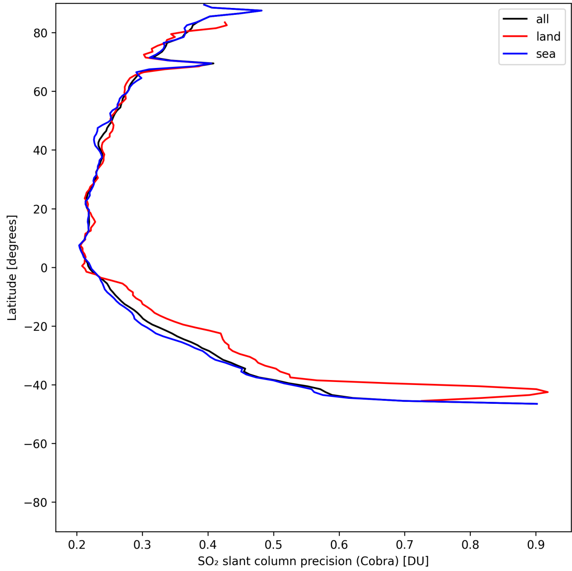
Figure 35: Zonal average of “SO 2 slant column precision (Cobra)” for 2025-07-10 to 2025-07-11.
