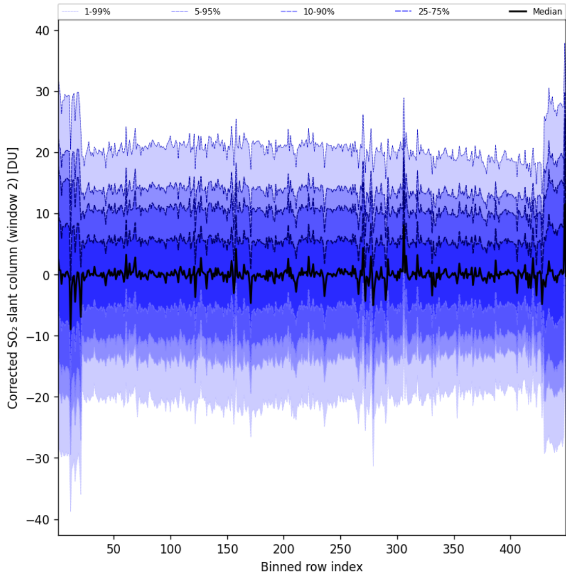
Figure 96: Along track statistics of “Corrected SO 2 slant column (window 2)” for 2025-07-10 to 2025-07-11
