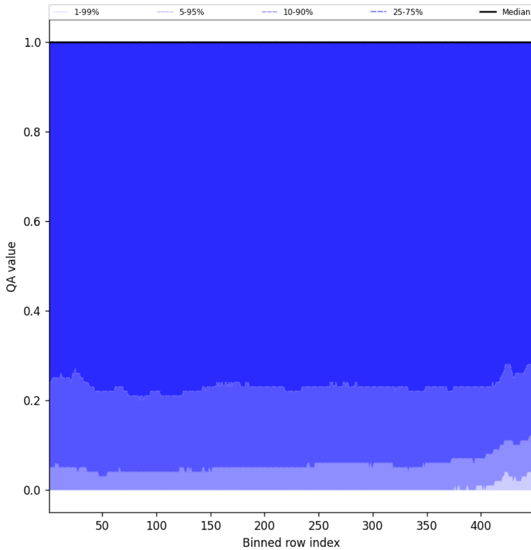
Figure 84: Along track statistics of “QA value” for 2025-07-10 to 2025-07-11
