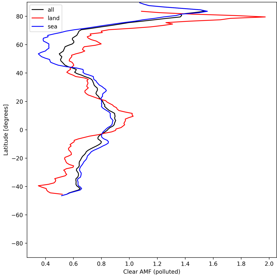
Figure 55: Zonal average of “Clear AMF (polluted)” for 2025-07-10 to 2025-07-11.
