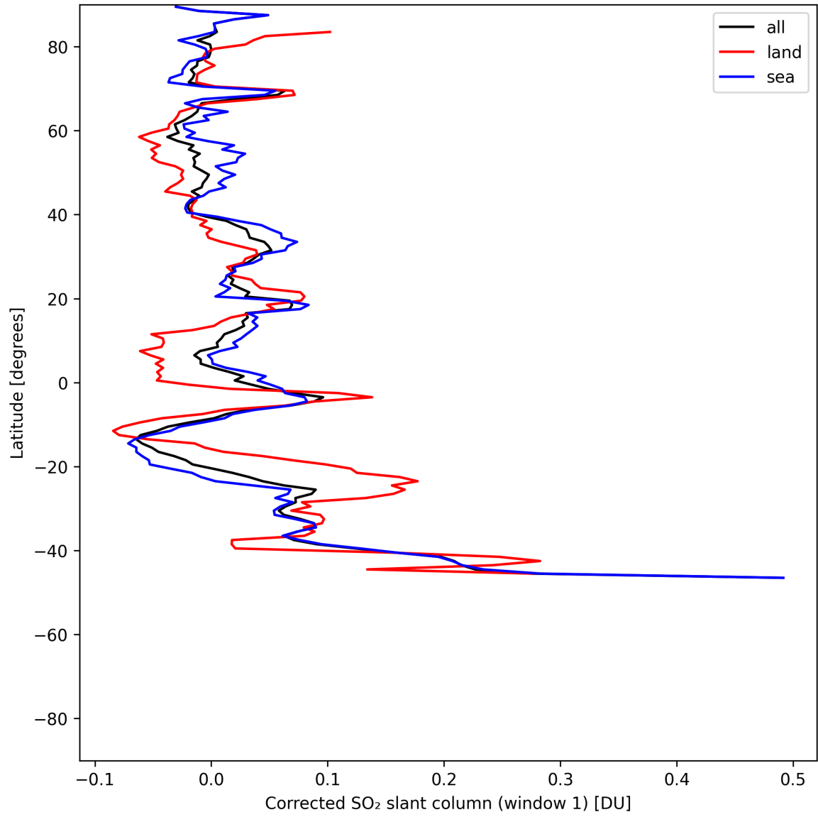
Figure 38: Zonal average of “Corrected SO 2 slant column (window 1)” for 2025-07-10 to 2025-07-11.
