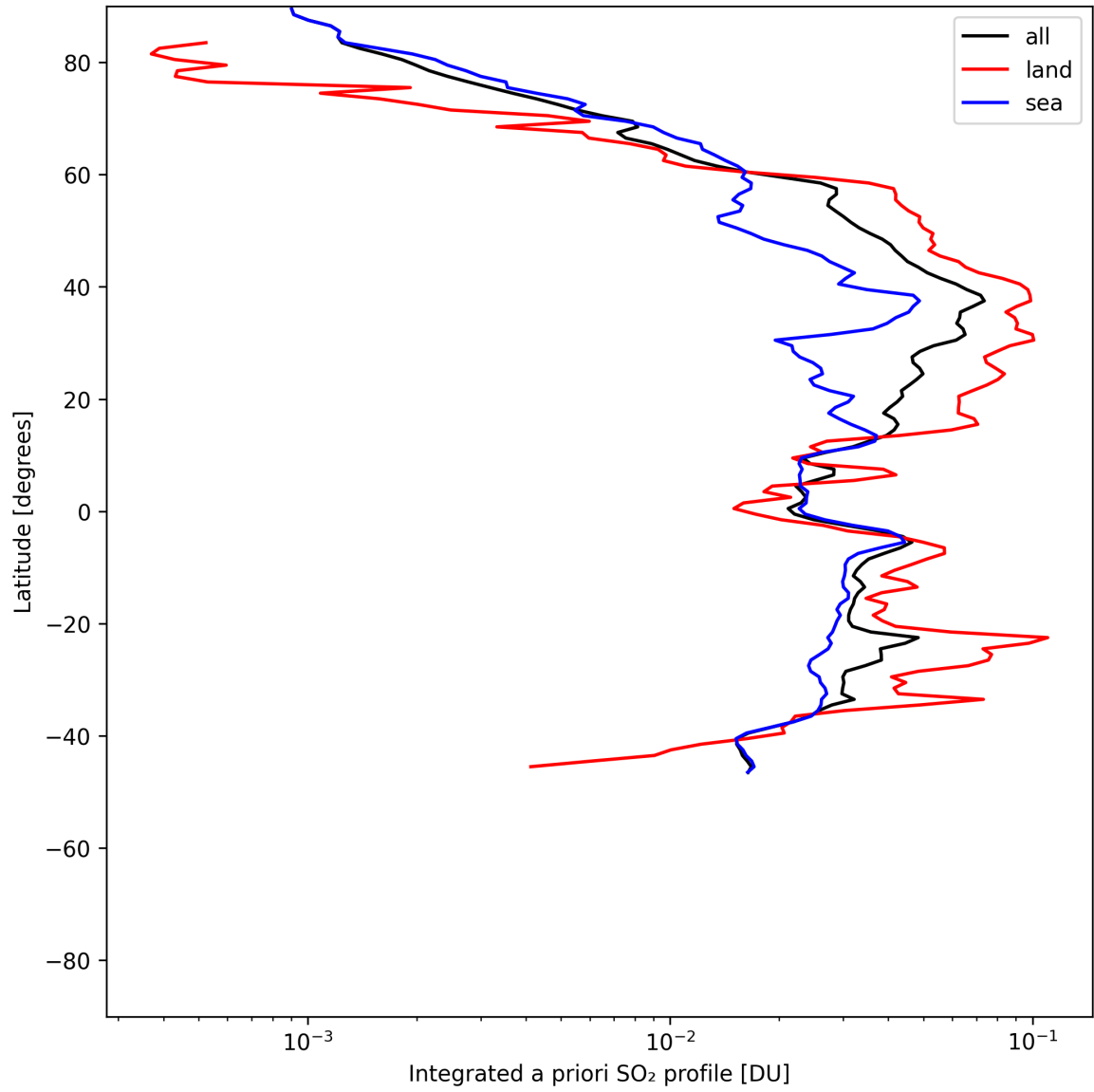
Figure 49: Zonal average of “Integrated a priori SO 2 profile” for 2025-07-10 to 2025-07-11.
