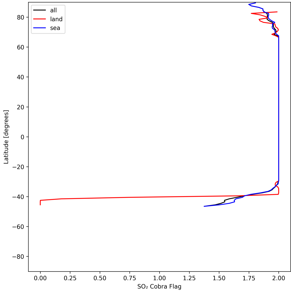
Figure 48: Zonal average of "SO 2 Cobra Flag" for 2025-07-10 to 2025-07-11.
