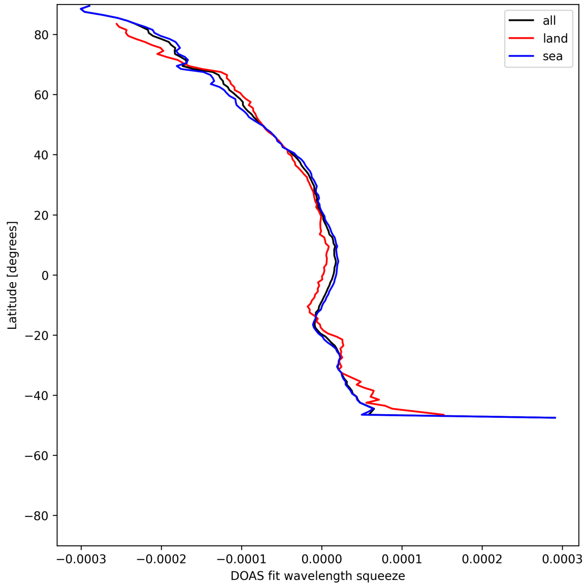
Figure 51: Zonal average of “DOAS fit wavelength squeeze” for 2025-07-11 to 2025-07-11.
