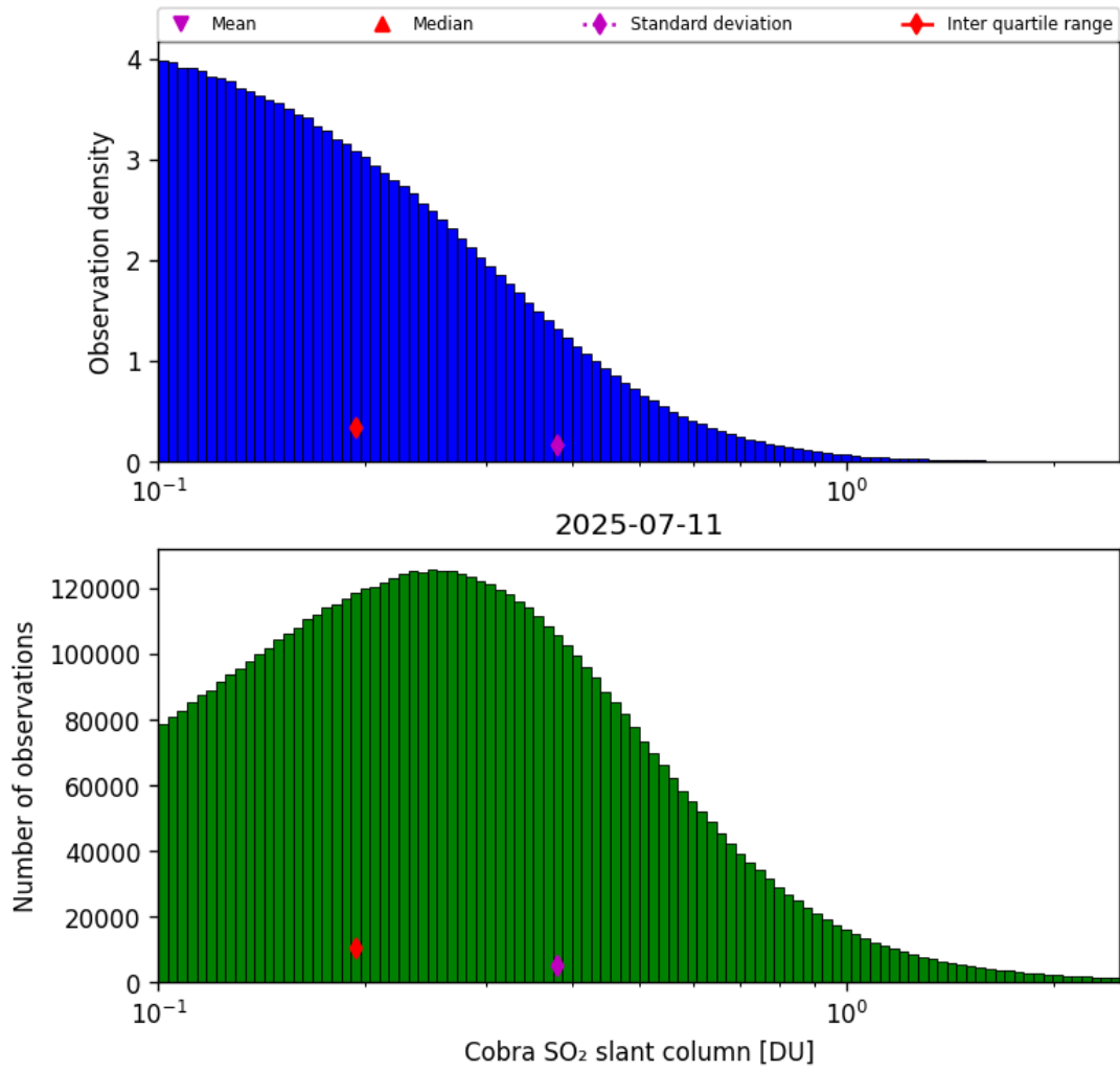
Figure 61: Histogram of “Cobra SO 2 slant column” for 2025-07-11 to 2025-07-11
