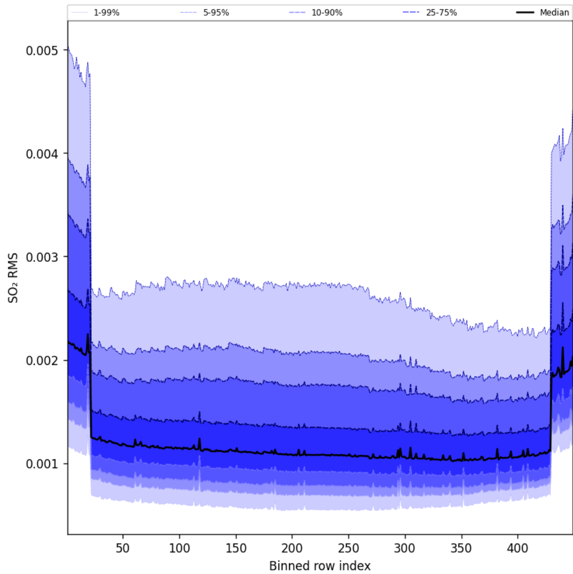
Figure 106: Along track statistics of “SO 2 RMS” for 2025-07-11 to 2025-07-11
