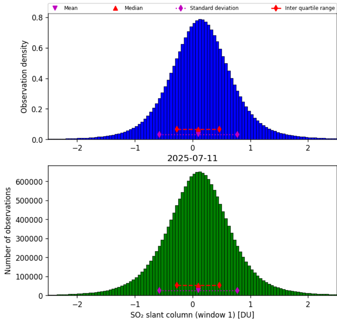
Figure 63: Histogram of “SO 2 slant column (window 1)” for 2025-07-11 to 2025-07-11
