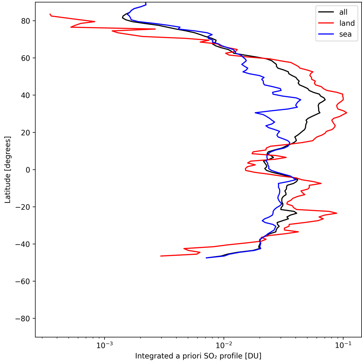
Figure 49: Zonal average of “Integrated a priori SO 2 profile” for 2025-07-11 to 2025-07-11.
