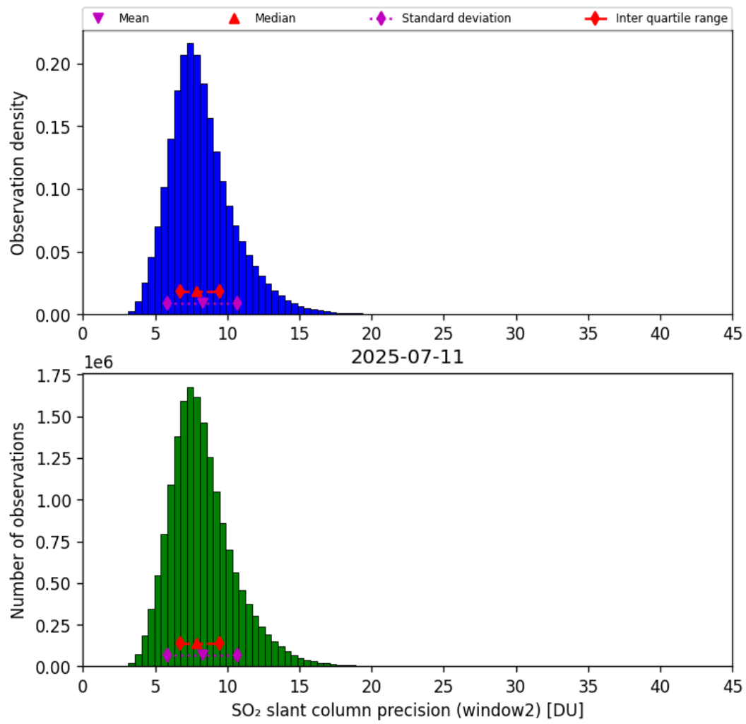
Figure 68: Histogram of “SO 2 slant column precision (window2)” for 2025-07-11 to 2025-07-11
