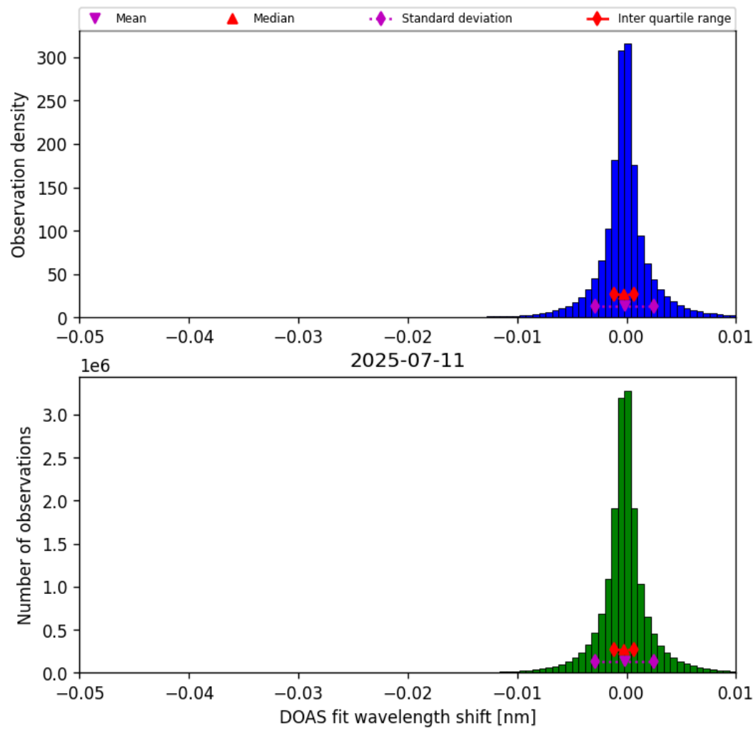
Figure 77: Histogram of “DOAS fit wavelength shift” for 2025-07-11 to 2025-07-11
