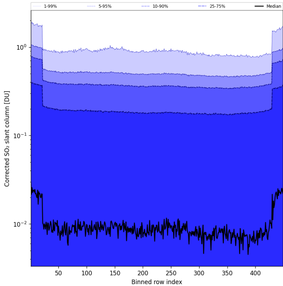
Figure 87: Along track statistics of “Corrected SO 2 slant column” for 2025-07-11 to 2025-07-11
