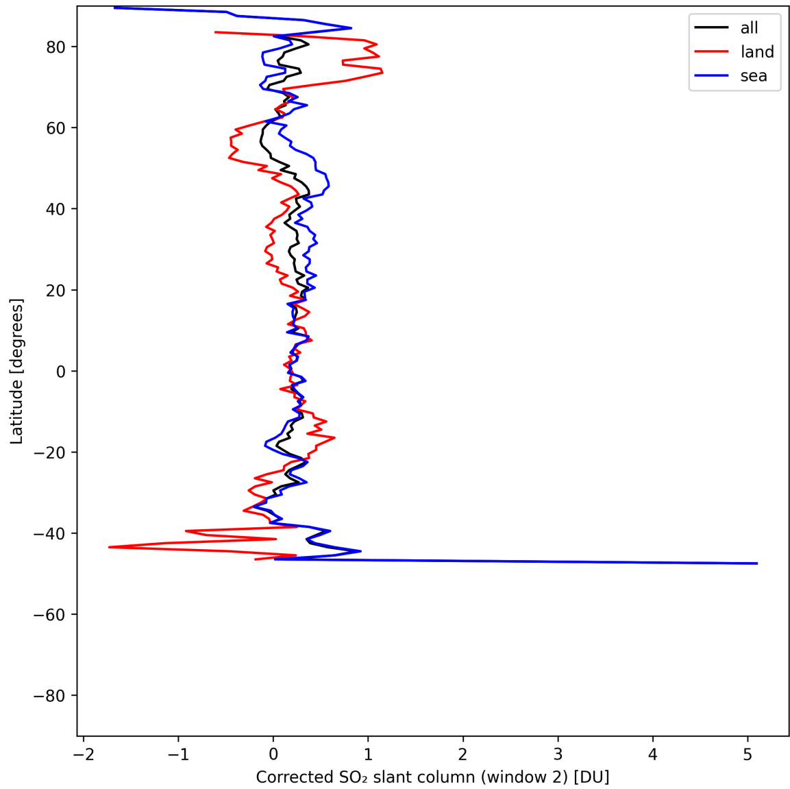
Figure 42: Zonal average of “Corrected SO 2 slant column (window 2)” for 2025-07-11 to 2025-07-11.
