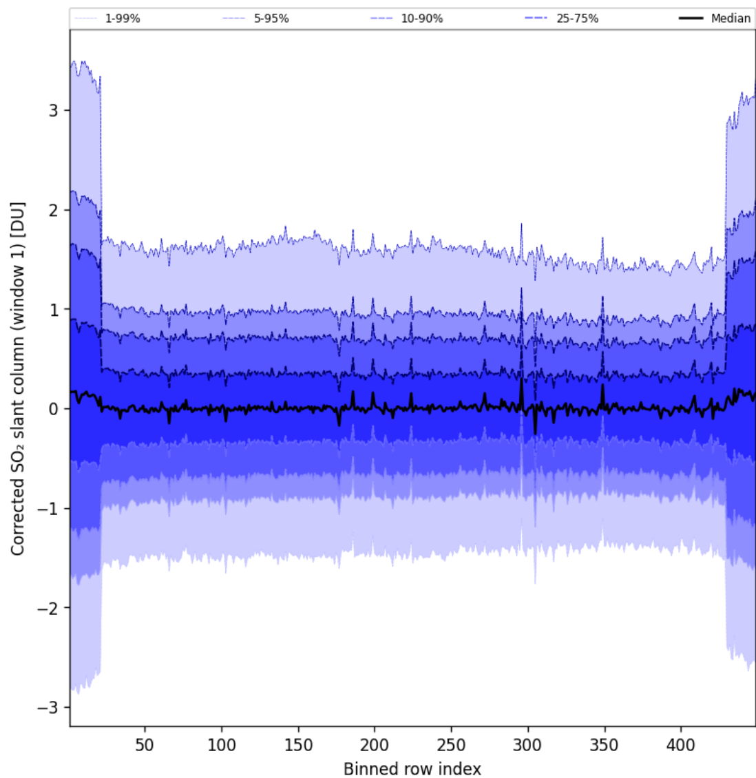
Figure 92: Along track statistics of “Corrected SO 2 slant column (window 1)” for 2025-07-11 to 2025-07-11
