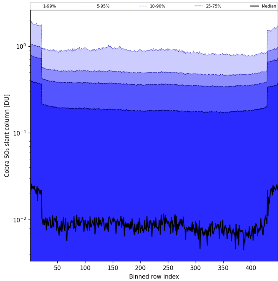
Figure 88: Along track statistics of “Cobra SO 2 slant column” for 2025-07-11 to 2025-07-11
