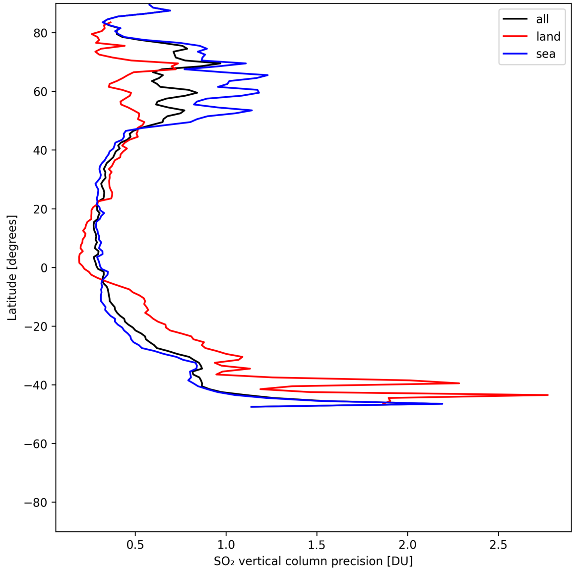
Figure 32: Zonal average of “SO 2 vertical column precision” for 2025-07-11 to 2025-07-11.
