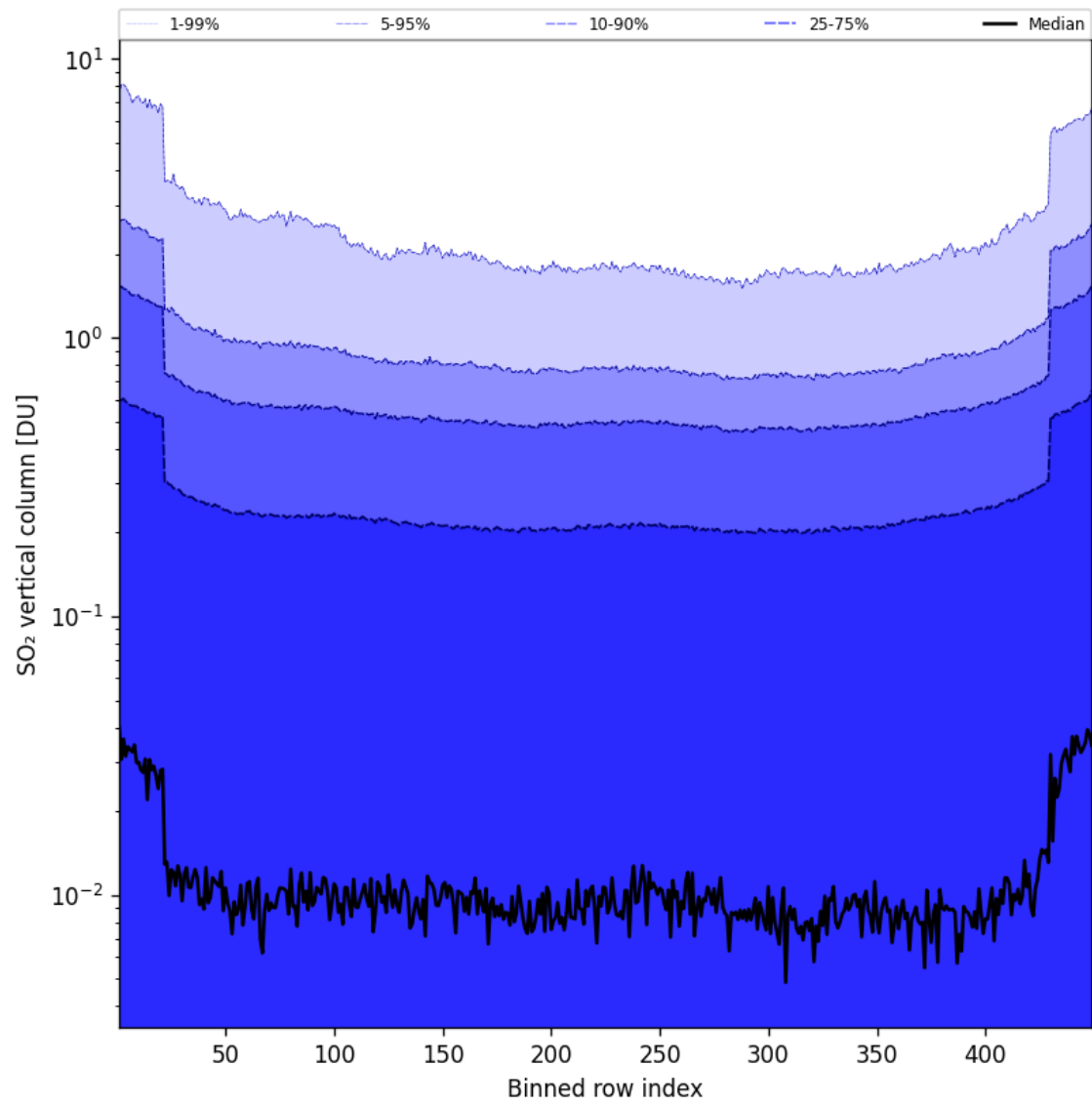
Figure 85: Along track statistics of “SO 2 vertical column” for 2025-07-11 to 2025-07-11
