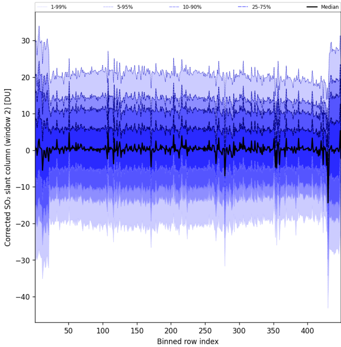
Figure 96: Along track statistics of “Corrected SO 2 slant column (window 2)” for 2025-07-11 to 2025-07-11
