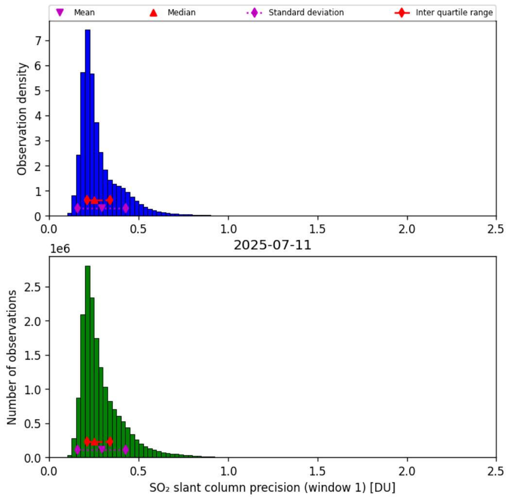
Figure 64: Histogram of “SO 2 slant column precision (window 1)” for 2025-07-11 to 2025-07-11
