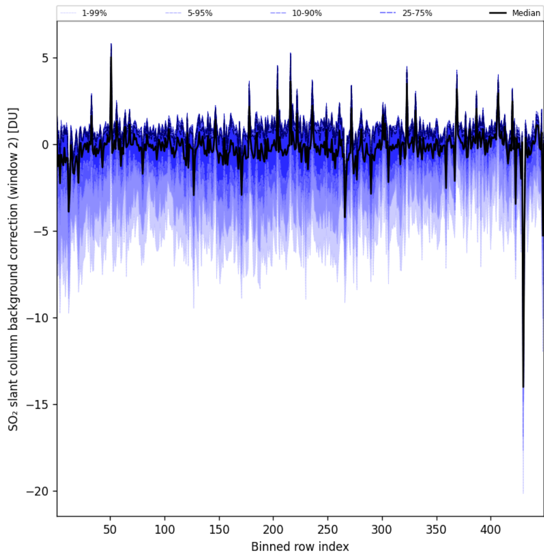
Figure 97: Along track statistics of “SO 2 slant column background correction (window 2)” for 2025-07-11 to 2025-07-11
