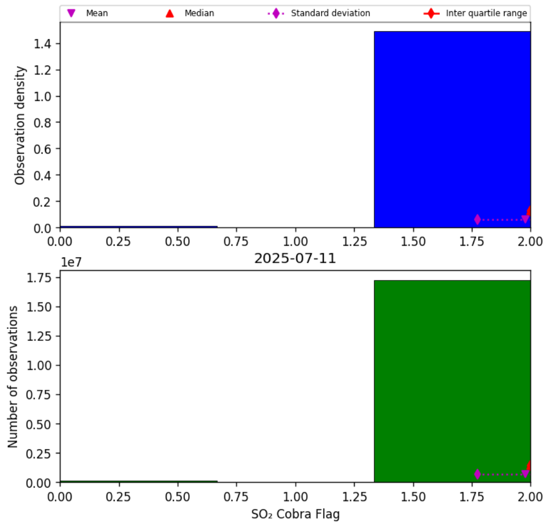
Figure 75: Histogram of “SO 2 Cobra Flag” for 2025-07-11 to 2025-07-11
