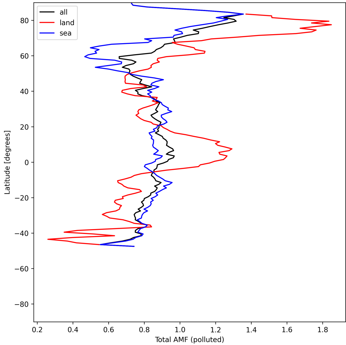
Figure 53: Zonal average of “Total AMF (polluted)” for 2025-07-11 to 2025-07-11.
