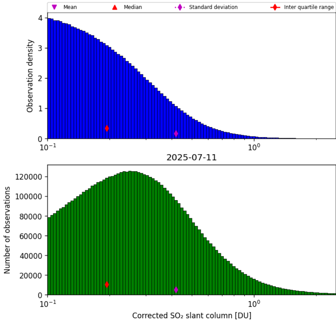
Figure 60: Histogram of “Corrected SO 2 slant column” for 2025-07-11 to 2025-07-11
