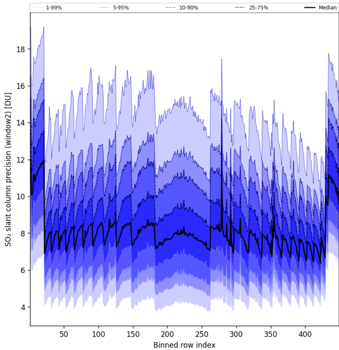
Figure 95: Along track statistics of “SO 2 slant column precision (window2)” for 2025-07-11 to 2025-07-11
