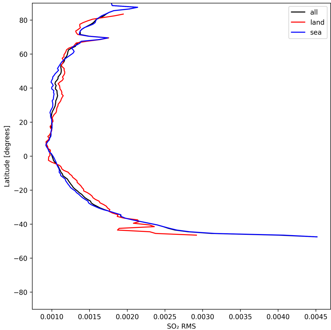
Figure 52: Zonal average of “SO 2 RMS” for 2025-07-11 to 2025-07-11.
