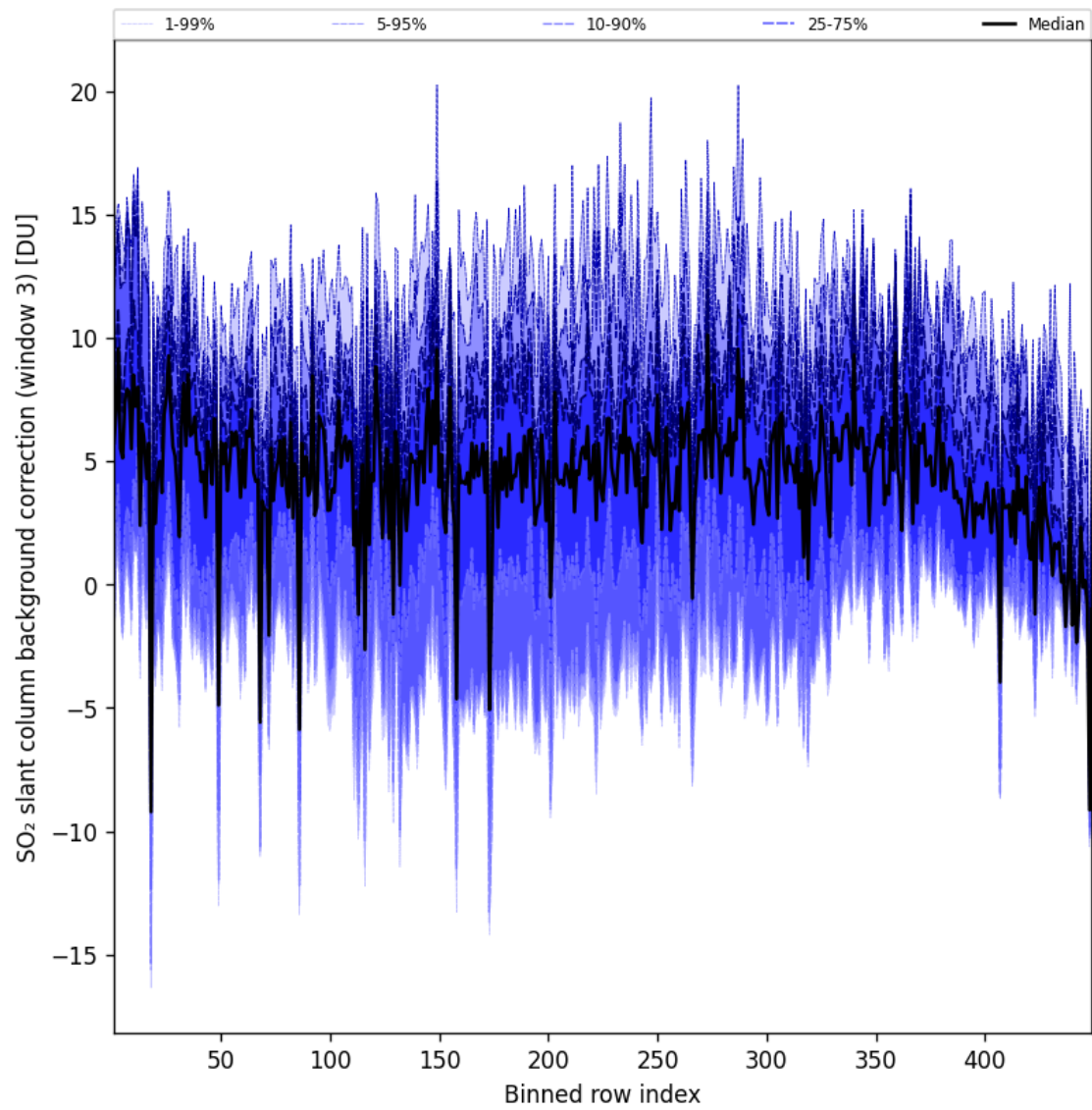
Figure 101: Along track statistics of “SO 2 slant column background correction (window 3)” for 2025-07-11 to 2025-07-11
