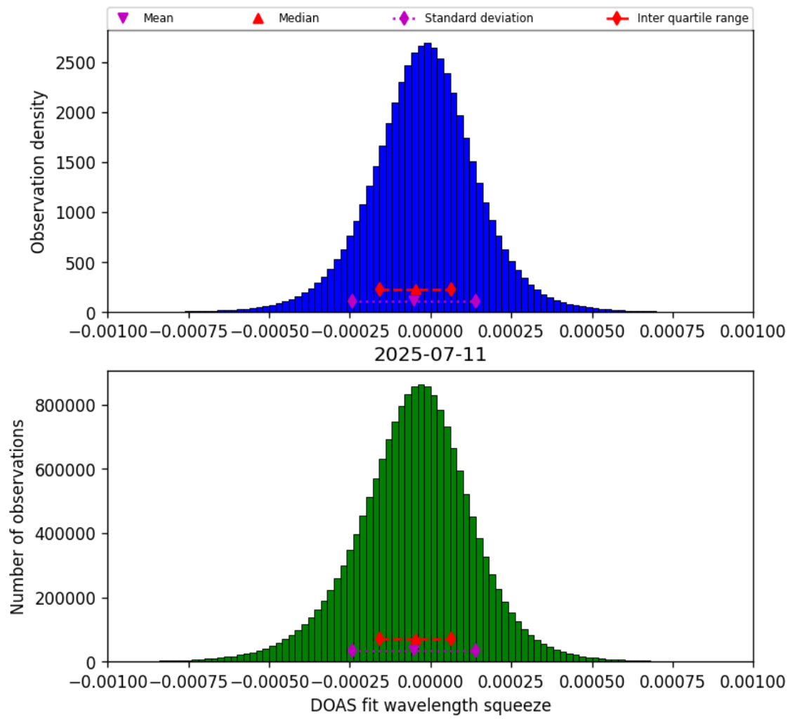
Figure 78: Histogram of “DOAS fit wavelength squeeze” for 2025-07-11 to 2025-07-11
