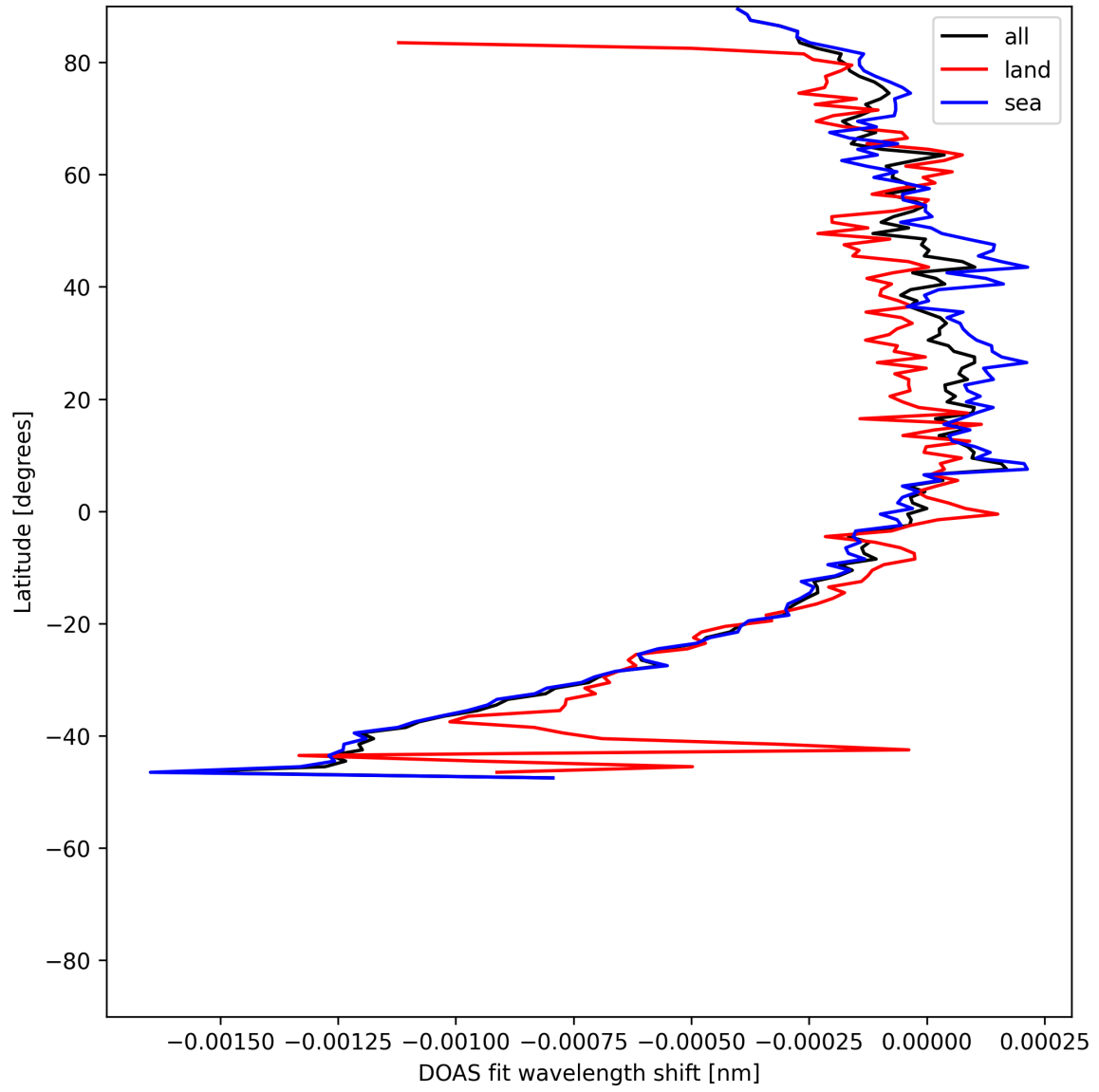
Figure 50: Zonal average of "DOAS fit wavelength shift" for 2025-07-11 to 2025-07-11.
