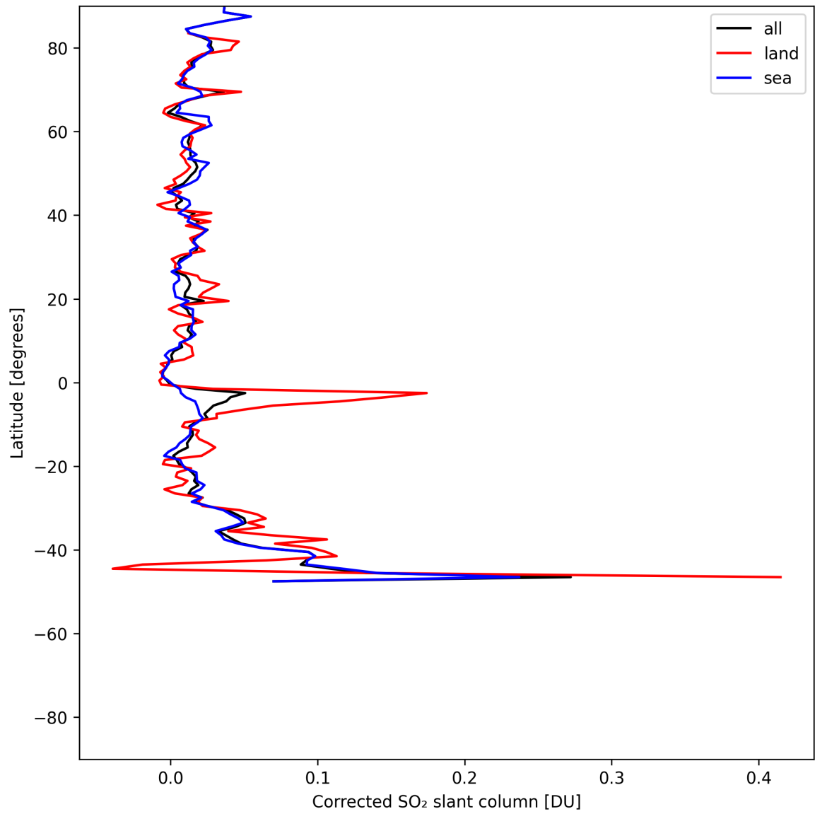
Figure 33: Zonal average of “Corrected SO 2 slant column” for 2025-07-11 to 2025-07-11.
