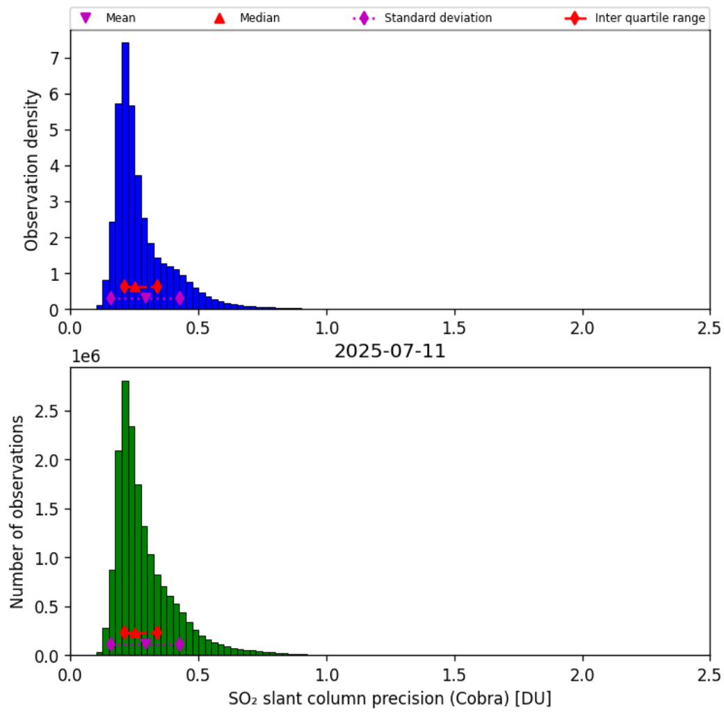
Figure 62: Histogram of “SO 2 slant column precision (Cobra)” for 2025-07-11 to 2025-07-11
