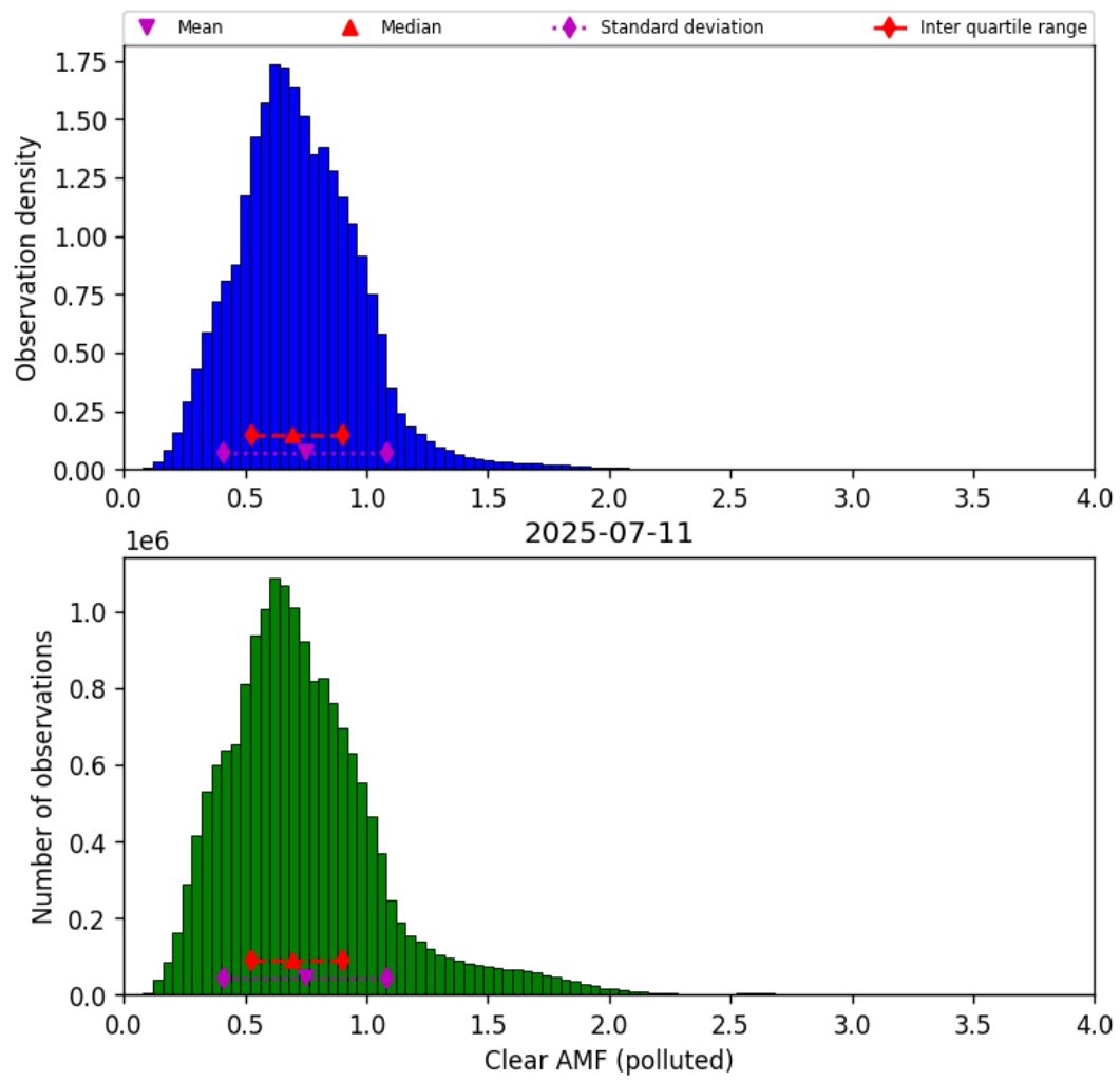
Figure 82: Histogram of “Clear AMF (polluted)” for 2025-07-11 to 2025-07-11
