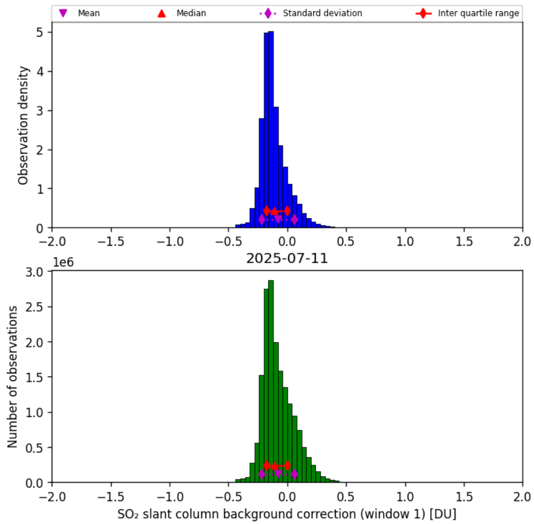
Figure 66: Histogram of “SO 2 slant column background correction (window 1)” for 2025-07-11 to 2025-07-11
