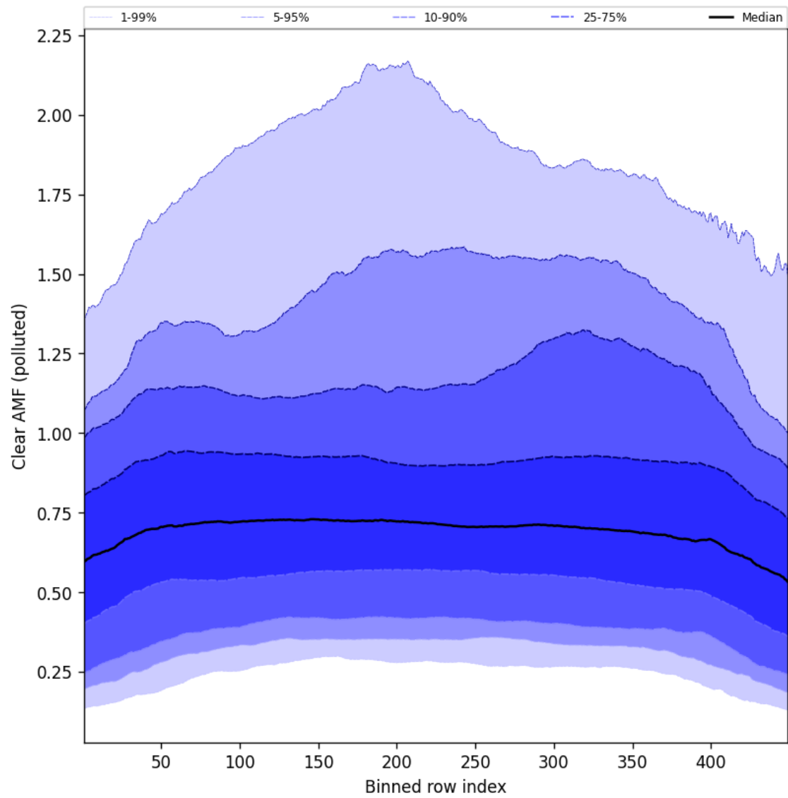
Figure 109: Along track statistics of “Clear AMF (polluted)” for 2025-07-11 to 2025-07-11
