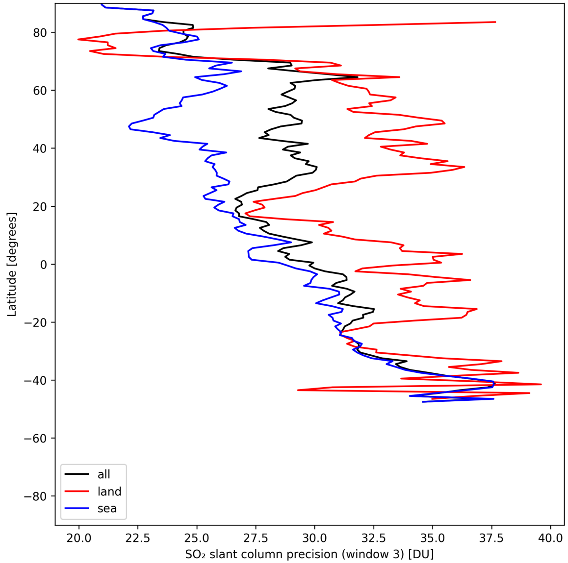
Figure 45: Zonal average of “SO 2 slant column precision (window 3)” for 2025-07-11 to 2025-07-11.
