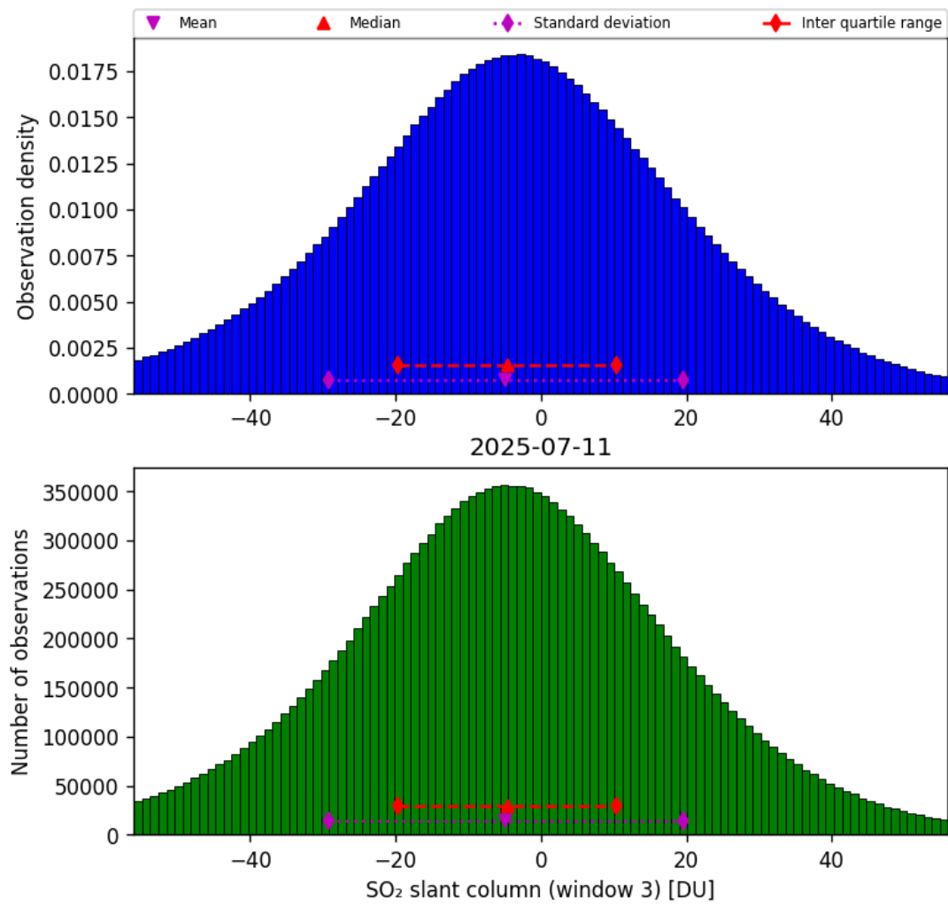
Figure 71: Histogram of “SO 2 slant column (window 3)” for 2025-07-11 to 2025-07-11
