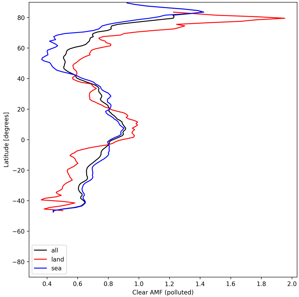
Figure 55: Zonal average of “Clear AMF (polluted)” for 2025-07-11 to 2025-07-11.
