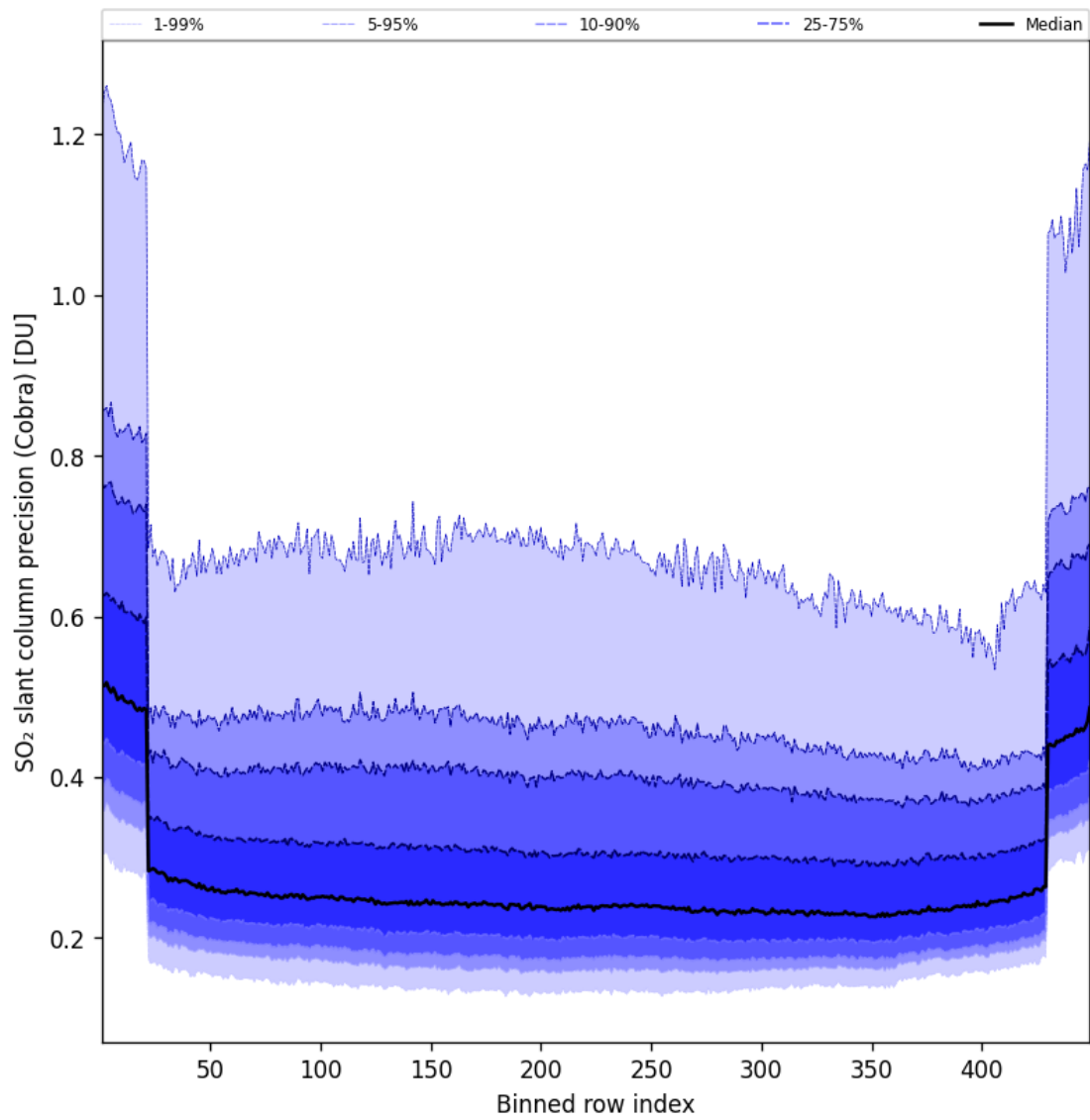
Figure 89: Along track statistics of “SO 2 slant column precision (Cobra)” for 2025-07-11 to 2025-07-11
