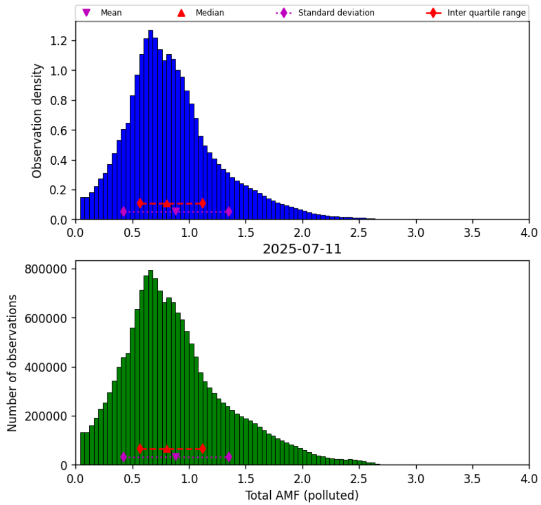
Figure 80: Histogram of “Total AMF (polluted)” for 2025-07-11 to 2025-07-11
