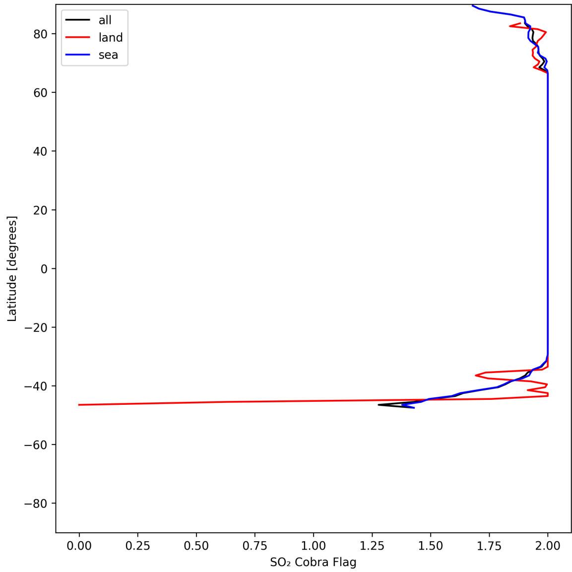
Figure 48: Zonal average of “SO 2 Cobra Flag” for 2025-07-11 to 2025-07-11.
