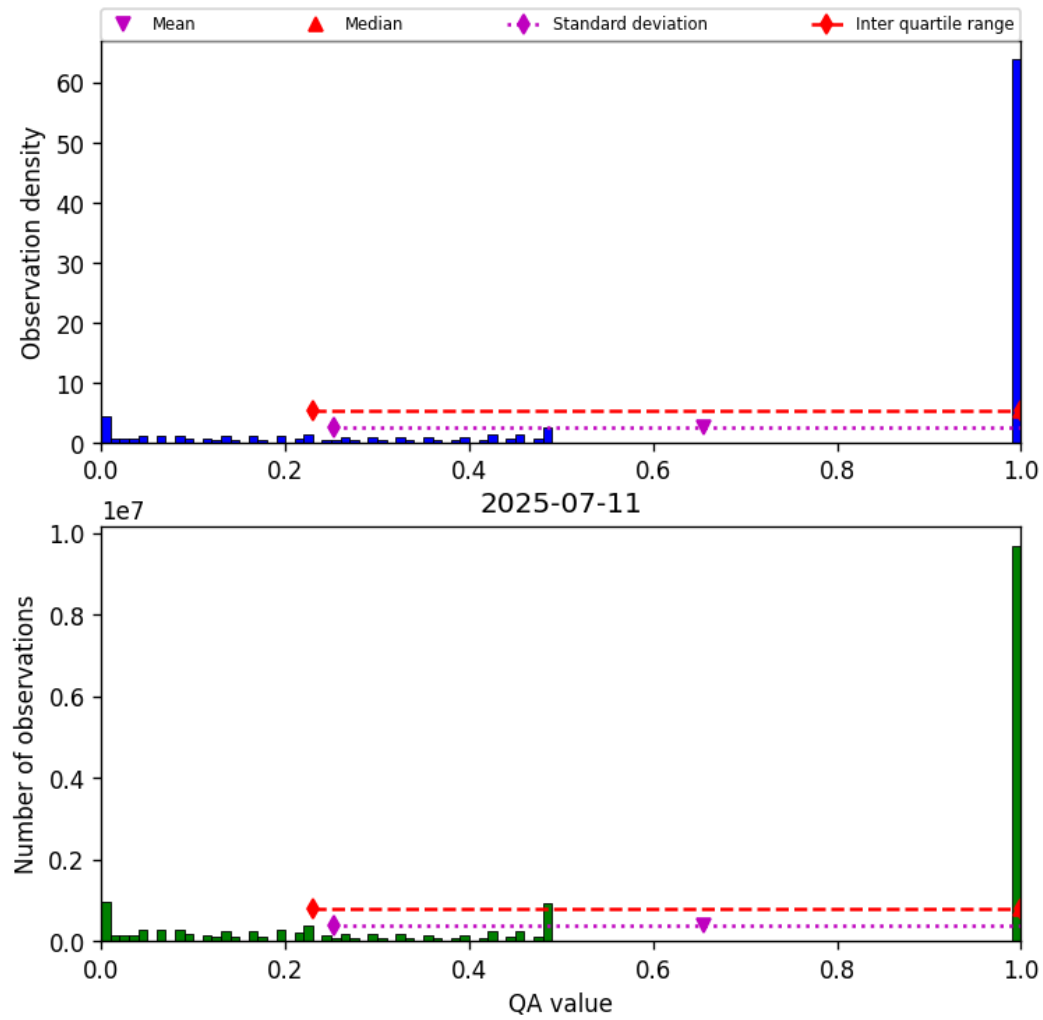
Figure 57: Histogram of “QA value” for 2025-07-11 to 2025-07-11
