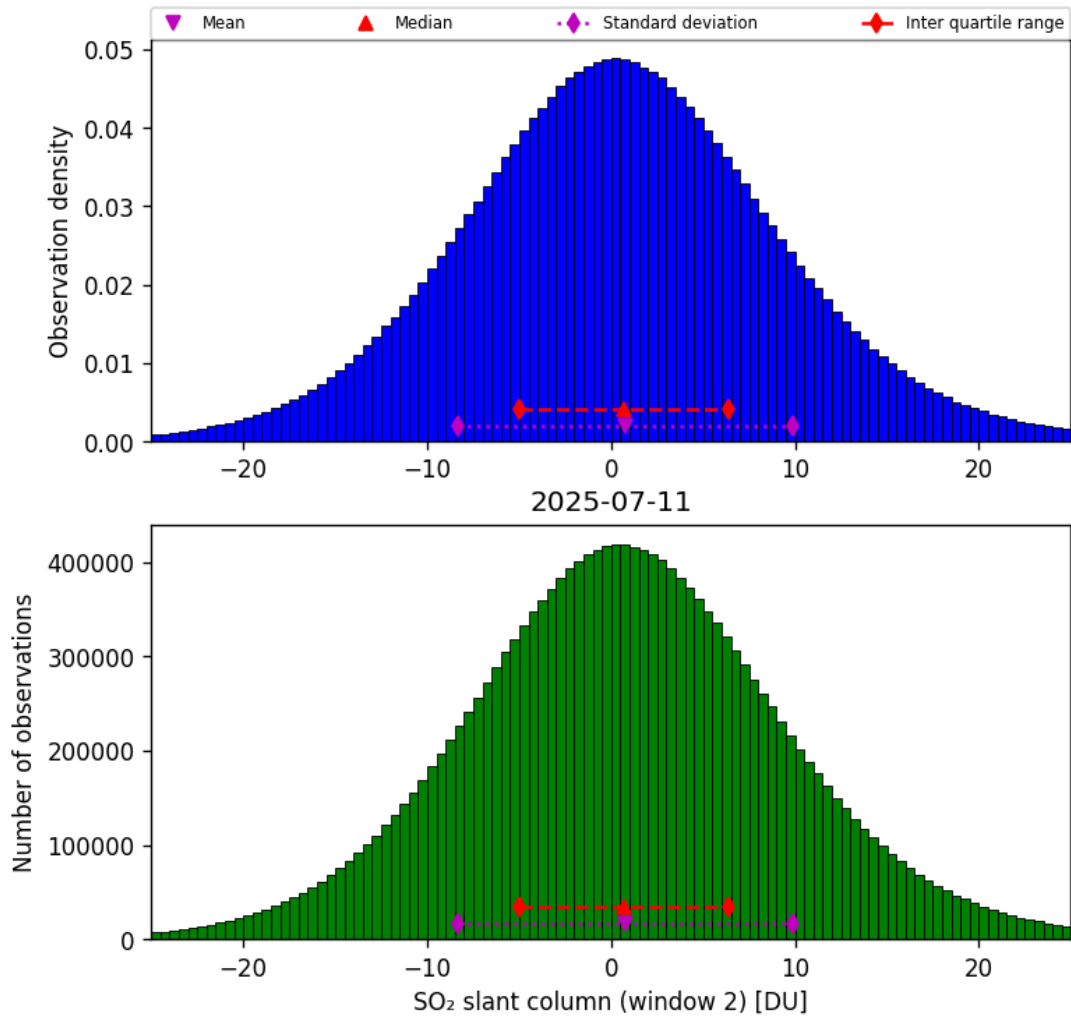
Figure 67: Histogram of “SO 2 slant column (window 2)” for 2025-07-11 to 2025-07-11
