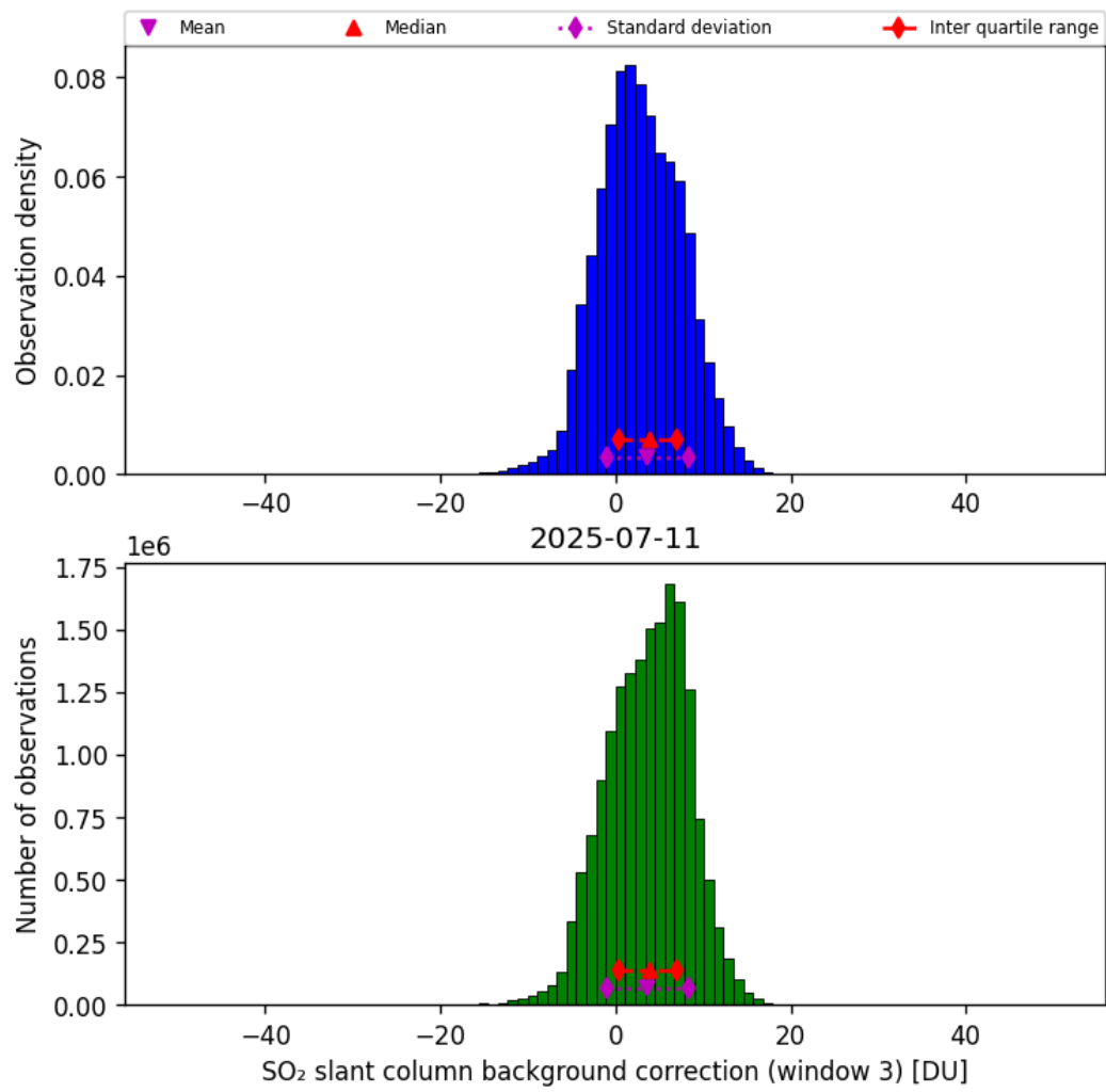
Figure 74: Histogram of “SO 2 slant column background correction (window 3)” for 2025-07-11 to 2025-07-11
