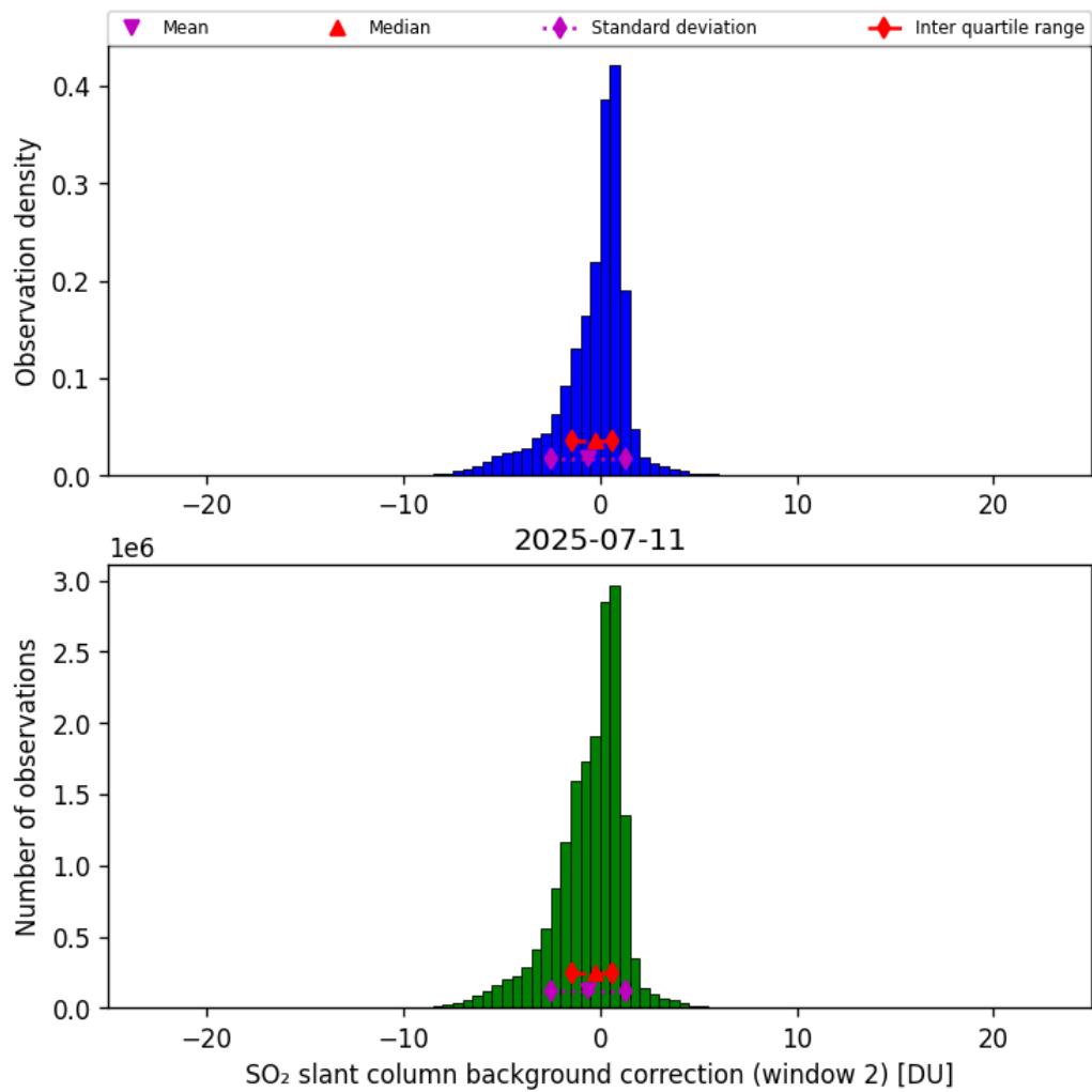
Figure 70: Histogram of “SO 2 slant column background correction (window 2)” for 2025-07-11 to 2025-07-11
