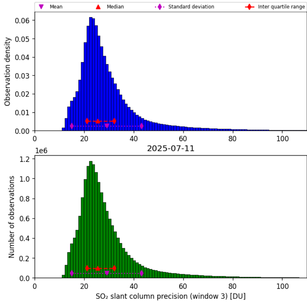
Figure 72: Histogram of “SO 2 slant column precision (window 3)” for 2025-07-11 to 2025-07-11
