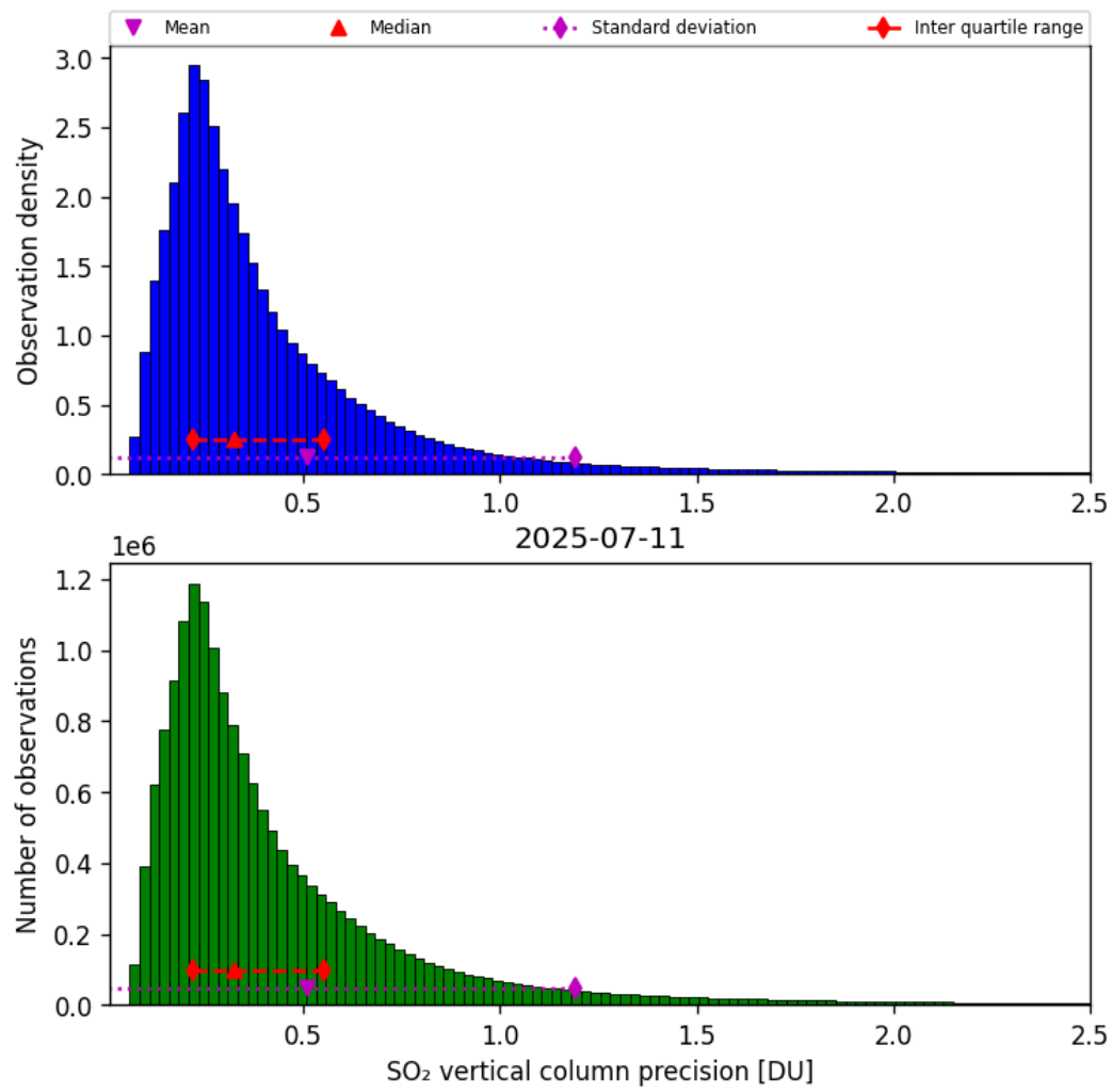
Figure 59: Histogram of “SO 2 vertical column precision” for 2025-07-11 to 2025-07-11
