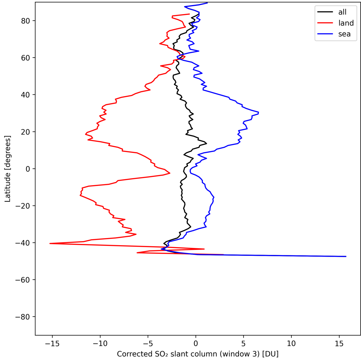
Figure 46: Zonal average of “Corrected SO 2 slant column (window 3)” for 2025-07-11 to 2025-07-11.
