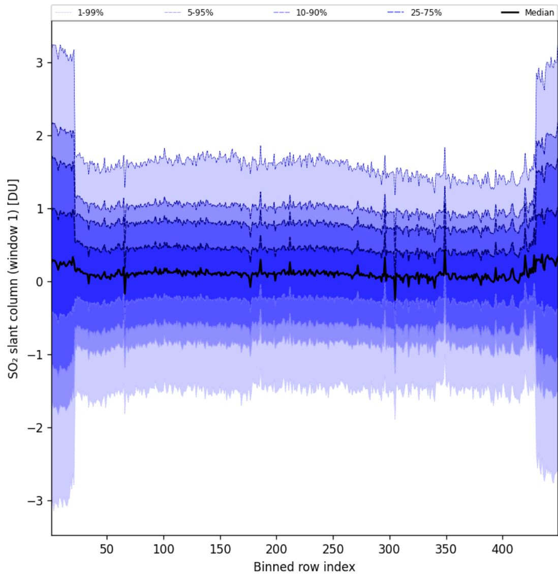
Figure 90: Along track statistics of “SO 2 slant column (window 1)” for 2025-07-11 to 2025-07-11
