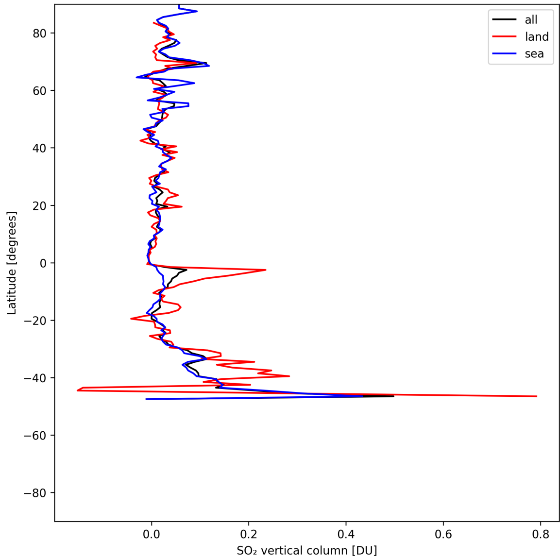
Figure 31: Zonal average of “SO 2 vertical column” for 2025-07-11 to 2025-07-11.
