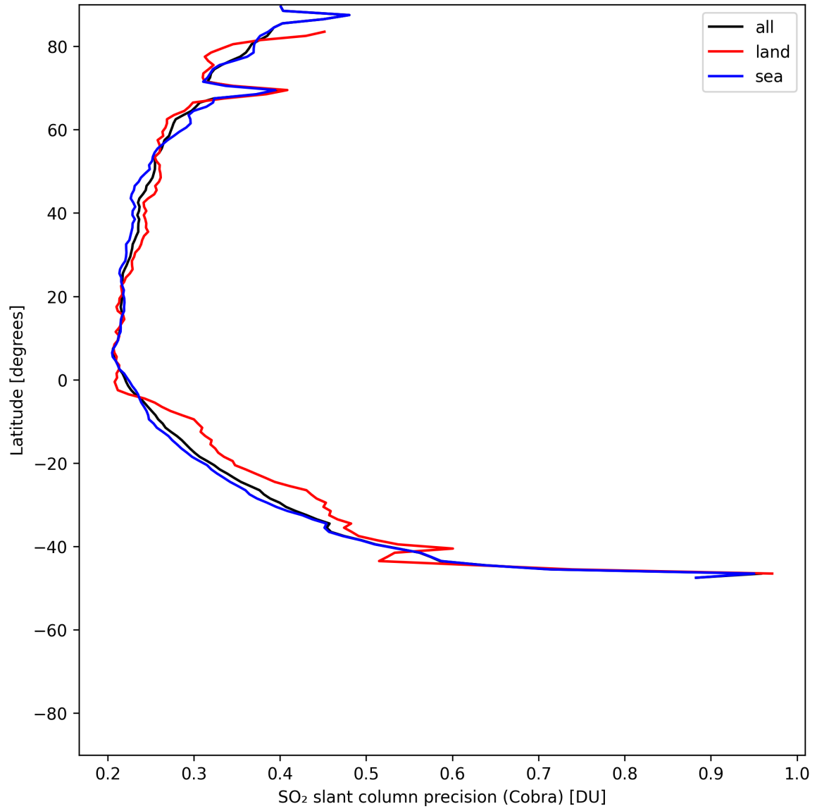
Figure 35: Zonal average of "SO 2 slant column precision (Cobra)" for 2025-07-11 to 2025-07-11.
