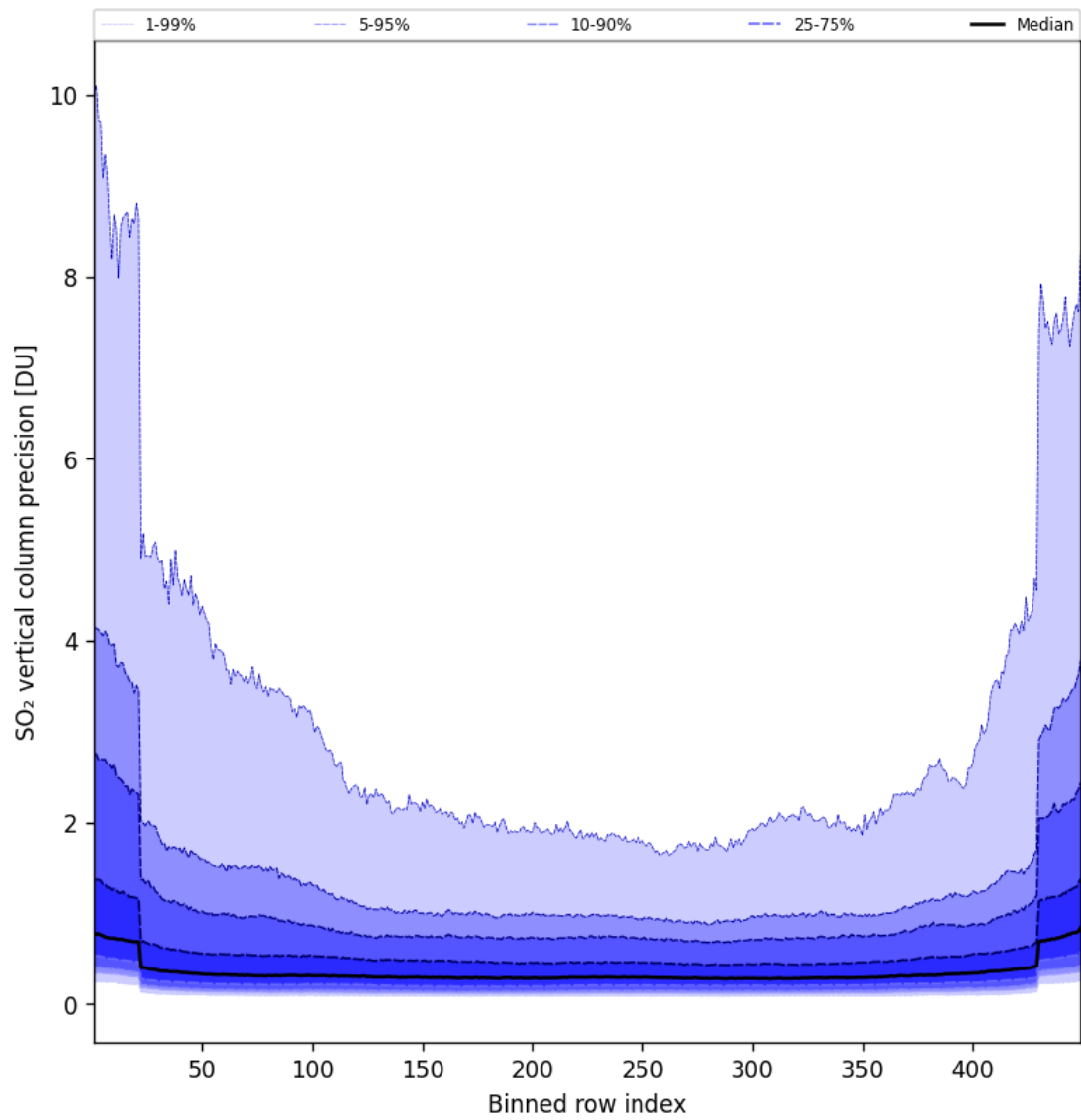
Figure 86: Along track statistics of “SO 2 vertical column precision” for 2025-07-11 to 2025-07-11
