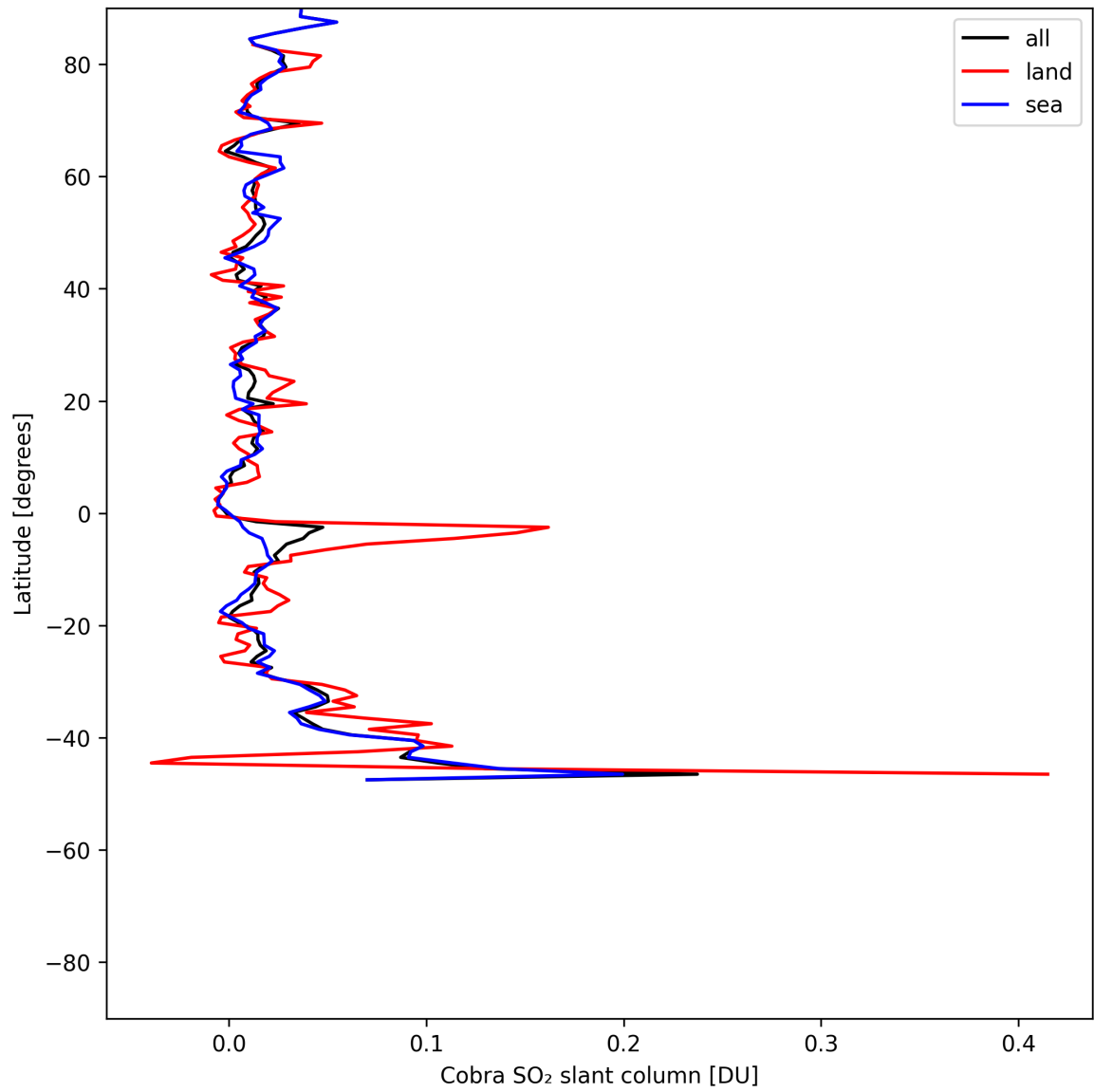
Figure 34: Zonal average of “Cobra SO 2 slant column” for 2025-07-11 to 2025-07-11.
