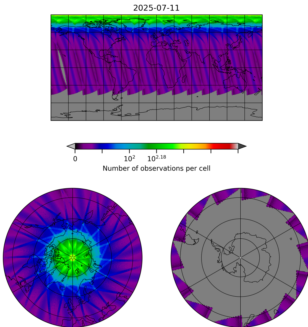
Figure 29: Map of the number of observations for 2025-07-11 to 2025-07-11
