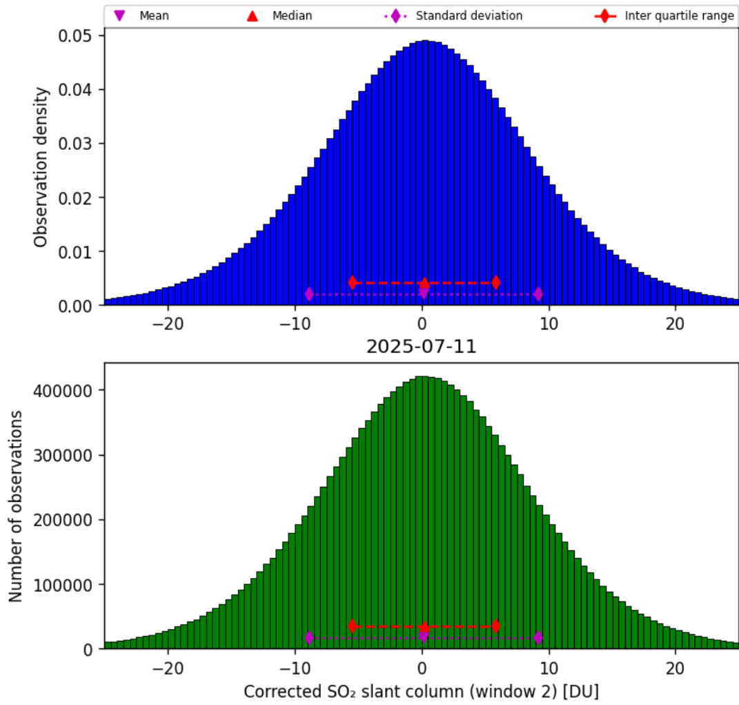
Figure 69: Histogram of “Corrected SO 2 slant column (window 2)” for 2025-07-11 to 2025-07-11
