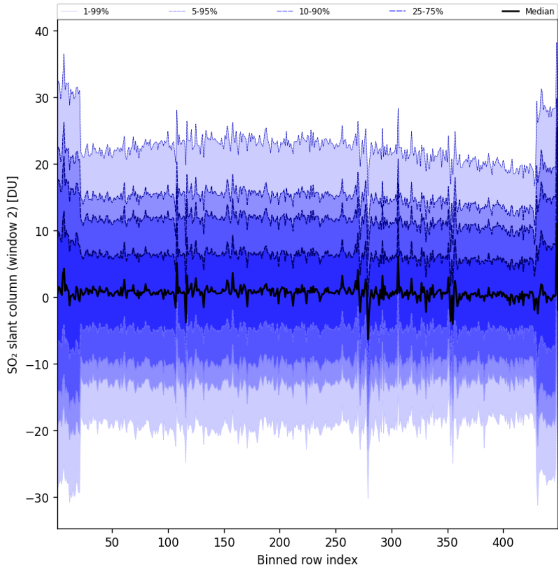
Figure 94: Along track statistics of “SO 2 slant column (window 2)” for 2025-07-11 to 2025-07-11
