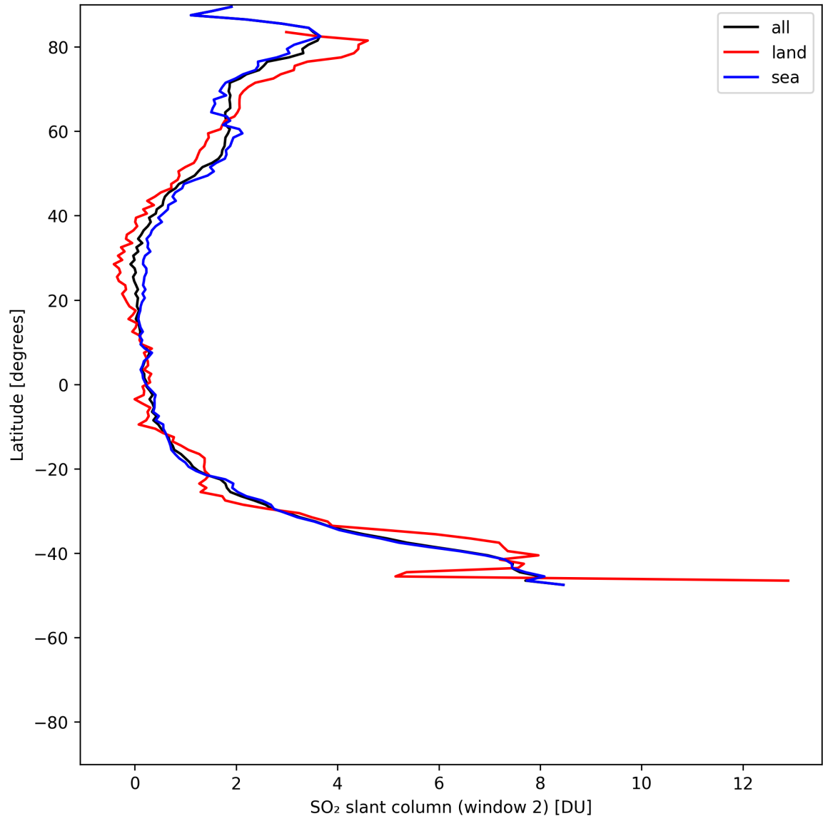
Figure 40: Zonal average of “SO 2 slant column (window 2)” for 2025-07-15 to 2025-07-16.
