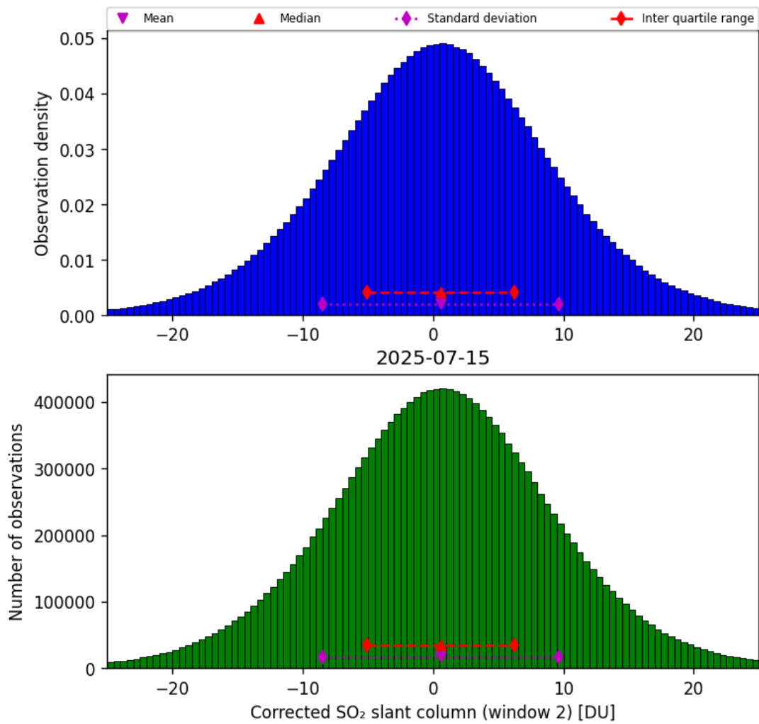
Figure 69: Histogram of “Corrected SO 2 slant column (window 2)” for 2025-07-15 to 2025-07-16
