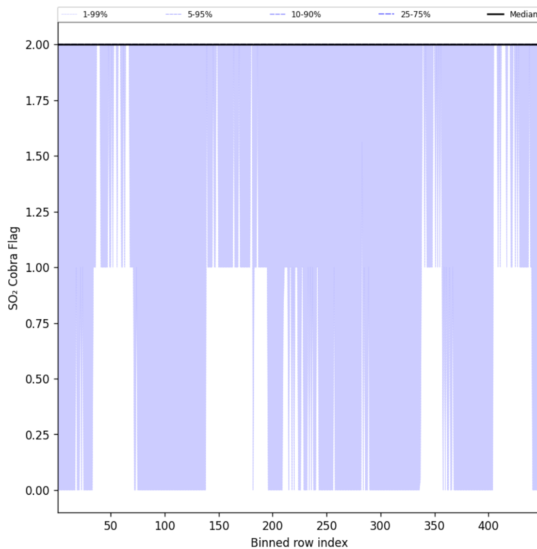
Figure 102: Along track statistics of “SO 2 Cobra Flag” for 2025-07-15 to 2025-07-16
