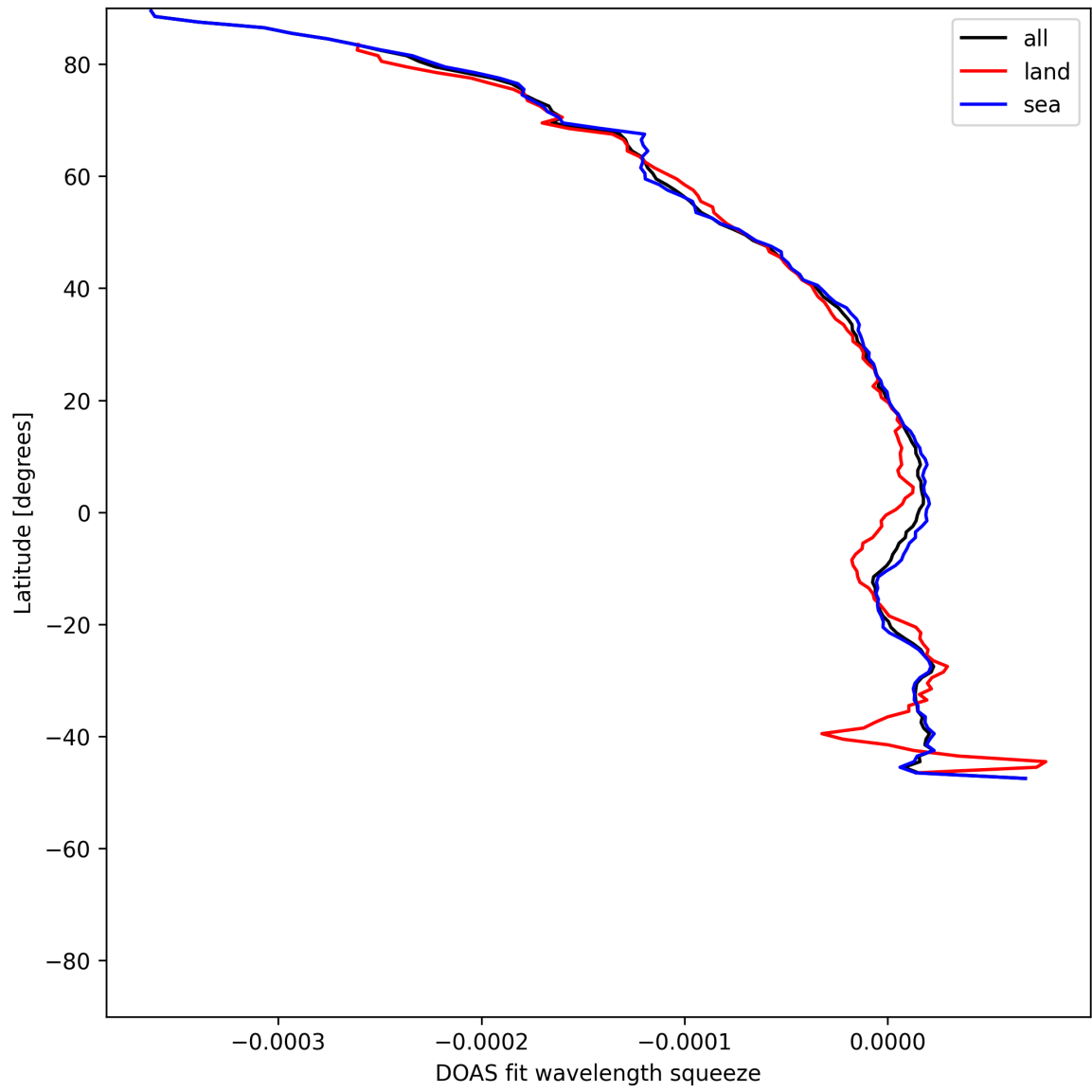
Figure 51: Zonal average of “DOAS fit wavelength squeeze” for 2025-07-15 to 2025-07-16.
