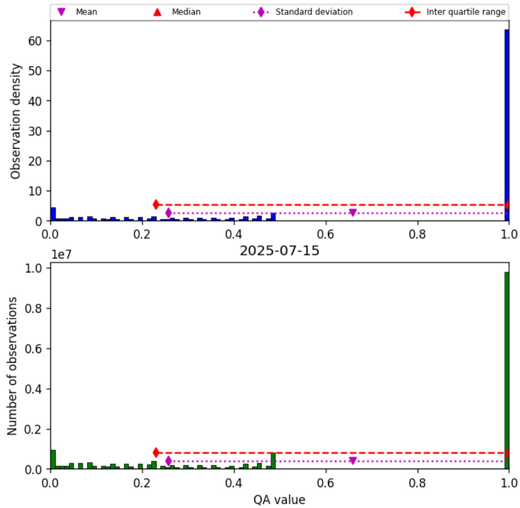
Figure 57: Histogram of “QA value” for 2025-07-15 to 2025-07-16
