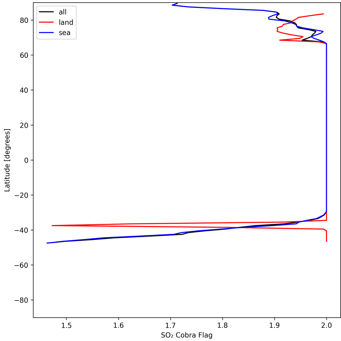
Figure 48: Zonal average of "SO 2 Cobra Flag" for 2025-07-15 to 2025-07-16.
