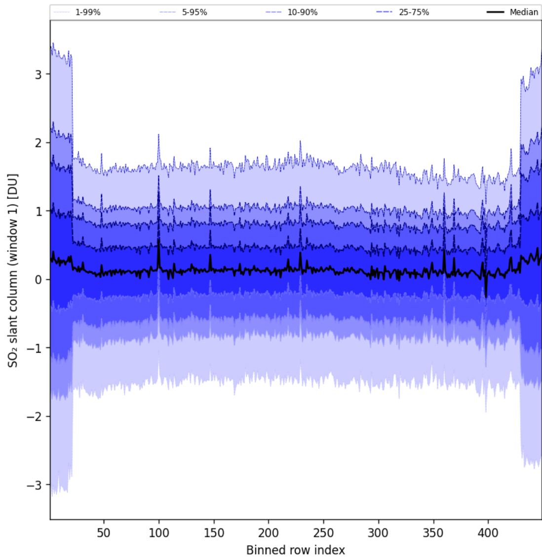
Figure 90: Along track statistics of “SO 2 slant column (window 1)” for 2025-07-15 to 2025-07-16
