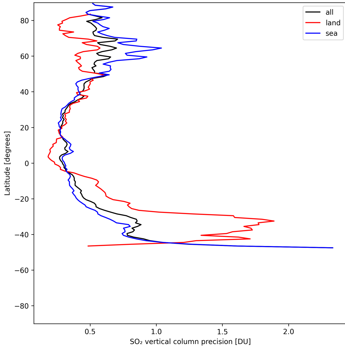
Figure 32: Zonal average of “SO 2 vertical column precision” for 2025-07-15 to 2025-07-16.
