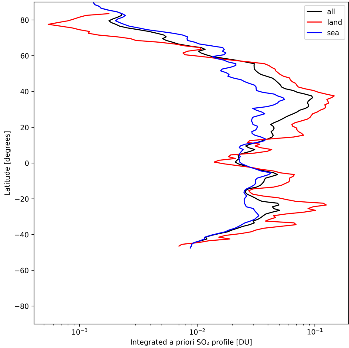
Figure 49: Zonal average of “Integrated a priori SO 2 profile” for 2025-07-15 to 2025-07-16.
