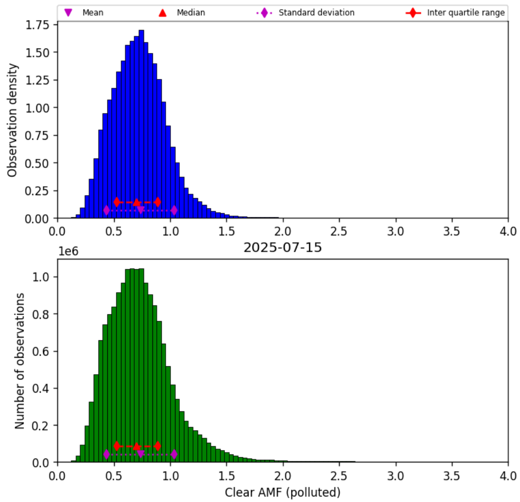
Figure 82: Histogram of “Clear AMF (polluted)” for 2025-07-15 to 2025-07-16
