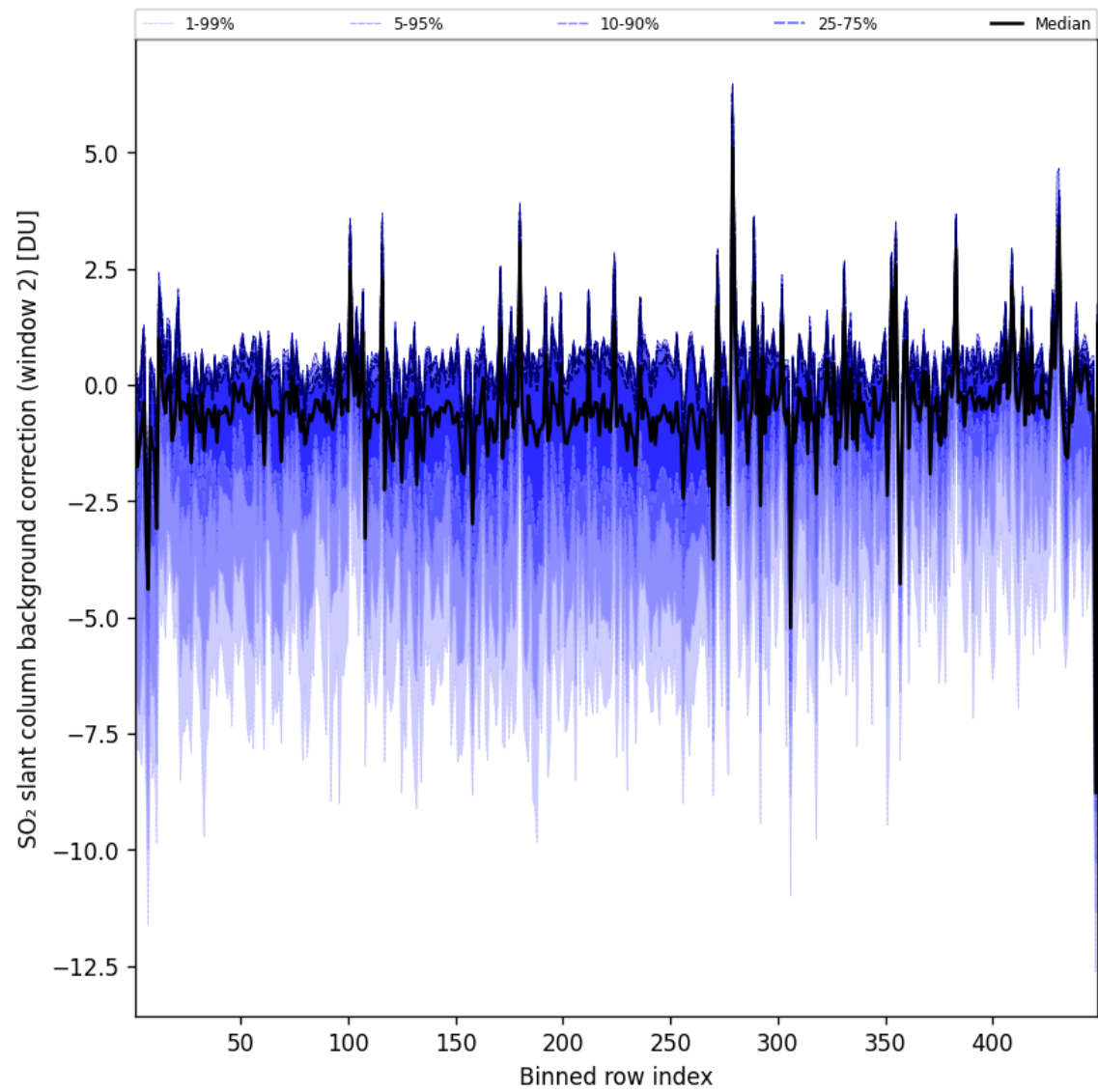
Figure 97: Along track statistics of “SO 2 slant column background correction (window 2)” for 2025-07-15 to 2025-07-16
