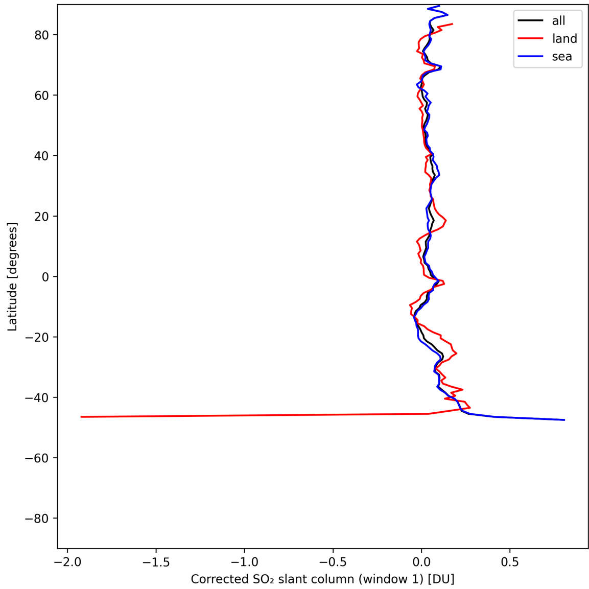
Figure 38: Zonal average of “Corrected SO 2 slant column (window 1)” for 2025-07-15 to 2025-07-16.
