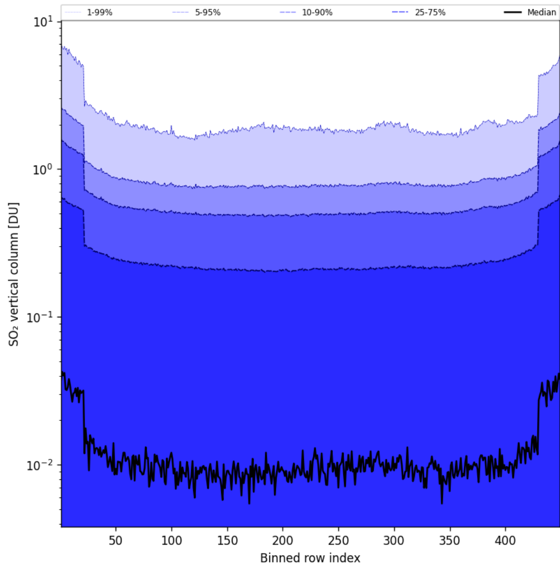
Figure 85: Along track statistics of “SO 2 vertical column” for 2025-07-15 to 2025-07-16
