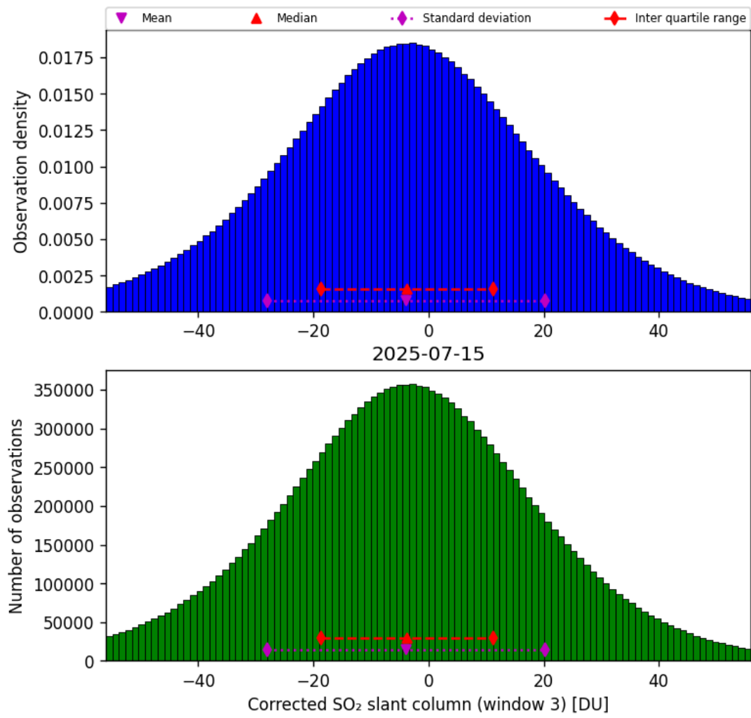
Figure 73: Histogram of “Corrected SO 2 slant column (window 3)” for 2025-07-15 to 2025-07-16
