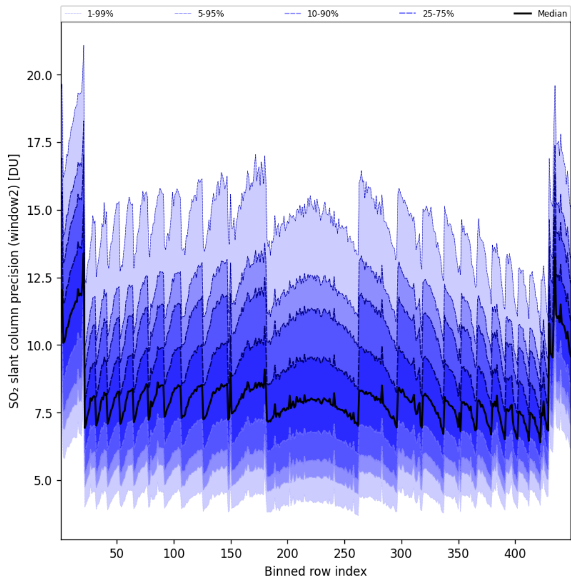
Figure 95: Along track statistics of “SO 2 slant column precision (window2)” for 2025-07-15 to 2025-07-16
