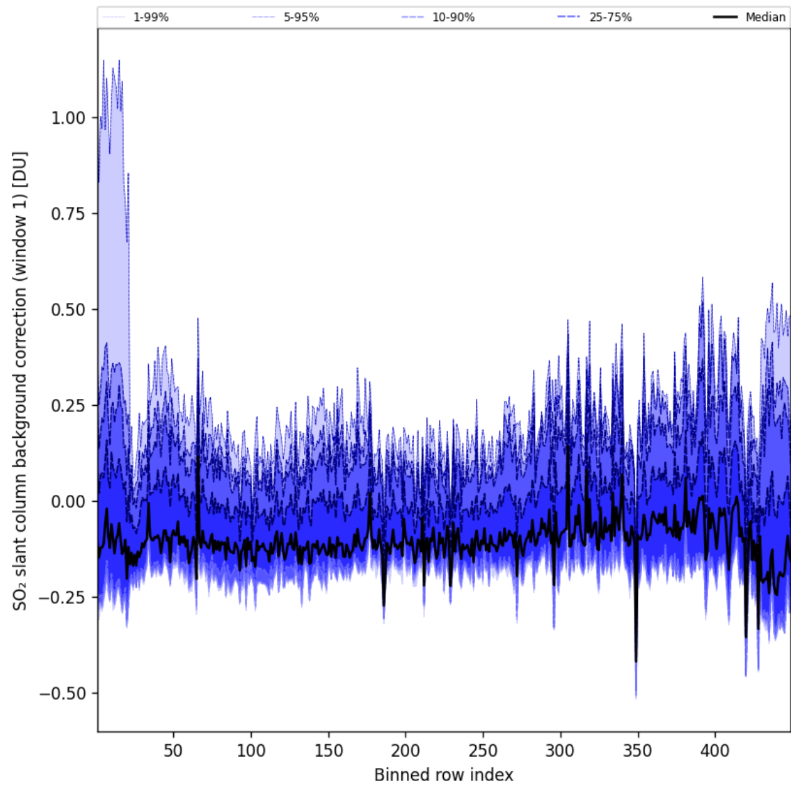
Figure 93: Along track statistics of “SO 2 slant column background correction (window 1)” for 2025-07-15 to 2025-07-16
