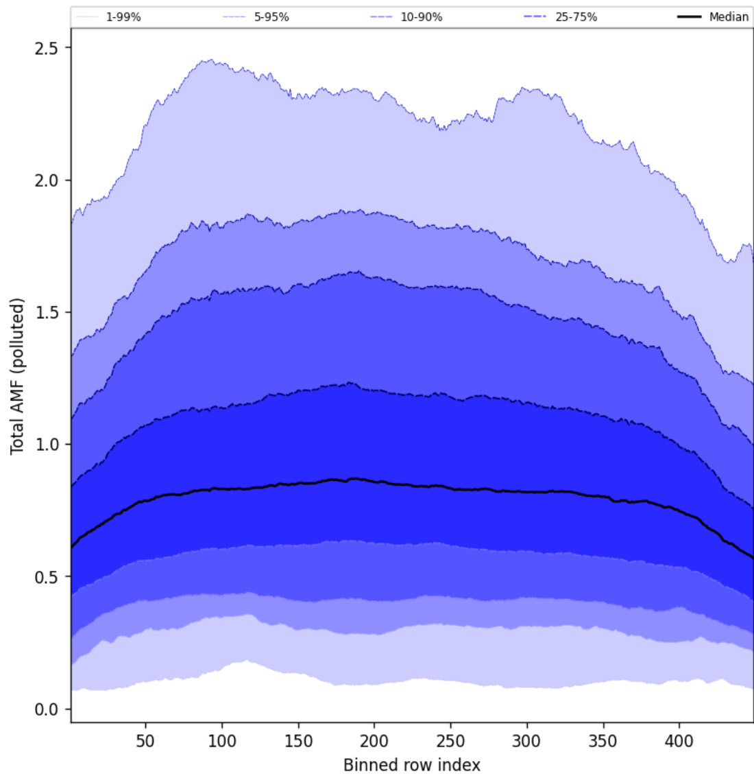
Figure 107: Along track statistics of “Total AMF (polluted)” for 2025-07-15 to 2025-07-16
