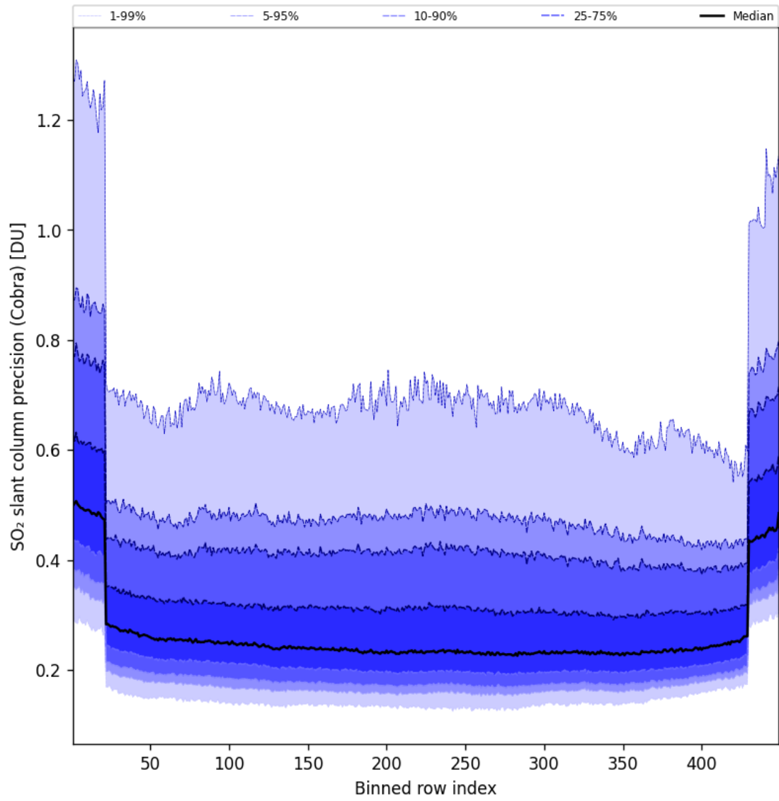
Figure 89: Along track statistics of “SO 2 slant column precision (Cobra)” for 2025-07-15 to 2025-07-16
