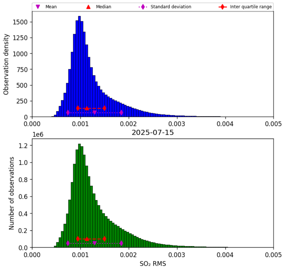
Figure 79: Histogram of “SO 2 RMS” for 2025-07-15 to 2025-07-16
