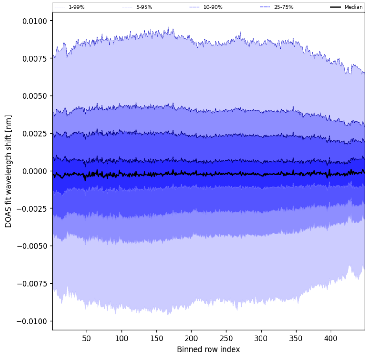
Figure 104: Along track statistics of “DOAS fit wavelength shift” for 2025-07-15 to 2025-07-16
