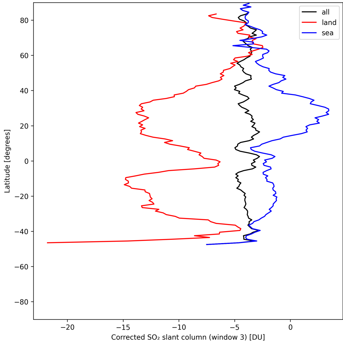
Figure 46: Zonal average of “Corrected SO 2 slant column (window 3)” for 2025-07-15 to 2025-07-16.
