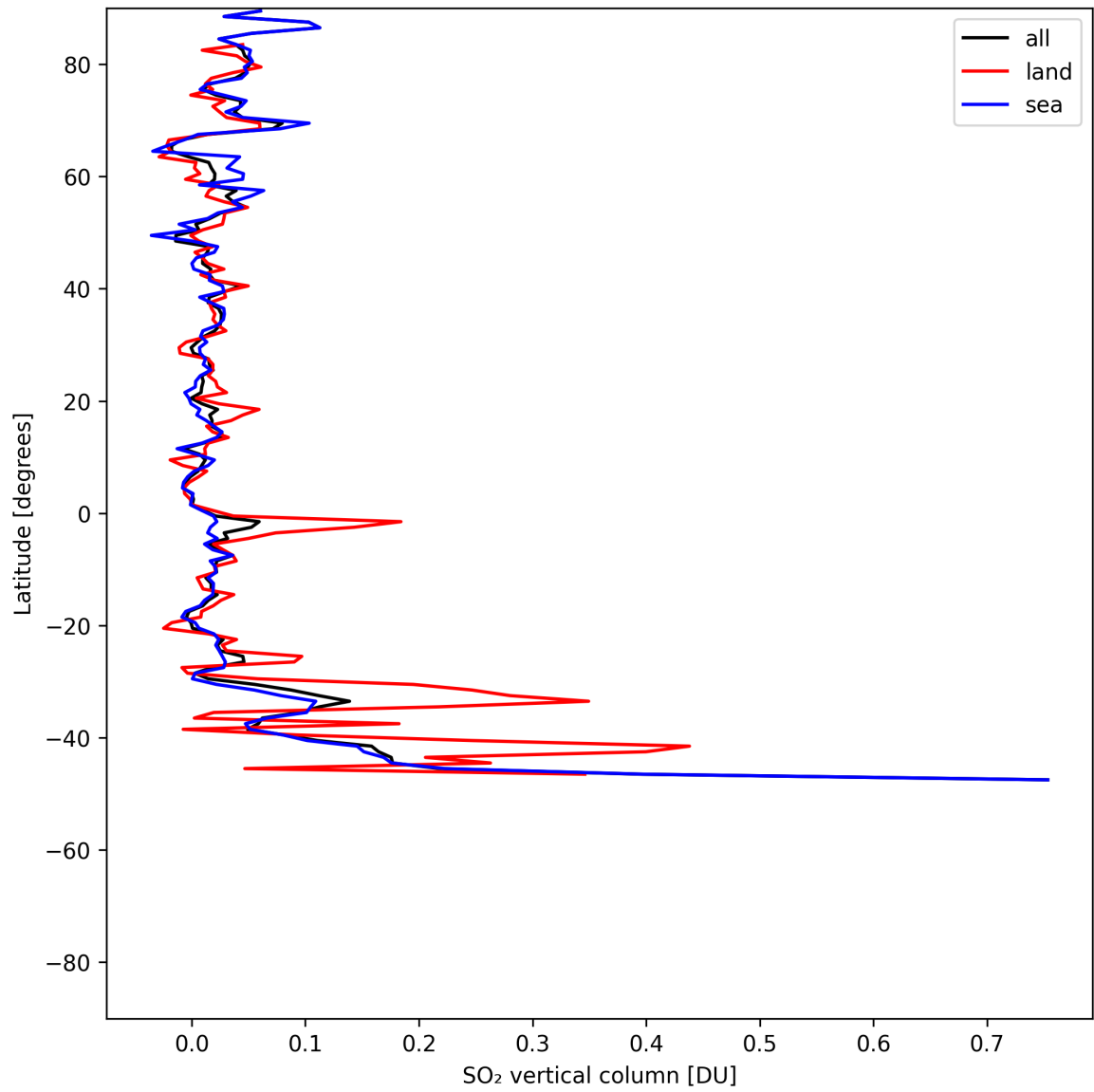
Figure 31: Zonal average of “SO 2 vertical column” for 2025-07-15 to 2025-07-16.
