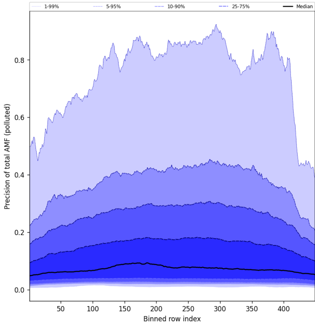
Figure 108: Along track statistics of “Precision of total AMF (polluted)” for 2025-07-15 to 2025-07-16
