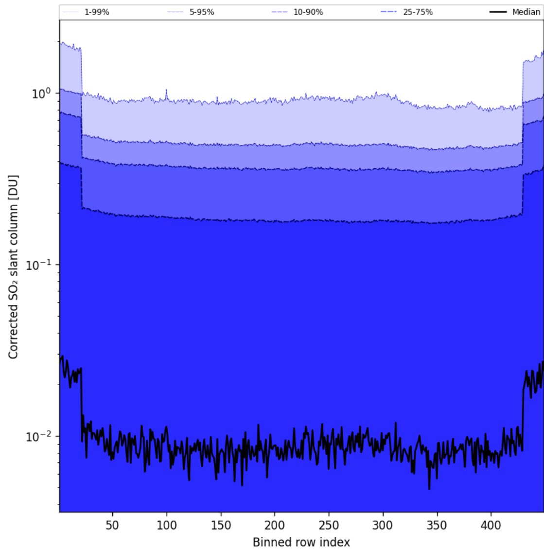
Figure 87: Along track statistics of “Corrected SO 2 slant column” for 2025-07-15 to 2025-07-16
