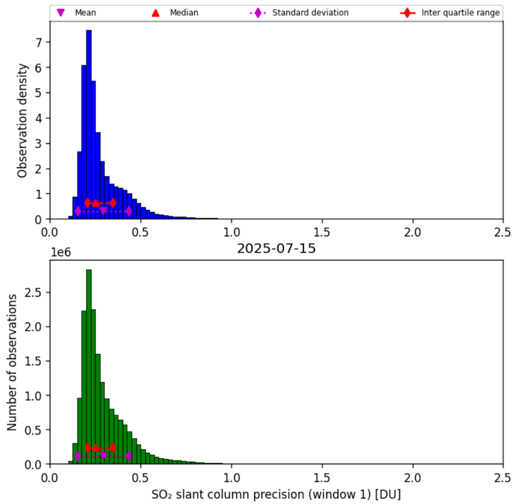
Figure 64: Histogram of “SO 2 slant column precision (window 1)” for 2025-07-15 to 2025-07-16
