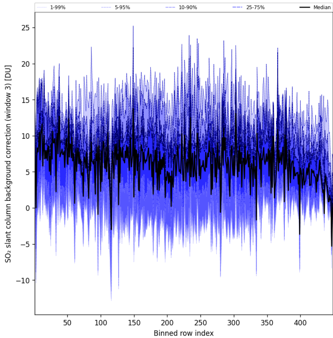
Figure 101: Along track statistics of “SO 2 slant column background correction (window 3)” for 2025-07-15 to 2025-07-16
