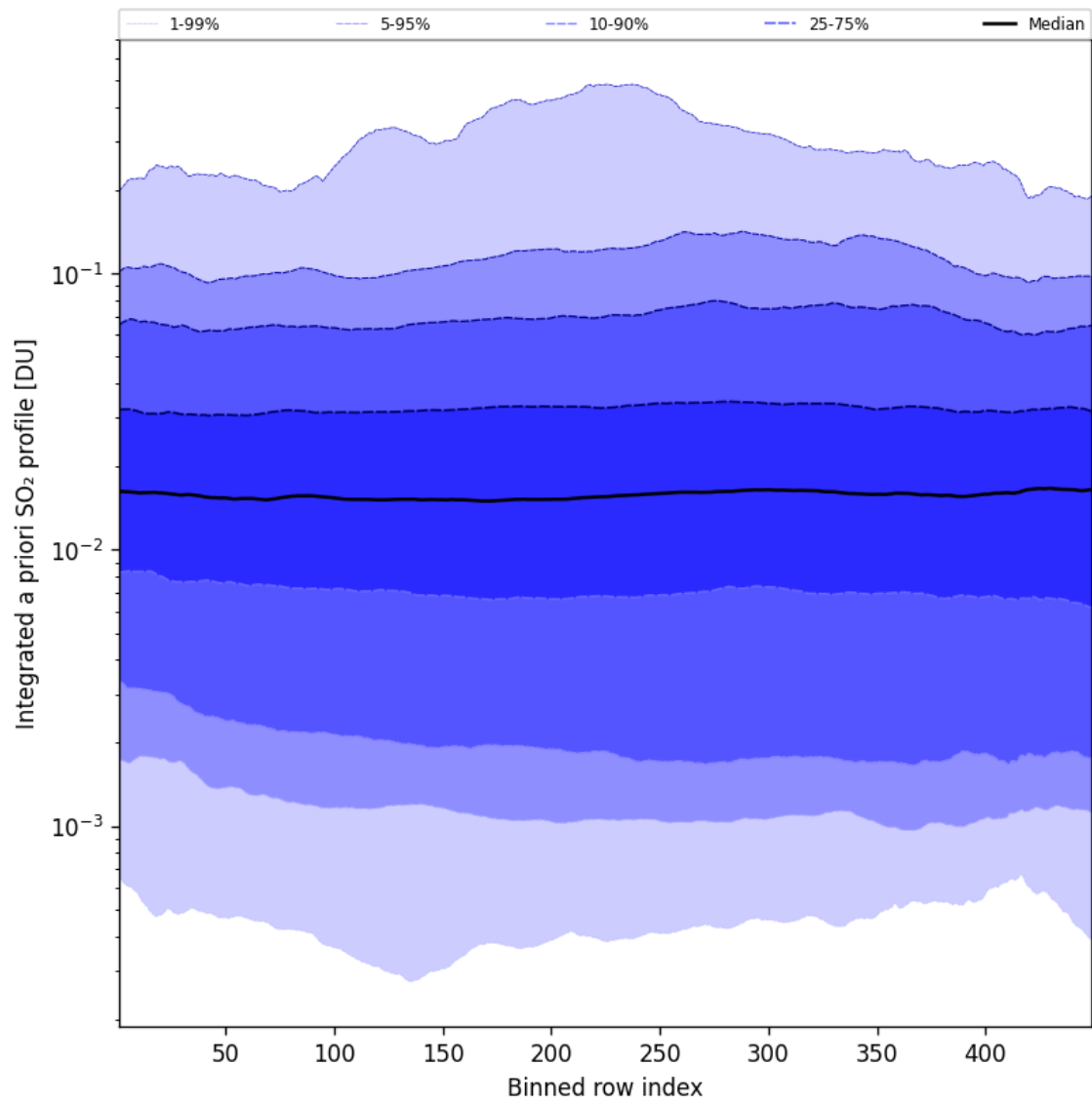
Figure 103: Along track statistics of “Integrated a priori SO 2 profile” for 2025-07-15 to 2025-07-16
