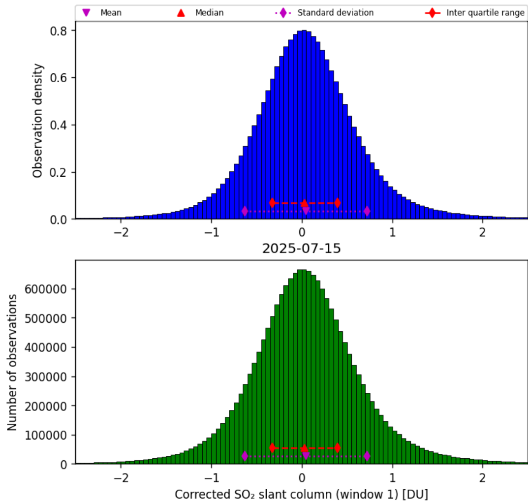
Figure 65: Histogram of “Corrected SO 2 slant column (window 1)” for 2025-07-15 to 2025-07-16
