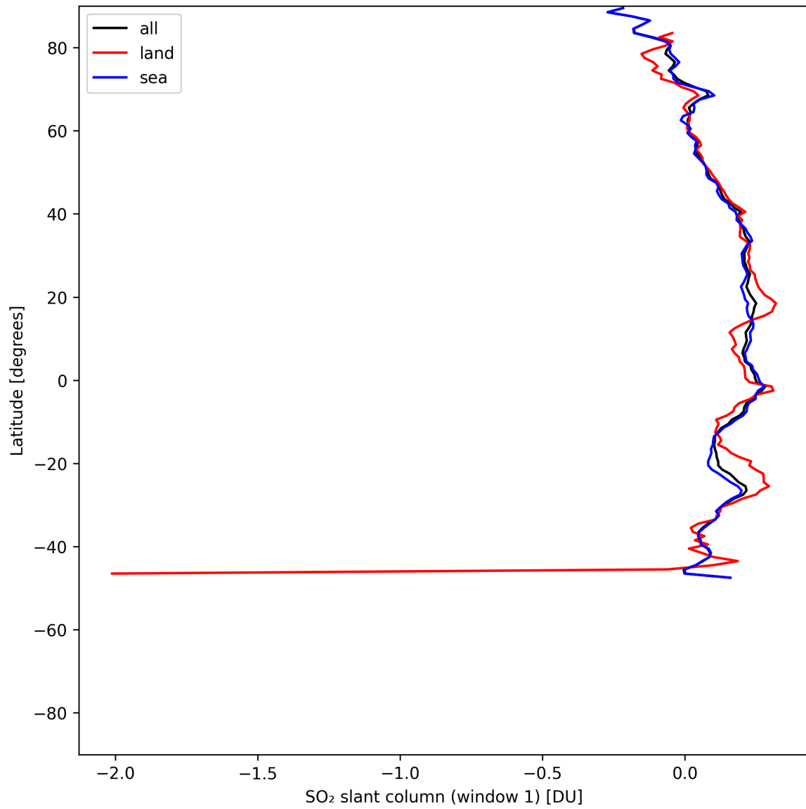
Figure 36: Zonal average of “SO 2 slant column (window 1)” for 2025-07-15 to 2025-07-16.
