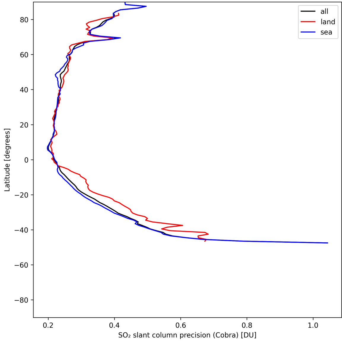
Figure 35: Zonal average of “SO 2 slant column precision (Cobra)” for 2025-07-15 to 2025-07-16.
