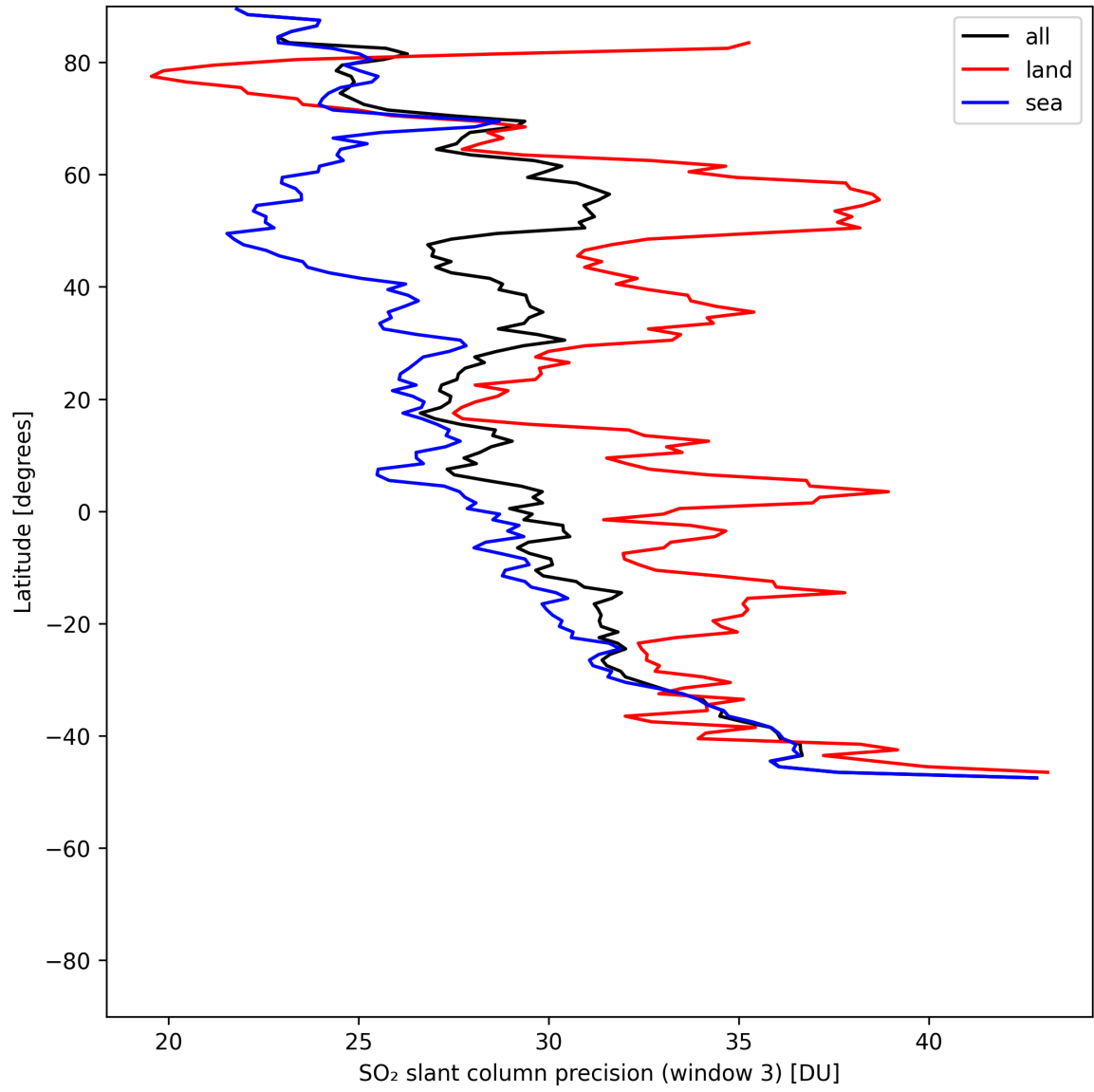
Figure 45: Zonal average of “SO 2 slant column precision (window 3)” for 2025-07-15 to 2025-07-16.
