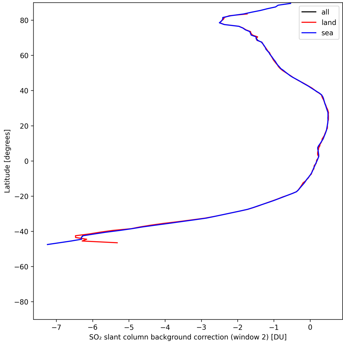
Figure 43: Zonal average of “SO 2 slant column background correction (window 2)” for 2025-07-15 to 2025-07-16.
