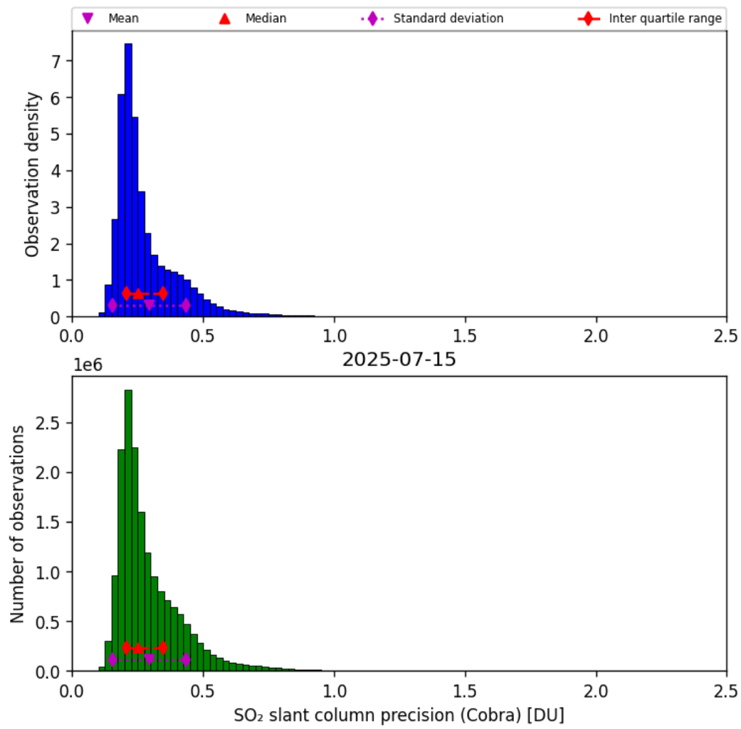
Figure 62: Histogram of “SO 2 slant column precision (Cobra)” for 2025-07-15 to 2025-07-16
