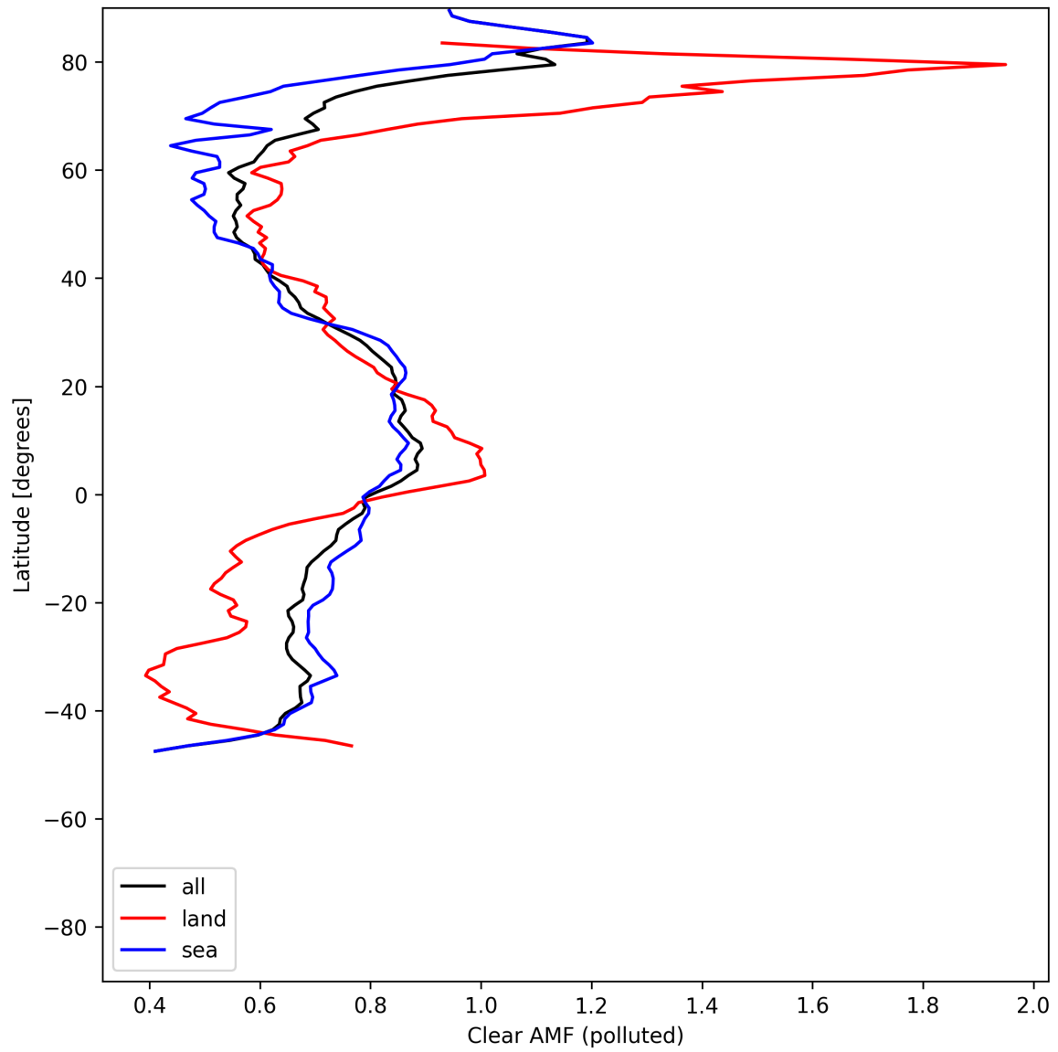
Figure 55: Zonal average of “Clear AMF (polluted)” for 2025-07-15 to 2025-07-16.
