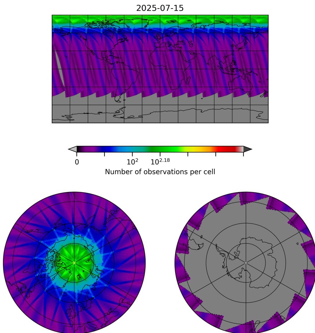
Figure 29: Map of the number of observations for 2025-07-15 to 2025-07-16
