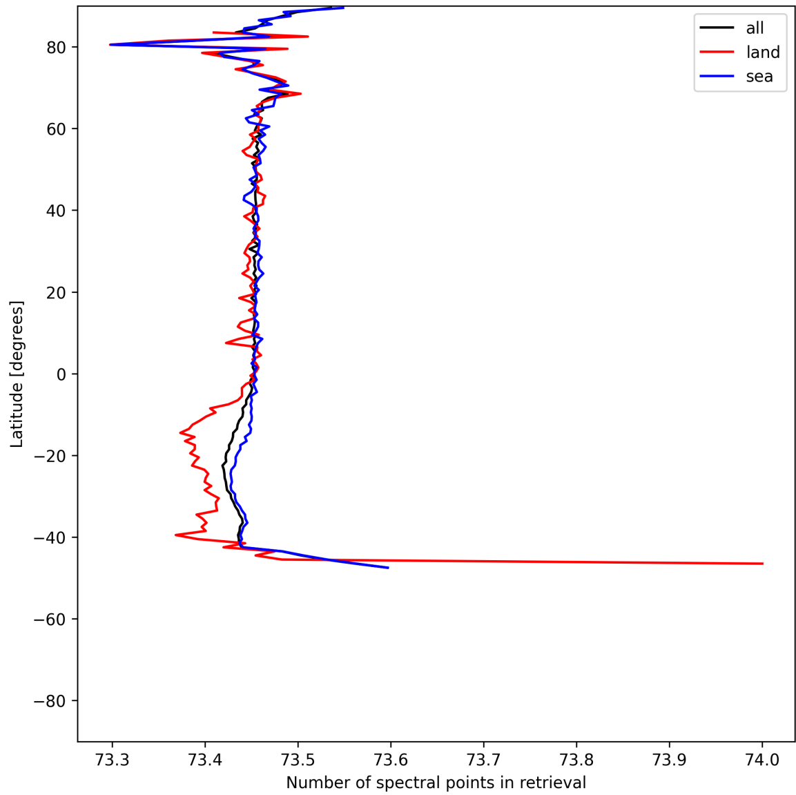
Figure 56: Zonal average of “Number of spectral points in retrieval” for 2025-07-15 to 2025-07-16.
