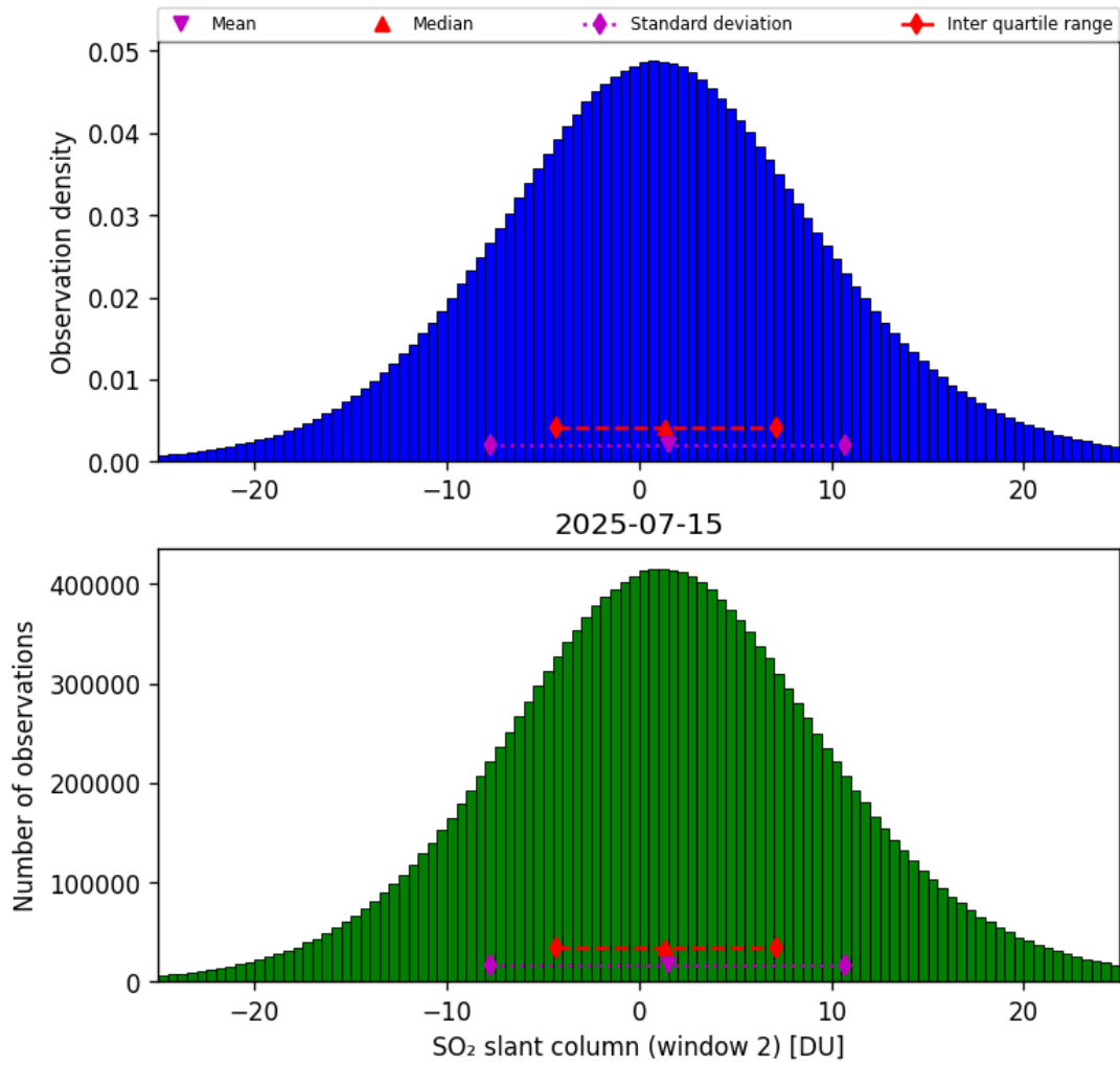
Figure 67: Histogram of “SO 2 slant column (window 2)” for 2025-07-15 to 2025-07-16
