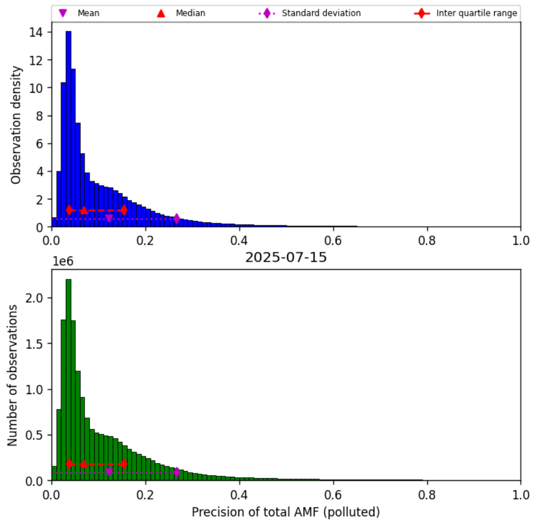
Figure 81: Histogram of “Precision of total AMF (polluted)” for 2025-07-15 to 2025-07-16
