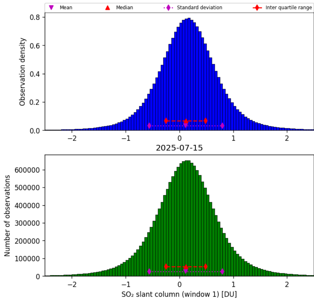
Figure 63: Histogram of “SO 2 slant column (window 1)” for 2025-07-15 to 2025-07-16
