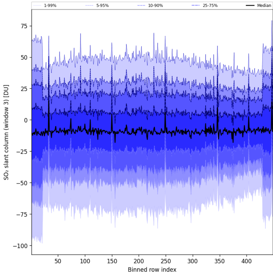
Figure 98: Along track statistics of “SO 2 slant column (window 3)” for 2025-07-15 to 2025-07-16
