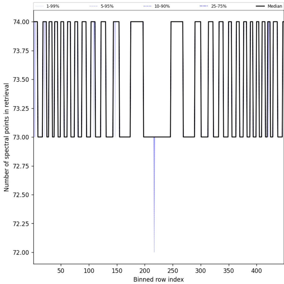
Figure 110: Along track statistics of “Number of spectral points in retrieval” for 2025-07-15 to 2025-07-16
