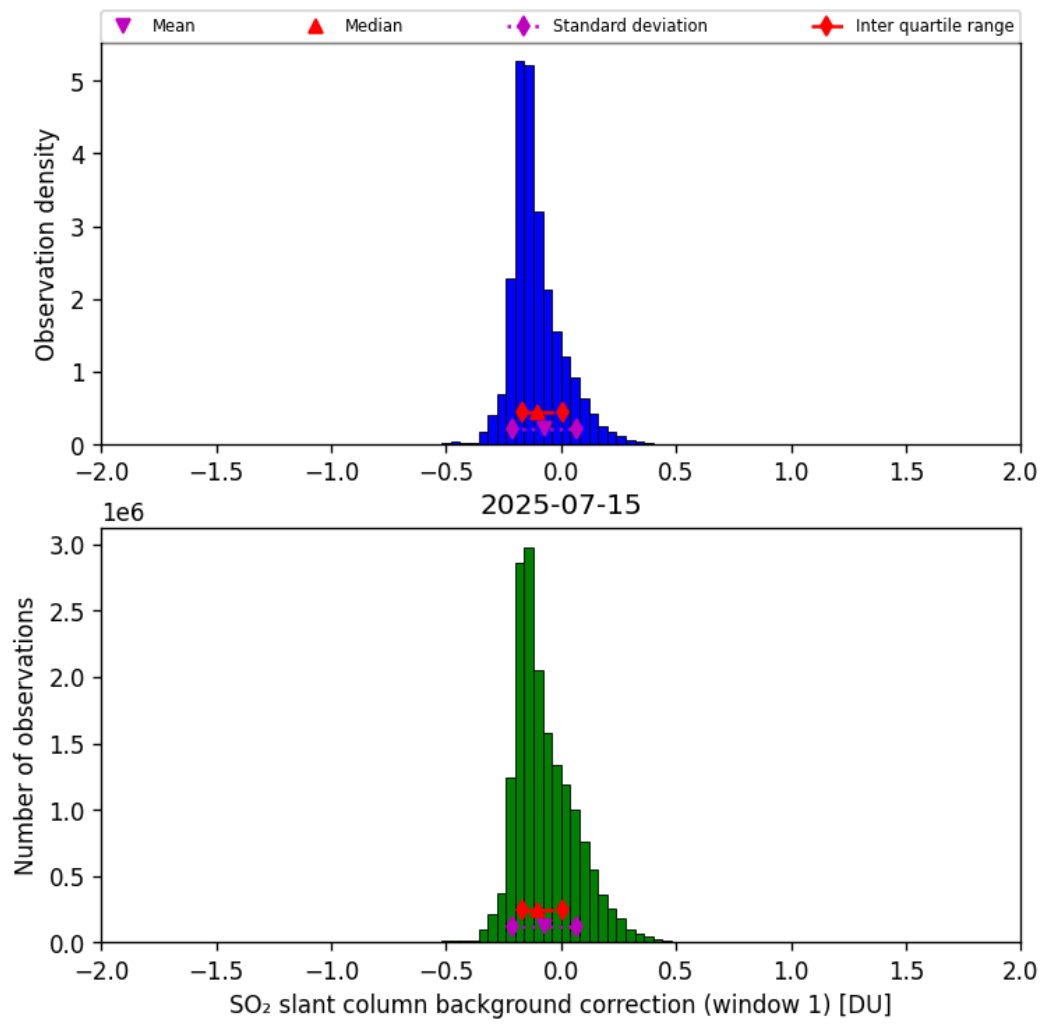
Figure 66: Histogram of “SO 2 slant column background correction (window 1)” for 2025-07-15 to 2025-07-16
