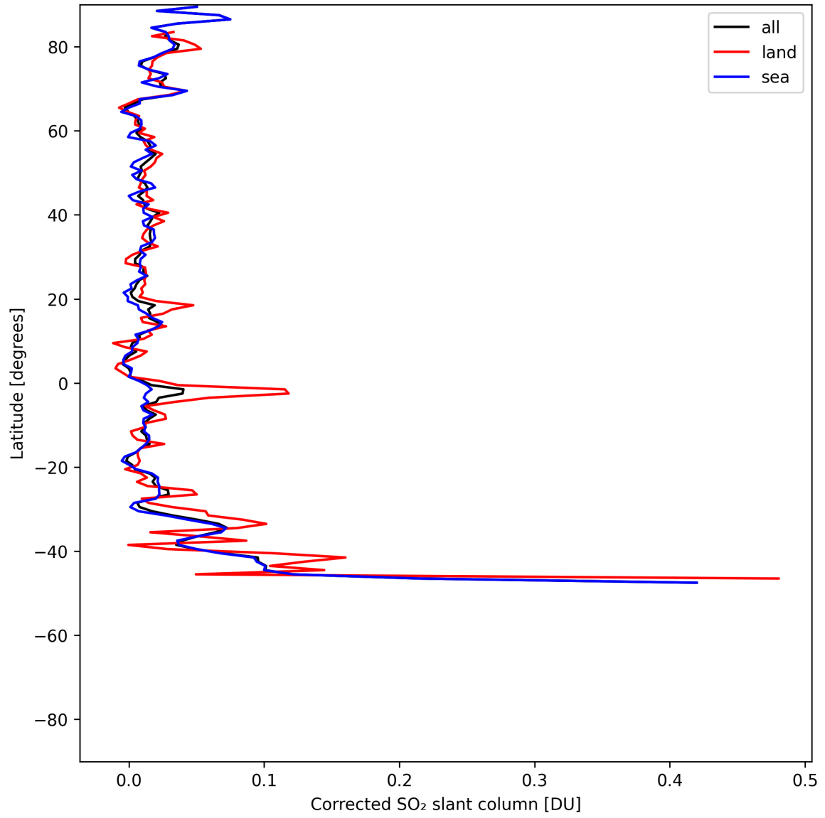
Figure 33: Zonal average of “Corrected SO 2 slant column” for 2025-07-15 to 2025-07-16.
