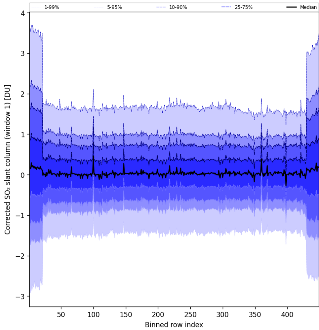
Figure 92: Along track statistics of “Corrected SO 2 slant column (window 1)” for 2025-07-15 to 2025-07-16
