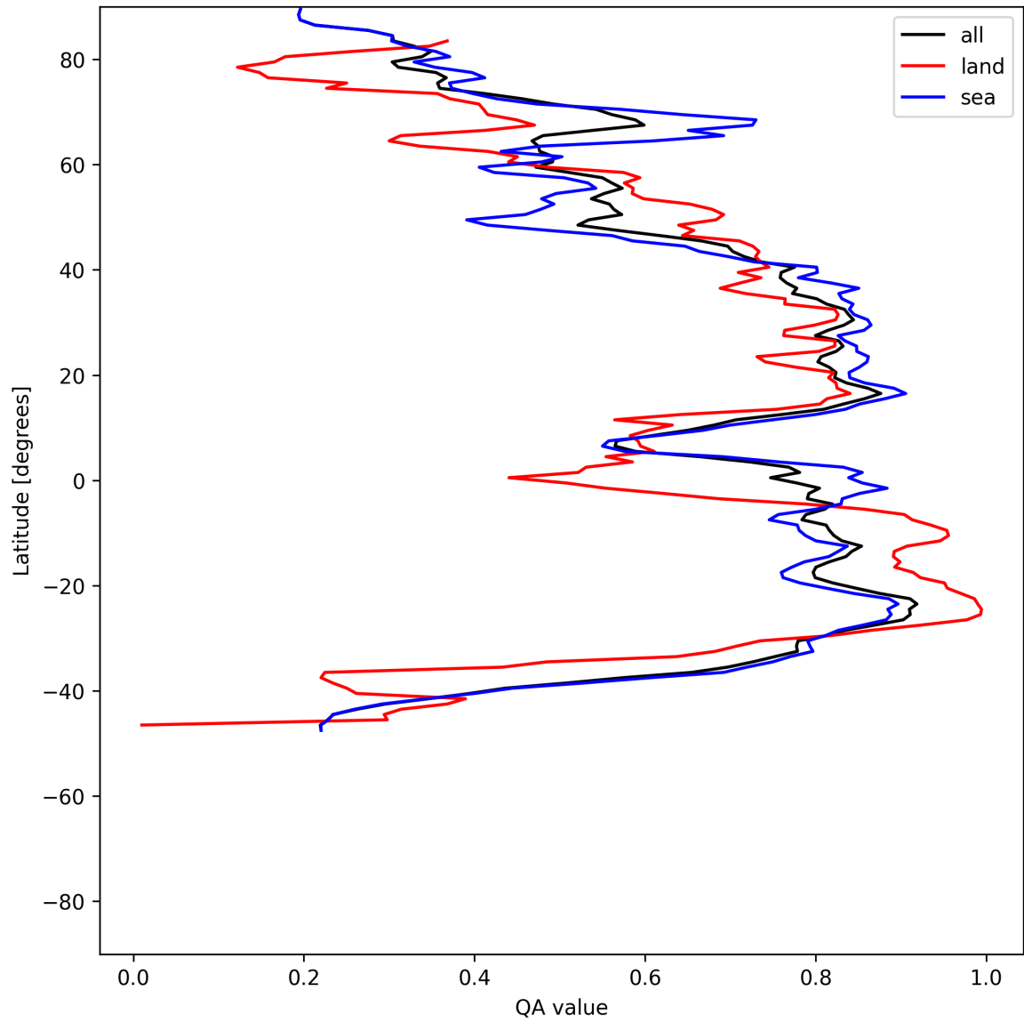
Figure 30: Zonal average of “QA value” for 2025-07-15 to 2025-07-16.
