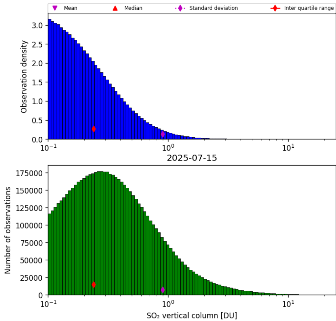
Figure 58: Histogram of “SO 2 vertical column” for 2025-07-15 to 2025-07-16
