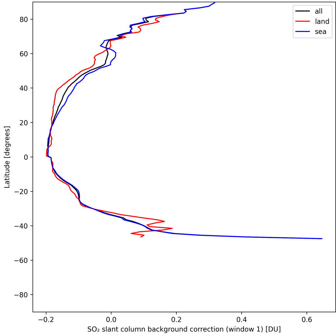
Figure 39: Zonal average of “SO 2 slant column background correction (window 1)” for 2025-07-15 to 2025-07-16.
