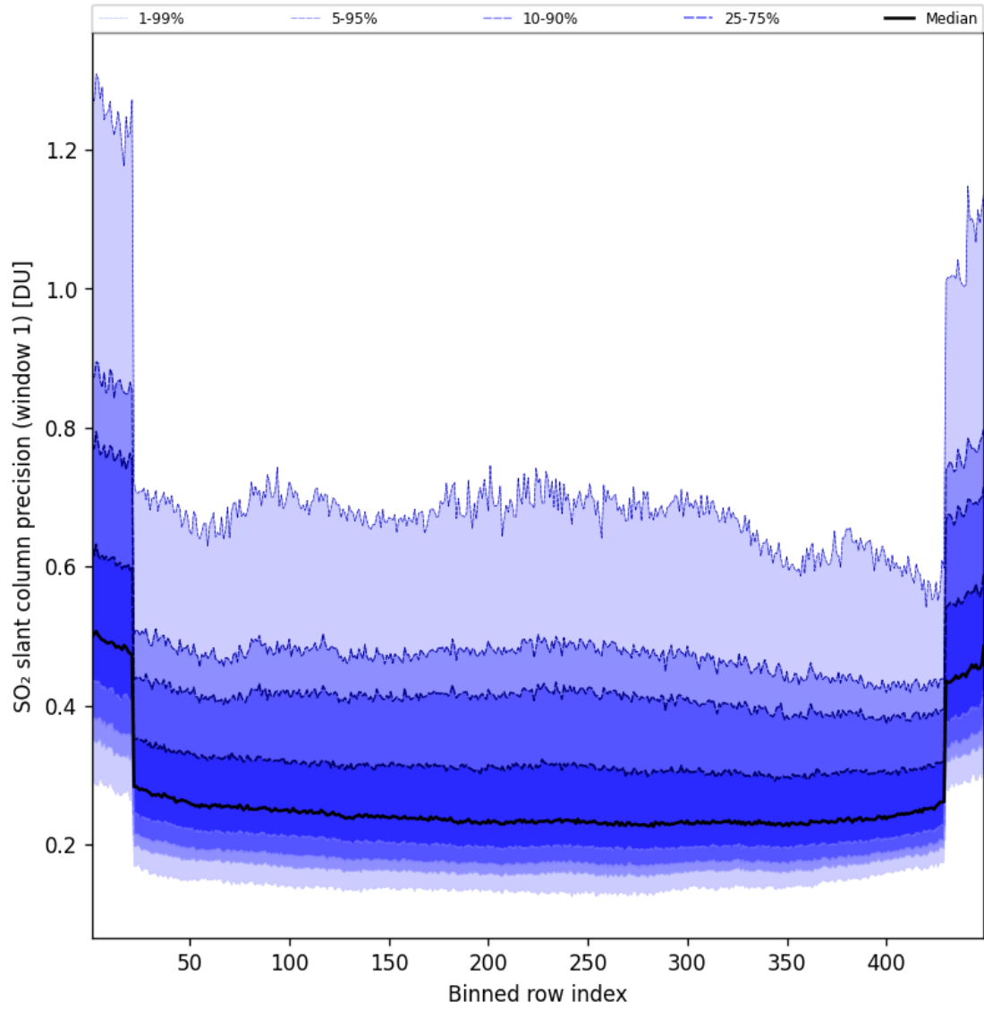
Figure 91: Along track statistics of “SO 2 slant column precision (window 1)” for 2025-07-15 to 2025-07-16
