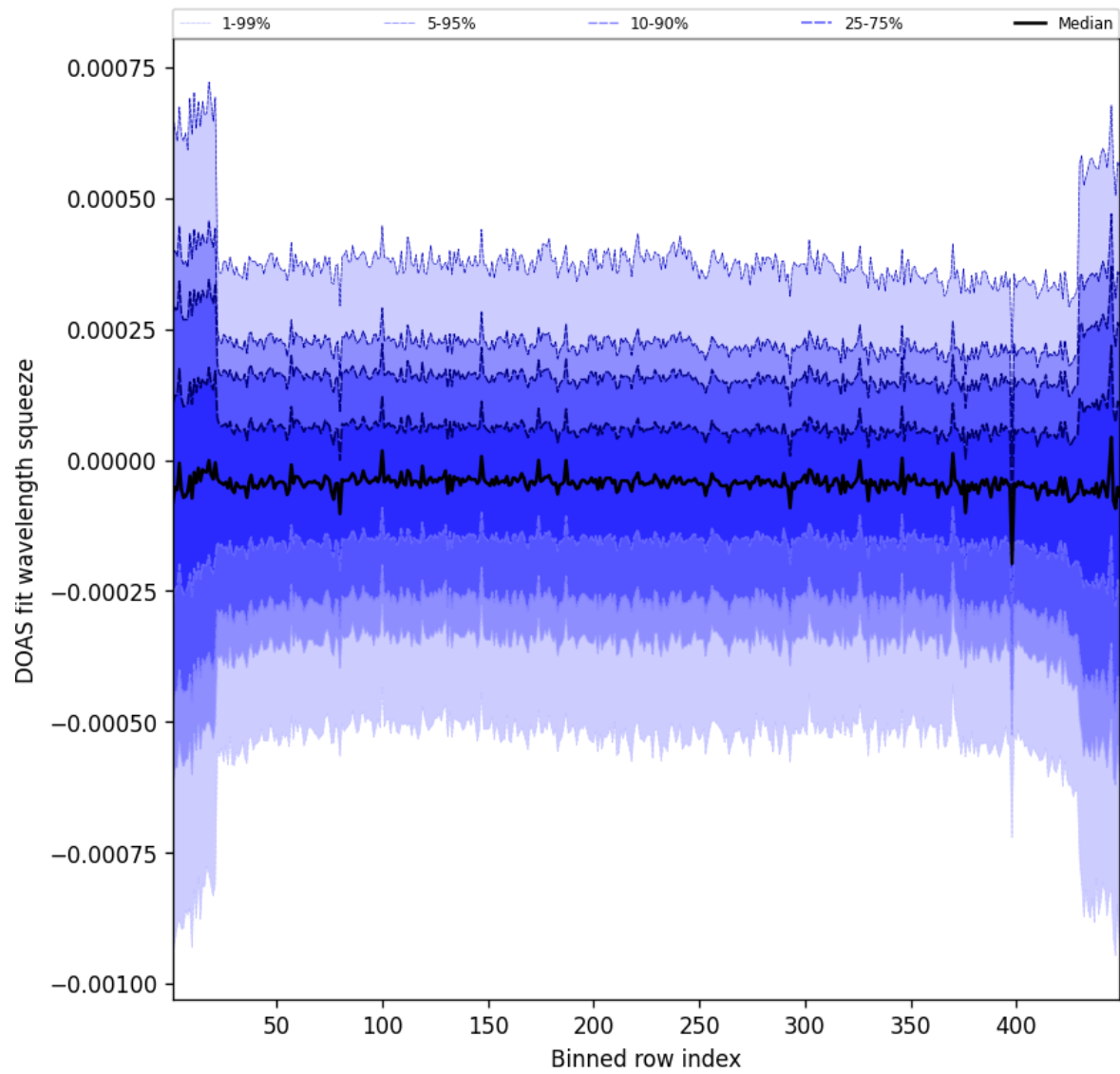
Figure 105: Along track statistics of “DOAS fit wavelength squeeze” for 2025-07-15 to 2025-07-16
