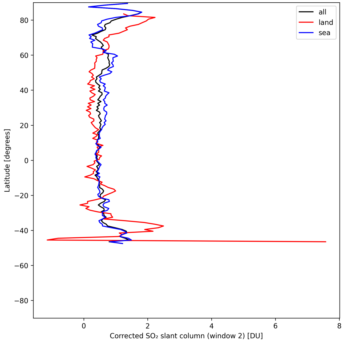
Figure 42: Zonal average of “Corrected SO 2 slant column (window 2)” for 2025-07-15 to 2025-07-16.
