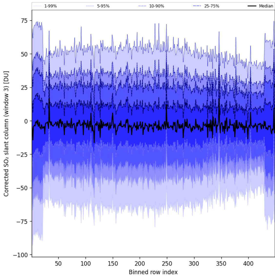
Figure 100: Along track statistics of "Corrected SO 2 slant column (window 3)" for 2025-07-15 to 2025-07-16
