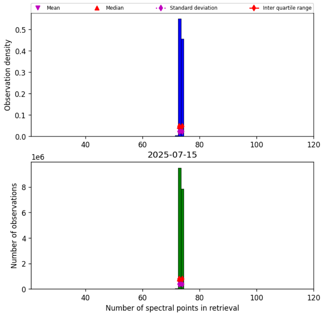
Figure 83: Histogram of “Number of spectral points in retrieval” for 2025-07-15 to 2025-07-16
