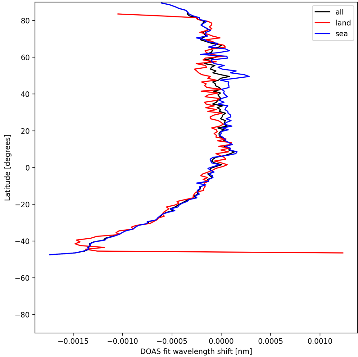
Figure 50: Zonal average of “DOAS fit wavelength shift” for 2025-07-15 to 2025-07-16.
