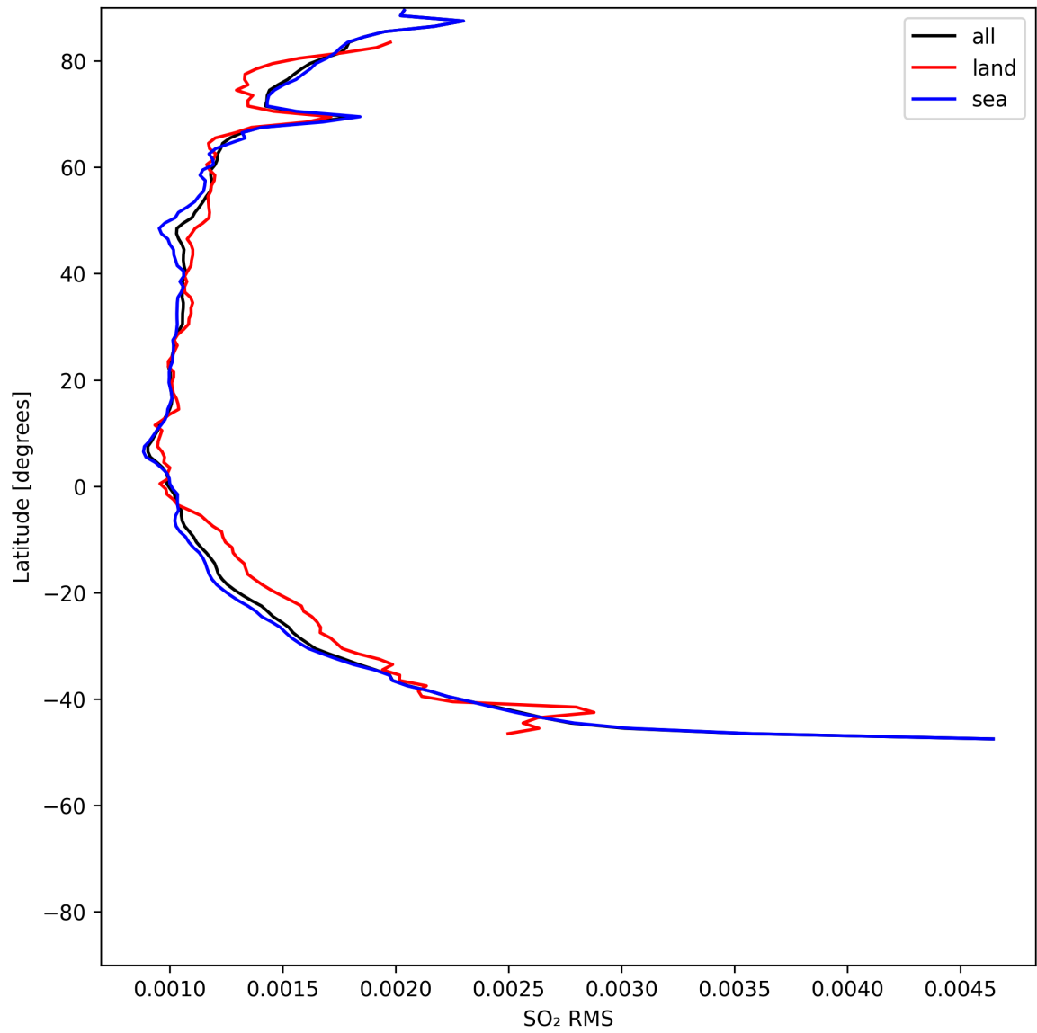
Figure 52: Zonal average of “SO 2 RMS” for 2025-07-15 to 2025-07-16.
