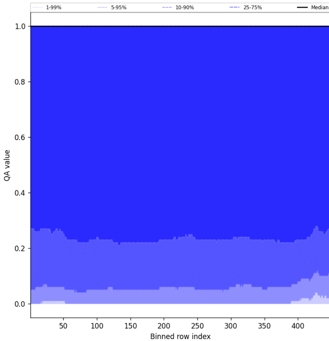
Figure 84: Along track statistics of “QA value” for 2025-07-15 to 2025-07-16
