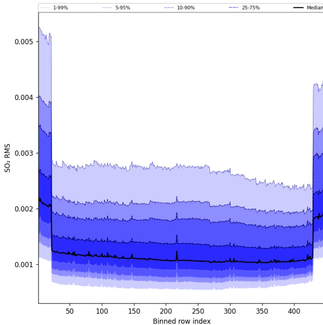
Figure 106: Along track statistics of “SO 2 RMS” for 2025-07-15 to 2025-07-16
