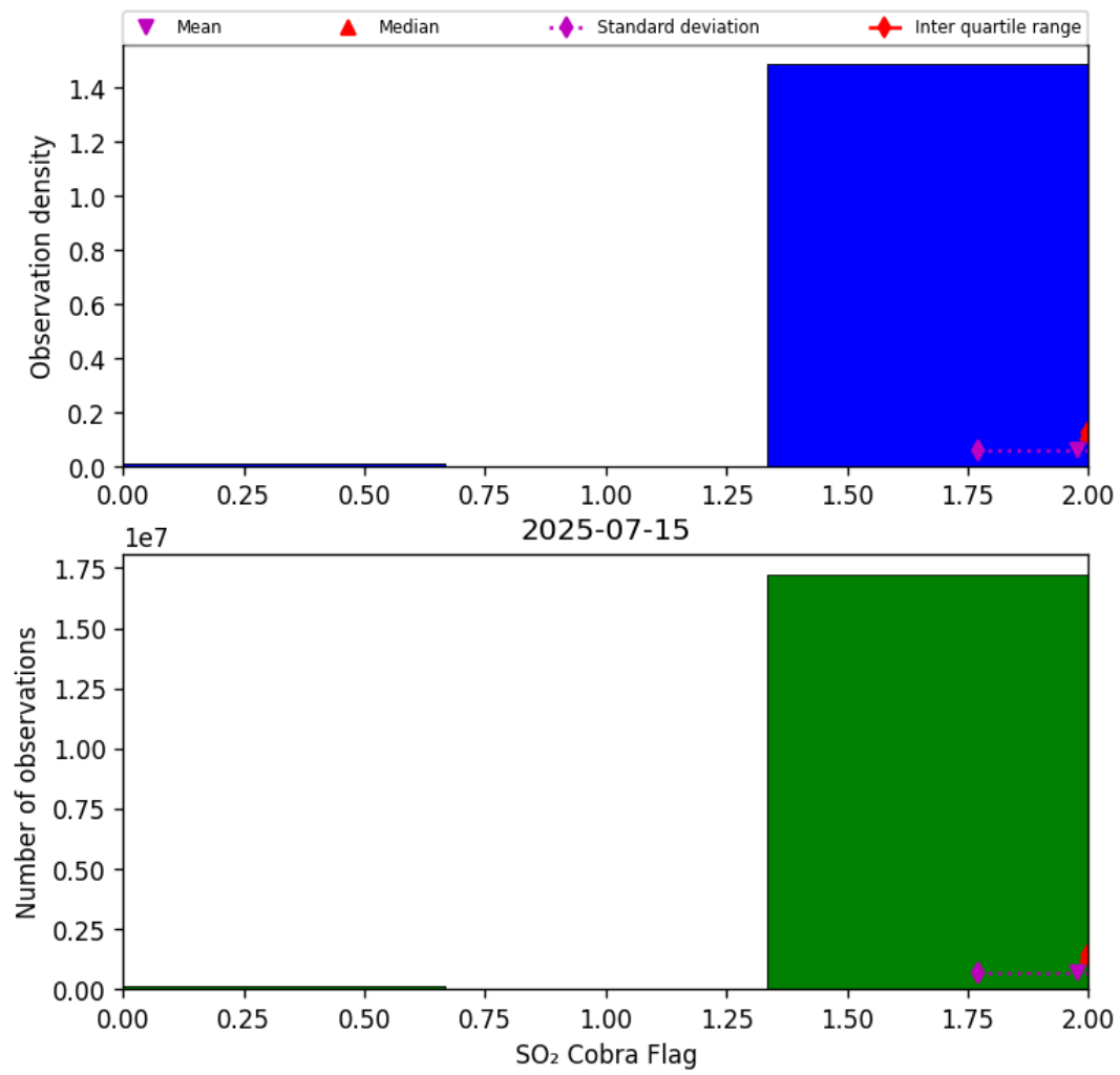
Figure 75: Histogram of “SO 2 Cobra Flag” for 2025-07-15 to 2025-07-16
