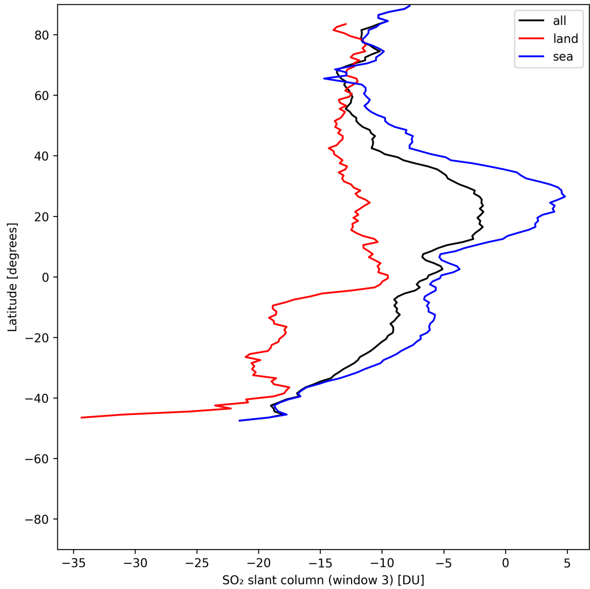
Figure 44: Zonal average of “SO 2 slant column (window 3)” for 2025-07-15 to 2025-07-16.
