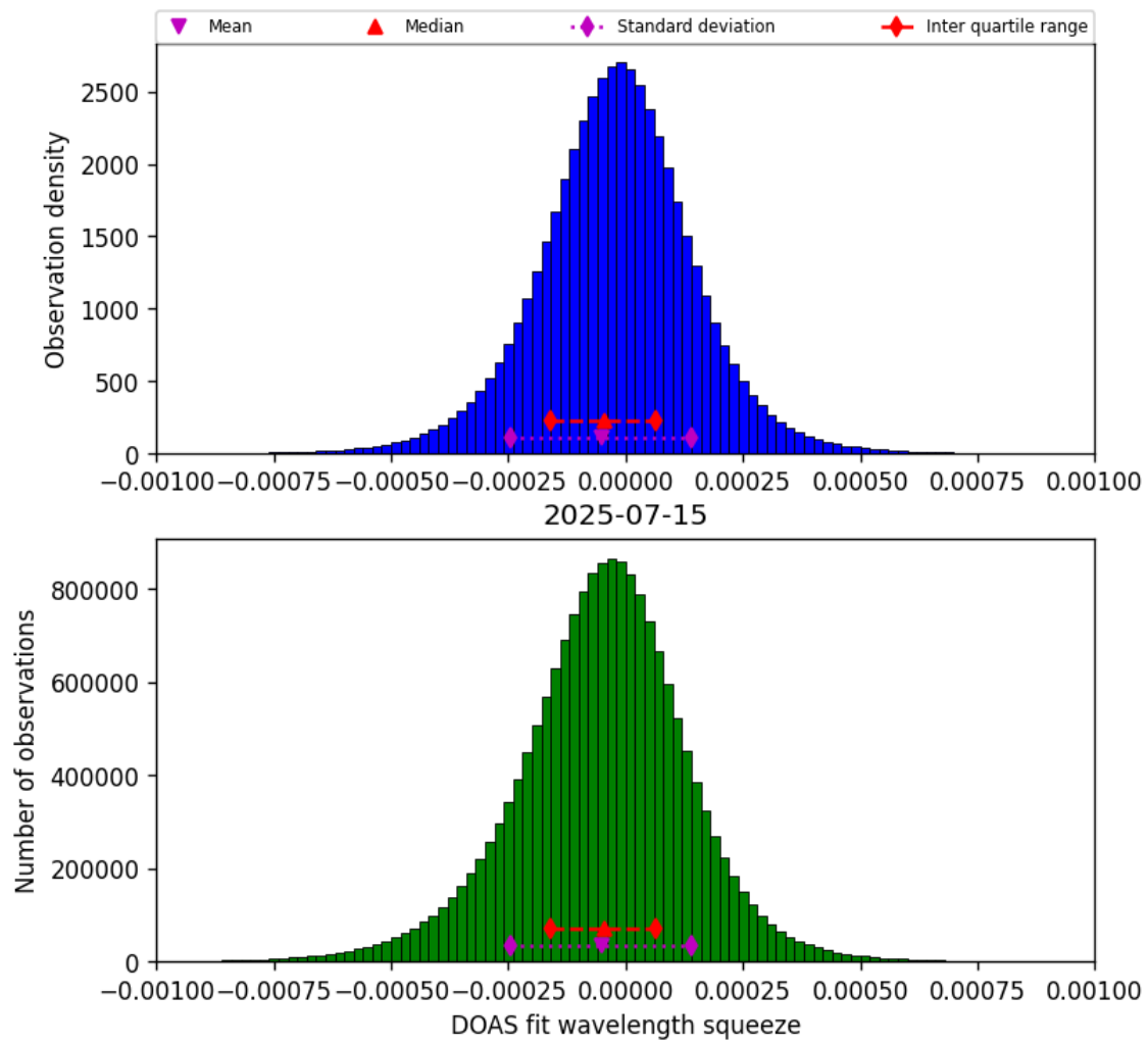
Figure 78: Histogram of “DOAS fit wavelength squeeze” for 2025-07-15 to 2025-07-16
