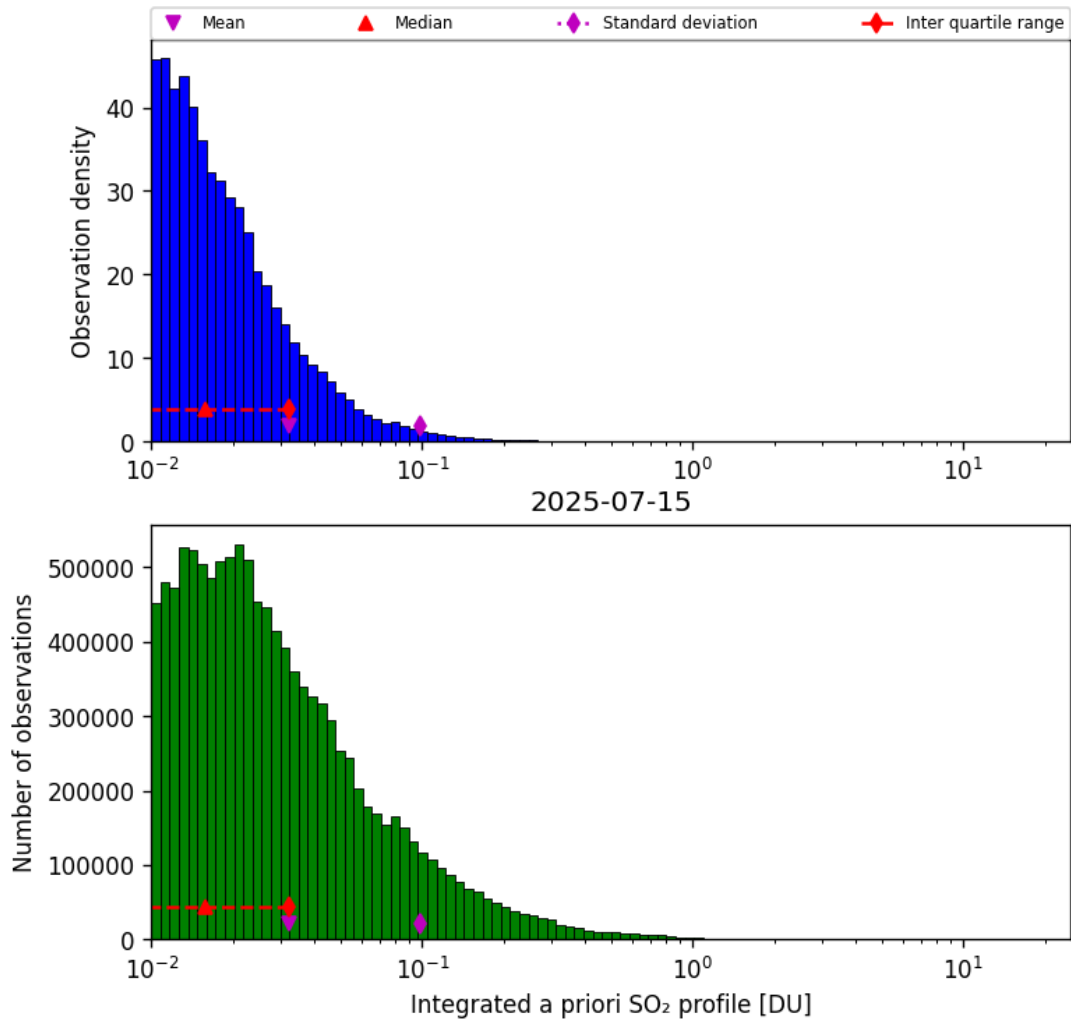
Figure 76: Histogram of “Integrated a priori SO 2 profile” for 2025-07-15 to 2025-07-16
