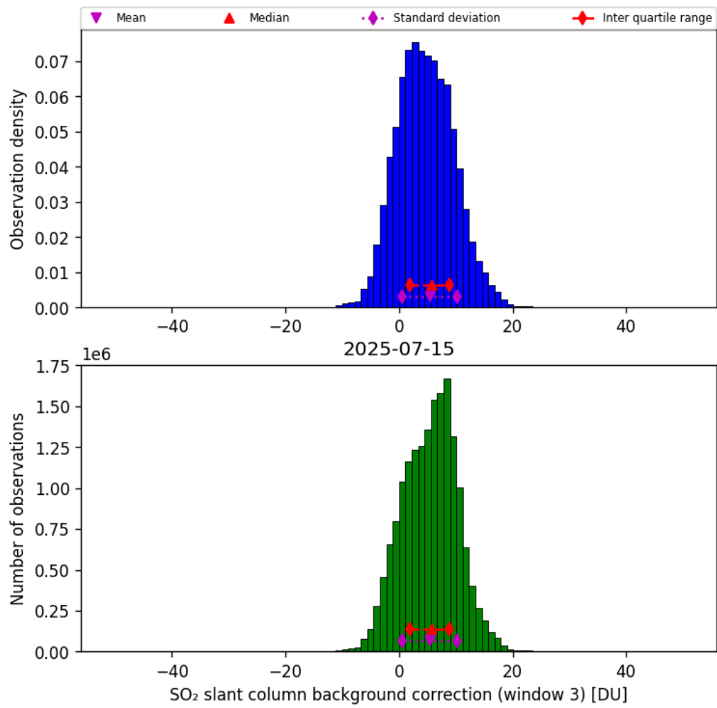
Figure 74: Histogram of “SO 2 slant column background correction (window 3)” for 2025-07-15 to 2025-07-16
