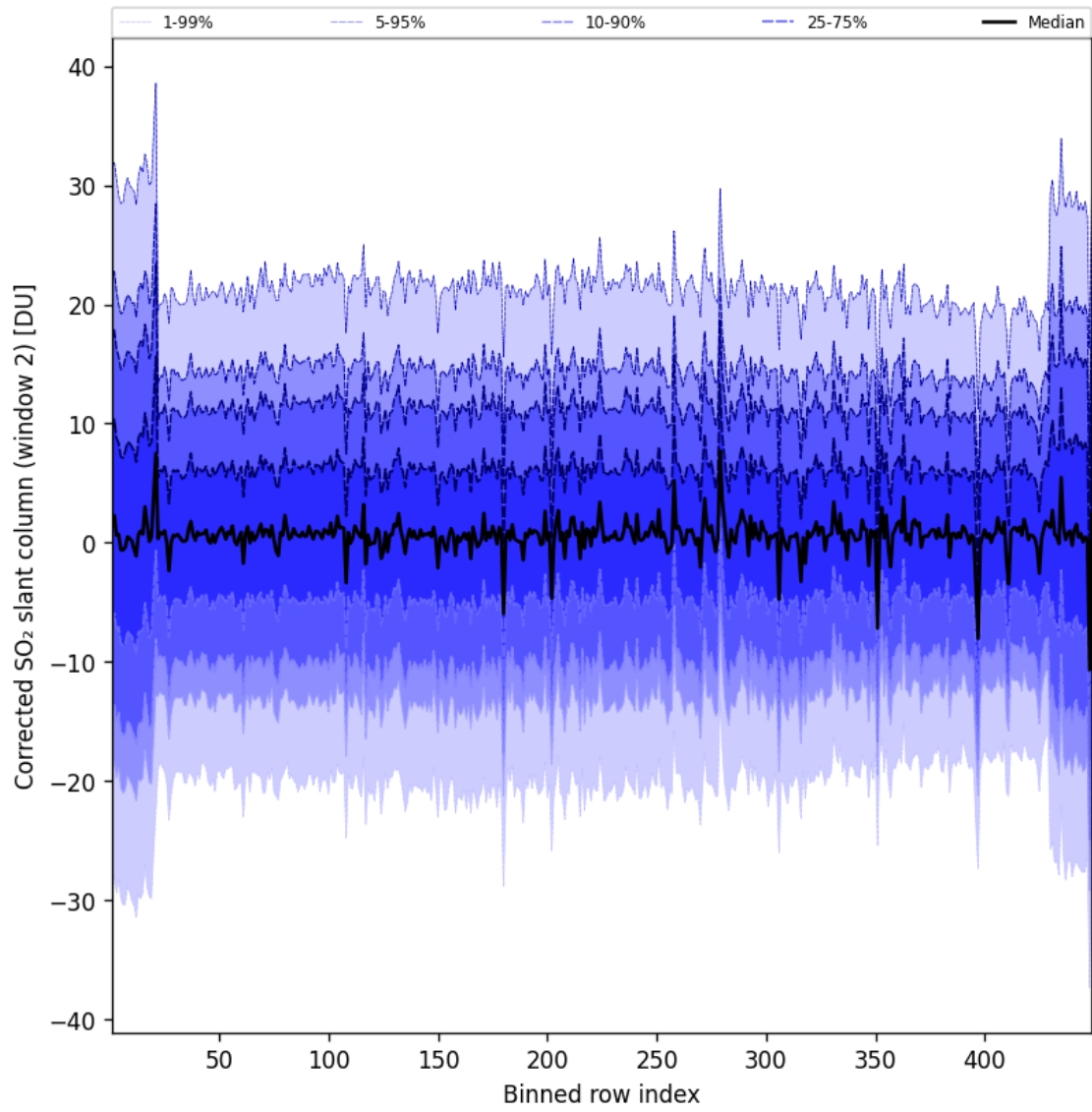
Figure 96: Along track statistics of “Corrected SO 2 slant column (window 2)” for 2025-07-15 to 2025-07-16
