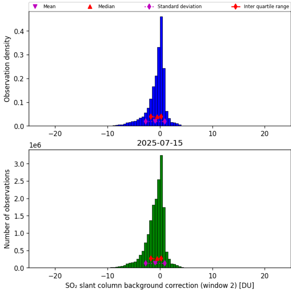
Figure 70: Histogram of “SO 2 slant column background correction (window 2)” for 2025-07-15 to 2025-07-16
