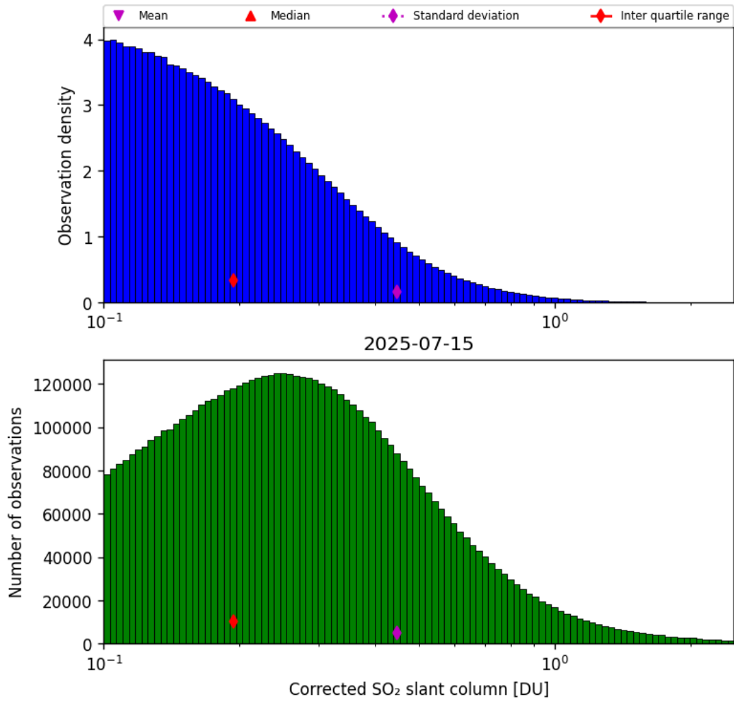
Figure 60: Histogram of “Corrected SO 2 slant column” for 2025-07-15 to 2025-07-16
