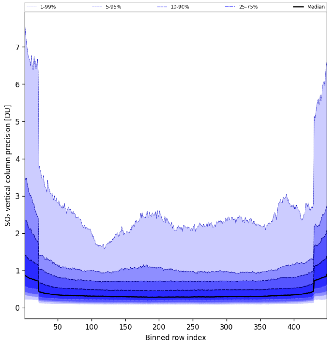
Figure 86: Along track statistics of “SO 2 vertical column precision” for 2025-07-15 to 2025-07-16
