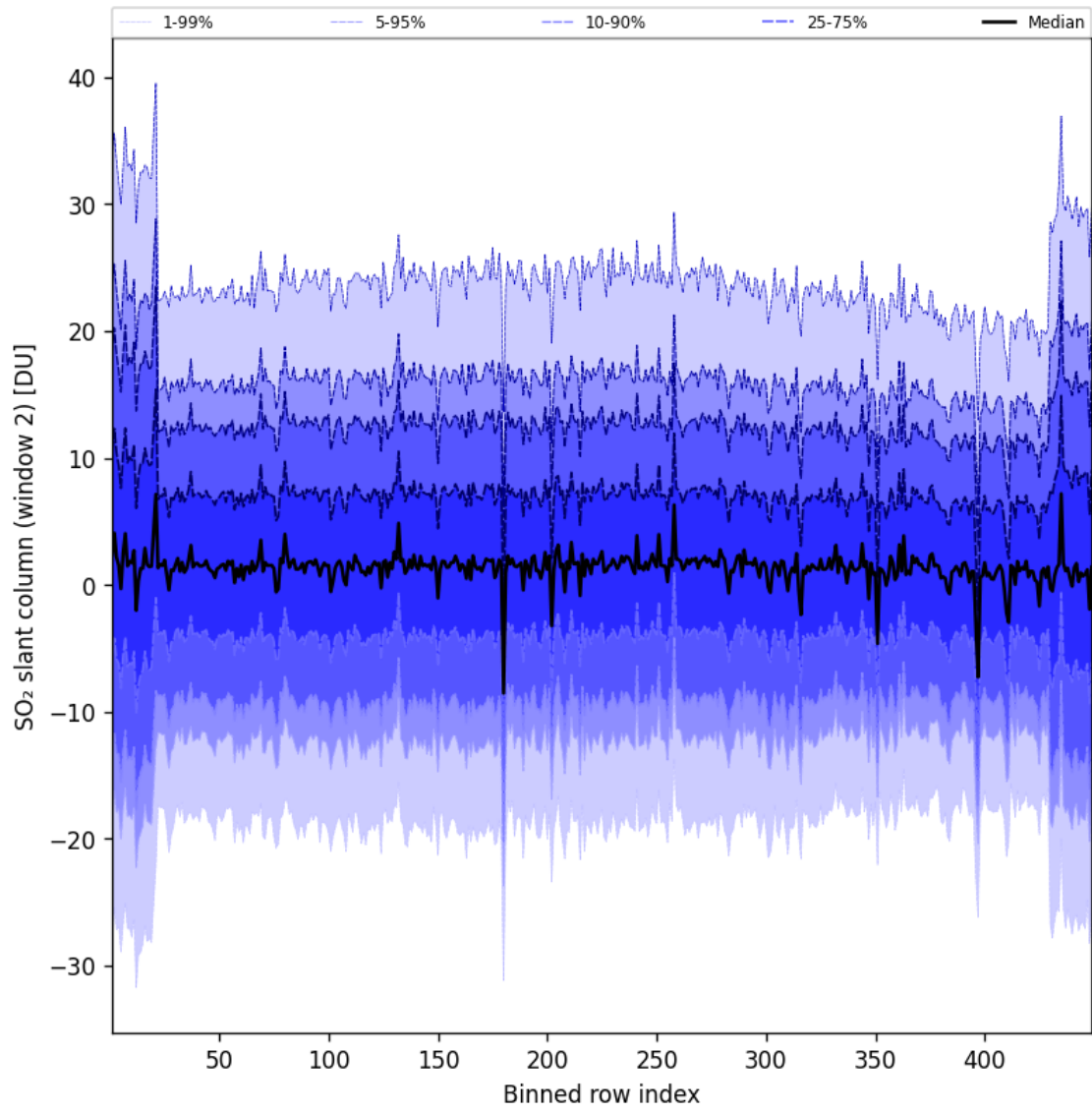
Figure 94: Along track statistics of “SO 2 slant column (window 2)” for 2025-07-15 to 2025-07-16
