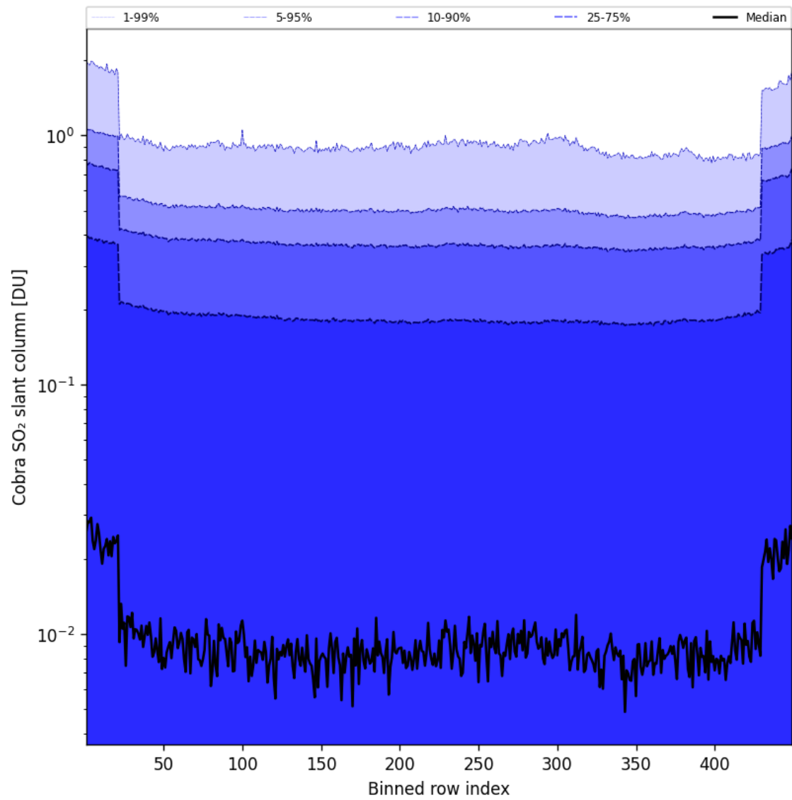
Figure 88: Along track statistics of “Cobra SO 2 slant column” for 2025-07-15 to 2025-07-16
