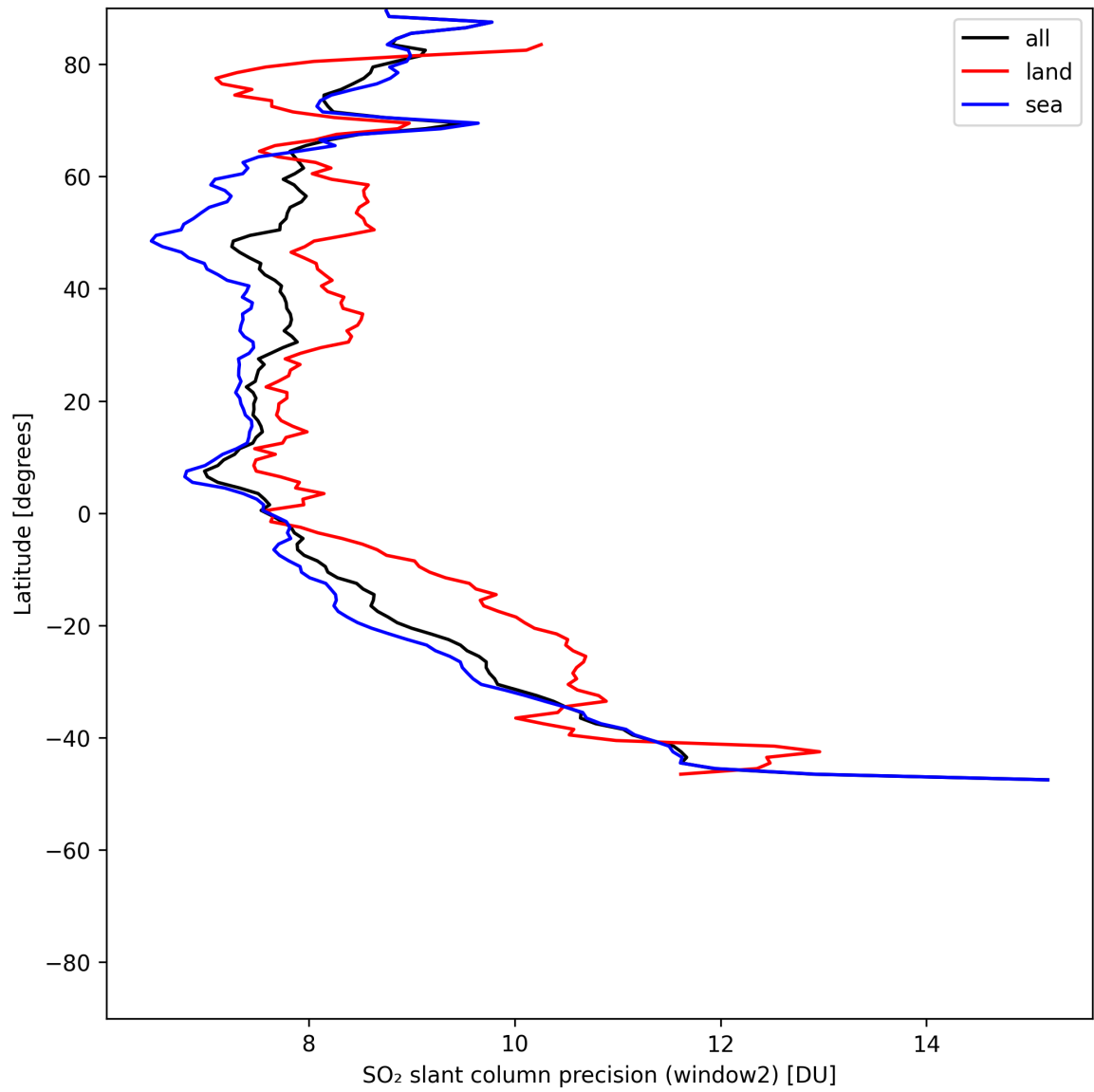
Figure 41: Zonal average of “SO 2 slant column precision (window2)” for 2025-07-15 to 2025-07-16.
