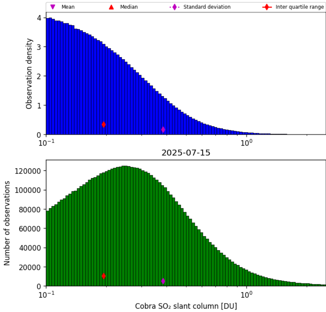
Figure 61: Histogram of “Cobra SO 2 slant column” for 2025-07-15 to 2025-07-16
