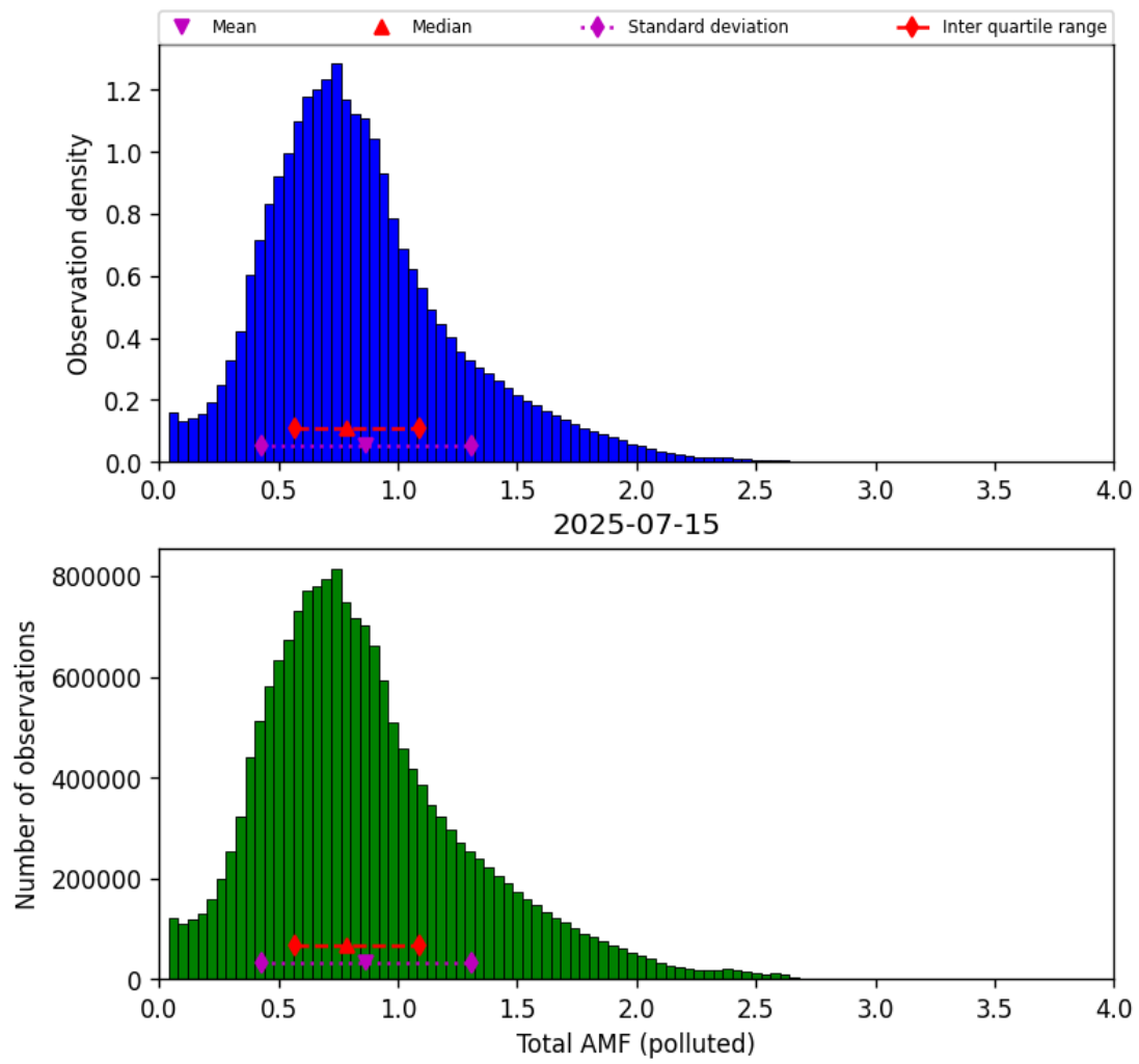
Figure 80: Histogram of “Total AMF (polluted)” for 2025-07-15 to 2025-07-16
