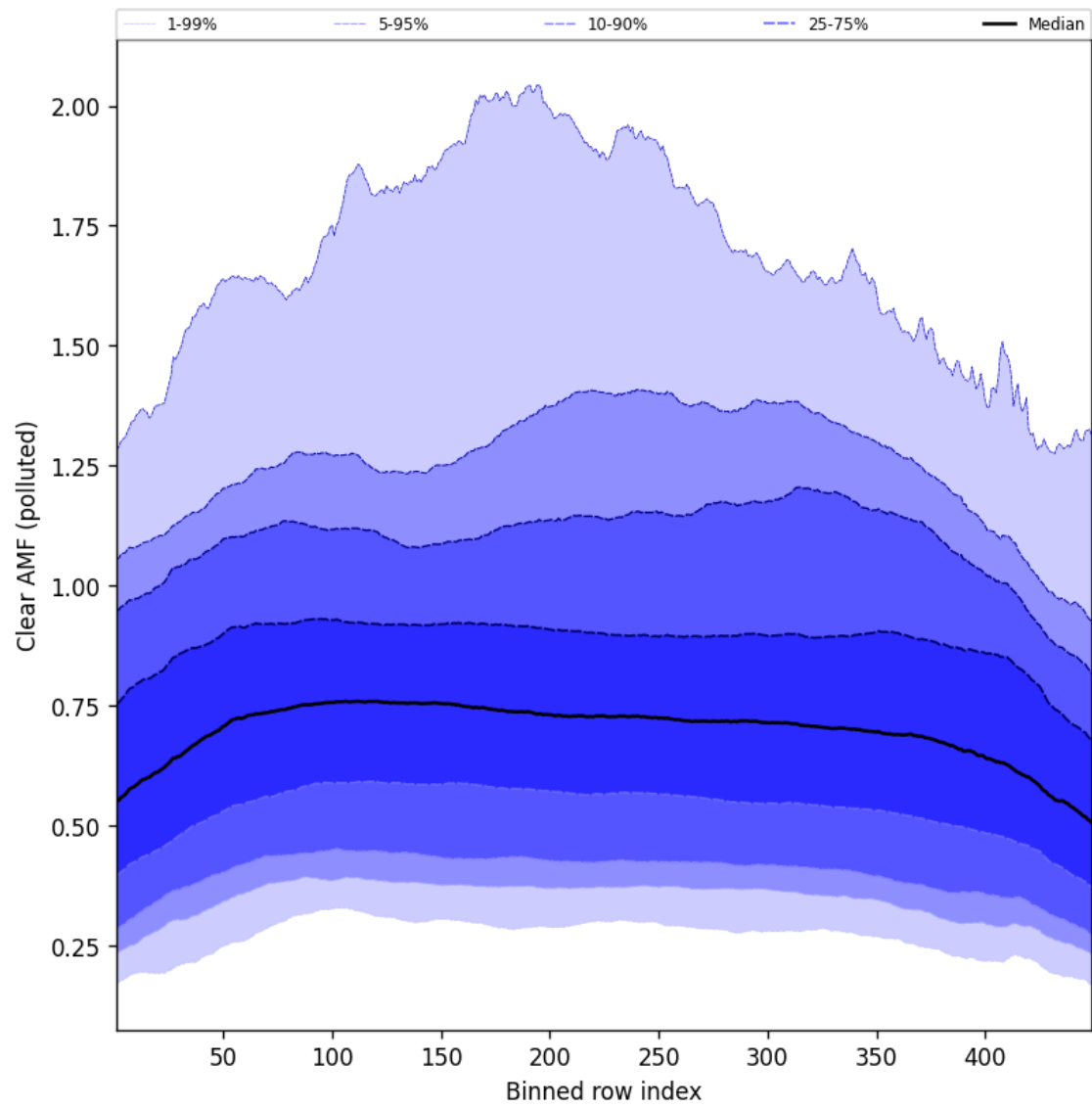
Figure 109: Along track statistics of “Clear AMF (polluted)” for 2025-07-15 to 2025-07-16
