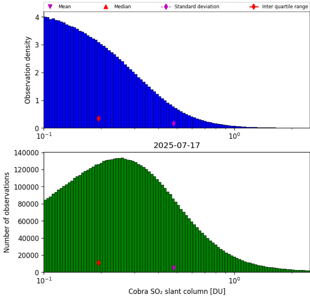
Figure 61: Histogram of “Cobra SO 2 slant column” for 2025-07-17 to 2025-07-18
