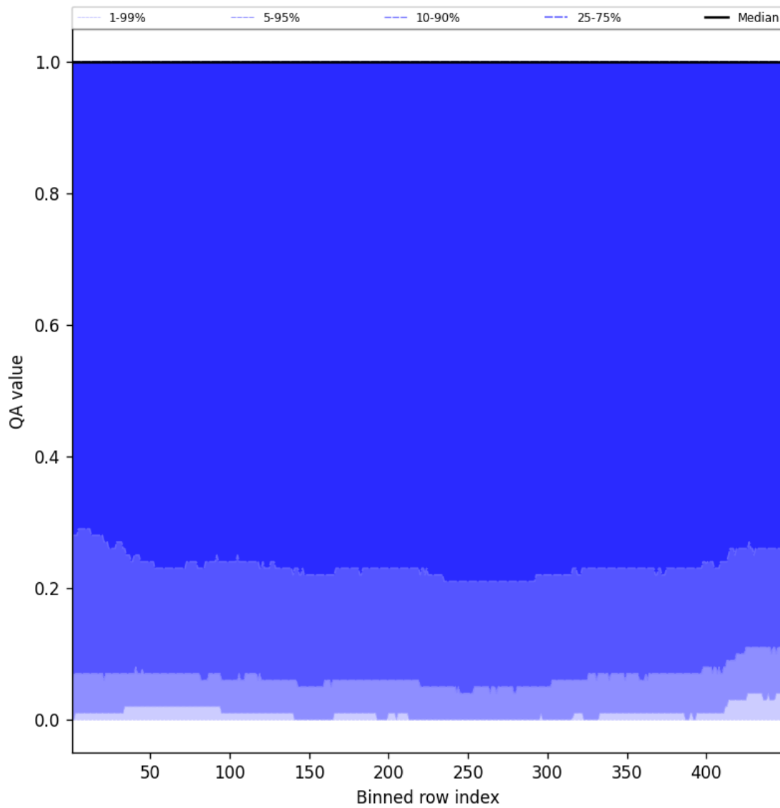
Figure 84: Along track statistics of “QA value” for 2025-07-17 to 2025-07-18
