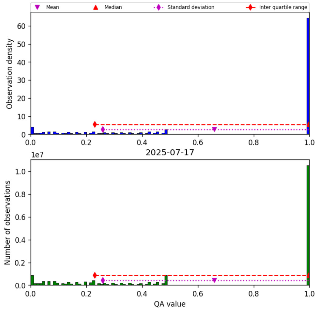
Figure 57: Histogram of “QA value” for 2025-07-17 to 2025-07-18
