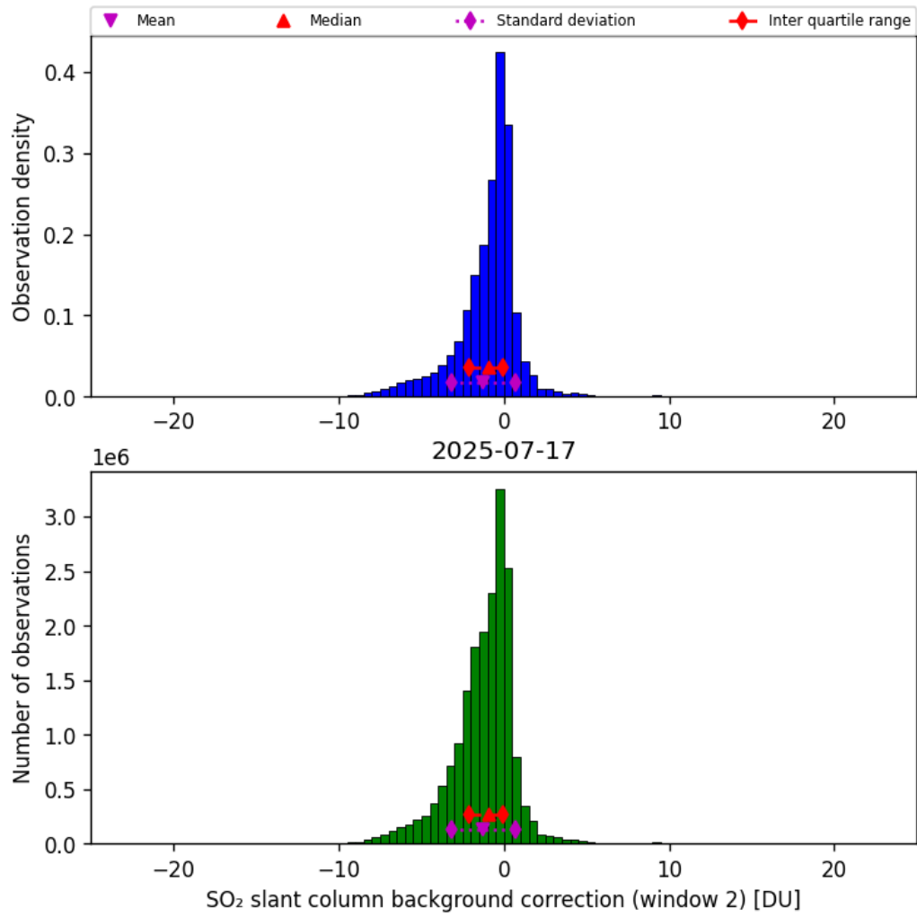
Figure 70: Histogram of “SO 2 slant column background correction (window 2)” for 2025-07-17 to 2025-07-18
