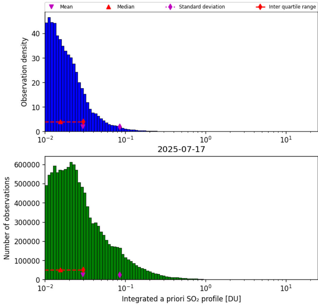
Figure 76: Histogram of “Integrated a priori SO 2 profile” for 2025-07-17 to 2025-07-18
