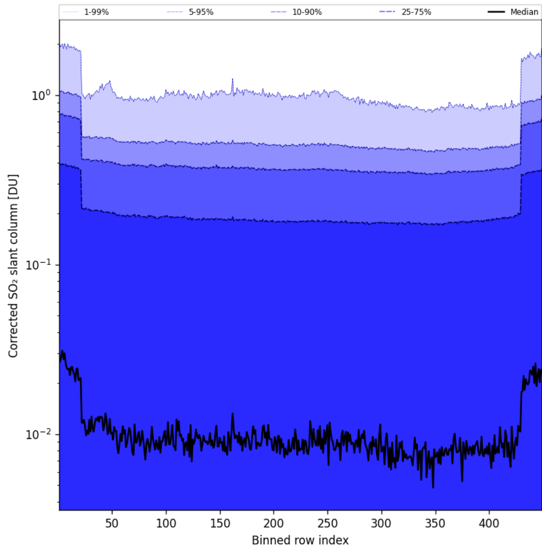
Figure 87: Along track statistics of "Corrected SO 2 slant column" for 2025-07-17 to 2025-07-18
