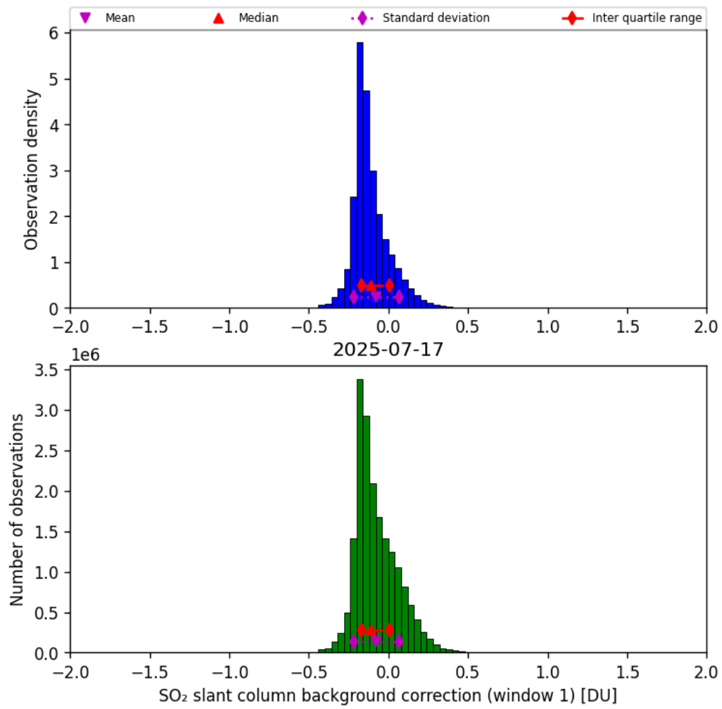
Figure 66: Histogram of “SO 2 slant column background correction (window 1)” for 2025-07-17 to 2025-07-18
