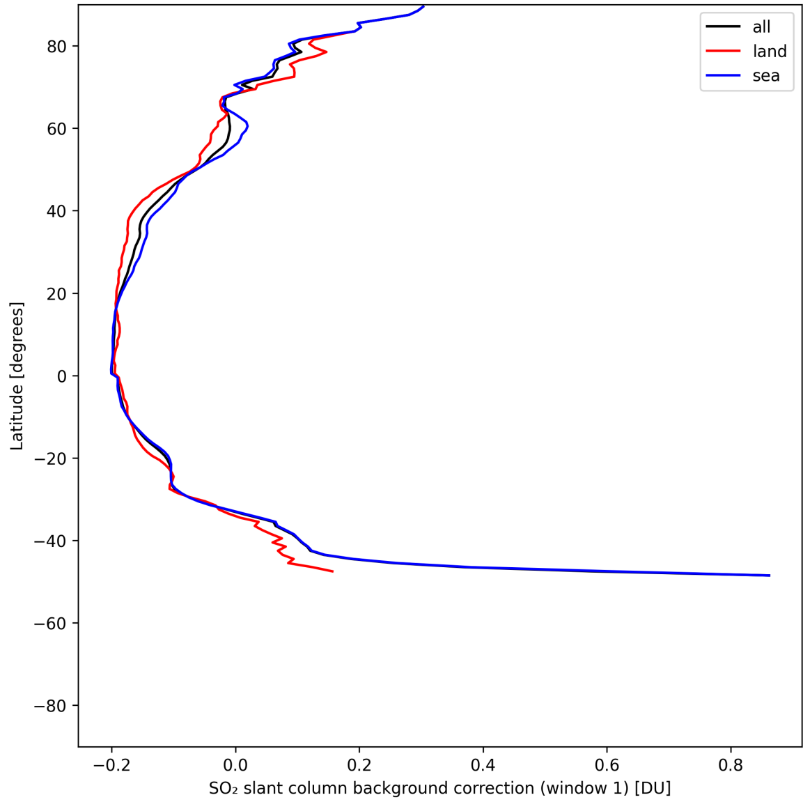
Figure 39: Zonal average of “SO 2 slant column background correction (window 1)” for 2025-07-17 to 2025-07-18.
