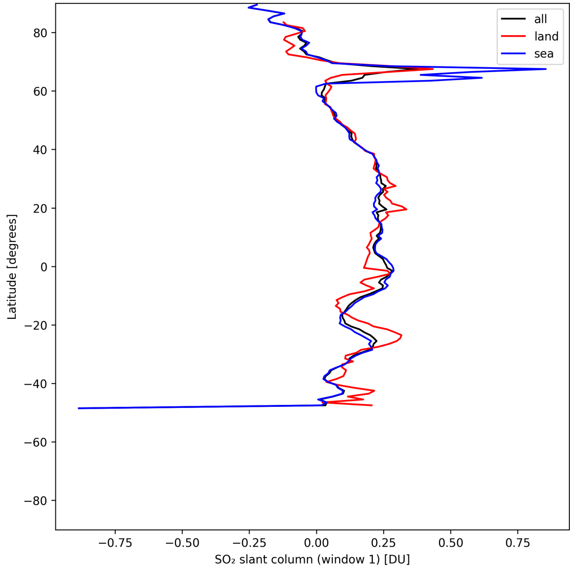
Figure 36: Zonal average of “SO 2 slant column (window 1)” for 2025-07-17 to 2025-07-18.
