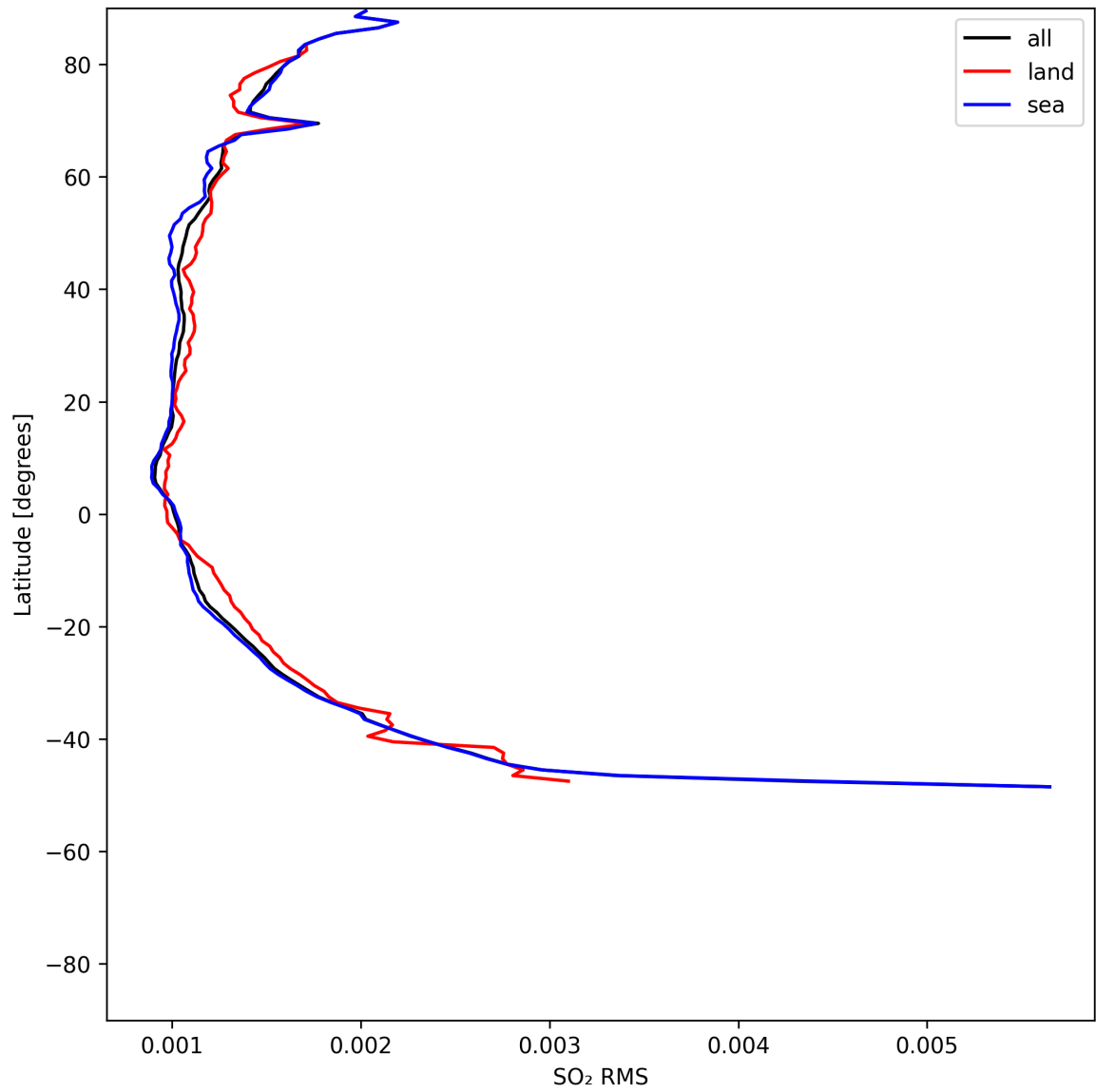
Figure 52: Zonal average of “SO 2 RMS” for 2025-07-17 to 2025-07-18.
