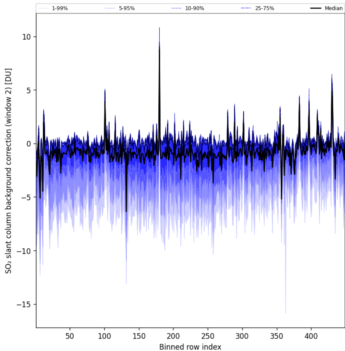
Figure 97: Along track statistics of “SO 2 slant column background correction (window 2)” for 2025-07-17 to 2025-07-18
