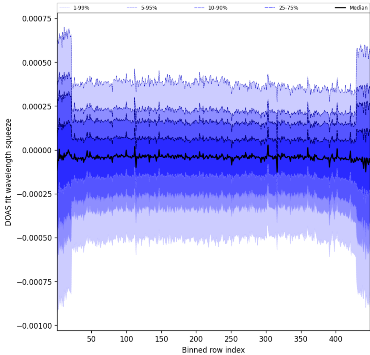
Figure 105: Along track statistics of “DOAS fit wavelength squeeze” for 2025-07-17 to 2025-07-18
