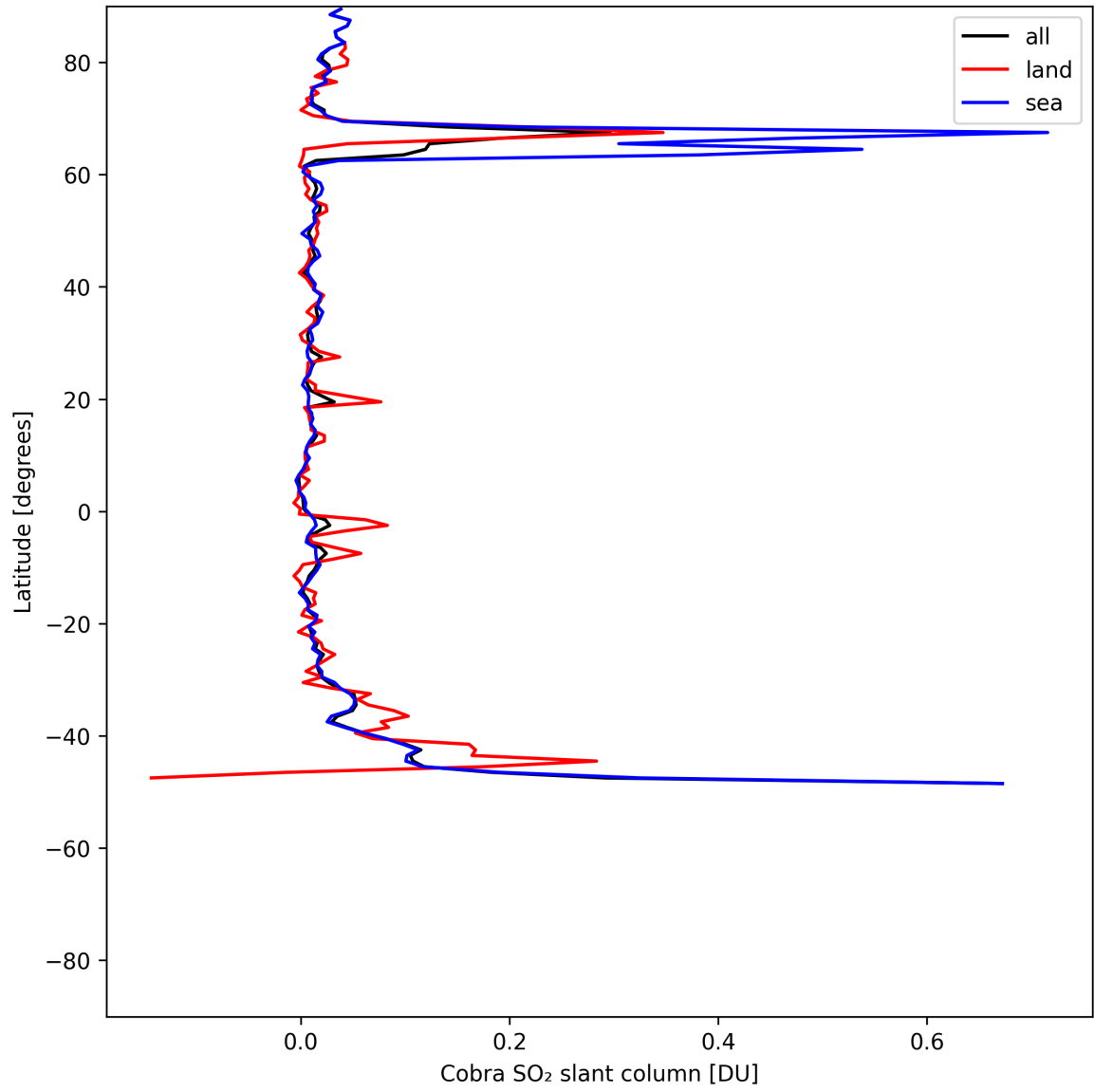
Figure 34: Zonal average of “Cobra SO 2 slant column” for 2025-07-17 to 2025-07-18.
