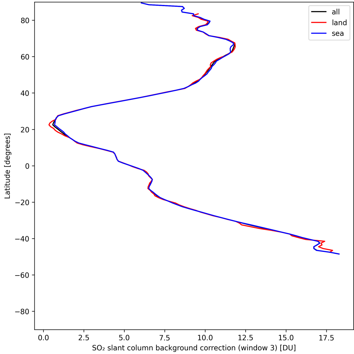
Figure 47: Zonal average of “SO 2 slant column background correction (window 3)” for 2025-07-17 to 2025-07-18.
