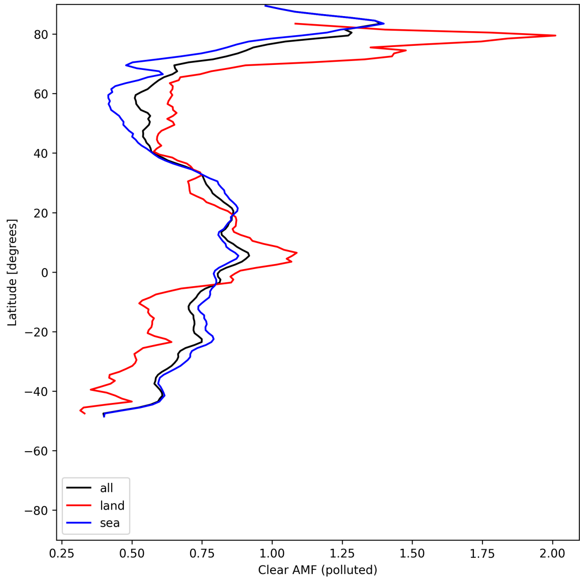
Figure 55: Zonal average of “Clear AMF (polluted)” for 2025-07-17 to 2025-07-18.
