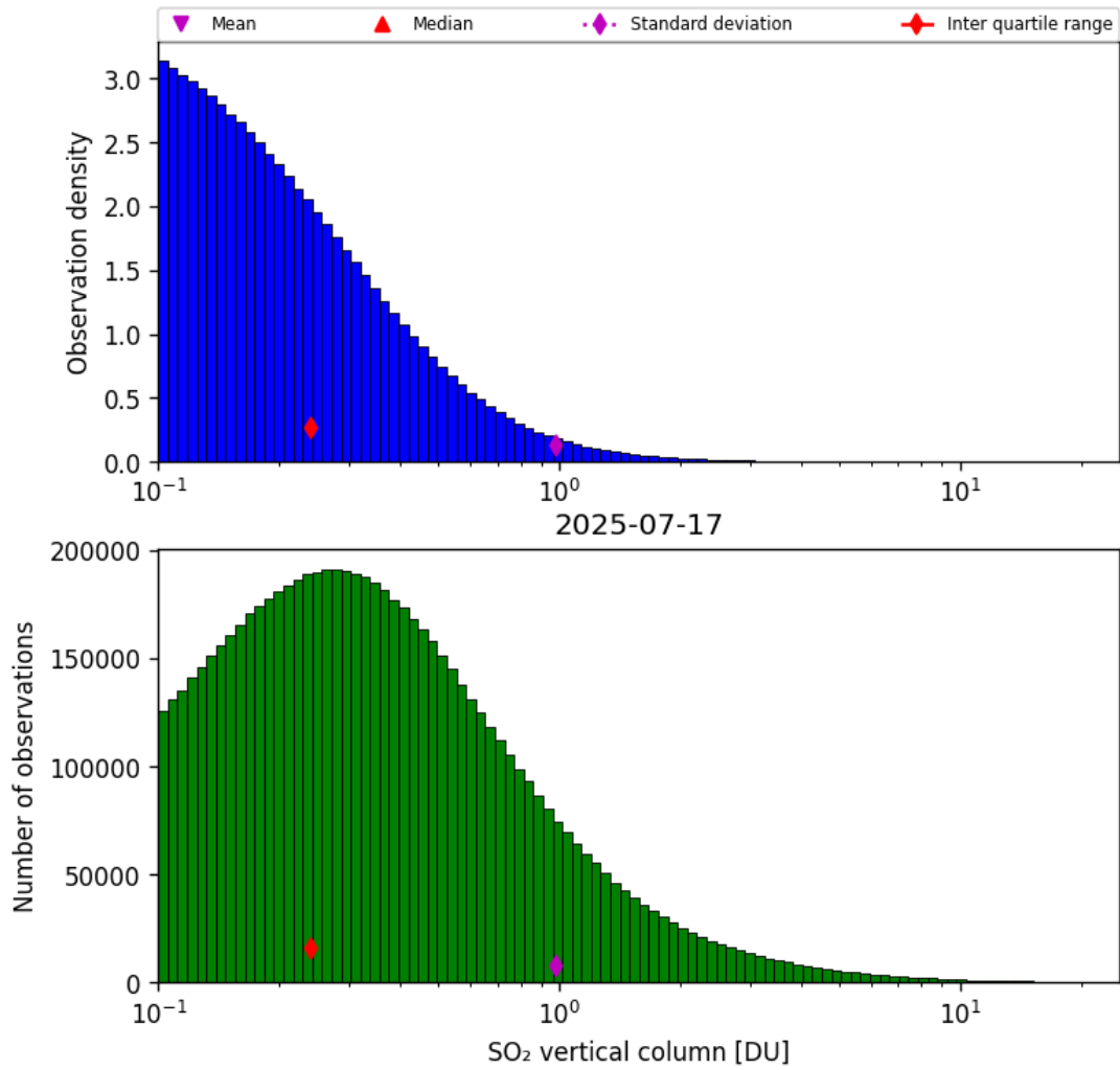
Figure 58: Histogram of “SO 2 vertical column” for 2025-07-17 to 2025-07-18
