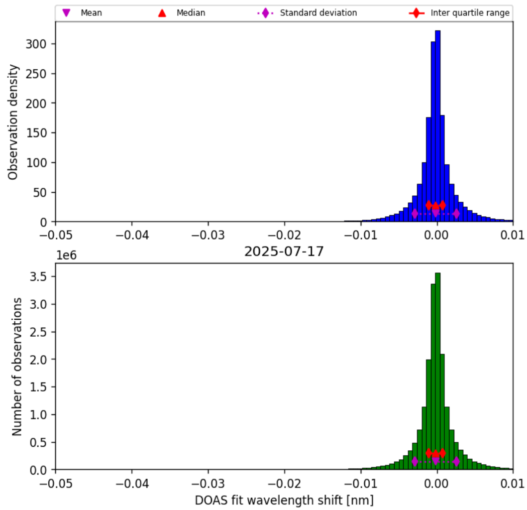
Figure 77: Histogram of “DOAS fit wavelength shift” for 2025-07-17 to 2025-07-18
