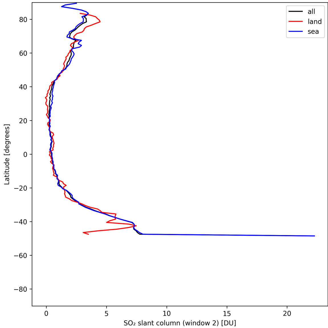
Figure 40: Zonal average of “SO 2 slant column (window 2)” for 2025-07-17 to 2025-07-18.
