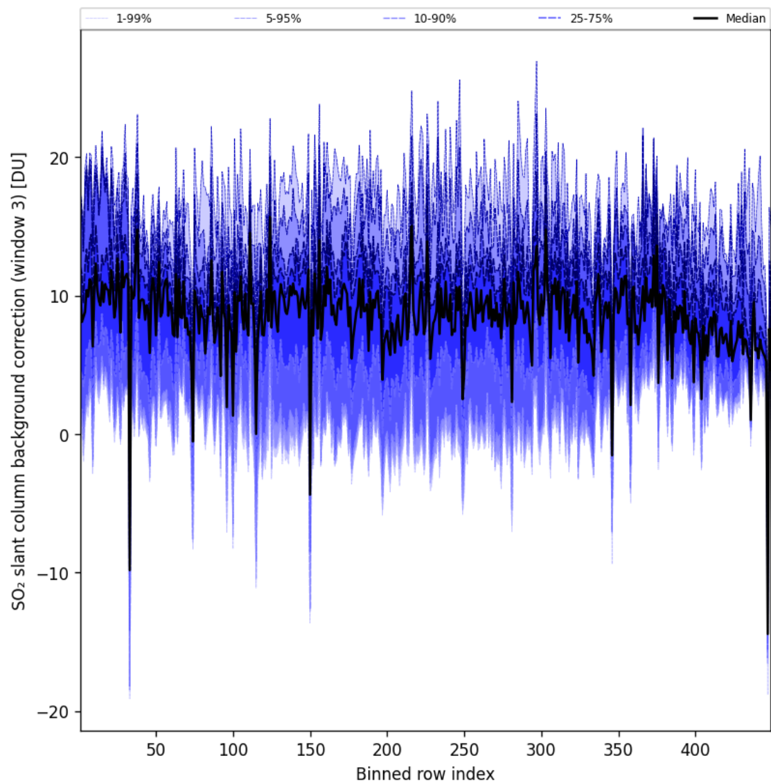
Figure 101: Along track statistics of “SO 2 slant column background correction (window 3)” for 2025-07-17 to 2025-07-18
