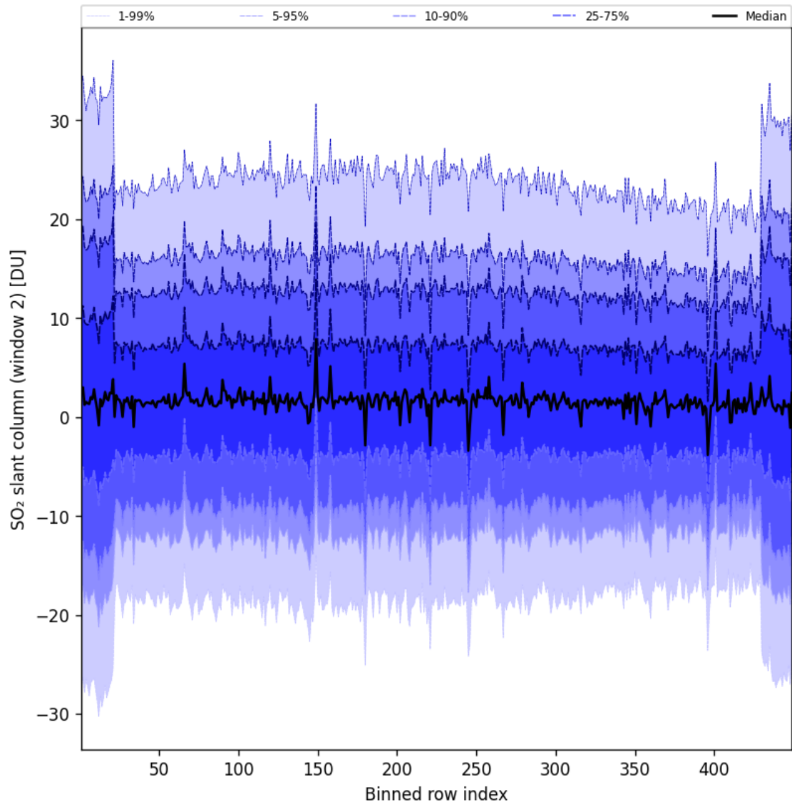
Figure 94: Along track statistics of “SO 2 slant column (window 2)” for 2025-07-17 to 2025-07-18
