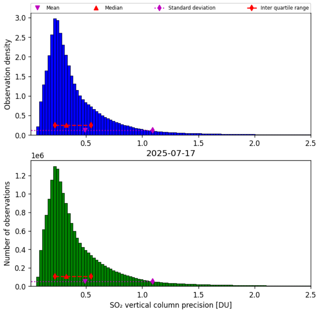
Figure 59: Histogram of “SO 2 vertical column precision” for 2025-07-17 to 2025-07-18
