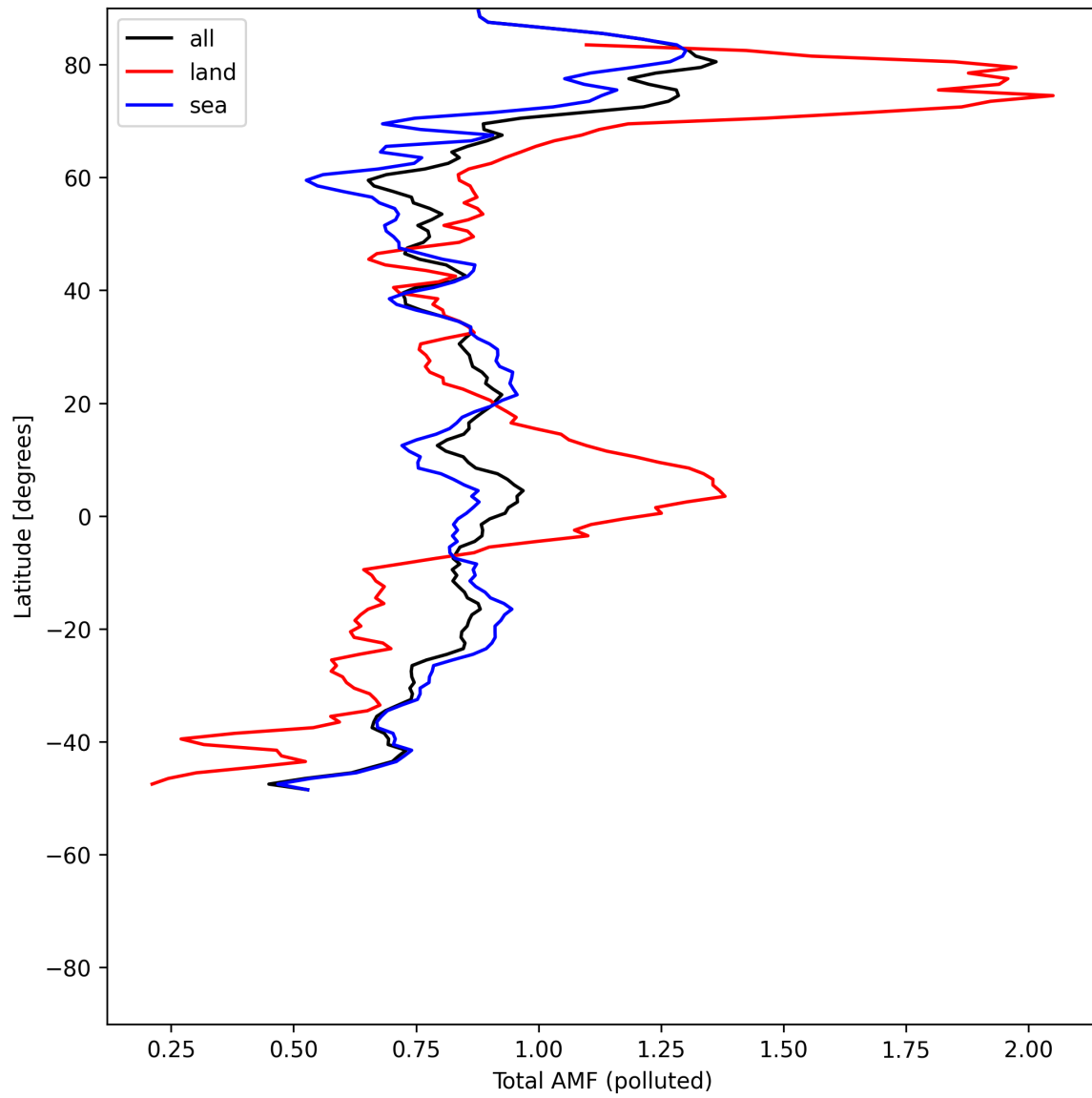
Figure 53: Zonal average of “Total AMF (polluted)” for 2025-07-17 to 2025-07-18.
