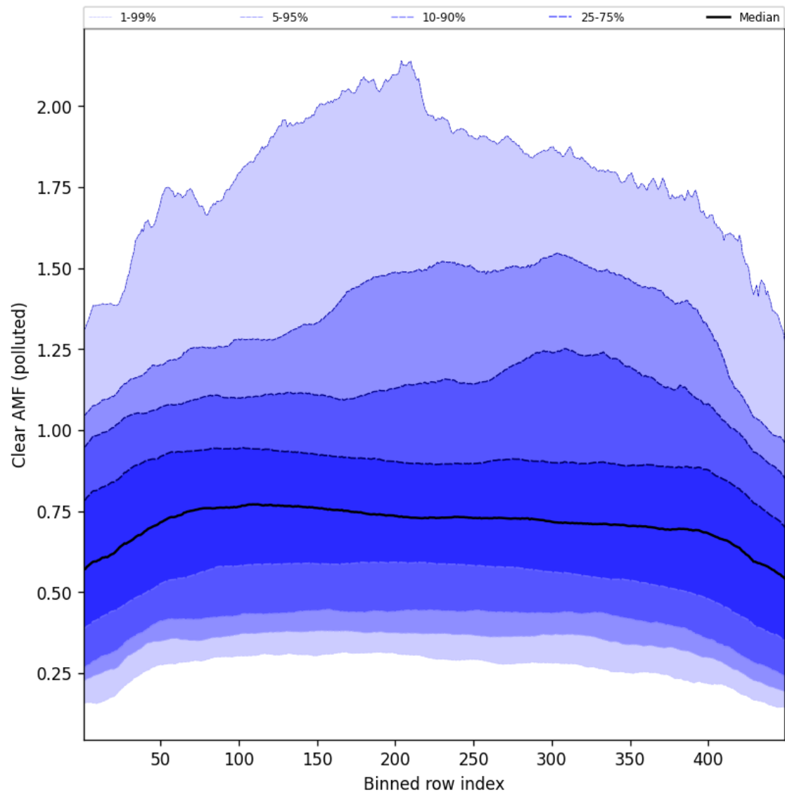
Figure 109: Along track statistics of “Clear AMF (polluted)” for 2025-07-17 to 2025-07-18
