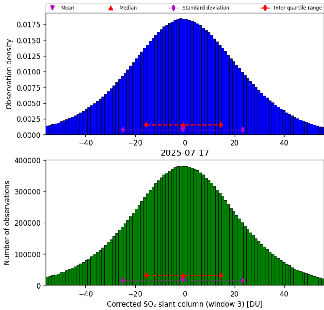
Figure 73: Histogram of “Corrected SO 2 slant column (window 3)” for 2025-07-17 to 2025-07-18
