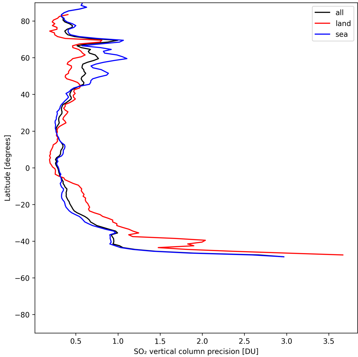
Figure 32: Zonal average of “SO 2 vertical column precision” for 2025-07-17 to 2025-07-18.
