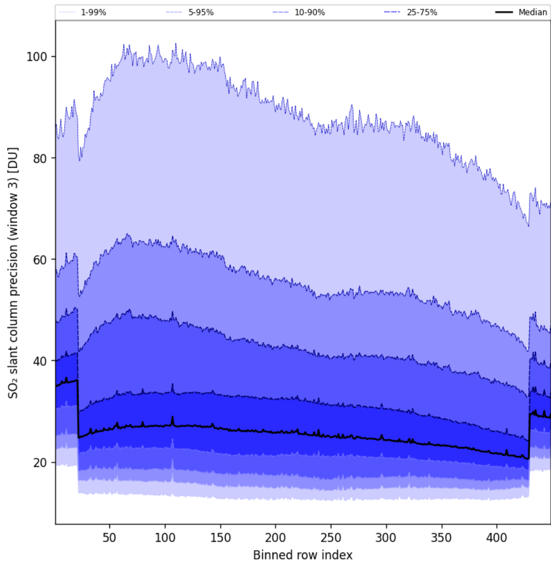
Figure 99: Along track statistics of “SO 2 slant column precision (window 3)” for 2025-07-17 to 2025-07-18
