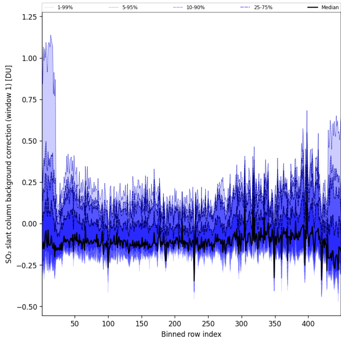
Figure 93: Along track statistics of “SO 2 slant column background correction (window 1)” for 2025-07-17 to 2025-07-18
