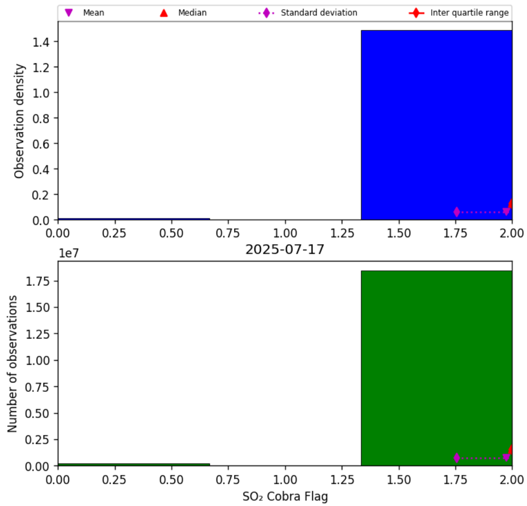
Figure 75: Histogram of “SO 2 Cobra Flag” for 2025-07-17 to 2025-07-18
