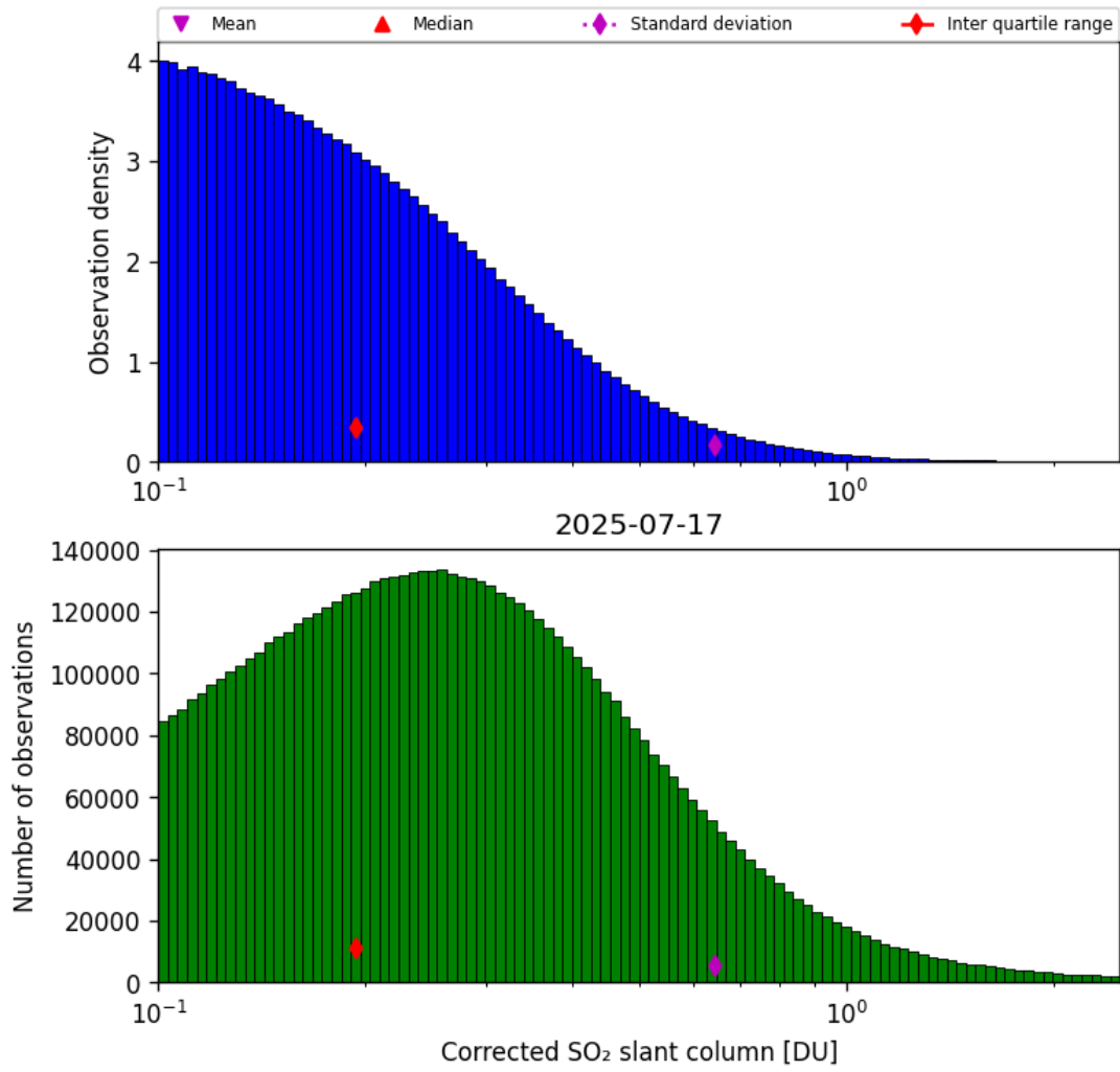
Figure 60: Histogram of “Corrected SO 2 slant column” for 2025-07-17 to 2025-07-18
