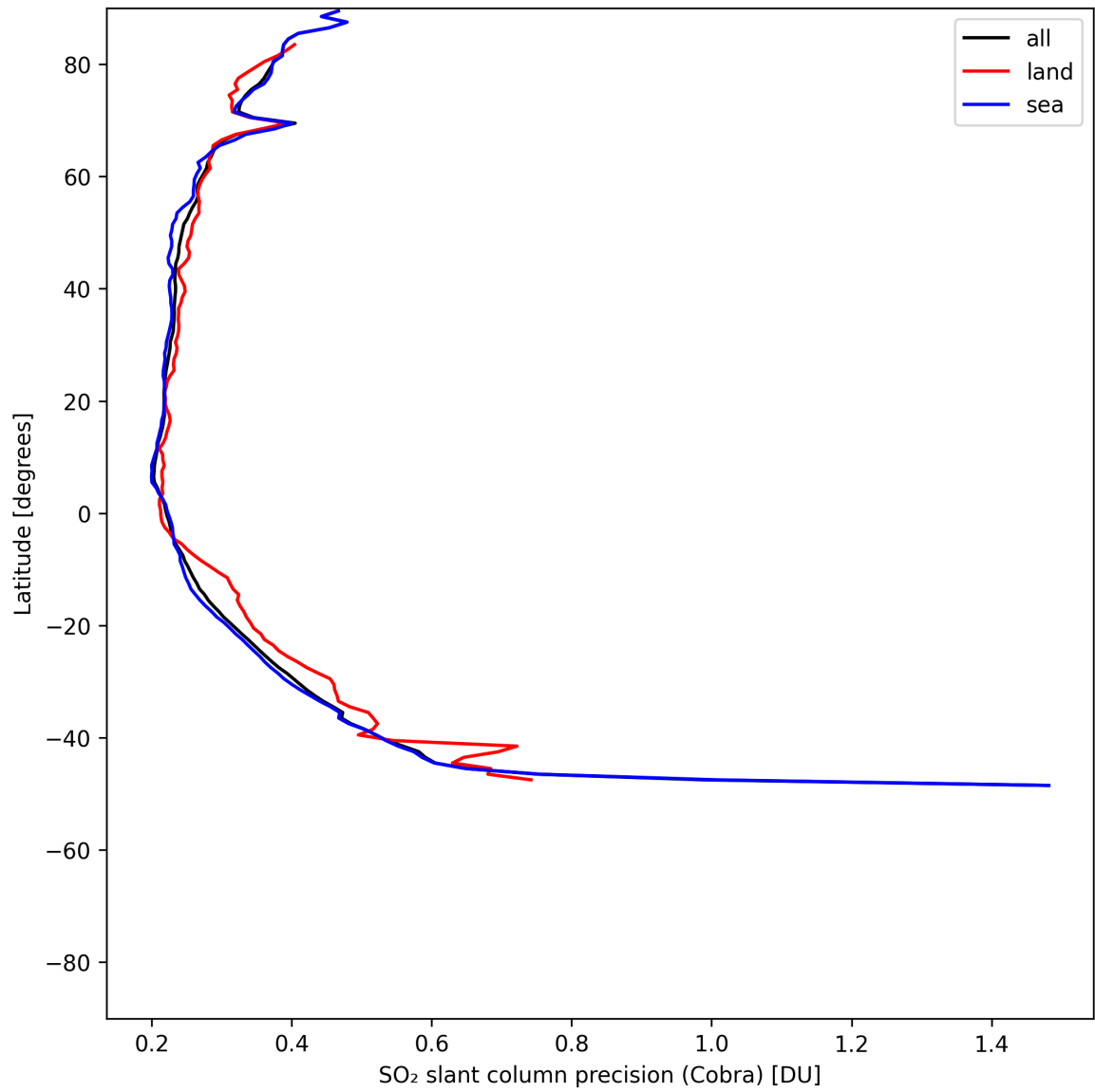
Figure 35: Zonal average of “SO 2 slant column precision (Cobra)” for 2025-07-17 to 2025-07-18.
