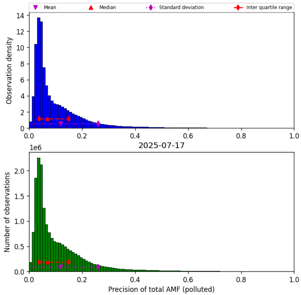
Figure 81: Histogram of “Precision of total AMF (polluted)” for 2025-07-17 to 2025-07-18
