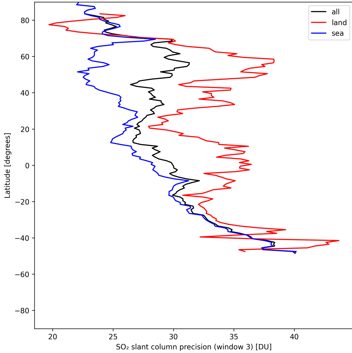
Figure 45: Zonal average of “SO 2 slant column precision (window 3)” for 2025-07-17 to 2025-07-18.
