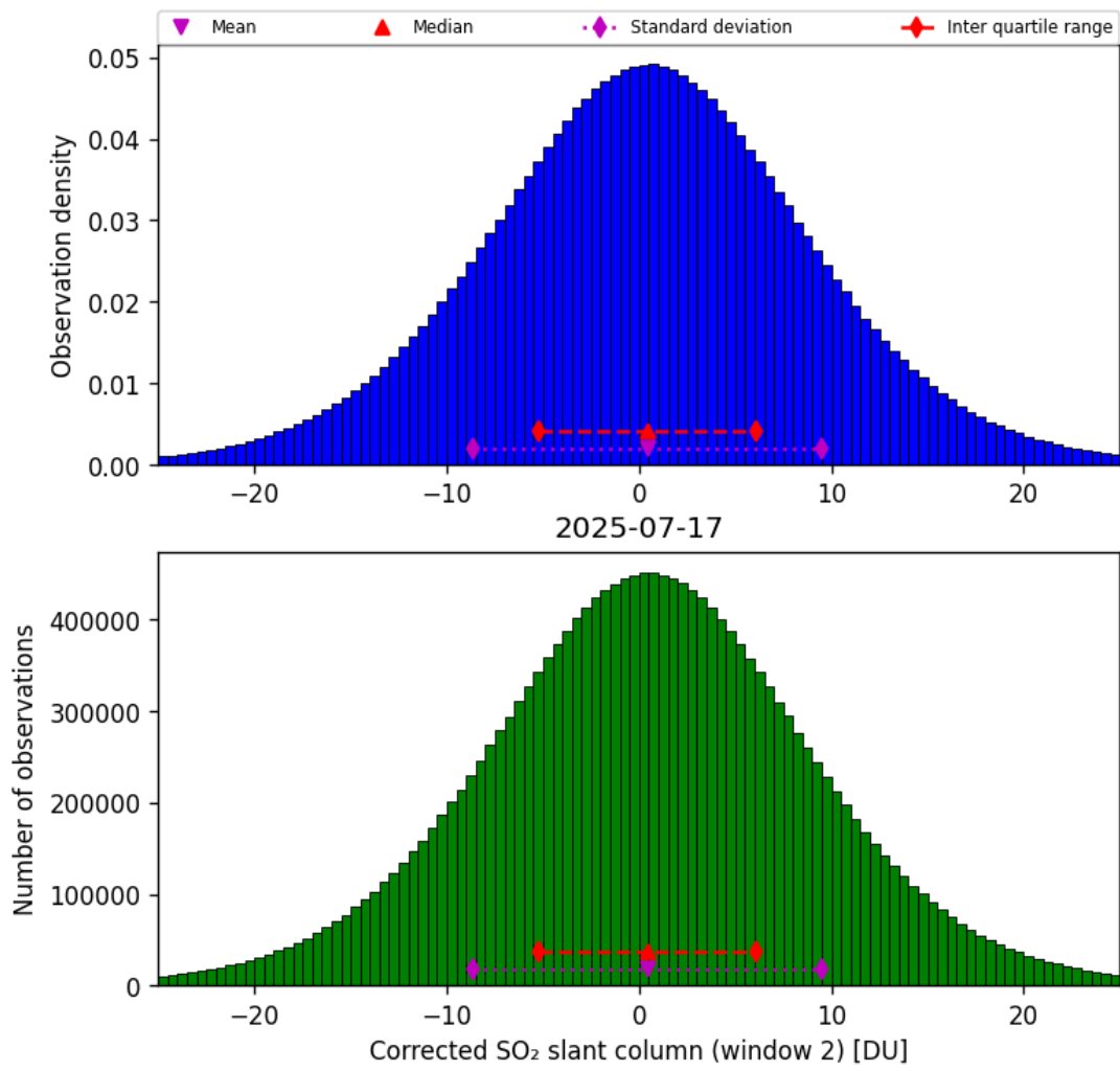
Figure 69: Histogram of “Corrected SO 2 slant column (window 2)” for 2025-07-17 to 2025-07-18
