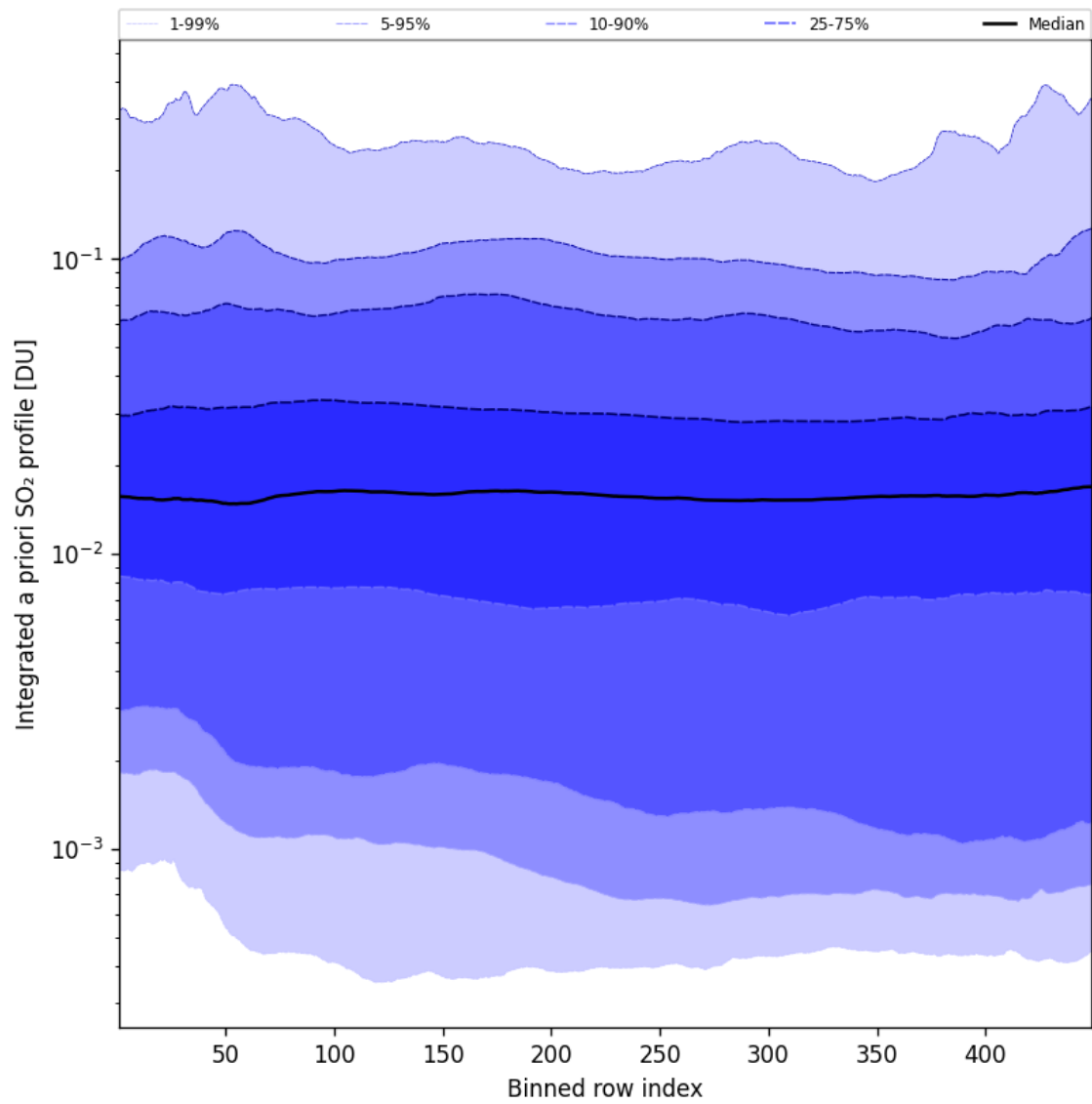
Figure 103: Along track statistics of “Integrated a priori SO 2 profile” for 2025-07-17 to 2025-07-18
