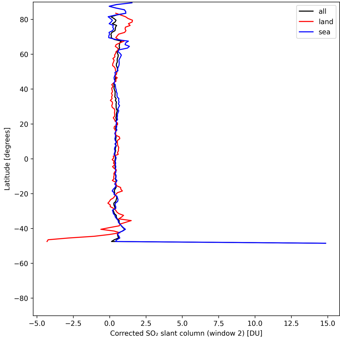
Figure 42: Zonal average of “Corrected SO 2 slant column (window 2)” for 2025-07-17 to 2025-07-18.
