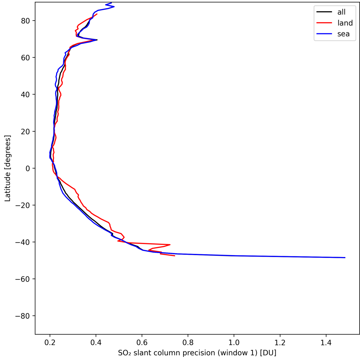
Figure 37: Zonal average of “SO 2 slant column precision (window 1)” for 2025-07-17 to 2025-07-18.
