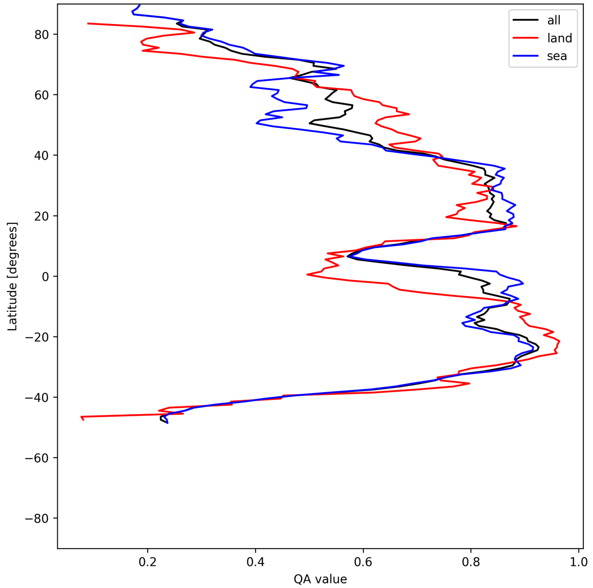
Figure 30: Zonal average of “QA value” for 2025-07-17 to 2025-07-18.
