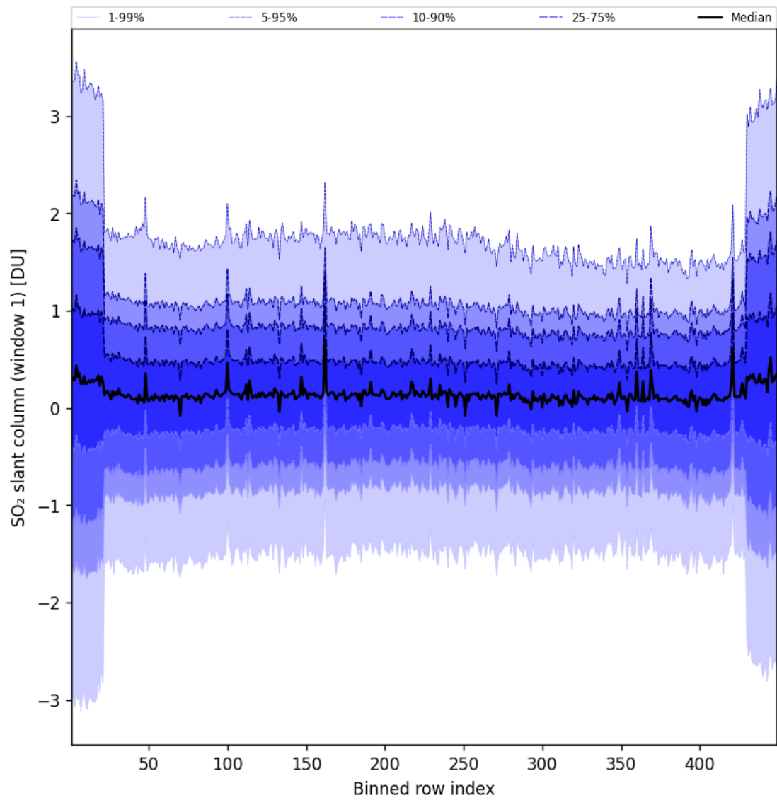
Figure 90: Along track statistics of “SO 2 slant column (window 1)” for 2025-07-17 to 2025-07-18
