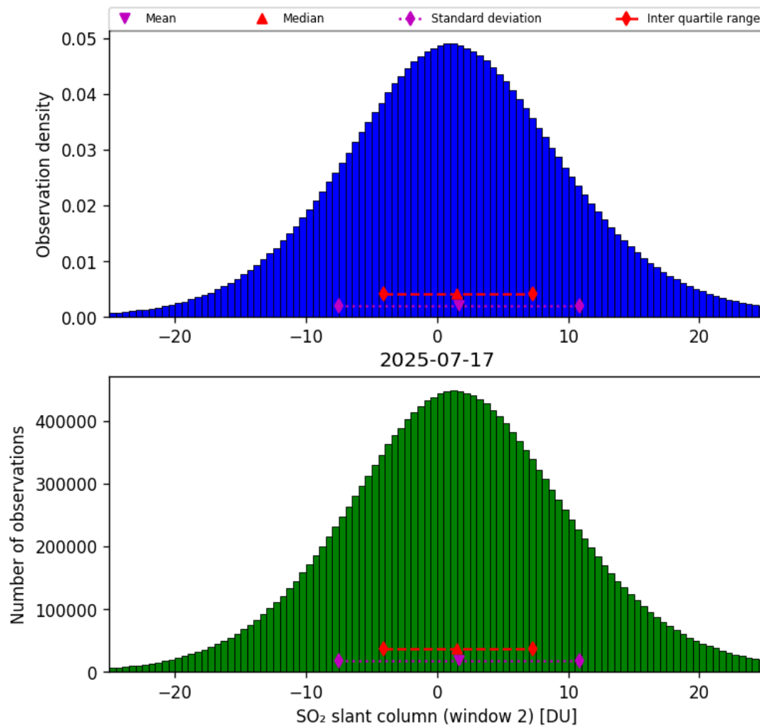
Figure 67: Histogram of “SO 2 slant column (window 2)” for 2025-07-17 to 2025-07-18
