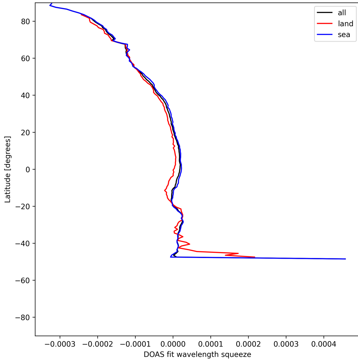
Figure 51: Zonal average of “DOAS fit wavelength squeeze” for 2025-07-17 to 2025-07-18.
