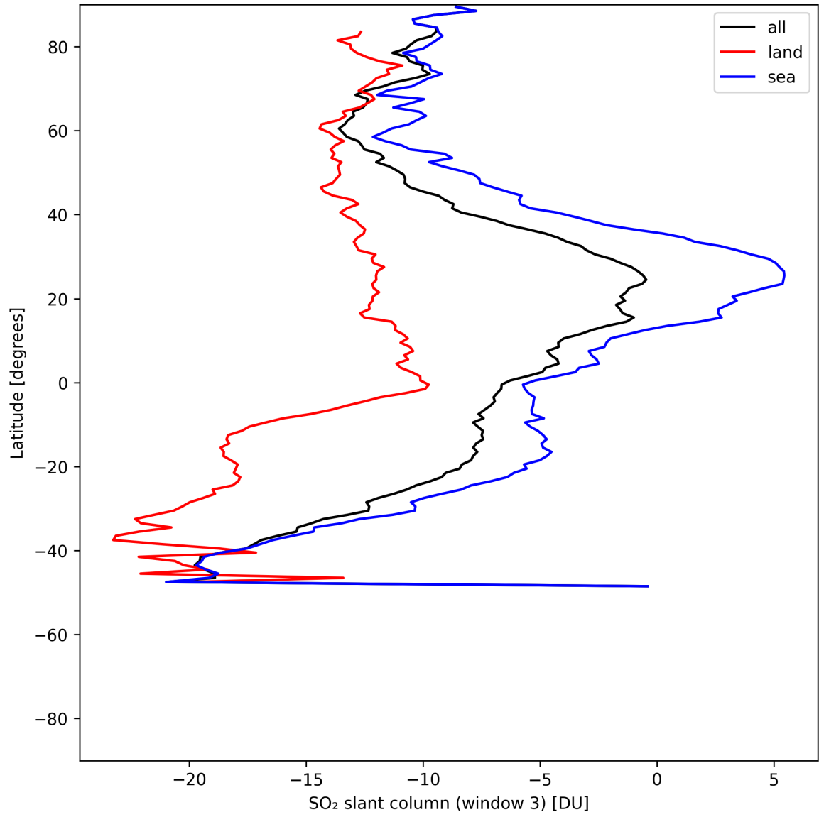
Figure 44: Zonal average of “SO 2 slant column (window 3)” for 2025-07-17 to 2025-07-18.
