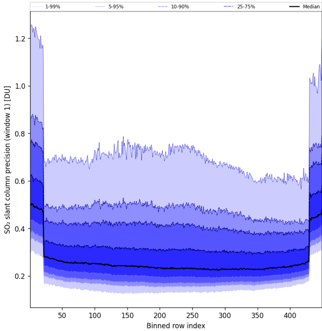
Figure 91: Along track statistics of “SO 2 slant column precision (window 1)” for 2025-07-17 to 2025-07-18
