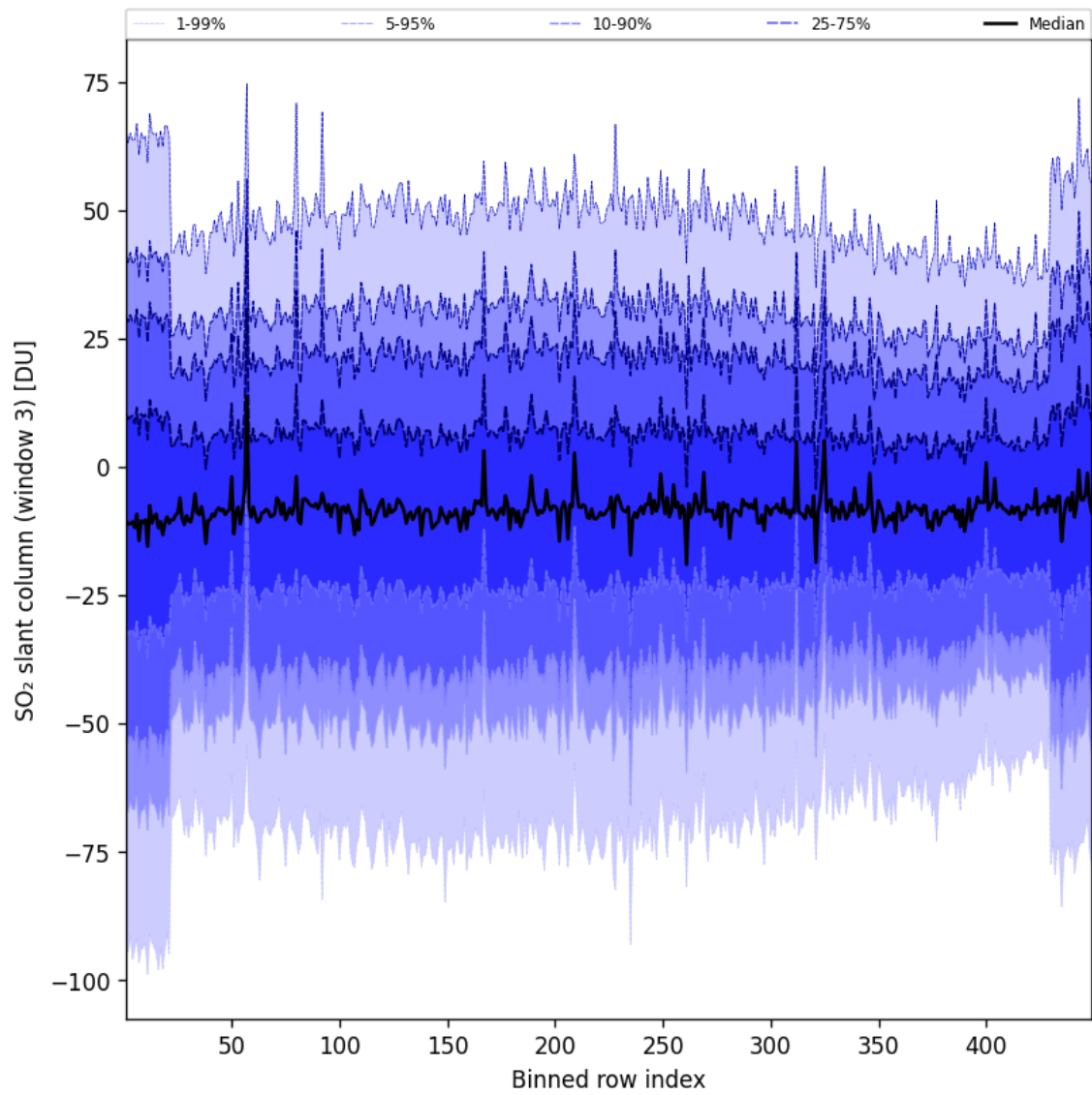
Figure 98: Along track statistics of “SO 2 slant column (window 3)” for 2025-07-17 to 2025-07-18
