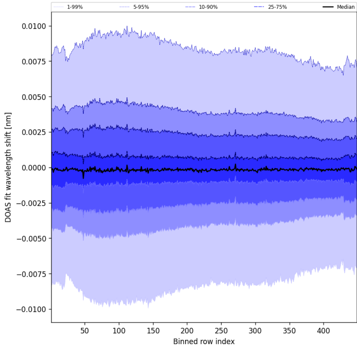
Figure 104: Along track statistics of “DOAS fit wavelength shift” for 2025-07-17 to 2025-07-18
