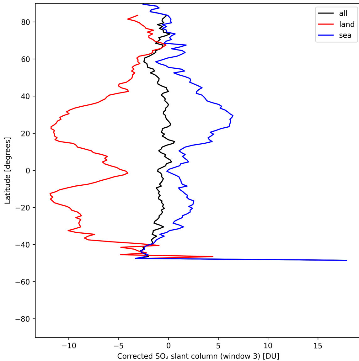
Figure 46: Zonal average of “Corrected SO 2 slant column (window 3)” for 2025-07-17 to 2025-07-18.
