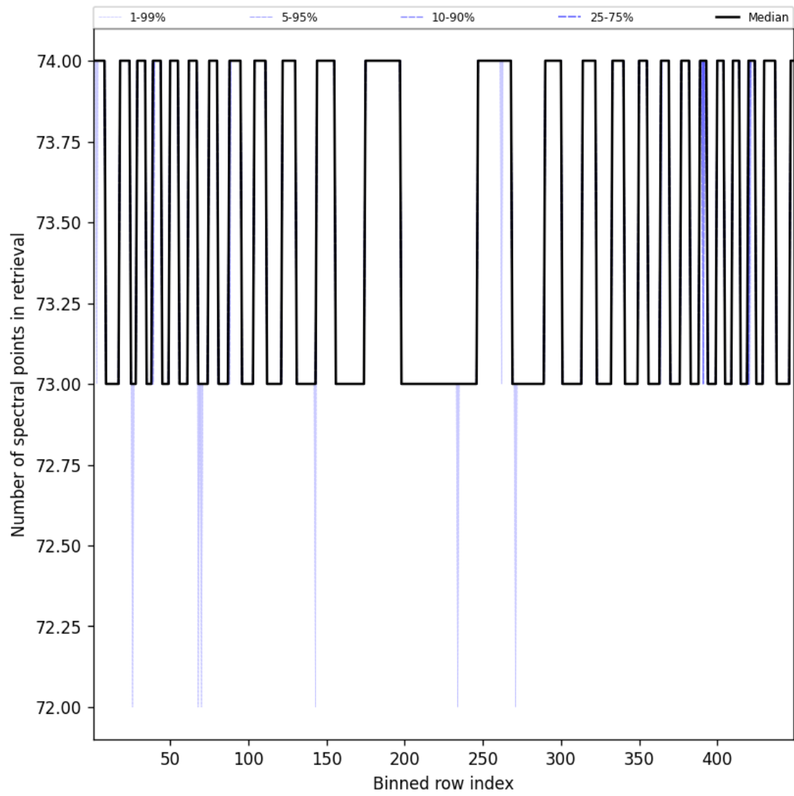
Figure 110: Along track statistics of “Number of spectral points in retrieval” for 2025-07-17 to 2025-07-18
