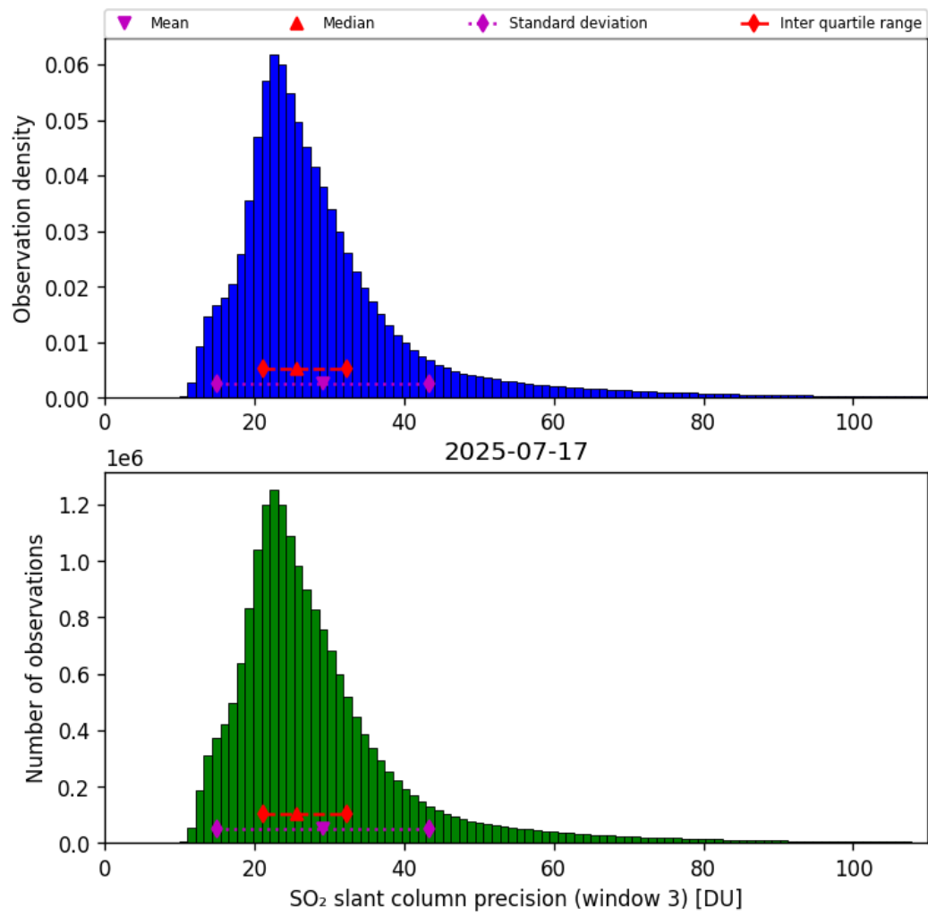
Figure 72: Histogram of “SO 2 slant column precision (window 3)” for 2025-07-17 to 2025-07-18
