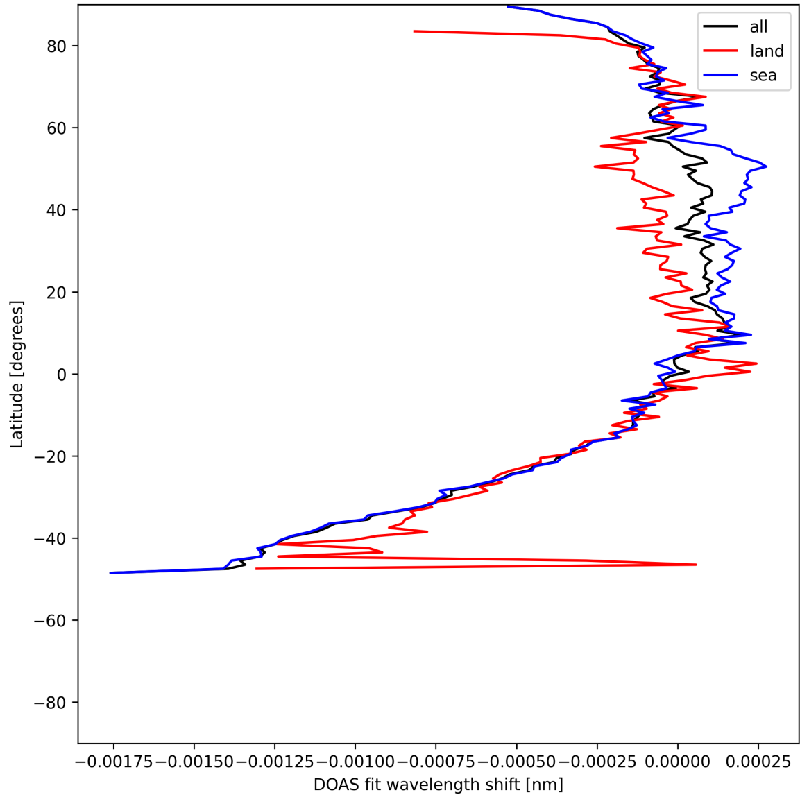
Figure 50: Zonal average of “DOAS fit wavelength shift” for 2025-07-17 to 2025-07-18.
