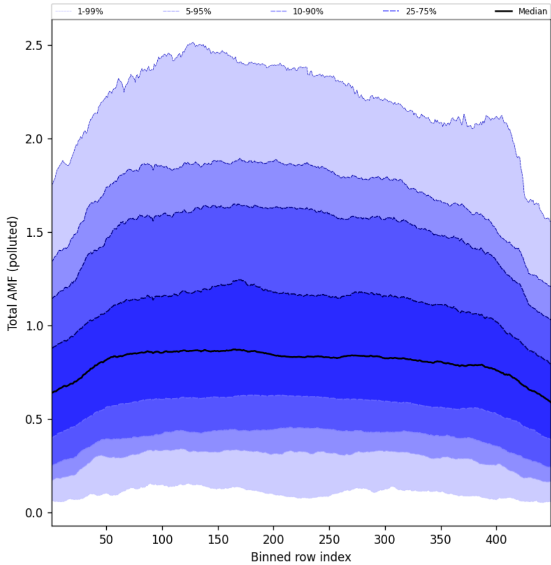
Figure 107: Along track statistics of “Total AMF (polluted)” for 2025-07-17 to 2025-07-18
