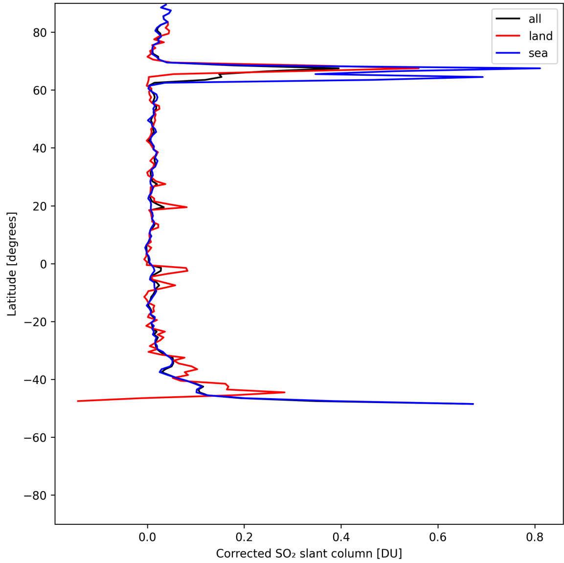
Figure 33: Zonal average of “Corrected SO 2 slant column” for 2025-07-17 to 2025-07-18.
