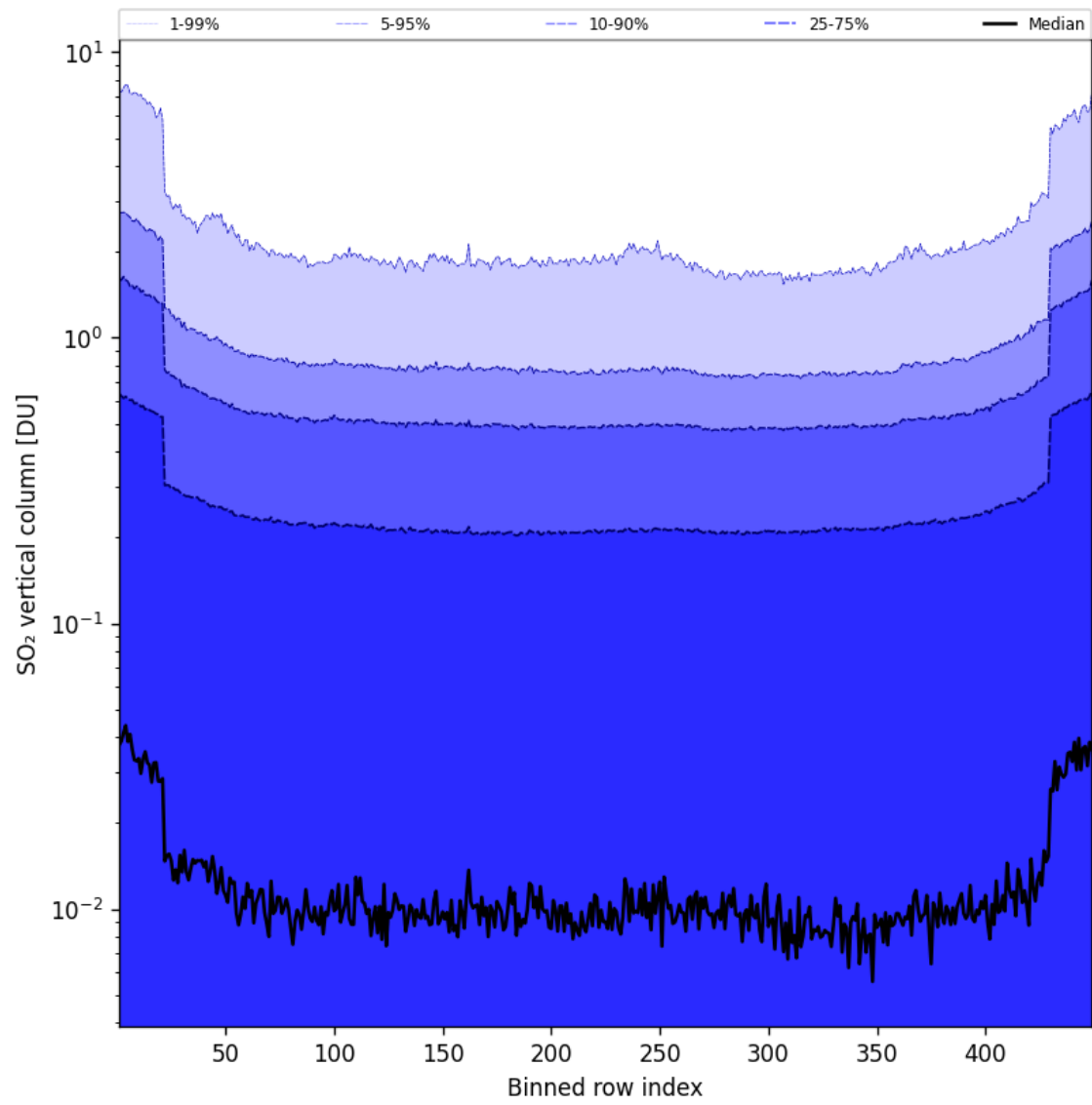
Figure 85: Along track statistics of “SO 2 vertical column” for 2025-07-17 to 2025-07-18
