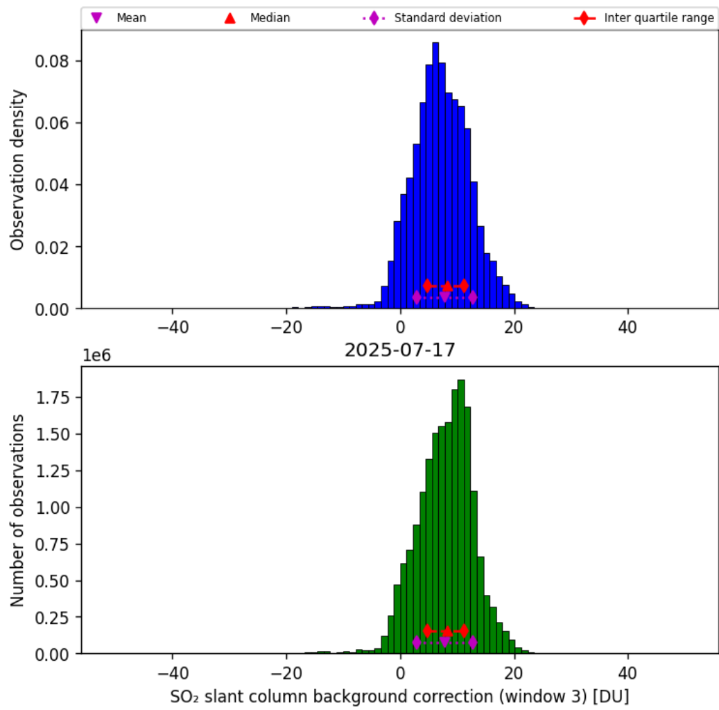
Figure 74: Histogram of “SO 2 slant column background correction (window 3)” for 2025-07-17 to 2025-07-18
