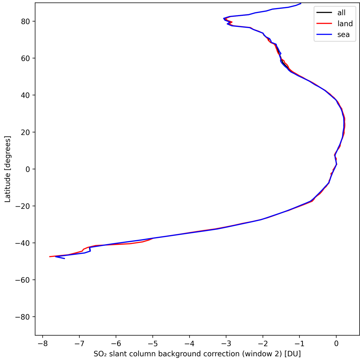
Figure 43: Zonal average of “SO 2 slant column background correction (window 2)” for 2025-07-17 to 2025-07-18.
