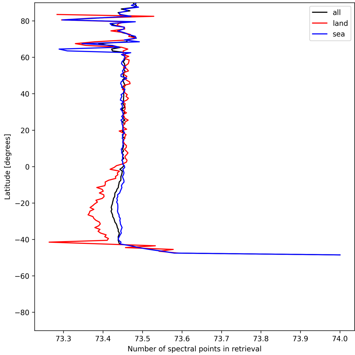
Figure 56: Zonal average of “Number of spectral points in retrieval” for 2025-07-17 to 2025-07-18.
