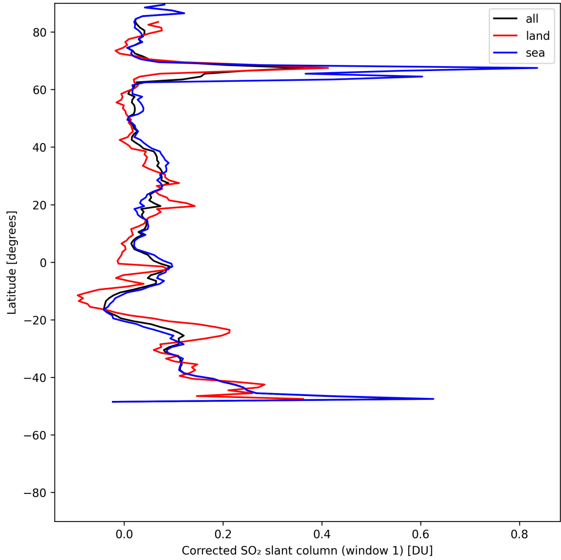
Figure 38: Zonal average of "Corrected SO 2 slant column (window 1)" for 2025-07-17 to 2025-07-18.
