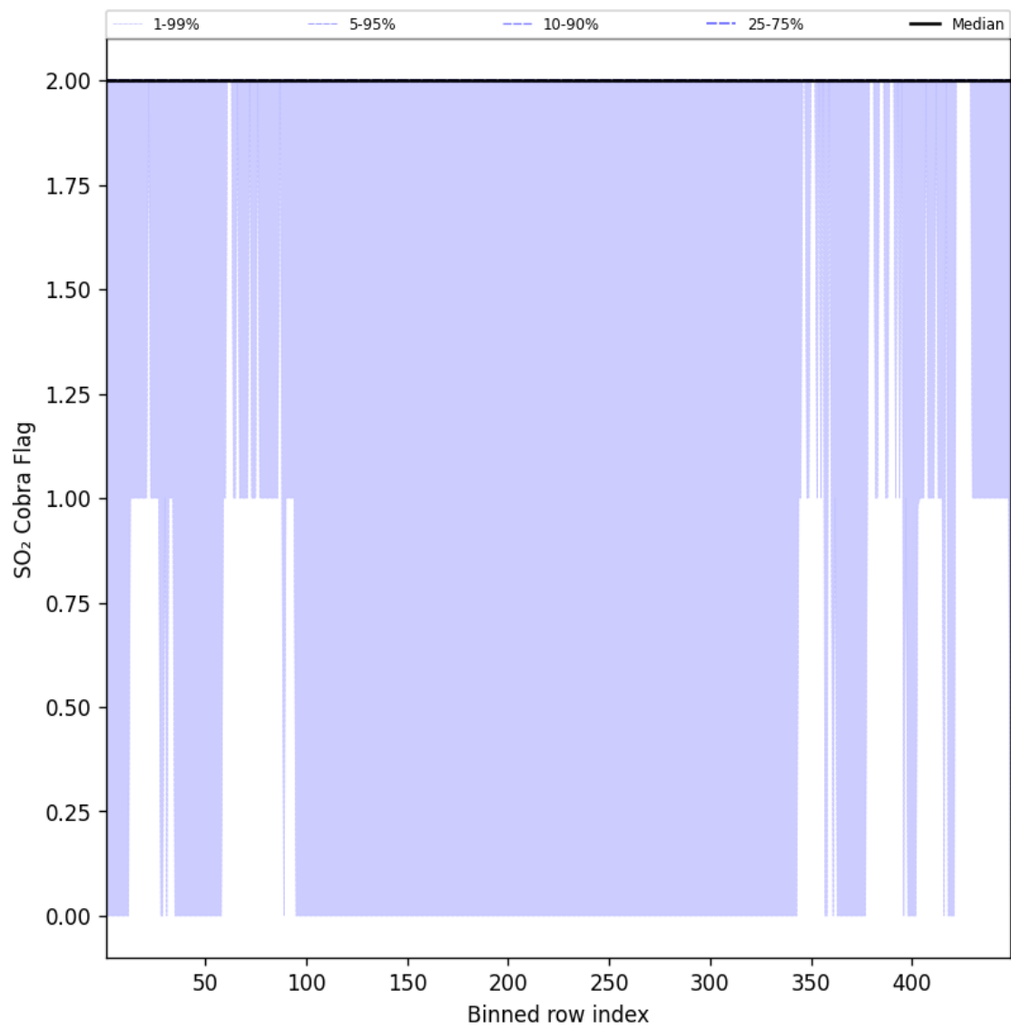
Figure 102: Along track statistics of “SO 2 Cobra Flag” for 2025-07-17 to 2025-07-18
