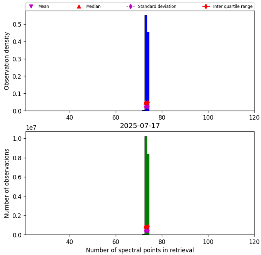
Figure 83: Histogram of “Number of spectral points in retrieval” for 2025-07-17 to 2025-07-18
