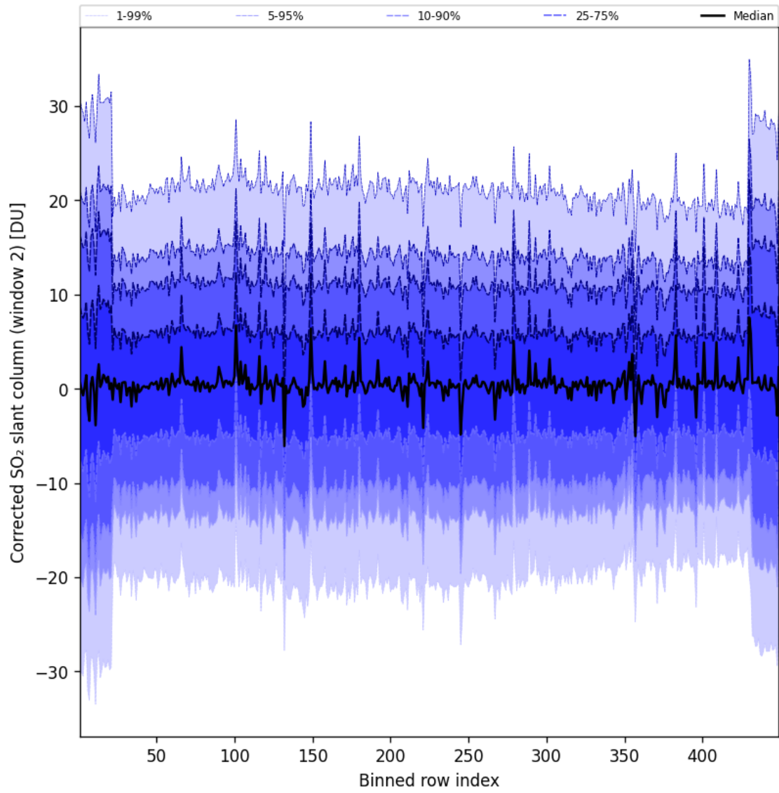
Figure 96: Along track statistics of "Corrected SO 2 slant column (window 2)" for 2025-07-17 to 2025-07-18
