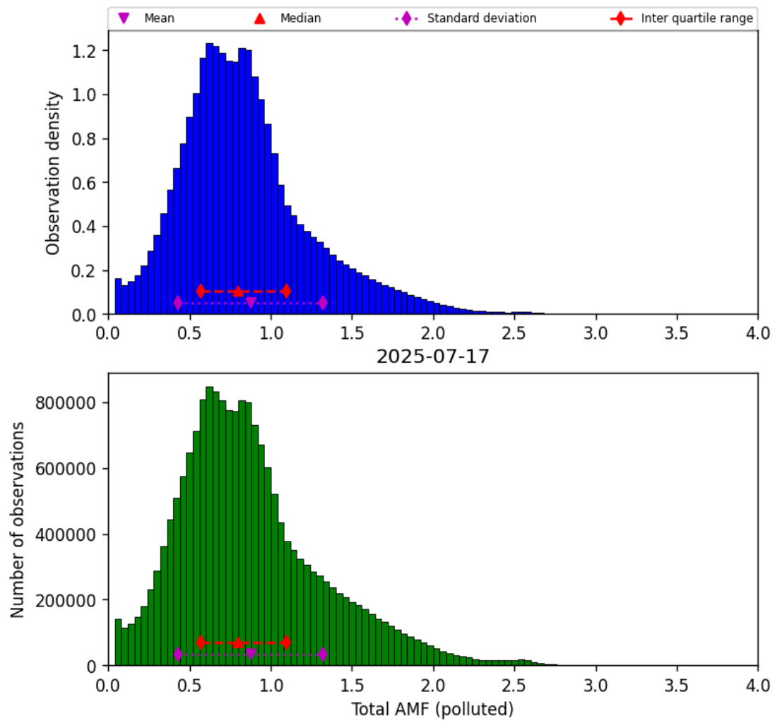
Figure 80: Histogram of “Total AMF (polluted)” for 2025-07-17 to 2025-07-18
