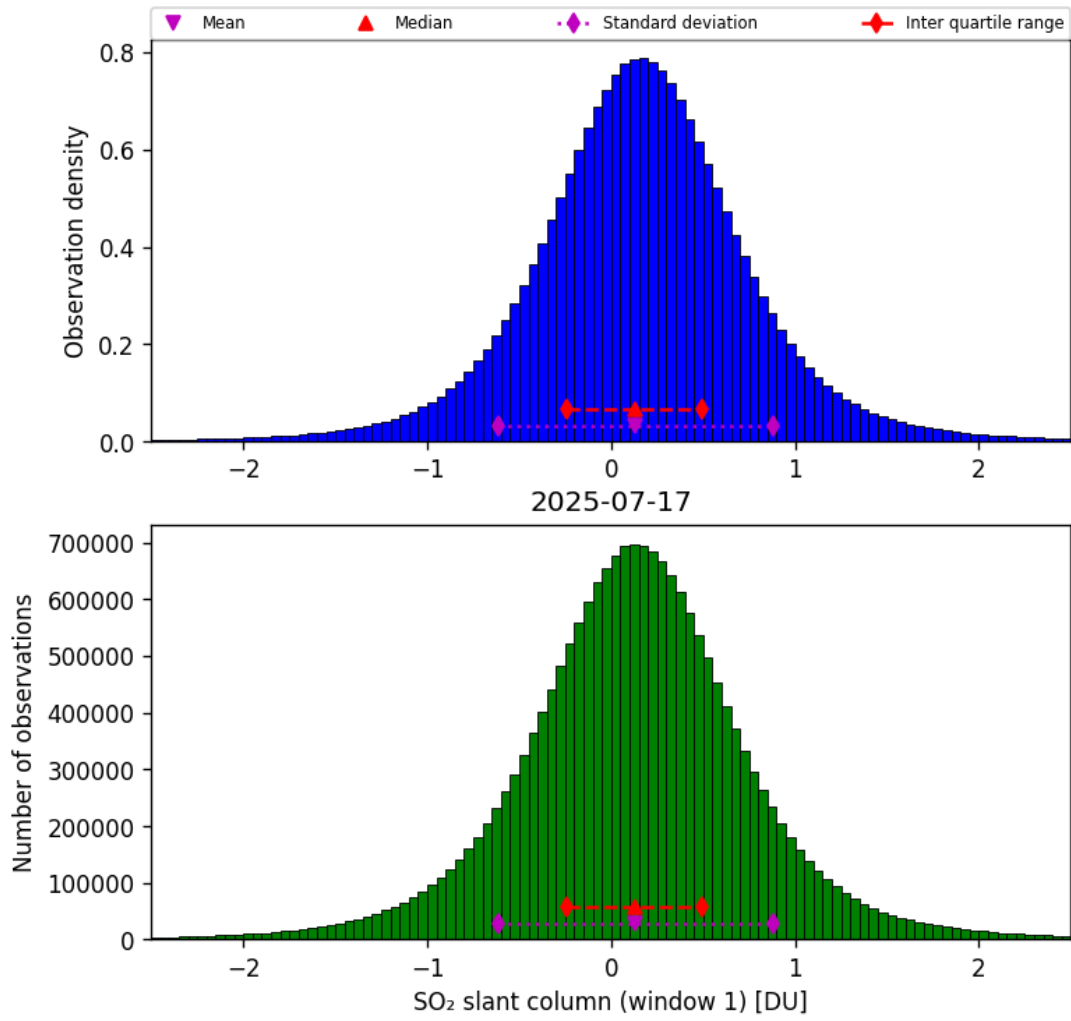
Figure 63: Histogram of “SO 2 slant column (window 1)” for 2025-07-17 to 2025-07-18
