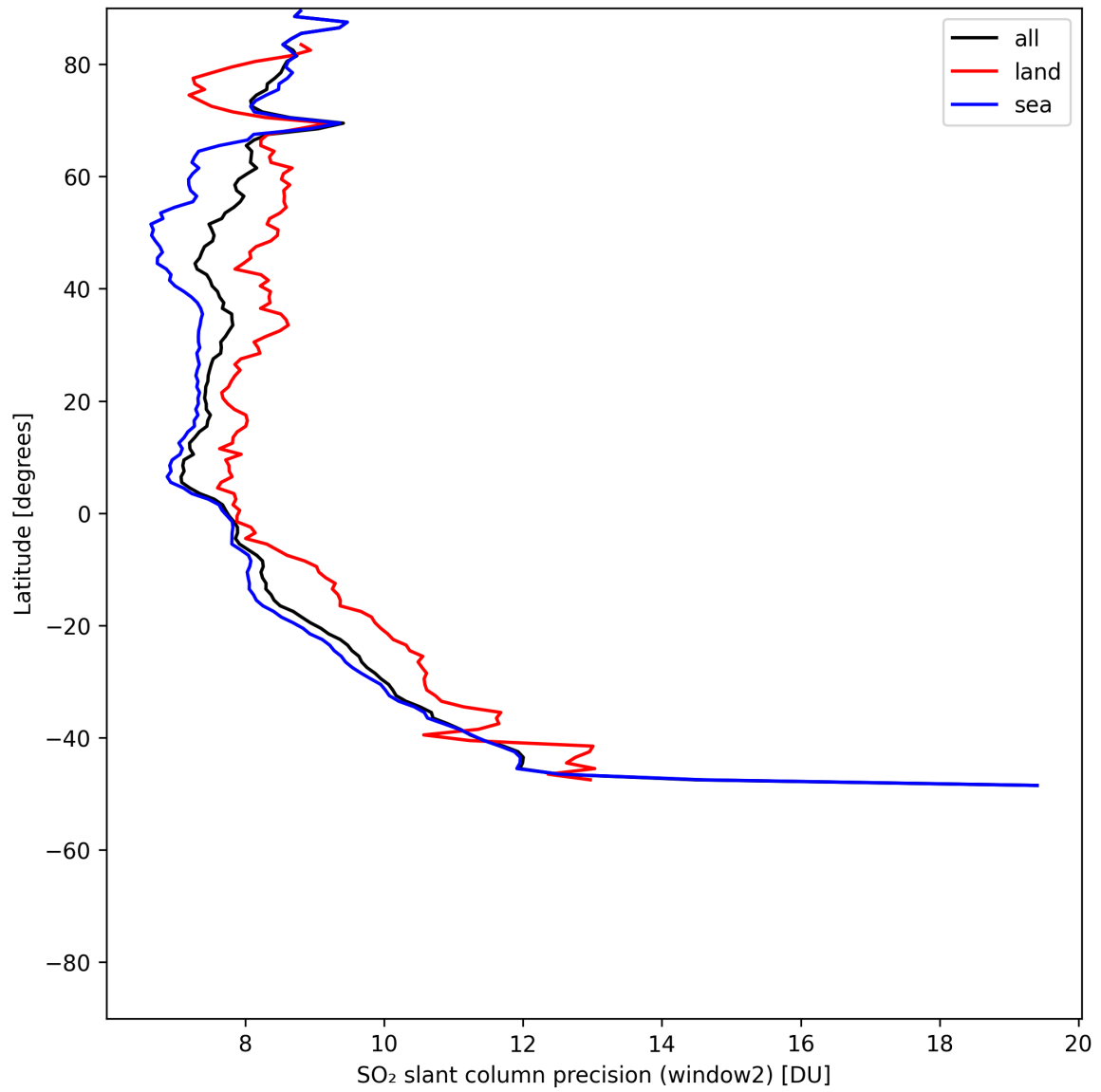
Figure 41: Zonal average of “SO 2 slant column precision (window2)” for 2025-07-17 to 2025-07-18.
