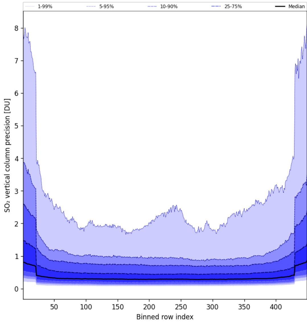
Figure 86: Along track statistics of “SO 2 vertical column precision” for 2025-07-17 to 2025-07-18
