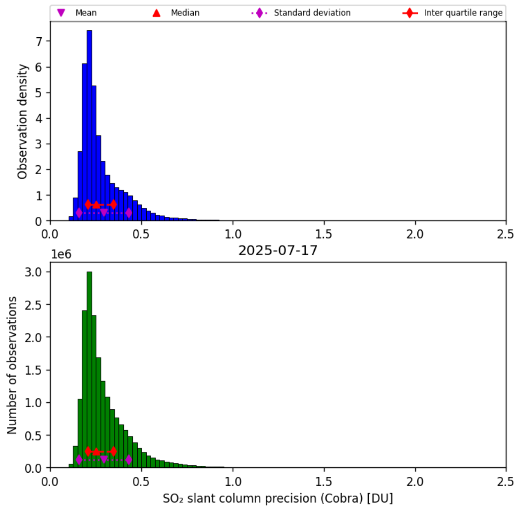
Figure 62: Histogram of “SO 2 slant column precision (Cobra)” for 2025-07-17 to 2025-07-18
