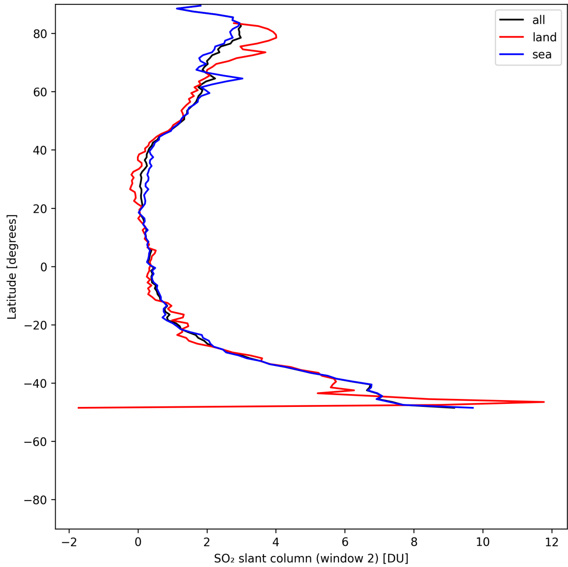
Figure 40: Zonal average of “SO 2 slant column (window 2)” for 2025-07-18 to 2025-07-19.
