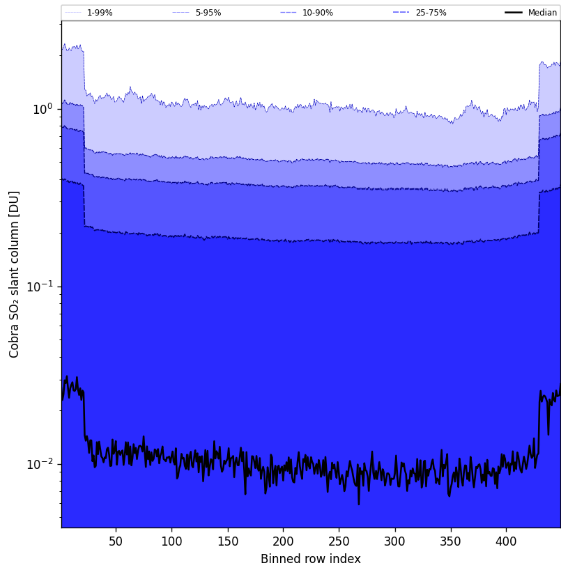
Figure 88: Along track statistics of “Cobra SO 2 slant column” for 2025-07-18 to 2025-07-19
