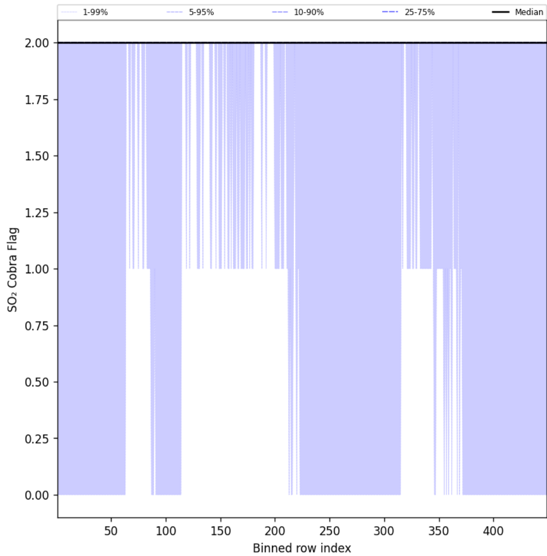
Figure 102: Along track statistics of “SO 2 Cobra Flag” for 2025-07-18 to 2025-07-19
