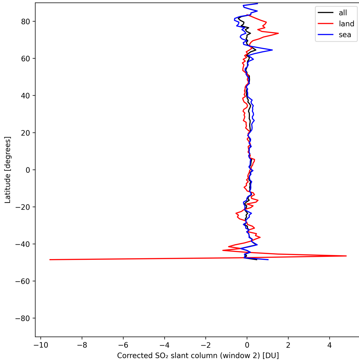
Figure 42: Zonal average of “Corrected SO 2 slant column (window 2)” for 2025-07-18 to 2025-07-19.
