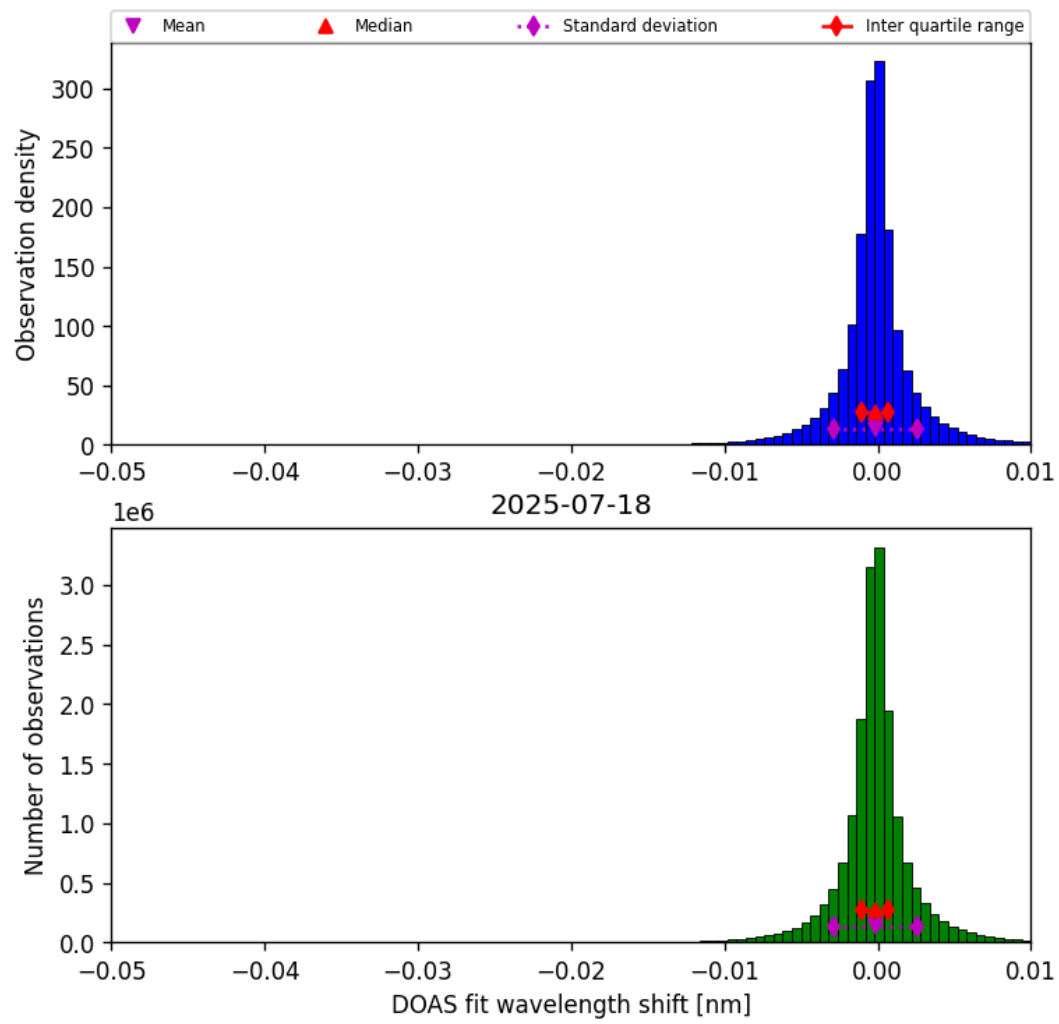
Figure 77: Histogram of “DOAS fit wavelength shift” for 2025-07-18 to 2025-07-19
