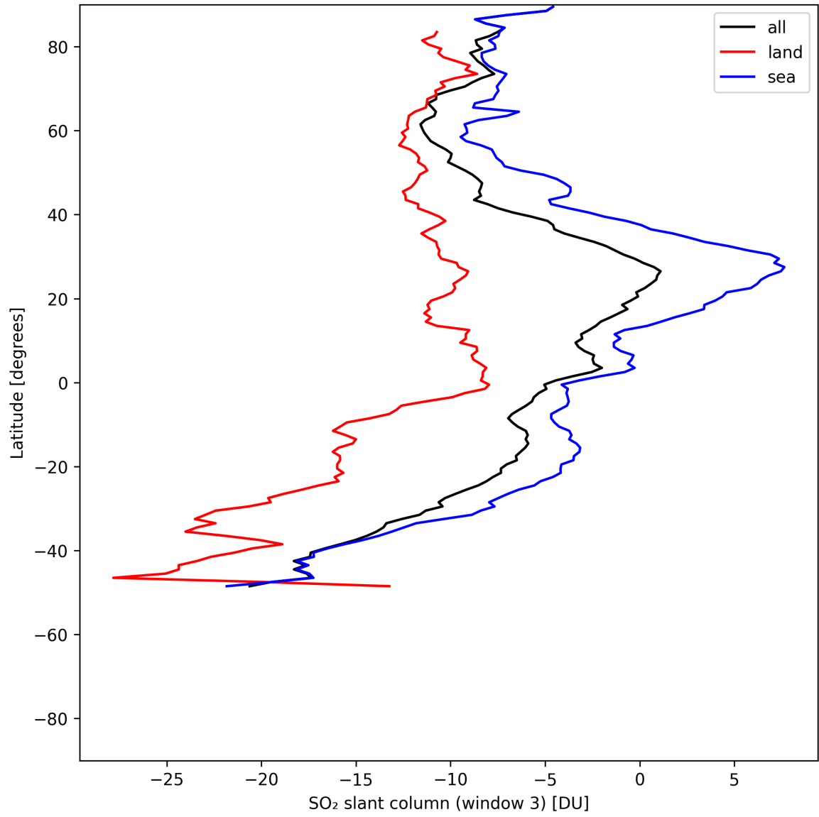
Figure 44: Zonal average of “SO 2 slant column (window 3)” for 2025-07-18 to 2025-07-19.
