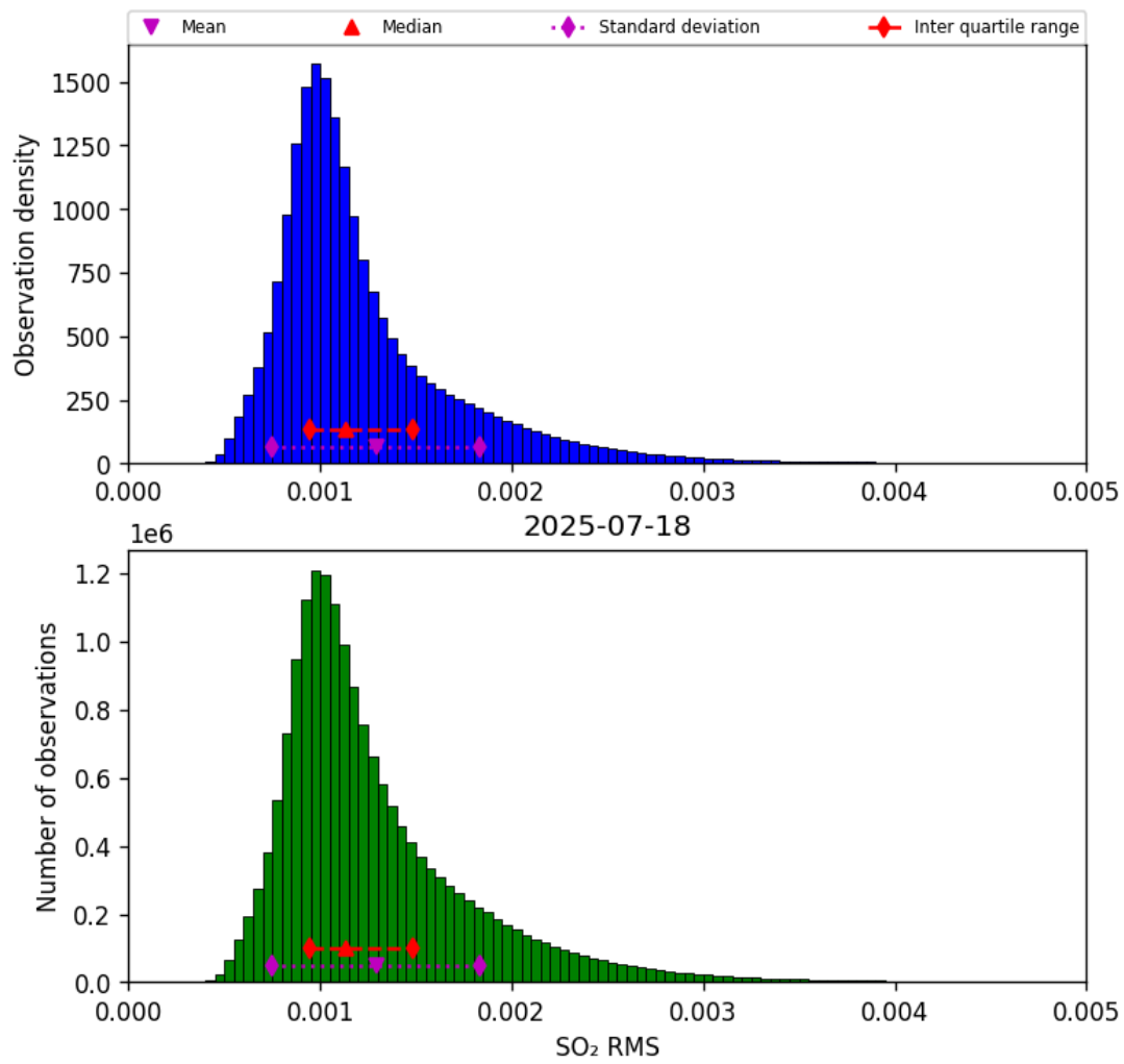
Figure 79: Histogram of “SO 2 RMS” for 2025-07-18 to 2025-07-19
