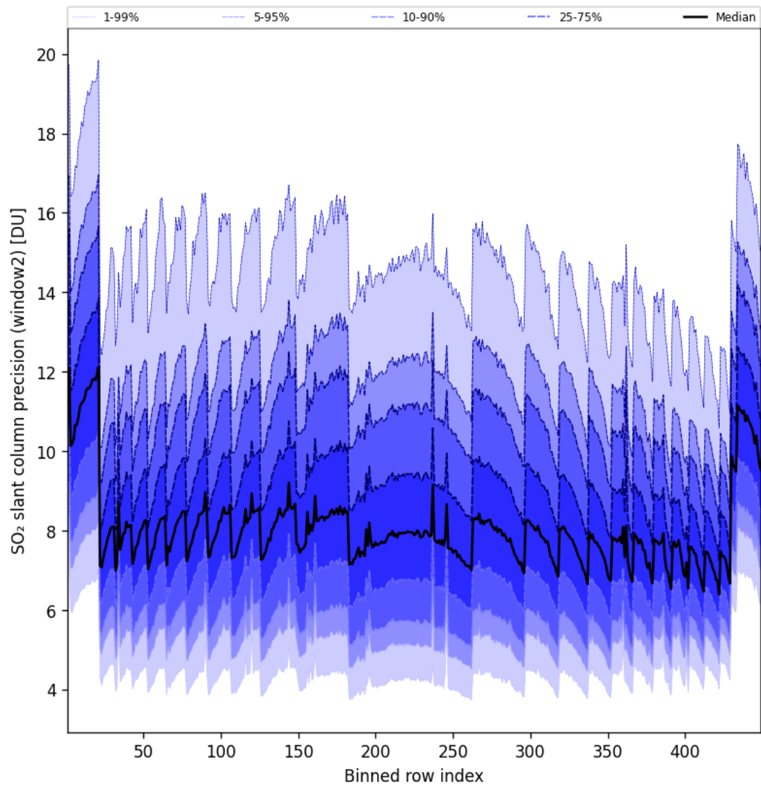
Figure 95: Along track statistics of “SO 2 slant column precision (window2)” for 2025-07-18 to 2025-07-19
