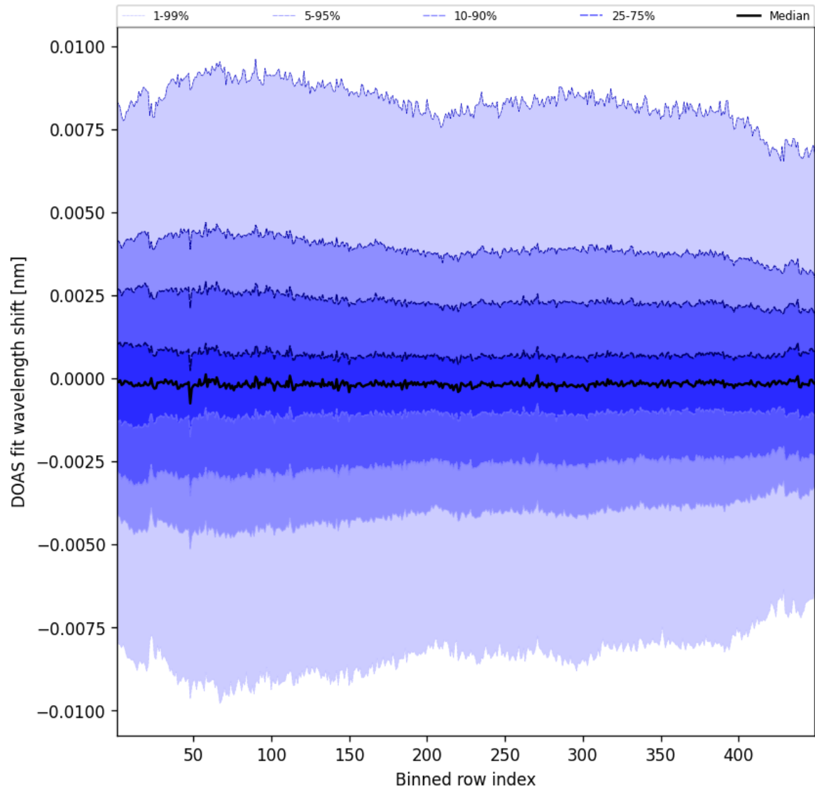
Figure 104: Along track statistics of “DOAS fit wavelength shift” for 2025-07-18 to 2025-07-19
