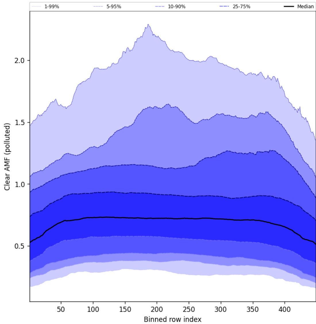
Figure 109: Along track statistics of “Clear AMF (polluted)” for 2025-07-18 to 2025-07-19
