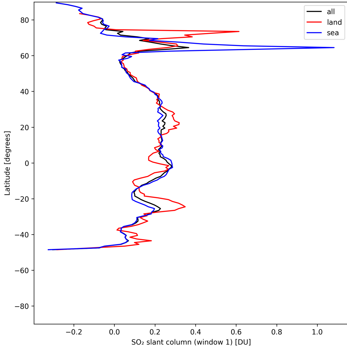
Figure 36: Zonal average of “SO 2 slant column (window 1)” for 2025-07-18 to 2025-07-19.
