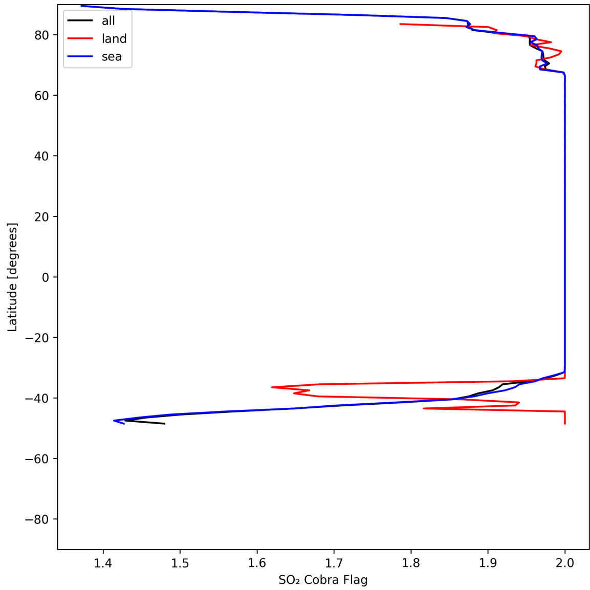
Figure 48: Zonal average of "SO 2 Cobra Flag" for 2025-07-18 to 2025-07-19.
