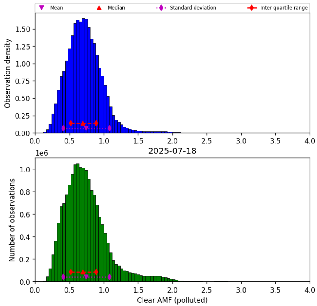
Figure 82: Histogram of "Clear AMF (polluted)" for 2025-07-18 to 2025-07-19
