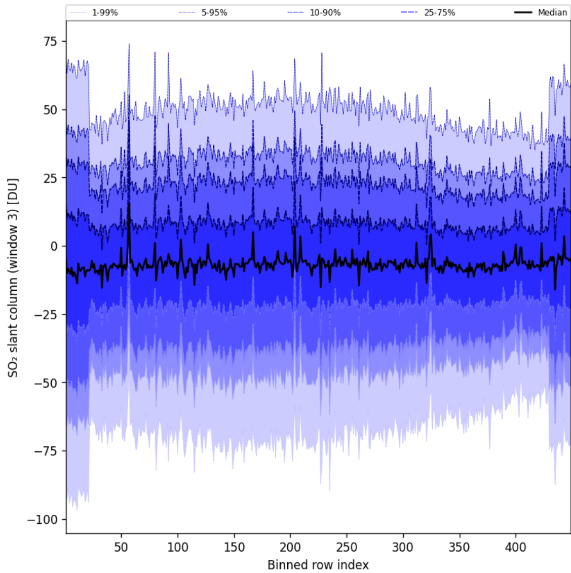
Figure 98: Along track statistics of “SO 2 slant column (window 3)” for 2025-07-18 to 2025-07-19
