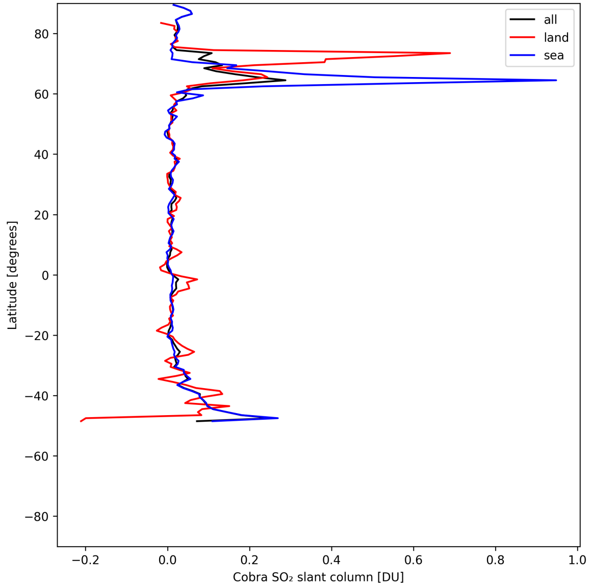
Figure 34: Zonal average of “Cobra SO 2 slant column” for 2025-07-18 to 2025-07-19.
