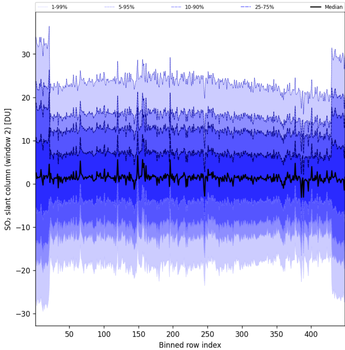
Figure 94: Along track statistics of “SO 2 slant column (window 2)” for 2025-07-18 to 2025-07-19
