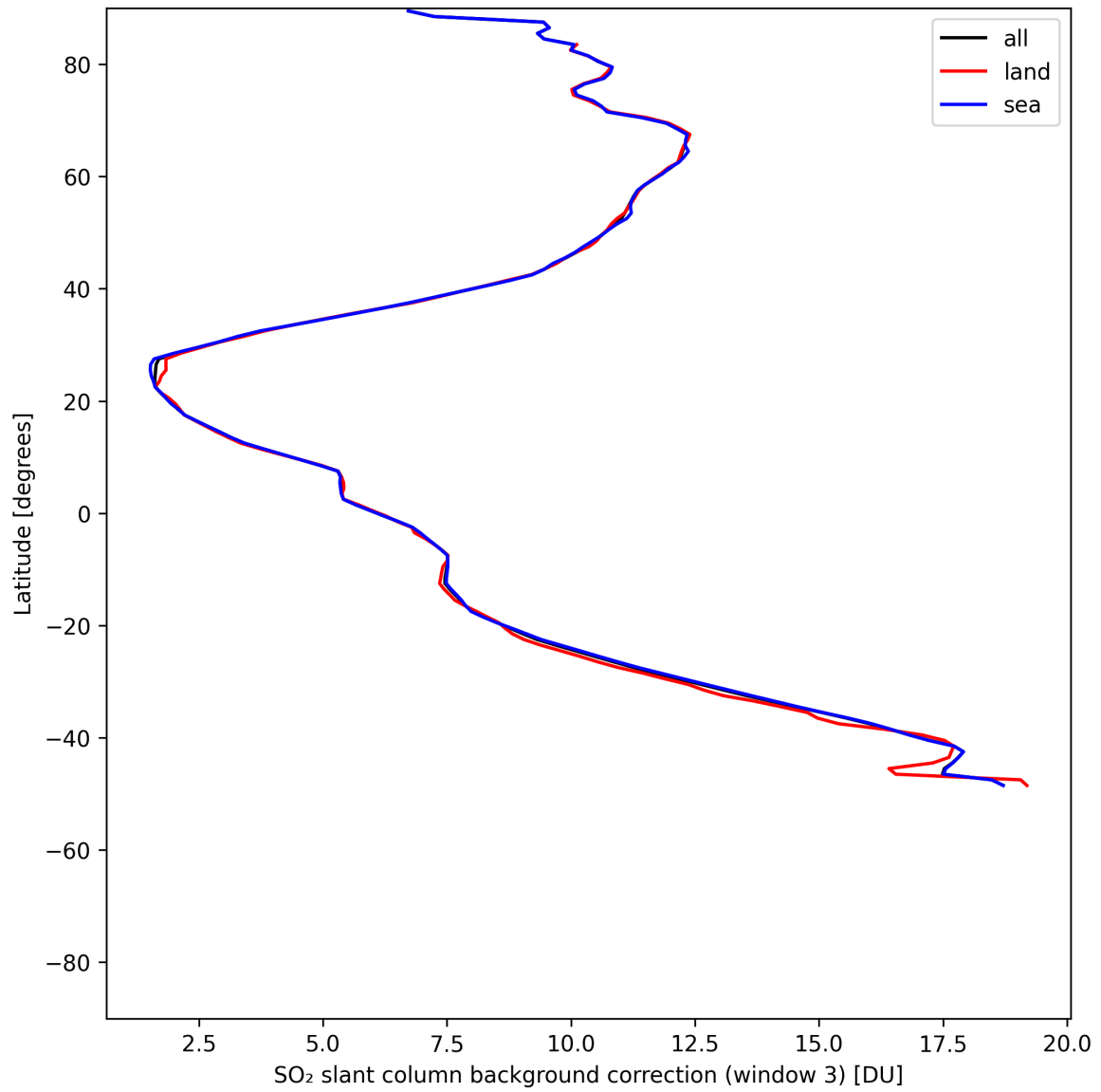
Figure 47: Zonal average of “SO 2 slant column background correction (window 3)” for 2025-07-18 to 2025-07-19.
