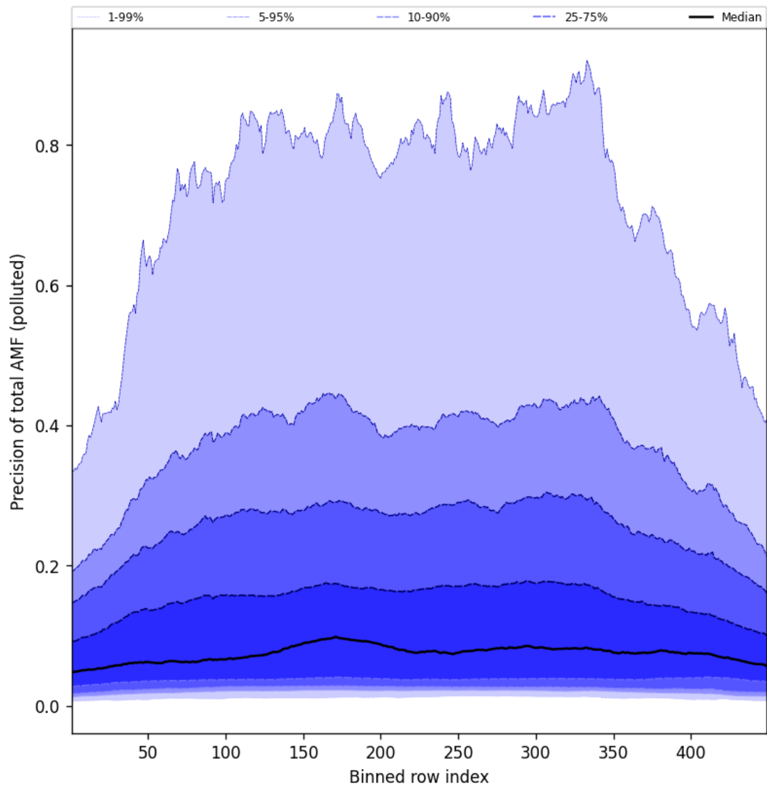
Figure 108: Along track statistics of “Precision of total AMF (polluted)” for 2025-07-18 to 2025-07-19
