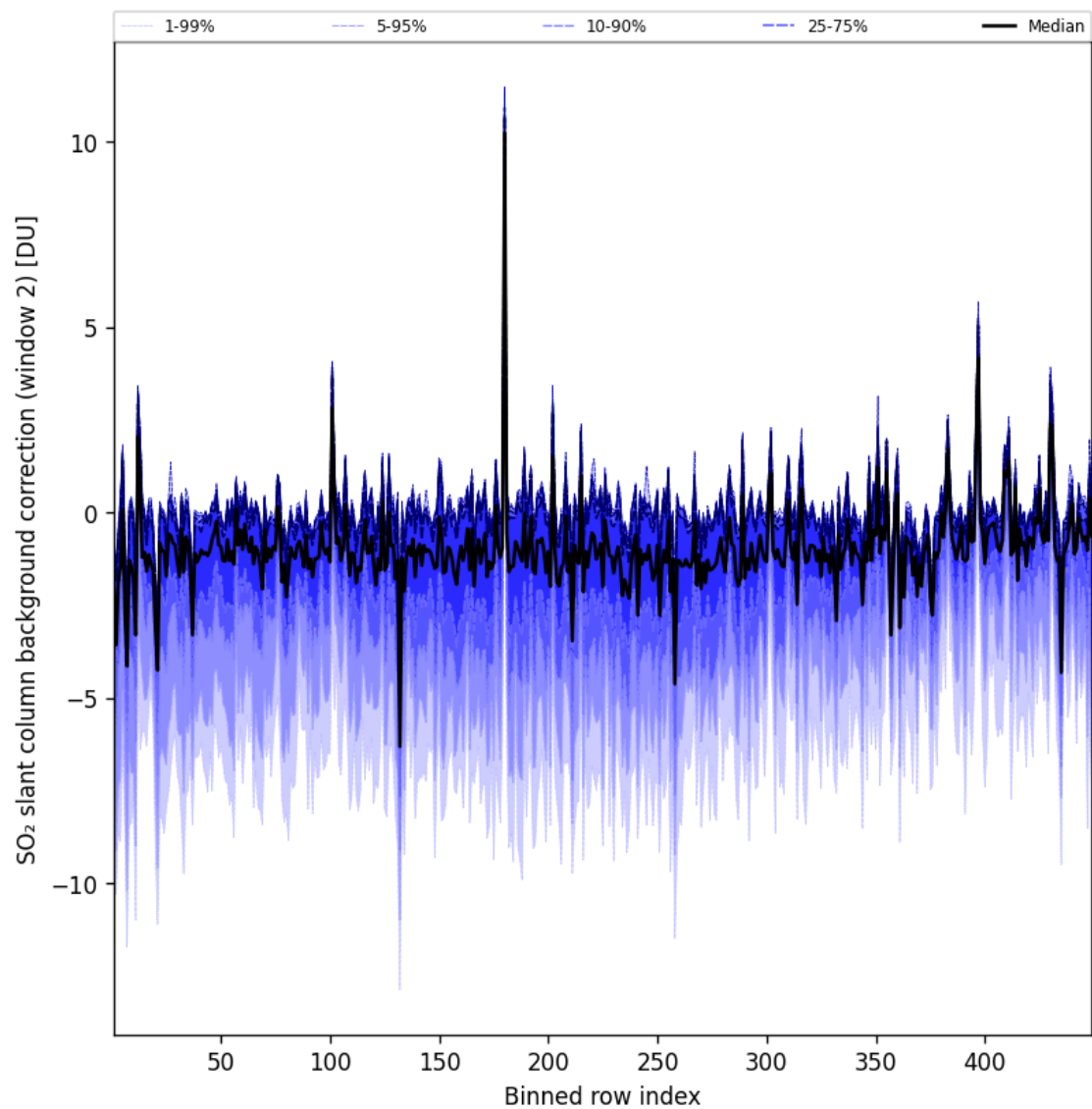
Figure 97: Along track statistics of “SO 2 slant column background correction (window 2)” for 2025-07-18 to 2025-07-19
