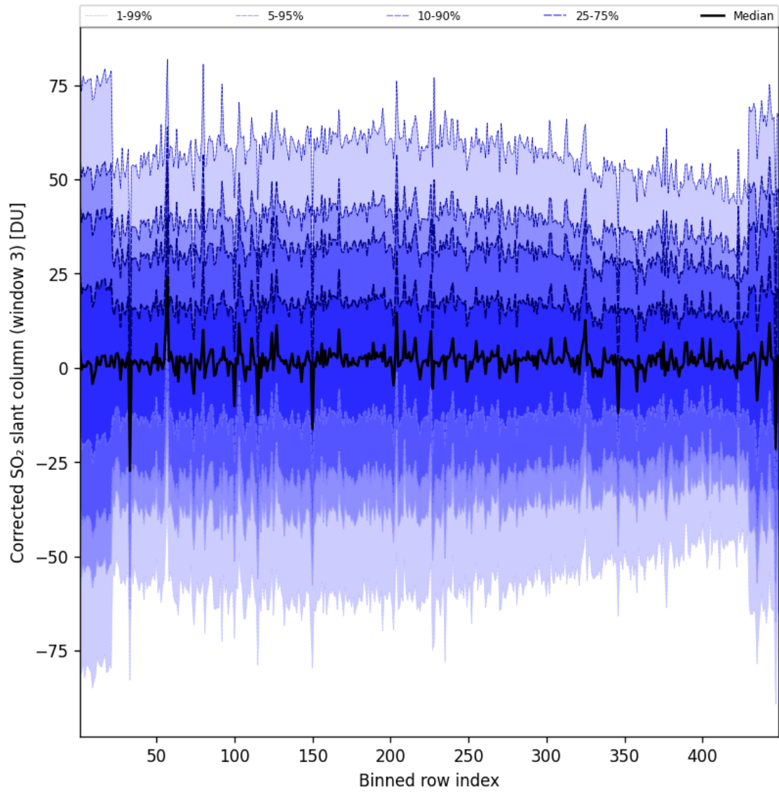
Figure 100: Along track statistics of “Corrected SO 2 slant column (window 3)” for 2025-07-18 to 2025-07-19
