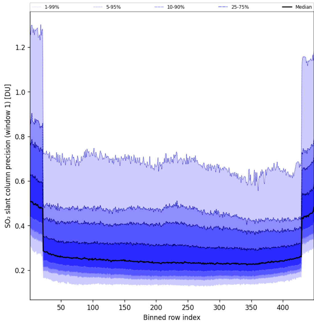
Figure 91: Along track statistics of “SO 2 slant column precision (window 1)” for 2025-07-18 to 2025-07-19
