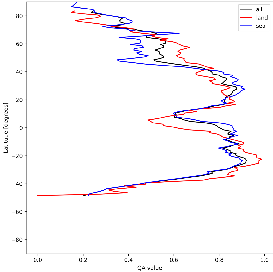
Figure 30: Zonal average of “QA value” for 2025-07-18 to 2025-07-19.
