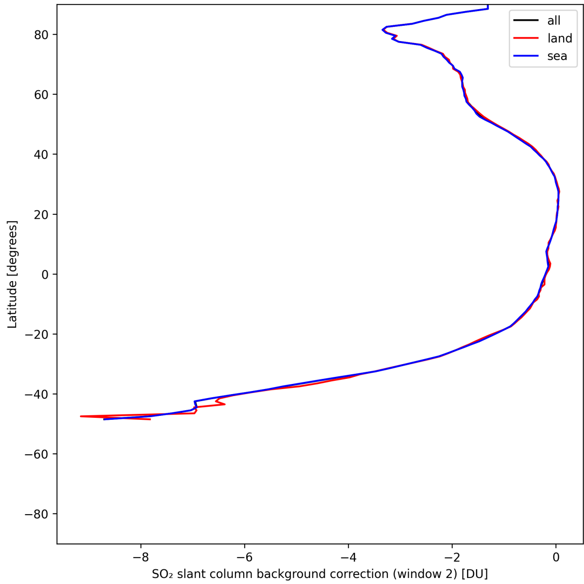
Figure 43: Zonal average of “SO 2 slant column background correction (window 2)” for 2025-07-18 to 2025-07-19.
