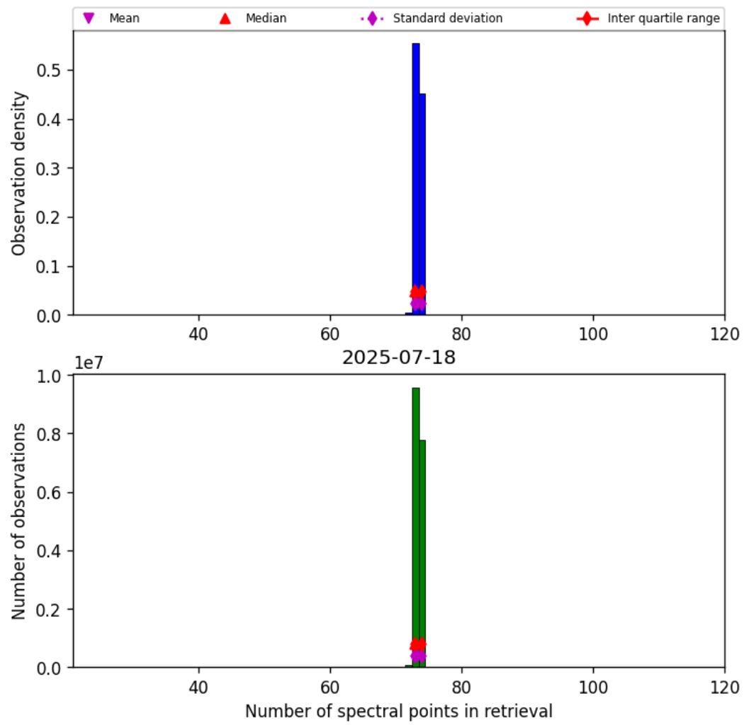
Figure 83: Histogram of “Number of spectral points in retrieval” for 2025-07-18 to 2025-07-19
