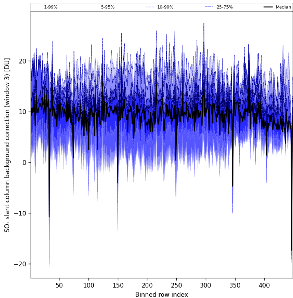
Figure 101: Along track statistics of “SO 2 slant column background correction (window 3)” for 2025-07-18 to 2025-07-19
