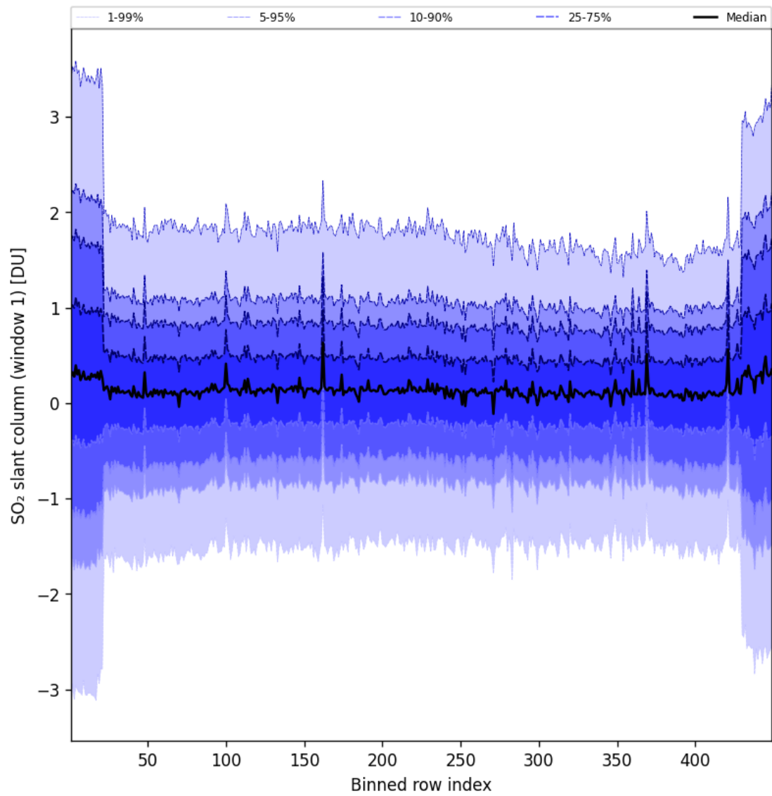
Figure 90: Along track statistics of “SO 2 slant column (window 1)” for 2025-07-18 to 2025-07-19
