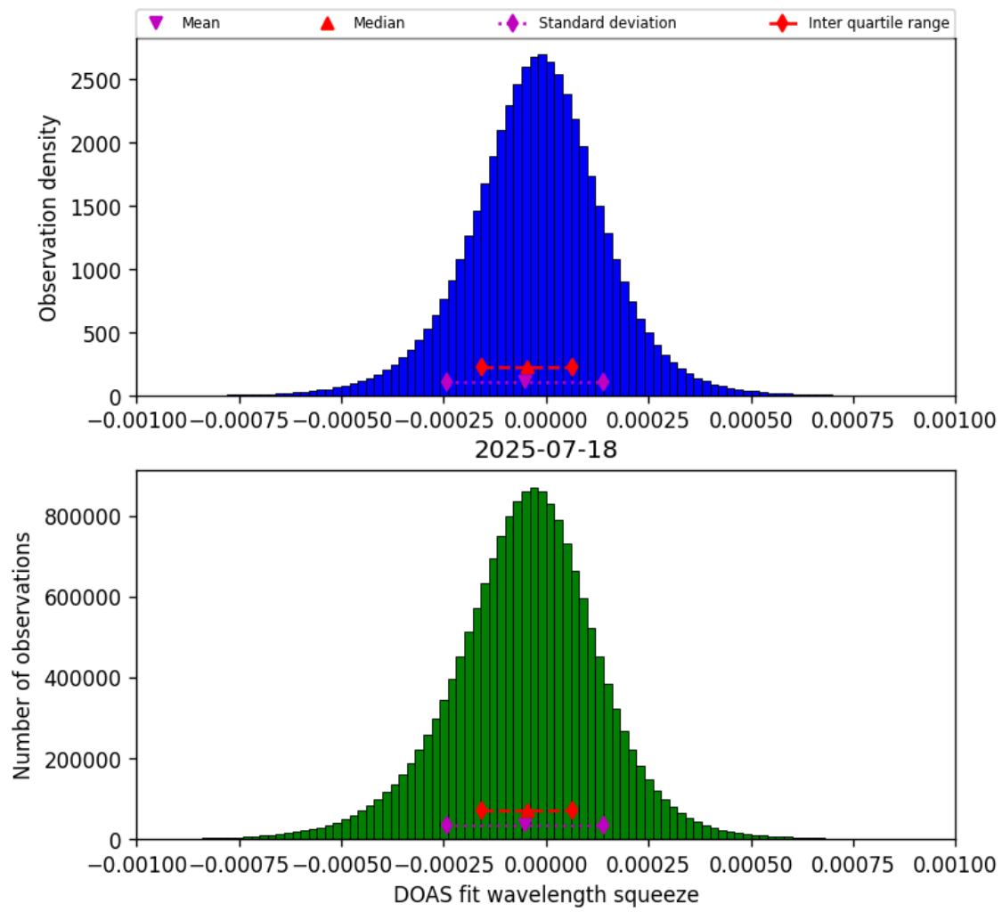
Figure 78: Histogram of “DOAS fit wavelength squeeze” for 2025-07-18 to 2025-07-19
