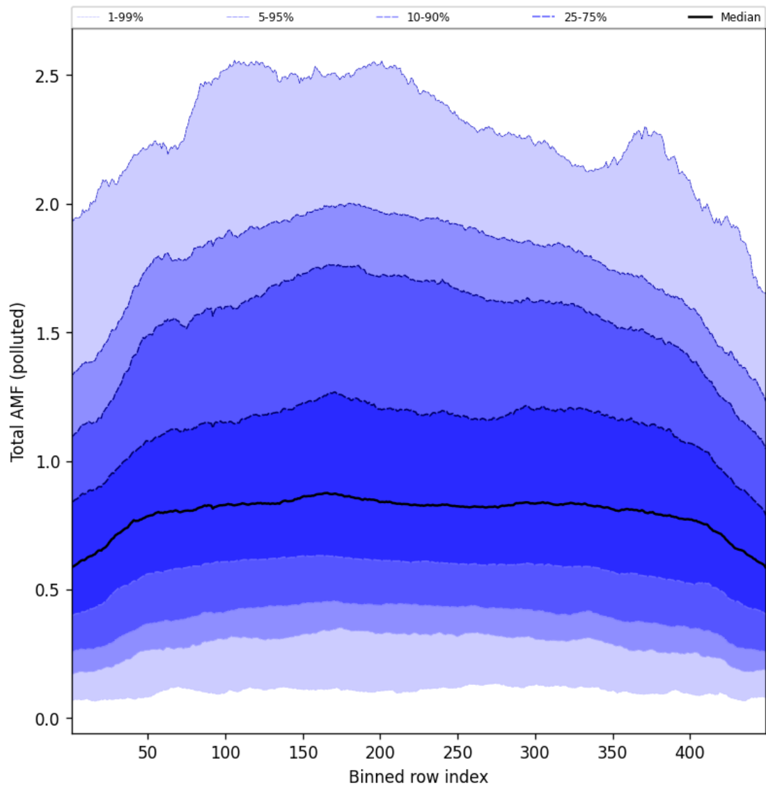
Figure 107: Along track statistics of “Total AMF (polluted)” for 2025-07-18 to 2025-07-19
