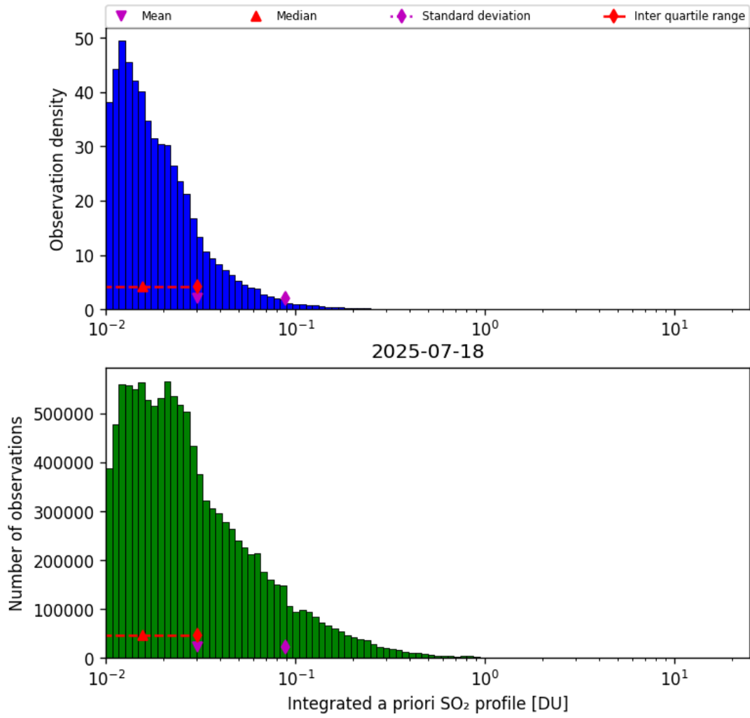
Figure 76: Histogram of “Integrated a priori SO 2 profile” for 2025-07-18 to 2025-07-19
