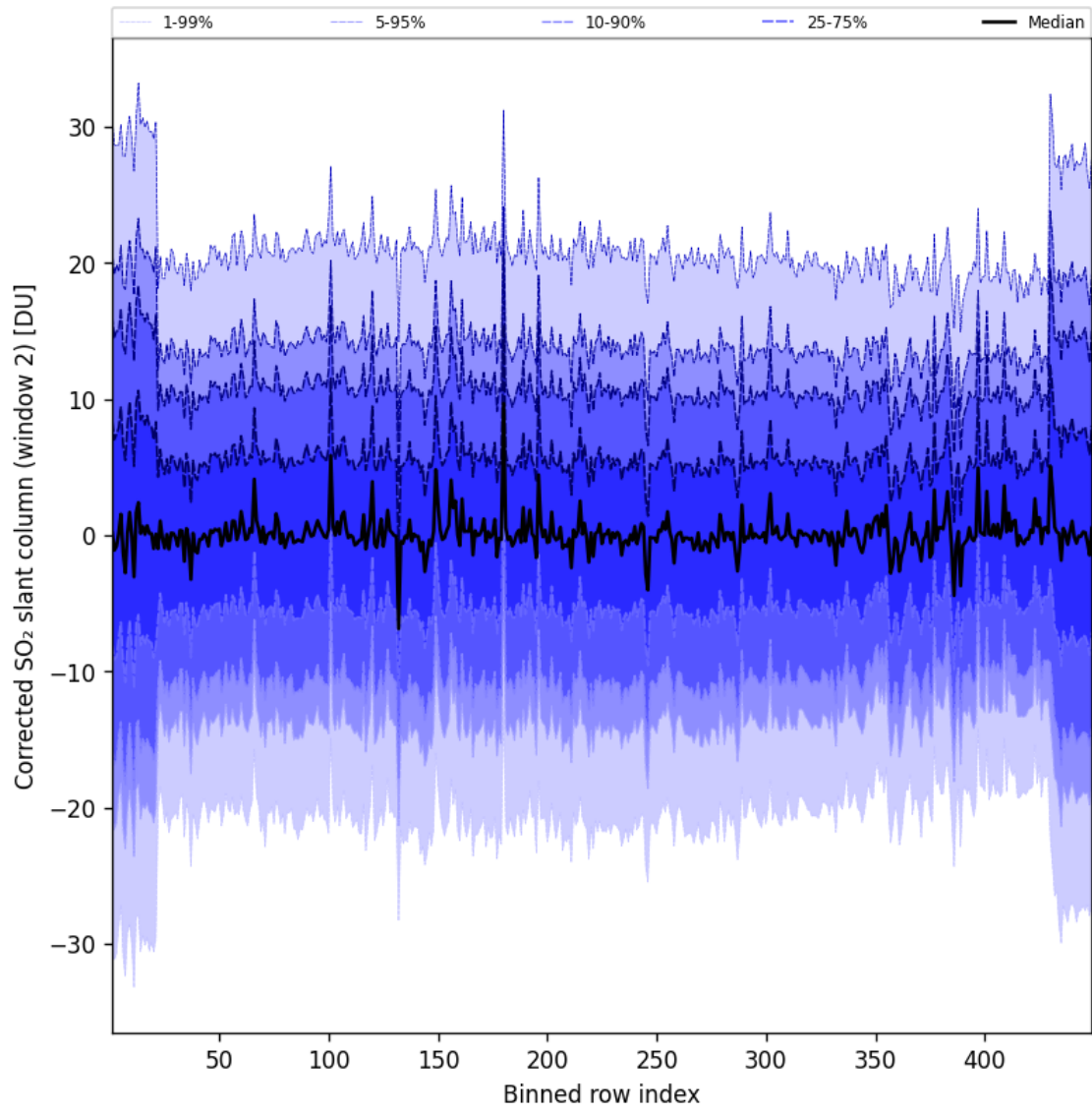
Figure 96: Along track statistics of “Corrected SO 2 slant column (window 2)” for 2025-07-18 to 2025-07-19
