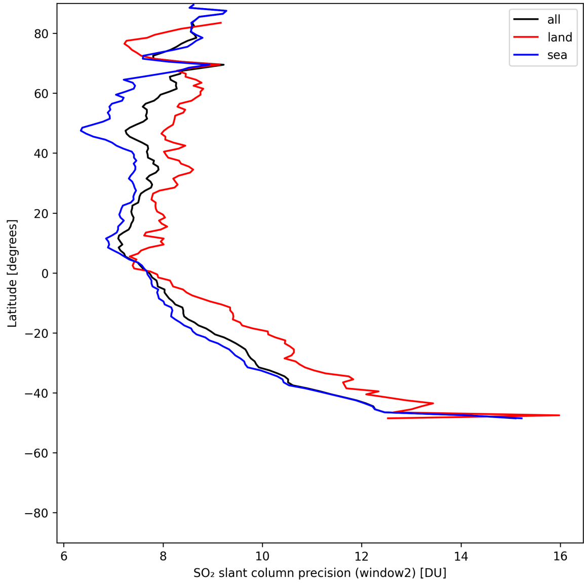
Figure 41: Zonal average of “SO 2 slant column precision (window2)” for 2025-07-18 to 2025-07-19.
