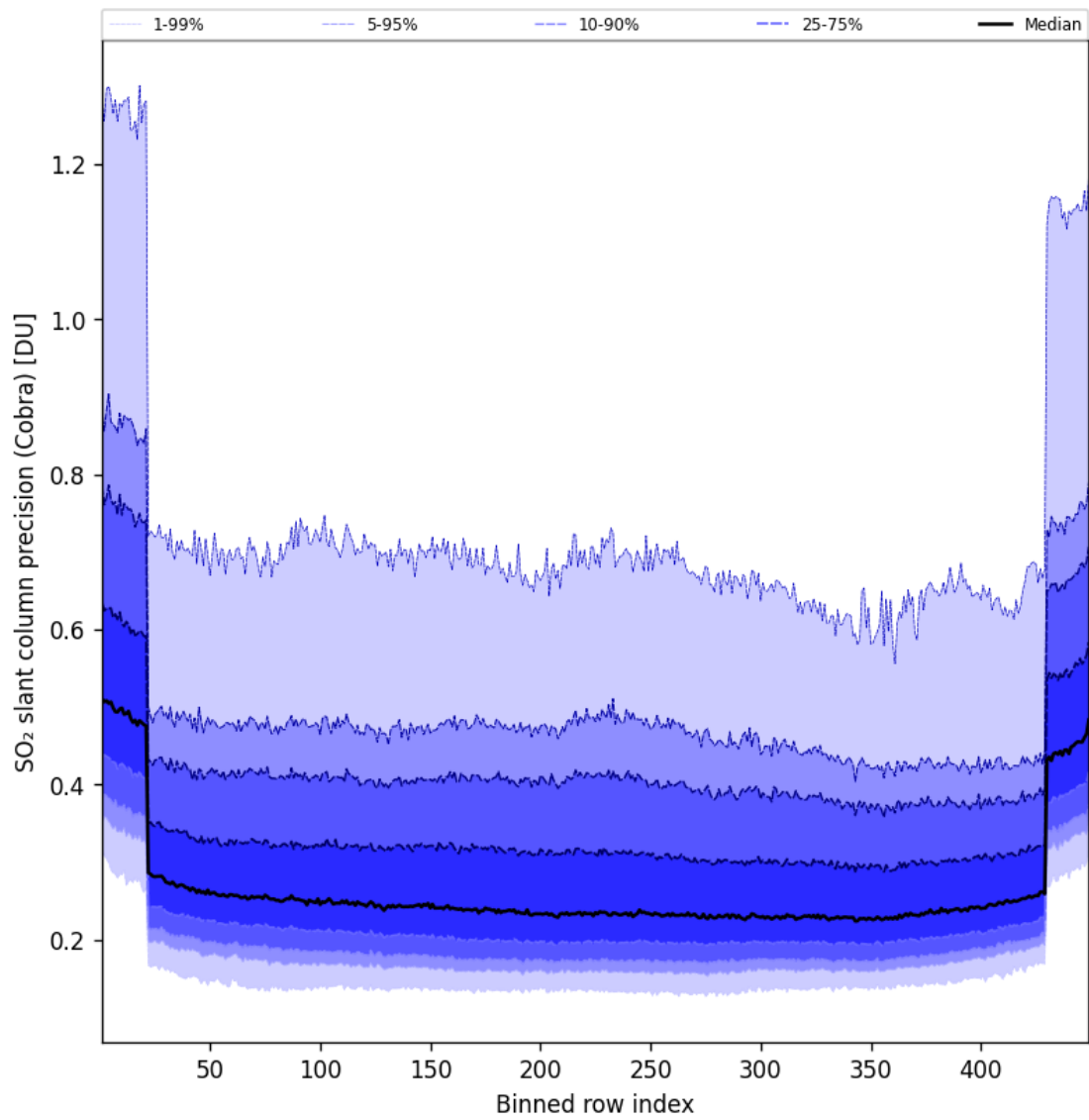
Figure 89: Along track statistics of “SO 2 slant column precision (Cobra)” for 2025-07-18 to 2025-07-19
