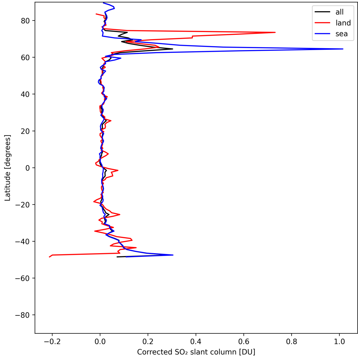
Figure 33: Zonal average of “Corrected SO 2 slant column” for 2025-07-18 to 2025-07-19.
