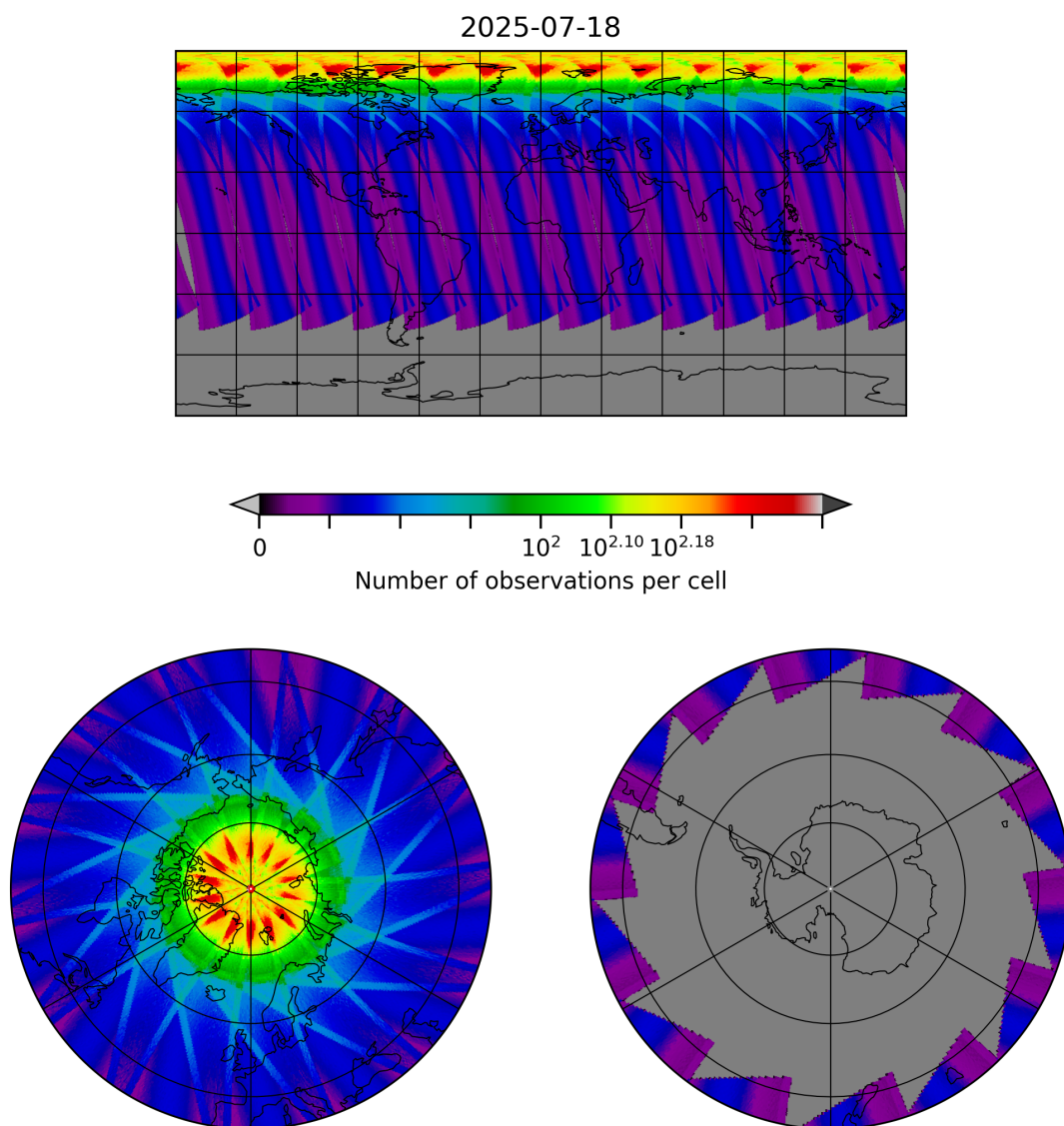
Figure 29: Map of the number of observations for 2025-07-18 to 2025-07-19
