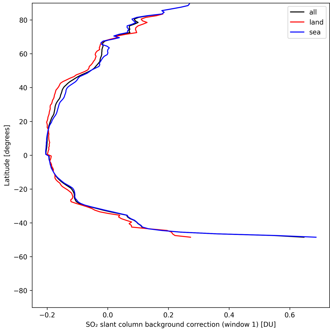
Figure 39: Zonal average of "SO 2 slant column background correction (window 1)" for 2025-07-18 to 2025-07-19.
