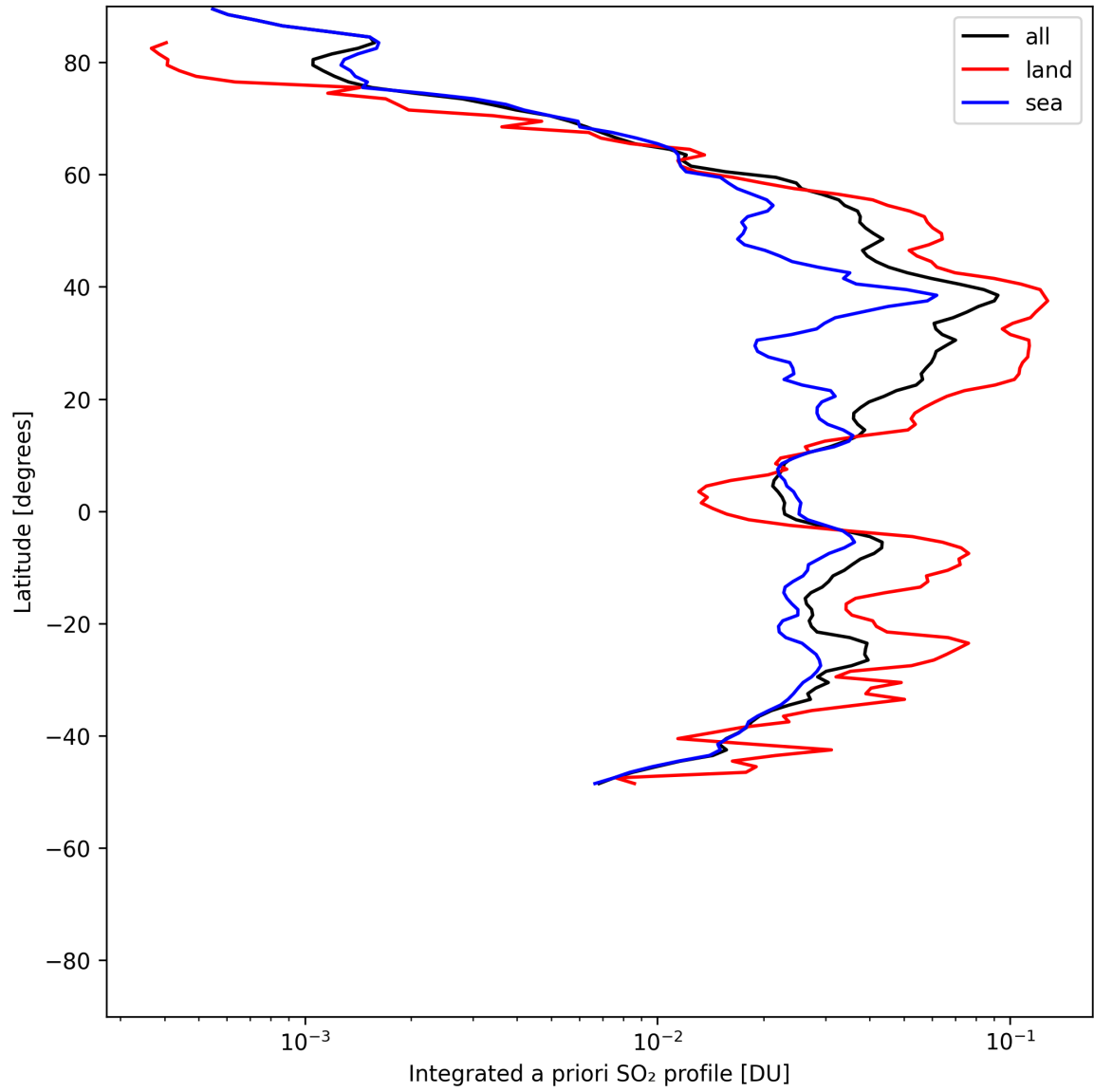
Figure 49: Zonal average of “Integrated a priori SO 2 profile” for 2025-07-18 to 2025-07-19.
