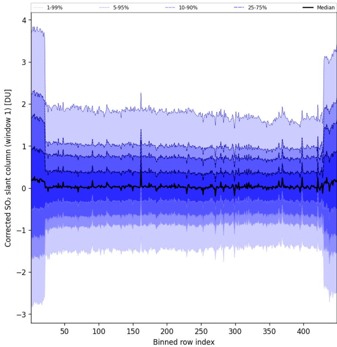
Figure 92: Along track statistics of “Corrected SO 2 slant column (window 1)” for 2025-07-18 to 2025-07-19
