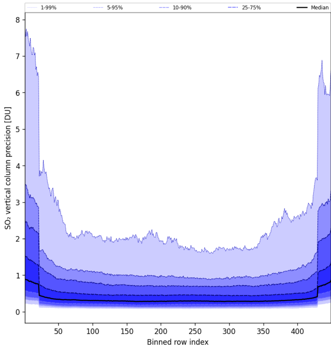
Figure 86: Along track statistics of “SO 2 vertical column precision” for 2025-07-18 to 2025-07-19
