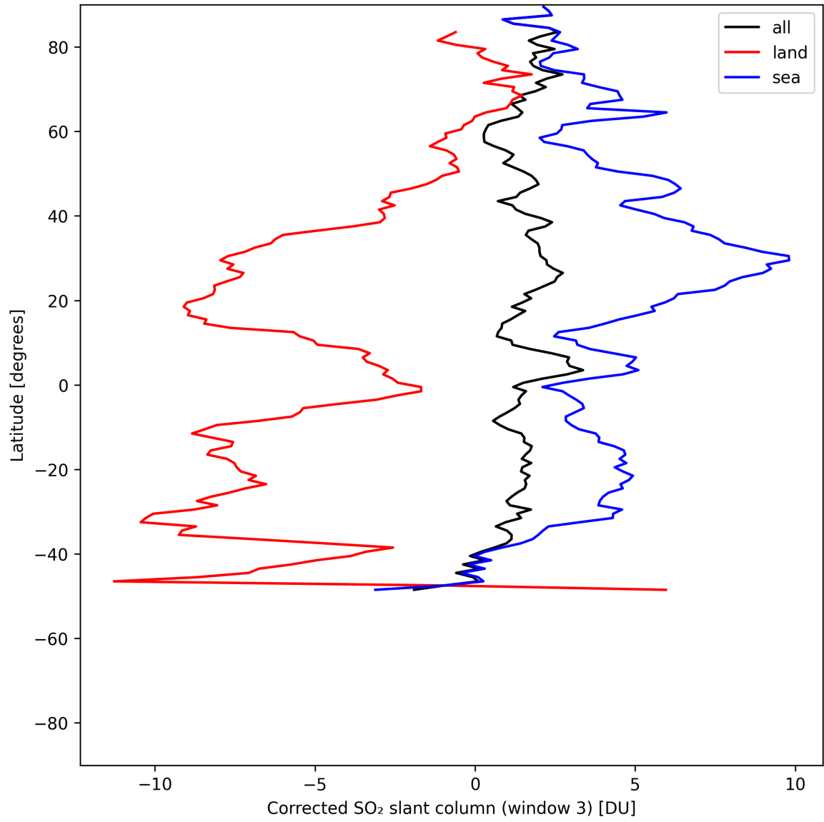
Figure 46: Zonal average of “Corrected SO 2 slant column (window 3)” for 2025-07-18 to 2025-07-19.
