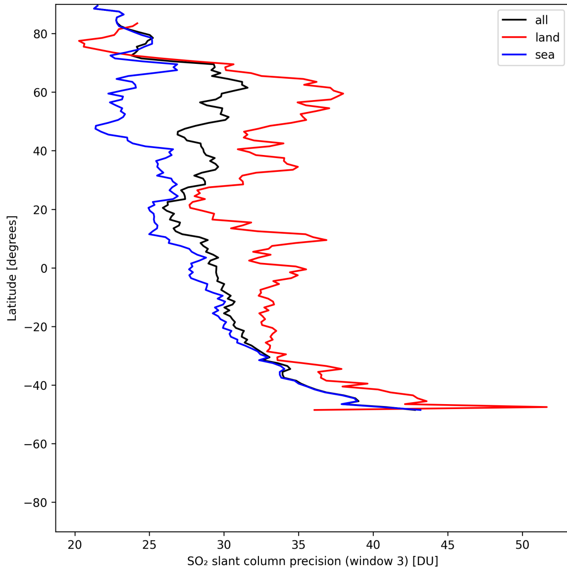
Figure 45: Zonal average of “SO 2 slant column precision (window 3)” for 2025-07-18 to 2025-07-19.
