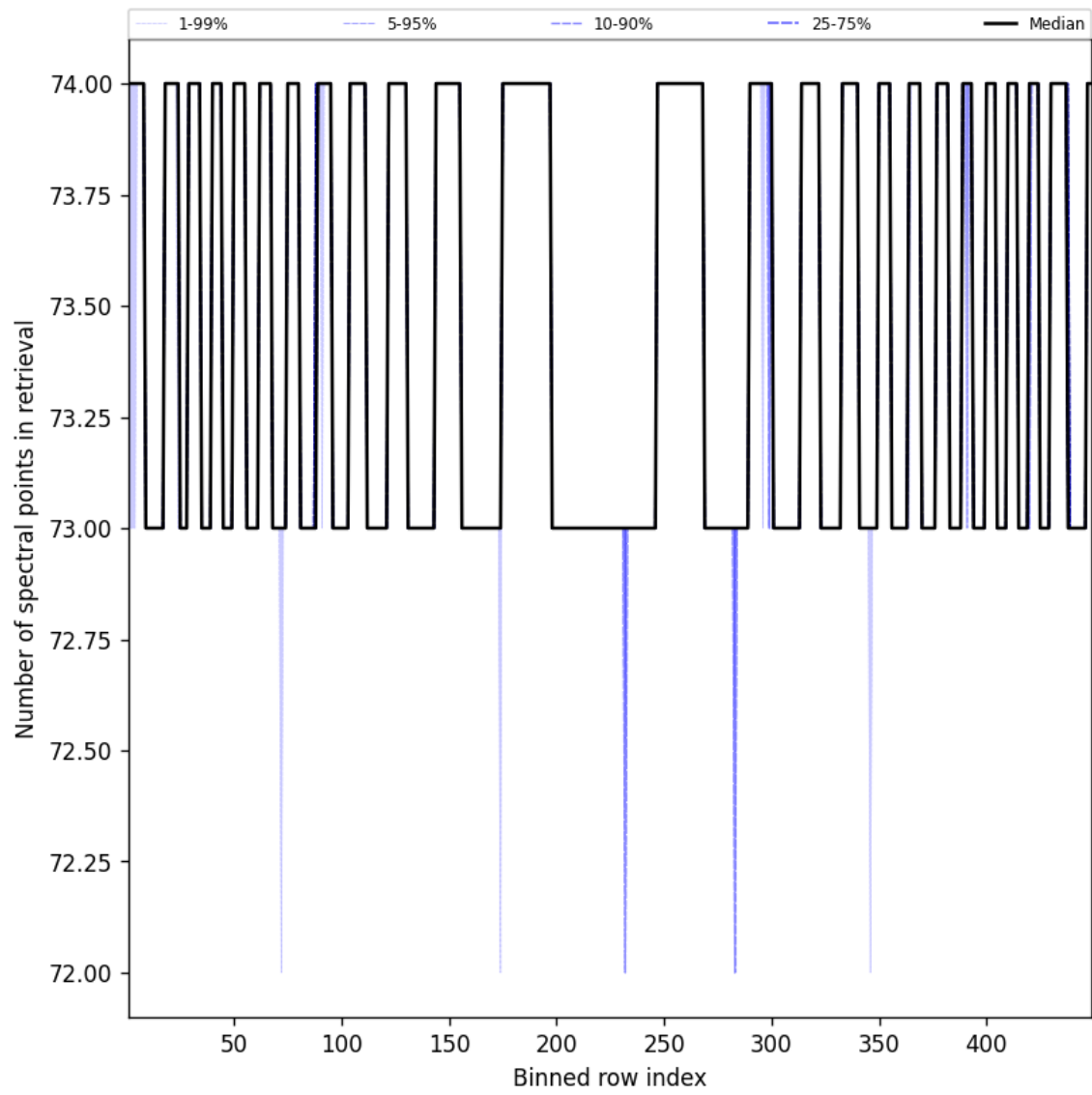
Figure 110: Along track statistics of “Number of spectral points in retrieval” for 2025-07-18 to 2025-07-19
