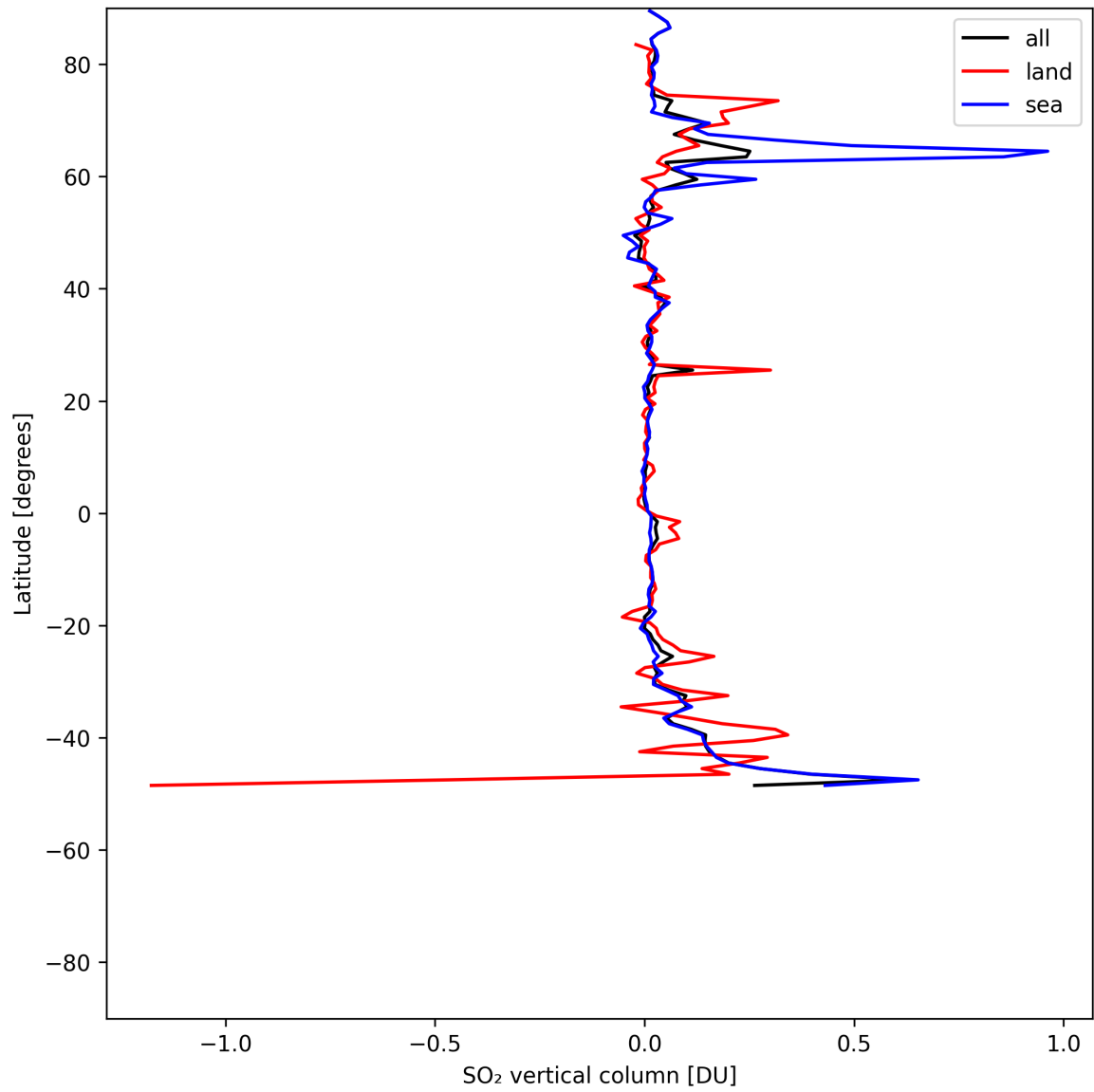
Figure 31: Zonal average of “SO 2 vertical column” for 2025-07-18 to 2025-07-19.
