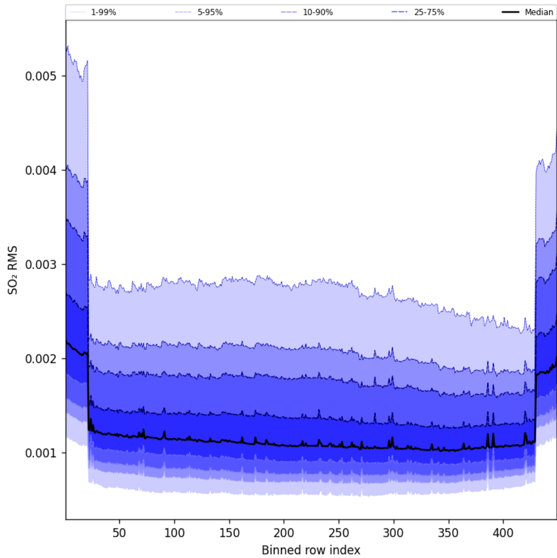
Figure 106: Along track statistics of “SO 2 RMS” for 2025-07-18 to 2025-07-19
