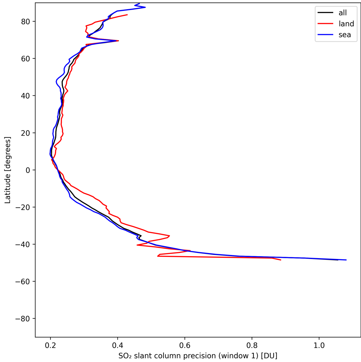
Figure 37: Zonal average of “SO 2 slant column precision (window 1)” for 2025-07-18 to 2025-07-19.
