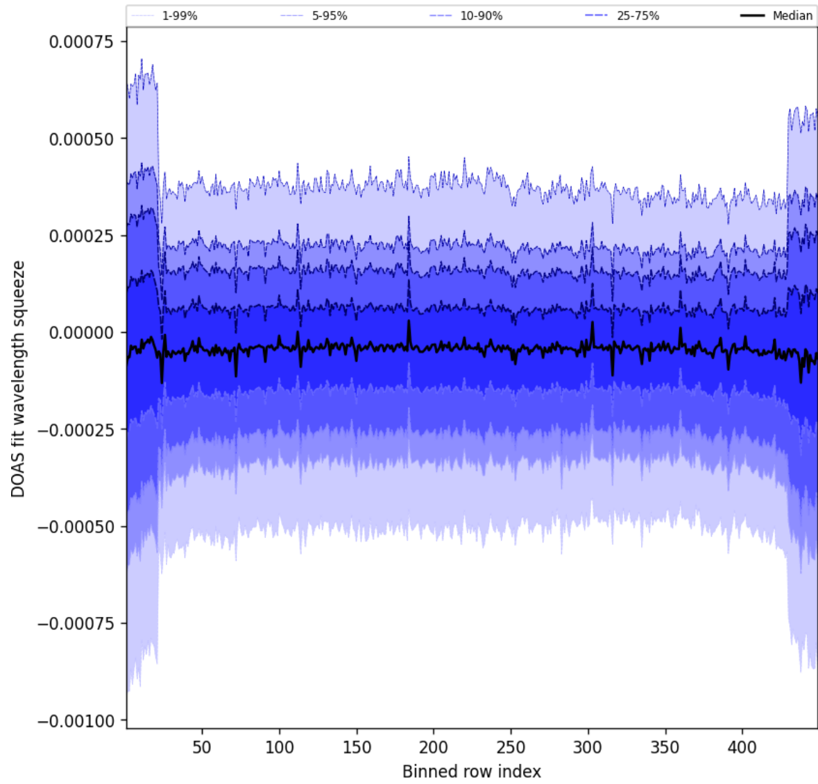
Figure 105: Along track statistics of “DOAS fit wavelength squeeze” for 2025-07-18 to 2025-07-19
