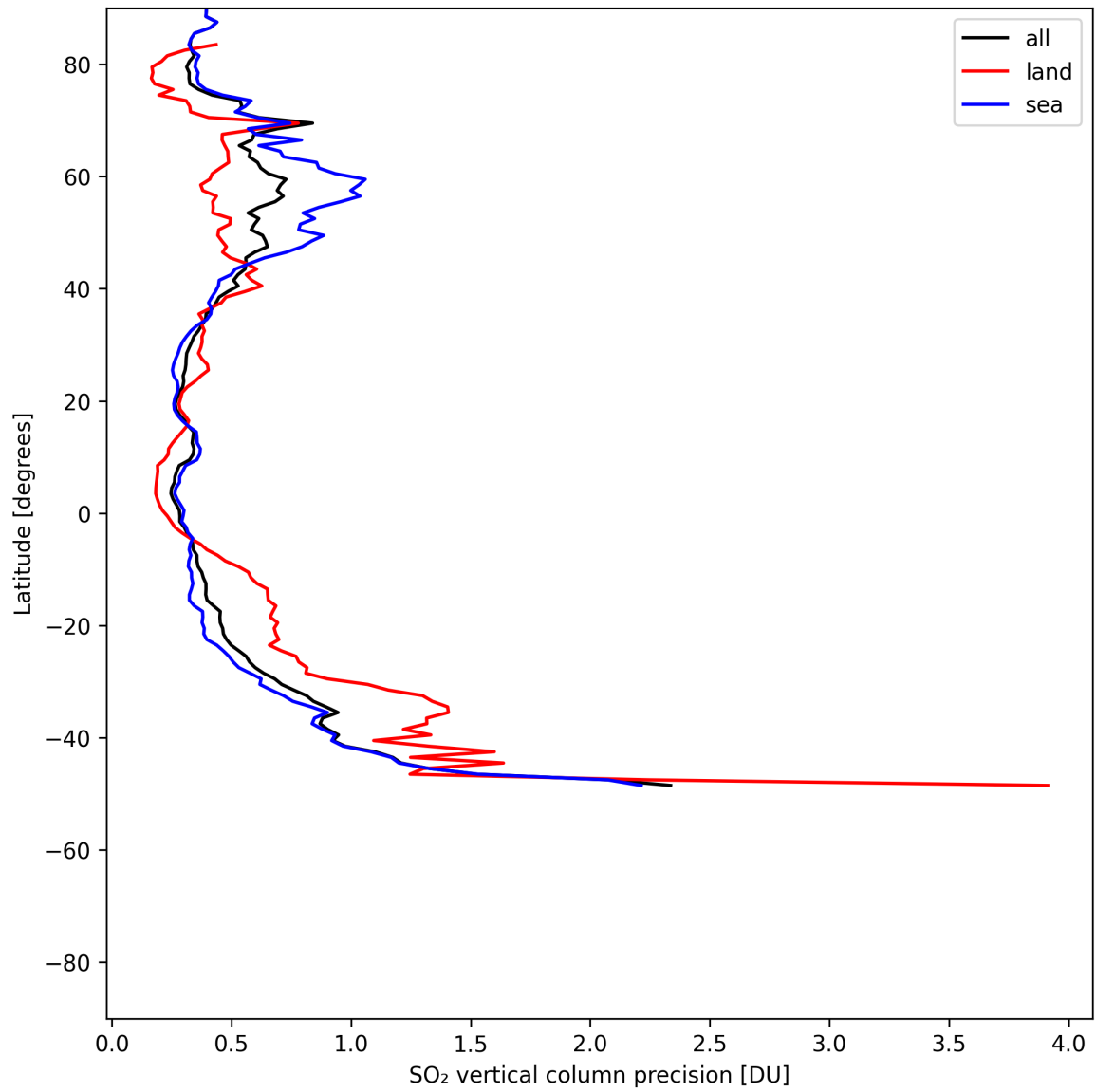
Figure 32: Zonal average of “SO 2 vertical column precision” for 2025-07-18 to 2025-07-19.
