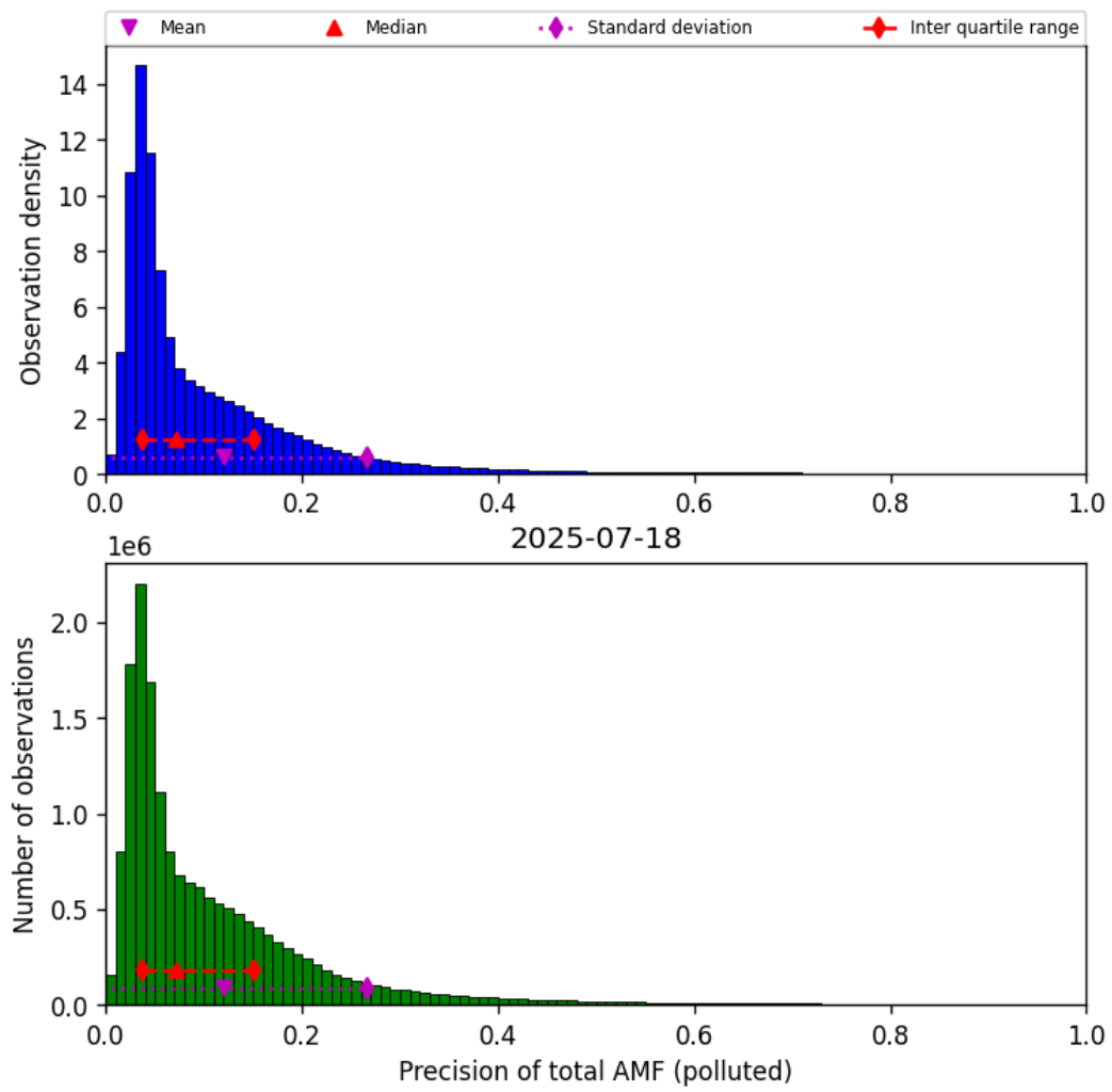
Figure 81: Histogram of “Precision of total AMF (polluted)” for 2025-07-18 to 2025-07-19
