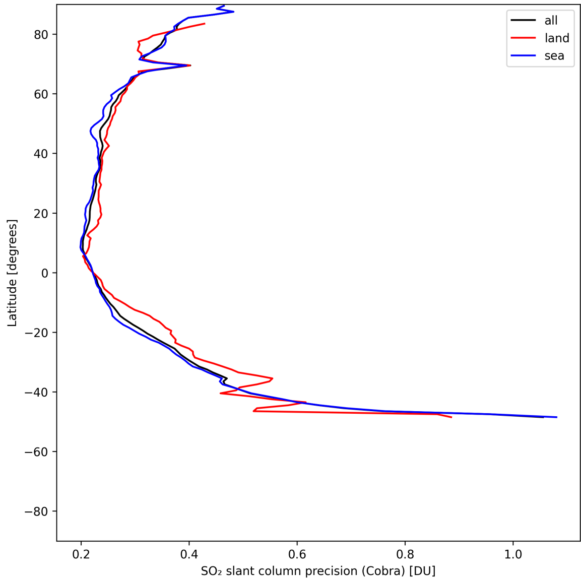
Figure 35: Zonal average of “SO 2 slant column precision (Cobra)” for 2025-07-18 to 2025-07-19.
