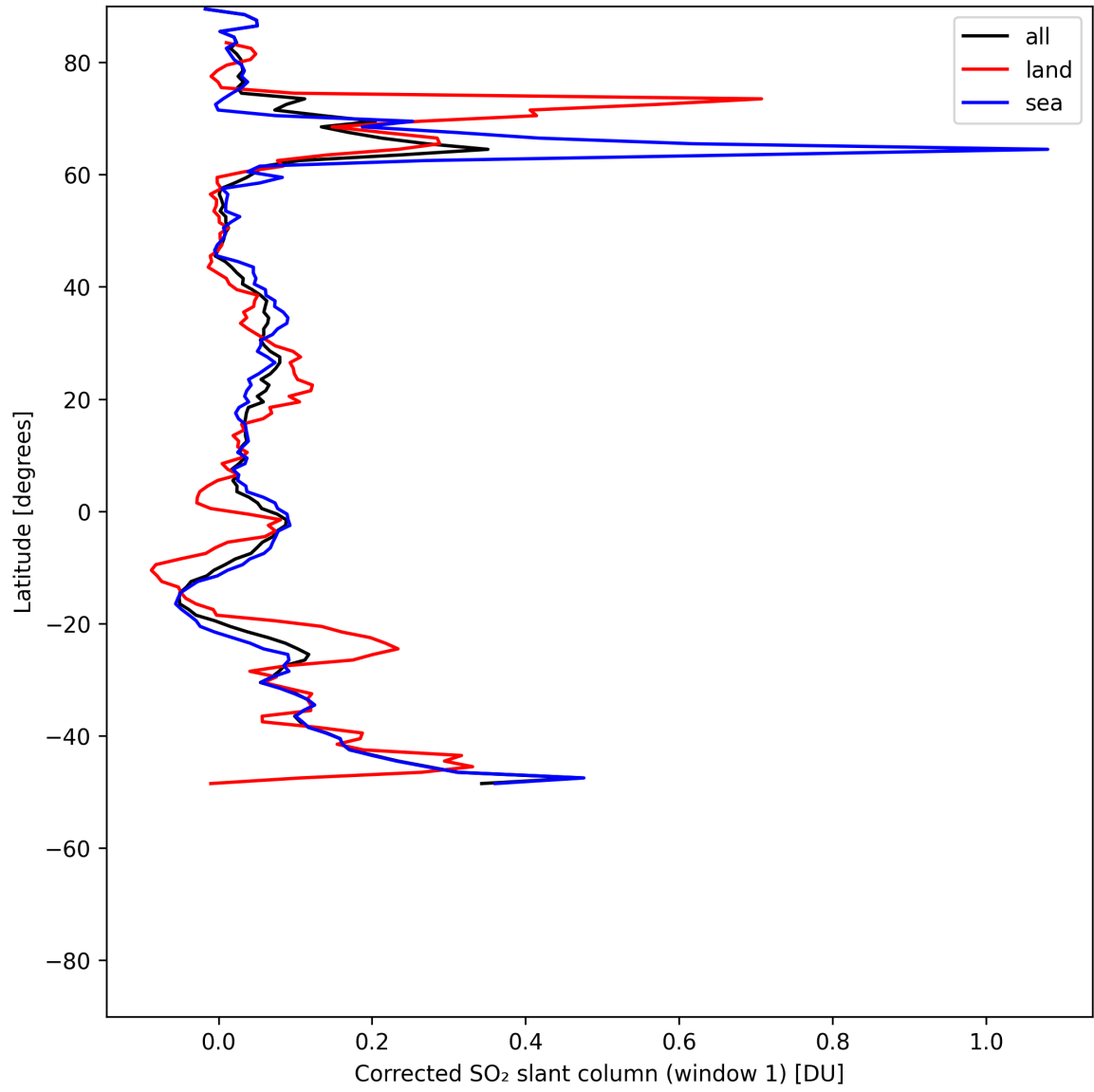
Figure 38: Zonal average of “Corrected SO 2 slant column (window 1)” for 2025-07-18 to 2025-07-19.
