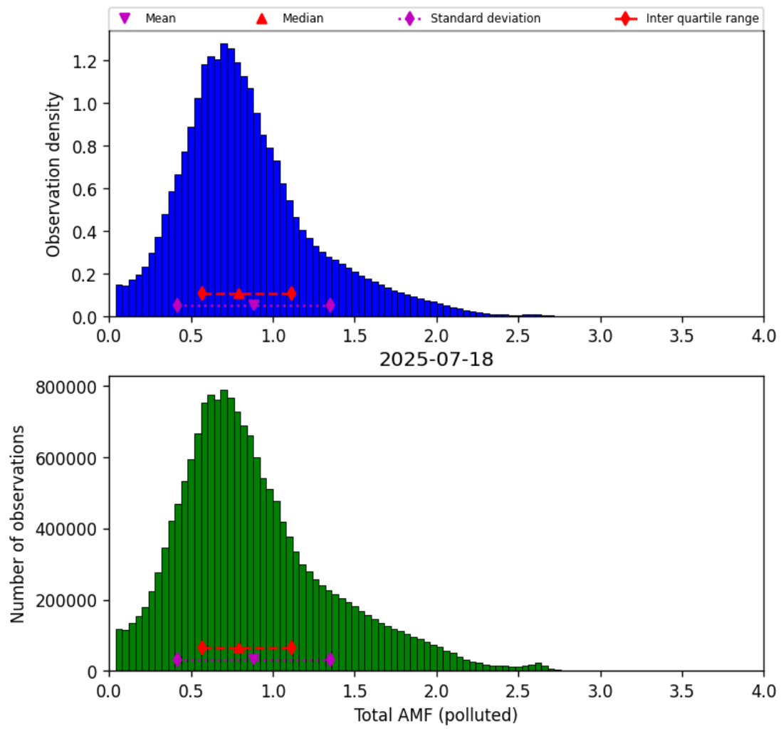
Figure 80: Histogram of “Total AMF (polluted)” for 2025-07-18 to 2025-07-19
