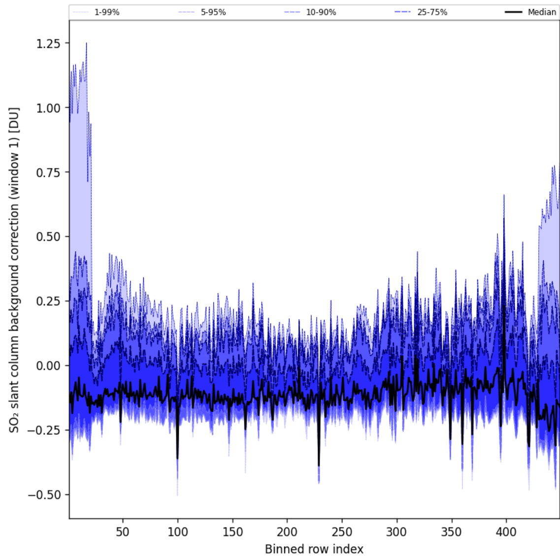
Figure 93: Along track statistics of “SO 2 slant column background correction (window 1)” for 2025-07-18 to 2025-07-19
