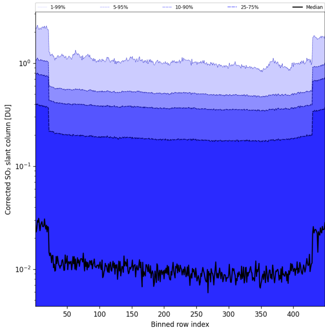
Figure 87: Along track statistics of "Corrected SO 2 slant column" for 2025-07-18 to 2025-07-19
