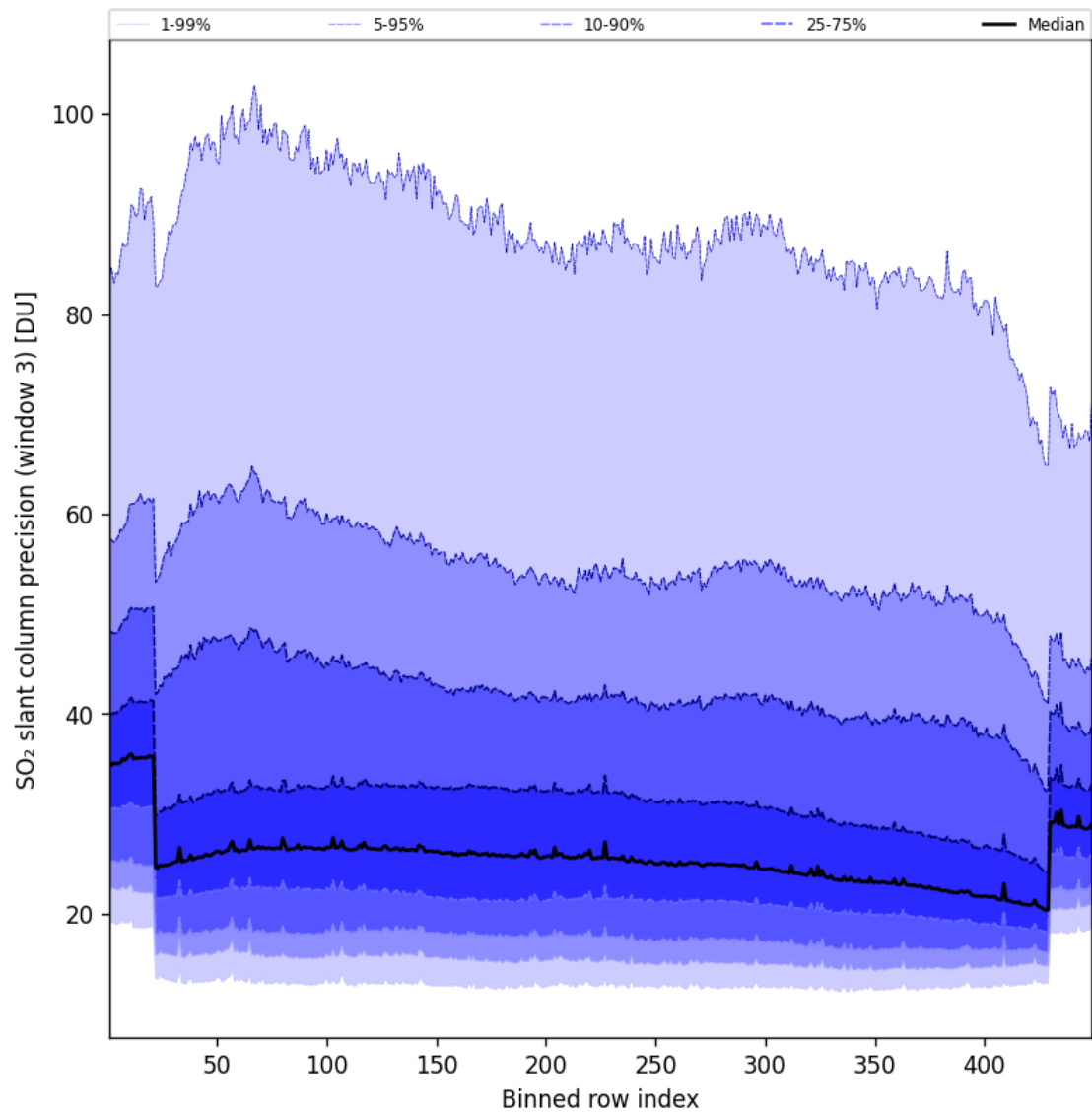
Figure 99: Along track statistics of “SO 2 slant column precision (window 3)” for 2025-07-18 to 2025-07-19
