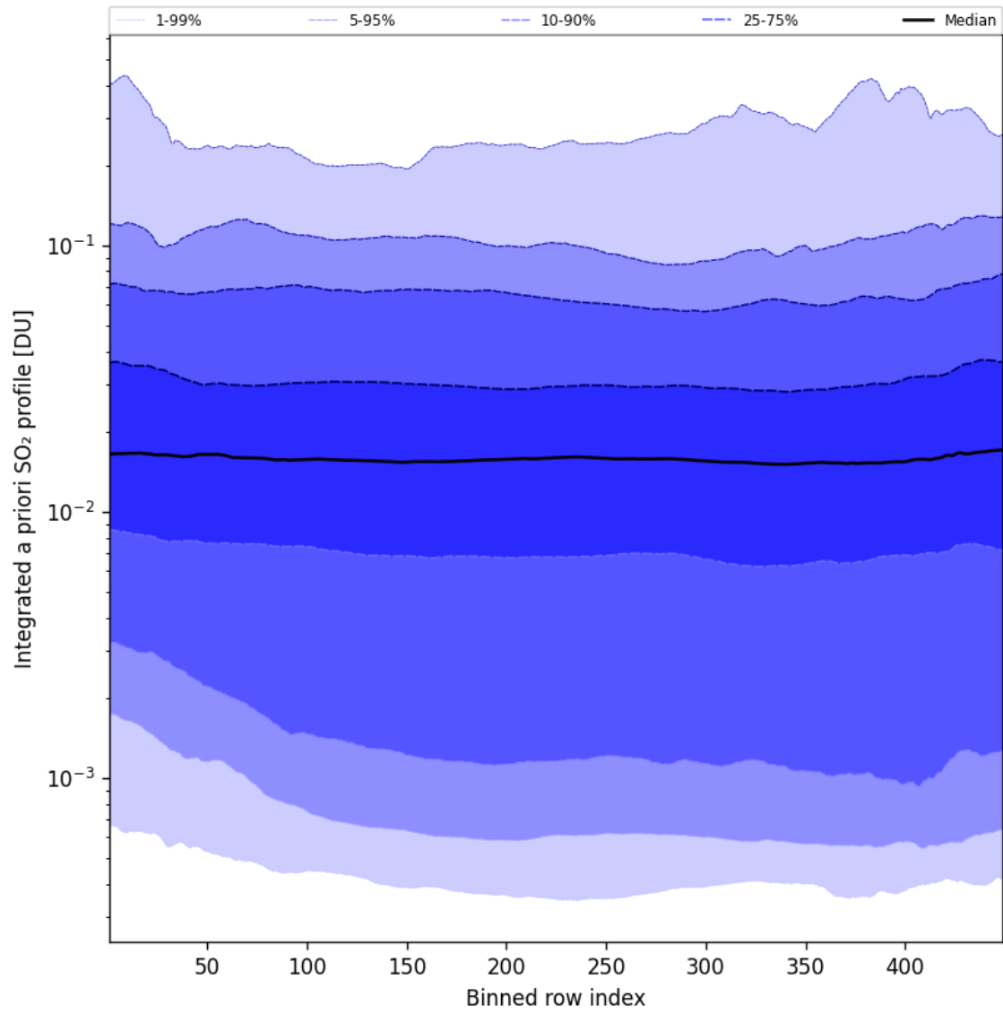
Figure 103: Along track statistics of “Integrated a priori SO 2 profile” for 2025-07-18 to 2025-07-19
