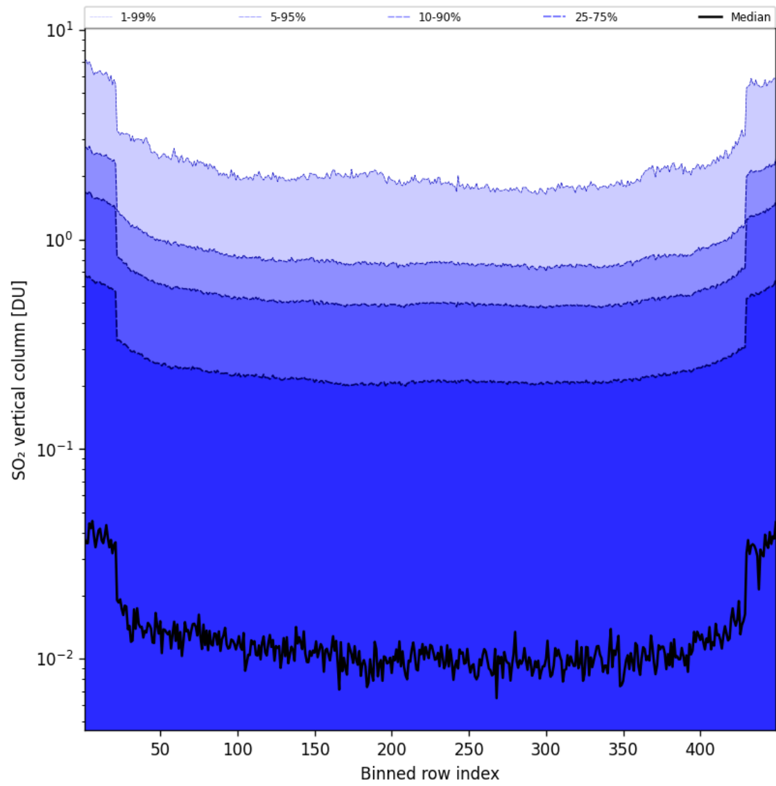
Figure 85: Along track statistics of “SO 2 vertical column” for 2025-07-18 to 2025-07-19
