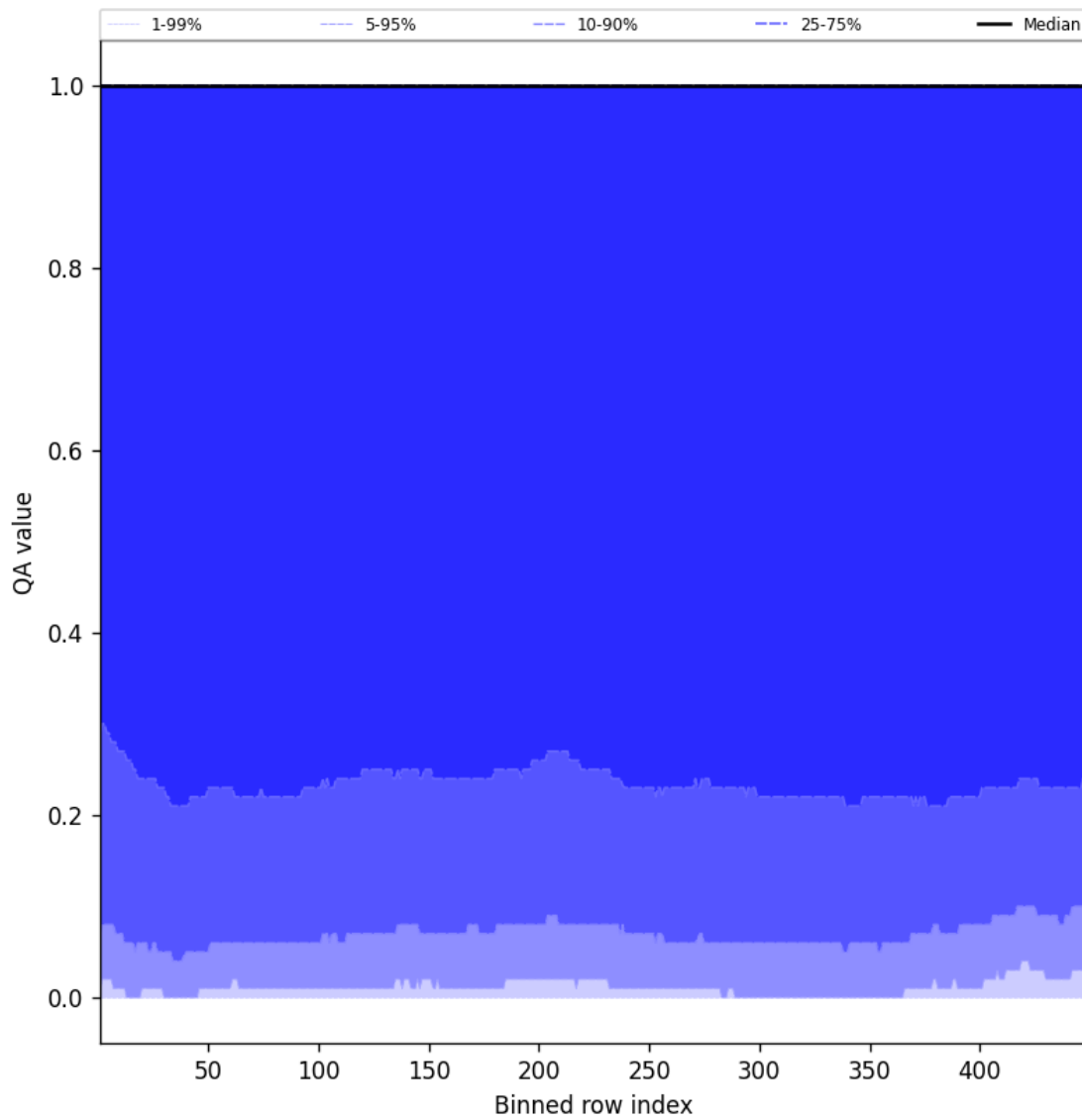
Figure 84: Along track statistics of “QA value” for 2025-07-18 to 2025-07-19
