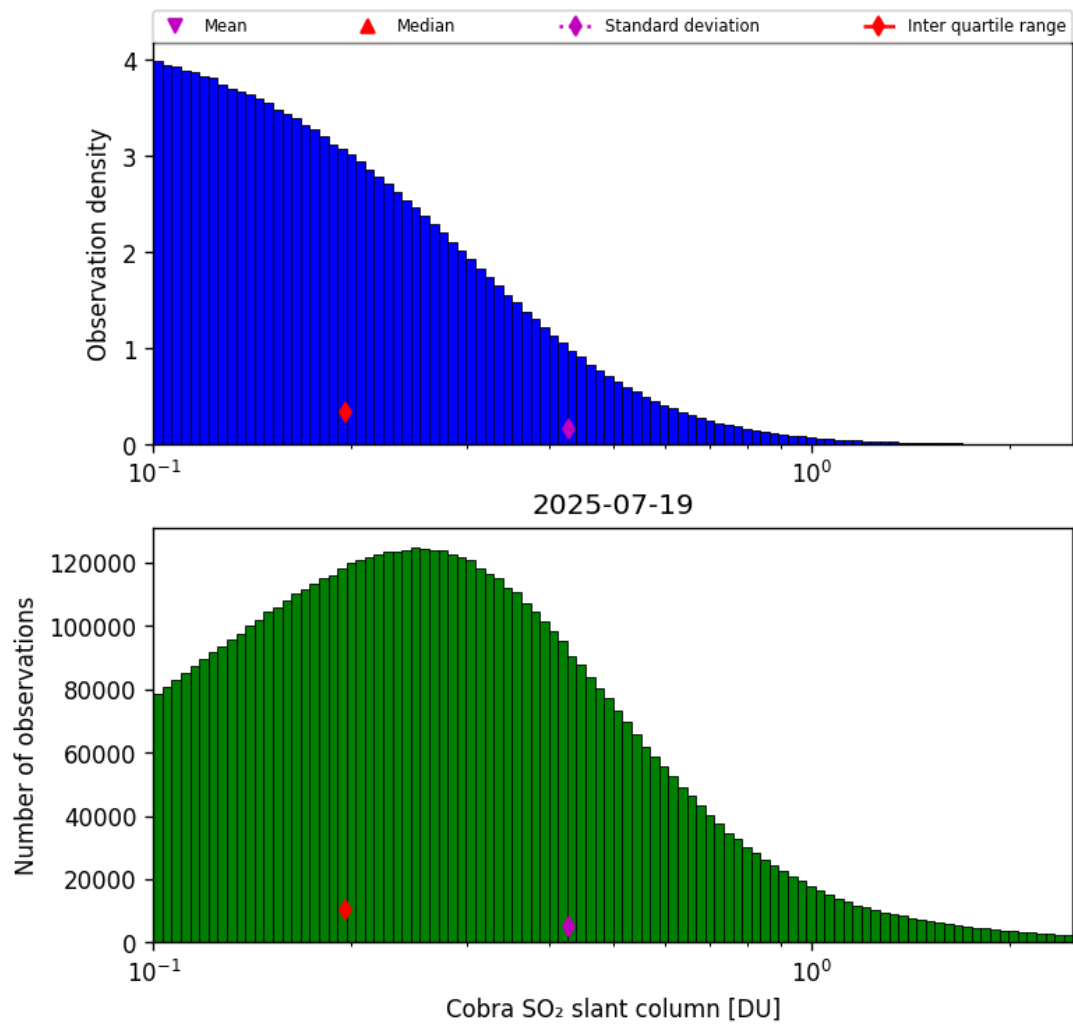
Figure 61: Histogram of “Cobra SO 2 slant column” for 2025-07-19 to 2025-07-20
