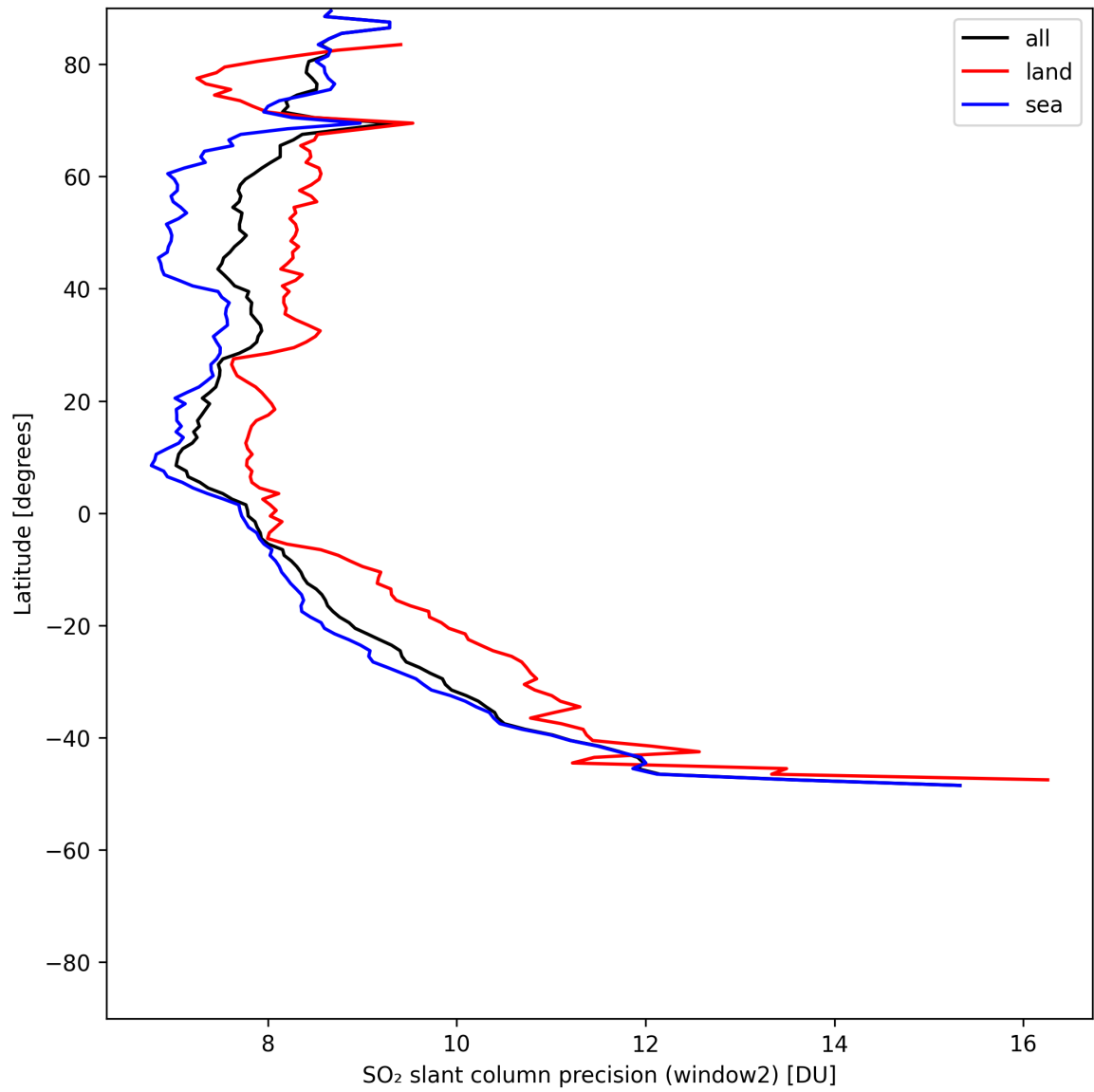
Figure 41: Zonal average of “SO 2 slant column precision (window2)” for 2025-07-19 to 2025-07-20.
