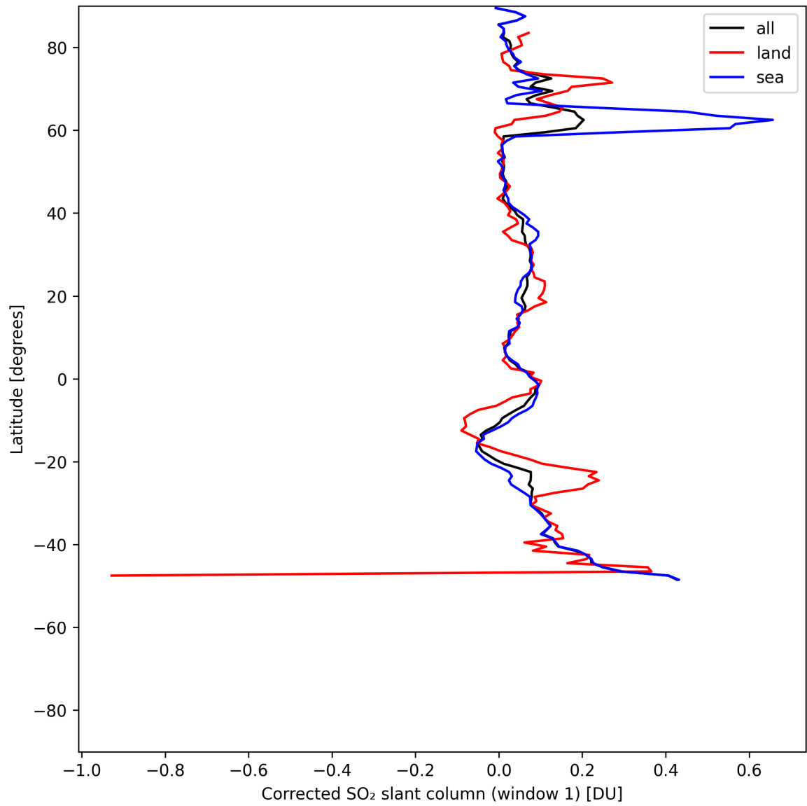
Figure 38: Zonal average of “Corrected SO 2 slant column (window 1)” for 2025-07-19 to 2025-07-20.
