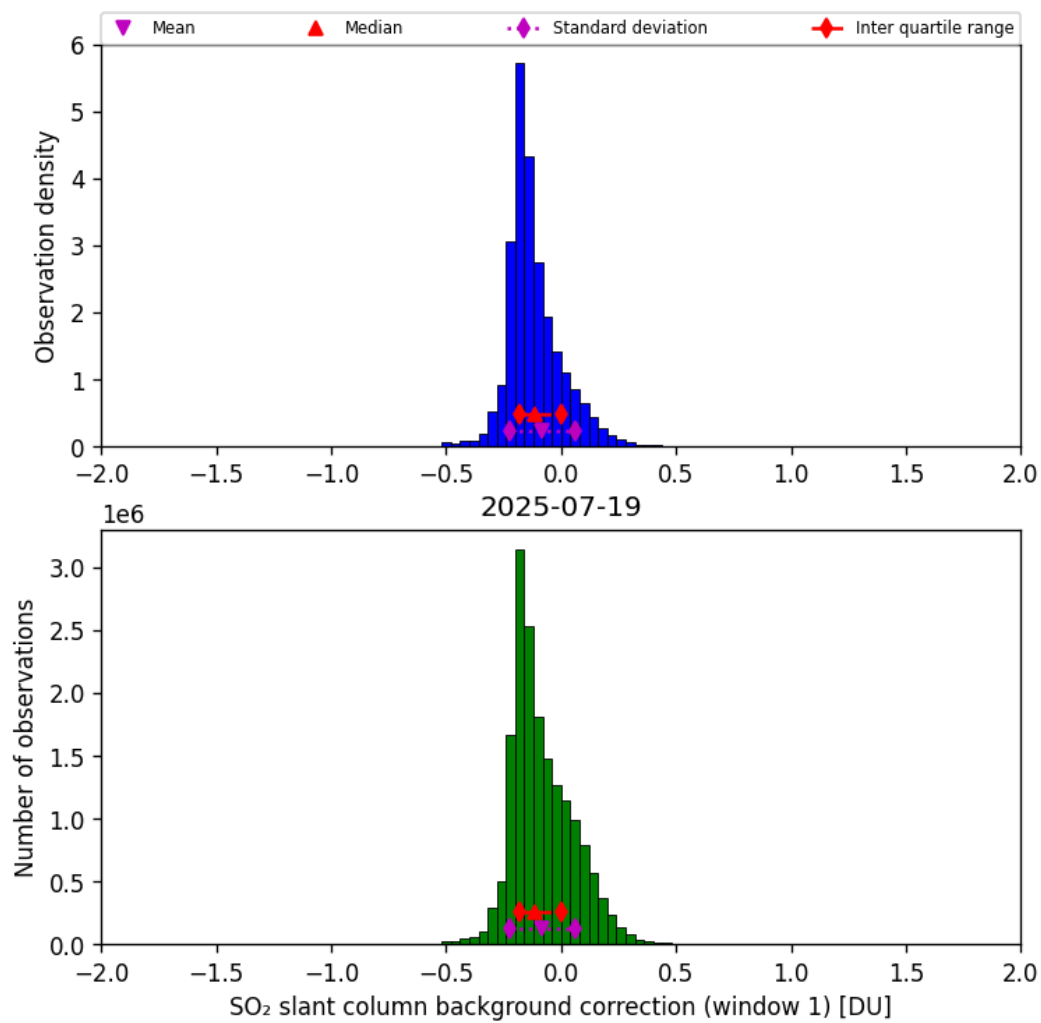
Figure 66: Histogram of “SO 2 slant column background correction (window 1)” for 2025-07-19 to 2025-07-20
