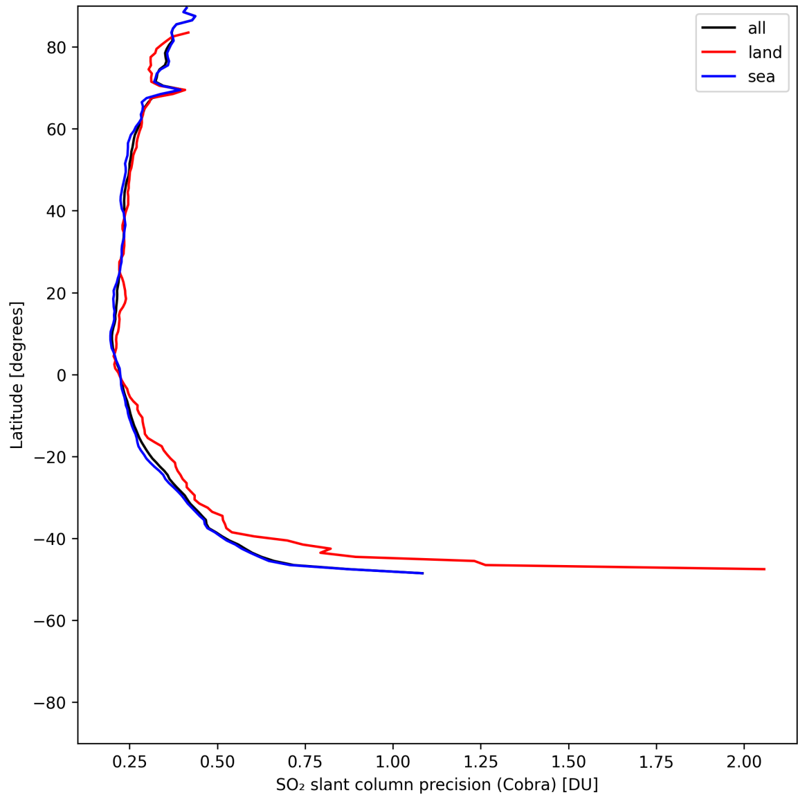
Figure 35: Zonal average of “SO 2 slant column precision (Cobra)” for 2025-07-19 to 2025-07-20.
