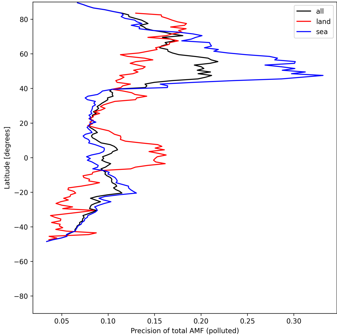
Figure 54: Zonal average of “Precision of total AMF (polluted)” for 2025-07-19 to 2025-07-20.
