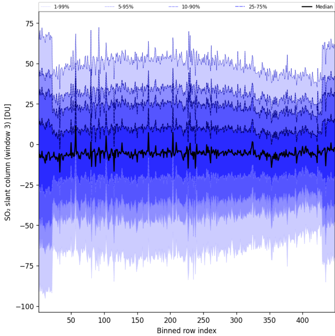
Figure 98: Along track statistics of “SO 2 slant column (window 3)” for 2025-07-19 to 2025-07-20
