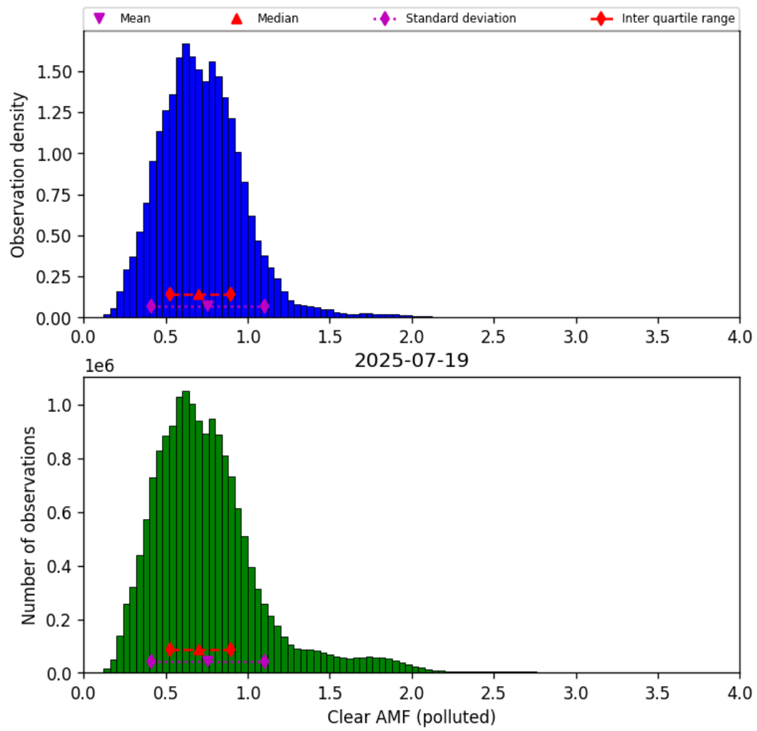
Figure 82: Histogram of “Clear AMF (polluted)” for 2025-07-19 to 2025-07-20
