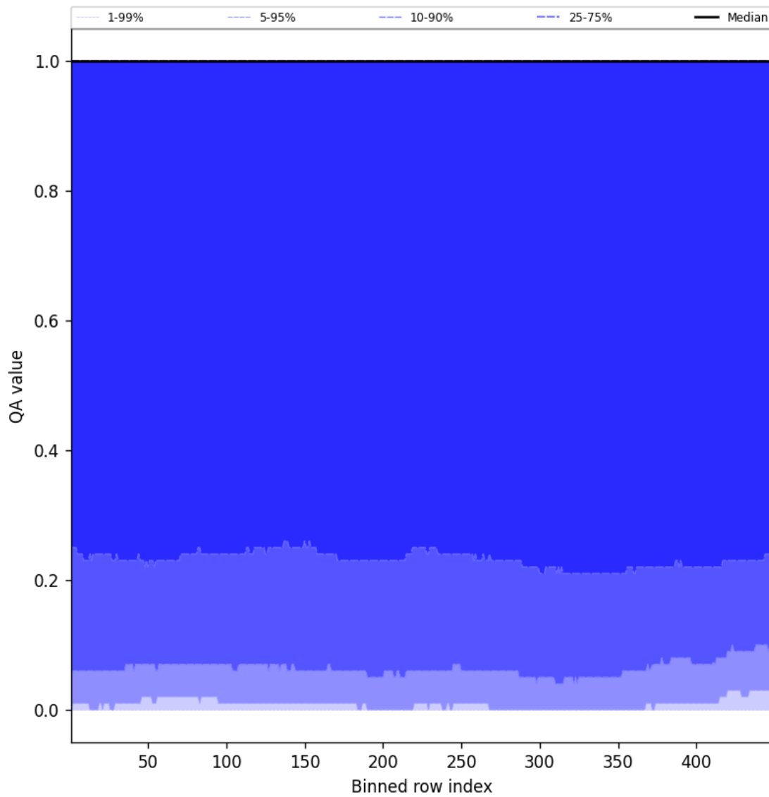
Figure 84: Along track statistics of “QA value” for 2025-07-19 to 2025-07-20
