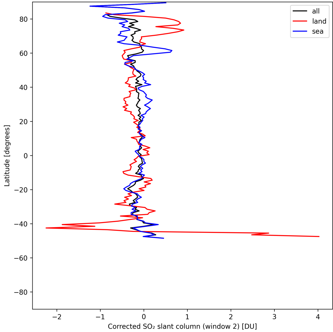
Figure 42: Zonal average of “Corrected SO 2 slant column (window 2)” for 2025-07-19 to 2025-07-20.
