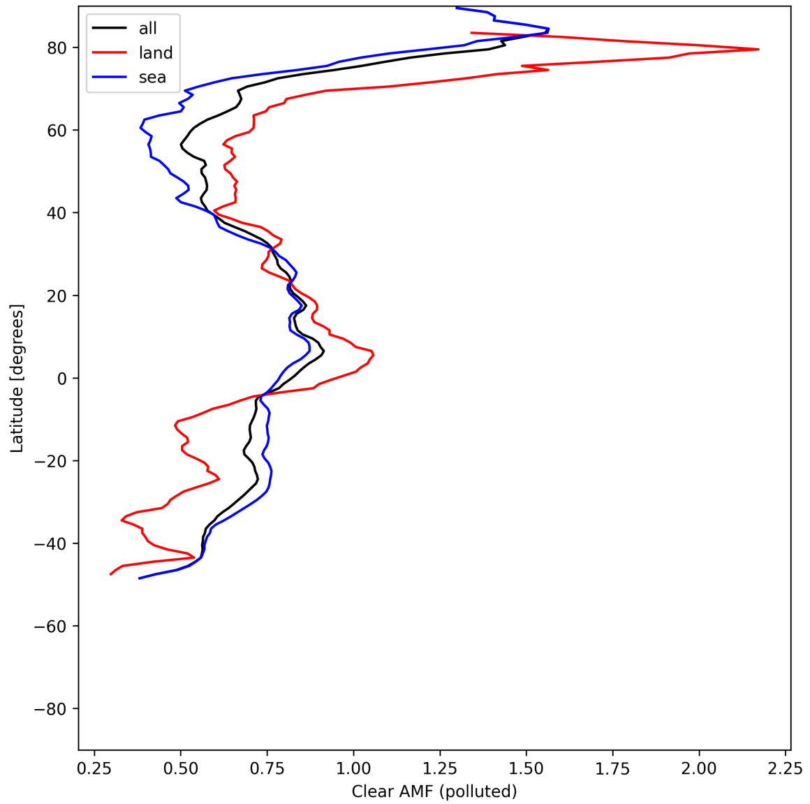
Figure 55: Zonal average of “Clear AMF (polluted)” for 2025-07-19 to 2025-07-20.
