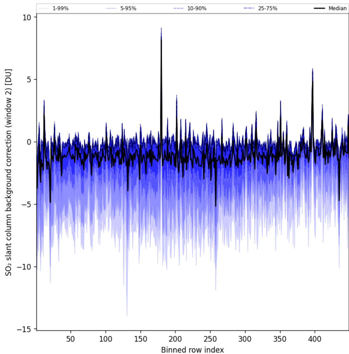
Figure 97: Along track statistics of “SO 2 slant column background correction (window 2)” for 2025-07-19 to 2025-07-20
