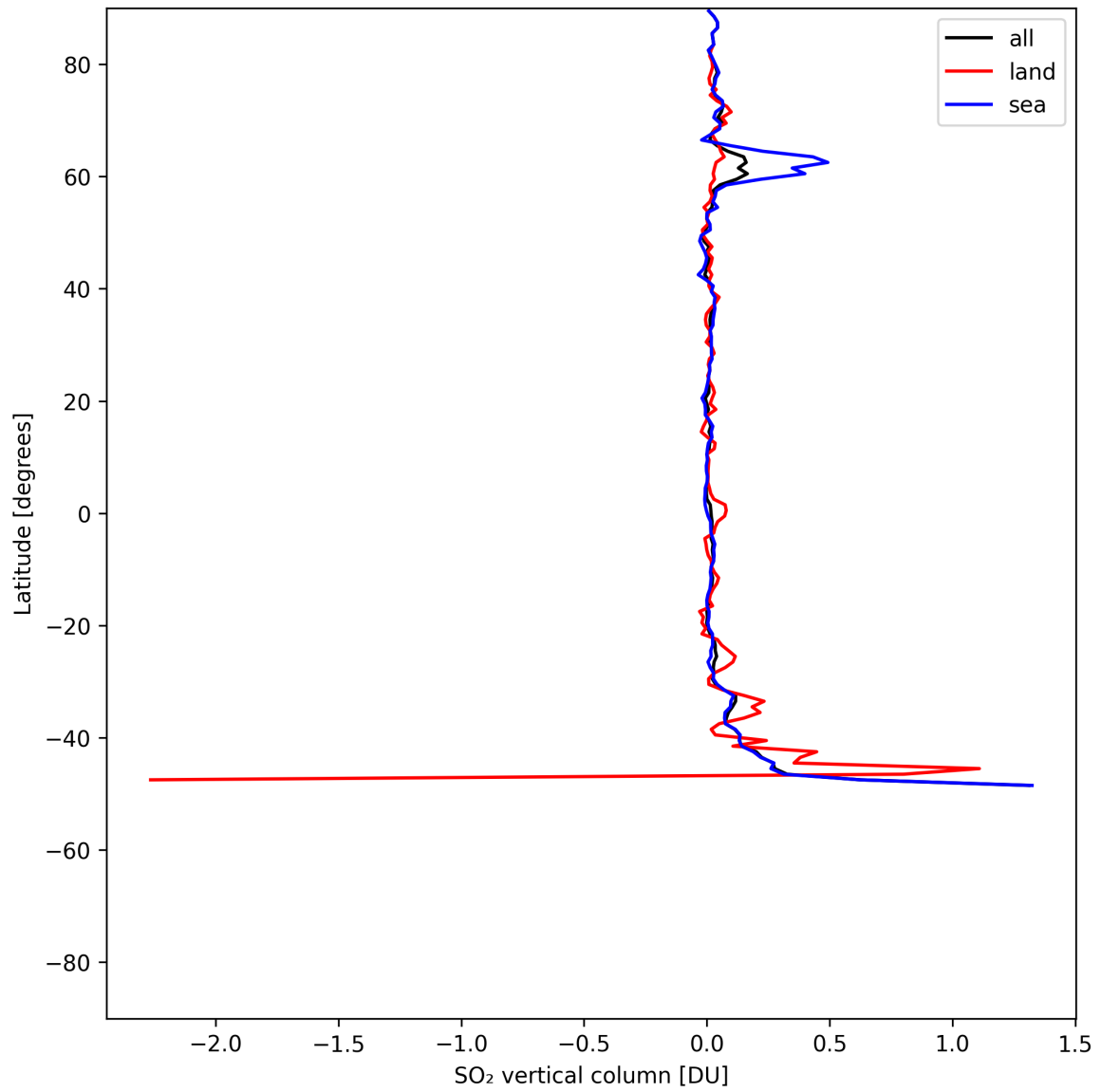
Figure 31: Zonal average of “SO 2 vertical column” for 2025-07-19 to 2025-07-20.
