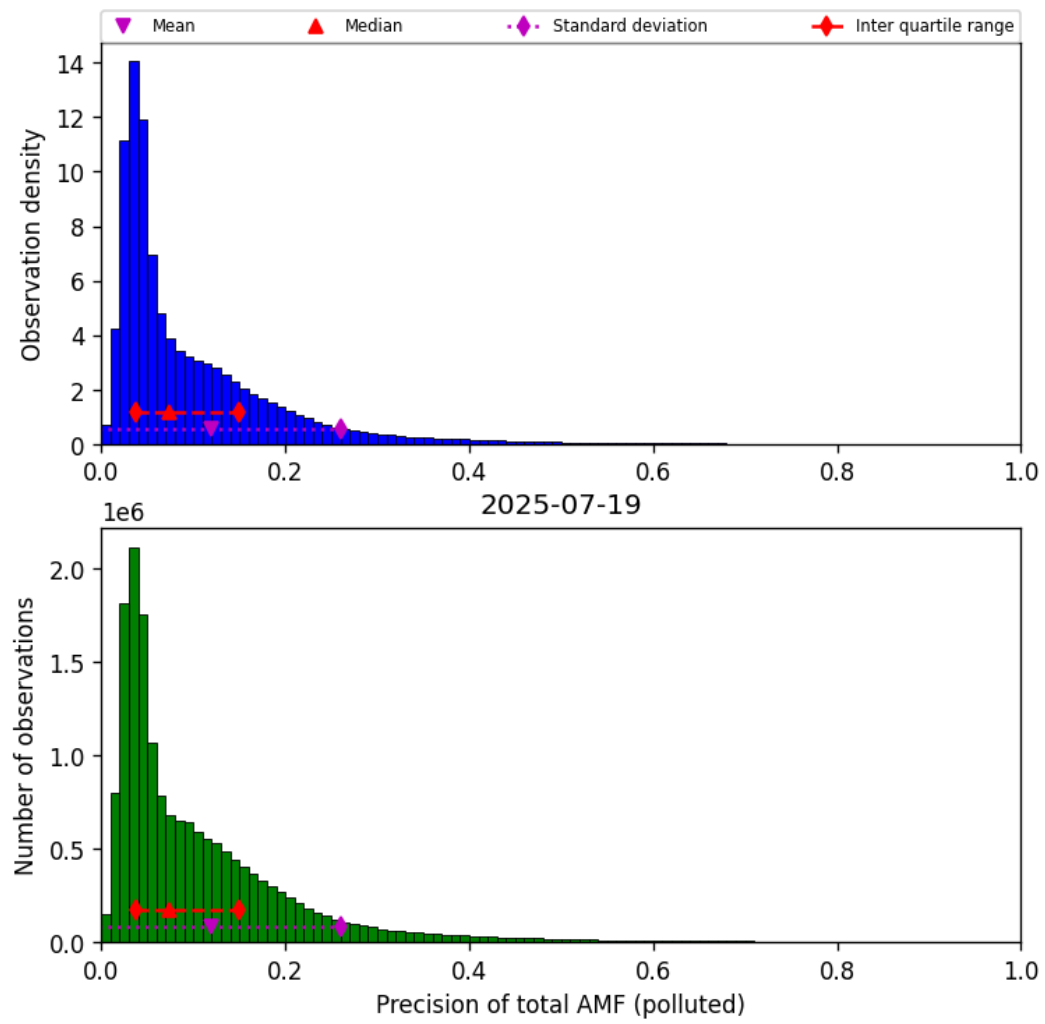
Figure 81: Histogram of “Precision of total AMF (polluted)” for 2025-07-19 to 2025-07-20
