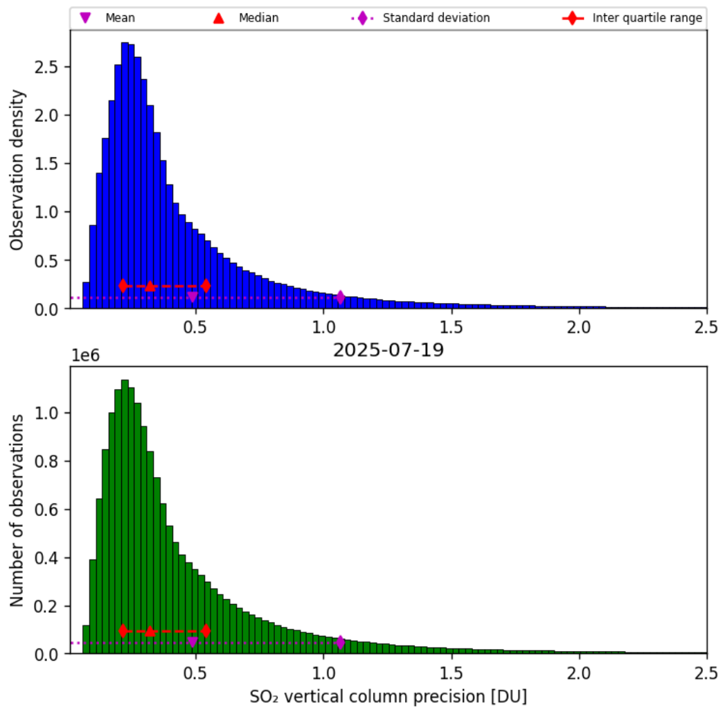
Figure 59: Histogram of “SO 2 vertical column precision” for 2025-07-19 to 2025-07-20
