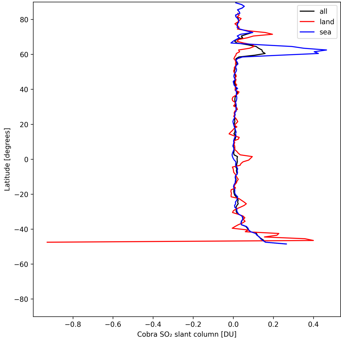
Figure 34: Zonal average of “Cobra SO 2 slant column” for 2025-07-19 to 2025-07-20.
