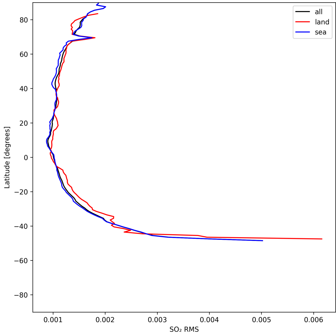
Figure 52: Zonal average of “SO 2 RMS” for 2025-07-19 to 2025-07-20.
