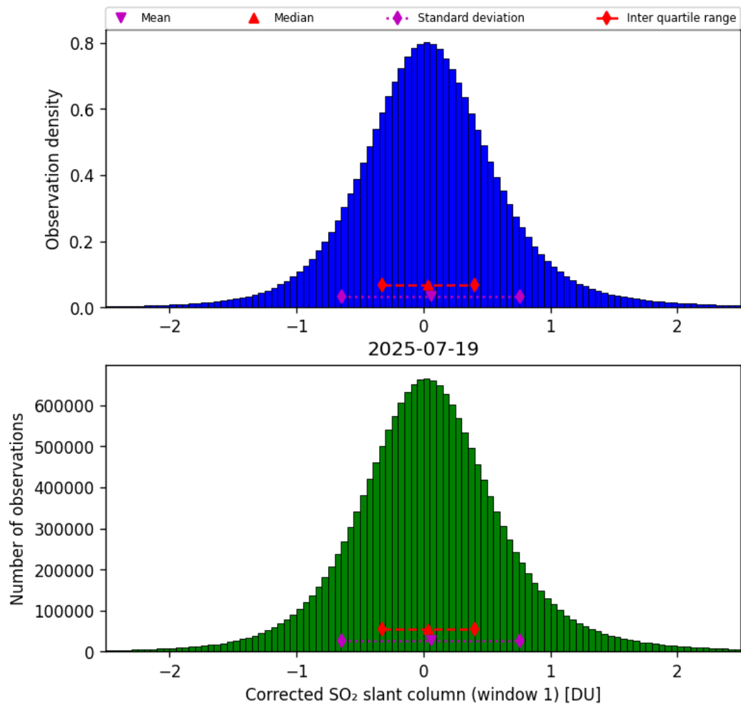
Figure 65: Histogram of “Corrected SO 2 slant column (window 1)” for 2025-07-19 to 2025-07-20
