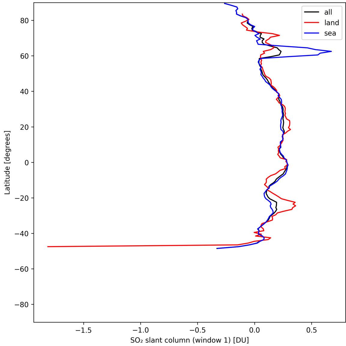
Figure 36: Zonal average of “SO 2 slant column (window 1)” for 2025-07-19 to 2025-07-20.
