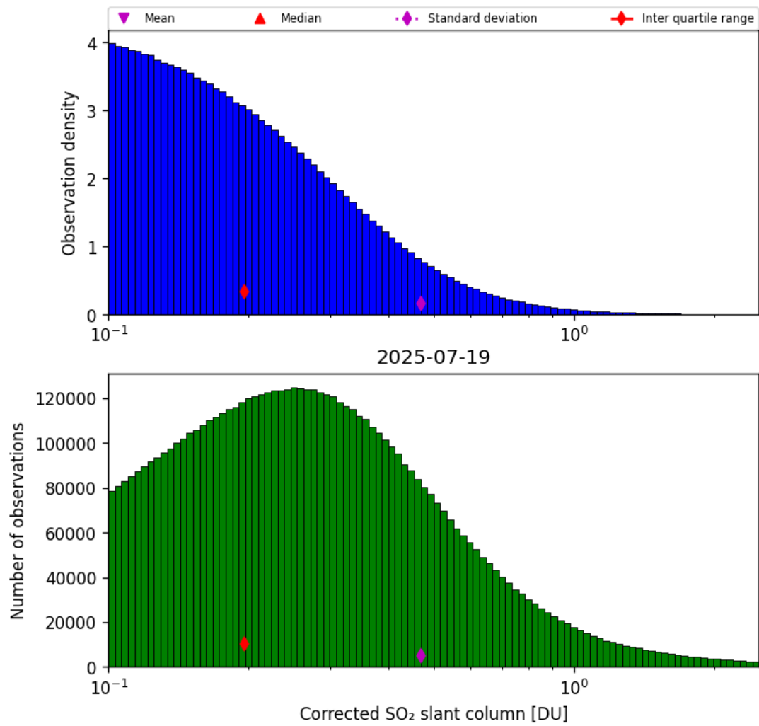
Figure 60: Histogram of “Corrected SO 2 slant column” for 2025-07-19 to 2025-07-20
