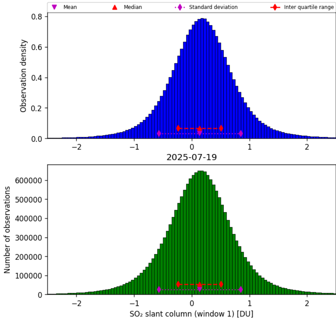
Figure 63: Histogram of “SO 2 slant column (window 1)” for 2025-07-19 to 2025-07-20
