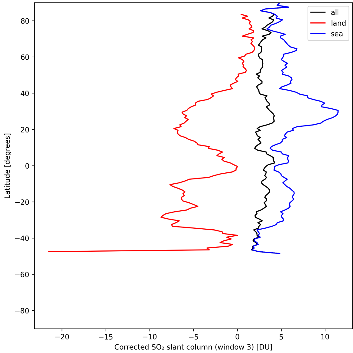
Figure 46: Zonal average of “Corrected SO 2 slant column (window 3)” for 2025-07-19 to 2025-07-20.
