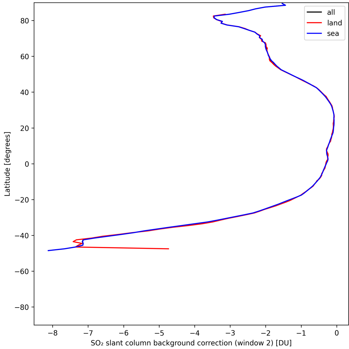
Figure 43: Zonal average of “SO 2 slant column background correction (window 2)” for 2025-07-19 to 2025-07-20.
