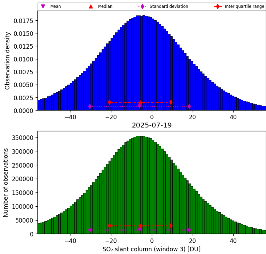
Figure 71: Histogram of “SO 2 slant column (window 3)” for 2025-07-19 to 2025-07-20
