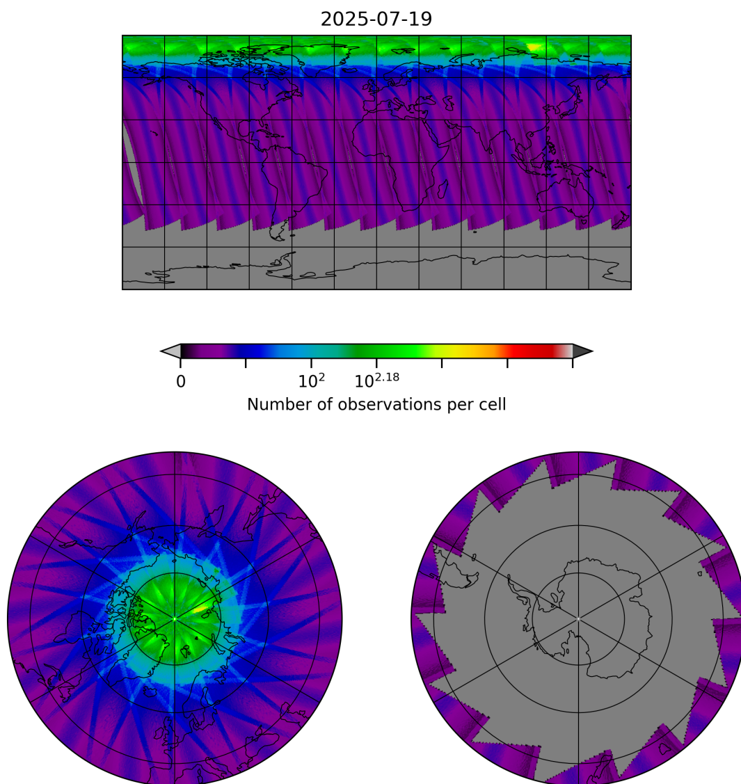
Figure 29: Map of the number of observations for 2025-07-19 to 2025-07-20
