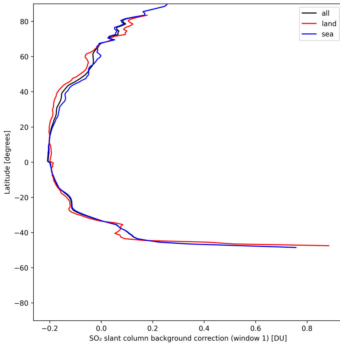
Figure 39: Zonal average of “SO 2 slant column background correction (window 1)” for 2025-07-19 to 2025-07-20.
