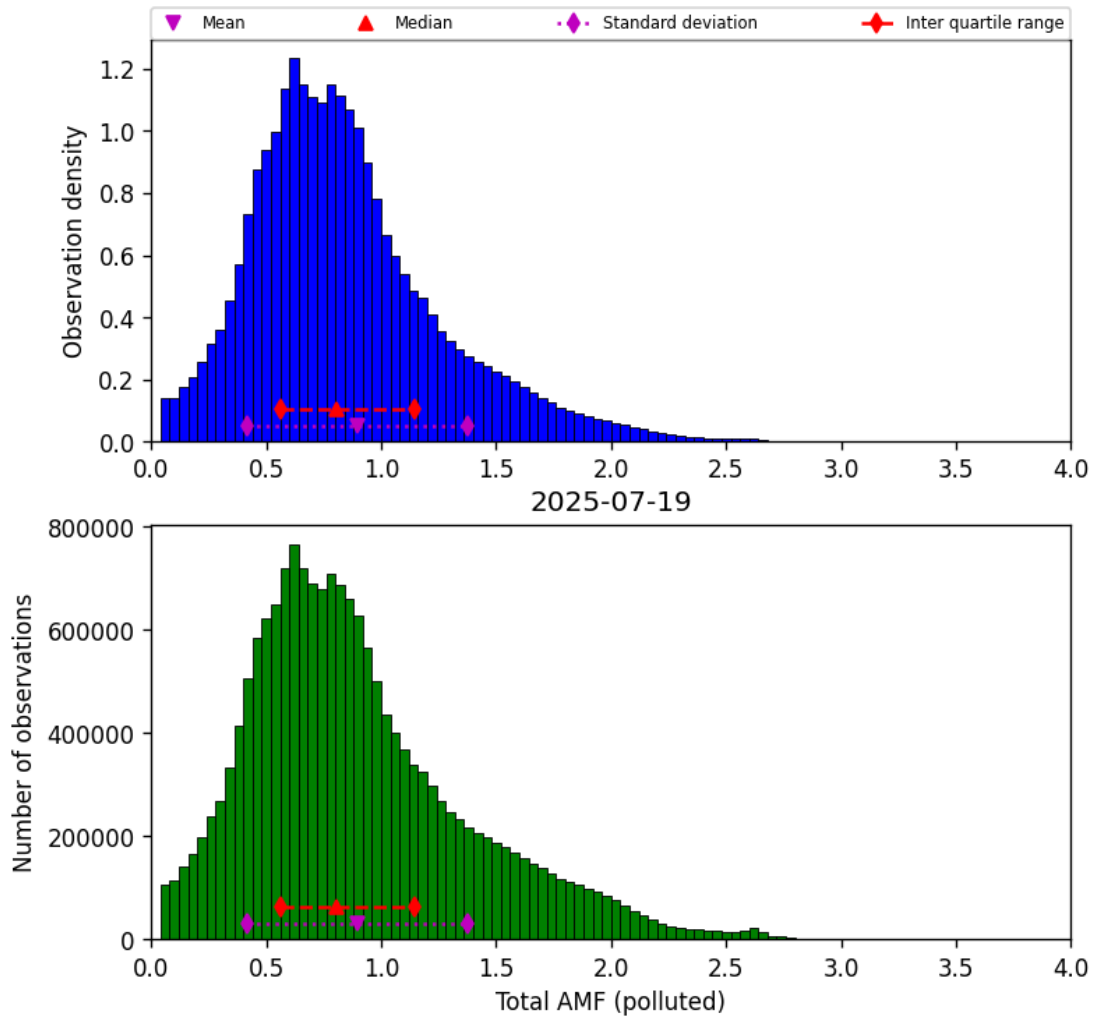
Figure 80: Histogram of “Total AMF (polluted)” for 2025-07-19 to 2025-07-20
