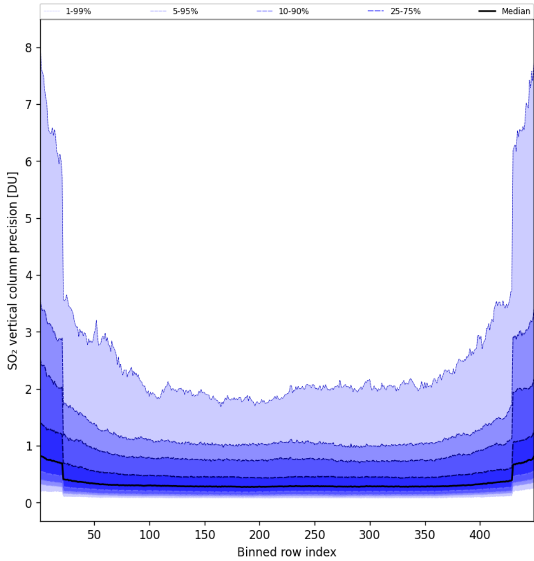
Figure 86: Along track statistics of “SO 2 vertical column precision” for 2025-07-19 to 2025-07-20
