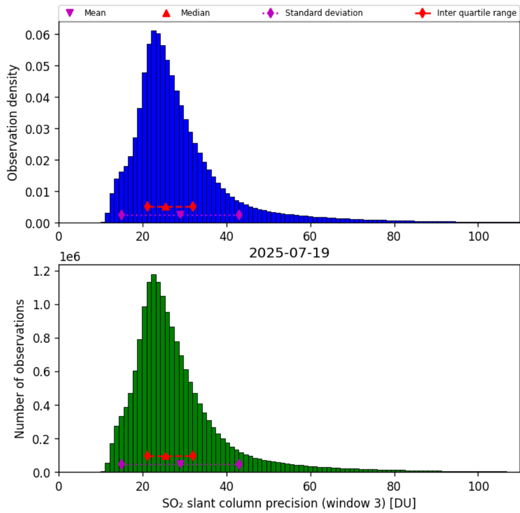
Figure 72: Histogram of “SO 2 slant column precision (window 3)” for 2025-07-19 to 2025-07-20
