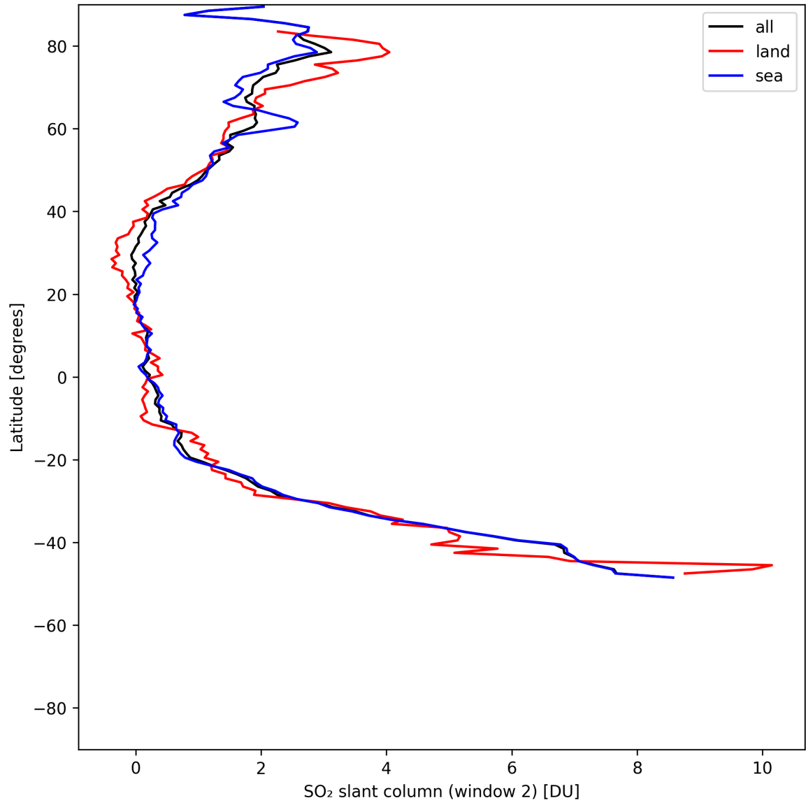
Figure 40: Zonal average of “SO 2 slant column (window 2)” for 2025-07-19 to 2025-07-20.
