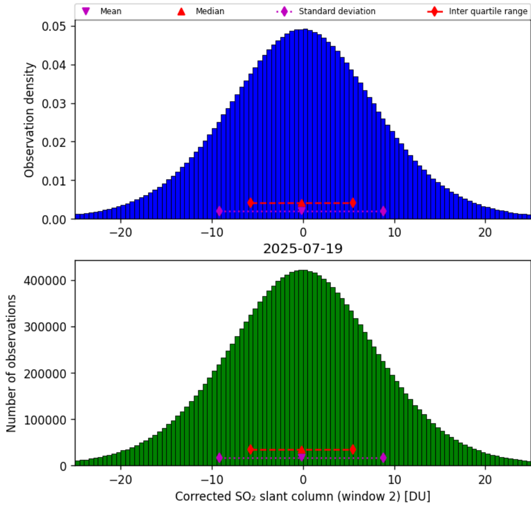
Figure 69: Histogram of “Corrected SO 2 slant column (window 2)” for 2025-07-19 to 2025-07-20
