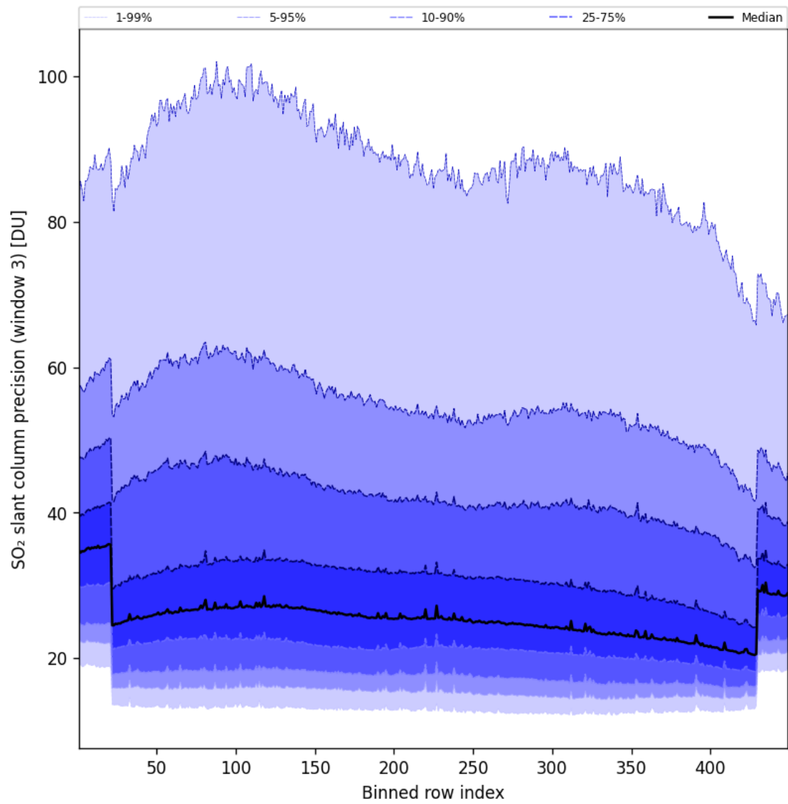
Figure 99: Along track statistics of “SO 2 slant column precision (window 3)” for 2025-07-19 to 2025-07-20
