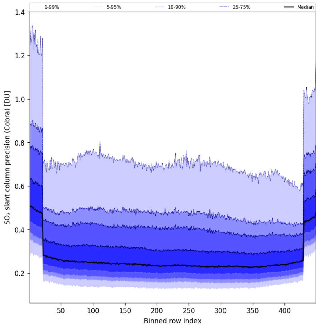
Figure 89: Along track statistics of “SO 2 slant column precision (Cobra)” for 2025-07-19 to 2025-07-20
