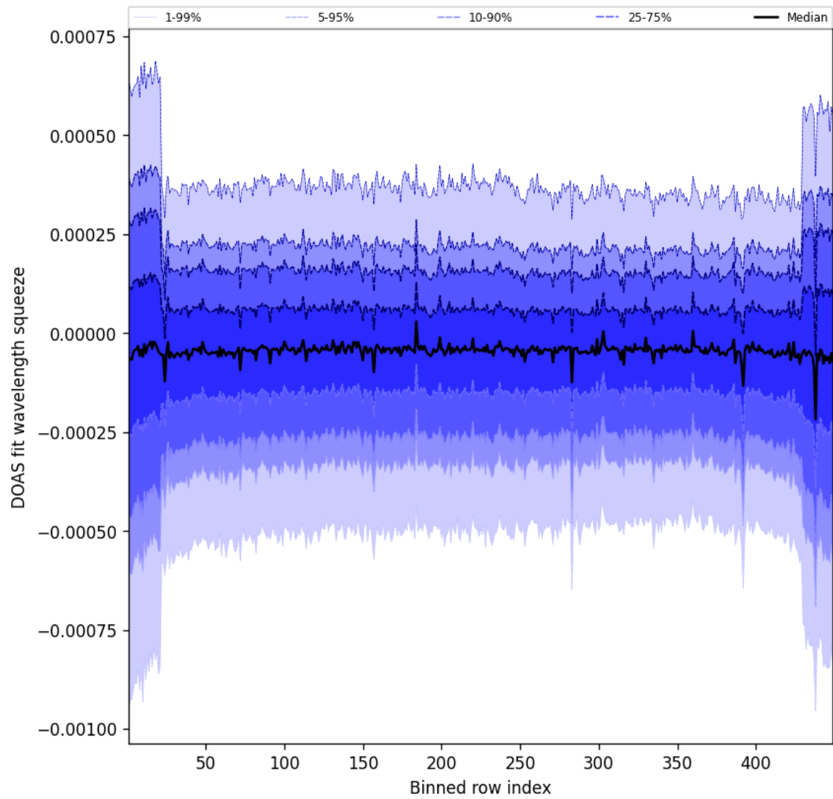
Figure 105: Along track statistics of “DOAS fit wavelength squeeze” for 2025-07-19 to 2025-07-20
