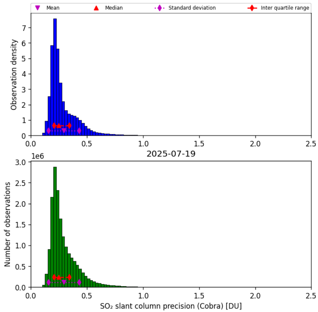
Figure 62: Histogram of “SO 2 slant column precision (Cobra)” for 2025-07-19 to 2025-07-20
