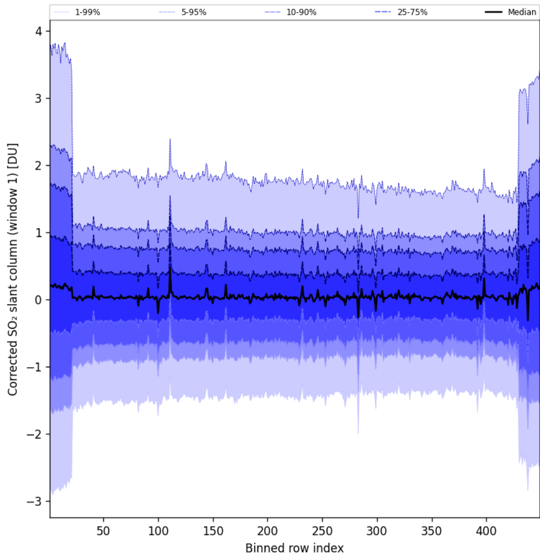
Figure 92: Along track statistics of “Corrected SO 2 slant column (window 1)” for 2025-07-19 to 2025-07-20
