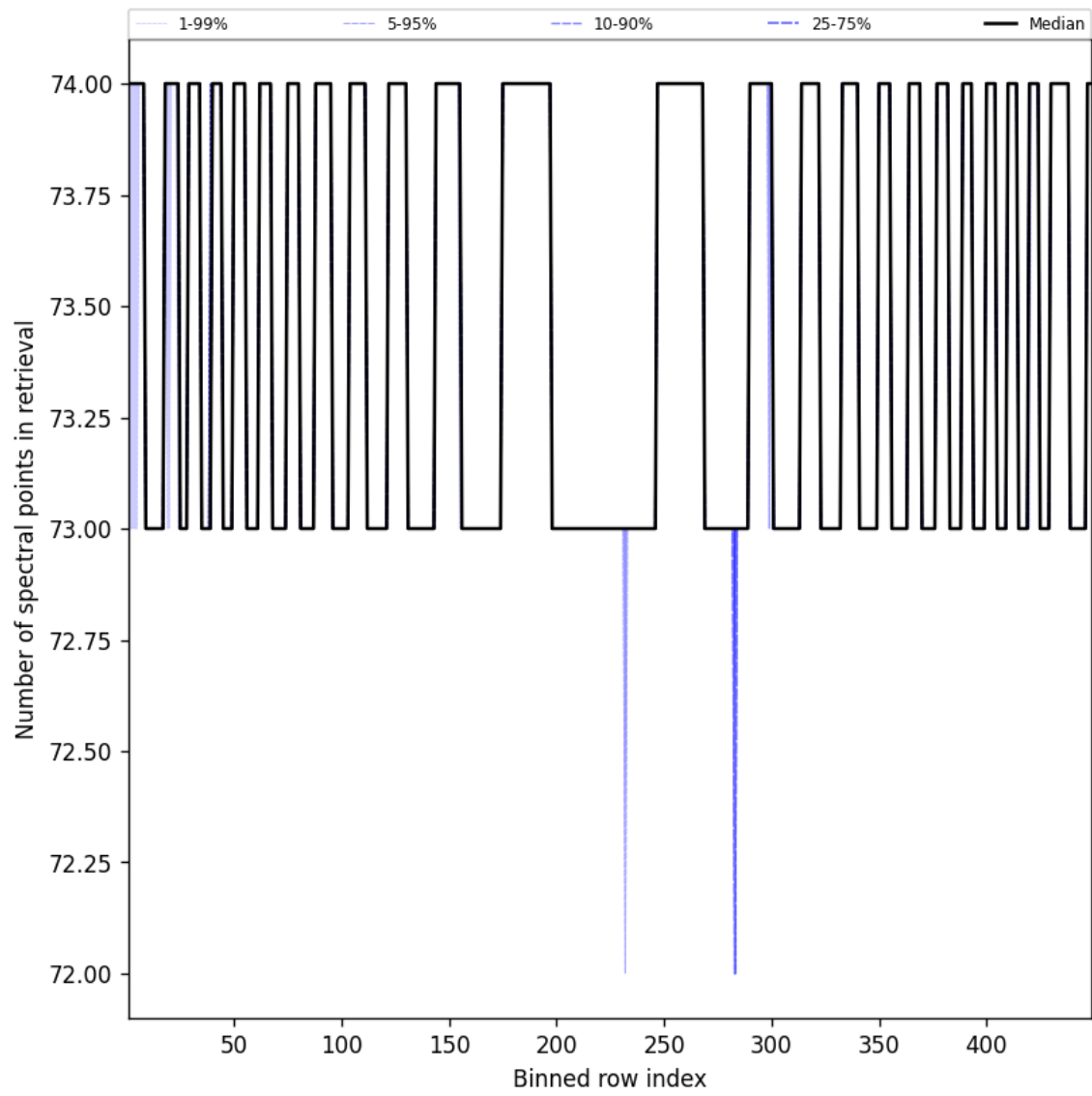
Figure 110: Along track statistics of “Number of spectral points in retrieval” for 2025-07-19 to 2025-07-20
