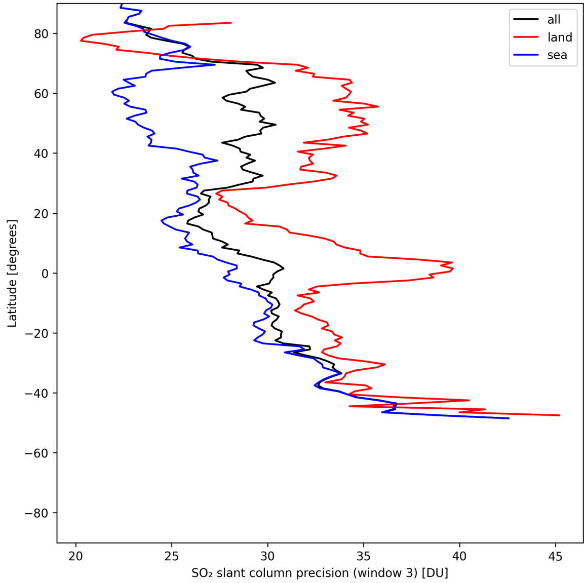
Figure 45: Zonal average of “SO 2 slant column precision (window 3)” for 2025-07-19 to 2025-07-20.
