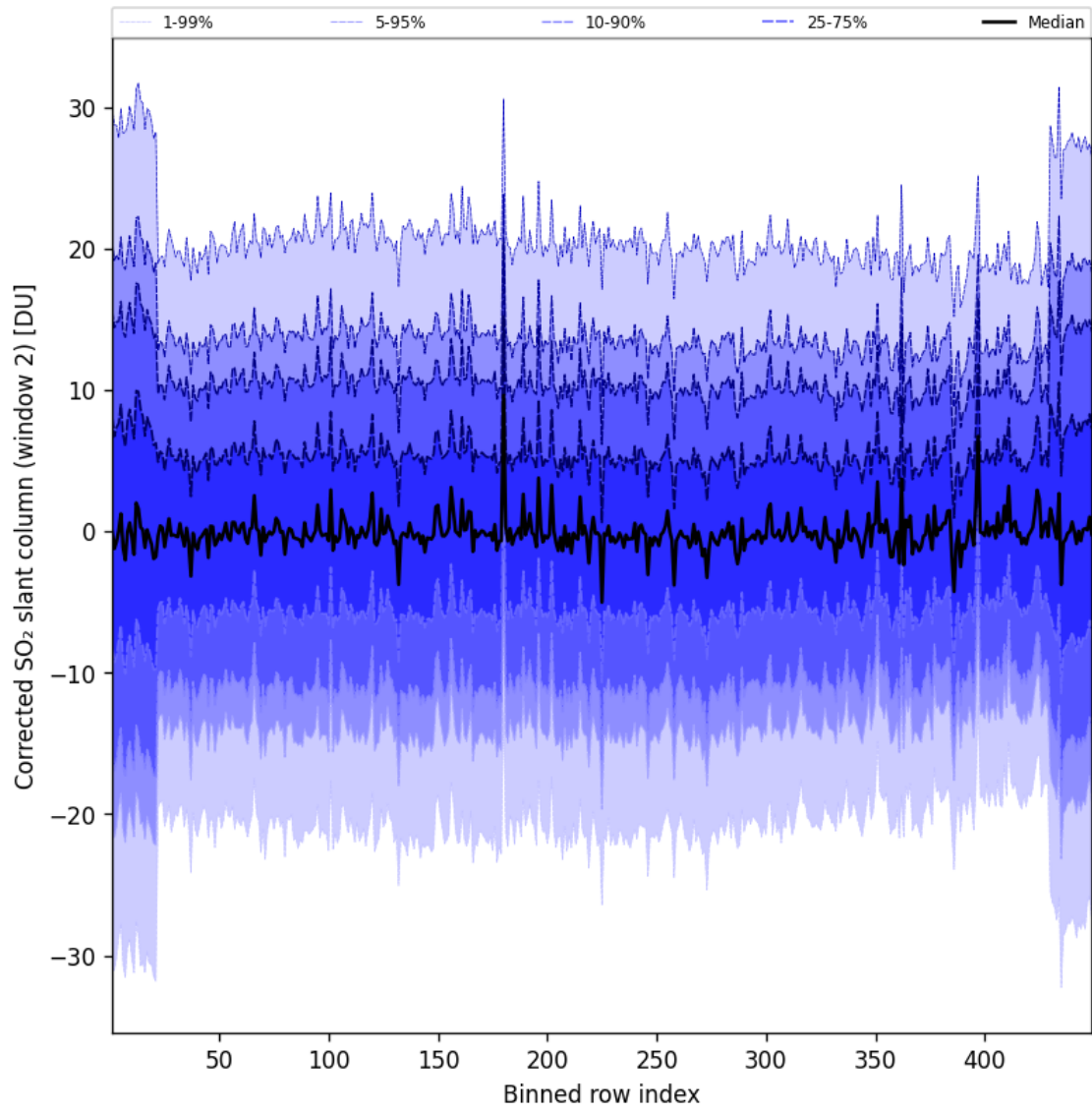
Figure 96: Along track statistics of “Corrected SO 2 slant column (window 2)” for 2025-07-19 to 2025-07-20
