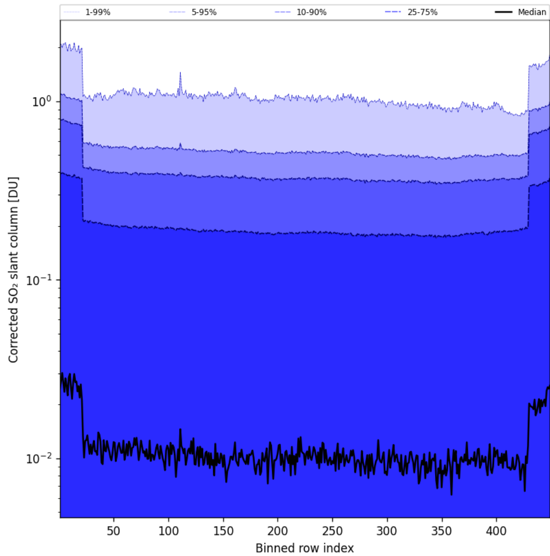
Figure 87: Along track statistics of “Corrected SO 2 slant column” for 2025-07-19 to 2025-07-20
