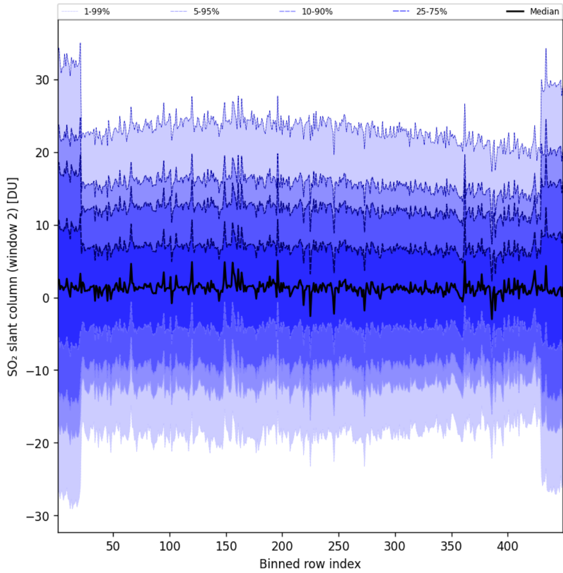
Figure 94: Along track statistics of “SO 2 slant column (window 2)” for 2025-07-19 to 2025-07-20
