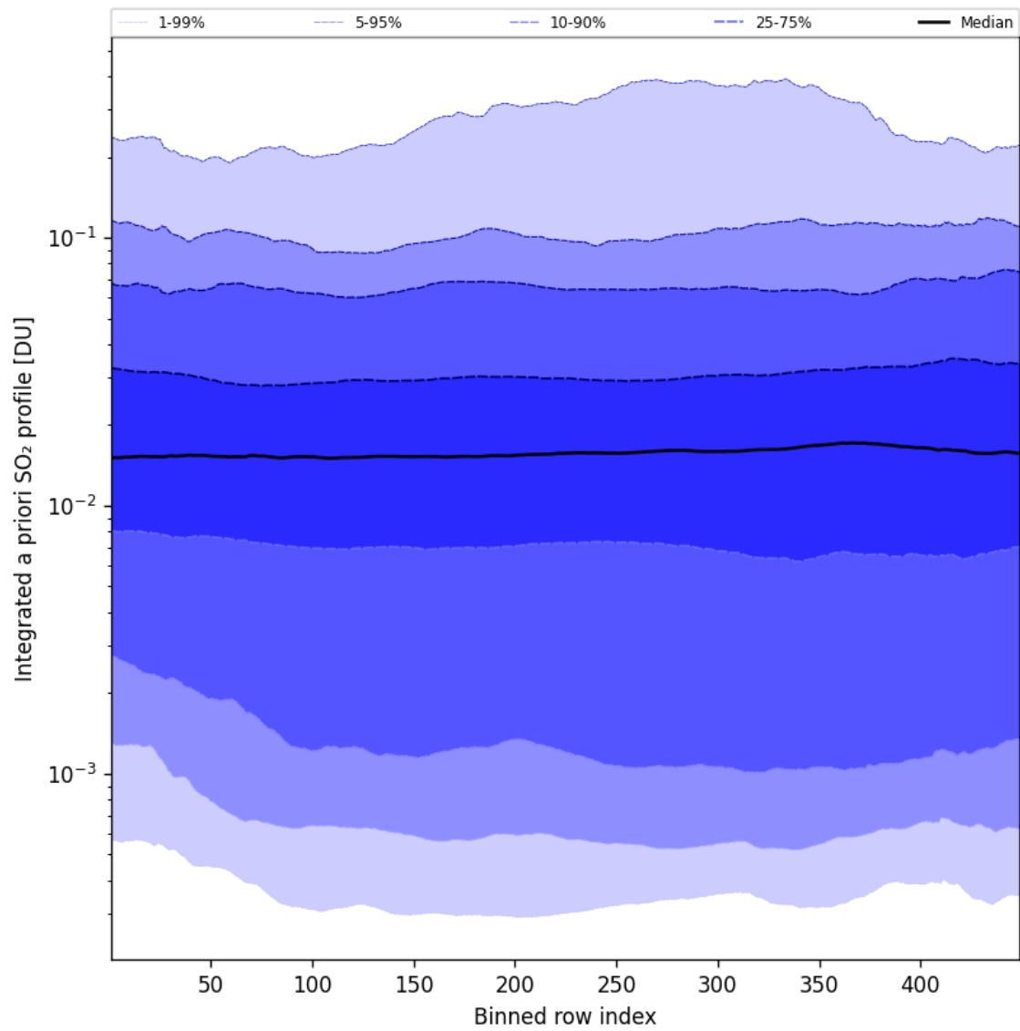
Figure 103: Along track statistics of “Integrated a priori SO 2 profile” for 2025-07-19 to 2025-07-20
