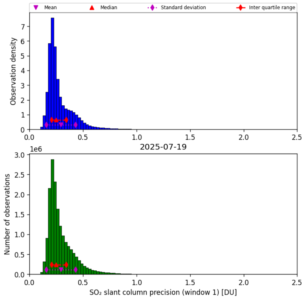
Figure 64: Histogram of “SO 2 slant column precision (window 1)” for 2025-07-19 to 2025-07-20
