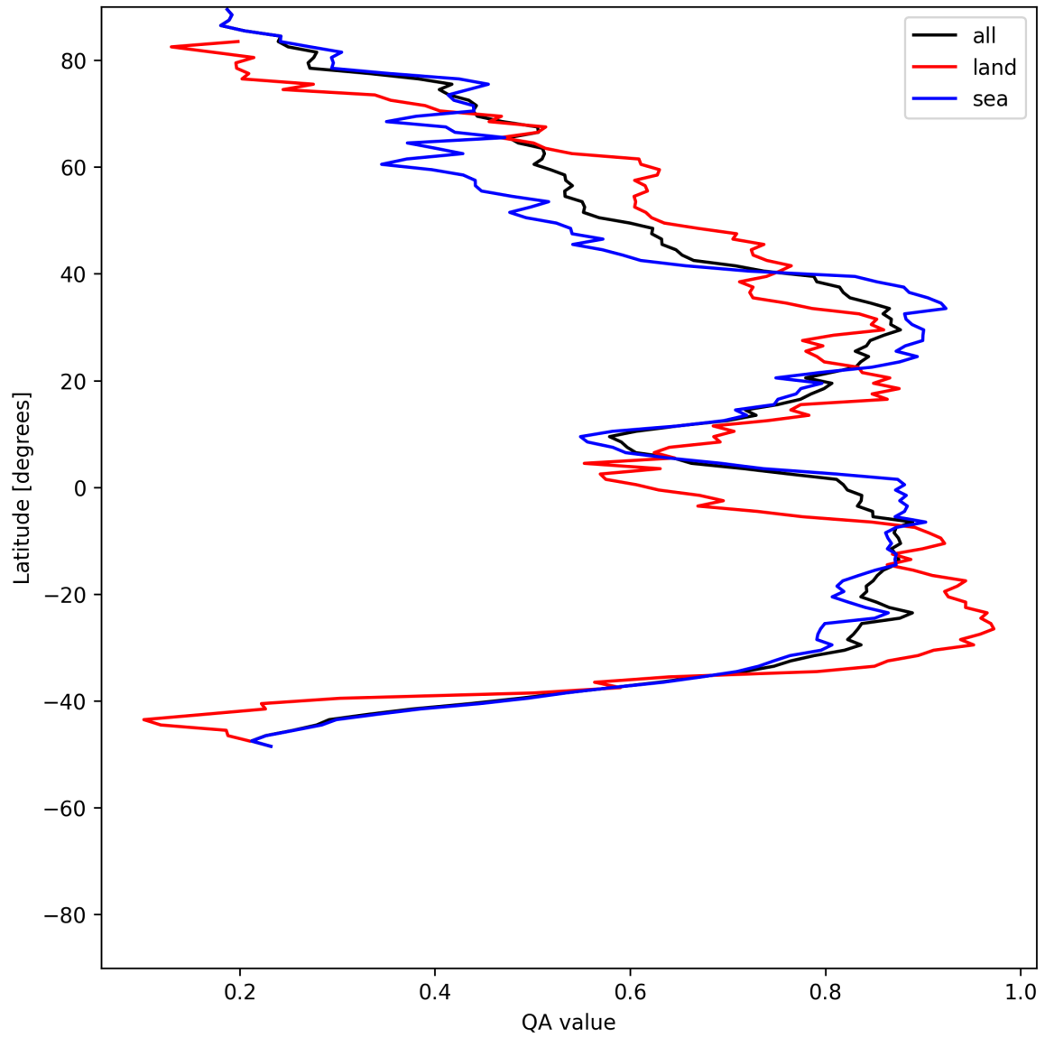
Figure 30: Zonal average of “QA value” for 2025-07-19 to 2025-07-20.
