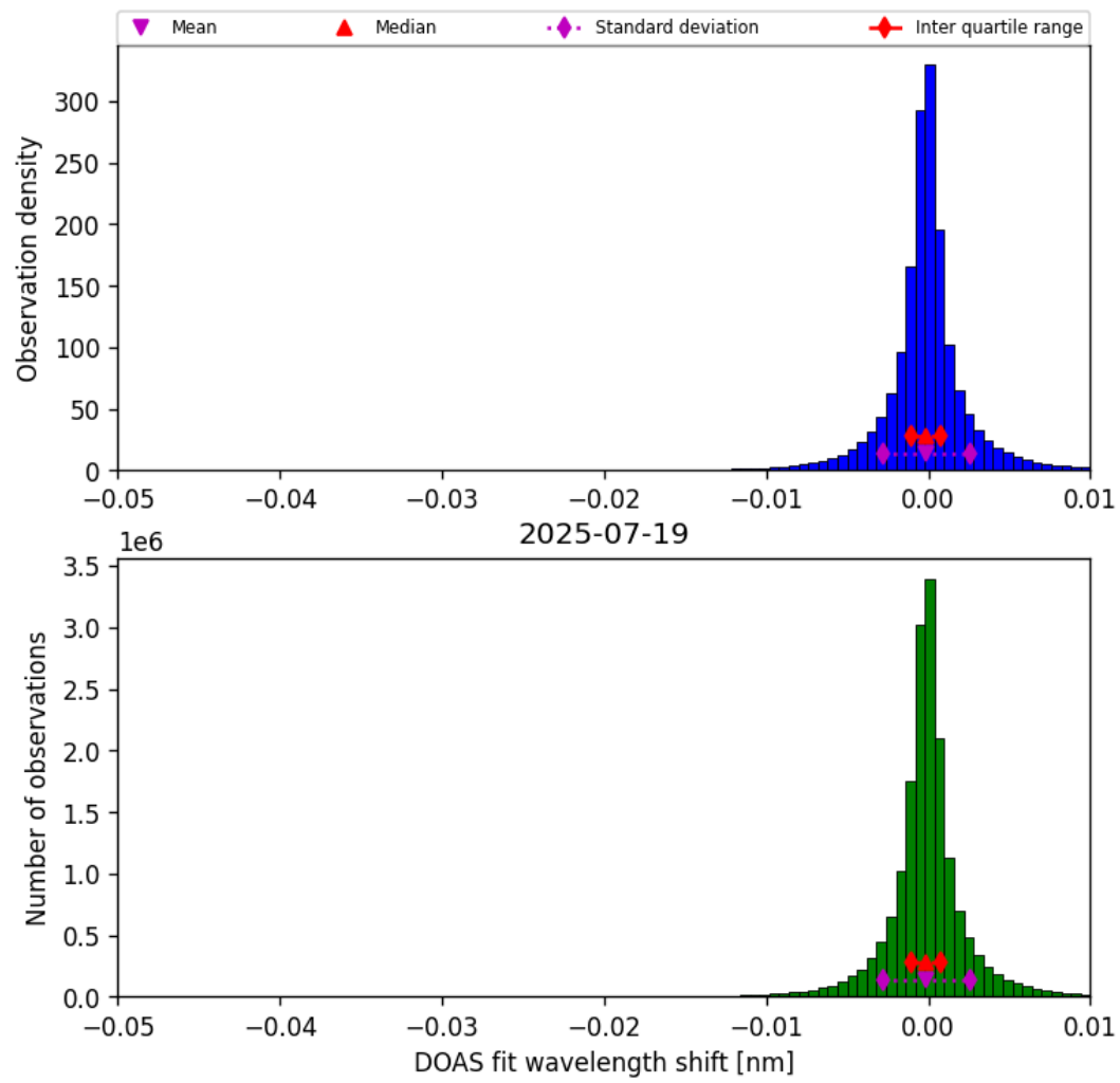
Figure 77: Histogram of “DOAS fit wavelength shift” for 2025-07-19 to 2025-07-20
