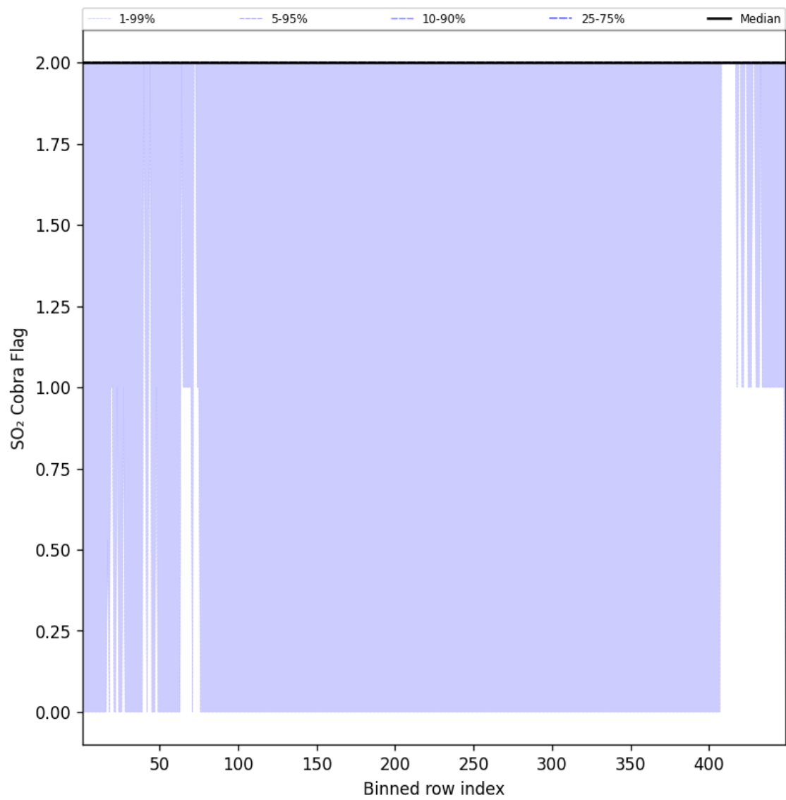
Figure 102: Along track statistics of “SO 2 Cobra Flag” for 2025-07-19 to 2025-07-20
