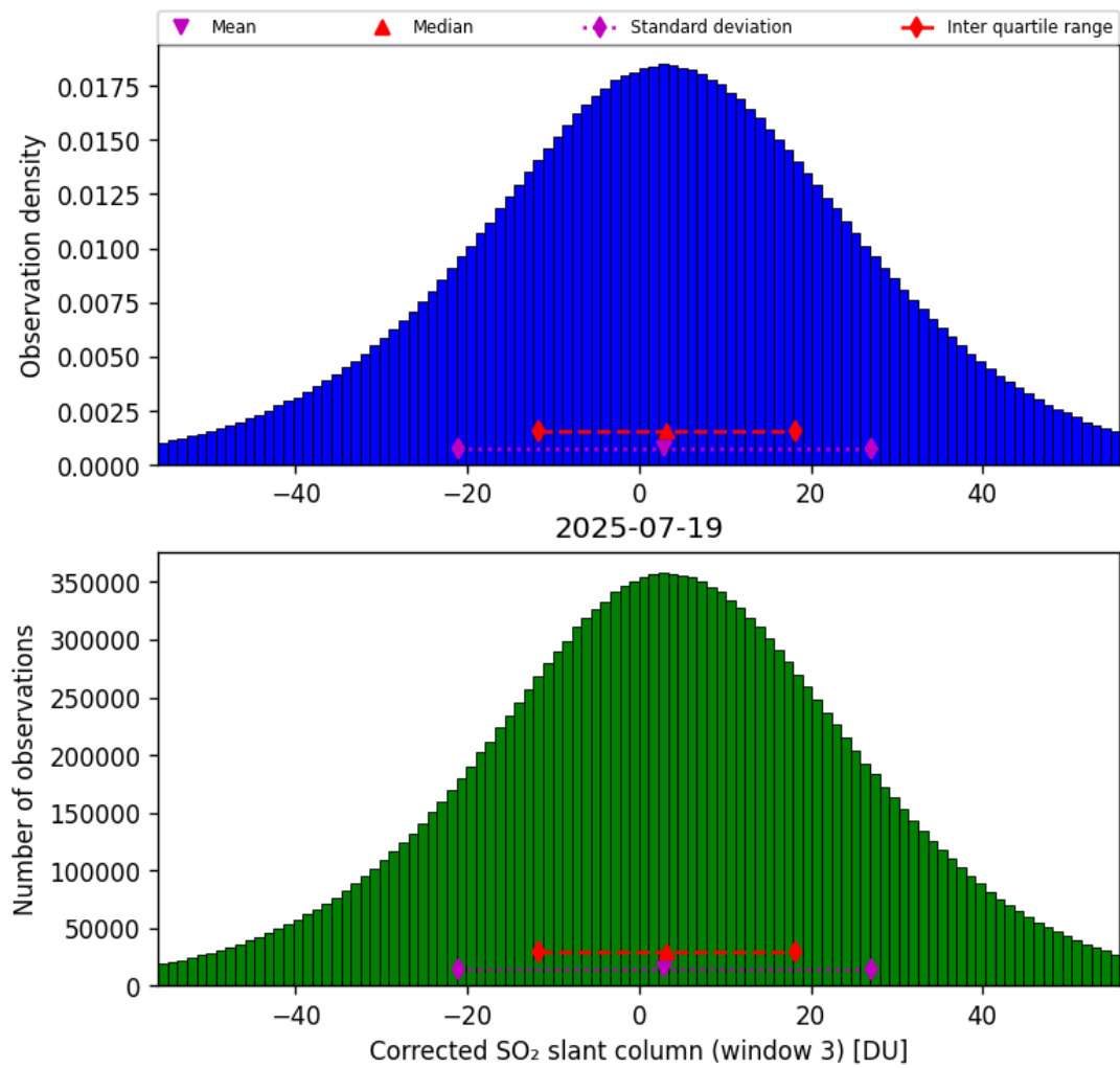
Figure 73: Histogram of “Corrected SO 2 slant column (window 3)” for 2025-07-19 to 2025-07-20
