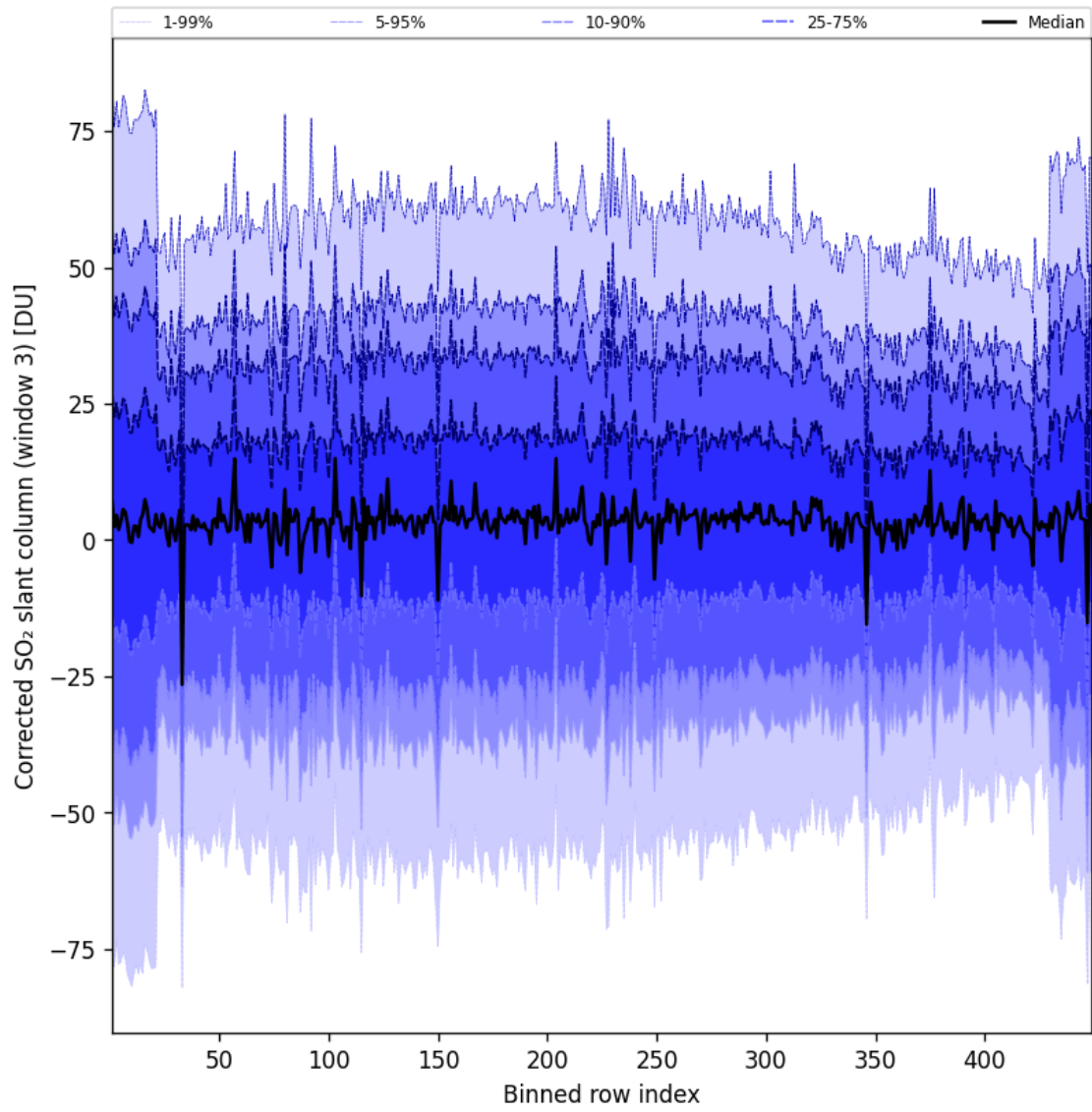
Figure 100: Along track statistics of “Corrected SO 2 slant column (window 3)” for 2025-07-19 to 2025-07-20
