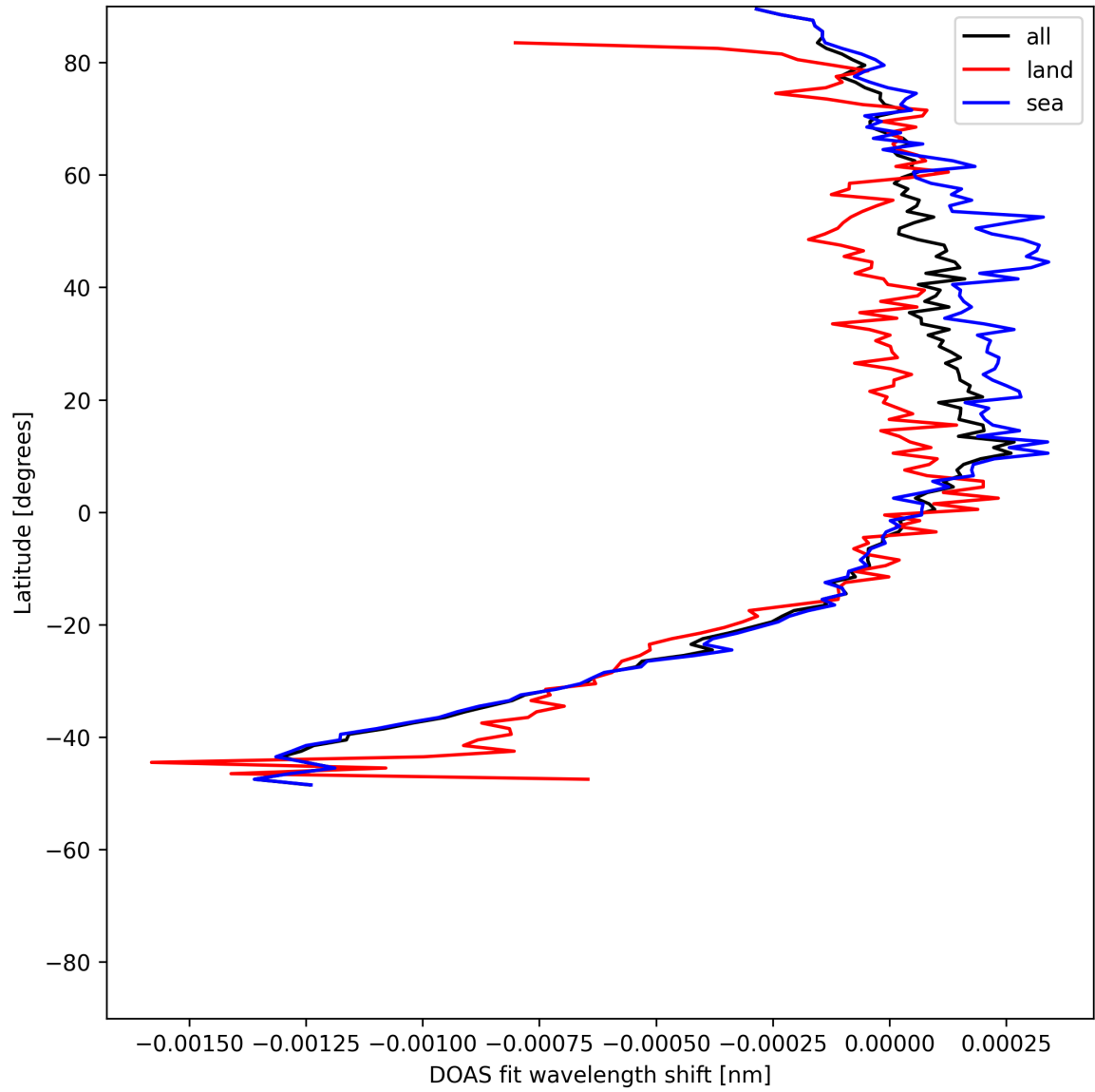
Figure 50: Zonal average of “DOAS fit wavelength shift” for 2025-07-19 to 2025-07-20.
