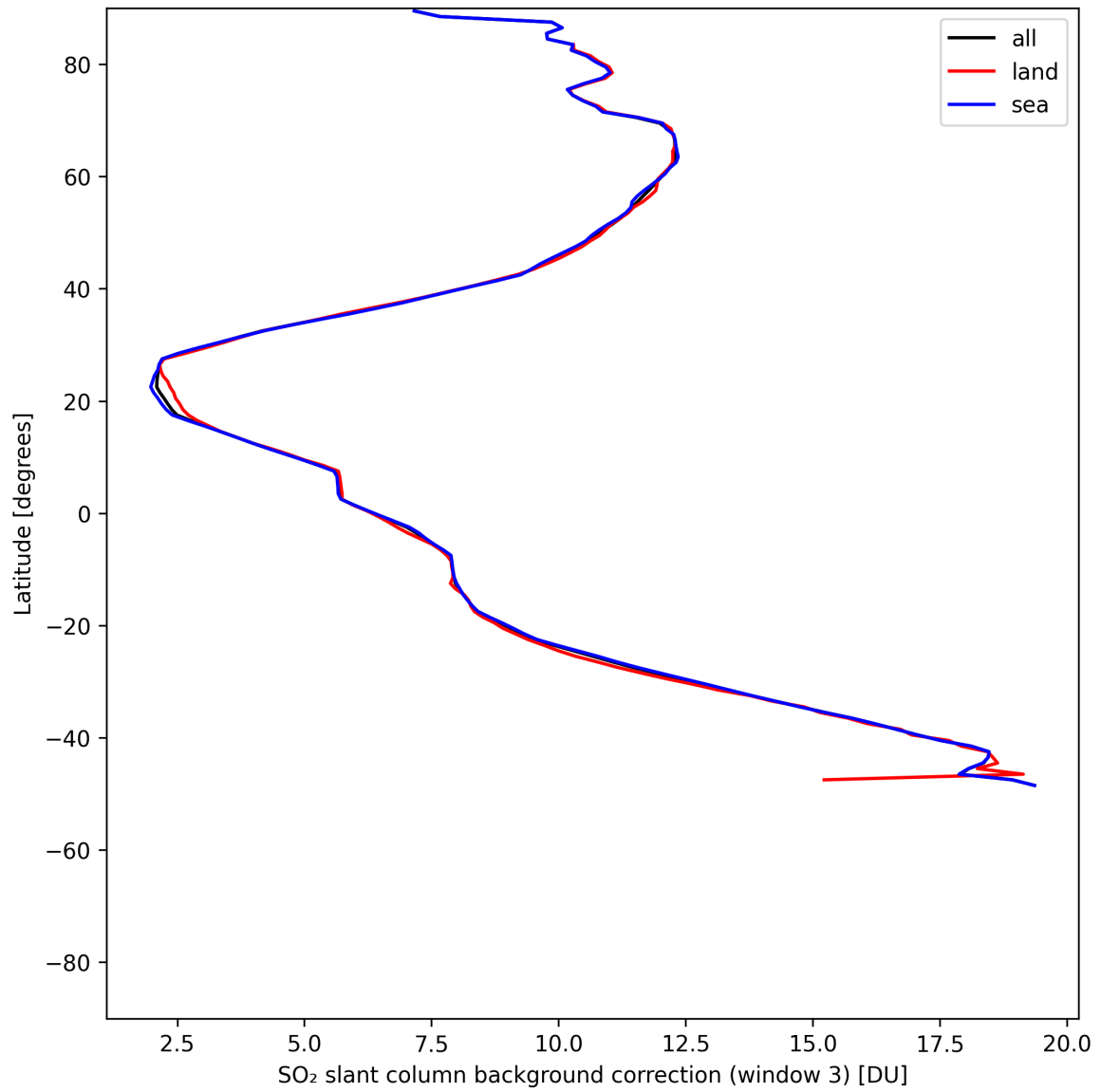
Figure 47: Zonal average of “SO 2 slant column background correction (window 3)” for 2025-07-19 to 2025-07-20.
