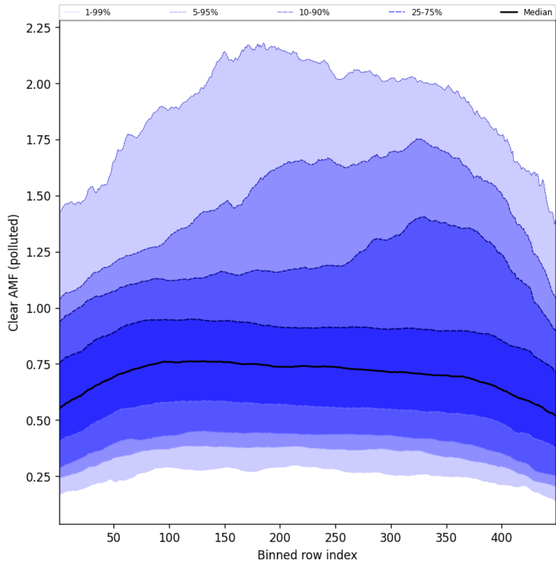
Figure 109: Along track statistics of “Clear AMF (polluted)” for 2025-07-19 to 2025-07-20
