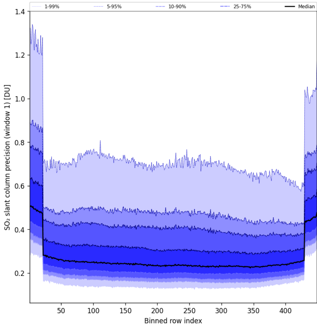
Figure 91: Along track statistics of “SO 2 slant column precision (window 1)” for 2025-07-19 to 2025-07-20
