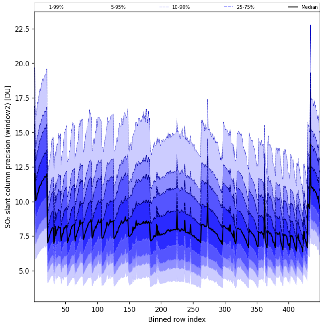
Figure 95: Along track statistics of “SO 2 slant column precision (window2)” for 2025-07-19 to 2025-07-20
