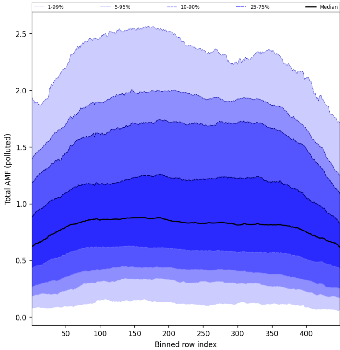
Figure 107: Along track statistics of “Total AMF (polluted)” for 2025-07-19 to 2025-07-20
