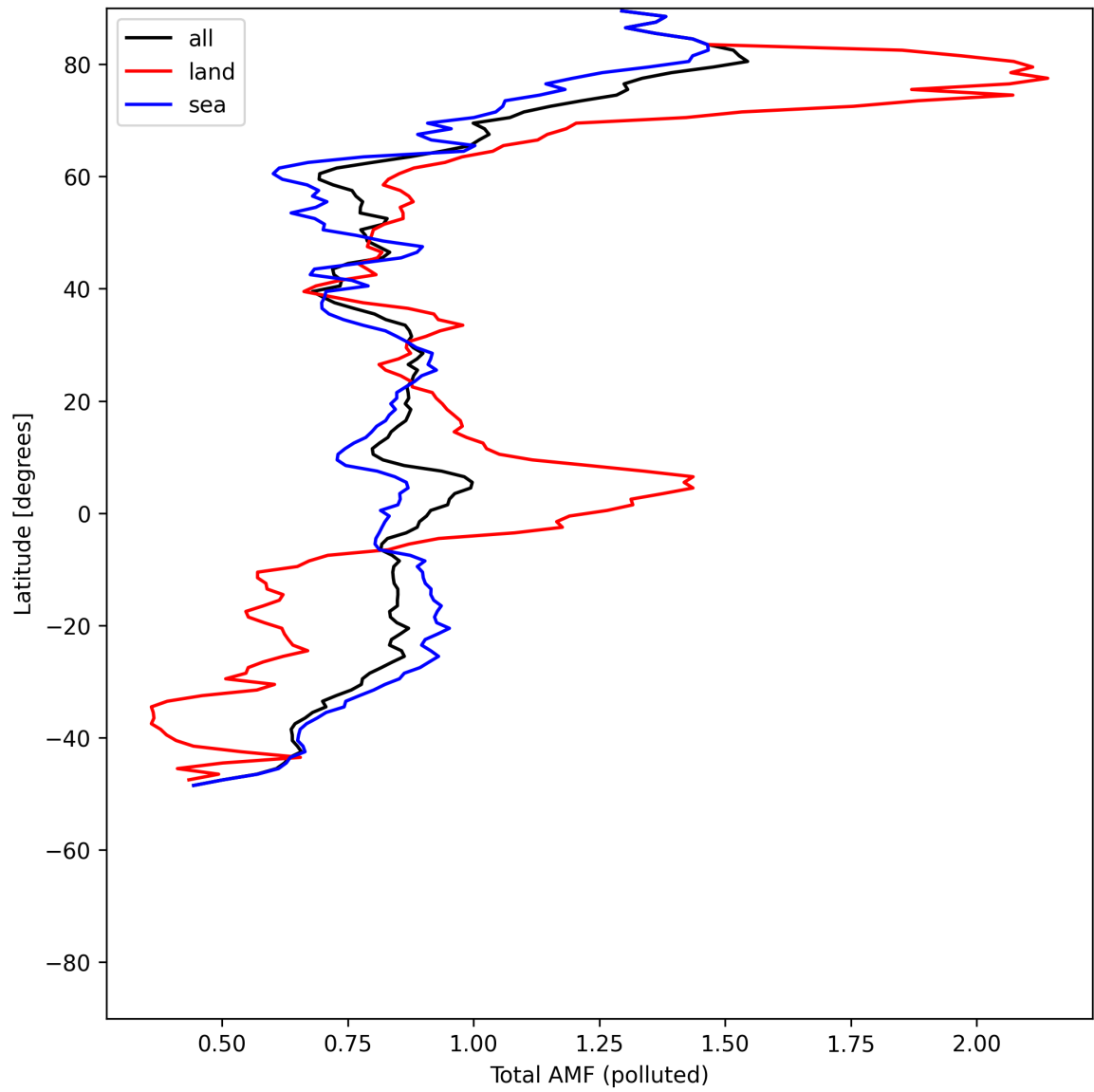
Figure 53: Zonal average of “Total AMF (polluted)” for 2025-07-19 to 2025-07-20.
