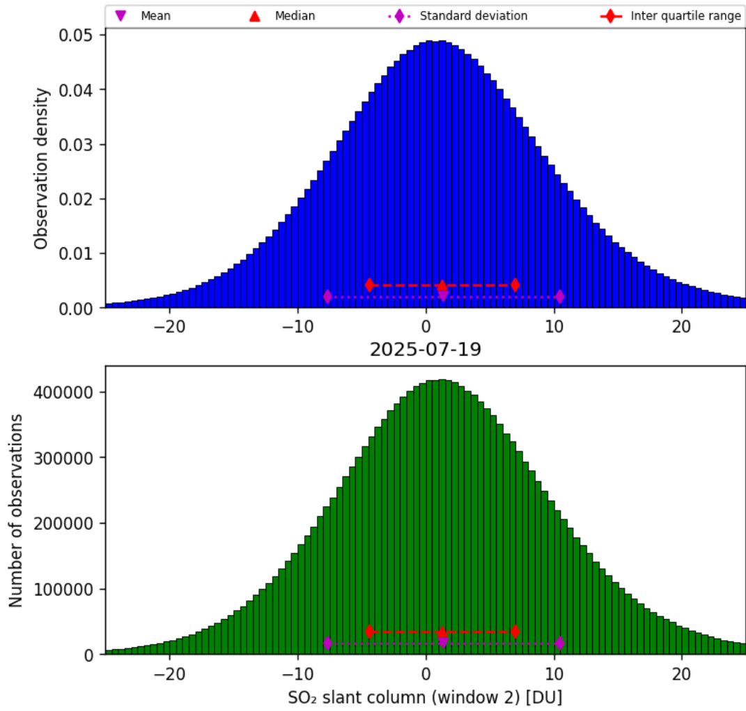
Figure 67: Histogram of “SO 2 slant column (window 2)” for 2025-07-19 to 2025-07-20
