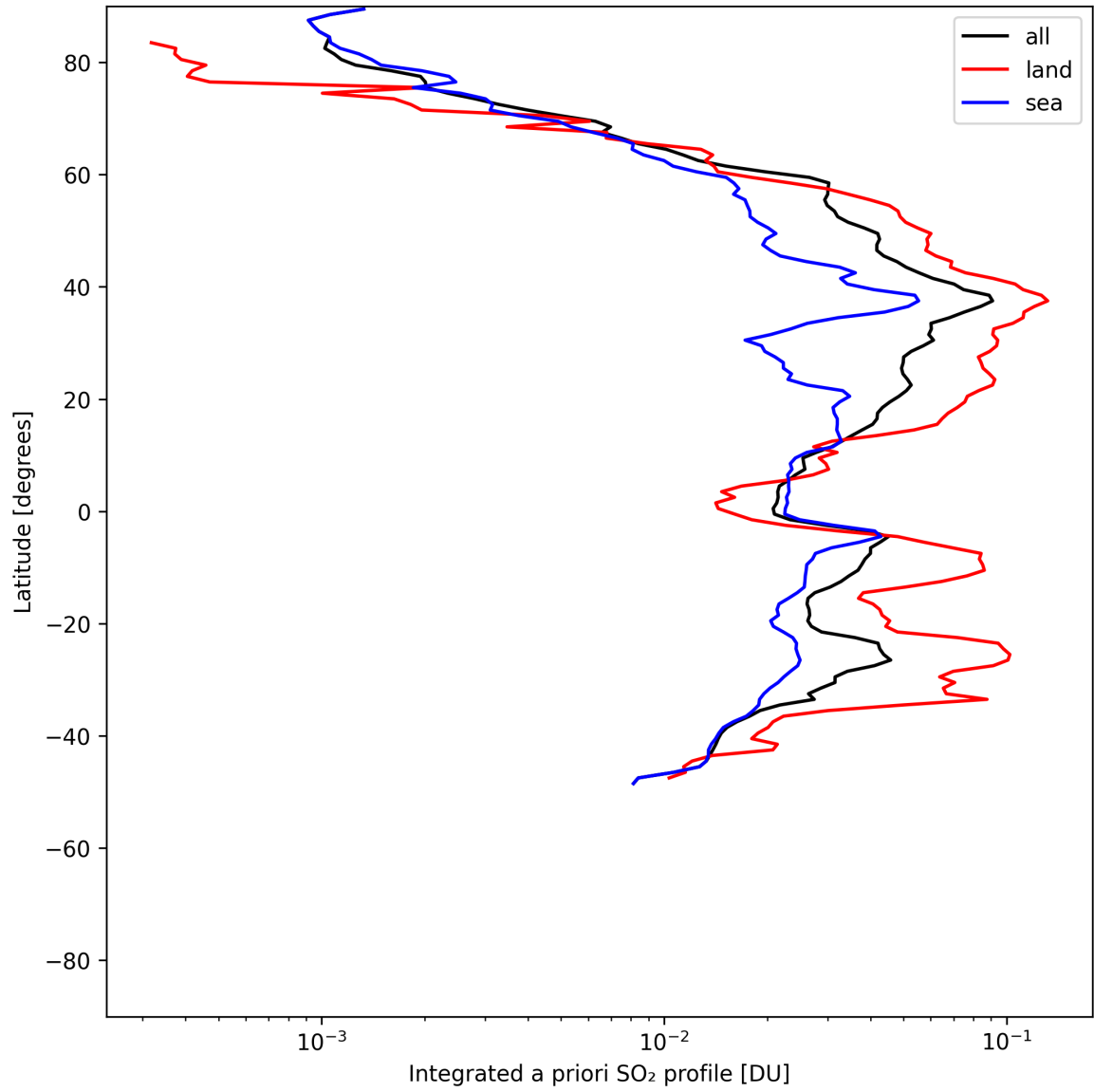
Figure 49: Zonal average of “Integrated a priori SO 2 profile” for 2025-07-19 to 2025-07-20.
