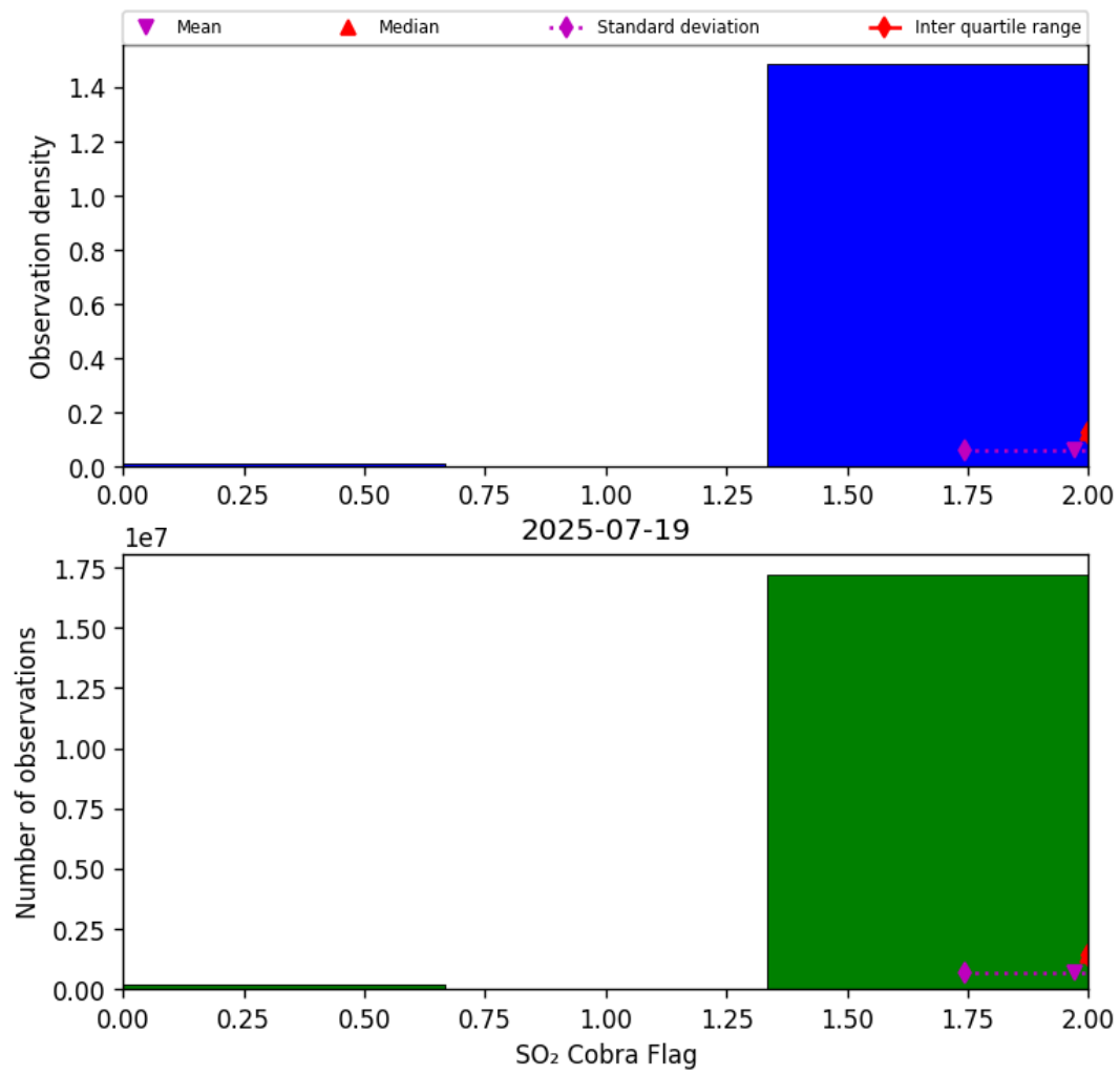
Figure 75: Histogram of “SO 2 Cobra Flag” for 2025-07-19 to 2025-07-20
