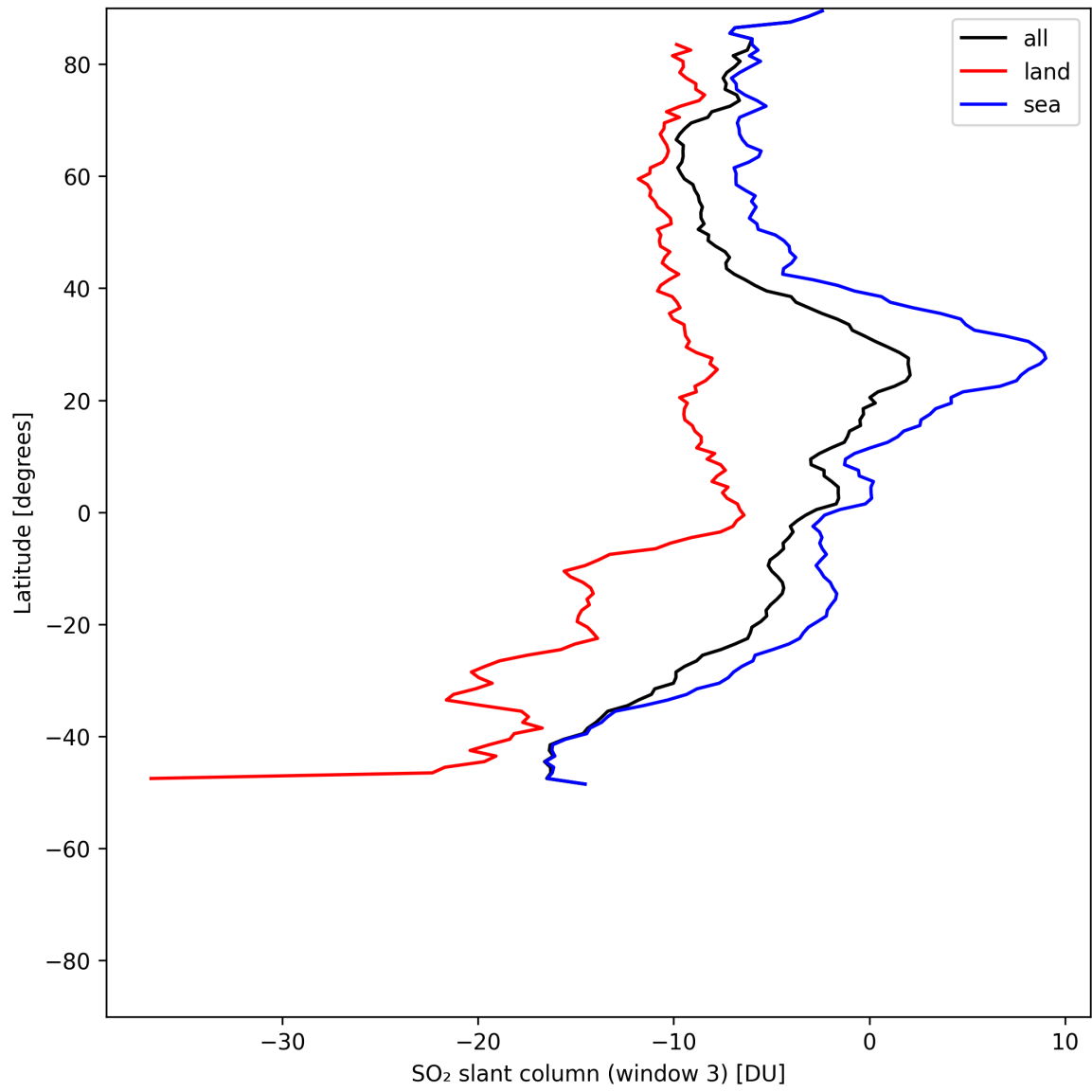
Figure 44: Zonal average of “SO 2 slant column (window 3)” for 2025-07-19 to 2025-07-20.
