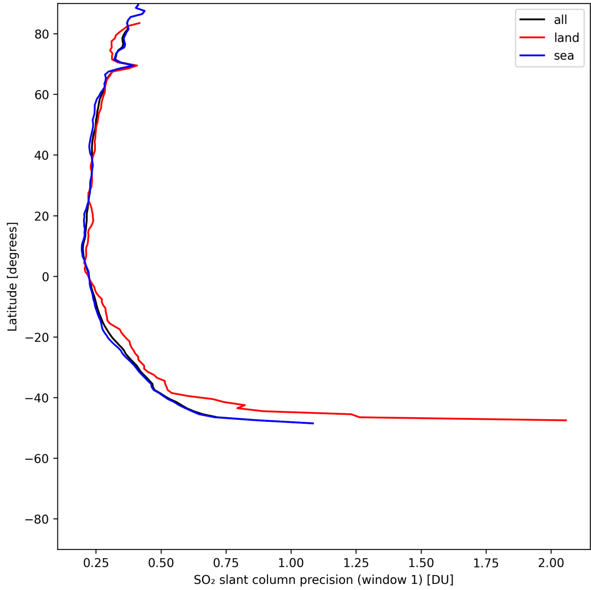
Figure 37: Zonal average of “SO 2 slant column precision (window 1)” for 2025-07-19 to 2025-07-20.
