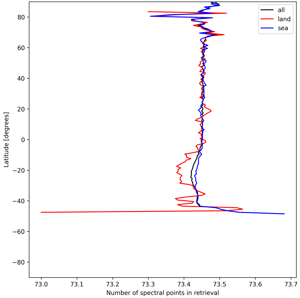
Figure 56: Zonal average of “Number of spectral points in retrieval” for 2025-07-19 to 2025-07-20.
