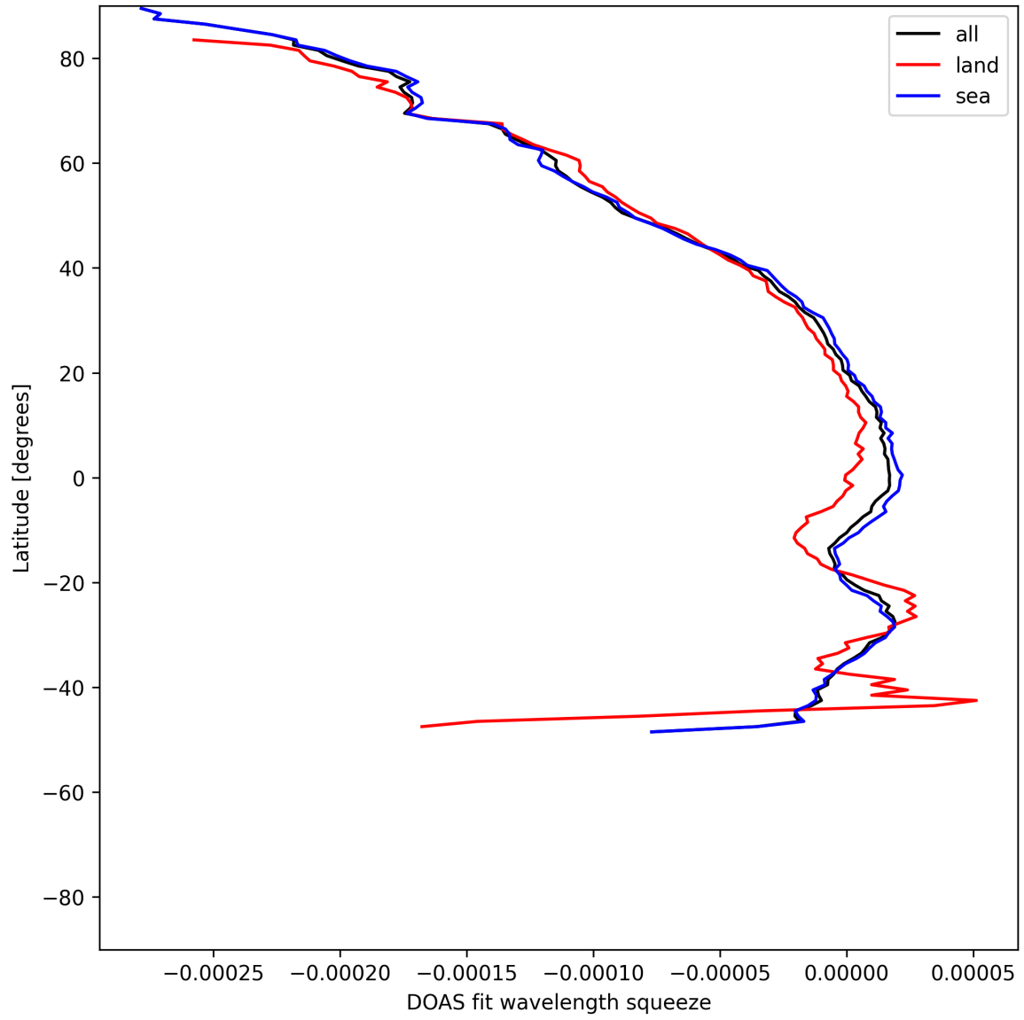
Figure 51: Zonal average of “DOAS fit wavelength squeeze” for 2025-07-19 to 2025-07-20.
