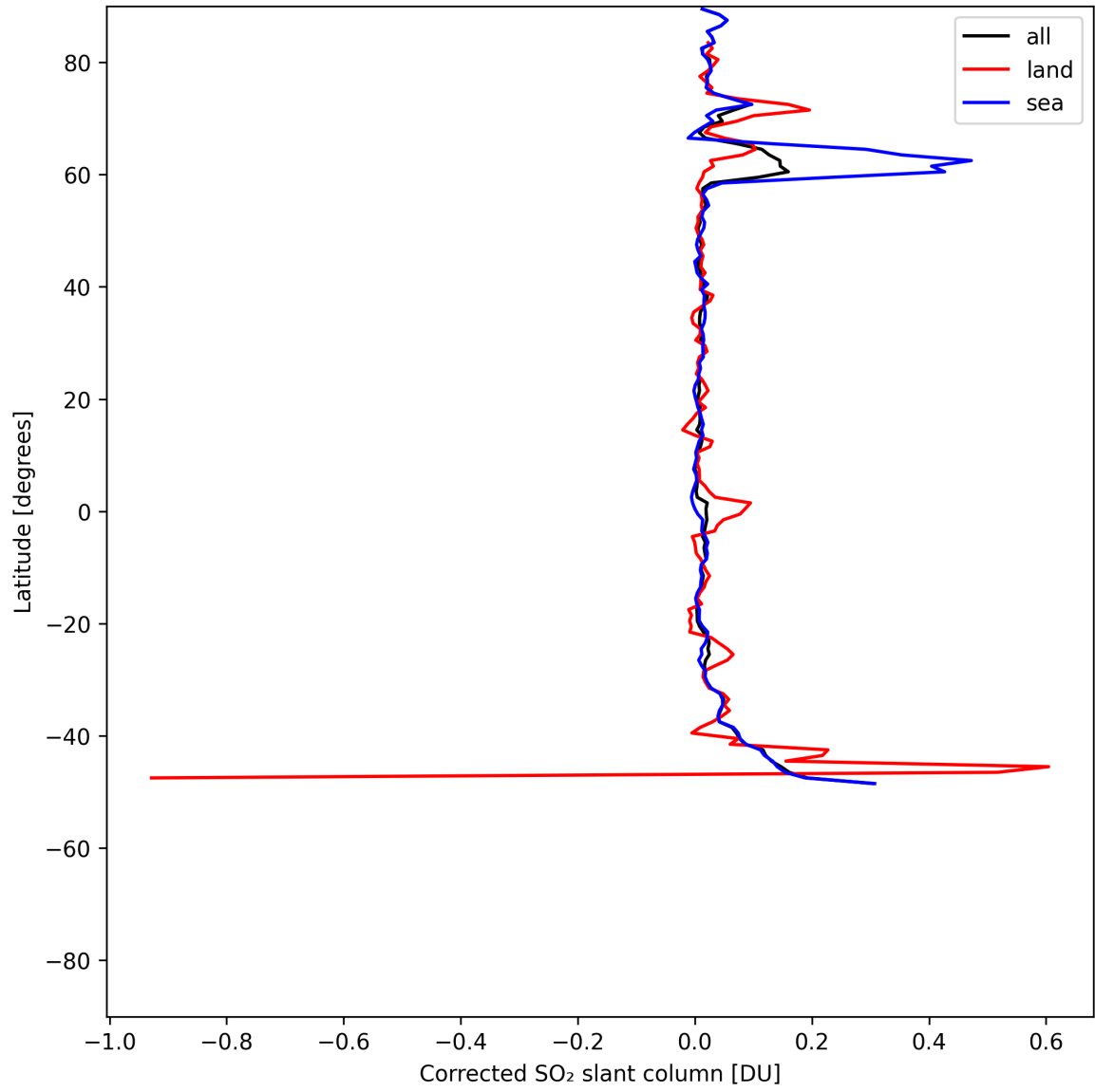
Figure 33: Zonal average of “Corrected SO 2 slant column” for 2025-07-19 to 2025-07-20.
