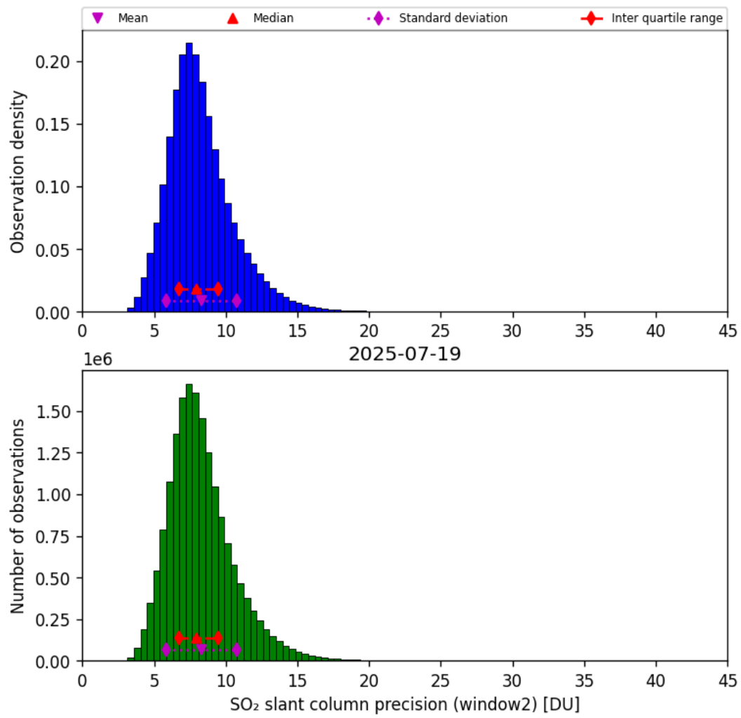
Figure 68: Histogram of “SO 2 slant column precision (window2)” for 2025-07-19 to 2025-07-20
