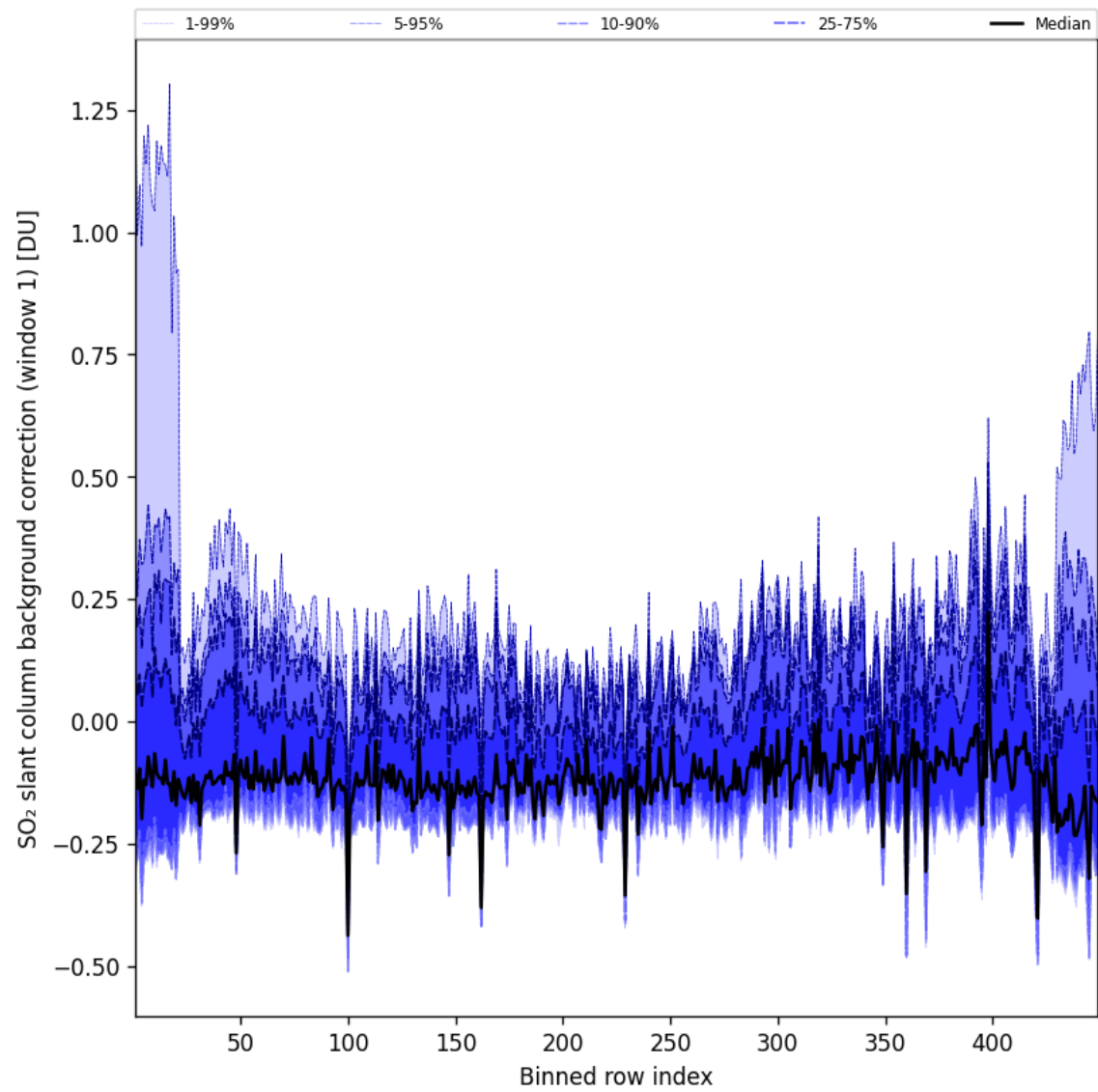
Figure 93: Along track statistics of “SO 2 slant column background correction (window 1)” for 2025-07-19 to 2025-07-20
