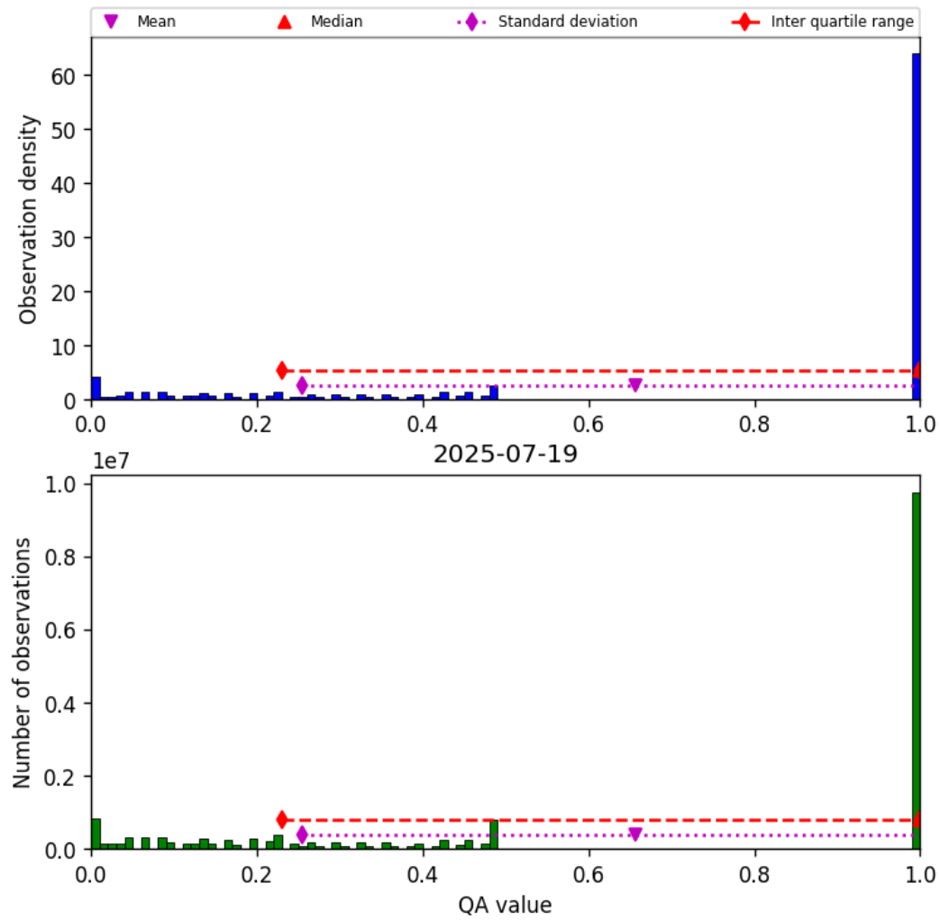
Figure 57: Histogram of “QA value” for 2025-07-19 to 2025-07-20
