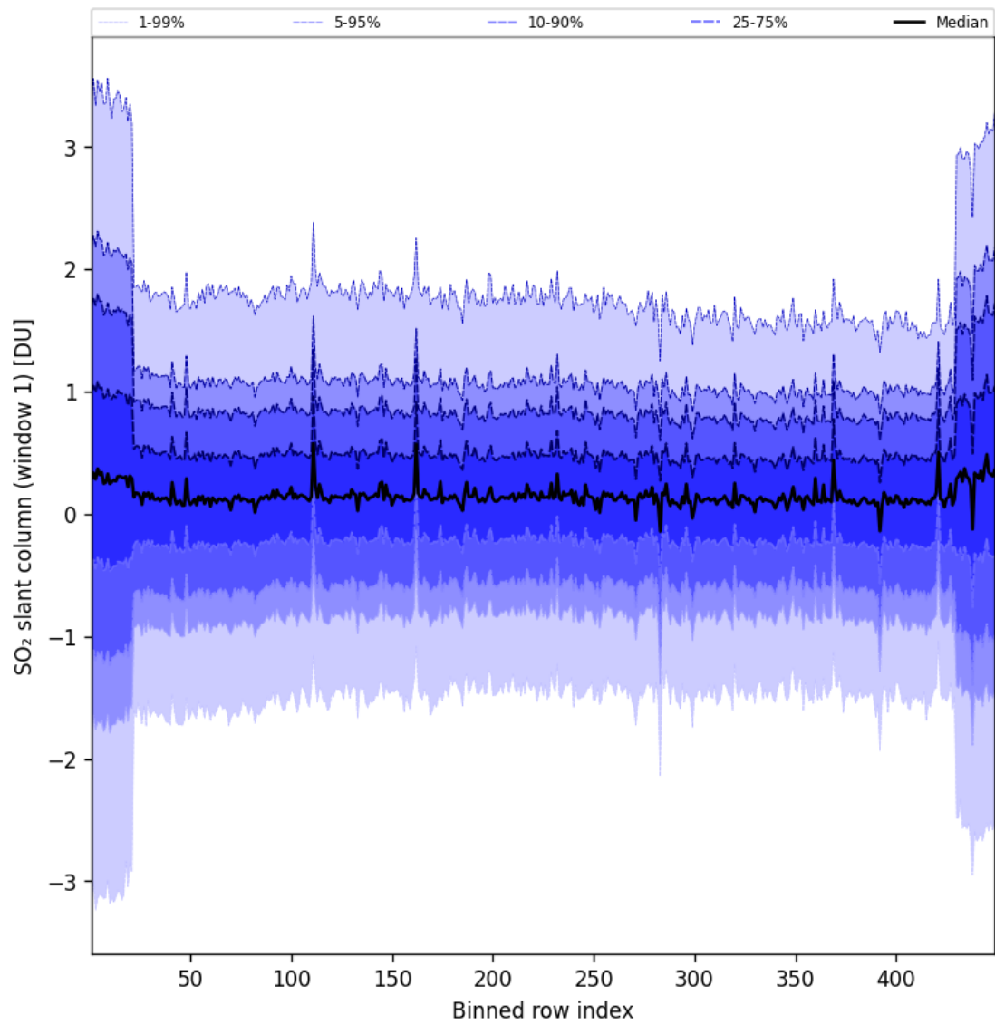
Figure 90: Along track statistics of “SO 2 slant column (window 1)” for 2025-07-19 to 2025-07-20
