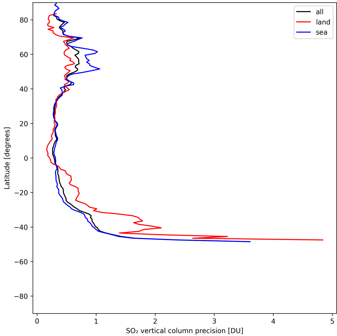
Figure 32: Zonal average of “SO 2 vertical column precision” for 2025-07-19 to 2025-07-20.
