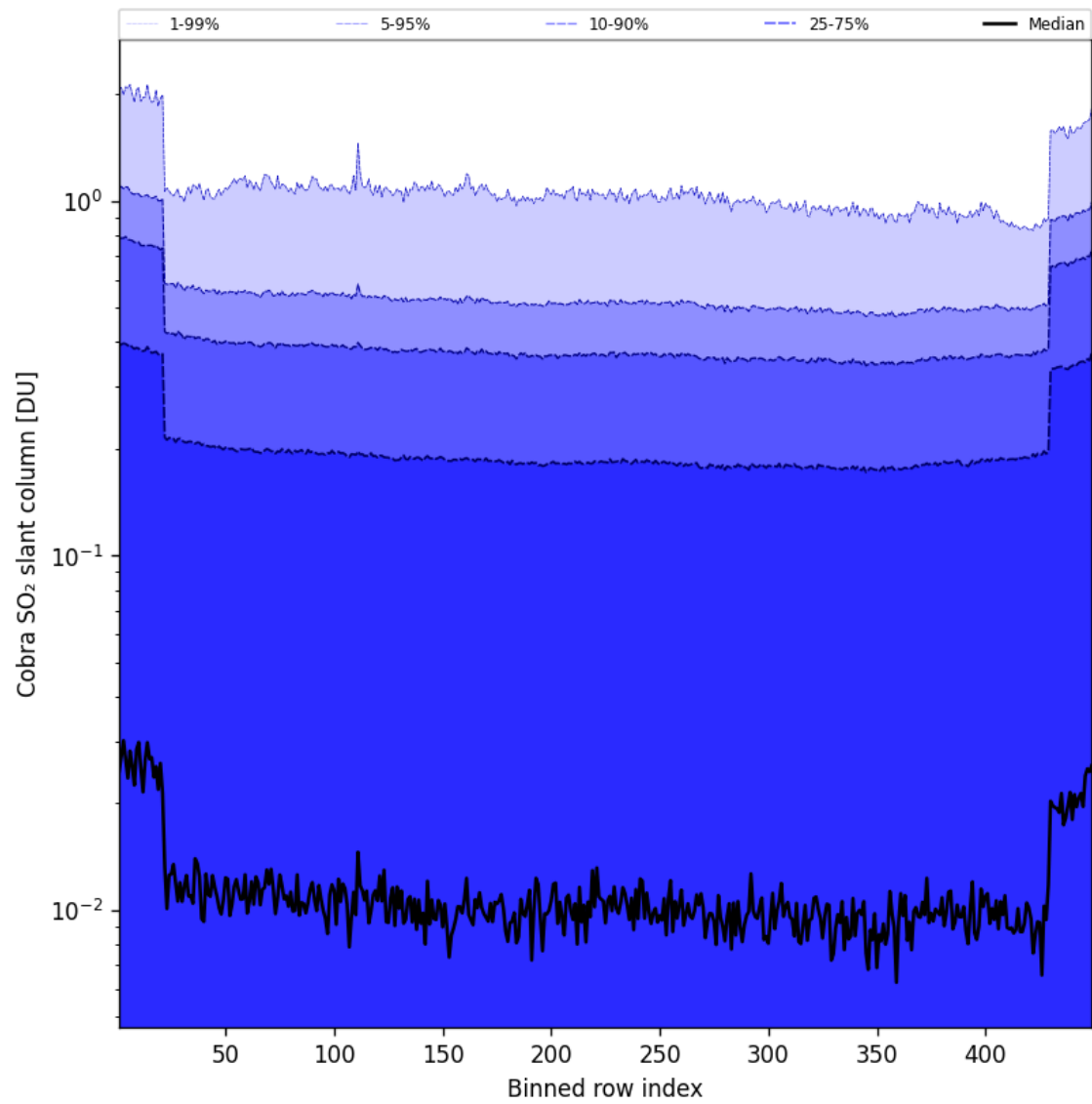
Figure 88: Along track statistics of “Cobra SO 2 slant column” for 2025-07-19 to 2025-07-20
