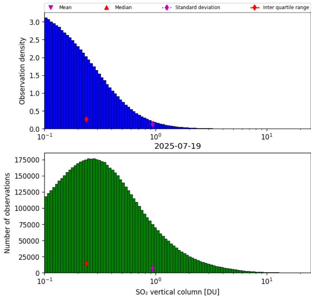
Figure 58: Histogram of “SO 2 vertical column” for 2025-07-19 to 2025-07-20
