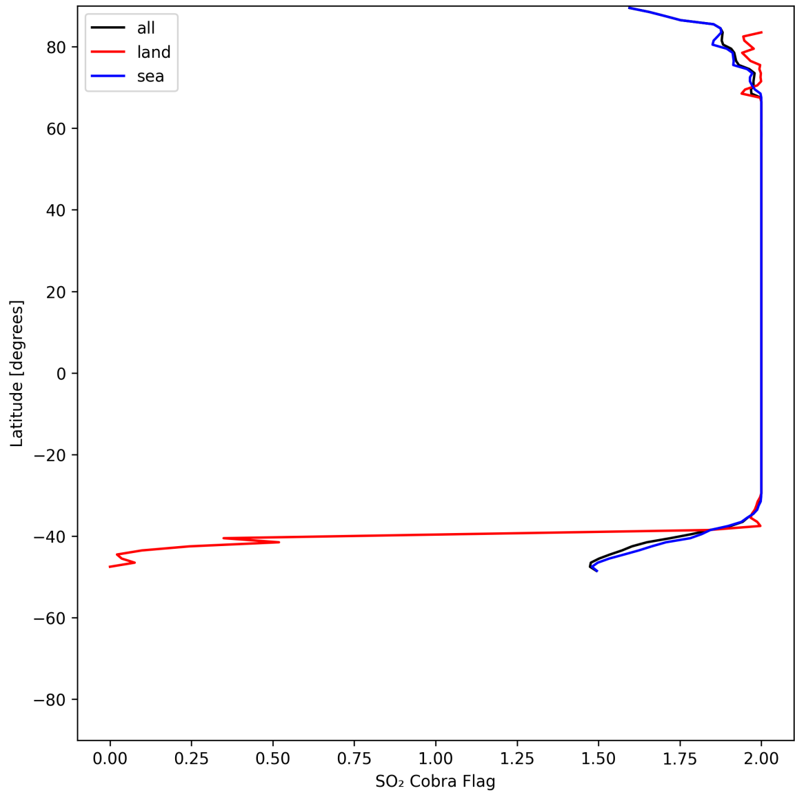
Figure 48: Zonal average of "SO 2 Cobra Flag" for 2025-07-19 to 2025-07-20.
