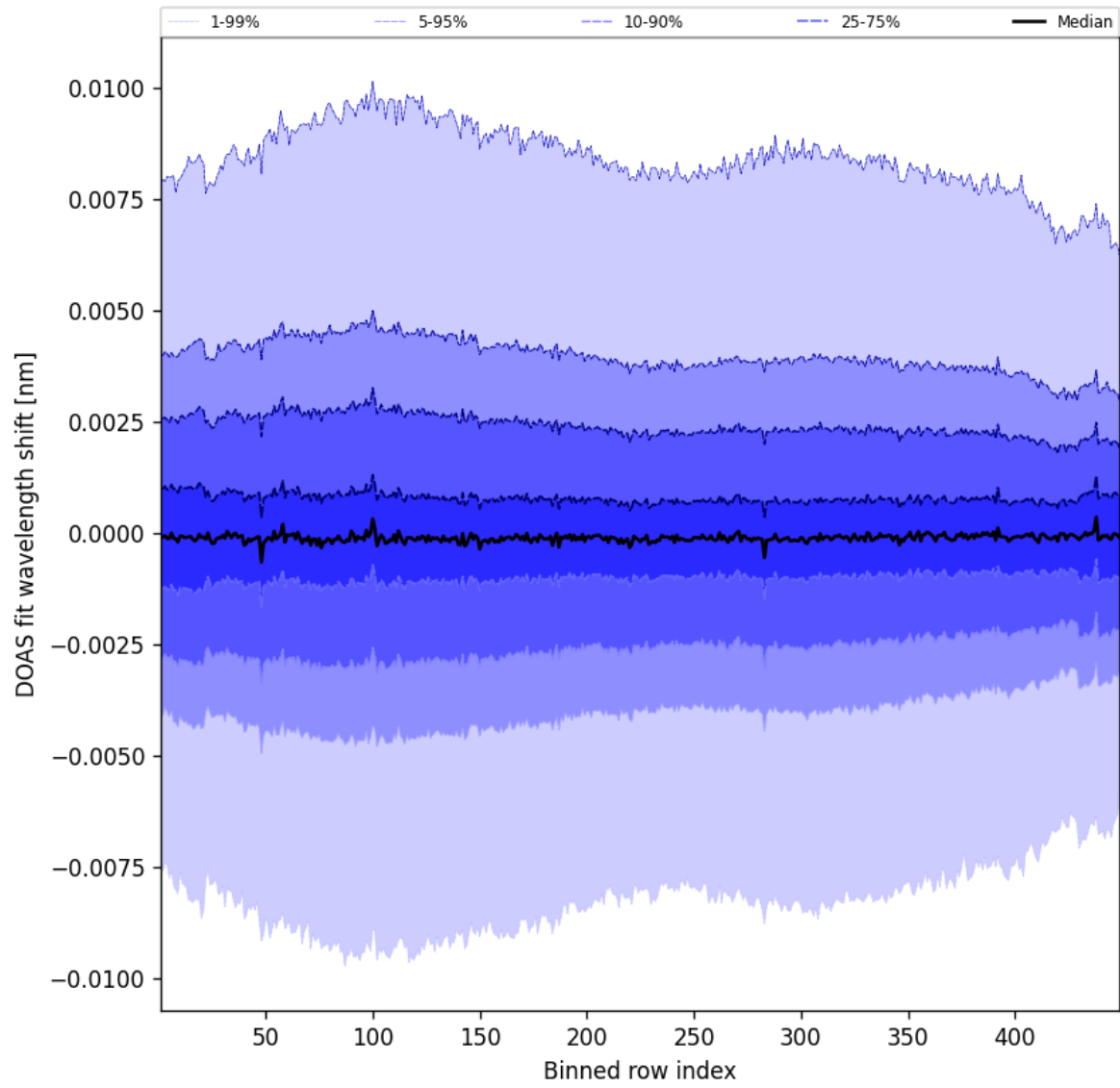
Figure 104: Along track statistics of “DOAS fit wavelength shift” for 2025-07-19 to 2025-07-20
