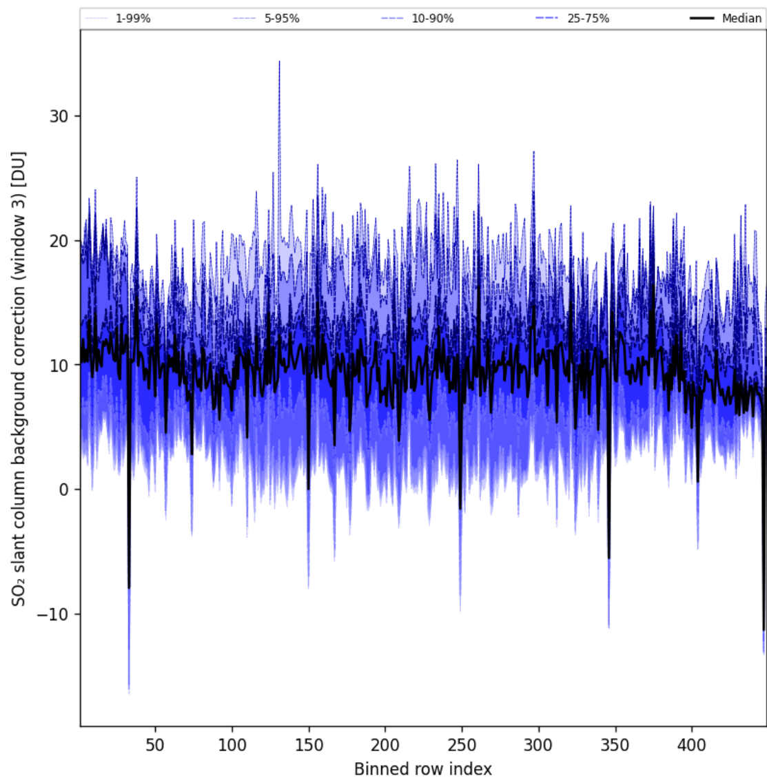
Figure 101: Along track statistics of “SO 2 slant column background correction (window 3)” for 2025-07-19 to 2025-07-20
