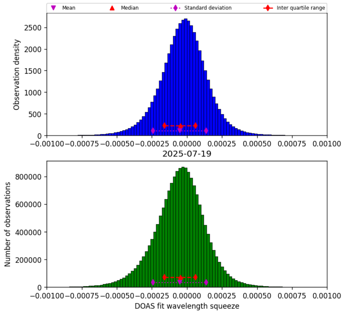
Figure 78: Histogram of “DOAS fit wavelength squeeze” for 2025-07-19 to 2025-07-20
