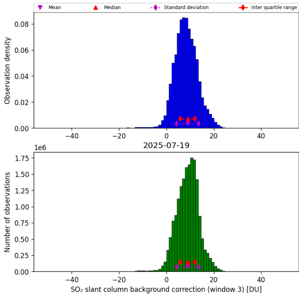
Figure 74: Histogram of “SO 2 slant column background correction (window 3)” for 2025-07-19 to 2025-07-20
