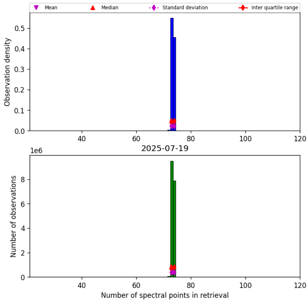
Figure 83: Histogram of “Number of spectral points in retrieval” for 2025-07-19 to 2025-07-20
