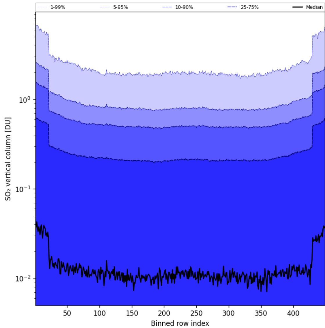
Figure 85: Along track statistics of “SO 2 vertical column” for 2025-07-19 to 2025-07-20
