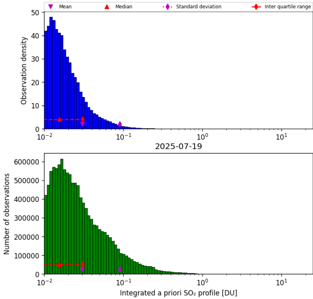
Figure 76: Histogram of “Integrated a priori SO 2 profile” for 2025-07-19 to 2025-07-20
