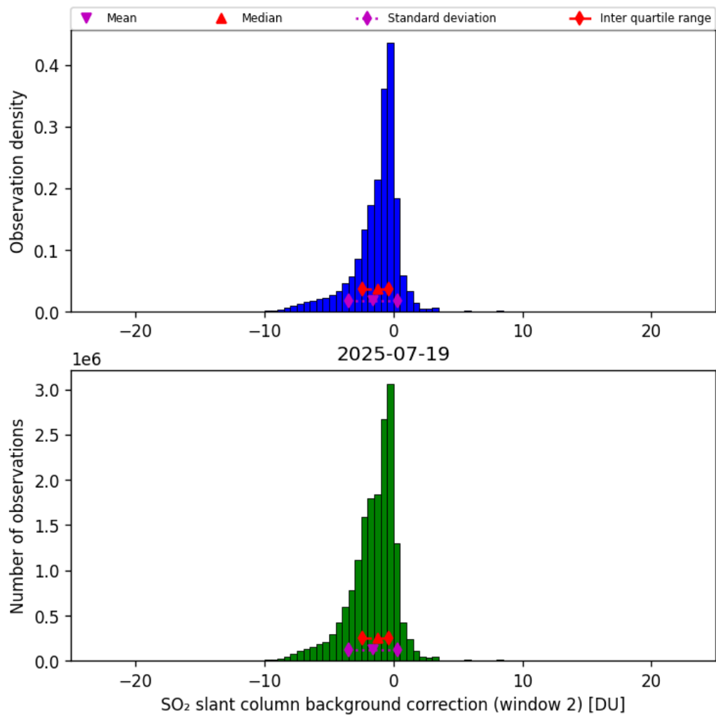
Figure 70: Histogram of “SO 2 slant column background correction (window 2)” for 2025-07-19 to 2025-07-20
