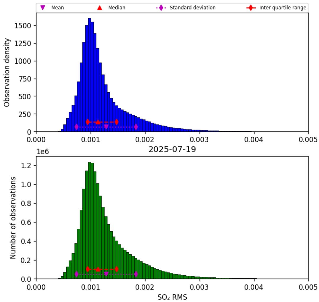
Figure 79: Histogram of “SO 2 RMS” for 2025-07-19 to 2025-07-20
