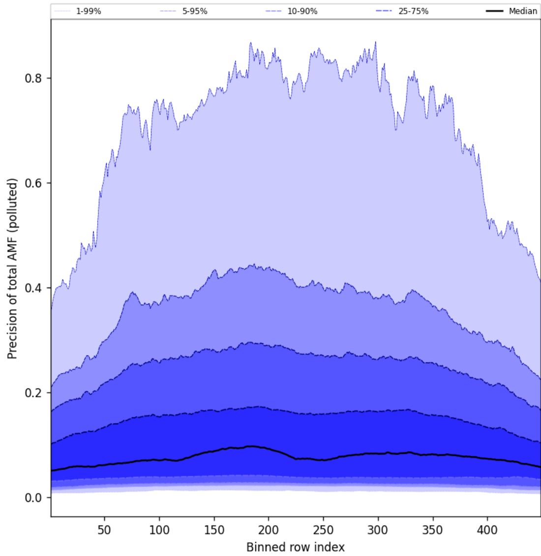
Figure 108: Along track statistics of “Precision of total AMF (polluted)” for 2025-07-19 to 2025-07-20
