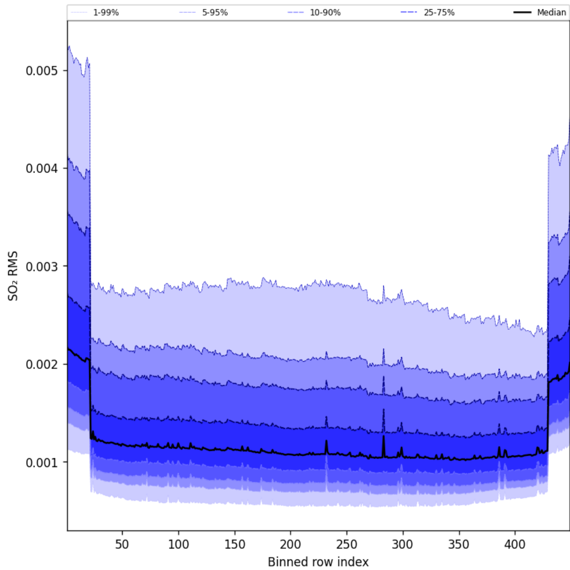
Figure 106: Along track statistics of “SO 2 RMS” for 2025-07-19 to 2025-07-20
