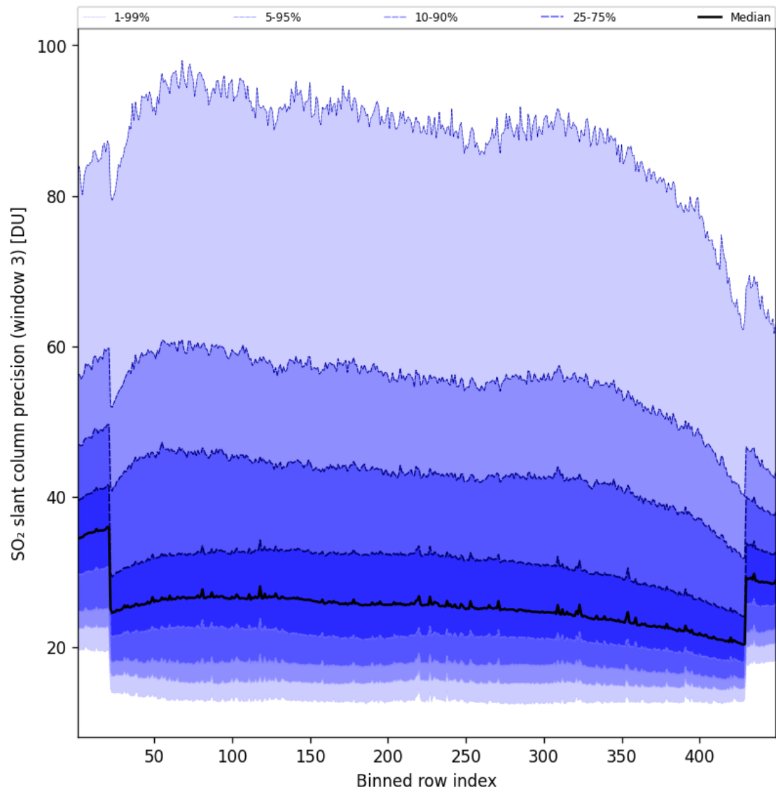
Figure 99: Along track statistics of “SO 2 slant column precision (window 3)” for 2025-07-20 to 2025-07-21
