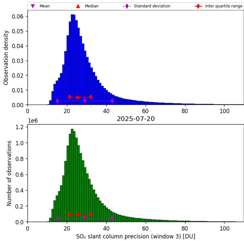
Figure 72: Histogram of “SO 2 slant column precision (window 3)” for 2025-07-20 to 2025-07-21
