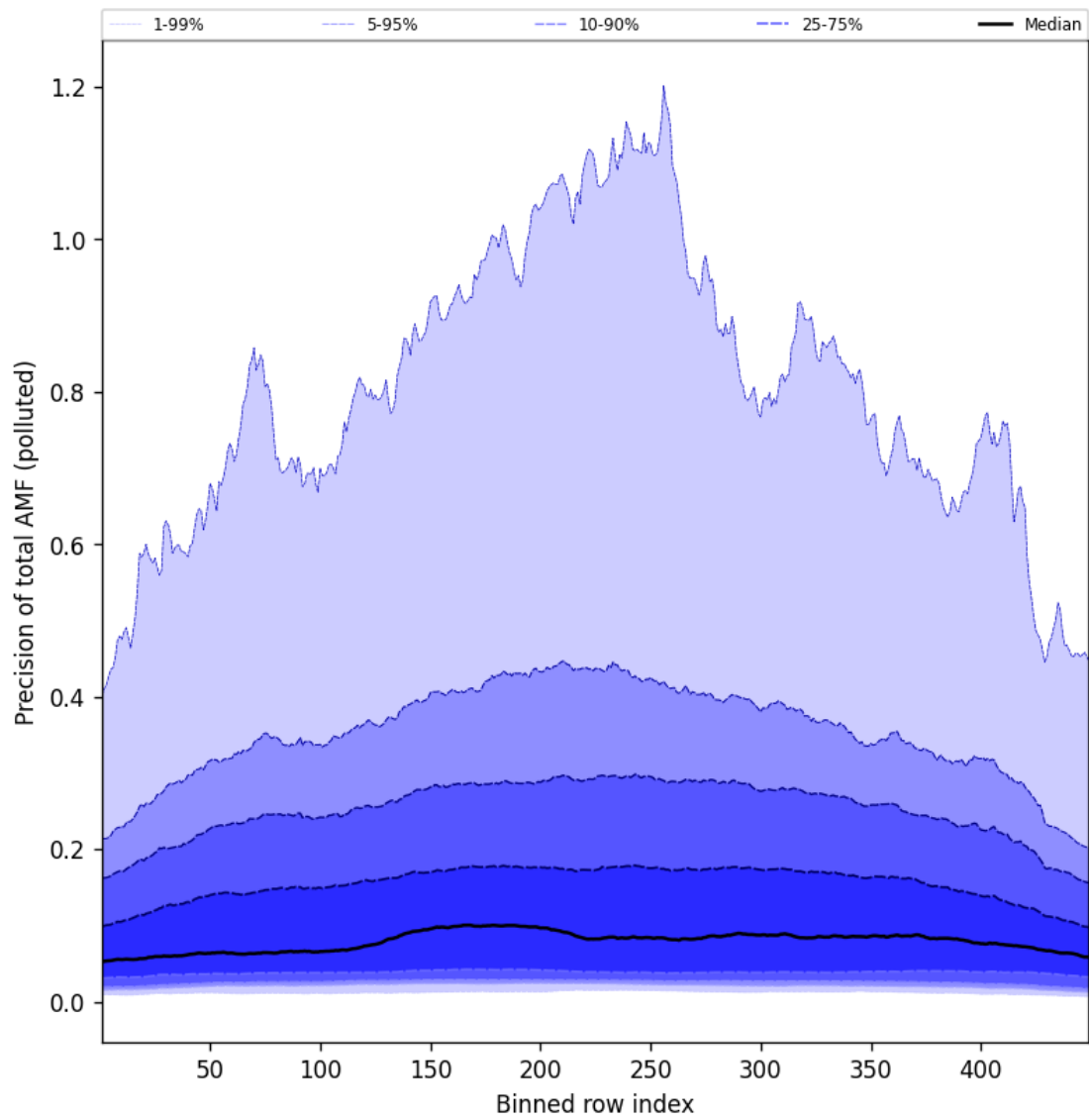
Figure 108: Along track statistics of “Precision of total AMF (polluted)” for 2025-07-20 to 2025-07-21
