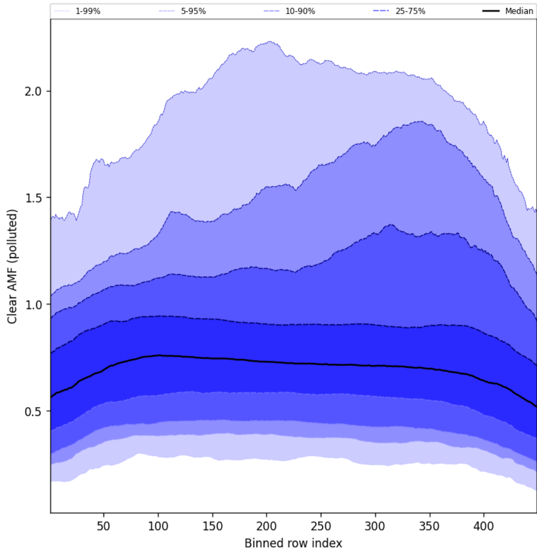
Figure 109: Along track statistics of “Clear AMF (polluted)” for 2025-07-20 to 2025-07-21
