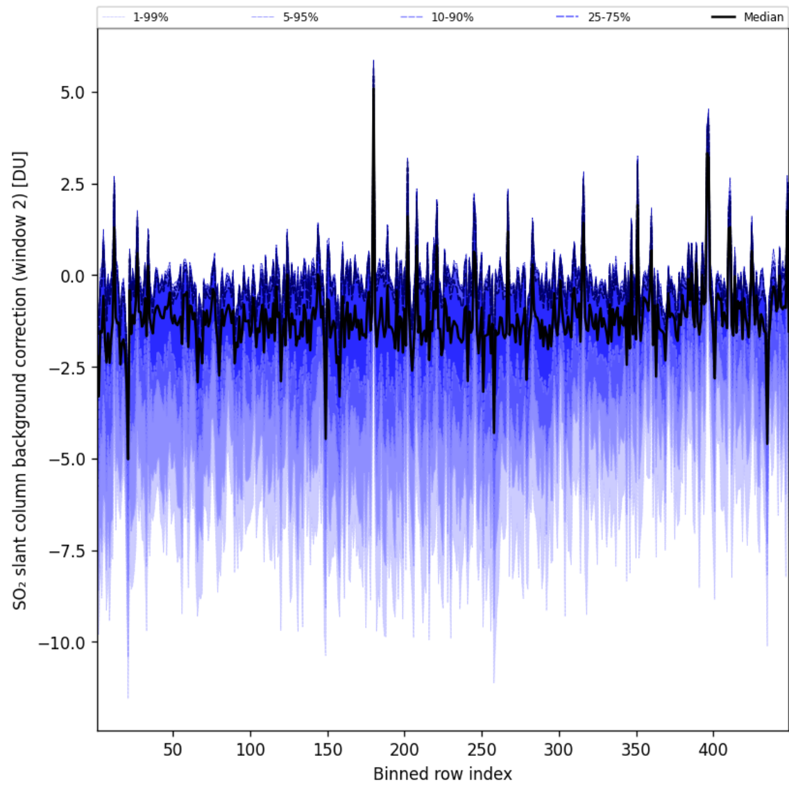
Figure 97: Along track statistics of “SO 2 slant column background correction (window 2)” for 2025-07-20 to 2025-07-21
