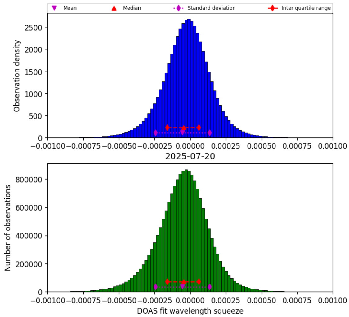
Figure 78: Histogram of “DOAS fit wavelength squeeze” for 2025-07-20 to 2025-07-21
