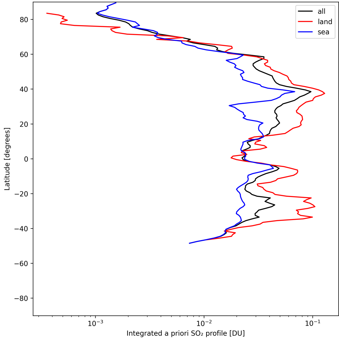
Figure 49: Zonal average of “Integrated a priori SO 2 profile” for 2025-07-20 to 2025-07-21.
