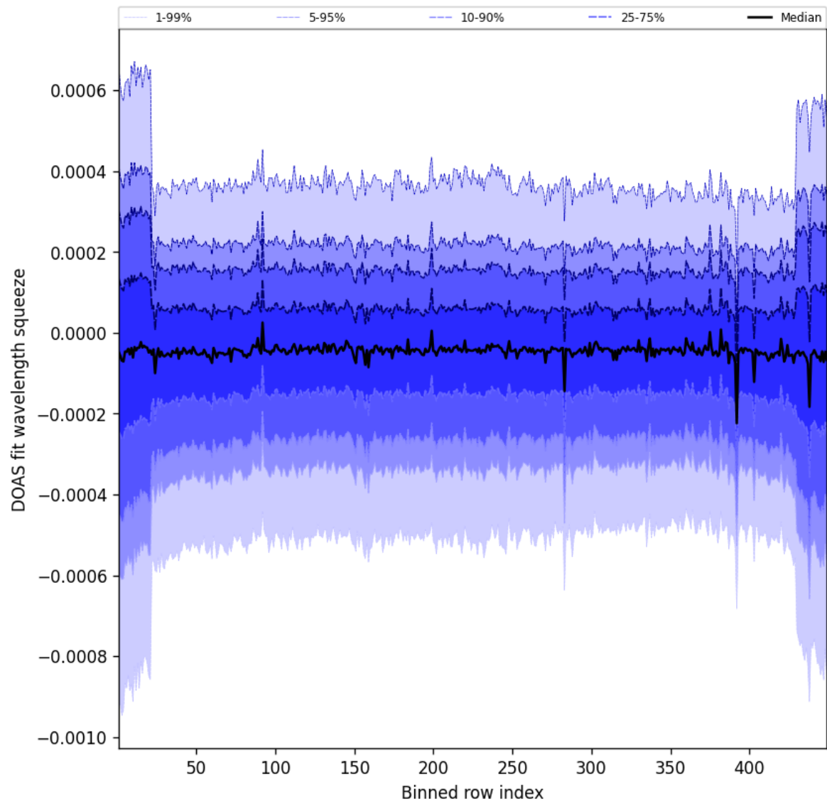
Figure 105: Along track statistics of “DOAS fit wavelength squeeze” for 2025-07-20 to 2025-07-21
