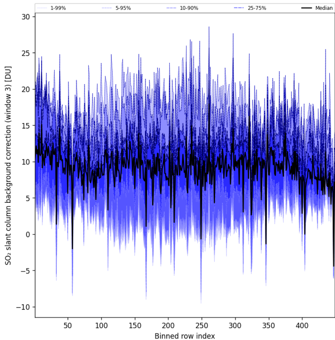
Figure 101: Along track statistics of “SO 2 slant column background correction (window 3)” for 2025-07-20 to 2025-07-21
