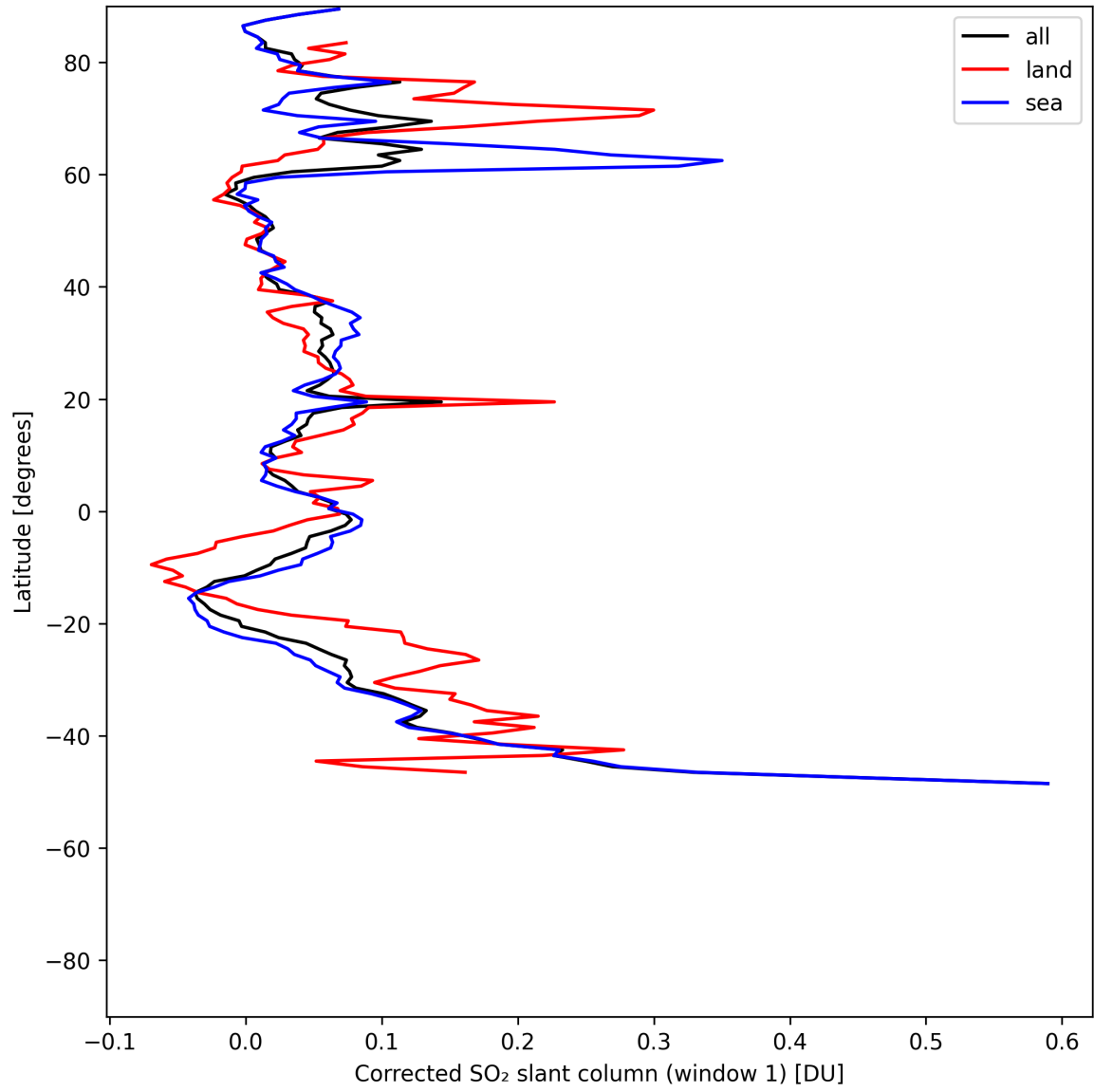
Figure 38: Zonal average of “Corrected SO 2 slant column (window 1)” for 2025-07-20 to 2025-07-21.
