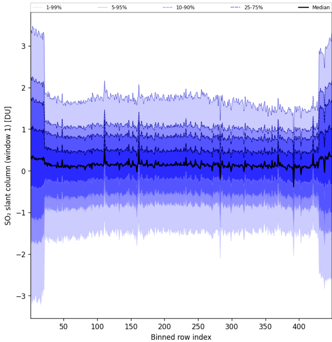
Figure 90: Along track statistics of “SO 2 slant column (window 1)” for 2025-07-20 to 2025-07-21
