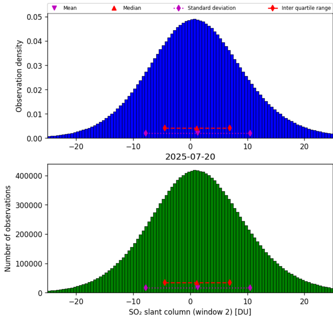
Figure 67: Histogram of “SO 2 slant column (window 2)” for 2025-07-20 to 2025-07-21
