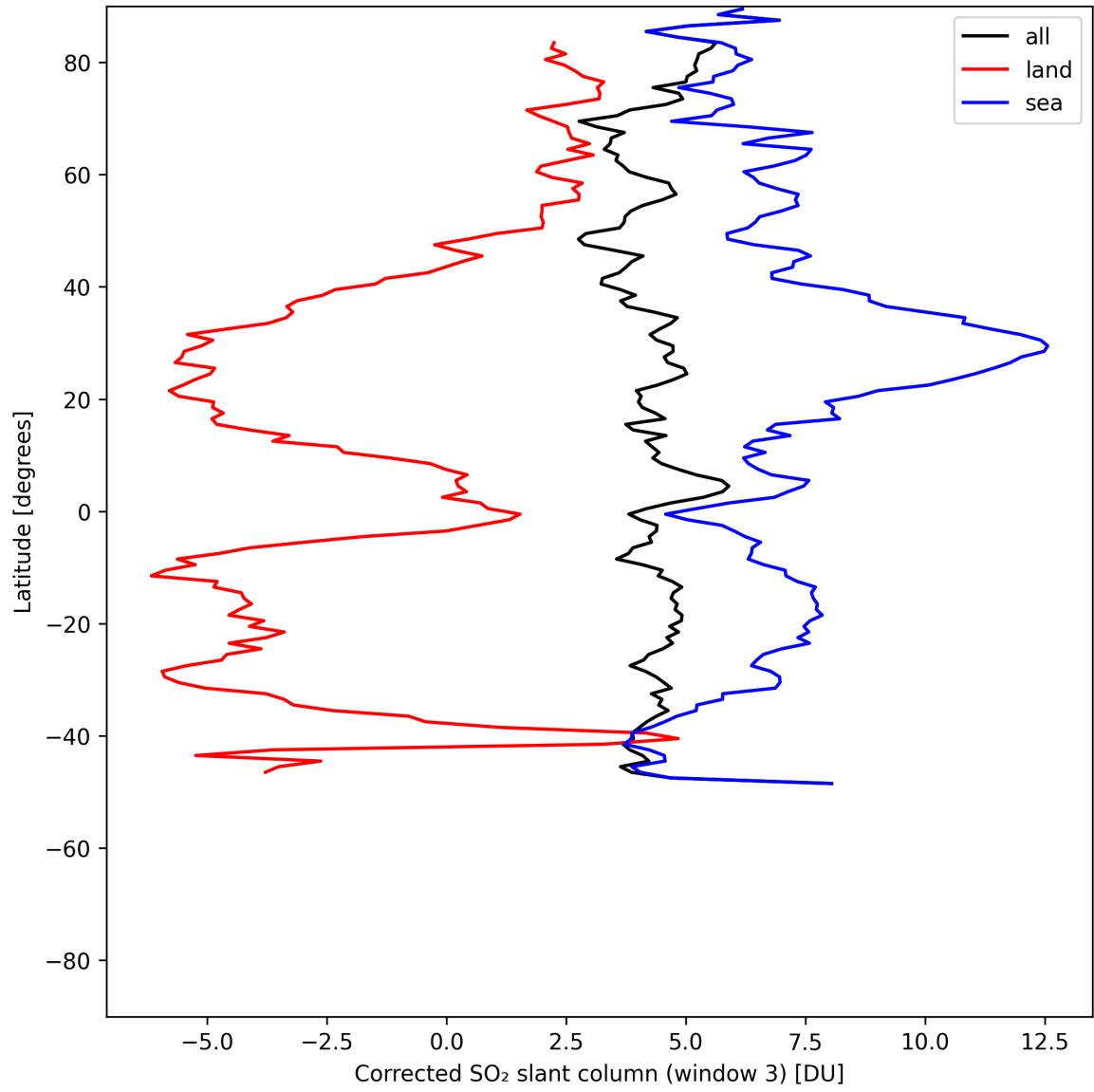
Figure 46: Zonal average of “Corrected SO 2 slant column (window 3)” for 2025-07-20 to 2025-07-21.
