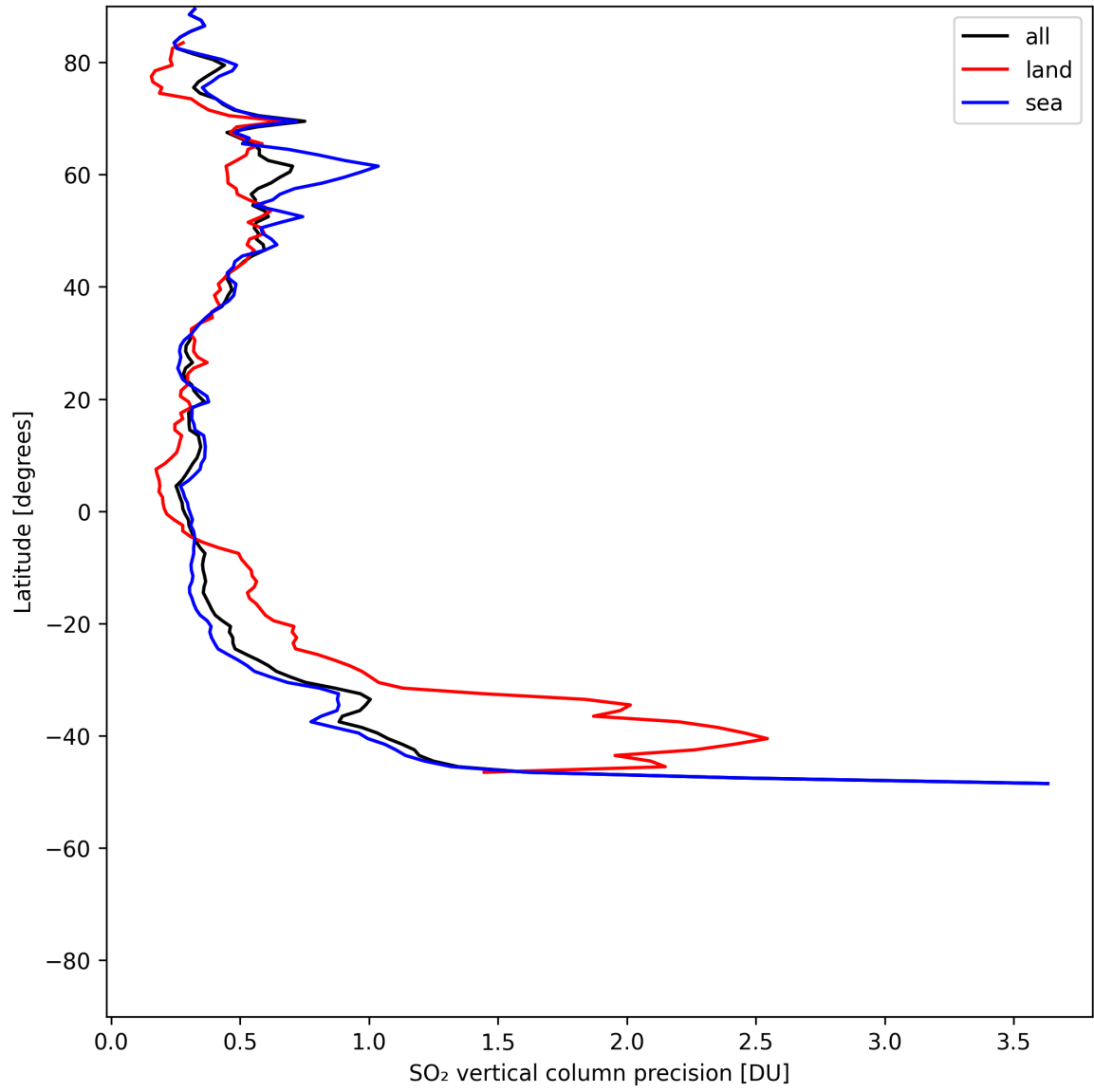
Figure 32: Zonal average of “SO 2 vertical column precision” for 2025-07-20 to 2025-07-21.
