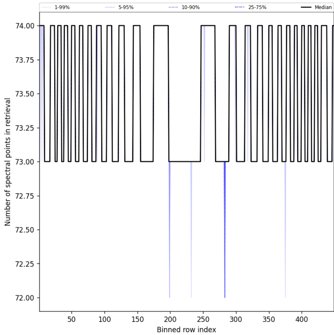
Figure 110: Along track statistics of “Number of spectral points in retrieval” for 2025-07-20 to 2025-07-21
