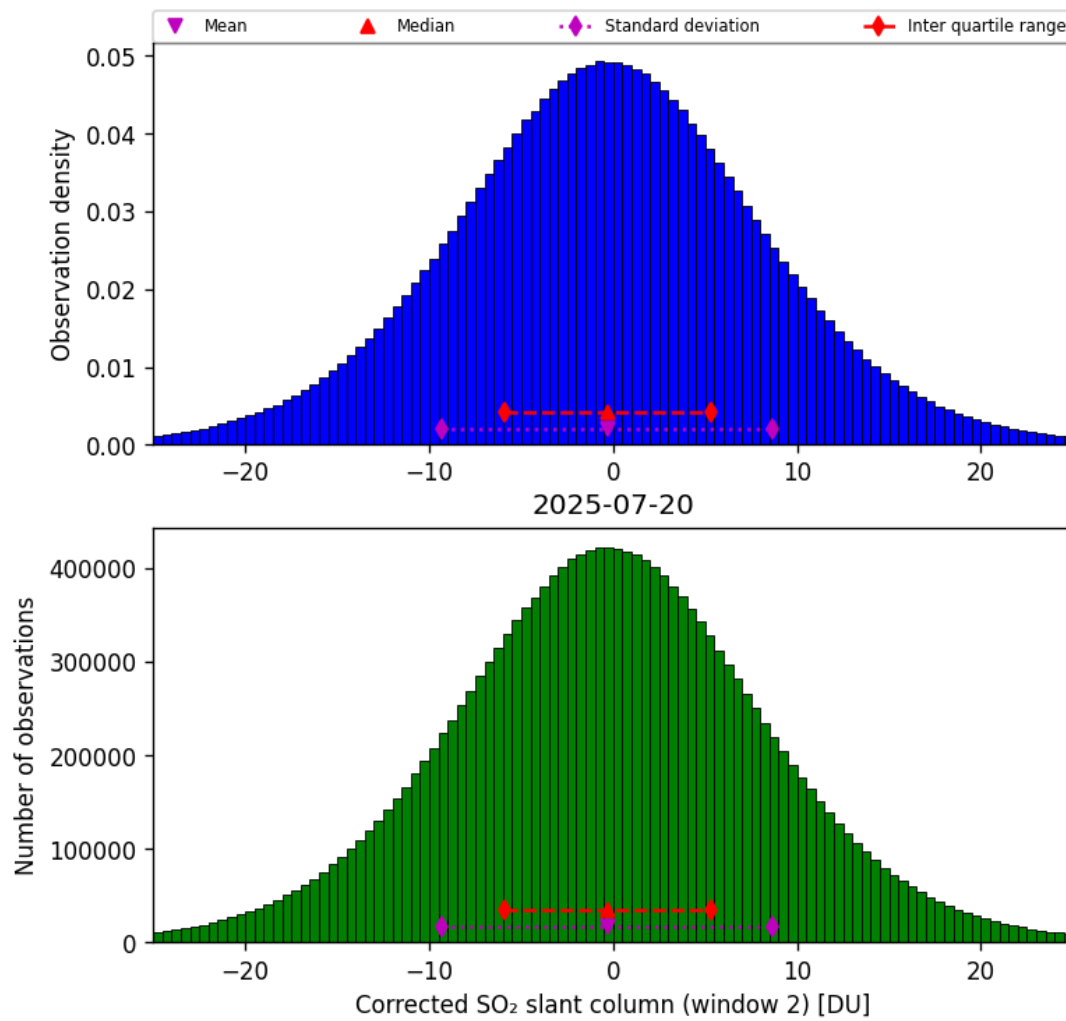
Figure 69: Histogram of “Corrected SO 2 slant column (window 2)” for 2025-07-20 to 2025-07-21
