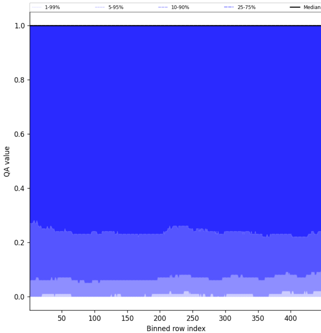
Figure 84: Along track statistics of “QA value” for 2025-07-20 to 2025-07-21
