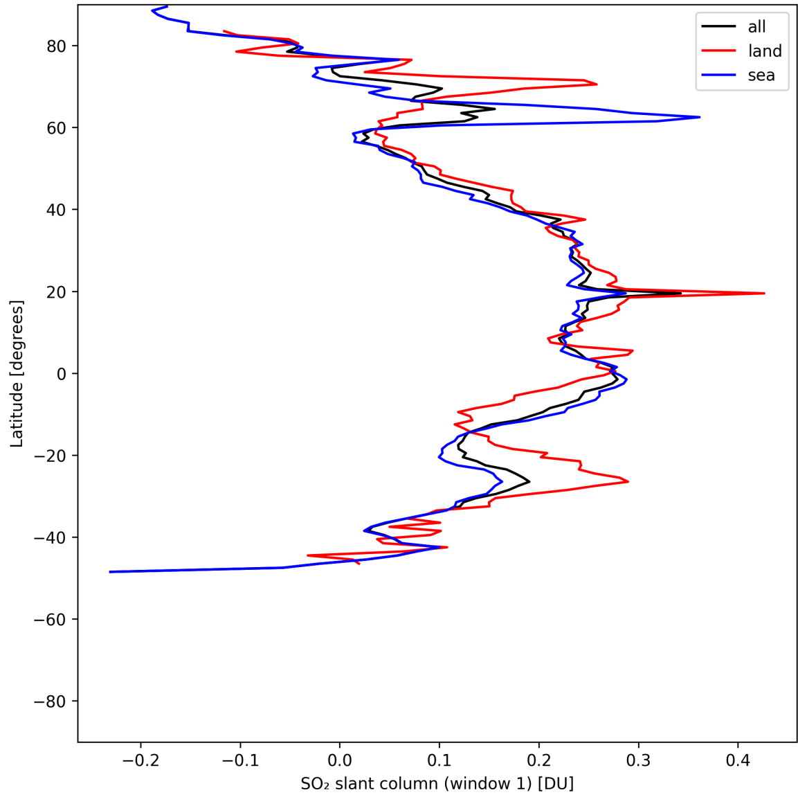
Figure 36: Zonal average of “SO 2 slant column (window 1)” for 2025-07-20 to 2025-07-21.
