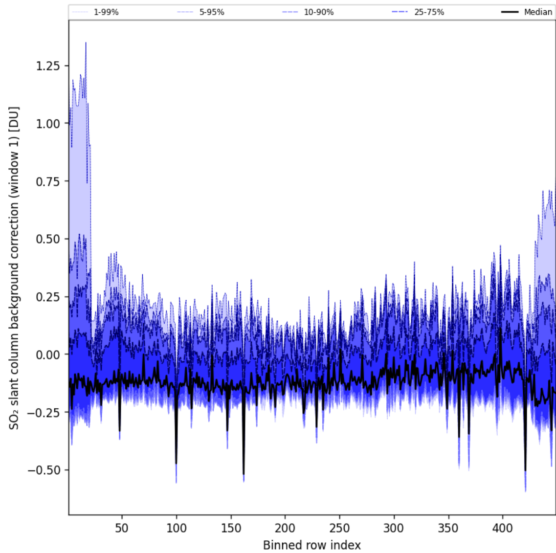
Figure 93: Along track statistics of “SO 2 slant column background correction (window 1)” for 2025-07-20 to 2025-07-21
