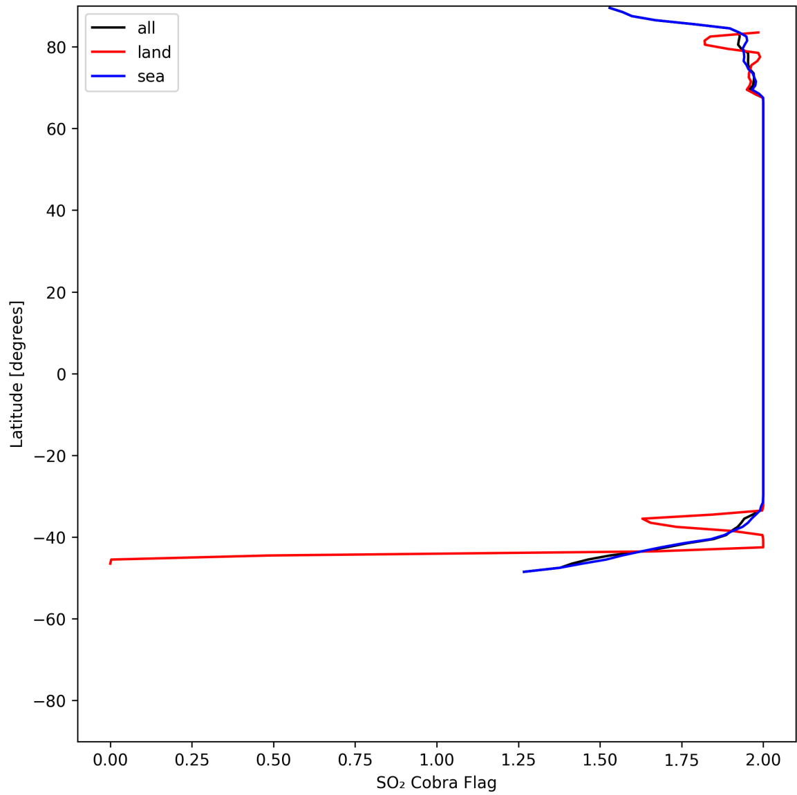
Figure 48: Zonal average of "SO 2 Cobra Flag" for 2025-07-20 to 2025-07-21.
