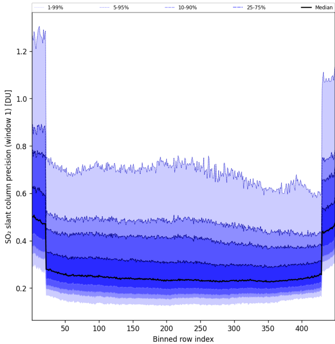
Figure 91: Along track statistics of “SO 2 slant column precision (window 1)” for 2025-07-20 to 2025-07-21
