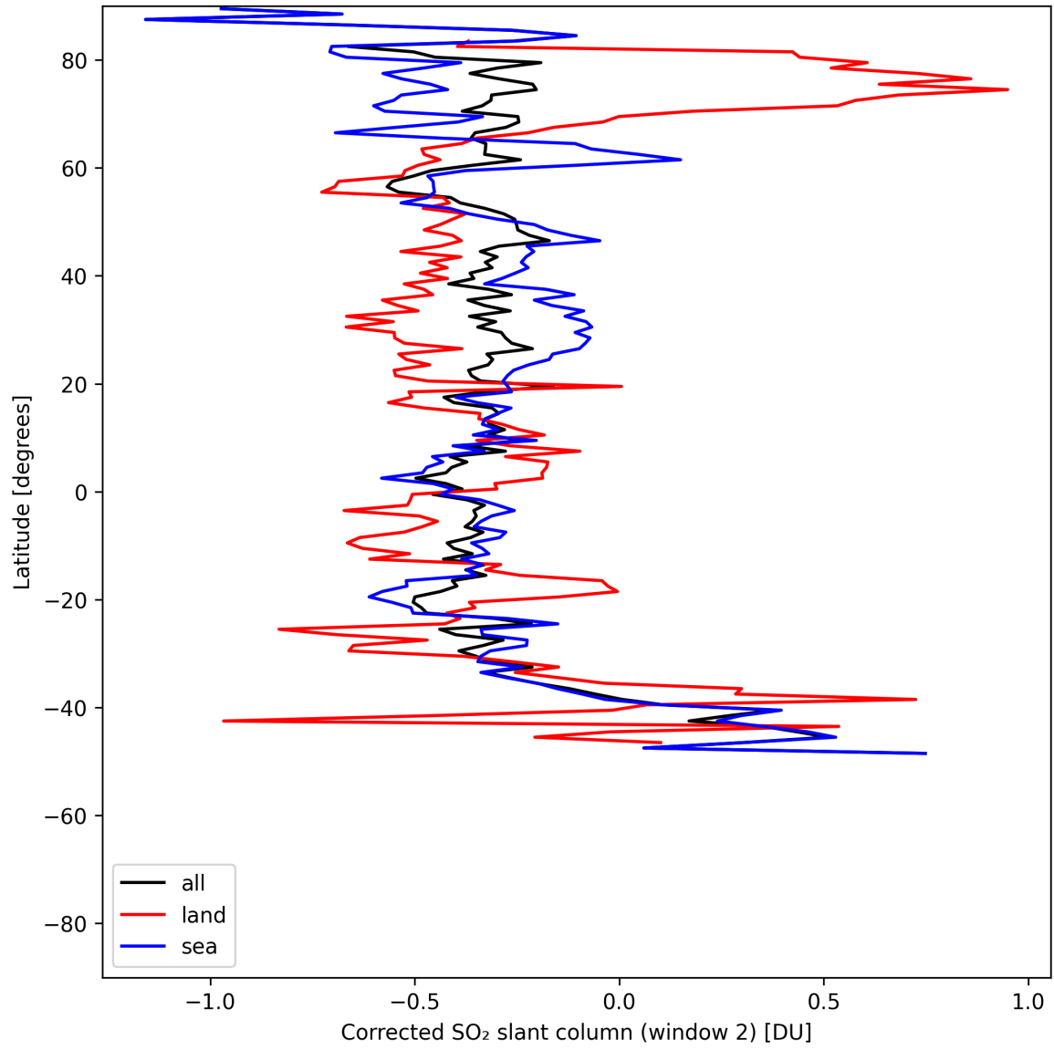
Figure 42: Zonal average of “Corrected SO 2 slant column (window 2)” for 2025-07-20 to 2025-07-21.
