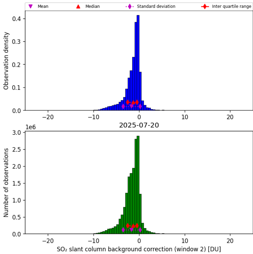
Figure 70: Histogram of “SO 2 slant column background correction (window 2)” for 2025-07-20 to 2025-07-21
