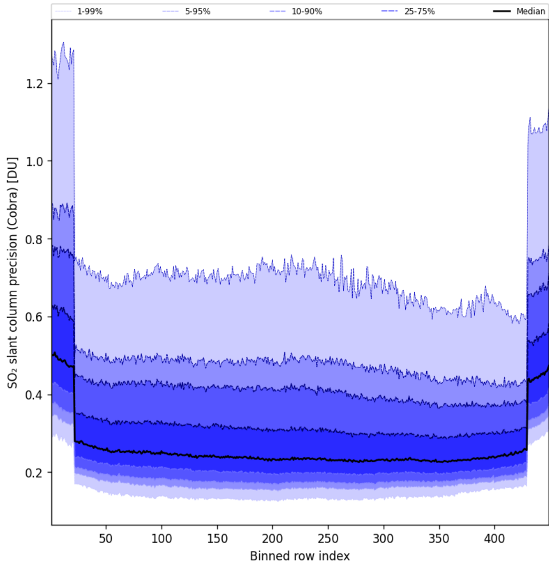
Figure 89: Along track statistics of “SO 2 slant column precision (Cobra)” for 2025-07-20 to 2025-07-21
