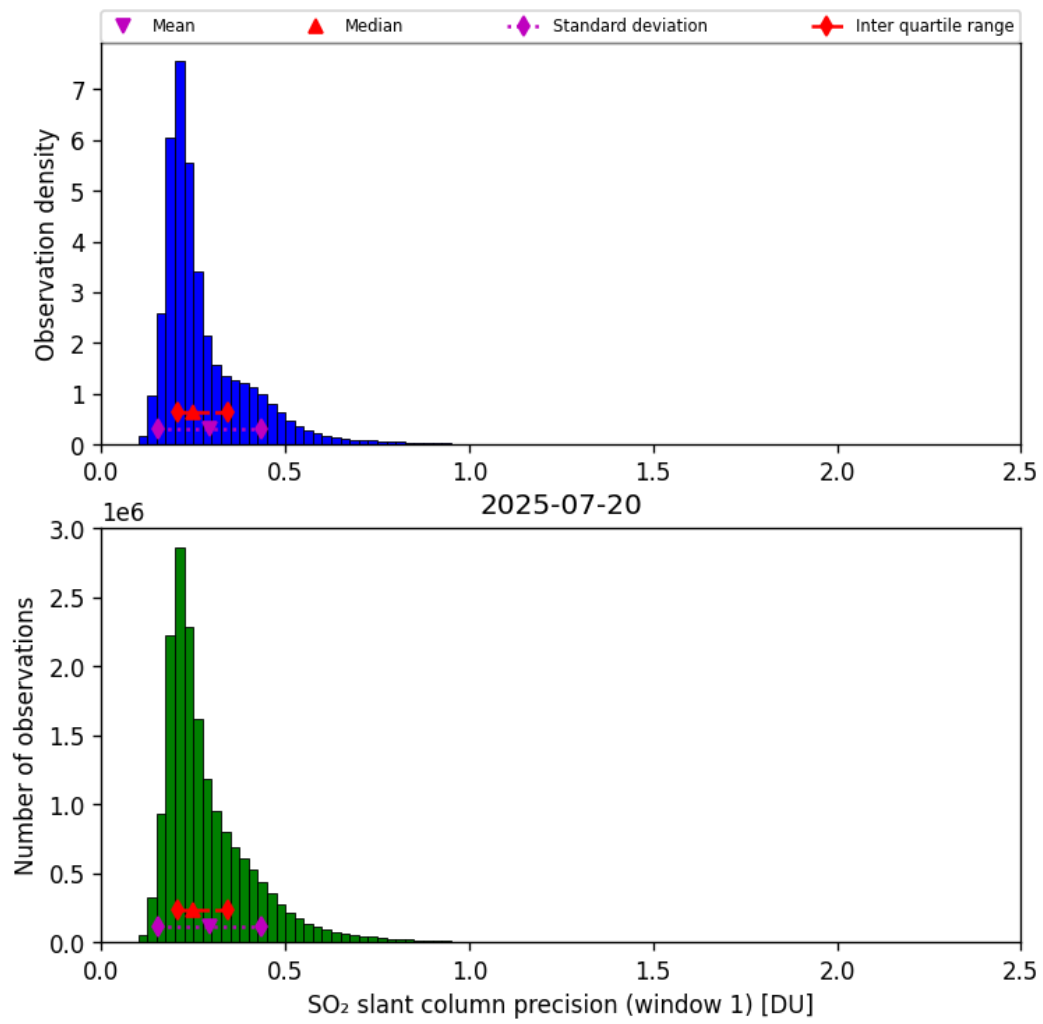
Figure 64: Histogram of “SO 2 slant column precision (window 1)” for 2025-07-20 to 2025-07-21
