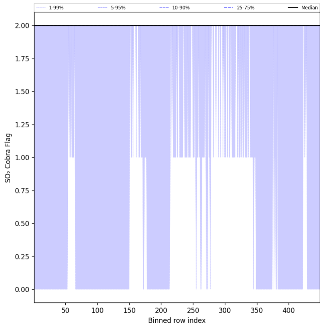
Figure 102: Along track statistics of “SO 2 Cobra Flag” for 2025-07-20 to 2025-07-21
