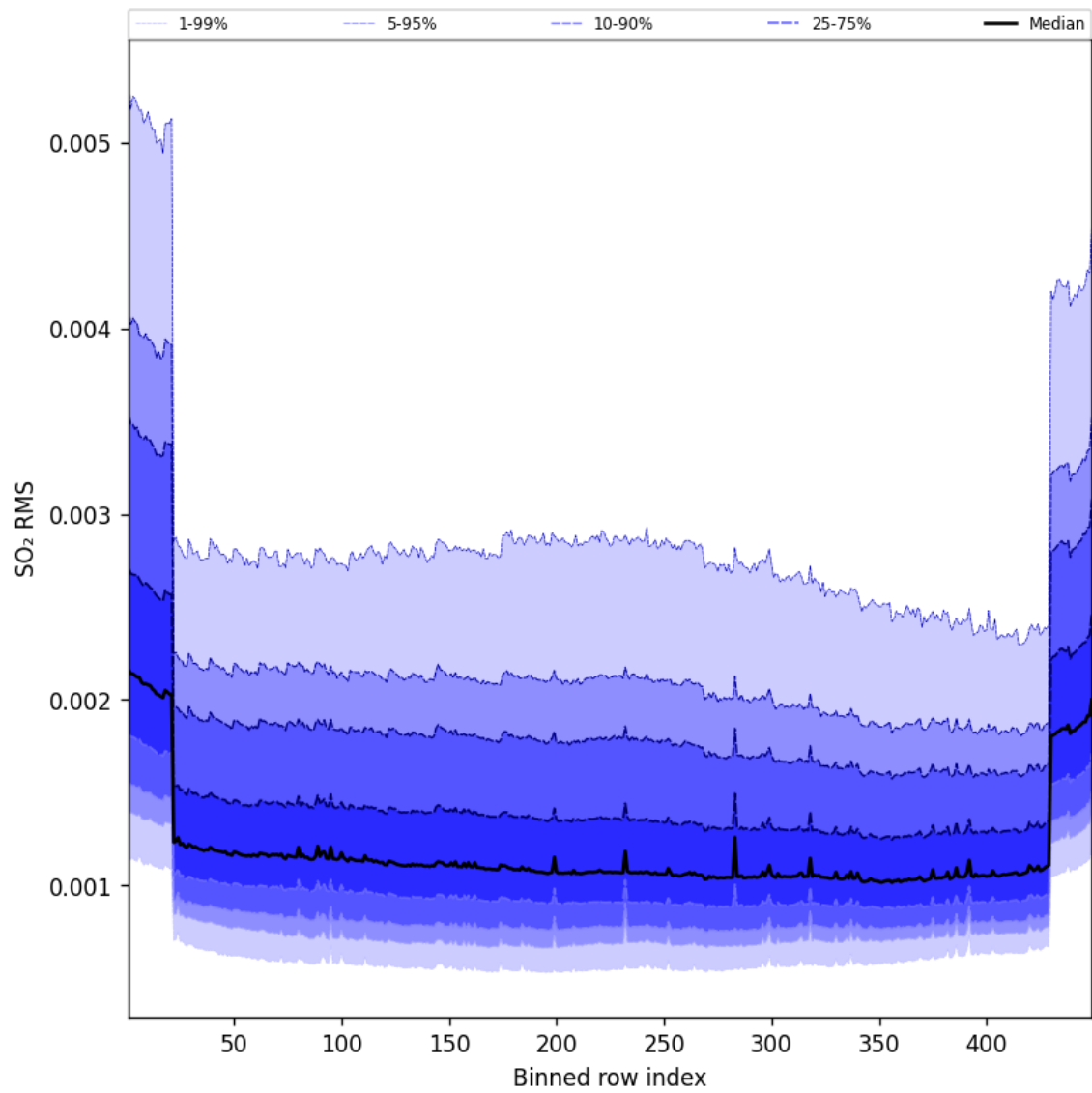
Figure 106: Along track statistics of “SO 2 RMS” for 2025-07-20 to 2025-07-21
