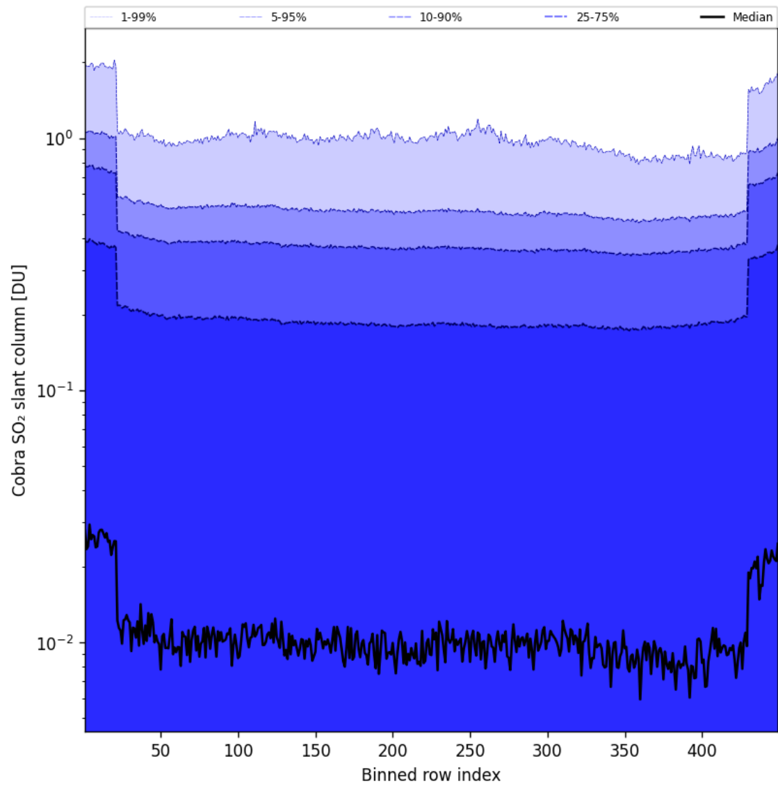
Figure 88: Along track statistics of “Cobra SO 2 slant column” for 2025-07-20 to 2025-07-21
