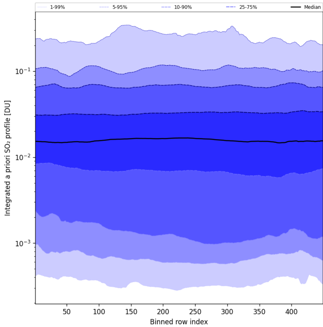
Figure 103: Along track statistics of “Integrated a priori SO 2 profile” for 2025-07-20 to 2025-07-21
