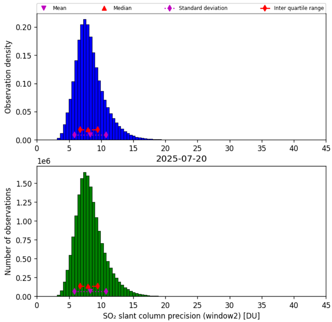
Figure 68: Histogram of “SO 2 slant column precision (window2)” for 2025-07-20 to 2025-07-21
