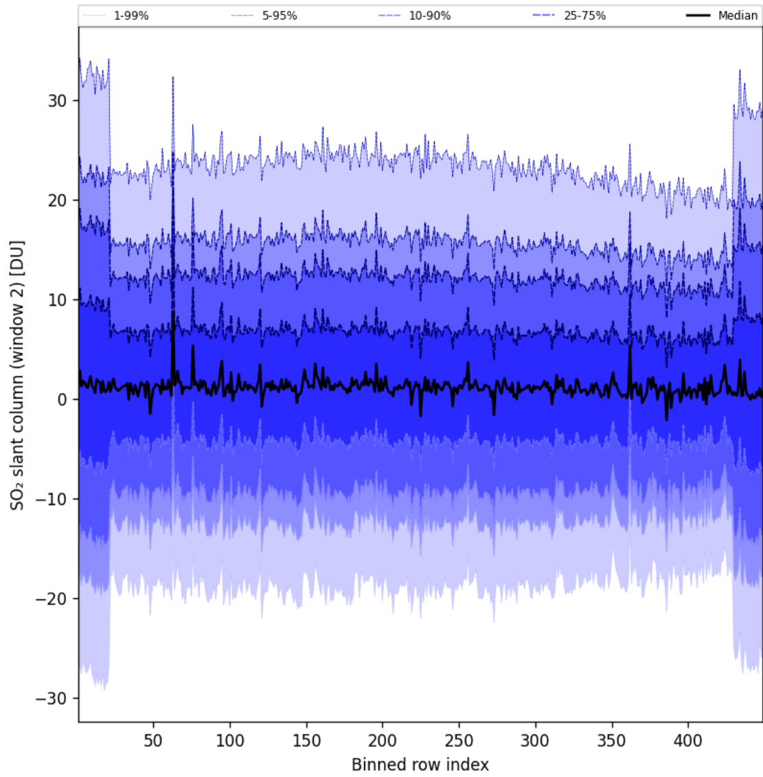
Figure 94: Along track statistics of “SO 2 slant column (window 2)” for 2025-07-20 to 2025-07-21
