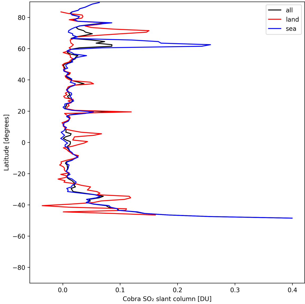
Figure 34: Zonal average of “Cobra SO 2 slant column” for 2025-07-20 to 2025-07-21.
