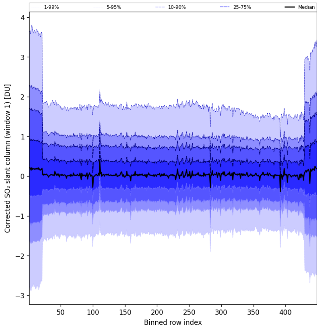
Figure 92: Along track statistics of “Corrected SO 2 slant column (window 1)” for 2025-07-20 to 2025-07-21
