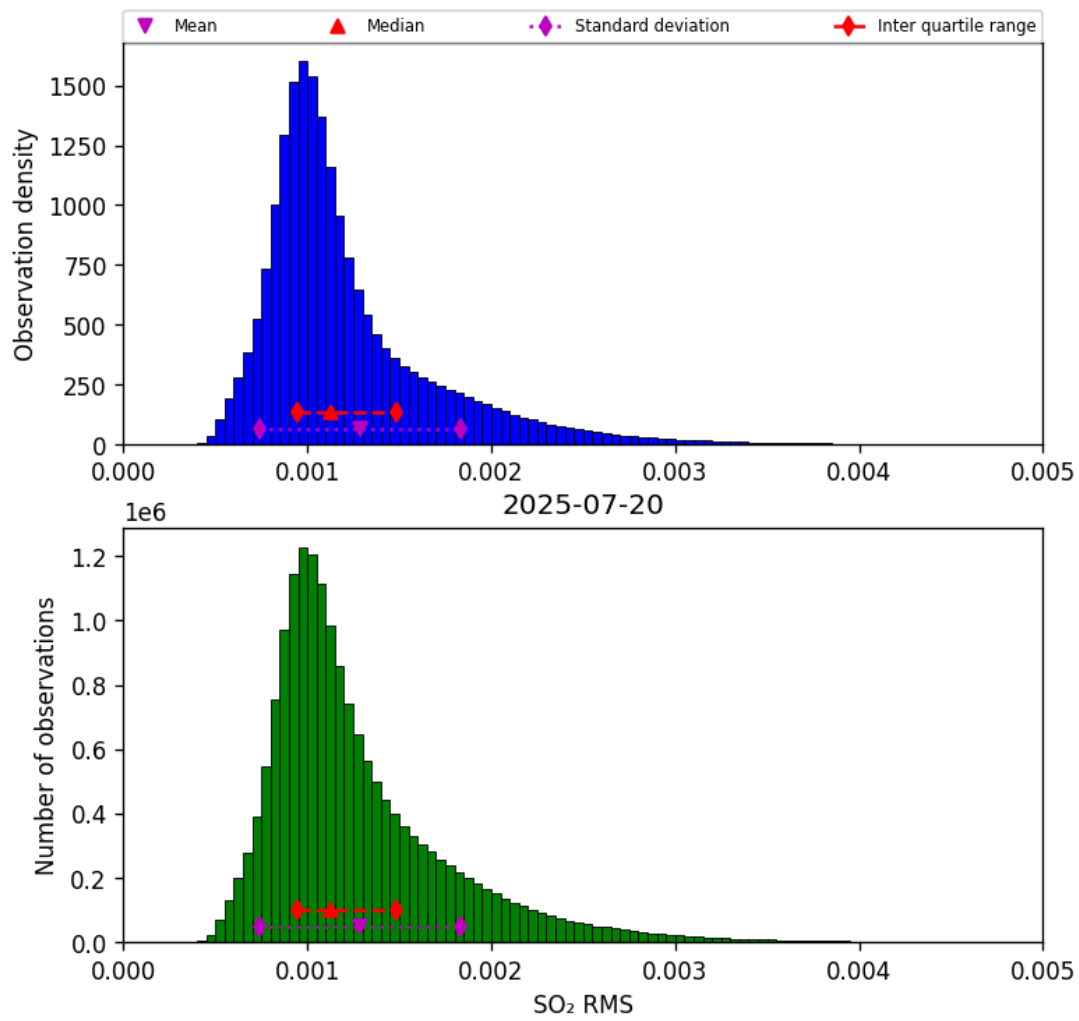
Figure 79: Histogram of “SO 2 RMS” for 2025-07-20 to 2025-07-21
