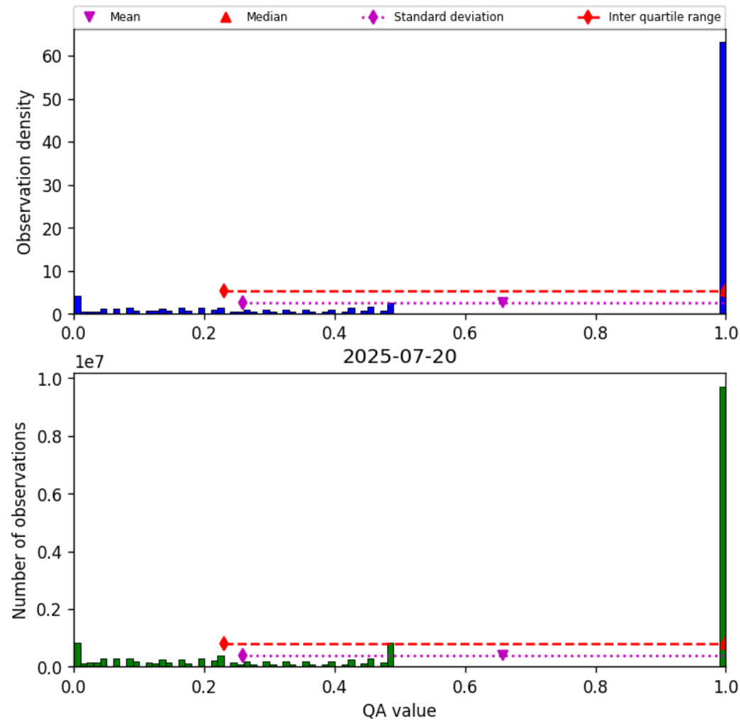
Figure 57: Histogram of “QA value” for 2025-07-20 to 2025-07-21
