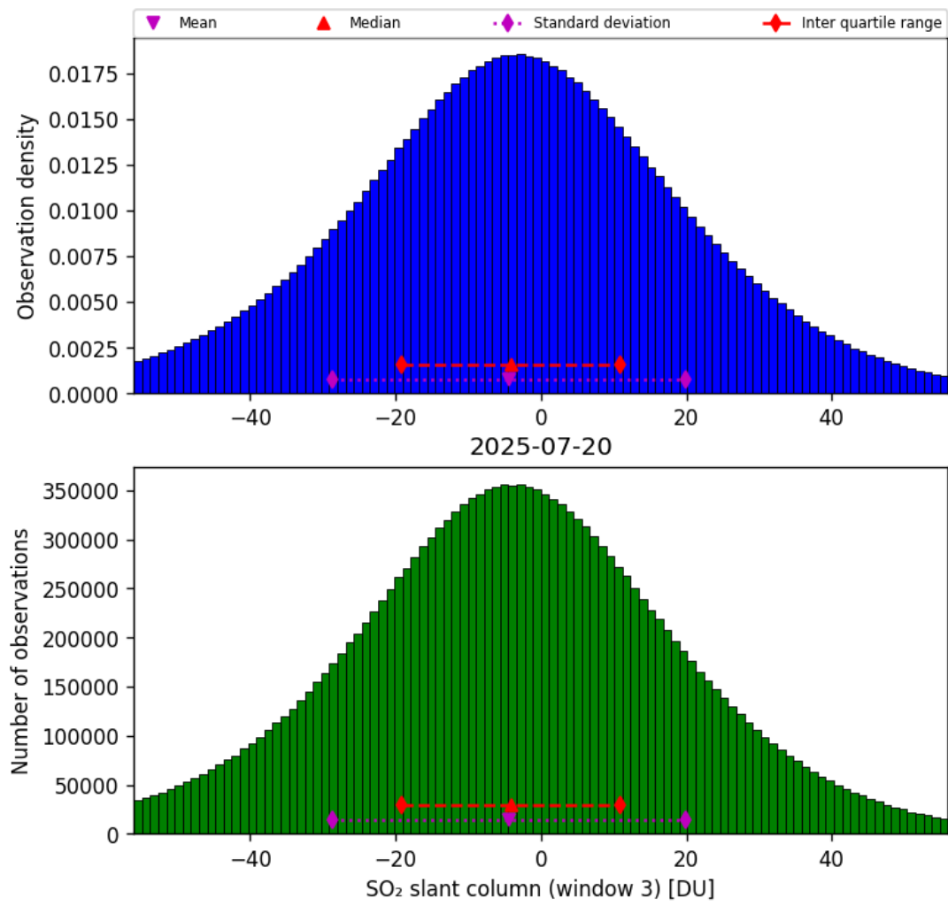
Figure 71: Histogram of “SO 2 slant column (window 3)” for 2025-07-20 to 2025-07-21
