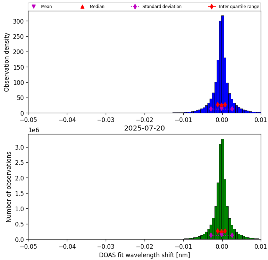
Figure 77: Histogram of “DOAS fit wavelength shift” for 2025-07-20 to 2025-07-21
