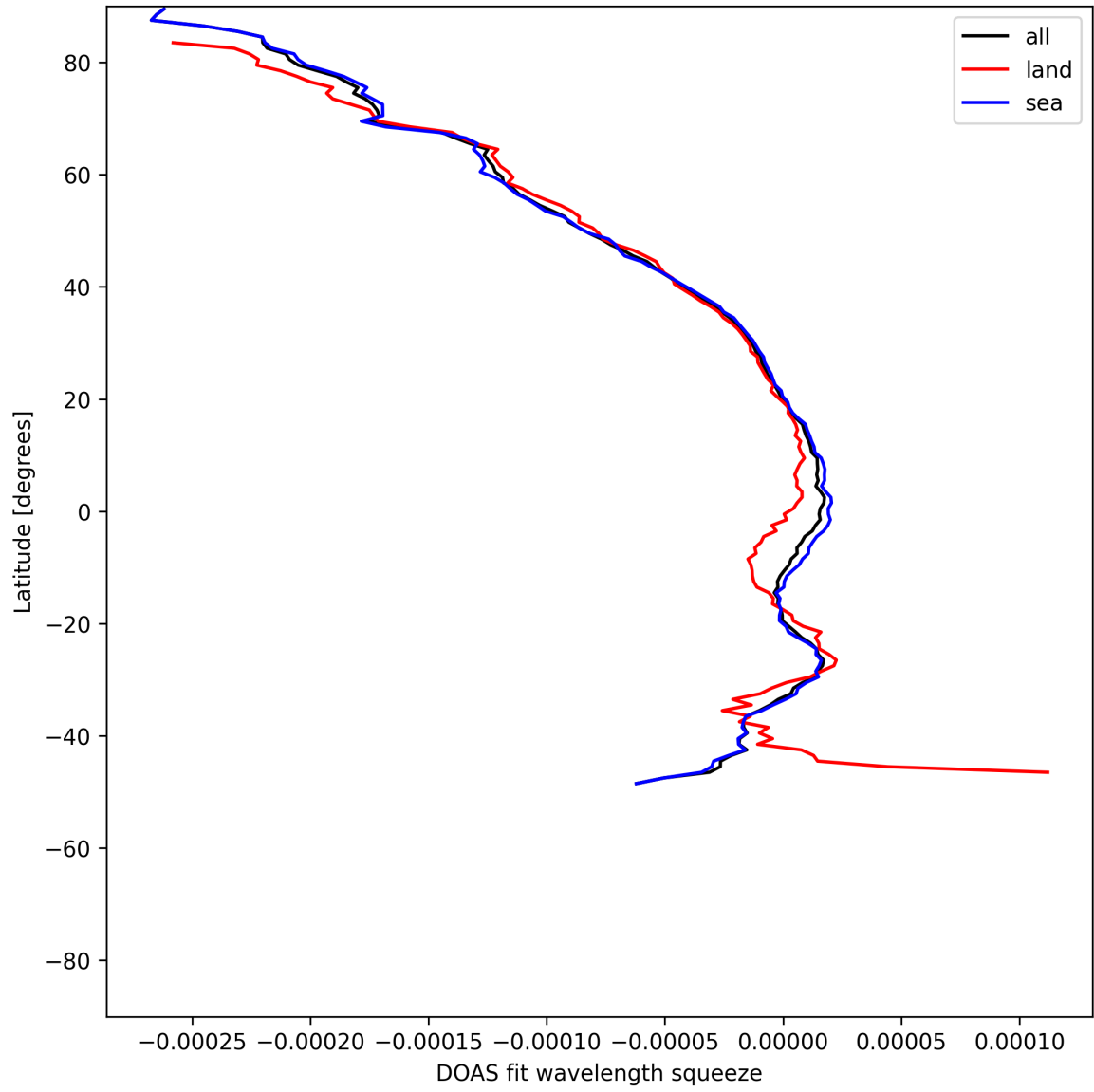
Figure 51: Zonal average of “DOAS fit wavelength squeeze” for 2025-07-20 to 2025-07-21.
