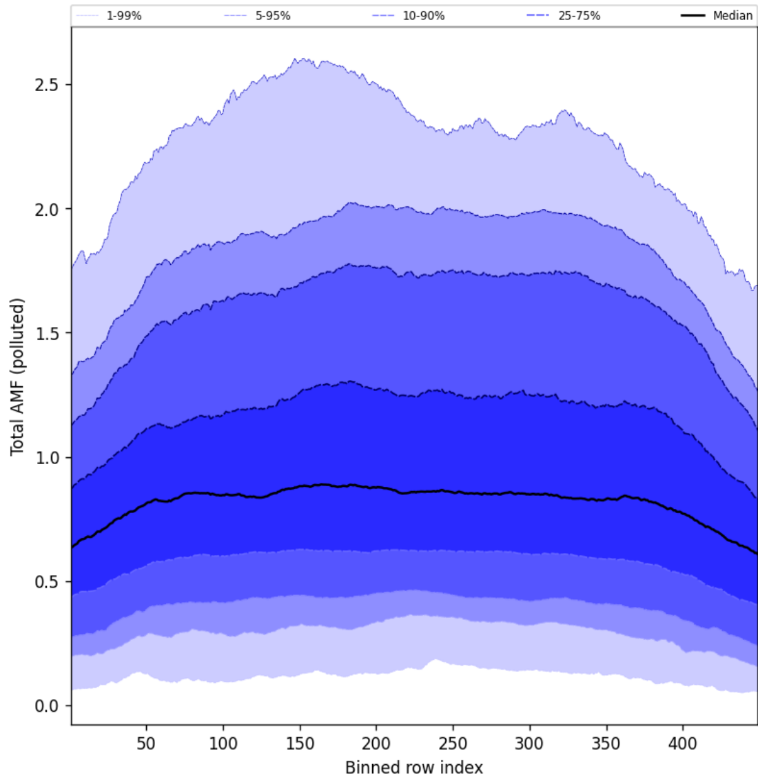
Figure 107: Along track statistics of “Total AMF (polluted)” for 2025-07-20 to 2025-07-21
