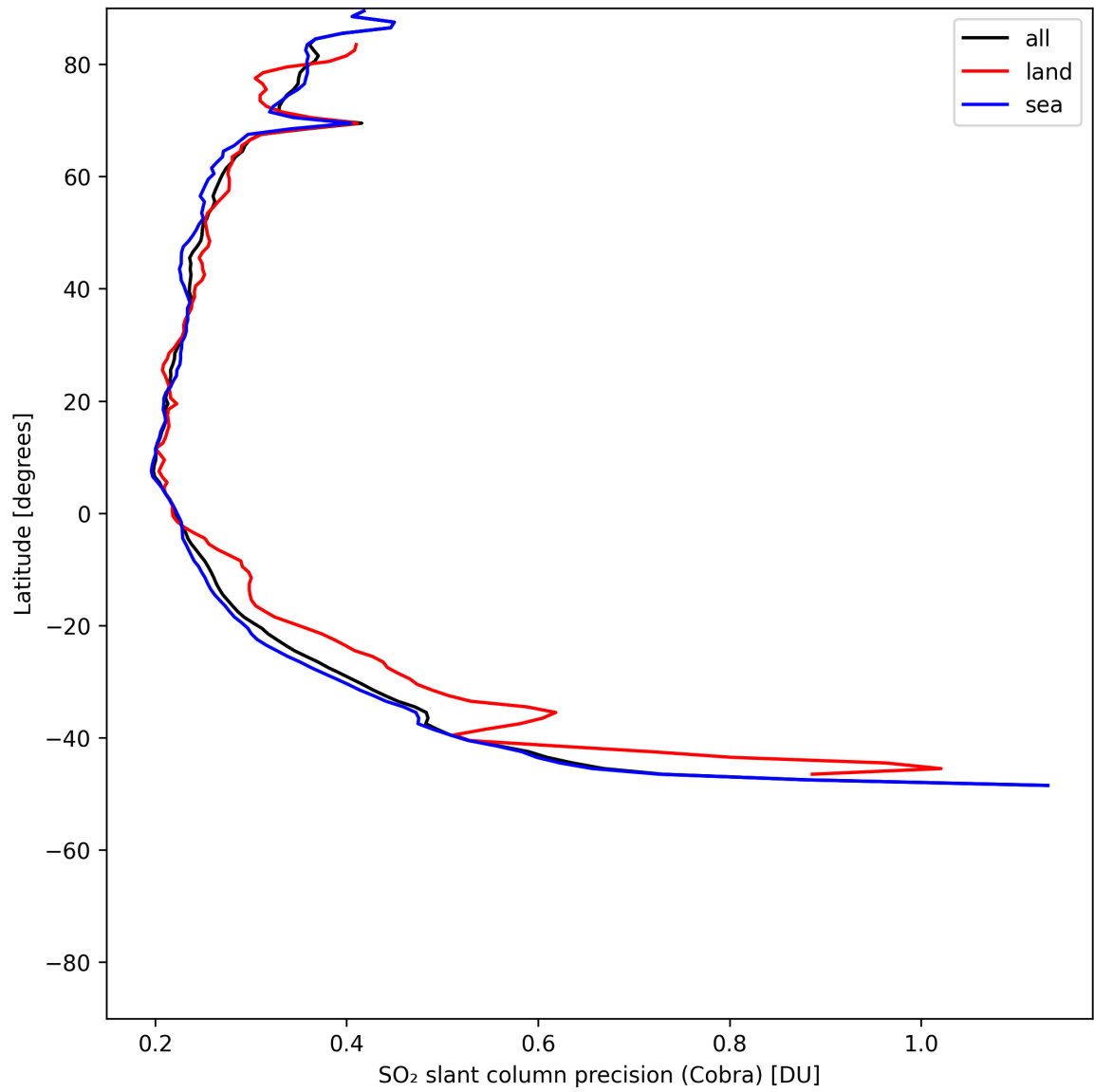
Figure 35: Zonal average of “SO 2 slant column precision (Cobra)” for 2025-07-20 to 2025-07-21.
