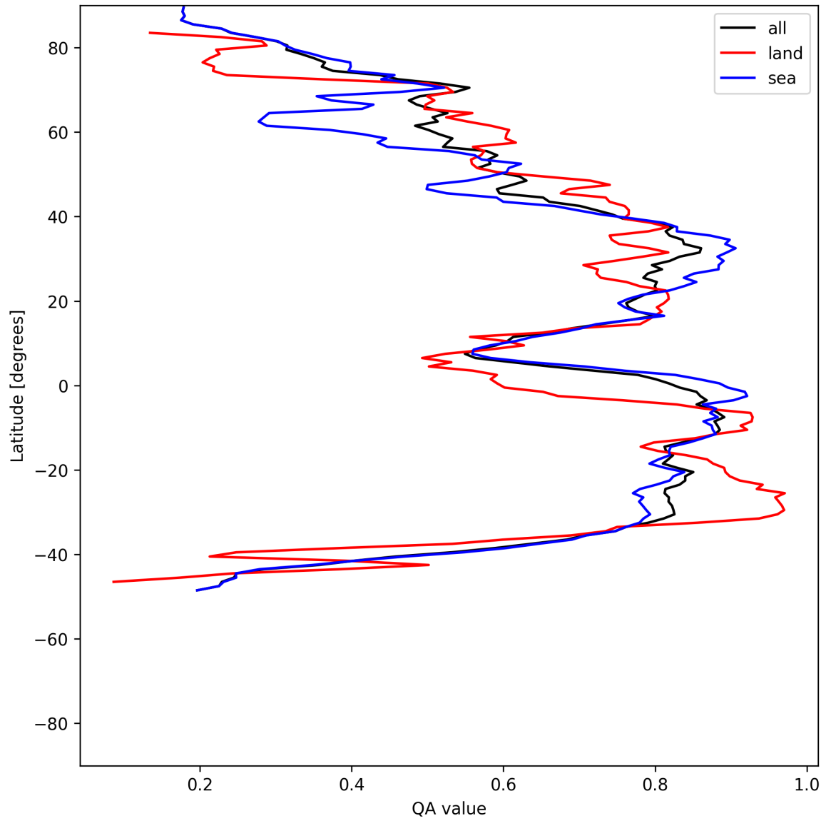
Figure 30: Zonal average of “QA value” for 2025-07-20 to 2025-07-21.
