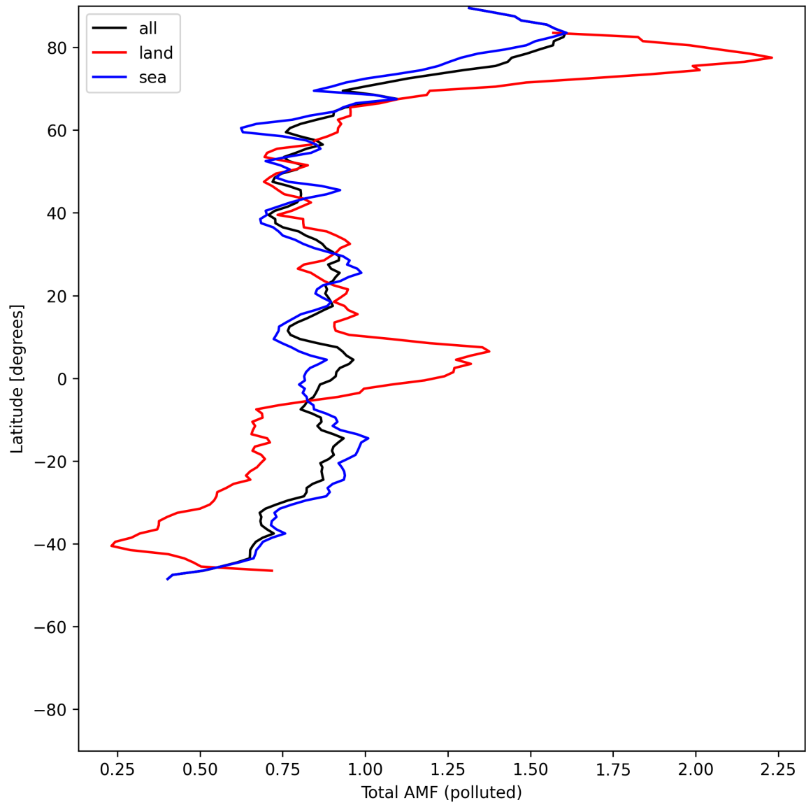
Figure 53: Zonal average of “Total AMF (polluted)” for 2025-07-20 to 2025-07-21.
