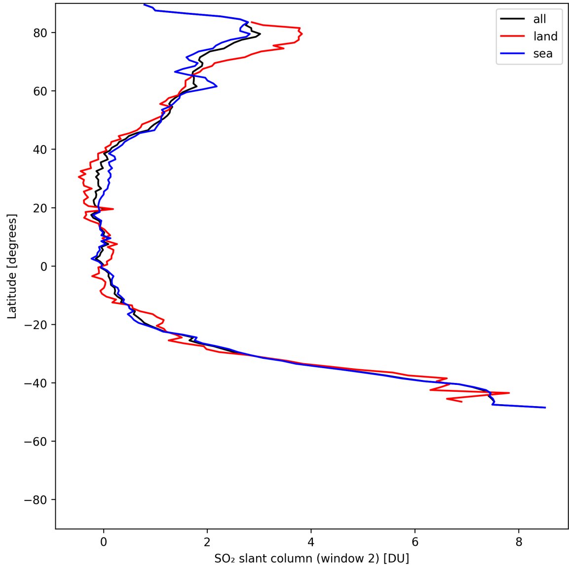
Figure 40: Zonal average of “SO 2 slant column (window 2)” for 2025-07-20 to 2025-07-21.
