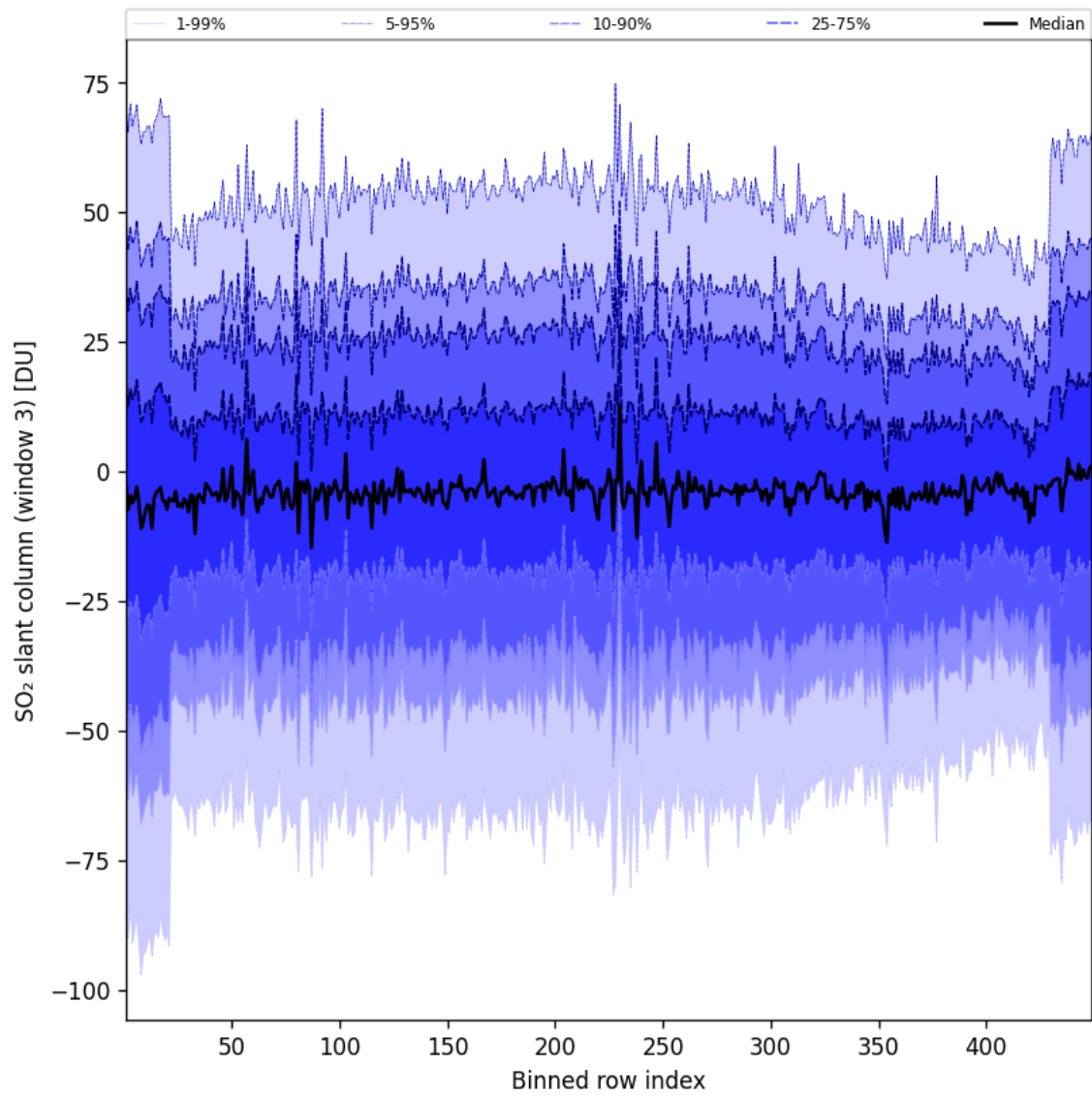
Figure 98: Along track statistics of “SO 2 slant column (window 3)” for 2025-07-20 to 2025-07-21
