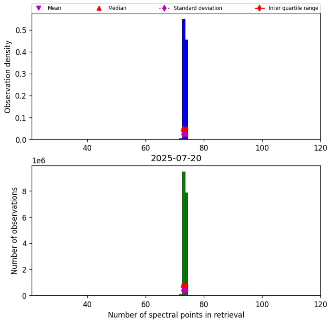
Figure 83: Histogram of “Number of spectral points in retrieval” for 2025-07-20 to 2025-07-21
