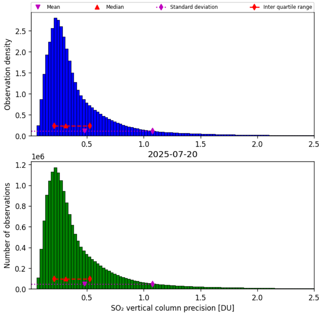
Figure 59: Histogram of “SO 2 vertical column precision” for 2025-07-20 to 2025-07-21
