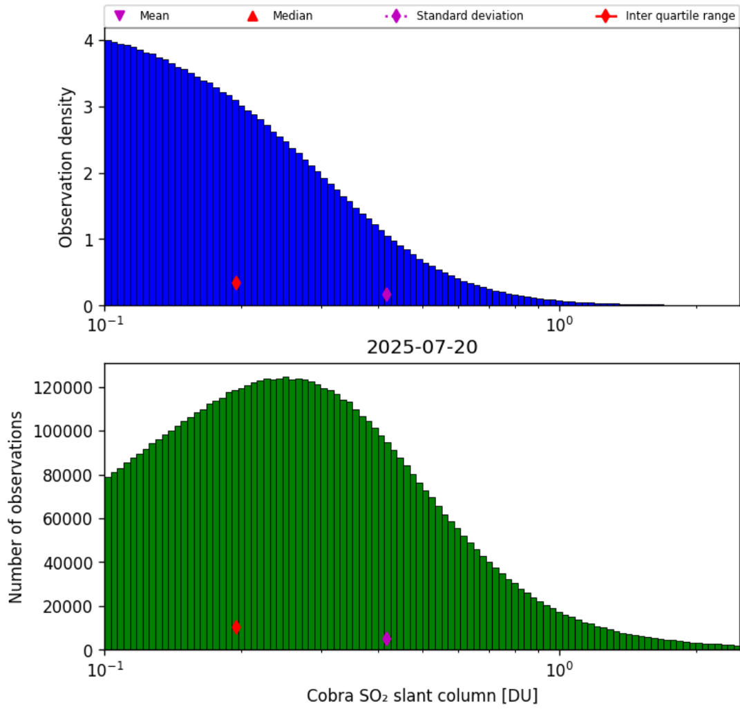
Figure 61: Histogram of “Cobra SO 2 slant column” for 2025-07-20 to 2025-07-21
