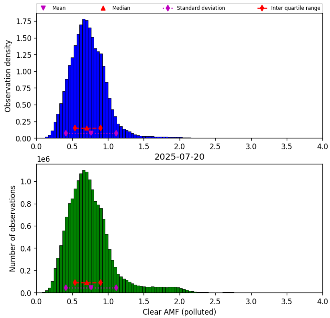
Figure 82: Histogram of “Clear AMF (polluted)” for 2025-07-20 to 2025-07-21
