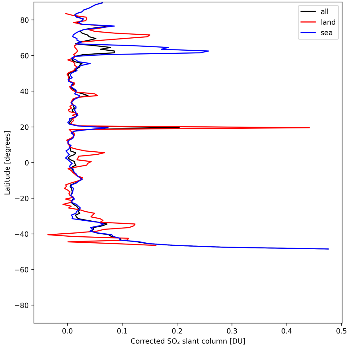
Figure 33: Zonal average of “Corrected SO 2 slant column” for 2025-07-20 to 2025-07-21.
