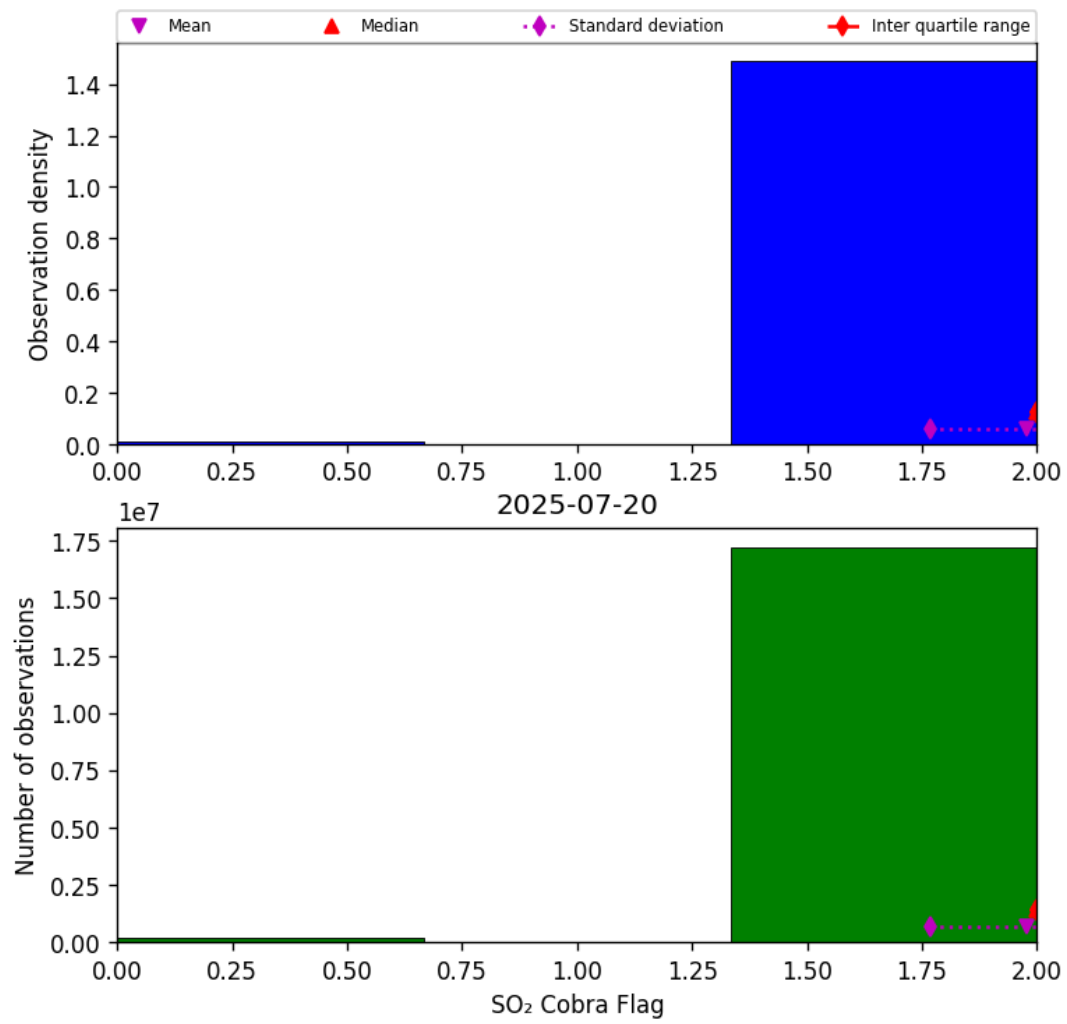
Figure 75: Histogram of “SO 2 Cobra Flag” for 2025-07-20 to 2025-07-21
