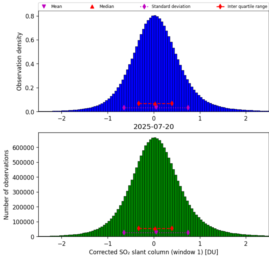
Figure 65: Histogram of “Corrected SO 2 slant column (window 1)” for 2025-07-20 to 2025-07-21
