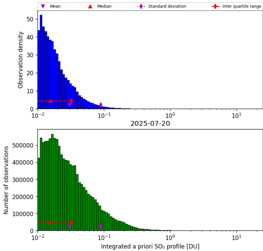
Figure 76: Histogram of “Integrated a priori SO 2 profile” for 2025-07-20 to 2025-07-21
