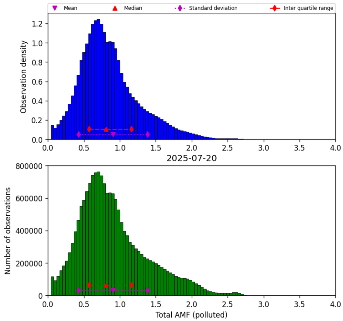
Figure 80: Histogram of “Total AMF (polluted)” for 2025-07-20 to 2025-07-21
