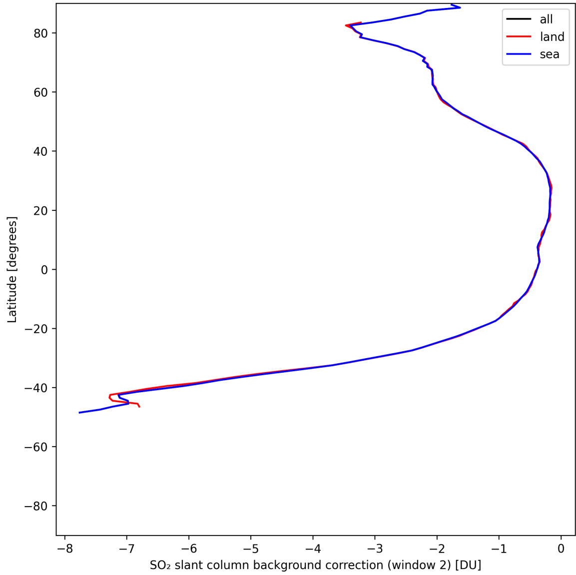
Figure 43: Zonal average of “SO 2 slant column background correction (window 2)” for 2025-07-20 to 2025-07-21.
