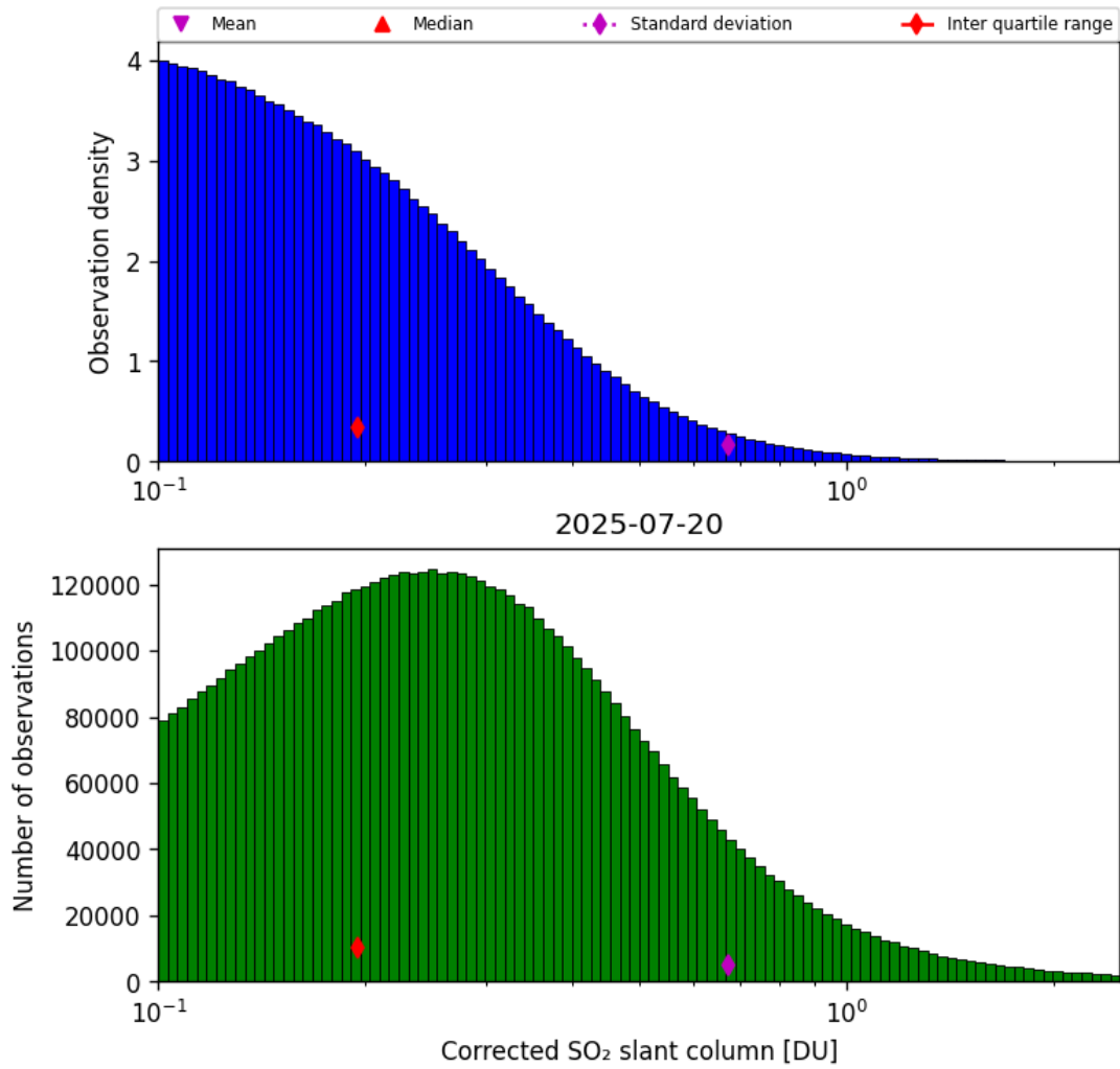
Figure 60: Histogram of “Corrected SO 2 slant column” for 2025-07-20 to 2025-07-21
