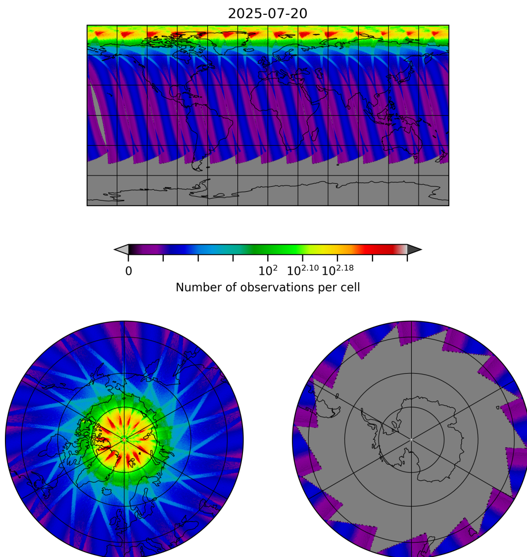
Figure 29: Map of the number of observations for 2025-07-20 to 2025-07-21
