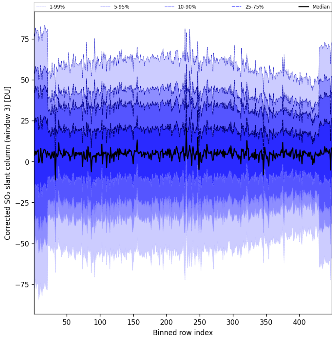
Figure 100: Along track statistics of “Corrected SO 2 slant column (window 3)” for 2025-07-20 to 2025-07-21
