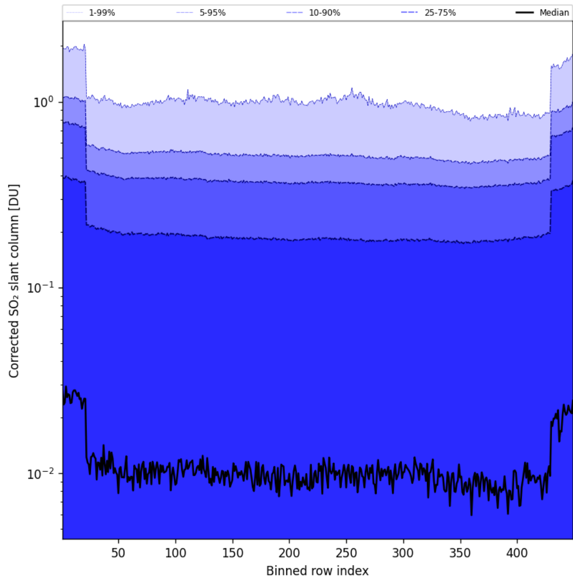
Figure 87: Along track statistics of “Corrected SO 2 slant column” for 2025-07-20 to 2025-07-21
