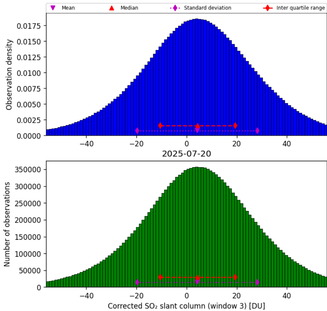
Figure 73: Histogram of “Corrected SO 2 slant column (window 3)” for 2025-07-20 to 2025-07-21
