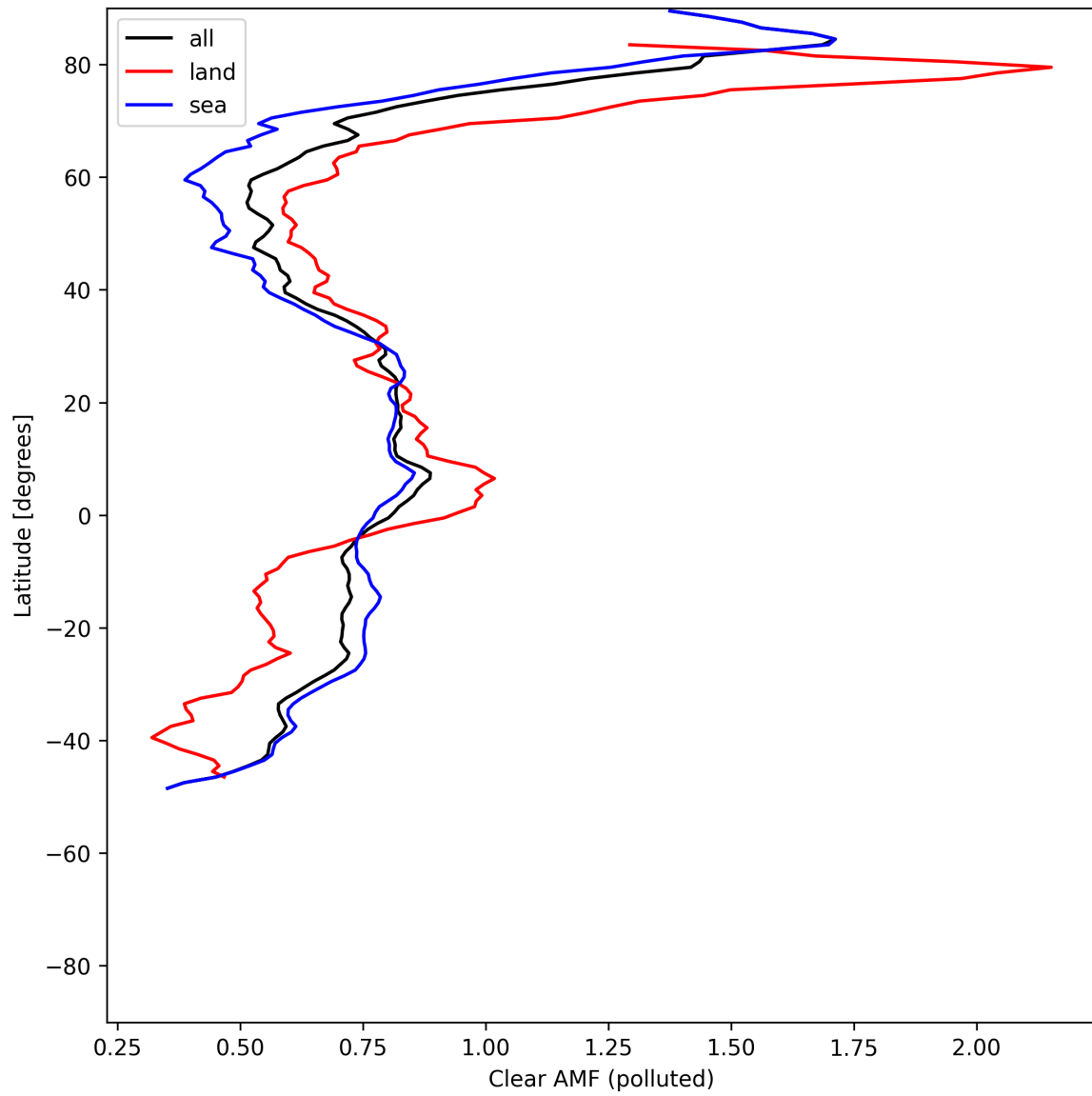
Figure 55: Zonal average of “Clear AMF (polluted)” for 2025-07-20 to 2025-07-21.
