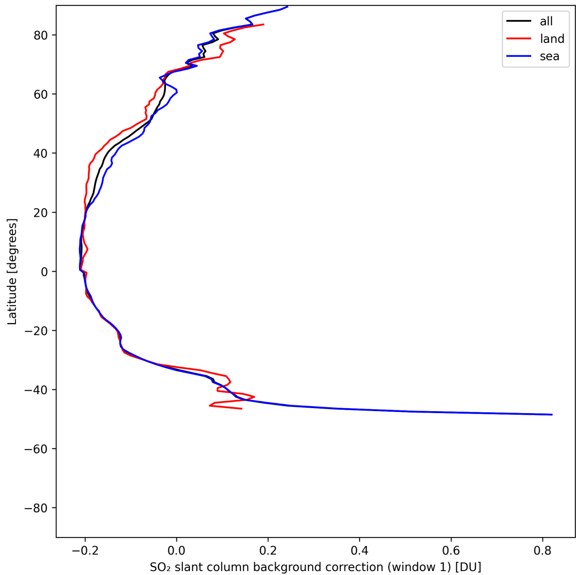
Figure 39: Zonal average of “SO 2 slant column background correction (window 1)” for 2025-07-20 to 2025-07-21.
