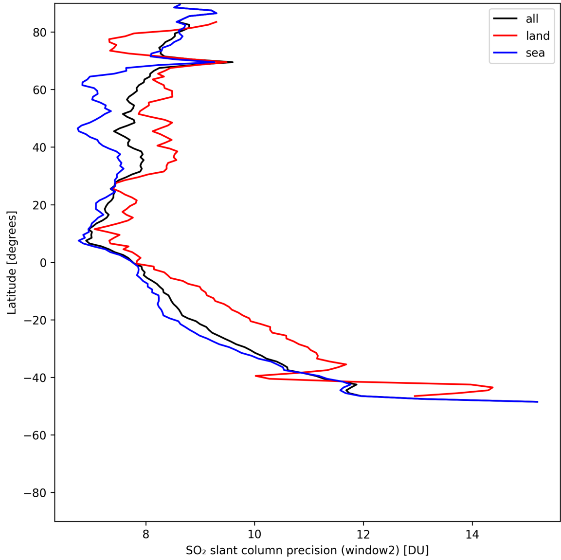
Figure 41: Zonal average of “SO 2 slant column precision (window2)” for 2025-07-20 to 2025-07-21.
