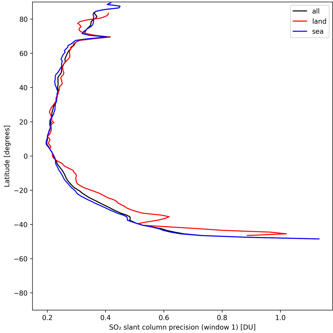
Figure 37: Zonal average of “SO 2 slant column precision (window 1)” for 2025-07-20 to 2025-07-21.
