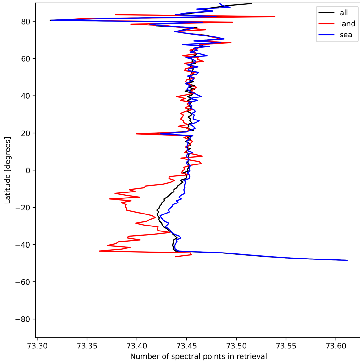
Figure 56: Zonal average of “Number of spectral points in retrieval” for 2025-07-20 to 2025-07-21.
