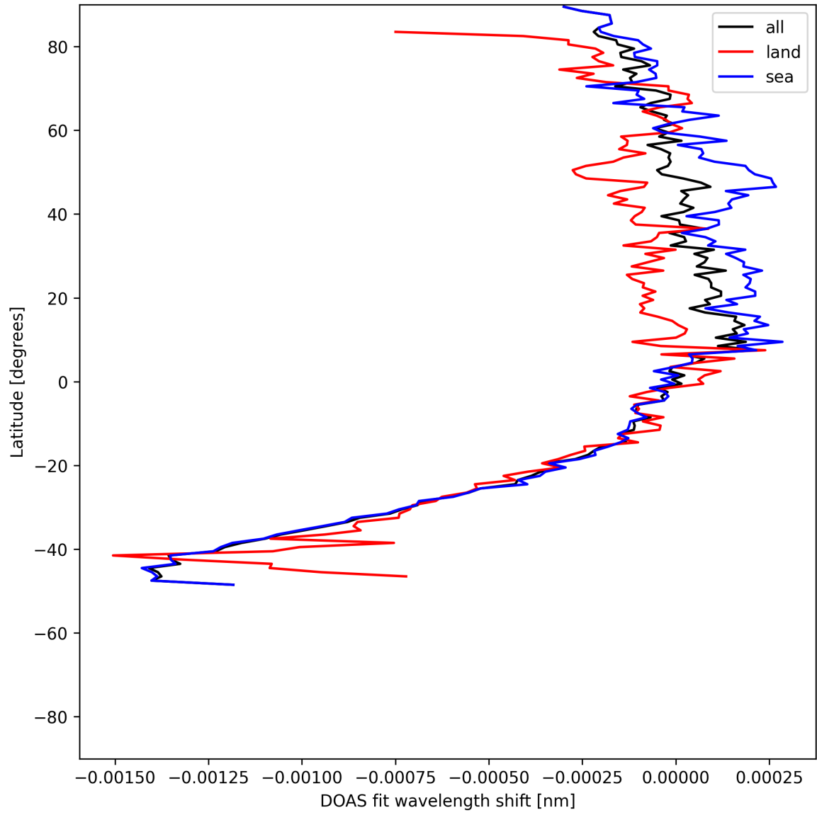
Figure 50: Zonal average of “DOAS fit wavelength shift” for 2025-07-20 to 2025-07-21.
