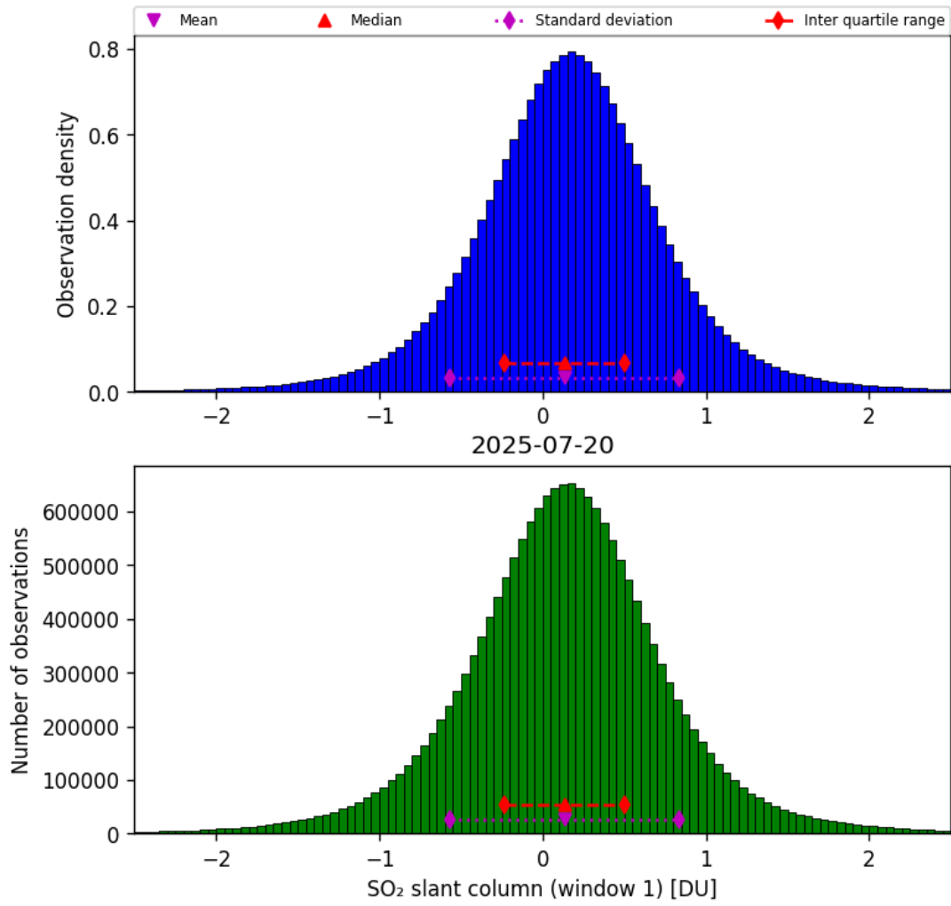
Figure 63: Histogram of “SO 2 slant column (window 1)” for 2025-07-20 to 2025-07-21
