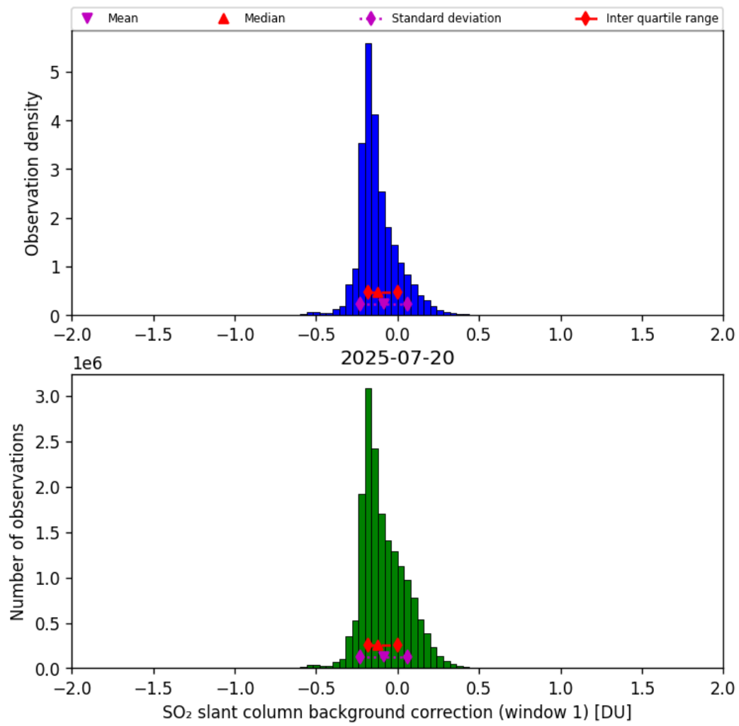
Figure 66: Histogram of “SO 2 slant column background correction (window 1)” for 2025-07-20 to 2025-07-21
