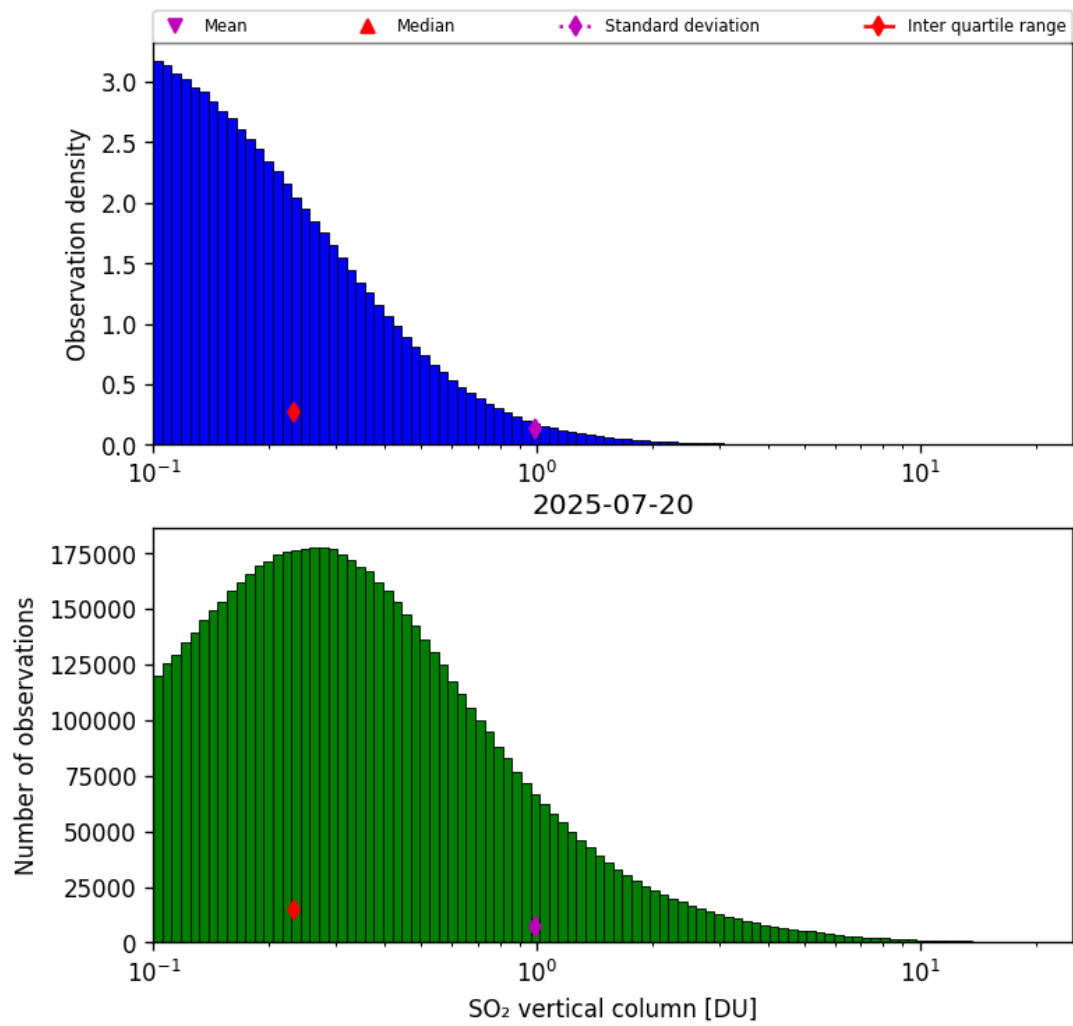
Figure 58: Histogram of “SO 2 vertical column” for 2025-07-20 to 2025-07-21
