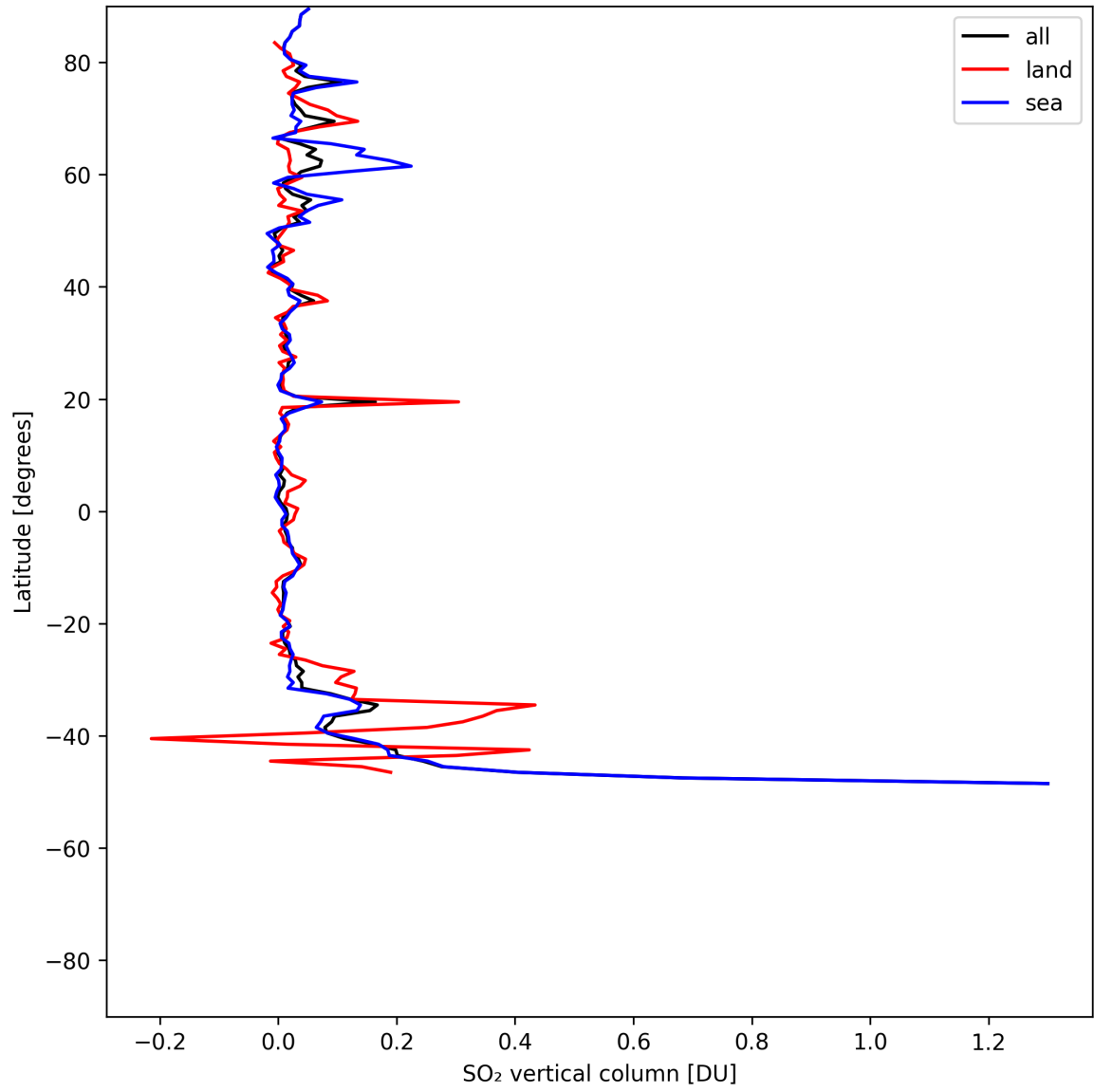
Figure 31: Zonal average of “SO 2 vertical column” for 2025-07-20 to 2025-07-21.
