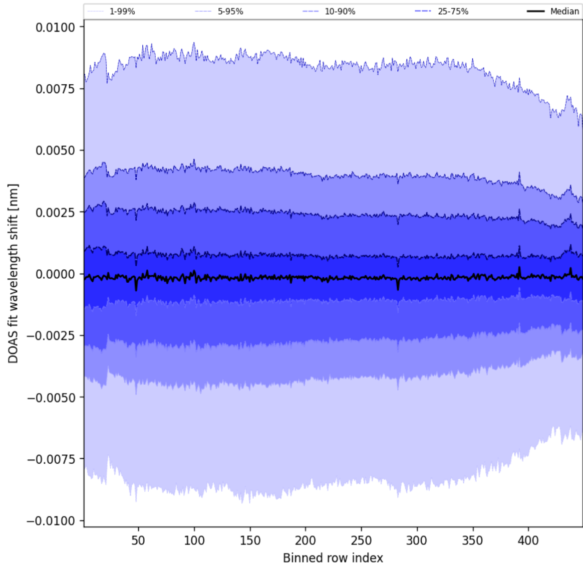
Figure 104: Along track statistics of “DOAS fit wavelength shift” for 2025-07-20 to 2025-07-21
