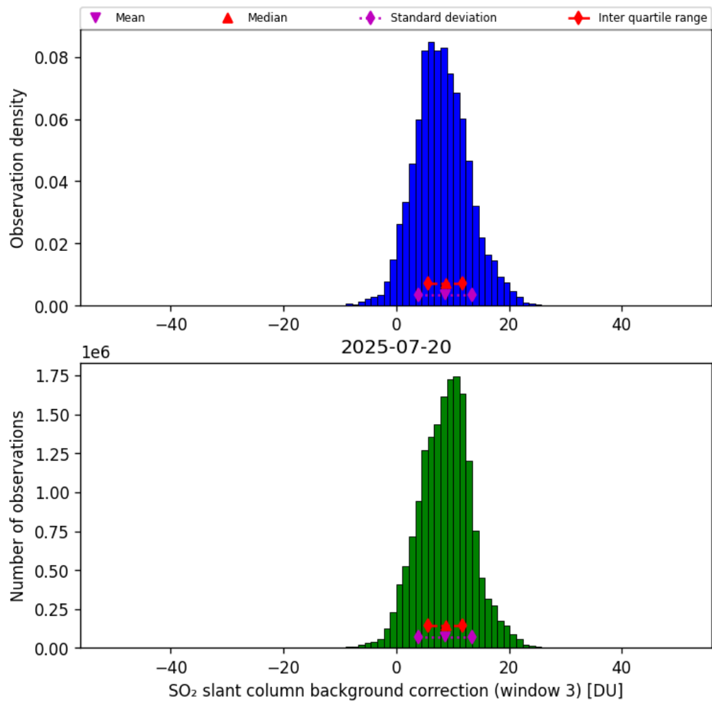
Figure 74: Histogram of “SO 2 slant column background correction (window 3)” for 2025-07-20 to 2025-07-21
