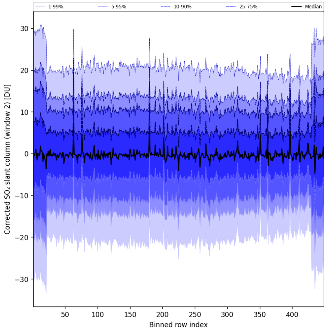
Figure 96: Along track statistics of “Corrected SO 2 slant column (window 2)” for 2025-07-20 to 2025-07-21
