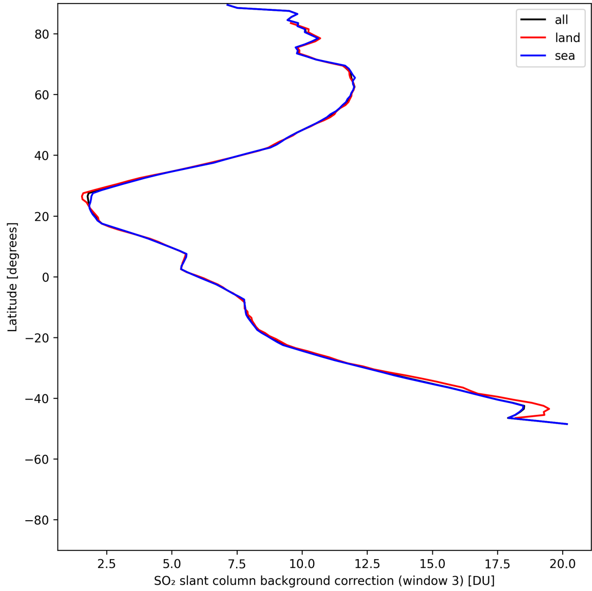
Figure 47: Zonal average of “SO 2 slant column background correction (window 3)” for 2025-07-20 to 2025-07-21.
