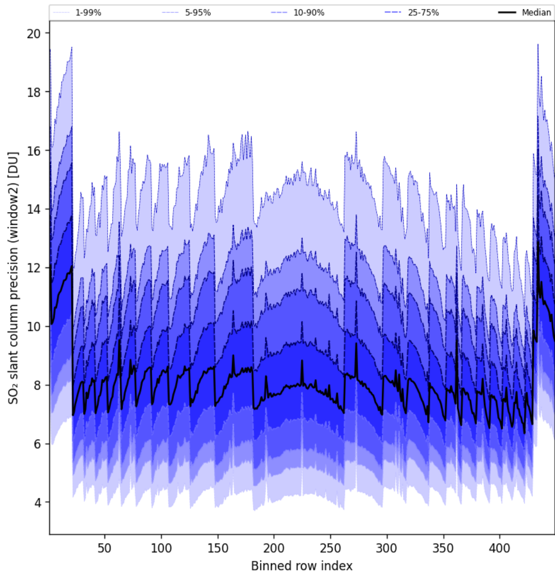
Figure 95: Along track statistics of “SO 2 slant column precision (window2)” for 2025-07-20 to 2025-07-21
