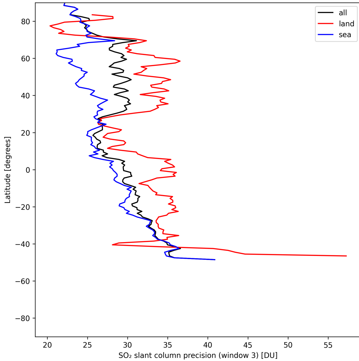
Figure 45: Zonal average of “SO 2 slant column precision (window 3)” for 2025-07-20 to 2025-07-21.
