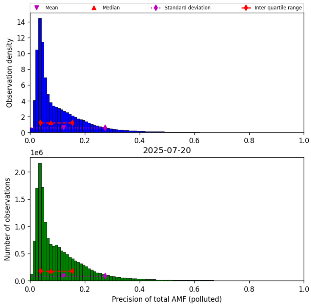
Figure 81: Histogram of “Precision of total AMF (polluted)” for 2025-07-20 to 2025-07-21
