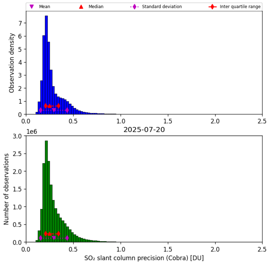
Figure 62: Histogram of “SO 2 slant column precision (Cobra)” for 2025-07-20 to 2025-07-21
