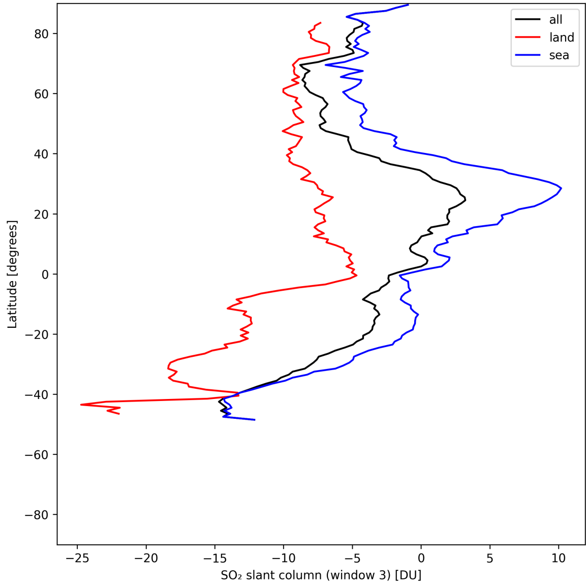
Figure 44: Zonal average of “SO 2 slant column (window 3)” for 2025-07-20 to 2025-07-21.
