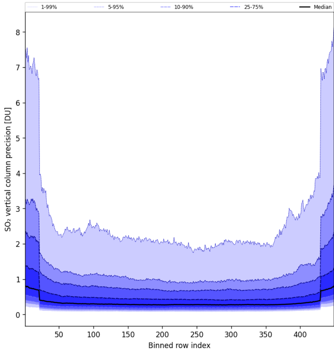
Figure 86: Along track statistics of “SO 2 vertical column precision” for 2025-07-20 to 2025-07-21
