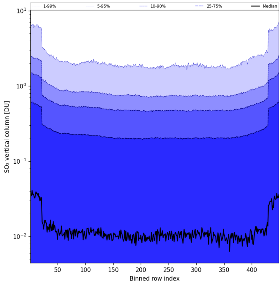
Figure 85: Along track statistics of “SO 2 vertical column” for 2025-07-20 to 2025-07-21
