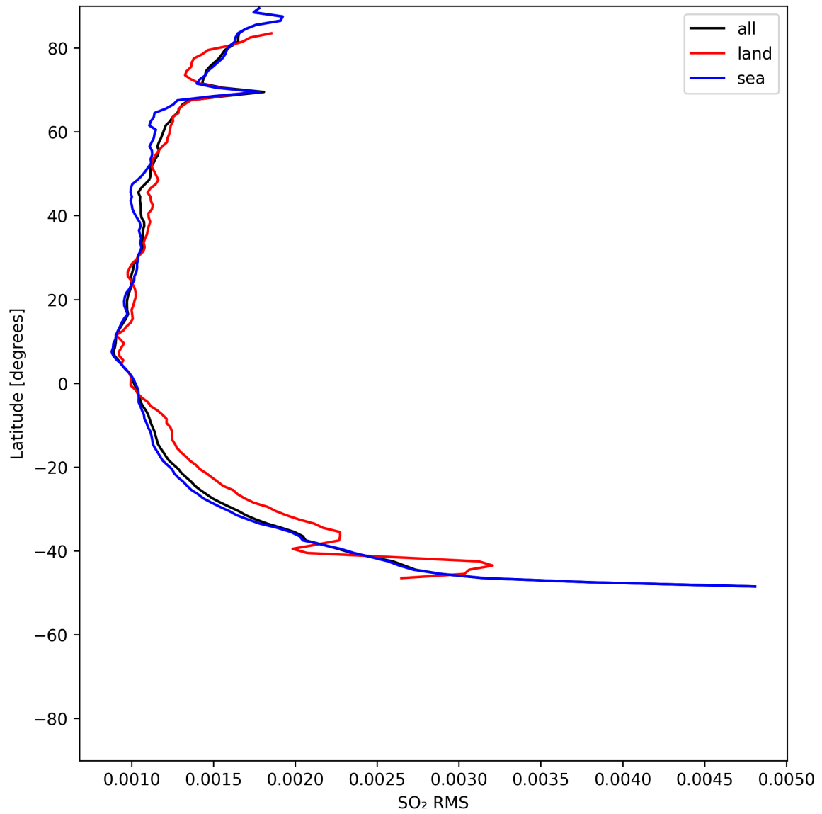
Figure 52: Zonal average of “SO 2 RMS” for 2025-07-20 to 2025-07-21.
