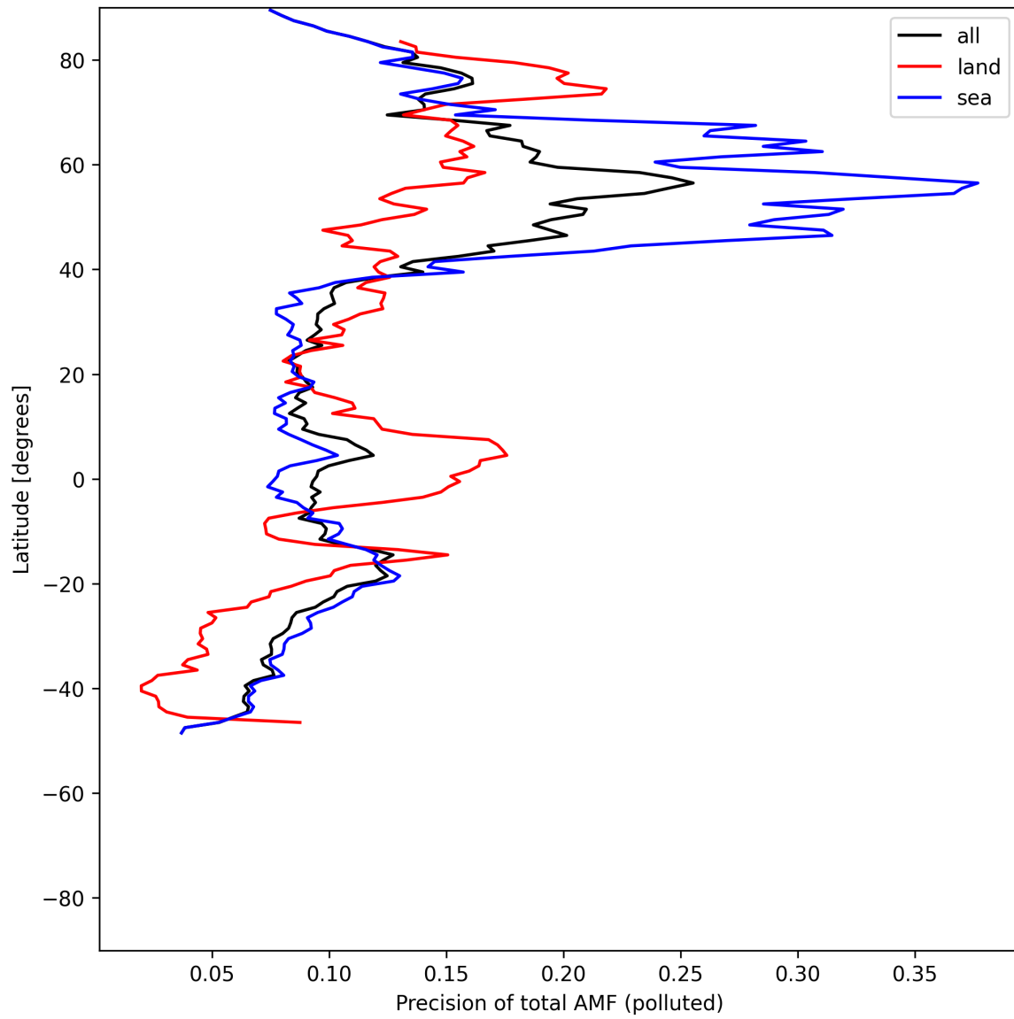
Figure 54: Zonal average of “Precision of total AMF (polluted)” for 2025-07-20 to 2025-07-21.
