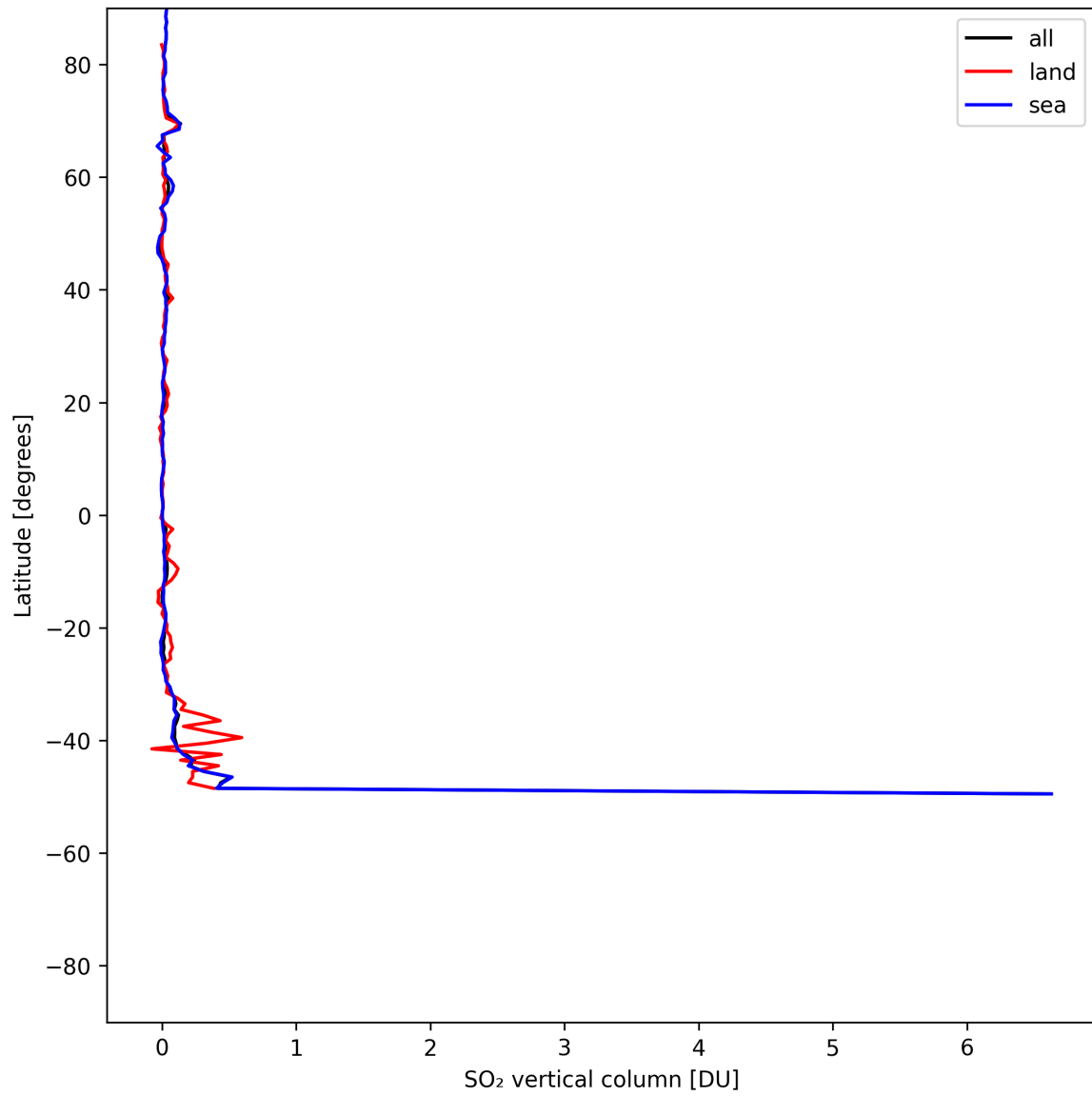
Figure 31: Zonal average of “SO 2 vertical column” for 2025-07-22 to 2025-07-22.
