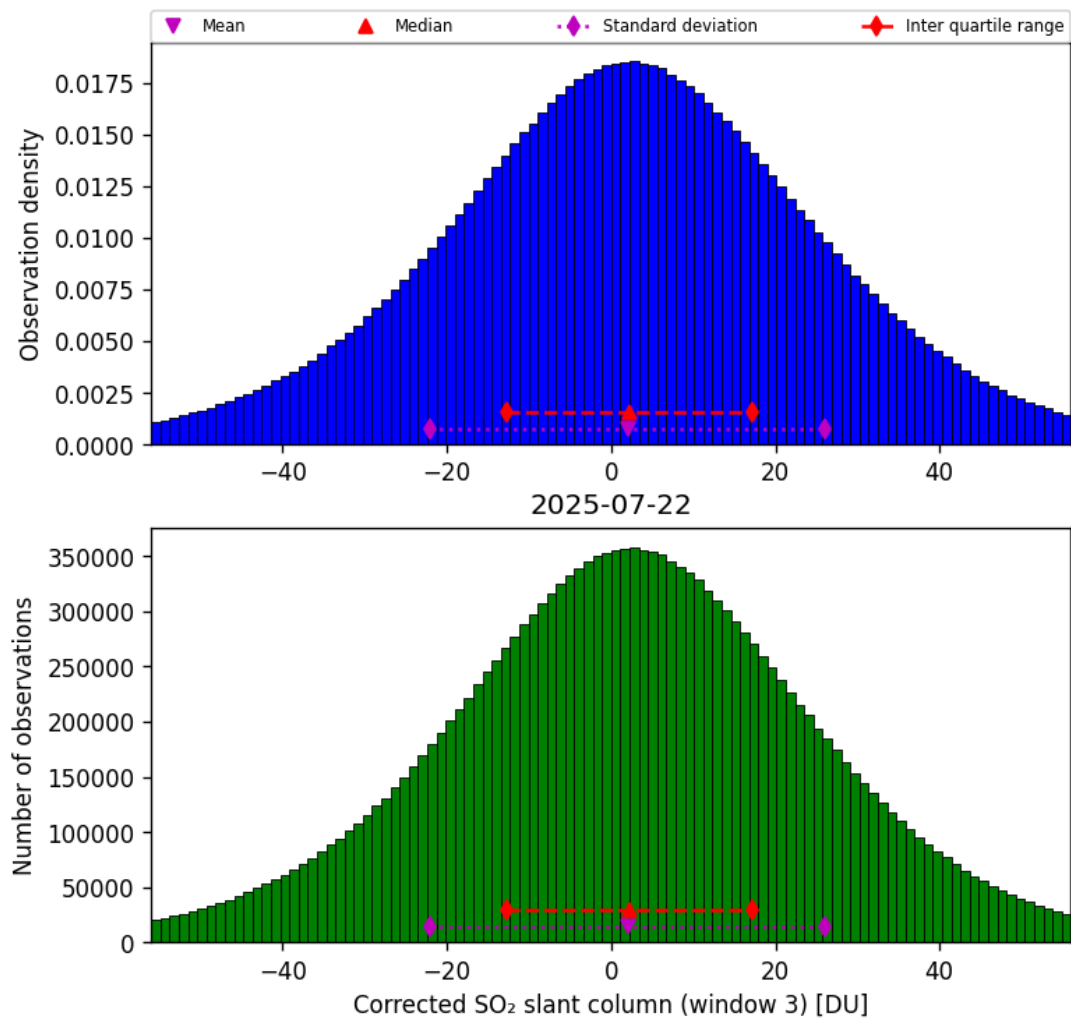
Figure 73: Histogram of “Corrected SO 2 slant column (window 3)” for 2025-07-22 to 2025-07-22
