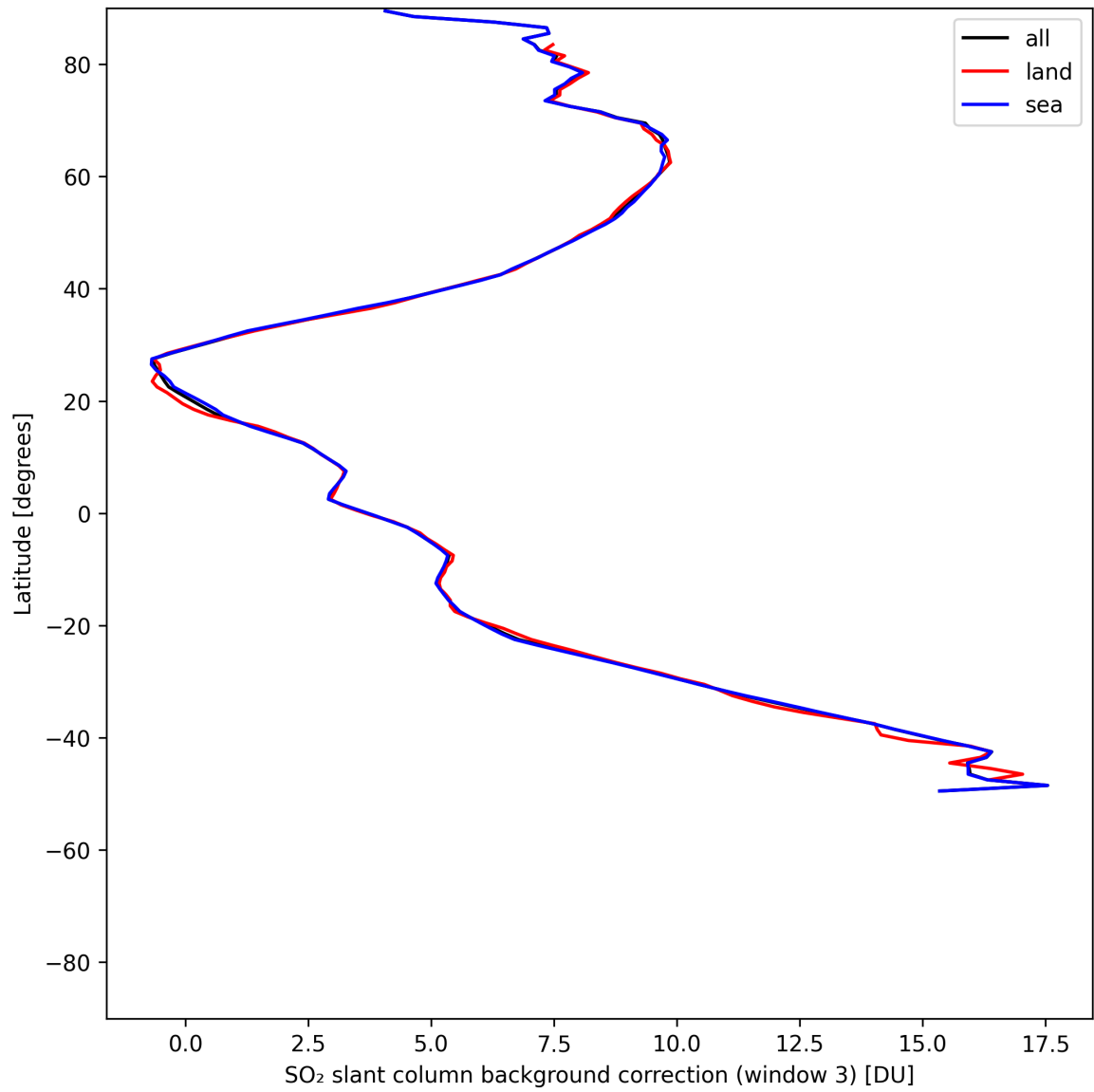
Figure 47: Zonal average of “SO 2 slant column background correction (window 3)” for 2025-07-22 to 2025-07-22.
