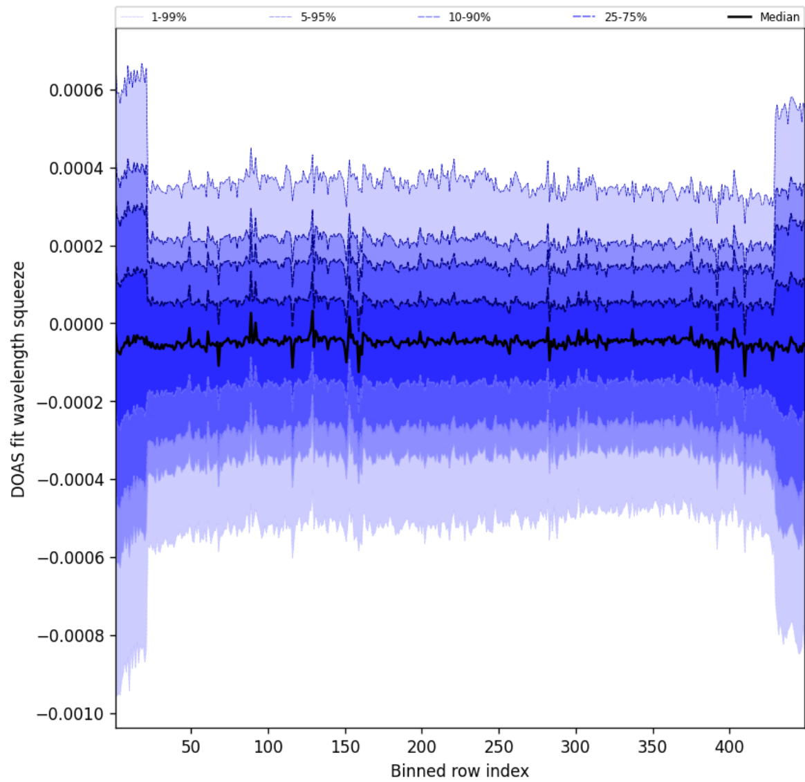
Figure 105: Along track statistics of “DOAS fit wavelength squeeze” for 2025-07-22 to 2025-07-22
