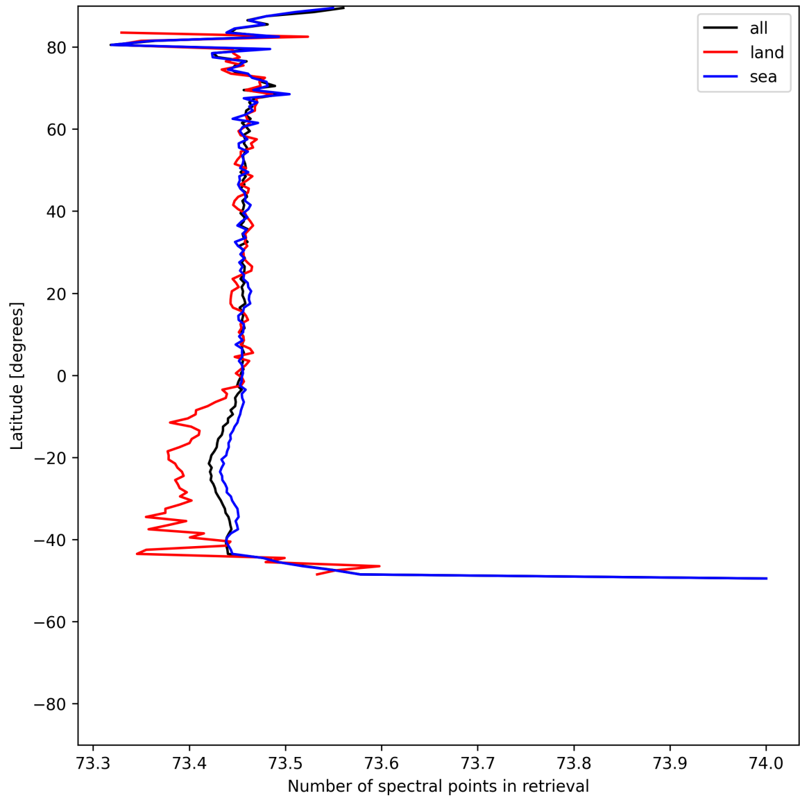
Figure 56: Zonal average of “Number of spectral points in retrieval” for 2025-07-22 to 2025-07-22.
