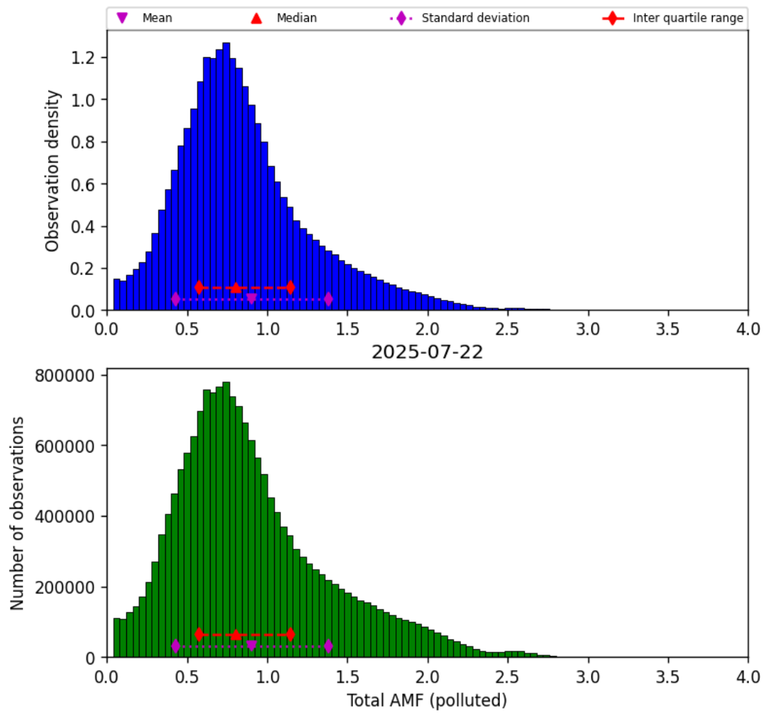
Figure 80: Histogram of “Total AMF (polluted)” for 2025-07-22 to 2025-07-22
