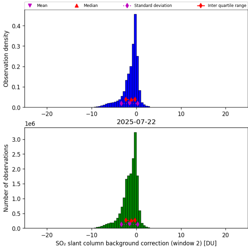
Figure 70: Histogram of “SO 2 slant column background correction (window 2)” for 2025-07-22 to 2025-07-22
