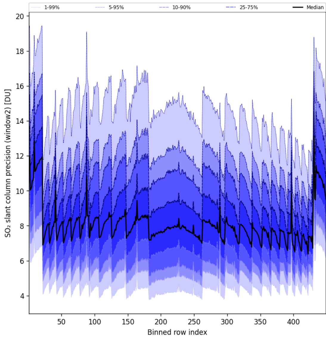
Figure 95: Along track statistics of “SO 2 slant column precision (window2)” for 2025-07-22 to 2025-07-22
