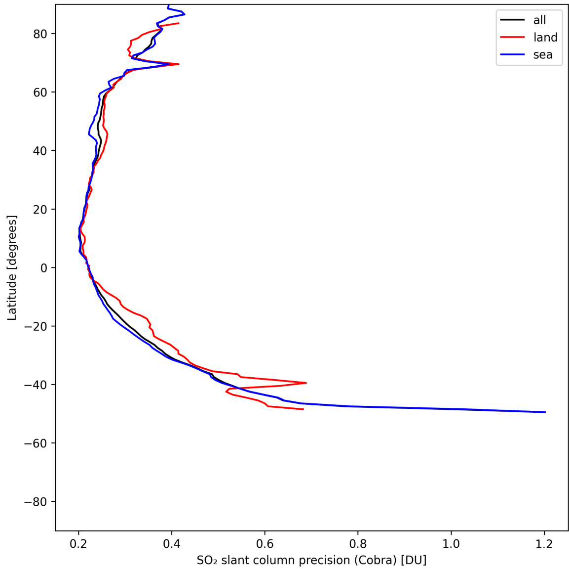
Figure 35: Zonal average of “SO 2 slant column precision (Cobra)” for 2025-07-22 to 2025-07-22.
