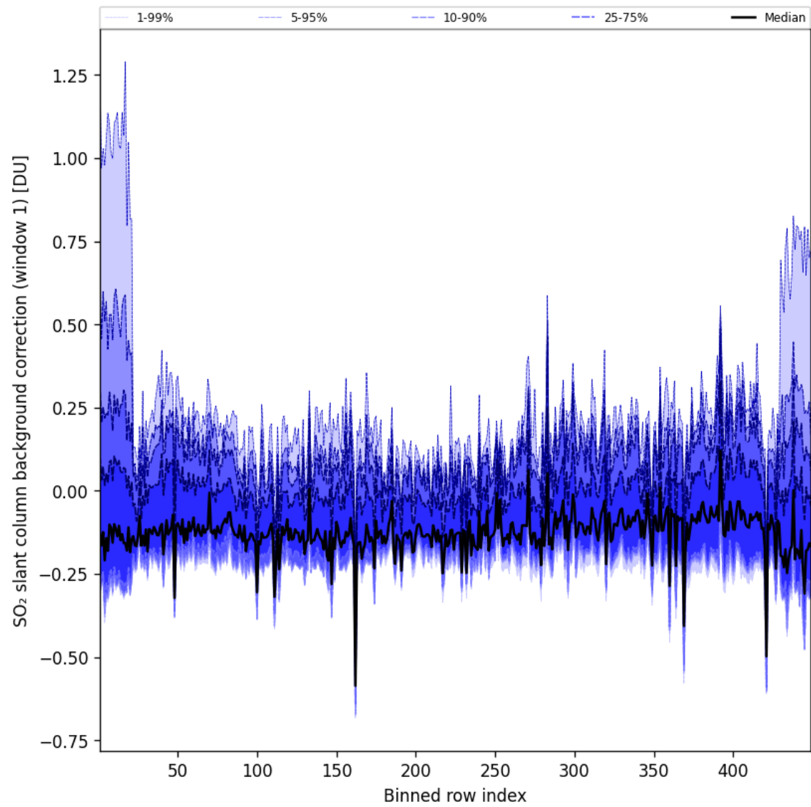
Figure 93: Along track statistics of “SO 2 slant column background correction (window 1)” for 2025-07-22 to 2025-07-22
