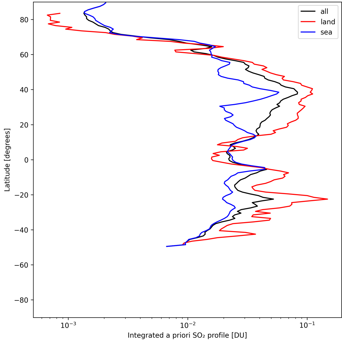
Figure 49: Zonal average of “Integrated a priori SO 2 profile” for 2025-07-22 to 2025-07-22.
