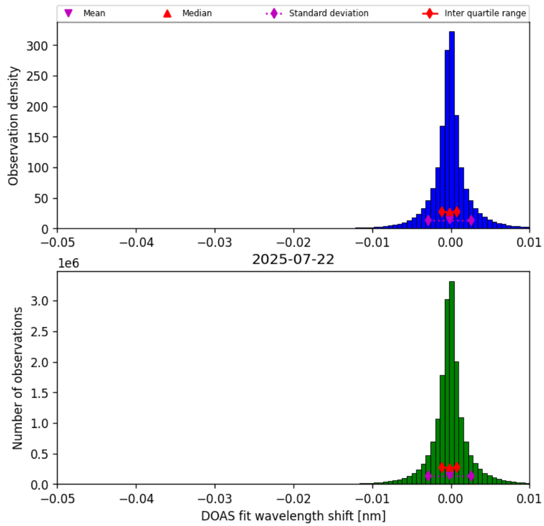
Figure 77: Histogram of “DOAS fit wavelength shift” for 2025-07-22 to 2025-07-22
