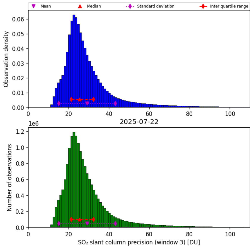
Figure 72: Histogram of “SO 2 slant column precision (window 3)” for 2025-07-22 to 2025-07-22
