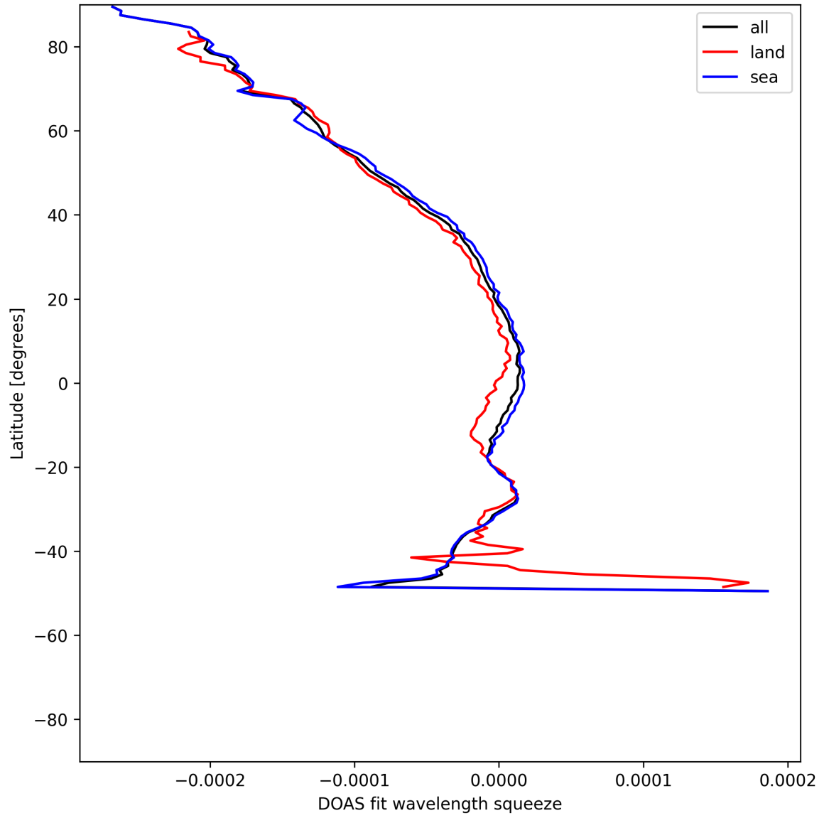
Figure 51: Zonal average of “DOAS fit wavelength squeeze” for 2025-07-22 to 2025-07-22.
