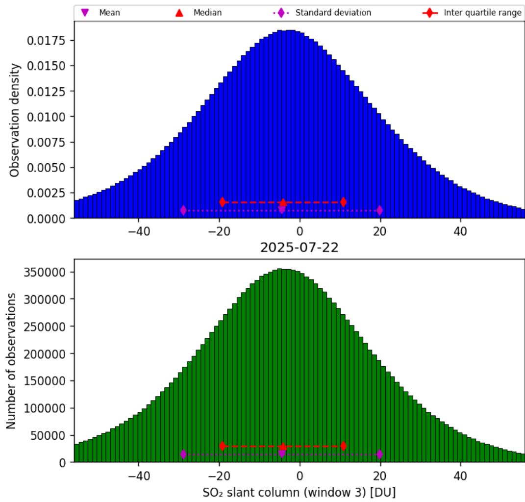
Figure 71: Histogram of “SO 2 slant column (window 3)” for 2025-07-22 to 2025-07-22
