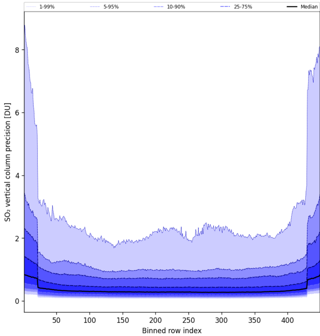
Figure 86: Along track statistics of “SO 2 vertical column precision” for 2025-07-22 to 2025-07-22
