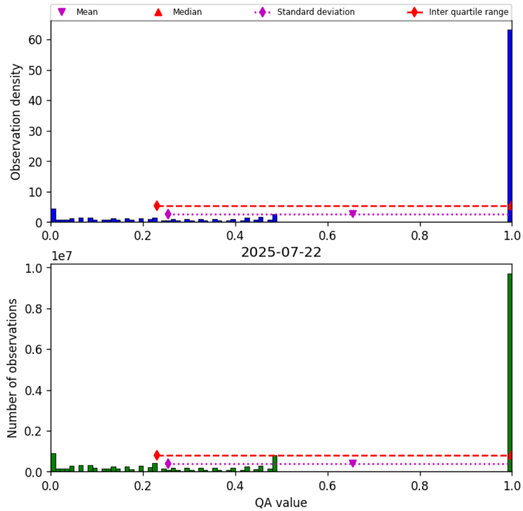
Figure 57: Histogram of “QA value” for 2025-07-22 to 2025-07-22
