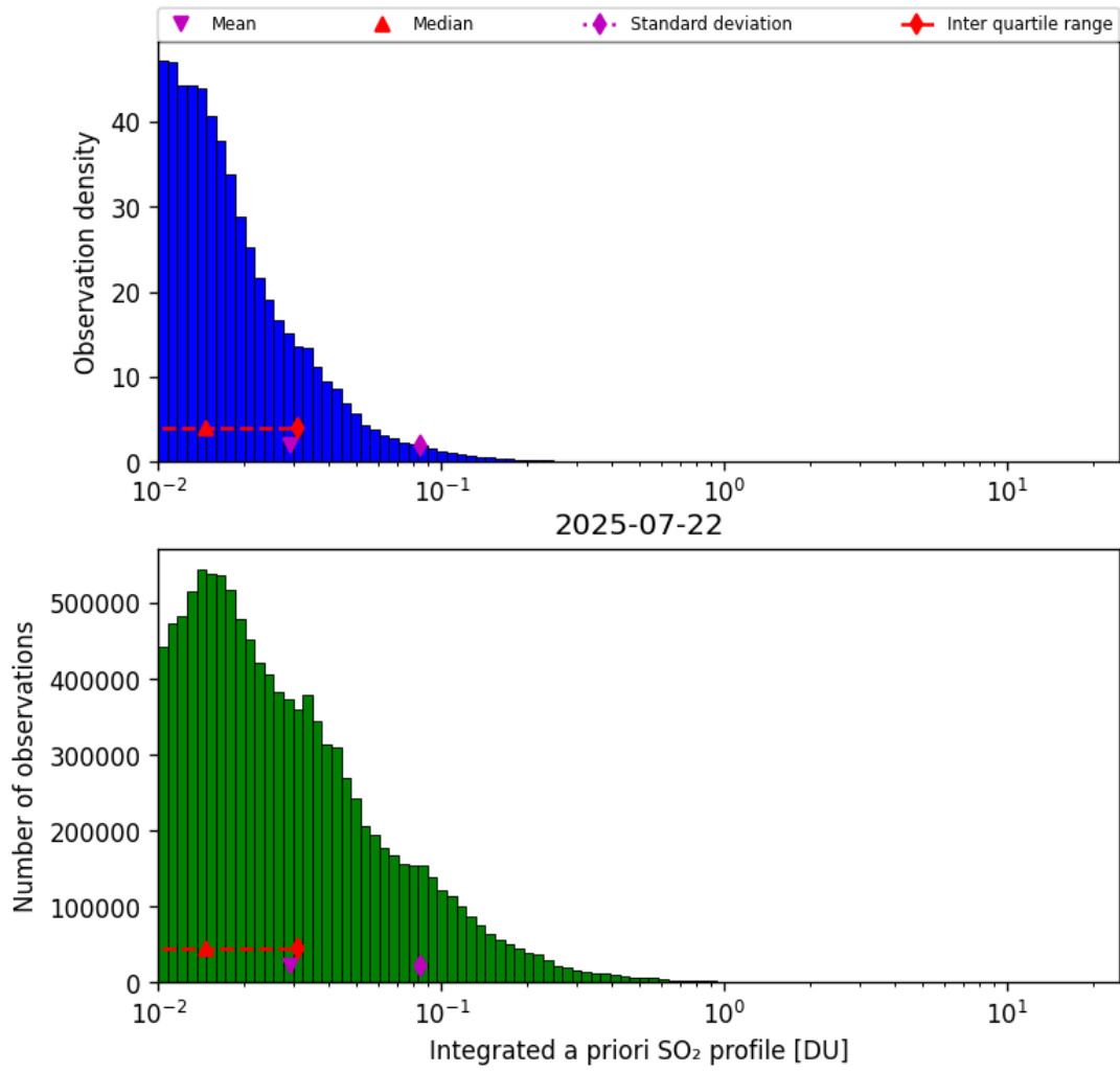
Figure 76: Histogram of “Integrated a priori SO 2 profile” for 2025-07-22 to 2025-07-22
