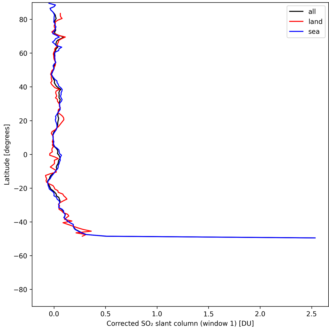
Figure 38: Zonal average of “Corrected SO 2 slant column (window 1)” for 2025-07-22 to 2025-07-22.
