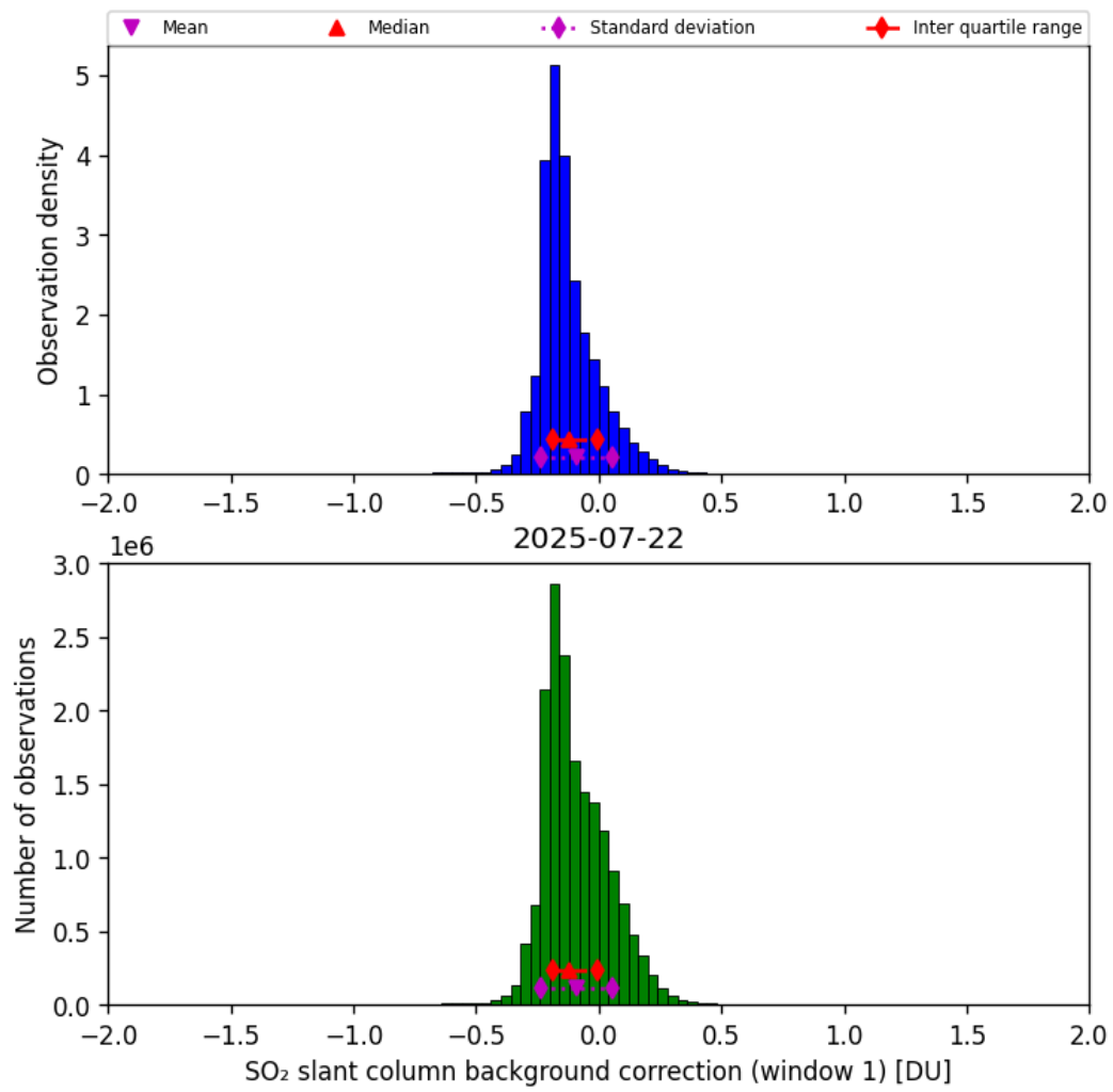
Figure 66: Histogram of “SO 2 slant column background correction (window 1)” for 2025-07-22 to 2025-07-22
