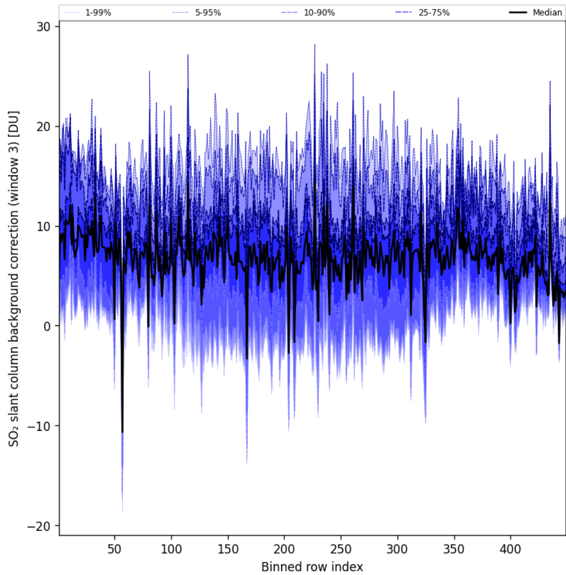
Figure 101: Along track statistics of “SO 2 slant column background correction (window 3)” for 2025-07-22 to 2025-07-22
