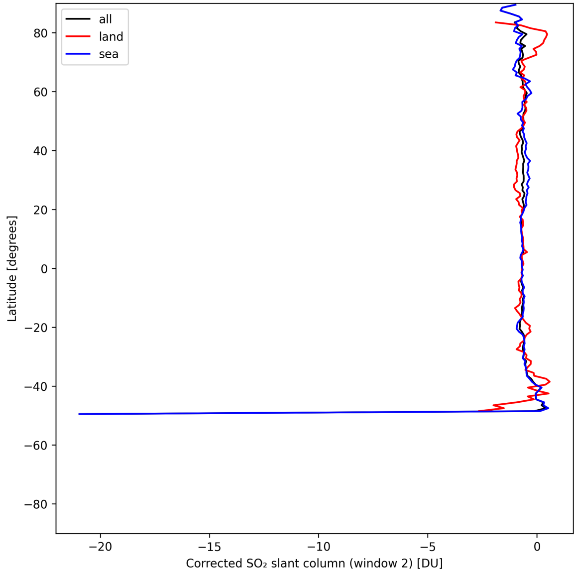
Figure 42: Zonal average of “Corrected SO 2 slant column (window 2)” for 2025-07-22 to 2025-07-22.
