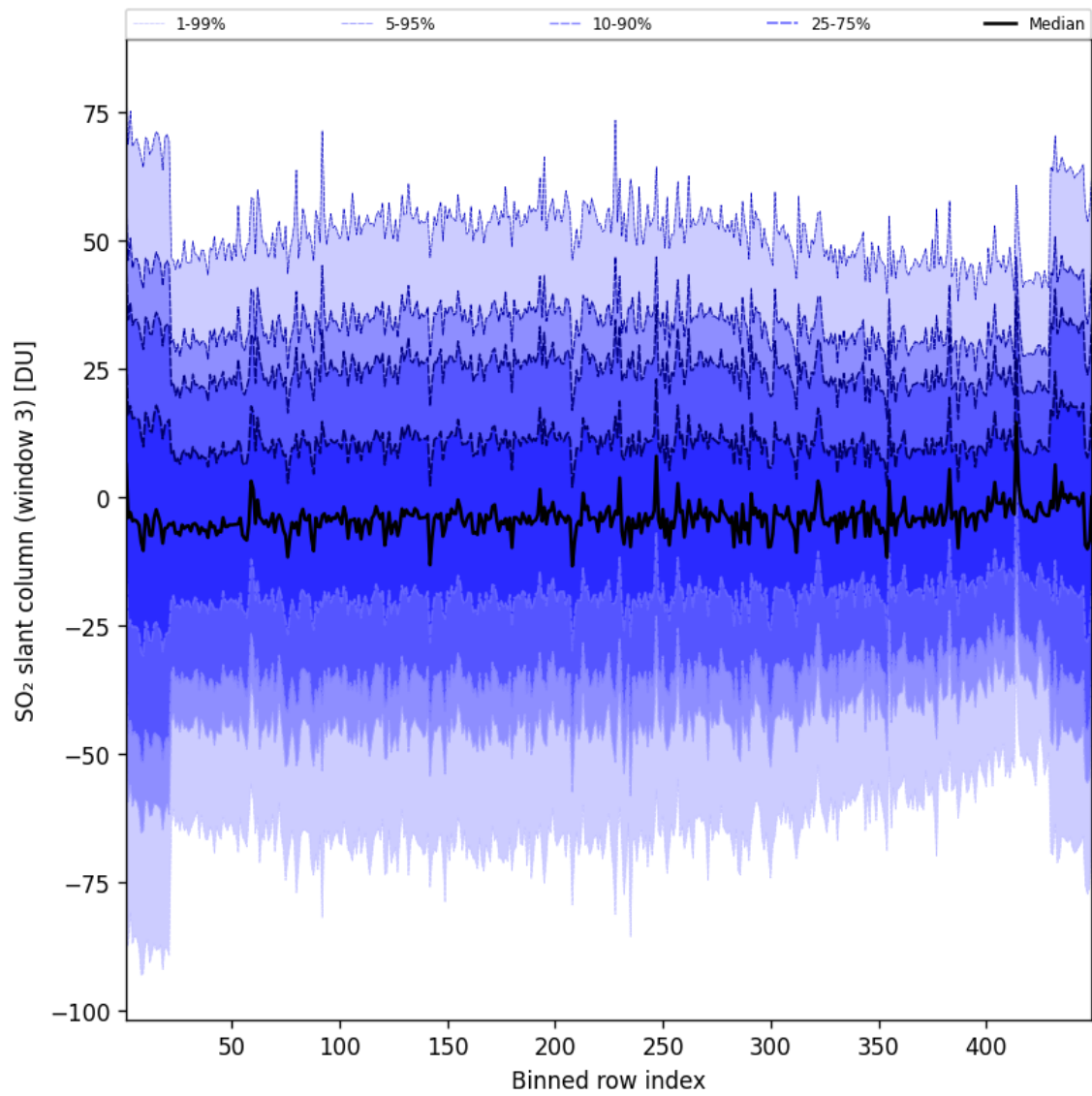
Figure 98: Along track statistics of “SO 2 slant column (window 3)” for 2025-07-22 to 2025-07-22
