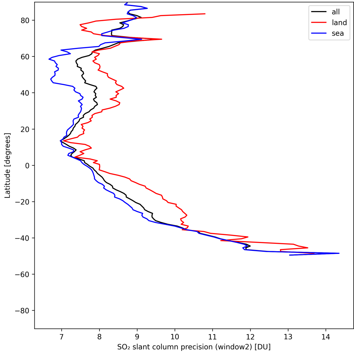
Figure 41: Zonal average of “SO 2 slant column precision (window2)” for 2025-07-22 to 2025-07-22.
