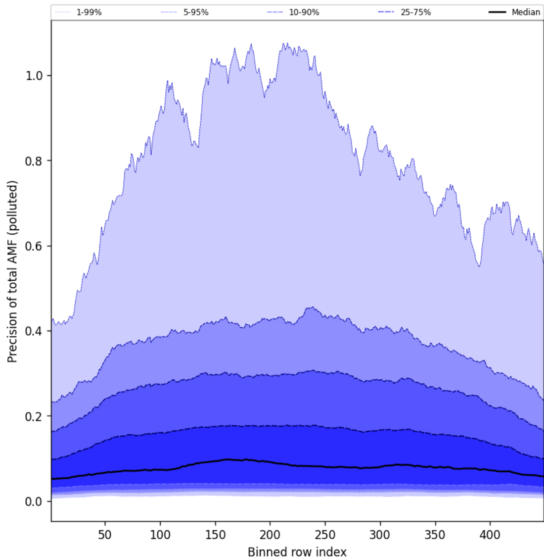
Figure 108: Along track statistics of “Precision of total AMF (polluted)” for 2025-07-22 to 2025-07-22
