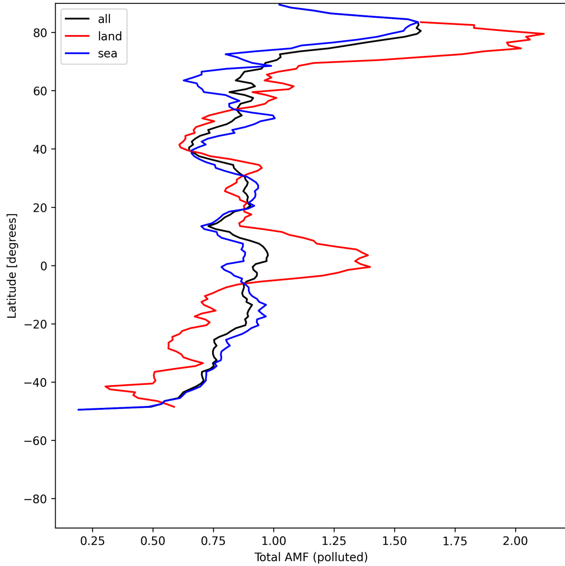
Figure 53: Zonal average of “Total AMF (polluted)” for 2025-07-22 to 2025-07-22.
