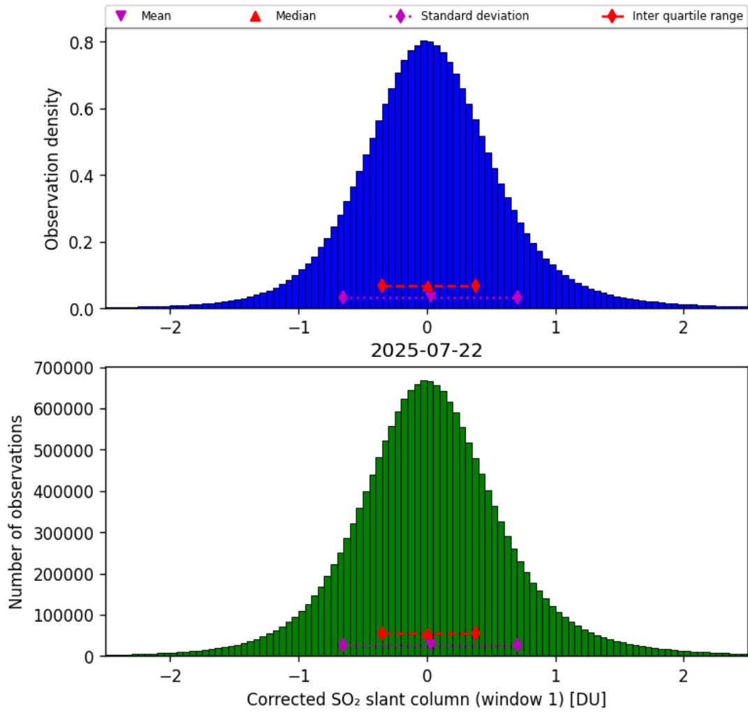
Figure 65: Histogram of “Corrected SO 2 slant column (window 1)” for 2025-07-22 to 2025-07-22
