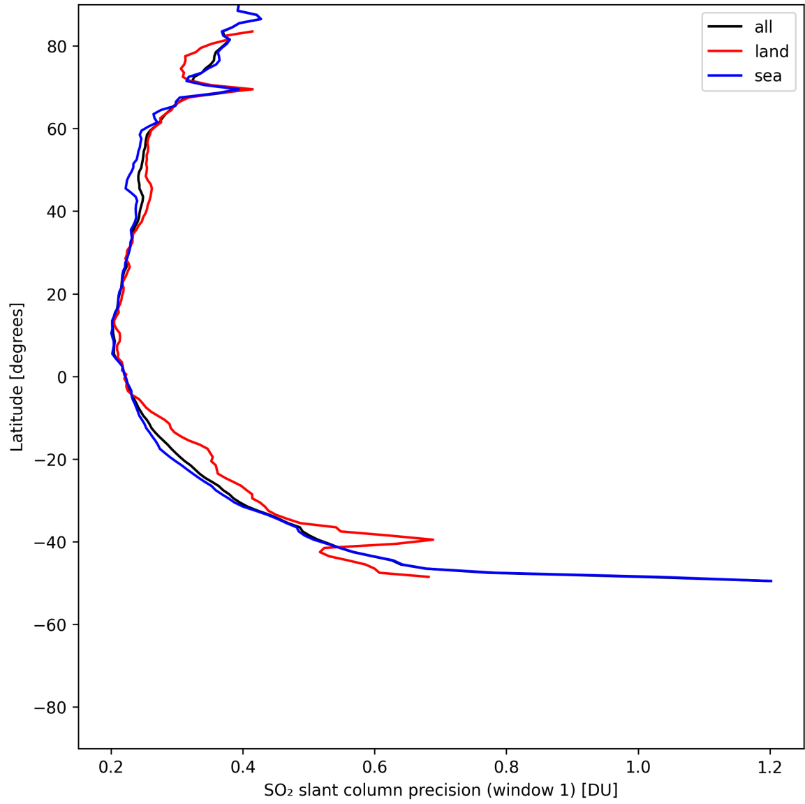
Figure 37: Zonal average of “SO 2 slant column precision (window 1)” for 2025-07-22 to 2025-07-22.
