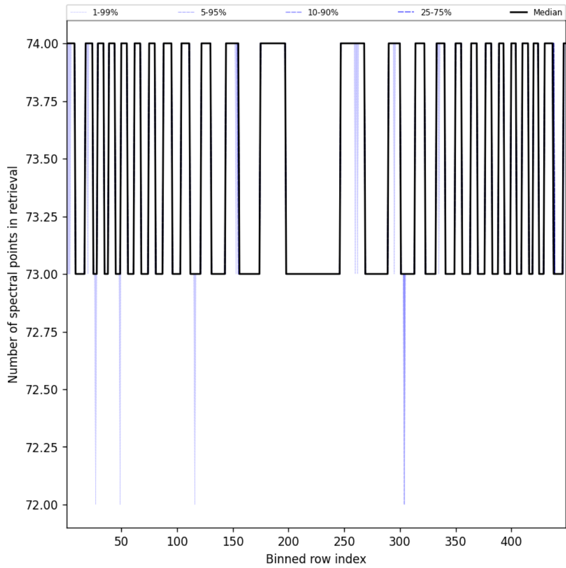
Figure 110: Along track statistics of “Number of spectral points in retrieval” for 2025-07-22 to 2025-07-22
