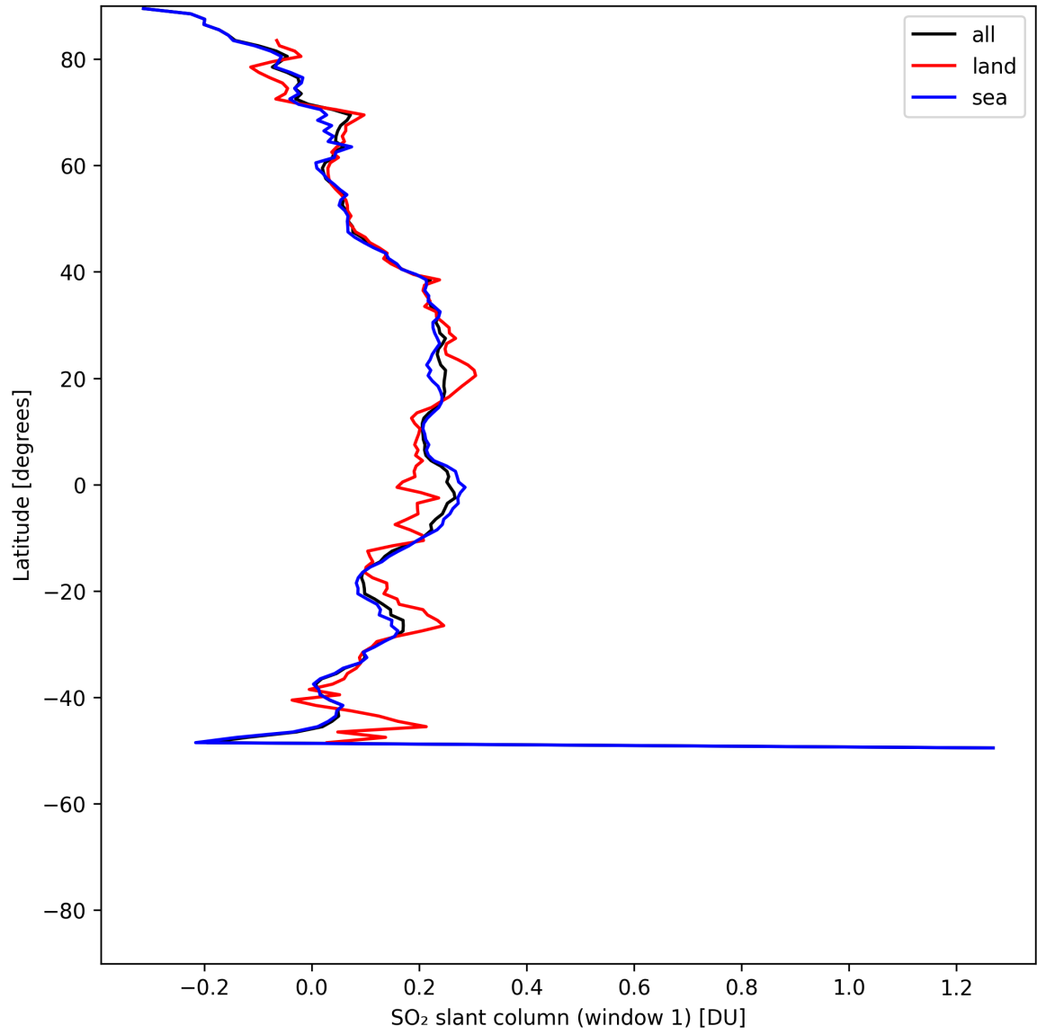
Figure 36: Zonal average of “SO 2 slant column (window 1)” for 2025-07-22 to 2025-07-22.
