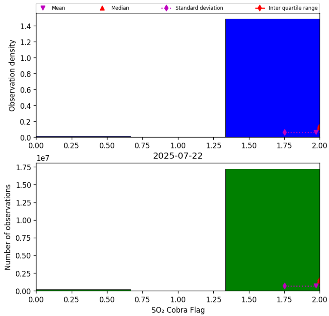
Figure 75: Histogram of “SO 2 Cobra Flag” for 2025-07-22 to 2025-07-22
