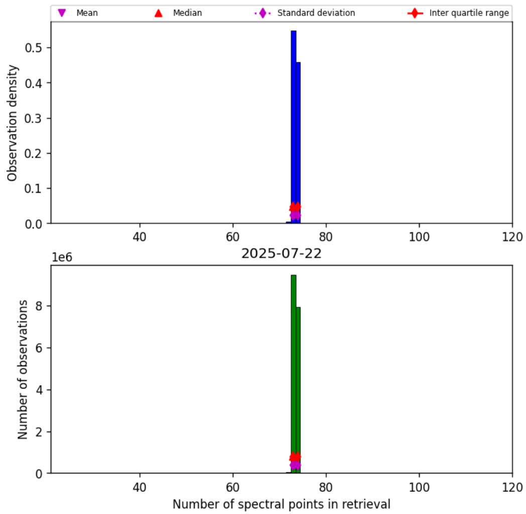
Figure 83: Histogram of “Number of spectral points in retrieval” for 2025-07-22 to 2025-07-22
