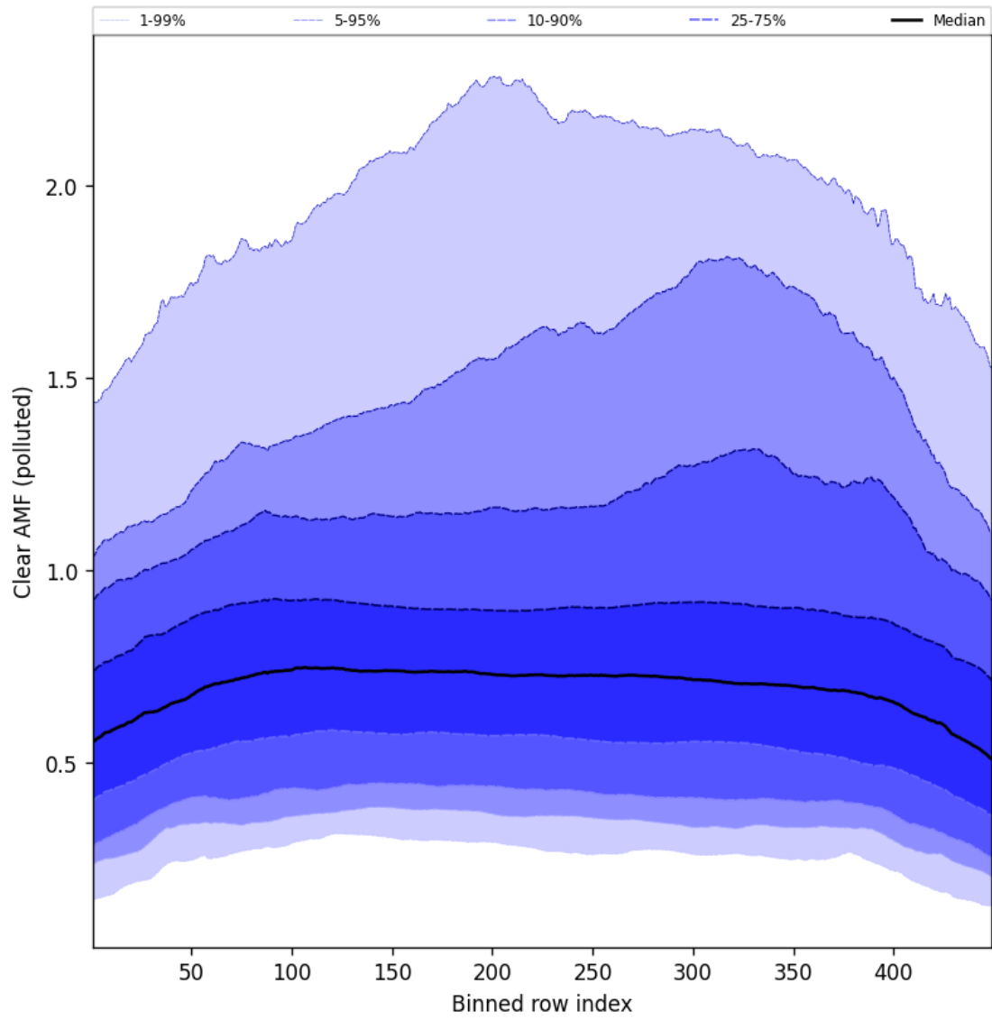
Figure 109: Along track statistics of “Clear AMF (polluted)” for 2025-07-22 to 2025-07-22
