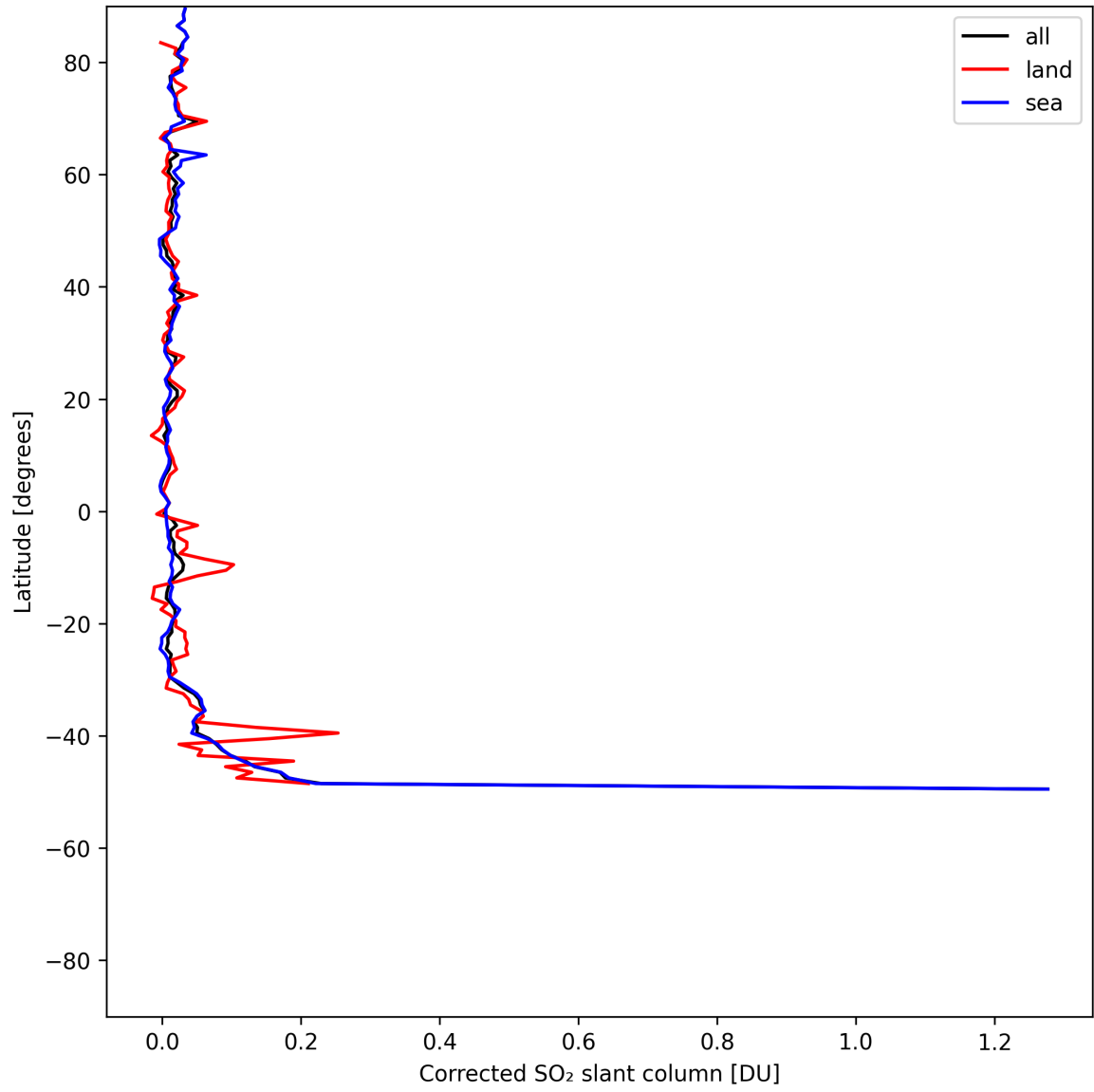
Figure 33: Zonal average of “Corrected SO 2 slant column” for 2025-07-22 to 2025-07-22.
