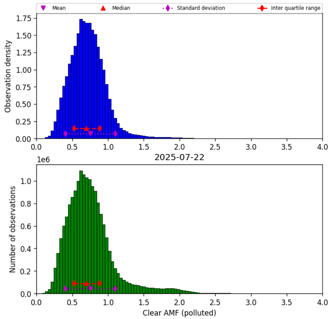
Figure 82: Histogram of “Clear AMF (polluted)” for 2025-07-22 to 2025-07-22
