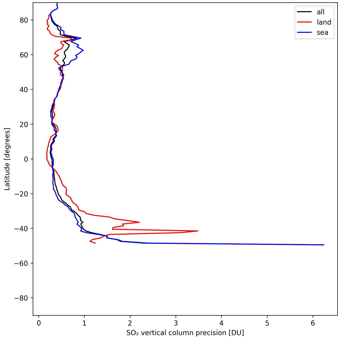
Figure 32: Zonal average of “SO 2 vertical column precision” for 2025-07-22 to 2025-07-22.
