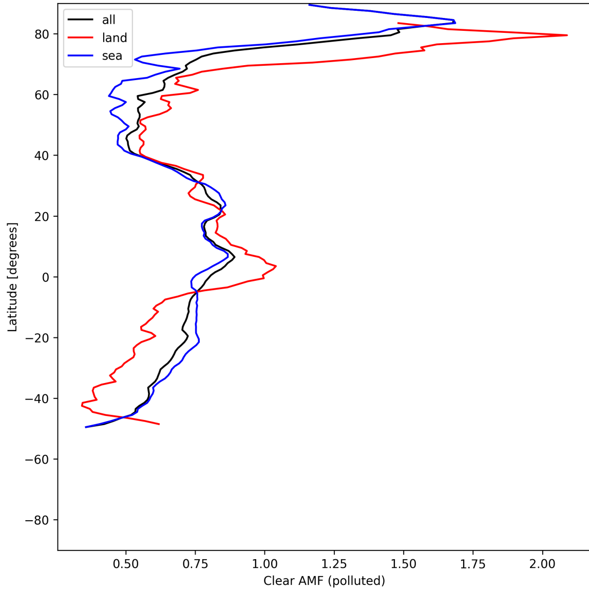
Figure 55: Zonal average of “Clear AMF (polluted)” for 2025-07-22 to 2025-07-22.
