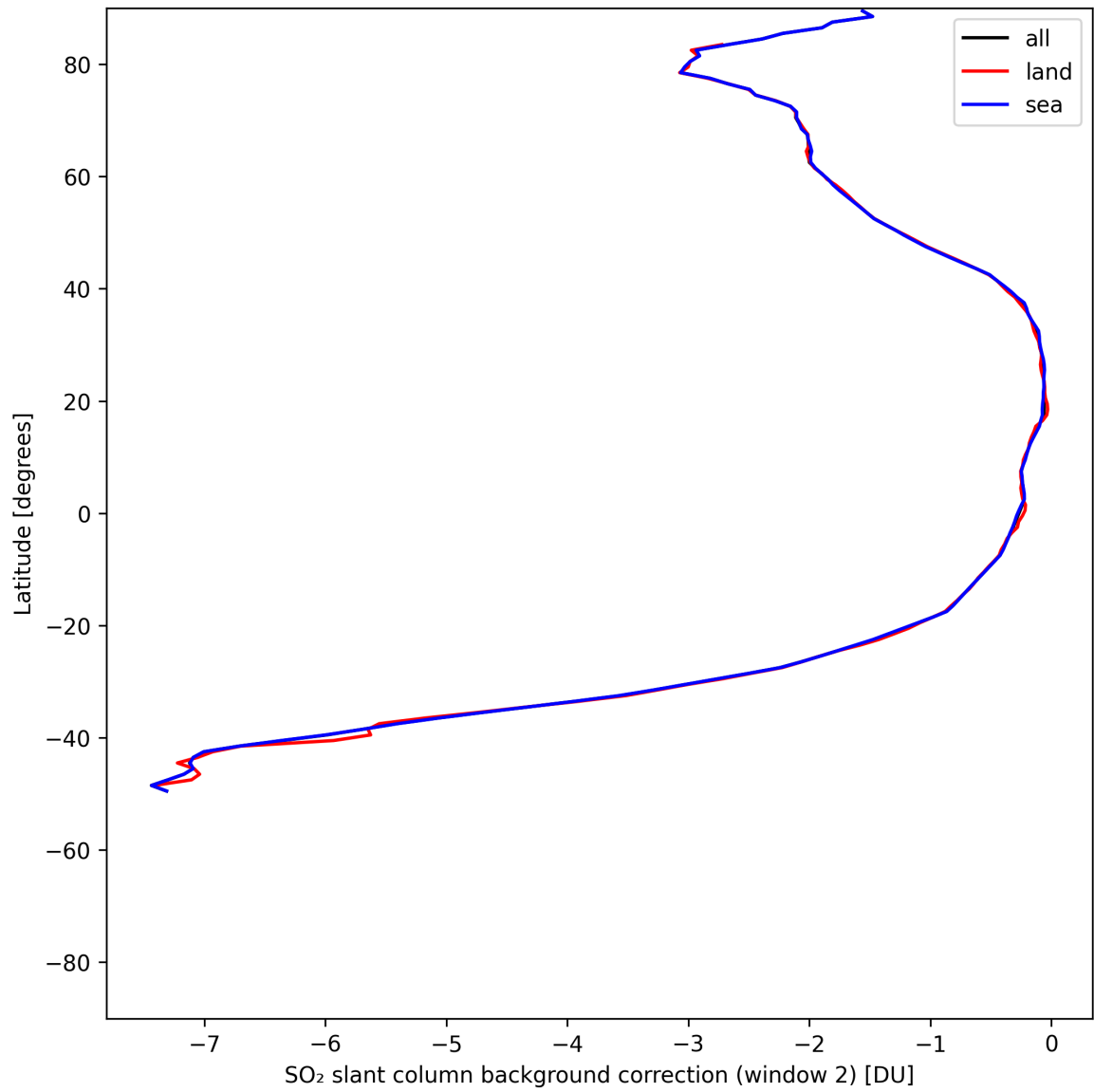
Figure 43: Zonal average of “SO 2 slant column background correction (window 2)” for 2025-07-22 to 2025-07-22.
