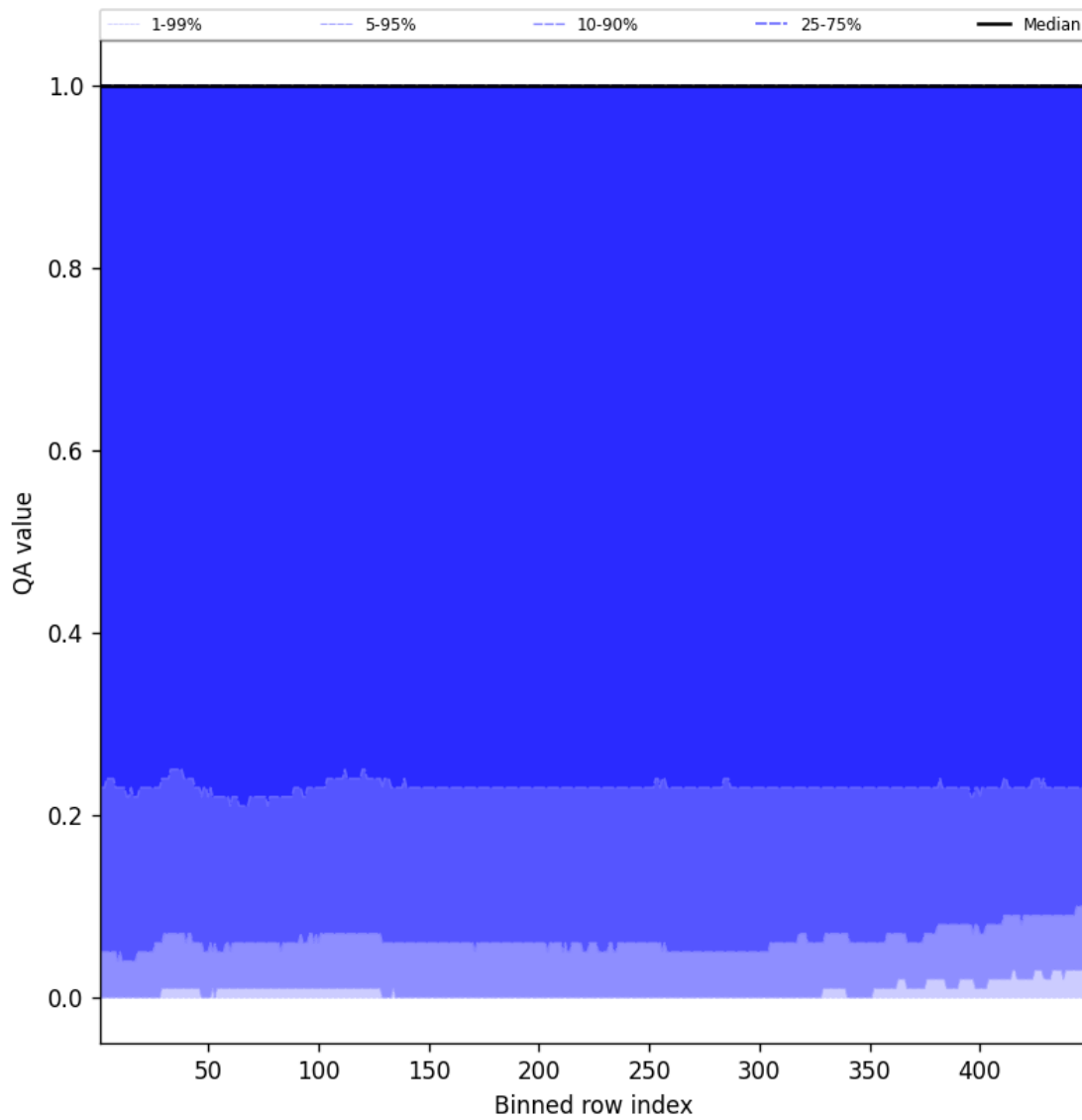
Figure 84: Along track statistics of “QA value” for 2025-07-22 to 2025-07-22
