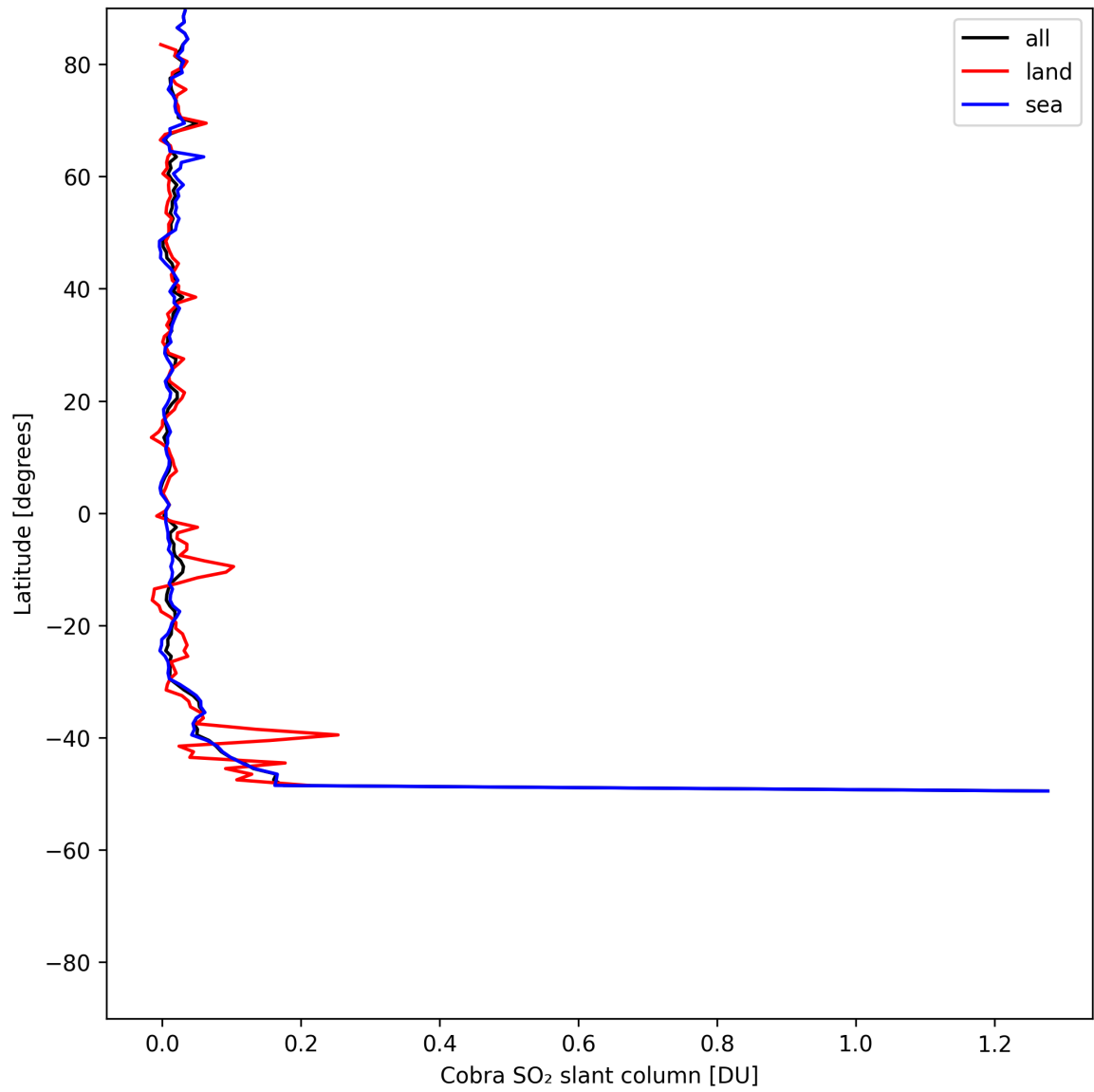
Figure 34: Zonal average of “Cobra SO 2 slant column” for 2025-07-22 to 2025-07-22.
