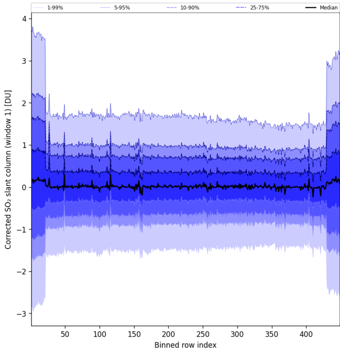
Figure 92: Along track statistics of “Corrected SO 2 slant column (window 1)” for 2025-07-22 to 2025-07-22
