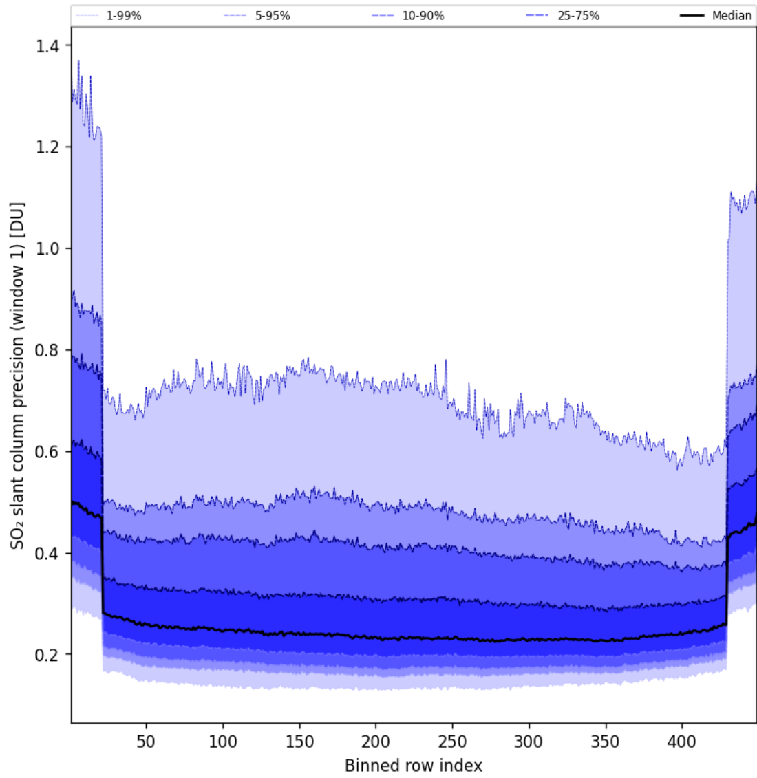
Figure 91: Along track statistics of “SO 2 slant column precision (window 1)” for 2025-07-22 to 2025-07-22
