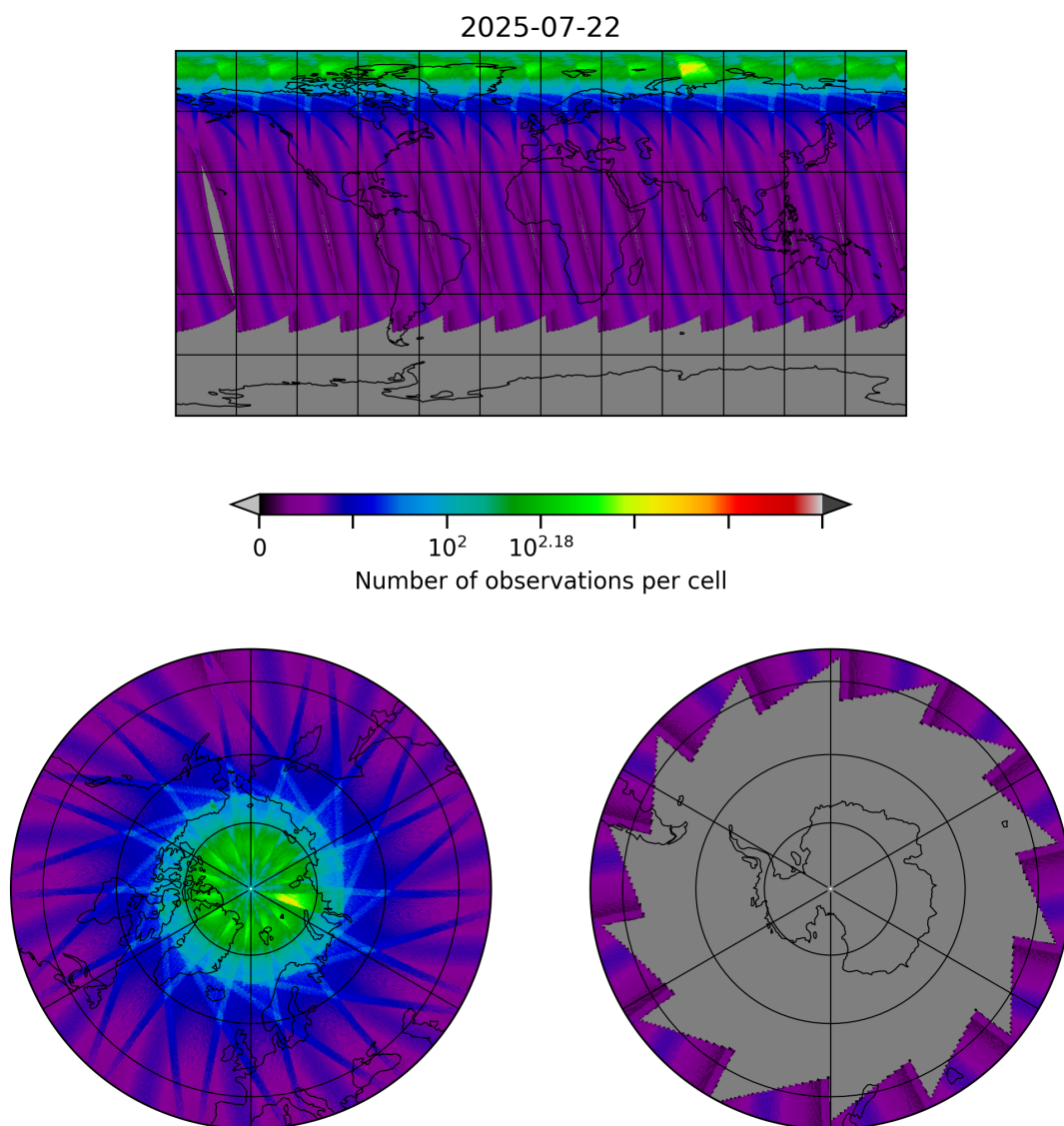
Figure 29: Map of the number of observations for 2025-07-22 to 2025-07-22
