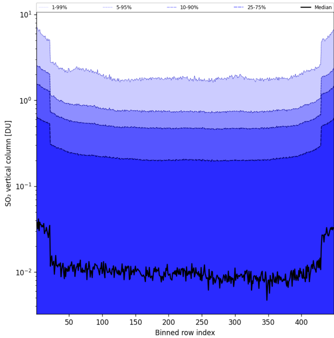
Figure 85: Along track statistics of “SO 2 vertical column” for 2025-07-22 to 2025-07-22
