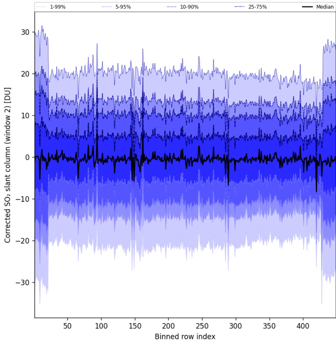
Figure 96: Along track statistics of “Corrected SO 2 slant column (window 2)” for 2025-07-22 to 2025-07-22
