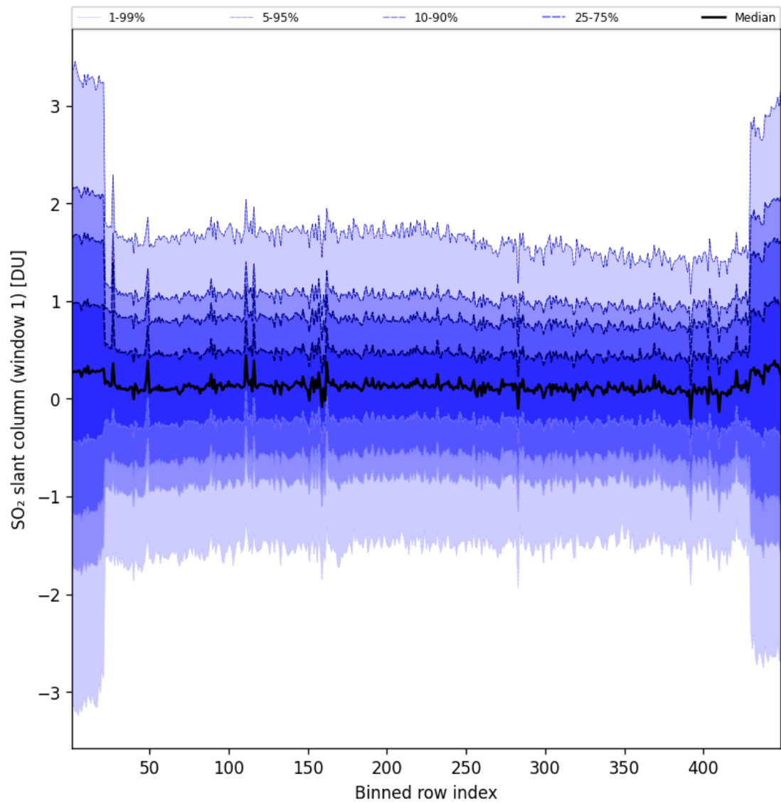
Figure 90: Along track statistics of “SO 2 slant column (window 1)” for 2025-07-22 to 2025-07-22
