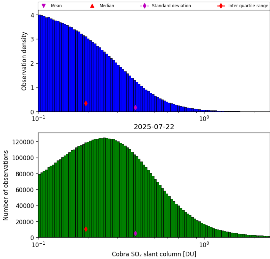
Figure 61: Histogram of “Cobra SO 2 slant column” for 2025-07-22 to 2025-07-22
