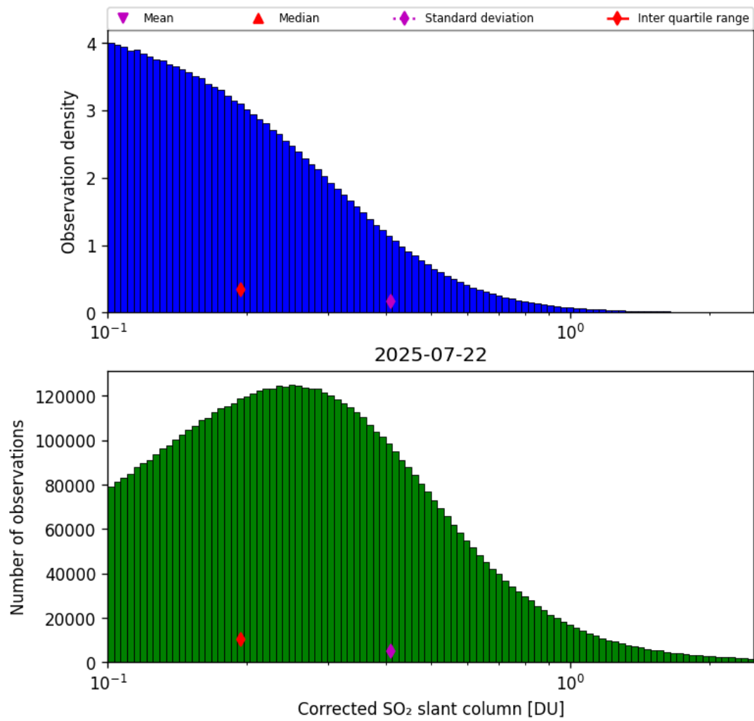
Figure 60: Histogram of “Corrected SO 2 slant column” for 2025-07-22 to 2025-07-22
