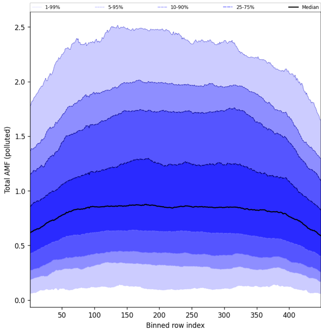
Figure 107: Along track statistics of “Total AMF (polluted)” for 2025-07-22 to 2025-07-22
