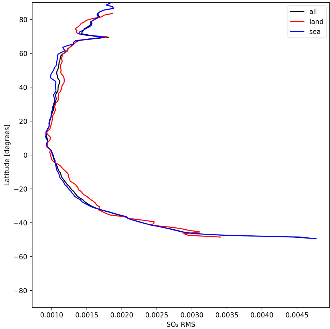
Figure 52: Zonal average of “SO 2 RMS” for 2025-07-22 to 2025-07-22.
