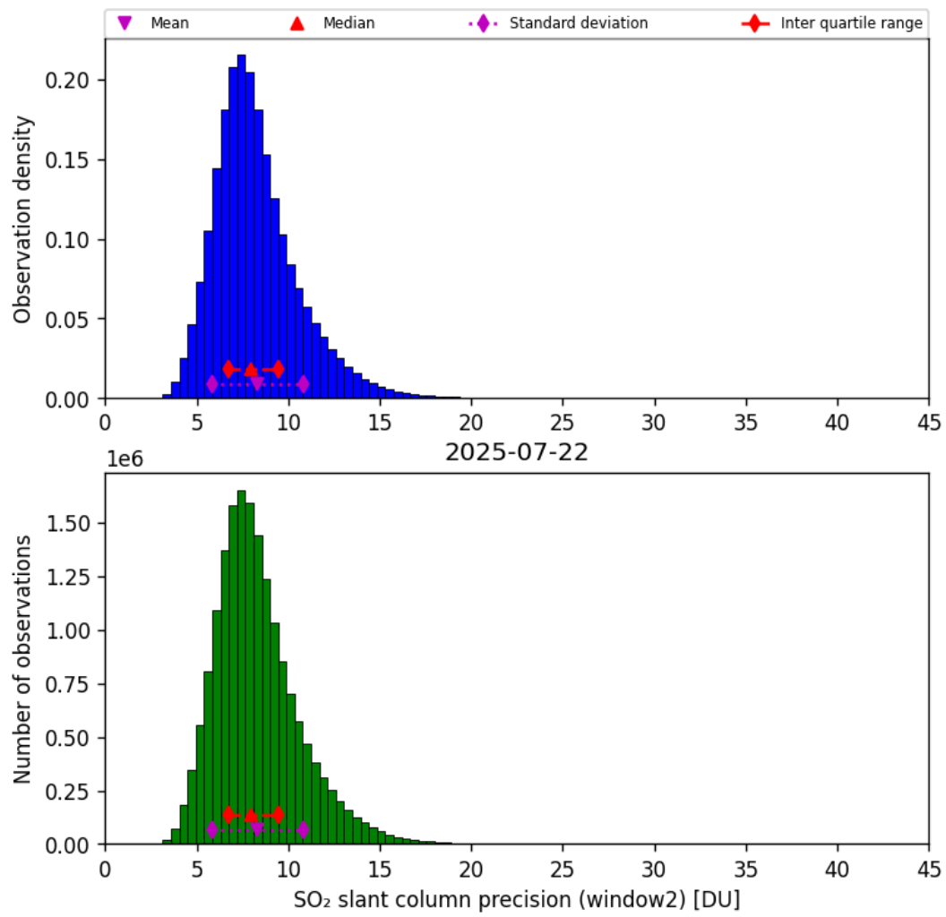
Figure 68: Histogram of “SO 2 slant column precision (window2)” for 2025-07-22 to 2025-07-22
