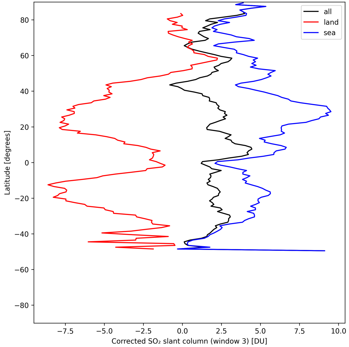
Figure 46: Zonal average of “Corrected SO 2 slant column (window 3)” for 2025-07-22 to 2025-07-22.
