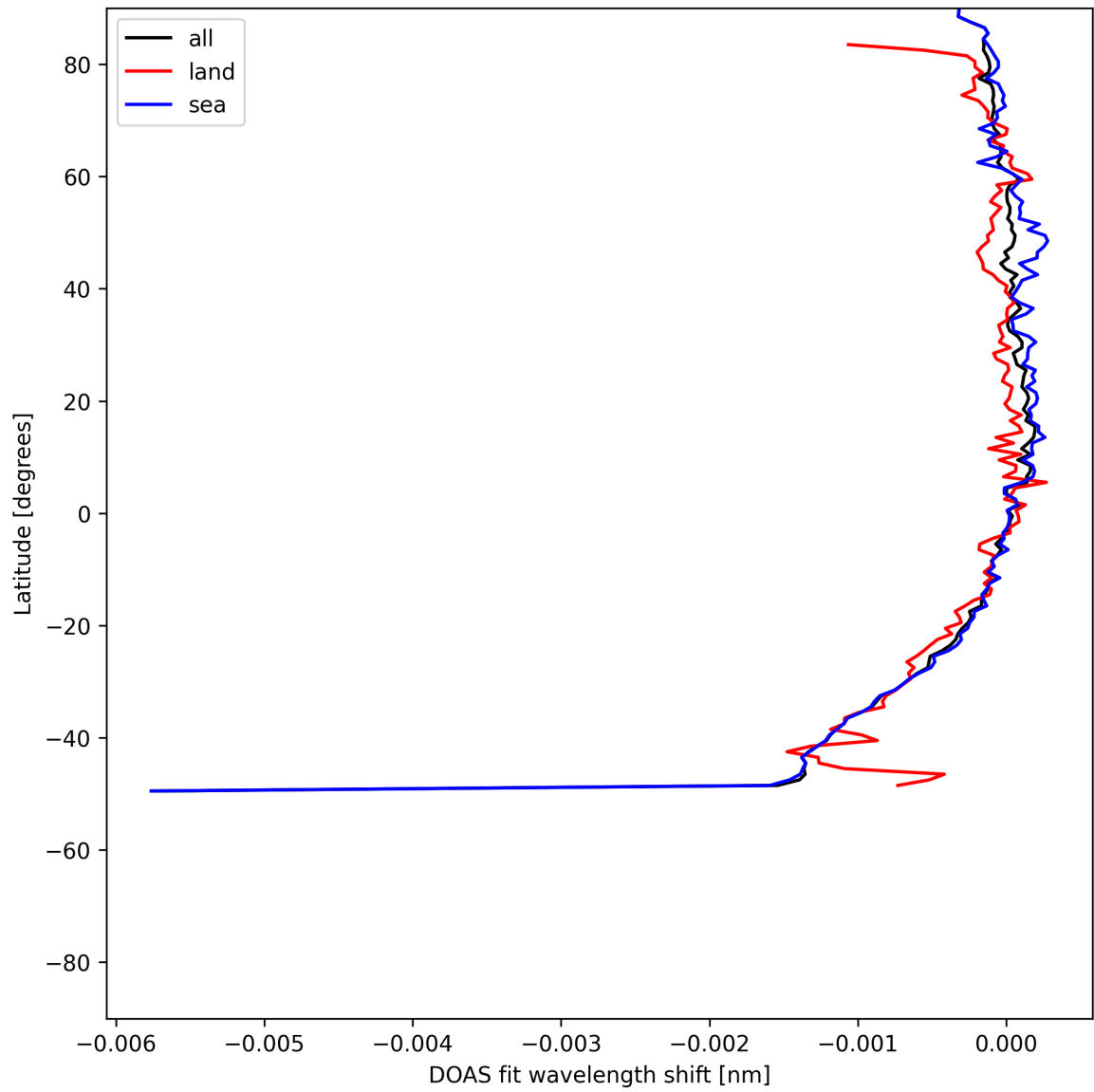
Figure 50: Zonal average of “DOAS fit wavelength shift” for 2025-07-22 to 2025-07-22.
