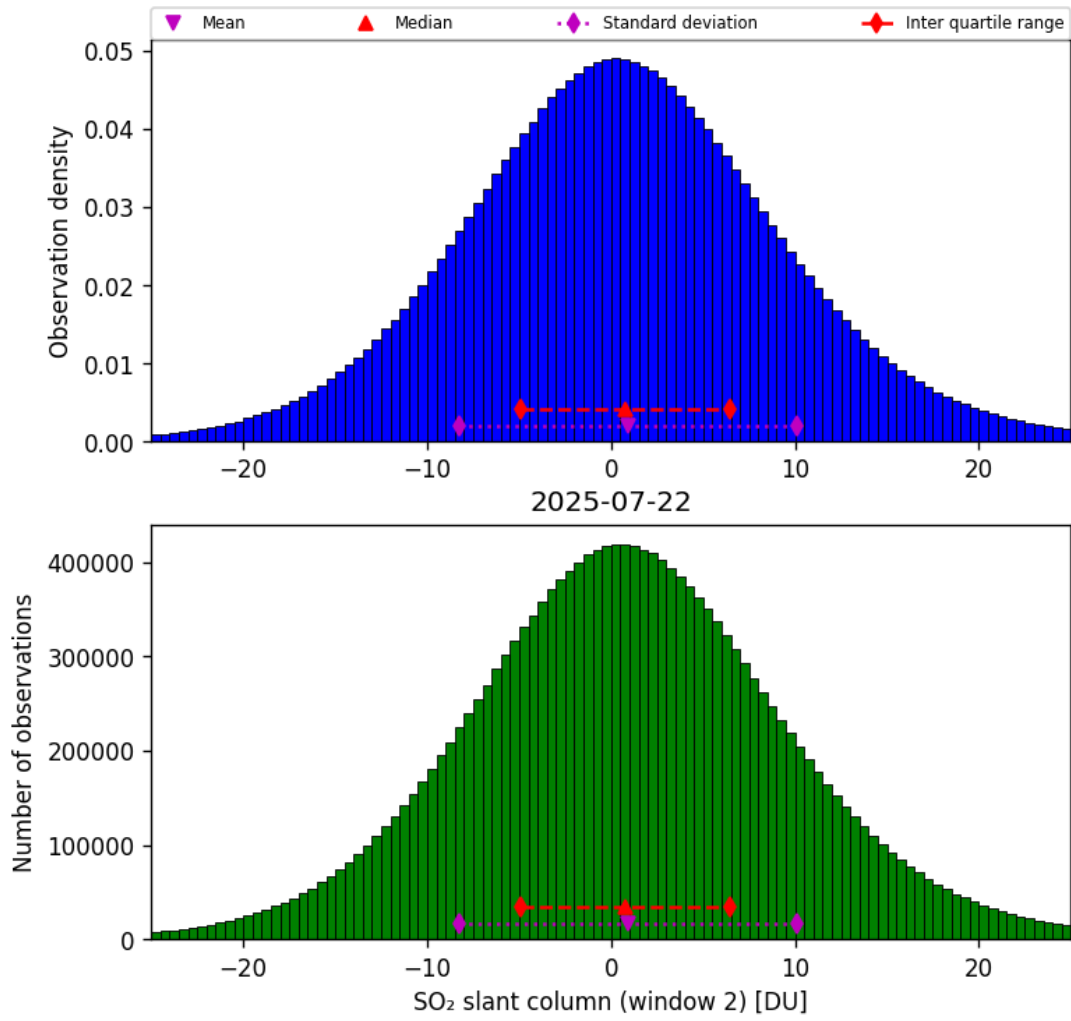
Figure 67: Histogram of “SO 2 slant column (window 2)” for 2025-07-22 to 2025-07-22
