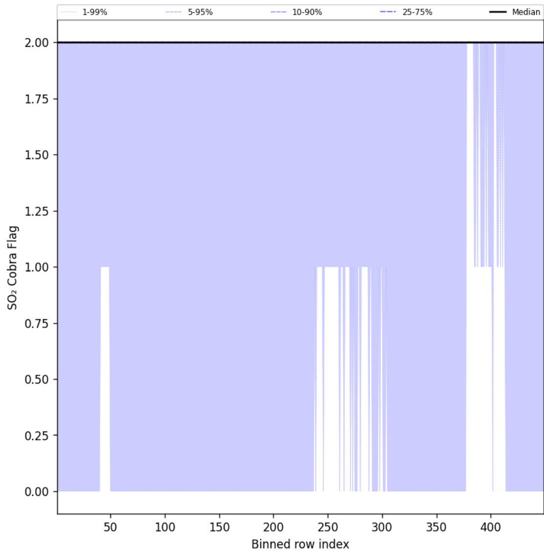
Figure 102: Along track statistics of “SO 2 Cobra Flag” for 2025-07-22 to 2025-07-22
