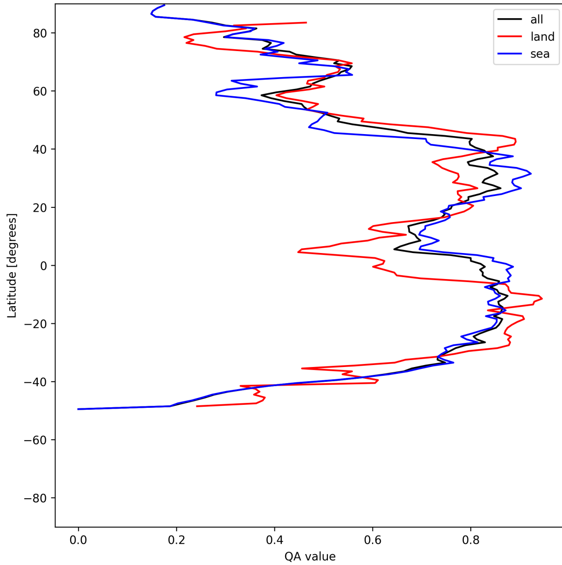
Figure 30: Zonal average of “QA value” for 2025-07-22 to 2025-07-22.
