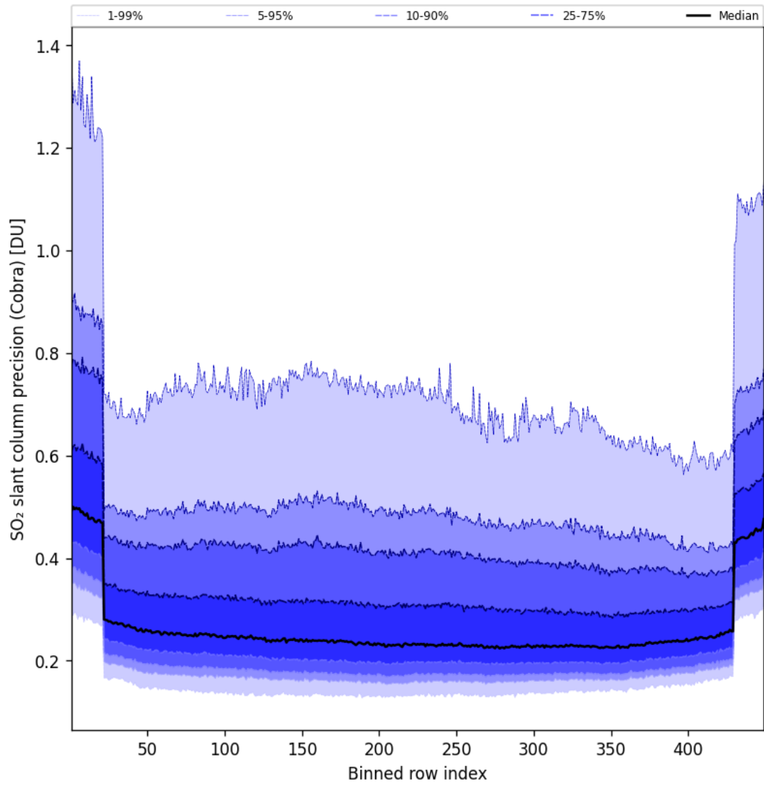
Figure 89: Along track statistics of “SO 2 slant column precision (Cobra)” for 2025-07-22 to 2025-07-22
