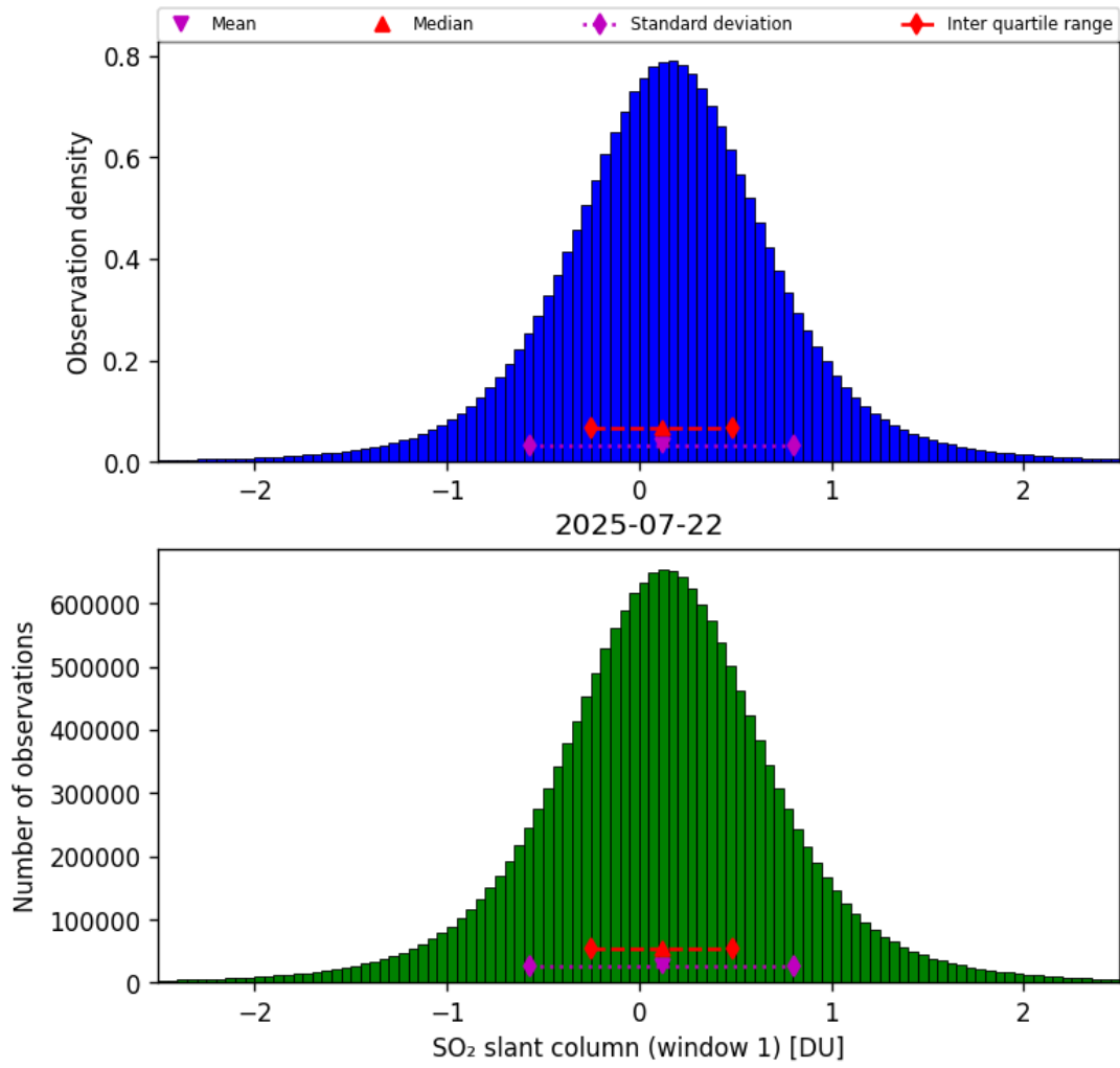
Figure 63: Histogram of “SO 2 slant column (window 1)” for 2025-07-22 to 2025-07-22
