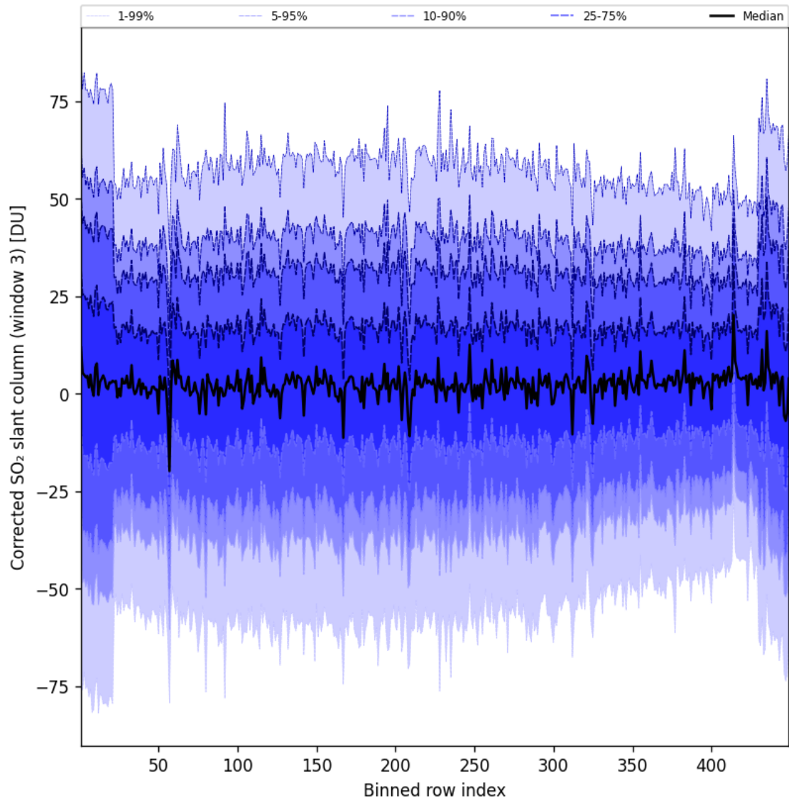
Figure 100: Along track statistics of “Corrected SO 2 slant column (window 3)” for 2025-07-22 to 2025-07-22
