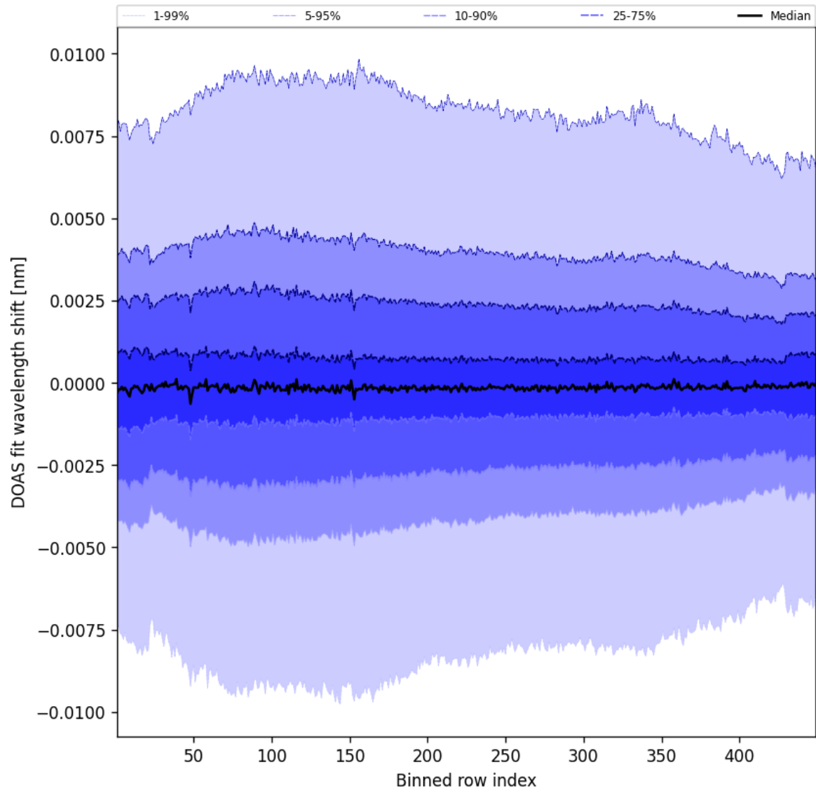
Figure 104: Along track statistics of “DOAS fit wavelength shift” for 2025-07-22 to 2025-07-22
