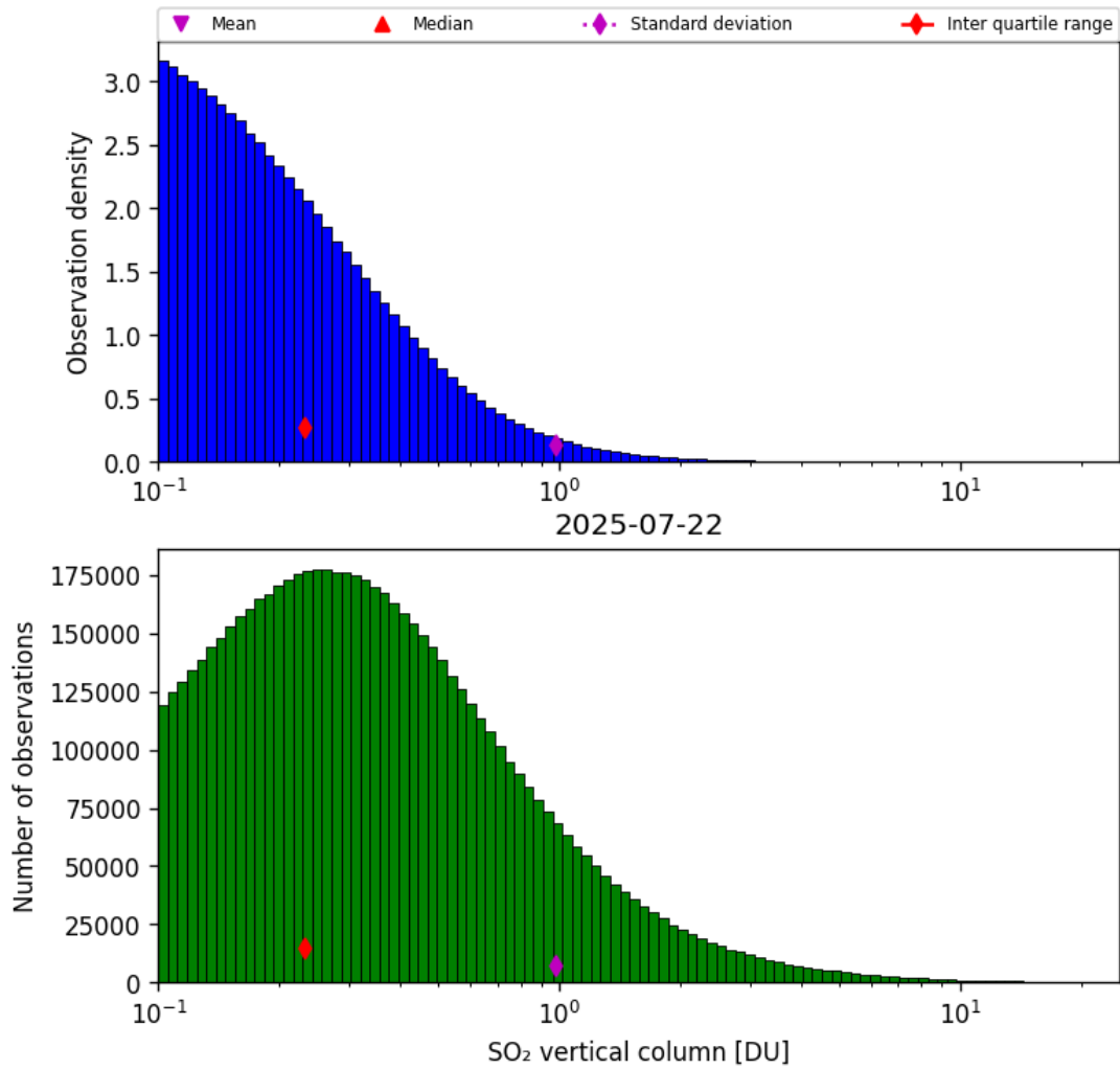
Figure 58: Histogram of “SO 2 vertical column” for 2025-07-22 to 2025-07-22
