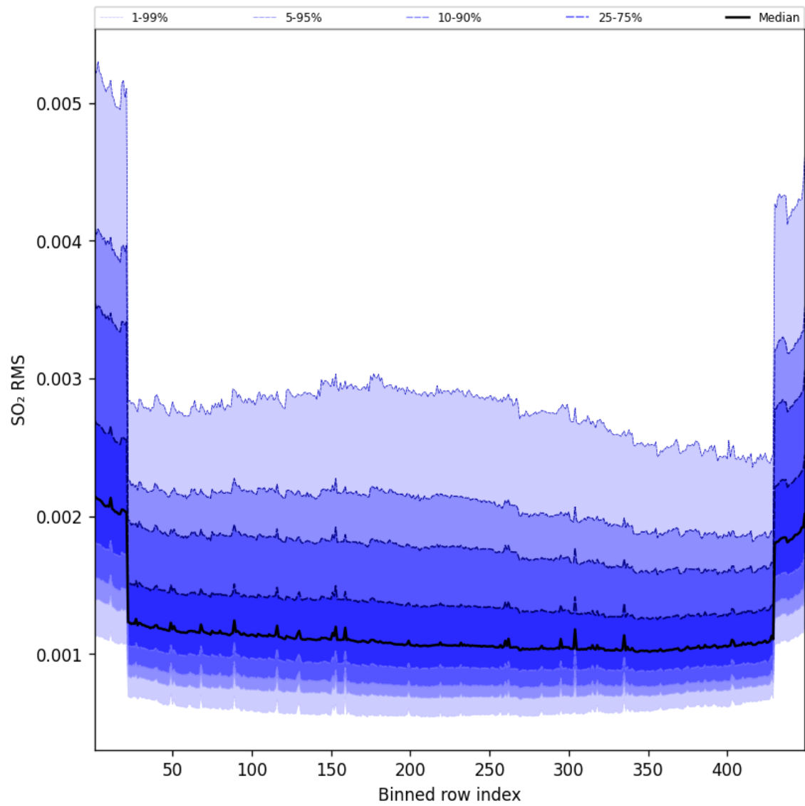
Figure 106: Along track statistics of “SO 2 RMS” for 2025-07-22 to 2025-07-22
