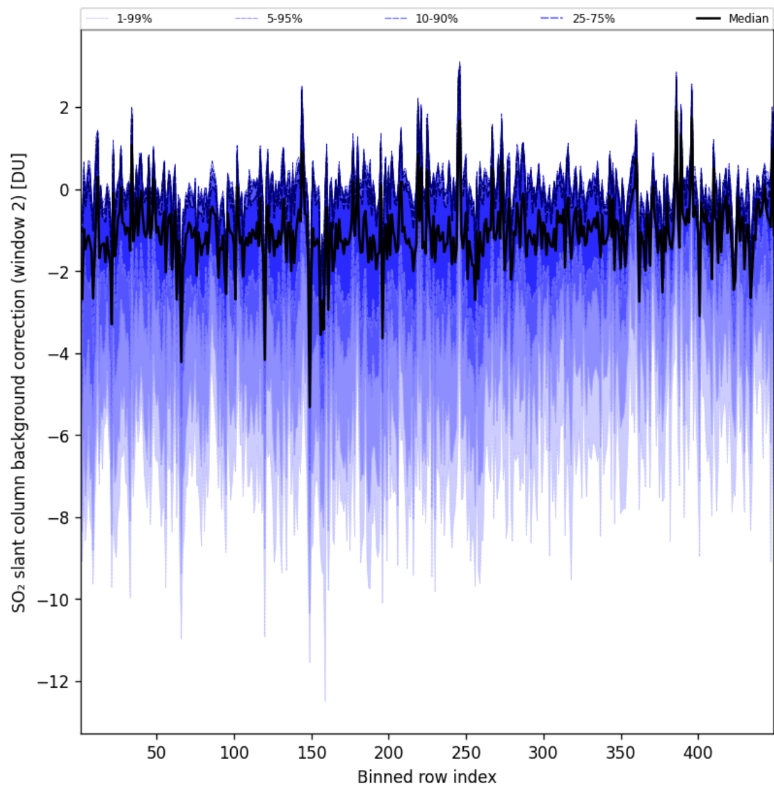
Figure 97: Along track statistics of “SO 2 slant column background correction (window 2)” for 2025-07-22 to 2025-07-22
