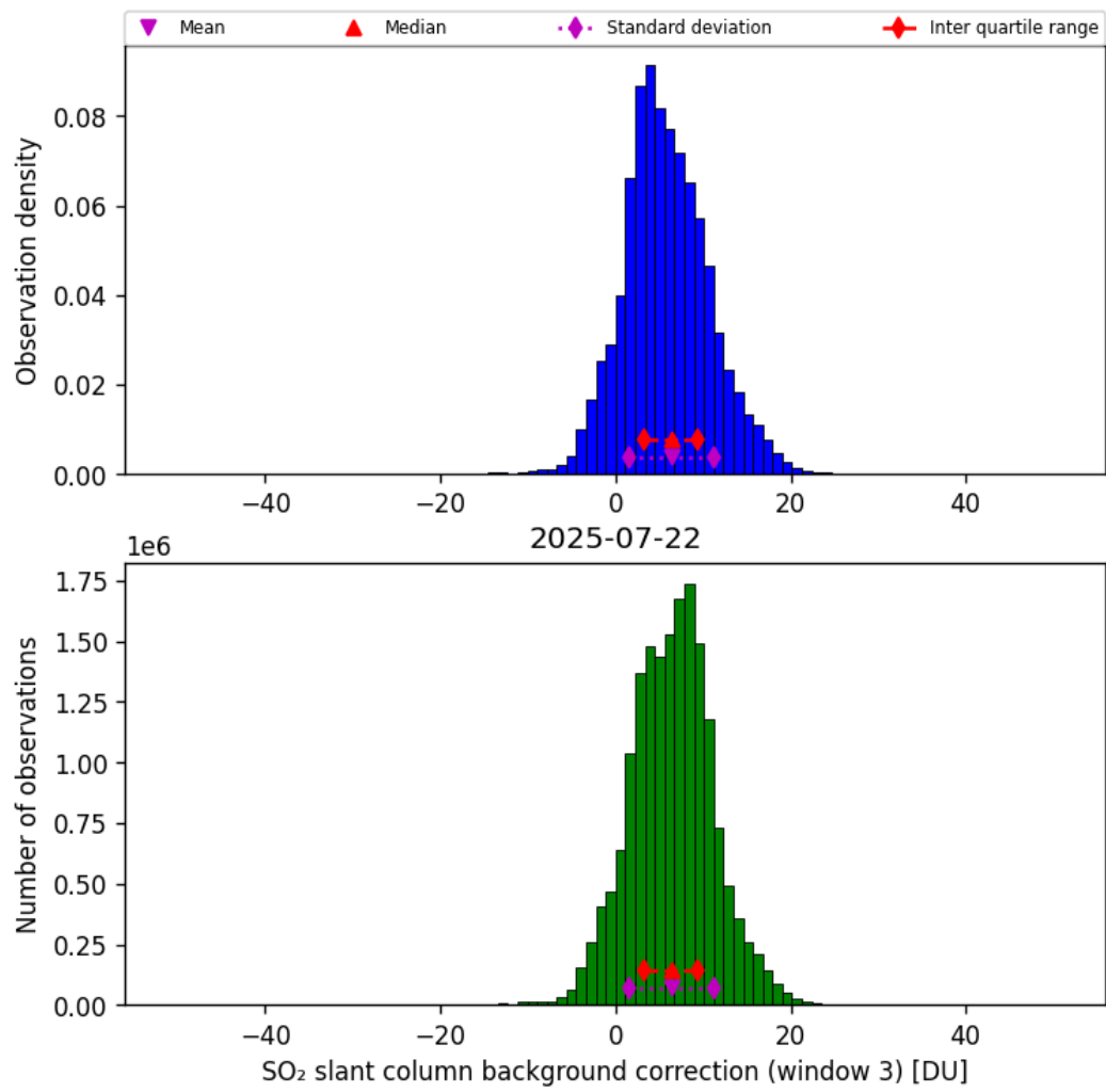
Figure 74: Histogram of “SO 2 slant column background correction (window 3)” for 2025-07-22 to 2025-07-22
