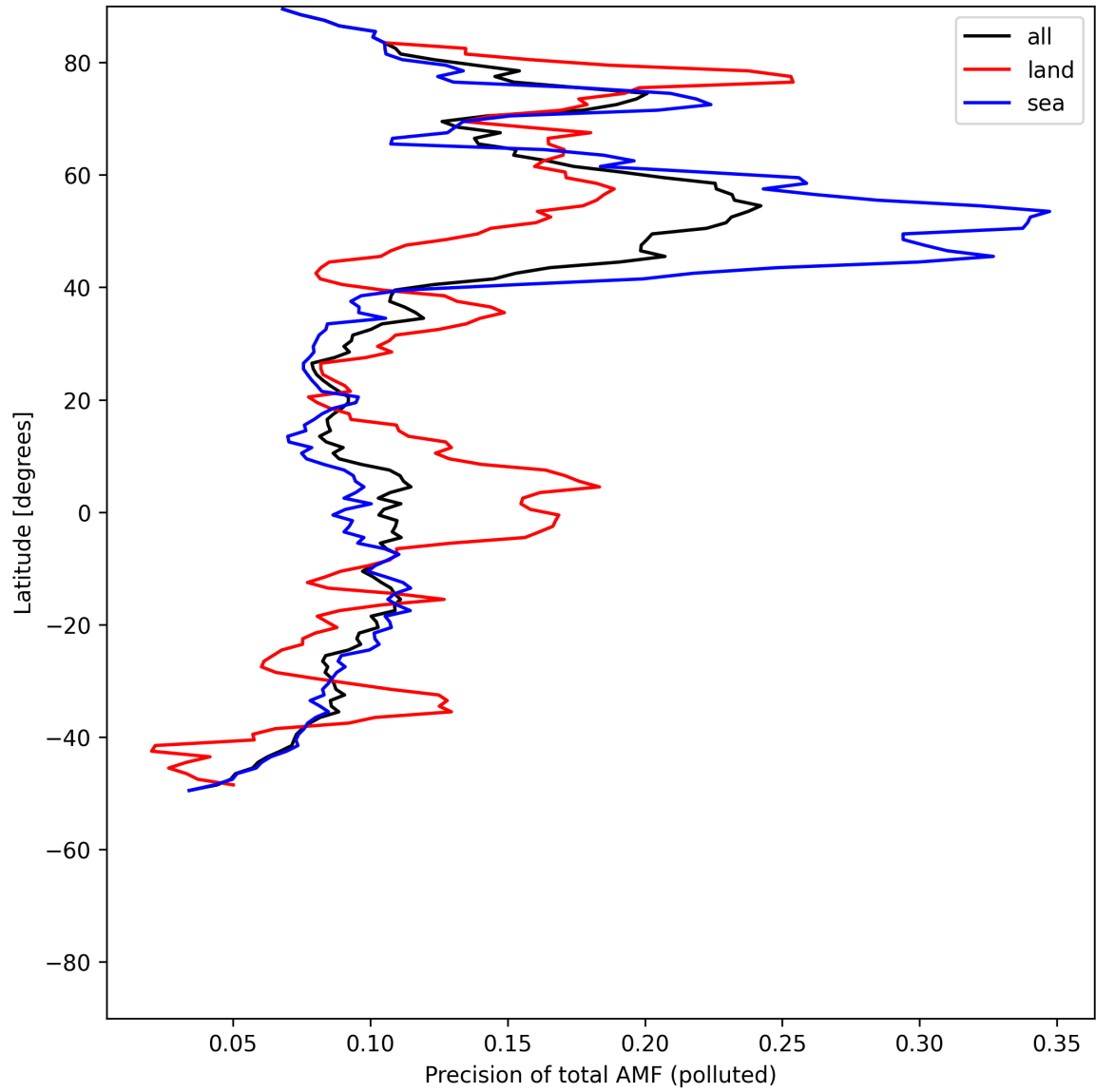
Figure 54: Zonal average of “Precision of total AMF (polluted)” for 2025-07-22 to 2025-07-22.
