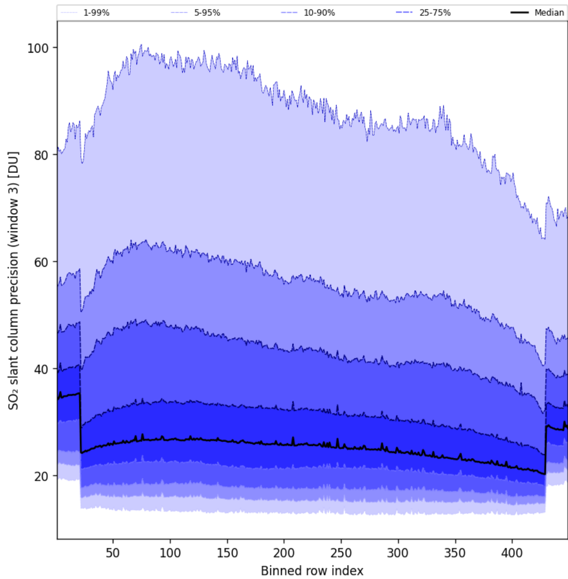
Figure 99: Along track statistics of “SO 2 slant column precision (window 3)” for 2025-07-22 to 2025-07-22
