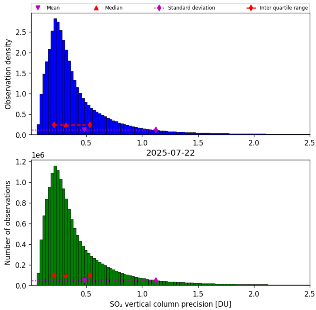
Figure 59: Histogram of “SO 2 vertical column precision” for 2025-07-22 to 2025-07-22
