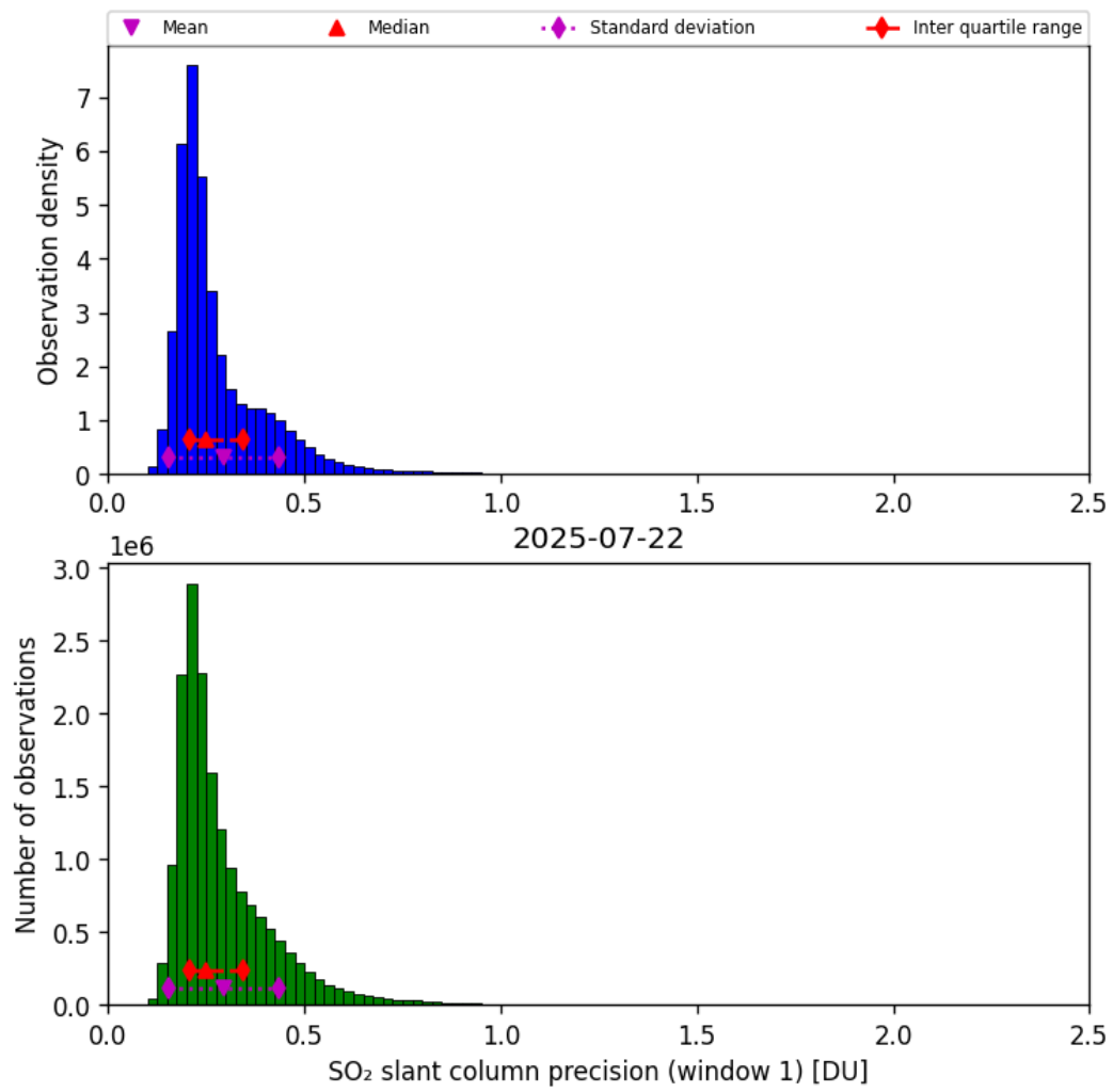
Figure 64: Histogram of “SO 2 slant column precision (window 1)” for 2025-07-22 to 2025-07-22
