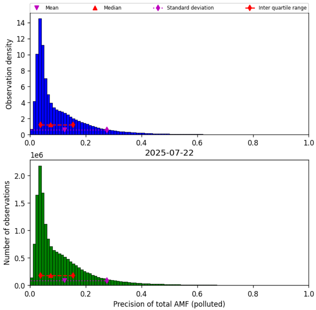
Figure 81: Histogram of “Precision of total AMF (polluted)” for 2025-07-22 to 2025-07-22
