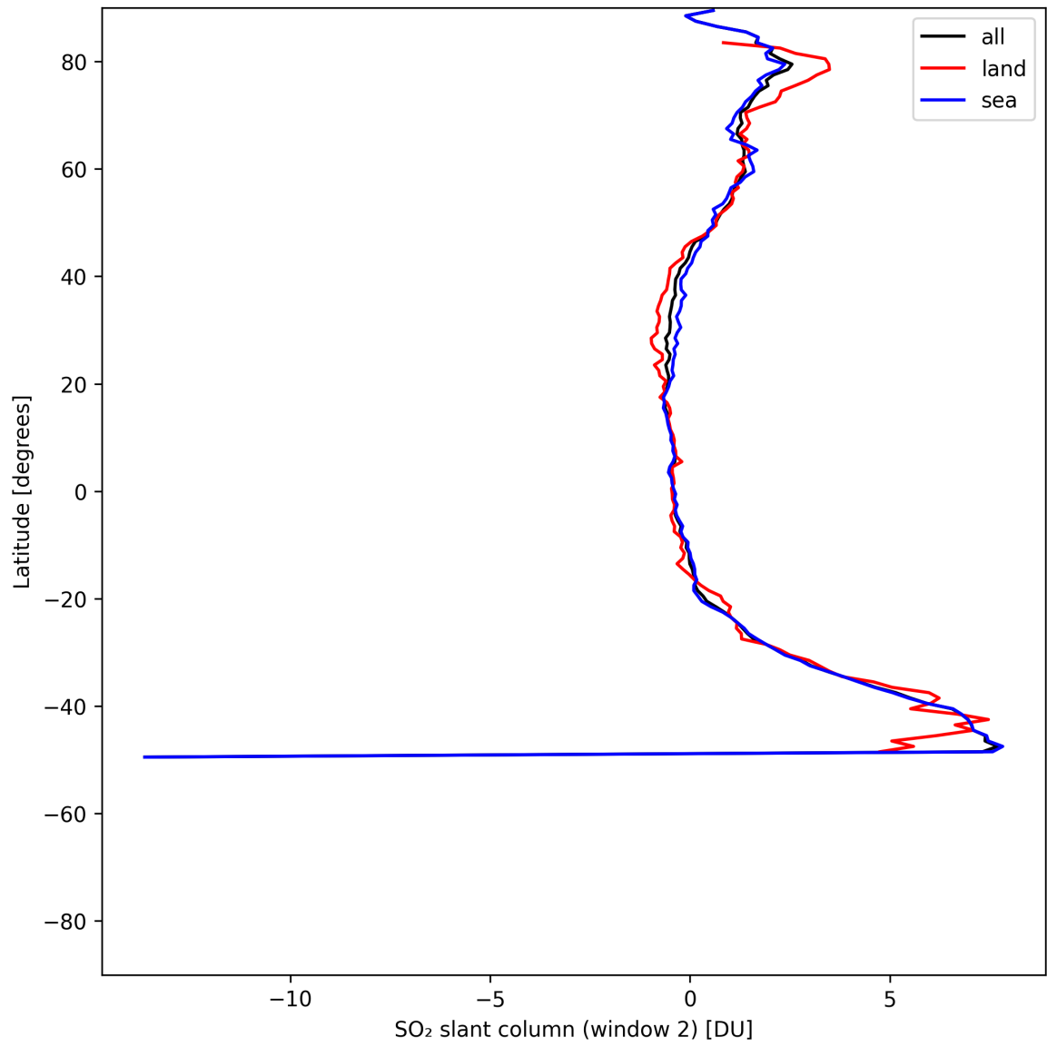
Figure 40: Zonal average of “SO 2 slant column (window 2)” for 2025-07-22 to 2025-07-22.
