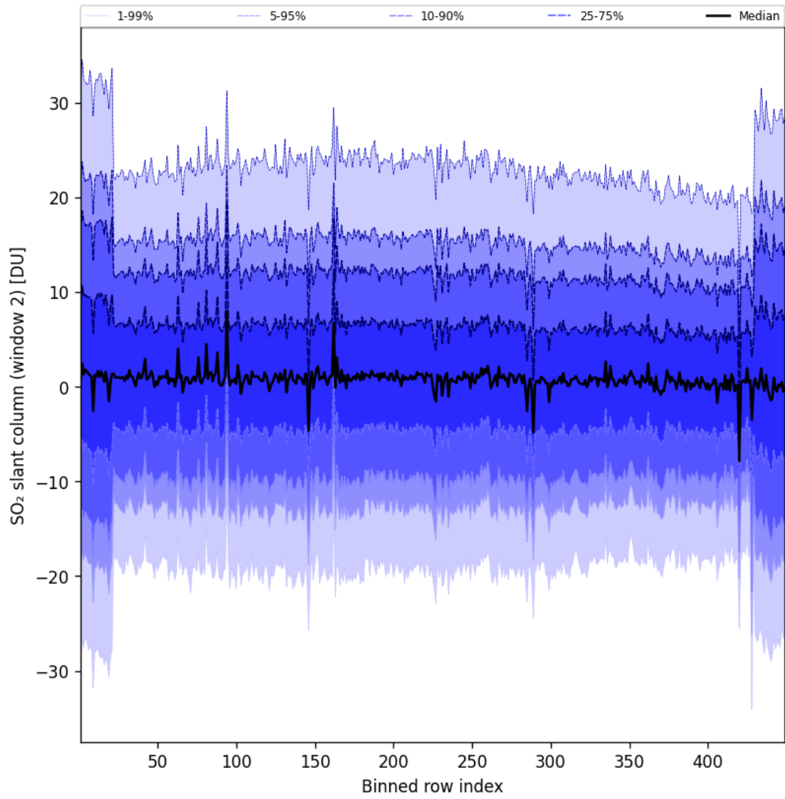
Figure 94: Along track statistics of “SO 2 slant column (window 2)” for 2025-07-22 to 2025-07-22
