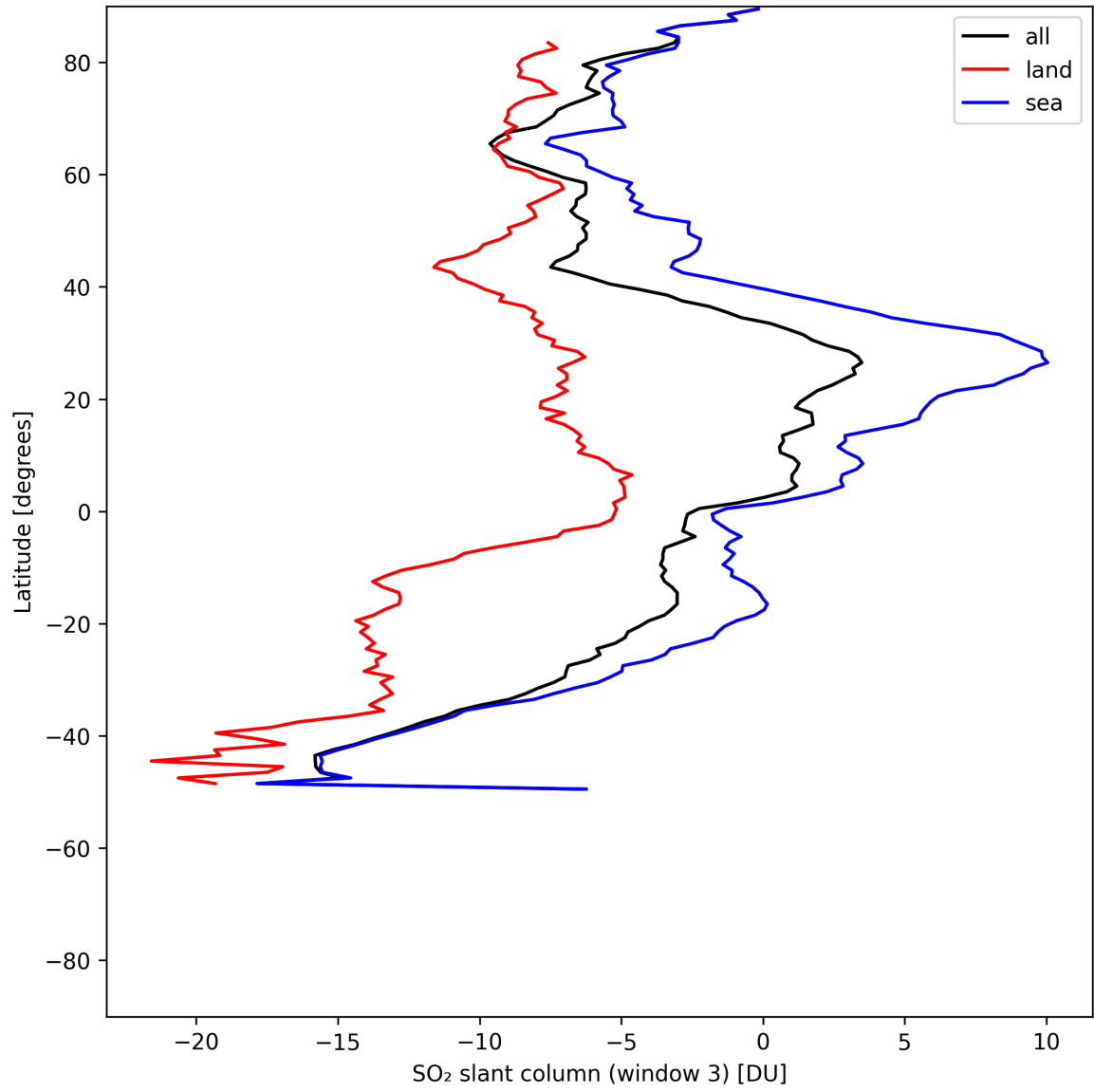
Figure 44: Zonal average of “SO 2 slant column (window 3)” for 2025-07-22 to 2025-07-22.
