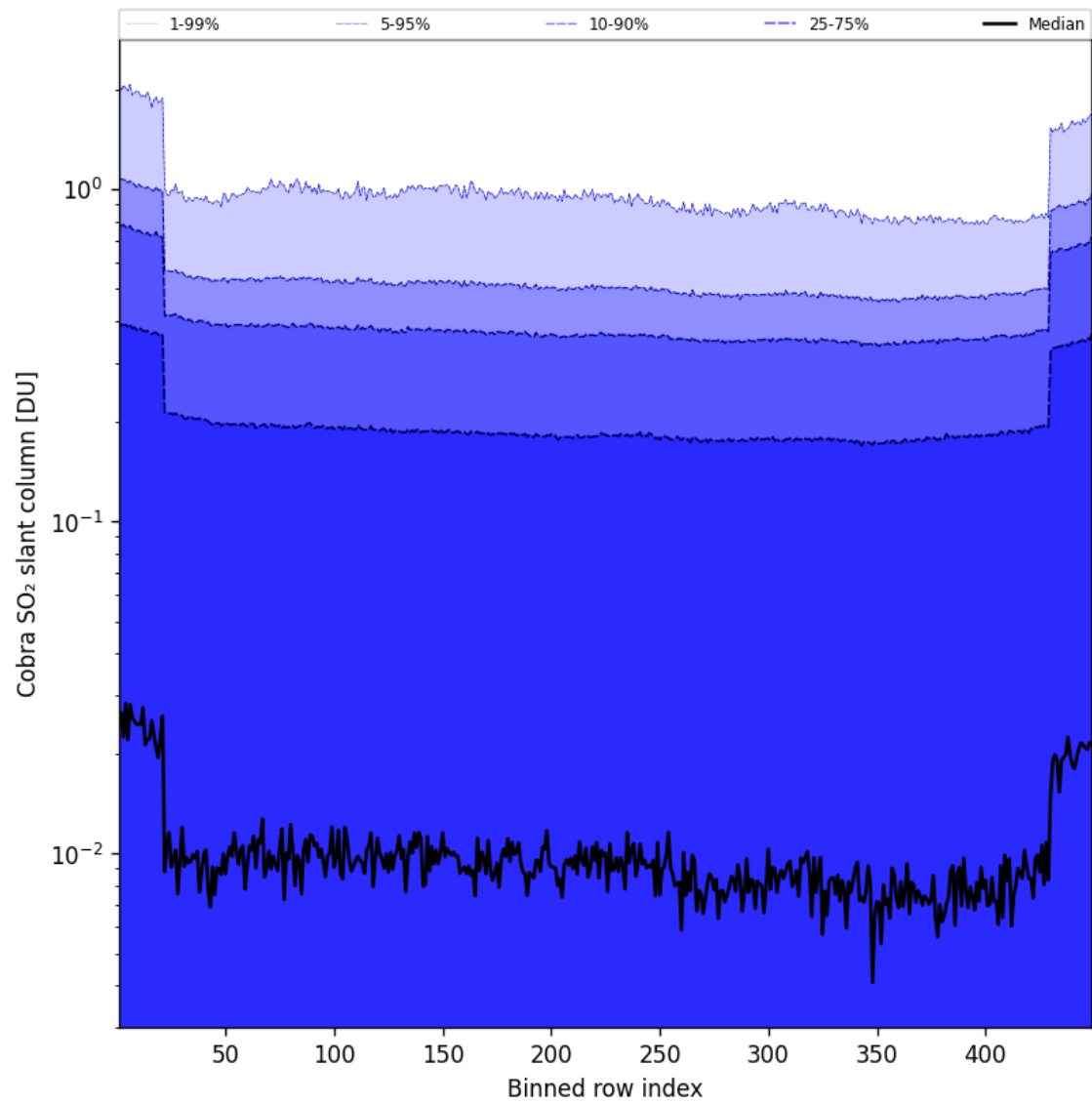
Figure 88: Along track statistics of “Cobra SO 2 slant column” for 2025-07-22 to 2025-07-22
