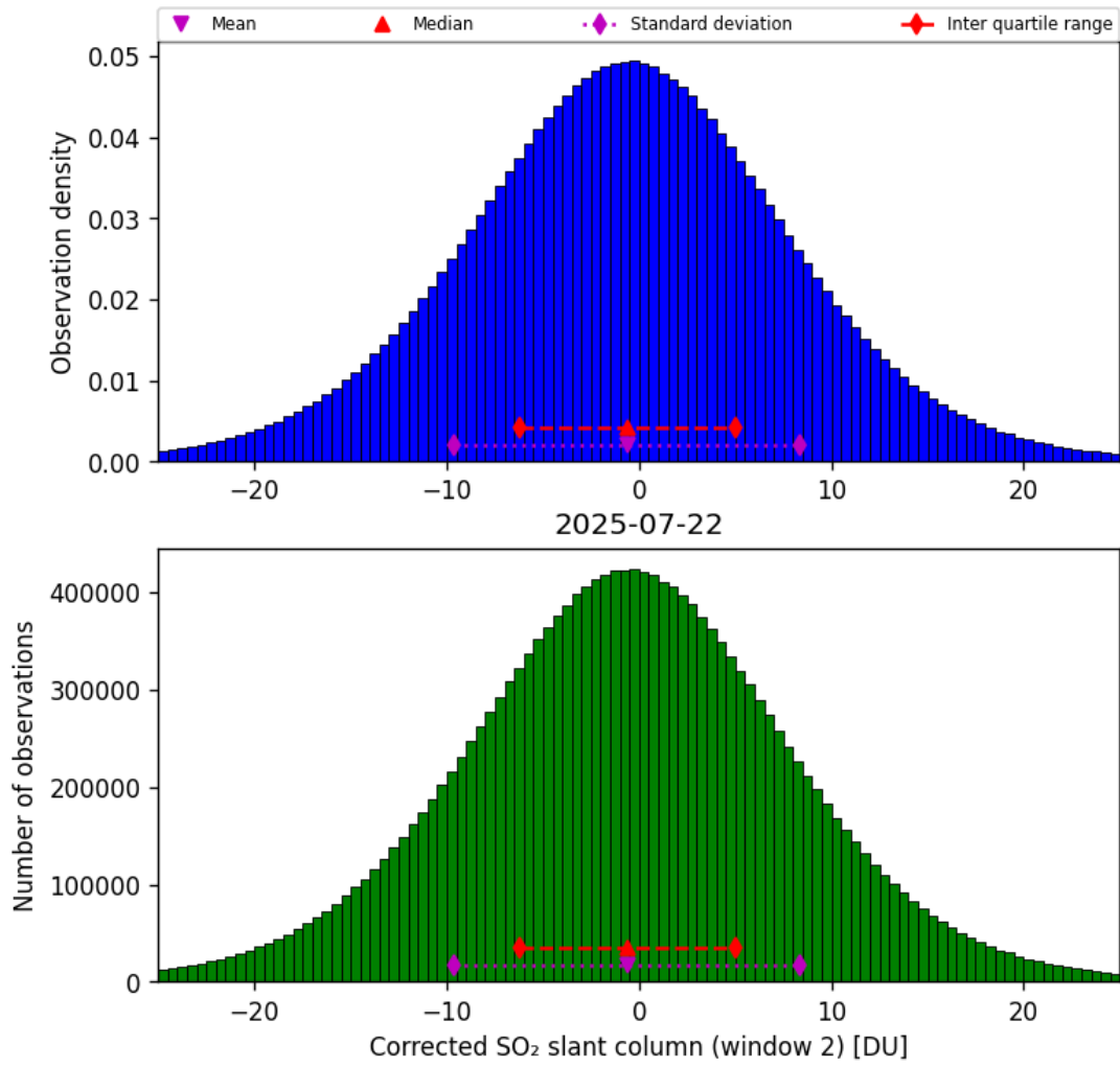
Figure 69: Histogram of “Corrected SO 2 slant column (window 2)” for 2025-07-22 to 2025-07-22
