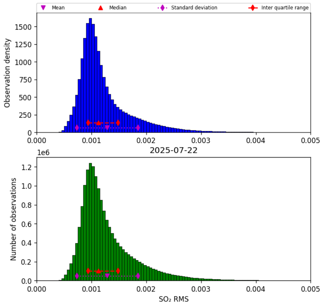
Figure 79: Histogram of “SO 2 RMS” for 2025-07-22 to 2025-07-22
