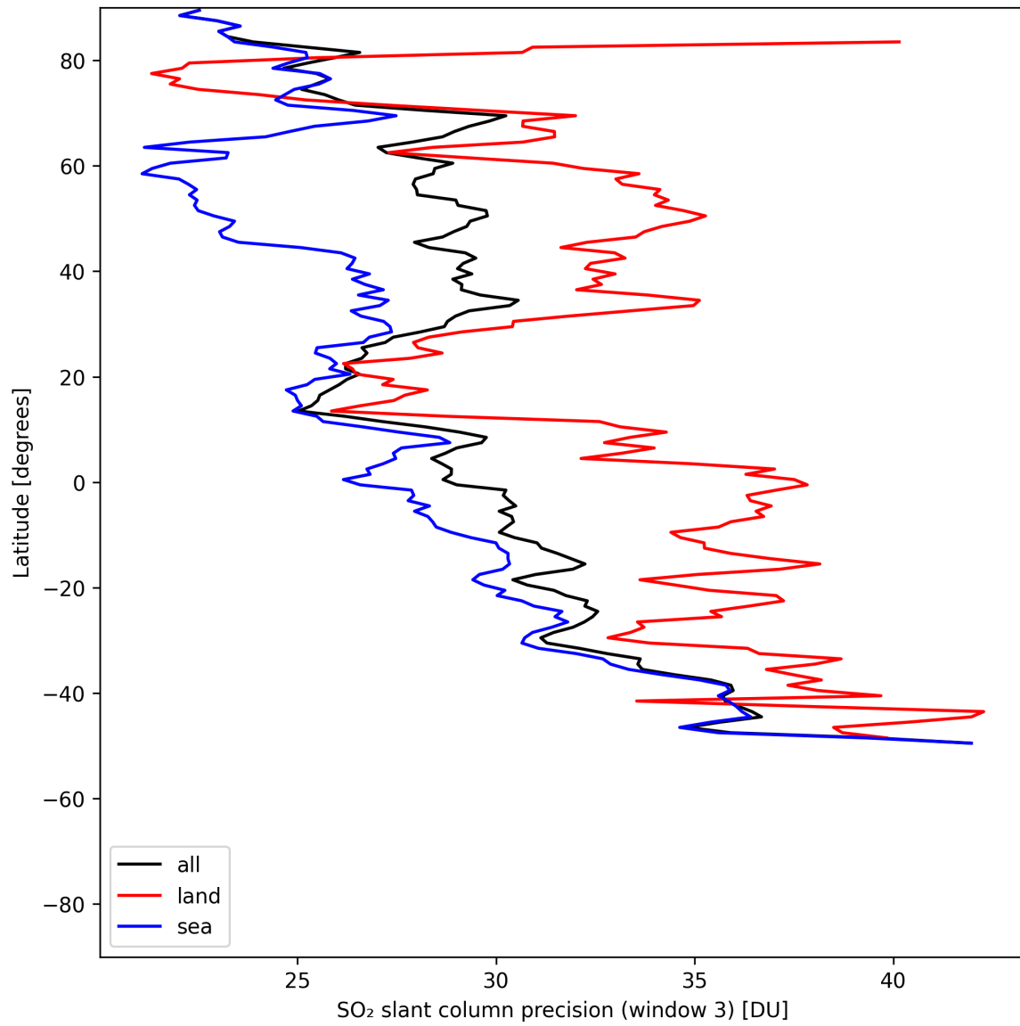
Figure 45: Zonal average of “SO 2 slant column precision (window 3)” for 2025-07-22 to 2025-07-22.
