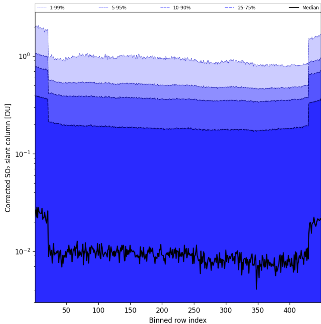
Figure 87: Along track statistics of "Corrected SO 2 slant column" for 2025-07-22 to 2025-07-22
