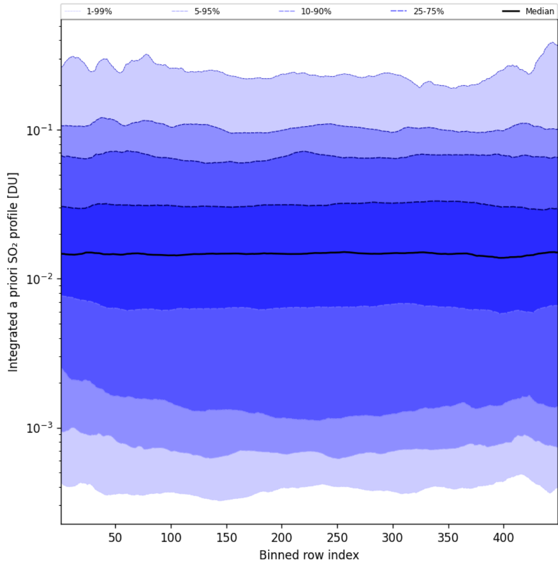
Figure 103: Along track statistics of “Integrated a priori SO 2 profile” for 2025-07-22 to 2025-07-22
