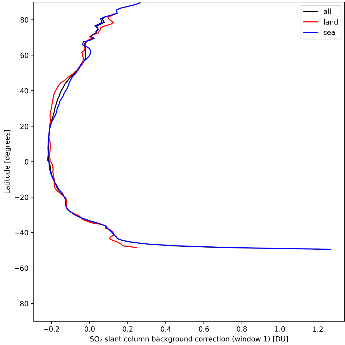
Figure 39: Zonal average of "SO 2 slant column background correction (window 1)" for 2025-07-22 to 2025-07-22.
