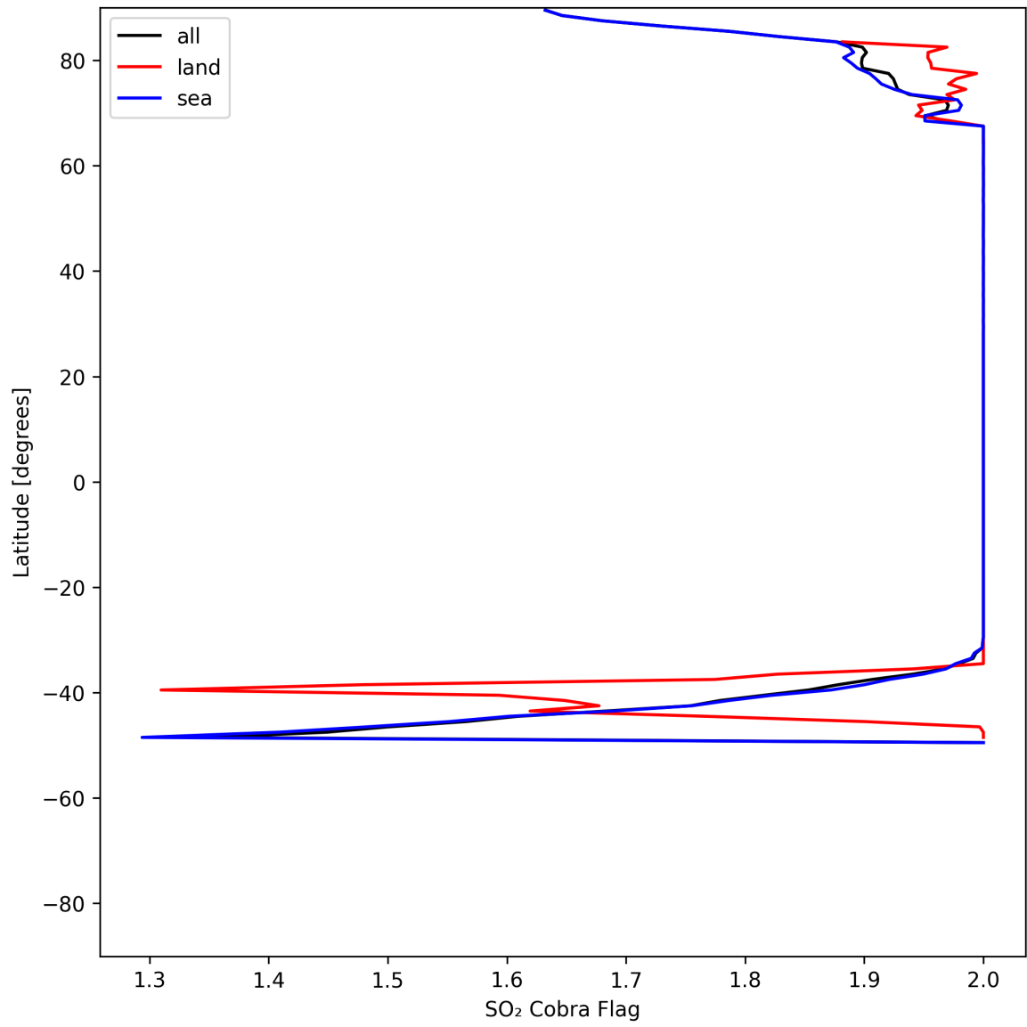
Figure 48: Zonal average of "SO 2 Cobra Flag" for 2025-07-22 to 2025-07-22.
