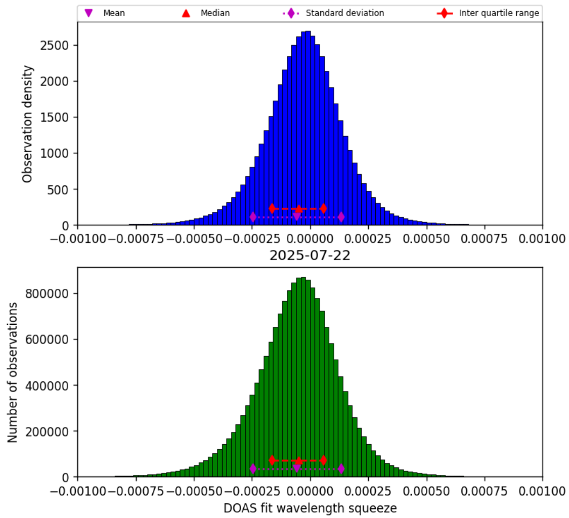
Figure 78: Histogram of “DOAS fit wavelength squeeze” for 2025-07-22 to 2025-07-22
