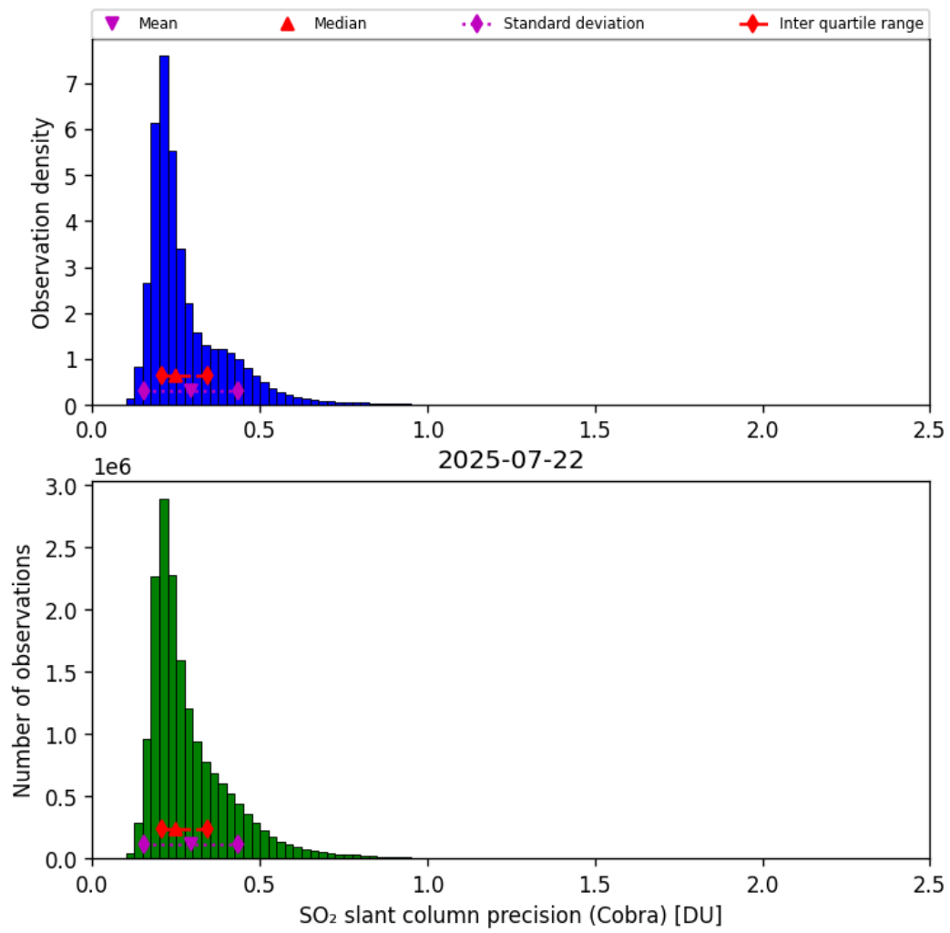
Figure 62: Histogram of “SO 2 slant column precision (Cobra)” for 2025-07-22 to 2025-07-22
