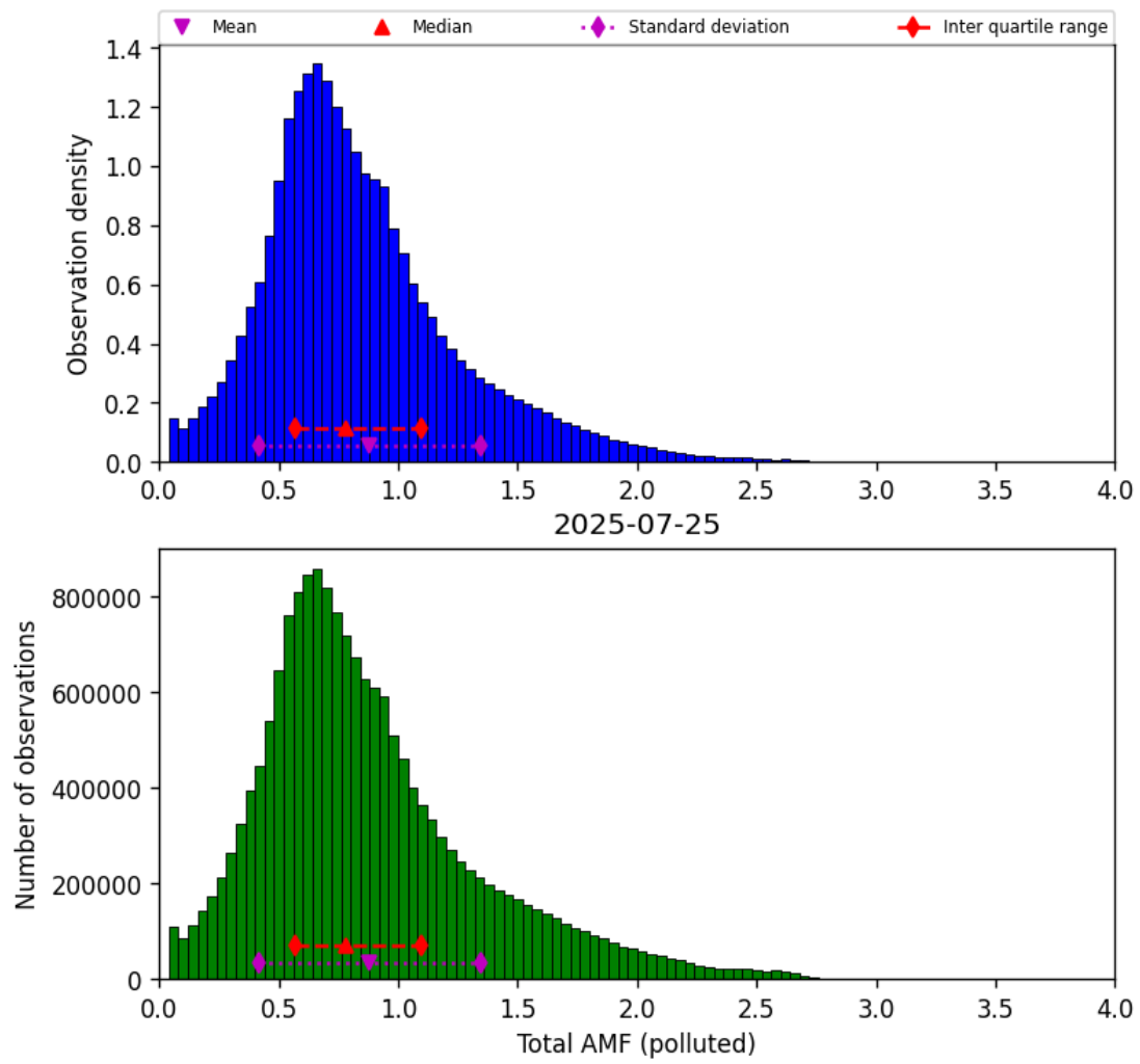
Figure 80: Histogram of “Total AMF (polluted)” for 2025-07-25 to 2025-07-26
