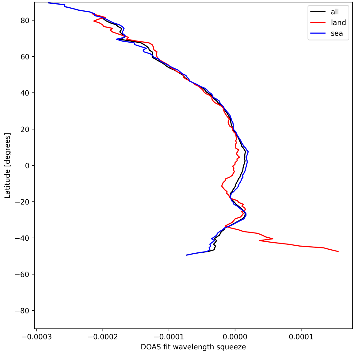
Figure 51: Zonal average of “DOAS fit wavelength squeeze” for 2025-07-25 to 2025-07-26.
