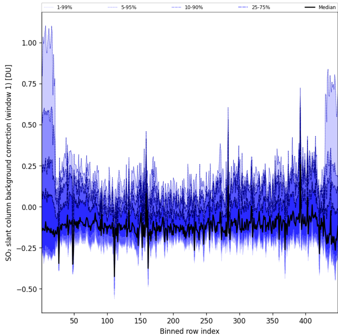
Figure 93: Along track statistics of “SO 2 slant column background correction (window 1)” for 2025-07-25 to 2025-07-26
