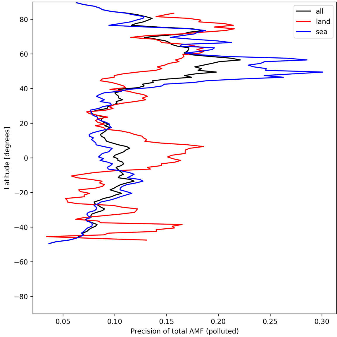
Figure 54: Zonal average of “Precision of total AMF (polluted)” for 2025-07-25 to 2025-07-26.
