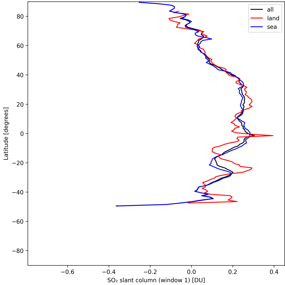
Figure 36: Zonal average of “SO 2 slant column (window 1)” for 2025-07-25 to 2025-07-26.
