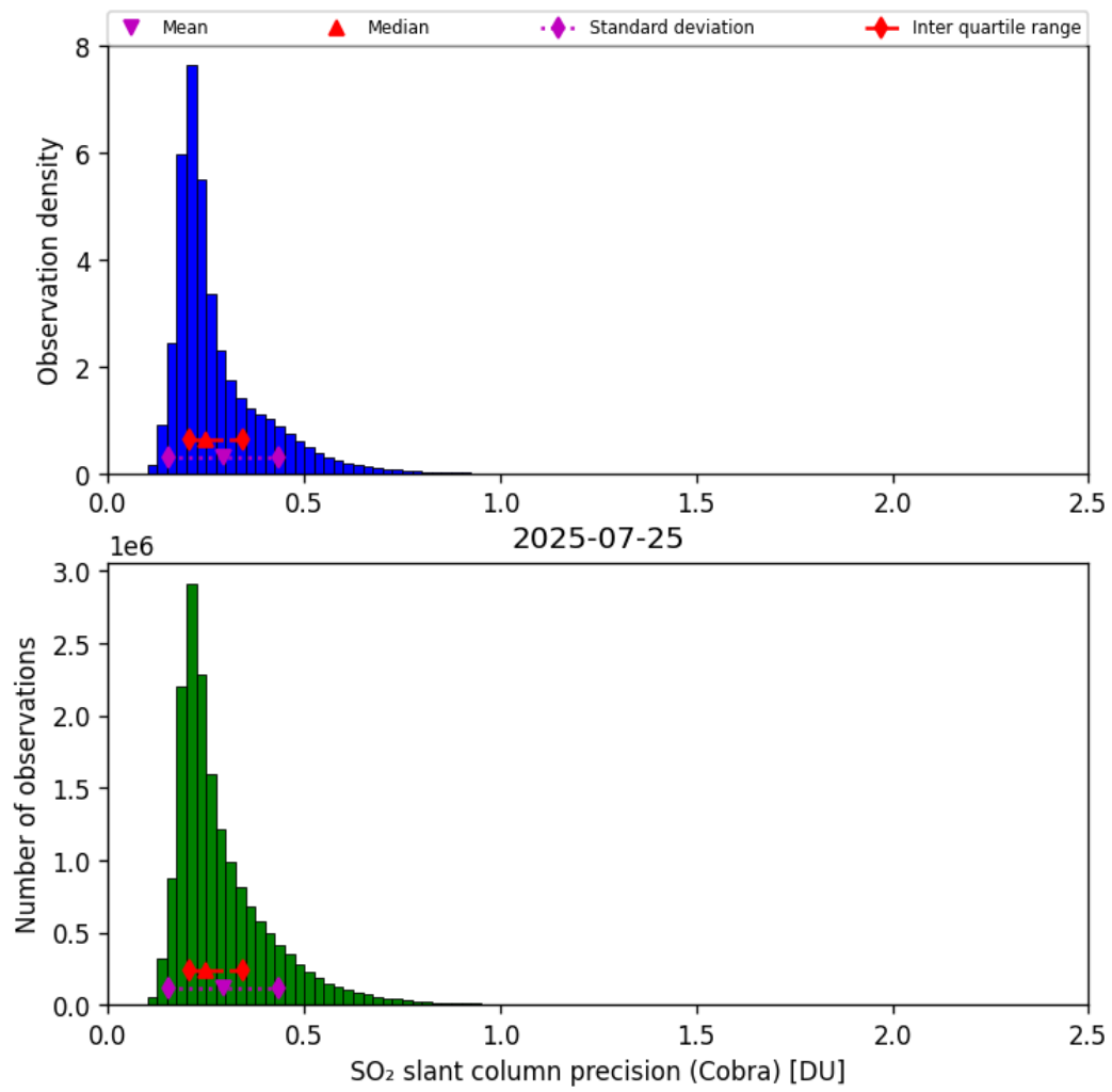
Figure 62: Histogram of “SO 2 slant column precision (Cobra)” for 2025-07-25 to 2025-07-26
