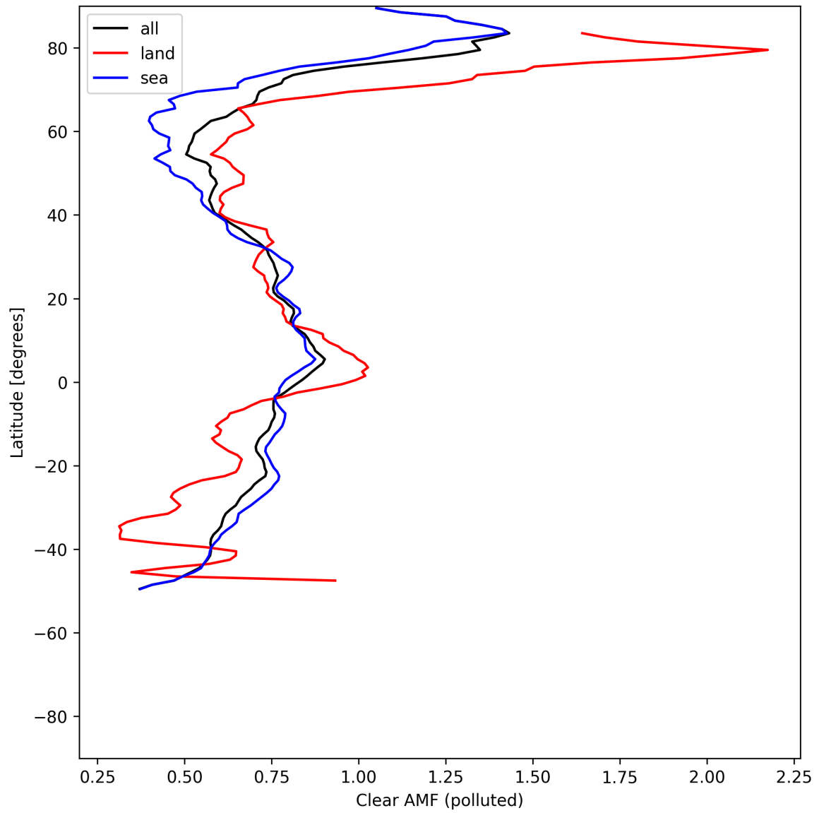
Figure 55: Zonal average of “Clear AMF (polluted)” for 2025-07-25 to 2025-07-26.
