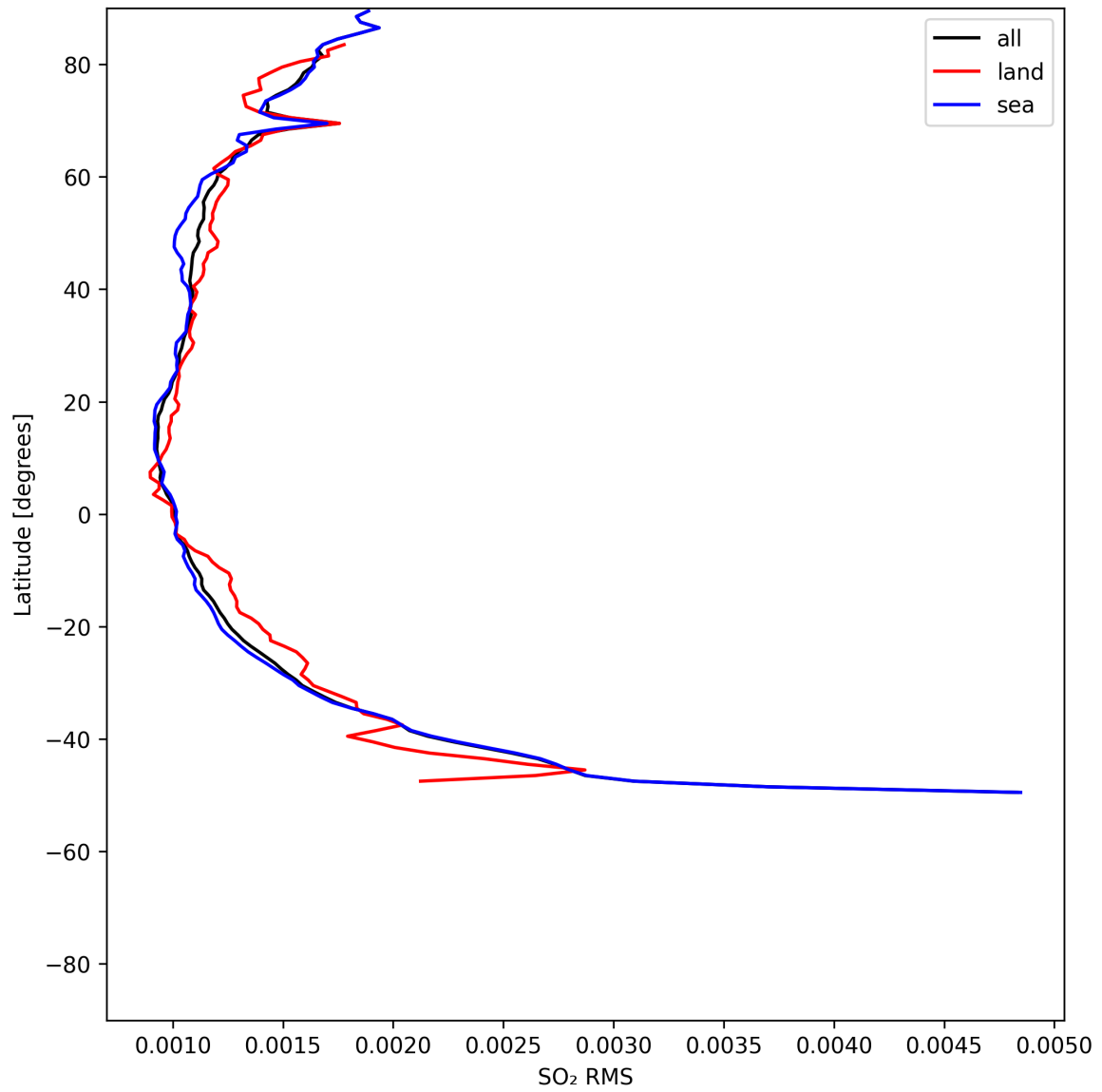
Figure 52: Zonal average of “SO 2 RMS” for 2025-07-25 to 2025-07-26.
