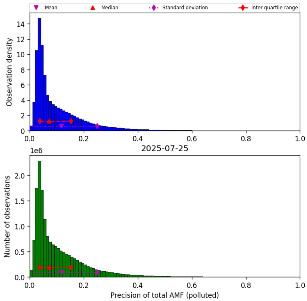
Figure 81: Histogram of “Precision of total AMF (polluted)” for 2025-07-25 to 2025-07-26
