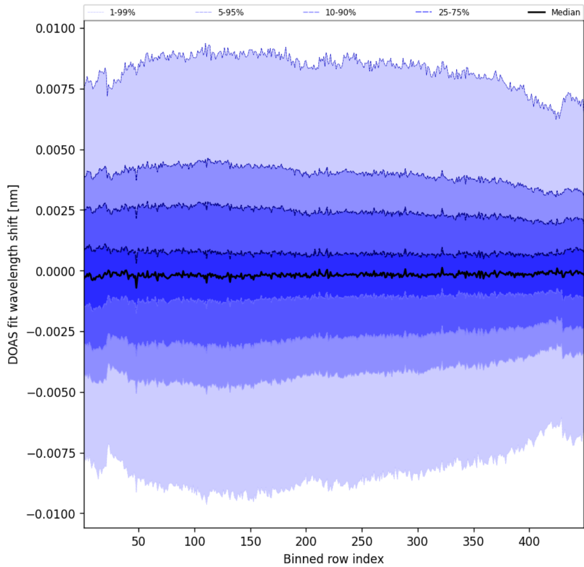
Figure 104: Along track statistics of “DOAS fit wavelength shift” for 2025-07-25 to 2025-07-26
