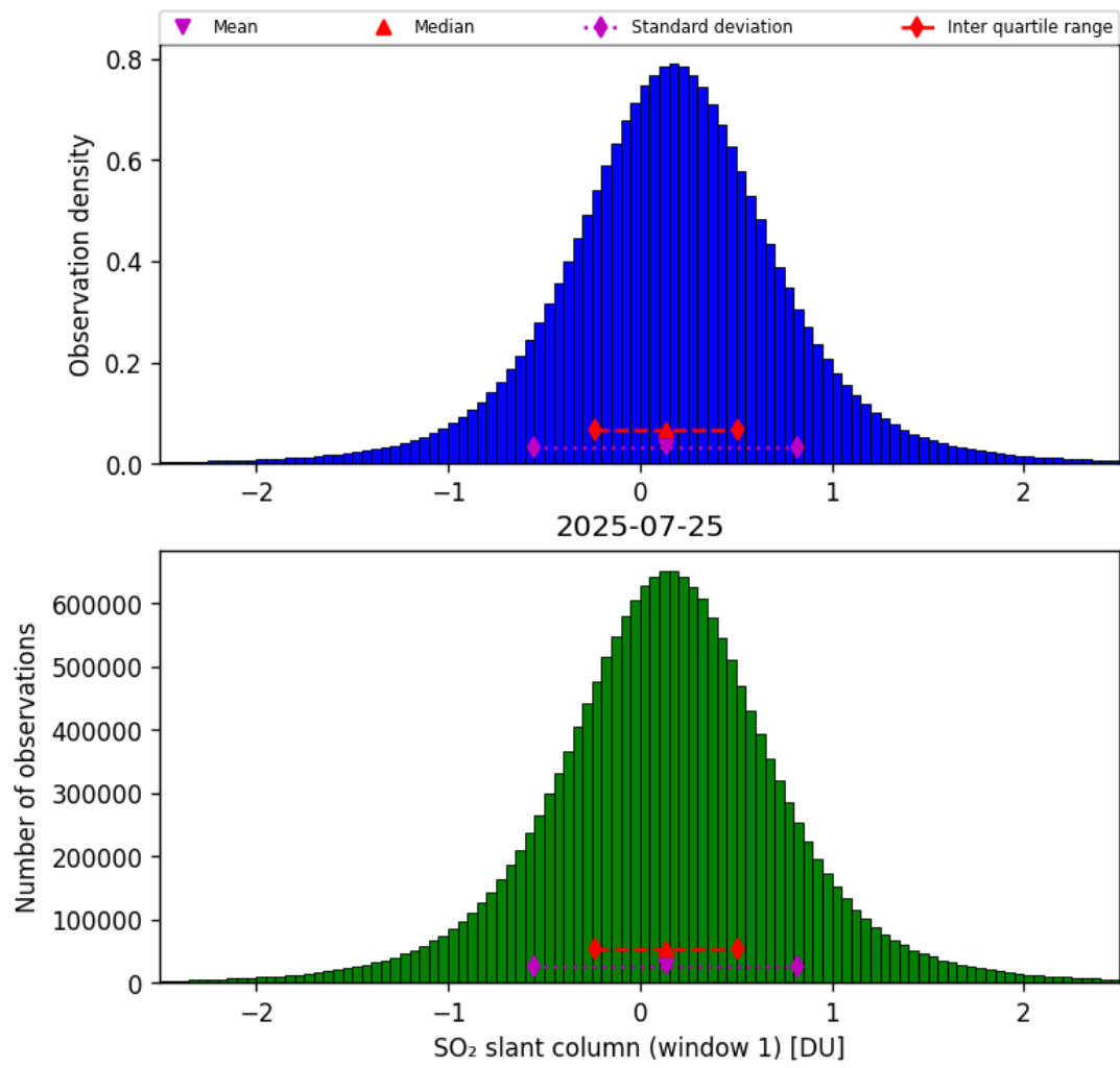
Figure 63: Histogram of “SO 2 slant column (window 1)” for 2025-07-25 to 2025-07-26
