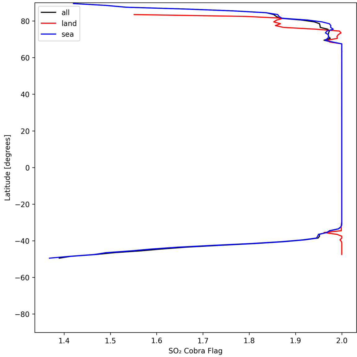
Figure 48: Zonal average of "SO 2 Cobra Flag" for 2025-07-25 to 2025-07-26.
