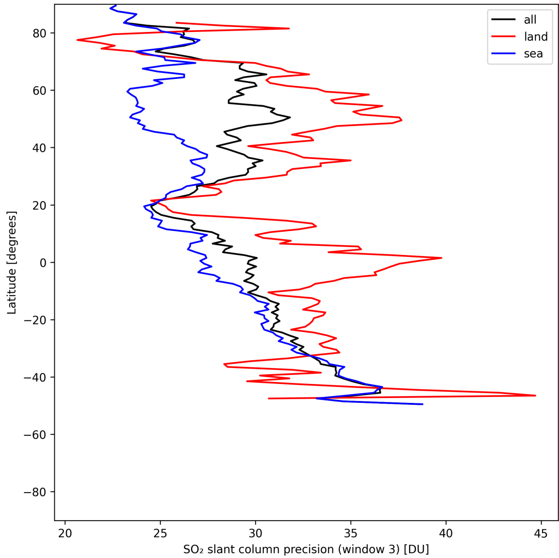
Figure 45: Zonal average of “SO 2 slant column precision (window 3)” for 2025-07-25 to 2025-07-26.
