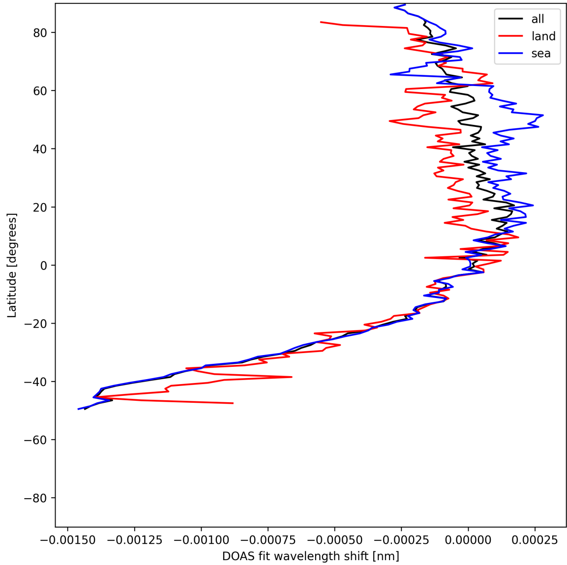
Figure 50: Zonal average of “DOAS fit wavelength shift” for 2025-07-25 to 2025-07-26.
