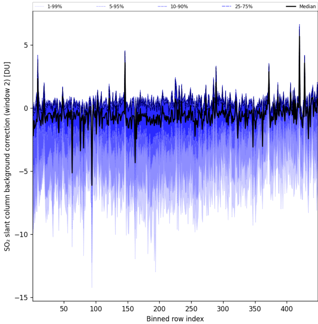
Figure 97: Along track statistics of “SO 2 slant column background correction (window 2)” for 2025-07-25 to 2025-07-26
