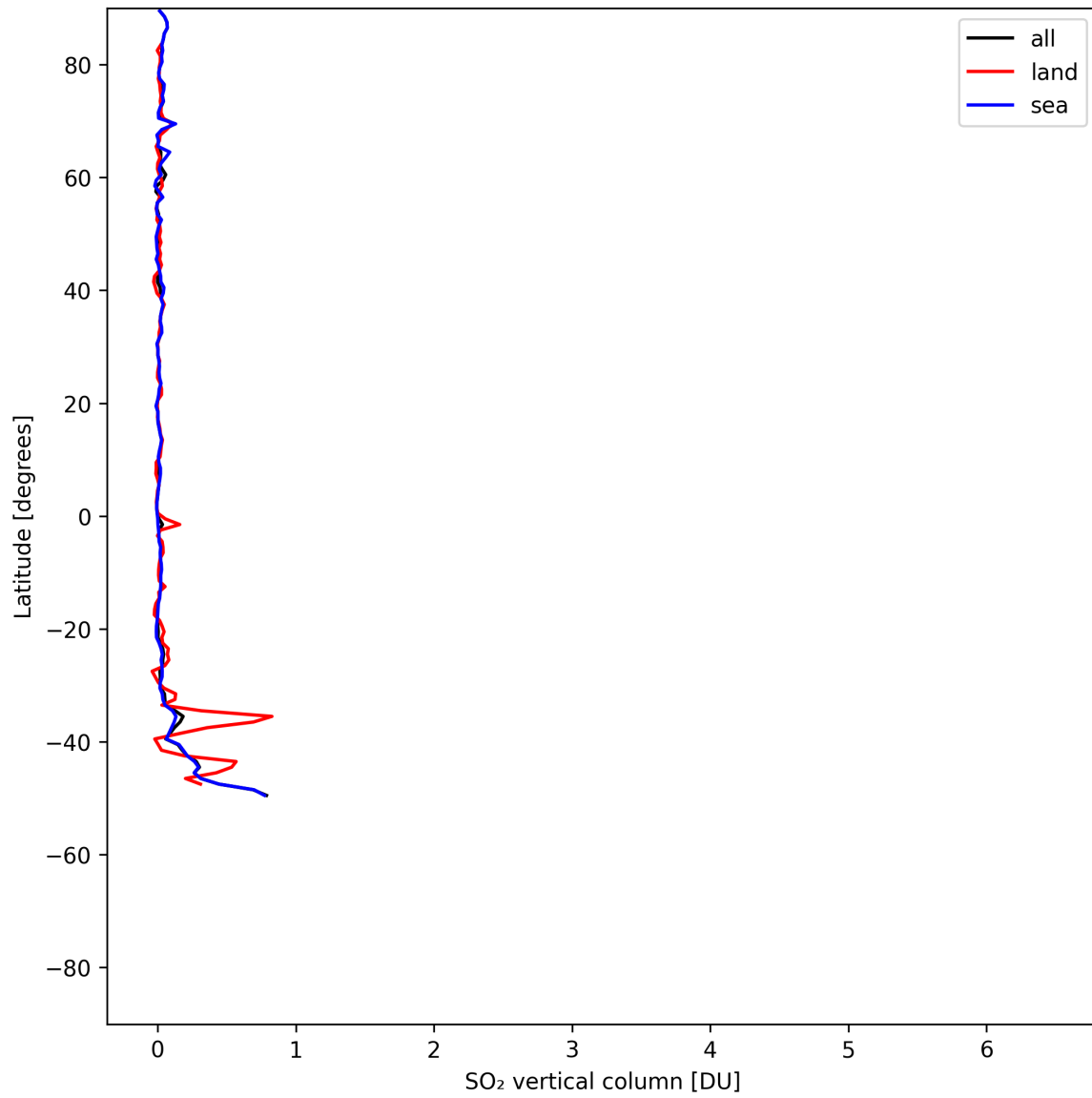
Figure 31: Zonal average of “SO 2 vertical column” for 2025-07-25 to 2025-07-26.
