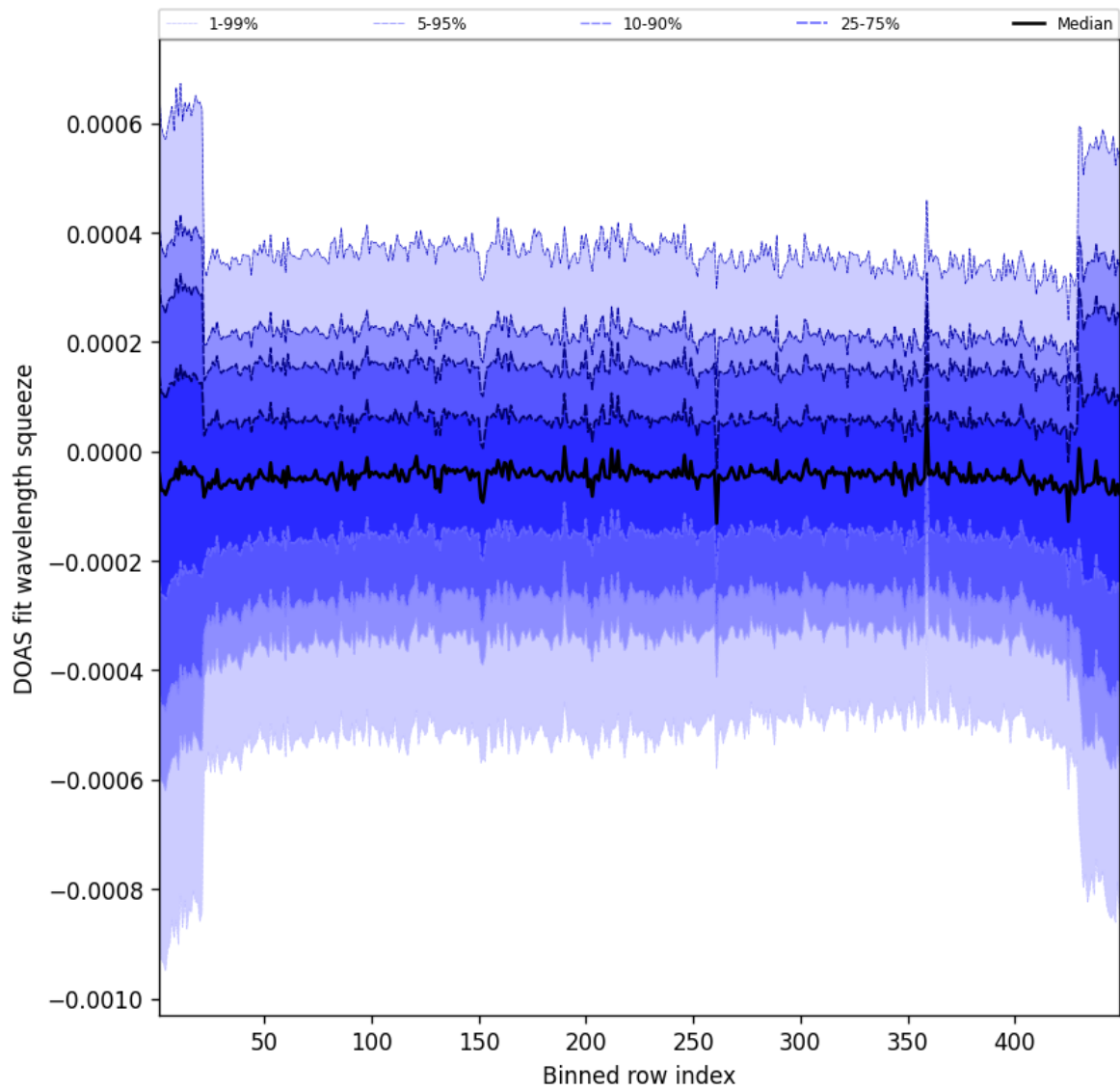
Figure 105: Along track statistics of “DOAS fit wavelength squeeze” for 2025-07-25 to 2025-07-26
