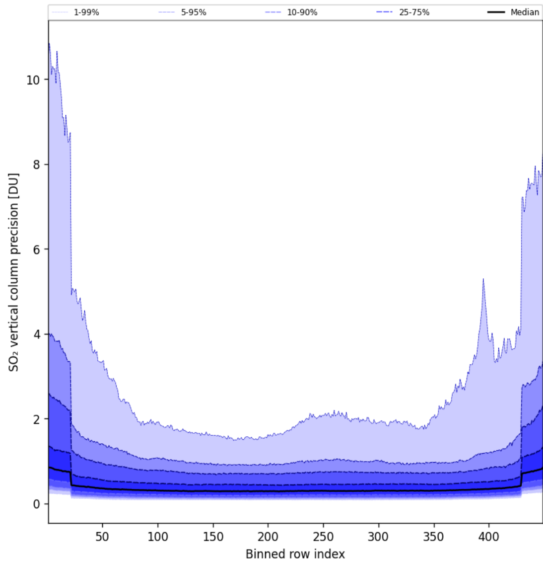
Figure 86: Along track statistics of “SO 2 vertical column precision” for 2025-07-25 to 2025-07-26
