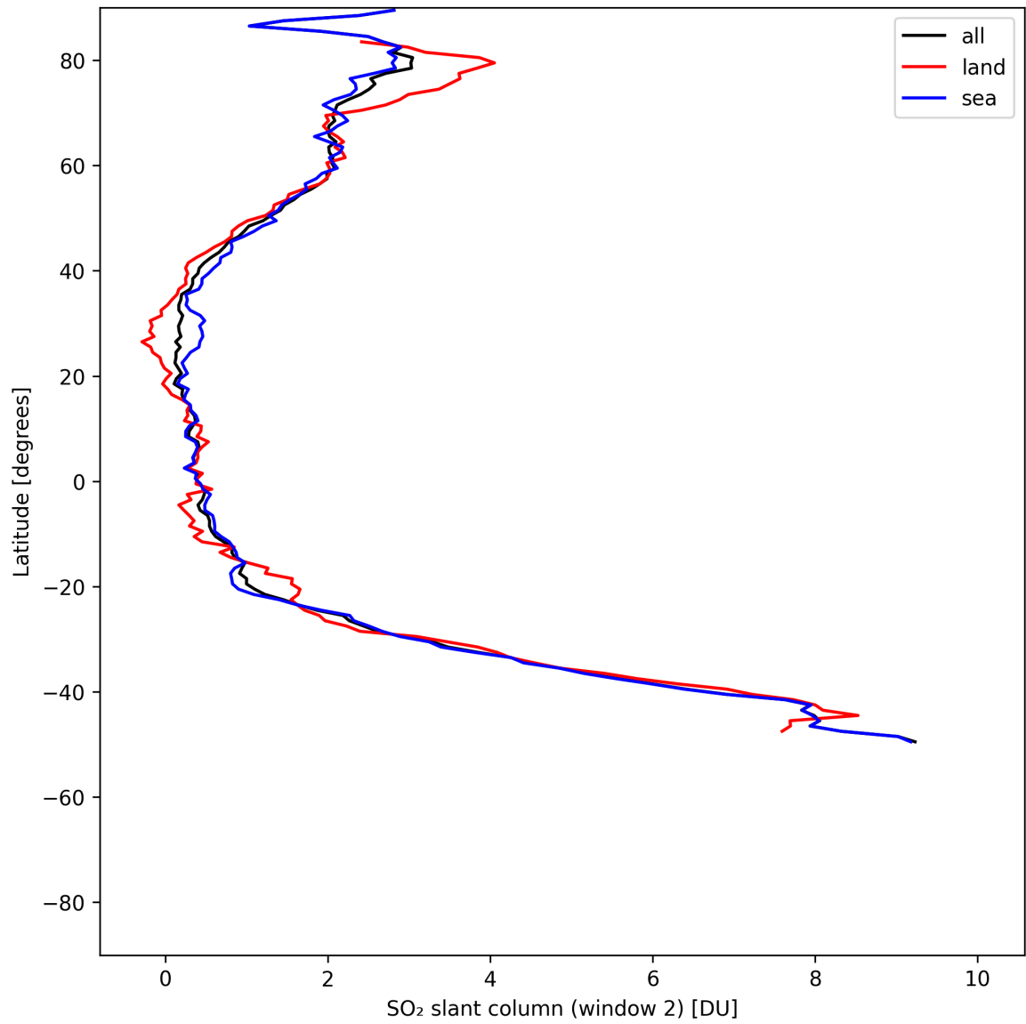
Figure 40: Zonal average of “SO 2 slant column (window 2)” for 2025-07-25 to 2025-07-26.
