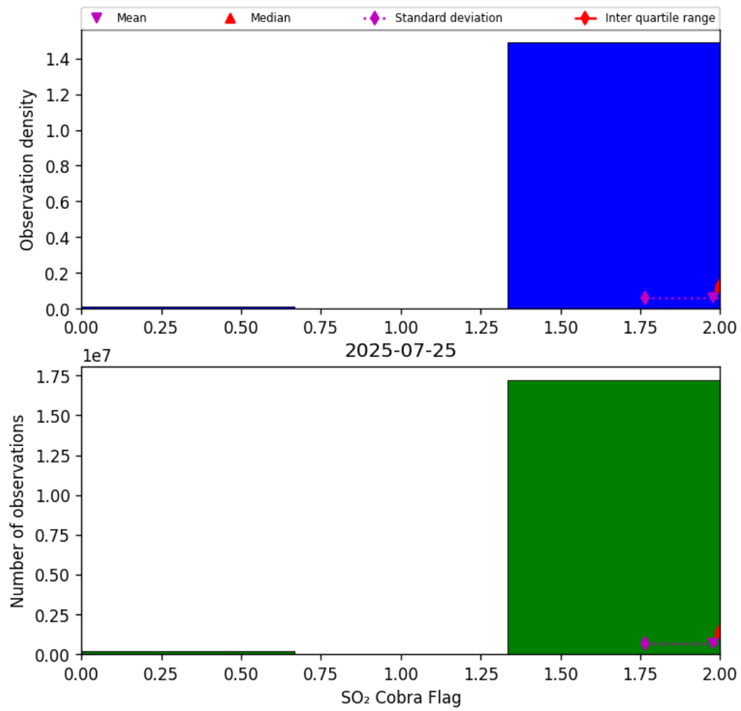
Figure 75: Histogram of “SO 2 Cobra Flag” for 2025-07-25 to 2025-07-26
