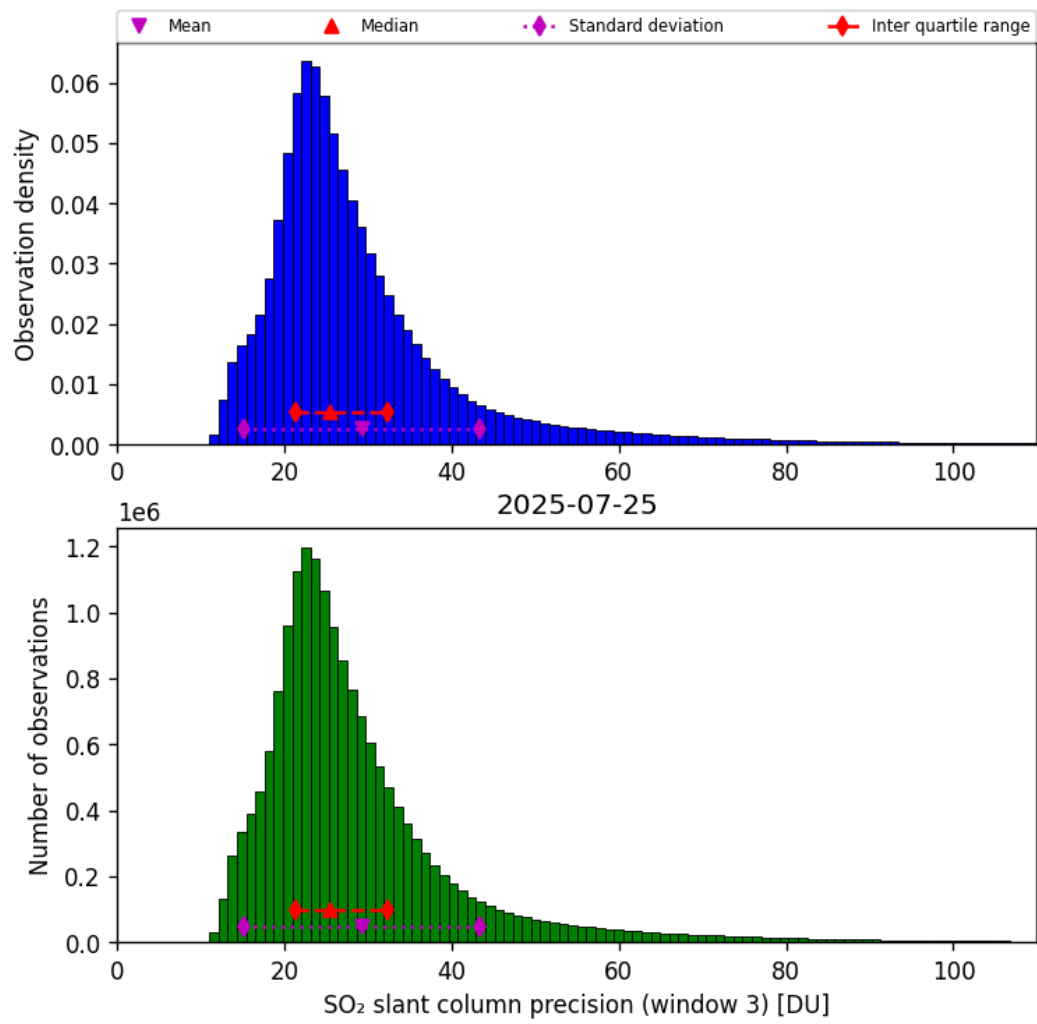
Figure 72: Histogram of “SO 2 slant column precision (window 3)” for 2025-07-25 to 2025-07-26
