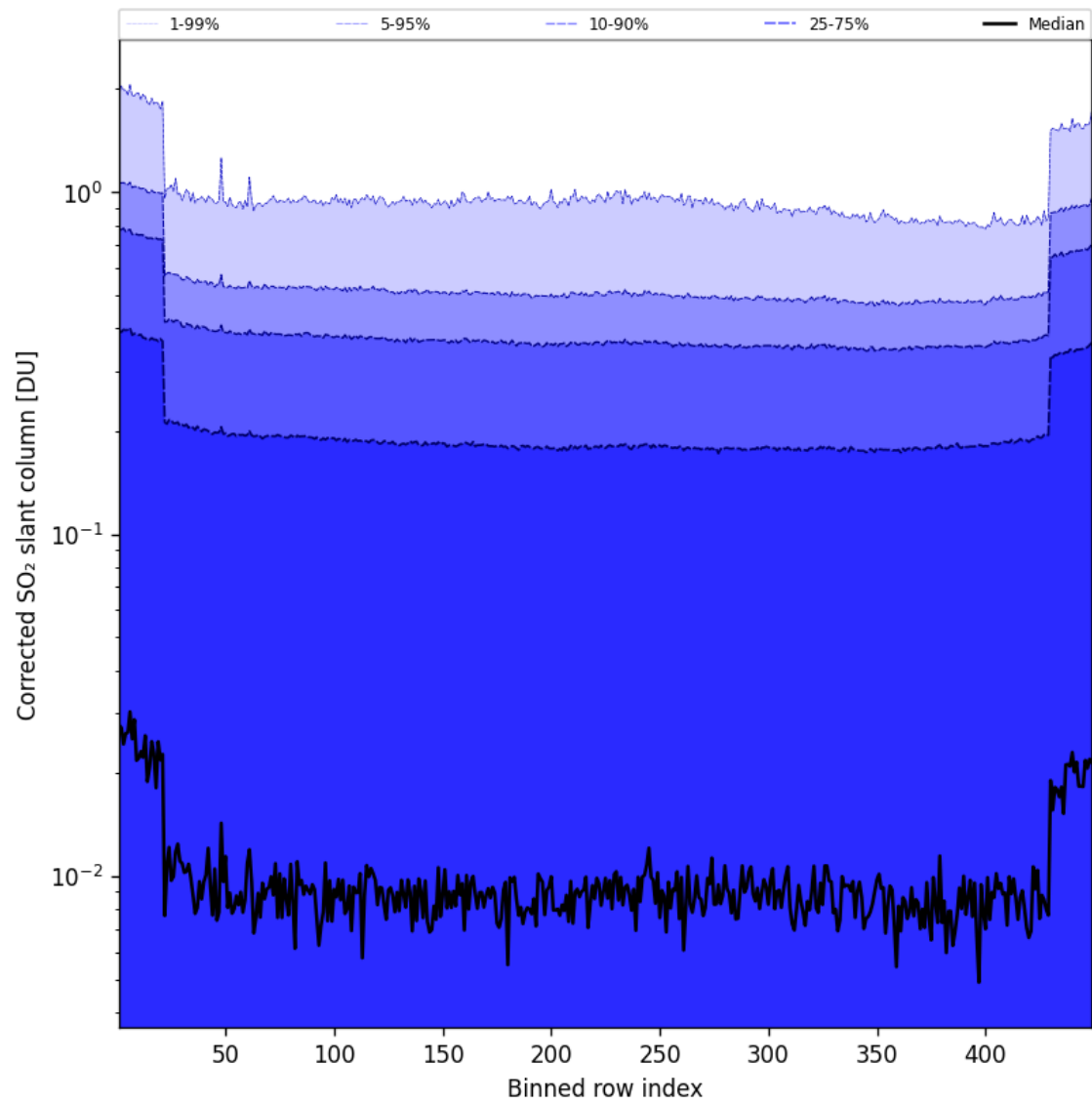
Figure 87: Along track statistics of "Corrected SO 2 slant column" for 2025-07-25 to 2025-07-26
