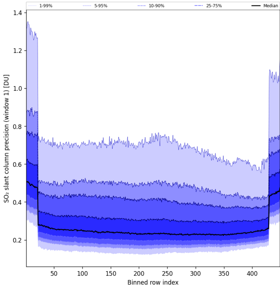
Figure 91: Along track statistics of “SO 2 slant column precision (window 1)” for 2025-07-25 to 2025-07-26
