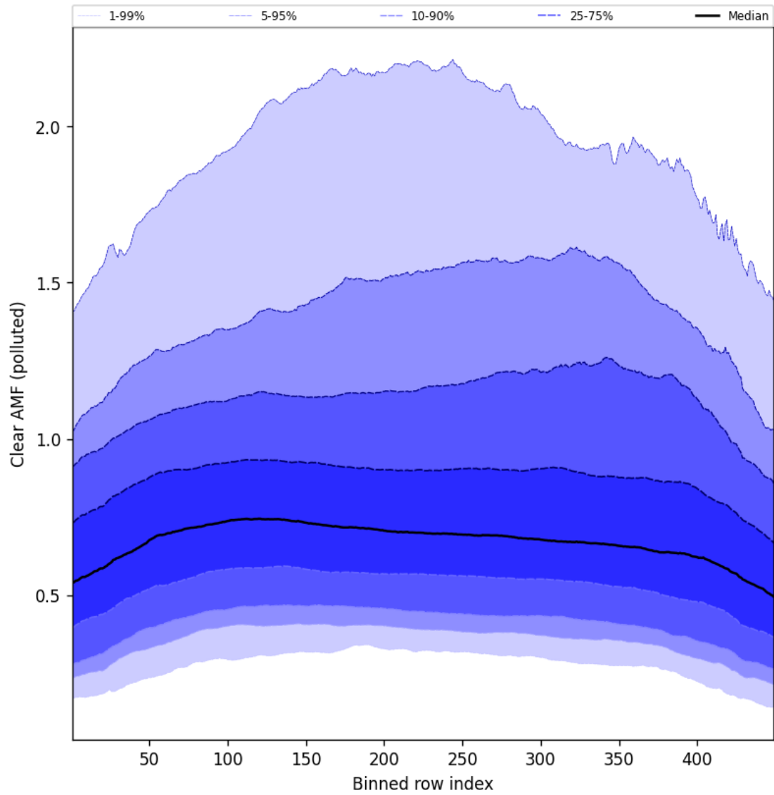
Figure 109: Along track statistics of “Clear AMF (polluted)” for 2025-07-25 to 2025-07-26
