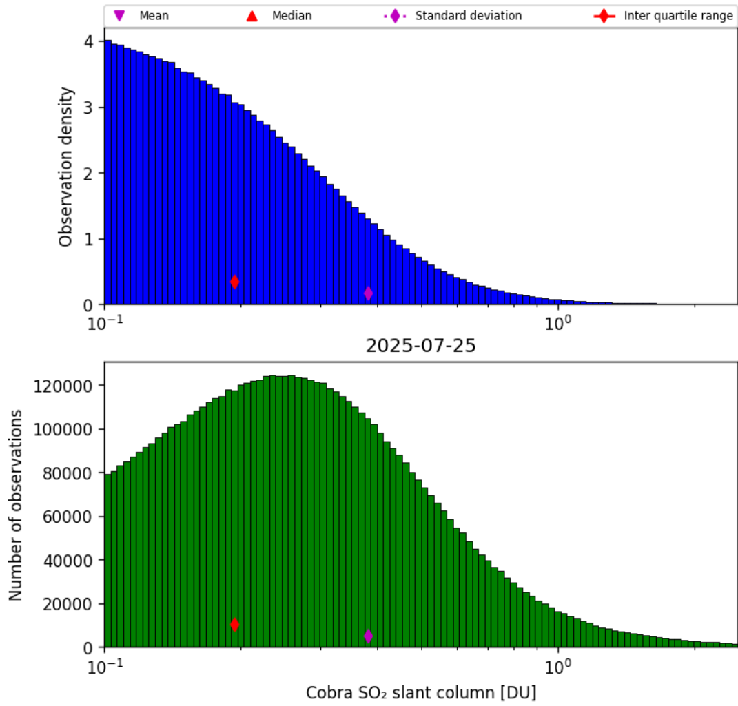
Figure 61: Histogram of “Cobra SO 2 slant column” for 2025-07-25 to 2025-07-26
