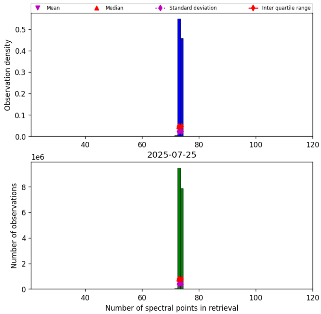
Figure 83: Histogram of “Number of spectral points in retrieval” for 2025-07-25 to 2025-07-26
