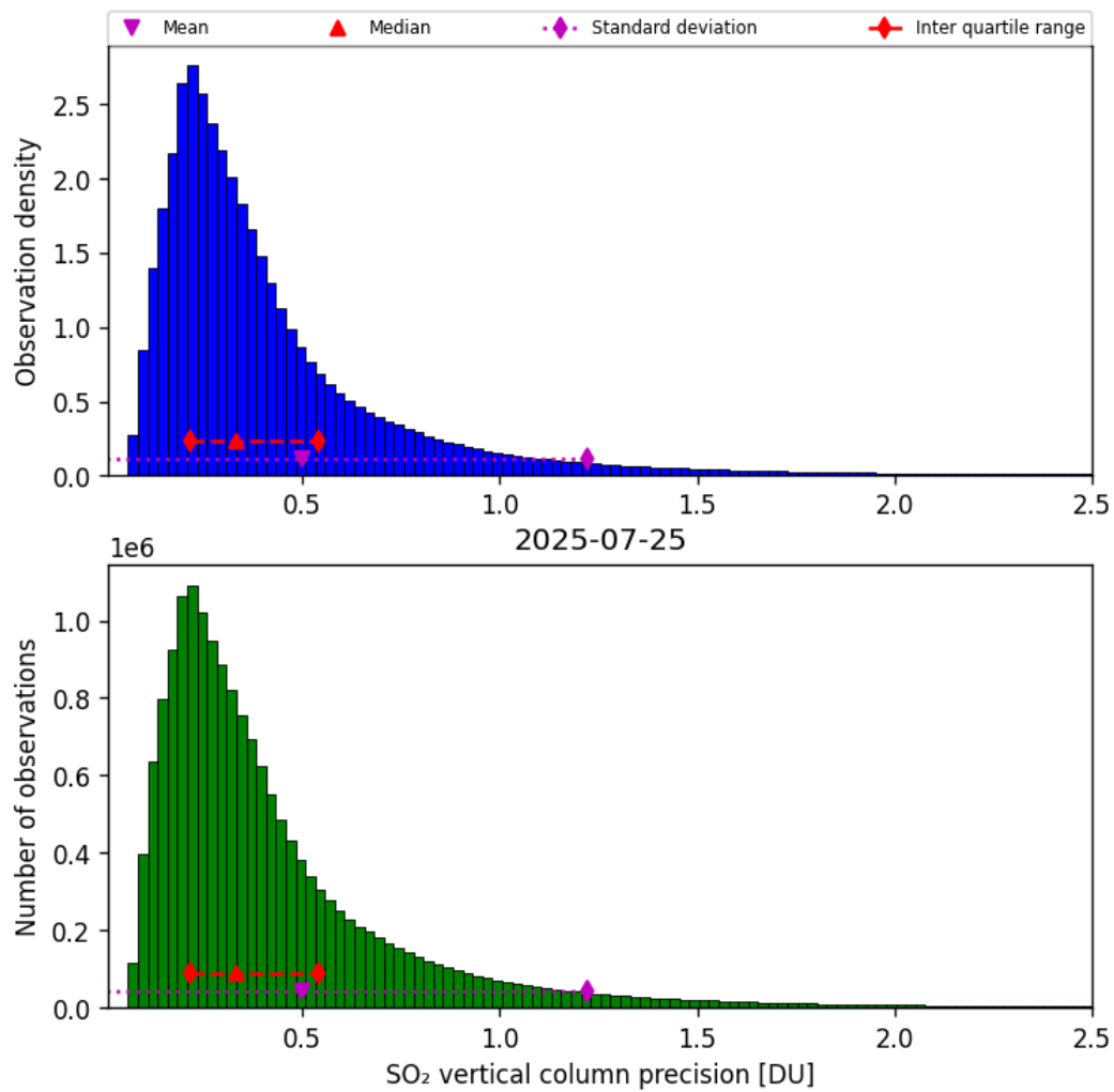
Figure 59: Histogram of “SO 2 vertical column precision” for 2025-07-25 to 2025-07-26
