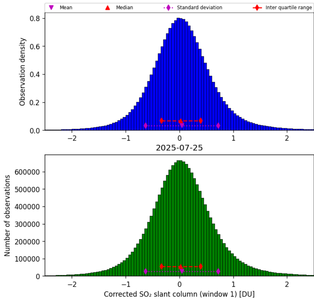
Figure 65: Histogram of “Corrected SO 2 slant column (window 1)” for 2025-07-25 to 2025-07-26
