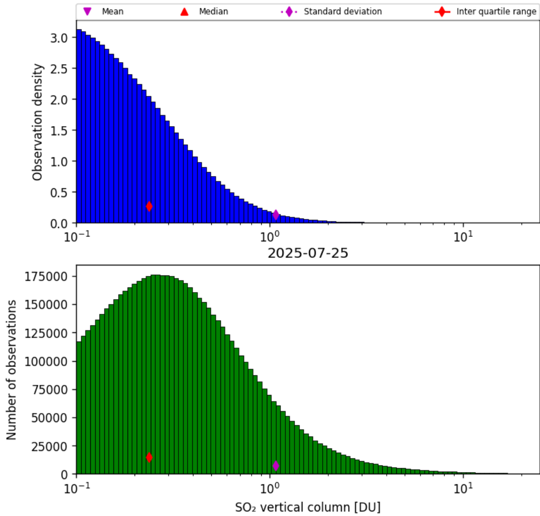
Figure 58: Histogram of “SO 2 vertical column” for 2025-07-25 to 2025-07-26
