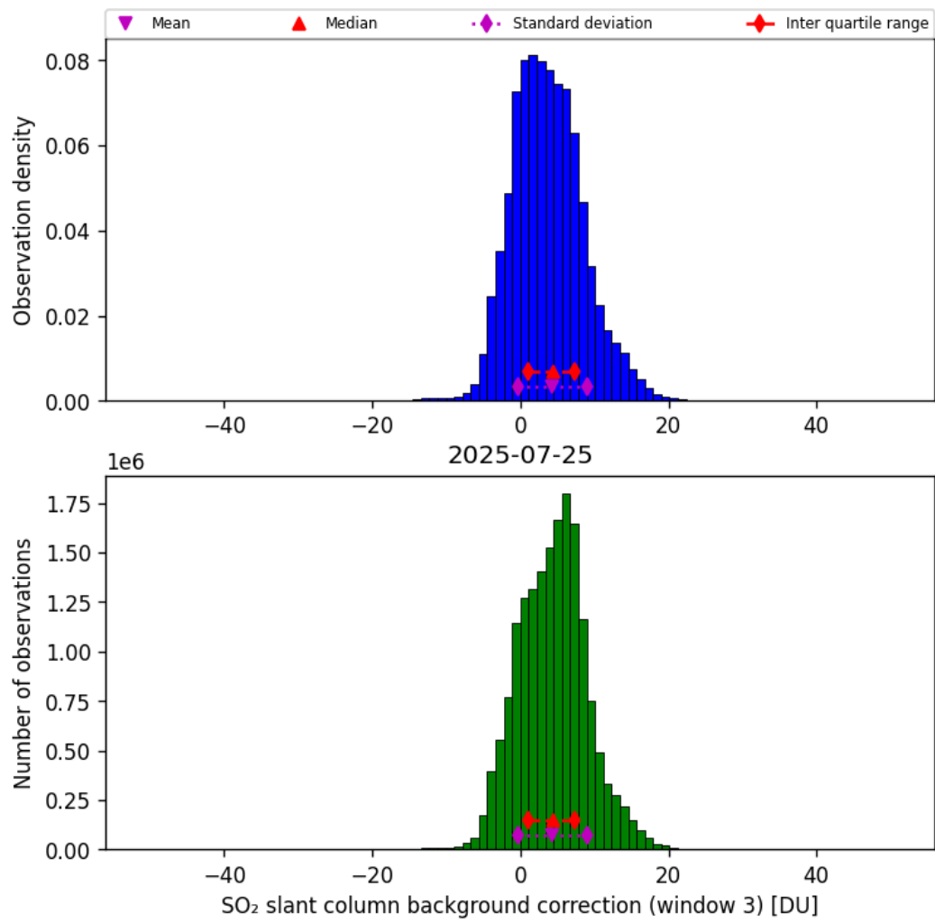
Figure 74: Histogram of “SO 2 slant column background correction (window 3)” for 2025-07-25 to 2025-07-26
