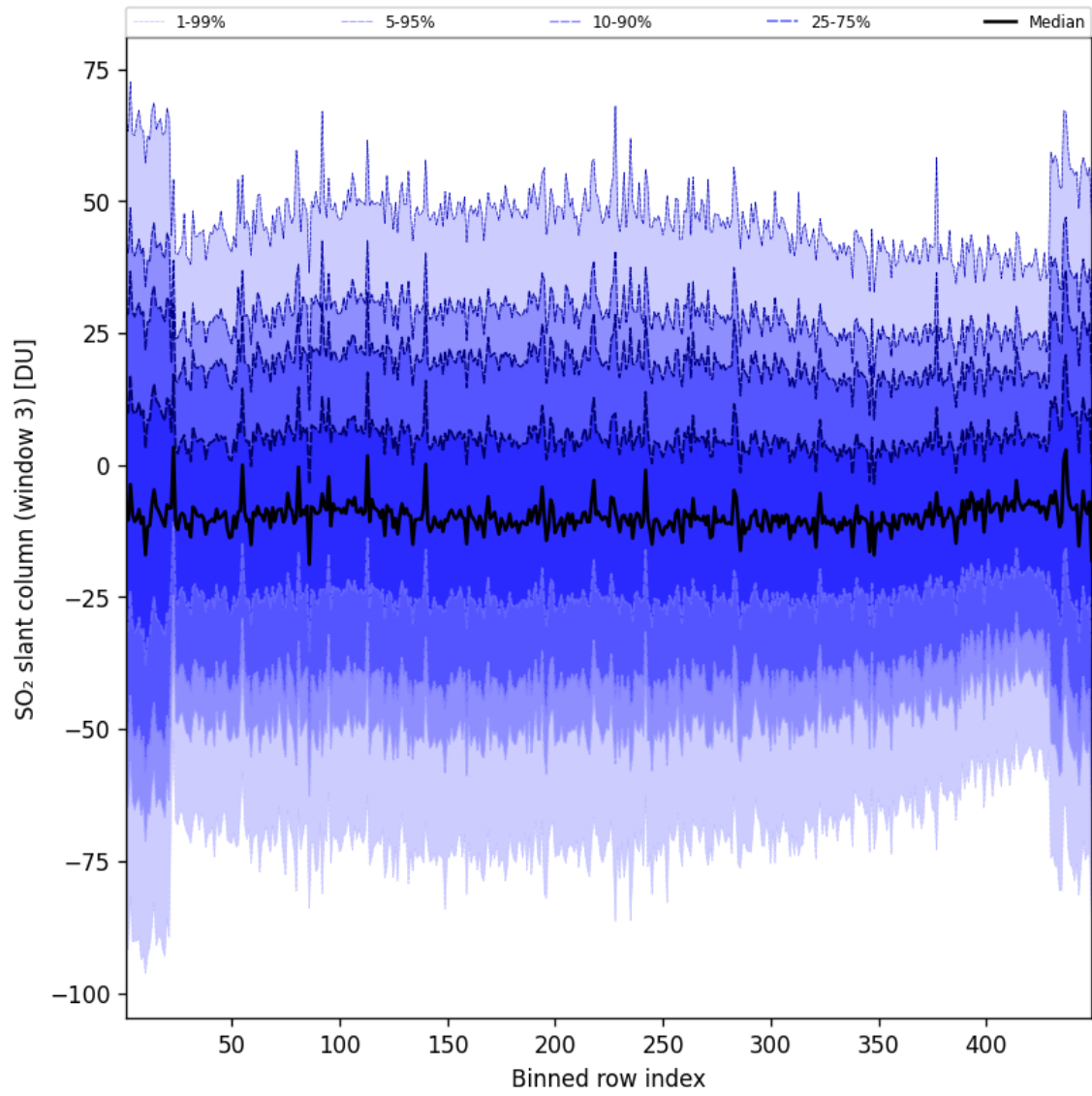
Figure 98: Along track statistics of “SO 2 slant column (window 3)” for 2025-07-25 to 2025-07-26
