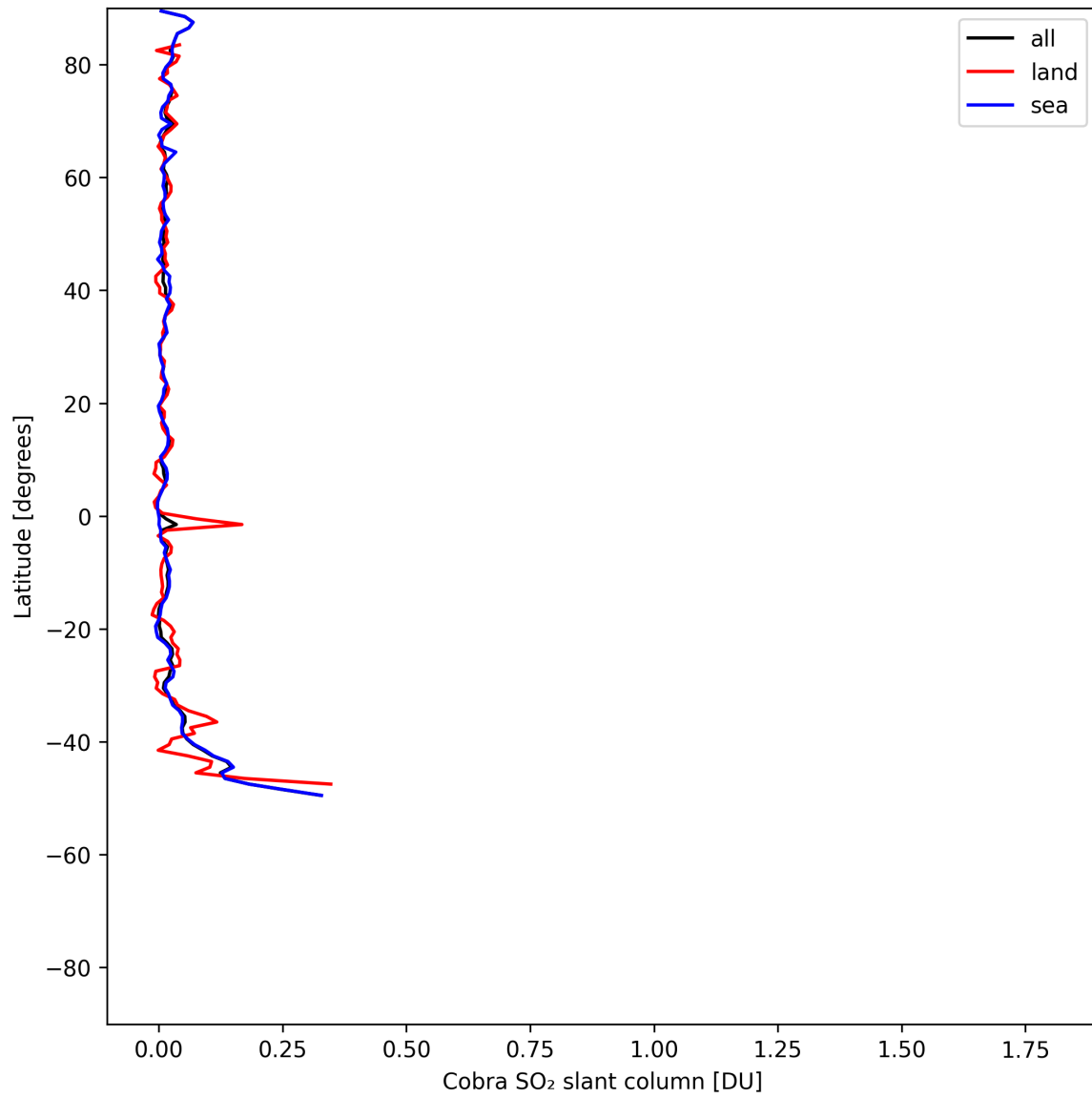
Figure 34: Zonal average of “Cobra SO 2 slant column” for 2025-07-25 to 2025-07-26.
