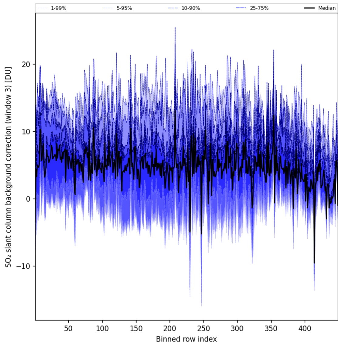
Figure 101: Along track statistics of “SO 2 slant column background correction (window 3)” for 2025-07-25 to 2025-07-26
