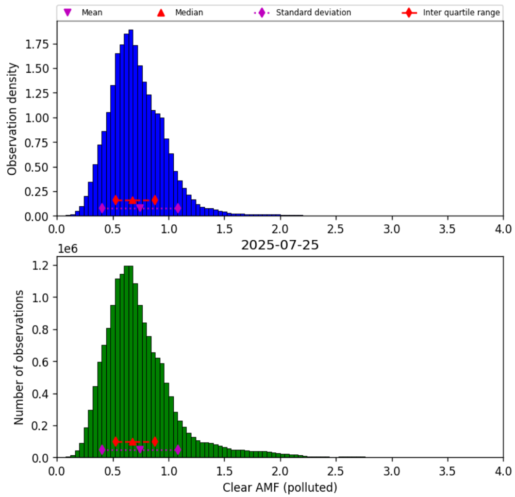
Figure 82: Histogram of “Clear AMF (polluted)” for 2025-07-25 to 2025-07-26
