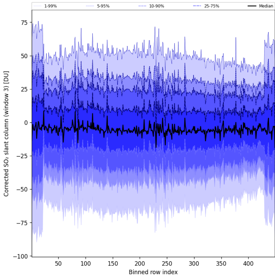
Figure 100: Along track statistics of “Corrected SO 2 slant column (window 3)” for 2025-07-25 to 2025-07-26
