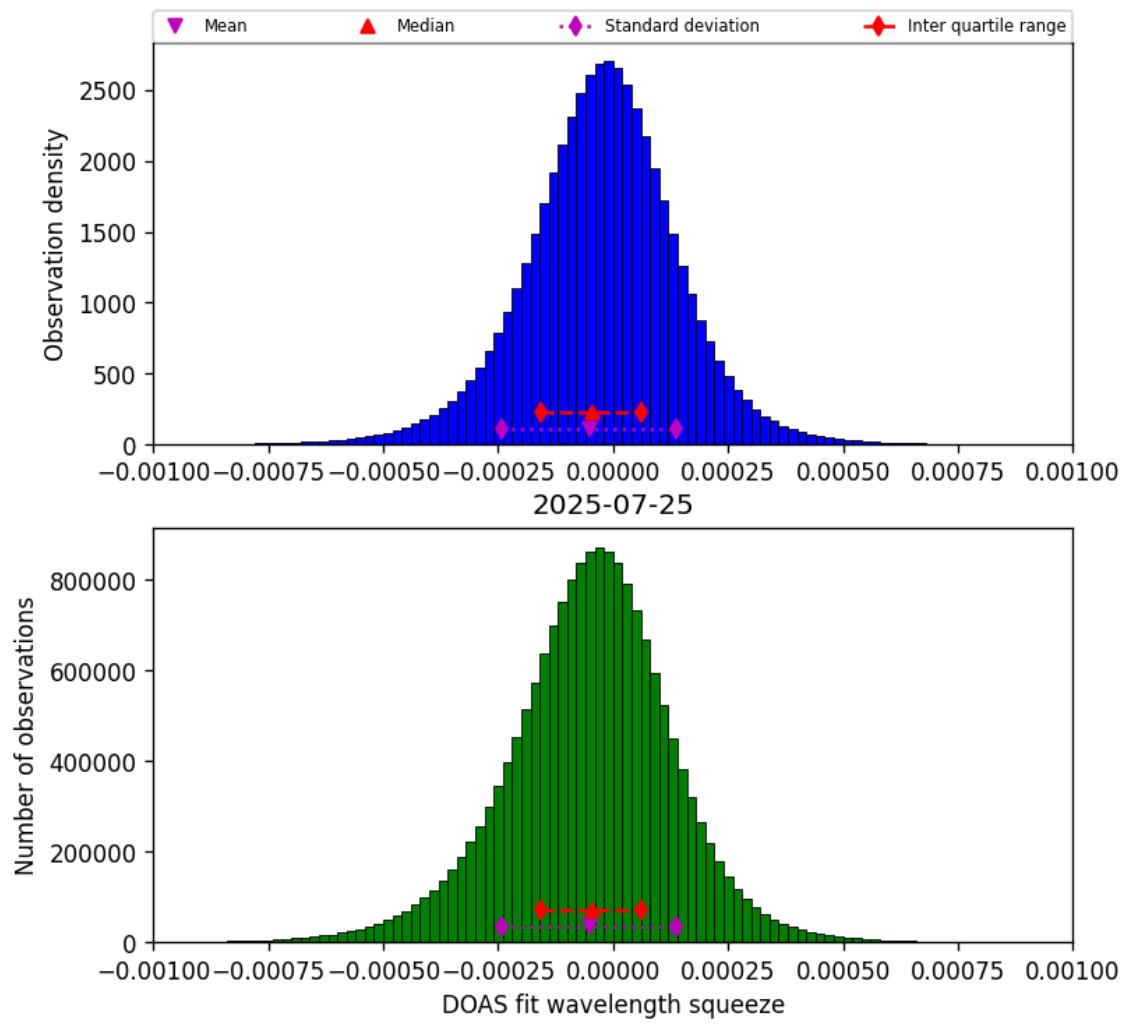
Figure 78: Histogram of “DOAS fit wavelength squeeze” for 2025-07-25 to 2025-07-26
