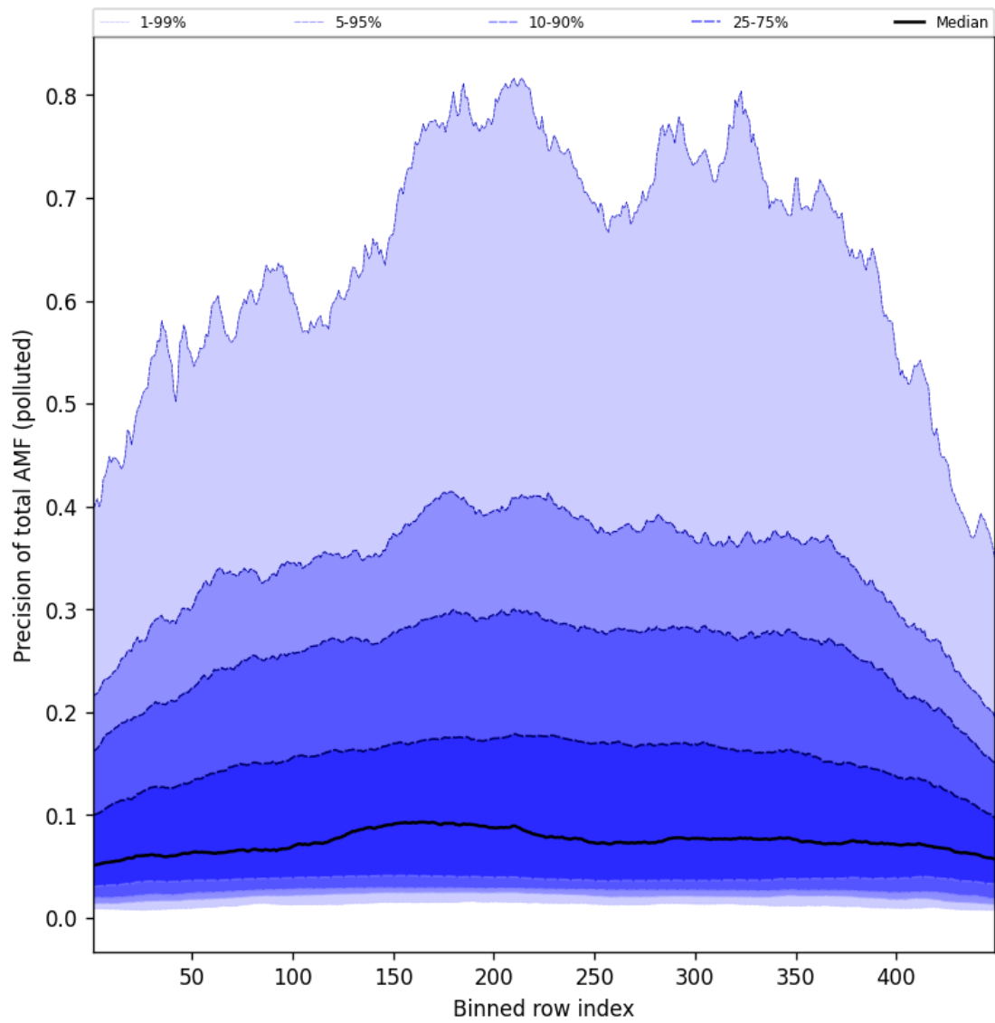
Figure 108: Along track statistics of “Precision of total AMF (polluted)” for 2025-07-25 to 2025-07-26
