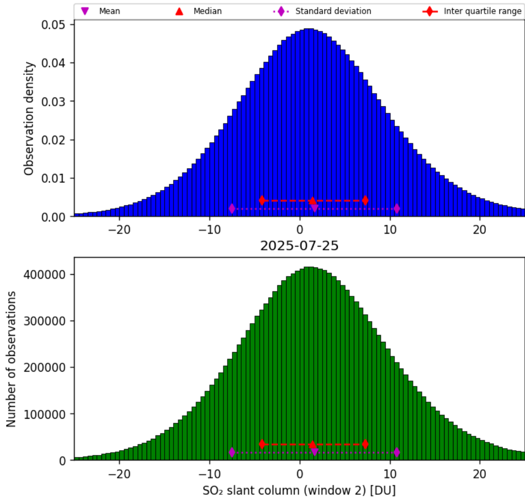
Figure 67: Histogram of “SO 2 slant column (window 2)” for 2025-07-25 to 2025-07-26
