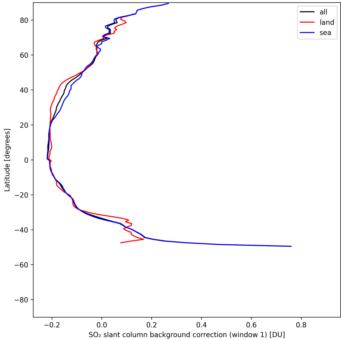
Figure 39: Zonal average of “SO 2 slant column background correction (window 1)” for 2025-07-25 to 2025-07-26.
