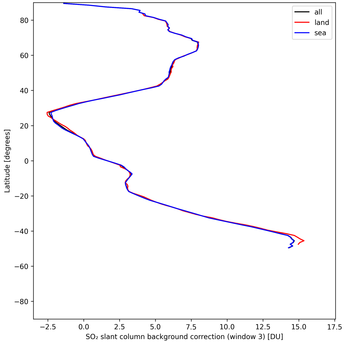
Figure 47: Zonal average of “SO 2 slant column background correction (window 3)” for 2025-07-25 to 2025-07-26.
