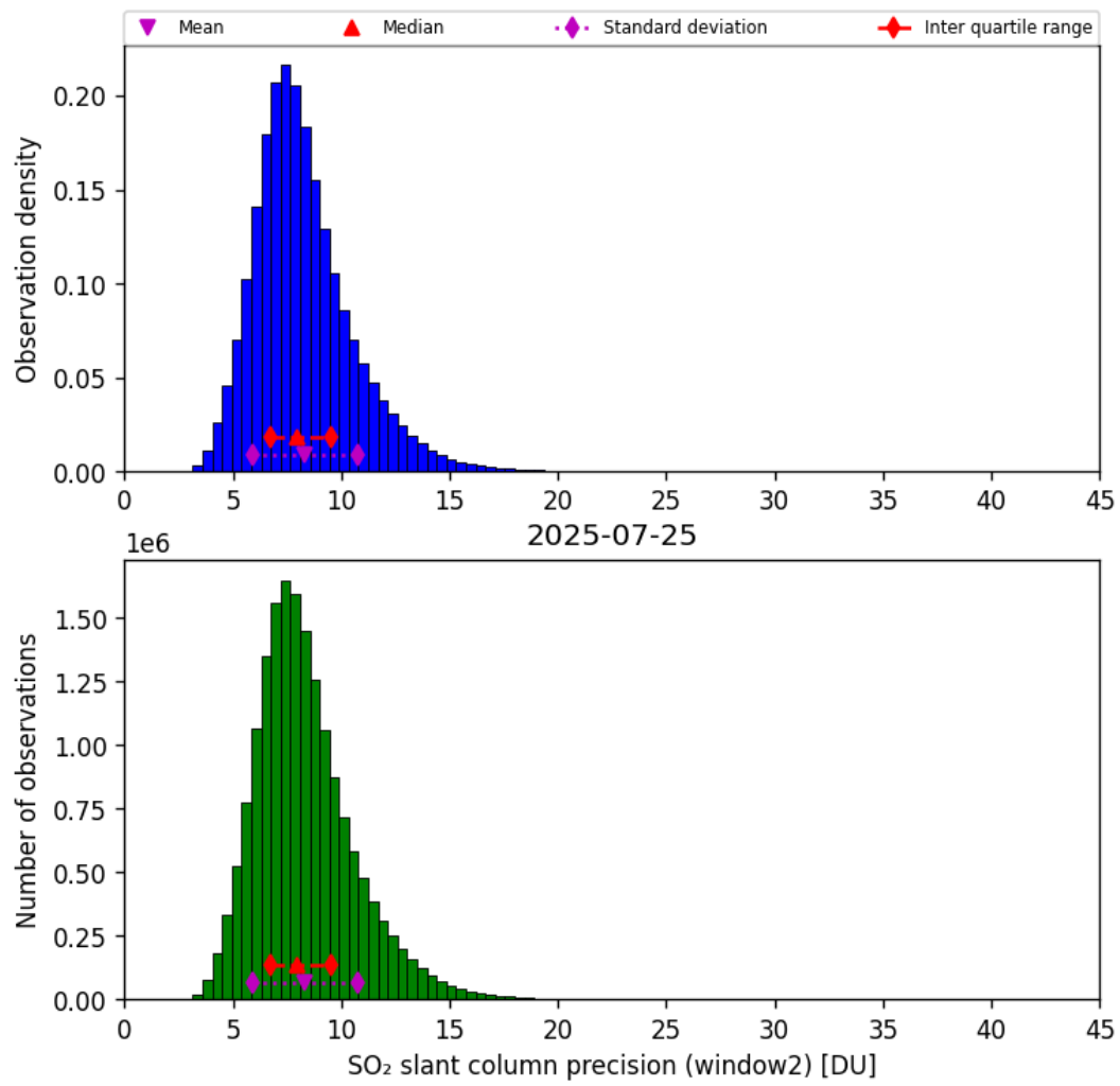
Figure 68: Histogram of “SO 2 slant column precision (window2)” for 2025-07-25 to 2025-07-26
