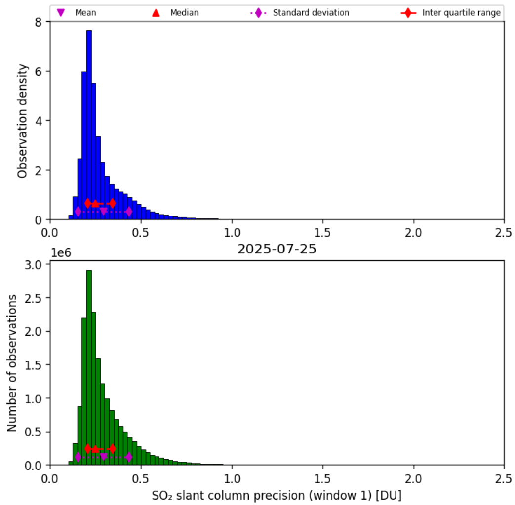
Figure 64: Histogram of “SO 2 slant column precision (window 1)” for 2025-07-25 to 2025-07-26
