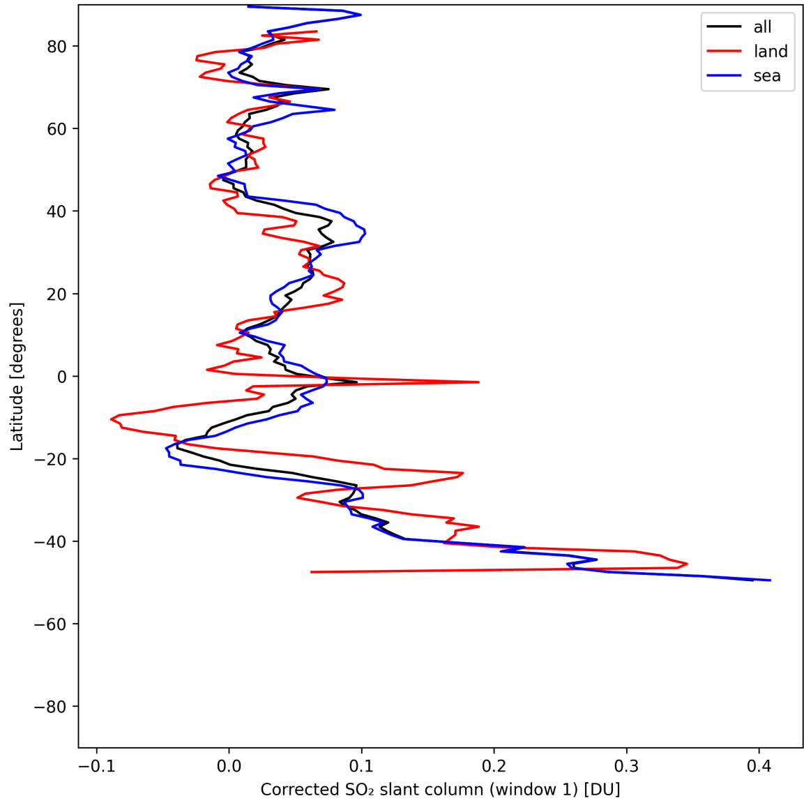
Figure 38: Zonal average of “Corrected SO 2 slant column (window 1)” for 2025-07-25 to 2025-07-26.
