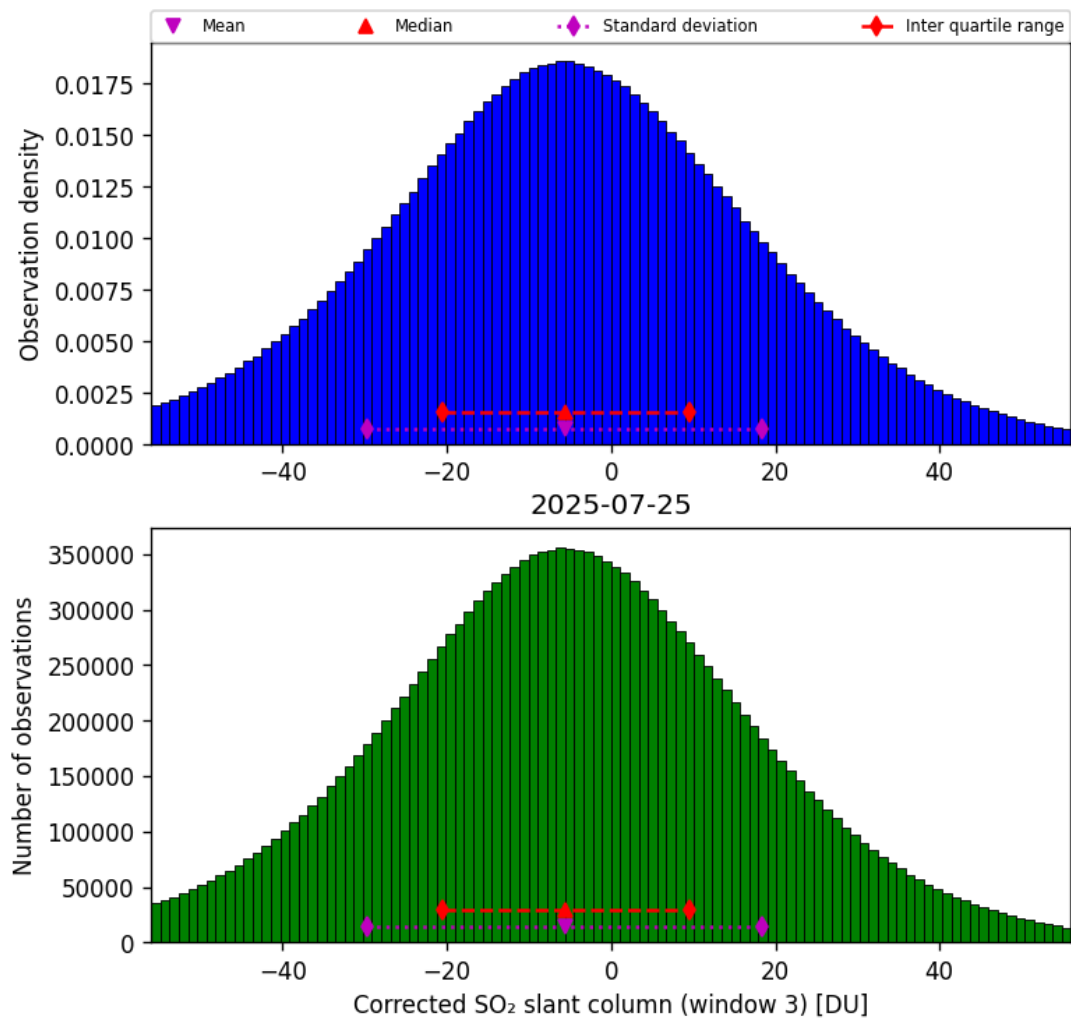
Figure 73: Histogram of “Corrected SO 2 slant column (window 3)” for 2025-07-25 to 2025-07-26
