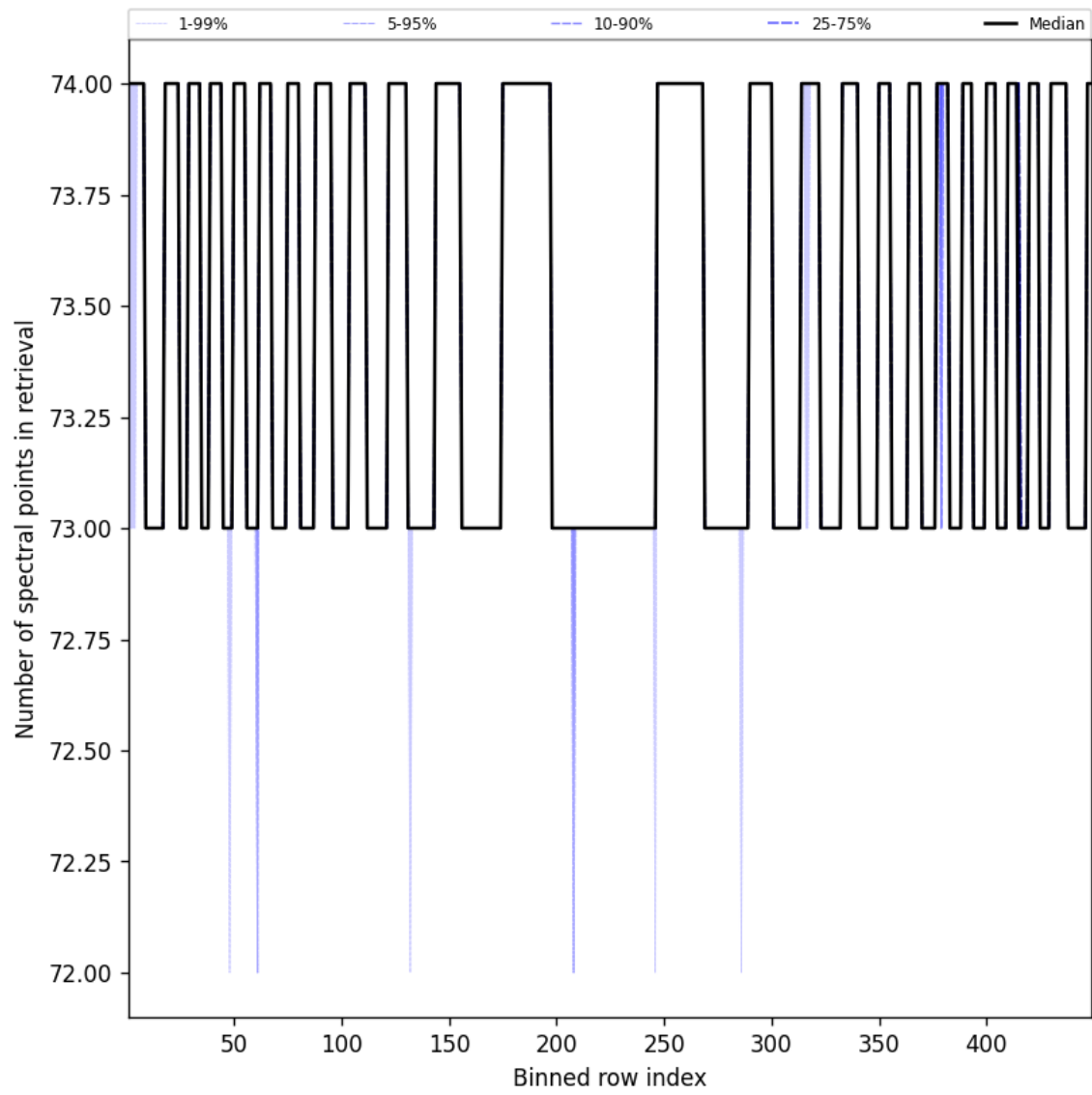
Figure 110: Along track statistics of “Number of spectral points in retrieval” for 2025-07-25 to 2025-07-26
