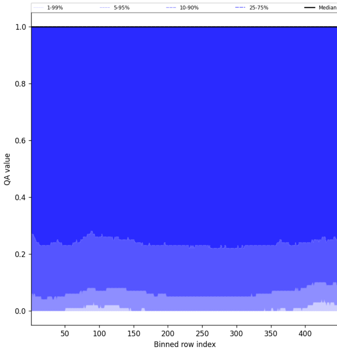
Figure 84: Along track statistics of “QA value” for 2025-07-25 to 2025-07-26
