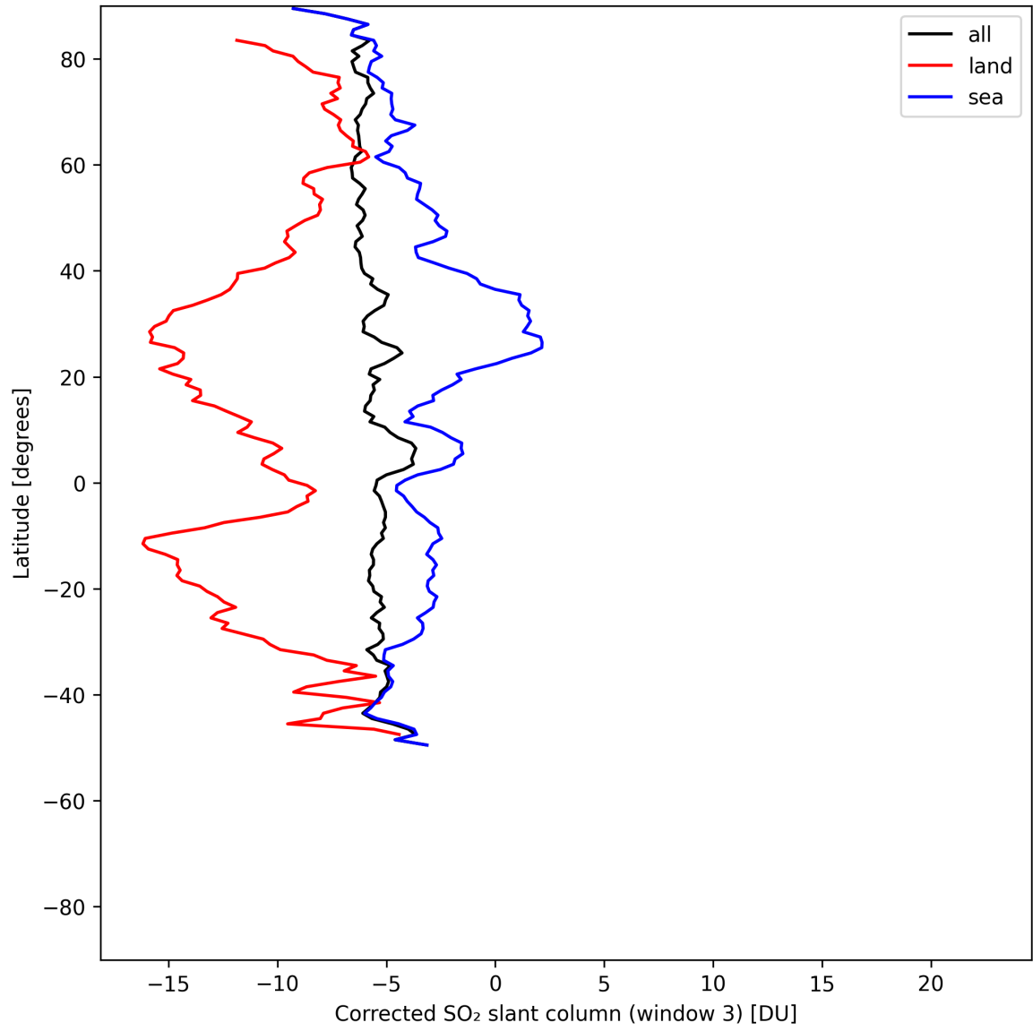
Figure 46: Zonal average of “Corrected SO 2 slant column (window 3)” for 2025-07-25 to 2025-07-26.
