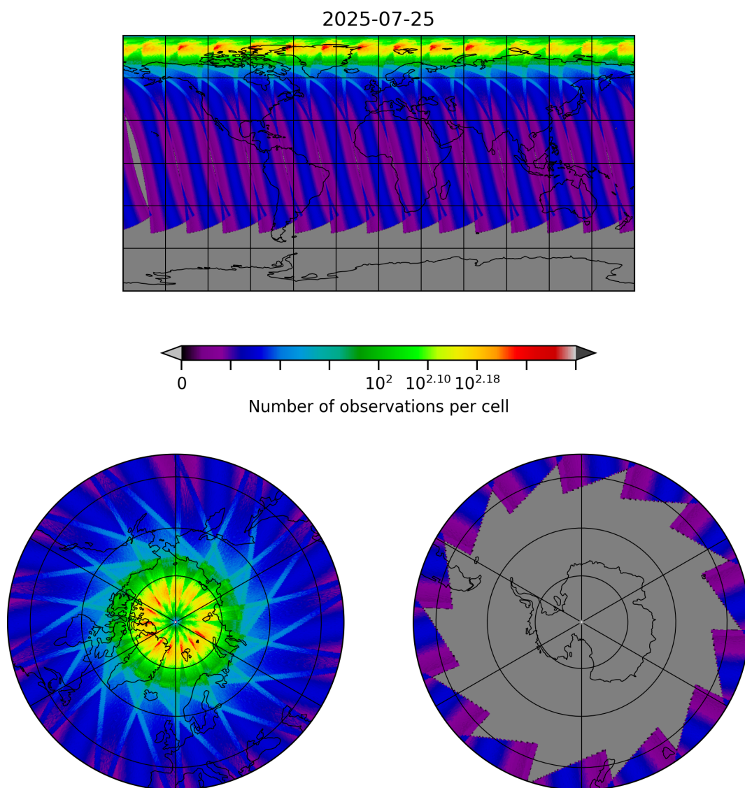
Figure 29: Map of the number of observations for 2025-07-25 to 2025-07-26
