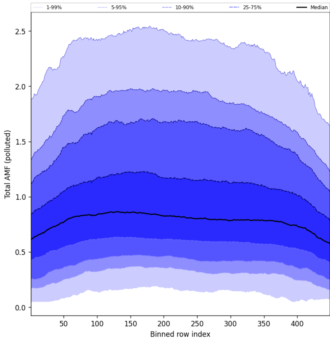
Figure 107: Along track statistics of “Total AMF (polluted)” for 2025-07-25 to 2025-07-26
