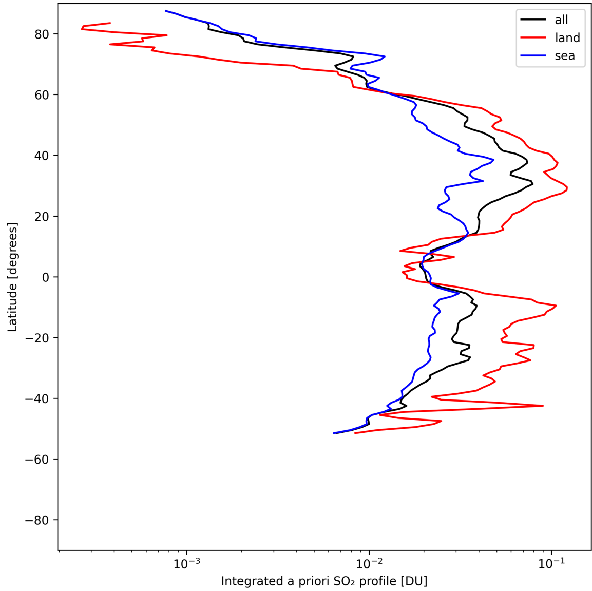
Figure 49: Zonal average of “Integrated a priori SO 2 profile” for 2025-08-02 to 2025-08-03.
