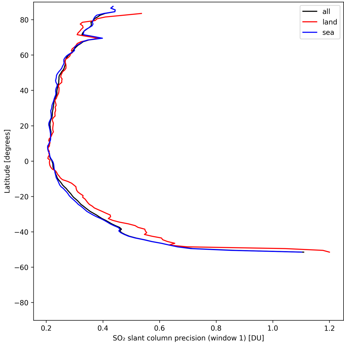
Figure 37: Zonal average of “SO 2 slant column precision (window 1)” for 2025-08-02 to 2025-08-03.
