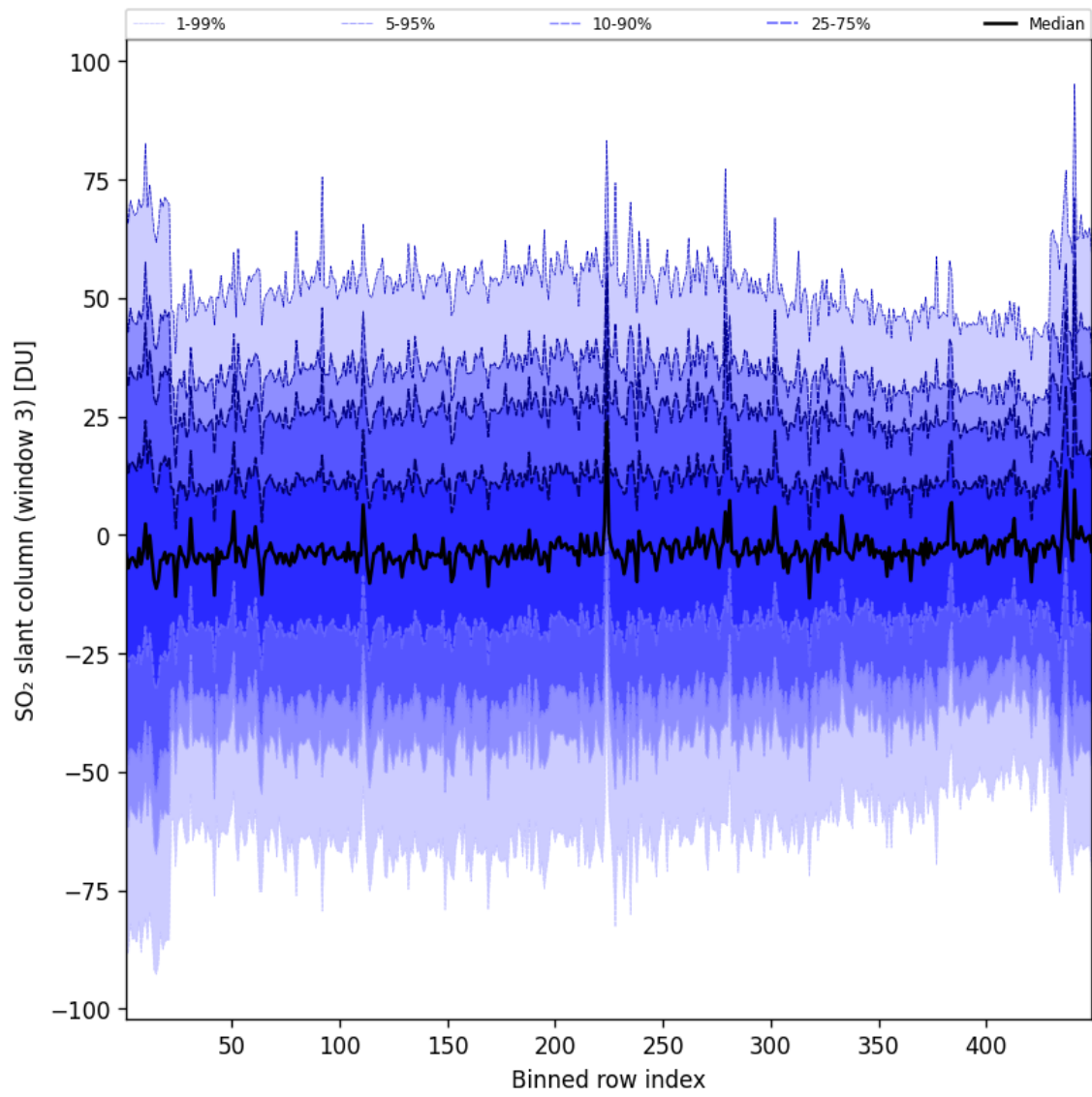
Figure 98: Along track statistics of “SO 2 slant column (window 3)” for 2025-08-02 to 2025-08-03
