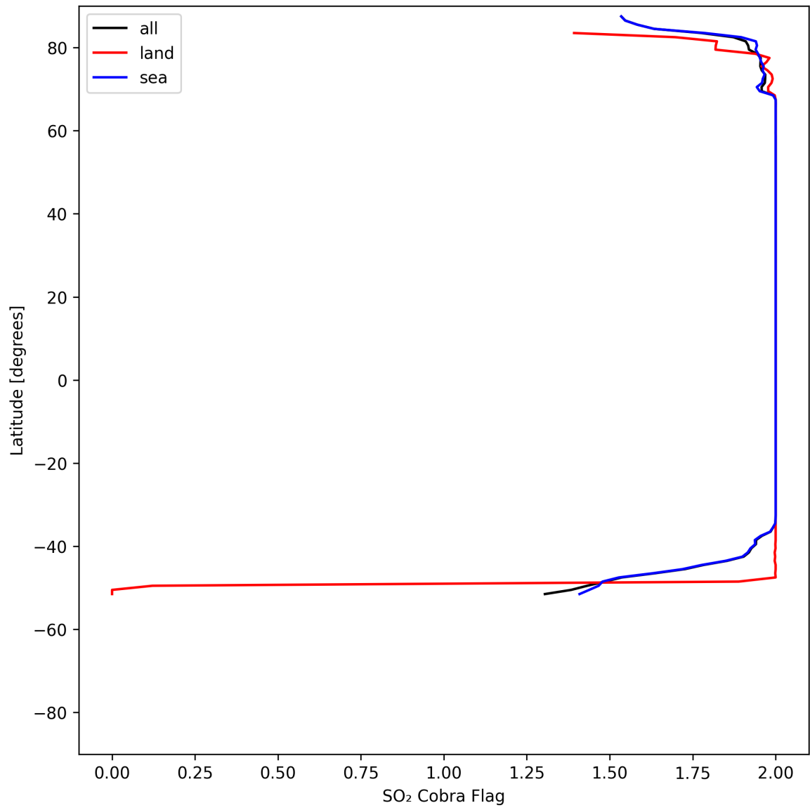
Figure 48: Zonal average of "SO 2 Cobra Flag" for 2025-08-02 to 2025-08-03.
