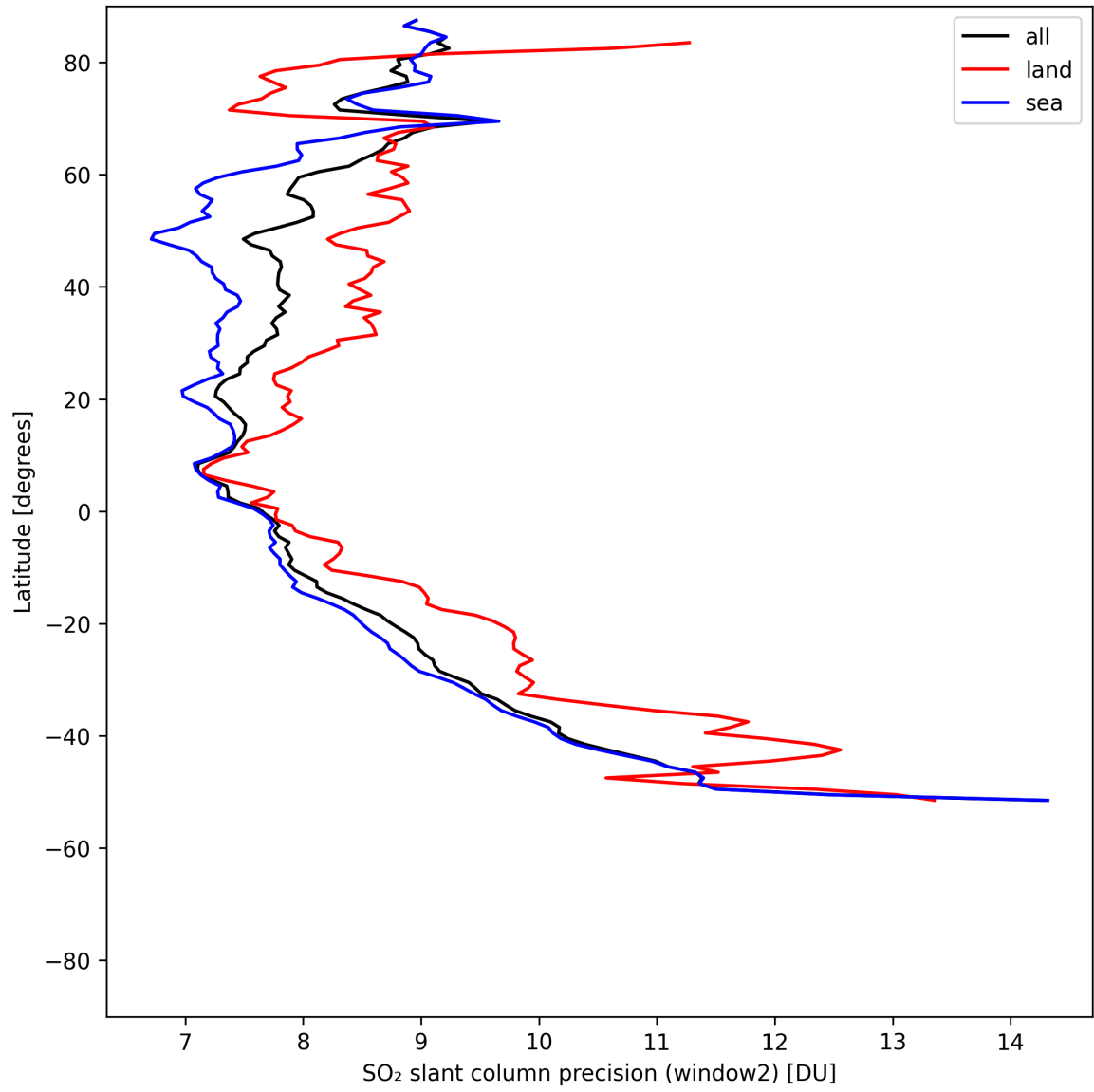
Figure 41: Zonal average of “SO 2 slant column precision (window2)” for 2025-08-02 to 2025-08-03.
