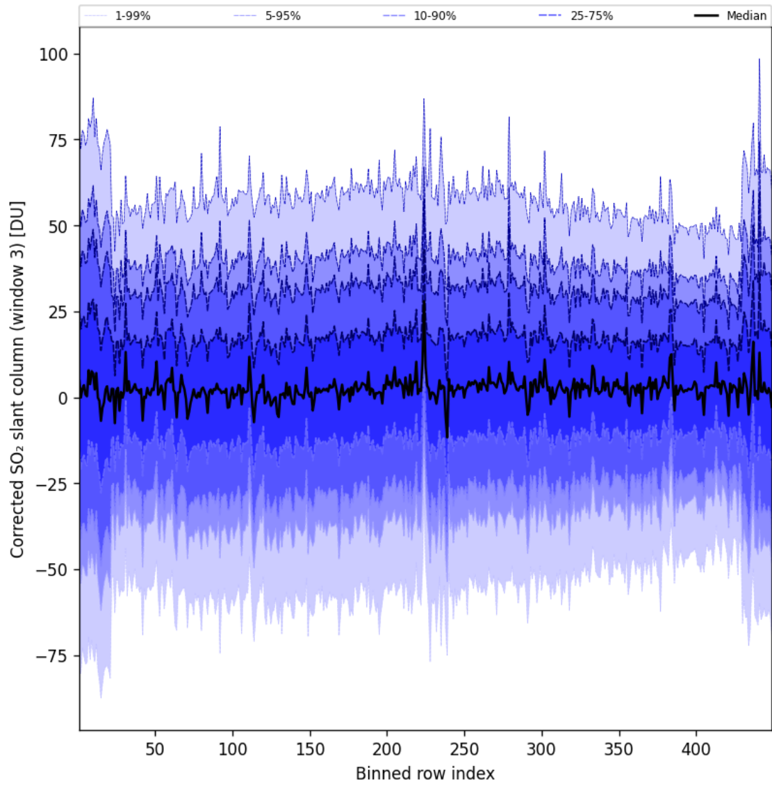
Figure 100: Along track statistics of “Corrected SO 2 slant column (window 3)” for 2025-08-02 to 2025-08-03
