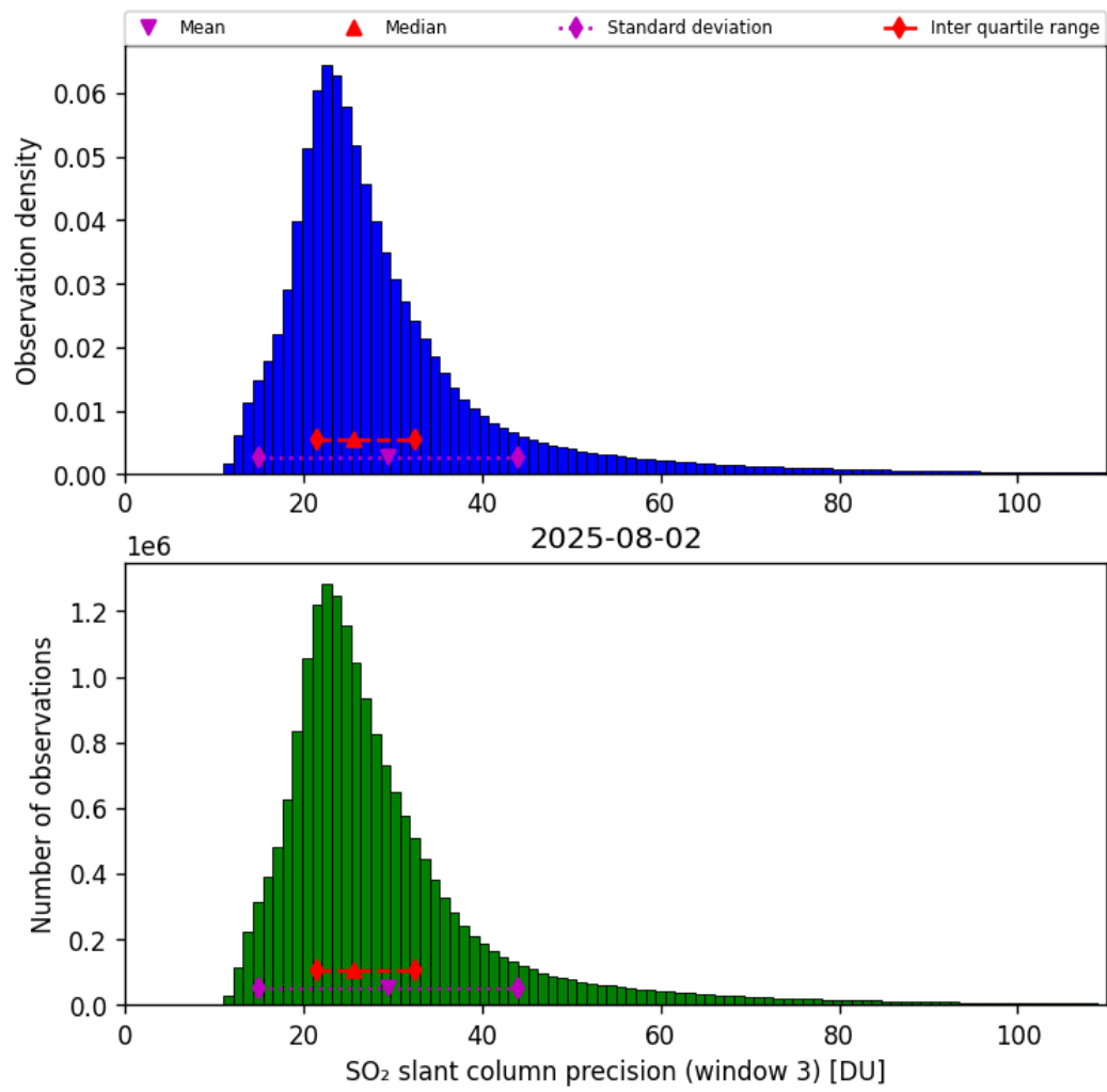
Figure 72: Histogram of “SO 2 slant column precision (window 3)” for 2025-08-02 to 2025-08-03
