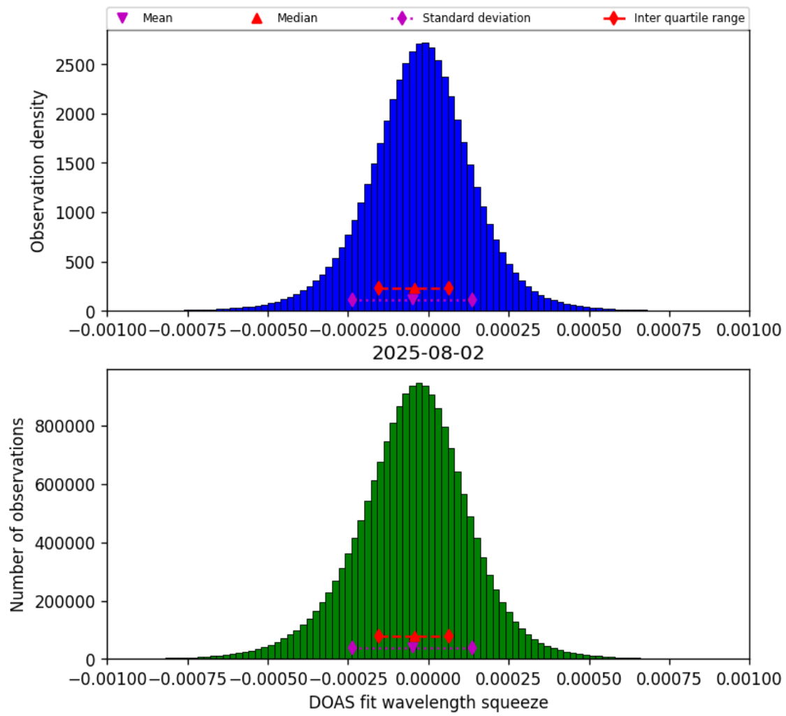
Figure 78: Histogram of “DOAS fit wavelength squeeze” for 2025-08-02 to 2025-08-03
