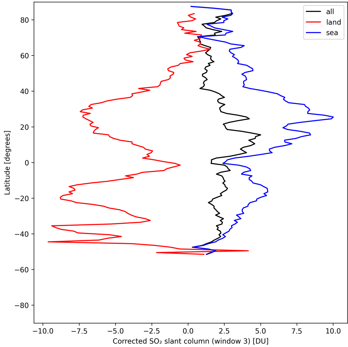
Figure 46: Zonal average of “Corrected SO 2 slant column (window 3)” for 2025-08-02 to 2025-08-03.
