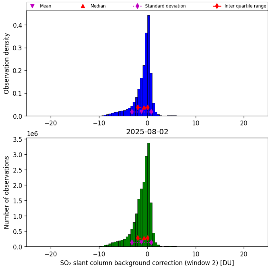
Figure 70: Histogram of “SO 2 slant column background correction (window 2)” for 2025-08-02 to 2025-08-03
