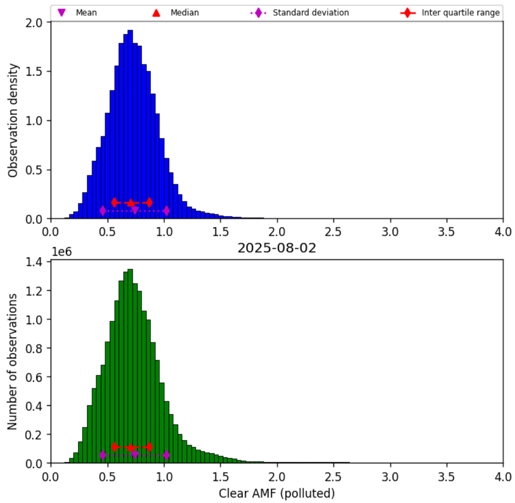
Figure 82: Histogram of “Clear AMF (polluted)” for 2025-08-02 to 2025-08-03
