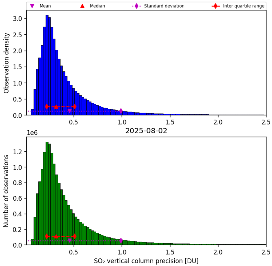
Figure 59: Histogram of “SO 2 vertical column precision” for 2025-08-02 to 2025-08-03
