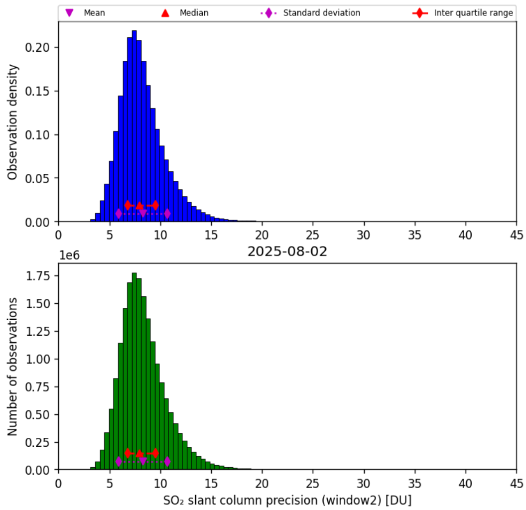
Figure 68: Histogram of “SO 2 slant column precision (window2)” for 2025-08-02 to 2025-08-03
