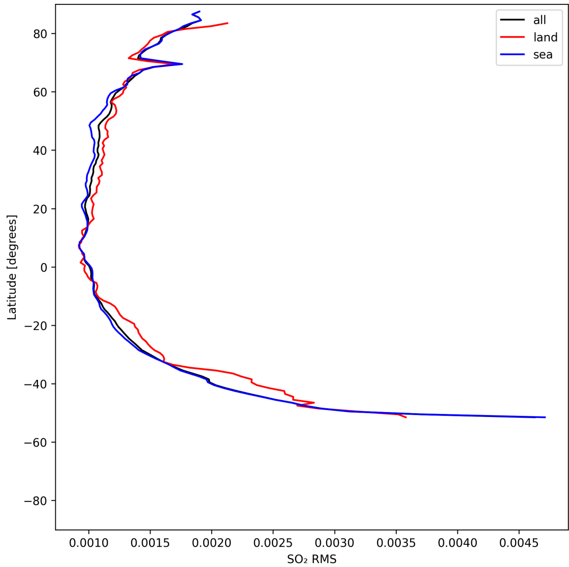
Figure 52: Zonal average of “SO 2 RMS” for 2025-08-02 to 2025-08-03.
