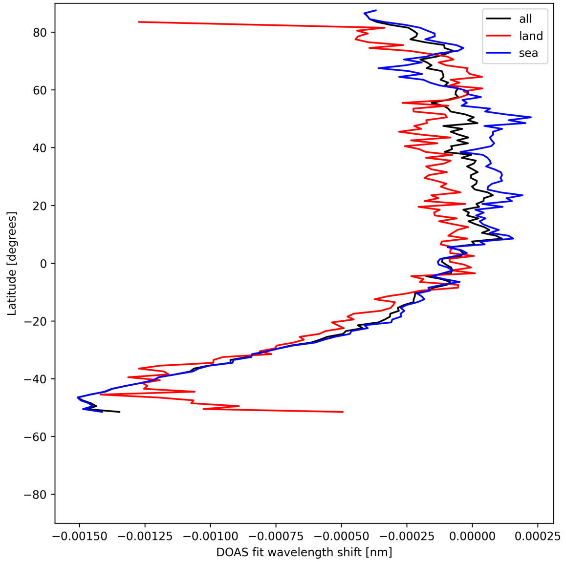
Figure 50: Zonal average of “DOAS fit wavelength shift” for 2025-08-02 to 2025-08-03.
