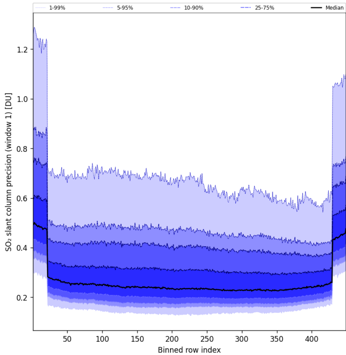
Figure 91: Along track statistics of “SO 2 slant column precision (window 1)” for 2025-08-02 to 2025-08-03
