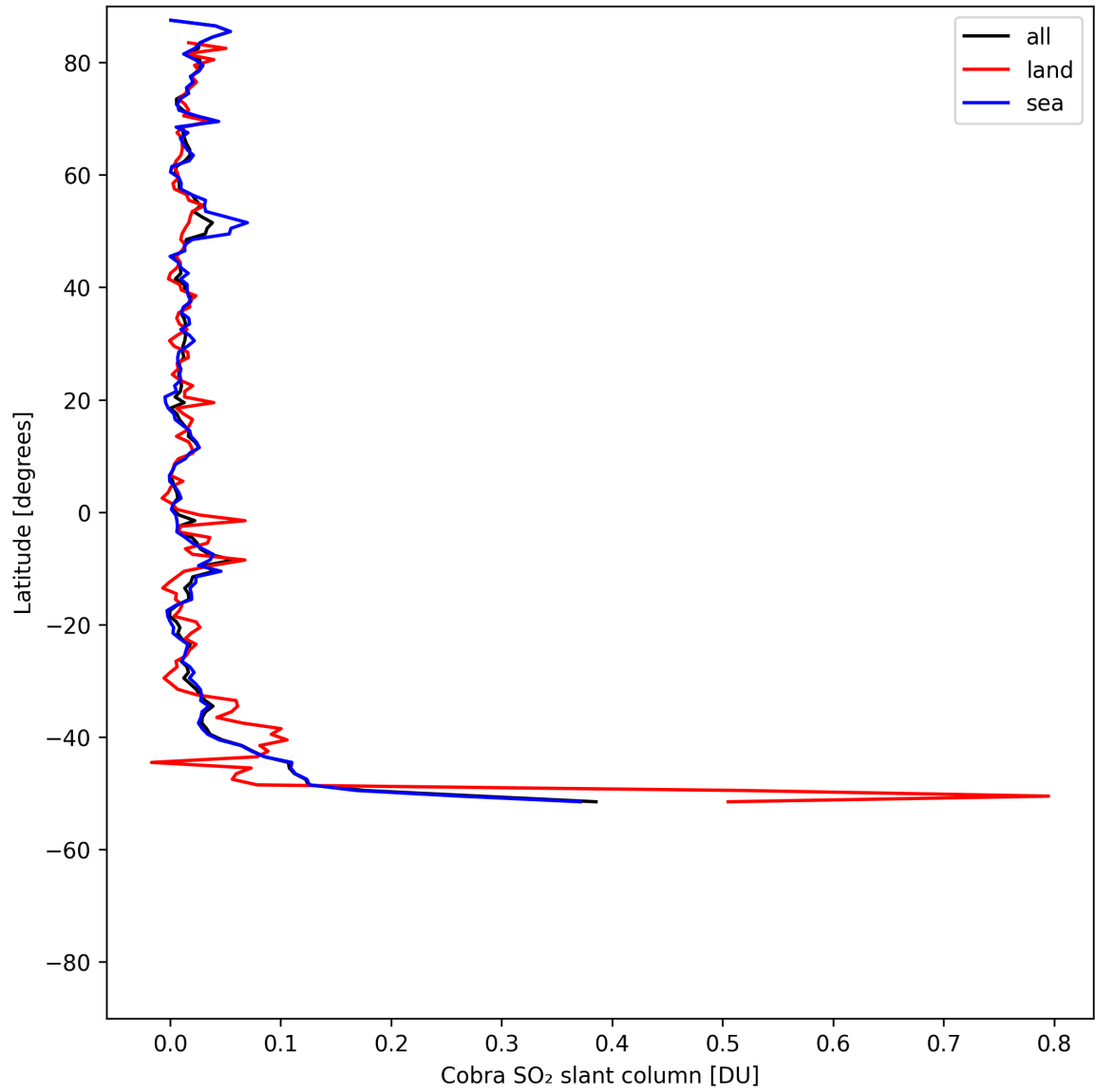
Figure 34: Zonal average of “Cobra SO 2 slant column” for 2025-08-02 to 2025-08-03.
