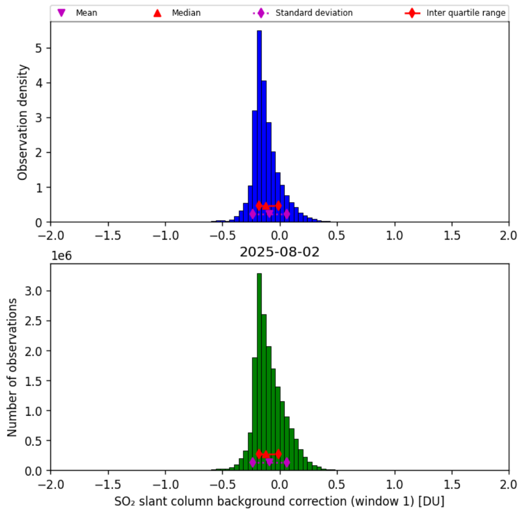
Figure 66: Histogram of “SO 2 slant column background correction (window 1)” for 2025-08-02 to 2025-08-03
