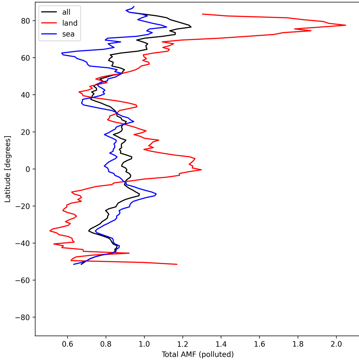
Figure 53: Zonal average of “Total AMF (polluted)” for 2025-08-02 to 2025-08-03.
