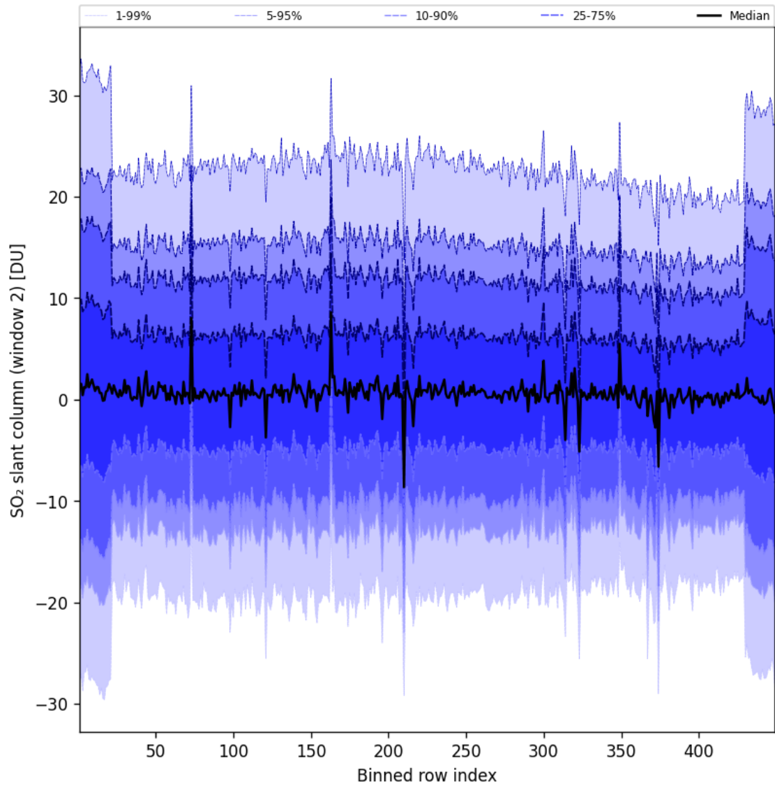
Figure 94: Along track statistics of “SO 2 slant column (window 2)” for 2025-08-02 to 2025-08-03
