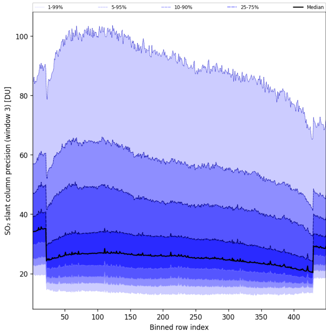
Figure 99: Along track statistics of “SO 2 slant column precision (window 3)” for 2025-08-02 to 2025-08-03
