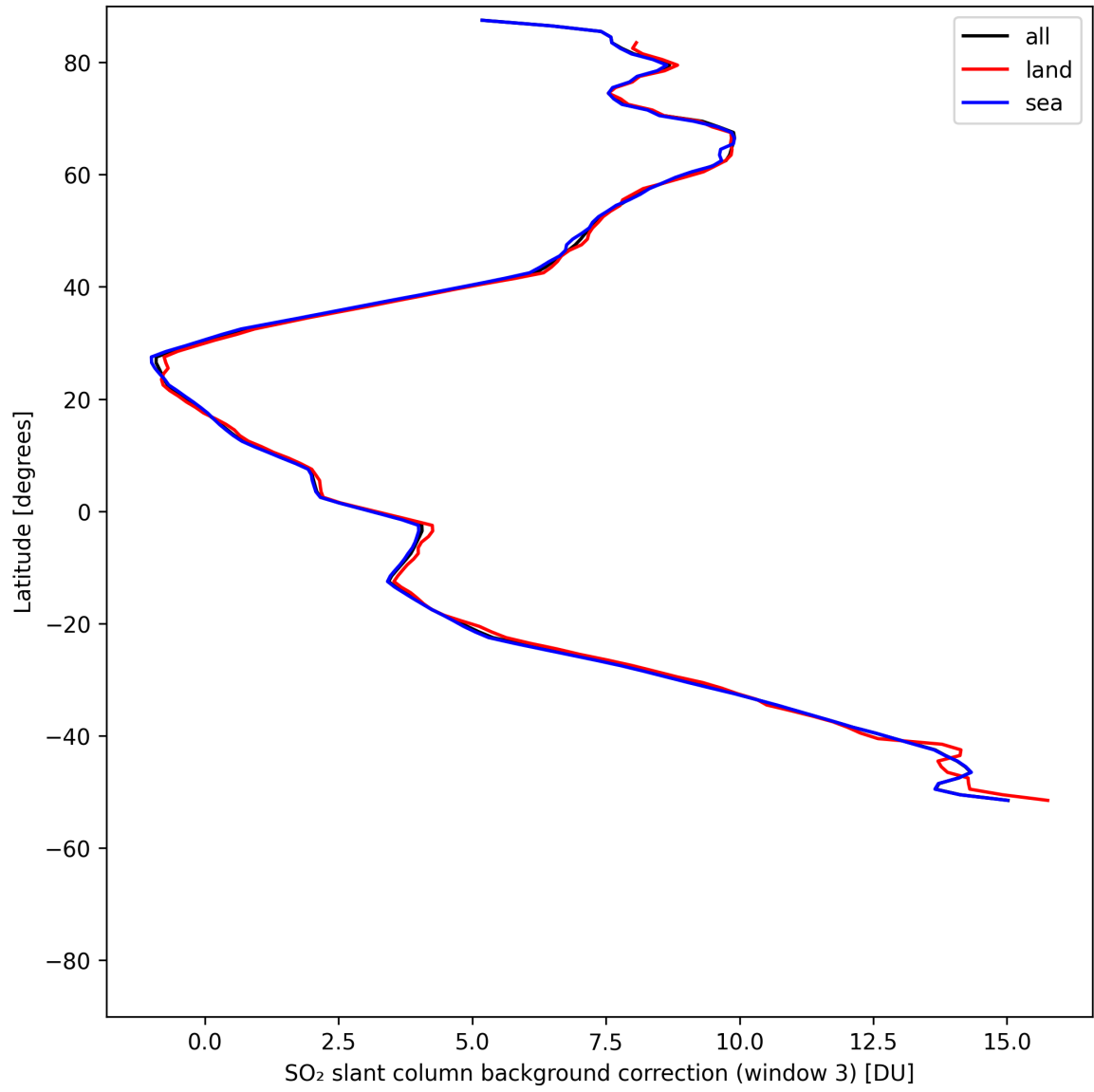
Figure 47: Zonal average of “SO 2 slant column background correction (window 3)” for 2025-08-02 to 2025-08-03.
