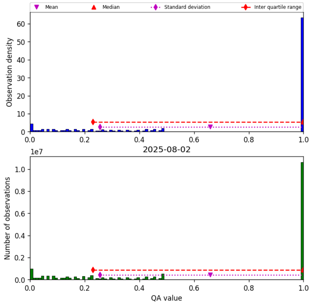
Figure 57: Histogram of “QA value” for 2025-08-02 to 2025-08-03
