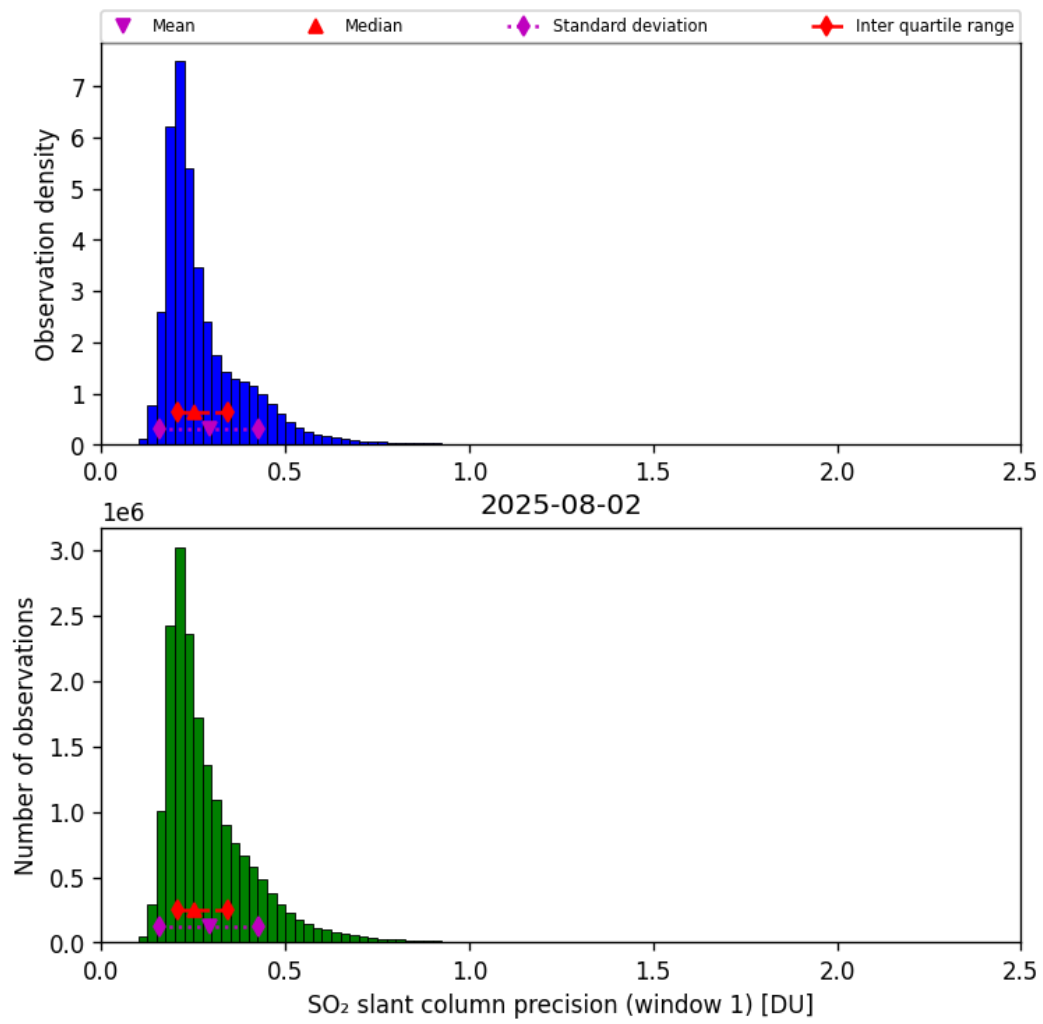
Figure 64: Histogram of “SO 2 slant column precision (window 1)” for 2025-08-02 to 2025-08-03
