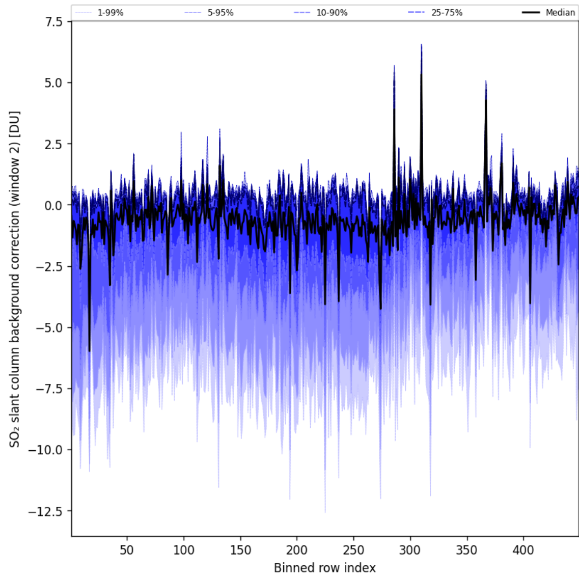
Figure 97: Along track statistics of “SO 2 slant column background correction (window 2)” for 2025-08-02 to 2025-08-03
