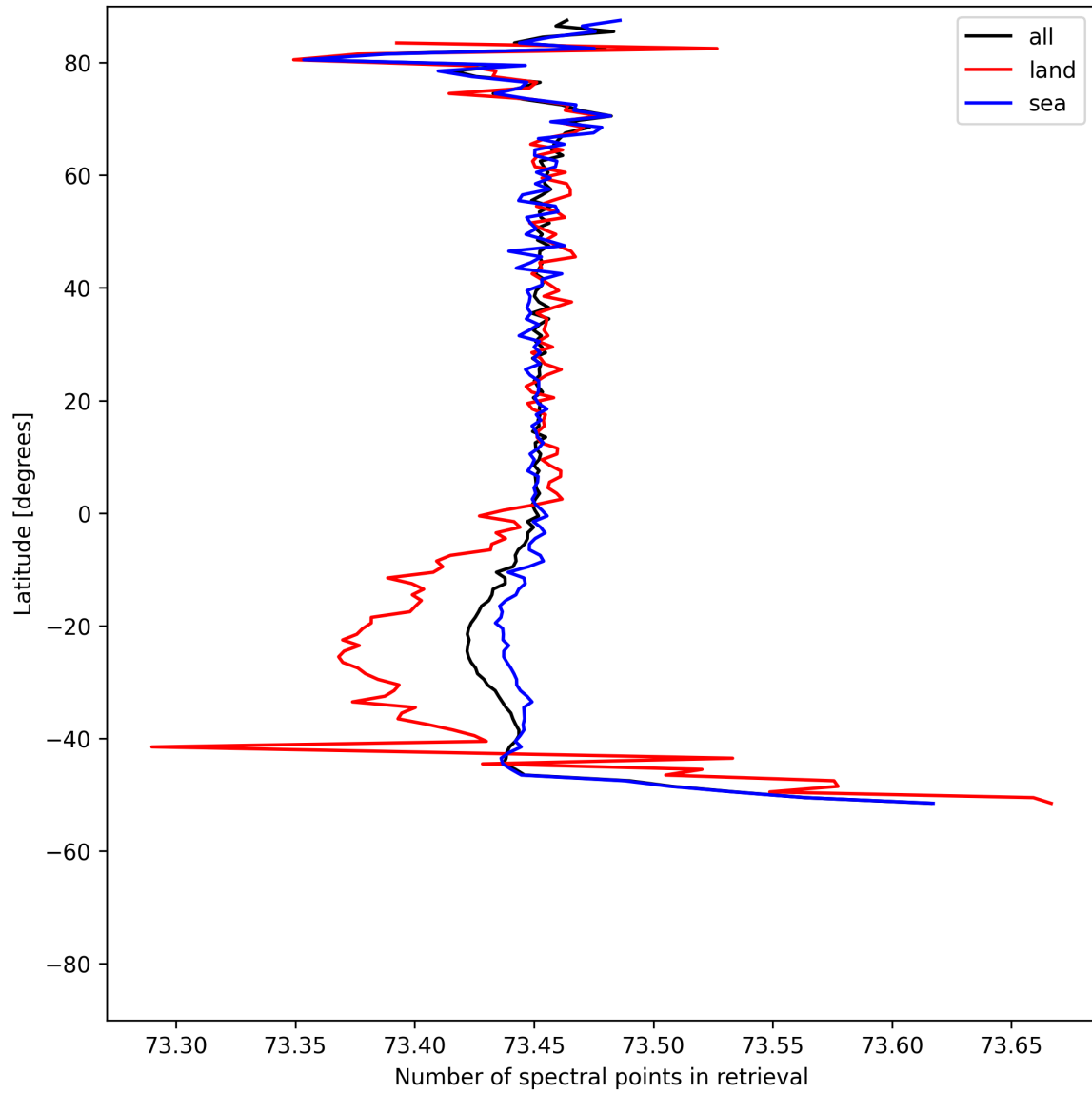
Figure 56: Zonal average of “Number of spectral points in retrieval” for 2025-08-02 to 2025-08-03.
