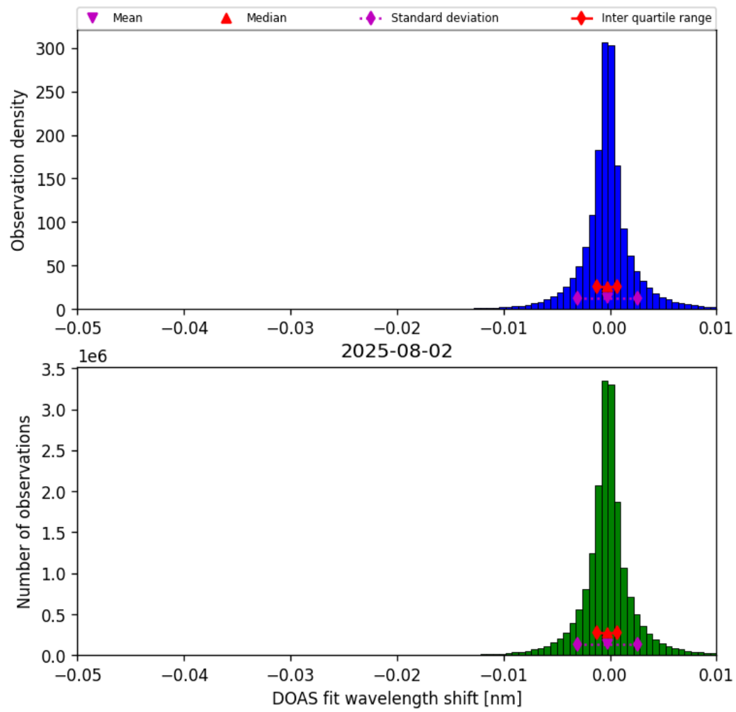
Figure 77: Histogram of “DOAS fit wavelength shift” for 2025-08-02 to 2025-08-03
