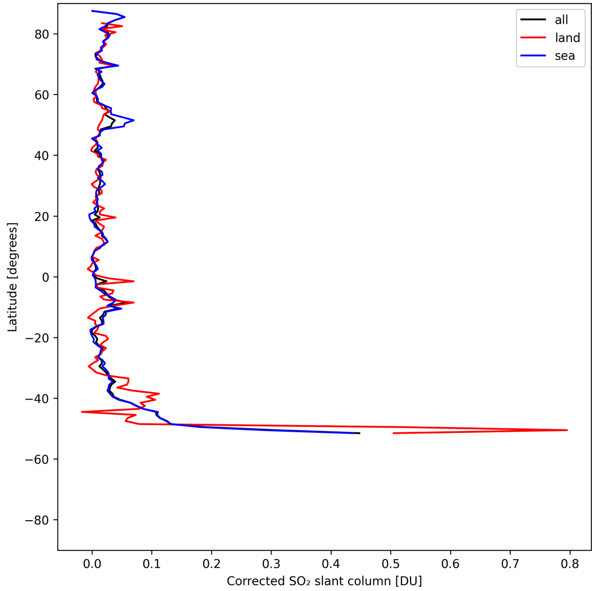
Figure 33: Zonal average of “Corrected SO 2 slant column” for 2025-08-02 to 2025-08-03.
