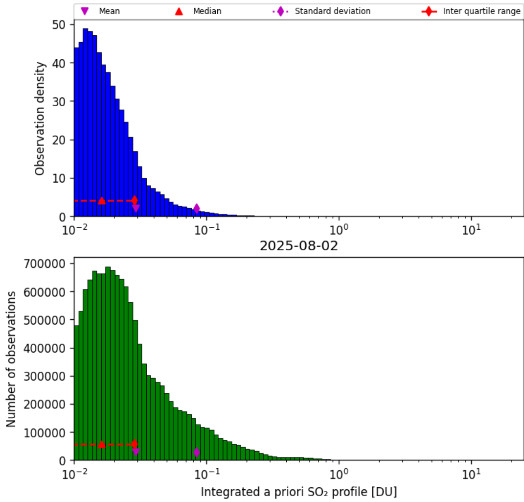
Figure 76: Histogram of “Integrated a priori SO 2 profile” for 2025-08-02 to 2025-08-03
