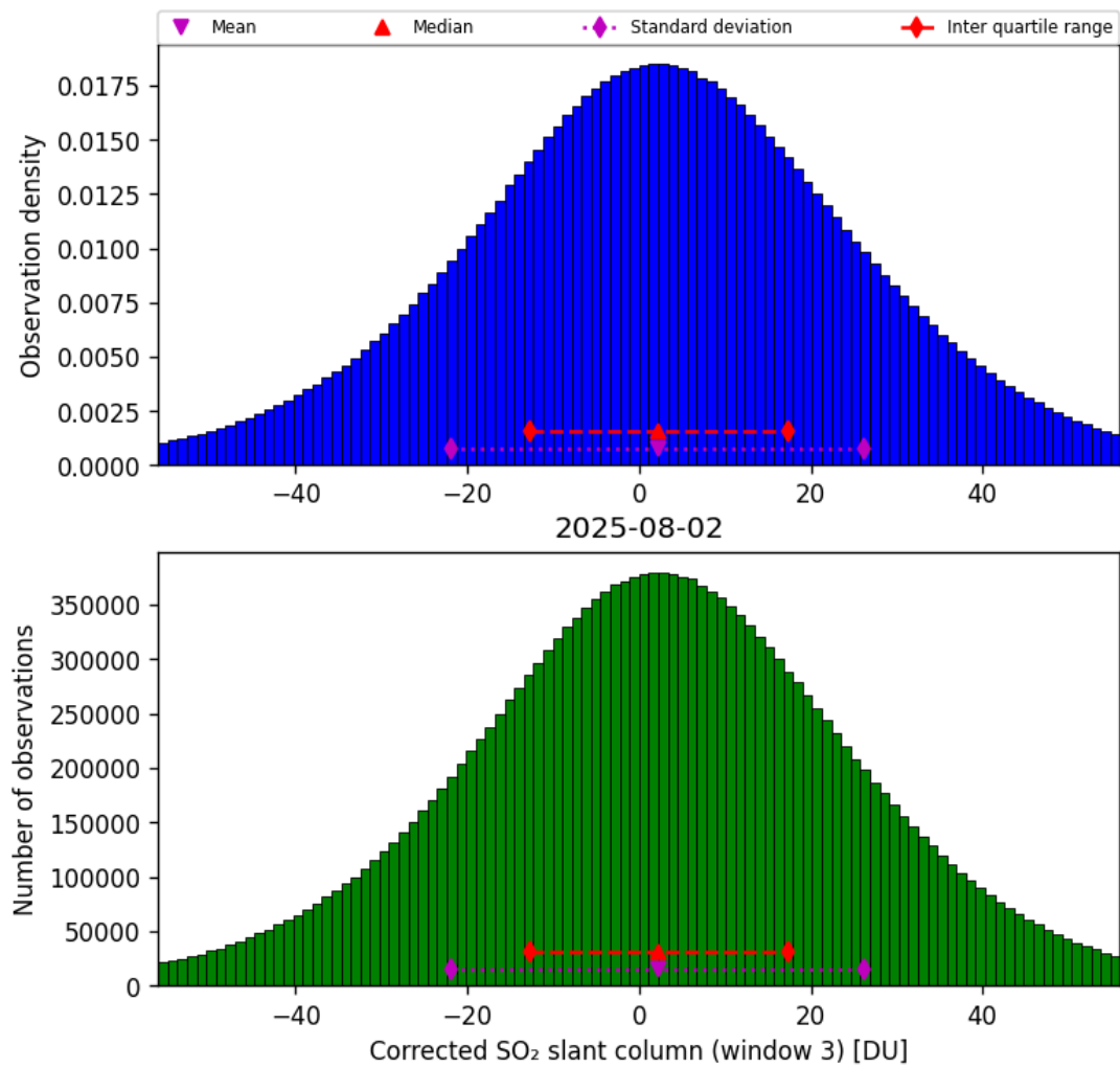
Figure 73: Histogram of “Corrected SO 2 slant column (window 3)” for 2025-08-02 to 2025-08-03
