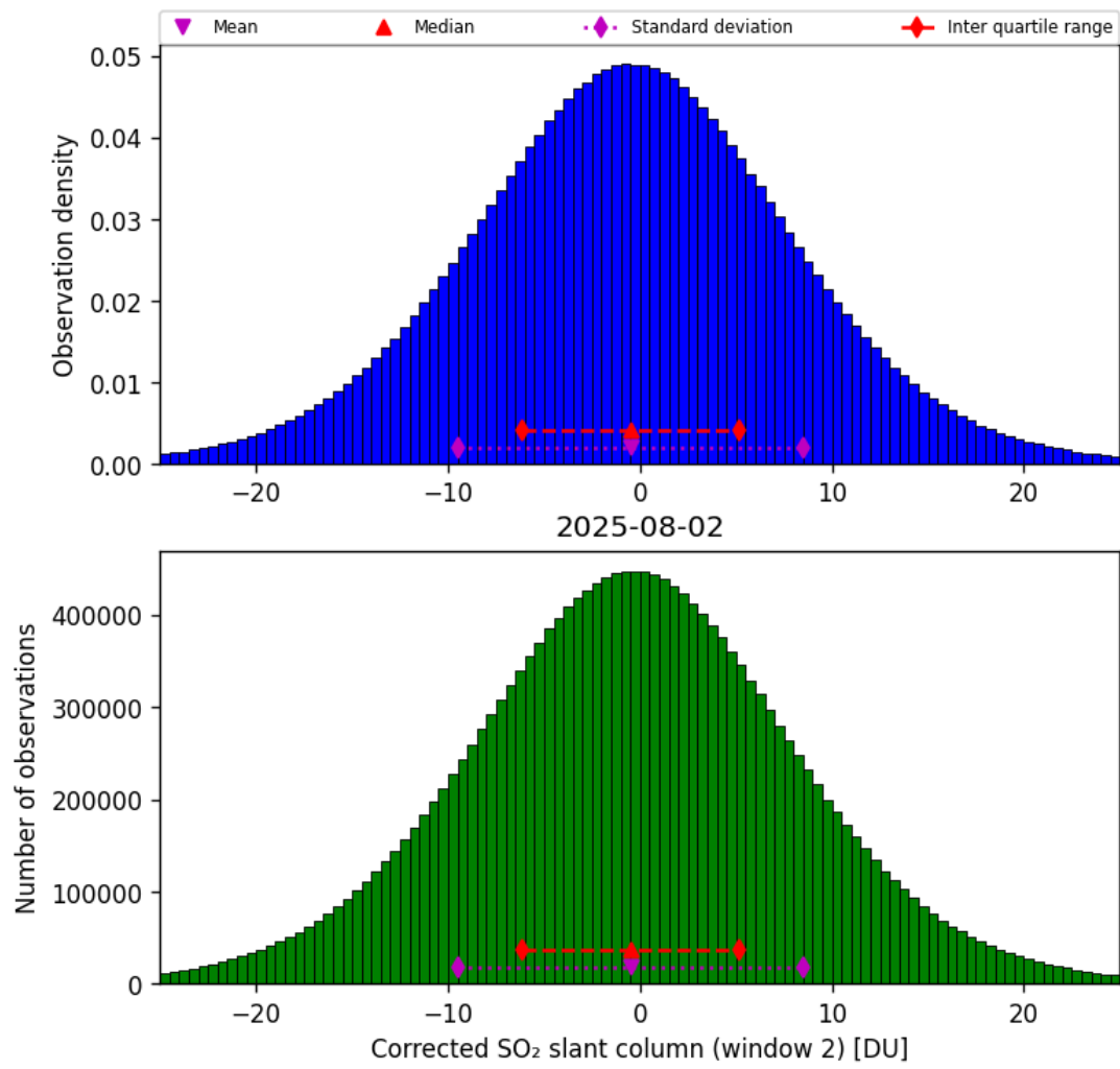
Figure 69: Histogram of “Corrected SO 2 slant column (window 2)” for 2025-08-02 to 2025-08-03
