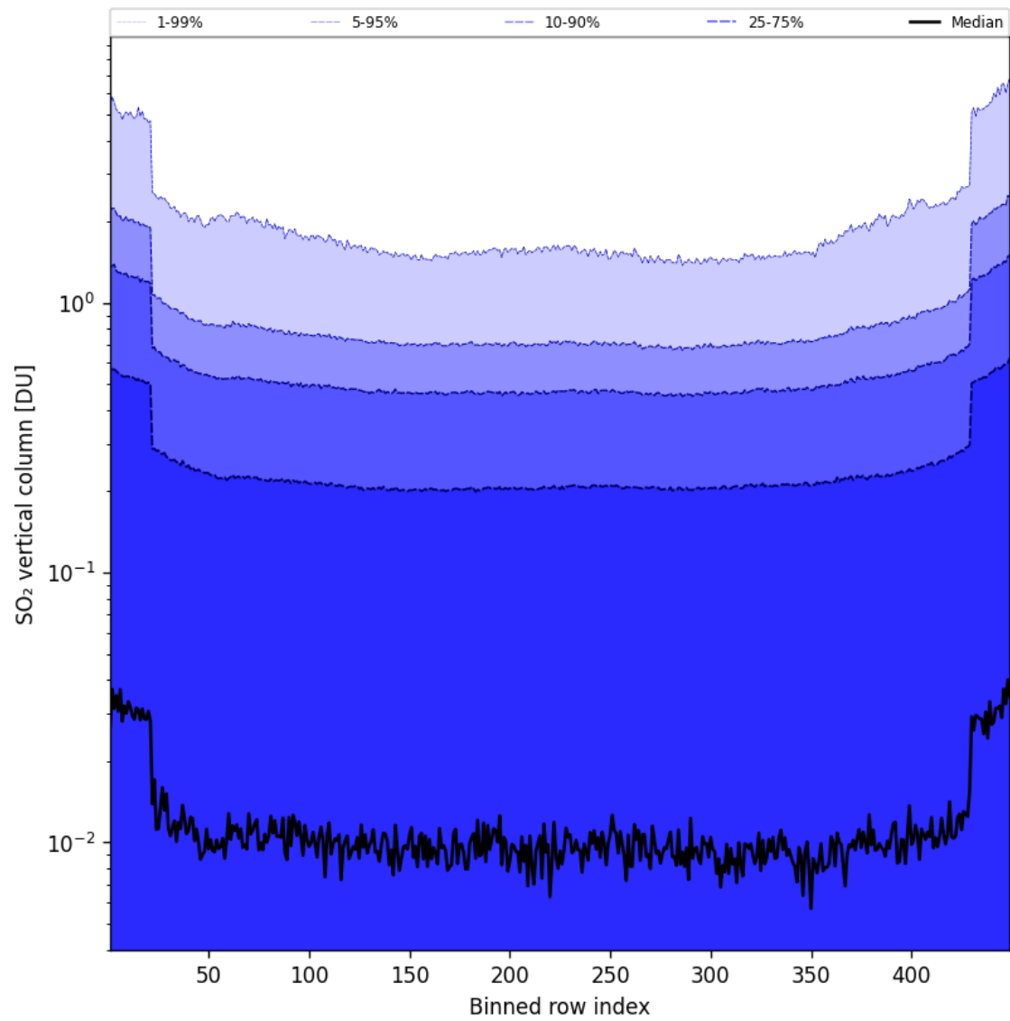
Figure 85: Along track statistics of “SO 2 vertical column” for 2025-08-02 to 2025-08-03
