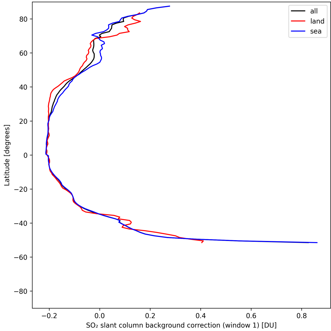
Figure 39: Zonal average of “SO 2 slant column background correction (window 1)” for 2025-08-02 to 2025-08-03.
