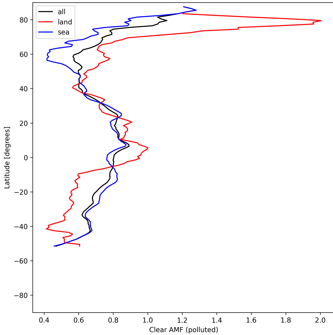
Figure 55: Zonal average of “Clear AMF (polluted)” for 2025-08-02 to 2025-08-03.
