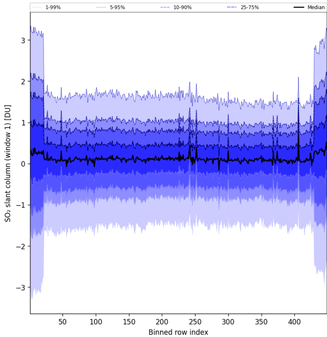
Figure 90: Along track statistics of “SO 2 slant column (window 1)” for 2025-08-02 to 2025-08-03
