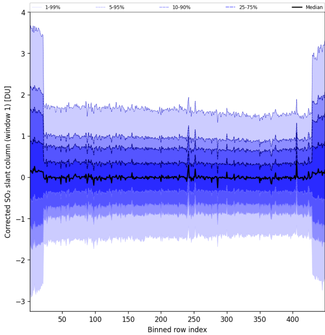
Figure 92: Along track statistics of “Corrected SO 2 slant column (window 1)” for 2025-08-02 to 2025-08-03
