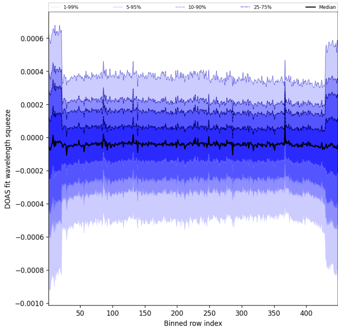
Figure 105: Along track statistics of “DOAS fit wavelength squeeze” for 2025-08-02 to 2025-08-03
