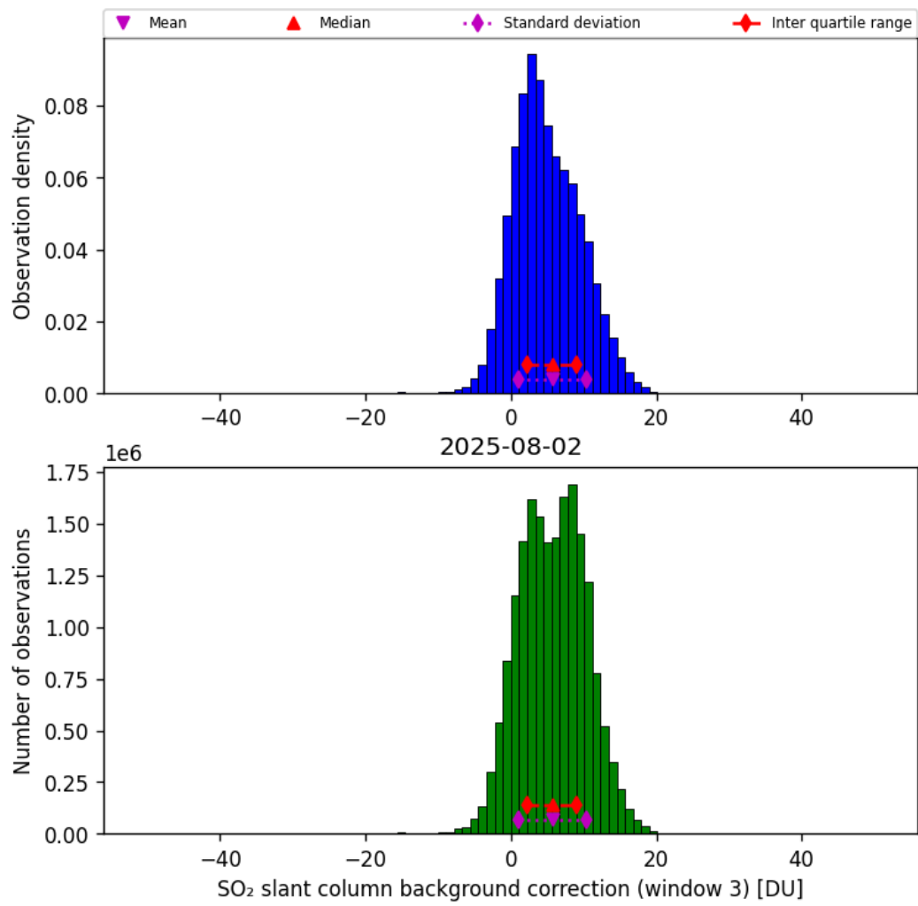
Figure 74: Histogram of “SO 2 slant column background correction (window 3)” for 2025-08-02 to 2025-08-03
