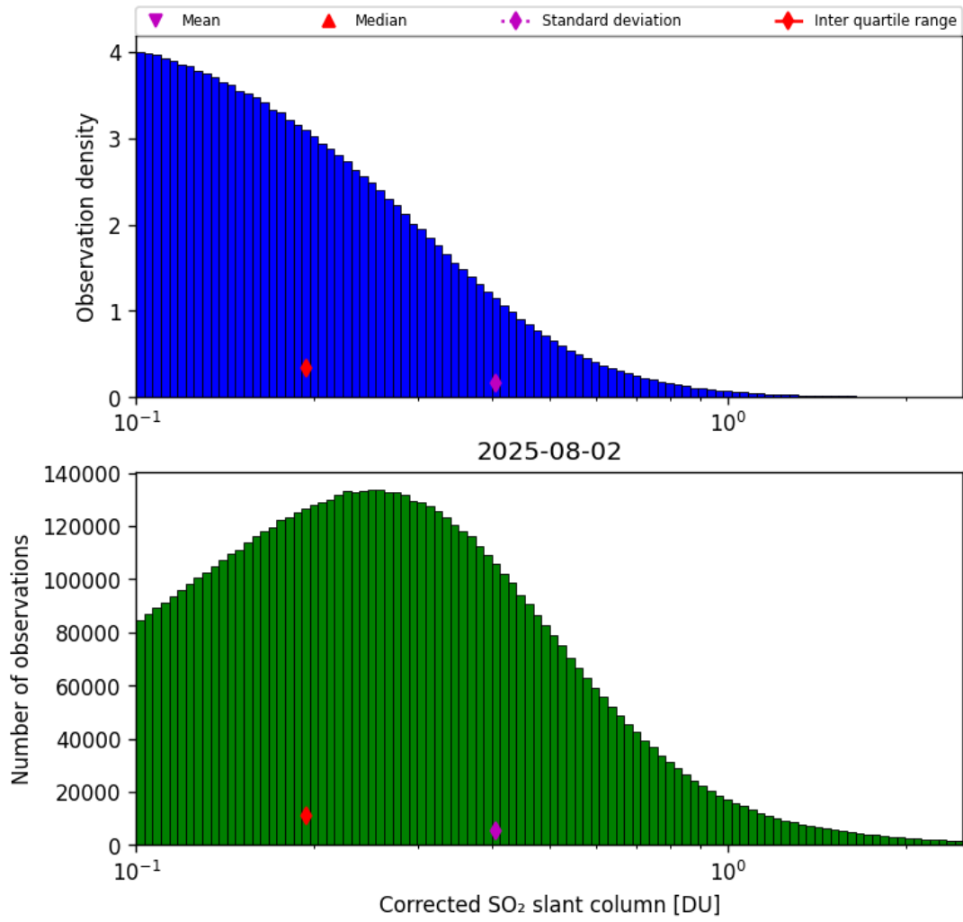
Figure 60: Histogram of “Corrected SO 2 slant column” for 2025-08-02 to 2025-08-03
