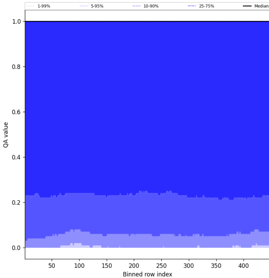
Figure 84: Along track statistics of “QA value” for 2025-08-02 to 2025-08-03
