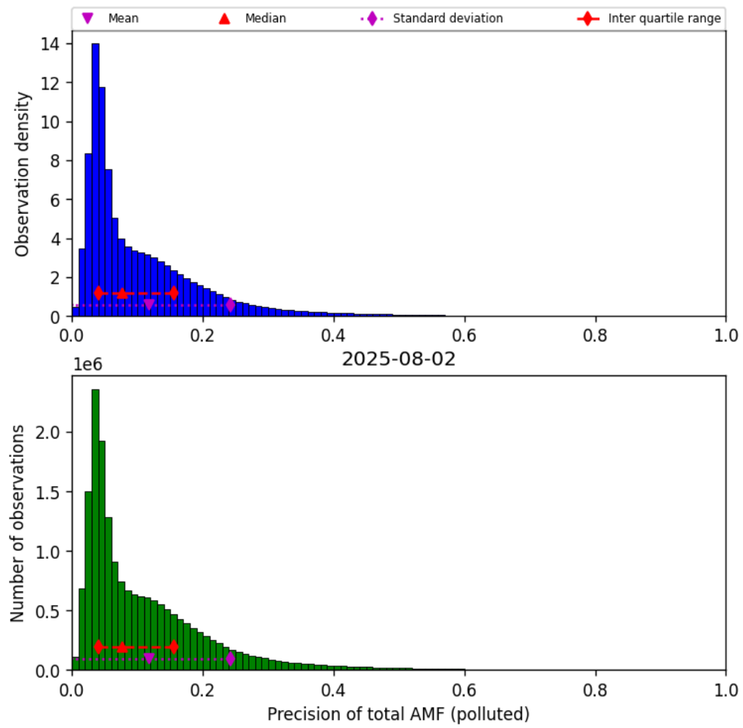
Figure 81: Histogram of “Precision of total AMF (polluted)” for 2025-08-02 to 2025-08-03
