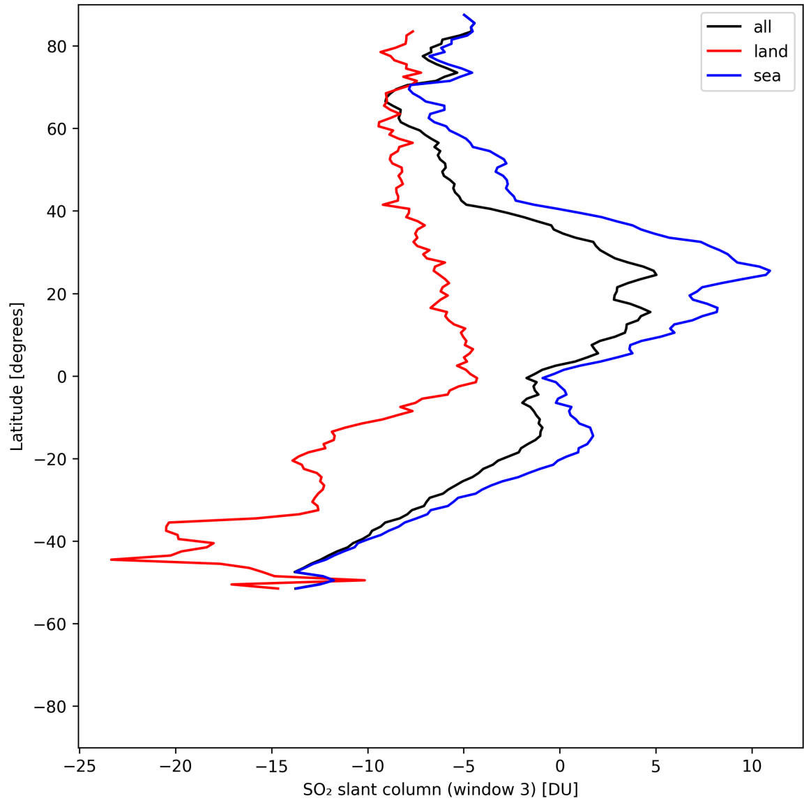
Figure 44: Zonal average of “SO 2 slant column (window 3)” for 2025-08-02 to 2025-08-03.
