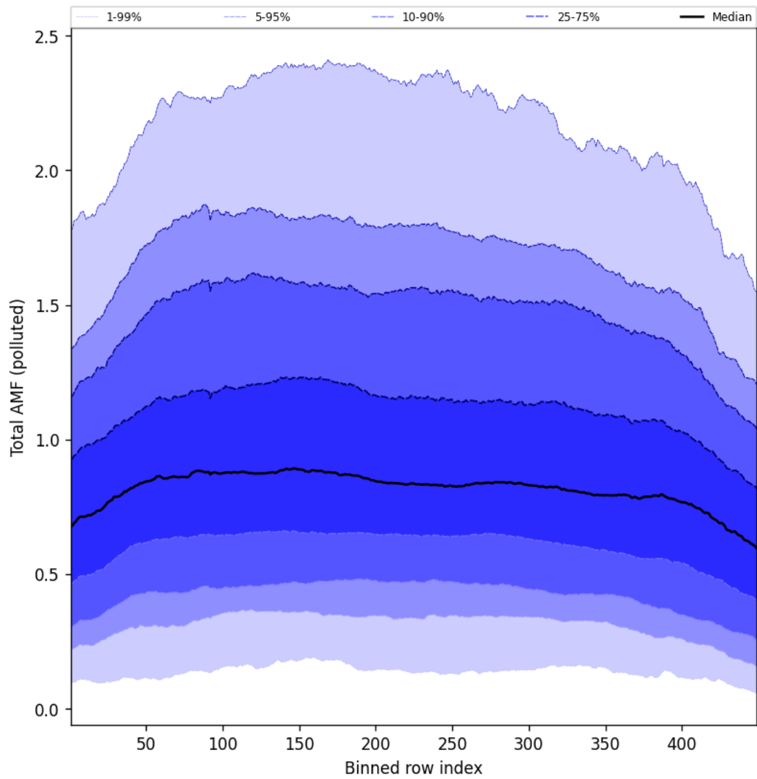
Figure 107: Along track statistics of “Total AMF (polluted)” for 2025-08-02 to 2025-08-03
