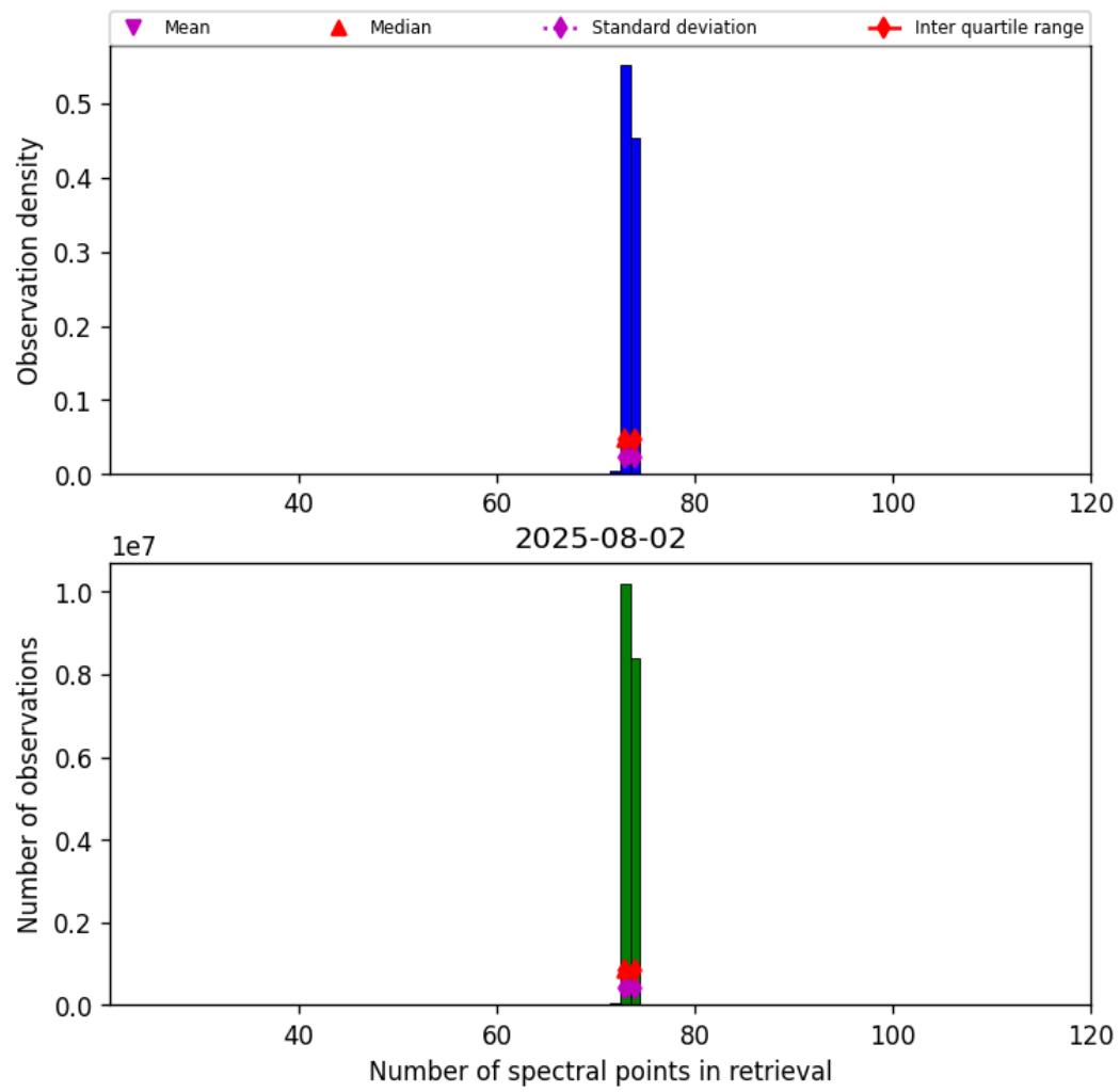
Figure 83: Histogram of “Number of spectral points in retrieval” for 2025-08-02 to 2025-08-03
