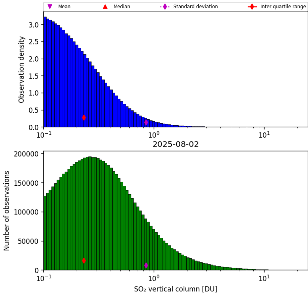
Figure 58: Histogram of “SO 2 vertical column” for 2025-08-02 to 2025-08-03
