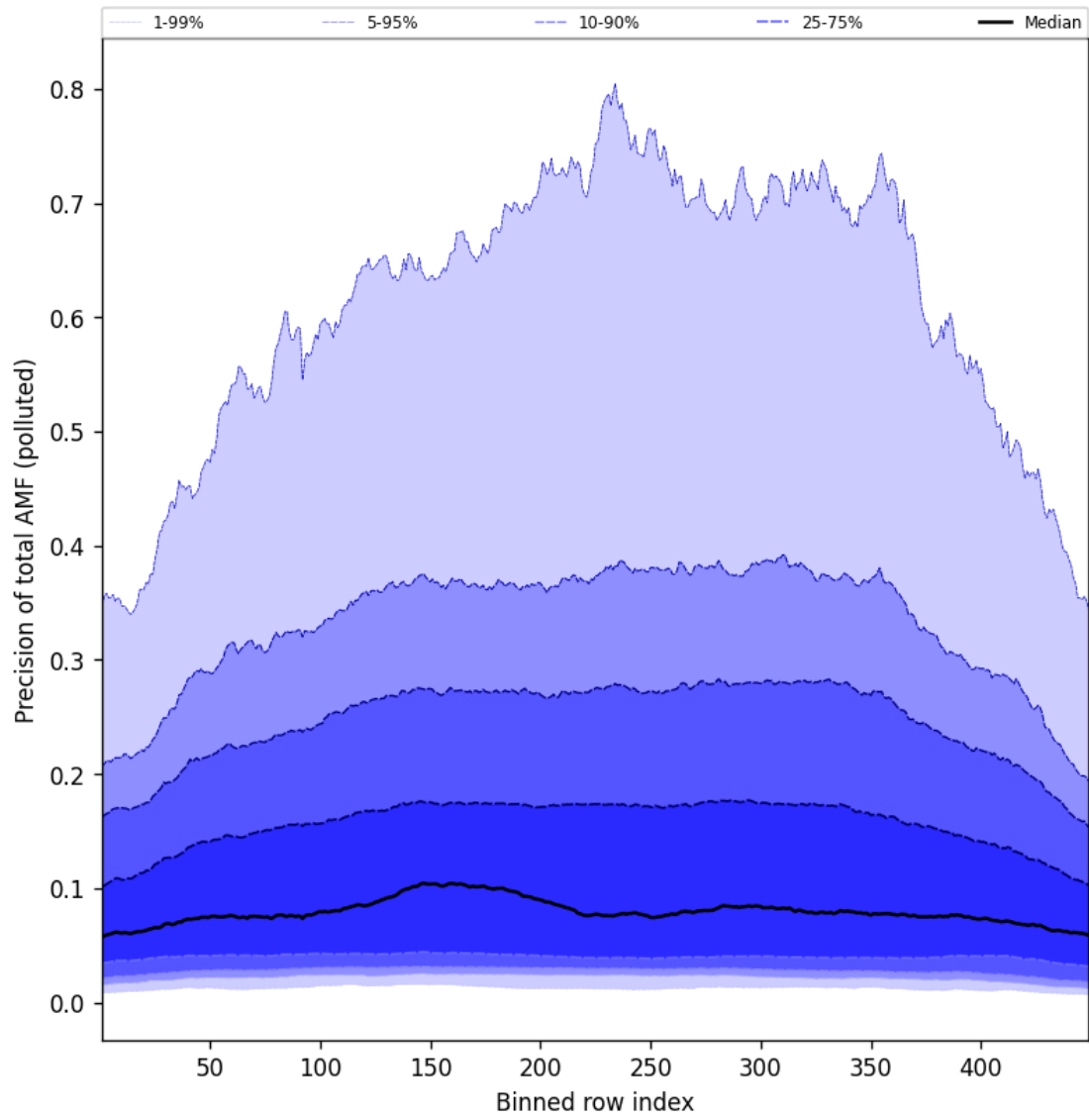
Figure 108: Along track statistics of “Precision of total AMF (polluted)” for 2025-08-02 to 2025-08-03
