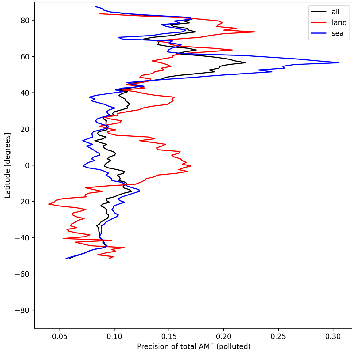
Figure 54: Zonal average of “Precision of total AMF (polluted)” for 2025-08-02 to 2025-08-03.
