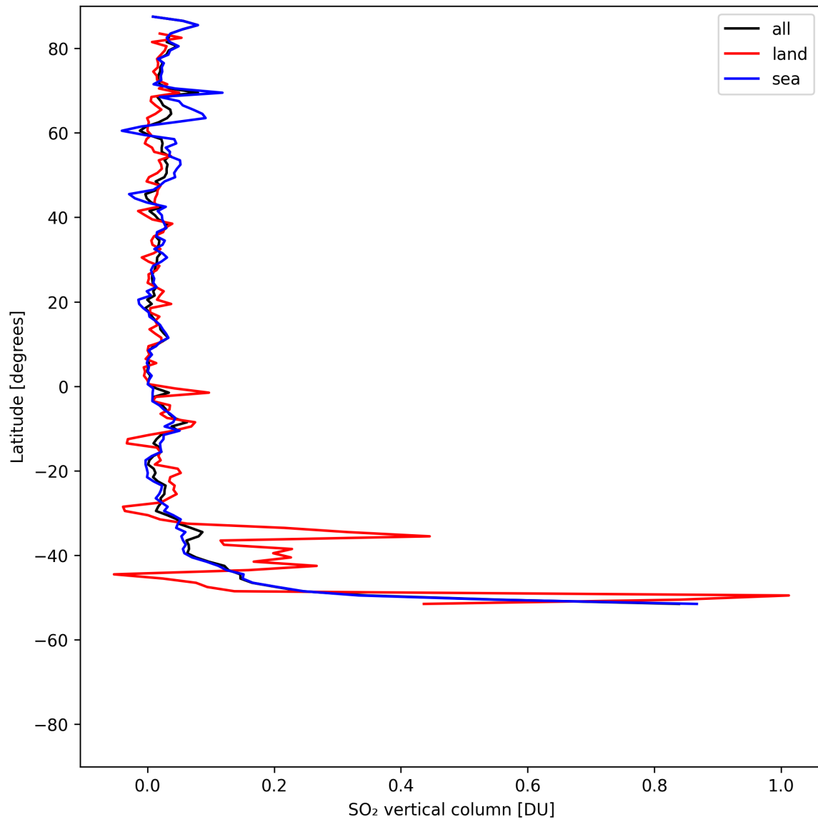
Figure 31: Zonal average of “SO 2 vertical column” for 2025-08-02 to 2025-08-03.
