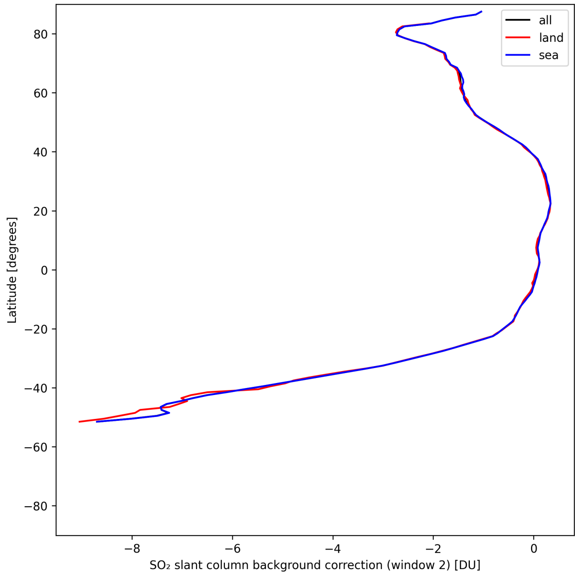
Figure 43: Zonal average of “SO 2 slant column background correction (window 2)” for 2025-08-02 to 2025-08-03.
