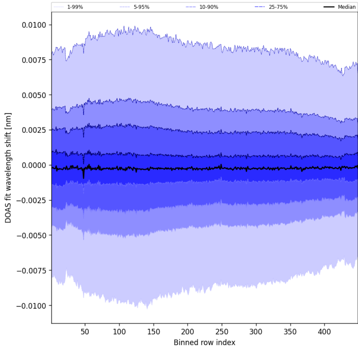
Figure 104: Along track statistics of “DOAS fit wavelength shift” for 2025-08-02 to 2025-08-03
