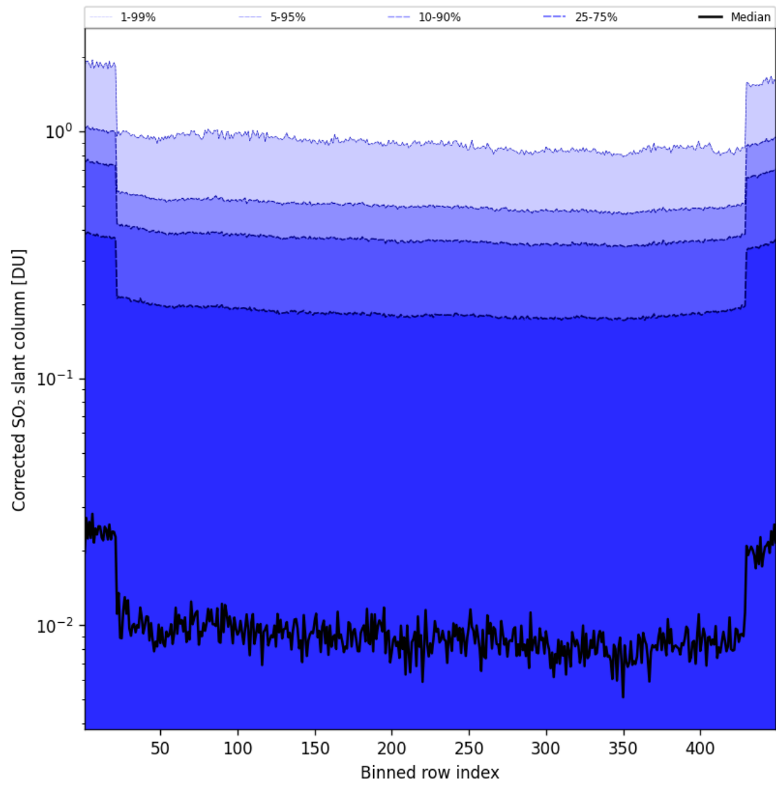
Figure 87: Along track statistics of "Corrected SO 2 slant column" for 2025-08-02 to 2025-08-03
