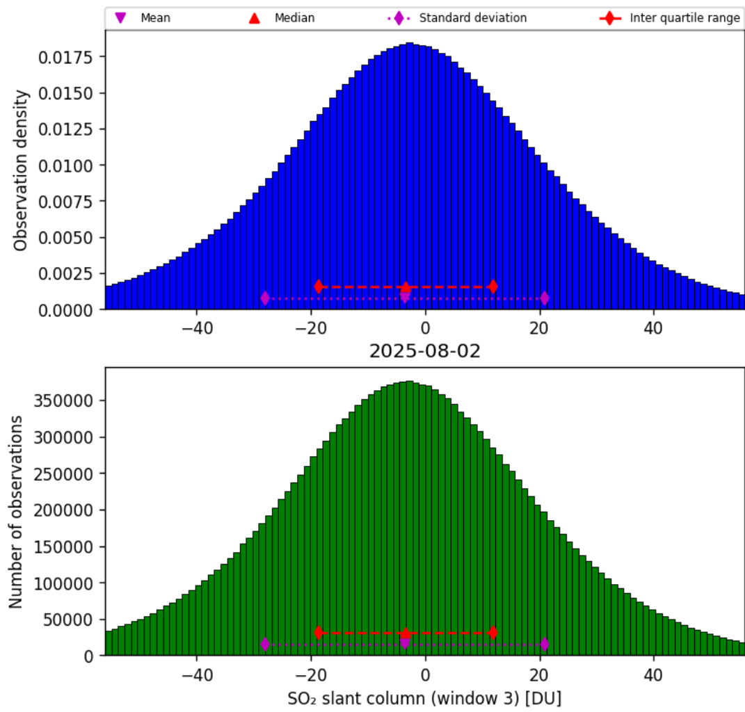
Figure 71: Histogram of “SO 2 slant column (window 3)” for 2025-08-02 to 2025-08-03
