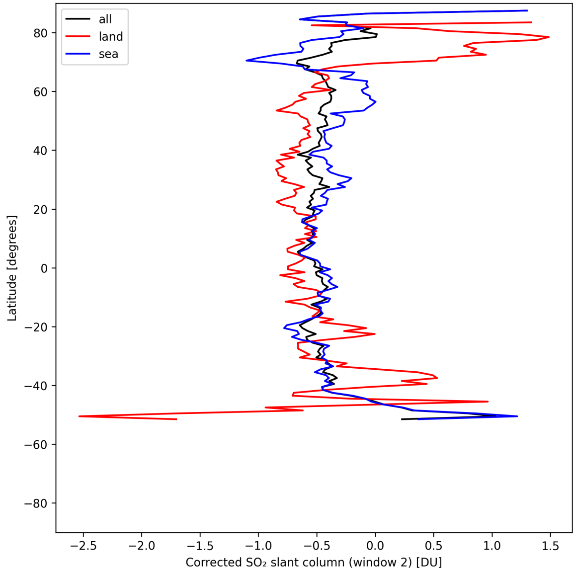
Figure 42: Zonal average of “Corrected SO 2 slant column (window 2)” for 2025-08-02 to 2025-08-03.
