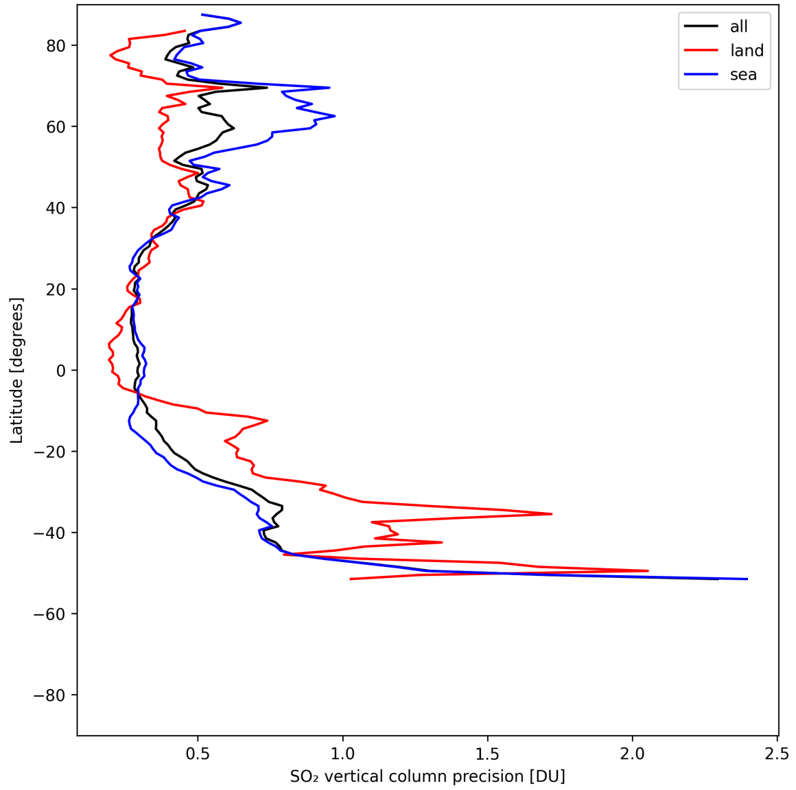
Figure 32: Zonal average of “SO 2 vertical column precision” for 2025-08-02 to 2025-08-03.
