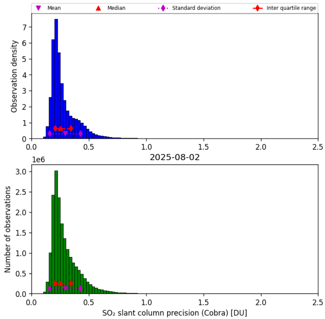
Figure 62: Histogram of “SO 2 slant column precision (Cobra)” for 2025-08-02 to 2025-08-03
