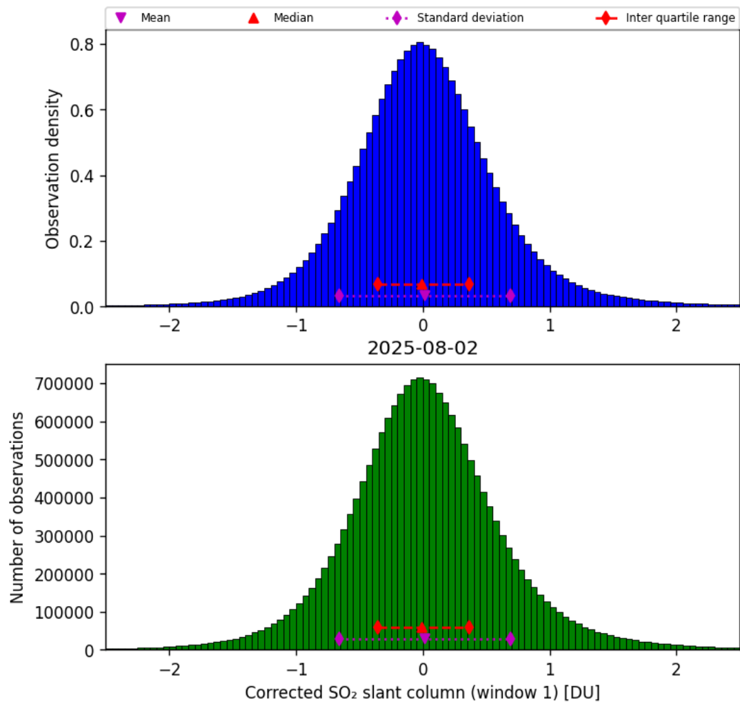
Figure 65: Histogram of “Corrected SO 2 slant column (window 1)” for 2025-08-02 to 2025-08-03
