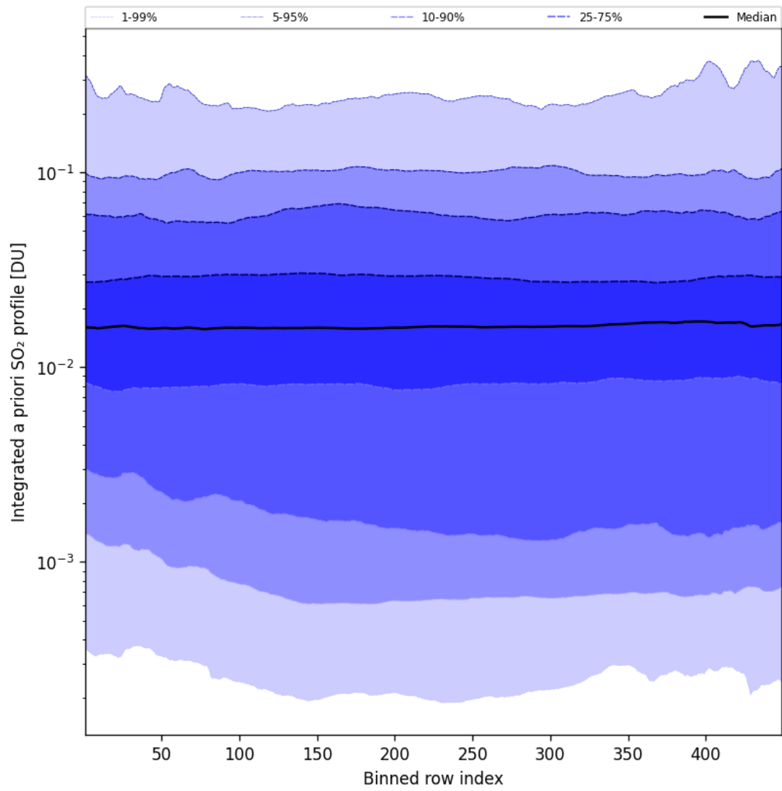
Figure 103: Along track statistics of “Integrated a priori SO 2 profile” for 2025-08-02 to 2025-08-03
