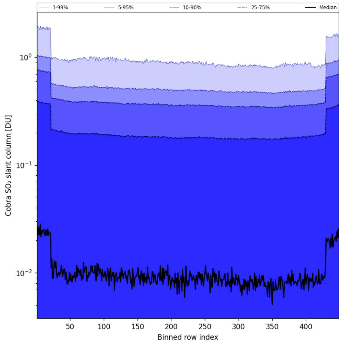
Figure 88: Along track statistics of “Cobra SO 2 slant column” for 2025-08-02 to 2025-08-03
