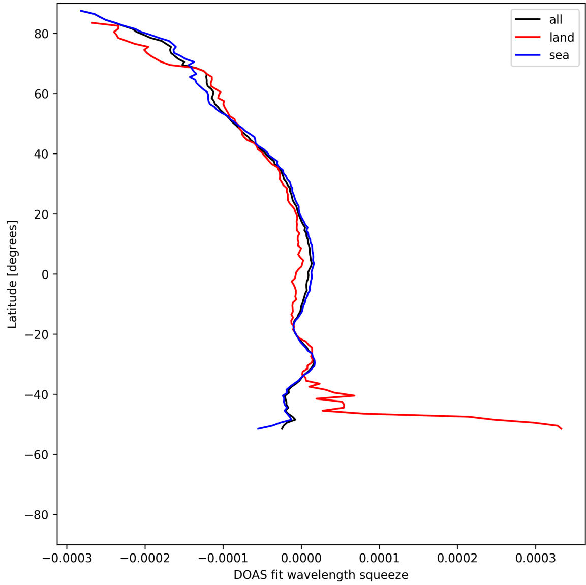
Figure 51: Zonal average of “DOAS fit wavelength squeeze” for 2025-08-02 to 2025-08-03.
