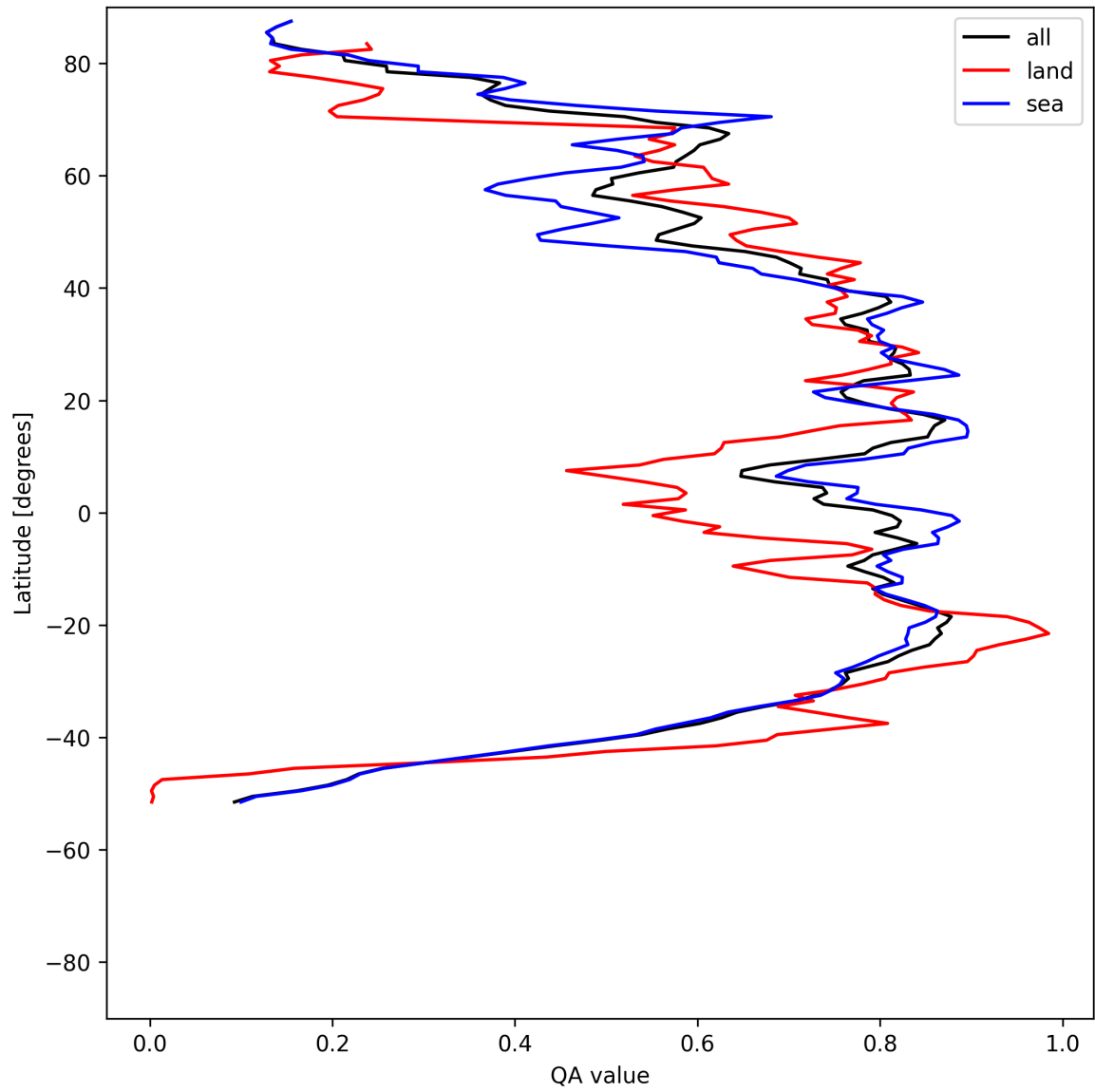
Figure 30: Zonal average of “QA value” for 2025-08-02 to 2025-08-03.
