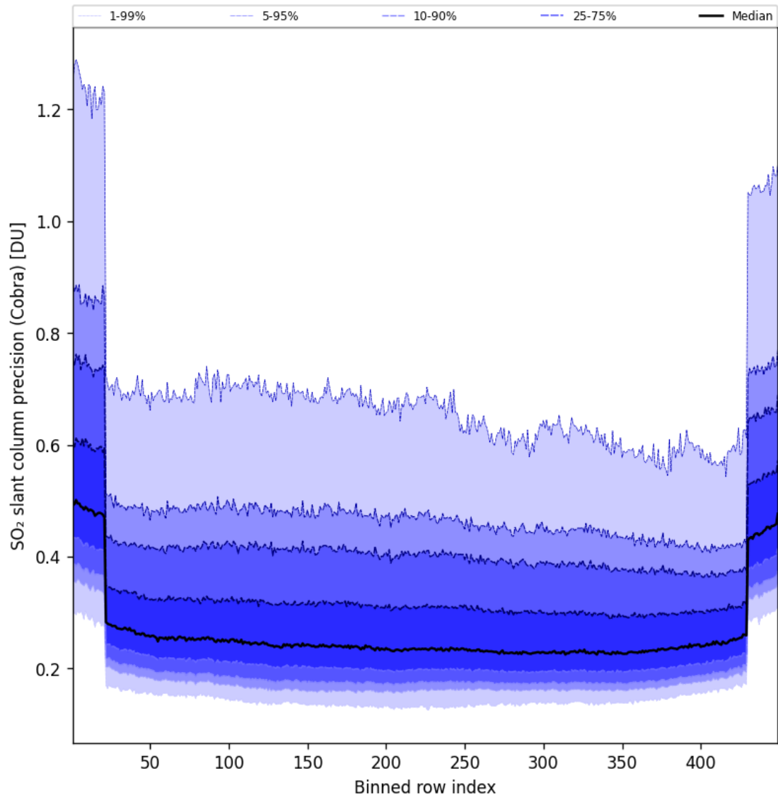
Figure 89: Along track statistics of “SO 2 slant column precision (Cobra)” for 2025-08-02 to 2025-08-03
