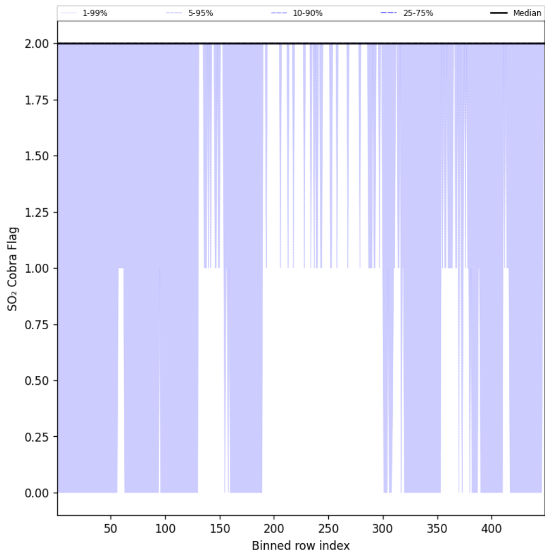
Figure 102: Along track statistics of “SO 2 Cobra Flag” for 2025-08-02 to 2025-08-03
