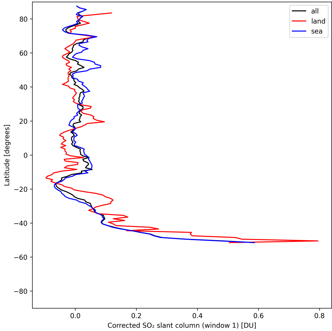
Figure 38: Zonal average of “Corrected SO 2 slant column (window 1)” for 2025-08-02 to 2025-08-03.
