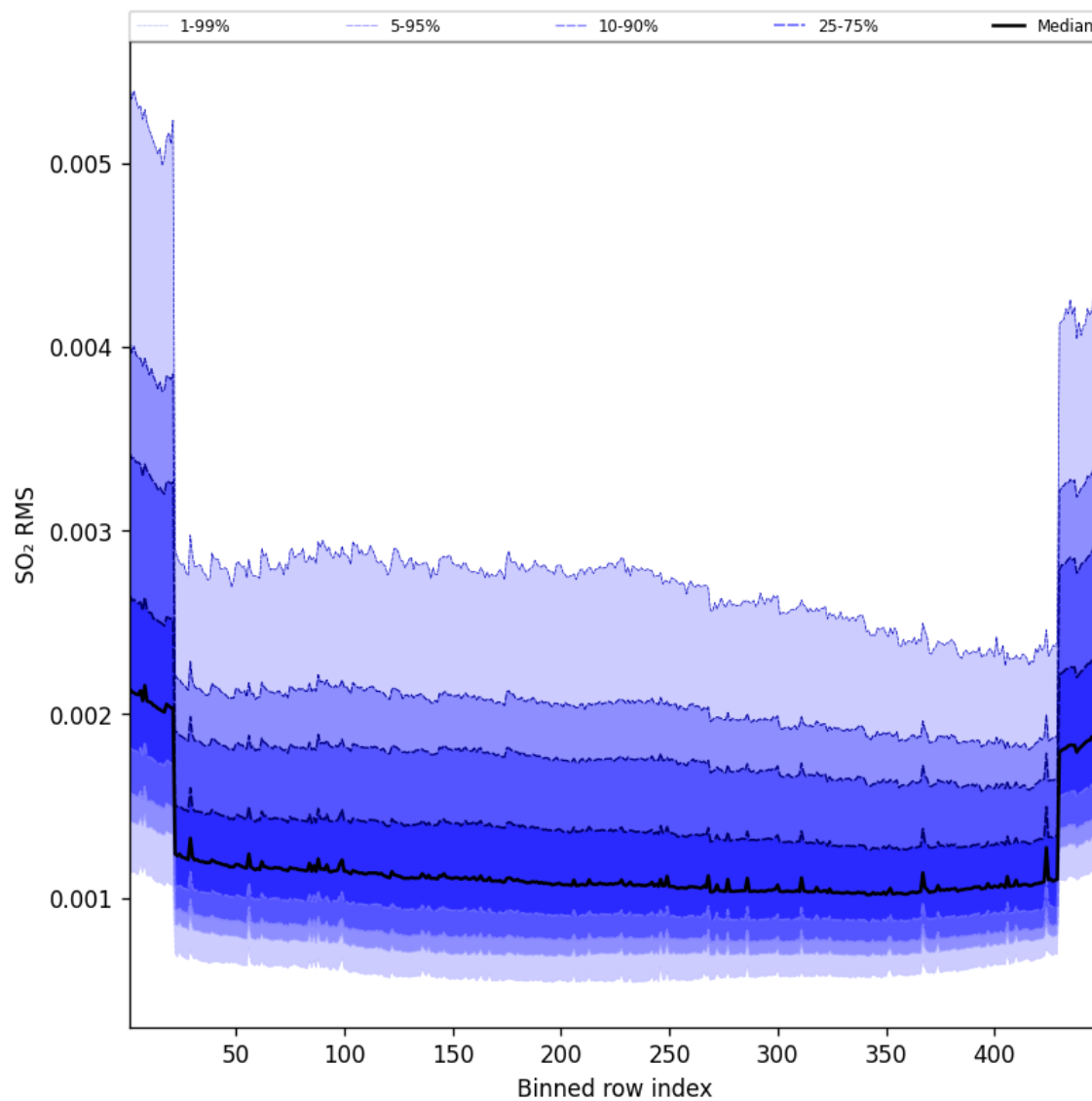
Figure 106: Along track statistics of “SO 2 RMS” for 2025-08-02 to 2025-08-03
