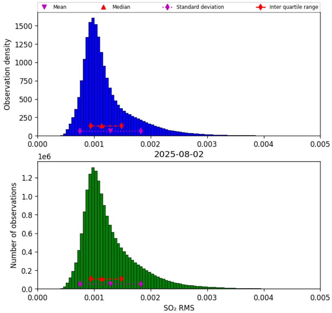
Figure 79: Histogram of “SO 2 RMS” for 2025-08-02 to 2025-08-03
