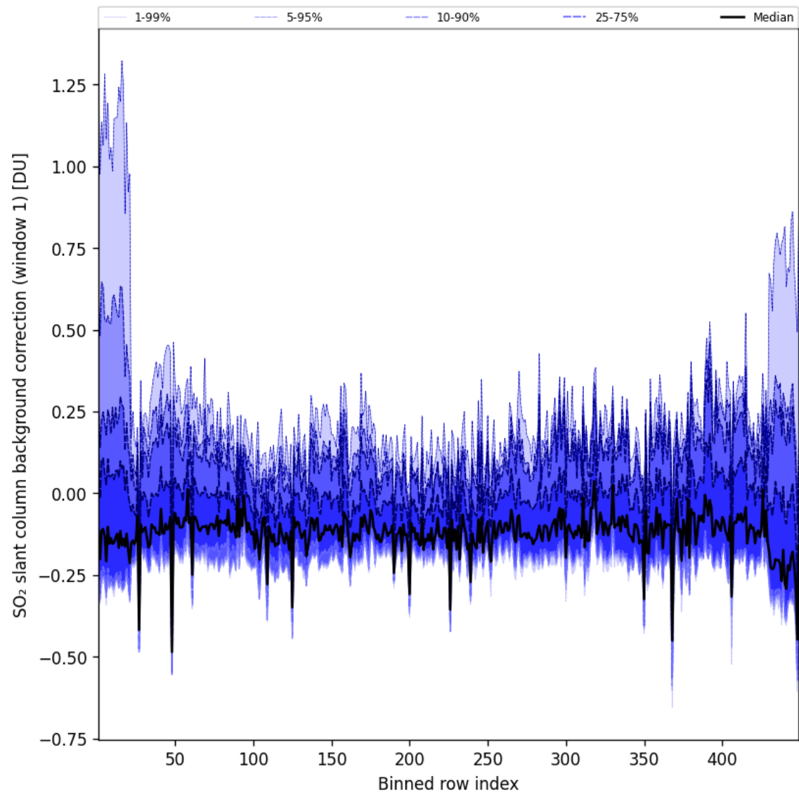
Figure 93: Along track statistics of “SO 2 slant column background correction (window 1)” for 2025-08-02 to 2025-08-03
