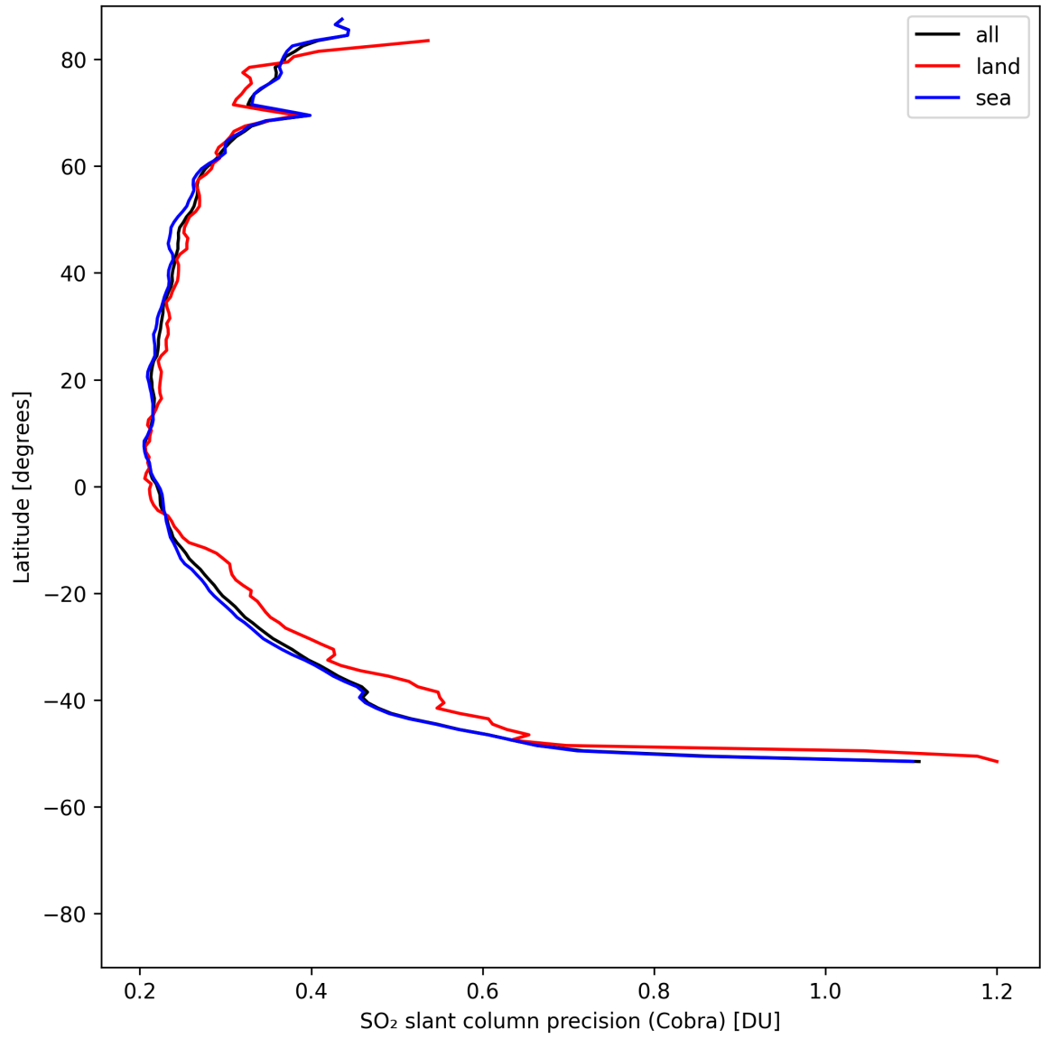
Figure 35: Zonal average of “SO 2 slant column precision (Cobra)” for 2025-08-02 to 2025-08-03.
