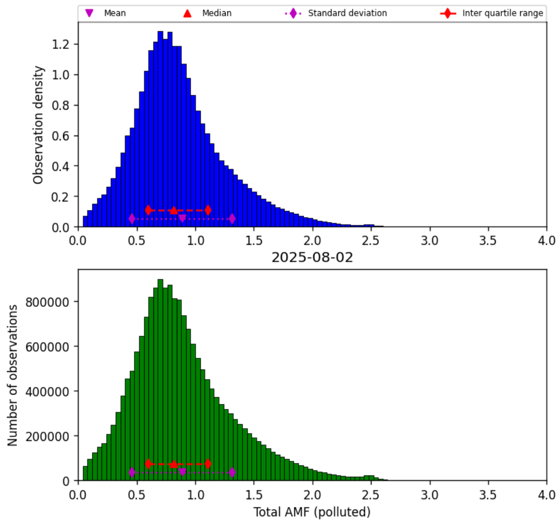
Figure 80: Histogram of “Total AMF (polluted)” for 2025-08-02 to 2025-08-03
