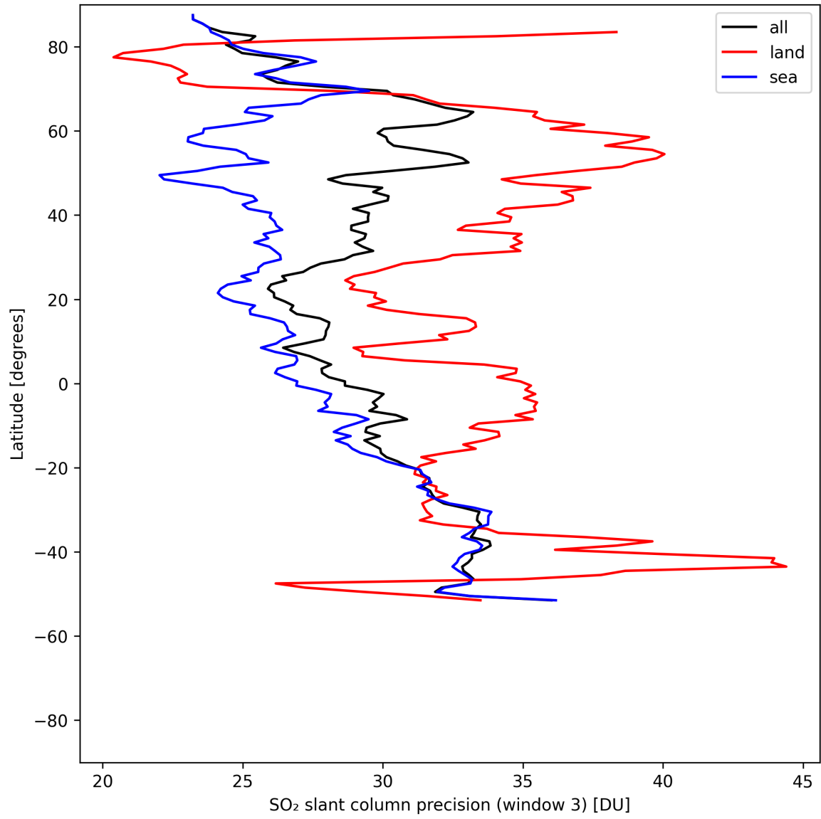
Figure 45: Zonal average of “SO 2 slant column precision (window 3)” for 2025-08-02 to 2025-08-03.
