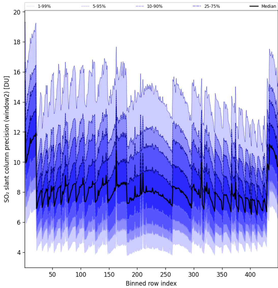
Figure 95: Along track statistics of “SO 2 slant column precision (window2)” for 2025-08-02 to 2025-08-03
