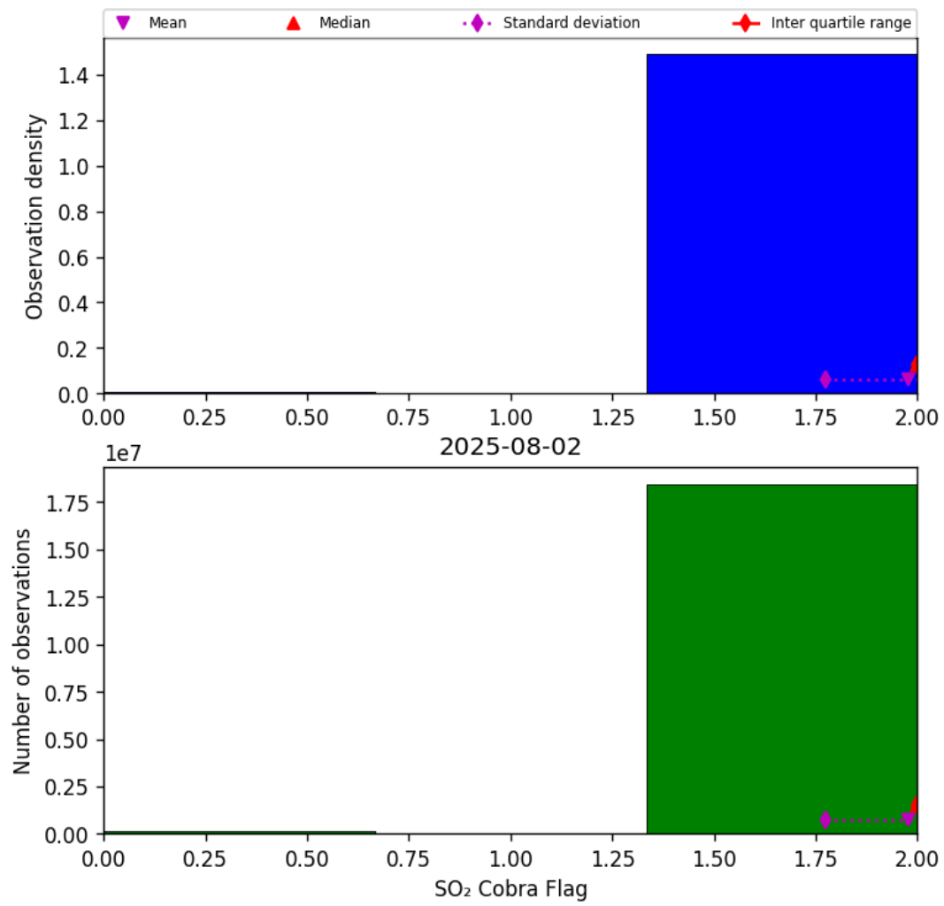
Figure 75: Histogram of "SO 2 Cobra Flag" for 2025-08-02 to 2025-08-03
