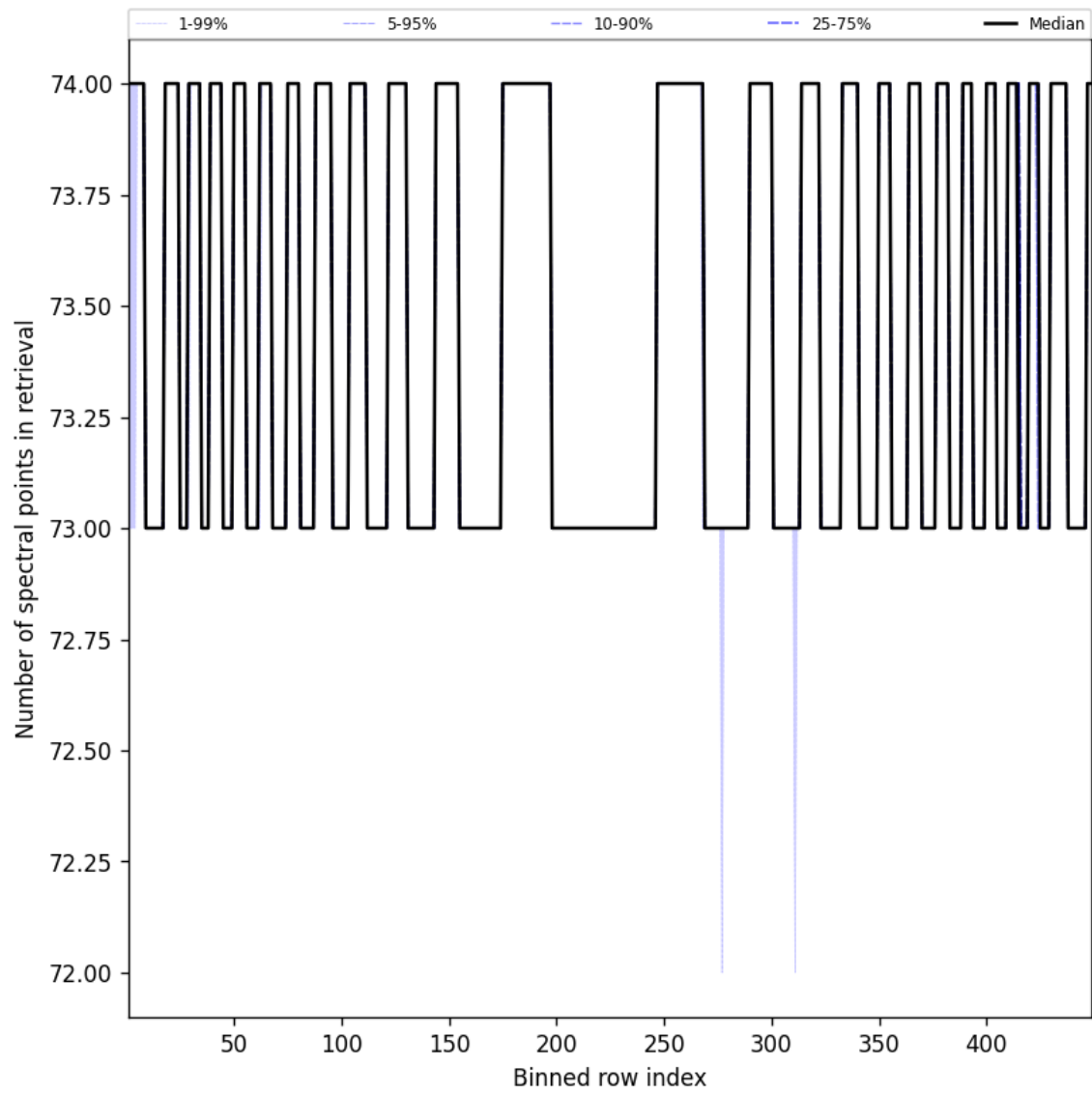
Figure 110: Along track statistics of “Number of spectral points in retrieval” for 2025-08-02 to 2025-08-03
