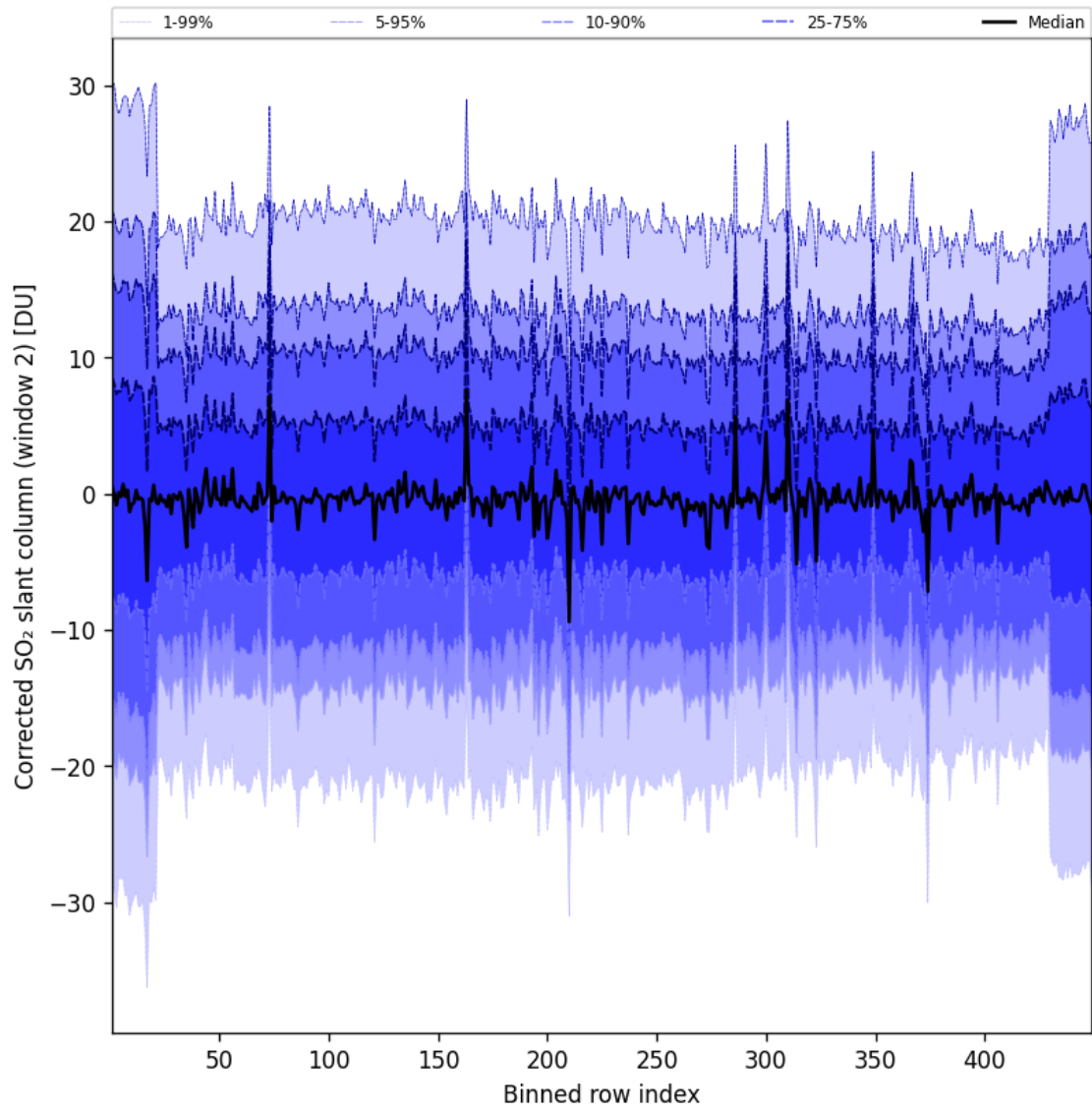
Figure 96: Along track statistics of “Corrected SO 2 slant column (window 2)” for 2025-08-02 to 2025-08-03
