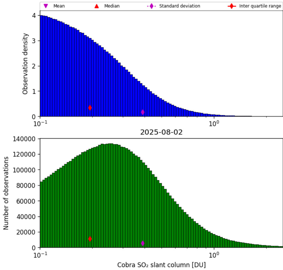
Figure 61: Histogram of “Cobra SO 2 slant column” for 2025-08-02 to 2025-08-03
