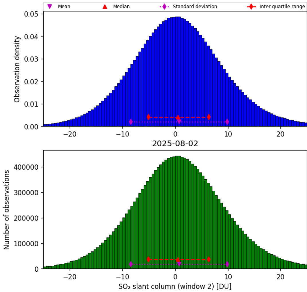
Figure 67: Histogram of “SO 2 slant column (window 2)” for 2025-08-02 to 2025-08-03
