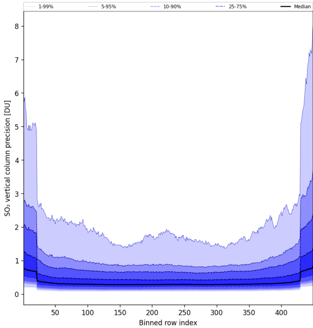
Figure 86: Along track statistics of “SO 2 vertical column precision” for 2025-08-02 to 2025-08-03
