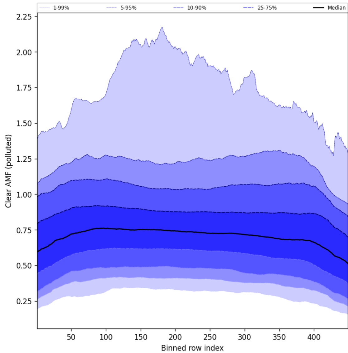
Figure 109: Along track statistics of “Clear AMF (polluted)” for 2025-08-02 to 2025-08-03
