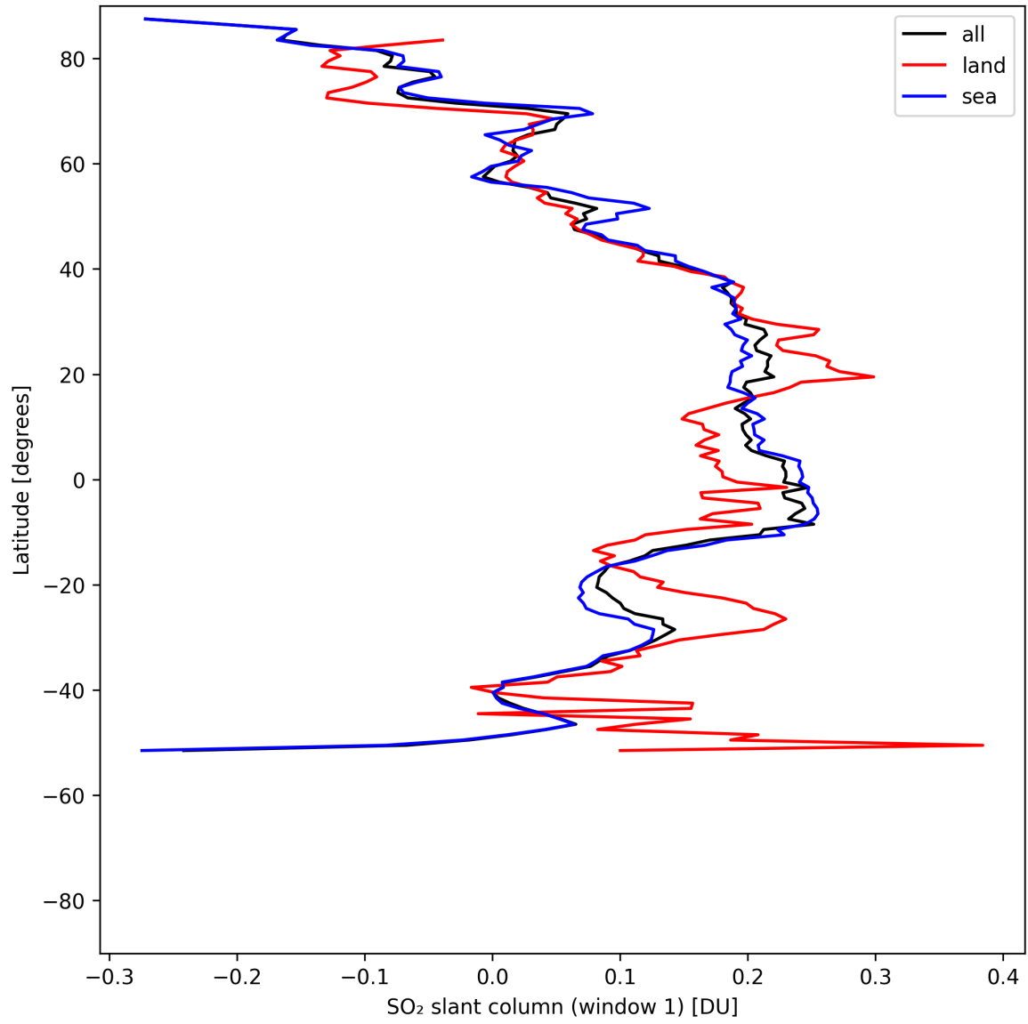
Figure 36: Zonal average of “SO 2 slant column (window 1)” for 2025-08-02 to 2025-08-03.
