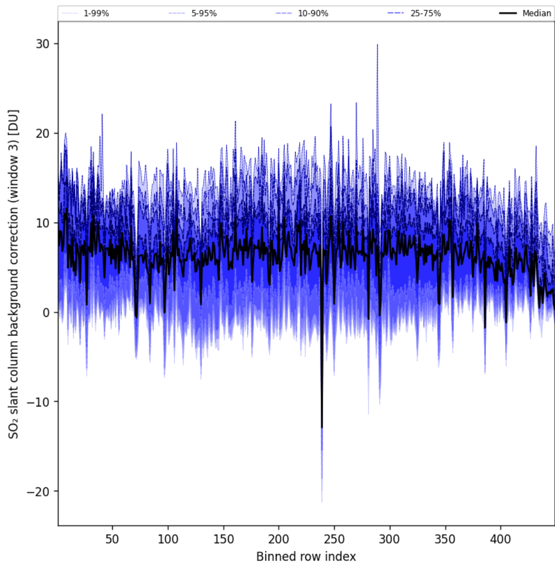
Figure 101: Along track statistics of “SO 2 slant column background correction (window 3)” for 2025-08-02 to 2025-08-03
