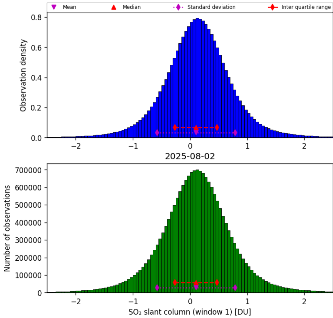
Figure 63: Histogram of “SO 2 slant column (window 1)” for 2025-08-02 to 2025-08-03
