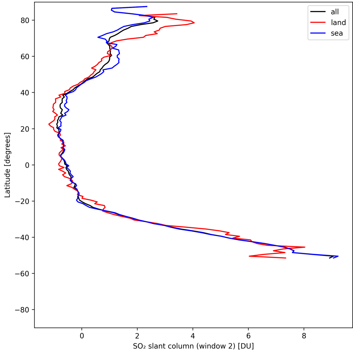
Figure 40: Zonal average of “SO 2 slant column (window 2)” for 2025-08-02 to 2025-08-03.
