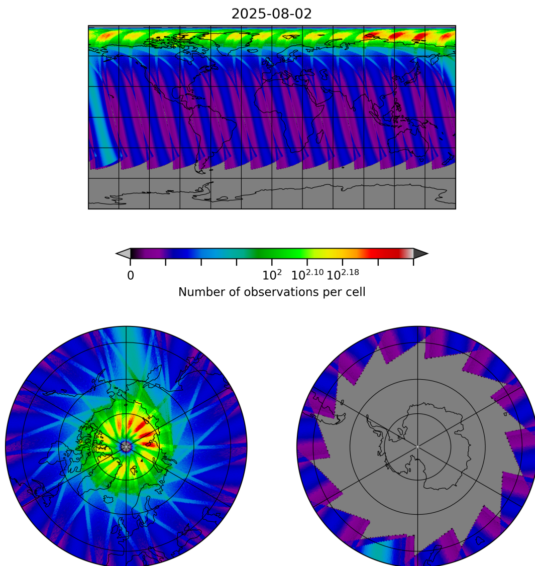
Figure 29: Map of the number of observations for 2025-08-02 to 2025-08-03
