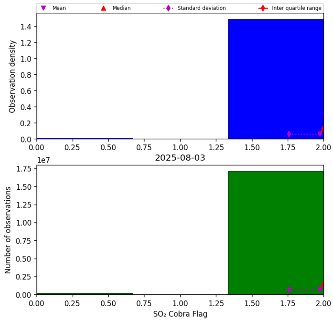
Figure 75: Histogram of “SO 2 Cobra Flag” for 2025-08-03 to 2025-08-04
