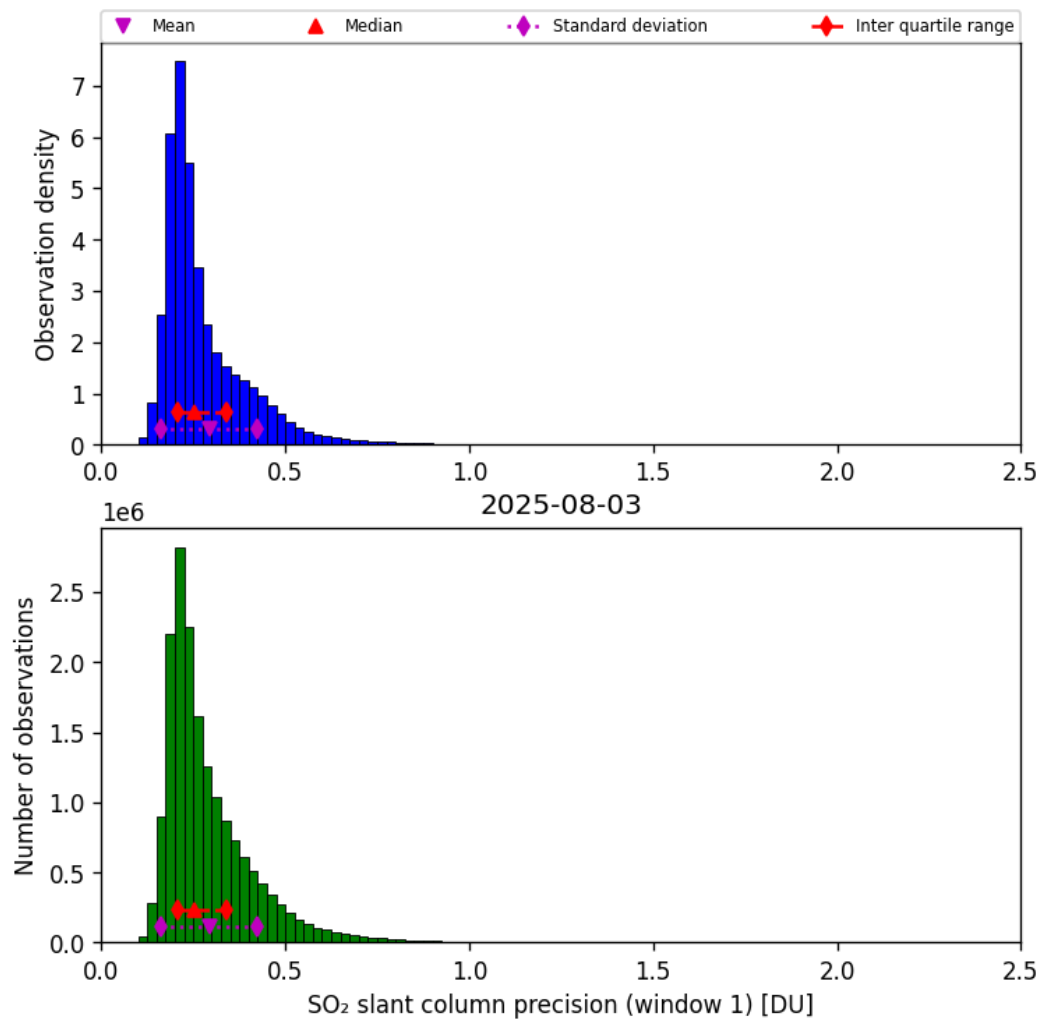
Figure 64: Histogram of “SO 2 slant column precision (window 1)” for 2025-08-03 to 2025-08-04
