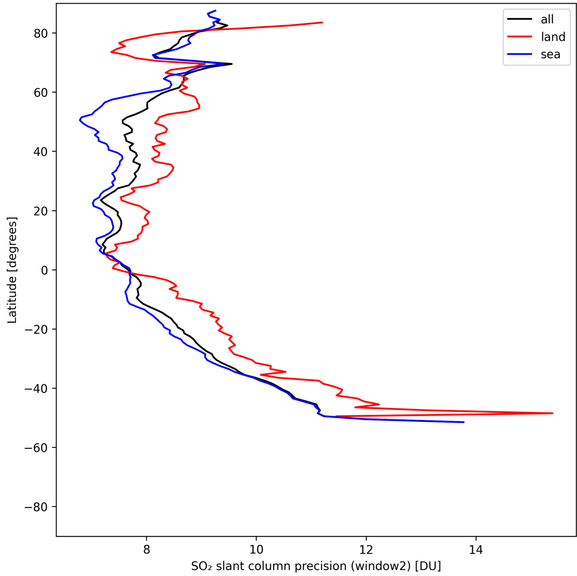
Figure 41: Zonal average of “SO 2 slant column precision (window2)” for 2025-08-03 to 2025-08-04.
