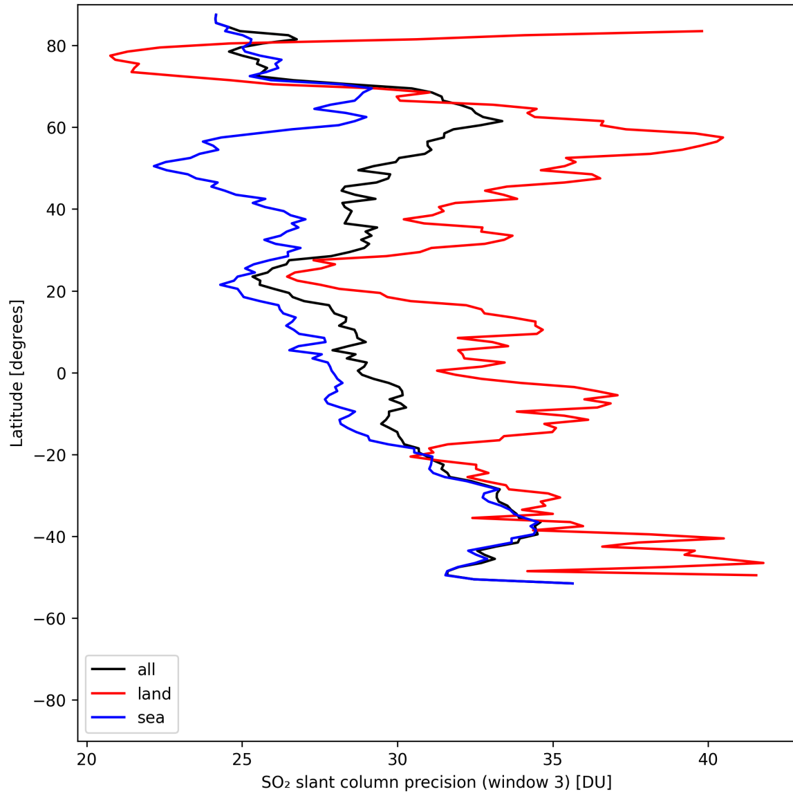
Figure 45: Zonal average of “SO 2 slant column precision (window 3)” for 2025-08-03 to 2025-08-04.
