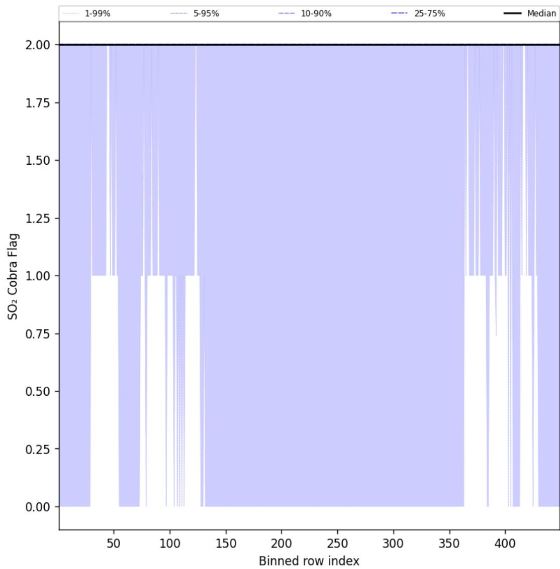
Figure 102: Along track statistics of “SO 2 Cobra Flag” for 2025-08-03 to 2025-08-04
