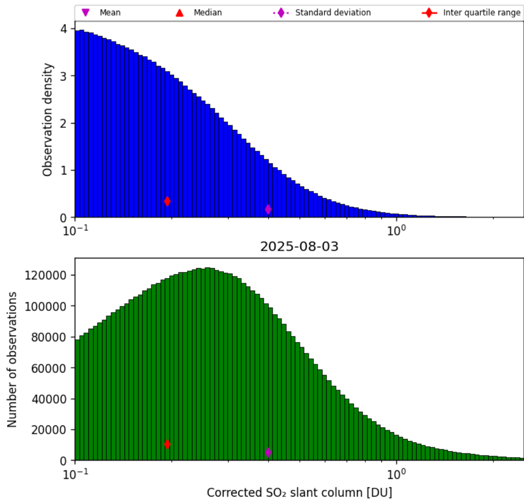
Figure 60: Histogram of “Corrected SO 2 slant column” for 2025-08-03 to 2025-08-04
