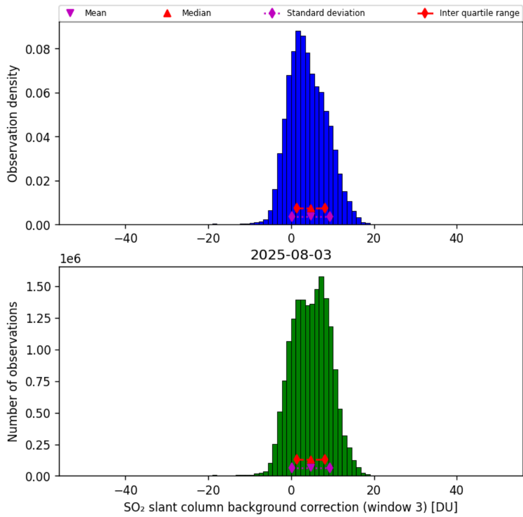
Figure 74: Histogram of “SO 2 slant column background correction (window 3)” for 2025-08-03 to 2025-08-04
