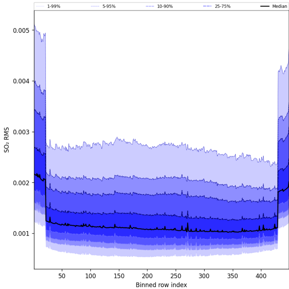
Figure 106: Along track statistics of “SO 2 RMS” for 2025-08-03 to 2025-08-04
