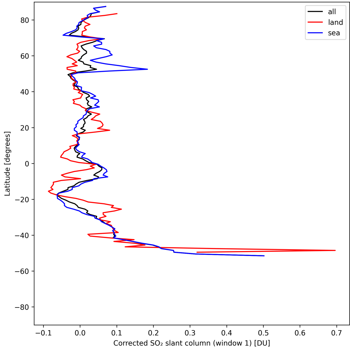
Figure 38: Zonal average of “Corrected SO 2 slant column (window 1)” for 2025-08-03 to 2025-08-04.
