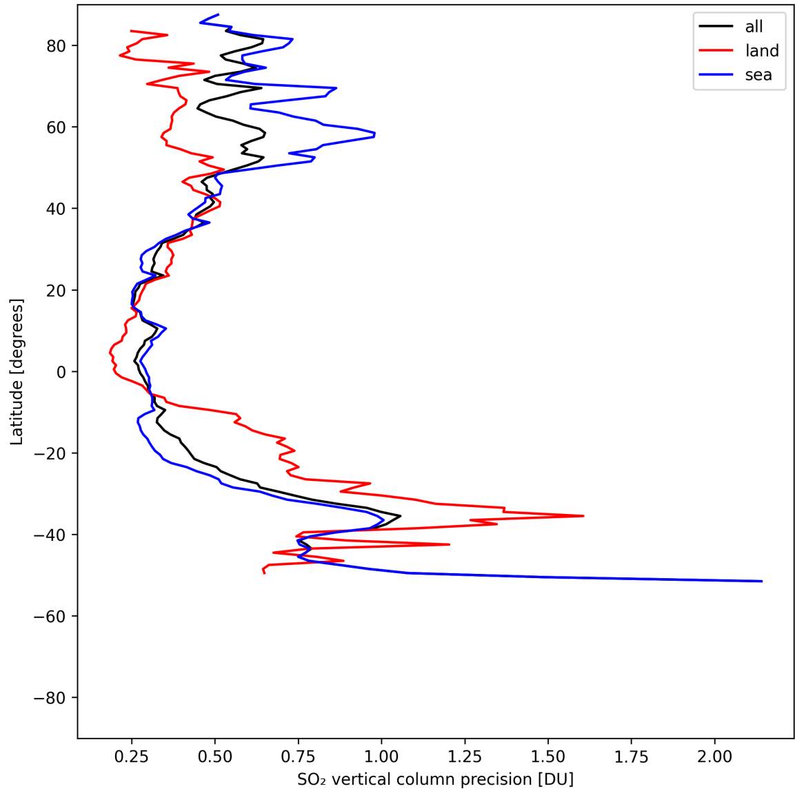
Figure 32: Zonal average of “SO 2 vertical column precision” for 2025-08-03 to 2025-08-04.
