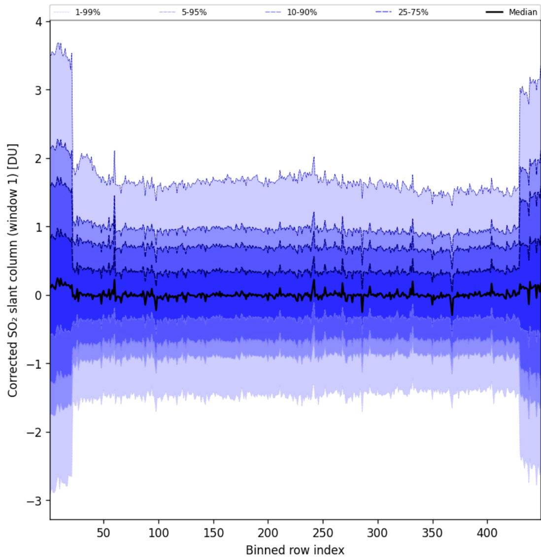
Figure 92: Along track statistics of “Corrected SO 2 slant column (window 1)” for 2025-08-03 to 2025-08-04
