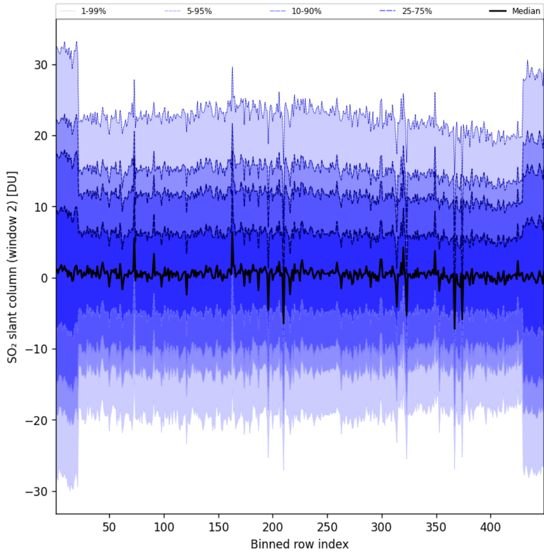
Figure 94: Along track statistics of “SO 2 slant column (window 2)” for 2025-08-03 to 2025-08-04
