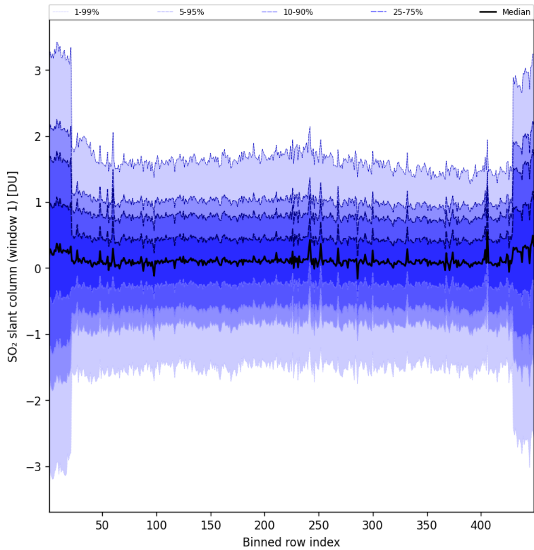
Figure 90: Along track statistics of “SO 2 slant column (window 1)” for 2025-08-03 to 2025-08-04
