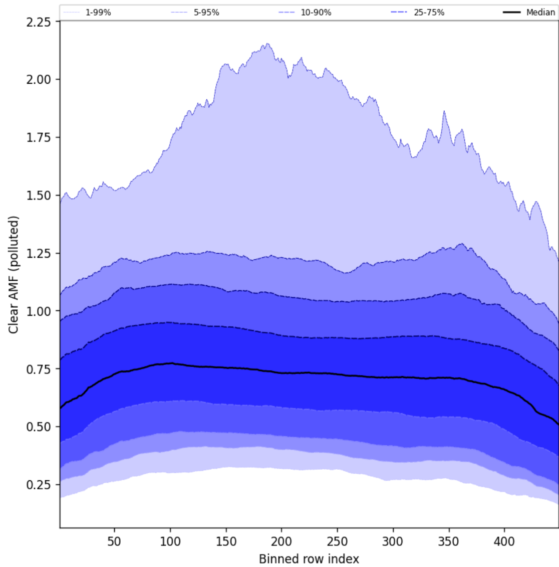
Figure 109: Along track statistics of “Clear AMF (polluted)” for 2025-08-03 to 2025-08-04
