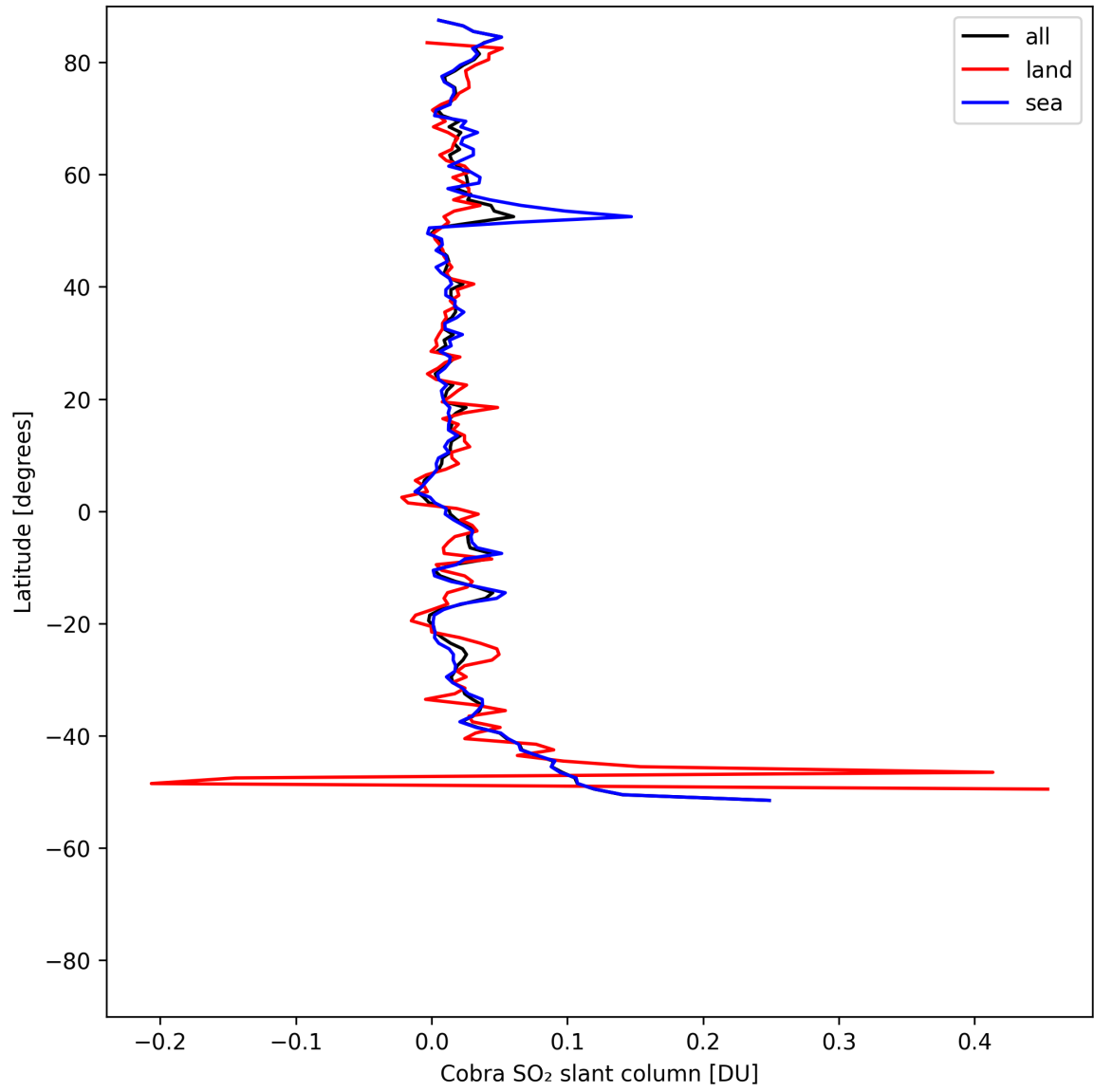
Figure 34: Zonal average of “Cobra SO 2 slant column” for 2025-08-03 to 2025-08-04.
