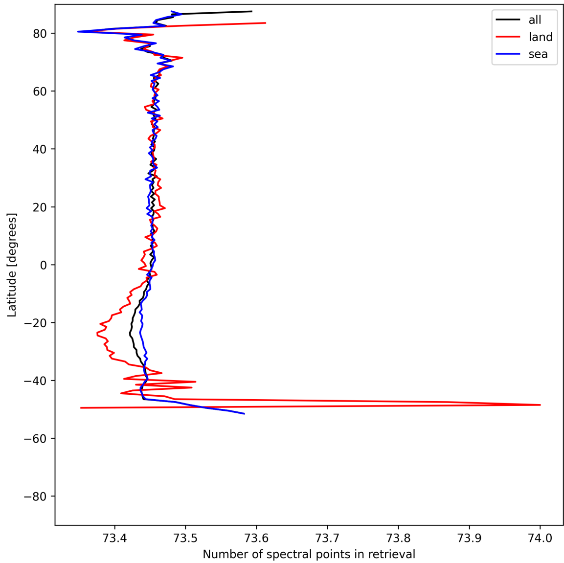
Figure 56: Zonal average of “Number of spectral points in retrieval” for 2025-08-03 to 2025-08-04.
