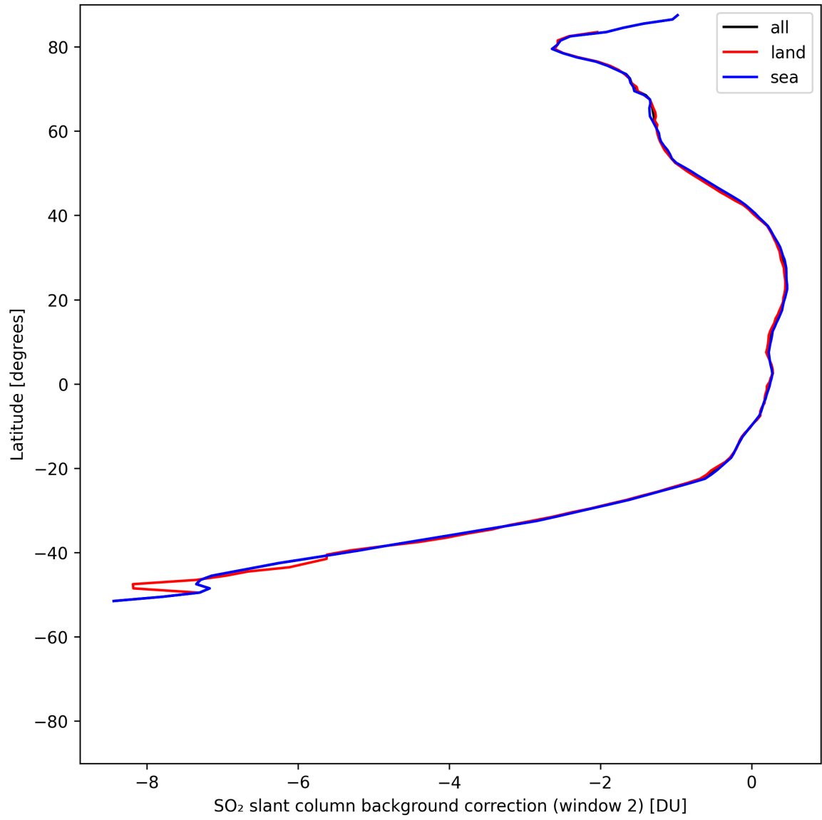
Figure 43: Zonal average of “SO 2 slant column background correction (window 2)” for 2025-08-03 to 2025-08-04.
