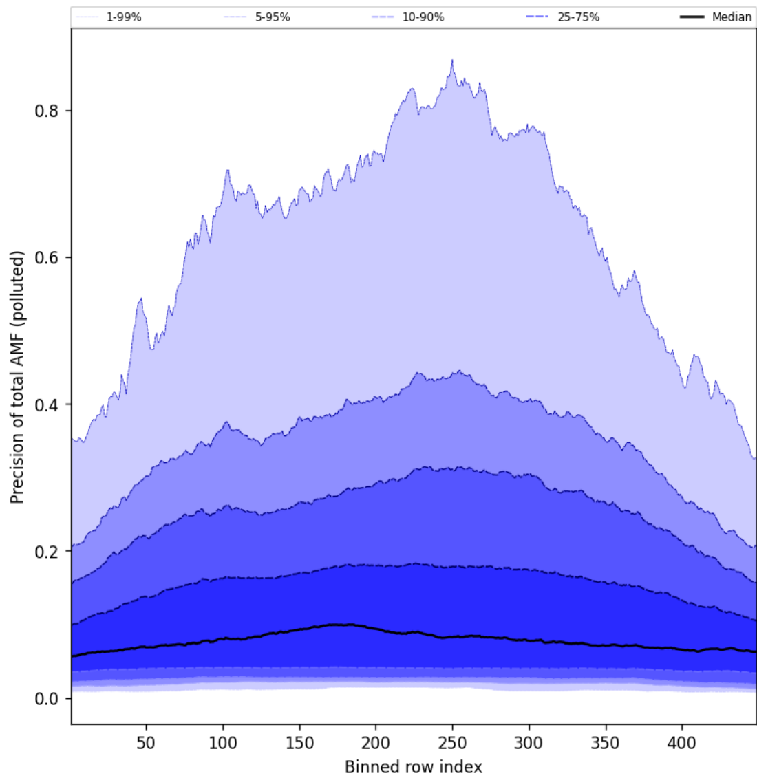
Figure 108: Along track statistics of “Precision of total AMF (polluted)” for 2025-08-03 to 2025-08-04
