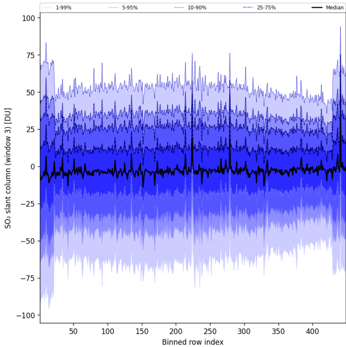
Figure 98: Along track statistics of “SO 2 slant column (window 3)” for 2025-08-03 to 2025-08-04
