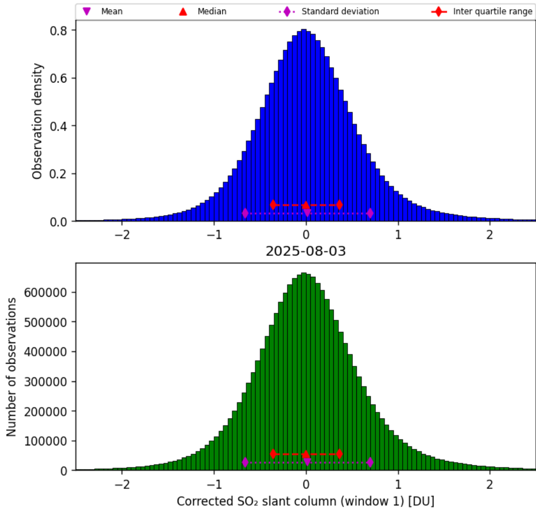
Figure 65: Histogram of “Corrected SO 2 slant column (window 1)” for 2025-08-03 to 2025-08-04
