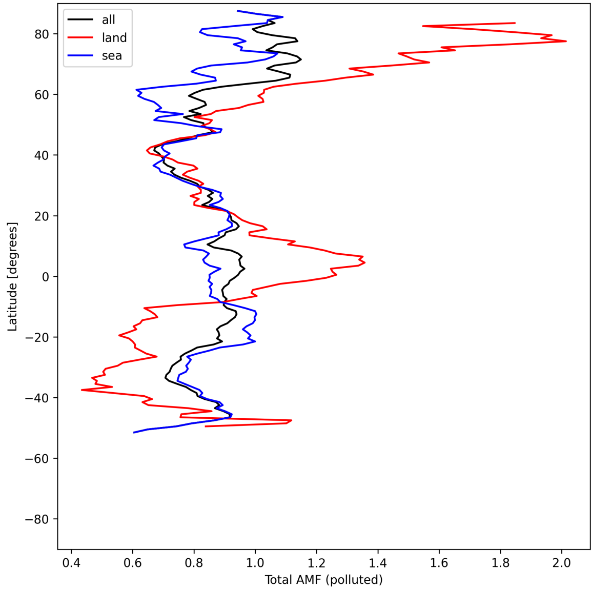
Figure 53: Zonal average of “Total AMF (polluted)” for 2025-08-03 to 2025-08-04.
