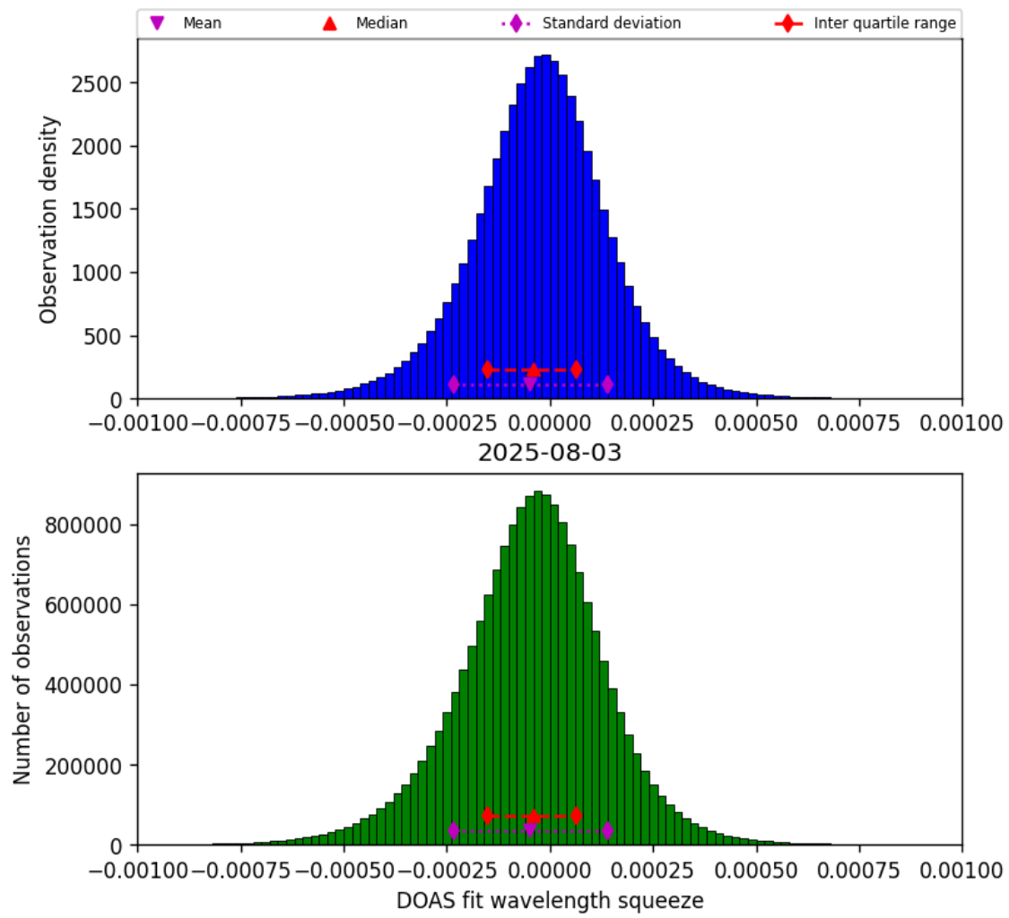
Figure 78: Histogram of “DOAS fit wavelength squeeze” for 2025-08-03 to 2025-08-04
