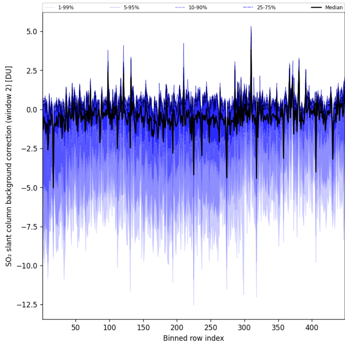
Figure 97: Along track statistics of “SO 2 slant column background correction (window 2)” for 2025-08-03 to 2025-08-04
