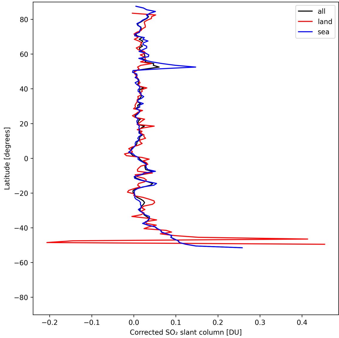
Figure 33: Zonal average of “Corrected SO 2 slant column” for 2025-08-03 to 2025-08-04.
