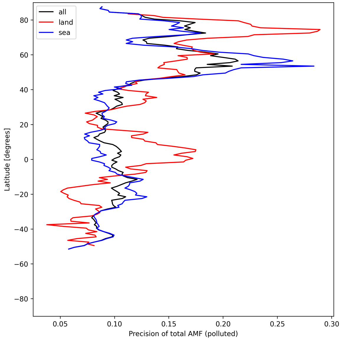
Figure 54: Zonal average of “Precision of total AMF (polluted)” for 2025-08-03 to 2025-08-04.
