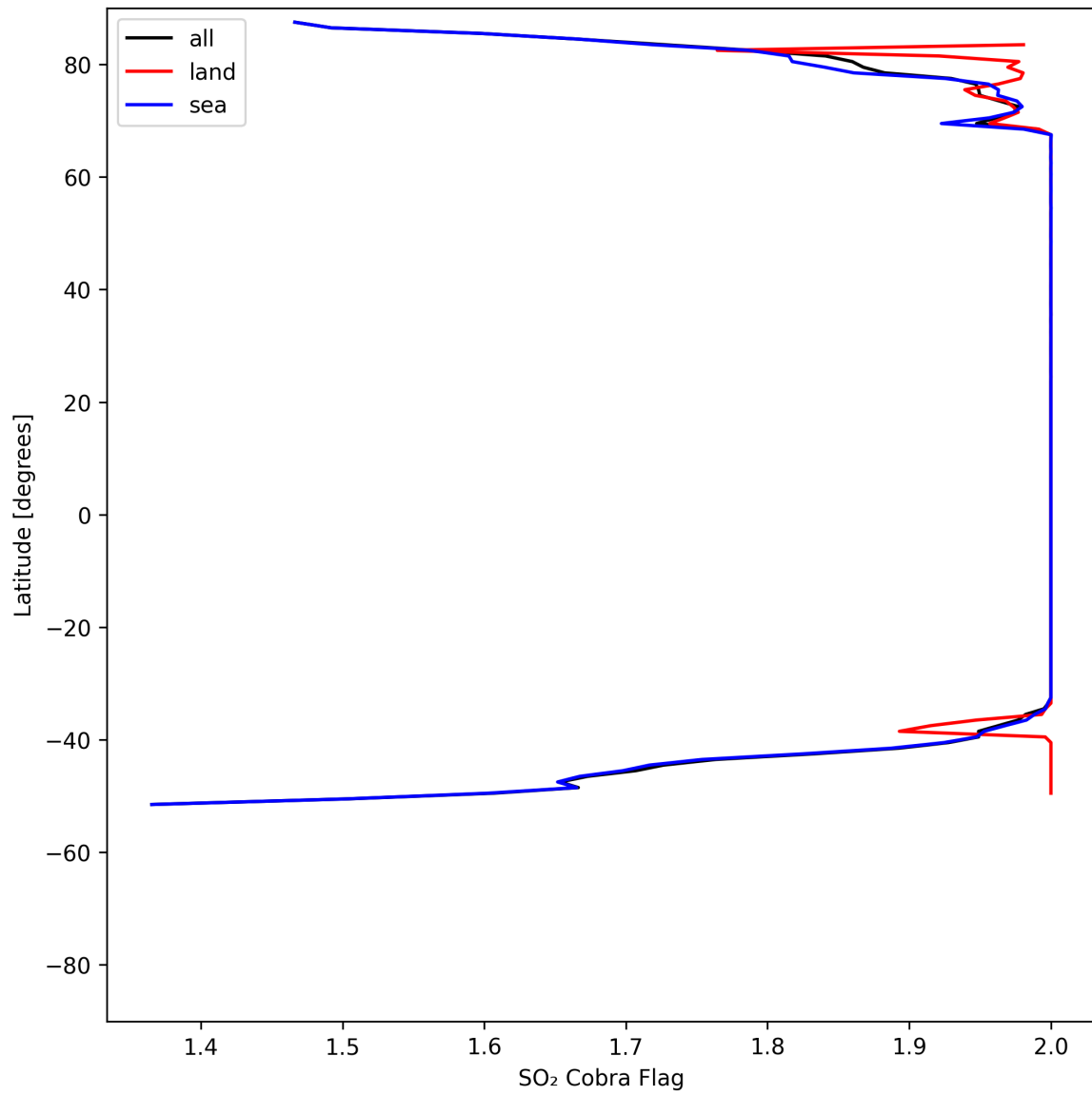
Figure 48: Zonal average of "SO 2 Cobra Flag" for 2025-08-03 to 2025-08-04.
