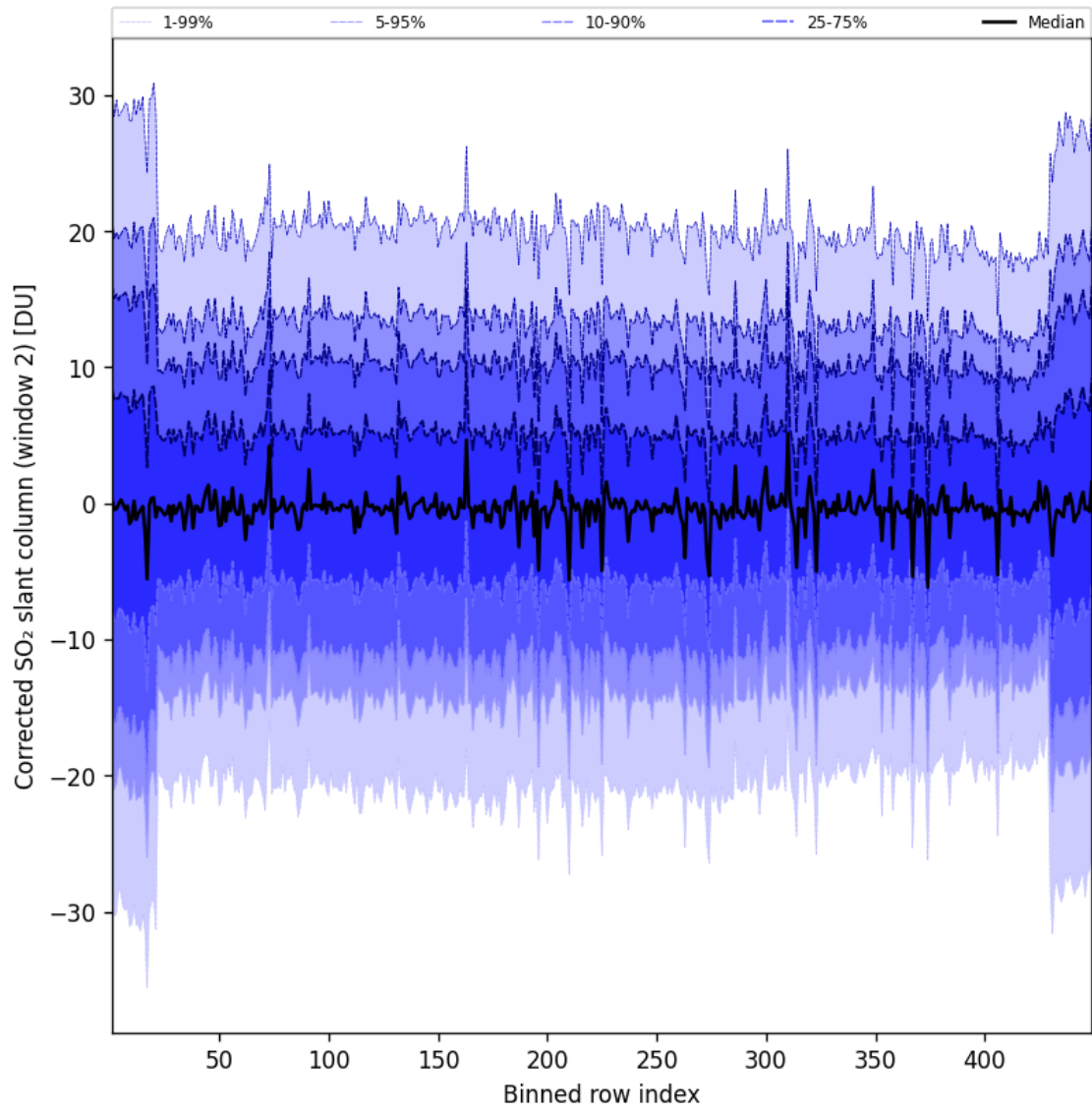
Figure 96: Along track statistics of “Corrected SO 2 slant column (window 2)” for 2025-08-03 to 2025-08-04
