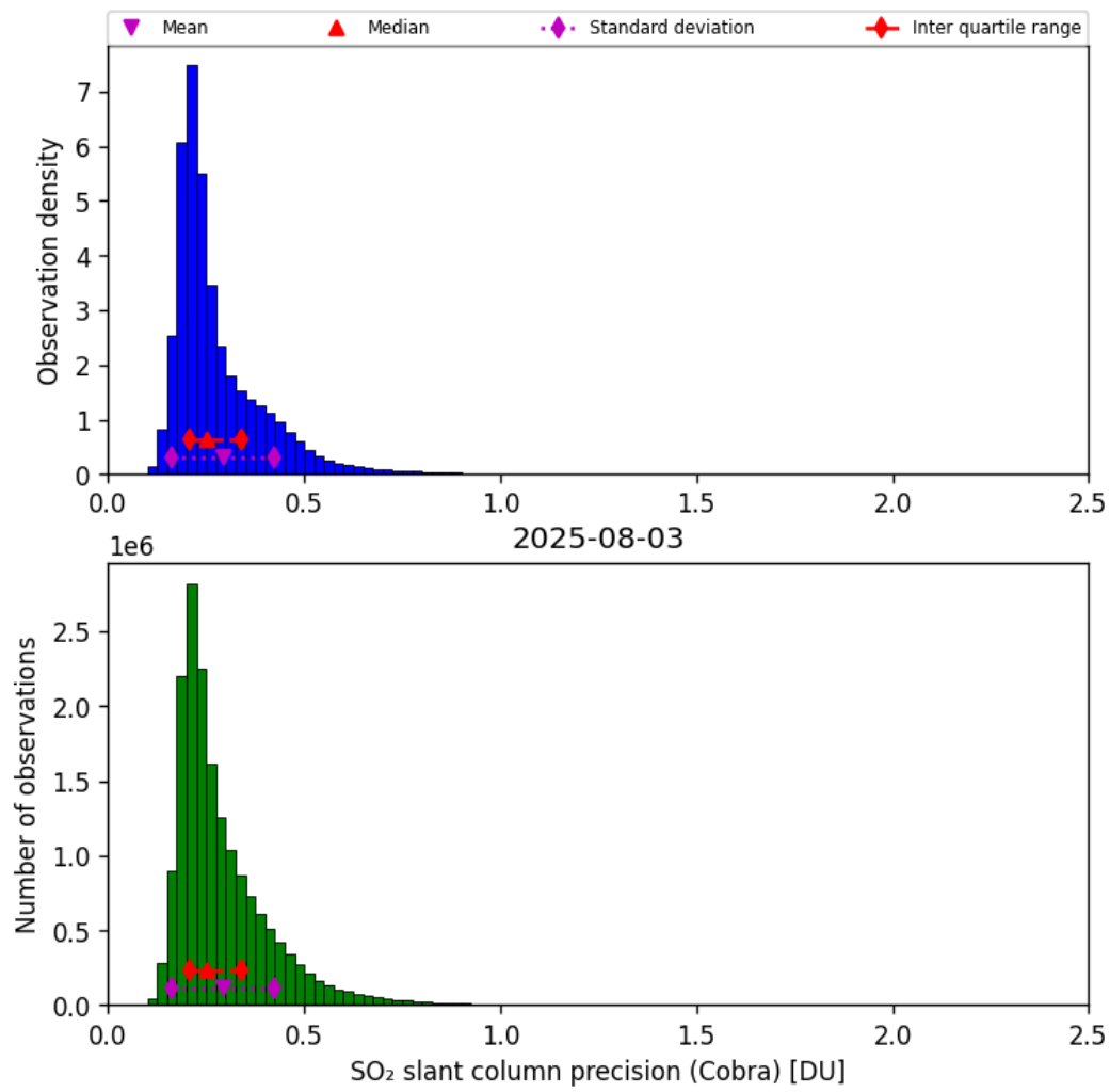
Figure 62: Histogram of “SO 2 slant column precision (Cobra)” for 2025-08-03 to 2025-08-04
