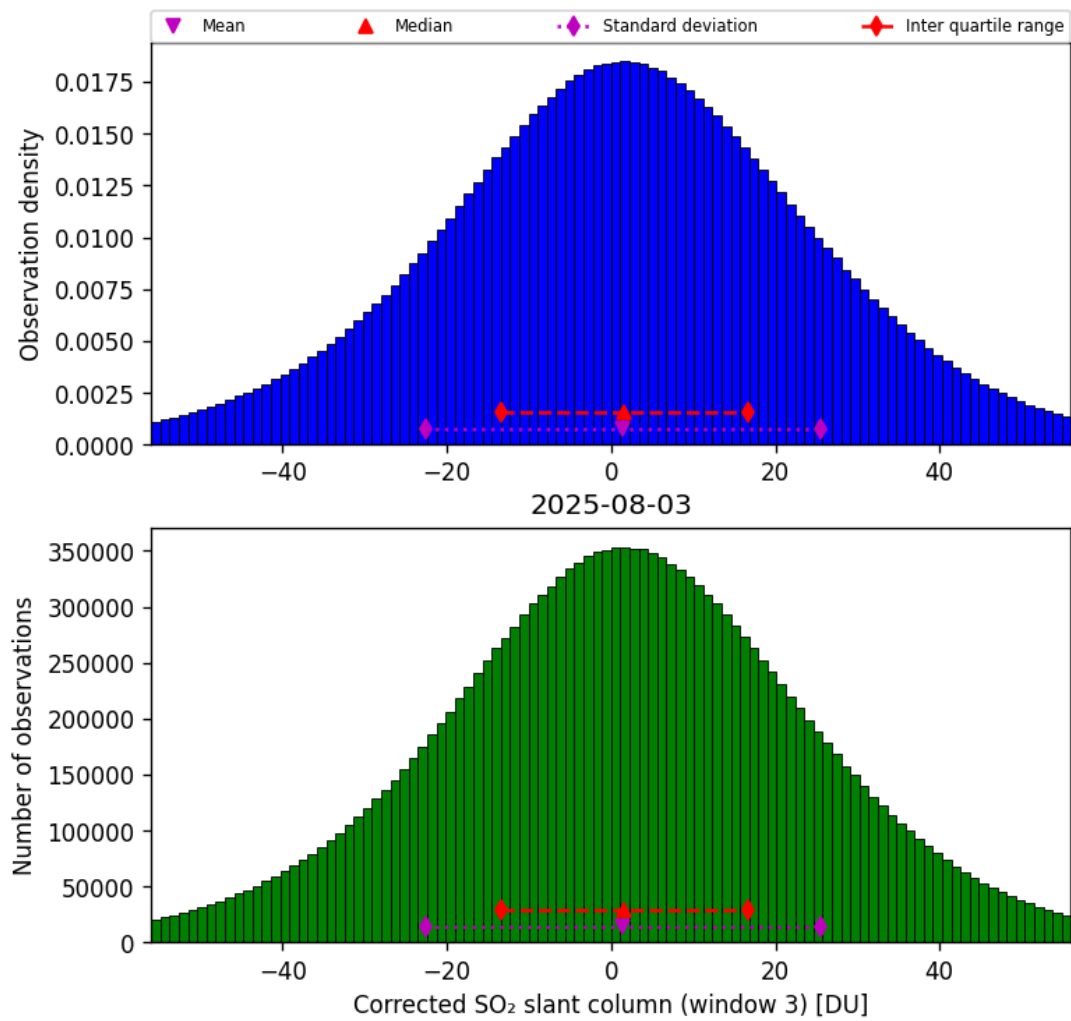
Figure 73: Histogram of “Corrected SO 2 slant column (window 3)” for 2025-08-03 to 2025-08-04
