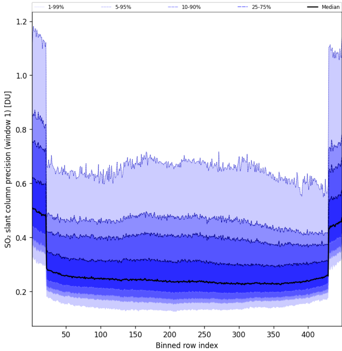
Figure 91: Along track statistics of “SO 2 slant column precision (window 1)” for 2025-08-03 to 2025-08-04
