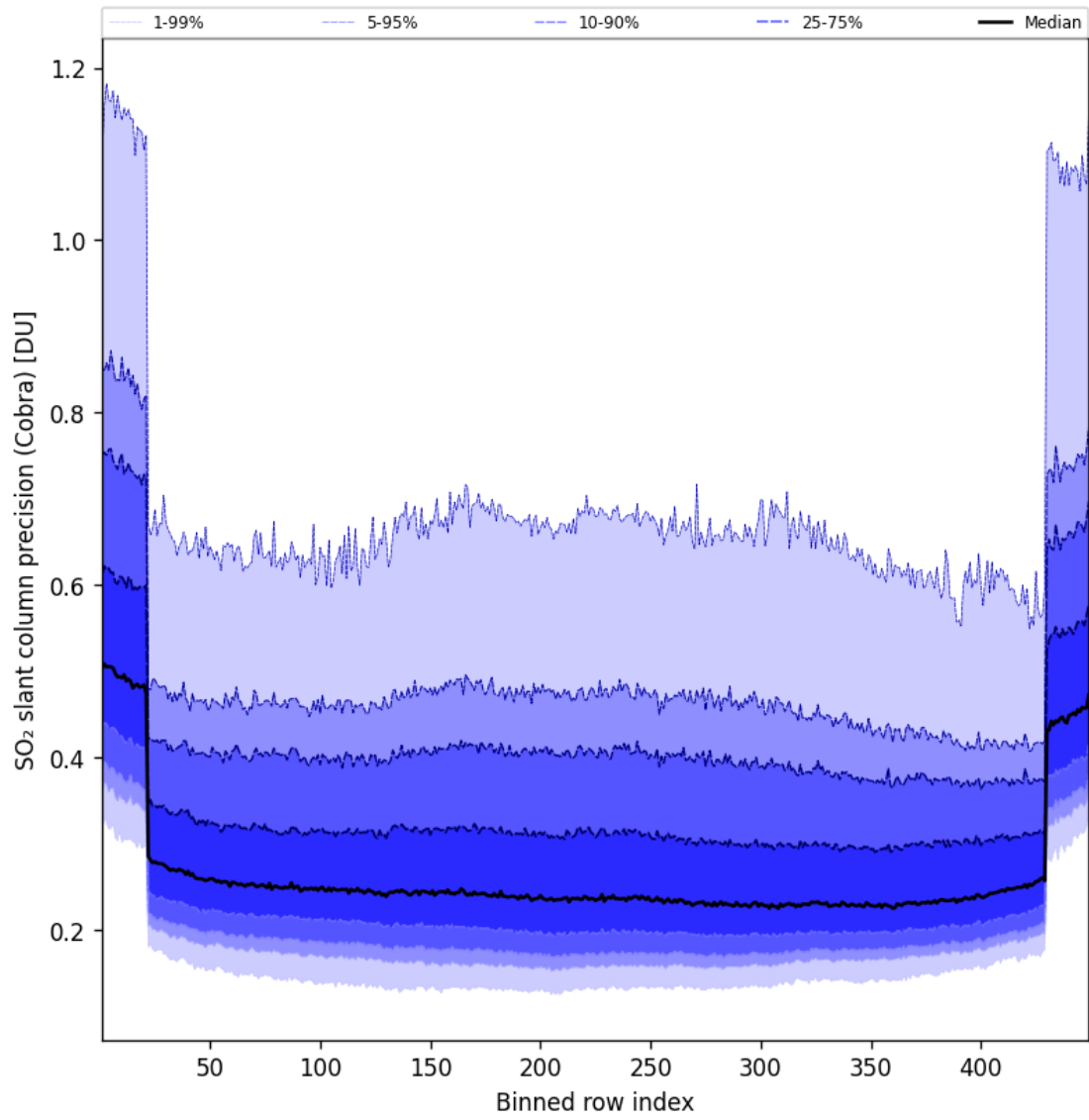
Figure 89: Along track statistics of “SO 2 slant column precision (Cobra)” for 2025-08-03 to 2025-08-04
