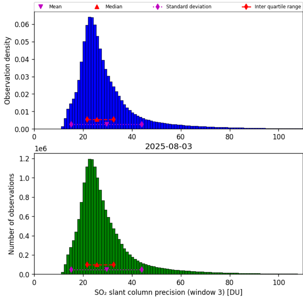
Figure 72: Histogram of “SO 2 slant column precision (window 3)” for 2025-08-03 to 2025-08-04
