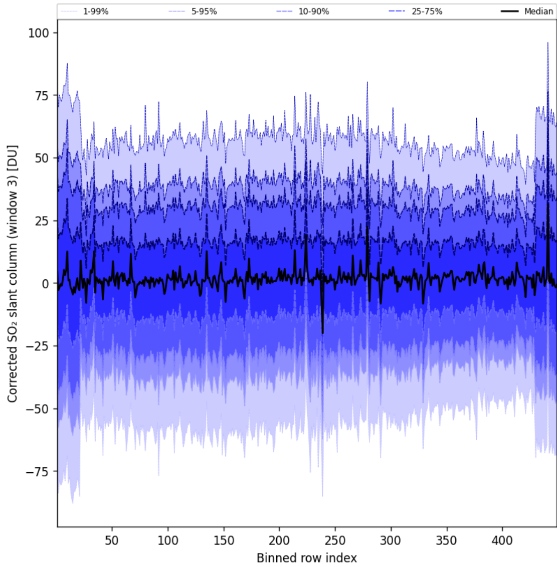
Figure 100: Along track statistics of “Corrected SO 2 slant column (window 3)” for 2025-08-03 to 2025-08-04
