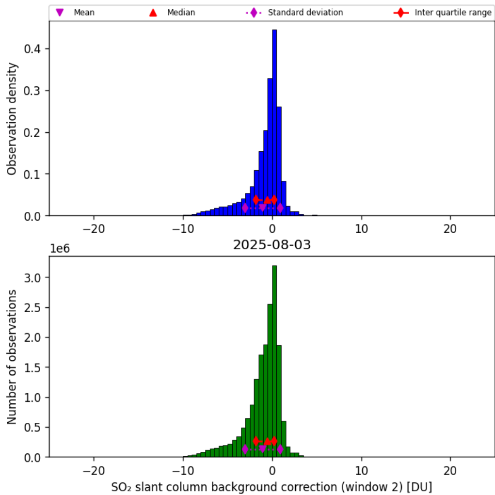
Figure 70: Histogram of “SO 2 slant column background correction (window 2)” for 2025-08-03 to 2025-08-04
