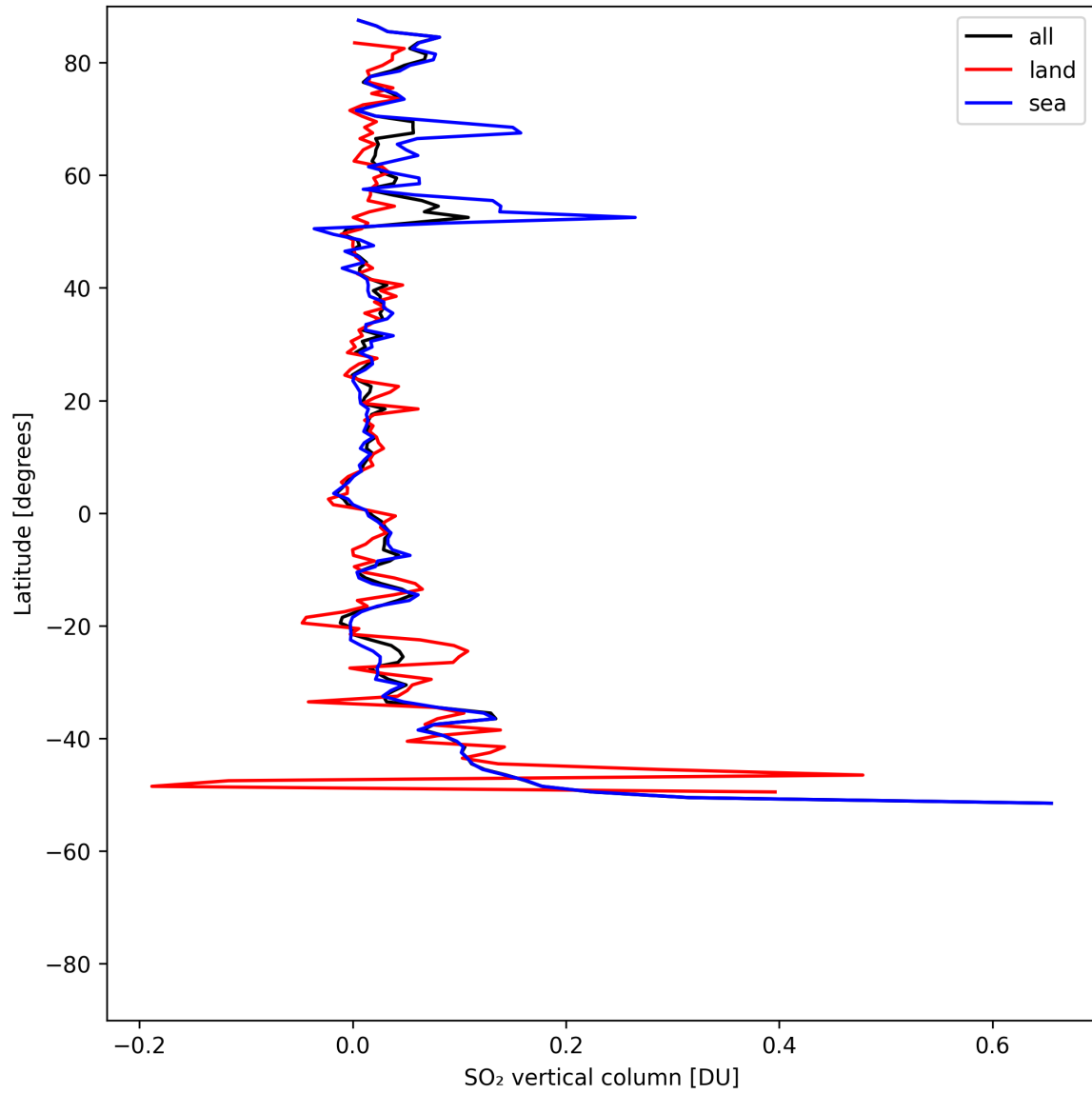
Figure 31: Zonal average of “SO 2 vertical column” for 2025-08-03 to 2025-08-04.
