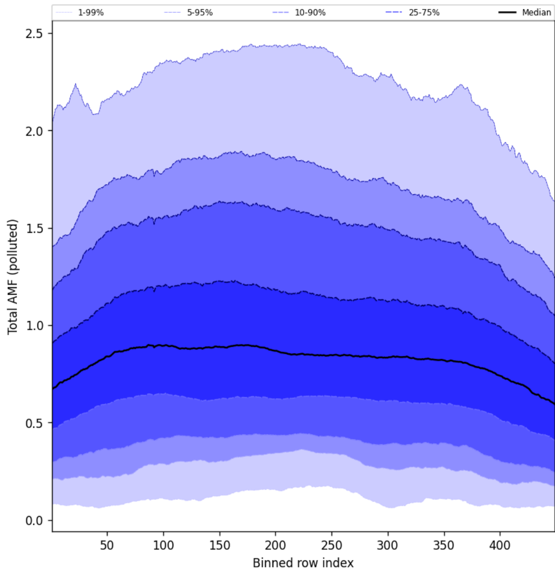
Figure 107: Along track statistics of “Total AMF (polluted)” for 2025-08-03 to 2025-08-04
