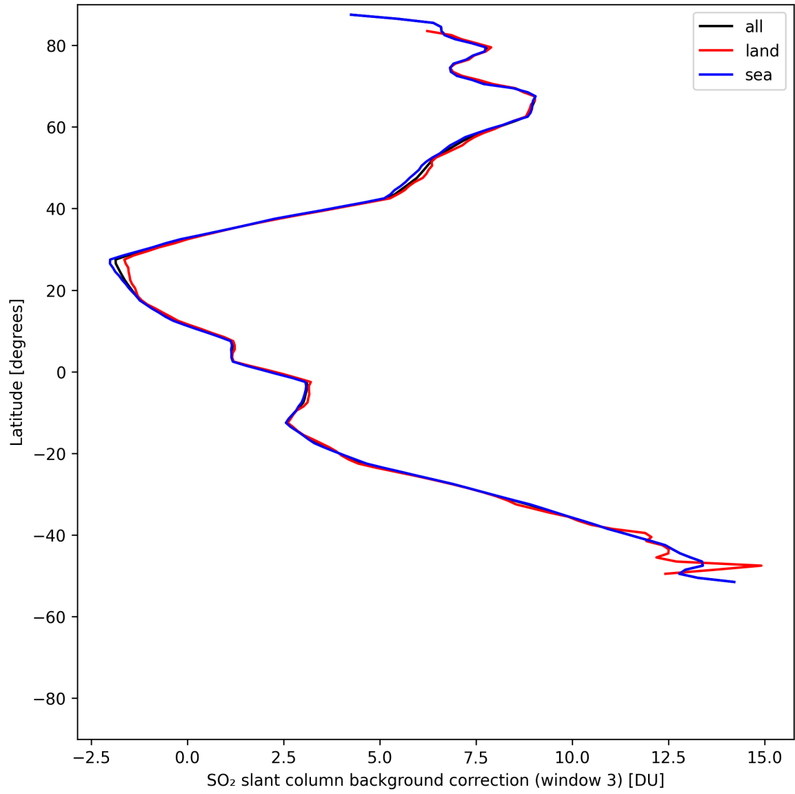
Figure 47: Zonal average of “SO 2 slant column background correction (window 3)” for 2025-08-03 to 2025-08-04.
