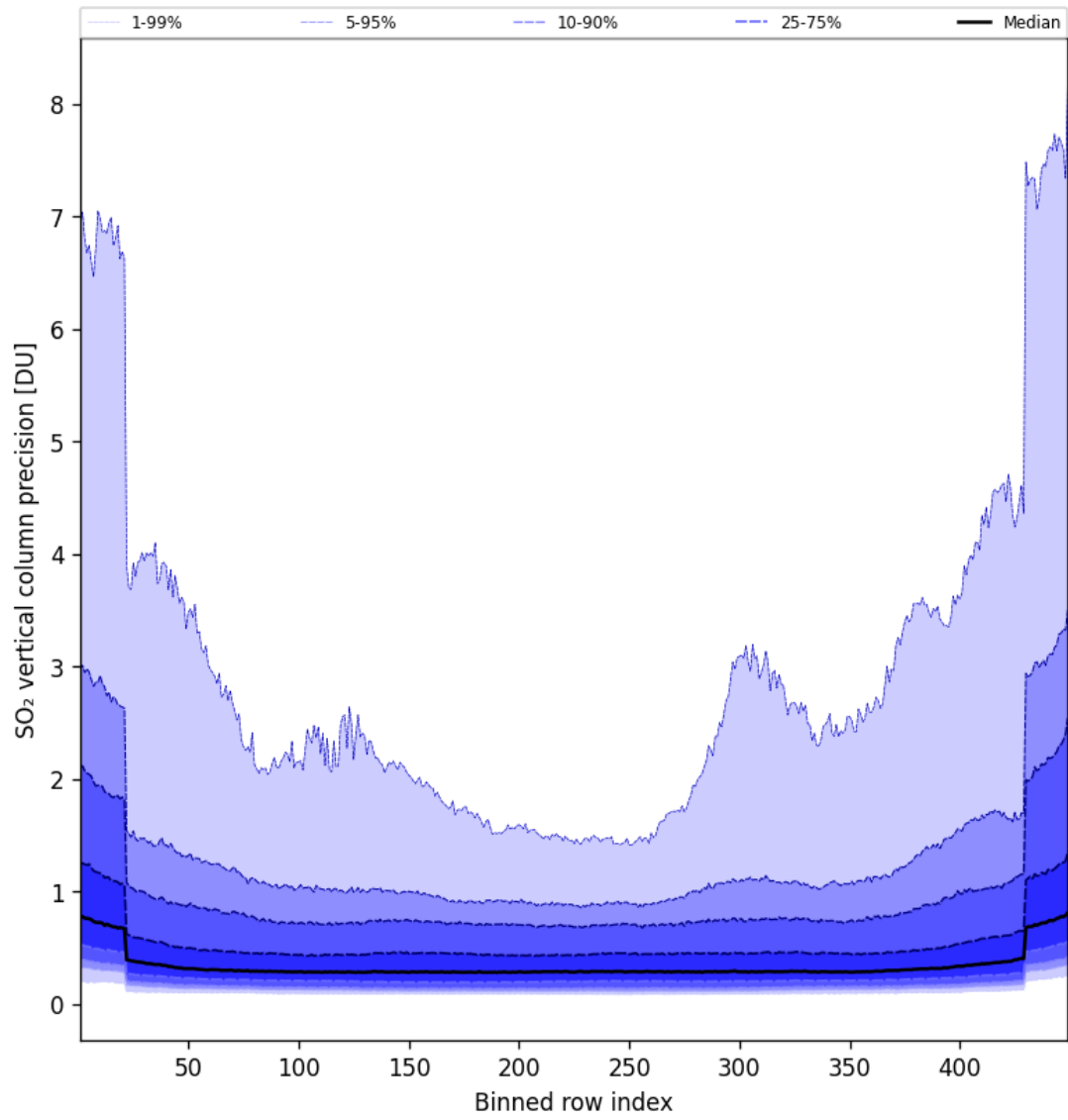
Figure 86: Along track statistics of “SO 2 vertical column precision” for 2025-08-03 to 2025-08-04
