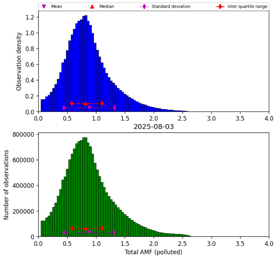
Figure 80: Histogram of “Total AMF (polluted)” for 2025-08-03 to 2025-08-04
