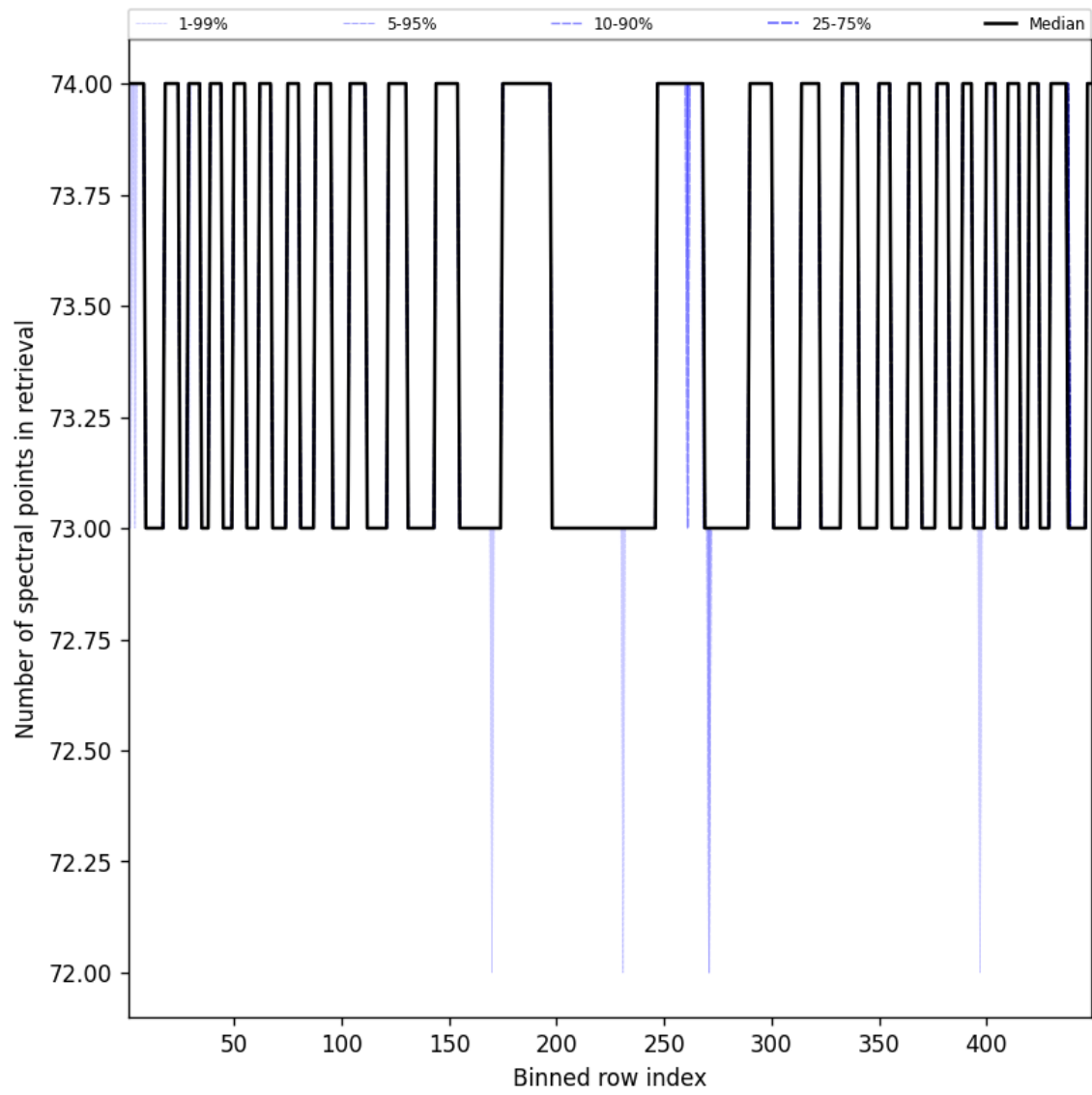
Figure 110: Along track statistics of “Number of spectral points in retrieval” for 2025-08-03 to 2025-08-04
