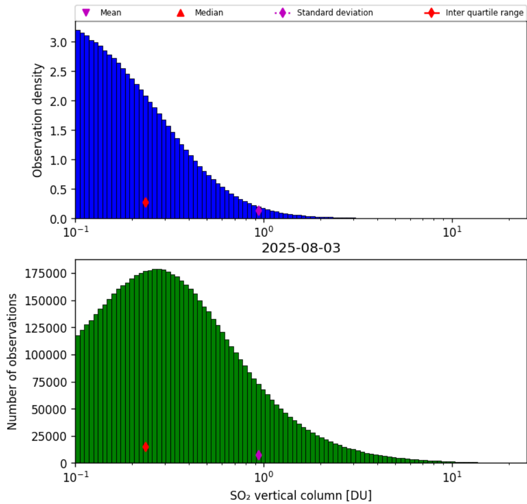
Figure 58: Histogram of “SO 2 vertical column” for 2025-08-03 to 2025-08-04
