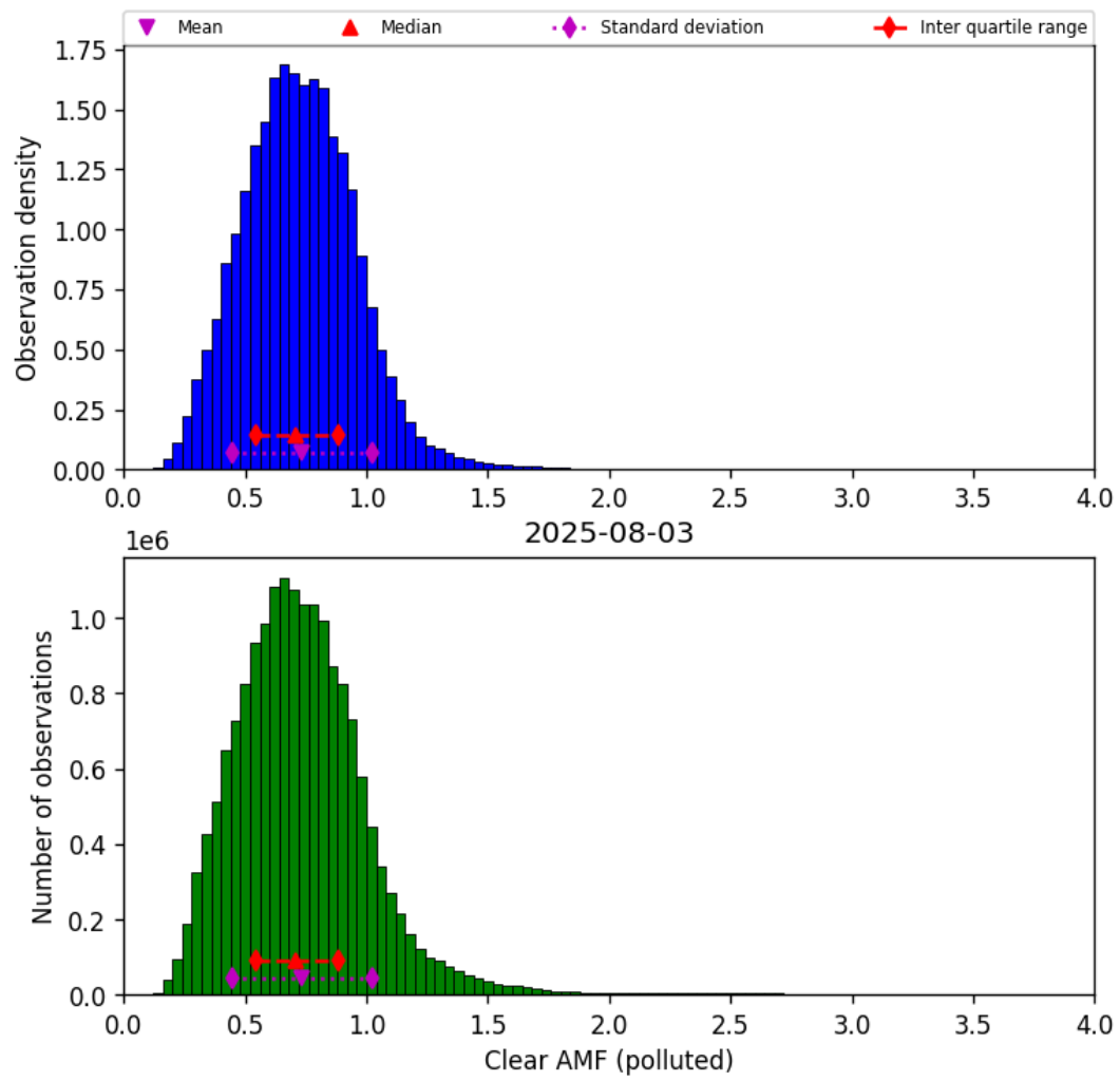
Figure 82: Histogram of “Clear AMF (polluted)” for 2025-08-03 to 2025-08-04
