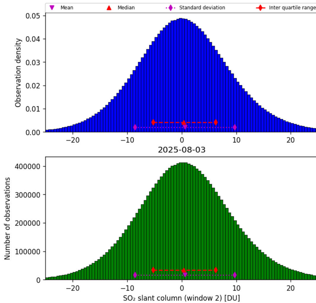
Figure 67: Histogram of “SO 2 slant column (window 2)” for 2025-08-03 to 2025-08-04
