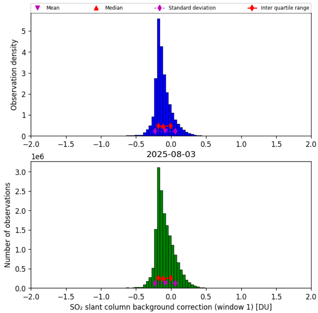
Figure 66: Histogram of “SO 2 slant column background correction (window 1)” for 2025-08-03 to 2025-08-04
