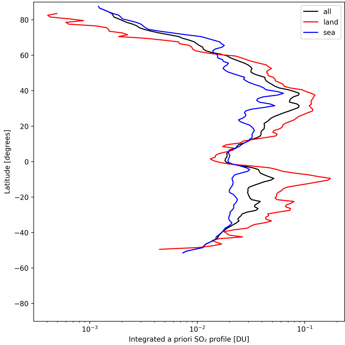
Figure 49: Zonal average of “Integrated a priori SO 2 profile” for 2025-08-03 to 2025-08-04.
