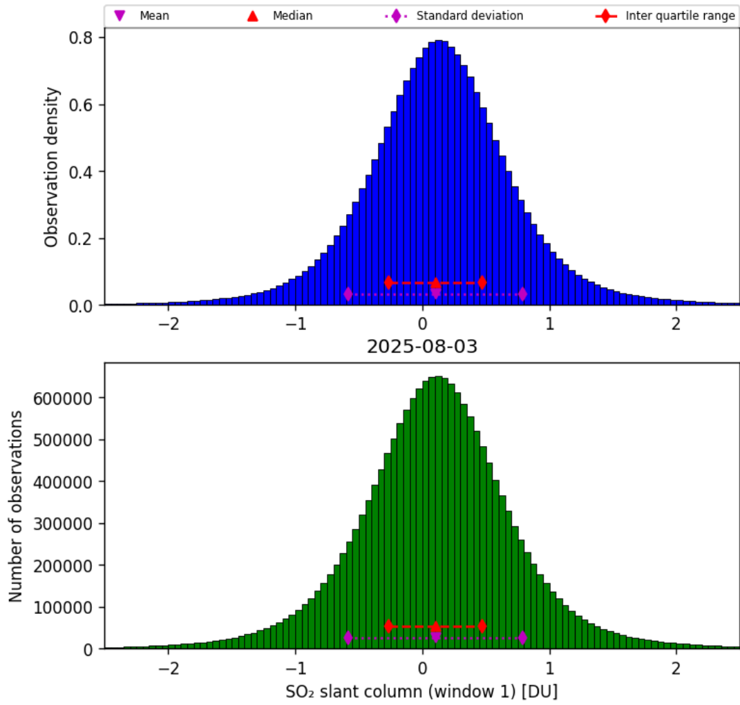
Figure 63: Histogram of “SO 2 slant column (window 1)” for 2025-08-03 to 2025-08-04
