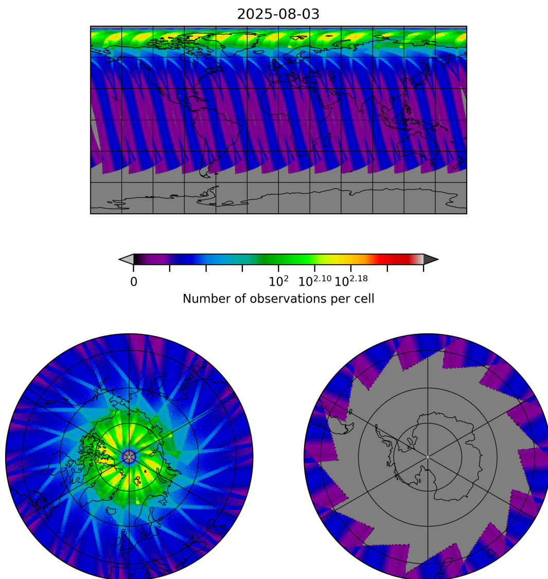
Figure 29: Map of the number of observations for 2025-08-03 to 2025-08-04
