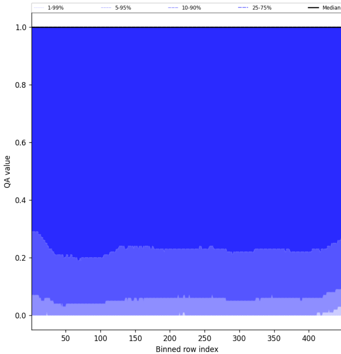
Figure 84: Along track statistics of “QA value” for 2025-08-03 to 2025-08-04
