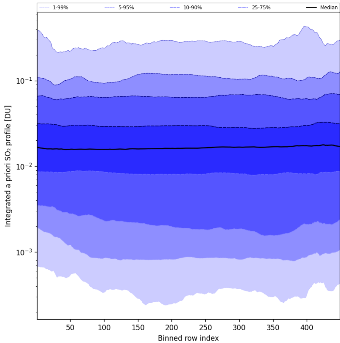
Figure 103: Along track statistics of “Integrated a priori SO 2 profile” for 2025-08-03 to 2025-08-04
