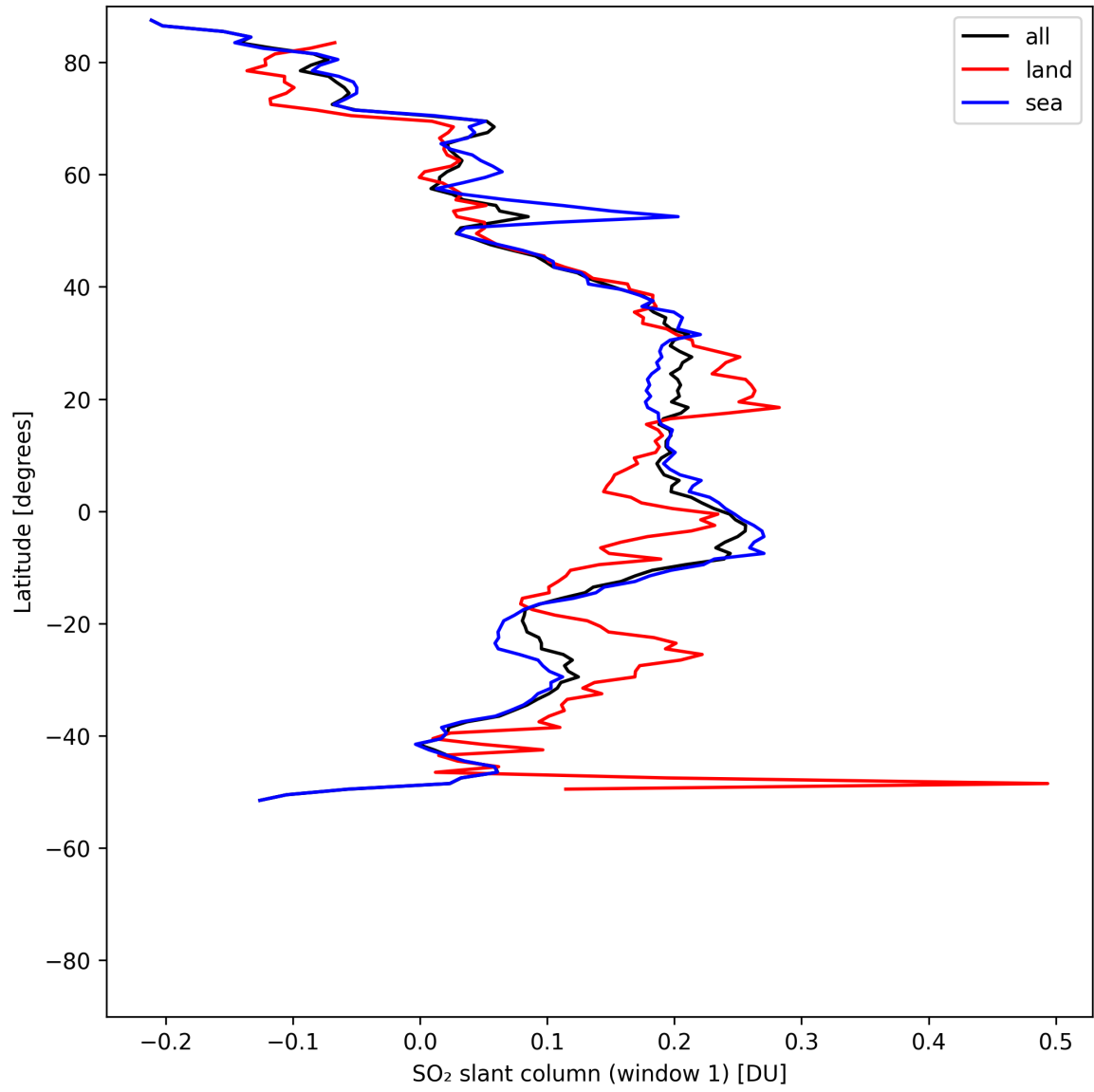
Figure 36: Zonal average of “SO 2 slant column (window 1)” for 2025-08-03 to 2025-08-04.
