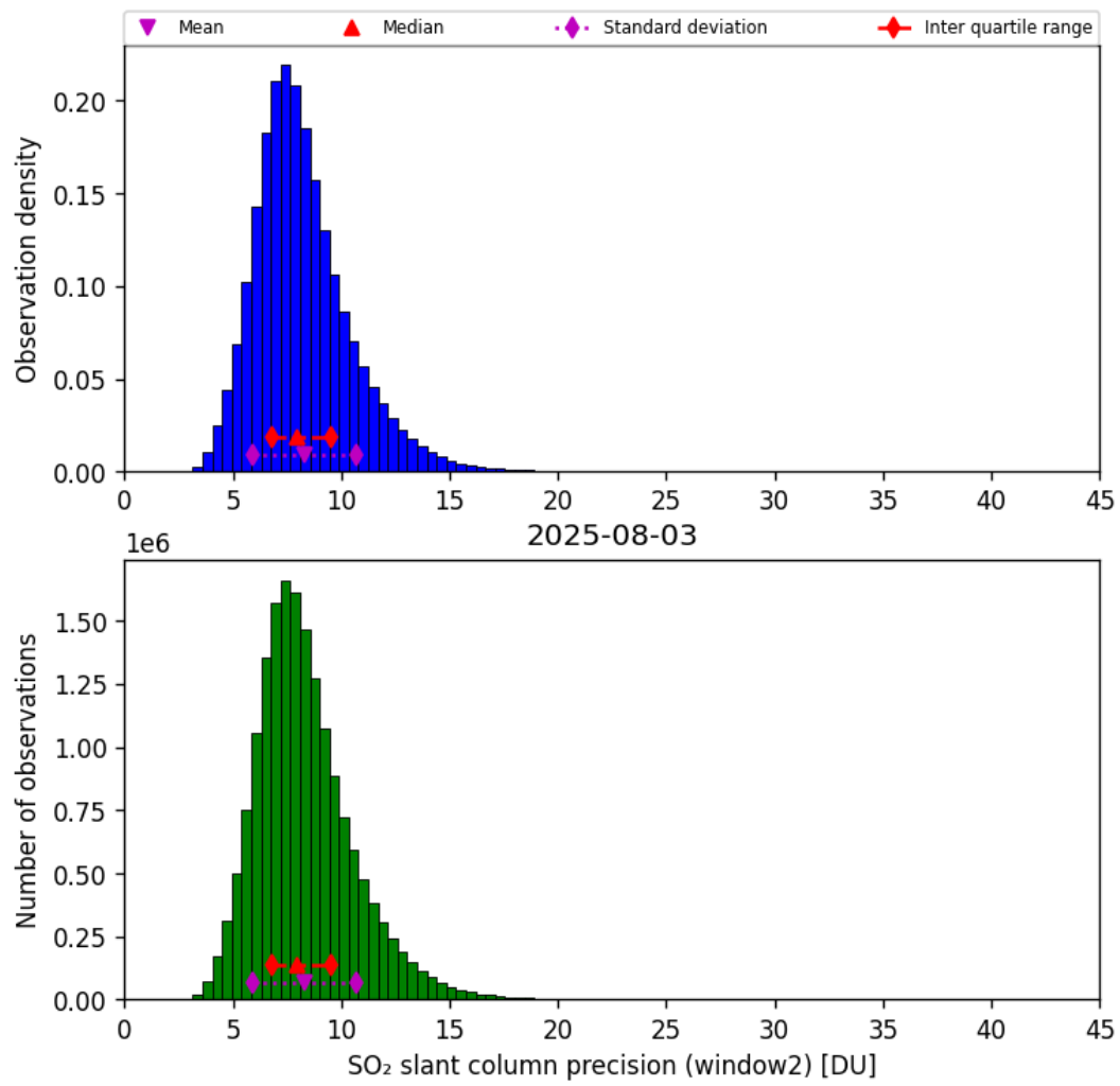
Figure 68: Histogram of “SO 2 slant column precision (window2)” for 2025-08-03 to 2025-08-04
