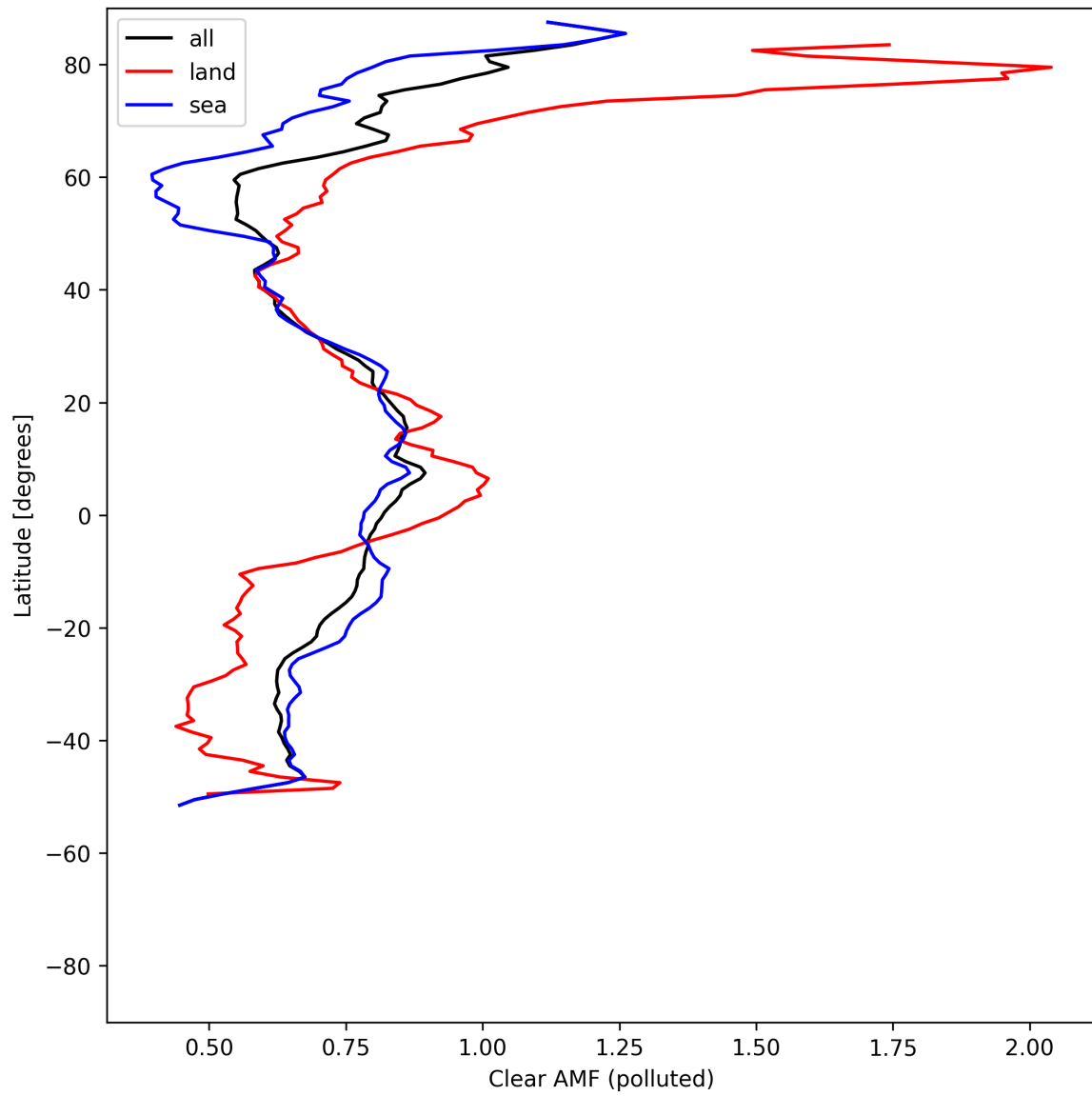
Figure 55: Zonal average of “Clear AMF (polluted)” for 2025-08-03 to 2025-08-04.
