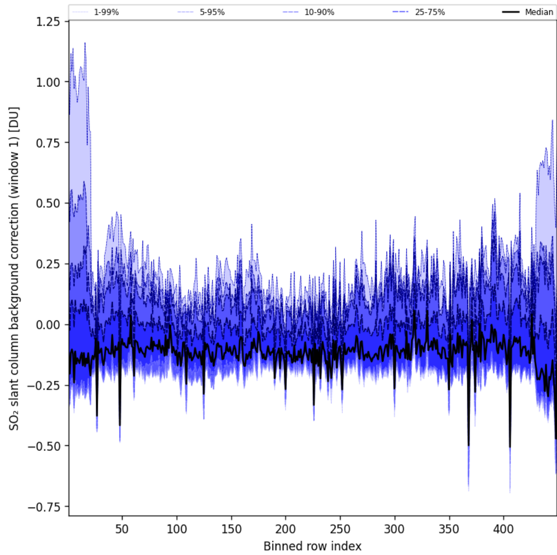
Figure 93: Along track statistics of “SO 2 slant column background correction (window 1)” for 2025-08-03 to 2025-08-04
