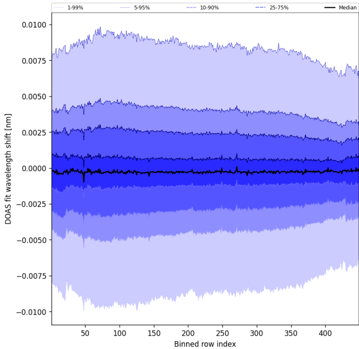
Figure 104: Along track statistics of “DOAS fit wavelength shift” for 2025-08-03 to 2025-08-04
