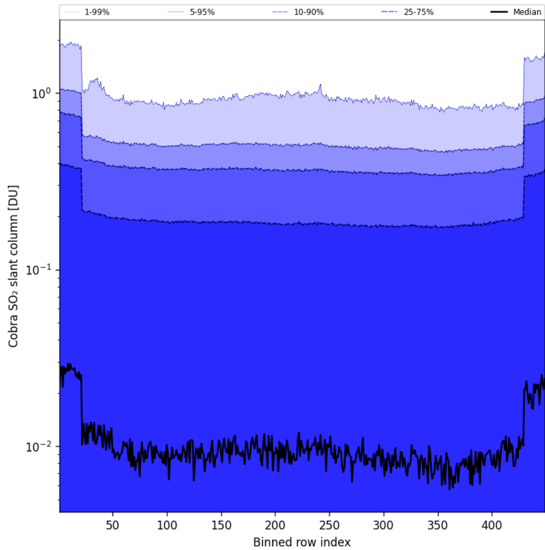
Figure 88: Along track statistics of “Cobra SO 2 slant column” for 2025-08-03 to 2025-08-04
