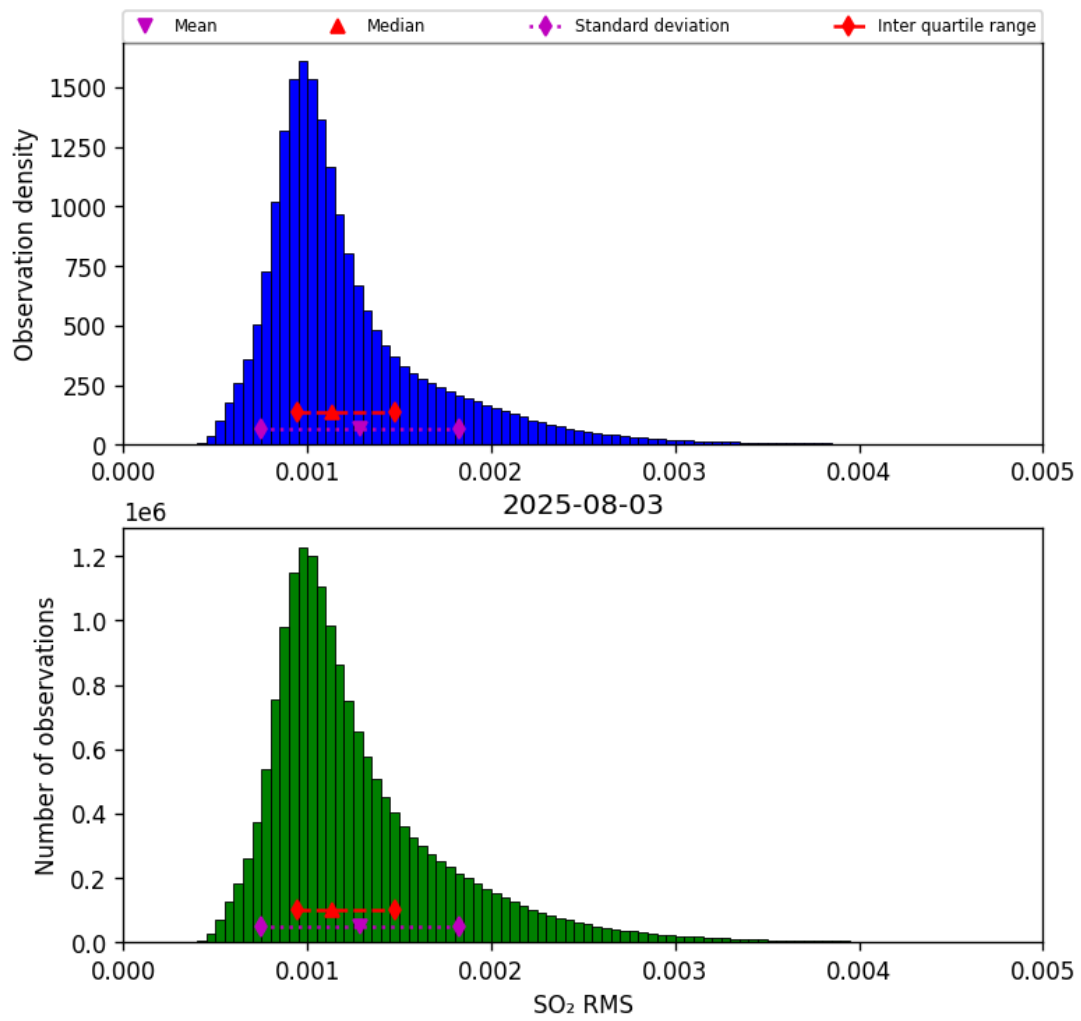
Figure 79: Histogram of “SO 2 RMS” for 2025-08-03 to 2025-08-04
