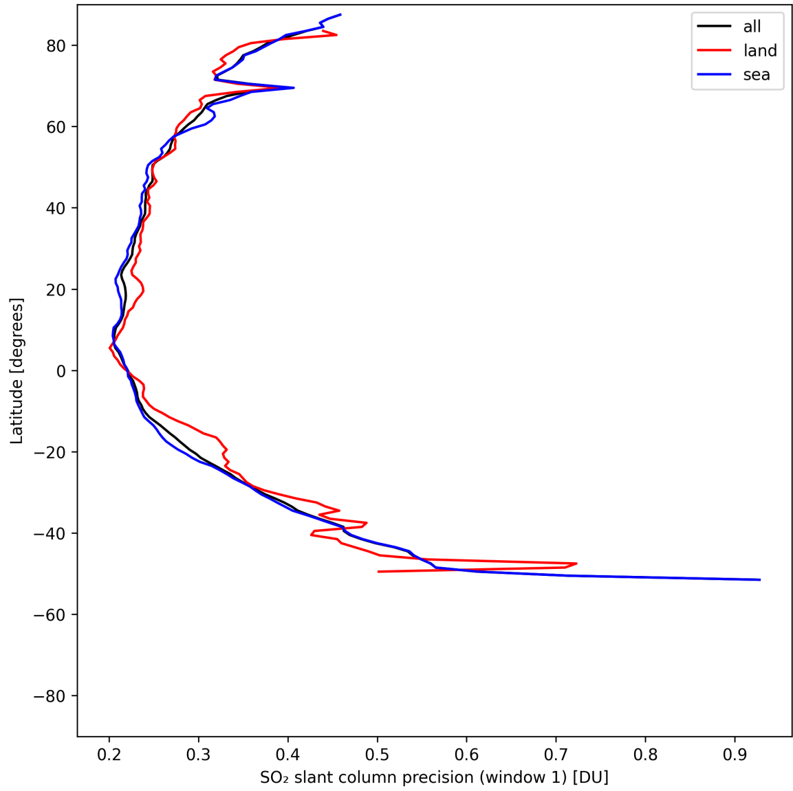
Figure 37: Zonal average of “SO 2 slant column precision (window 1)” for 2025-08-03 to 2025-08-04.
