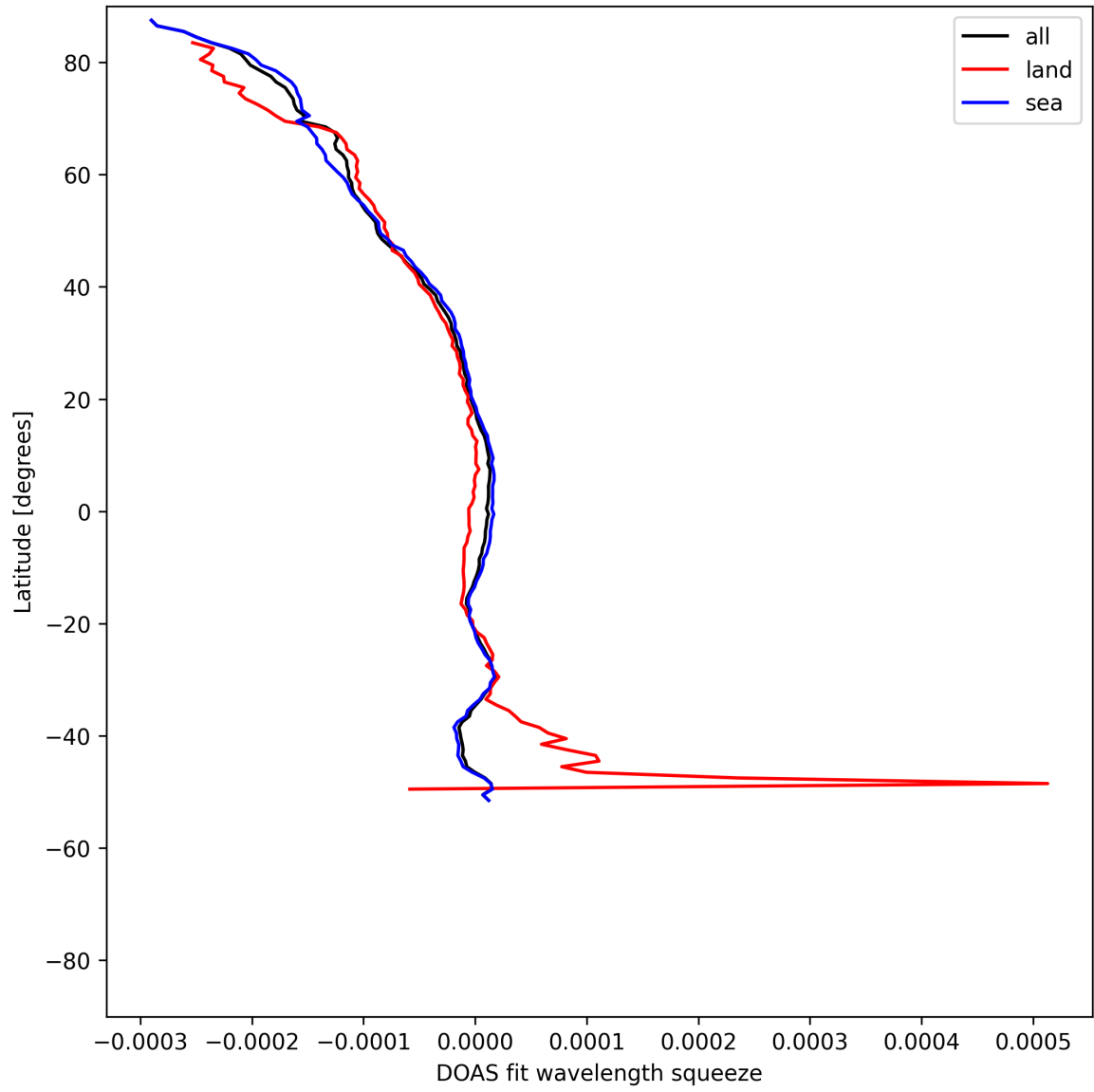
Figure 51: Zonal average of “DOAS fit wavelength squeeze” for 2025-08-03 to 2025-08-04.
