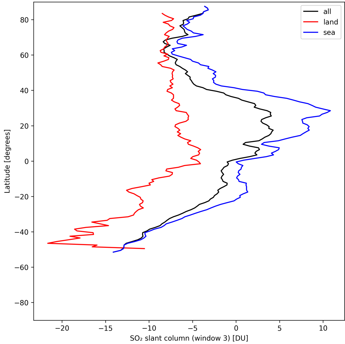
Figure 44: Zonal average of “SO 2 slant column (window 3)” for 2025-08-03 to 2025-08-04.
