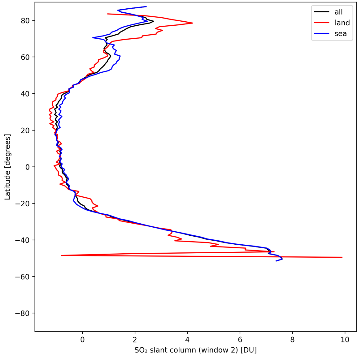
Figure 40: Zonal average of “SO 2 slant column (window 2)” for 2025-08-03 to 2025-08-04.
