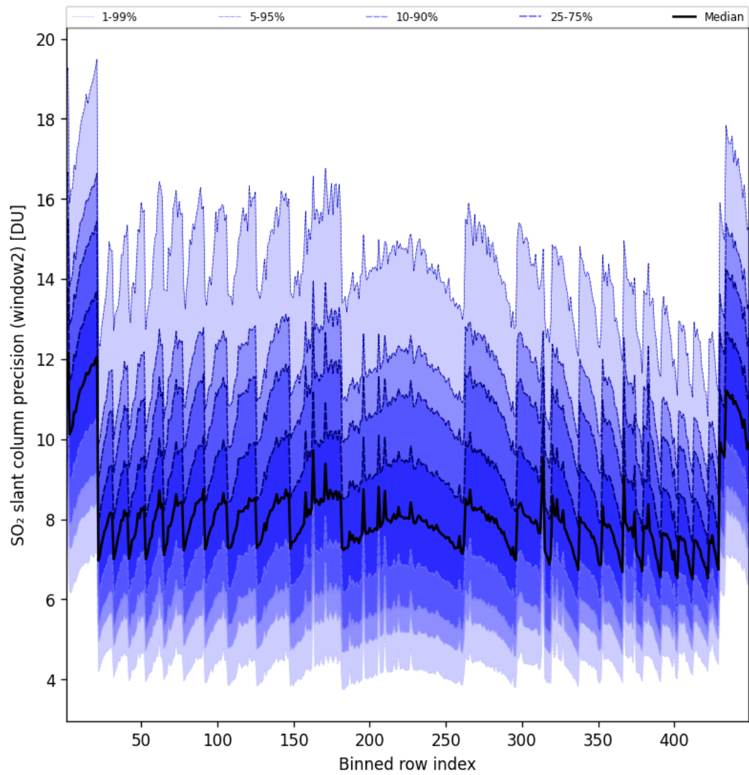
Figure 95: Along track statistics of “SO 2 slant column precision (window2)” for 2025-08-03 to 2025-08-04
