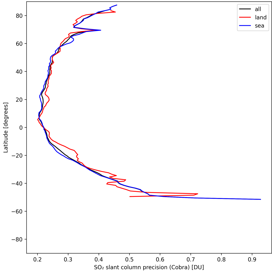
Figure 35: Zonal average of “SO 2 slant column precision (Cobra)” for 2025-08-03 to 2025-08-04.
