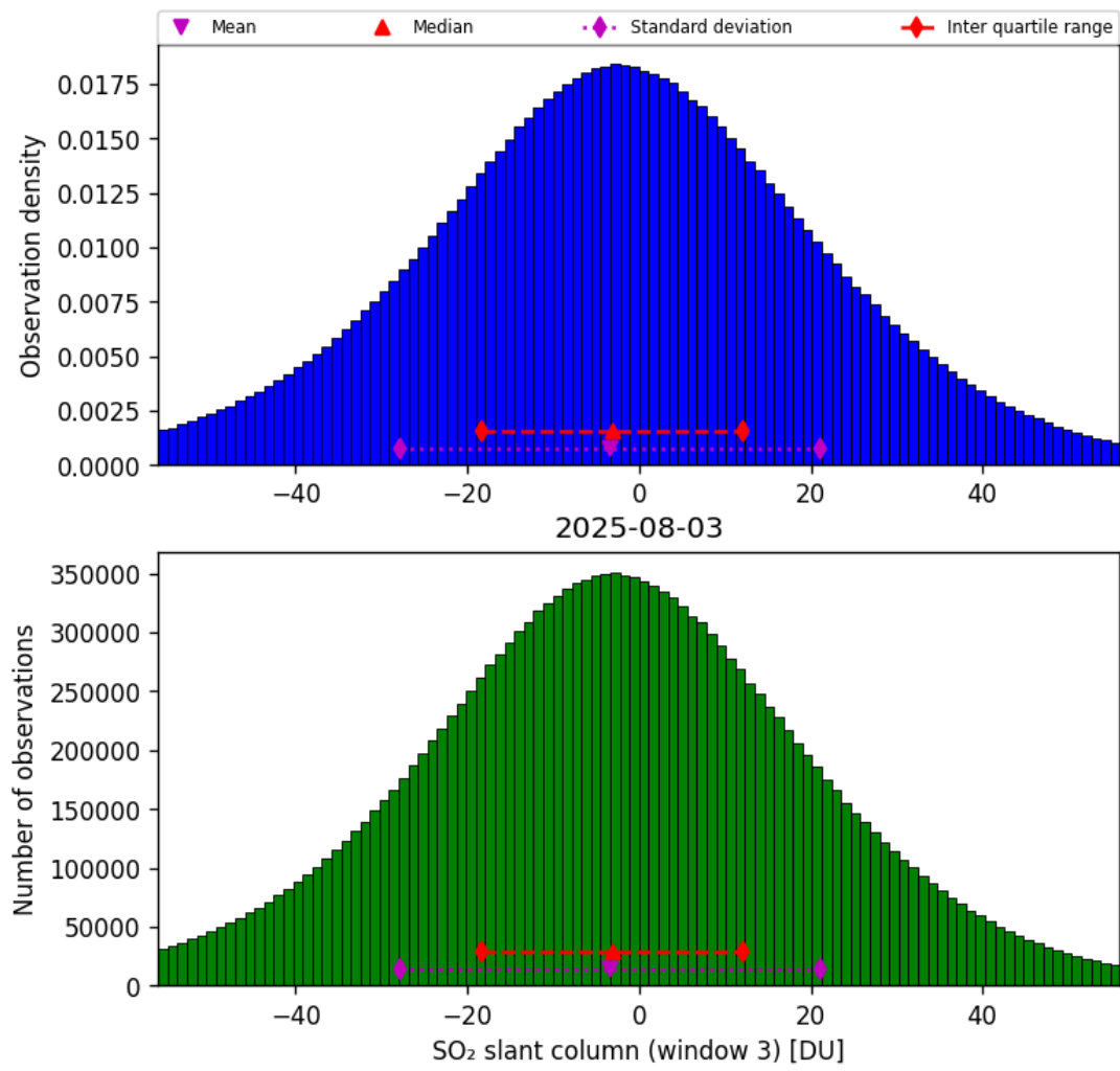
Figure 71: Histogram of “SO 2 slant column (window 3)” for 2025-08-03 to 2025-08-04
