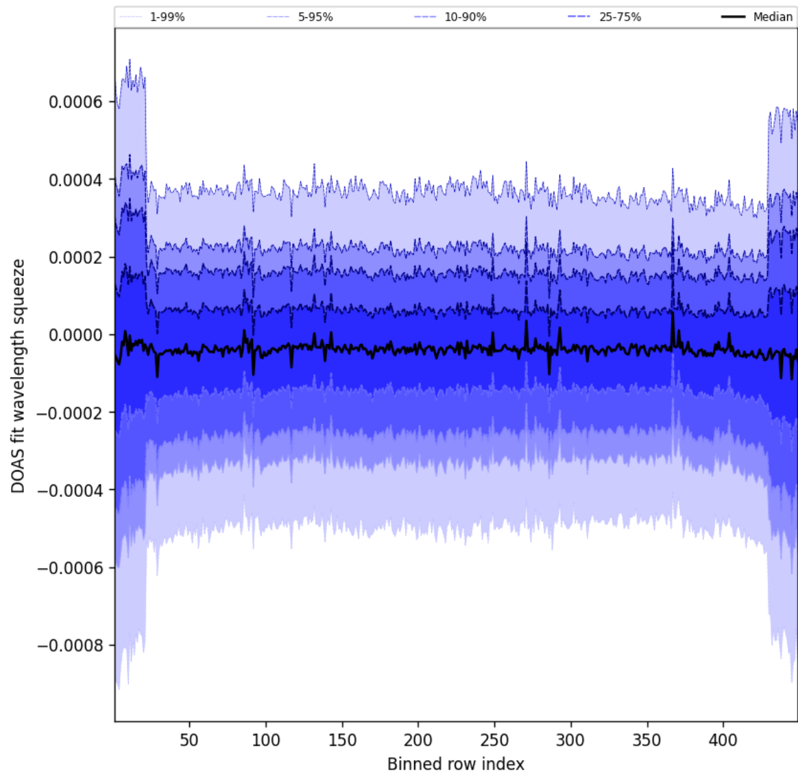
Figure 105: Along track statistics of “DOAS fit wavelength squeeze” for 2025-08-03 to 2025-08-04
