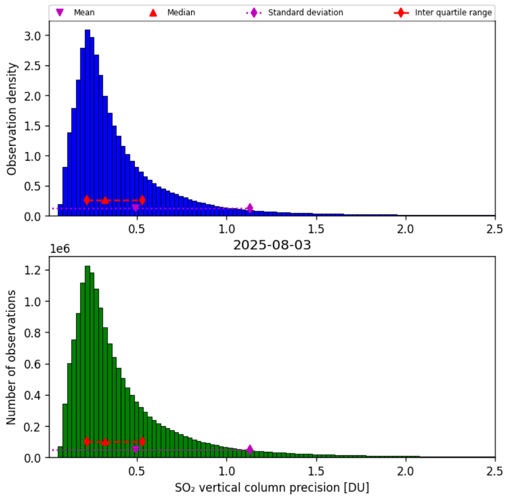
Figure 59: Histogram of “SO 2 vertical column precision” for 2025-08-03 to 2025-08-04
