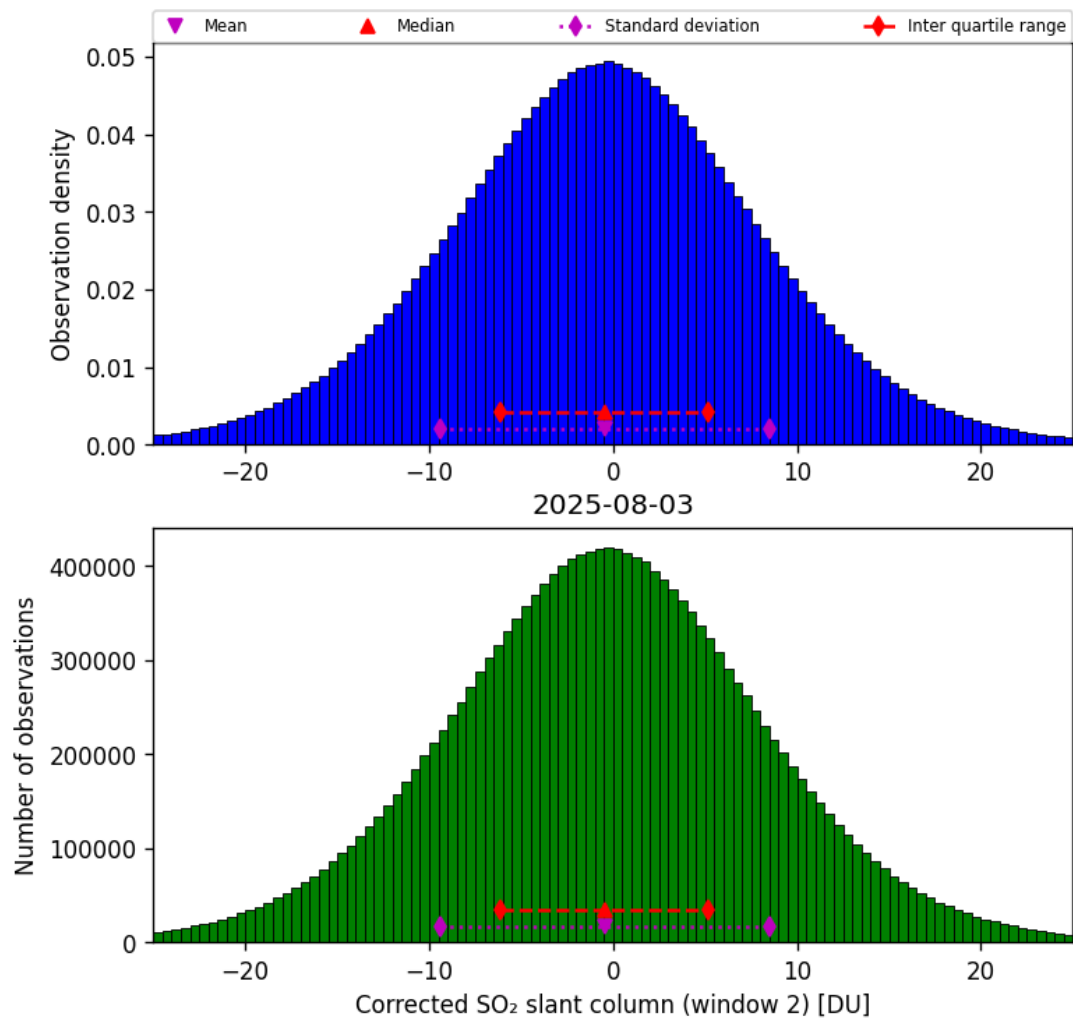
Figure 69: Histogram of “Corrected SO 2 slant column (window 2)” for 2025-08-03 to 2025-08-04
