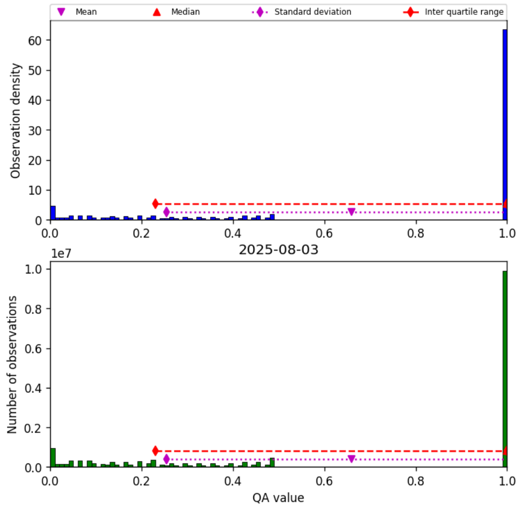
Figure 57: Histogram of “QA value” for 2025-08-03 to 2025-08-04
