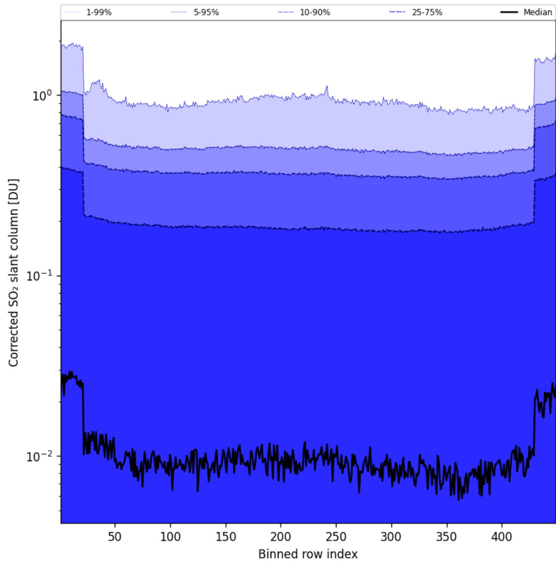
Figure 87: Along track statistics of “Corrected SO 2 slant column” for 2025-08-03 to 2025-08-04
