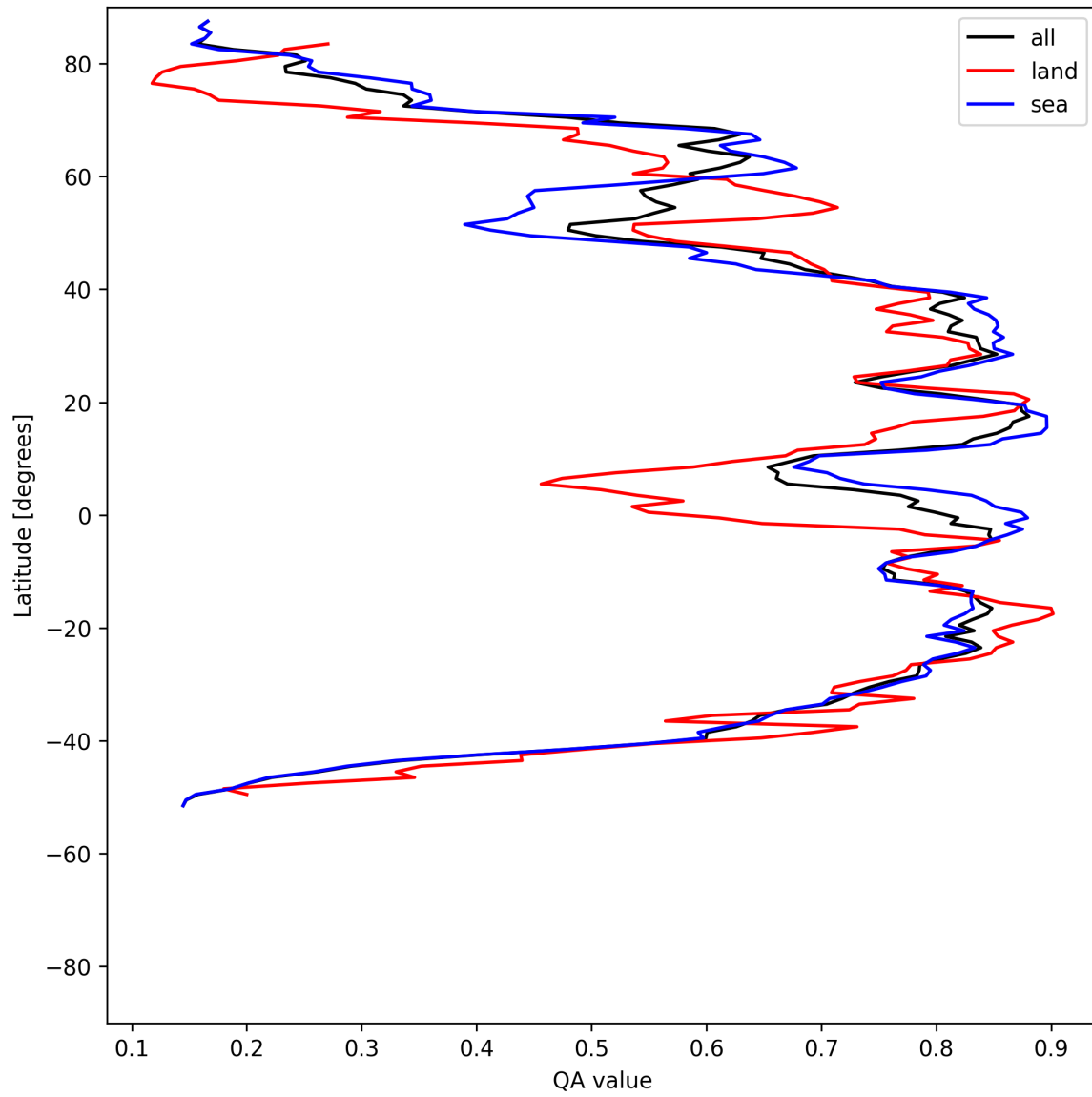
Figure 30: Zonal average of “QA value” for 2025-08-03 to 2025-08-04.
