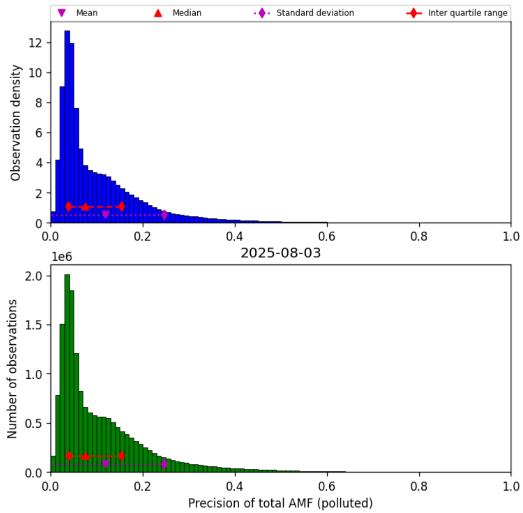
Figure 81: Histogram of “Precision of total AMF (polluted)” for 2025-08-03 to 2025-08-04
