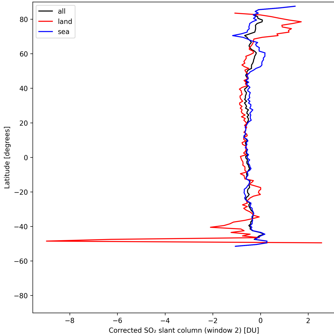
Figure 42: Zonal average of “Corrected SO 2 slant column (window 2)” for 2025-08-03 to 2025-08-04.
