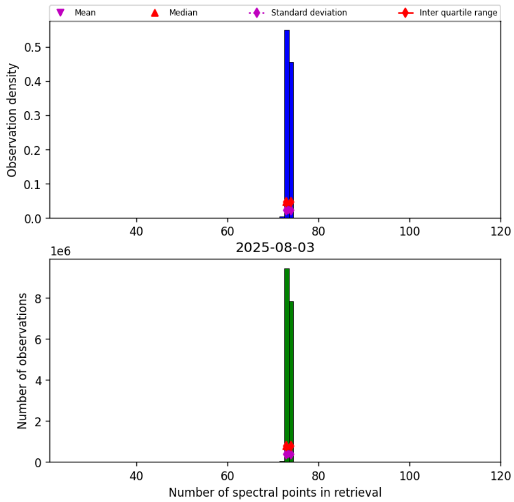
Figure 83: Histogram of “Number of spectral points in retrieval” for 2025-08-03 to 2025-08-04
