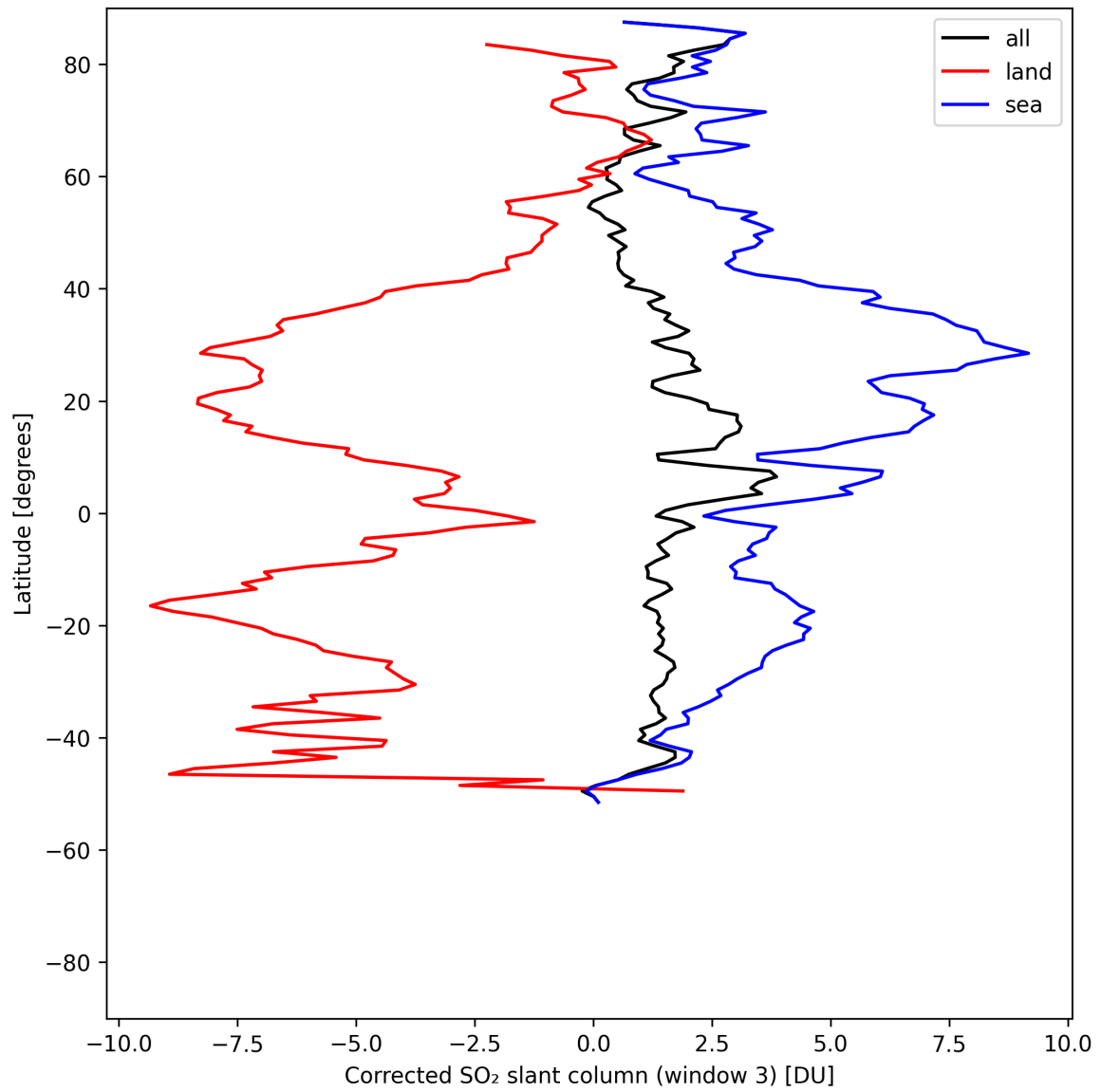
Figure 46: Zonal average of “Corrected SO 2 slant column (window 3)” for 2025-08-03 to 2025-08-04.
