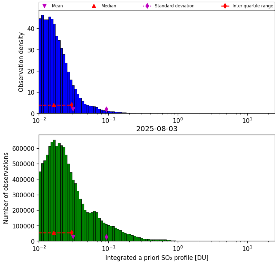
Figure 76: Histogram of “Integrated a priori SO 2 profile” for 2025-08-03 to 2025-08-04
