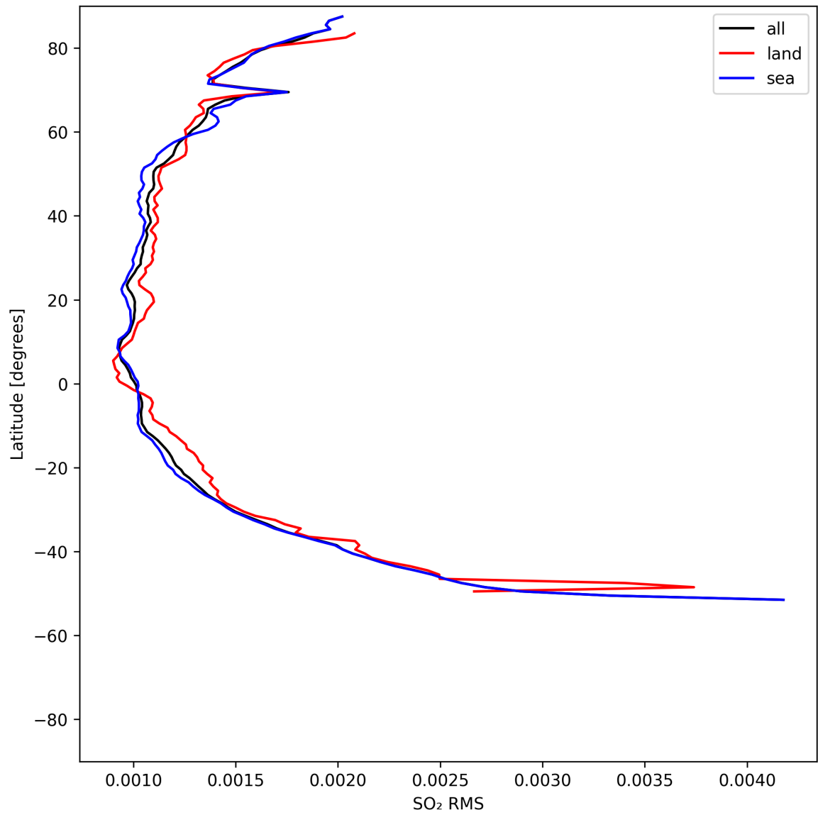
Figure 52: Zonal average of “SO 2 RMS” for 2025-08-03 to 2025-08-04.
