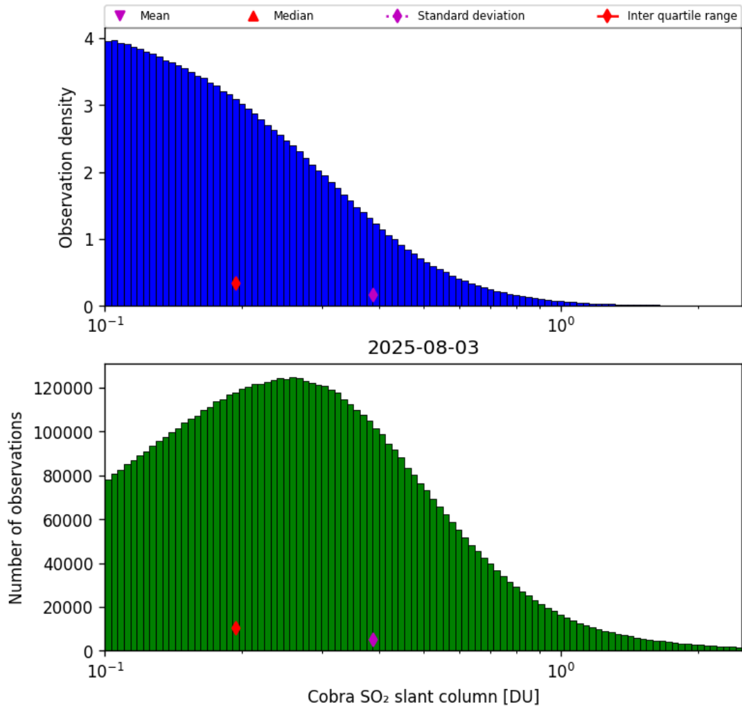
Figure 61: Histogram of “Cobra SO 2 slant column” for 2025-08-03 to 2025-08-04
