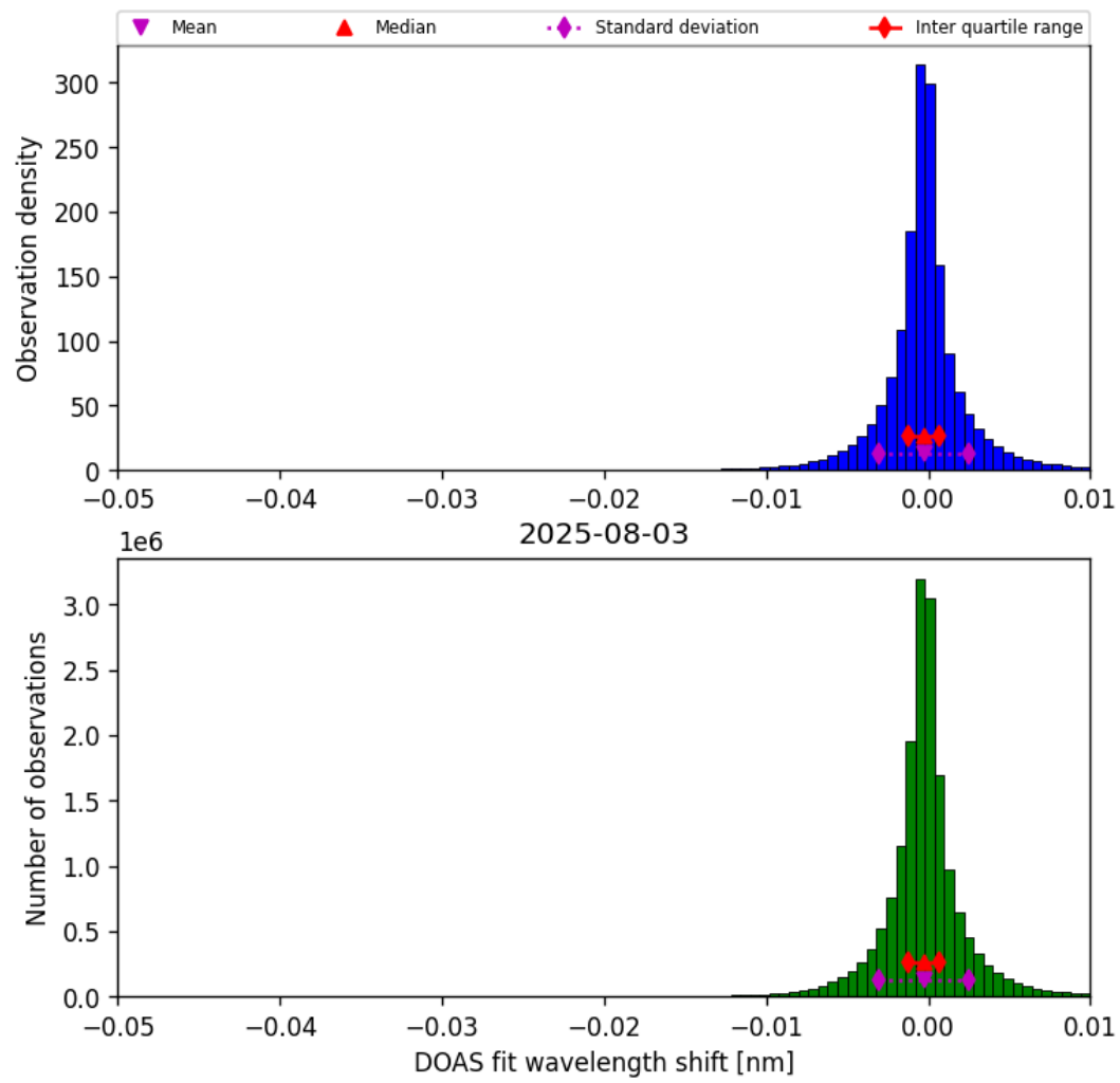
Figure 77: Histogram of “DOAS fit wavelength shift” for 2025-08-03 to 2025-08-04
