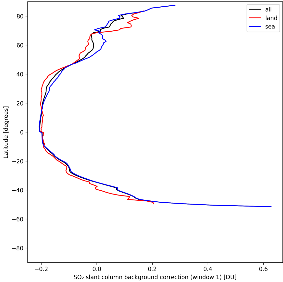
Figure 39: Zonal average of “SO 2 slant column background correction (window 1)” for 2025-08-03 to 2025-08-04.
