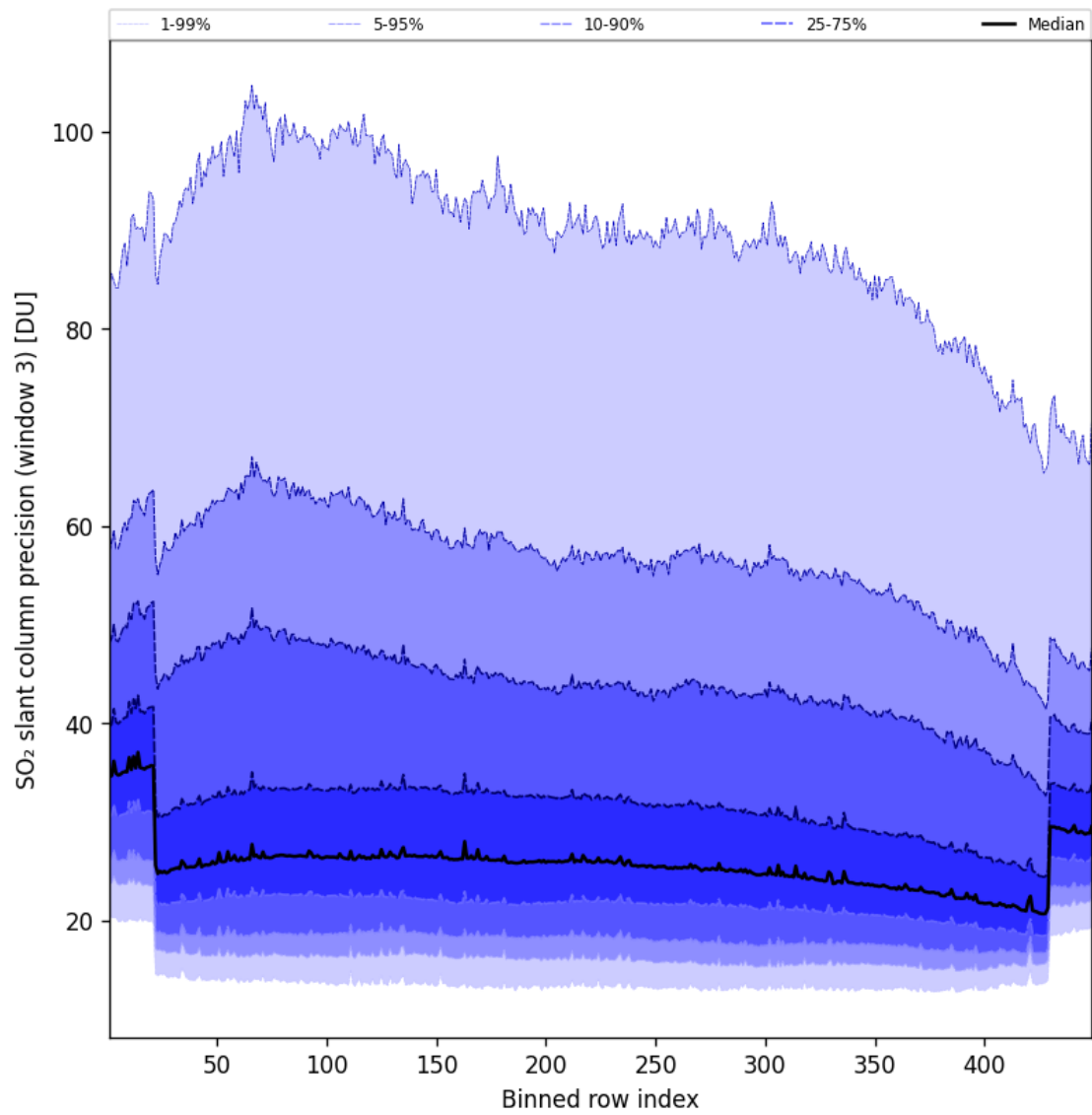
Figure 99: Along track statistics of “SO 2 slant column precision (window 3)” for 2025-08-03 to 2025-08-04
