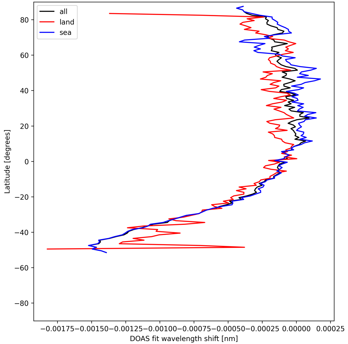
Figure 50: Zonal average of “DOAS fit wavelength shift” for 2025-08-03 to 2025-08-04.
