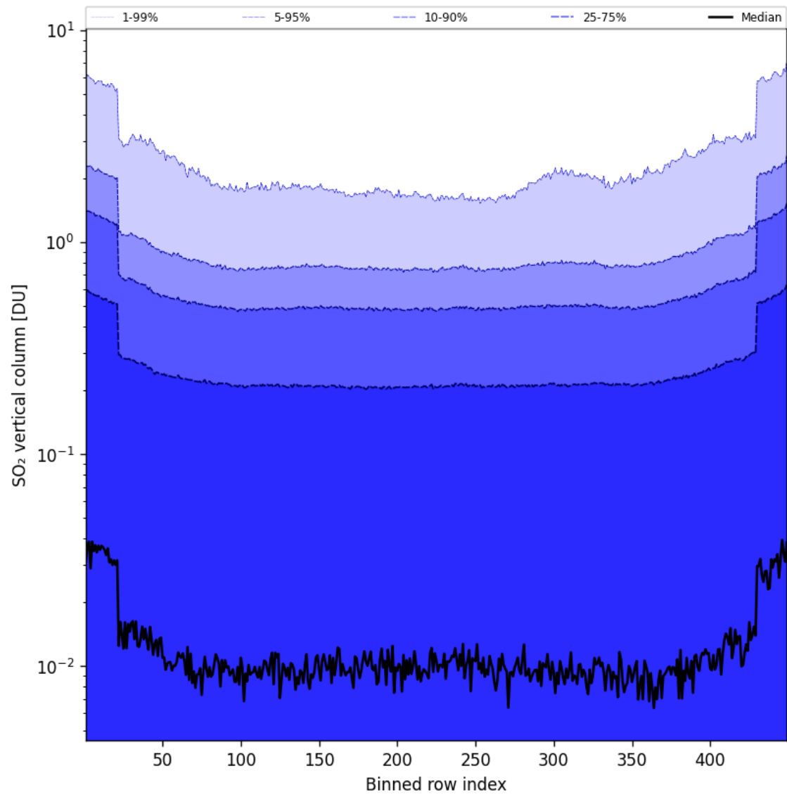
Figure 85: Along track statistics of “SO 2 vertical column” for 2025-08-03 to 2025-08-04
