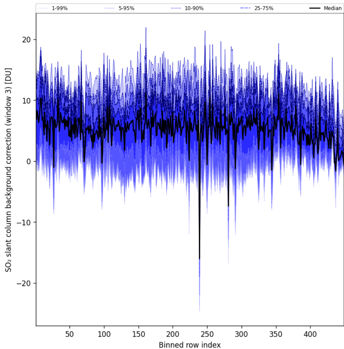
Figure 101: Along track statistics of “SO 2 slant column background correction (window 3)” for 2025-08-03 to 2025-08-04
