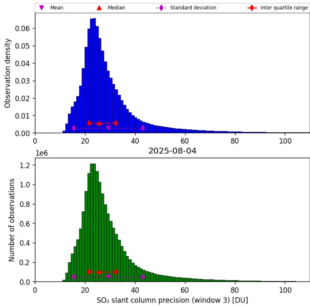
Figure 72: Histogram of “SO 2 slant column precision (window 3)” for 2025-08-04 to 2025-08-05
