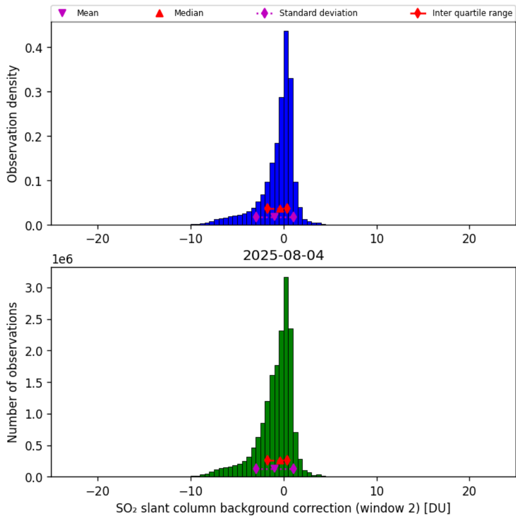
Figure 70: Histogram of “SO 2 slant column background correction (window 2)” for 2025-08-04 to 2025-08-05
