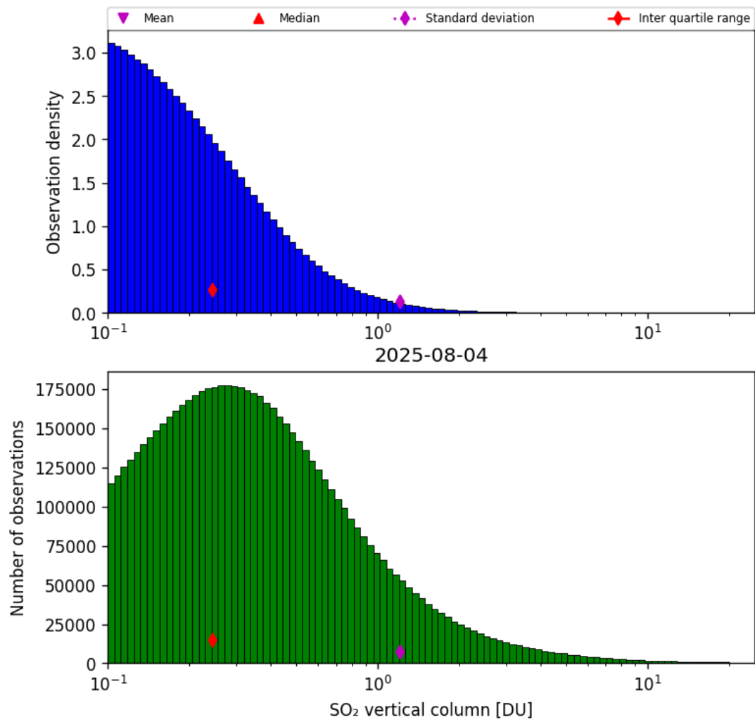
Figure 58: Histogram of “SO 2 vertical column” for 2025-08-04 to 2025-08-05
