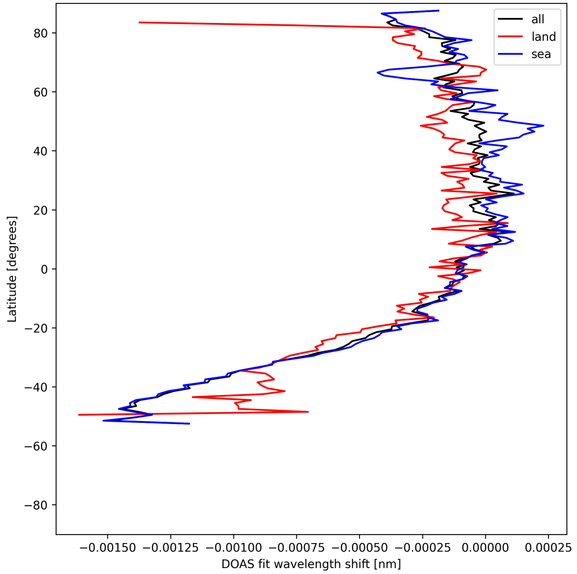
Figure 50: Zonal average of “DOAS fit wavelength shift” for 2025-08-04 to 2025-08-05.
