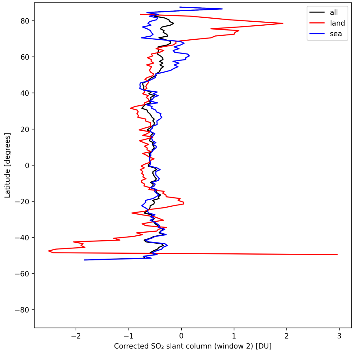
Figure 42: Zonal average of “Corrected SO 2 slant column (window 2)” for 2025-08-04 to 2025-08-05.
