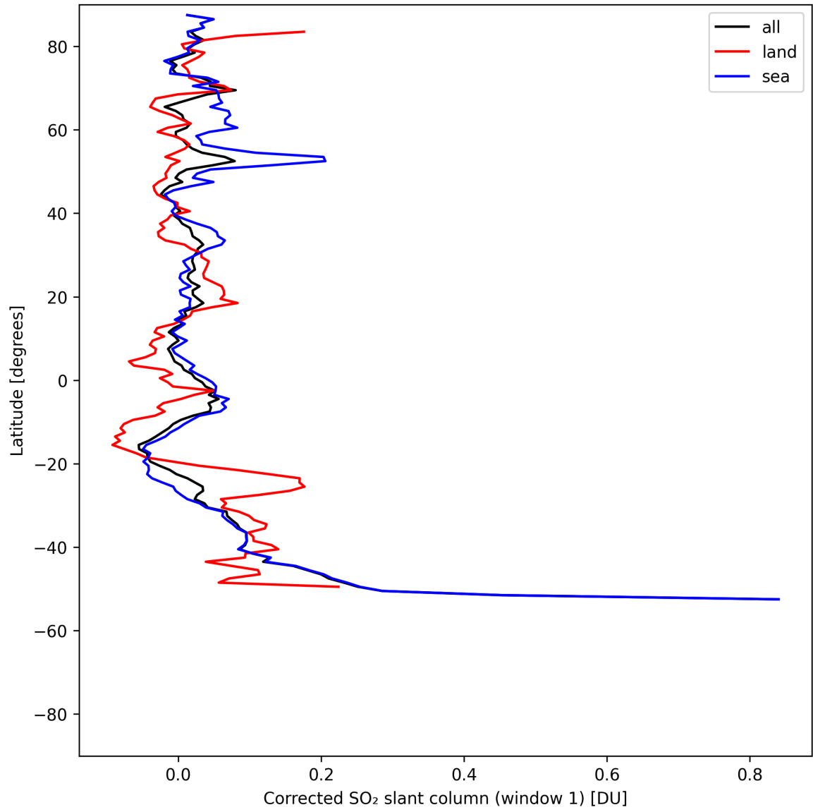
Figure 38: Zonal average of “Corrected SO 2 slant column (window 1)” for 2025-08-04 to 2025-08-05.
