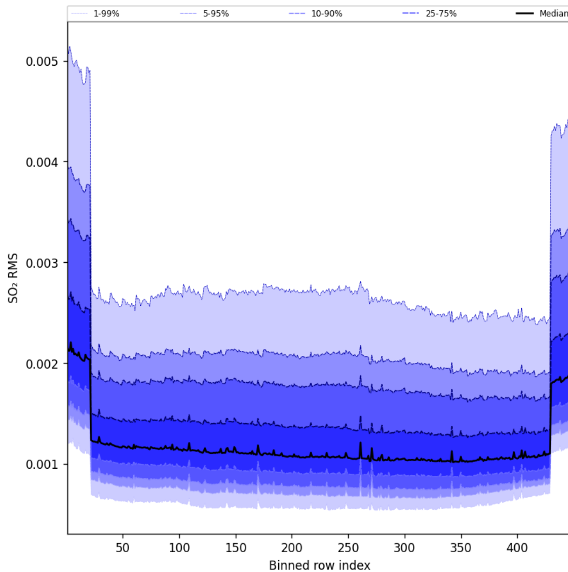
Figure 106: Along track statistics of “SO 2 RMS” for 2025-08-04 to 2025-08-05
