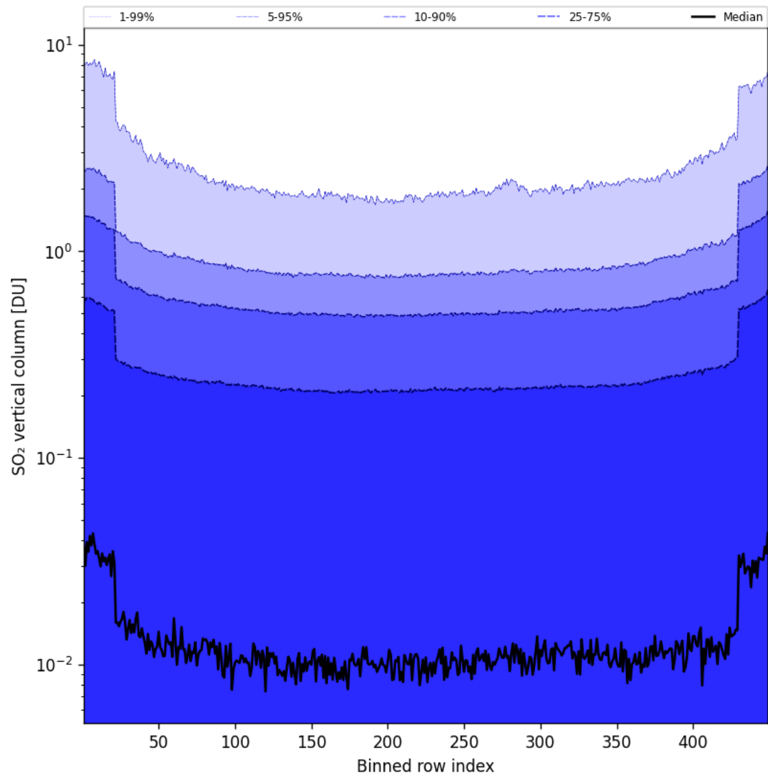
Figure 85: Along track statistics of “SO 2 vertical column” for 2025-08-04 to 2025-08-05
