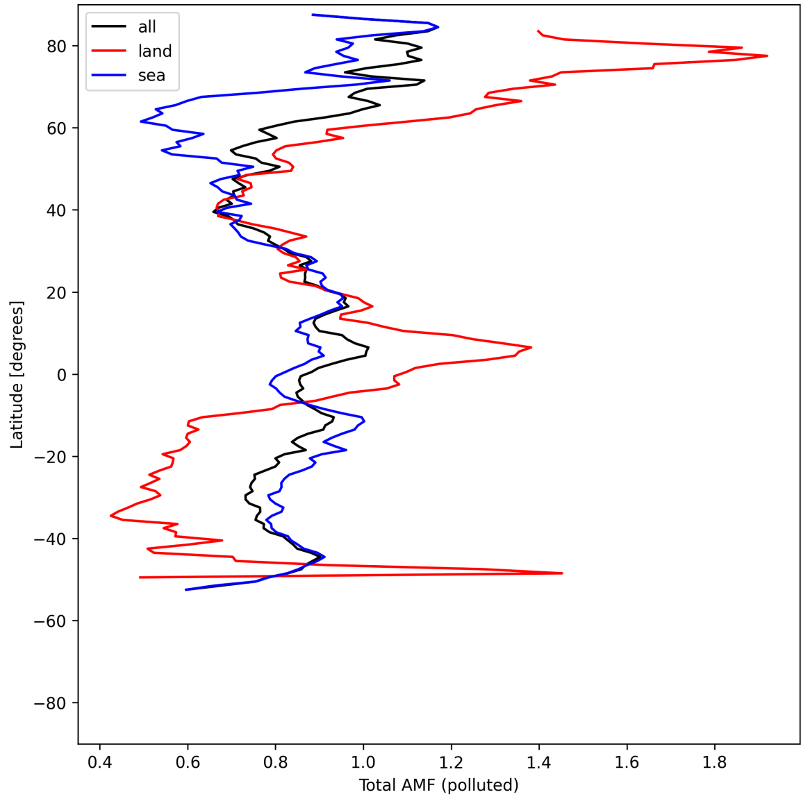
Figure 53: Zonal average of “Total AMF (polluted)” for 2025-08-04 to 2025-08-05.
