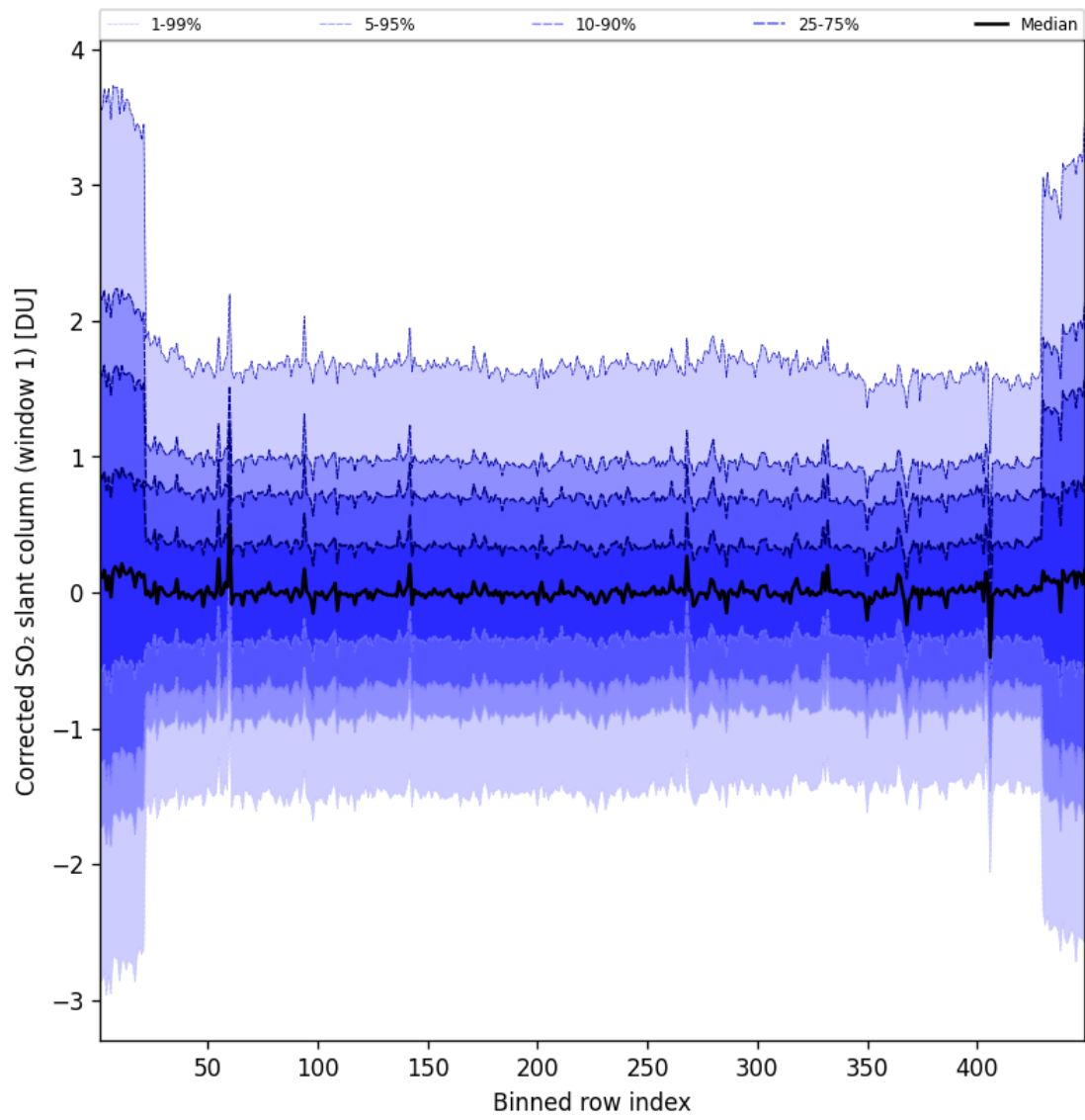
Figure 92: Along track statistics of "Corrected SO 2 slant column (window 1)" for 2025-08-04 to 2025-08-05
