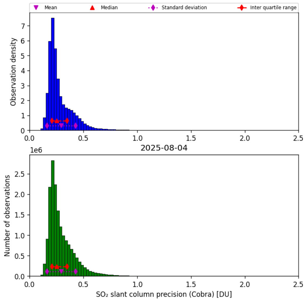
Figure 62: Histogram of “SO 2 slant column precision (Cobra)” for 2025-08-04 to 2025-08-05
