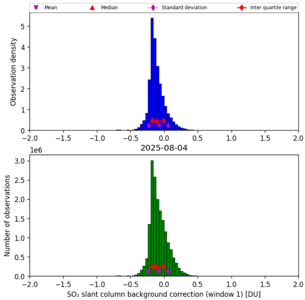
Figure 66: Histogram of “SO 2 slant column background correction (window 1)” for 2025-08-04 to 2025-08-05
