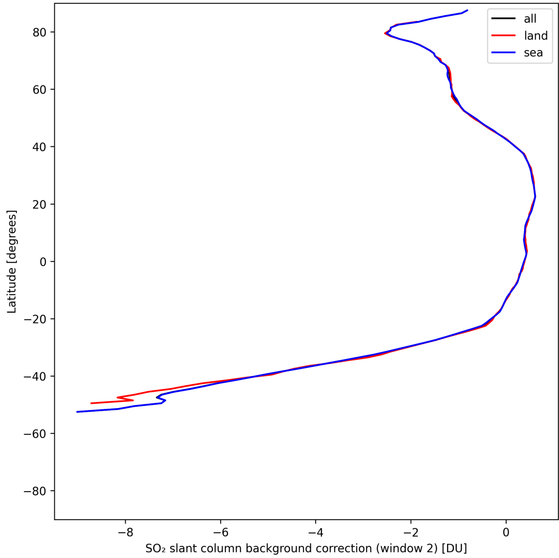
Figure 43: Zonal average of “SO 2 slant column background correction (window 2)” for 2025-08-04 to 2025-08-05.
