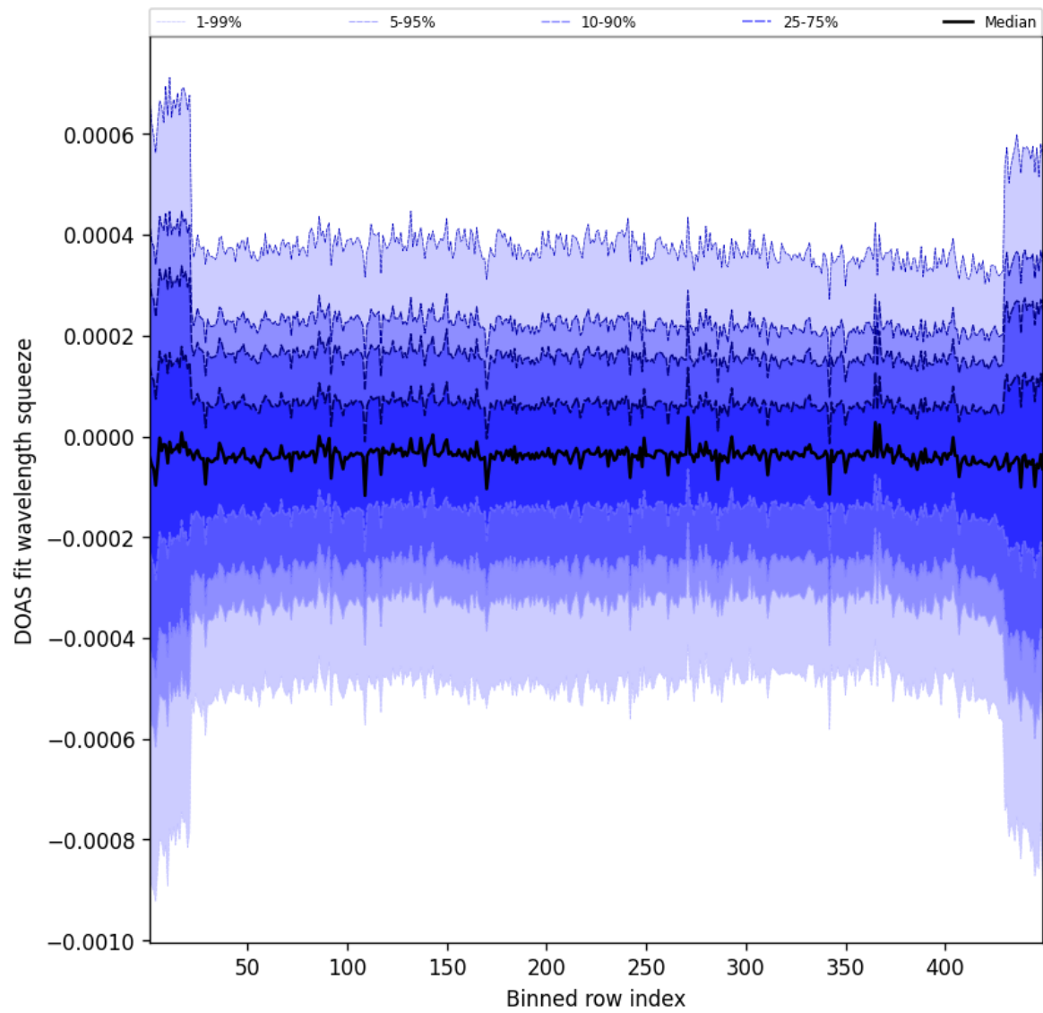
Figure 105: Along track statistics of “DOAS fit wavelength squeeze” for 2025-08-04 to 2025-08-05
