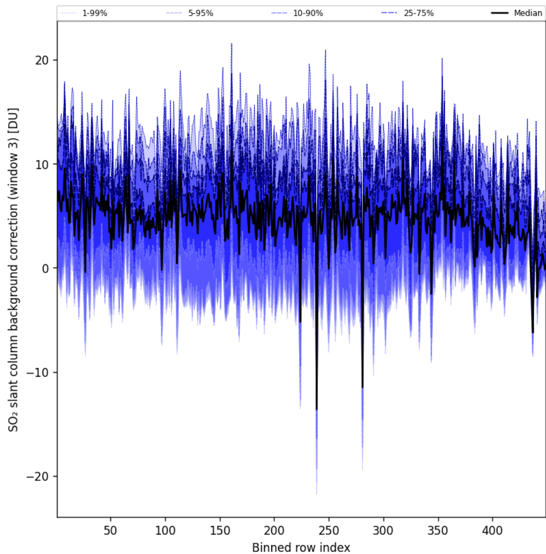
Figure 101: Along track statistics of “SO 2 slant column background correction (window 3)” for 2025-08-04 to 2025-08-05
