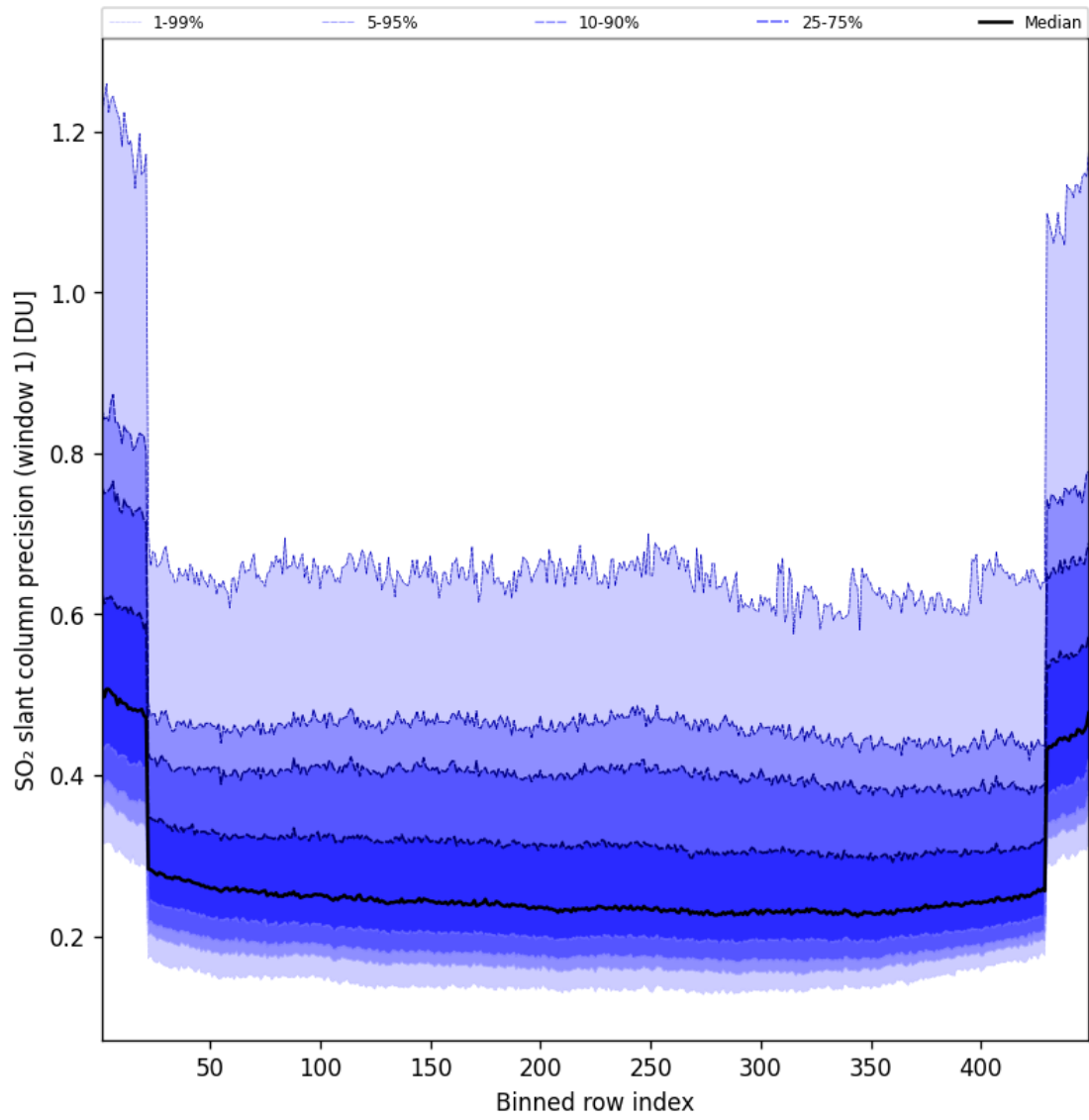
Figure 91: Along track statistics of “SO 2 slant column precision (window 1)” for 2025-08-04 to 2025-08-05
