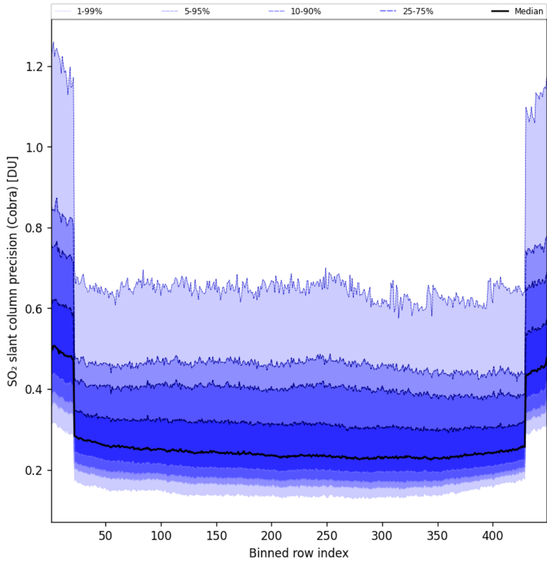
Figure 89: Along track statistics of “SO 2 slant column precision (Cobra)” for 2025-08-04 to 2025-08-05
