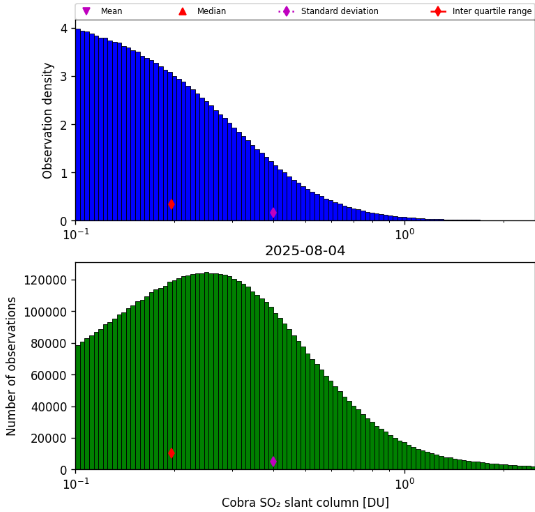
Figure 61: Histogram of “Cobra SO 2 slant column” for 2025-08-04 to 2025-08-05
