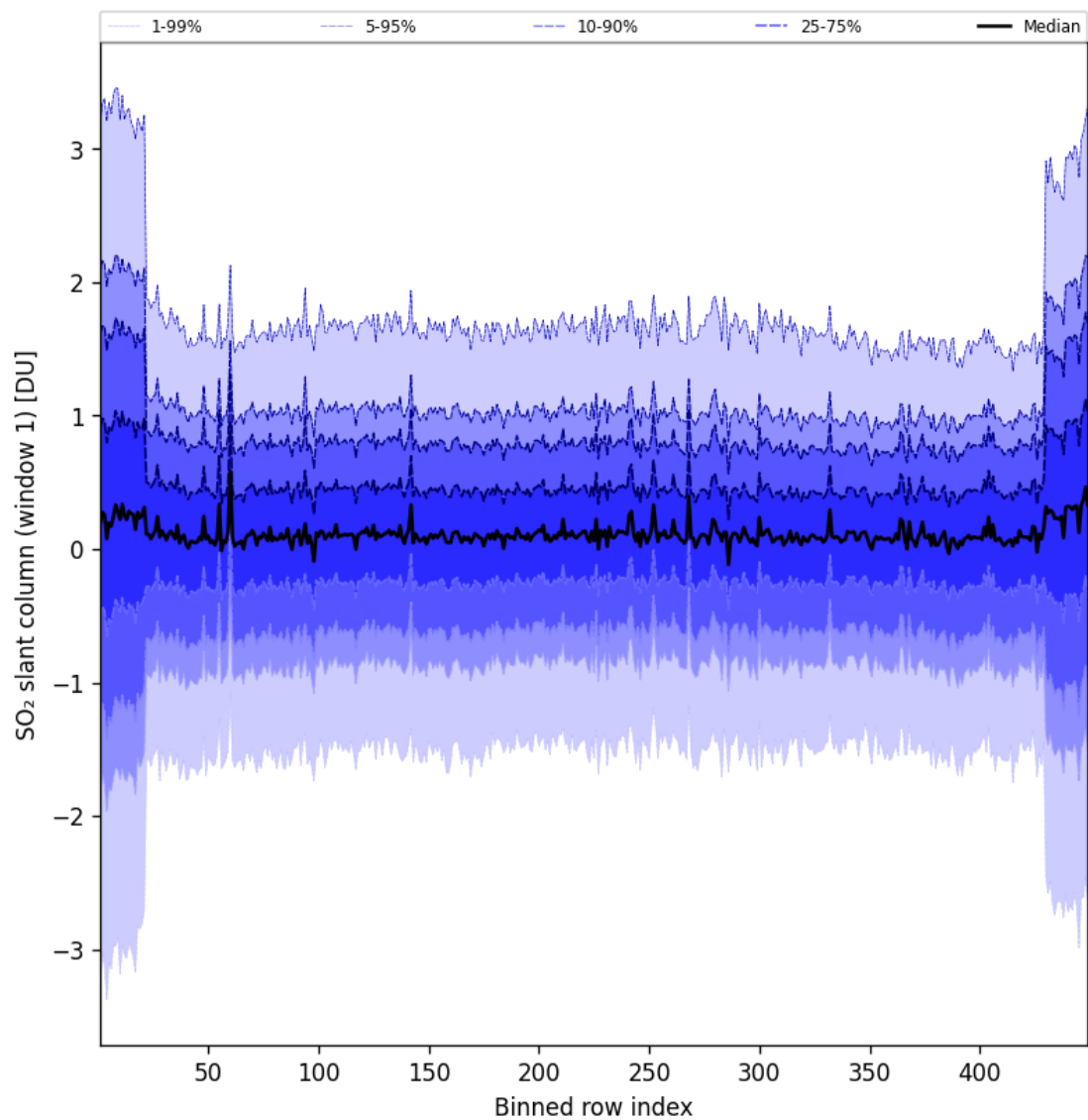
Figure 90: Along track statistics of “SO 2 slant column (window 1)” for 2025-08-04 to 2025-08-05
