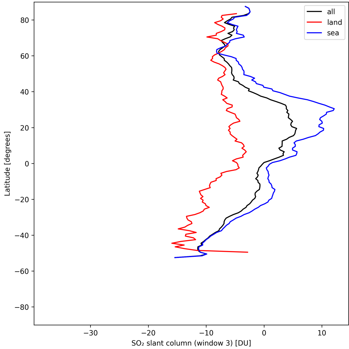
Figure 44: Zonal average of “SO 2 slant column (window 3)” for 2025-08-04 to 2025-08-05.
