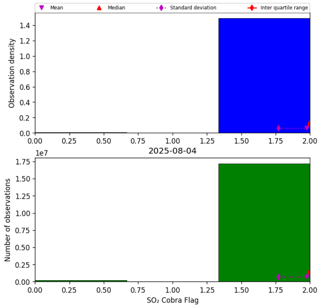
Figure 75: Histogram of “SO 2 Cobra Flag” for 2025-08-04 to 2025-08-05
