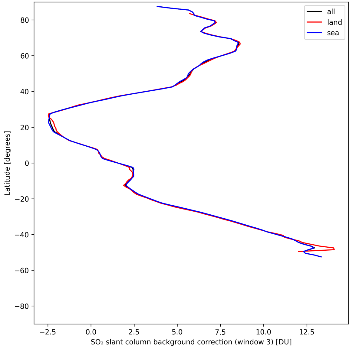
Figure 47: Zonal average of “SO 2 slant column background correction (window 3)” for 2025-08-04 to 2025-08-05.
