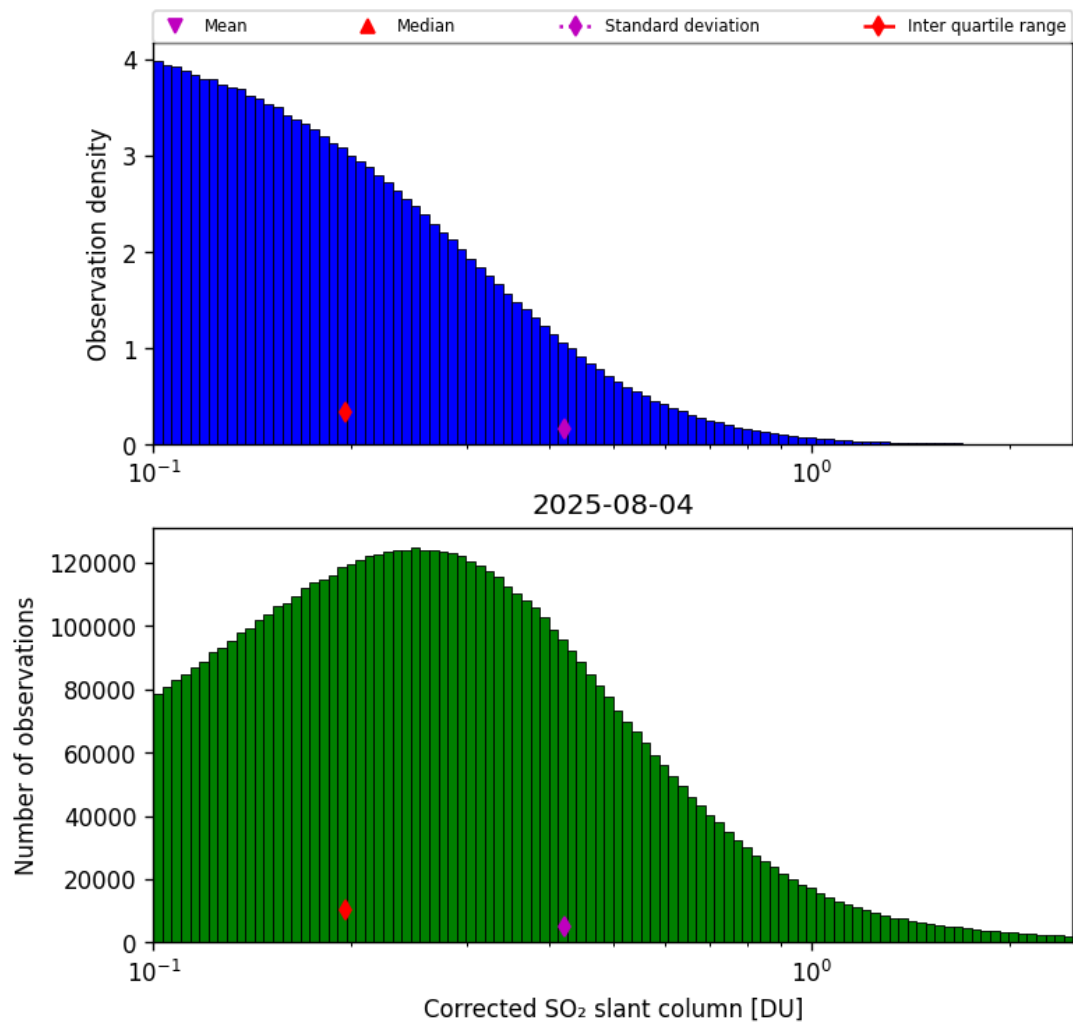
Figure 60: Histogram of “Corrected SO 2 slant column” for 2025-08-04 to 2025-08-05
