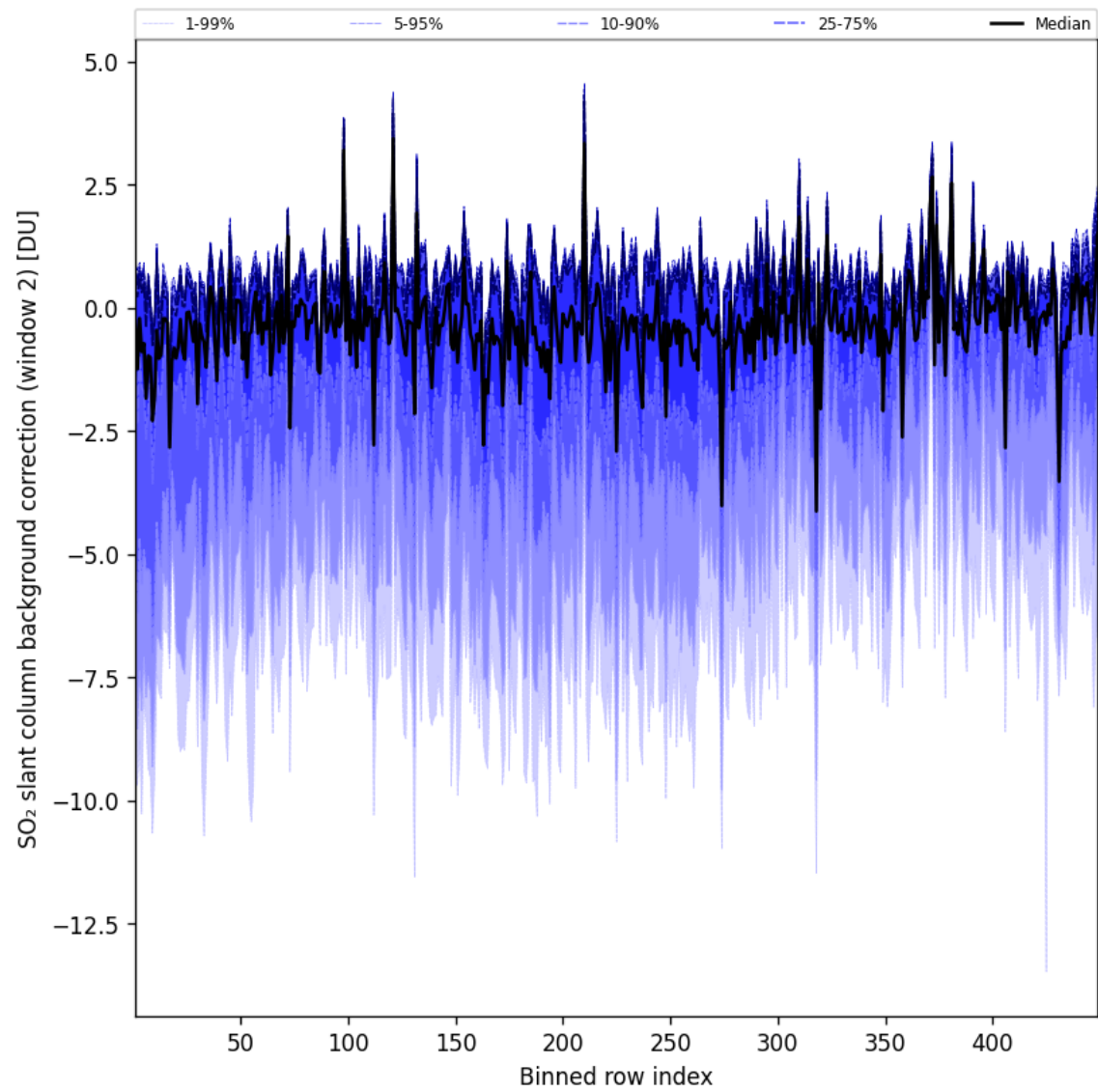
Figure 97: Along track statistics of “SO 2 slant column background correction (window 2)” for 2025-08-04 to 2025-08-05
