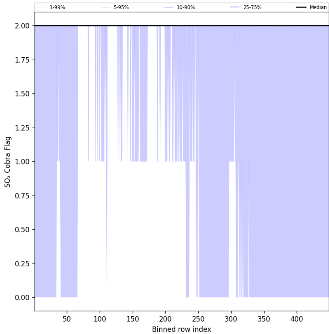
Figure 102: Along track statistics of “SO 2 Cobra Flag” for 2025-08-04 to 2025-08-05
