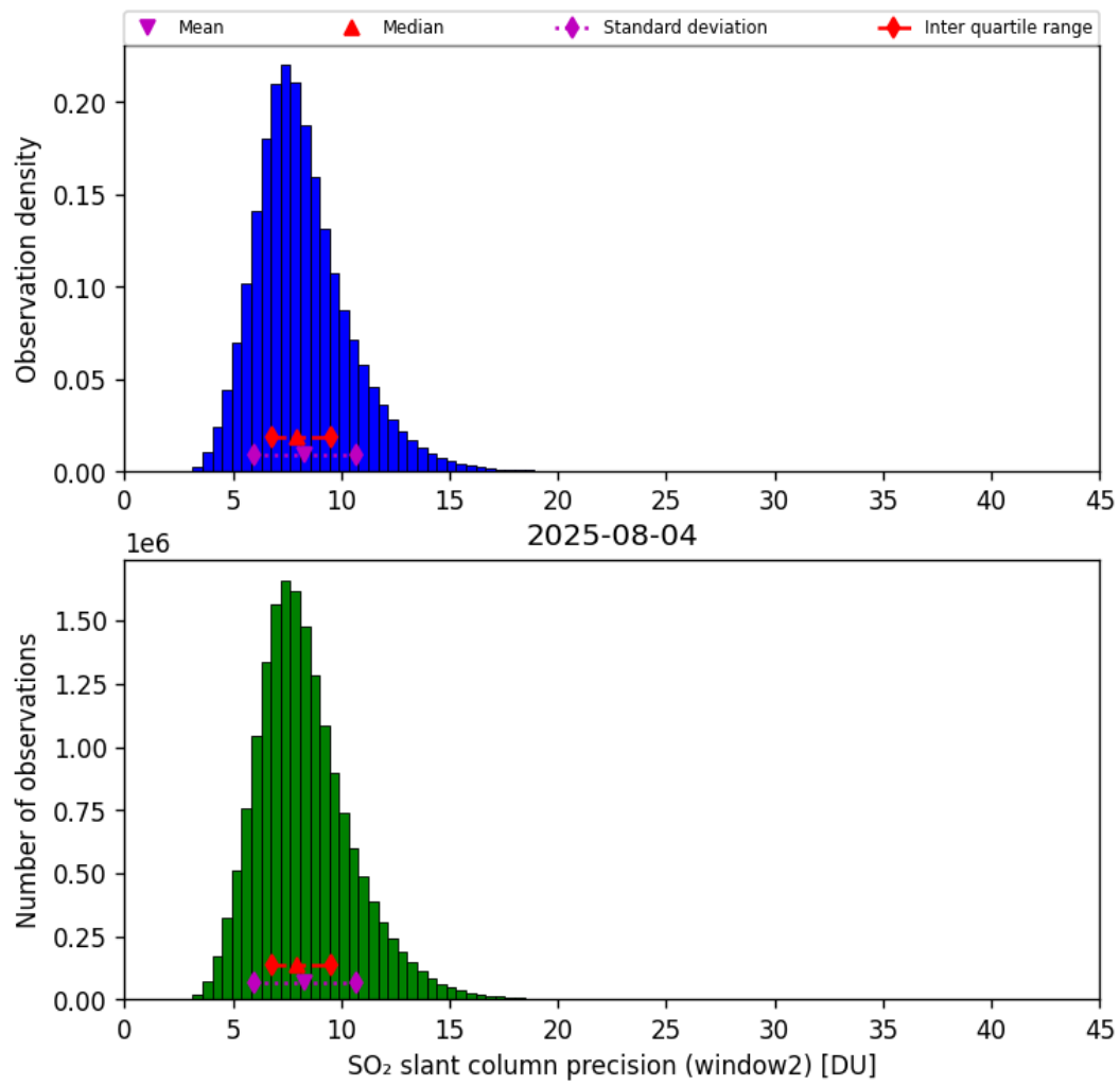
Figure 68: Histogram of “SO 2 slant column precision (window2)” for 2025-08-04 to 2025-08-05
