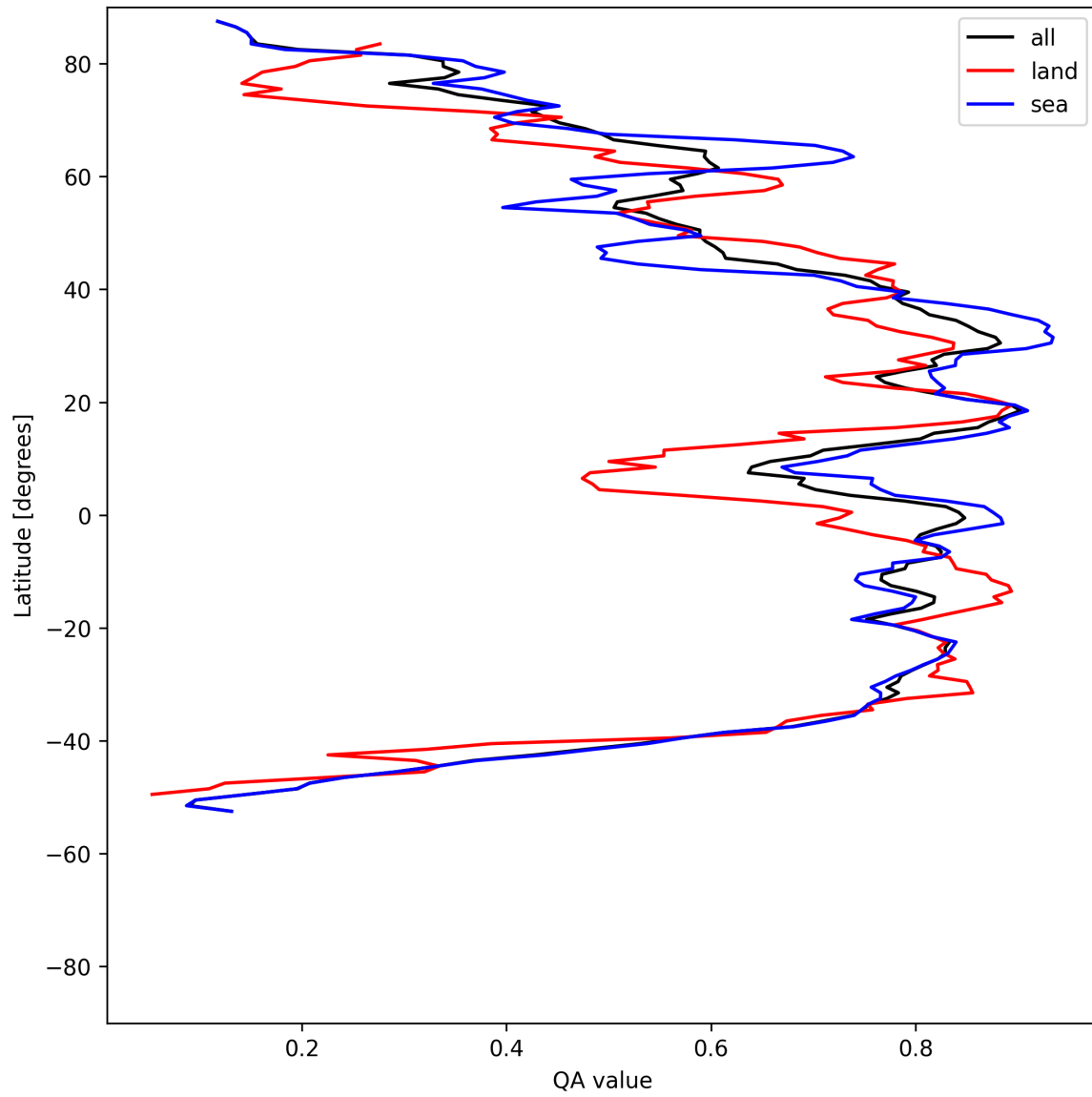
Figure 30: Zonal average of “QA value” for 2025-08-04 to 2025-08-05.
