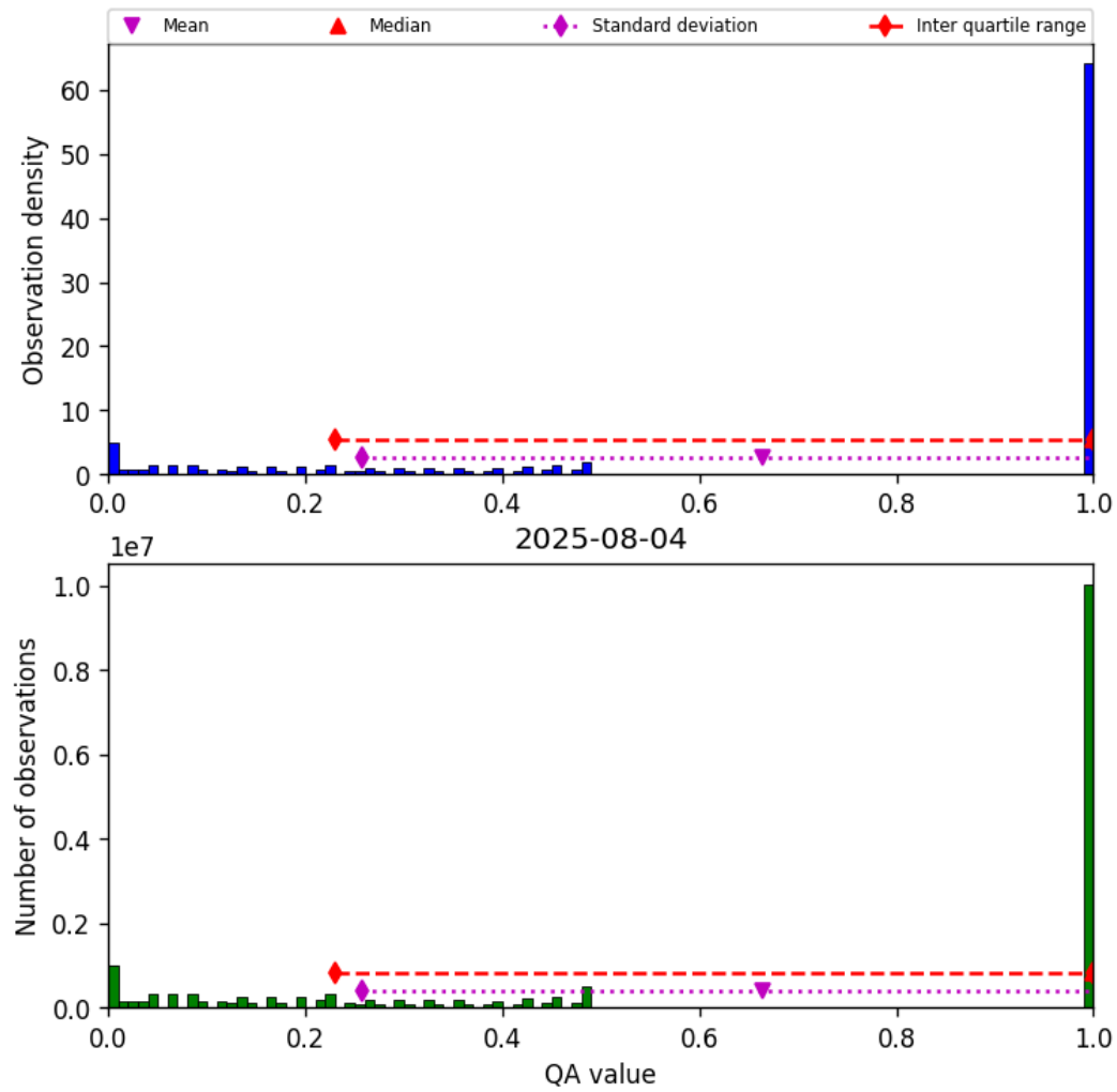
Figure 57: Histogram of “QA value” for 2025-08-04 to 2025-08-05
