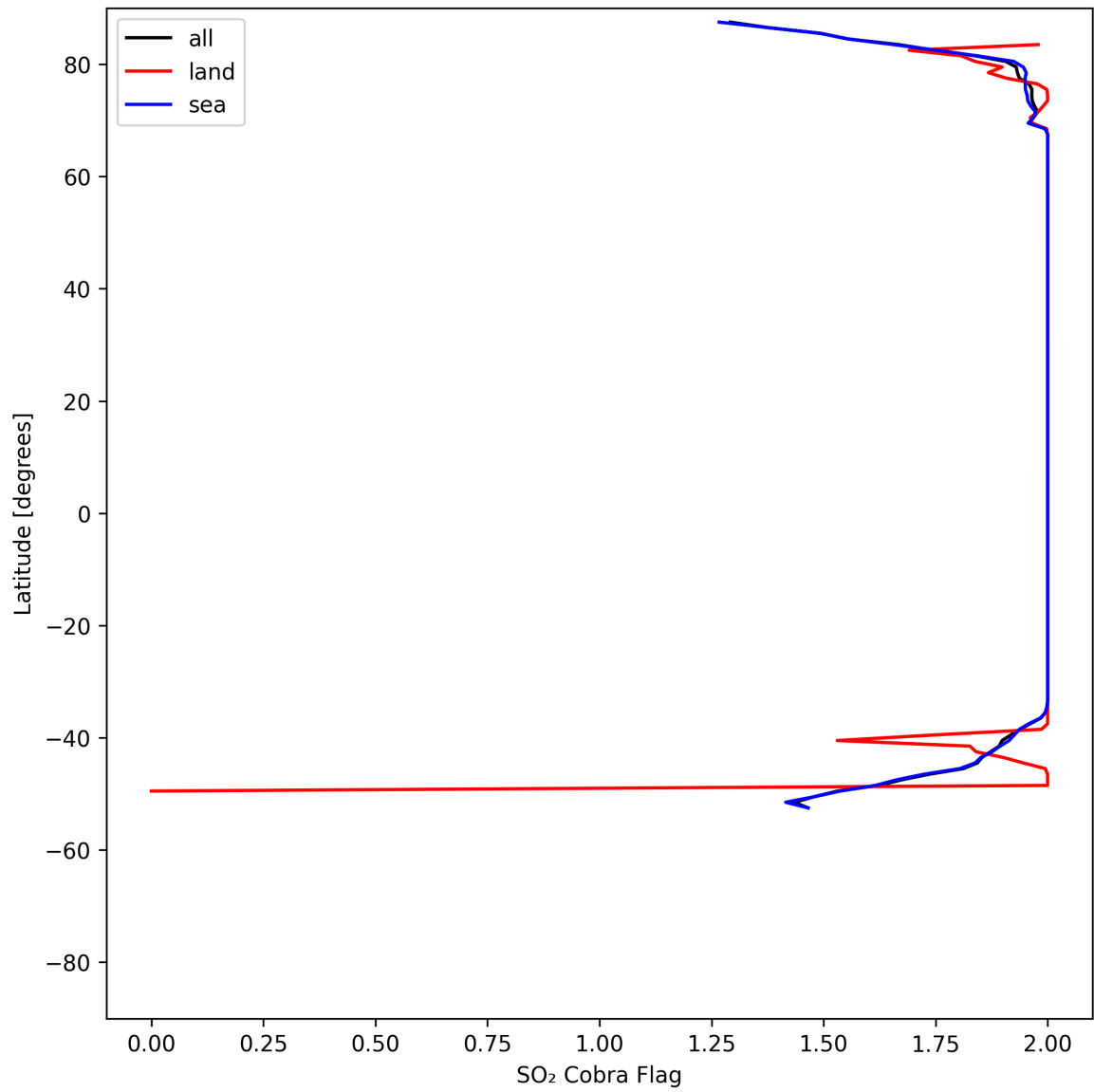
Figure 48: Zonal average of “SO 2 Cobra Flag” for 2025-08-04 to 2025-08-05.
