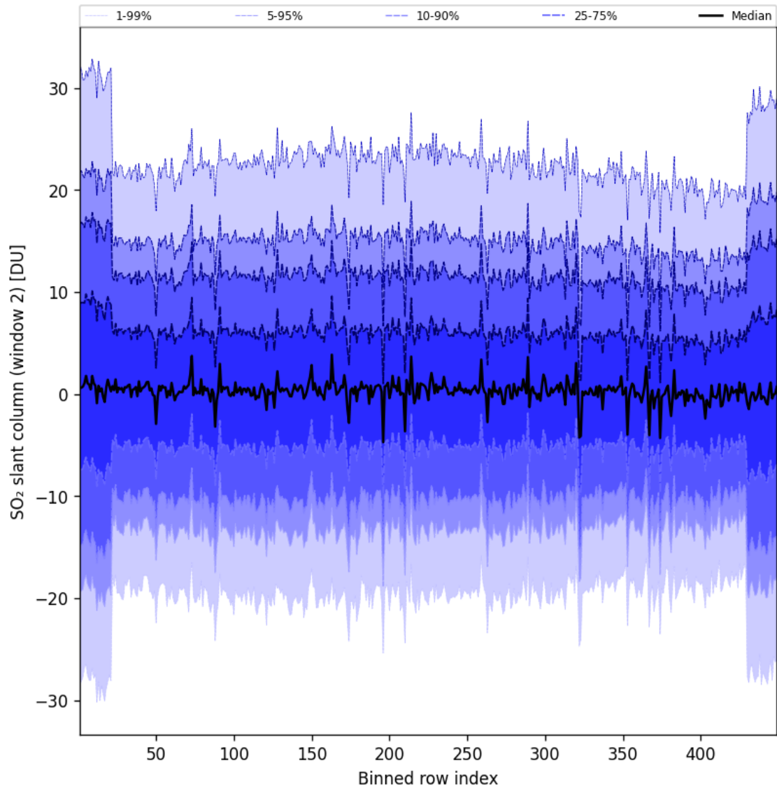
Figure 94: Along track statistics of “SO 2 slant column (window 2)” for 2025-08-04 to 2025-08-05
