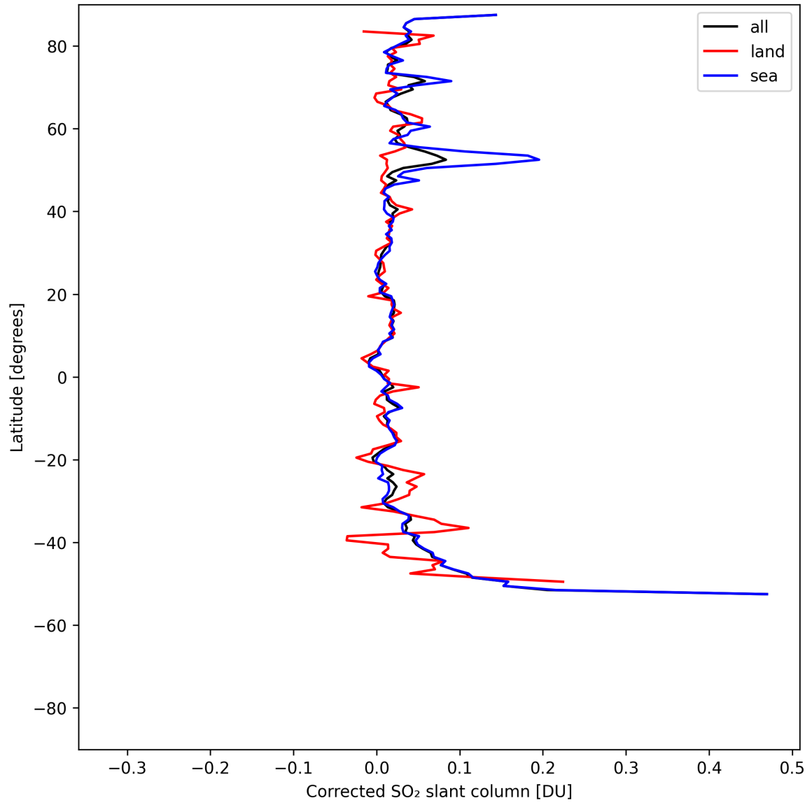
Figure 33: Zonal average of “Corrected SO 2 slant column” for 2025-08-04 to 2025-08-05.
