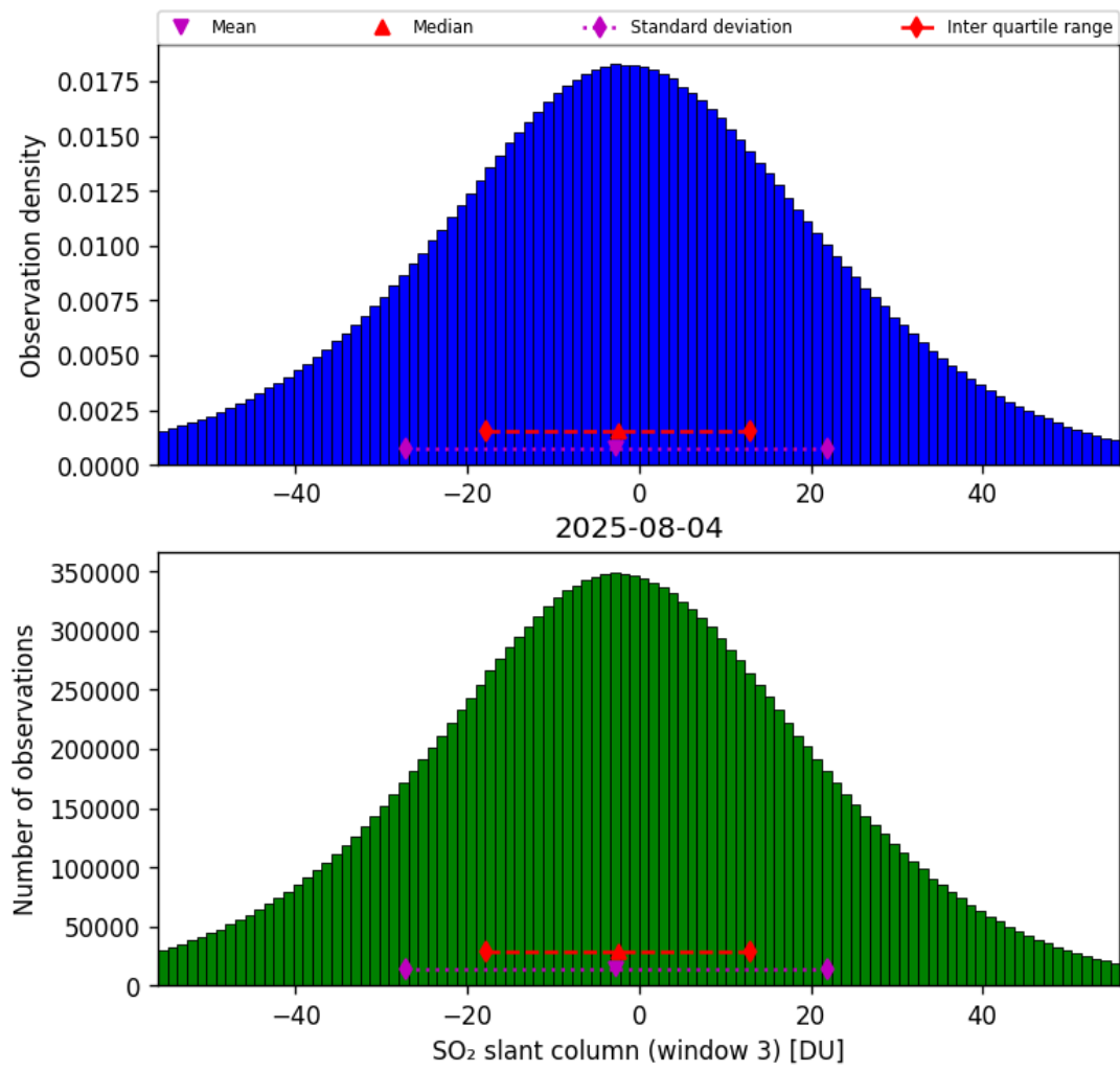
Figure 71: Histogram of “SO 2 slant column (window 3)” for 2025-08-04 to 2025-08-05
