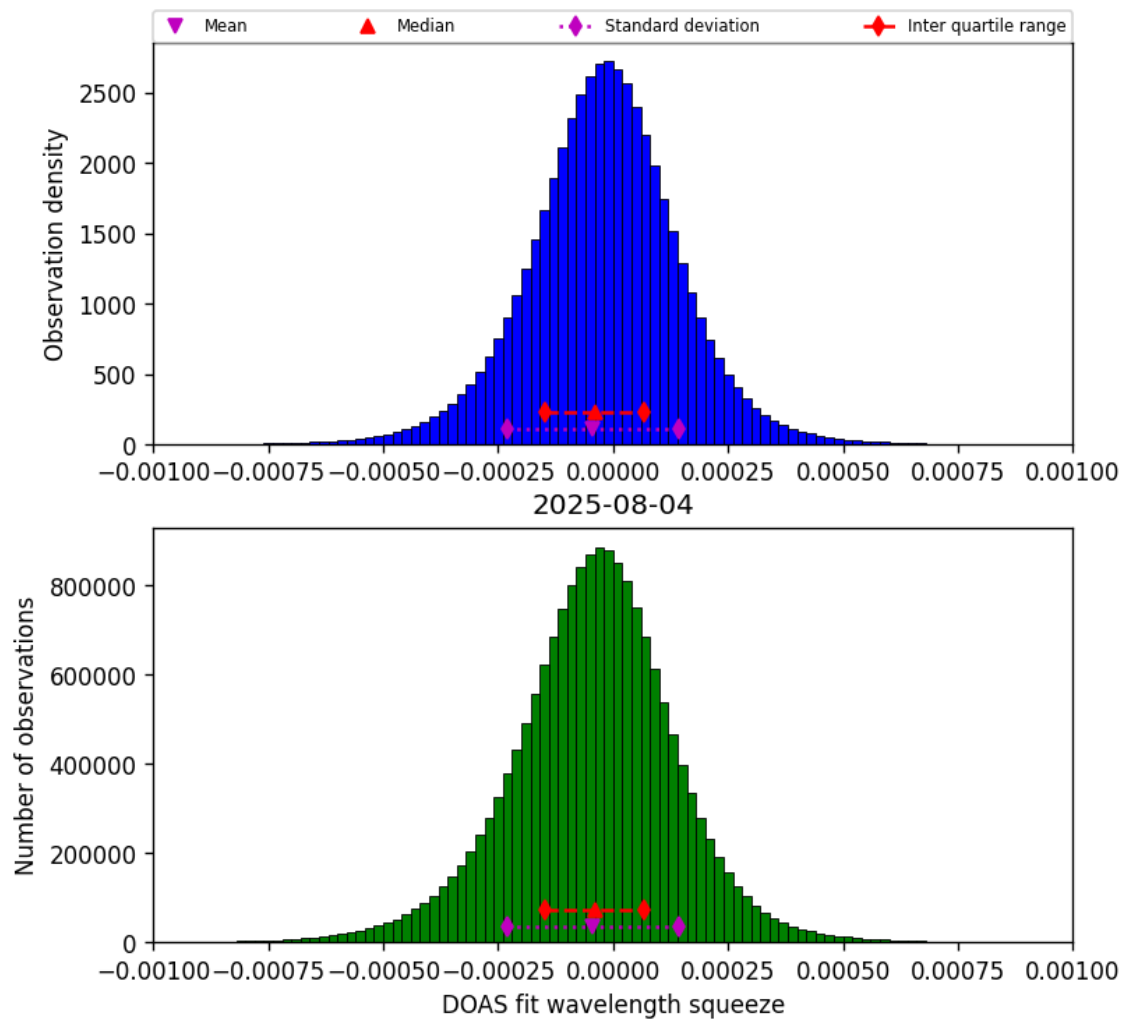
Figure 78: Histogram of “DOAS fit wavelength squeeze” for 2025-08-04 to 2025-08-05
