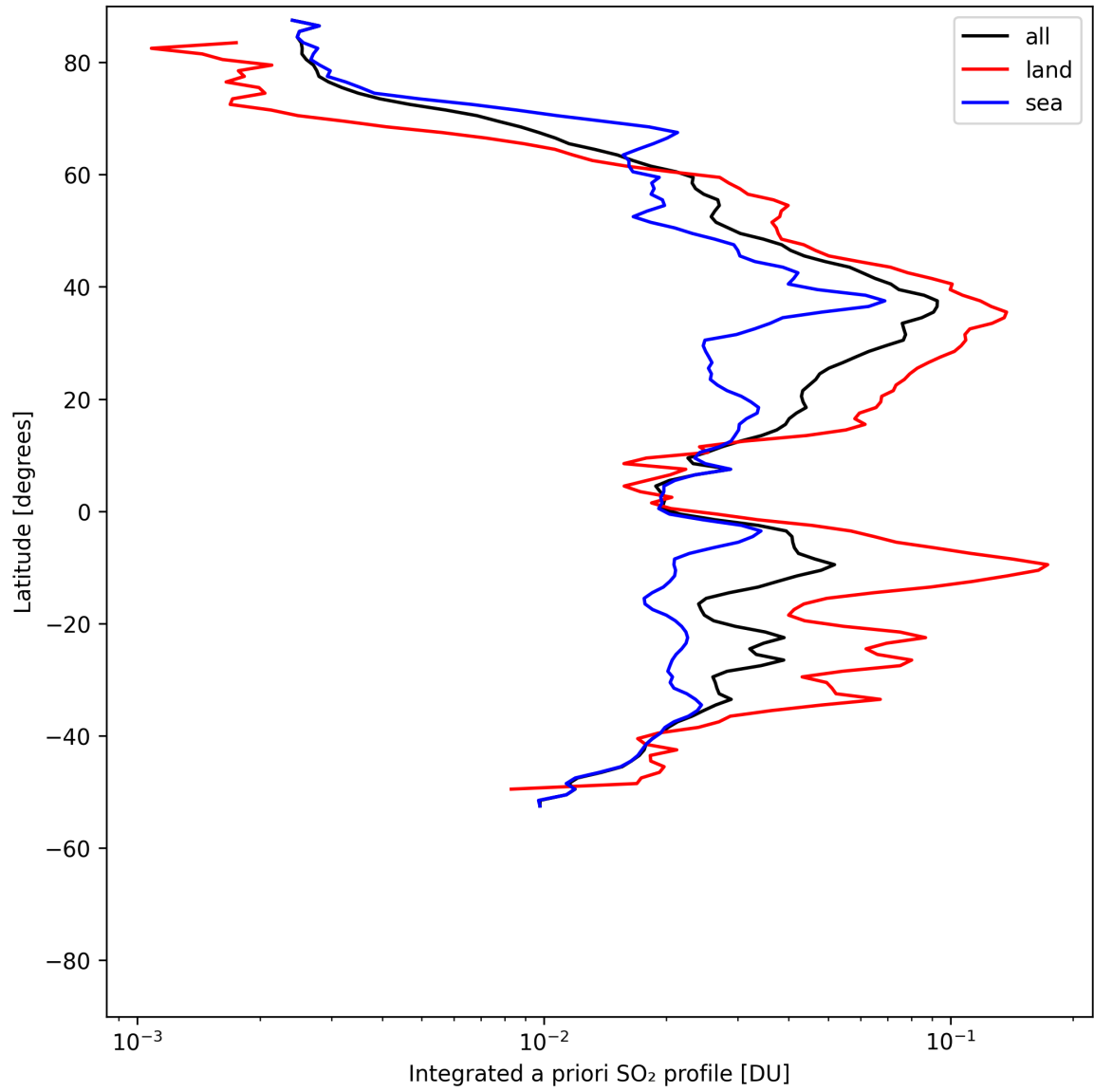
Figure 49: Zonal average of “Integrated a priori SO 2 profile” for 2025-08-04 to 2025-08-05.
