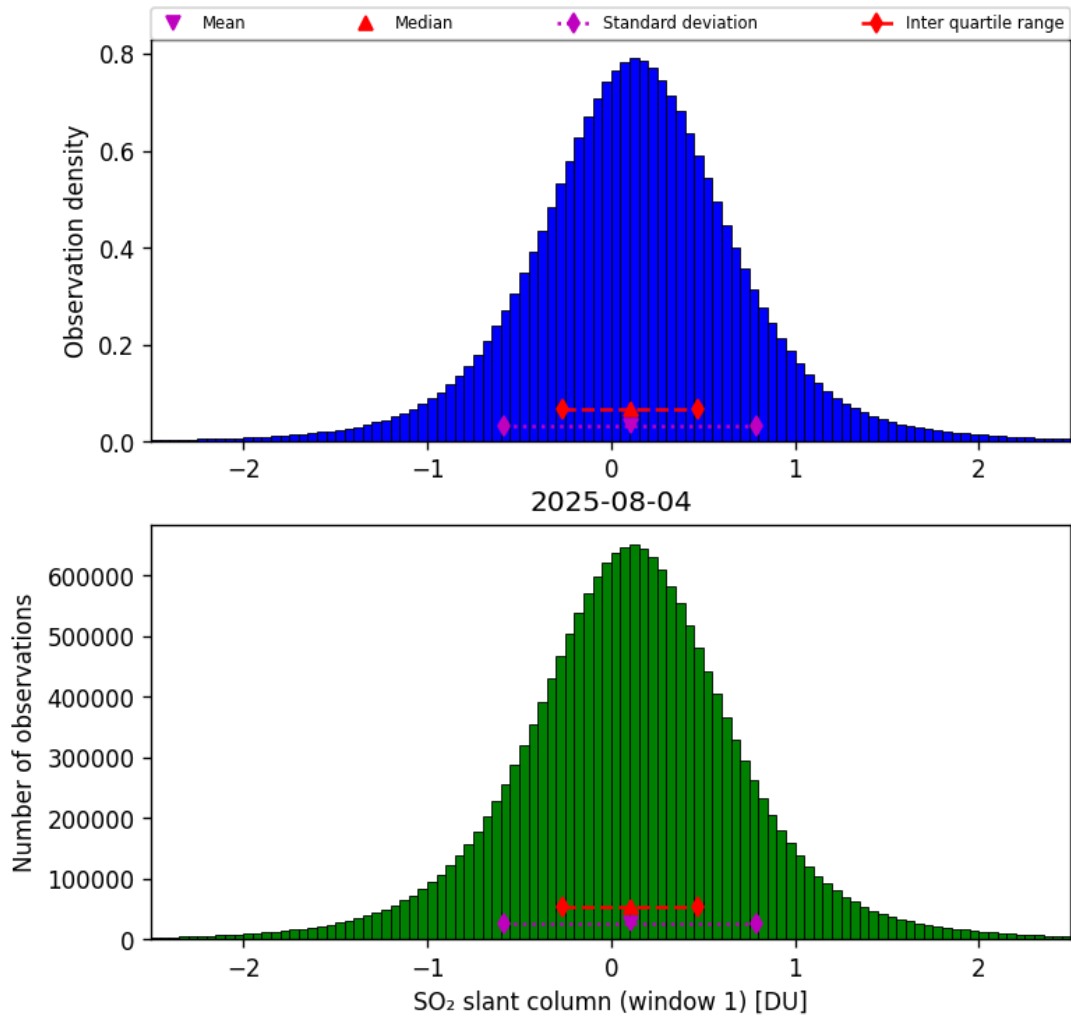
Figure 63: Histogram of “SO 2 slant column (window 1)” for 2025-08-04 to 2025-08-05
