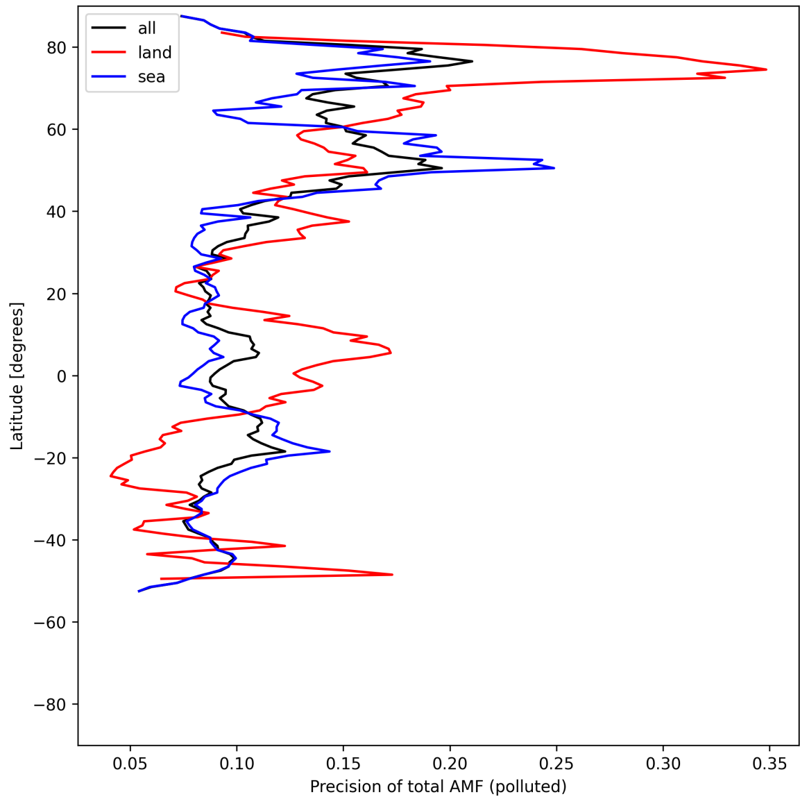
Figure 54: Zonal average of “Precision of total AMF (polluted)” for 2025-08-04 to 2025-08-05.
