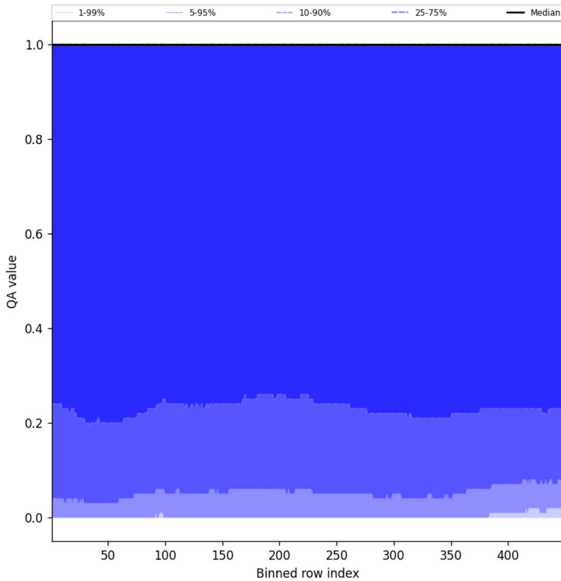
Figure 84: Along track statistics of “QA value” for 2025-08-04 to 2025-08-05
