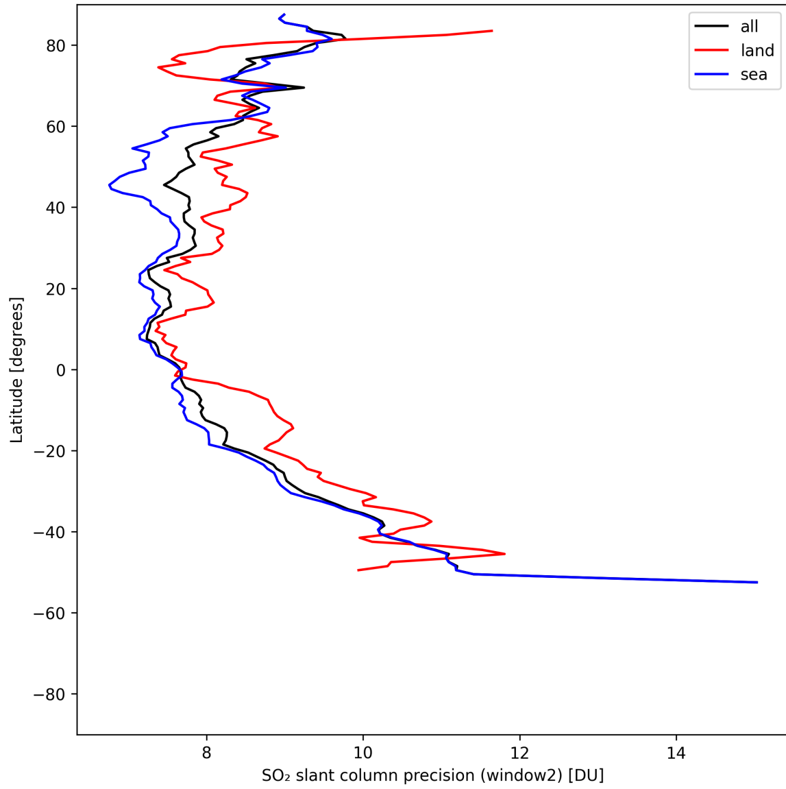
Figure 41: Zonal average of “SO 2 slant column precision (window2)” for 2025-08-04 to 2025-08-05.
