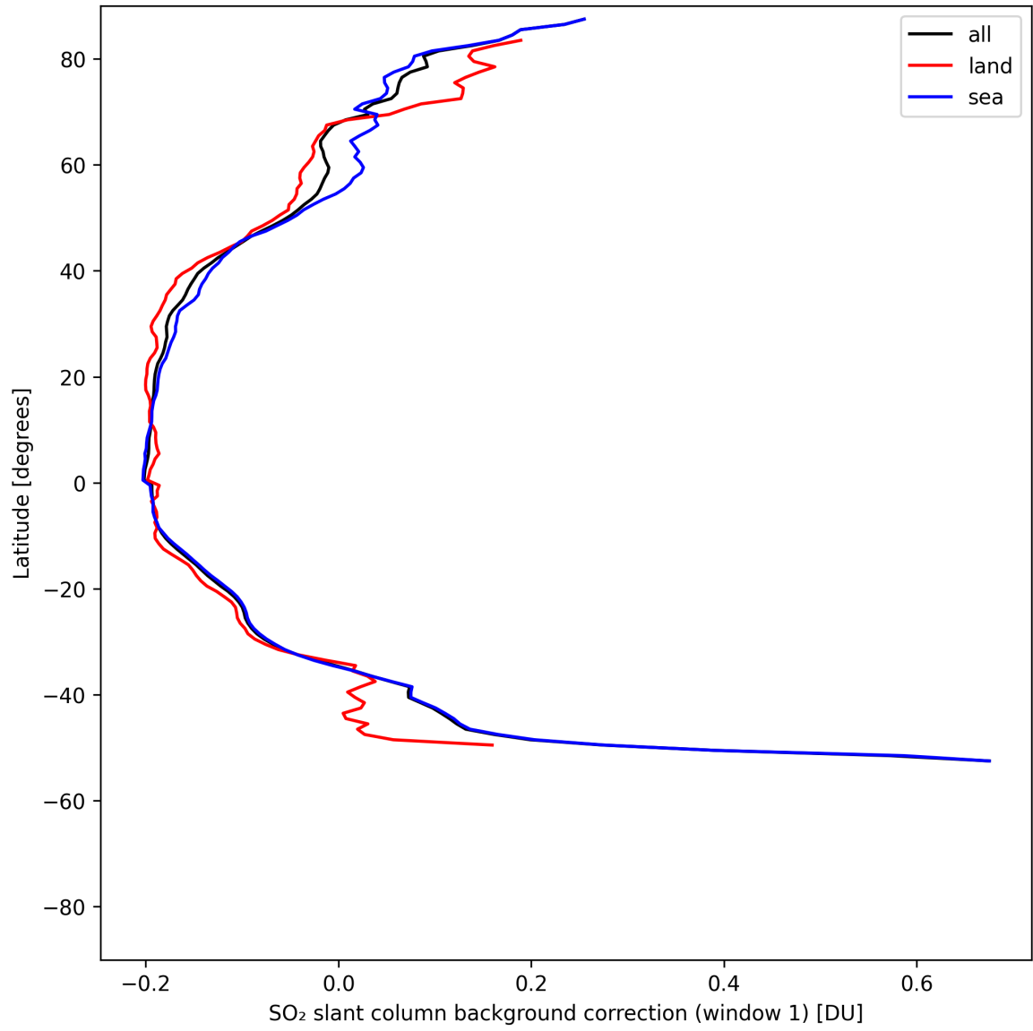
Figure 39: Zonal average of “SO 2 slant column background correction (window 1)” for 2025-08-04 to 2025-08-05.
