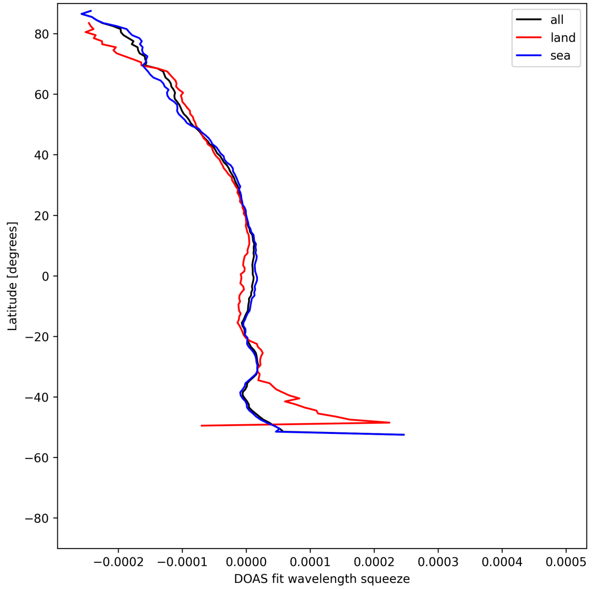
Figure 51: Zonal average of “DOAS fit wavelength squeeze” for 2025-08-04 to 2025-08-05.
