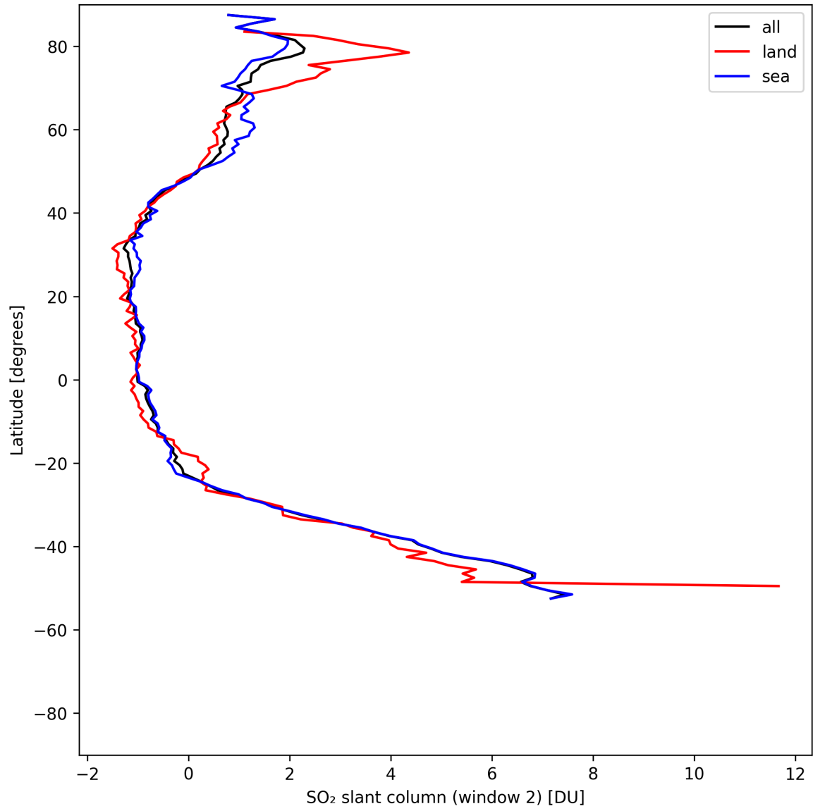
Figure 40: Zonal average of “SO 2 slant column (window 2)” for 2025-08-04 to 2025-08-05.
