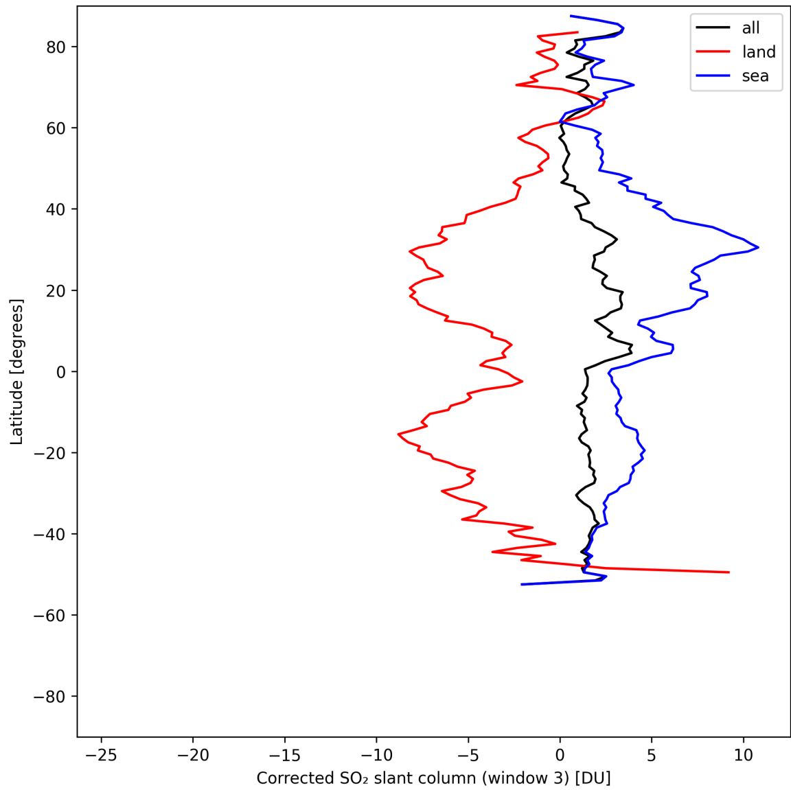
Figure 46: Zonal average of “Corrected SO 2 slant column (window 3)” for 2025-08-04 to 2025-08-05.
