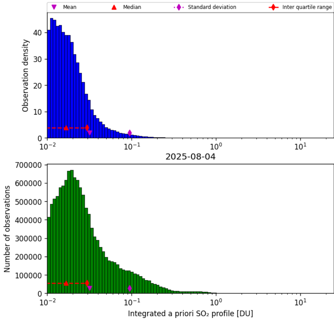
Figure 76: Histogram of “Integrated a priori SO 2 profile” for 2025-08-04 to 2025-08-05
