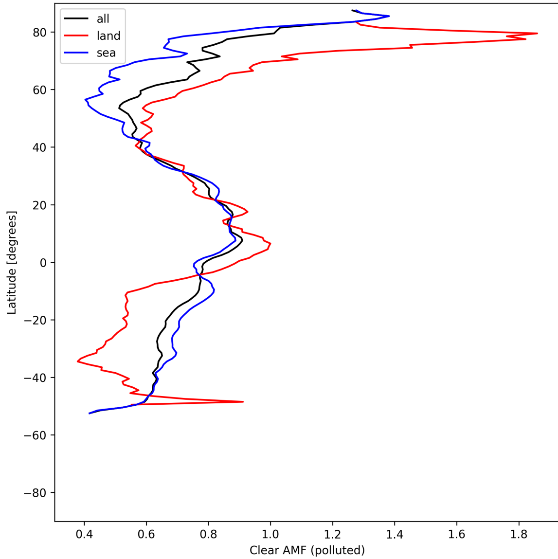
Figure 55: Zonal average of “Clear AMF (polluted)” for 2025-08-04 to 2025-08-05.
