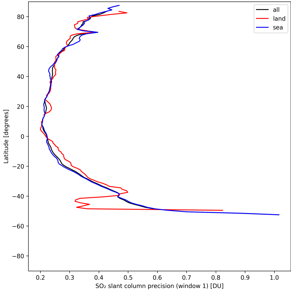
Figure 37: Zonal average of “SO 2 slant column precision (window 1)” for 2025-08-04 to 2025-08-05.
