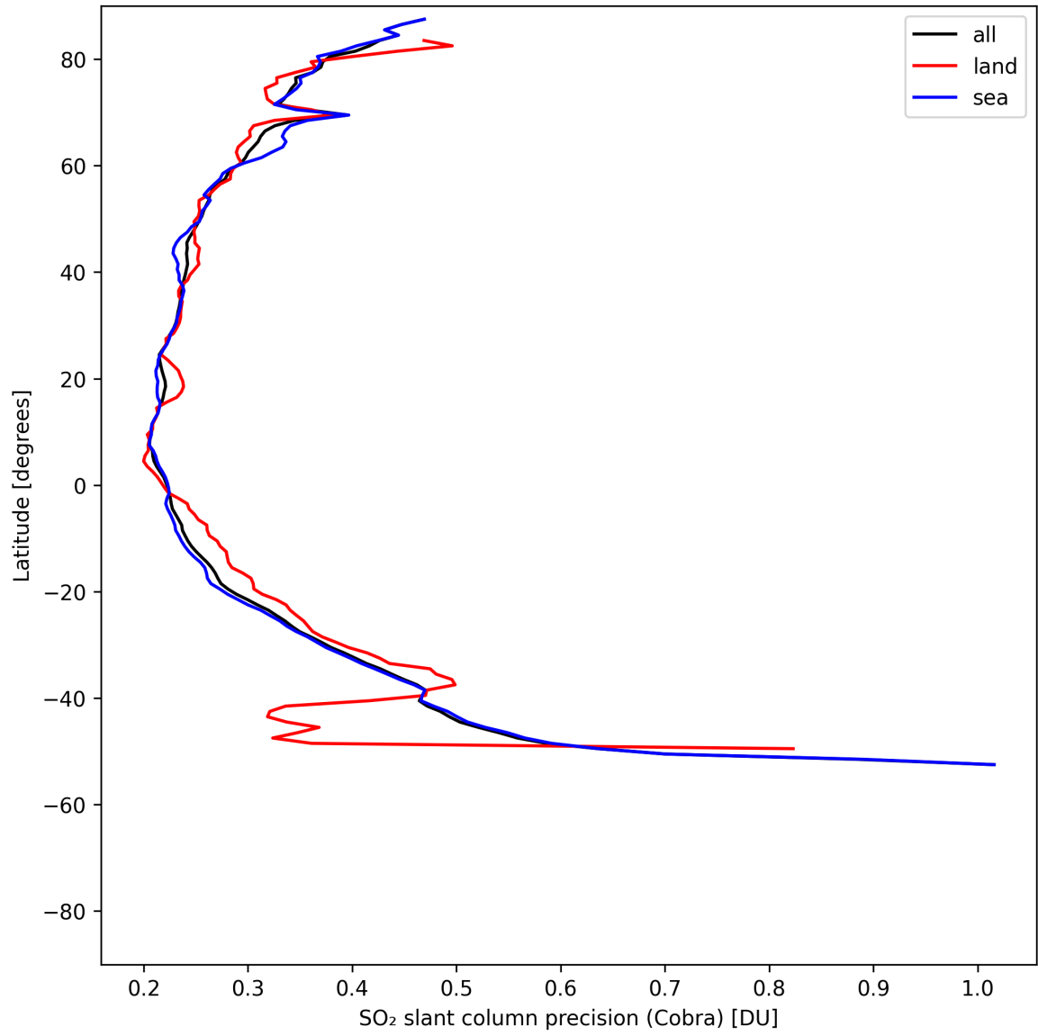
Figure 35: Zonal average of “SO 2 slant column precision (Cobra)” for 2025-08-04 to 2025-08-05.
