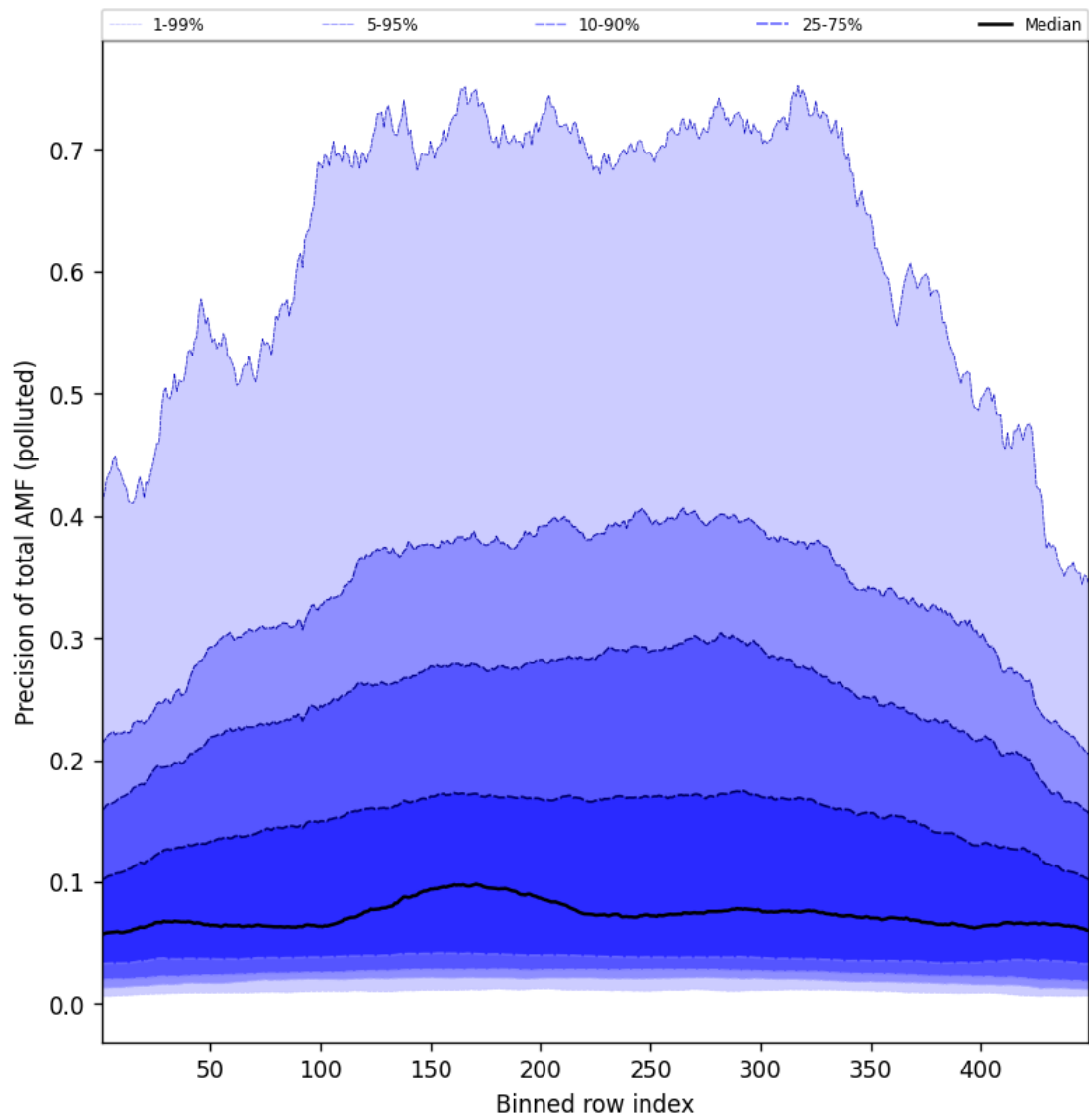
Figure 108: Along track statistics of “Precision of total AMF (polluted)” for 2025-08-04 to 2025-08-05
