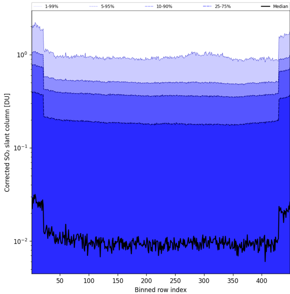
Figure 87: Along track statistics of "Corrected SO 2 slant column" for 2025-08-04 to 2025-08-05
