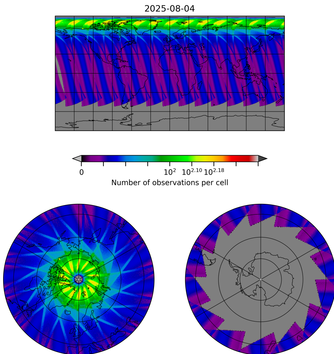
Figure 29: Map of the number of observations for 2025-08-04 to 2025-08-05
