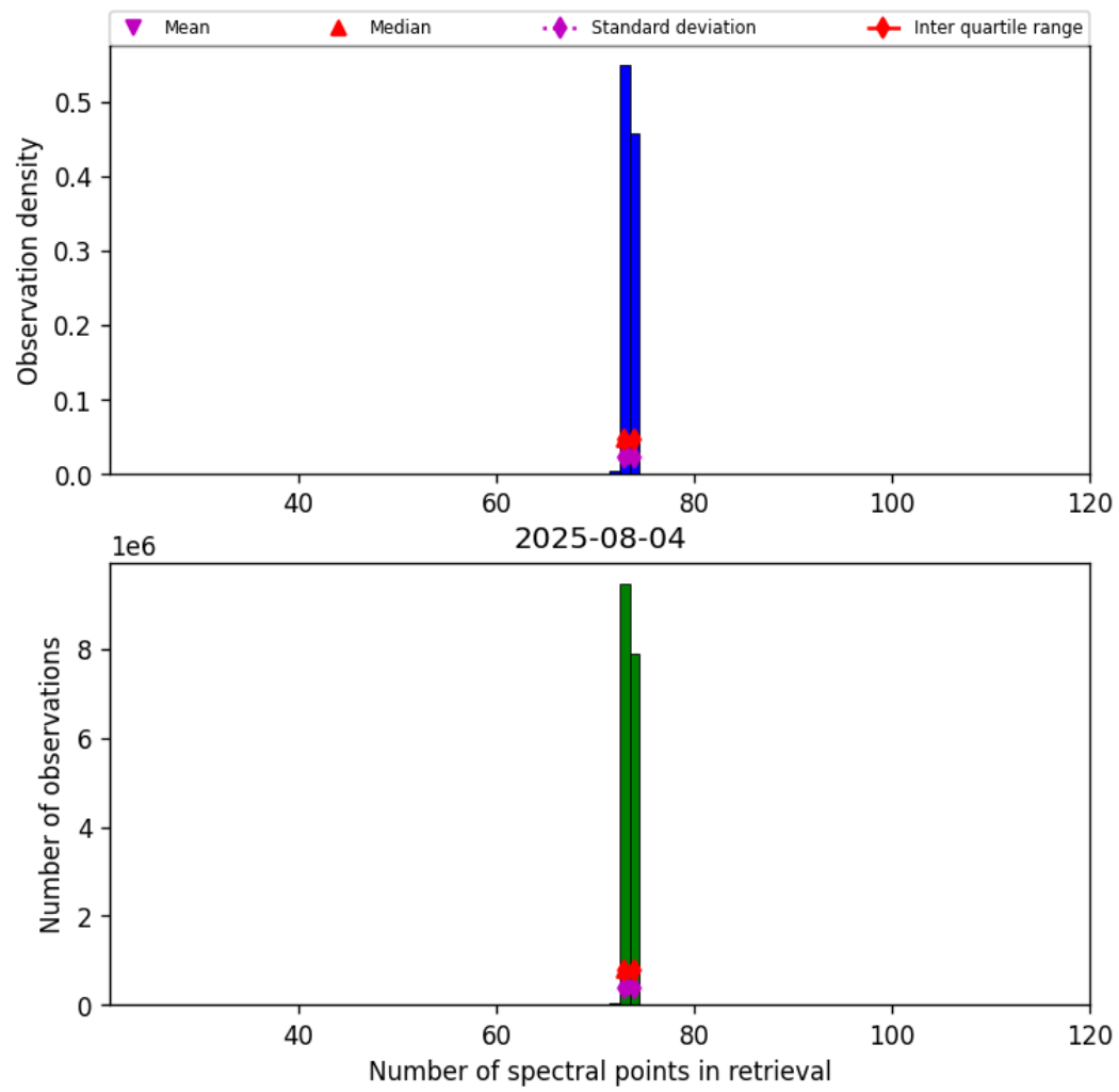
Figure 83: Histogram of “Number of spectral points in retrieval” for 2025-08-04 to 2025-08-05
