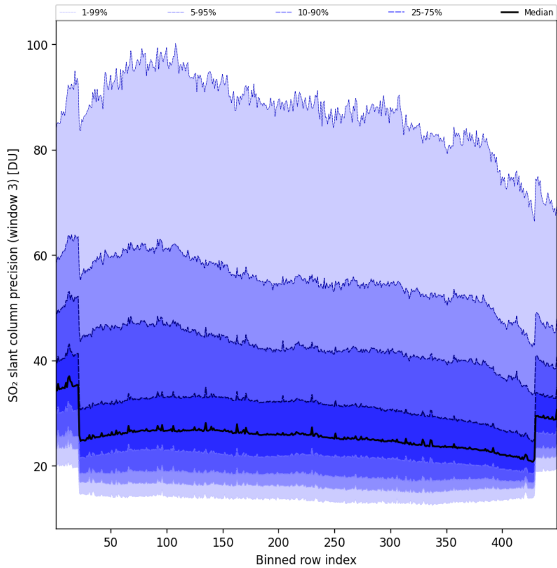
Figure 99: Along track statistics of “SO 2 slant column precision (window 3)” for 2025-08-04 to 2025-08-05
