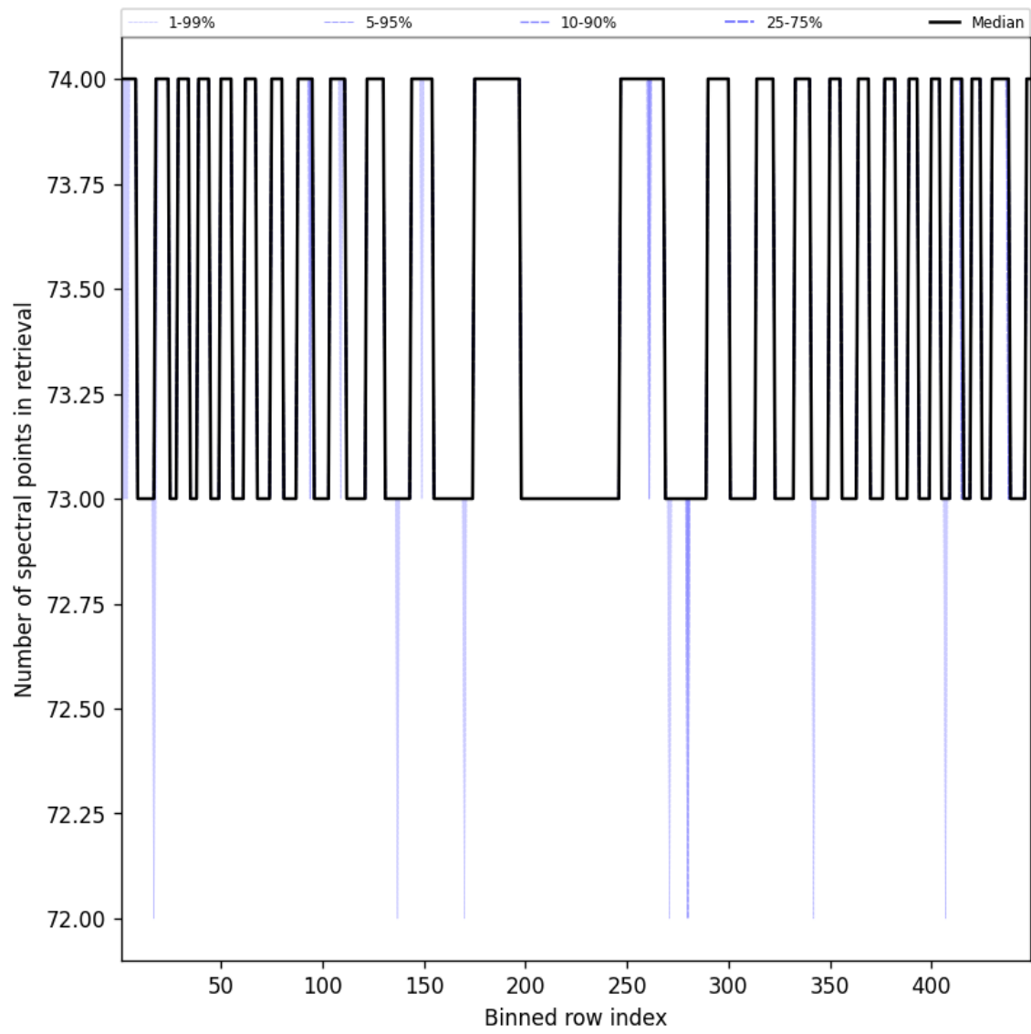
Figure 110: Along track statistics of “Number of spectral points in retrieval” for 2025-08-04 to 2025-08-05
