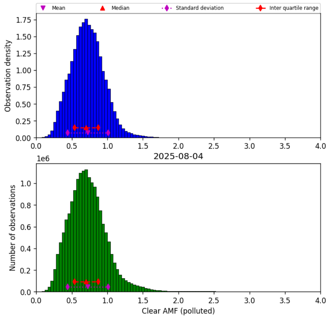
Figure 82: Histogram of “Clear AMF (polluted)” for 2025-08-04 to 2025-08-05
