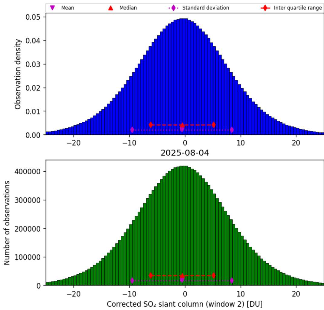
Figure 69: Histogram of “Corrected SO 2 slant column (window 2)” for 2025-08-04 to 2025-08-05
