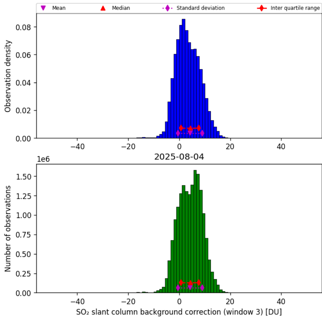
Figure 74: Histogram of “SO 2 slant column background correction (window 3)” for 2025-08-04 to 2025-08-05
