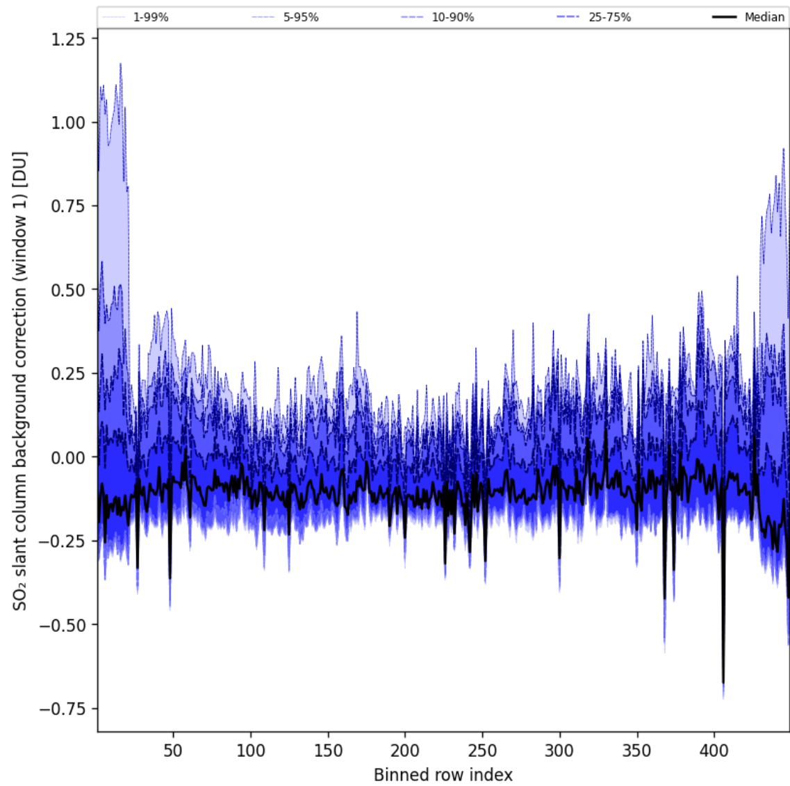
Figure 93: Along track statistics of “SO 2 slant column background correction (window 1)” for 2025-08-04 to 2025-08-05
