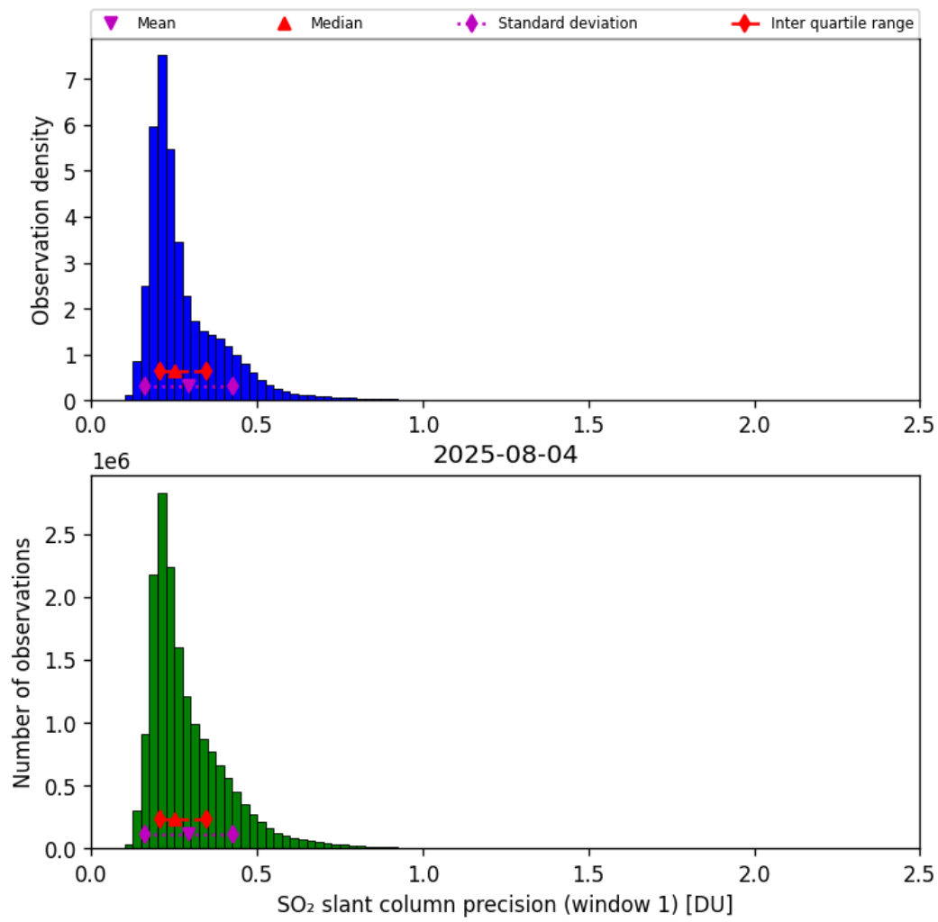
Figure 64: Histogram of “SO 2 slant column precision (window 1)” for 2025-08-04 to 2025-08-05
