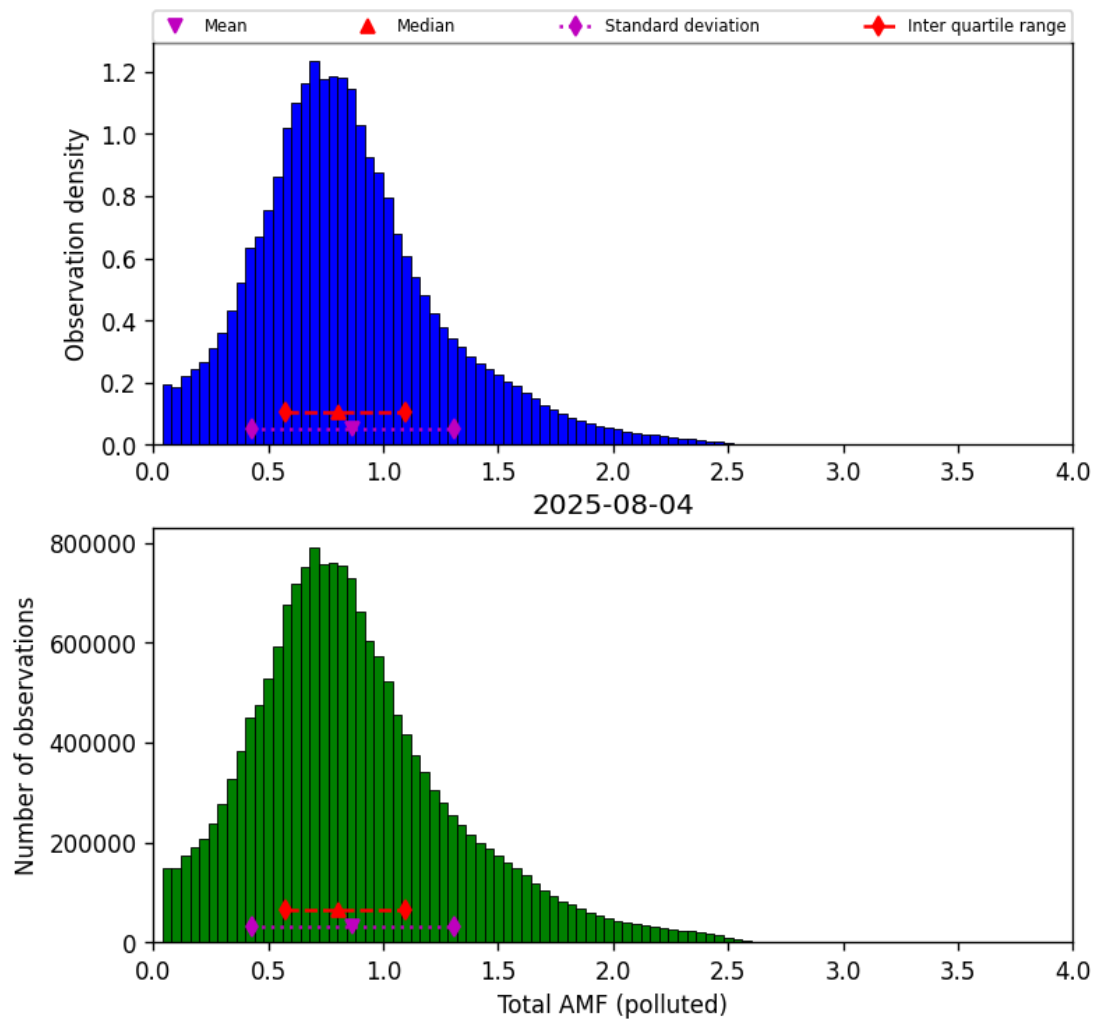
Figure 80: Histogram of “Total AMF (polluted)” for 2025-08-04 to 2025-08-05
