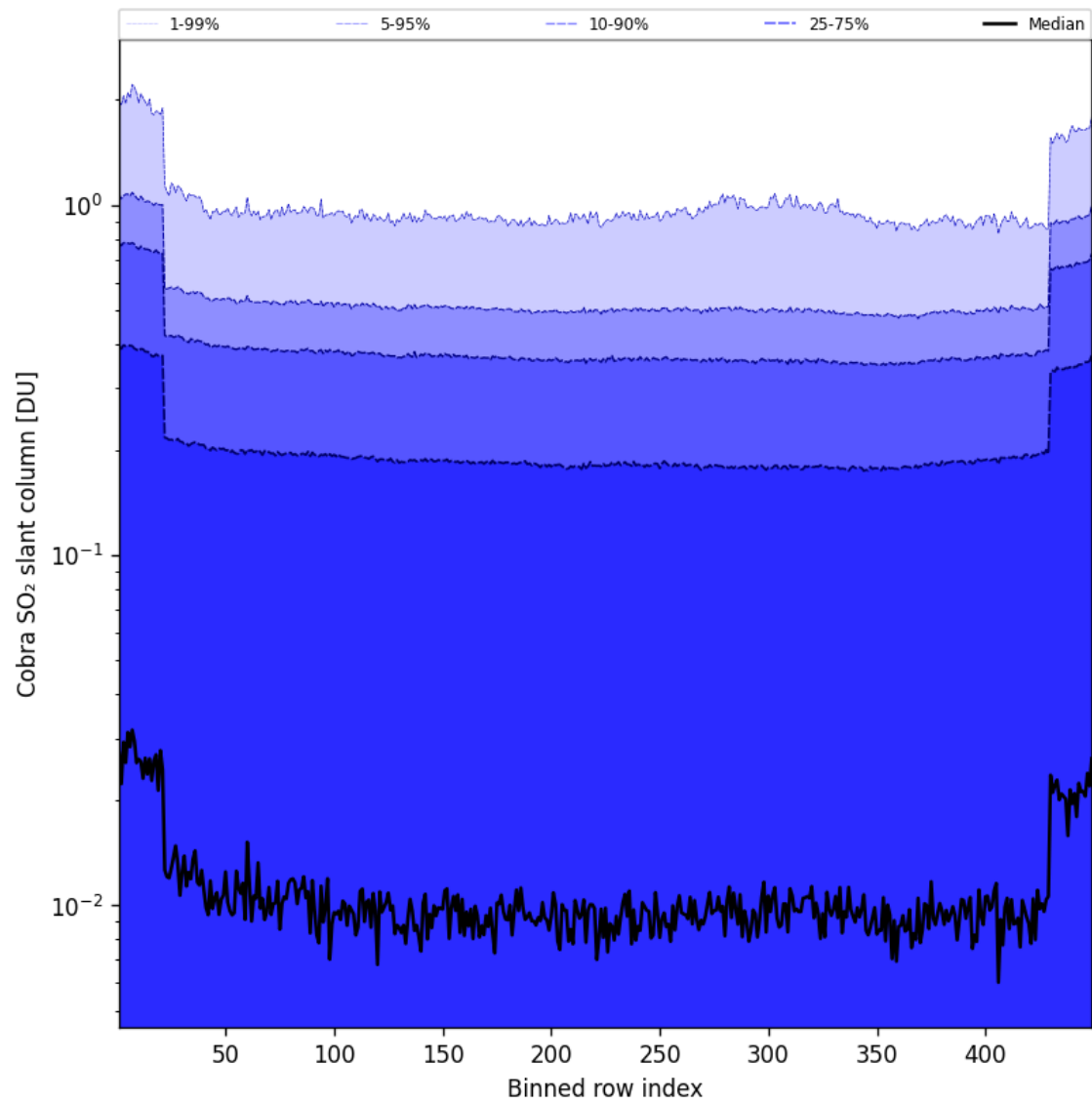
Figure 88: Along track statistics of “Cobra SO 2 slant column” for 2025-08-04 to 2025-08-05
