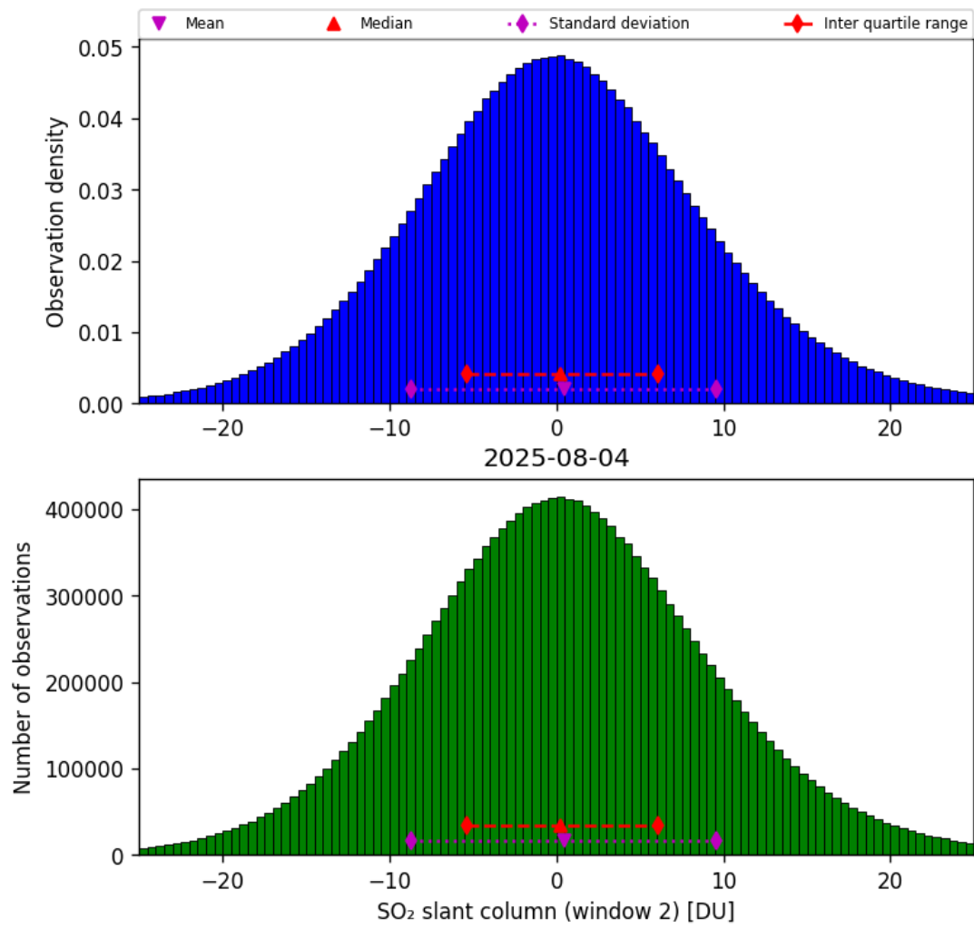
Figure 67: Histogram of “SO 2 slant column (window 2)” for 2025-08-04 to 2025-08-05
