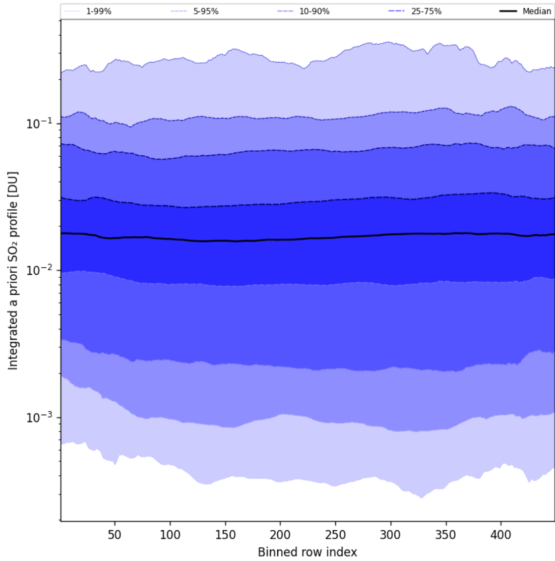
Figure 103: Along track statistics of “Integrated a priori SO 2 profile” for 2025-08-04 to 2025-08-05
