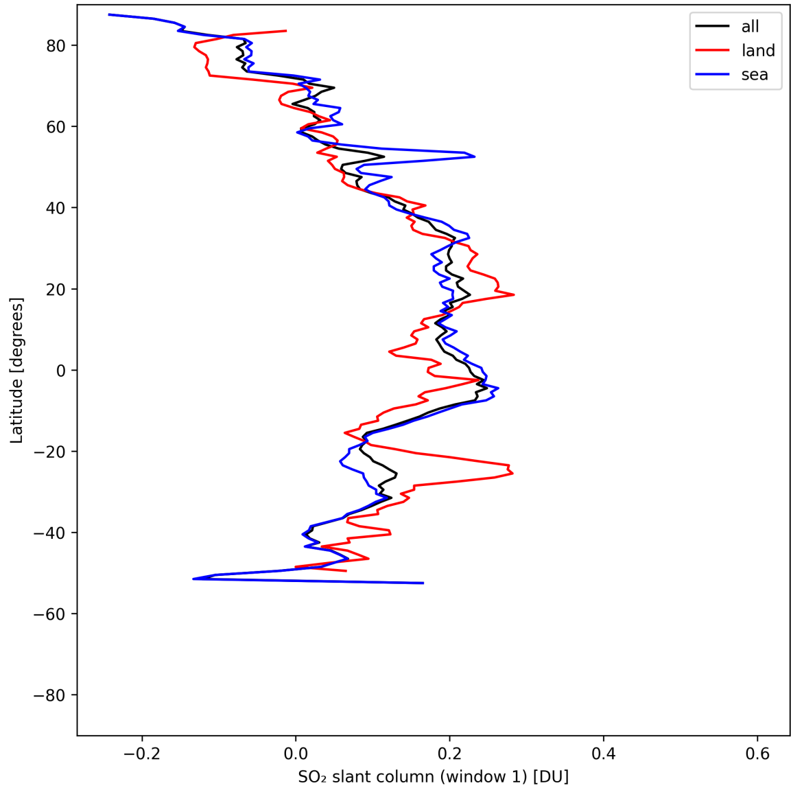
Figure 36: Zonal average of “SO 2 slant column (window 1)” for 2025-08-04 to 2025-08-05.
