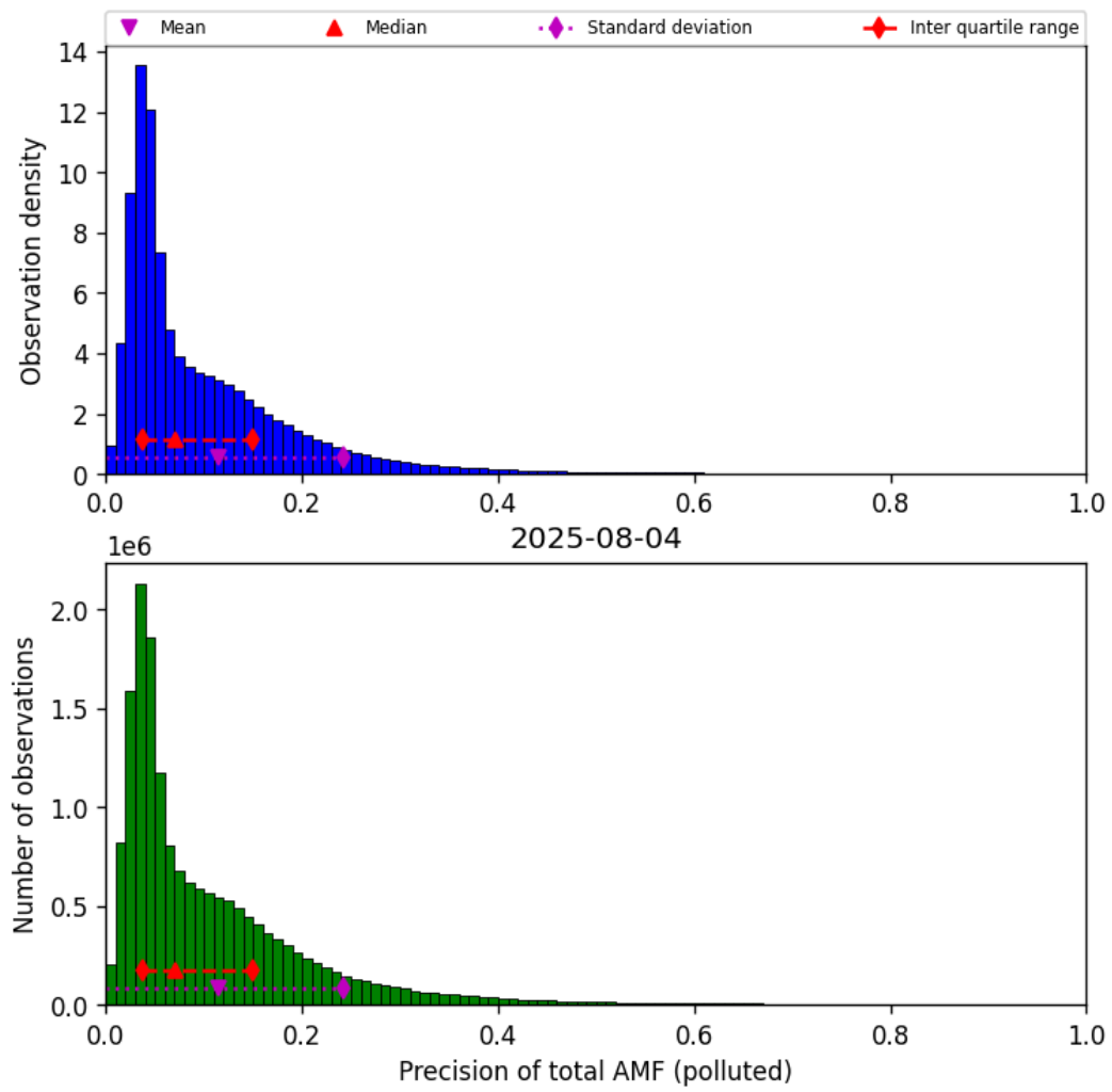
Figure 81: Histogram of “Precision of total AMF (polluted)” for 2025-08-04 to 2025-08-05
