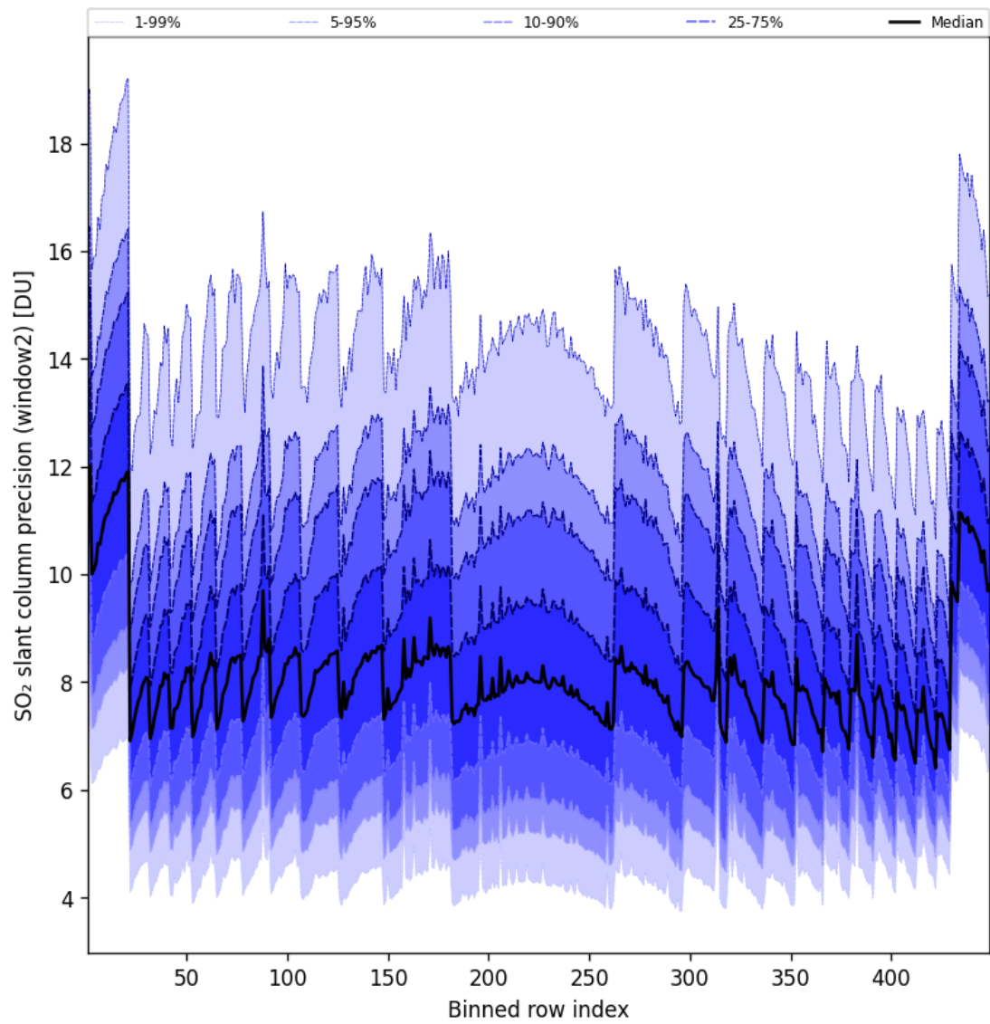
Figure 95: Along track statistics of “SO 2 slant column precision (window2)” for 2025-08-04 to 2025-08-05
