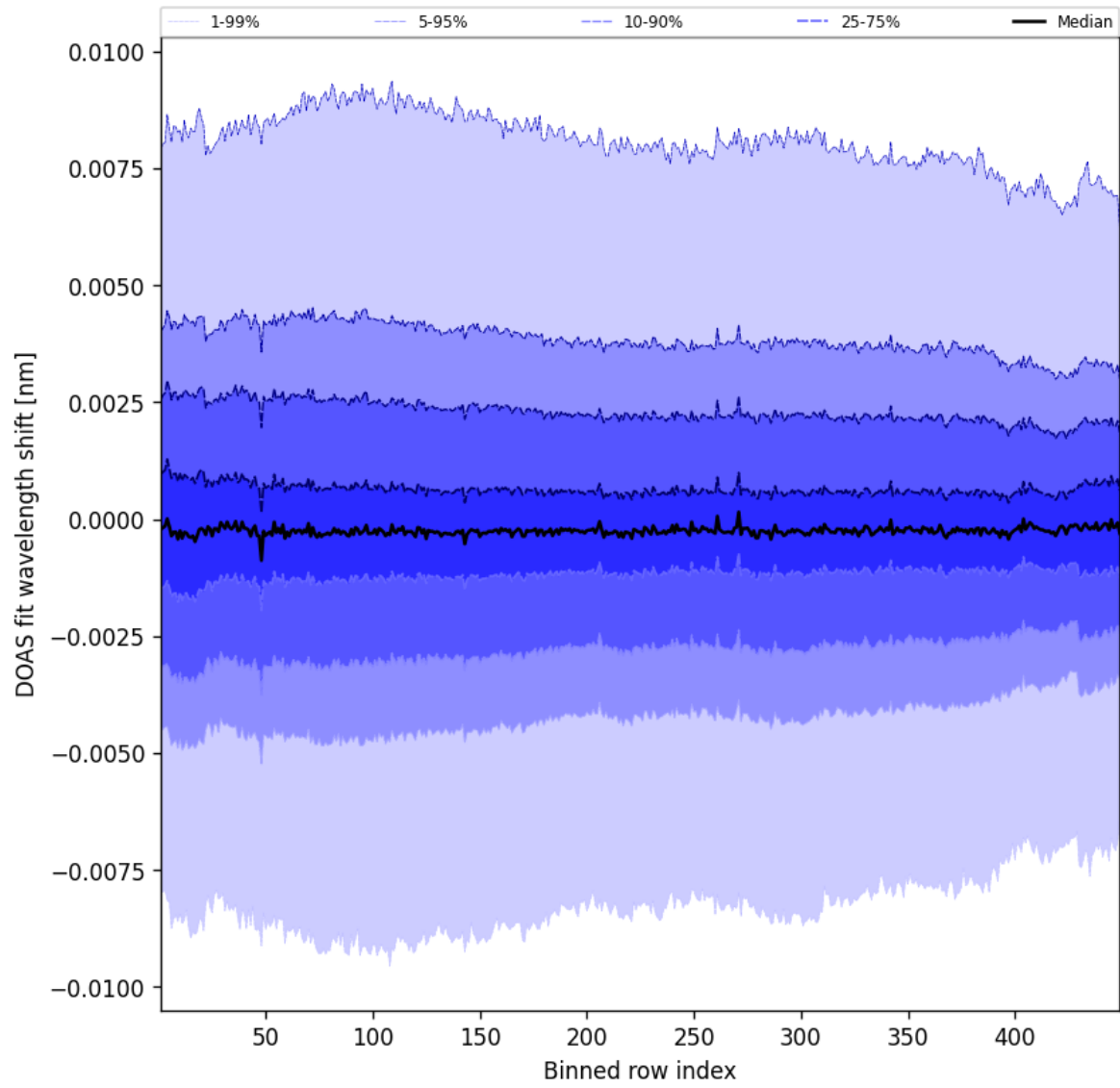
Figure 104: Along track statistics of “DOAS fit wavelength shift” for 2025-08-04 to 2025-08-05
