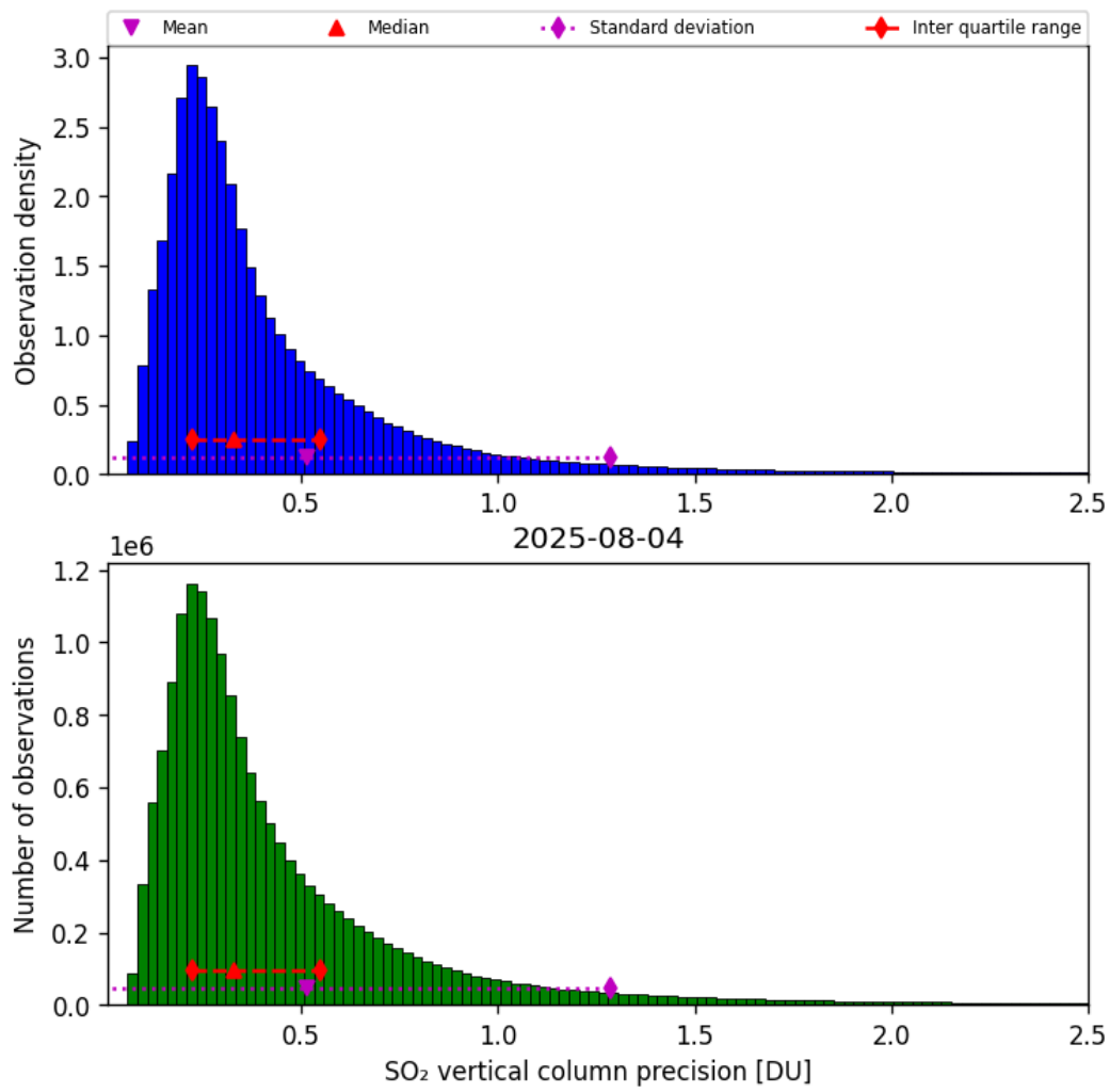
Figure 59: Histogram of “SO 2 vertical column precision” for 2025-08-04 to 2025-08-05
