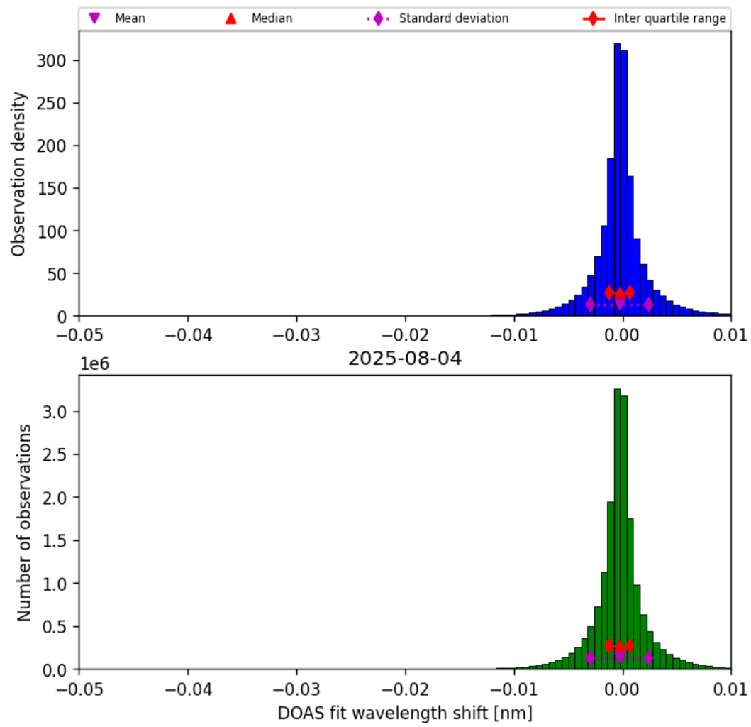
Figure 77: Histogram of “DOAS fit wavelength shift” for 2025-08-04 to 2025-08-05
