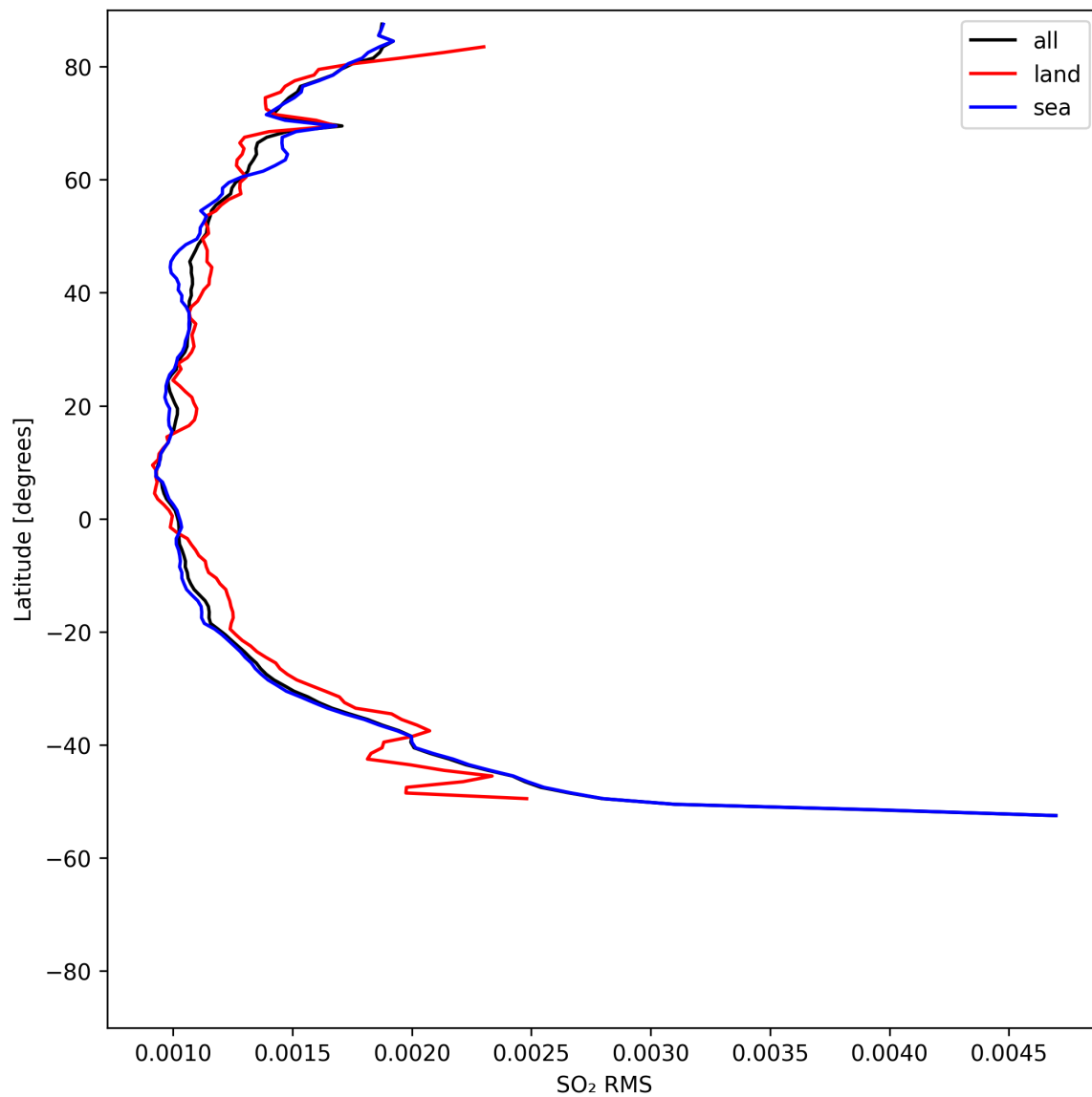
Figure 52: Zonal average of “SO 2 RMS” for 2025-08-04 to 2025-08-05.
