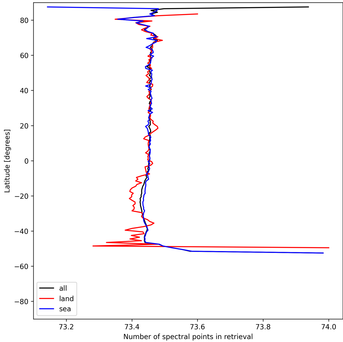
Figure 56: Zonal average of “Number of spectral points in retrieval” for 2025-08-04 to 2025-08-05.
