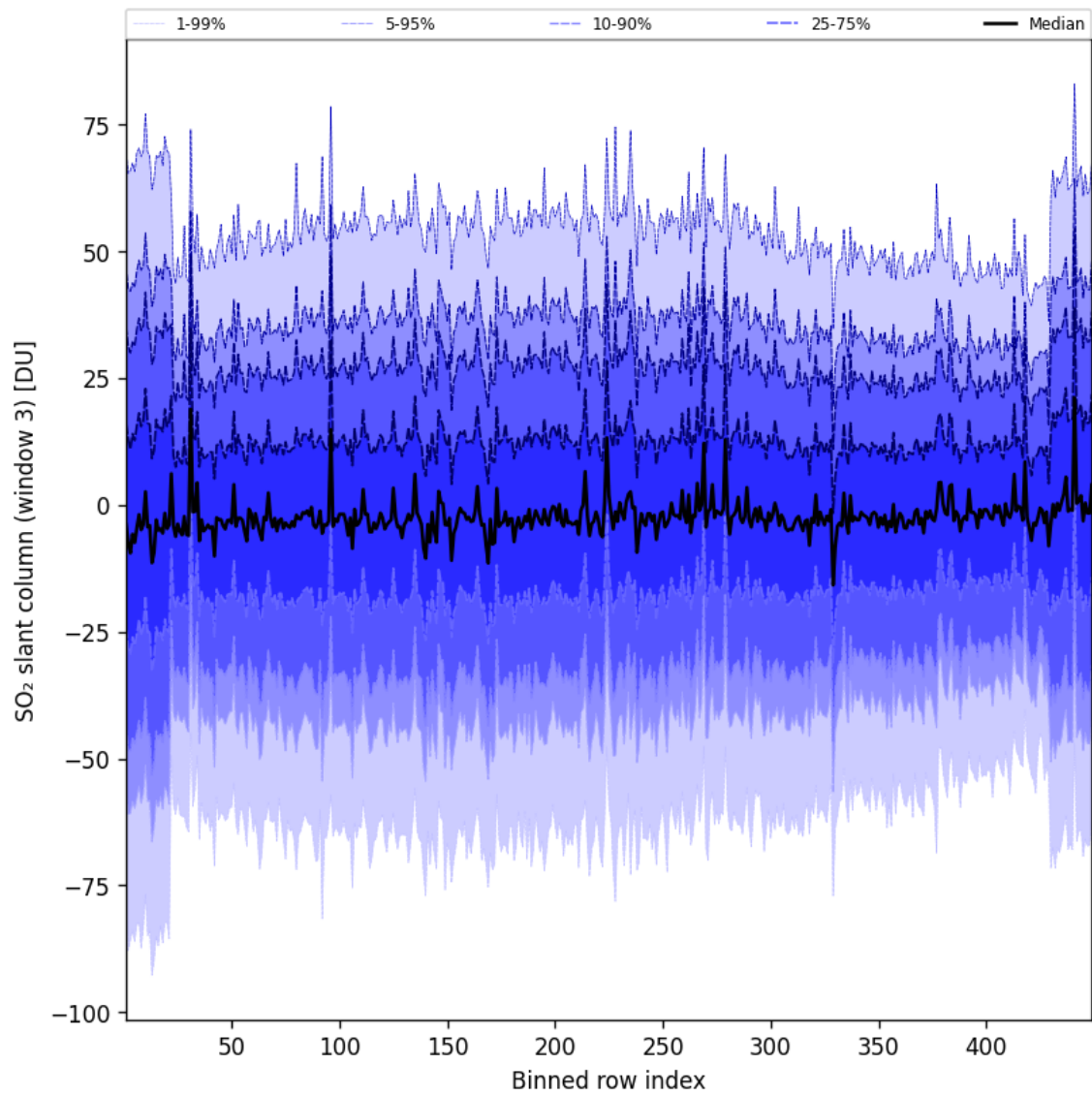
Figure 98: Along track statistics of “SO 2 slant column (window 3)” for 2025-08-04 to 2025-08-05
