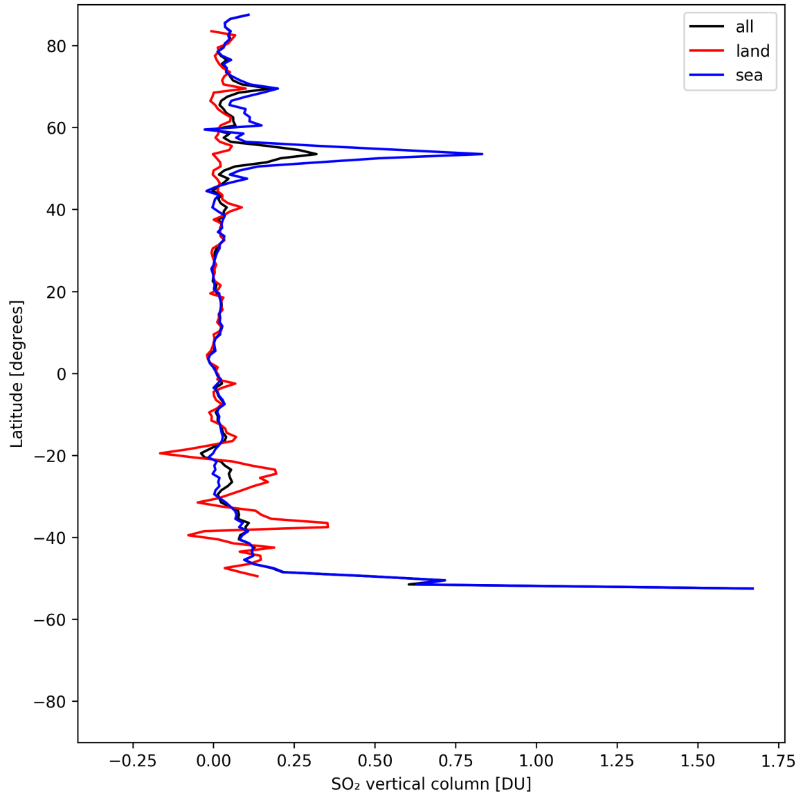
Figure 31: Zonal average of “SO 2 vertical column” for 2025-08-04 to 2025-08-05.
