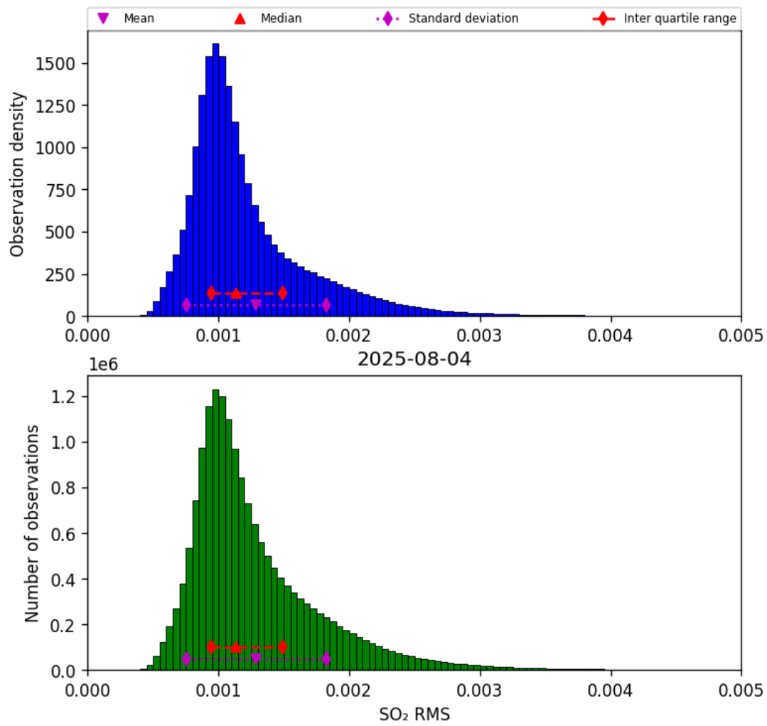
Figure 79: Histogram of “SO 2 RMS” for 2025-08-04 to 2025-08-05
