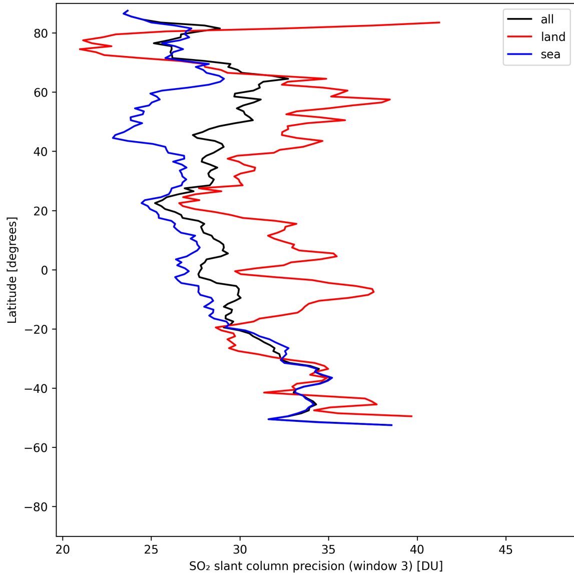
Figure 45: Zonal average of “SO 2 slant column precision (window 3)” for 2025-08-04 to 2025-08-05.
