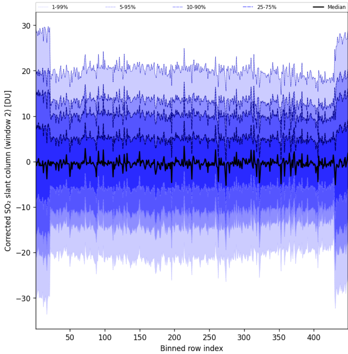
Figure 96: Along track statistics of “Corrected SO 2 slant column (window 2)” for 2025-08-04 to 2025-08-05
