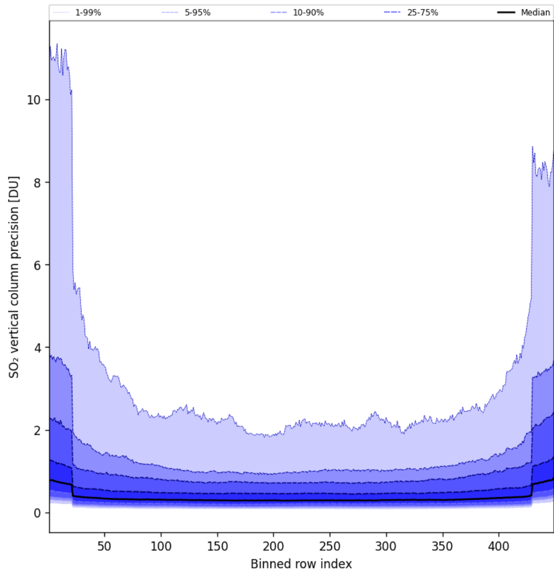
Figure 86: Along track statistics of “SO 2 vertical column precision” for 2025-08-04 to 2025-08-05
