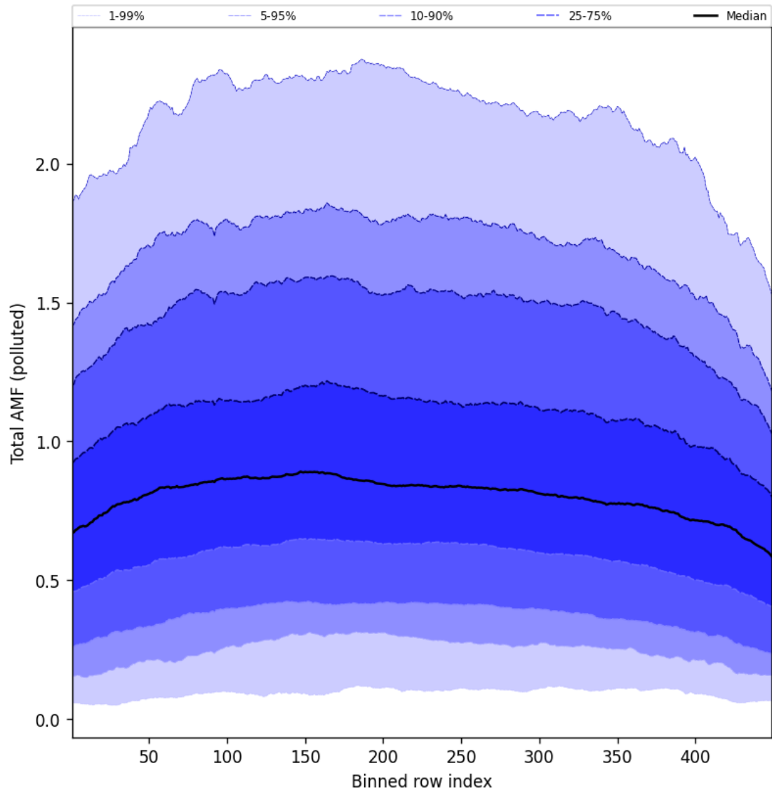
Figure 107: Along track statistics of “Total AMF (polluted)” for 2025-08-04 to 2025-08-05
