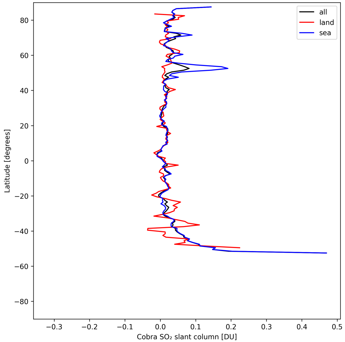
Figure 34: Zonal average of “Cobra SO 2 slant column” for 2025-08-04 to 2025-08-05.
