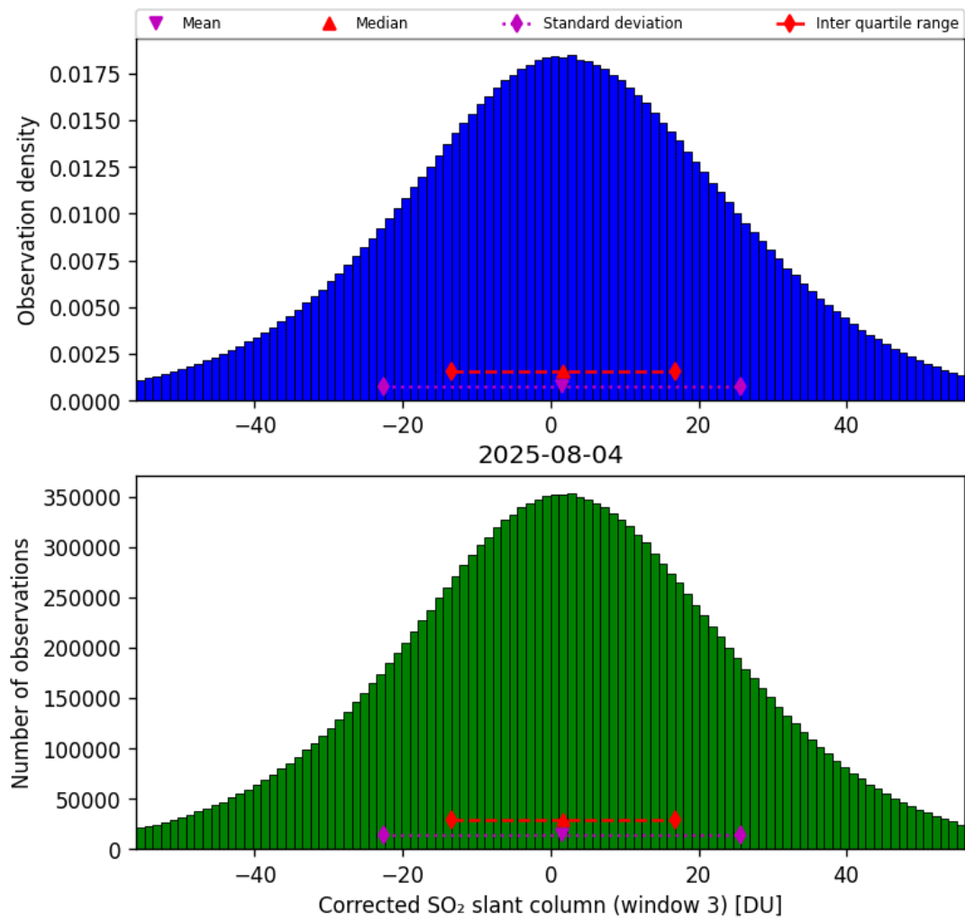
Figure 73: Histogram of “Corrected SO 2 slant column (window 3)” for 2025-08-04 to 2025-08-05
