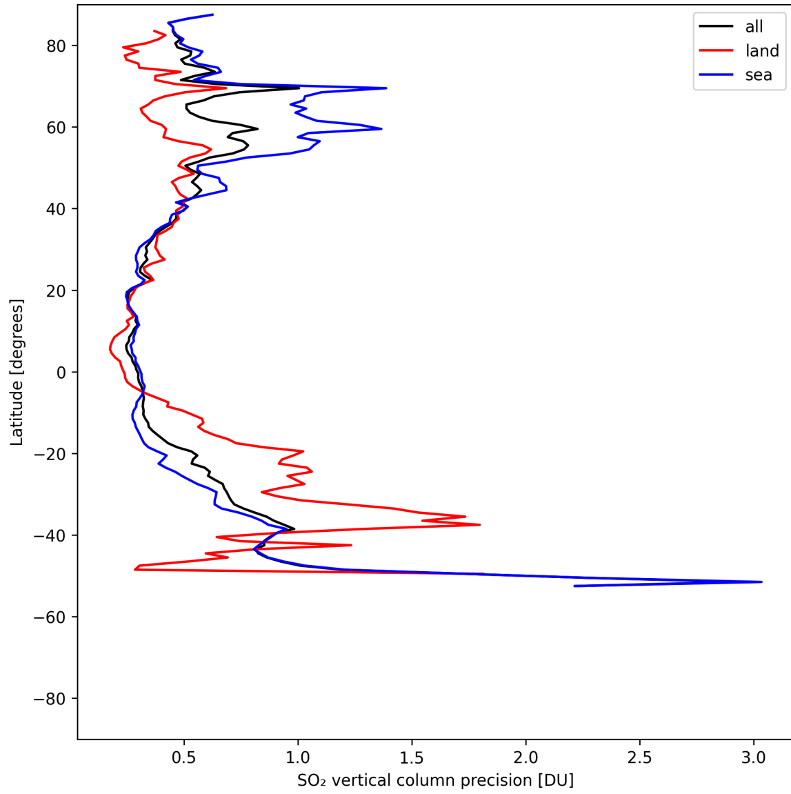
Figure 32: Zonal average of “SO 2 vertical column precision” for 2025-08-04 to 2025-08-05.
