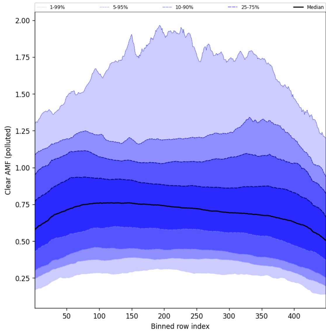
Figure 109: Along track statistics of “Clear AMF (polluted)” for 2025-08-04 to 2025-08-05
