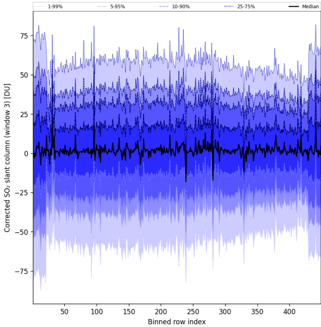
Figure 100: Along track statistics of “Corrected SO 2 slant column (window 3)” for 2025-08-04 to 2025-08-05
