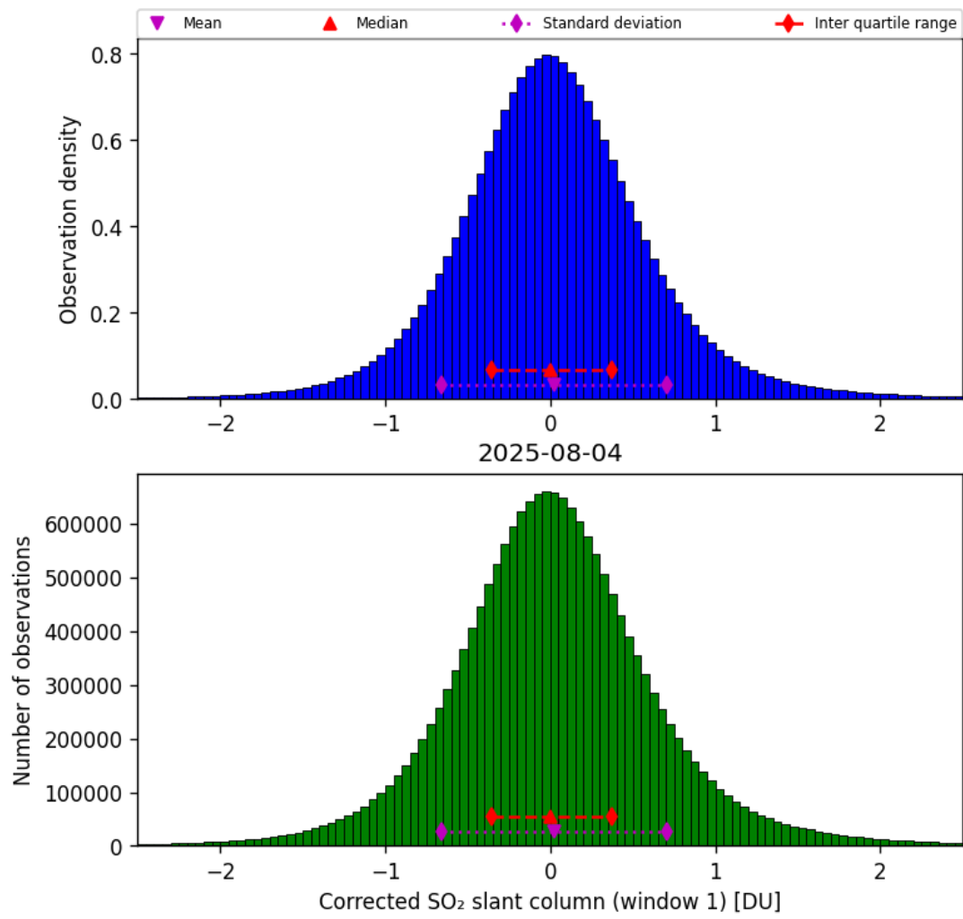
Figure 65: Histogram of “Corrected SO 2 slant column (window 1)” for 2025-08-04 to 2025-08-05
