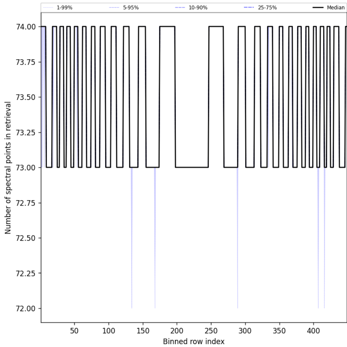
Figure 110: Along track statistics of “Number of spectral points in retrieval” for 2025-08-06 to 2025-08-07
