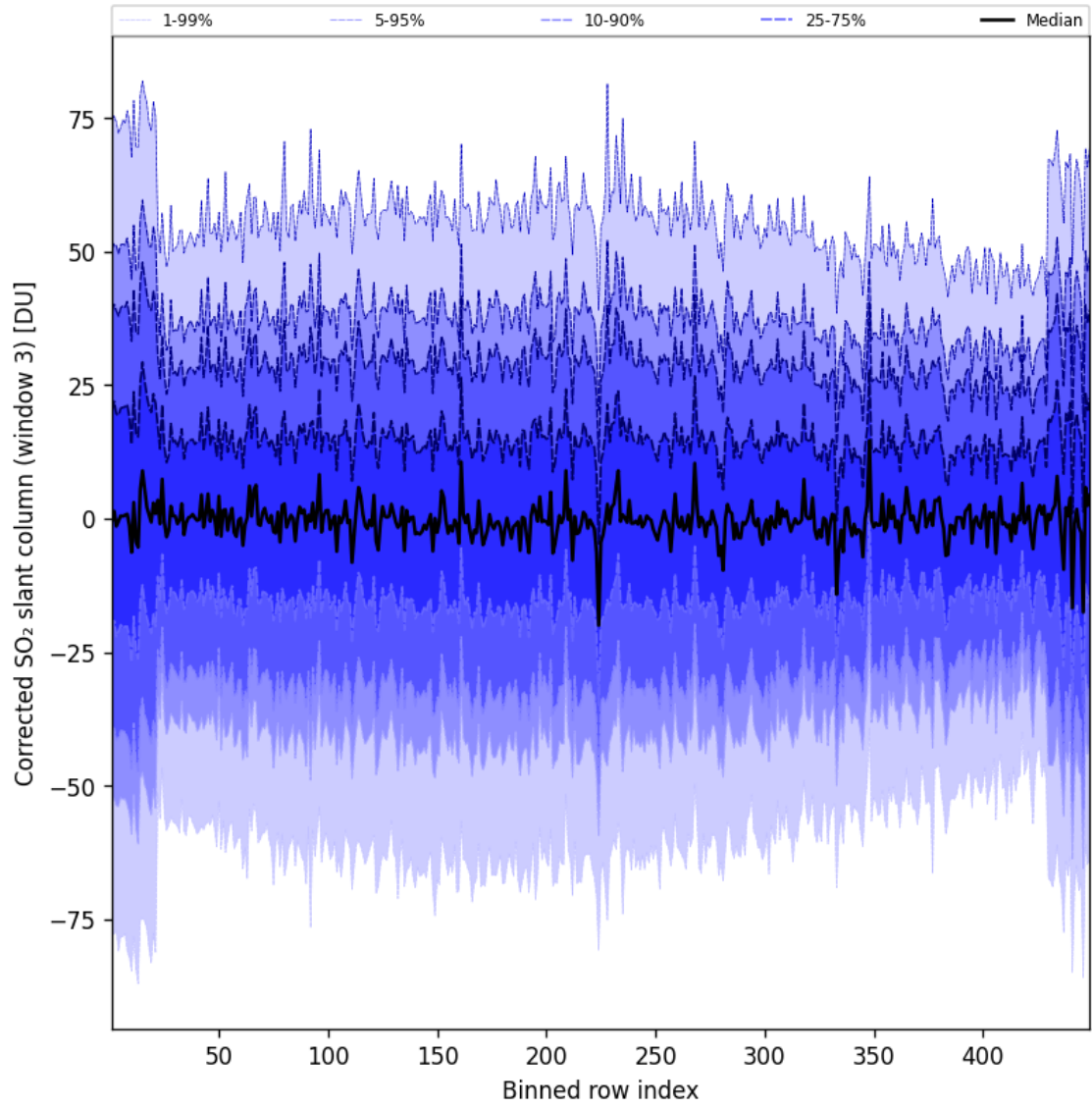
Figure 100: Along track statistics of “Corrected SO 2 slant column (window 3)” for 2025-08-06 to 2025-08-07
