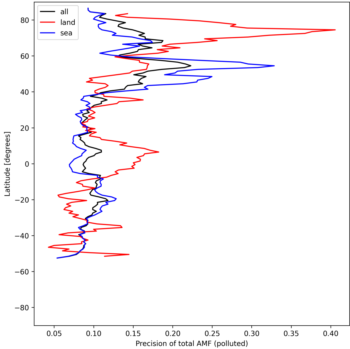
Figure 54: Zonal average of “Precision of total AMF (polluted)” for 2025-08-06 to 2025-08-07.
