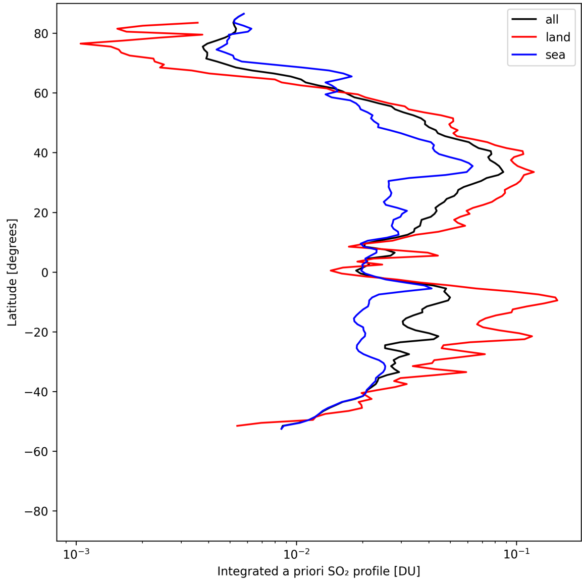
Figure 49: Zonal average of “Integrated a priori SO 2 profile” for 2025-08-06 to 2025-08-07.
