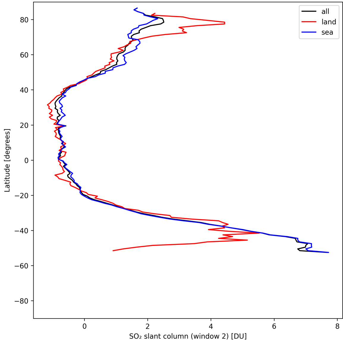
Figure 40: Zonal average of “SO 2 slant column (window 2)” for 2025-08-06 to 2025-08-07.
