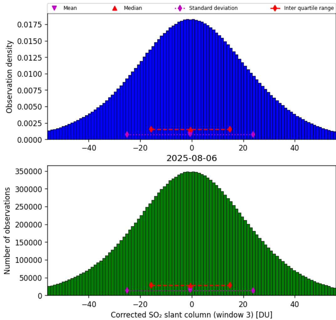
Figure 73: Histogram of “Corrected SO 2 slant column (window 3)” for 2025-08-06 to 2025-08-07
