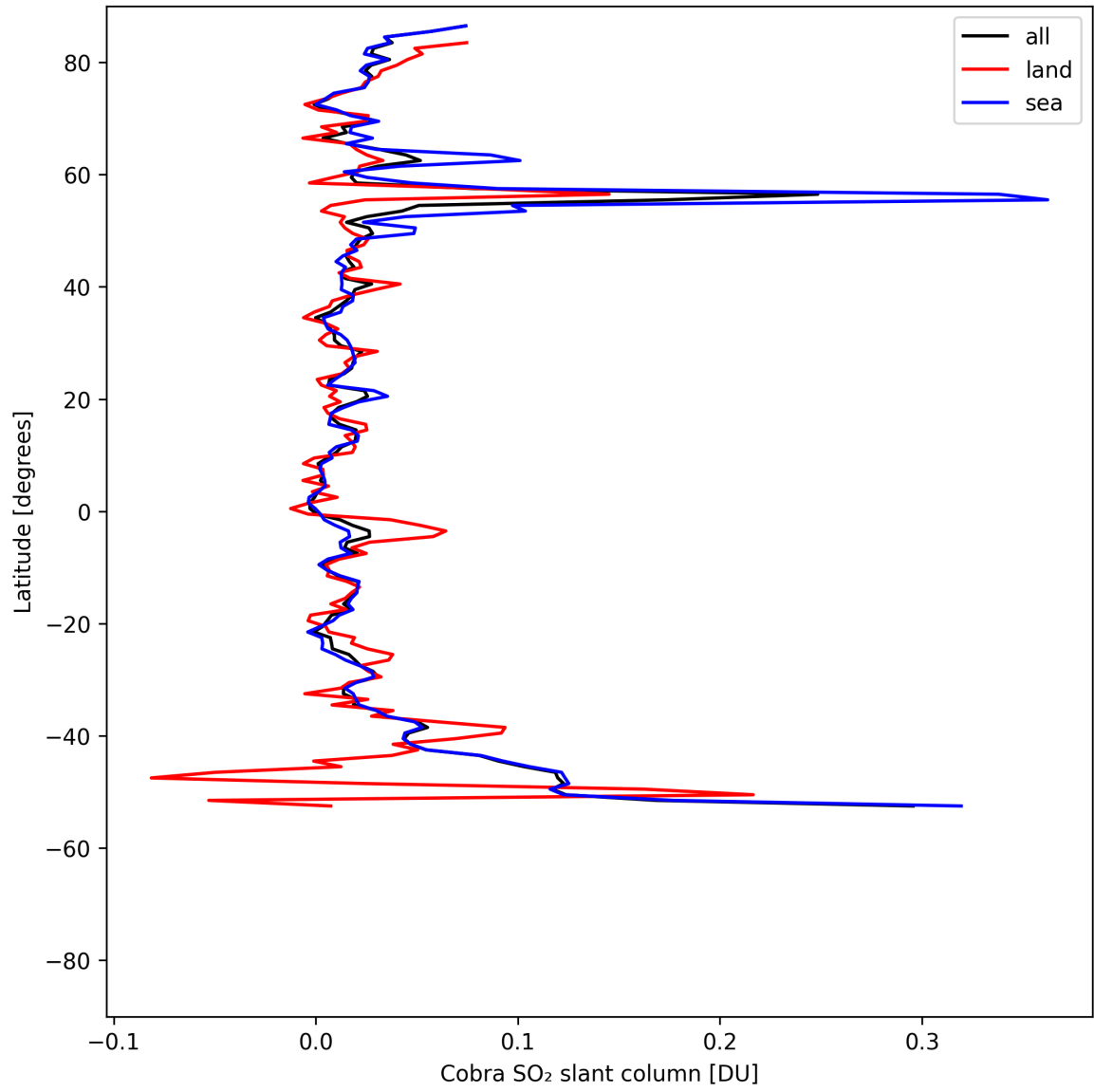
Figure 34: Zonal average of “Cobra SO 2 slant column” for 2025-08-07 to 2025-08-07.
