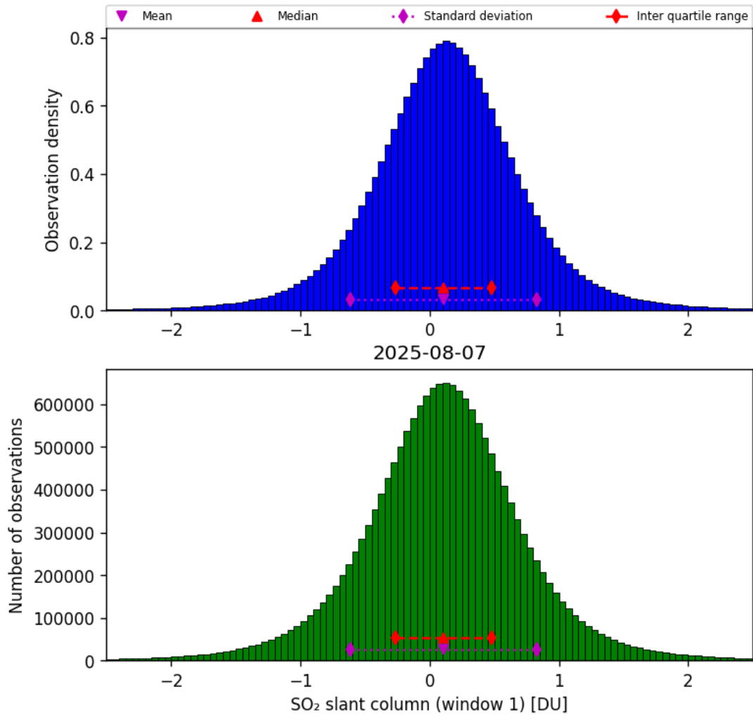
Figure 63: Histogram of “SO 2 slant column (window 1)” for 2025-08-07 to 2025-08-07
