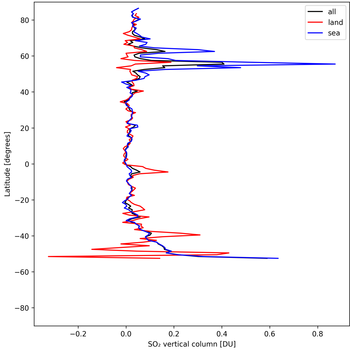
Figure 31: Zonal average of “SO 2 vertical column” for 2025-08-07 to 2025-08-07.
