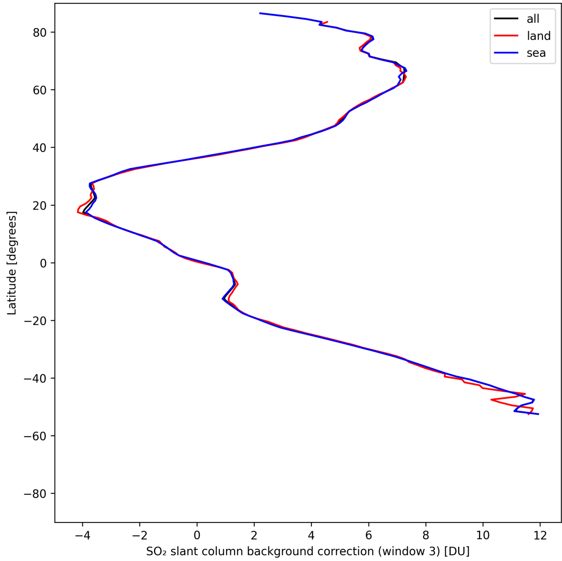
Figure 47: Zonal average of “SO 2 slant column background correction (window 3)” for 2025-08-07 to 2025-08-07.
