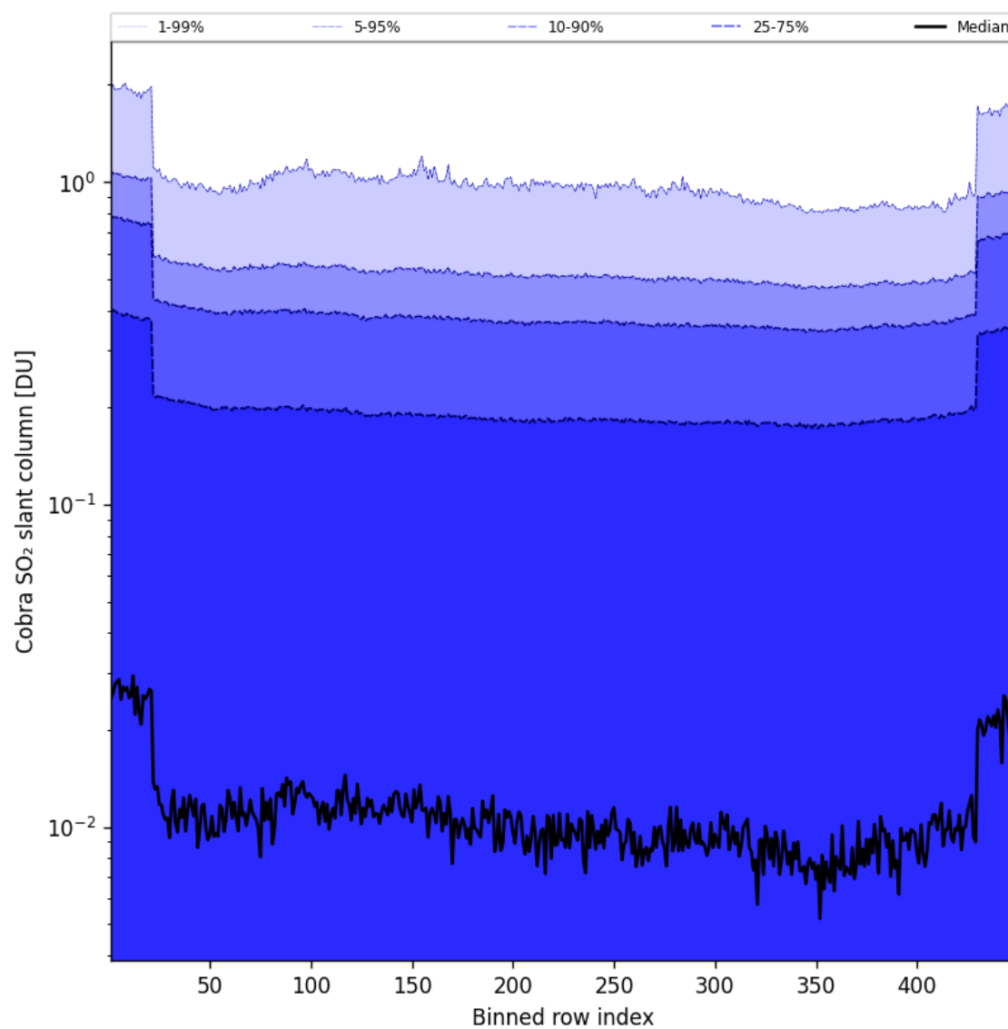
Figure 88: Along track statistics of “Cobra SO 2 slant column” for 2025-08-07 to 2025-08-07
