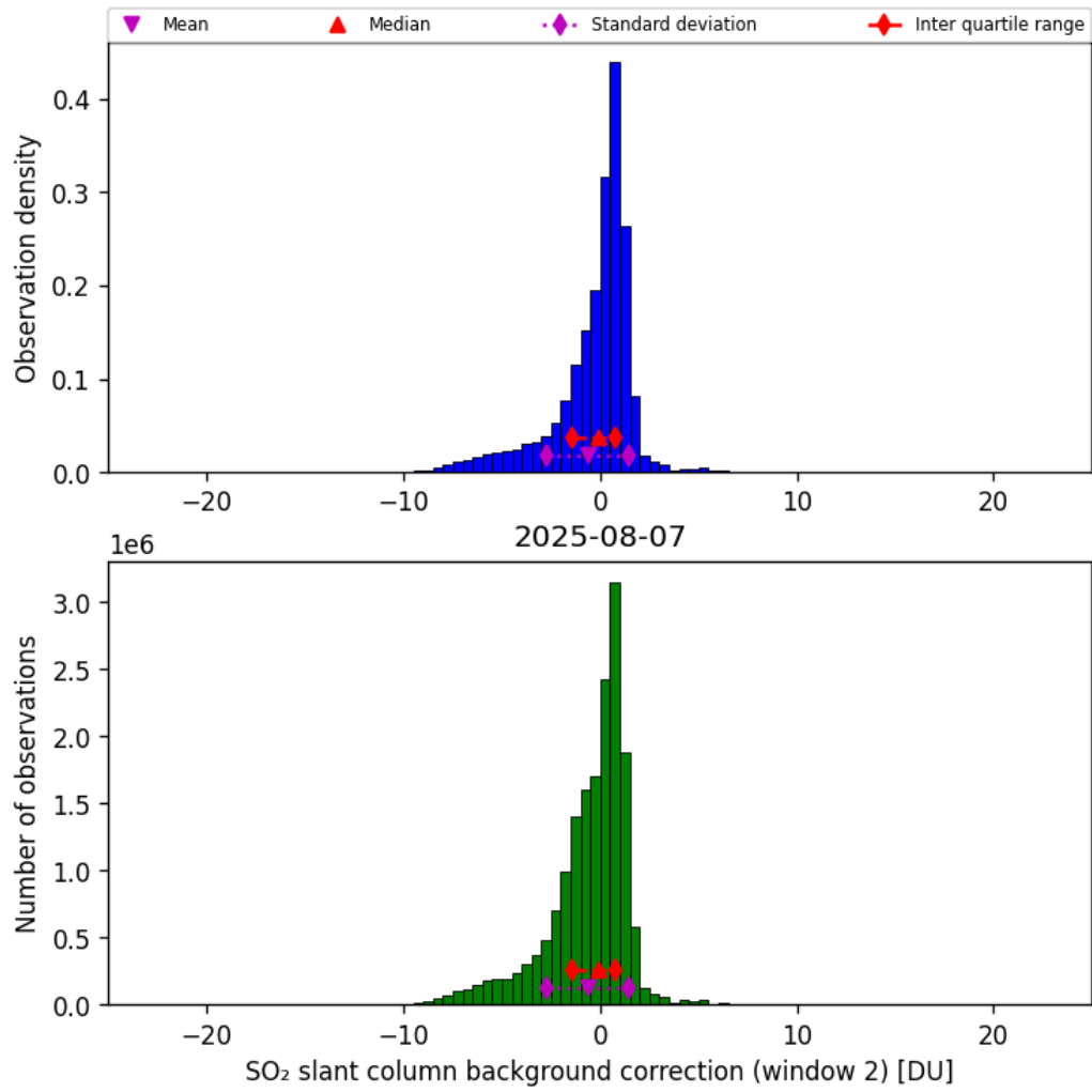
Figure 70: Histogram of “SO 2 slant column background correction (window 2)” for 2025-08-07 to 2025-08-07
