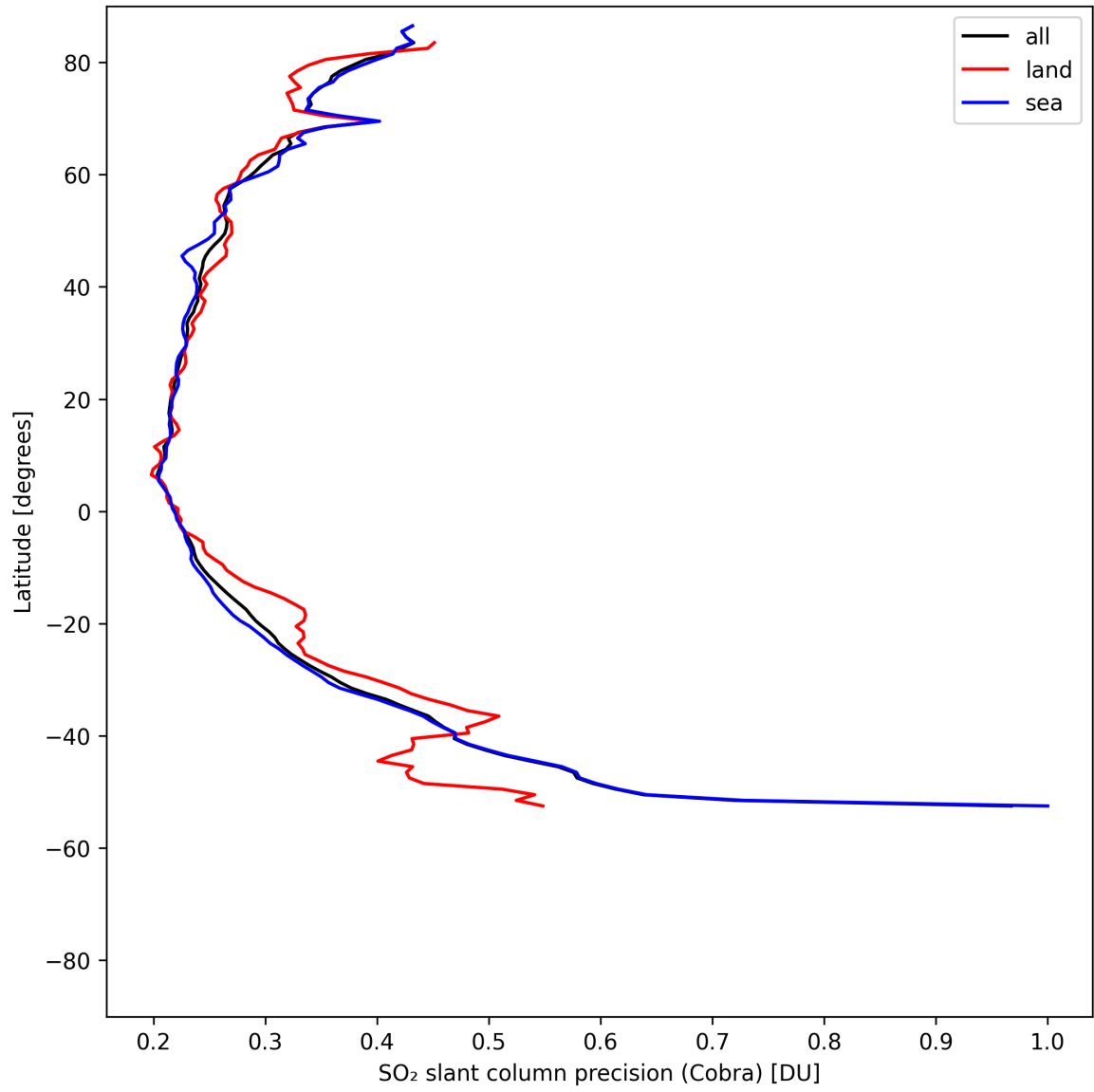
Figure 35: Zonal average of “SO 2 slant column precision (Cobra)” for 2025-08-07 to 2025-08-07.
