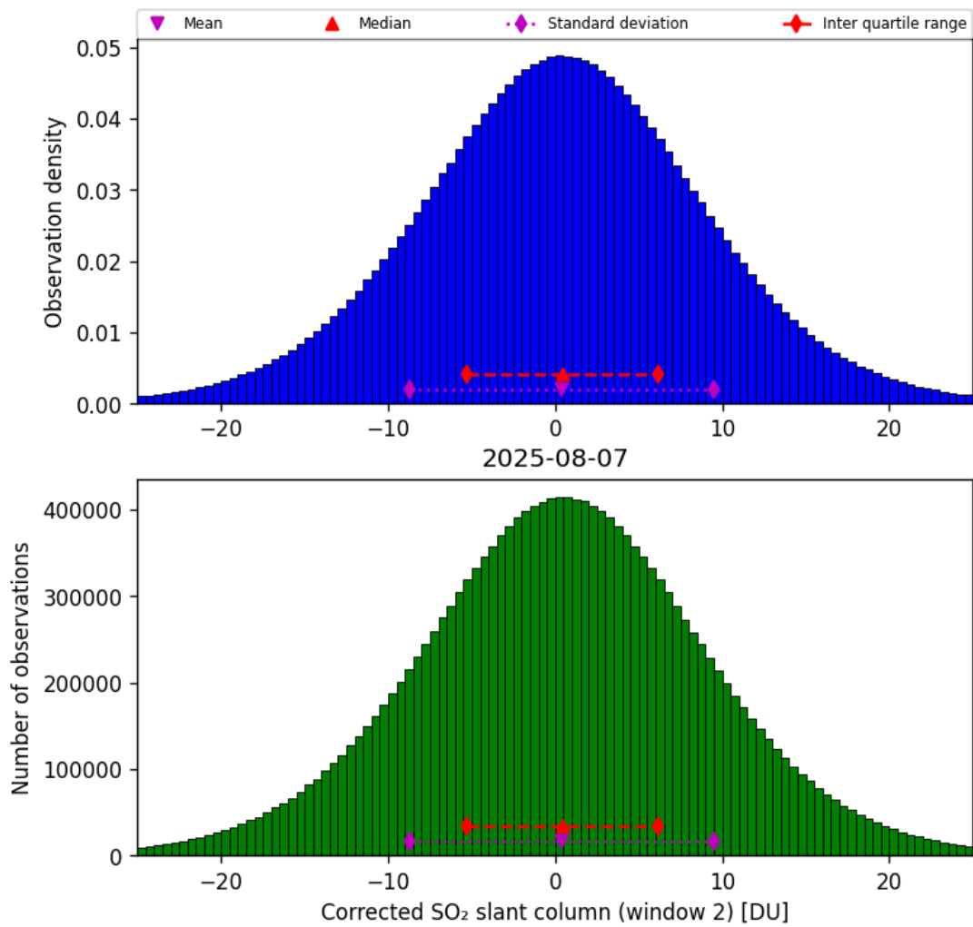
Figure 69: Histogram of “Corrected SO 2 slant column (window 2)” for 2025-08-07 to 2025-08-07
