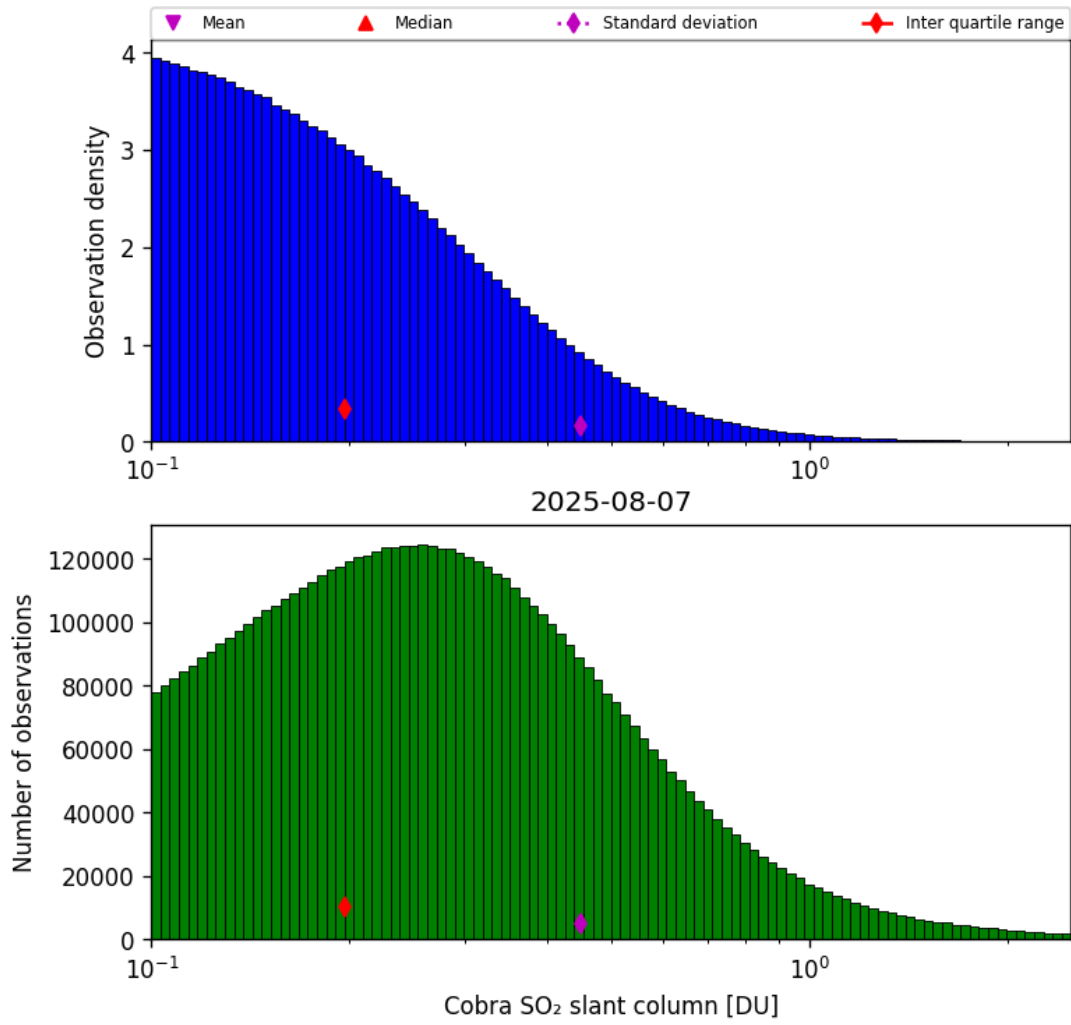
Figure 61: Histogram of “Cobra SO 2 slant column” for 2025-08-07 to 2025-08-07
