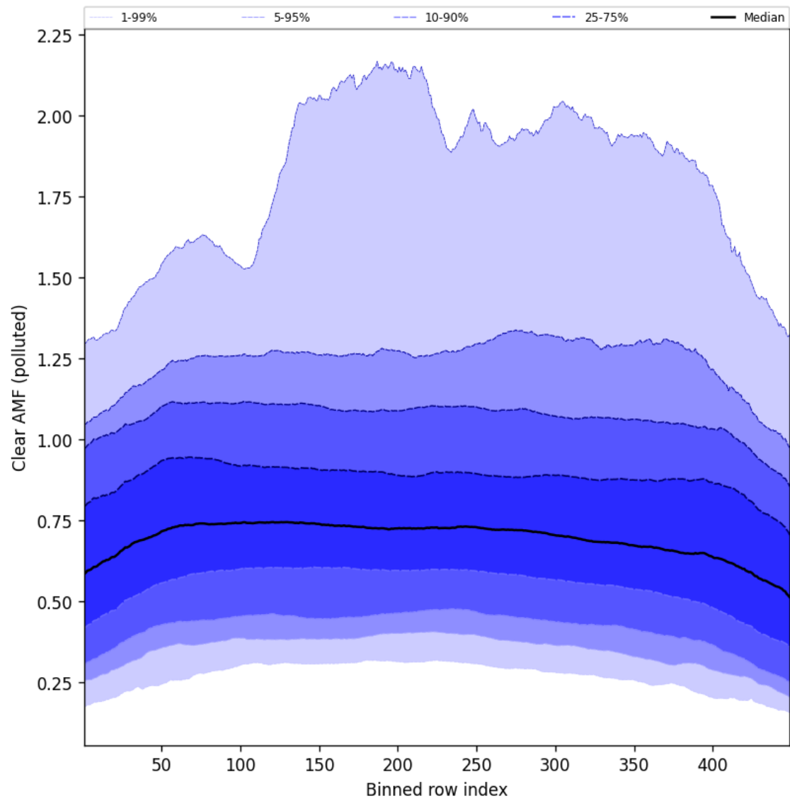
Figure 109: Along track statistics of “Clear AMF (polluted)” for 2025-08-07 to 2025-08-07
