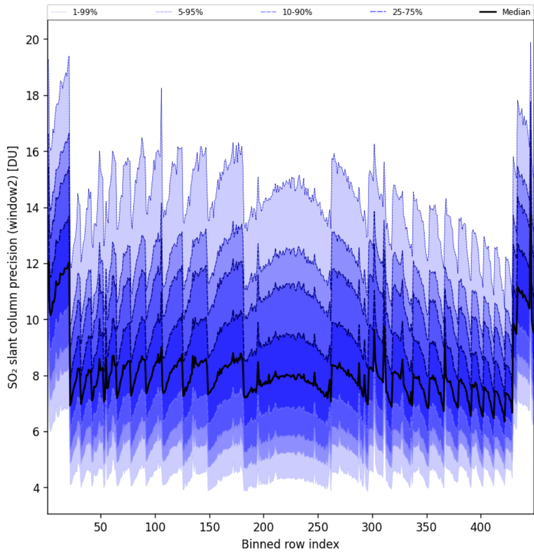
Figure 95: Along track statistics of “SO 2 slant column precision (window2)” for 2025-08-07 to 2025-08-07
