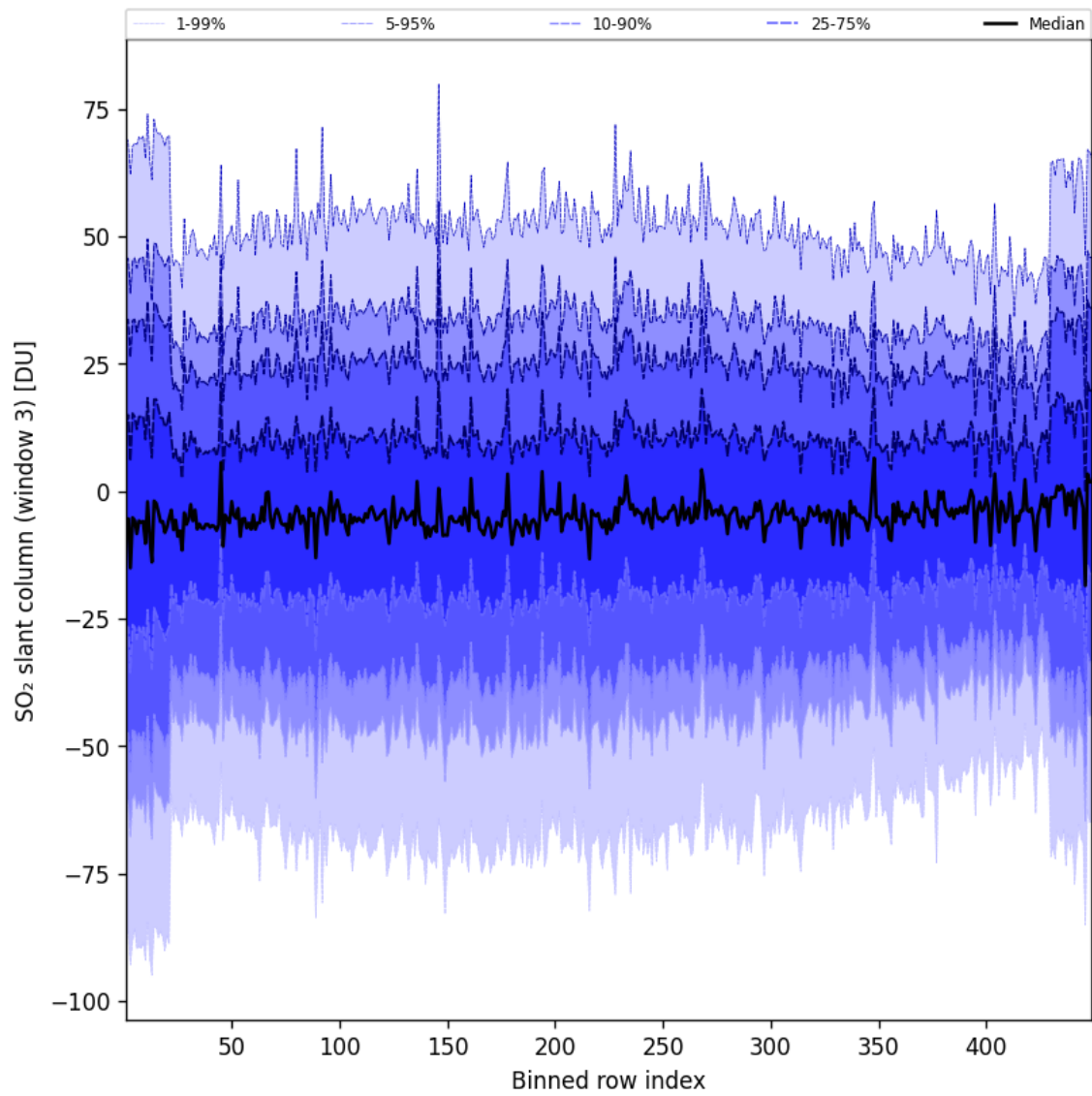
Figure 98: Along track statistics of “SO 2 slant column (window 3)” for 2025-08-07 to 2025-08-07
