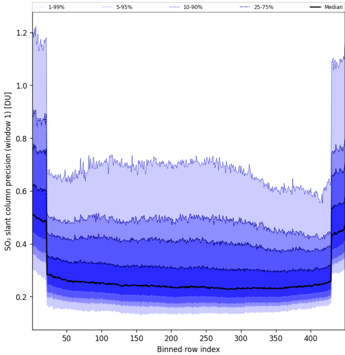
Figure 91: Along track statistics of “SO 2 slant column precision (window 1)” for 2025-08-07 to 2025-08-07
