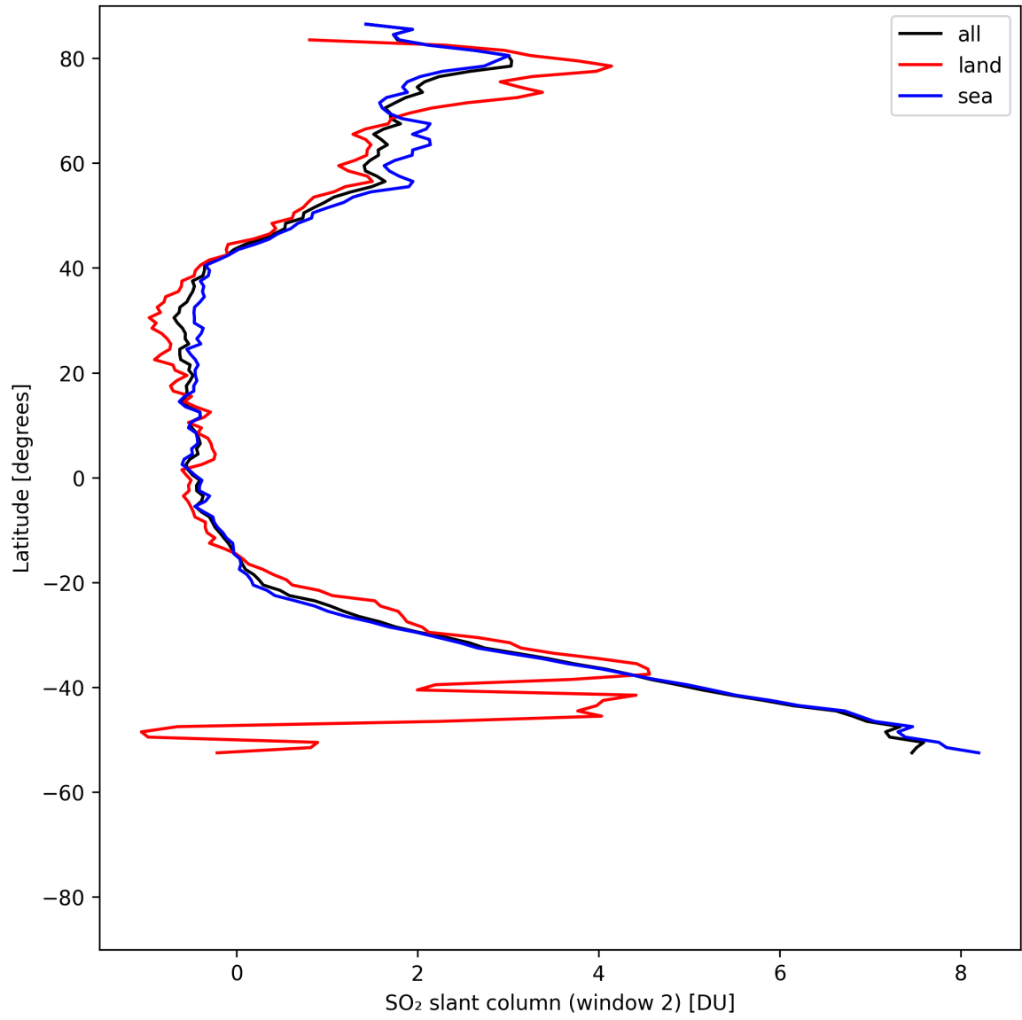
Figure 40: Zonal average of “SO 2 slant column (window 2)” for 2025-08-07 to 2025-08-07.
