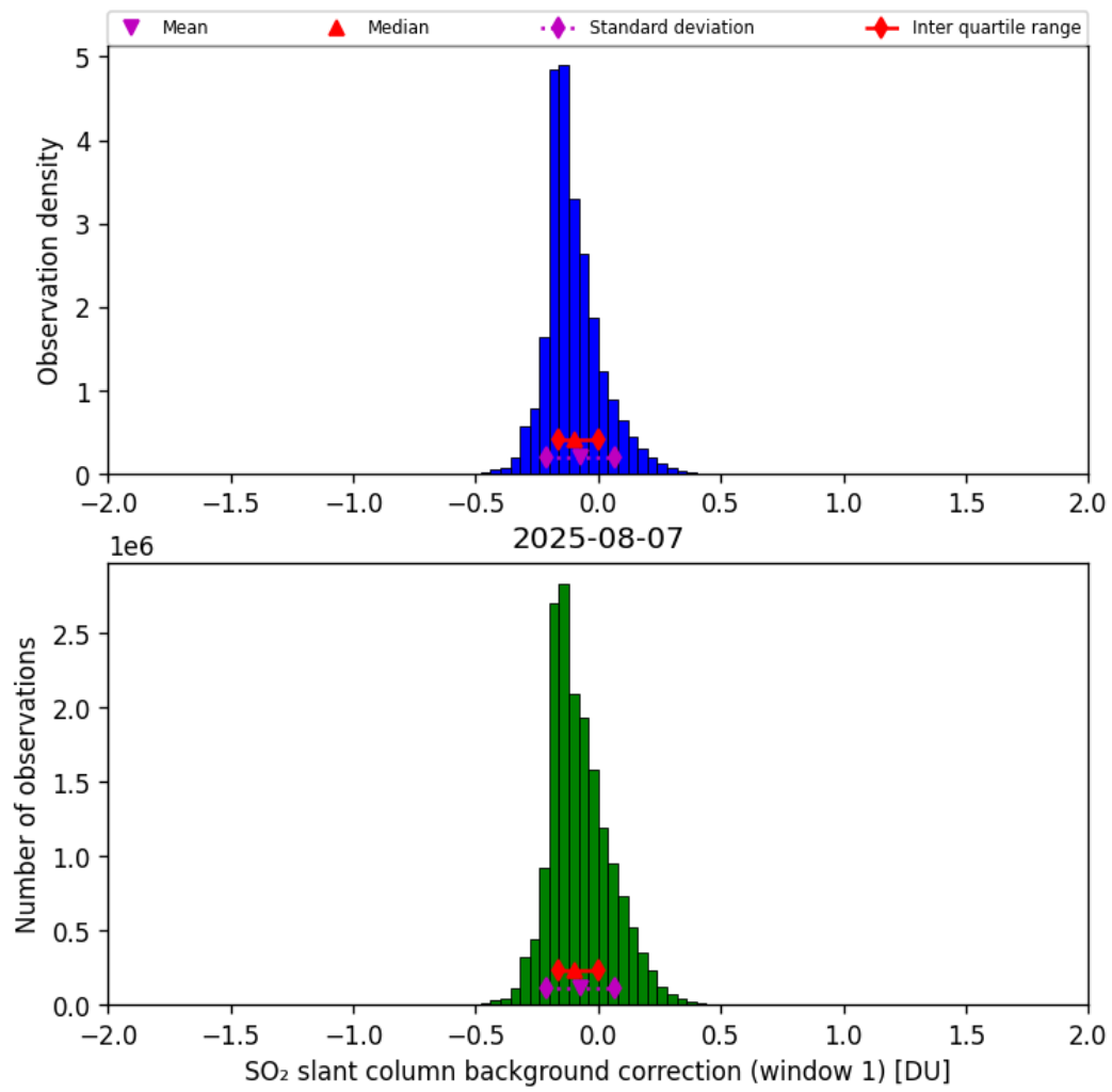
Figure 66: Histogram of “SO 2 slant column background correction (window 1)” for 2025-08-07 to 2025-08-07
