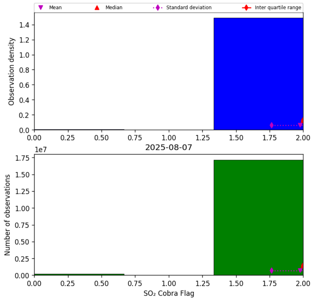
Figure 75: Histogram of “SO 2 Cobra Flag” for 2025-08-07 to 2025-08-07
