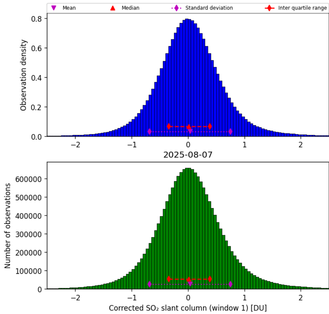
Figure 65: Histogram of “Corrected SO 2 slant column (window 1)” for 2025-08-07 to 2025-08-07
