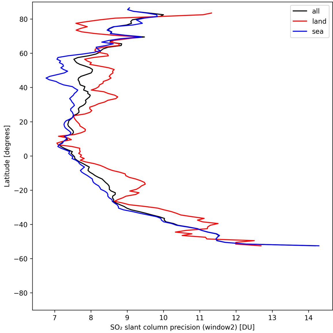
Figure 41: Zonal average of “SO 2 slant column precision (window2)” for 2025-08-07 to 2025-08-07.
