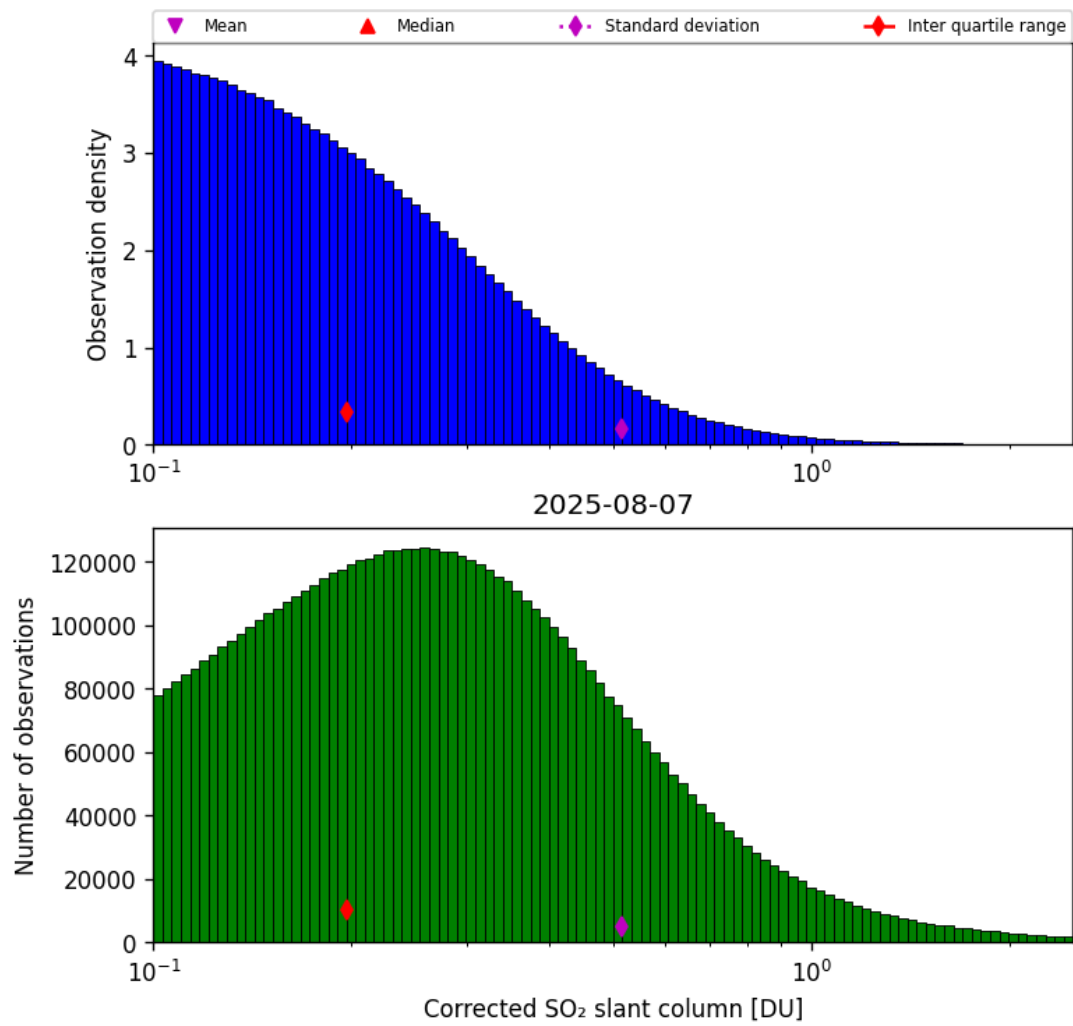
Figure 60: Histogram of “Corrected SO 2 slant column” for 2025-08-07 to 2025-08-07
