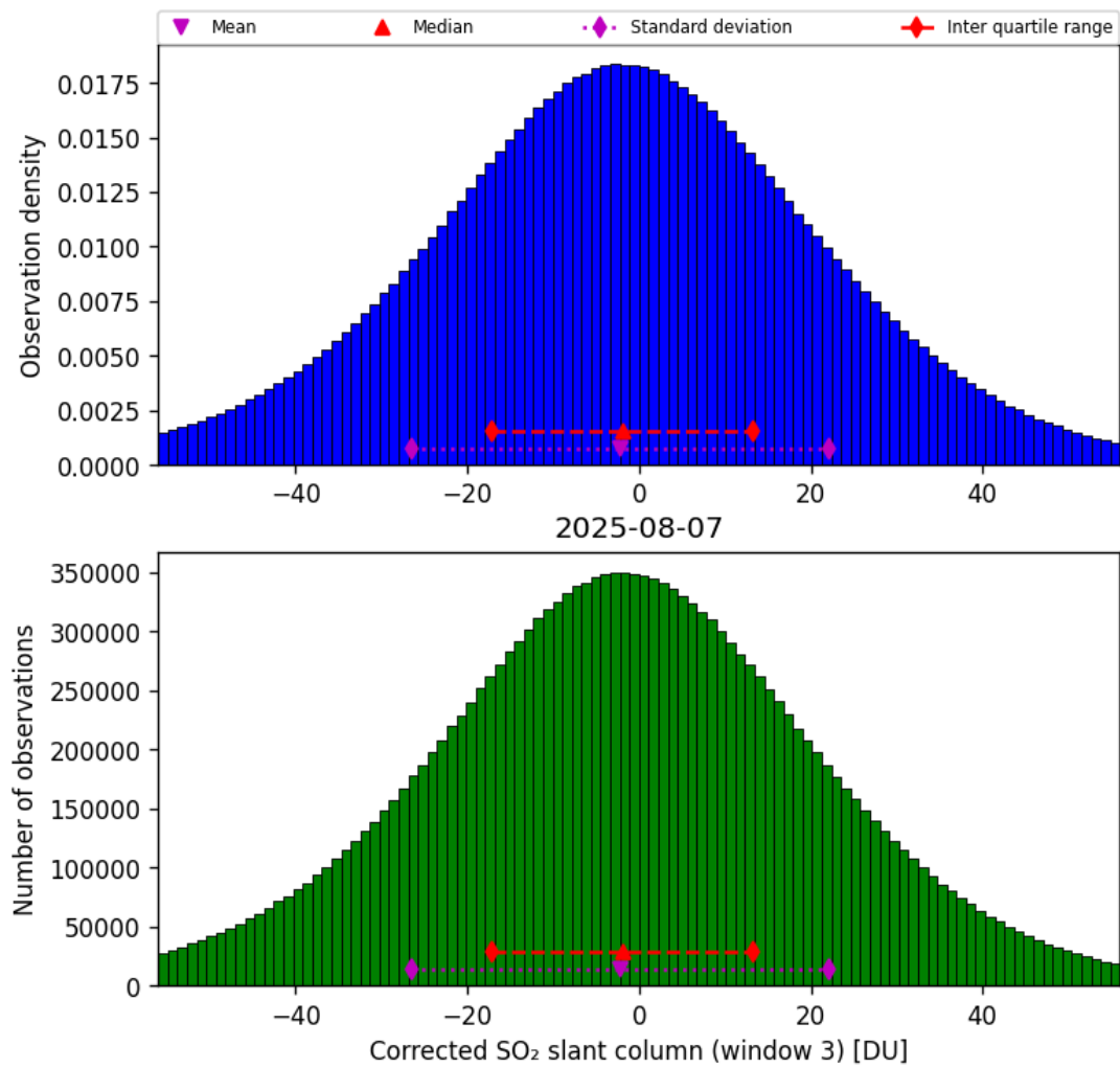
Figure 73: Histogram of “Corrected SO 2 slant column (window 3)” for 2025-08-07 to 2025-08-07
