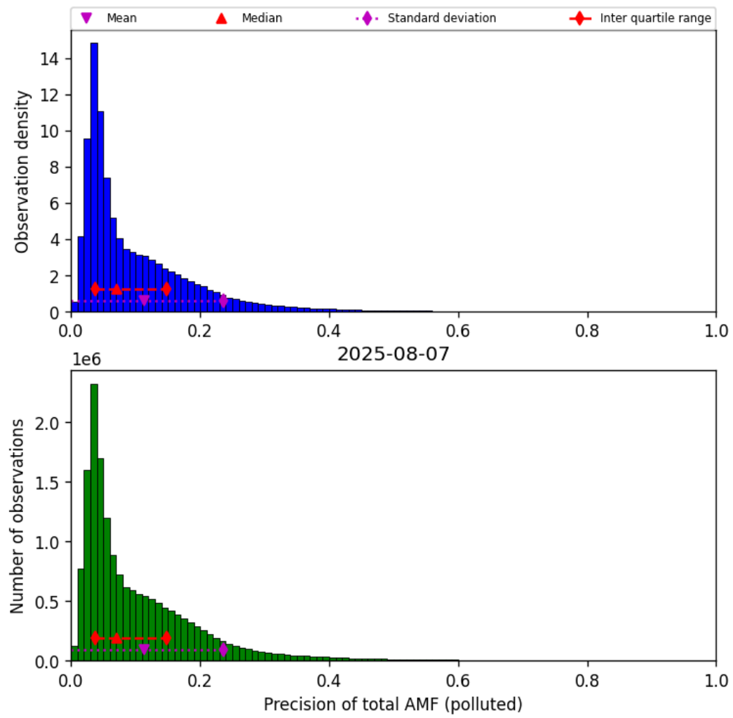
Figure 81: Histogram of “Precision of total AMF (polluted)” for 2025-08-07 to 2025-08-07
