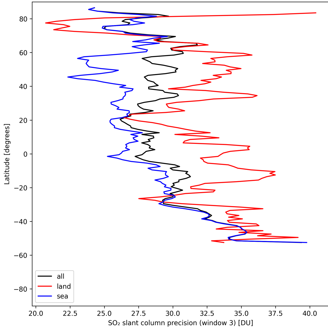
Figure 45: Zonal average of “SO 2 slant column precision (window 3)” for 2025-08-07 to 2025-08-07.
