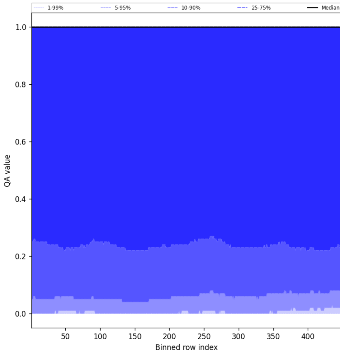
Figure 84: Along track statistics of “QA value” for 2025-08-07 to 2025-08-07
