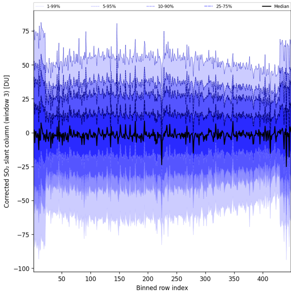
Figure 100: Along track statistics of “Corrected SO 2 slant column (window 3)” for 2025-08-07 to 2025-08-07
