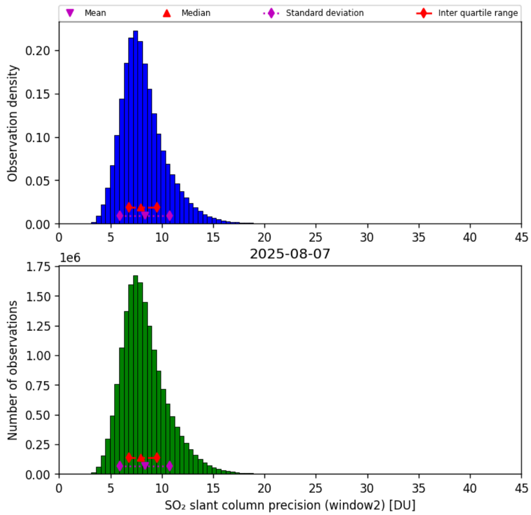
Figure 68: Histogram of “SO 2 slant column precision (window2)” for 2025-08-07 to 2025-08-07
