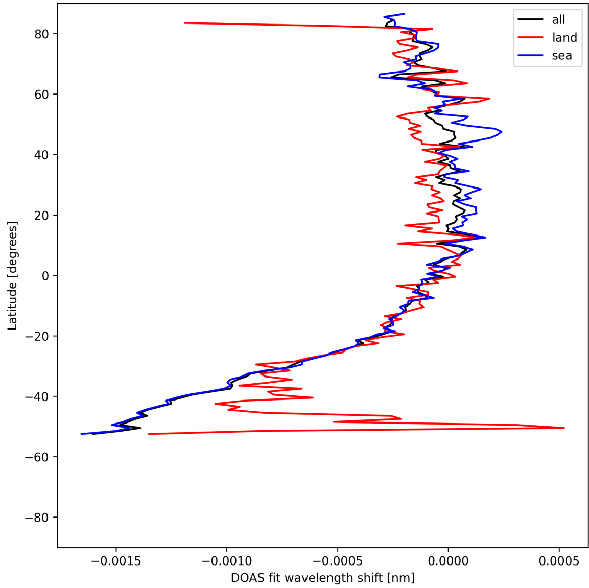
Figure 50: Zonal average of “DOAS fit wavelength shift” for 2025-08-07 to 2025-08-07.
