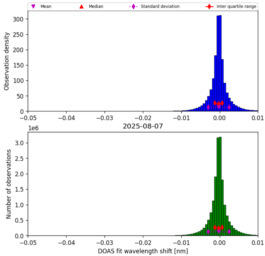
Figure 77: Histogram of “DOAS fit wavelength shift” for 2025-08-07 to 2025-08-07
