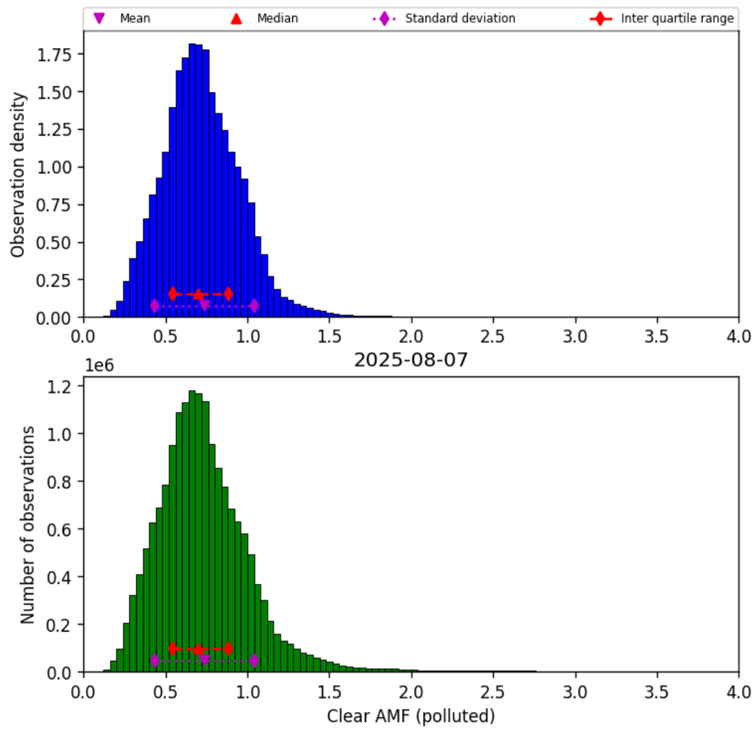
Figure 82: Histogram of “Clear AMF (polluted)” for 2025-08-07 to 2025-08-07
