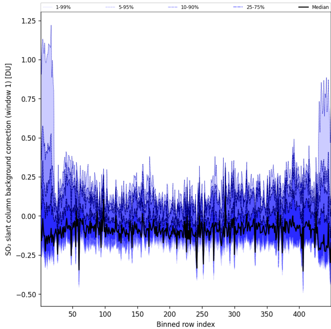
Figure 93: Along track statistics of “SO 2 slant column background correction (window 1)” for 2025-08-07 to 2025-08-07
