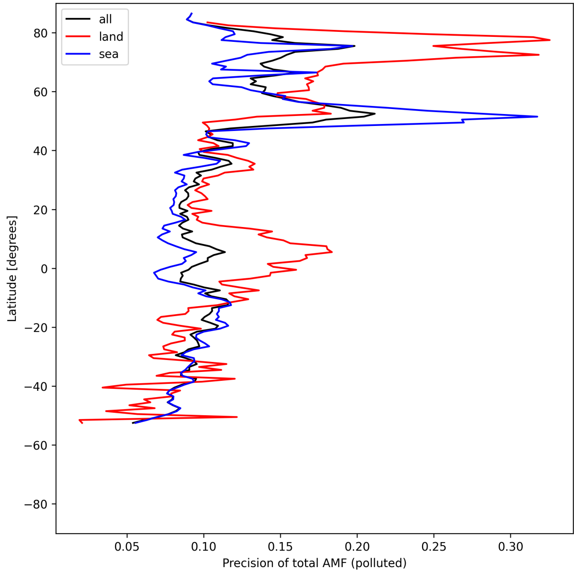
Figure 54: Zonal average of “Precision of total AMF (polluted)” for 2025-08-07 to 2025-08-07.
