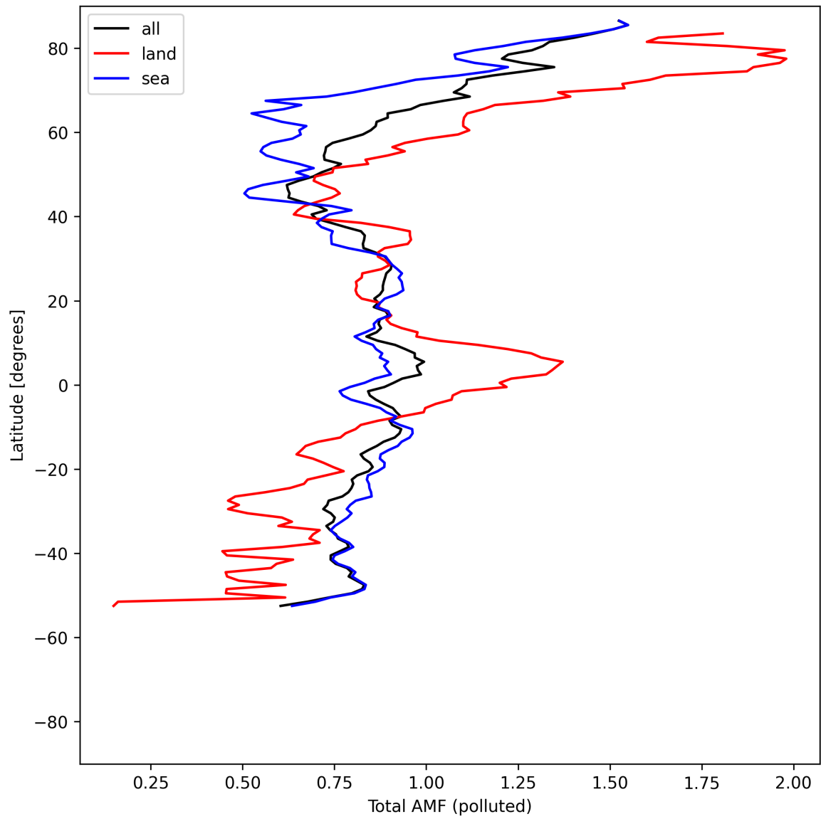
Figure 53: Zonal average of “Total AMF (polluted)” for 2025-08-07 to 2025-08-07.
