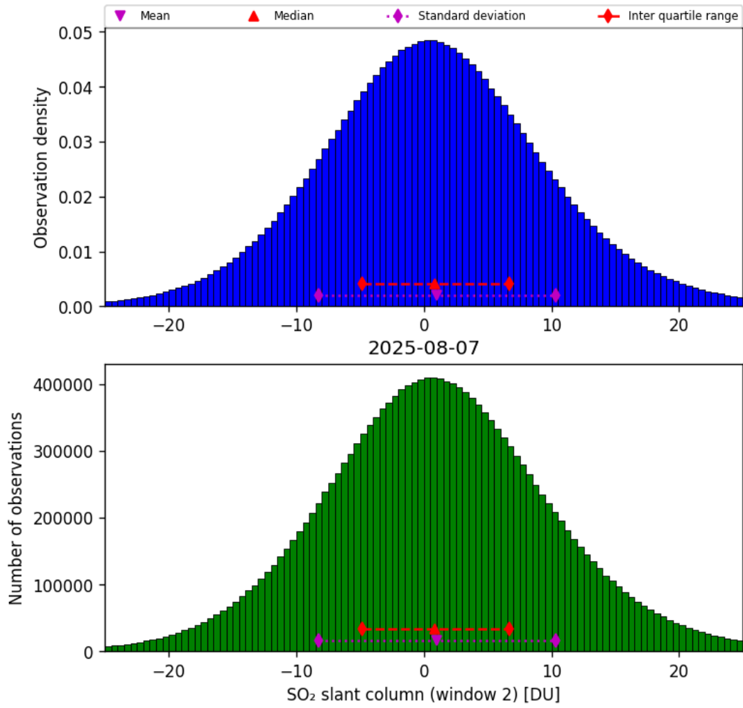
Figure 67: Histogram of “SO 2 slant column (window 2)” for 2025-08-07 to 2025-08-07
