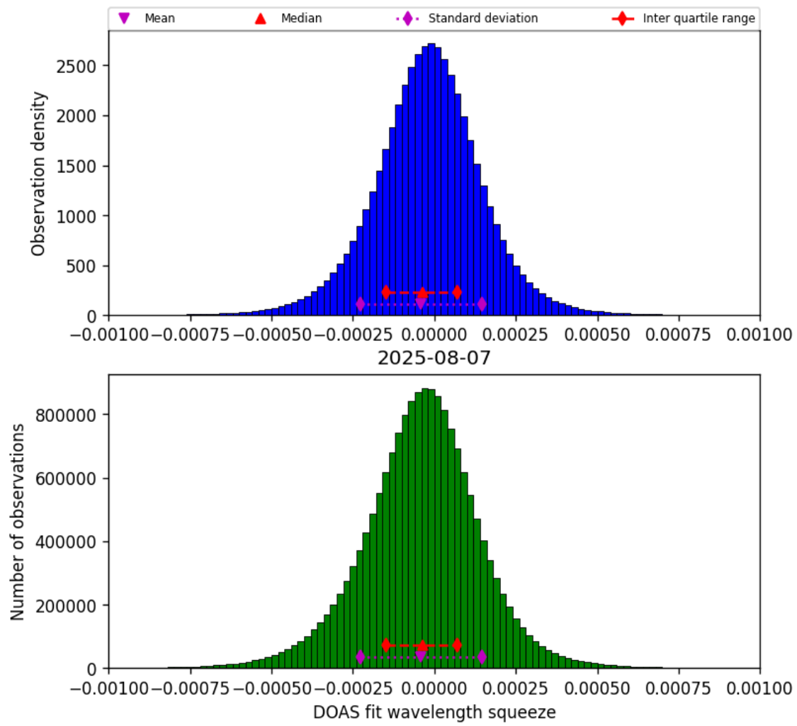
Figure 78: Histogram of “DOAS fit wavelength squeeze” for 2025-08-07 to 2025-08-07
