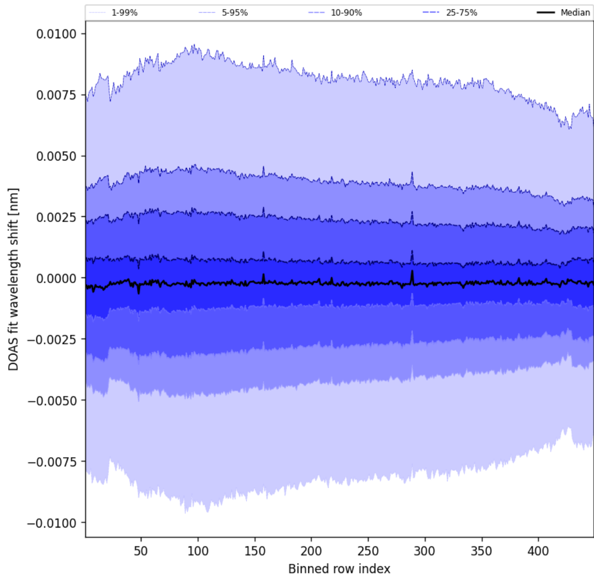
Figure 104: Along track statistics of “DOAS fit wavelength shift” for 2025-08-07 to 2025-08-07
