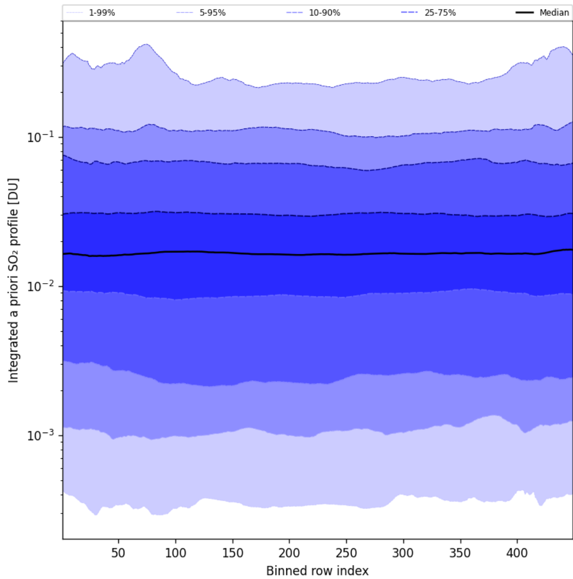
Figure 103: Along track statistics of “Integrated a priori SO 2 profile” for 2025-08-07 to 2025-08-07
