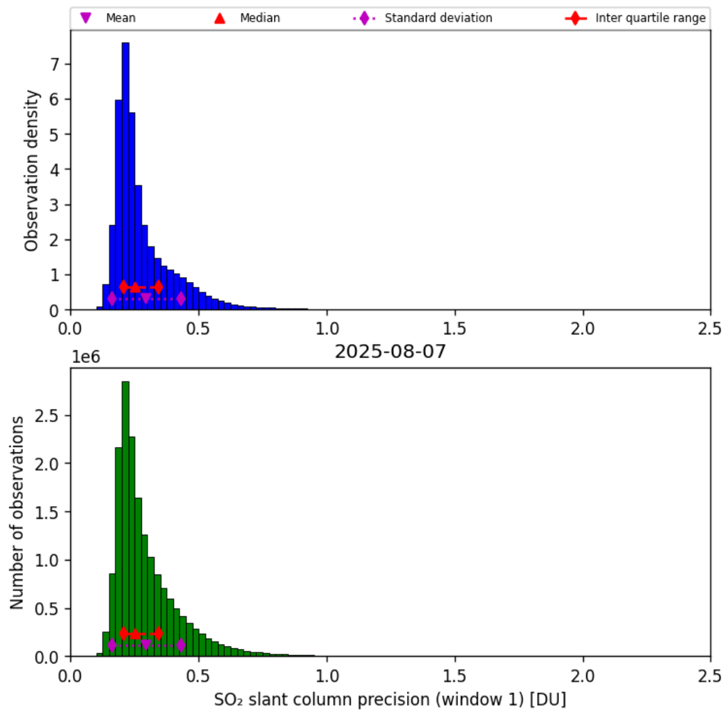
Figure 64: Histogram of “SO 2 slant column precision (window 1)” for 2025-08-07 to 2025-08-07
