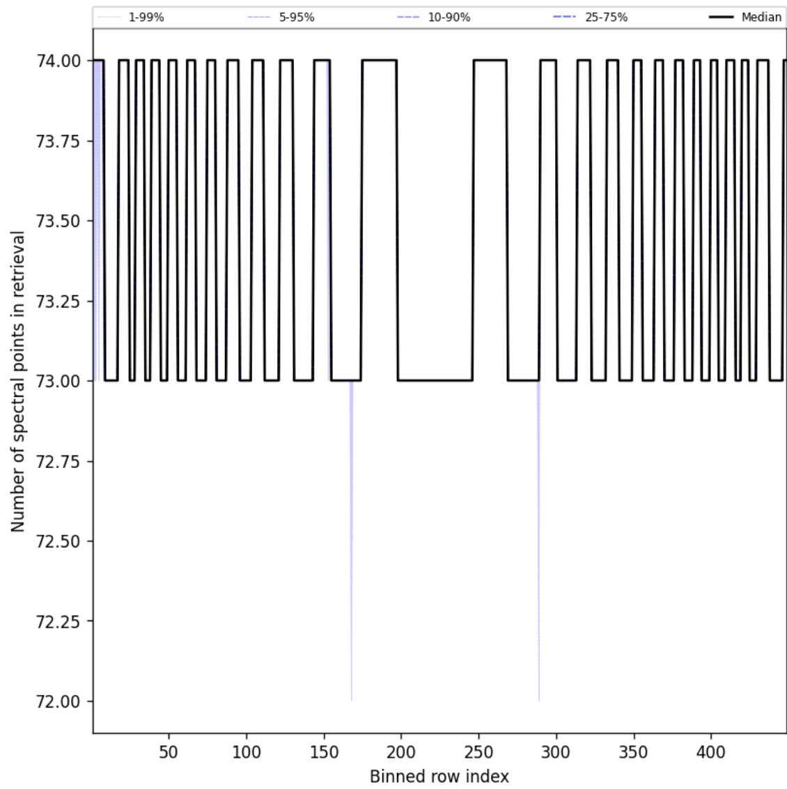
Figure 110: Along track statistics of “Number of spectral points in retrieval” for 2025-08-07 to 2025-08-07
