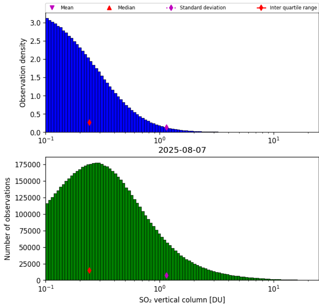
Figure 58: Histogram of “SO 2 vertical column” for 2025-08-07 to 2025-08-07
