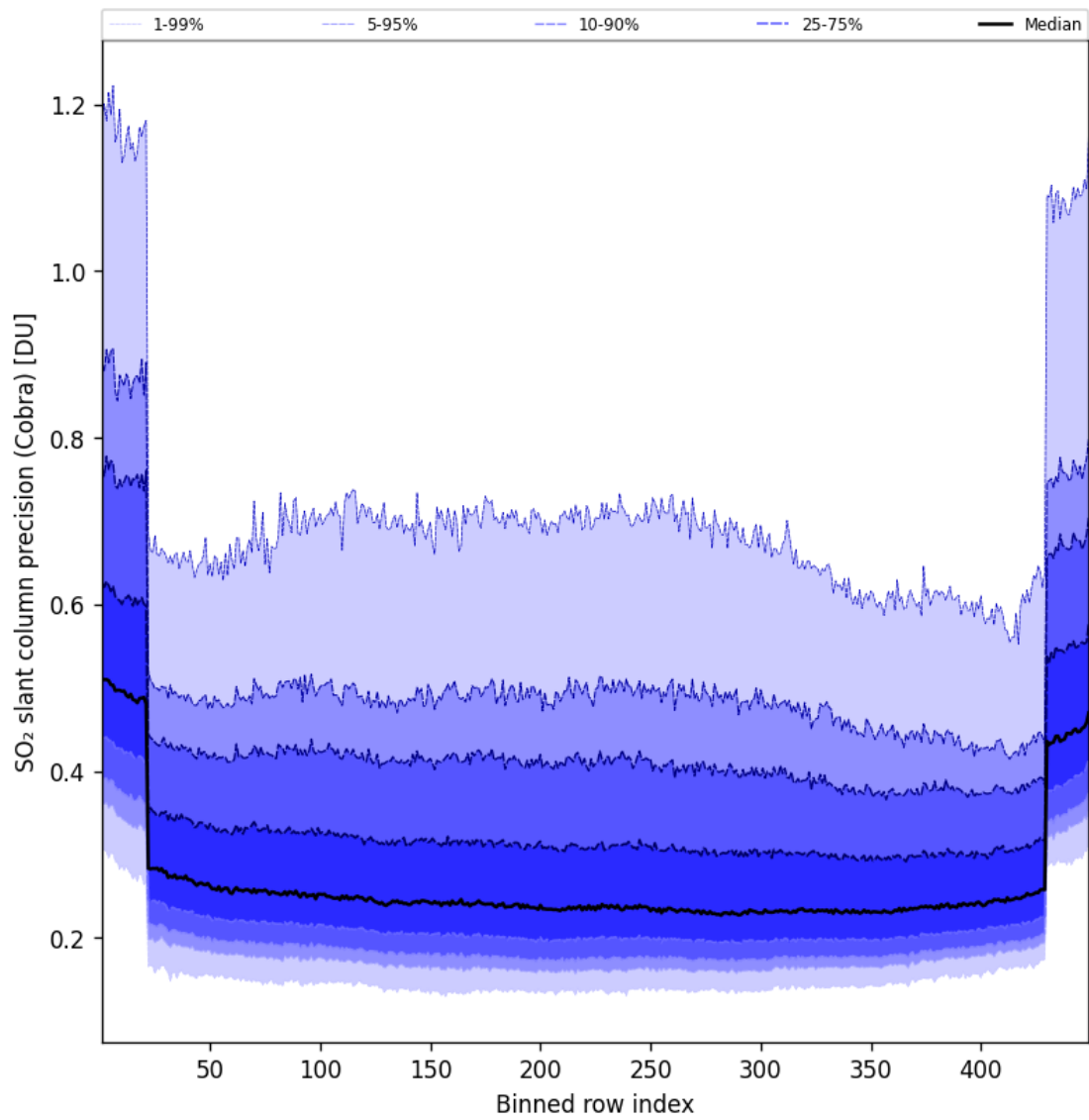
Figure 89: Along track statistics of “SO 2 slant column precision (Cobra)” for 2025-08-07 to 2025-08-07
