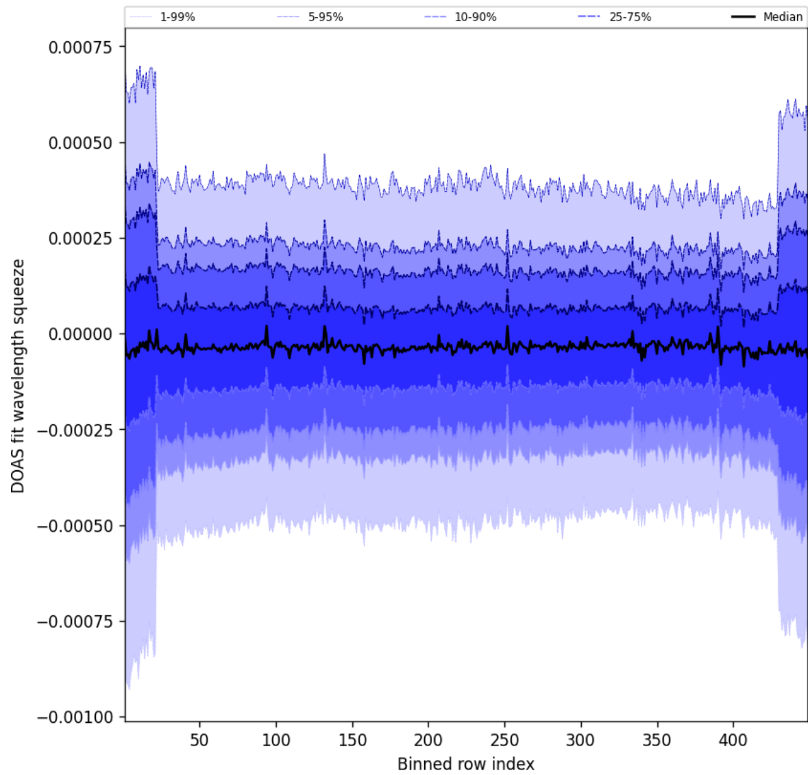
Figure 105: Along track statistics of “DOAS fit wavelength squeeze” for 2025-08-07 to 2025-08-07
