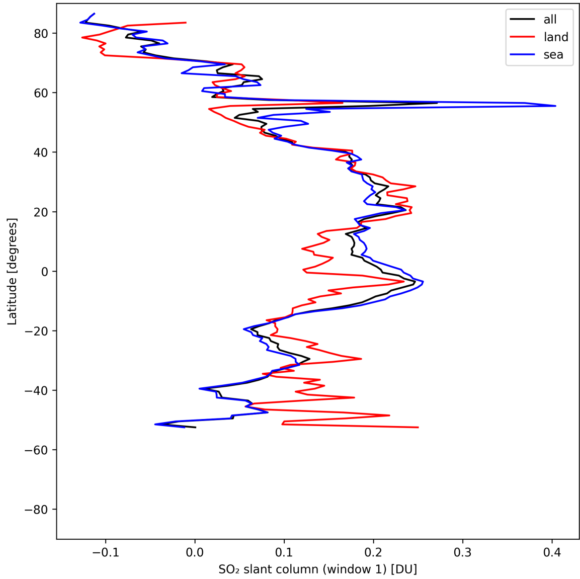
Figure 36: Zonal average of “SO 2 slant column (window 1)” for 2025-08-07 to 2025-08-07.
