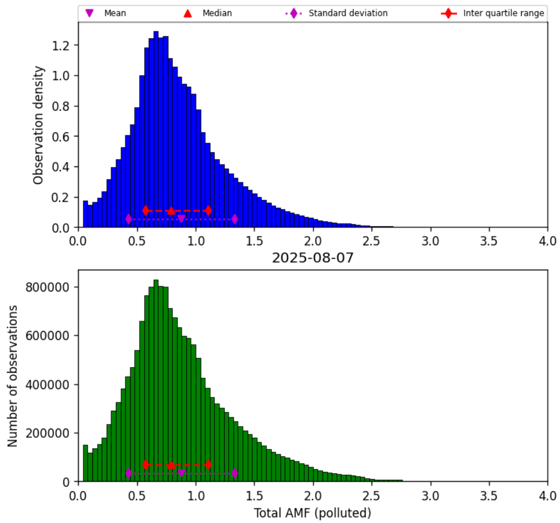
Figure 80: Histogram of “Total AMF (polluted)” for 2025-08-07 to 2025-08-07
