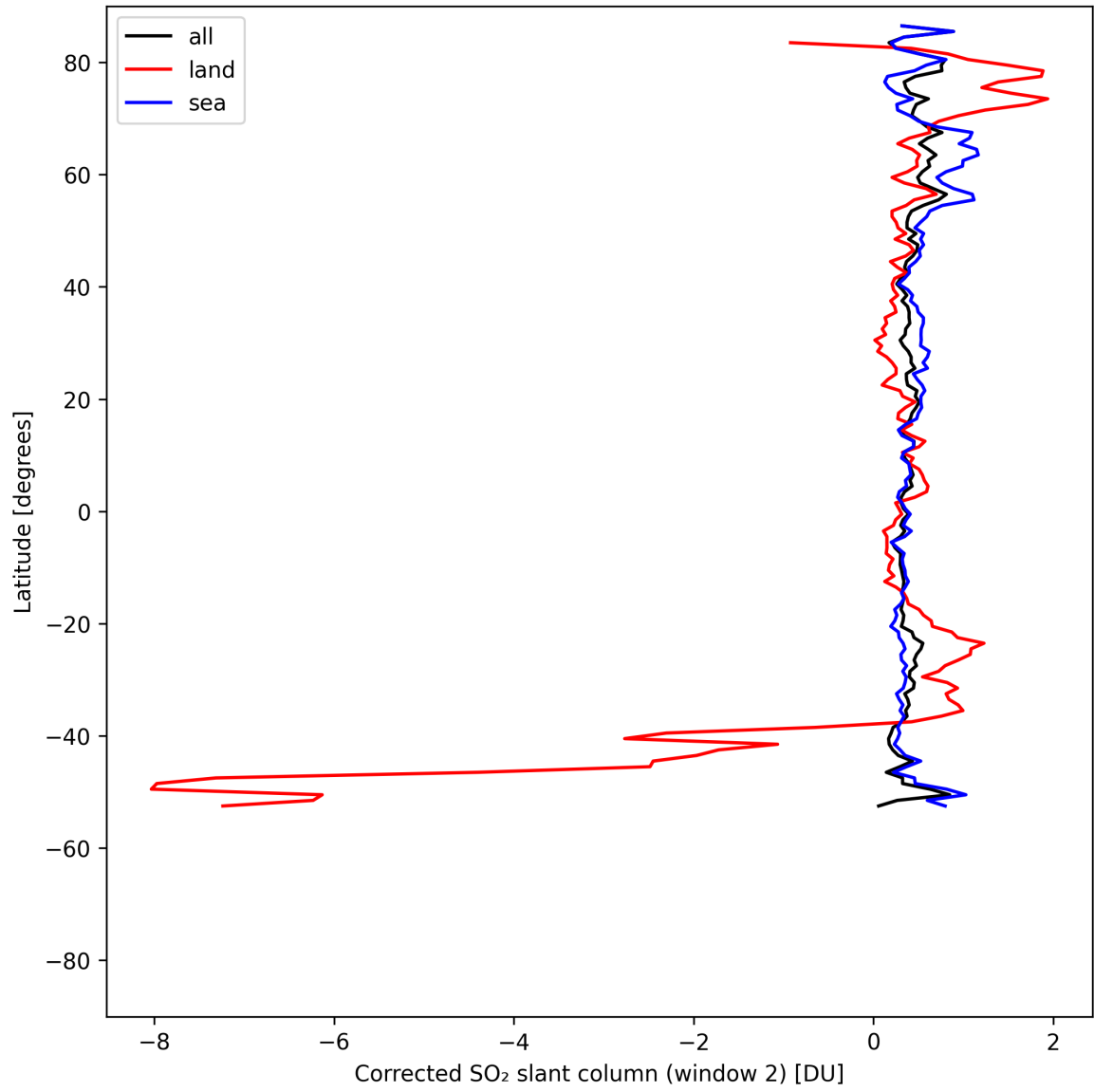
Figure 42: Zonal average of “Corrected SO 2 slant column (window 2)” for 2025-08-07 to 2025-08-07.
