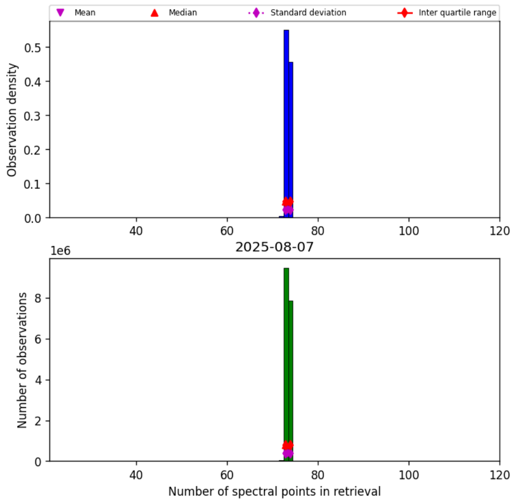
Figure 83: Histogram of “Number of spectral points in retrieval” for 2025-08-07 to 2025-08-07
