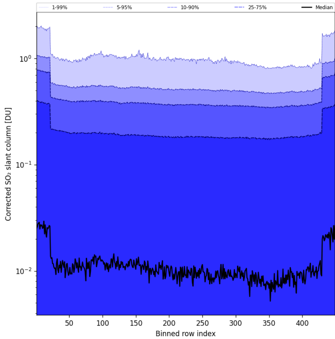
Figure 87: Along track statistics of “Corrected SO 2 slant column” for 2025-08-07 to 2025-08-07
