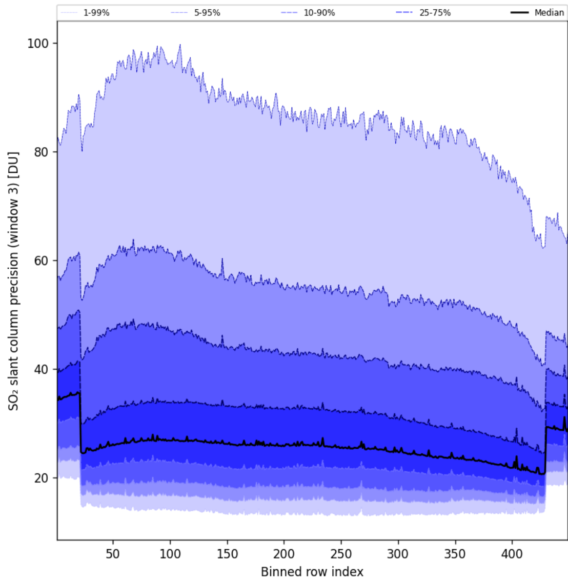
Figure 99: Along track statistics of “SO 2 slant column precision (window 3)” for 2025-08-07 to 2025-08-07
