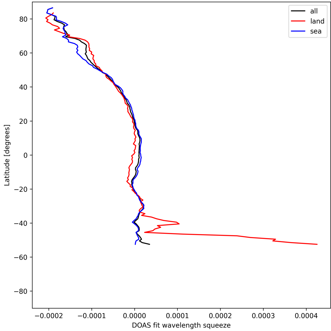
Figure 51: Zonal average of “DOAS fit wavelength squeeze” for 2025-08-07 to 2025-08-07.
