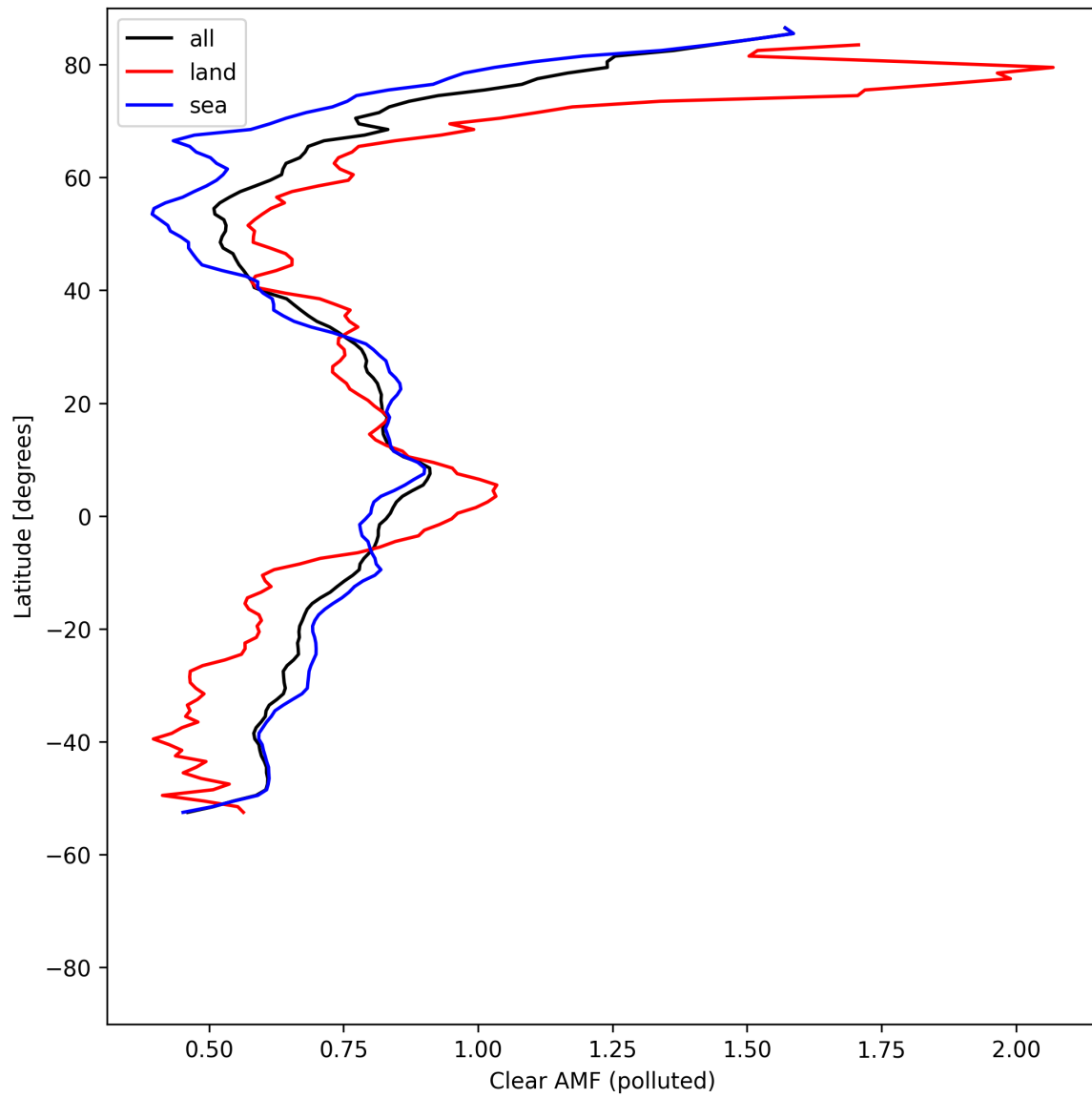
Figure 55: Zonal average of “Clear AMF (polluted)” for 2025-08-07 to 2025-08-07.
