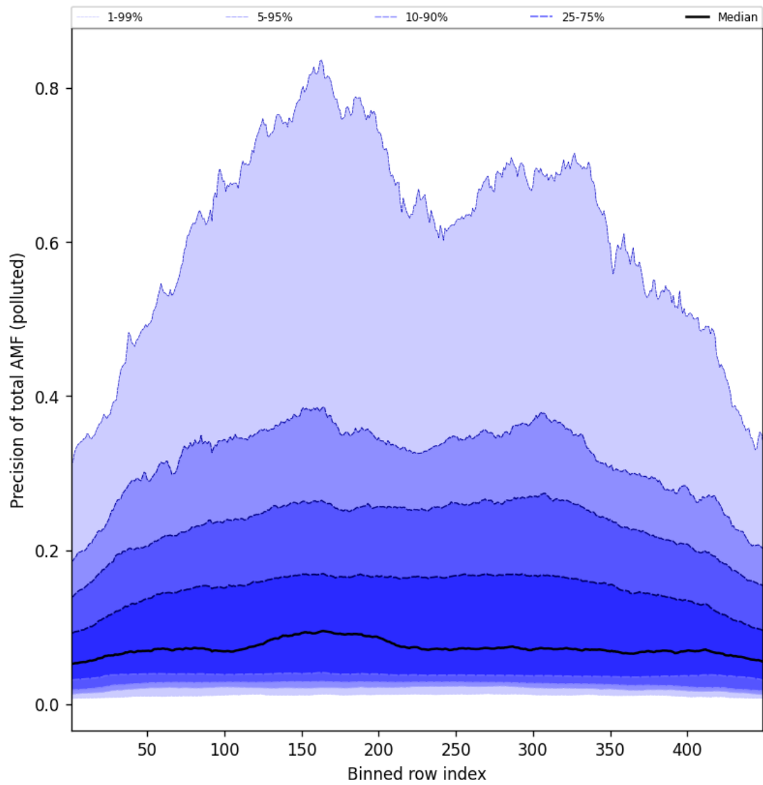
Figure 108: Along track statistics of “Precision of total AMF (polluted)” for 2025-08-07 to 2025-08-07
