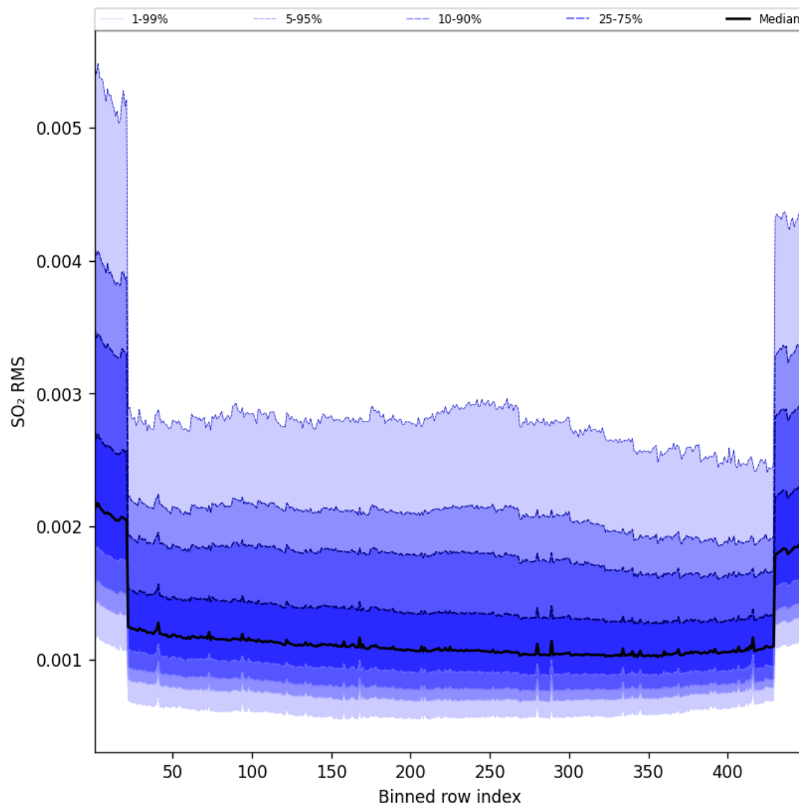
Figure 106: Along track statistics of “SO 2 RMS” for 2025-08-07 to 2025-08-07
