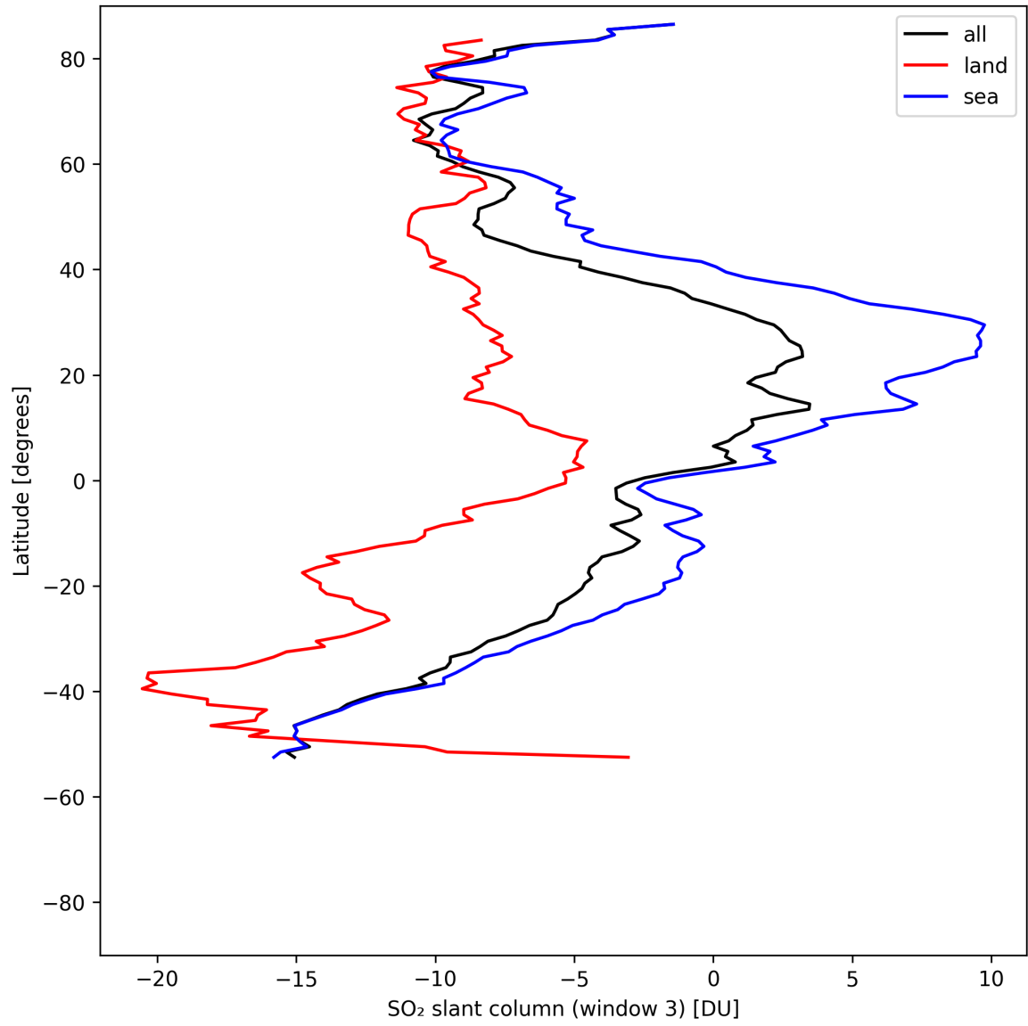
Figure 44: Zonal average of “SO 2 slant column (window 3)” for 2025-08-07 to 2025-08-07.
