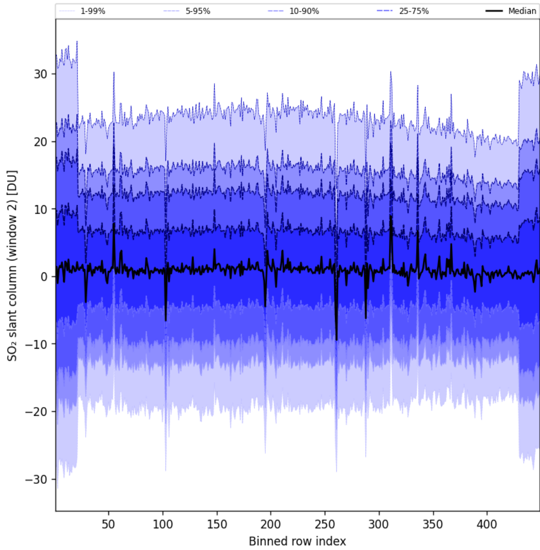
Figure 94: Along track statistics of “SO 2 slant column (window 2)” for 2025-08-07 to 2025-08-07
