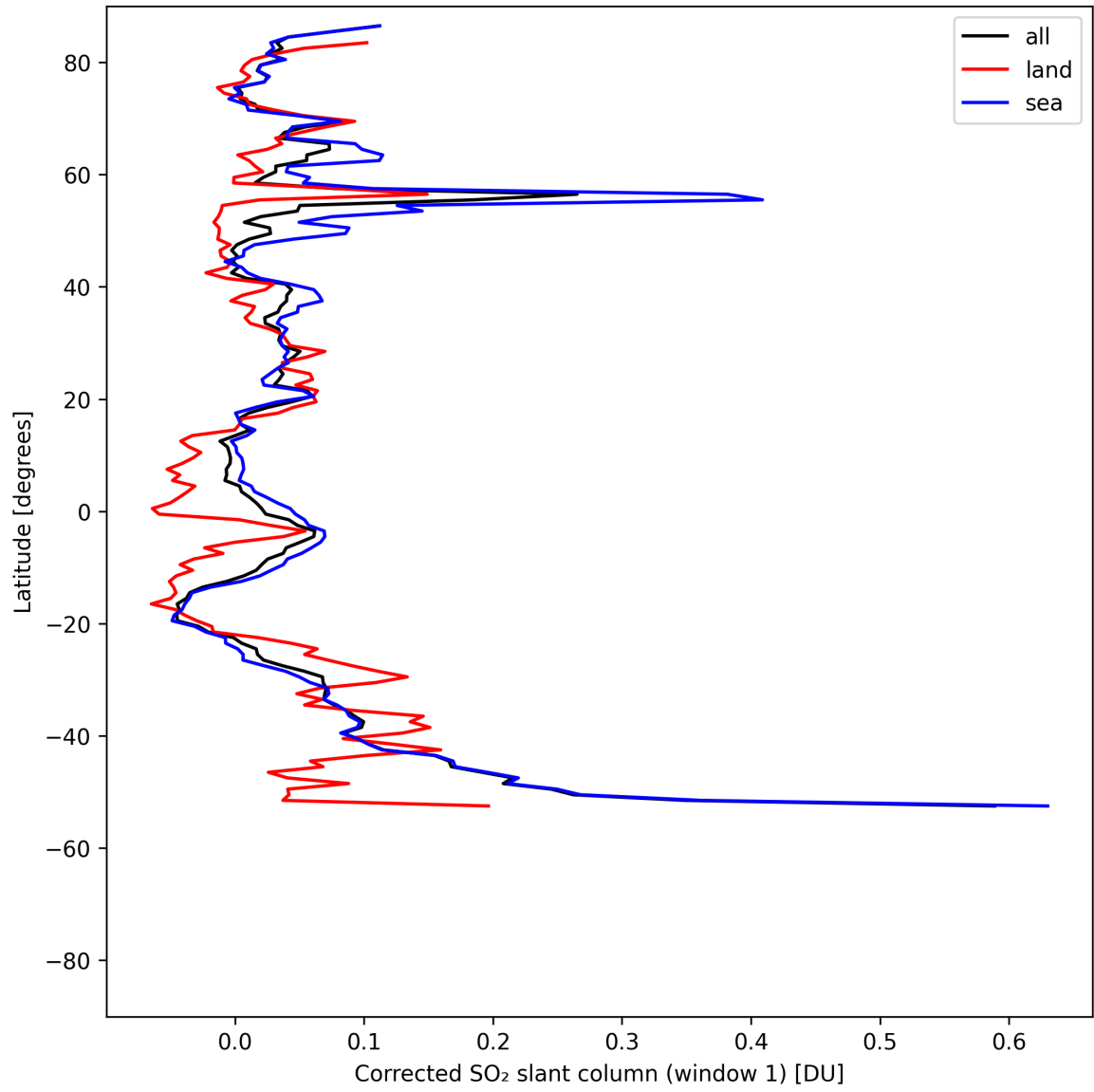
Figure 38: Zonal average of “Corrected SO 2 slant column (window 1)” for 2025-08-07 to 2025-08-07.
