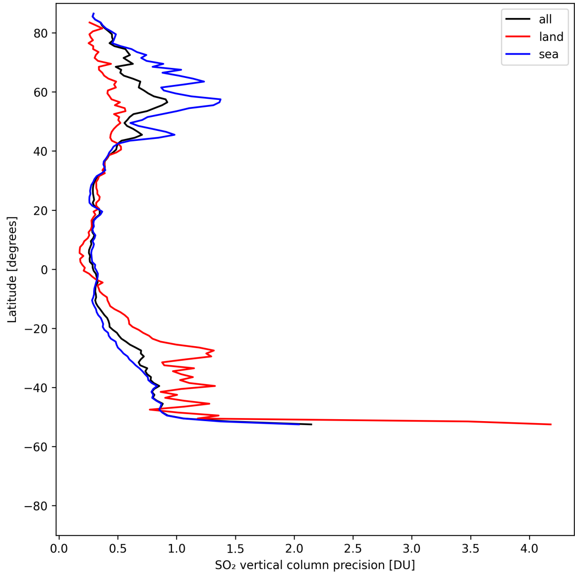
Figure 32: Zonal average of “SO 2 vertical column precision” for 2025-08-07 to 2025-08-07.
