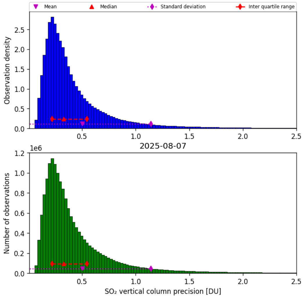
Figure 59: Histogram of “SO 2 vertical column precision” for 2025-08-07 to 2025-08-07
