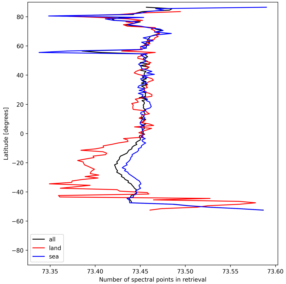
Figure 56: Zonal average of “Number of spectral points in retrieval” for 2025-08-07 to 2025-08-07.
