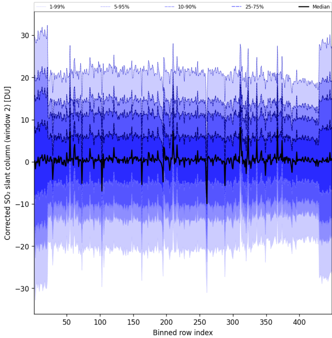
Figure 96: Along track statistics of “Corrected SO 2 slant column (window 2)” for 2025-08-07 to 2025-08-07
