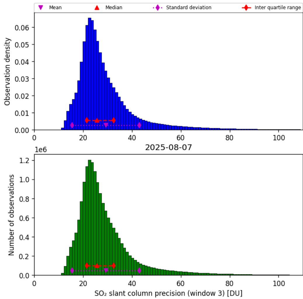
Figure 72: Histogram of “SO 2 slant column precision (window 3)” for 2025-08-07 to 2025-08-07
