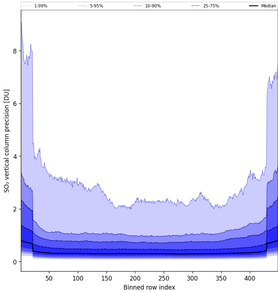
Figure 86: Along track statistics of “SO 2 vertical column precision” for 2025-08-07 to 2025-08-07
