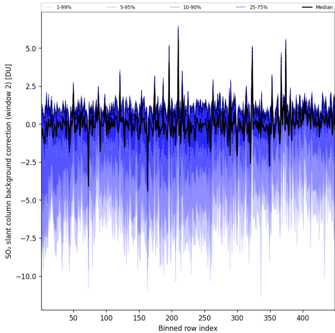
Figure 97: Along track statistics of “SO 2 slant column background correction (window 2)” for 2025-08-07 to 2025-08-07
