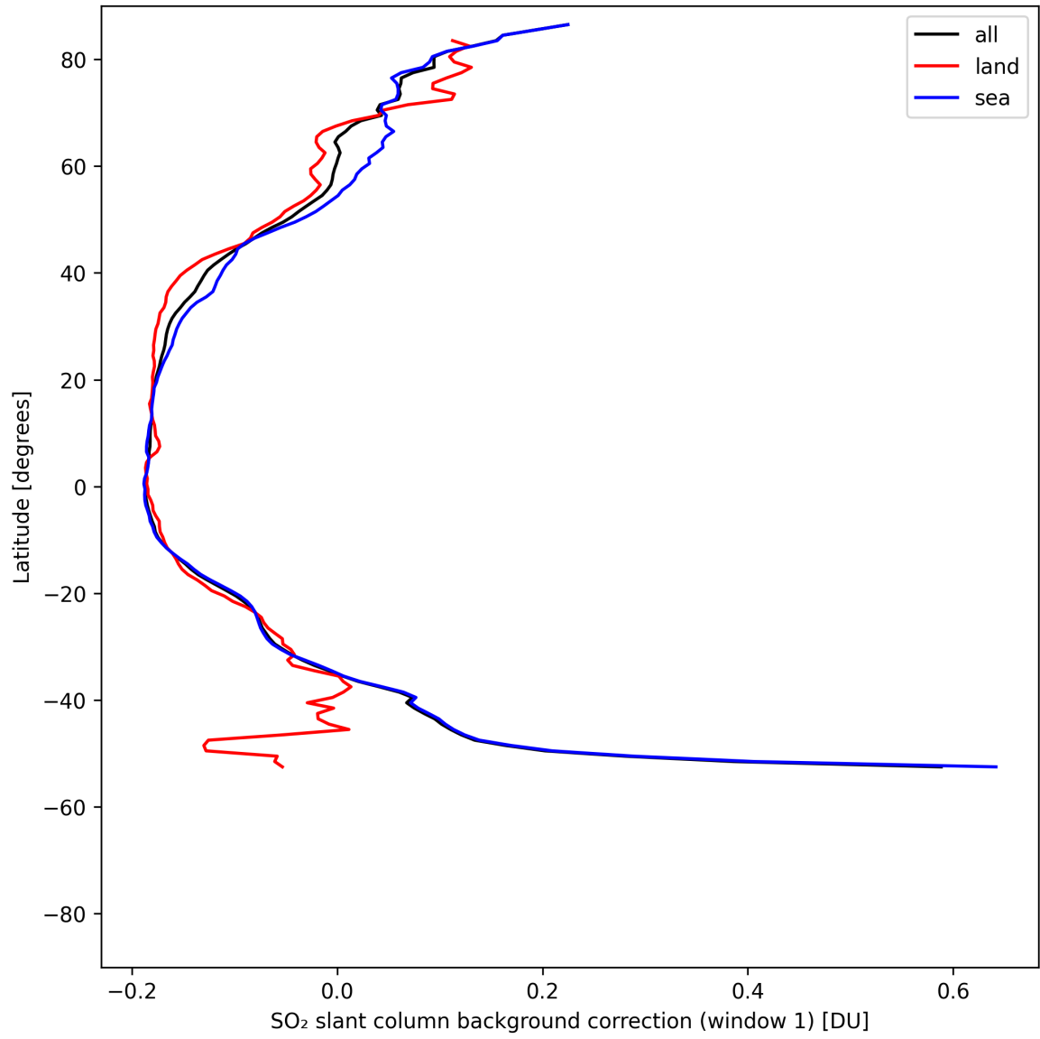
Figure 39: Zonal average of “SO 2 slant column background correction (window 1)” for 2025-08-07 to 2025-08-07.
