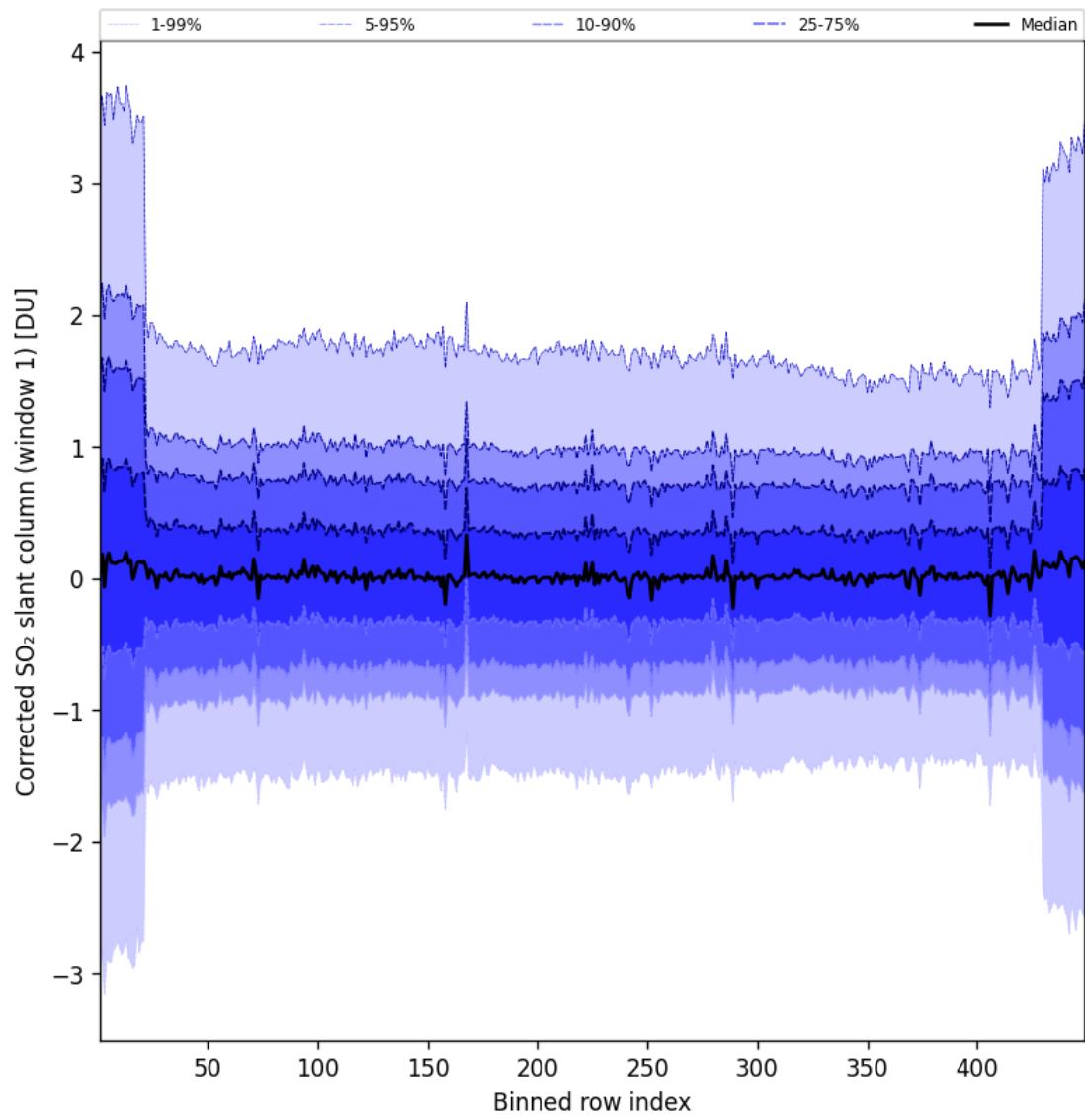
Figure 92: Along track statistics of “Corrected SO 2 slant column (window 1)” for 2025-08-07 to 2025-08-07
