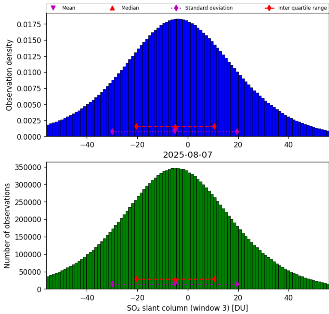
Figure 71: Histogram of “SO 2 slant column (window 3)” for 2025-08-07 to 2025-08-07
