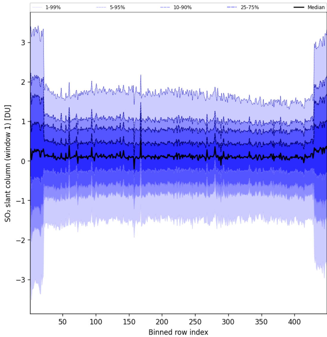
Figure 90: Along track statistics of “SO 2 slant column (window 1)” for 2025-08-07 to 2025-08-07
