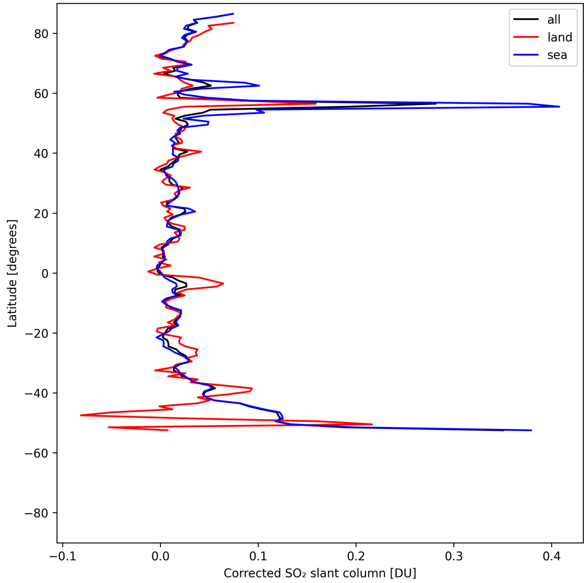
Figure 33: Zonal average of “Corrected SO 2 slant column” for 2025-08-07 to 2025-08-07.
