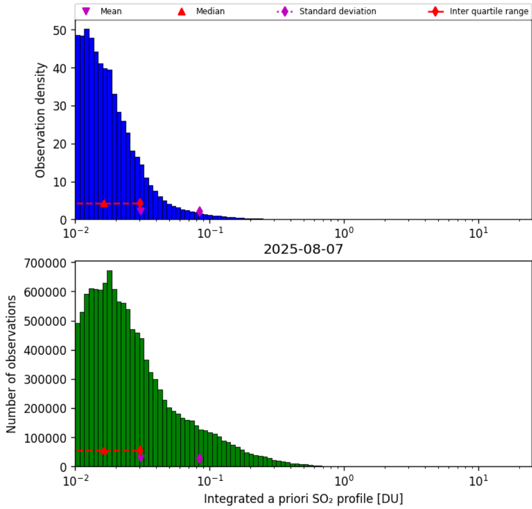
Figure 76: Histogram of “Integrated a priori SO 2 profile” for 2025-08-07 to 2025-08-07
