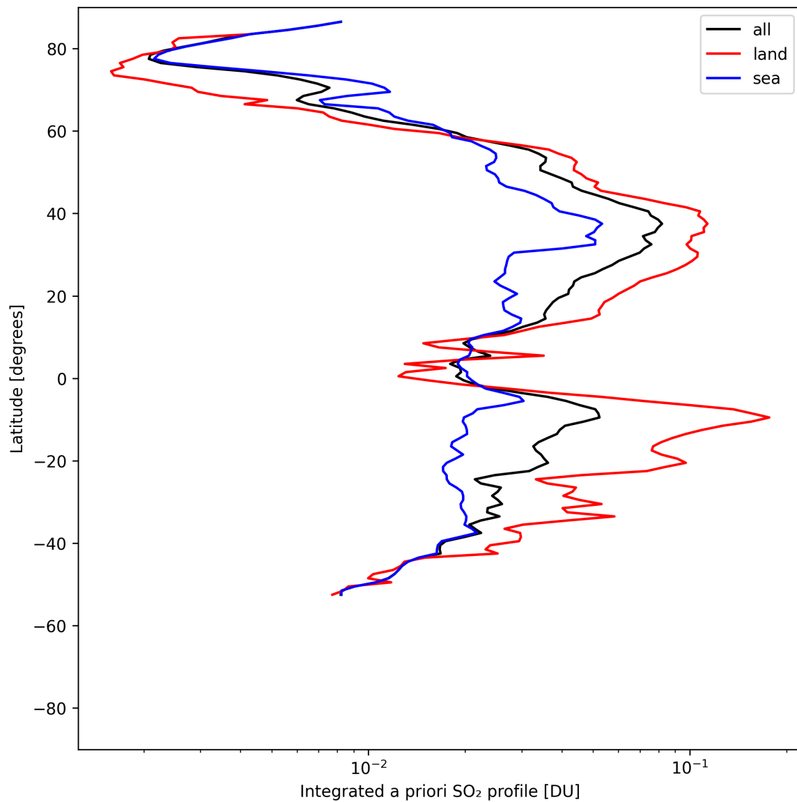
Figure 49: Zonal average of “Integrated a priori SO 2 profile” for 2025-08-07 to 2025-08-07.
