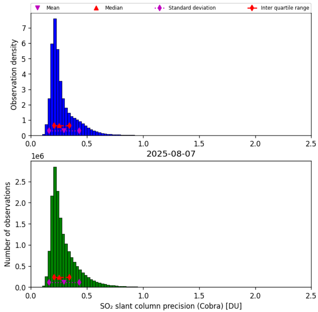
Figure 62: Histogram of “SO 2 slant column precision (Cobra)” for 2025-08-07 to 2025-08-07
