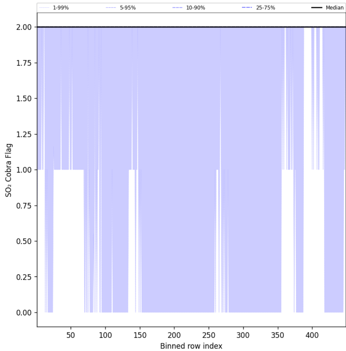
Figure 102: Along track statistics of “SO 2 Cobra Flag” for 2025-08-07 to 2025-08-07
