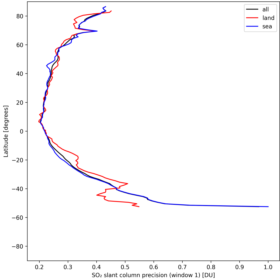
Figure 37: Zonal average of “SO 2 slant column precision (window 1)” for 2025-08-07 to 2025-08-07.
