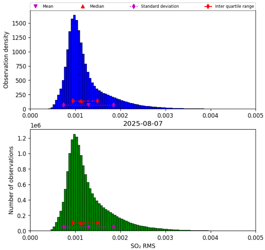
Figure 79: Histogram of “SO 2 RMS” for 2025-08-07 to 2025-08-07
