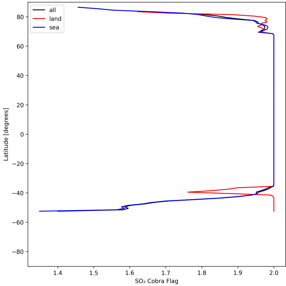
Figure 48: Zonal average of "SO 2 Cobra Flag" for 2025-08-07 to 2025-08-07.
