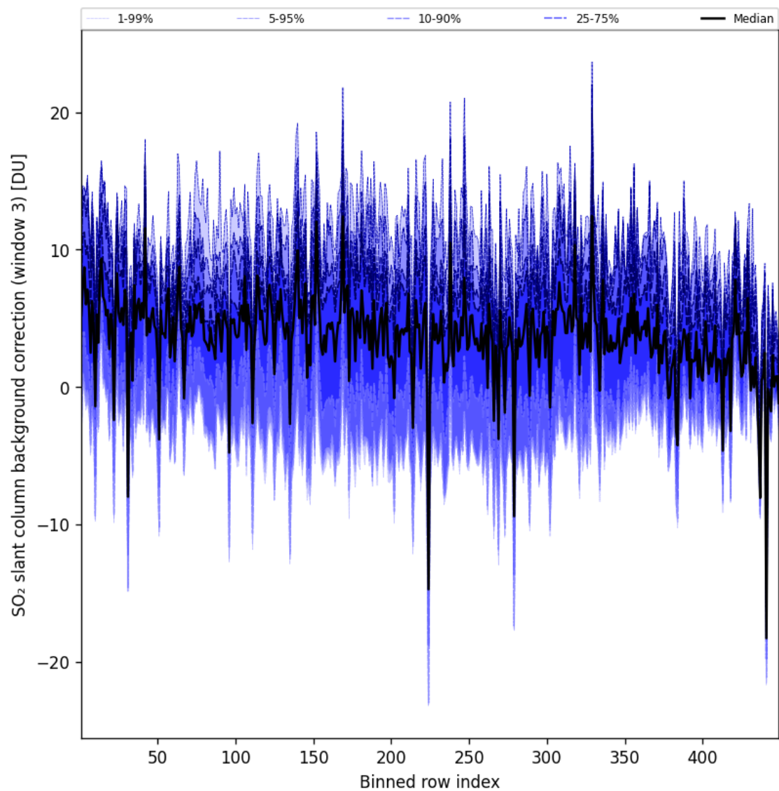
Figure 101: Along track statistics of “SO 2 slant column background correction (window 3)” for 2025-08-07 to 2025-08-07
