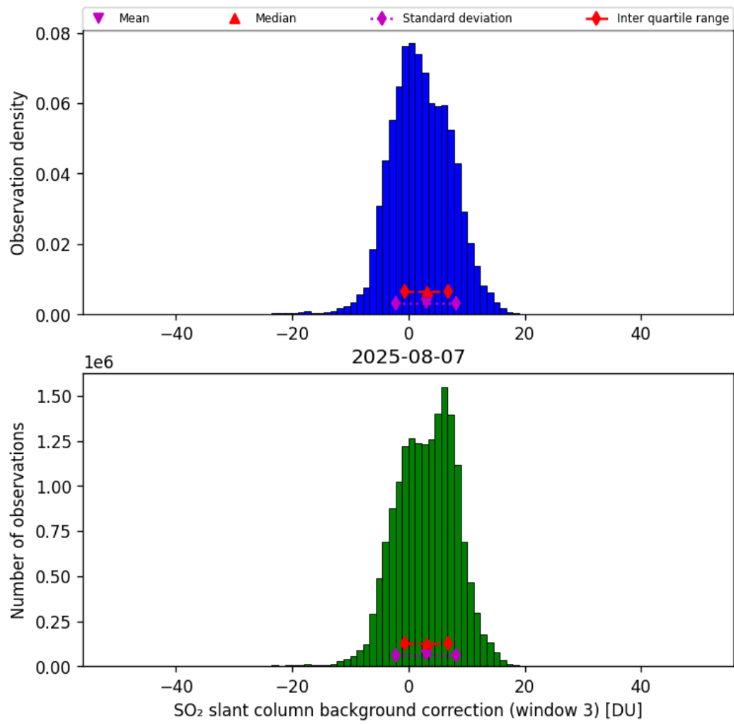
Figure 74: Histogram of “SO 2 slant column background correction (window 3)” for 2025-08-07 to 2025-08-07
