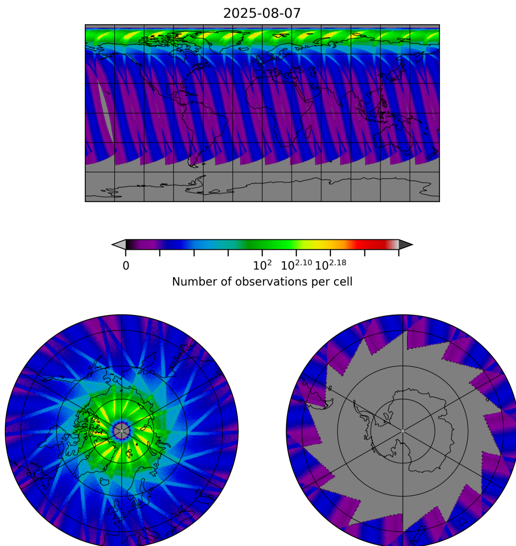
Figure 29: Map of the number of observations for 2025-08-07 to 2025-08-07
