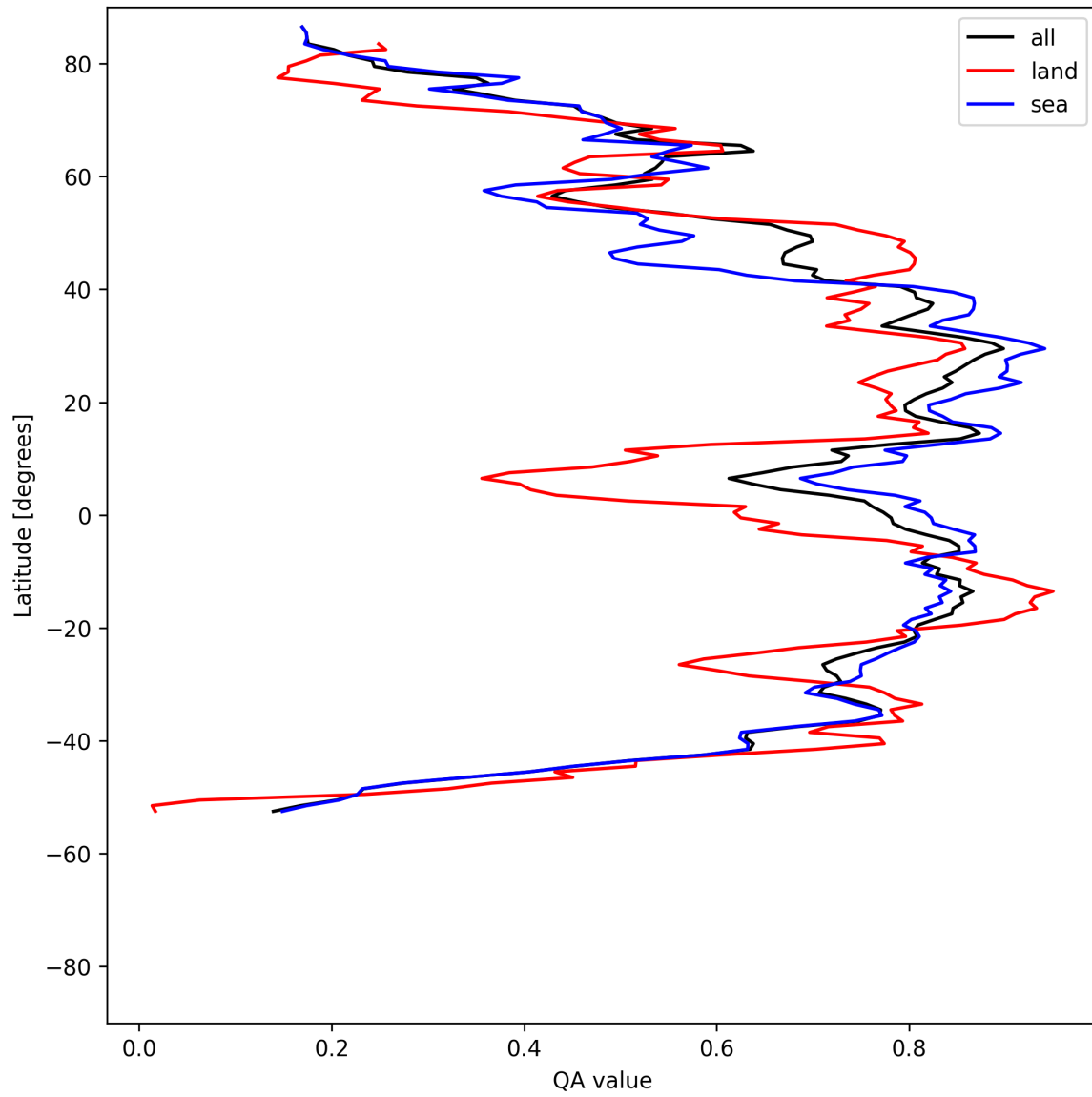
Figure 30: Zonal average of “QA value” for 2025-08-07 to 2025-08-07.
