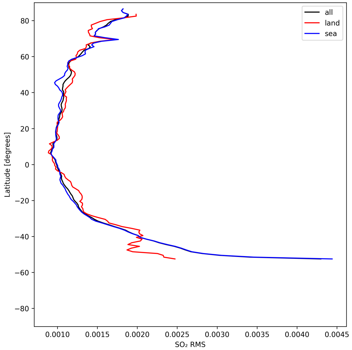
Figure 52: Zonal average of “SO 2 RMS” for 2025-08-07 to 2025-08-07.
