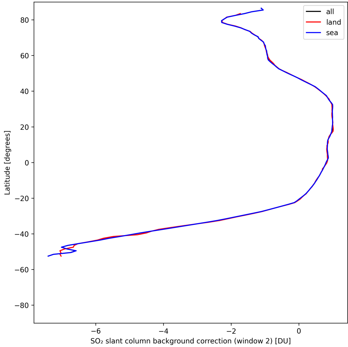
Figure 43: Zonal average of “SO 2 slant column background correction (window 2)” for 2025-08-07 to 2025-08-07.
