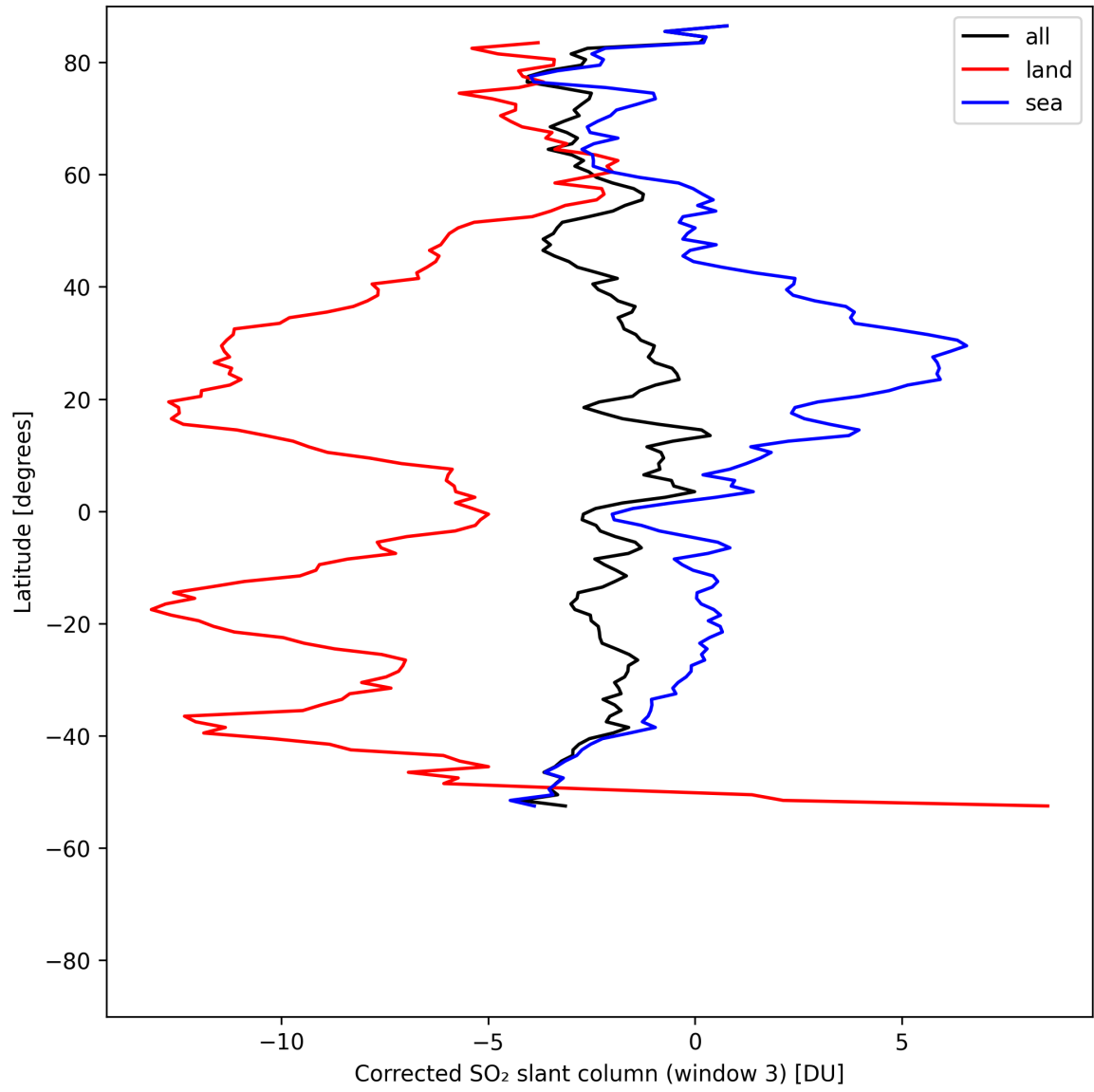
Figure 46: Zonal average of “Corrected SO 2 slant column (window 3)” for 2025-08-07 to 2025-08-07.
