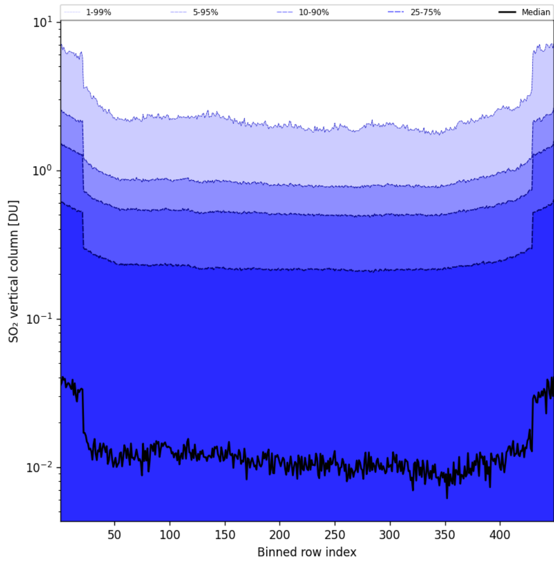
Figure 85: Along track statistics of “SO 2 vertical column” for 2025-08-07 to 2025-08-07
