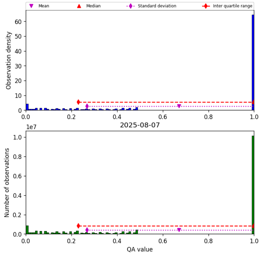
Figure 57: Histogram of “QA value” for 2025-08-07 to 2025-08-07
