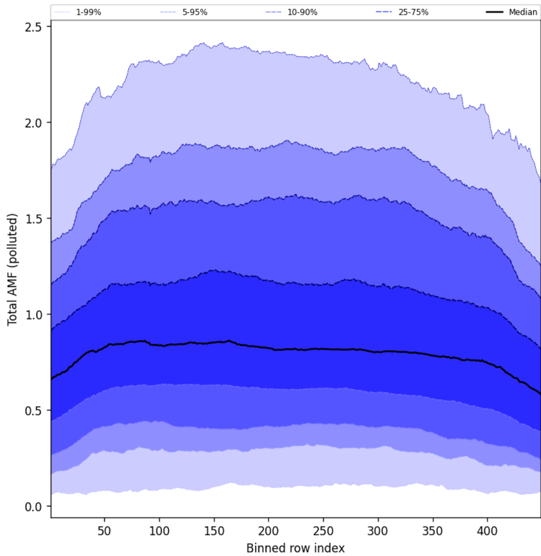
Figure 107: Along track statistics of “Total AMF (polluted)” for 2025-08-07 to 2025-08-07
